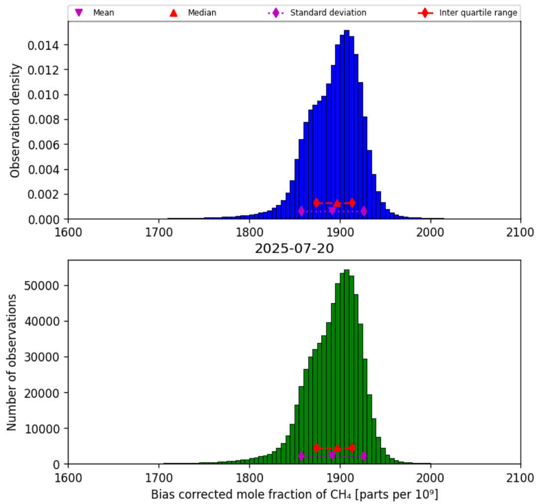
Figure 25: Histogram of “Bias corrected mole fraction of CH 4 ” for 2025-07-19 to 2025-07-21
