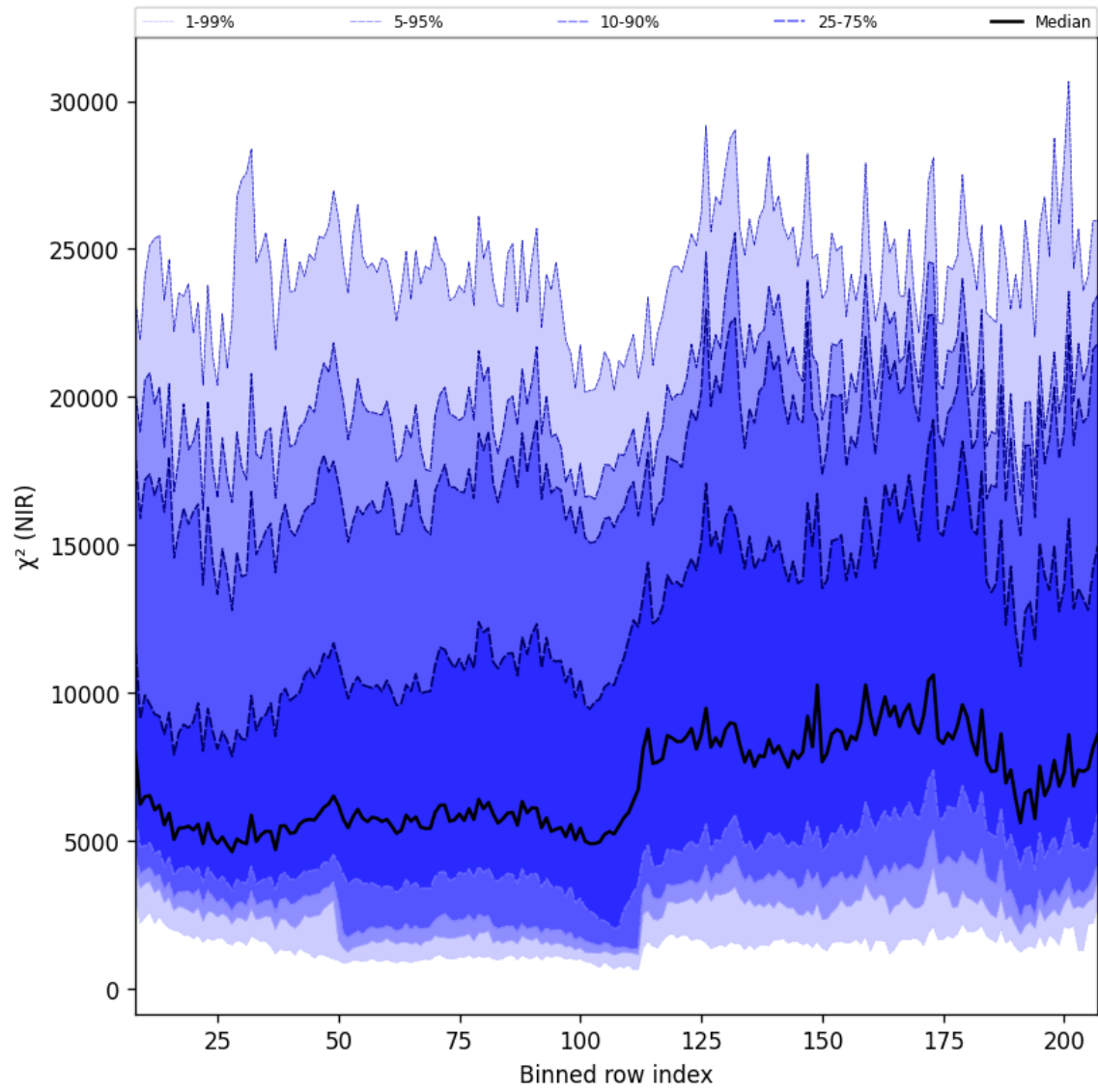
Figure 40: Along track statistics of “ \chi^2 (NIR)” for 2025-07-19 to 2025-07-21
