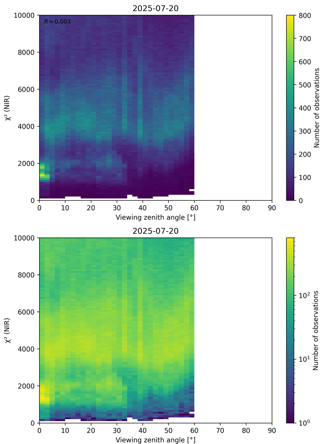
Figure 105: Scatter density plot of “Viewing zenith angle” against “ \chi^2 (NIR)” for 2025-07-19 to 2025-07-21.
