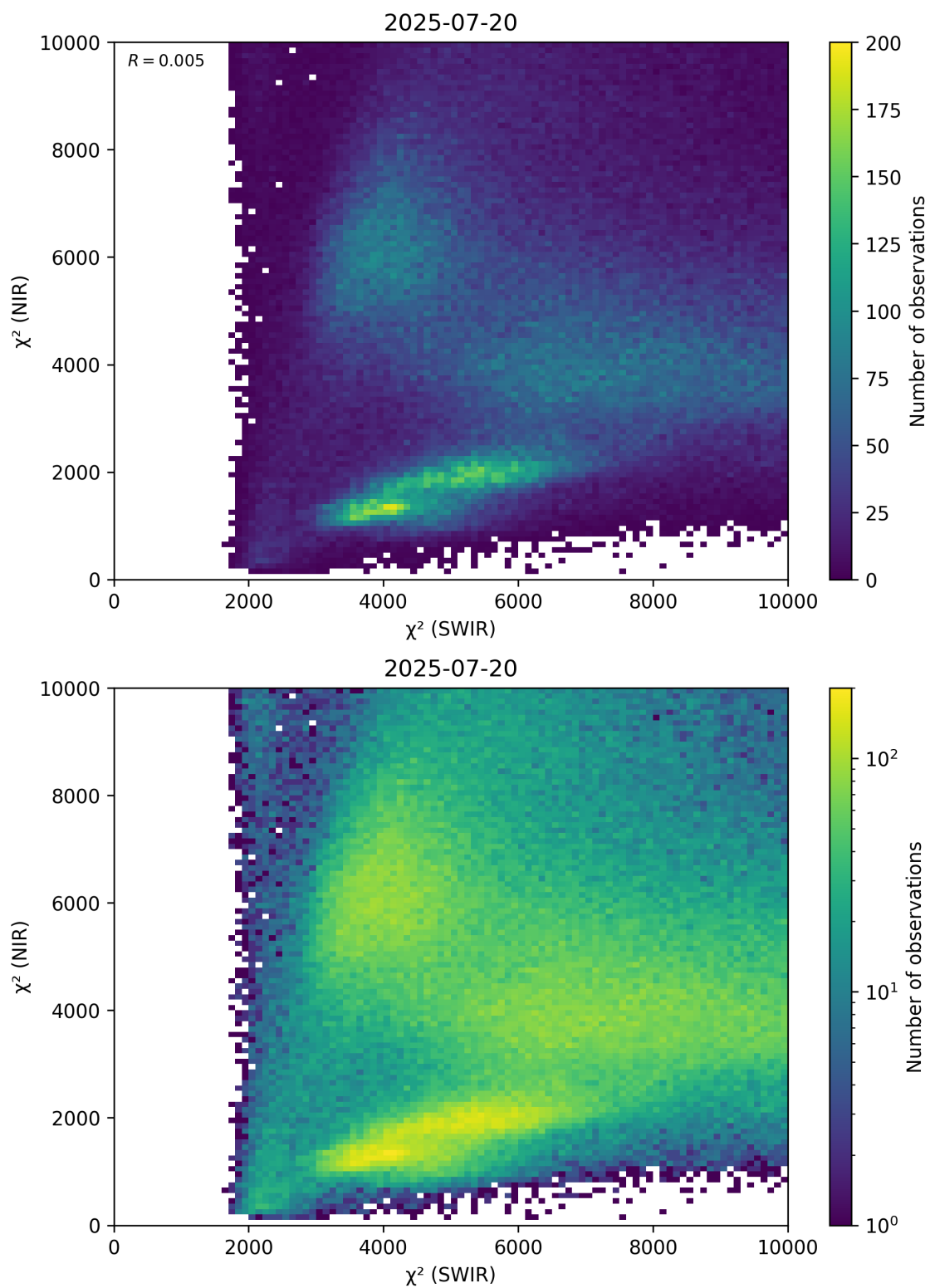
Figure 47: Scatter density plot of “ \chi^2 (SWIR)” against “ \chi^2 (NIR)” for 2025-07-19 to 2025-07-21.
