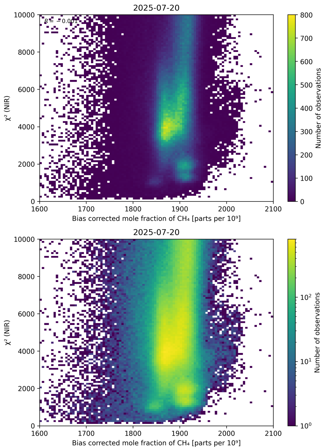
Figure 63: Scatter density plot of “Bias corrected mole fraction of \text{CH}_4 ” against “ \chi^2 (NIR)” for 2025-07-19 to 2025-07-21.
