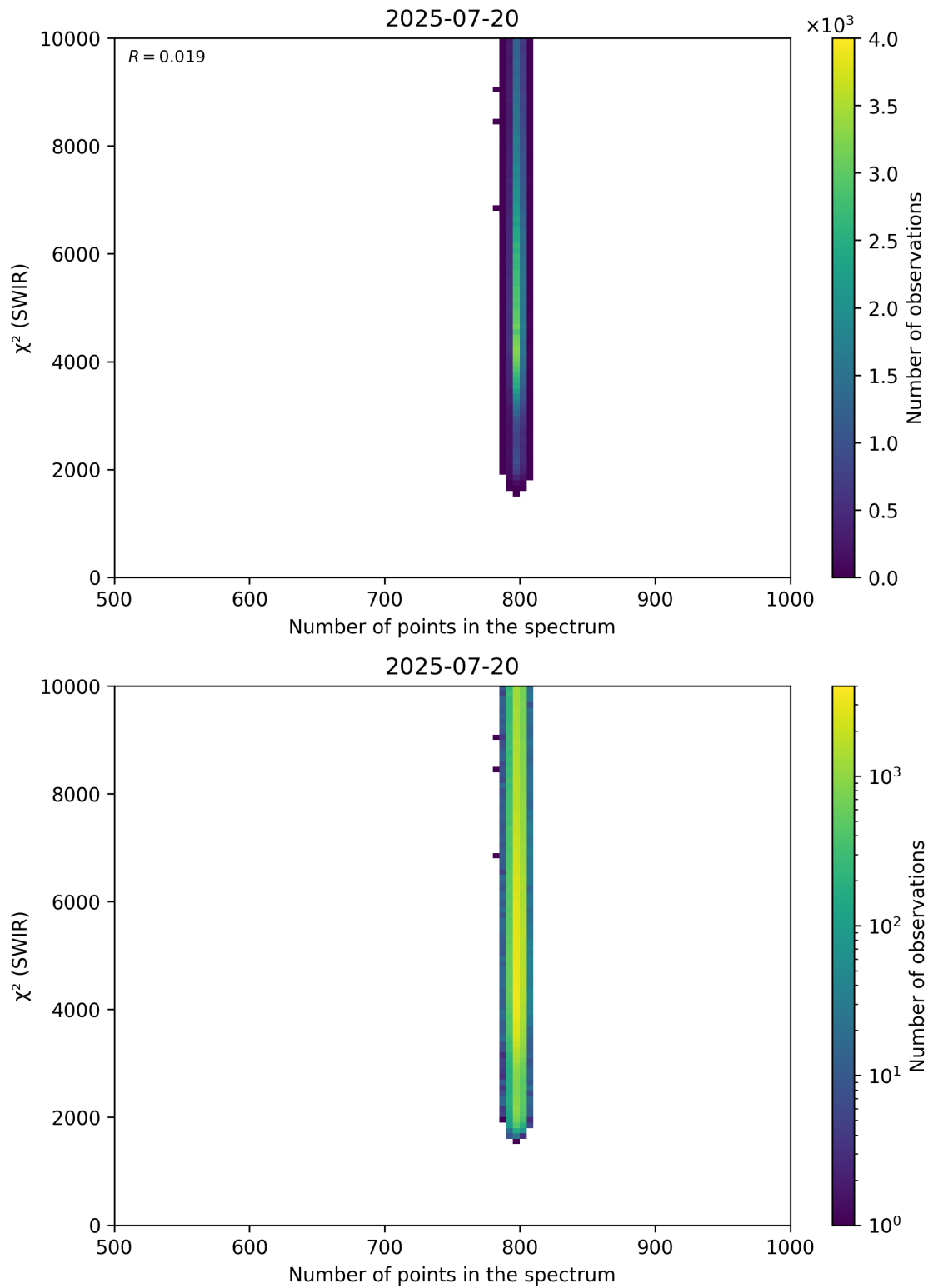
Figure 89: Scatter density plot of “Number of points in the spectrum” against “ \chi^2 (SWIR)” for 2025-07-19 to 2025-07-21.
