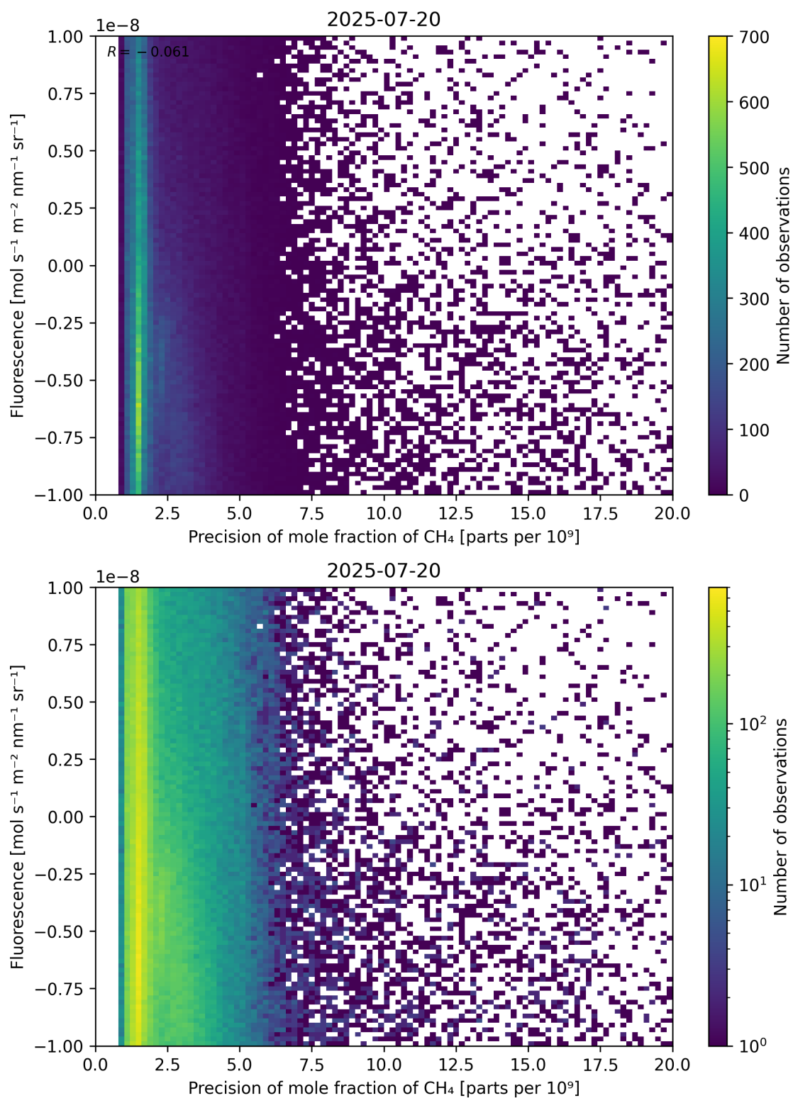
Figure 81: Scatter density plot of “Precision of mole fraction of \text{CH}_4 ” against “Fluorescence” for 2025-07-19 to 2025-07-21.
