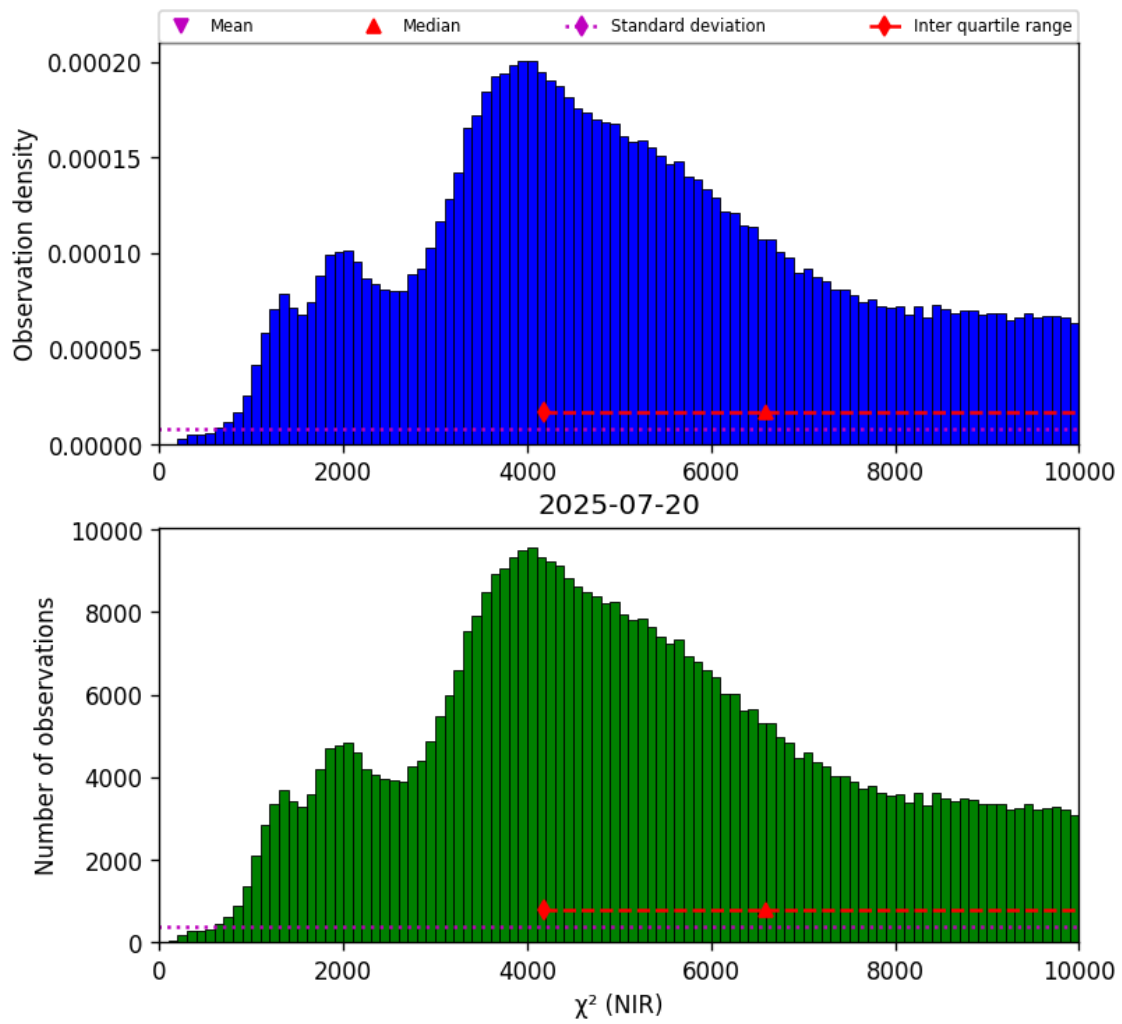
Figure 29: Histogram of “ \chi^2 (NIR)” for 2025-07-19 to 2025-07-21
