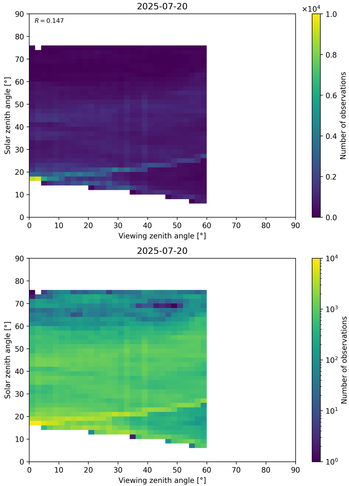
Figure 115: Scatter density plot of “Viewing zenith angle” against “Solar zenith angle” for 2025-07-19 to 2025-07-21.
