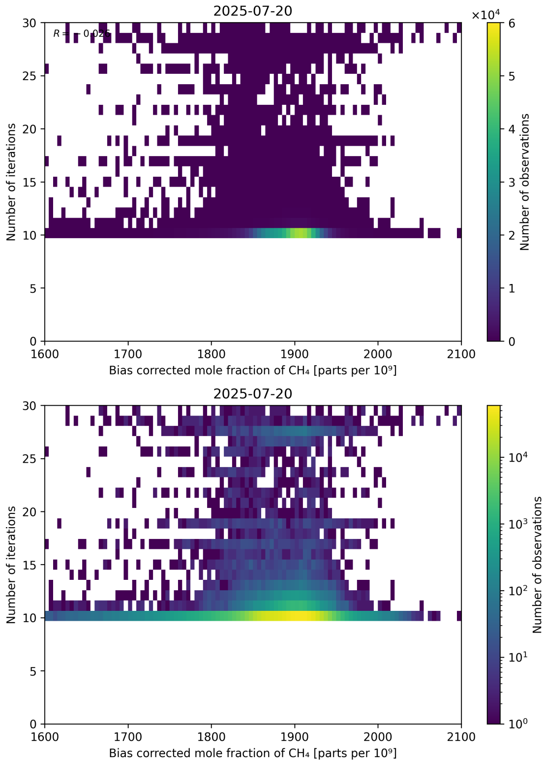
Figure 67: Scatter density plot of “Bias corrected mole fraction of CH 4 ” against “Number of iterations” for 2025-07-19 to 2025-07-21.
