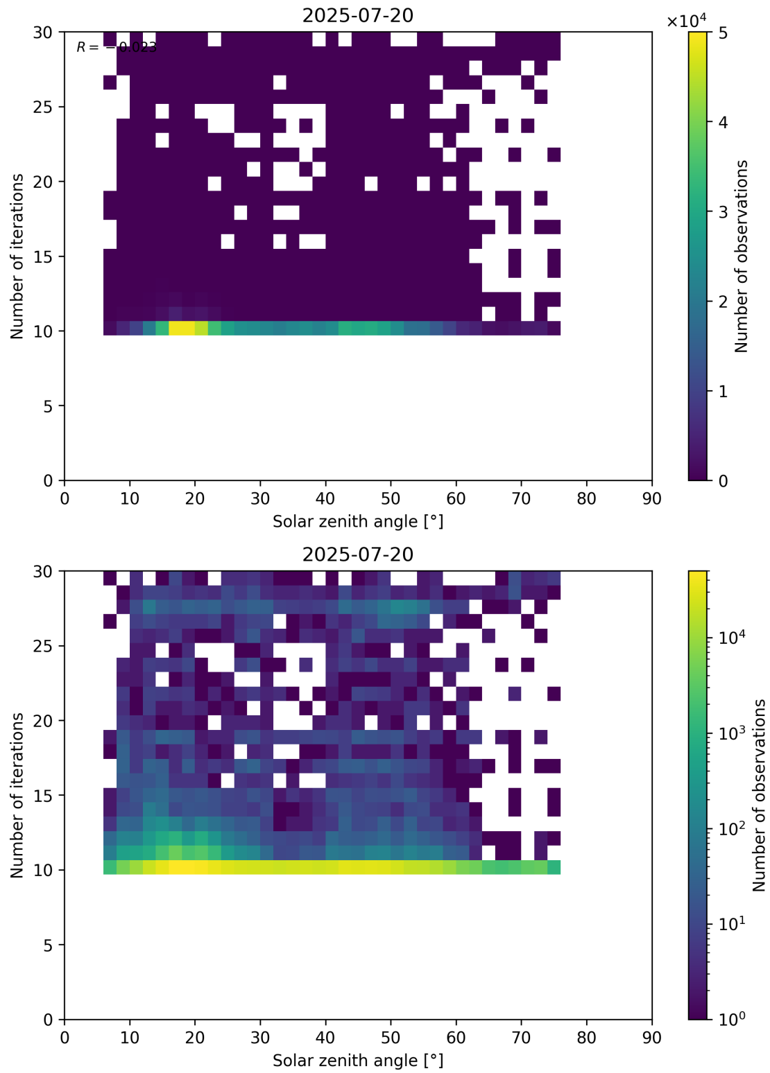
Figure 102: Scatter density plot of “Solar zenith angle” against “Number of iterations” for 2025-07-19 to 2025-07-21.
