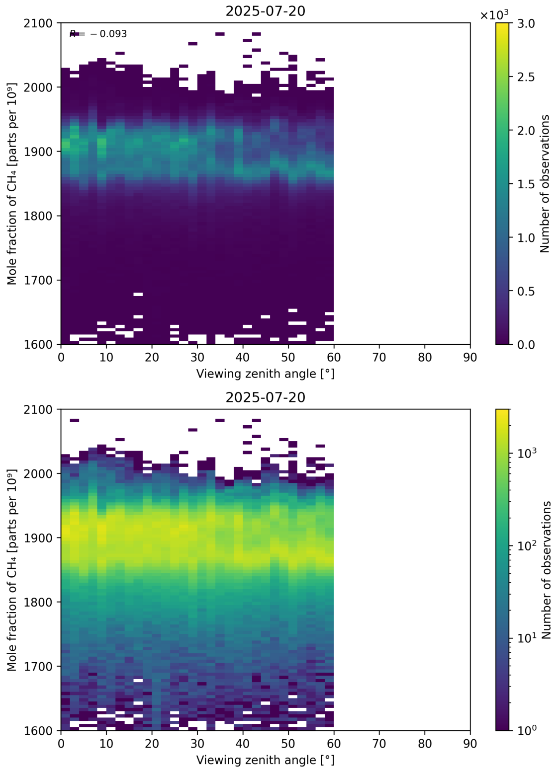
Figure 110: Scatter density plot of “Viewing zenith angle” against “Mole fraction of CH 4 ” for 2025-07-19 to 2025-07-21.
