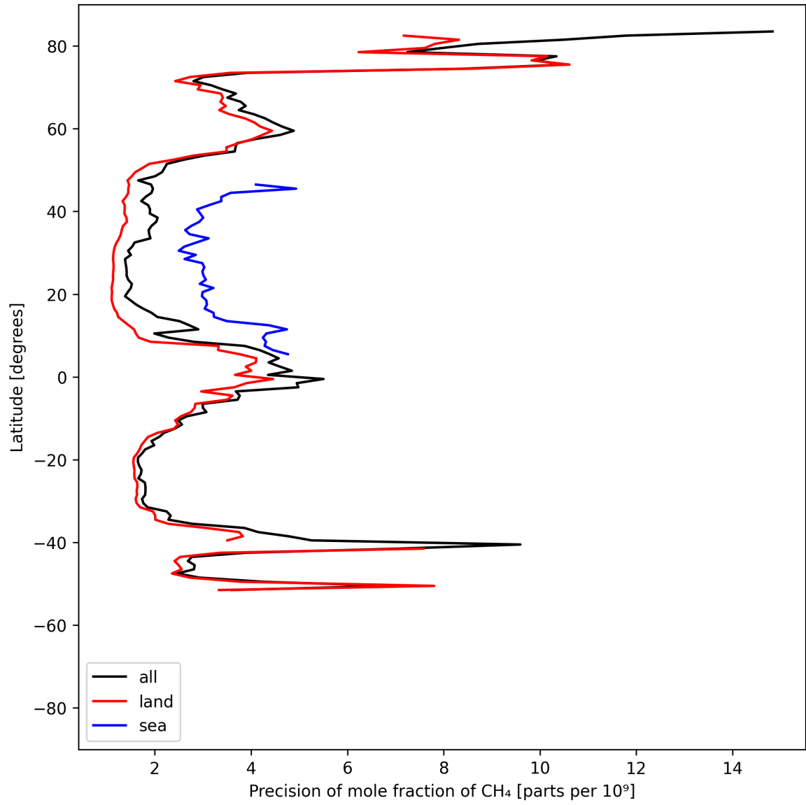
Figure 13: Zonal average of “Precision of mole fraction of CH 4 ” for 2025-07-19 to 2025-07-21.
