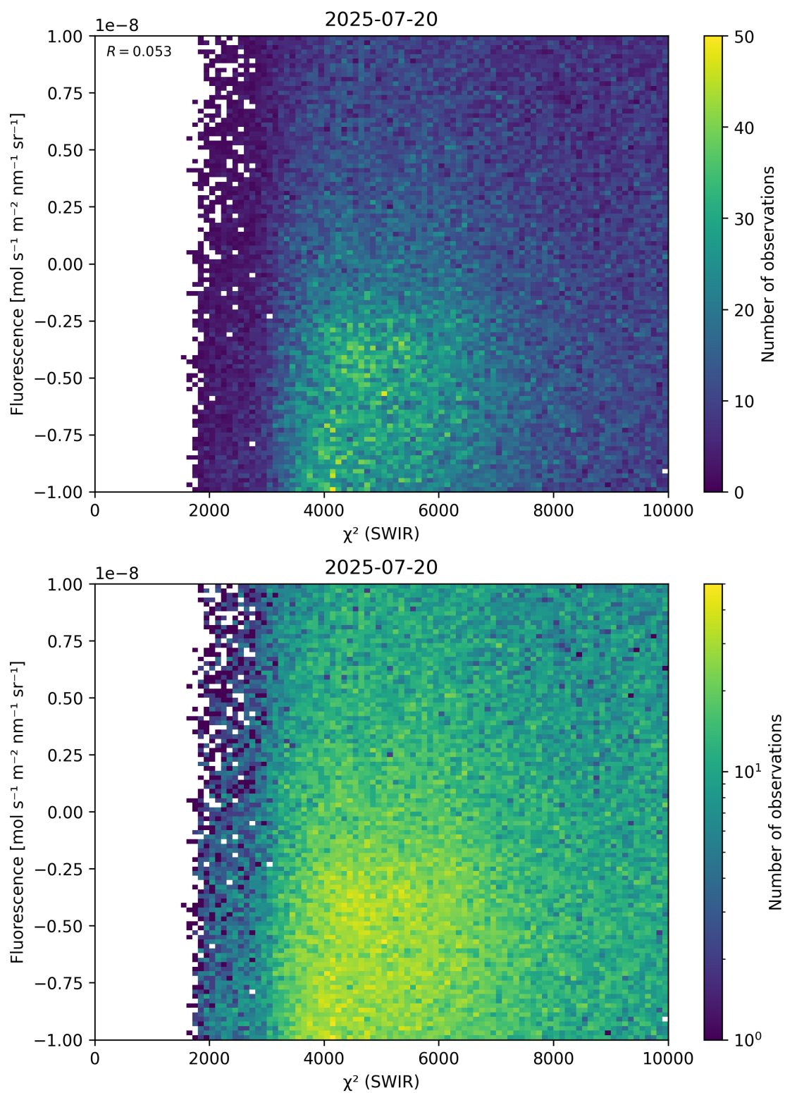
Figure 49: Scatter density plot of “ \chi^2 (SWIR)” against “Fluorescence” for 2025-07-19 to 2025-07-21.
