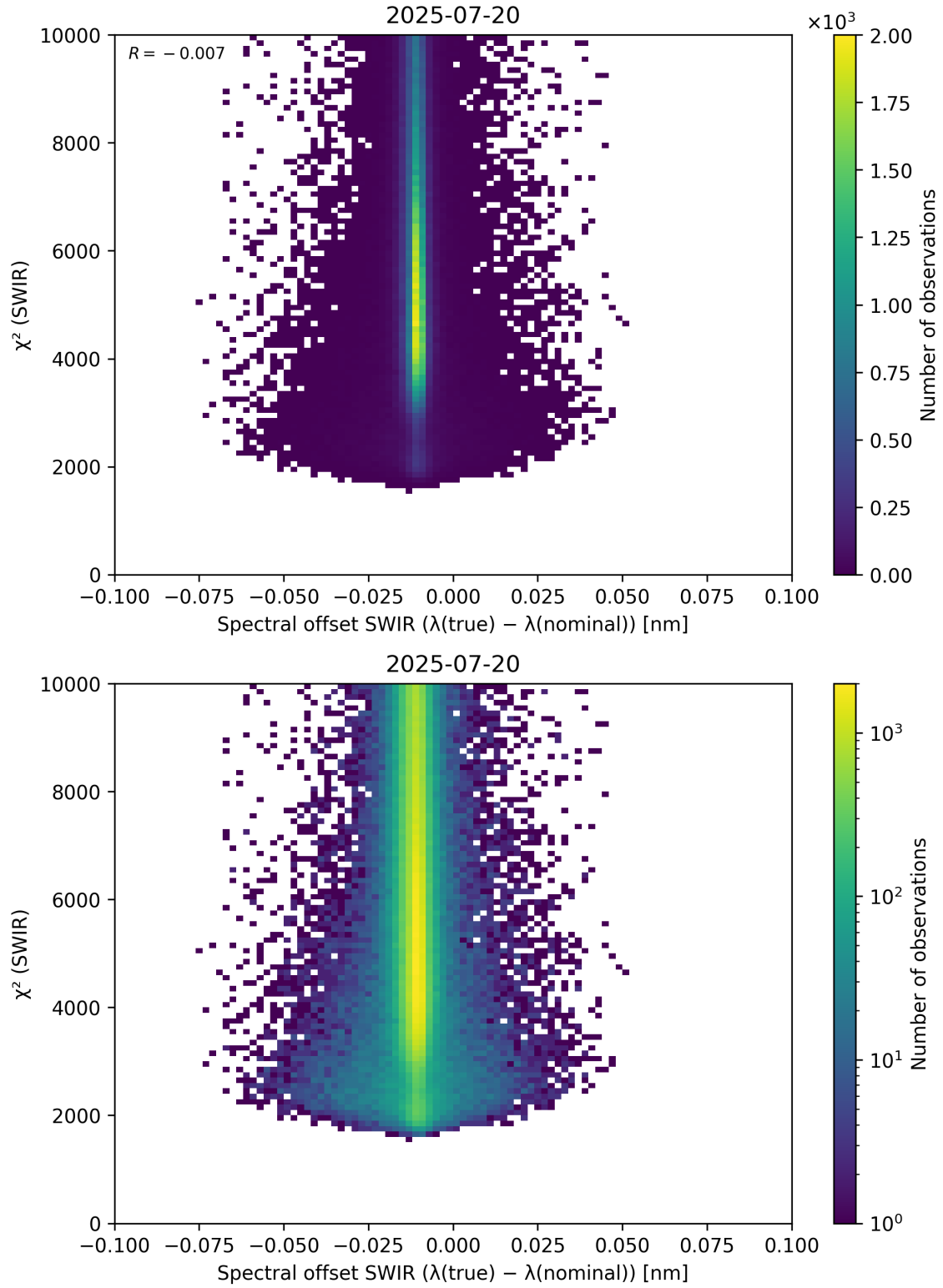
Figure 118: Scatter density plot of “Spectral offset SWIR ( \lambda_{\text{true}} - \lambda_{\text{nominal}} )” against “ \chi^2 (SWIR)” for 2025-07-19 to 2025-07-21.
