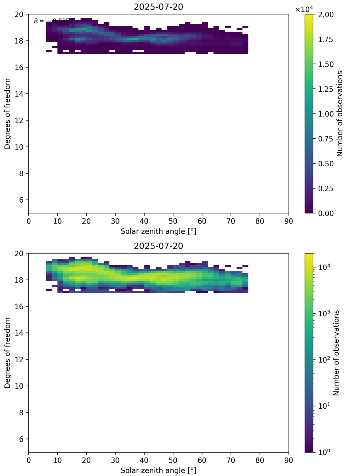
Figure 96: Scatter density plot of “Solar zenith angle” against “Degrees of freedom” for 2025-07-19 to 2025-07-21.
