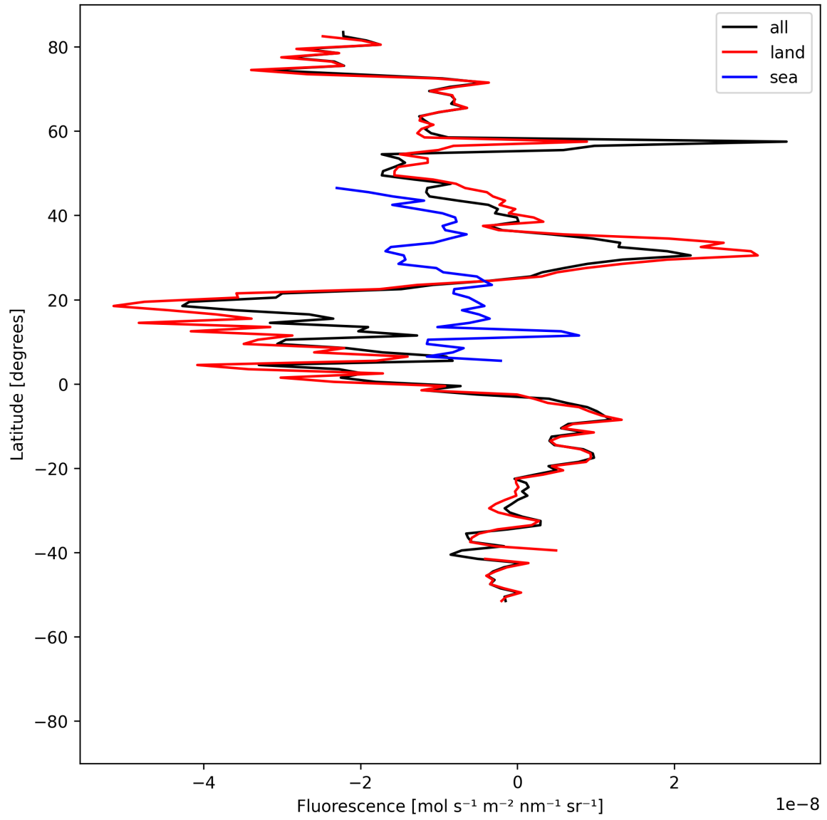
Figure 21: Zonal average of “Fluorescence” for 2025-07-19 to 2025-07-21.
