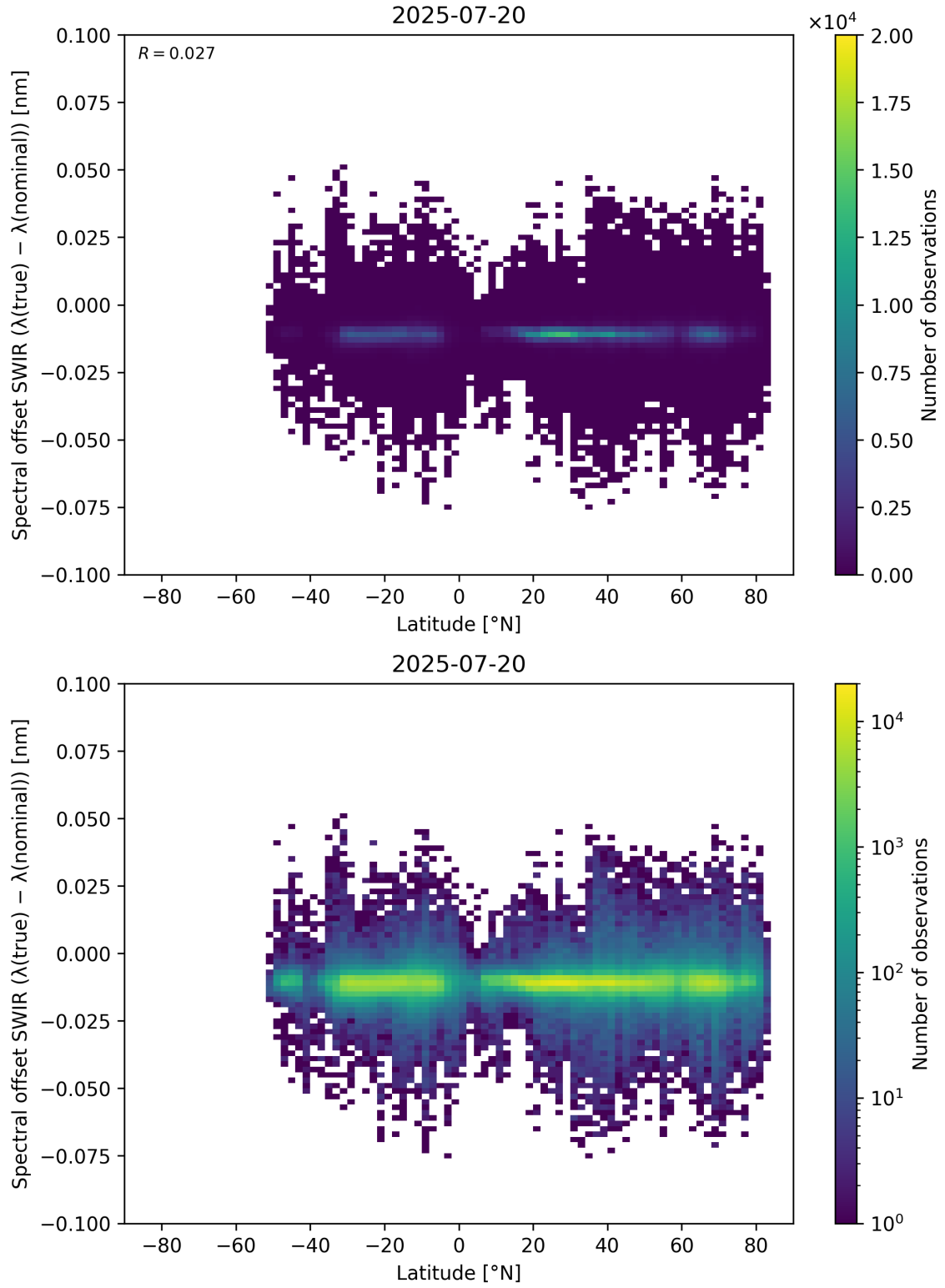
Figure 62: Scatter density plot of “Latitude” against “Spectral offset SWIR ( \lambda_{\text{true}} - \lambda_{\text{nominal}} )” for 2025-07-19 to 2025-07-21.
