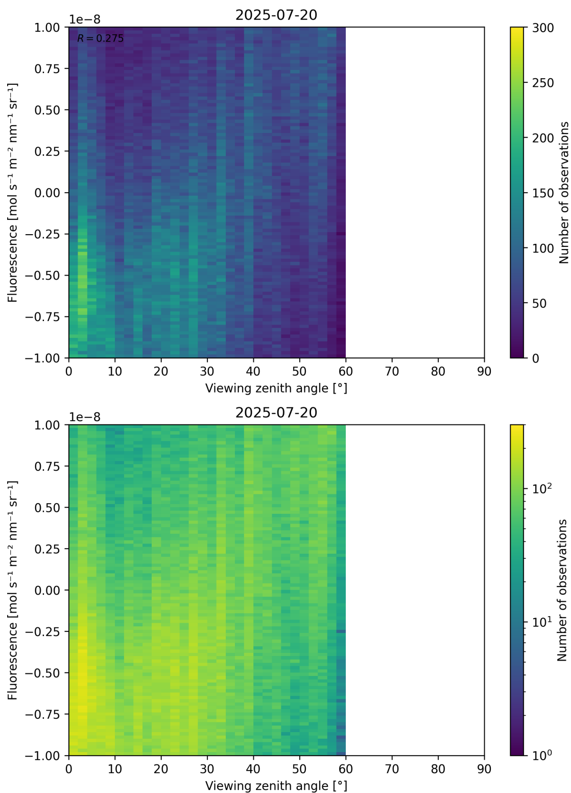
Figure 108: Scatter density plot of “Viewing zenith angle” against “Fluorescence” for 2025-07-19 to 2025-07-21.
