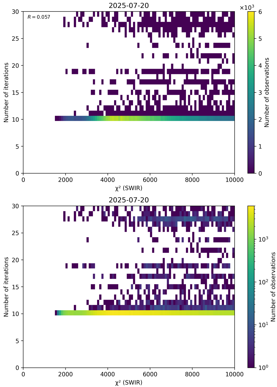
Figure 50: Scatter density plot of “ \chi^2 (SWIR)” against “Number of iterations” for 2025-07-19 to 2025-07-21.
