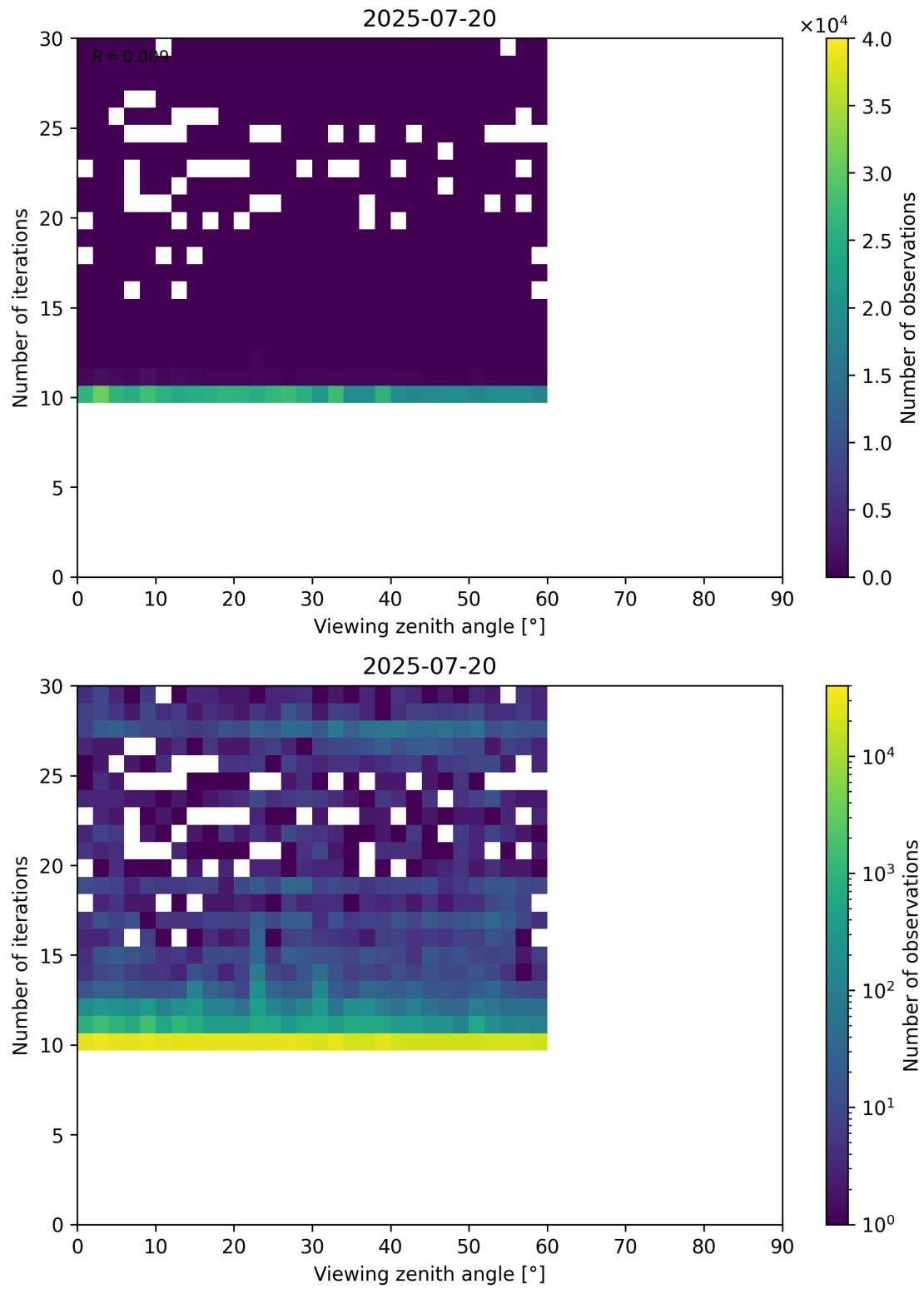
Figure 113: Scatter density plot of “Viewing zenith angle” against “Number of iterations” for 2025-07-19 to 2025-07-21.
