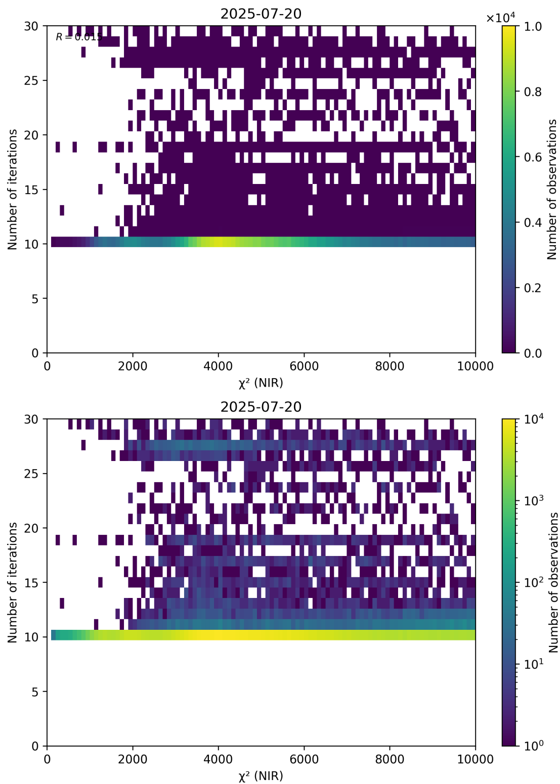
Figure 46: Scatter density plot of “ \chi^2 (NIR)” against “Number of iterations” for 2025-07-19 to 2025-07-21.
