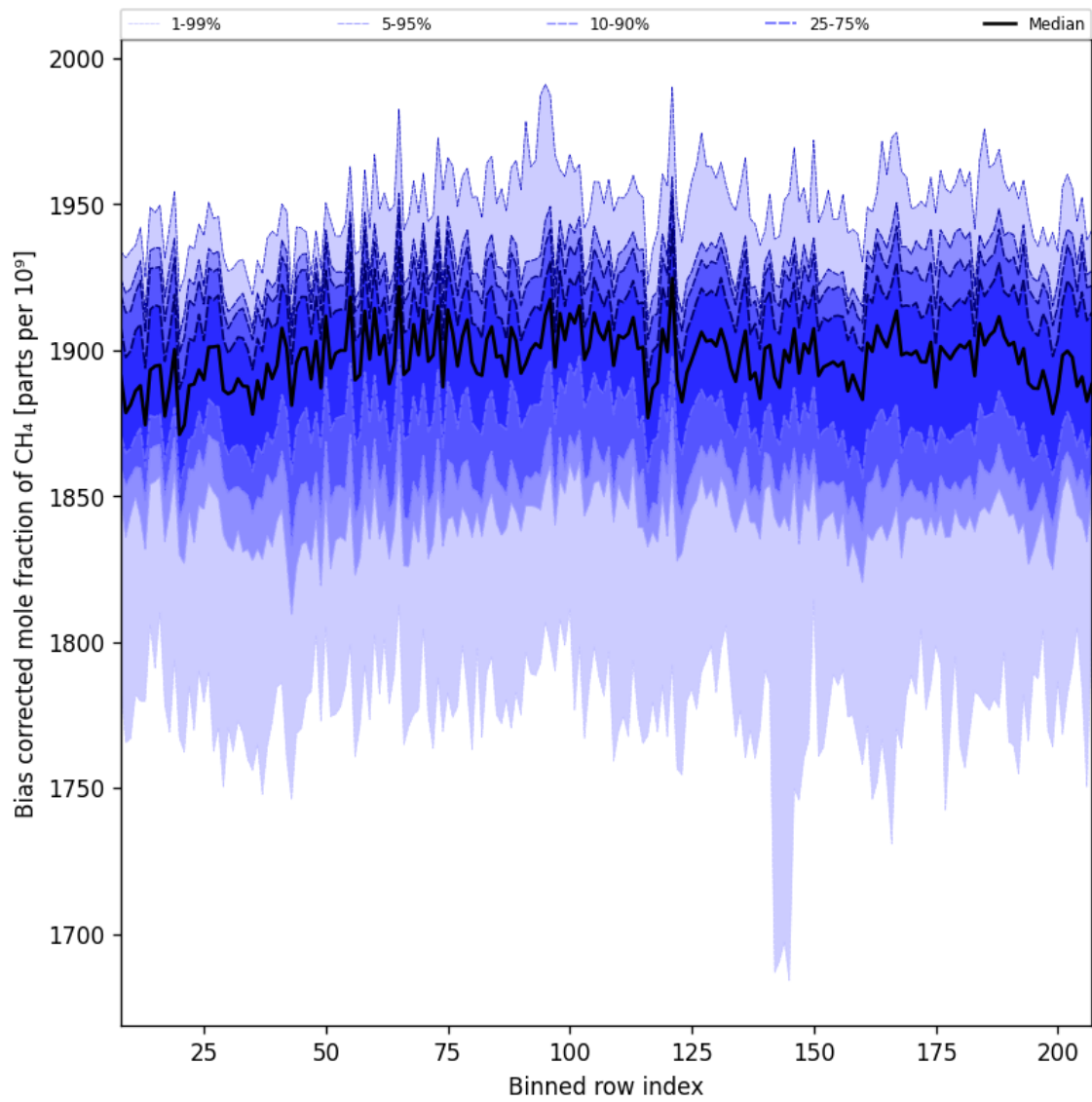
Figure 36: Along track statistics of “Bias corrected mole fraction of CH 4 ” for 2025-07-19 to 2025-07-21
