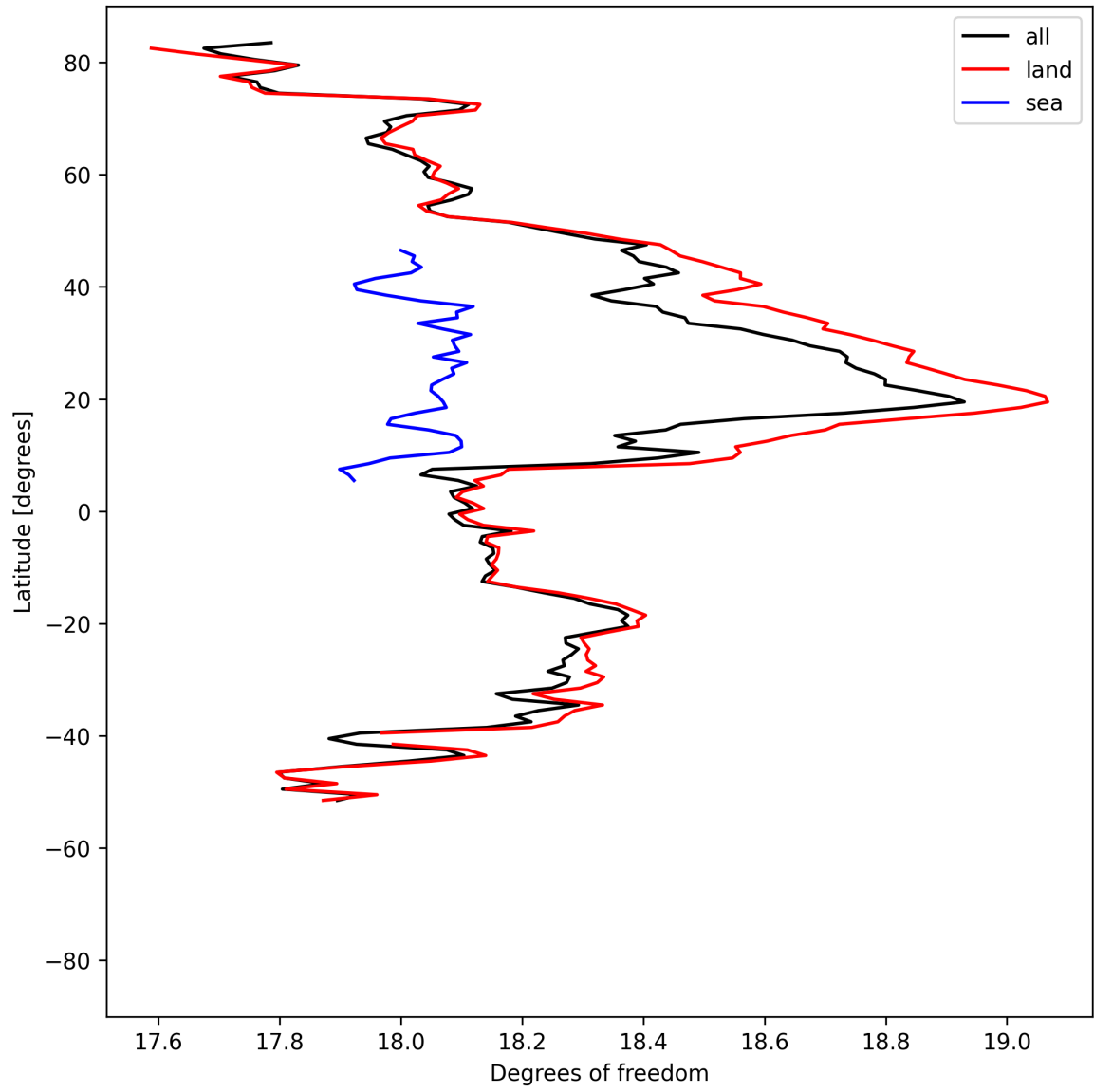
Figure 19: Zonal average of “Degrees of freedom” for 2025-07-19 to 2025-07-21.
