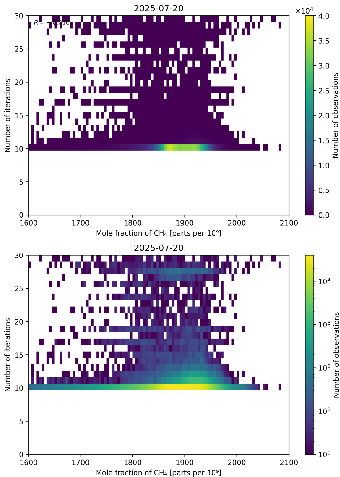
Figure 76: Scatter density plot of “Mole fraction of CH 4 ” against “Number of iterations” for 2025-07-19 to 2025-07-21.
