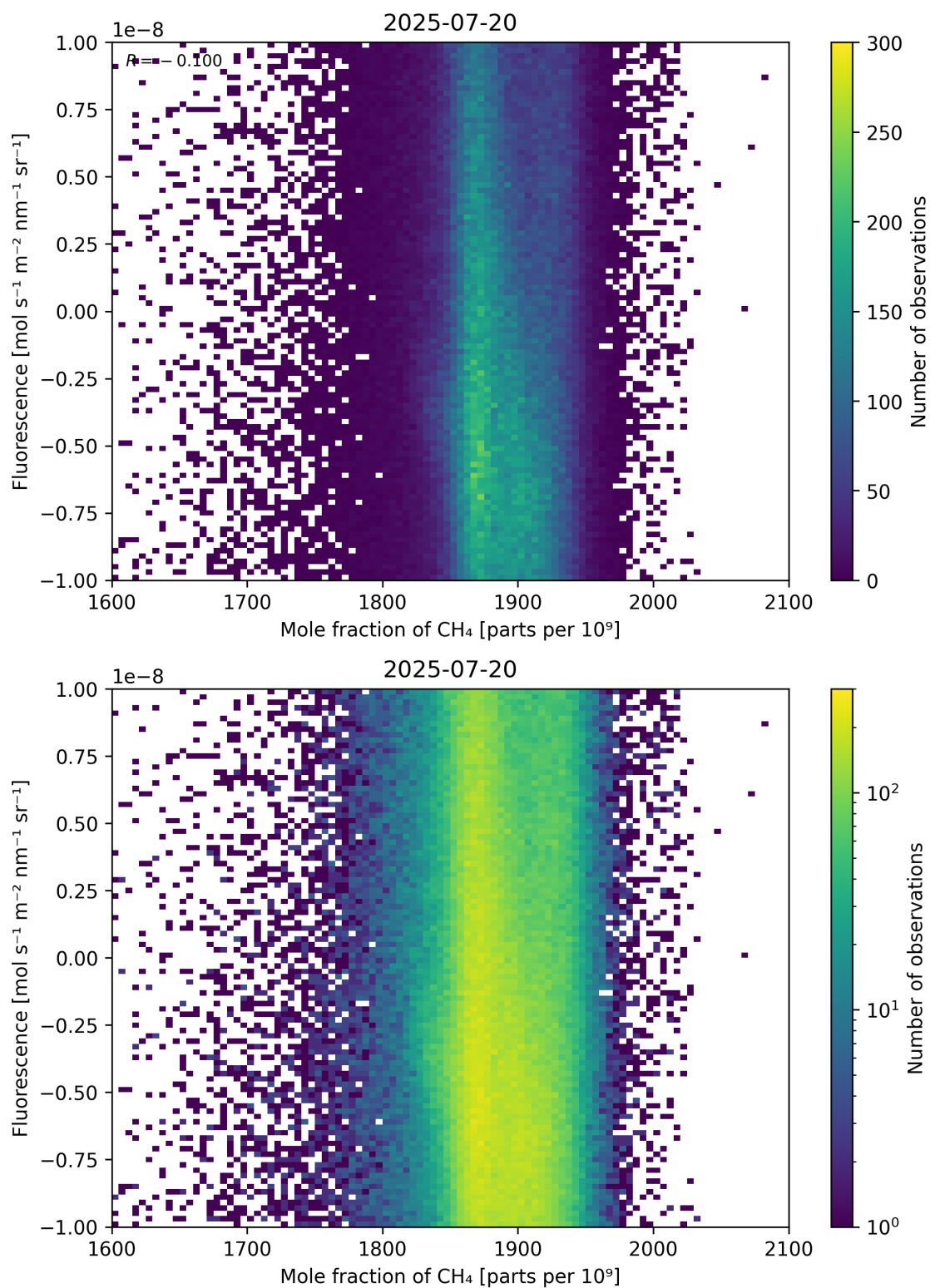
Figure 73: Scatter density plot of “Mole fraction of \text{CH}_4 ” against “Fluorescence” for 2025-07-19 to 2025-07-21.
