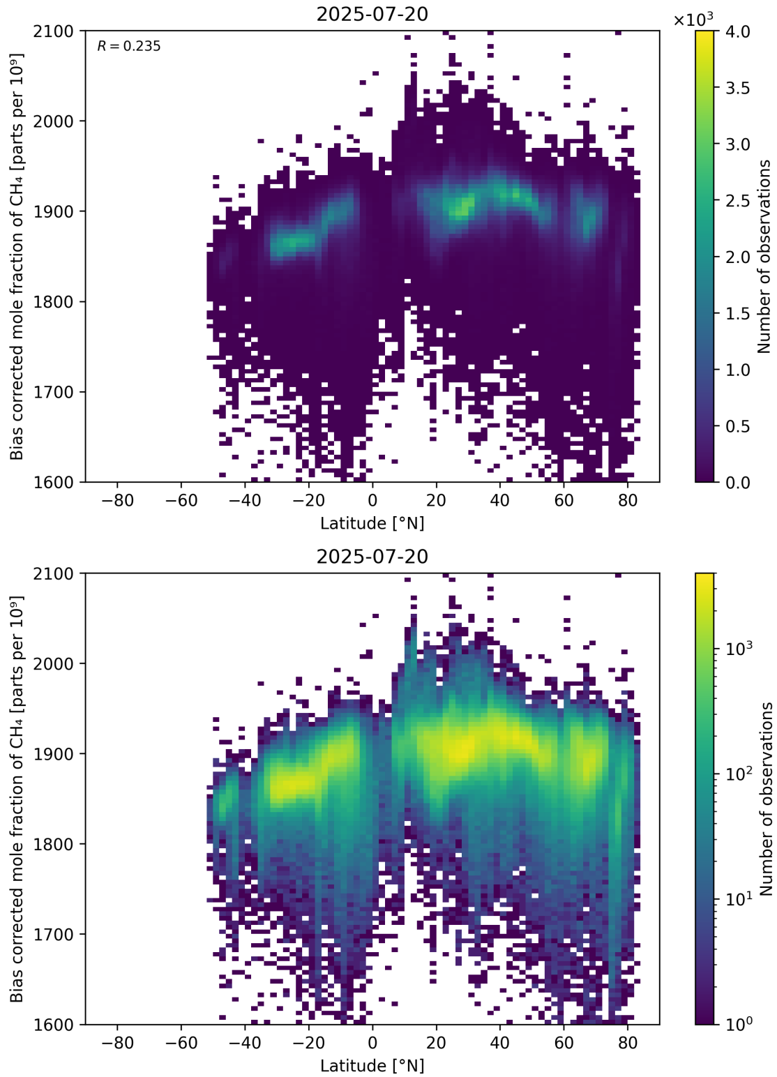
Figure 58: Scatter density plot of “Latitude” against “Bias corrected mole fraction of CH 4 ” for 2025-07-19 to 2025-07-21.
