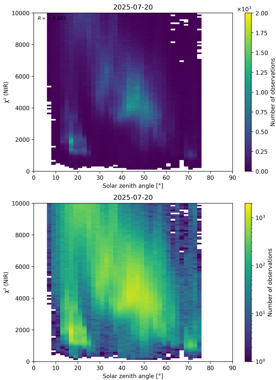
Figure 94: Scatter density plot of “Solar zenith angle” against “ \chi^2 (NIR)” for 2025-07-19 to 2025-07-21.
