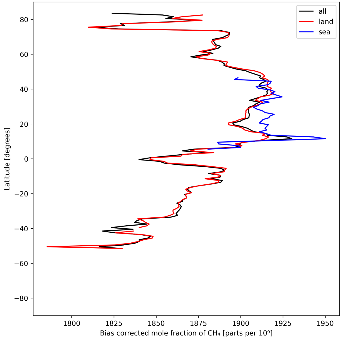
Figure 14: Zonal average of “Bias corrected mole fraction of \text{CH}_4 ” for 2025-07-19 to 2025-07-21.
