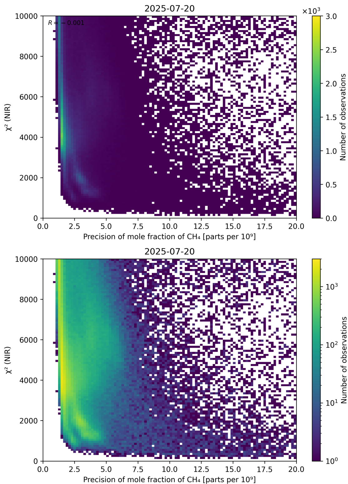
Figure 78: Scatter density plot of “Precision of mole fraction of \text{CH}_4 ” against “ \chi^2 (NIR)” for 2025-07-19 to 2025-07-21.
