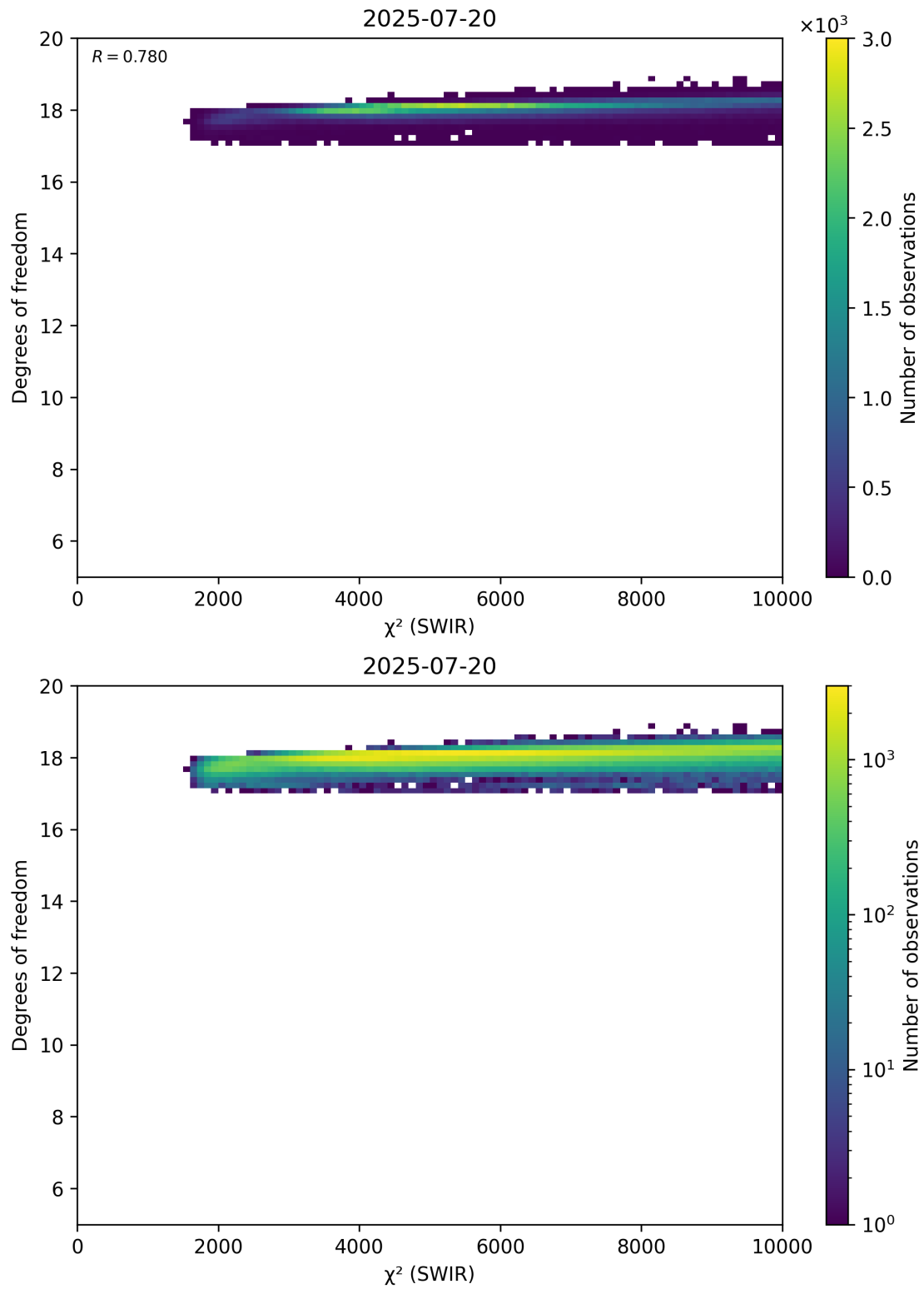
Figure 48: Scatter density plot of “ \chi^2 (SWIR)” against “Degrees of freedom” for 2025-07-19 to 2025-07-21.
