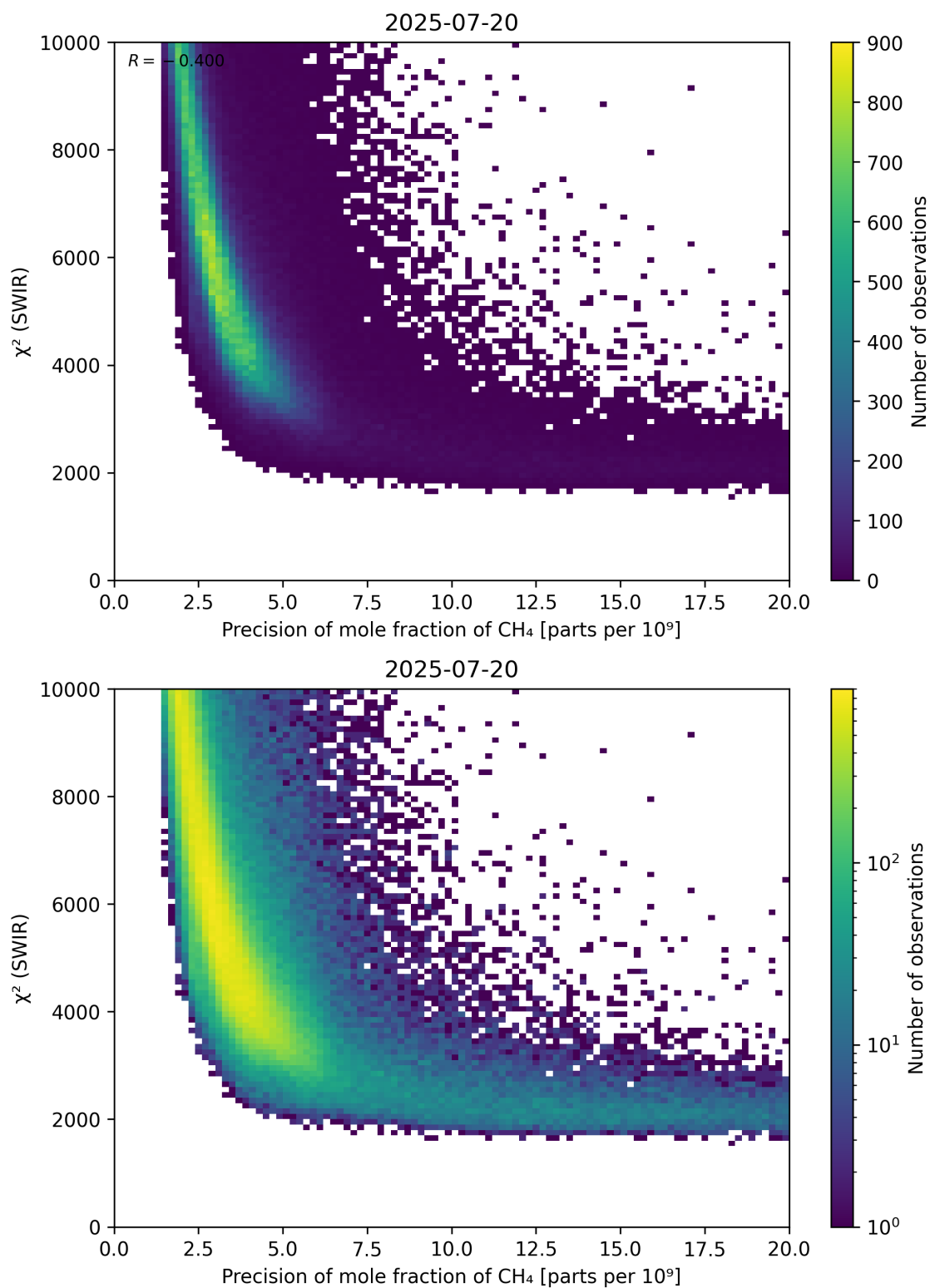
Figure 79: Scatter density plot of “Precision of mole fraction of \text{CH}_4 ” against “ \chi^2 (SWIR)” for 2025-07-19 to 2025-07-21.
