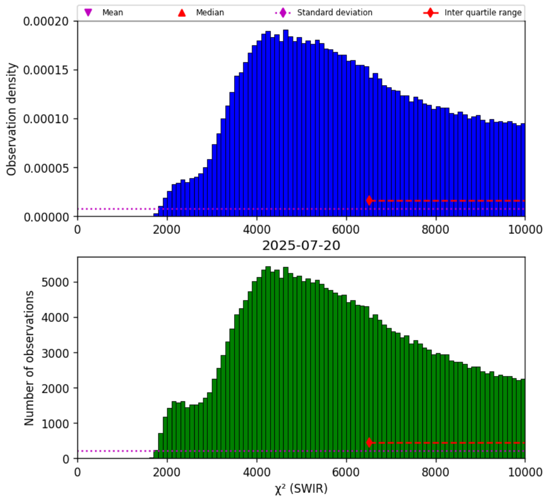
Figure 28: Histogram of " \chi^2 (SWIR)" for 2025-07-19 to 2025-07-21
