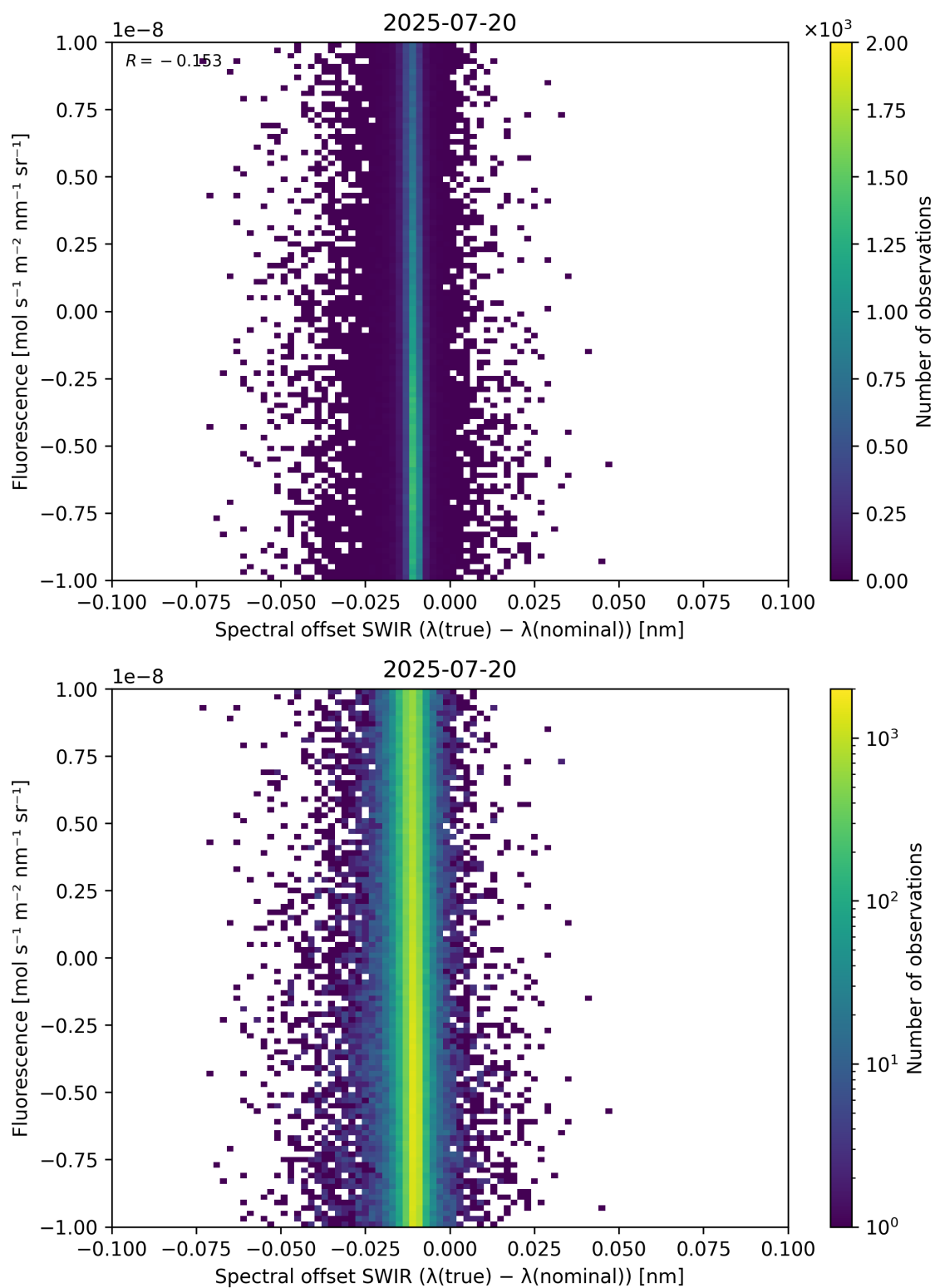
Figure 120: Scatter density plot of “Spectral offset SWIR ( \lambda_{\text{true}} - \lambda_{\text{nominal}} )” against “Fluorescence” for 2025-07-19 to 2025-07-21.
