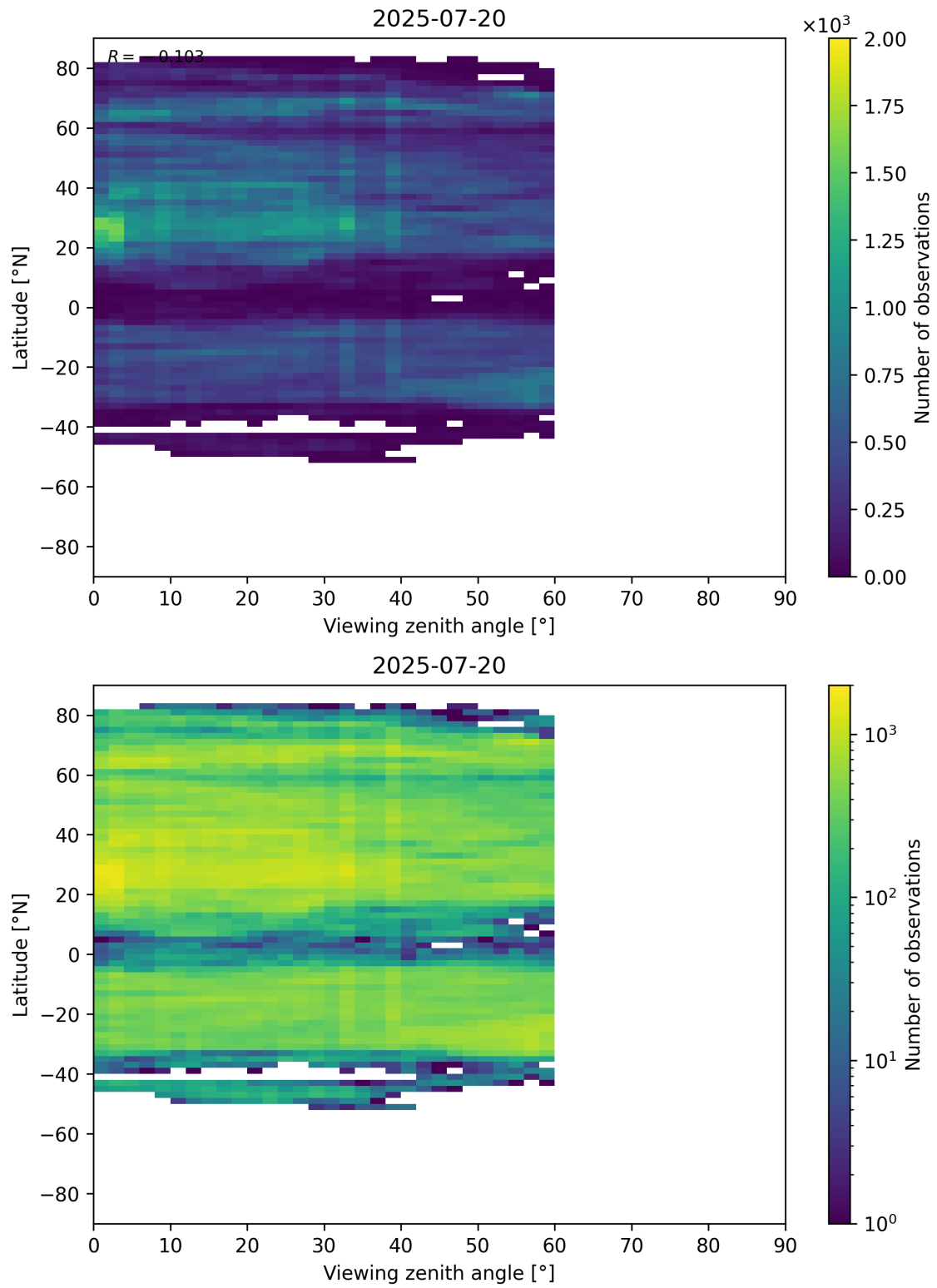
Figure 109: Scatter density plot of “Viewing zenith angle” against “Latitude” for 2025-07-19 to 2025-07-21.
