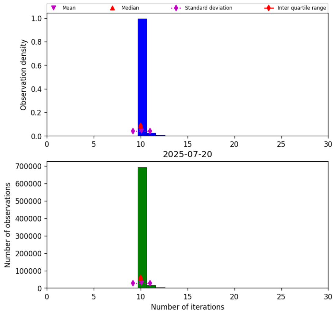
Figure 31: Histogram of "Number of iterations" for 2025-07-19 to 2025-07-21
