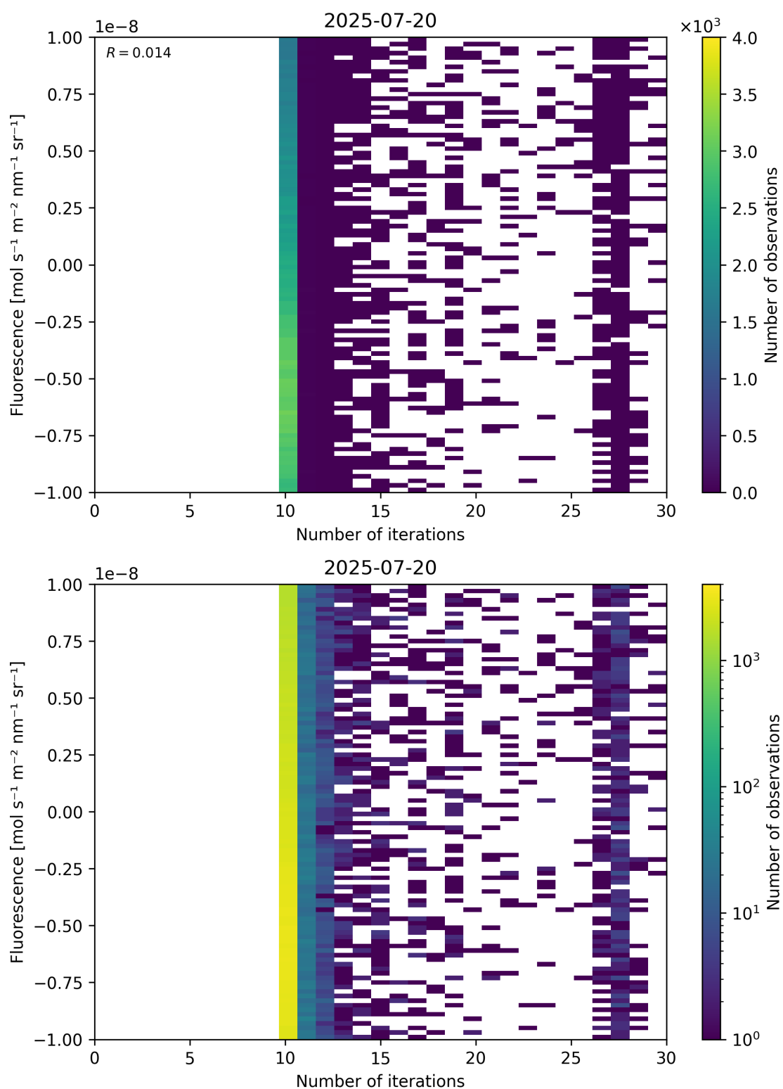
Figure 87: Scatter density plot of “Number of iterations” against “Fluorescence” for 2025-07-19 to 2025-07-21.
