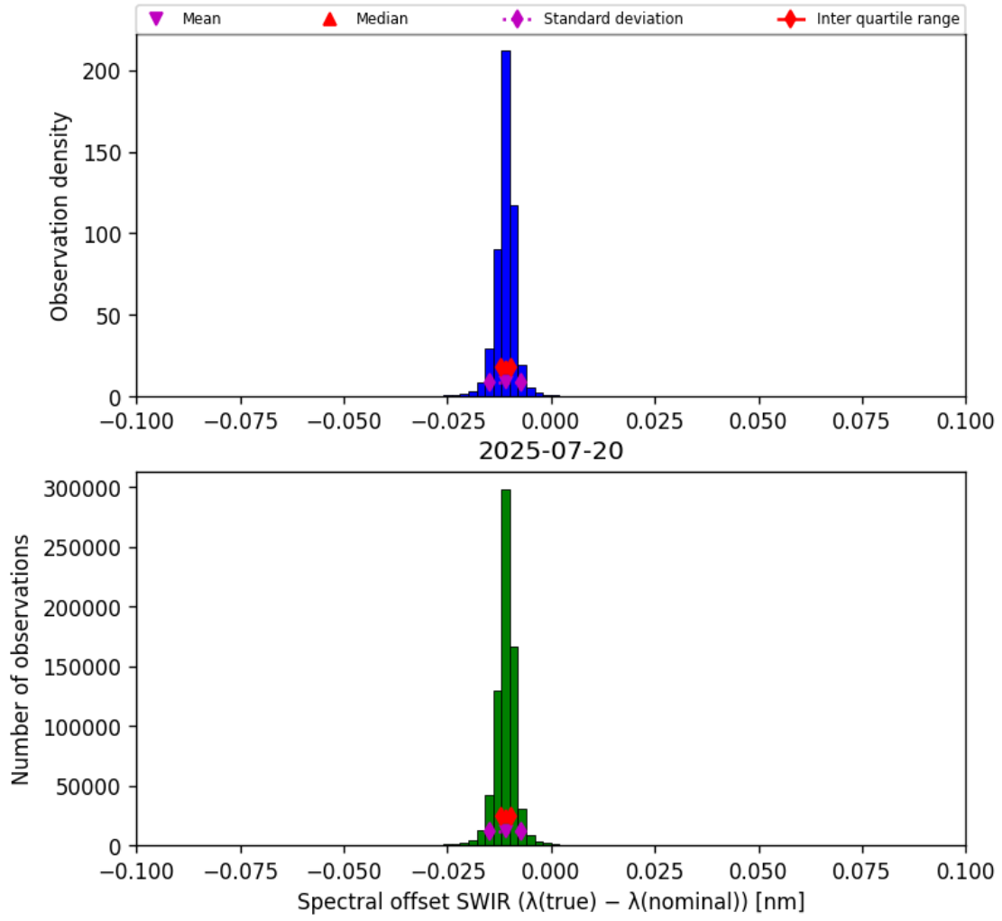
Figure 27: Histogram of “Spectral offset SWIR ( \lambda_{\text{true}} - \lambda_{\text{nominal}} )” for 2025-07-19 to 2025-07-21
