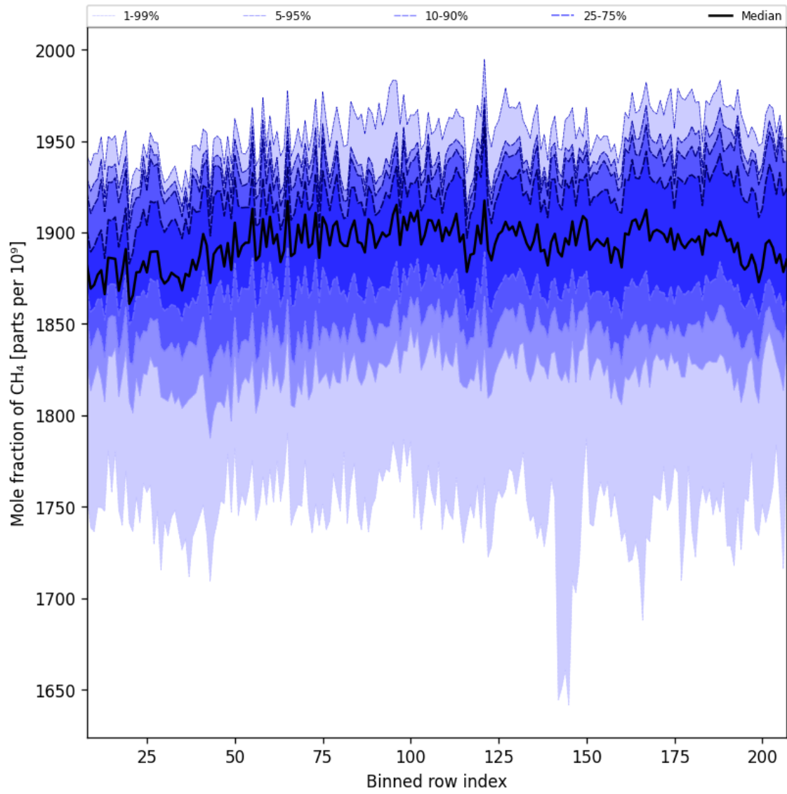
Figure 34: Along track statistics of “Mole fraction of CH 4 ” for 2025-07-19 to 2025-07-21
