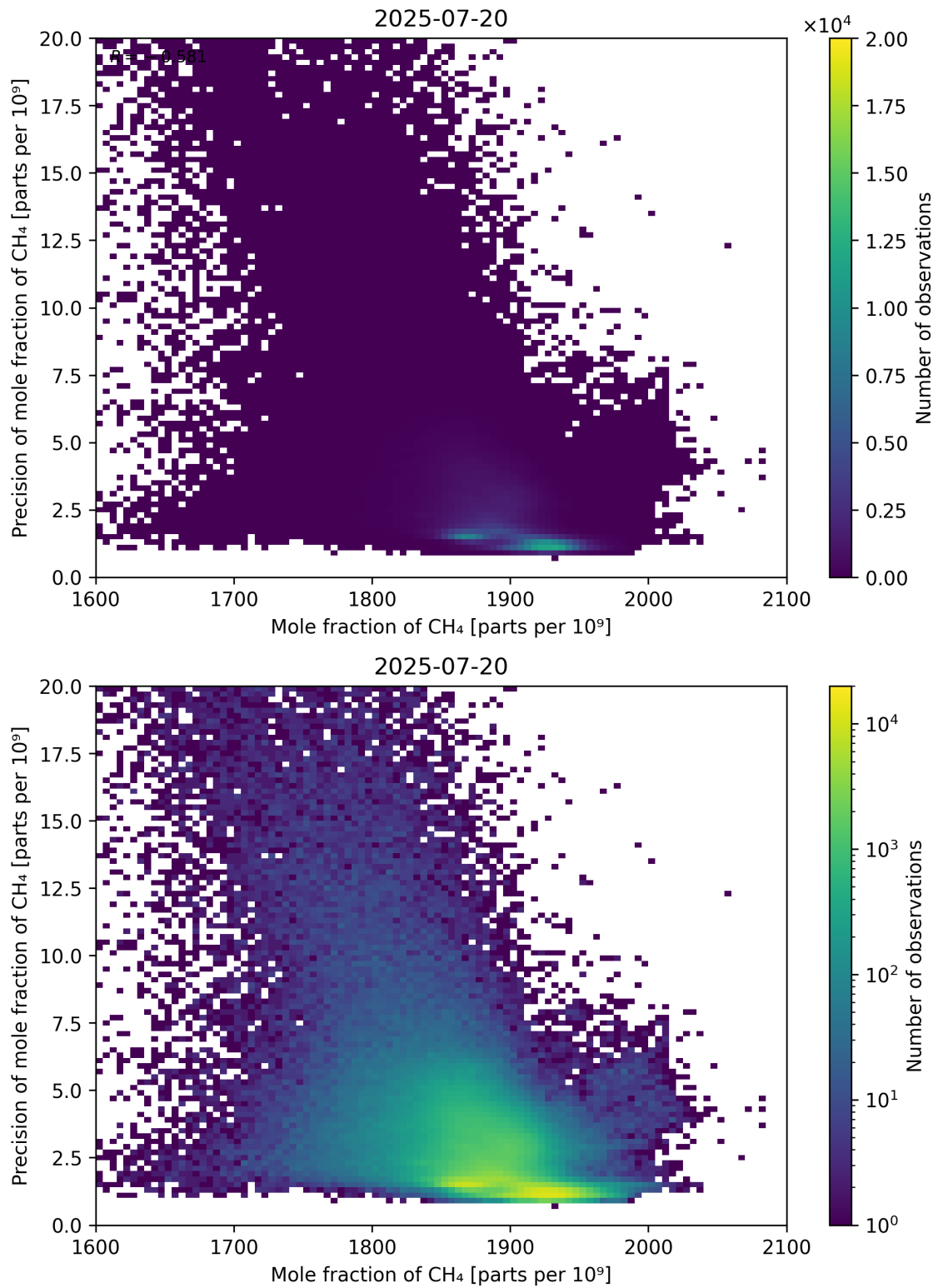
Figure 75: Scatter density plot of “Mole fraction of CH 4 ” against “Precision of mole fraction of CH 4 ” for 2025-07-19 to 2025-07-21.
