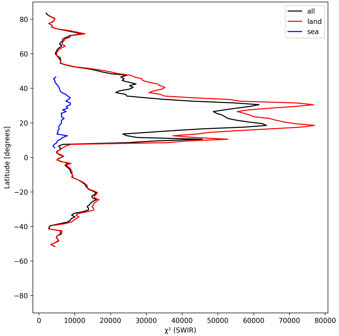
Figure 17: Zonal average of “ \chi^2 (SWIR)” for 2025-07-19 to 2025-07-21.
