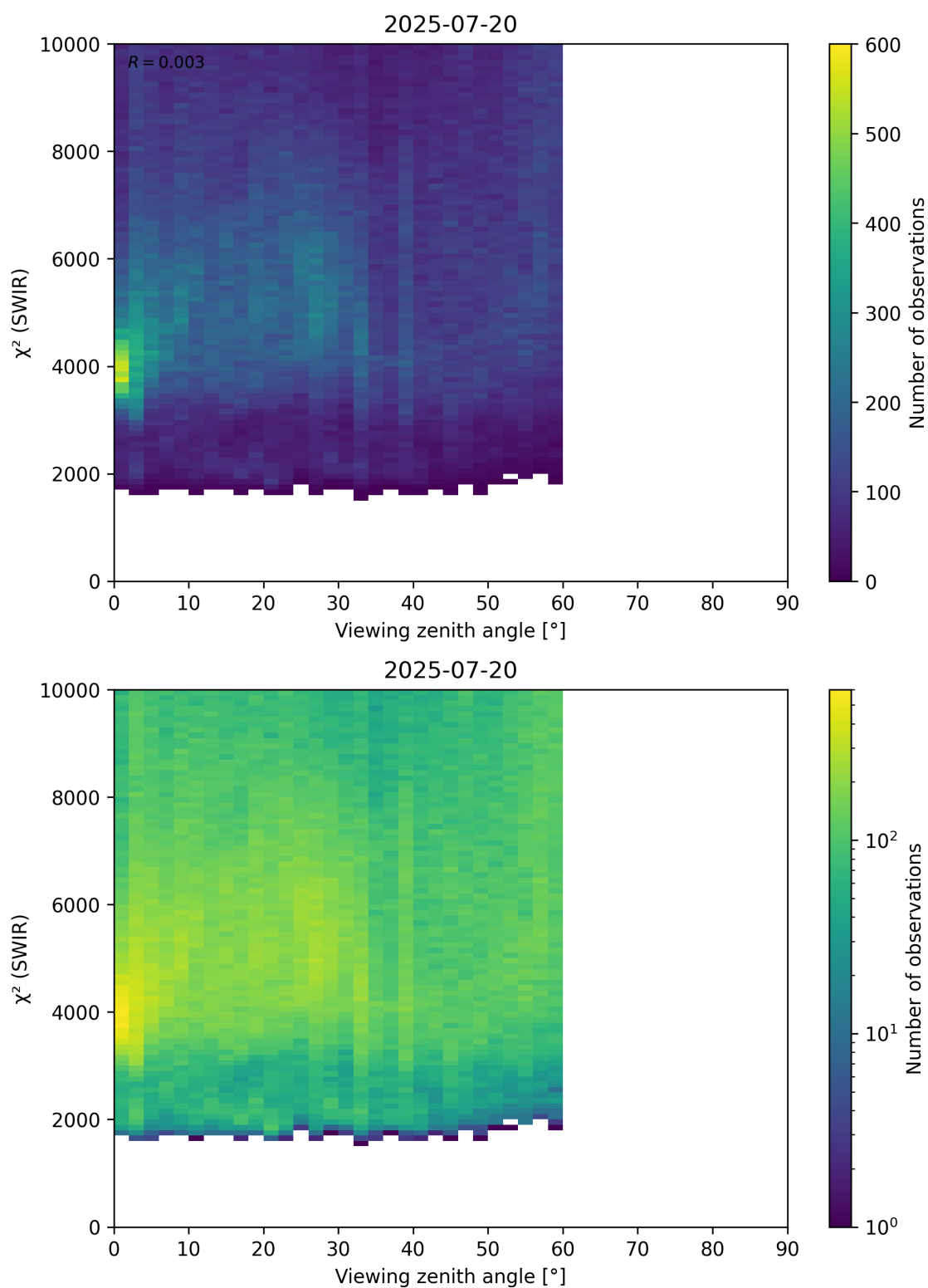
Figure 106: Scatter density plot of “Viewing zenith angle” against “ \chi^2 (SWIR)” for 2025-07-19 to 2025-07-21.
