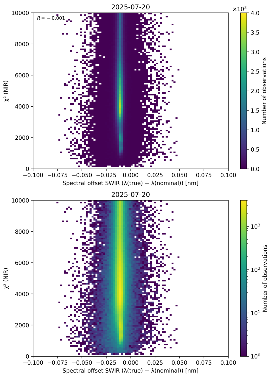
Figure 117: Scatter density plot of “Spectral offset SWIR ( \lambda_{\text{true}} - \lambda_{\text{nominal}} )” against “ \chi^2 (NIR)” for 2025-07-19 to 2025-07-21.
