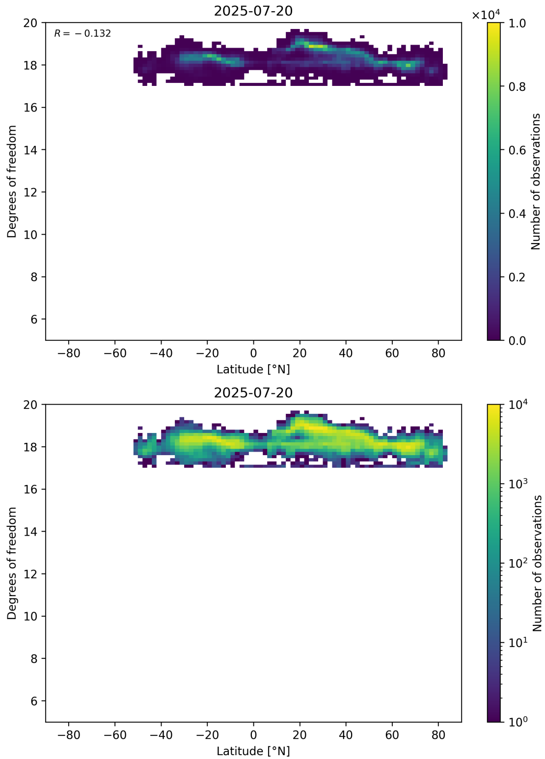
Figure 55: Scatter density plot of “Latitude” against “Degrees of freedom” for 2025-07-19 to 2025-07-21.
