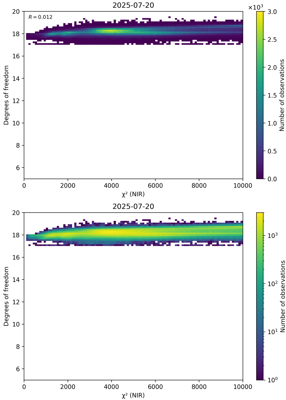
Figure 44: Scatter density plot of “ \chi^2 (NIR)” against “Degrees of freedom” for 2025-07-19 to 2025-07-21.
