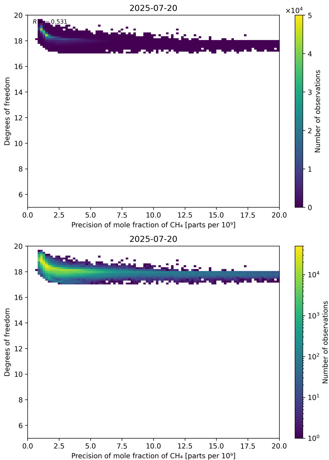
Figure 80: Scatter density plot of “Precision of mole fraction of CH 4 ” against “Degrees of freedom” for 2025-07-19 to 2025-07-21.
