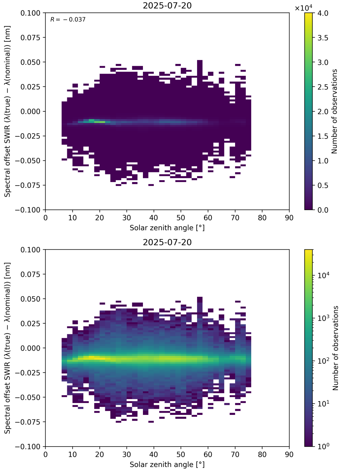
Figure 104: Scatter density plot of “Solar zenith angle” against “Spectral offset SWIR ( \lambda_{\text{true}} - \lambda_{\text{nominal}} )” for 2025-07-19 to 2025-07-21.
