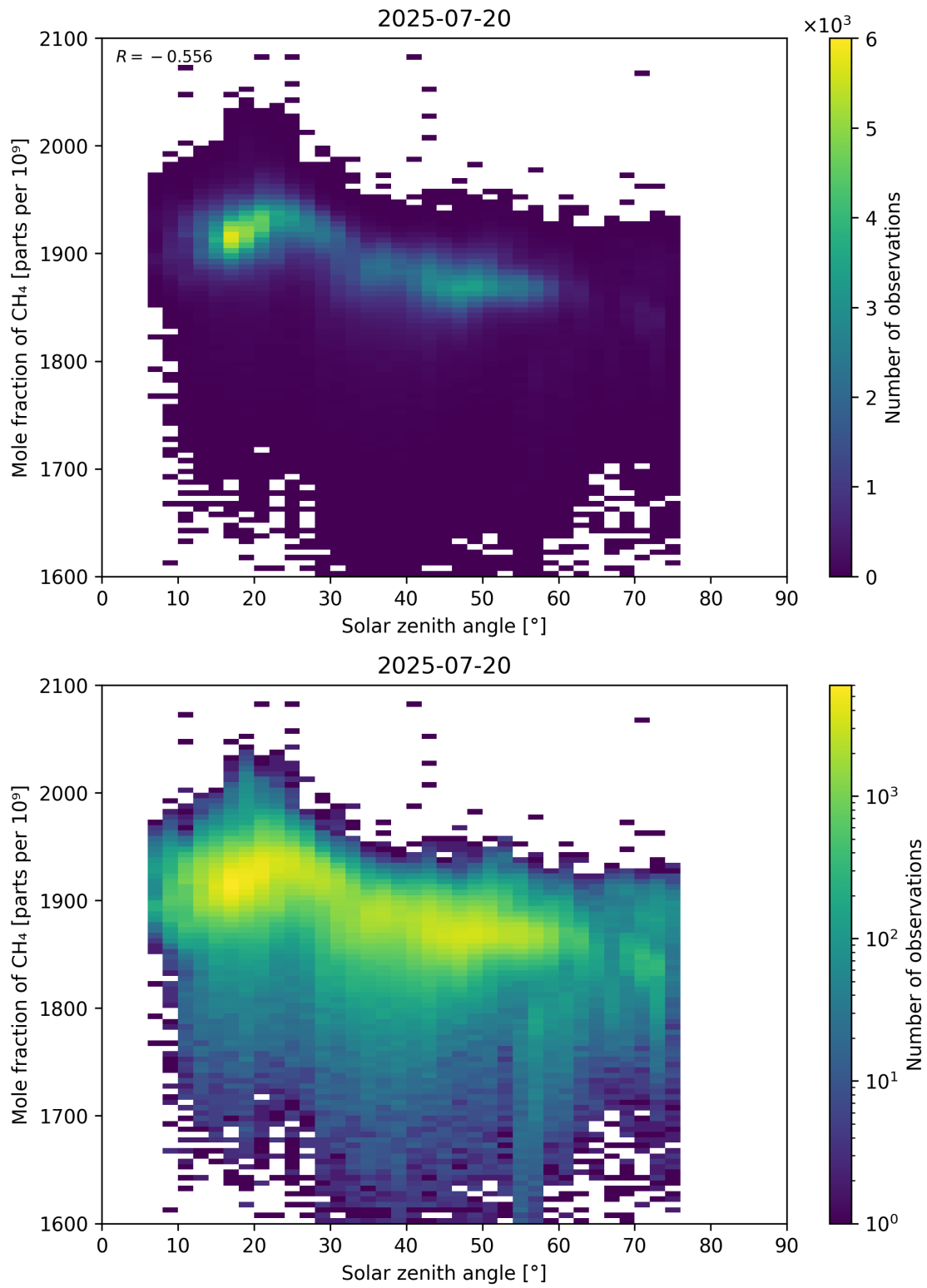
Figure 99: Scatter density plot of “Solar zenith angle” against “Mole fraction of CH 4 ” for 2025-07-19 to 2025-07-21.
