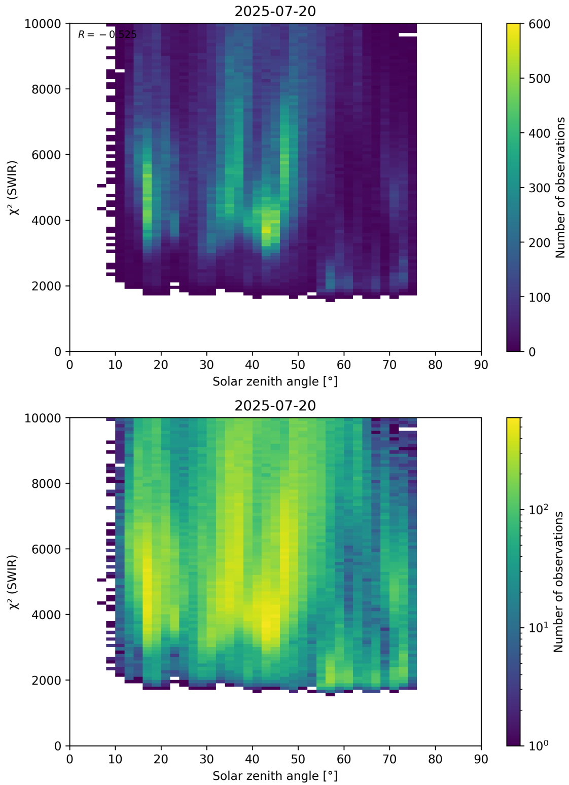
Figure 95: Scatter density plot of “Solar zenith angle” against “ \chi^2 (SWIR)” for 2025-07-19 to 2025-07-21.
