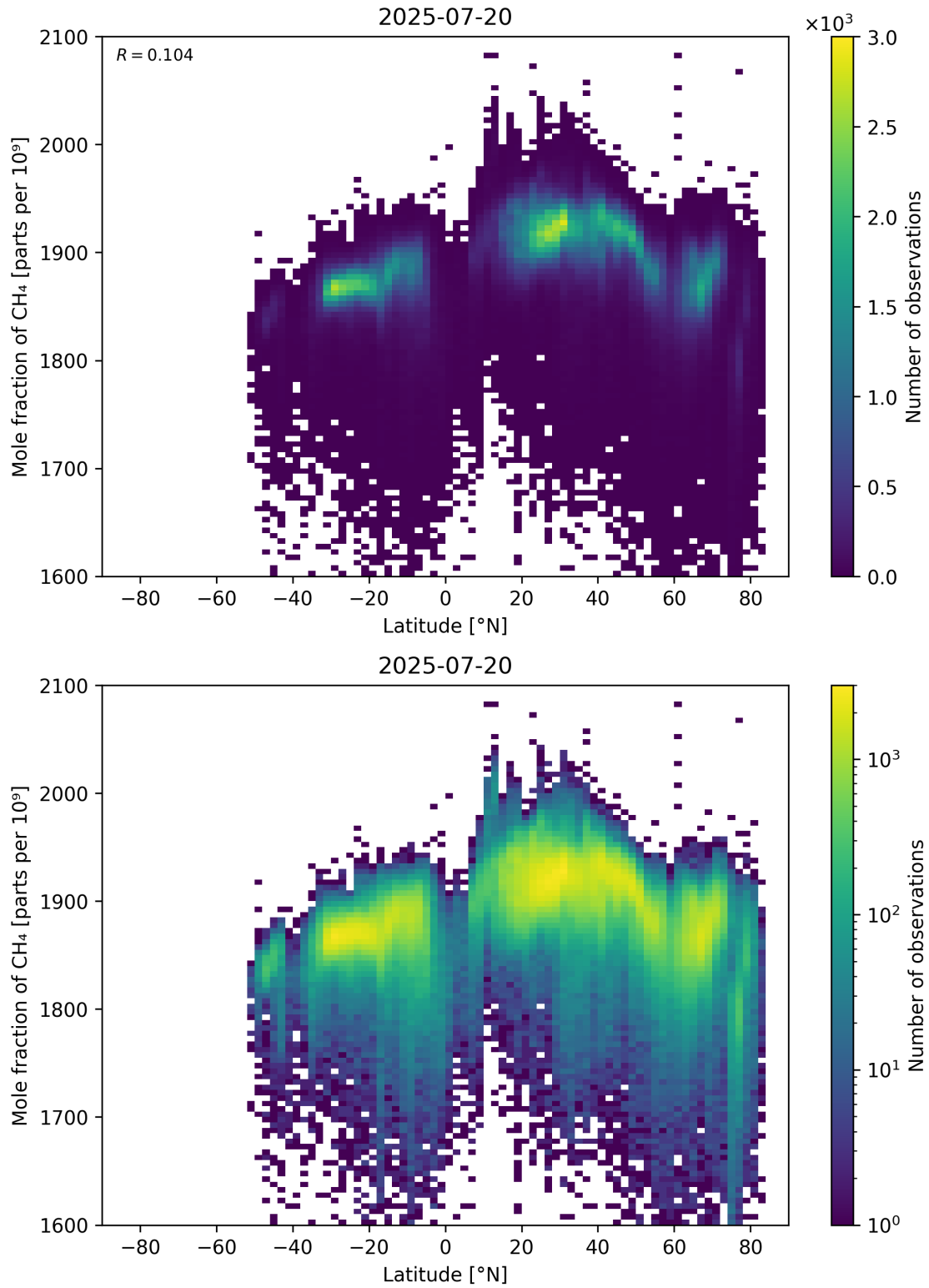
Figure 57: Scatter density plot of “Latitude” against “Mole fraction of \text{CH}_4 ” for 2025-07-19 to 2025-07-21.
