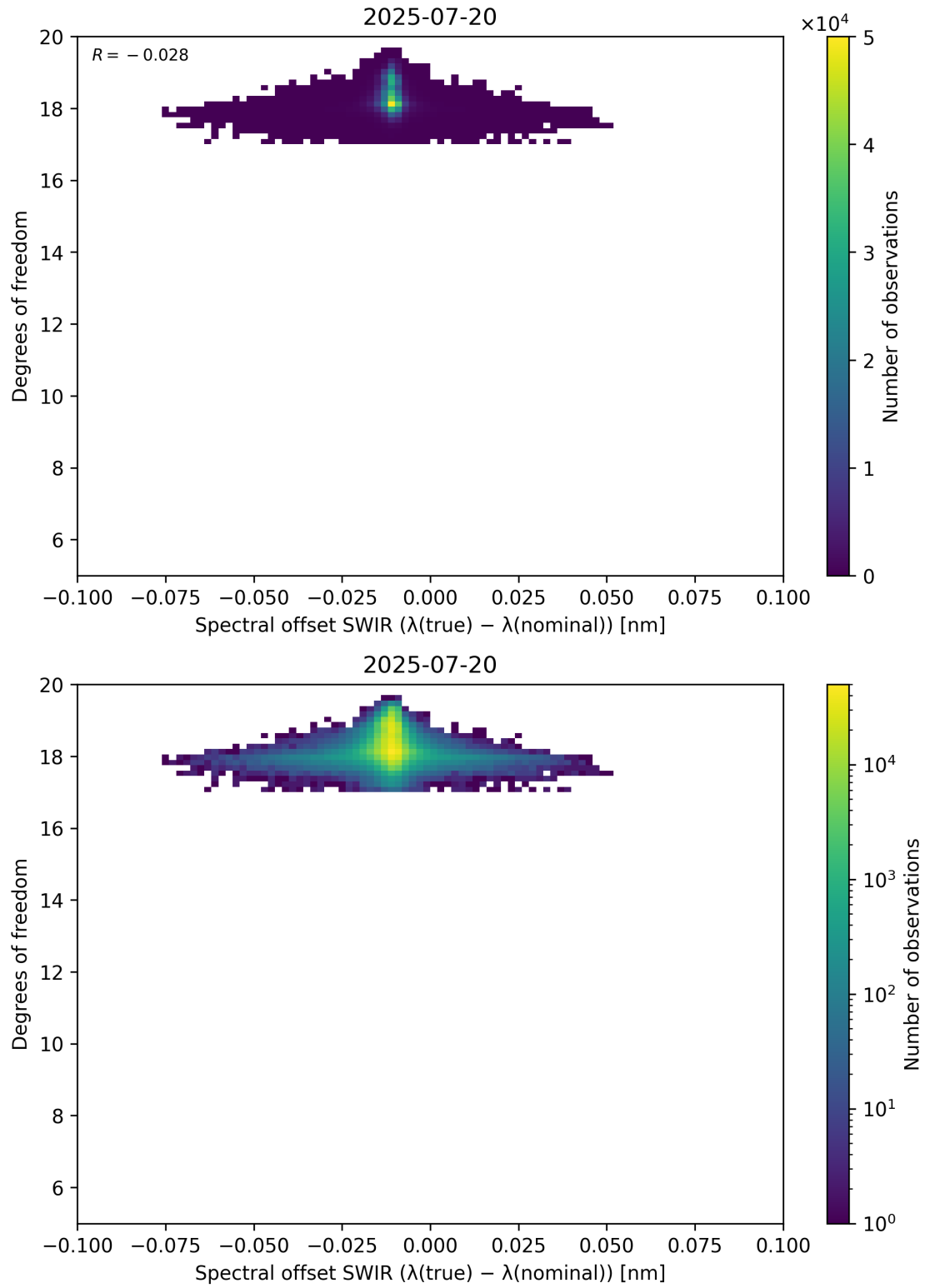
Figure 119: Scatter density plot of “Spectral offset SWIR ( \lambda_{\text{true}} - \lambda_{\text{nominal}} )” against “Degrees of freedom” for 2025-07-19 to 2025-07-21.
