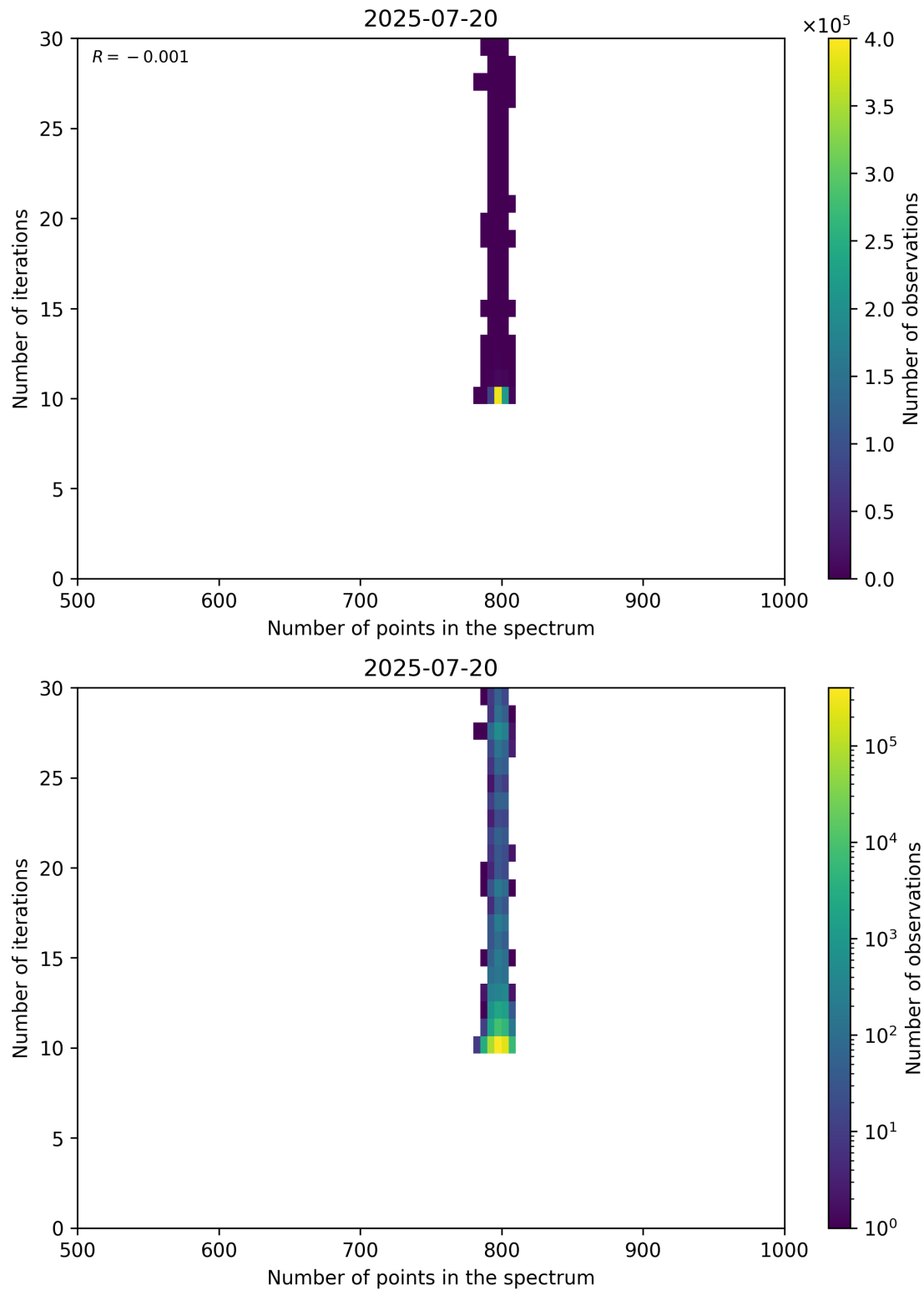
Figure 92: Scatter density plot of “Number of points in the spectrum” against “Number of iterations” for 2025-07-19 to 2025-07-21.
