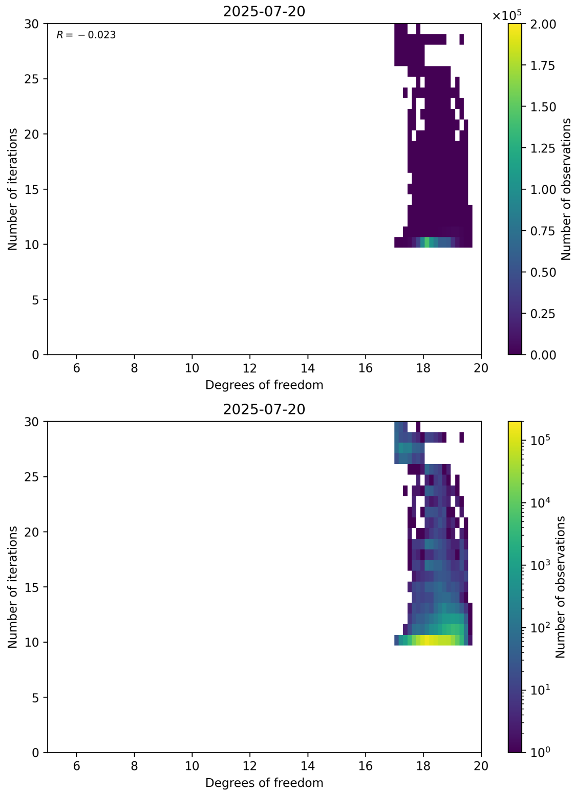
Figure 52: Scatter density plot of “Degrees of freedom” against “Number of iterations” for 2025-07-19 to 2025-07-21.
