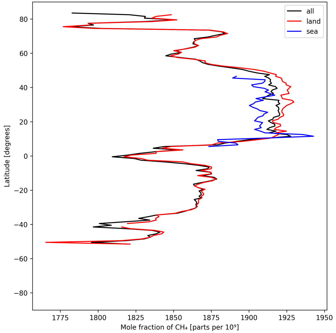
Figure 12: Zonal average of “Mole fraction of \text{CH}_4 ” for 2025-07-19 to 2025-07-21.
