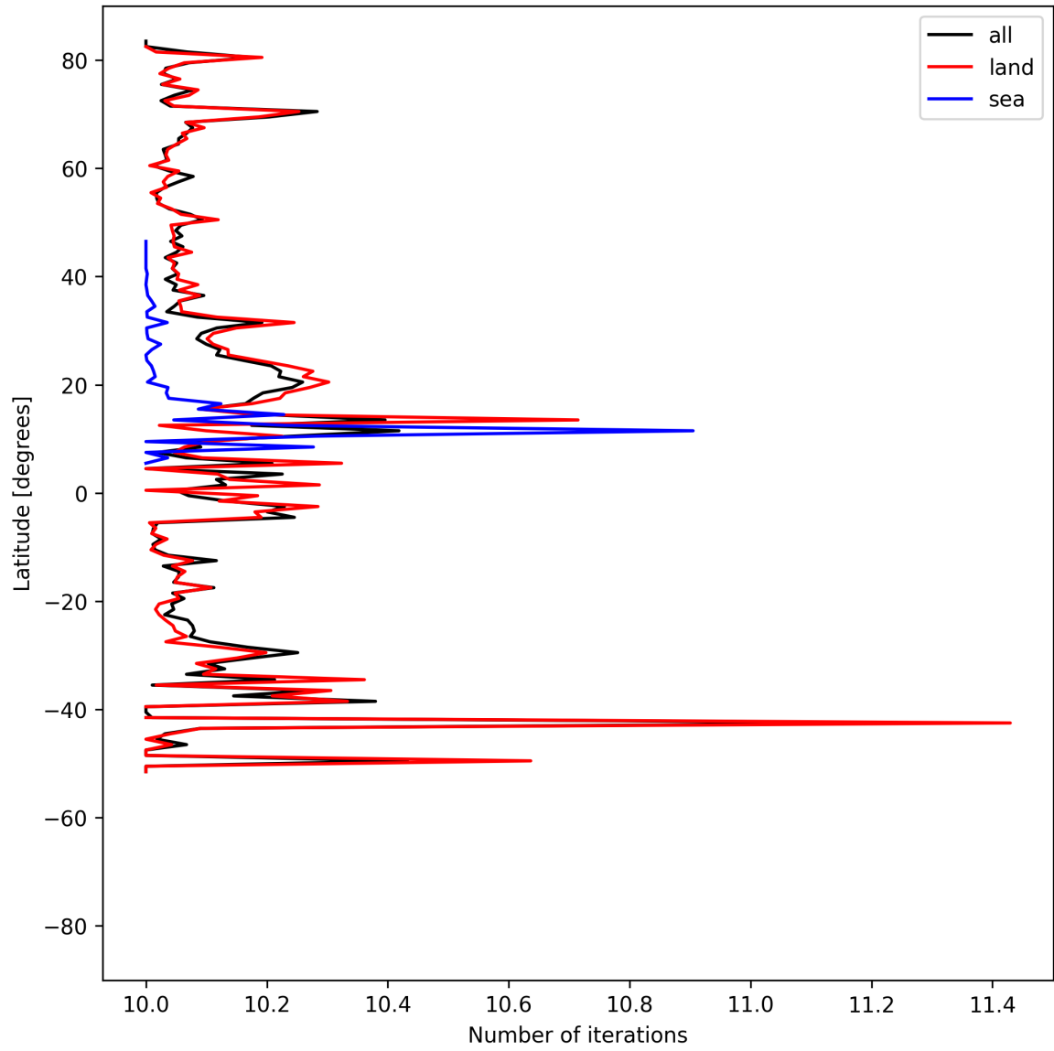
Figure 20: Zonal average of “Number of iterations” for 2025-07-19 to 2025-07-21.
