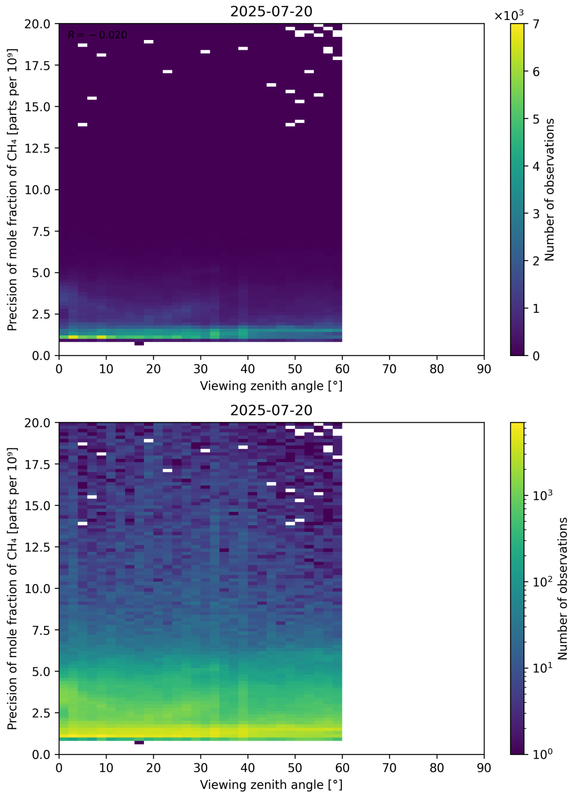
Figure 112: Scatter density plot of “Viewing zenith angle” against “Precision of mole fraction of CH 4 ” for 2025-07-19 to 2025-07-21.
