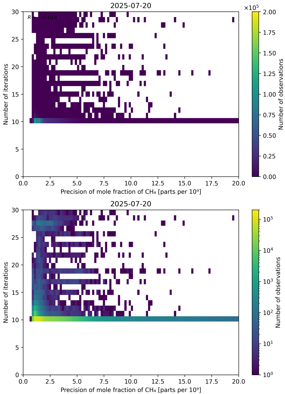
Figure 83: Scatter density plot of “Precision of mole fraction of CH 4 ” against “Number of iterations” for 2025-07-19 to 2025-07-21.
