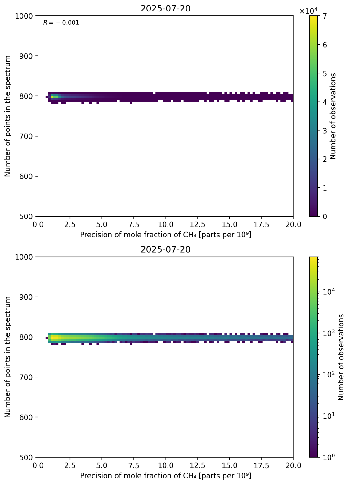
Figure 84: Scatter density plot of “Precision of mole fraction of CH 4 ” against “Number of points in the spectrum” for 2025-07-19 to 2025-07-21.
