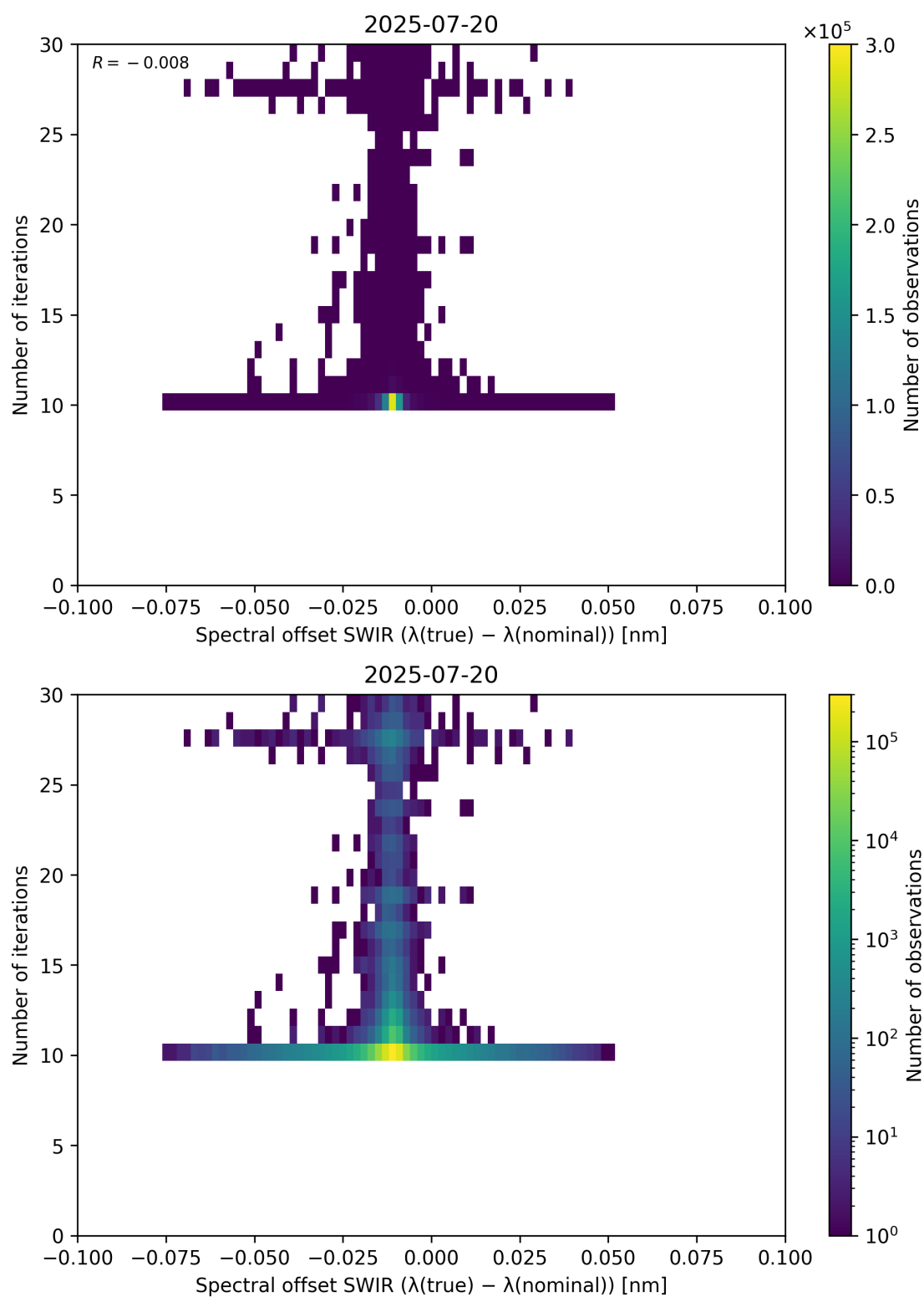
Figure 121: Scatter density plot of “Spectral offset SWIR ( \lambda_{\text{true}} - \lambda_{\text{nominal}} )” against “Number of iterations” for 2025-07-19 to 2025-07-21.
