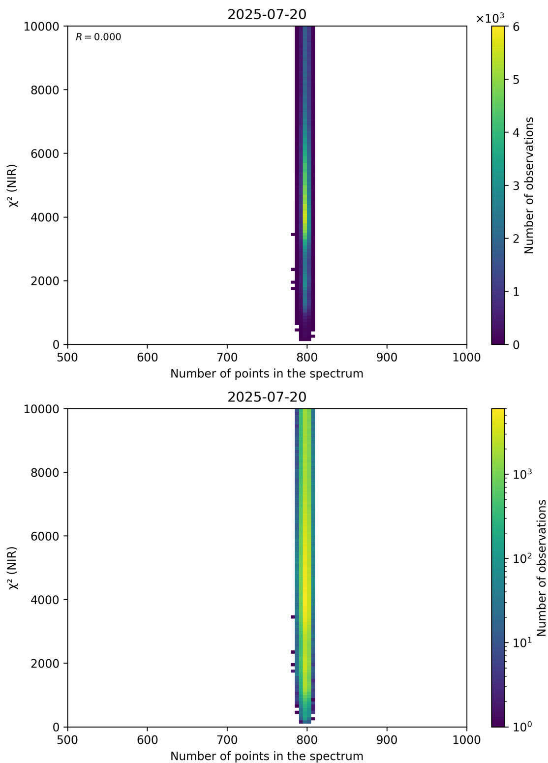
Figure 88: Scatter density plot of “Number of points in the spectrum” against “ \chi^2 (NIR)” for 2025-07-19 to 2025-07-21.
