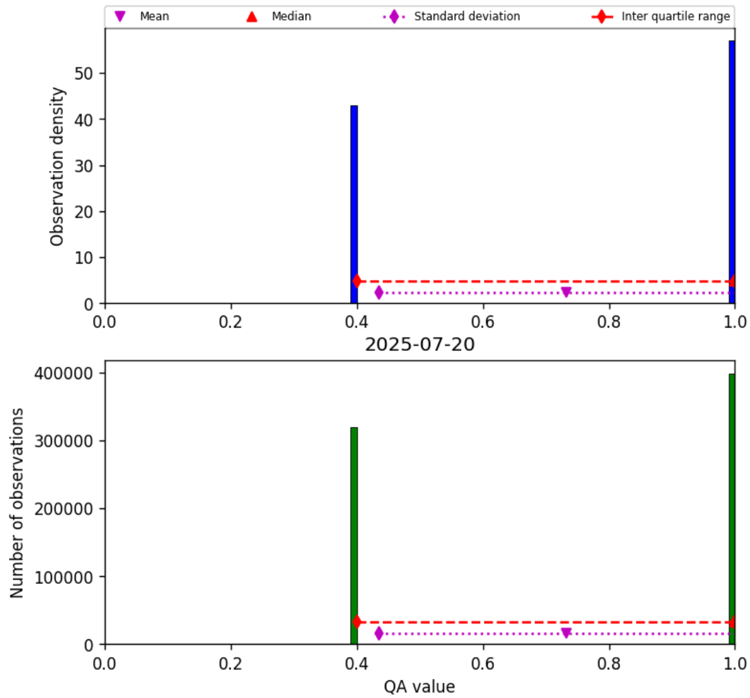
Figure 22: Histogram of “QA value” for 2025-07-19 to 2025-07-21
