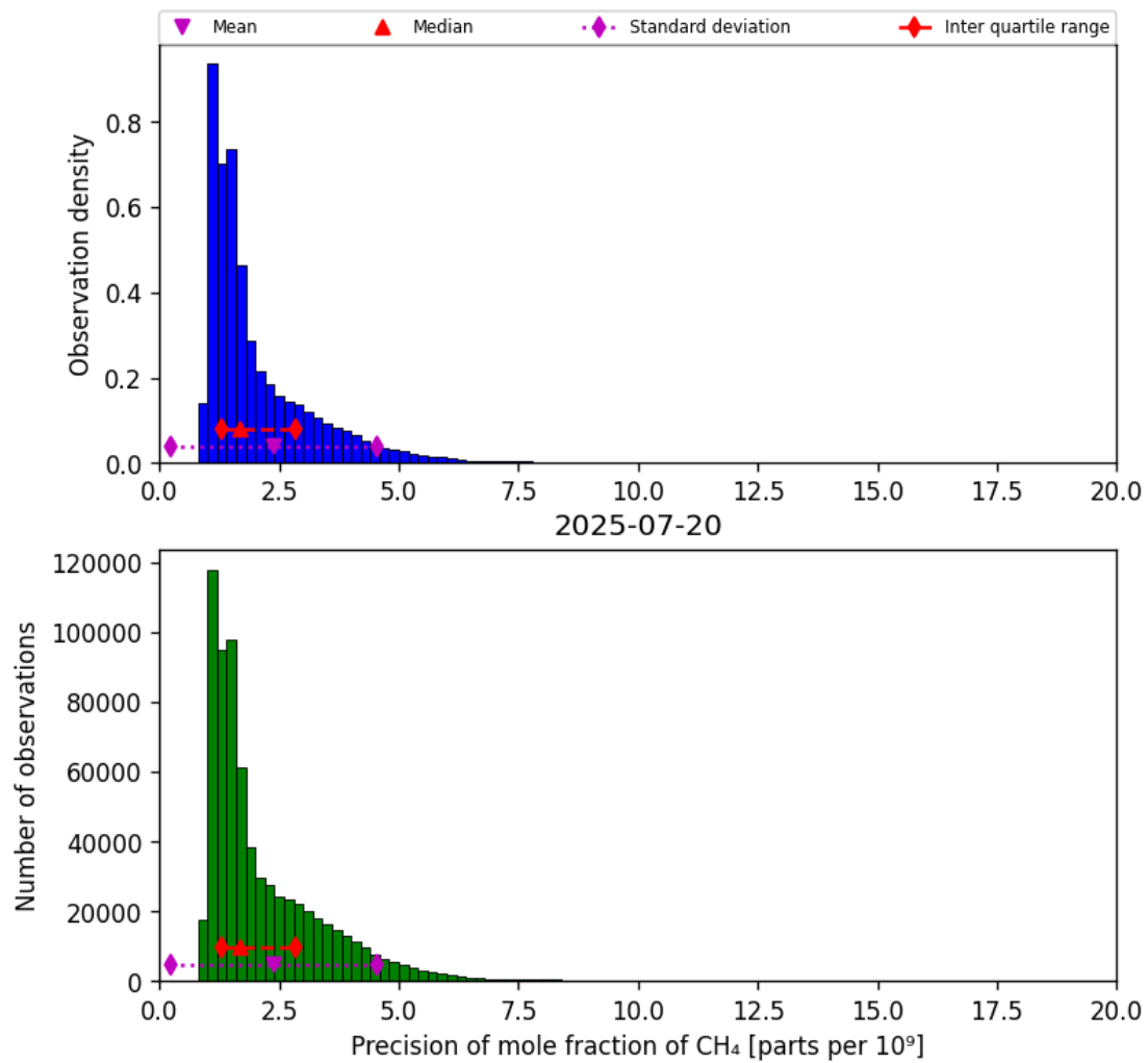
Figure 24: Histogram of “Precision of mole fraction of CH 4 ” for 2025-07-19 to 2025-07-21
