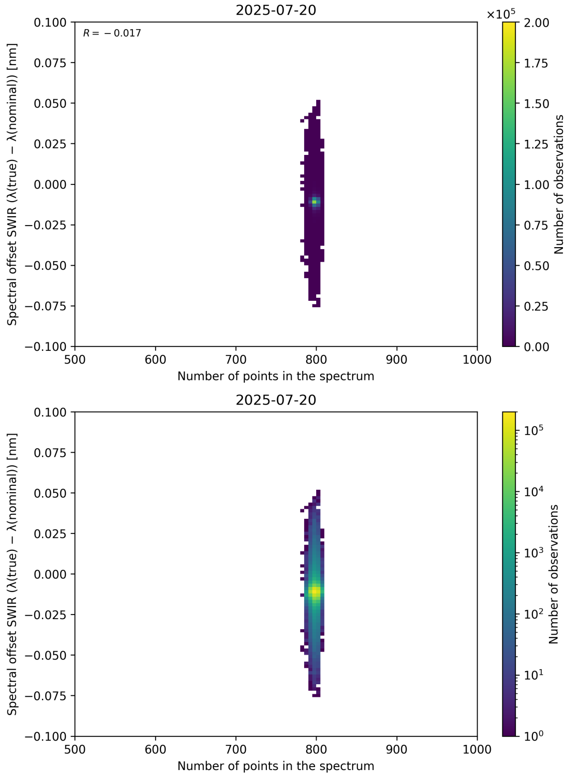
Figure 93: Scatter density plot of “Number of points in the spectrum” against “Spectral offset SWIR ( \lambda_{\text{true}} - \lambda_{\text{nominal}} )” for 2025-07-19 to 2025-07-21.
