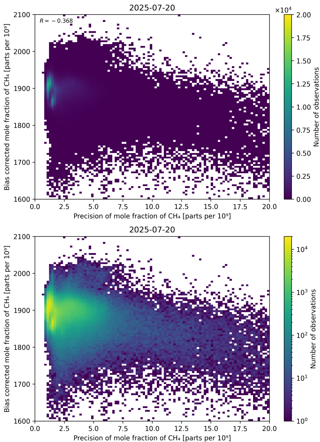
Figure 82: Scatter density plot of “Precision of mole fraction of CH 4 ” against “Bias corrected mole fraction of CH 4 ” for 2025-07-19 to 2025-07-21.
