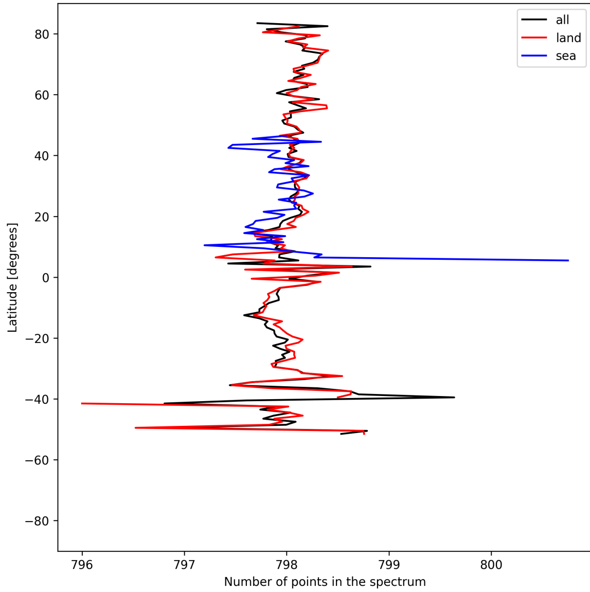
Figure 15: Zonal average of “Number of points in the spectrum” for 2025-07-19 to 2025-07-21.
