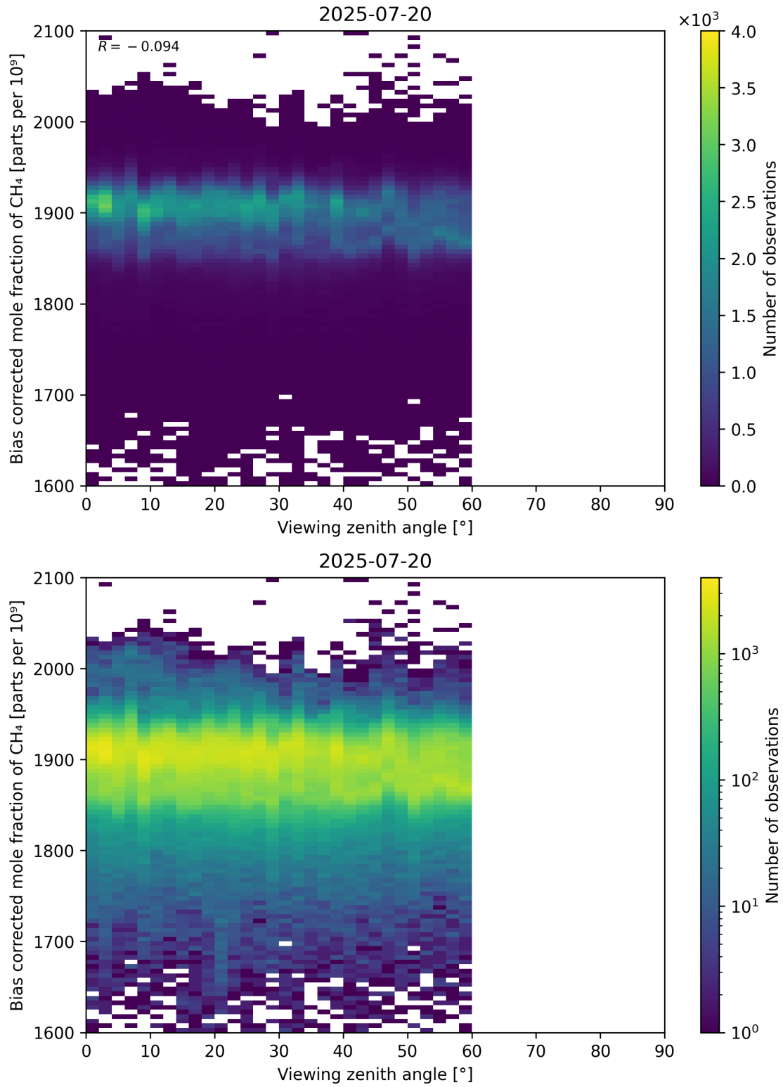
Figure 111: Scatter density plot of “Viewing zenith angle” against “Bias corrected mole fraction of CH 4 ” for 2025-07-19 to 2025-07-21.
