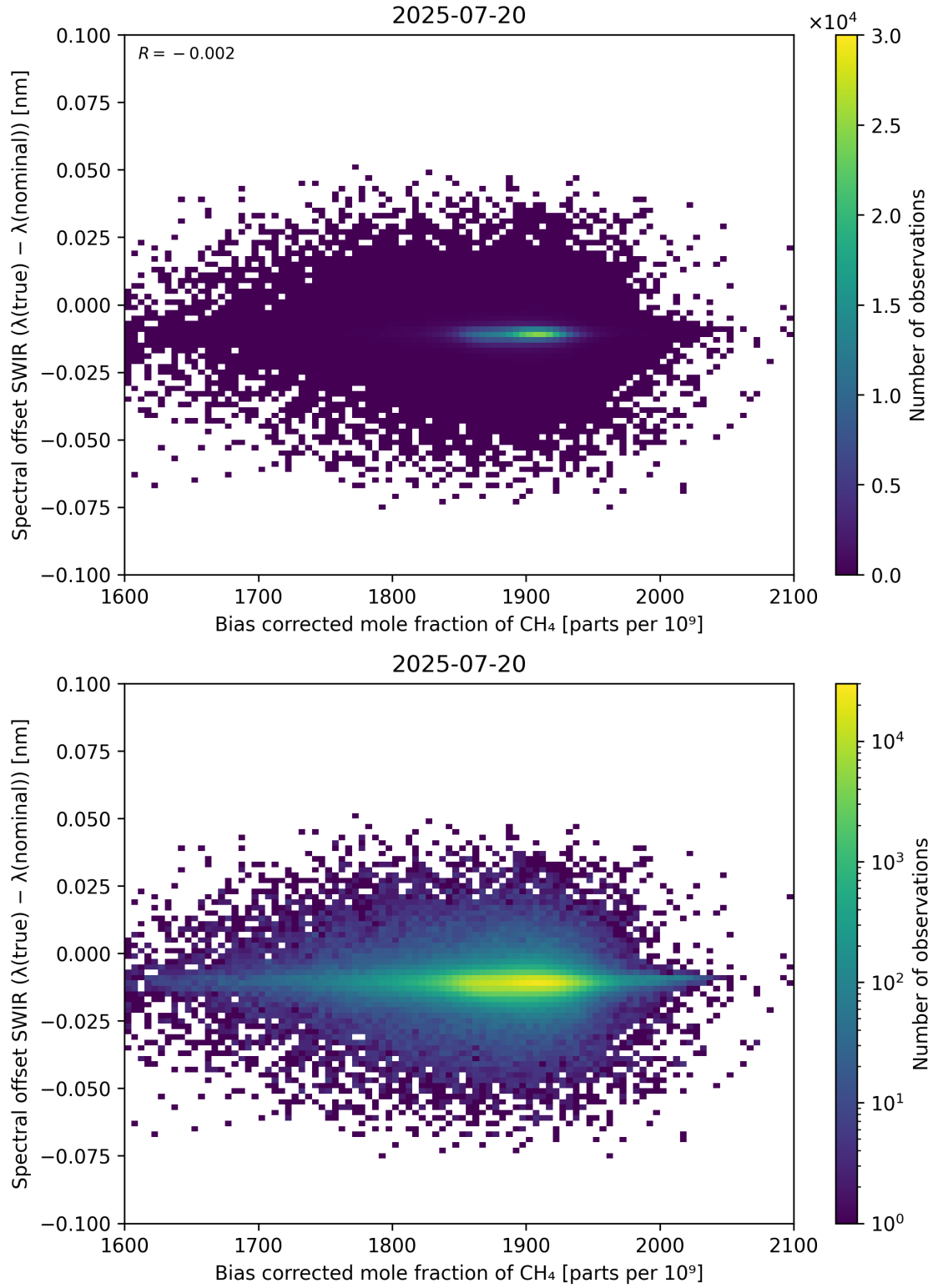
Figure 69: Scatter density plot of “Bias corrected mole fraction of \text{CH}_4 ” against “Spectral offset SWIR ( \lambda_{\text{true}} - \lambda_{\text{nominal}} )” for 2025-07-19 to 2025-07-21.
