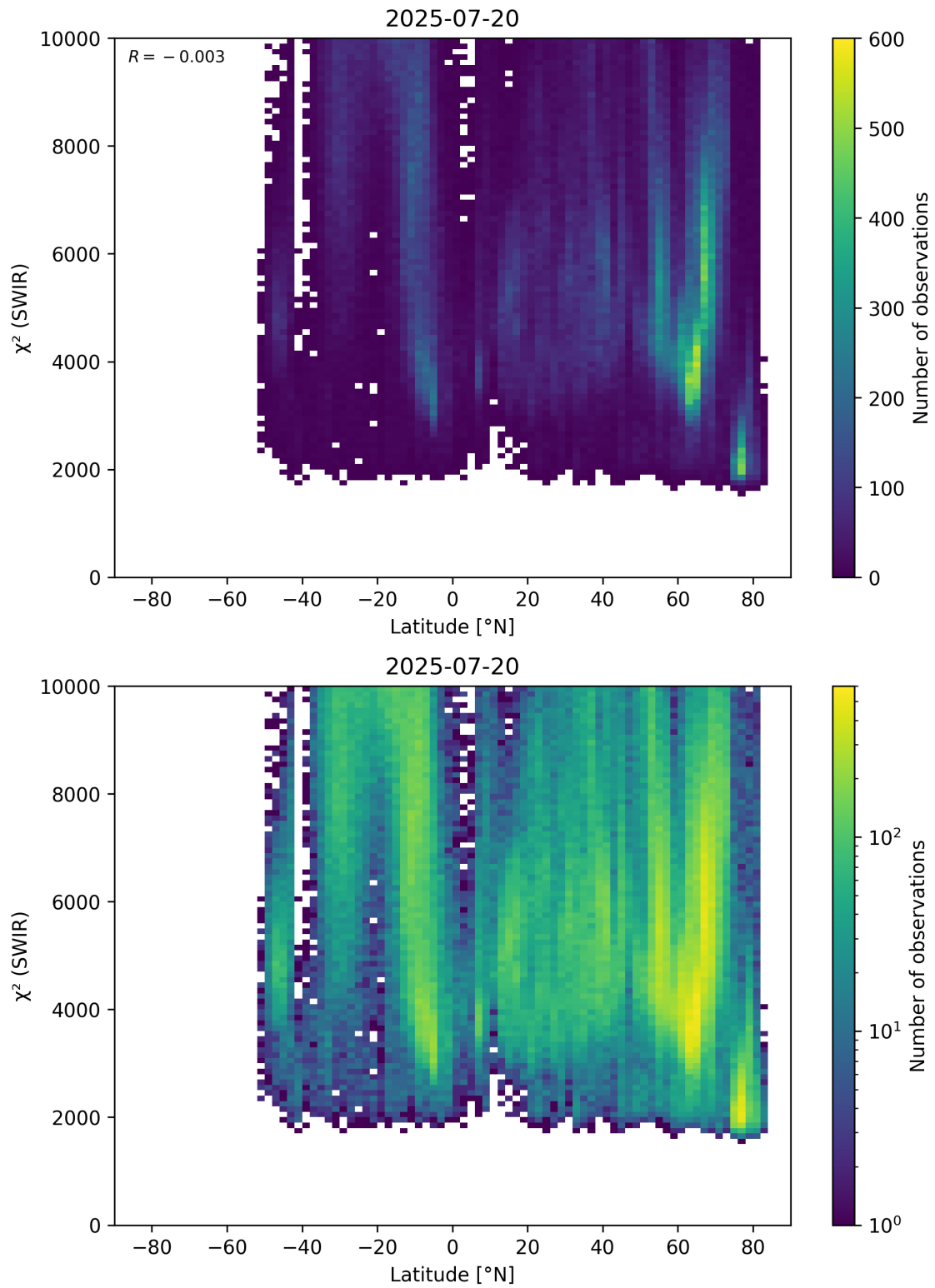
Figure 54: Scatter density plot of “Latitude” against “ \chi^2 (SWIR)” for 2025-07-19 to 2025-07-21.
