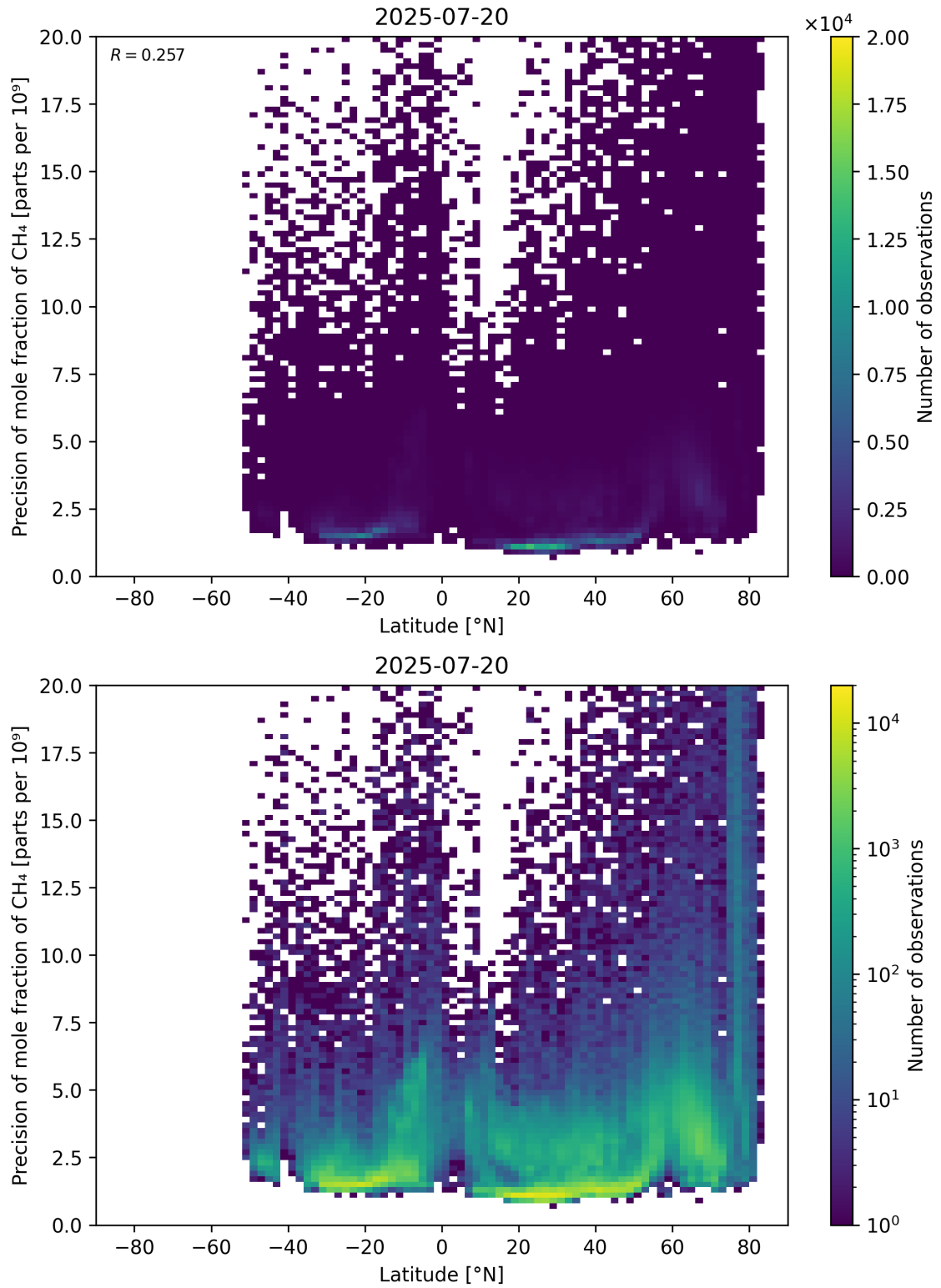
Figure 59: Scatter density plot of “Latitude” against “Precision of mole fraction of \text{CH}_4 ” for 2025-07-19 to 2025-07-21.
