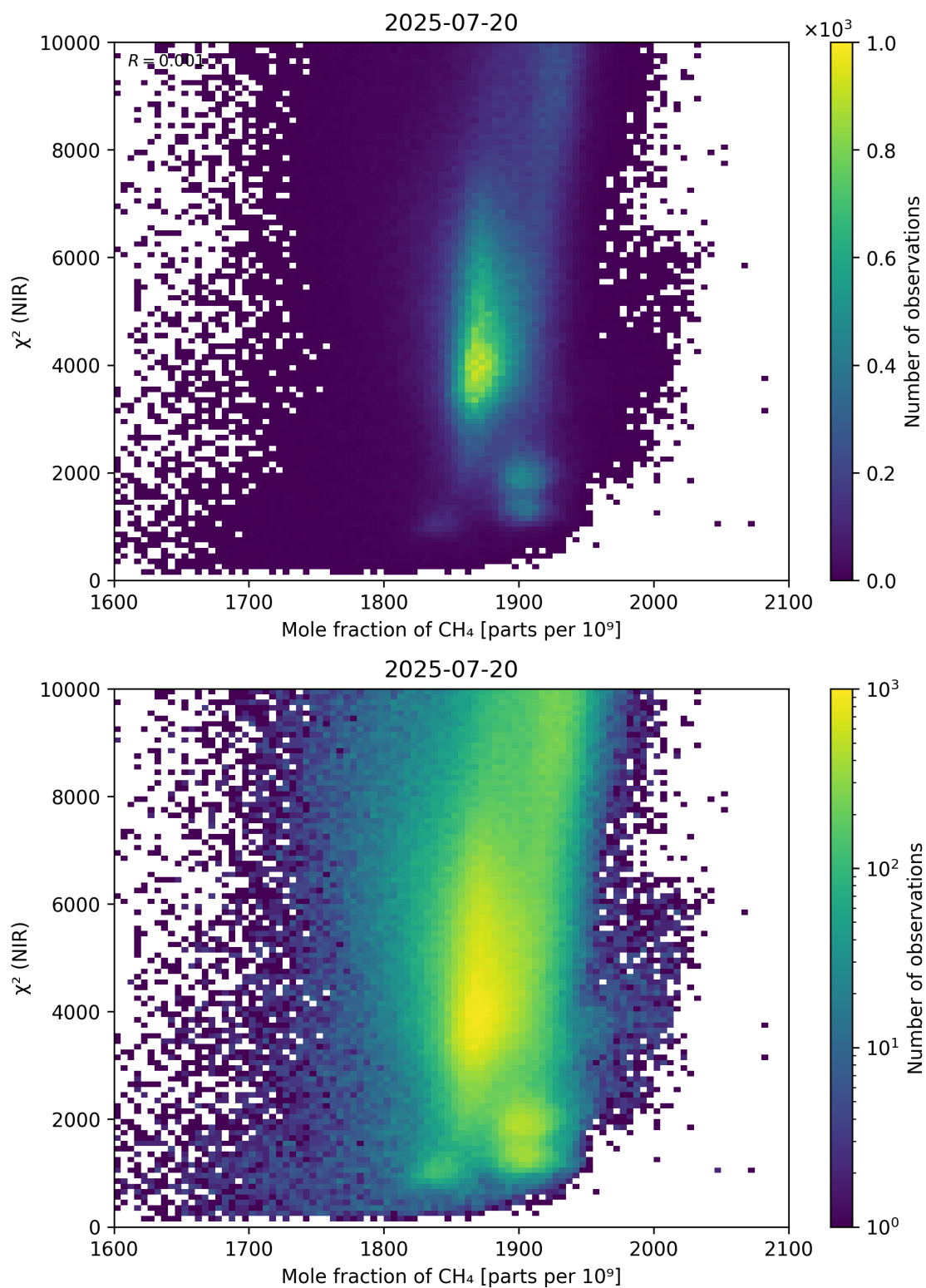
Figure 70: Scatter density plot of “Mole fraction of CH 4 ” against “ \chi^2 (NIR)” for 2025-07-19 to 2025-07-21.
