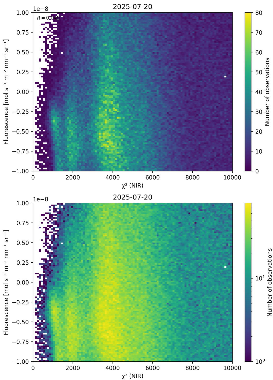
Figure 45: Scatter density plot of “ \chi^2 (NIR)” against “Fluorescence” for 2025-07-19 to 2025-07-21.
