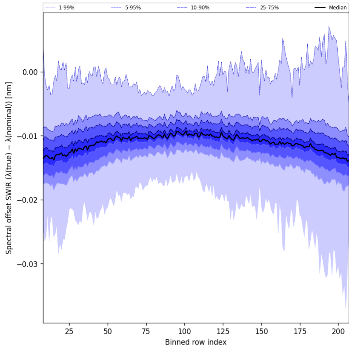
Figure 38: Along track statistics of “Spectral offset SWIR ( \lambda_{\text{true}} - \lambda_{\text{nominal}} )” for 2025-07-19 to 2025-07-21
