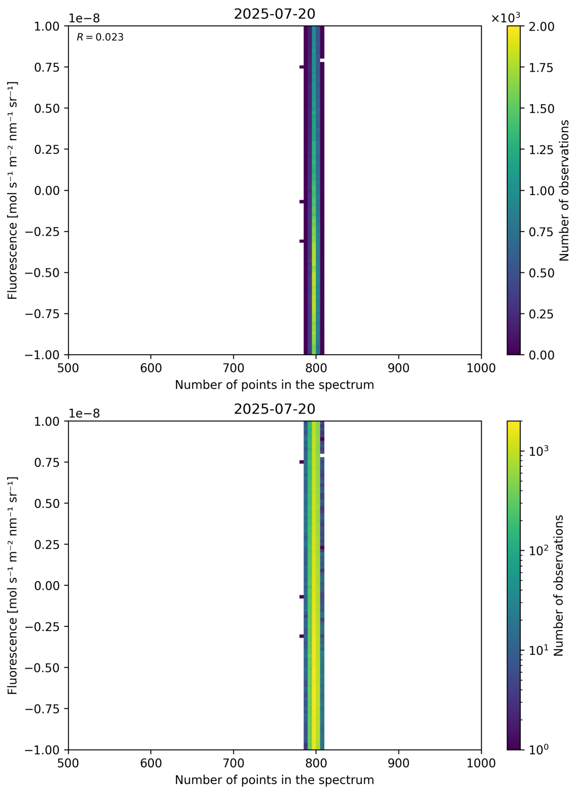
Figure 91: Scatter density plot of “Number of points in the spectrum” against “Fluorescence” for 2025-07-19 to 2025-07-21.
