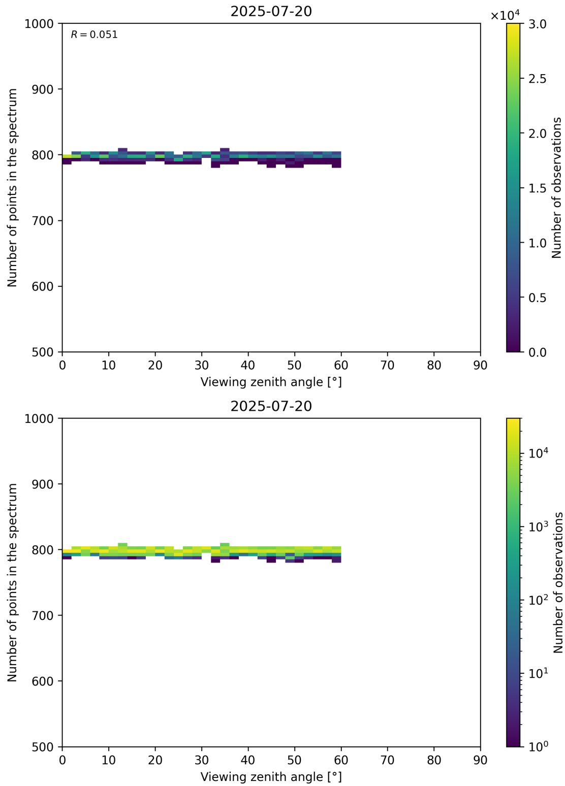
Figure 114: Scatter density plot of “Viewing zenith angle” against “Number of points in the spectrum” for 2025-07-19 to 2025-07-21.
