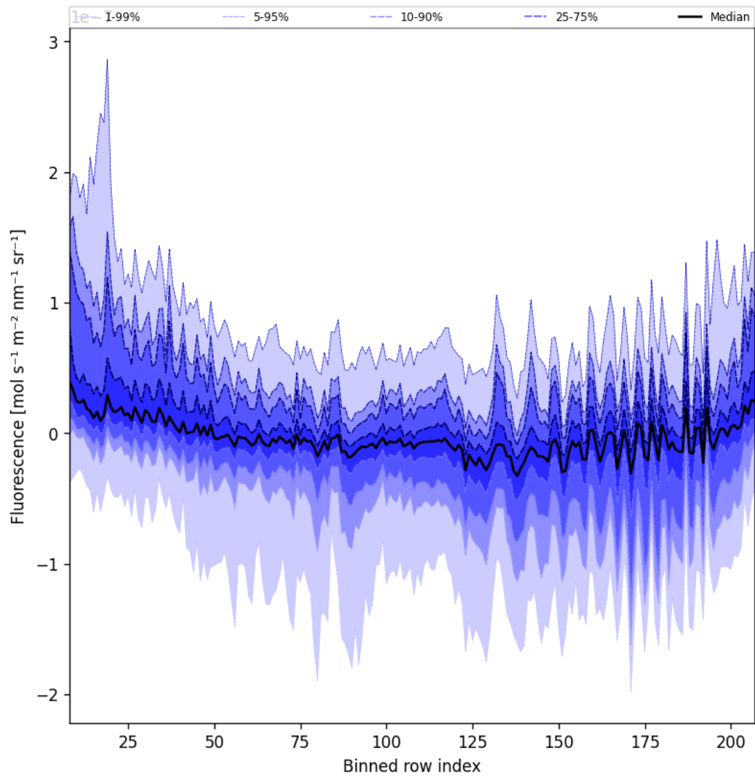
Figure 43: Along track statistics of “Fluorescence” for 2025-07-19 to 2025-07-21
