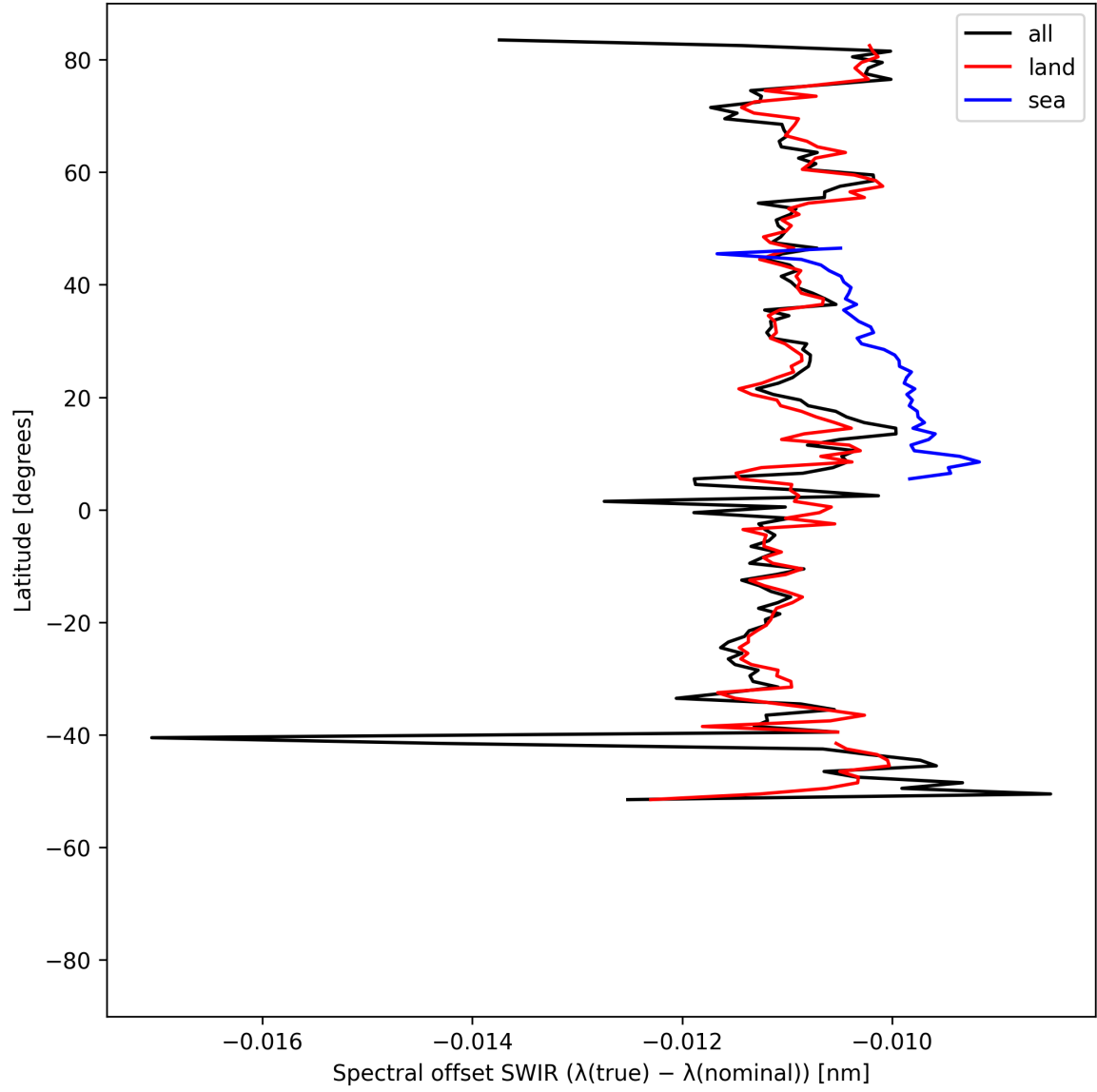
Figure 16: Zonal average of “Spectral offset SWIR ( \lambda_{\text{true}} - \lambda_{\text{nominal}} )” for 2025-07-19 to 2025-07-21.
