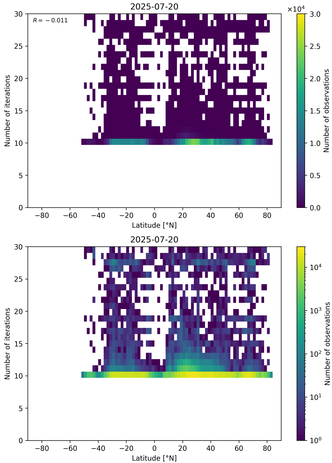
Figure 60: Scatter density plot of “Latitude” against “Number of iterations” for 2025-07-19 to 2025-07-21.
