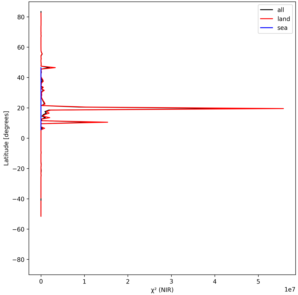
Figure 18: Zonal average of “ \chi^2 (NIR)” for 2025-07-19 to 2025-07-21.
