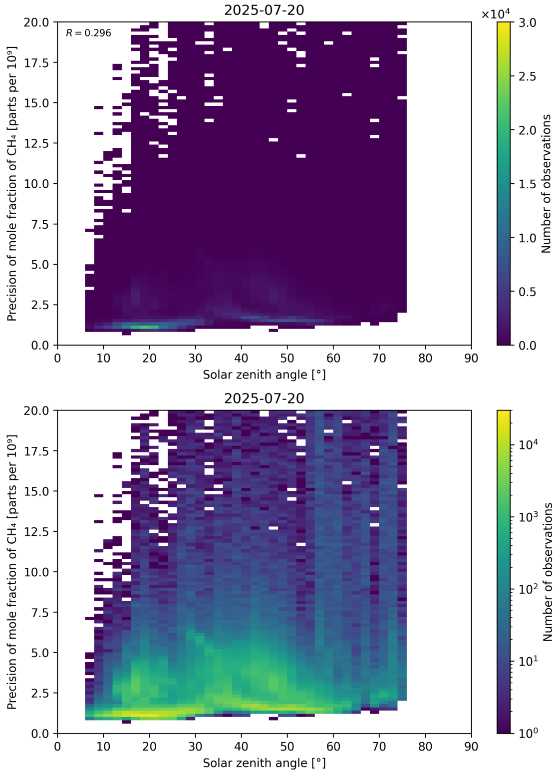
Figure 101: Scatter density plot of “Solar zenith angle” against “Precision of mole fraction of \text{CH}_4 ” for 2025-07-19 to 2025-07-21.
