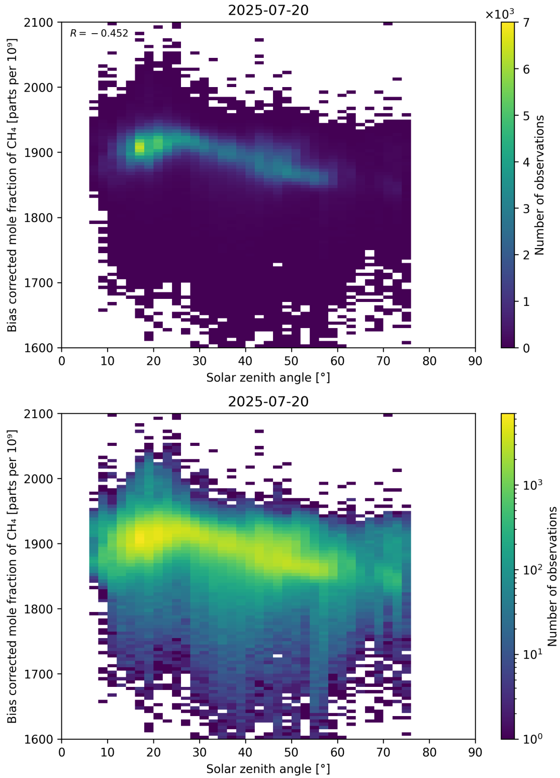
Figure 100: Scatter density plot of “Solar zenith angle” against “Bias corrected mole fraction of CH 4 ” for 2025-07-19 to 2025-07-21.
