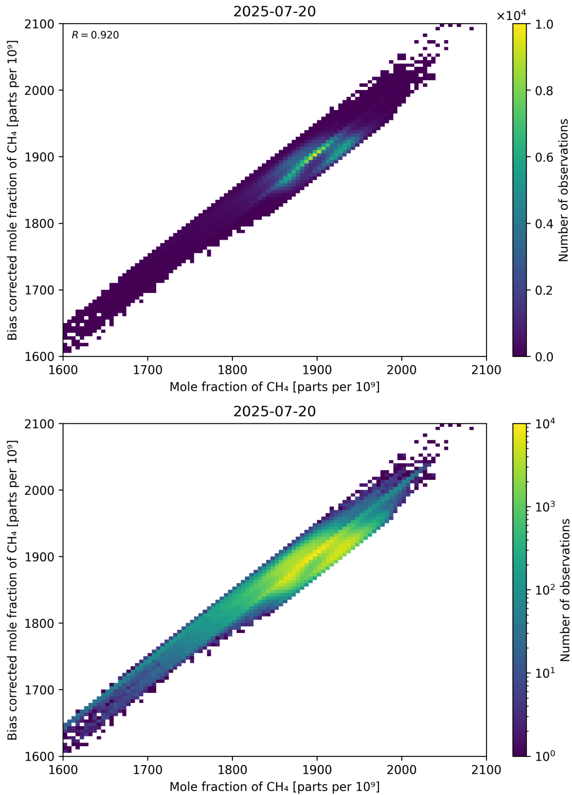
Figure 74: Scatter density plot of “Mole fraction of CH 4 ” against “Bias corrected mole fraction of CH 4 ” for 2025-07-19 to 2025-07-21.
