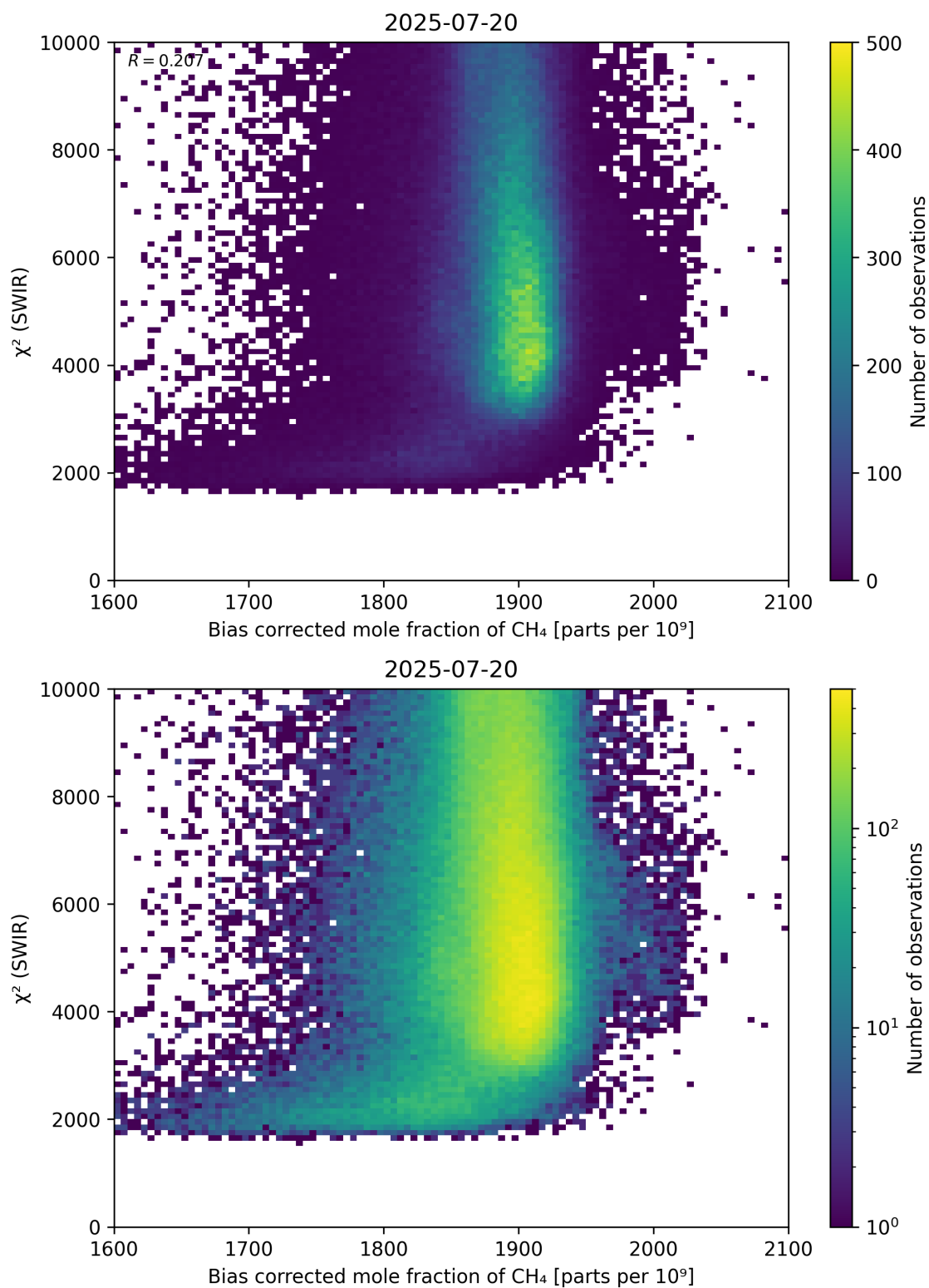
Figure 64: Scatter density plot of “Bias corrected mole fraction of \text{CH}_4 ” against “ \chi^2 (SWIR)” for 2025-07-19 to 2025-07-21.
