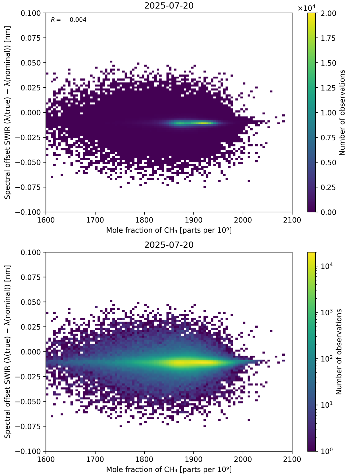
Figure 86: Scatter density plot of “Mole fraction of CH 4 ” against “Spectral offset SWIR ( \lambda_{\text{true}} - \lambda_{\text{nominal}} )” for 2025-07-19 to 2025-07-21.
