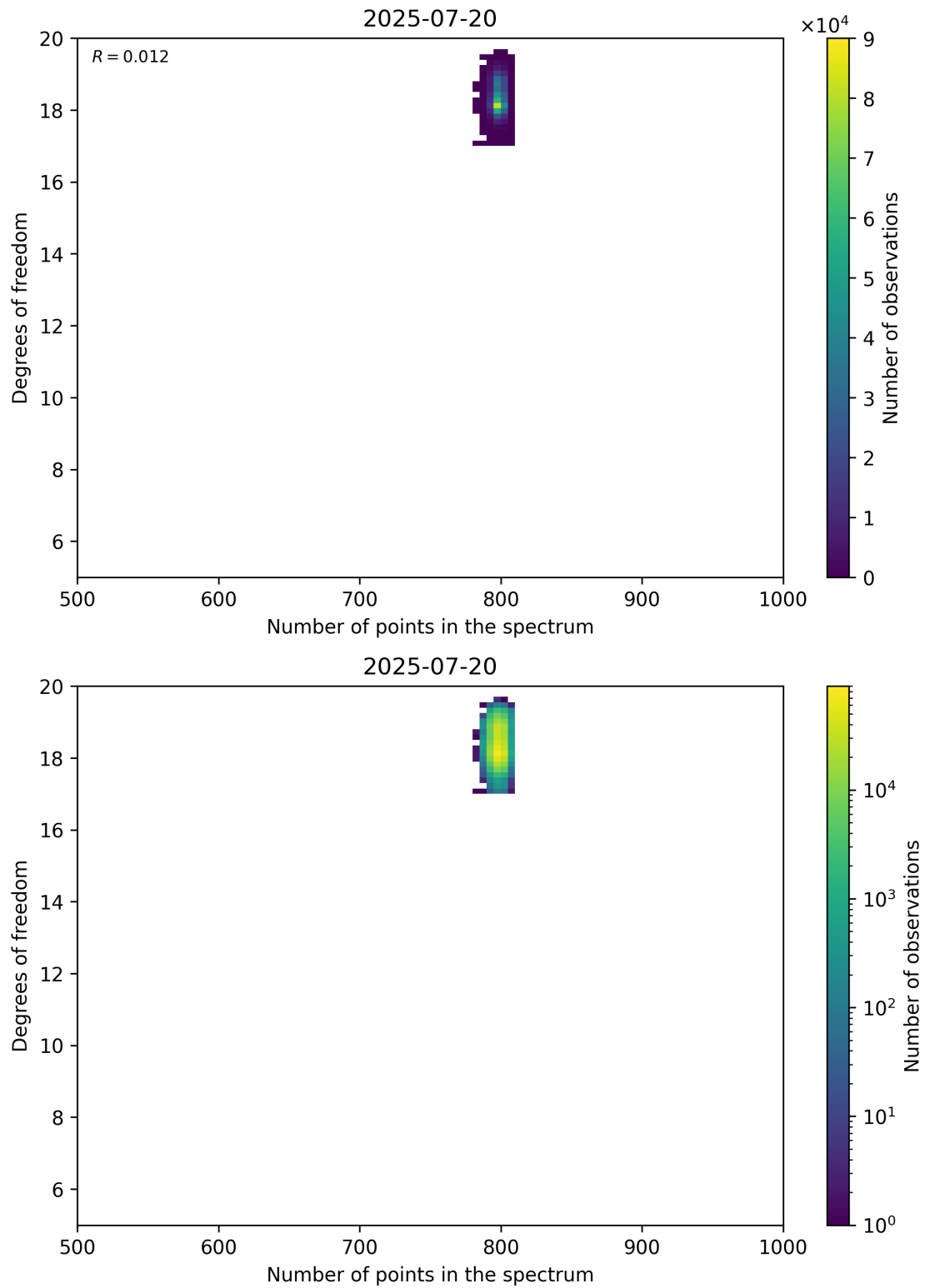
Figure 90: Scatter density plot of “Number of points in the spectrum” against “Degrees of freedom” for 2025-07-19 to 2025-07-21.
