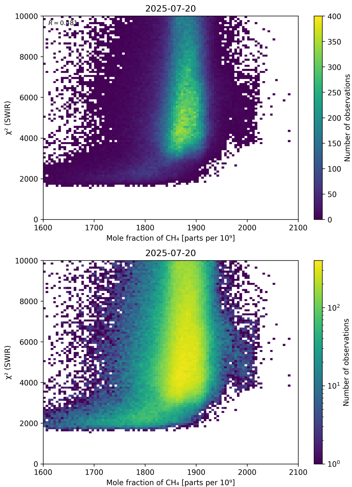
Figure 71: Scatter density plot of “Mole fraction of \text{CH}_4 ” against “ \chi^2 (SWIR)” for 2025-07-19 to 2025-07-21.
