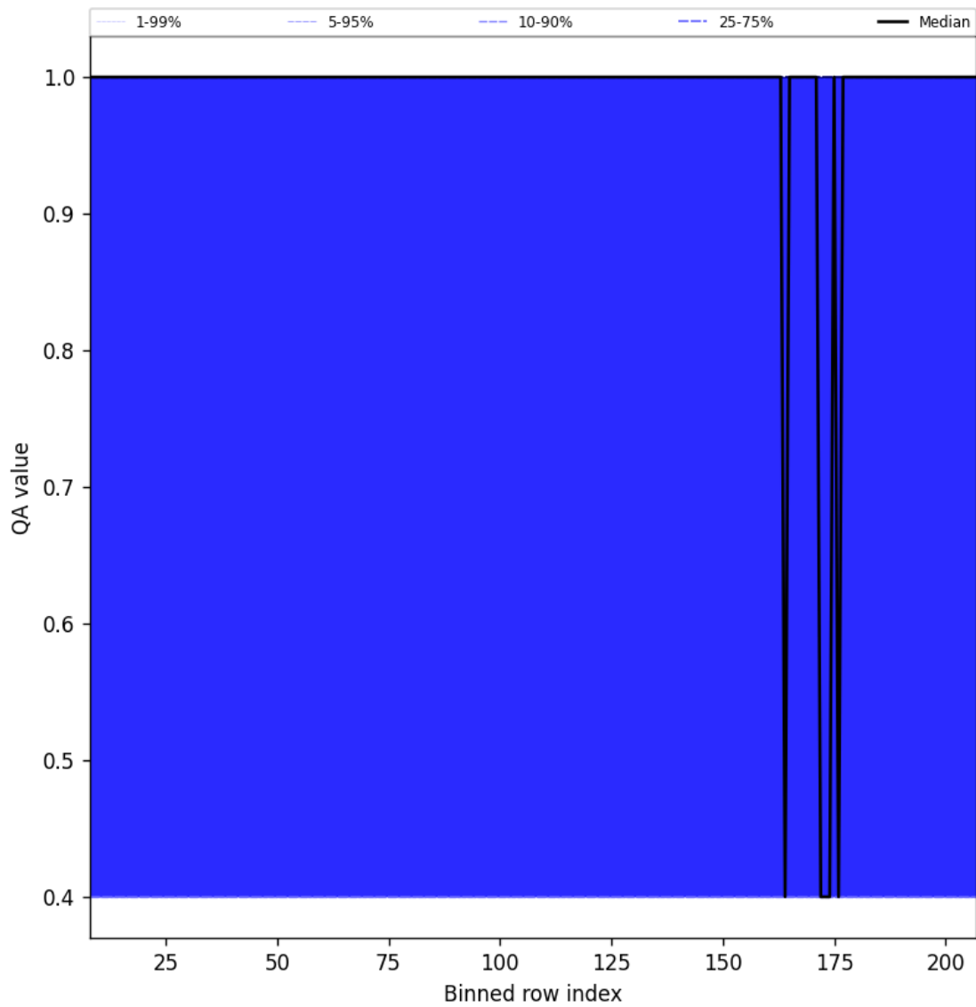
Figure 33: Along track statistics of “QA value” for 2025-07-19 to 2025-07-21
