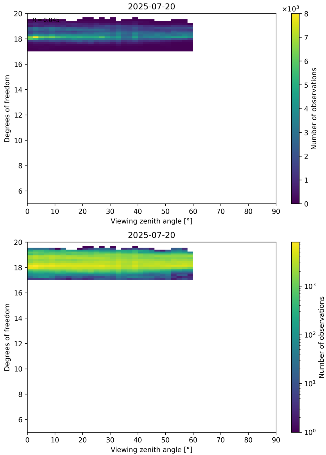
Figure 107: Scatter density plot of “Viewing zenith angle” against “Degrees of freedom” for 2025-07-19 to 2025-07-21.
