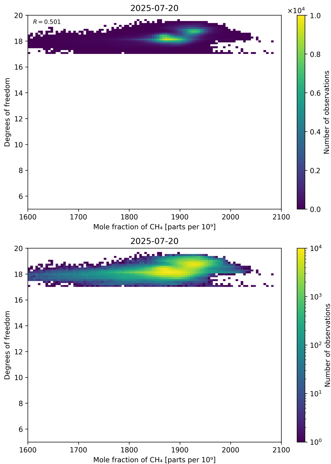
Figure 72: Scatter density plot of “Mole fraction of CH 4 ” against “Degrees of freedom” for 2025-07-19 to 2025-07-21.
