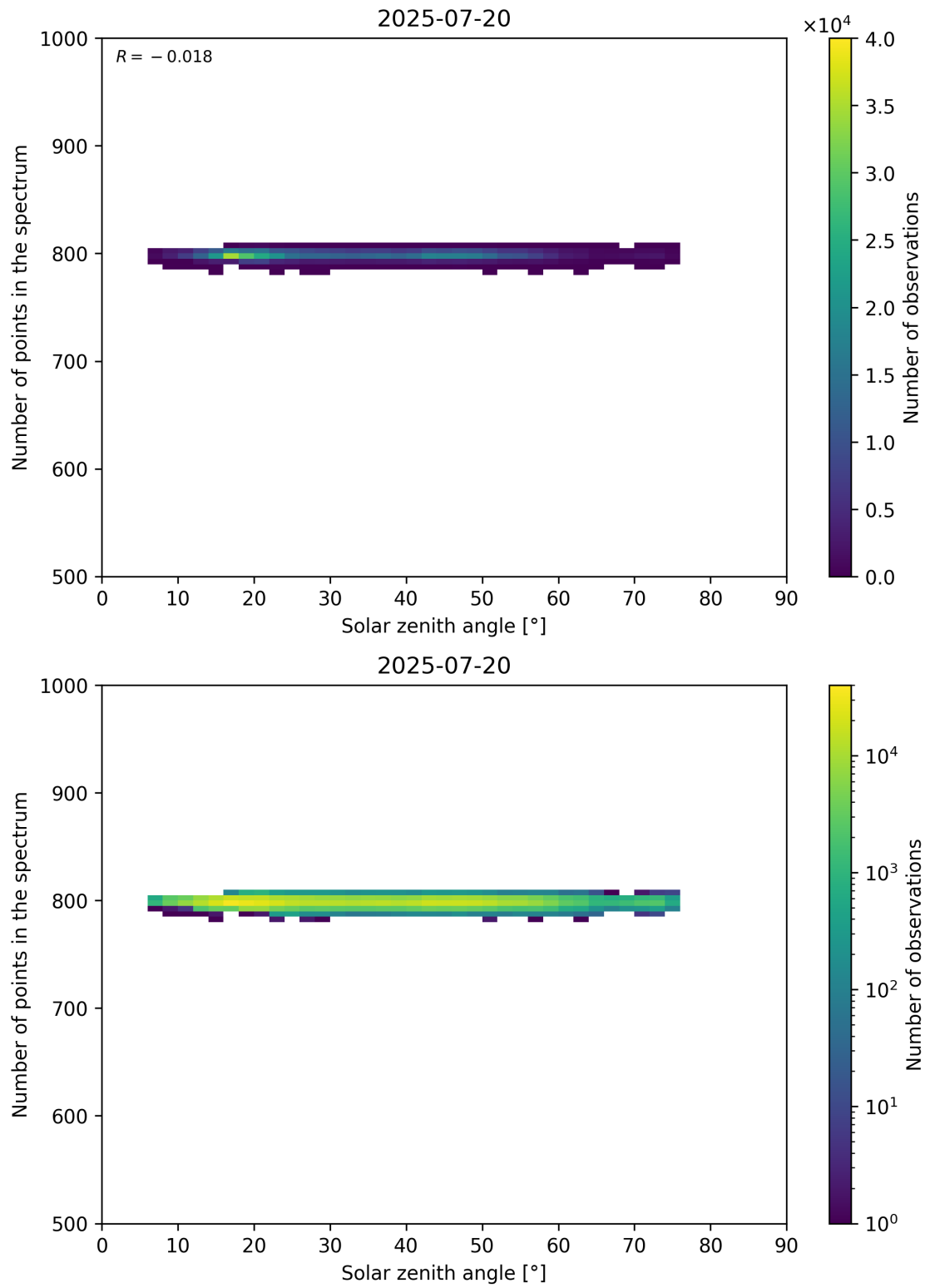
Figure 103: Scatter density plot of “Solar zenith angle” against “Number of points in the spectrum” for 2025-07-19 to 2025-07-21.
