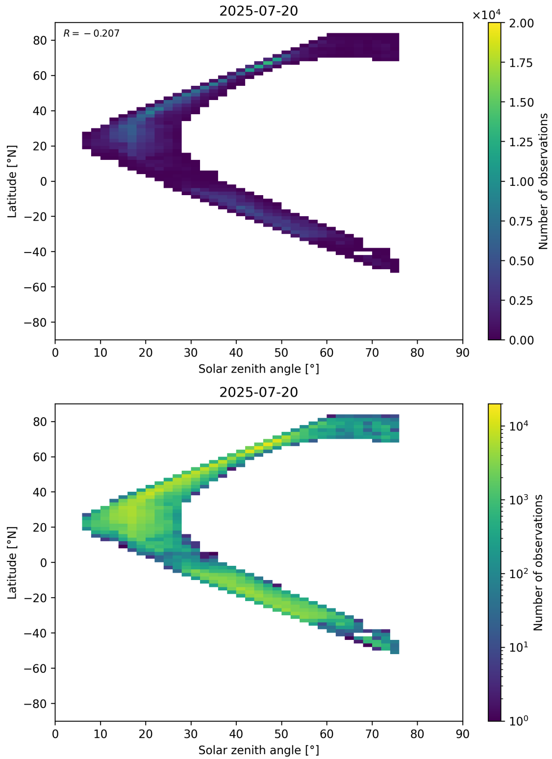
Figure 98: Scatter density plot of “Solar zenith angle” against “Latitude” for 2025-07-19 to 2025-07-21.
