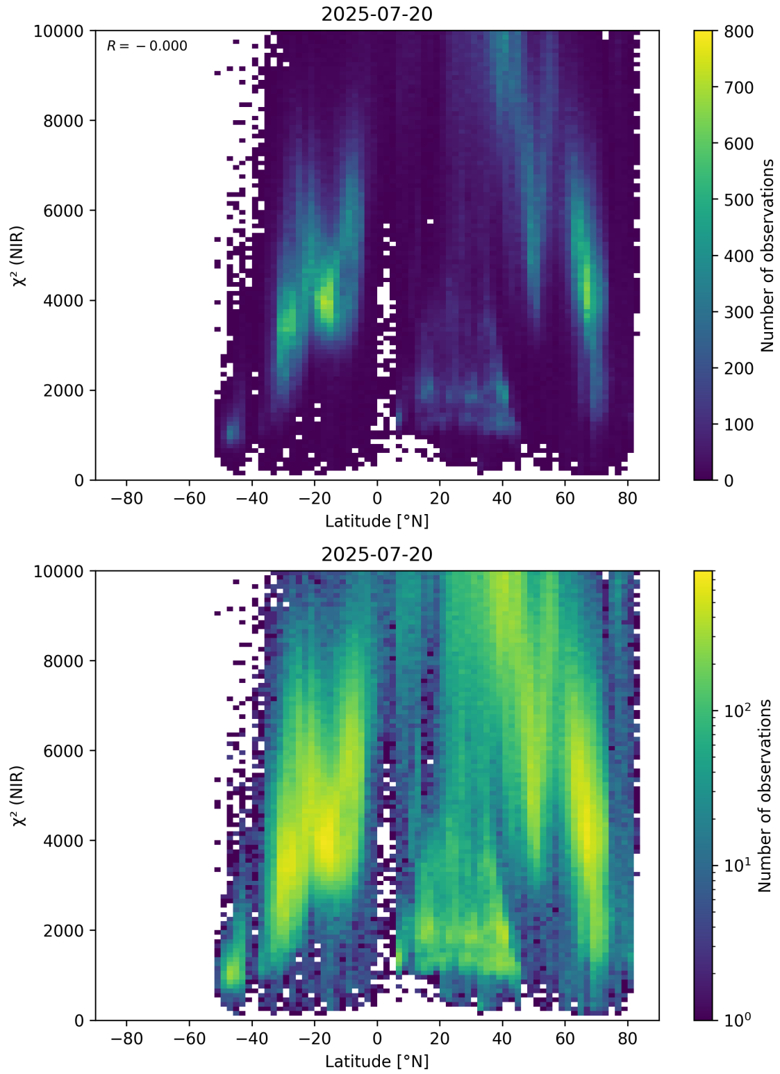
Figure 53: Scatter density plot of “Latitude” against “ \chi^2 (NIR)” for 2025-07-19 to 2025-07-21.
