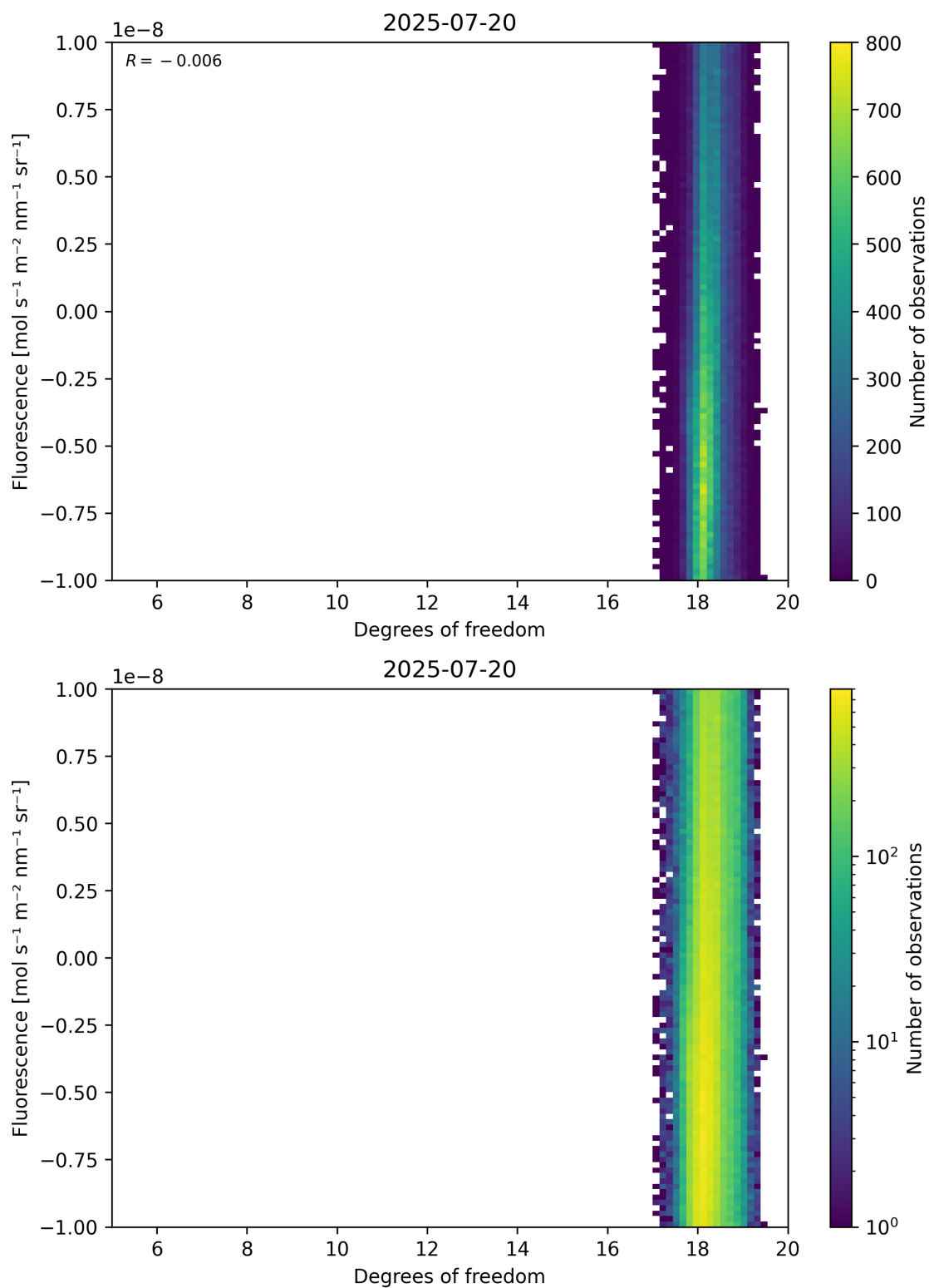
Figure 51: Scatter density plot of “Degrees of freedom” against “Fluorescence” for 2025-07-19 to 2025-07-21.
