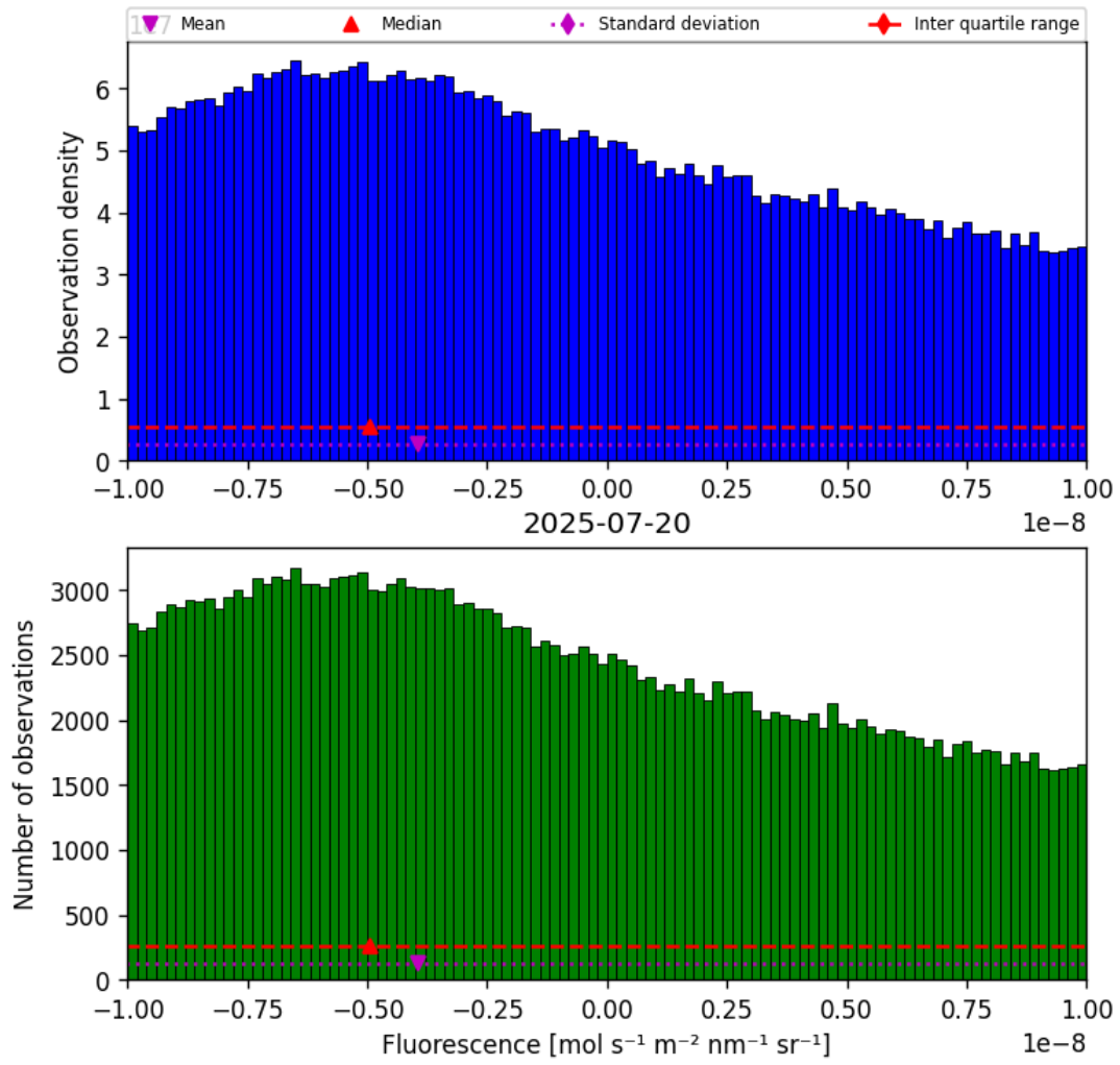
Figure 32: Histogram of “Fluorescence” for 2025-07-19 to 2025-07-21
