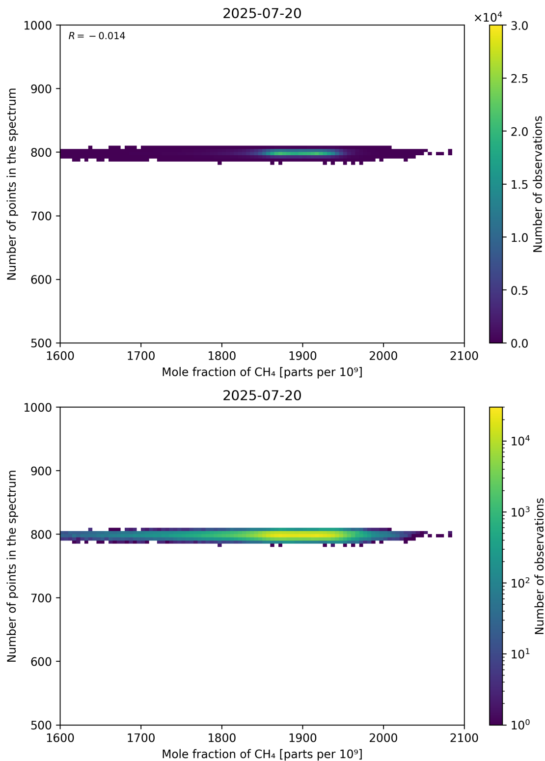
Figure 77: Scatter density plot of “Mole fraction of CH 4 ” against “Number of points in the spectrum” for 2025-07-19 to 2025-07-21.
