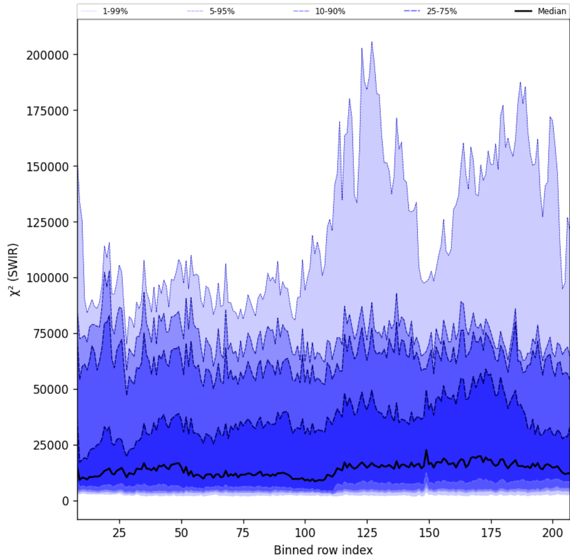
Figure 39: Along track statistics of “ \chi^2 (SWIR)” for 2025-07-19 to 2025-07-21
