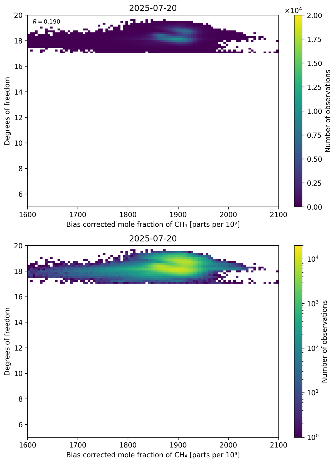
Figure 65: Scatter density plot of “Bias corrected mole fraction of \text{CH}_4 ” against “Degrees of freedom” for 2025-07-19 to 2025-07-21.
