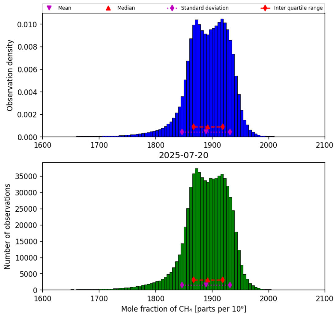
Figure 23: Histogram of “Mole fraction of CH 4 ” for 2025-07-19 to 2025-07-21
