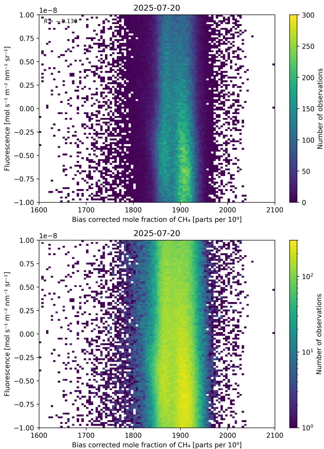
Figure 66: Scatter density plot of “Bias corrected mole fraction of \text{CH}_4 ” against “Fluorescence” for 2025-07-19 to 2025-07-21.
