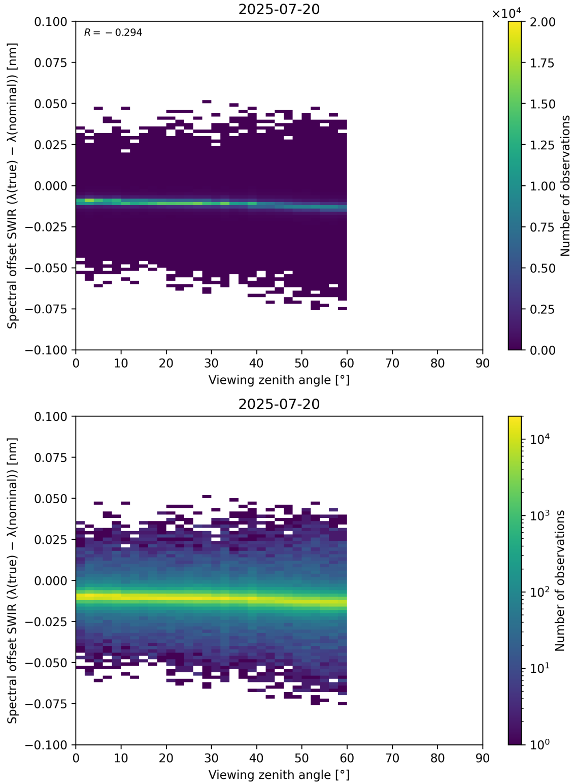
Figure 116: Scatter density plot of “Viewing zenith angle” against “Spectral offset SWIR ( \lambda_{\text{true}} - \lambda_{\text{nominal}} )” for 2025-07-19 to 2025-07-21.
