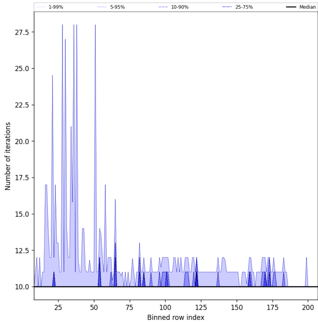
Figure 42: Along track statistics of “Number of iterations” for 2025-07-19 to 2025-07-21
