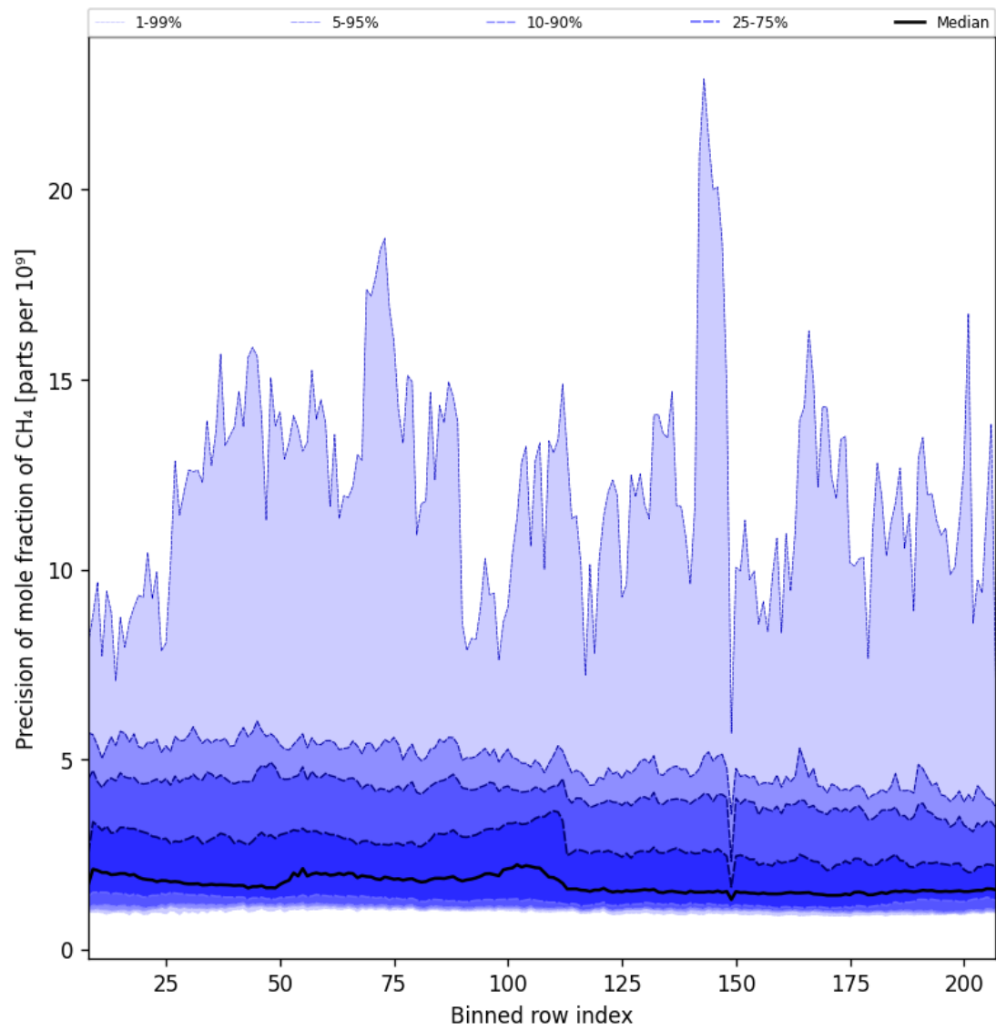
Figure 35: Along track statistics of “Precision of mole fraction of CH 4 ” for 2025-07-19 to 2025-07-21
