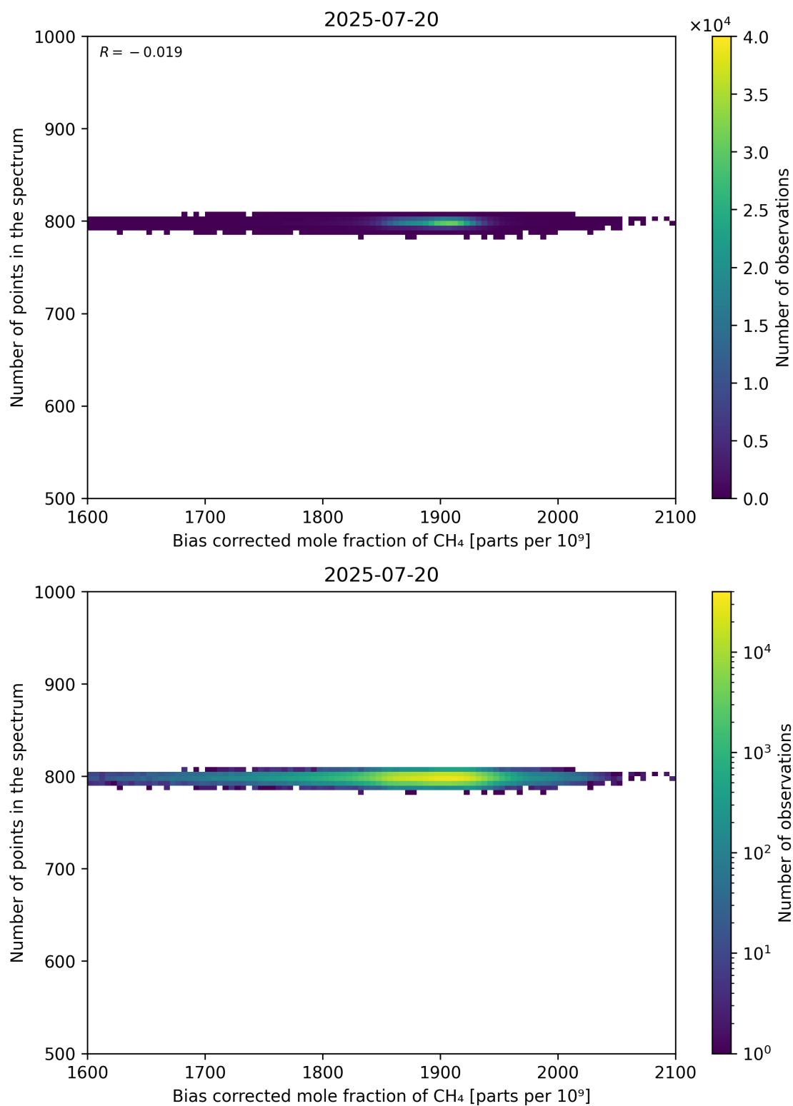
Figure 68: Scatter density plot of “Bias corrected mole fraction of CH 4 ” against “Number of points in the spectrum” for 2025-07-19 to 2025-07-21.
