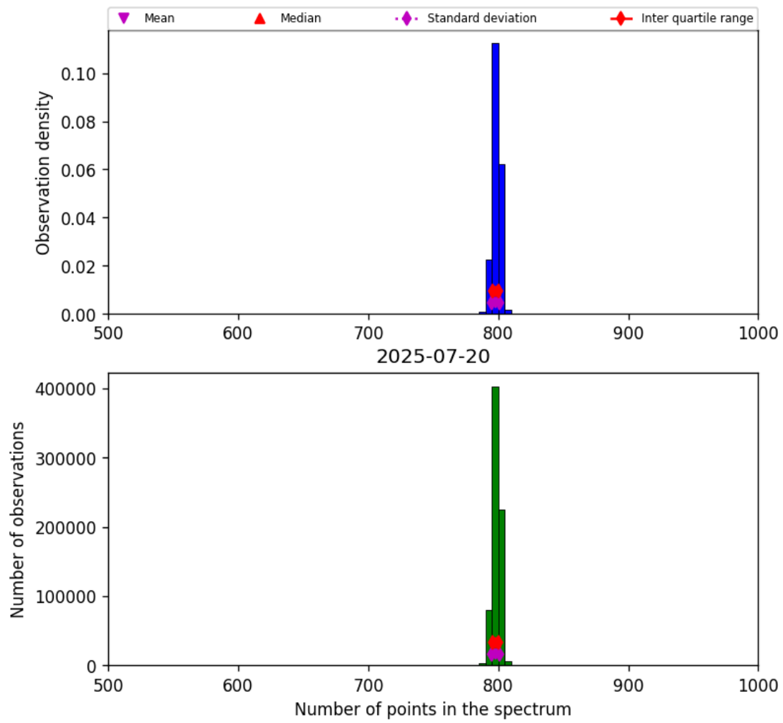
Figure 26: Histogram of “Number of points in the spectrum” for 2025-07-19 to 2025-07-21
