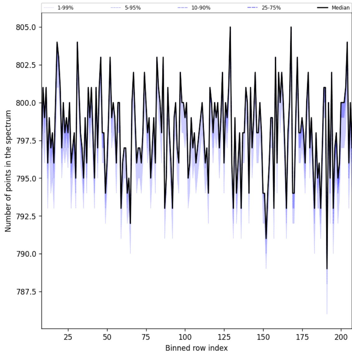
Figure 37: Along track statistics of “Number of points in the spectrum” for 2025-07-19 to 2025-07-21
