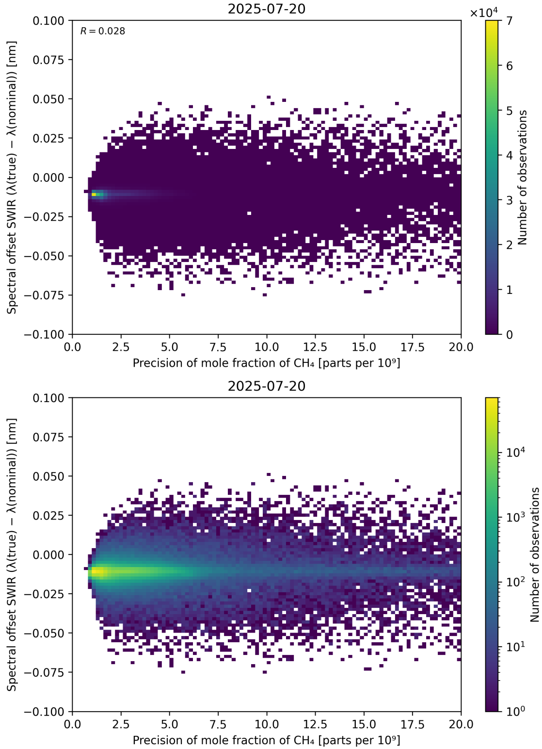
Figure 85: Scatter density plot of “Precision of mole fraction of \text{CH}_4 ” against “Spectral offset SWIR ( \lambda_{\text{true}} - \lambda_{\text{nominal}} )” for 2025-07-19 to 2025-07-21.
