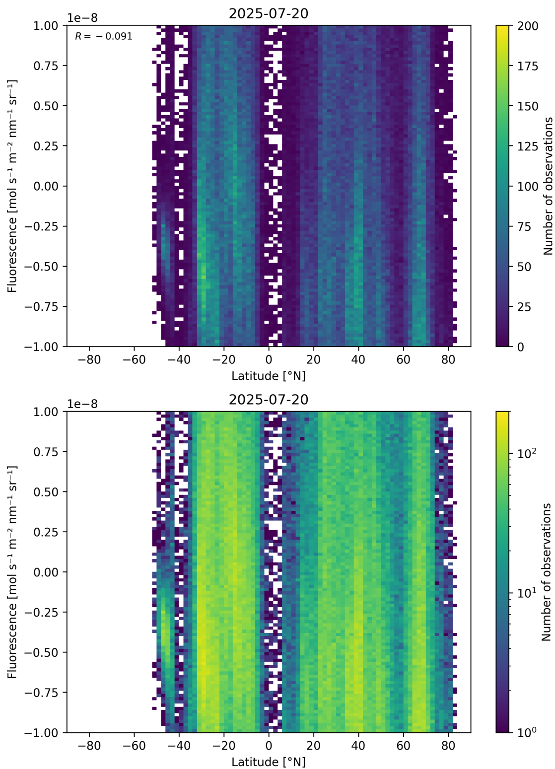
Figure 56: Scatter density plot of “Latitude” against “Fluorescence” for 2025-07-19 to 2025-07-21.
