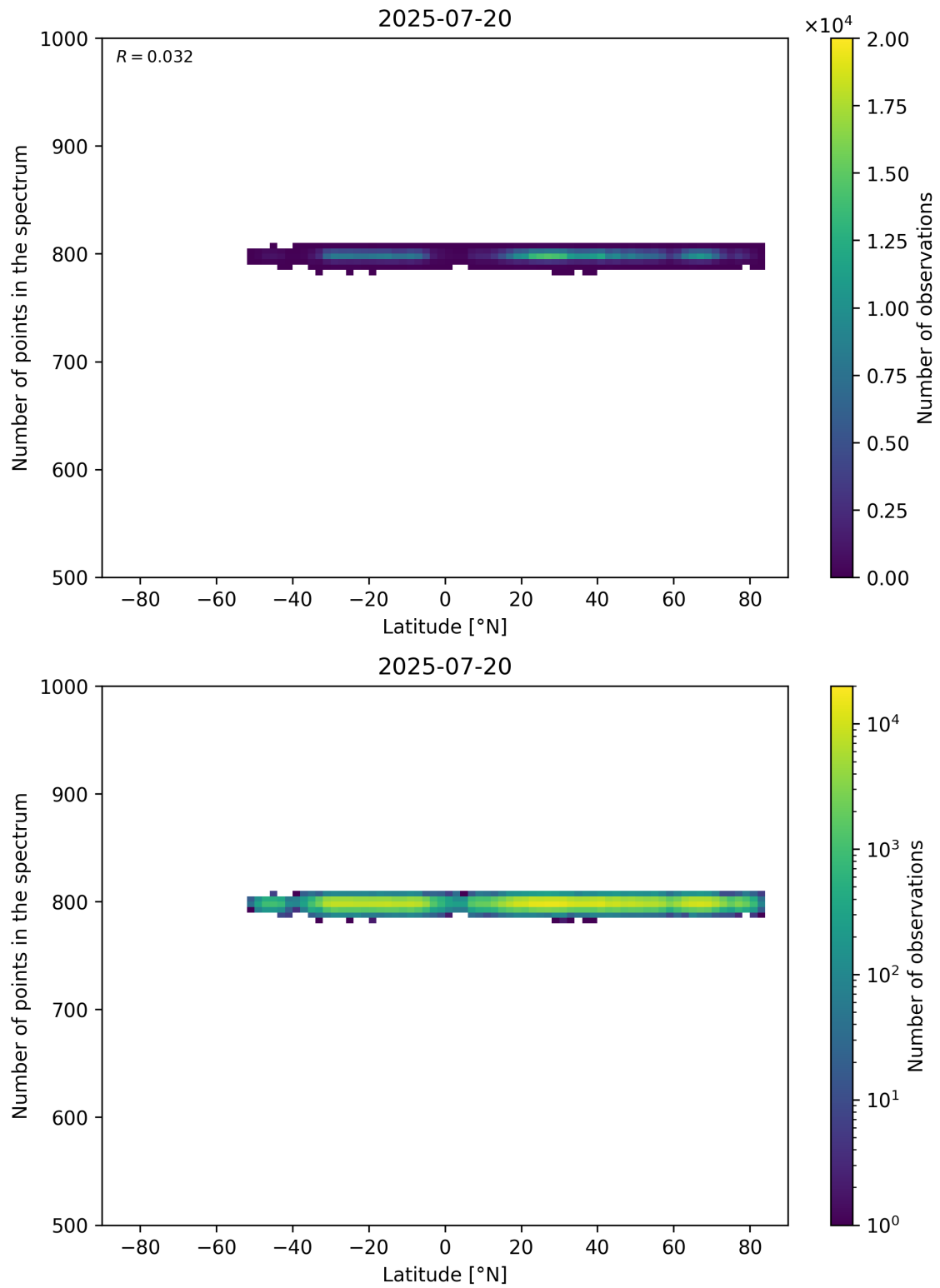
Figure 61: Scatter density plot of “Latitude” against “Number of points in the spectrum” for 2025-07-19 to 2025-07-21.
