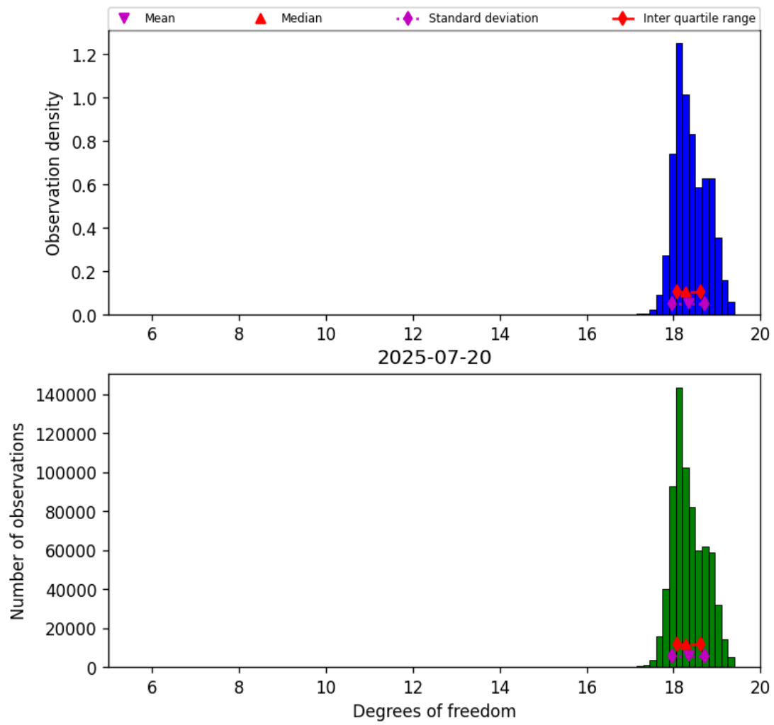
Figure 30: Histogram of “Degrees of freedom” for 2025-07-19 to 2025-07-21
