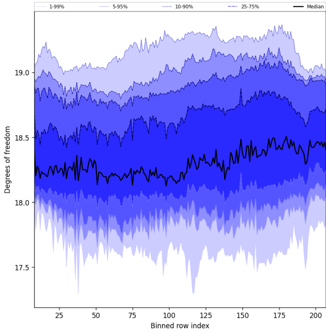
Figure 41: Along track statistics of “Degrees of freedom” for 2025-07-19 to 2025-07-21
