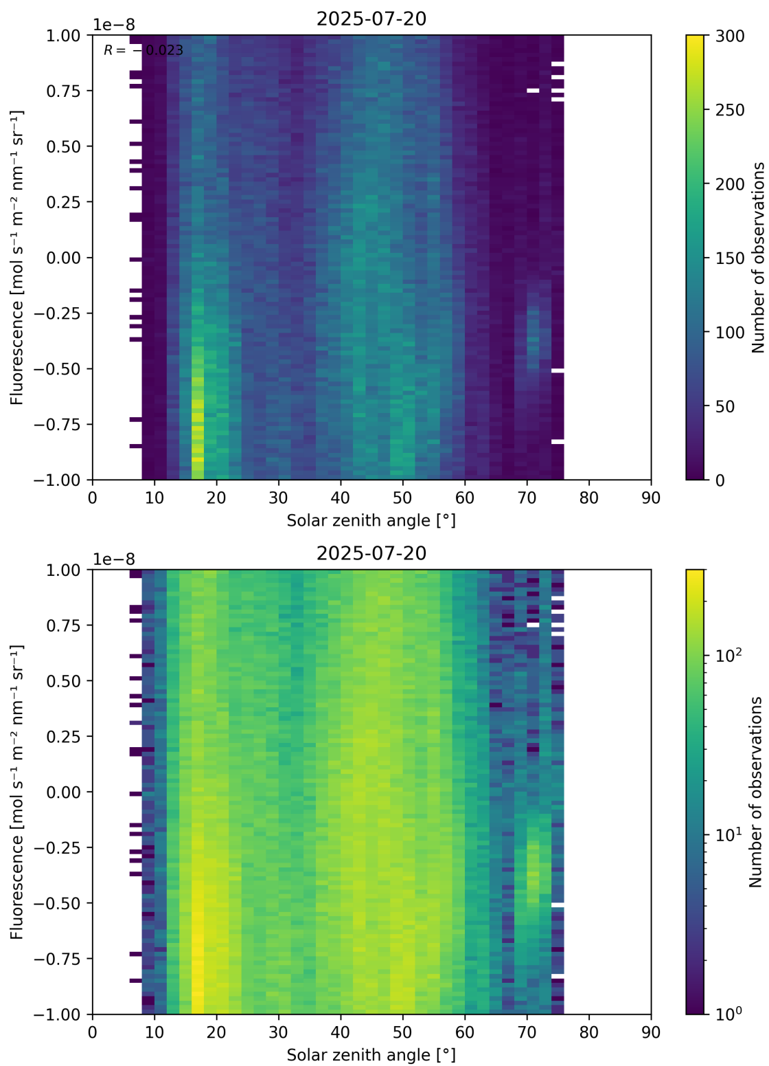
Figure 97: Scatter density plot of “Solar zenith angle” against “Fluorescence” for 2025-07-19 to 2025-07-21.
