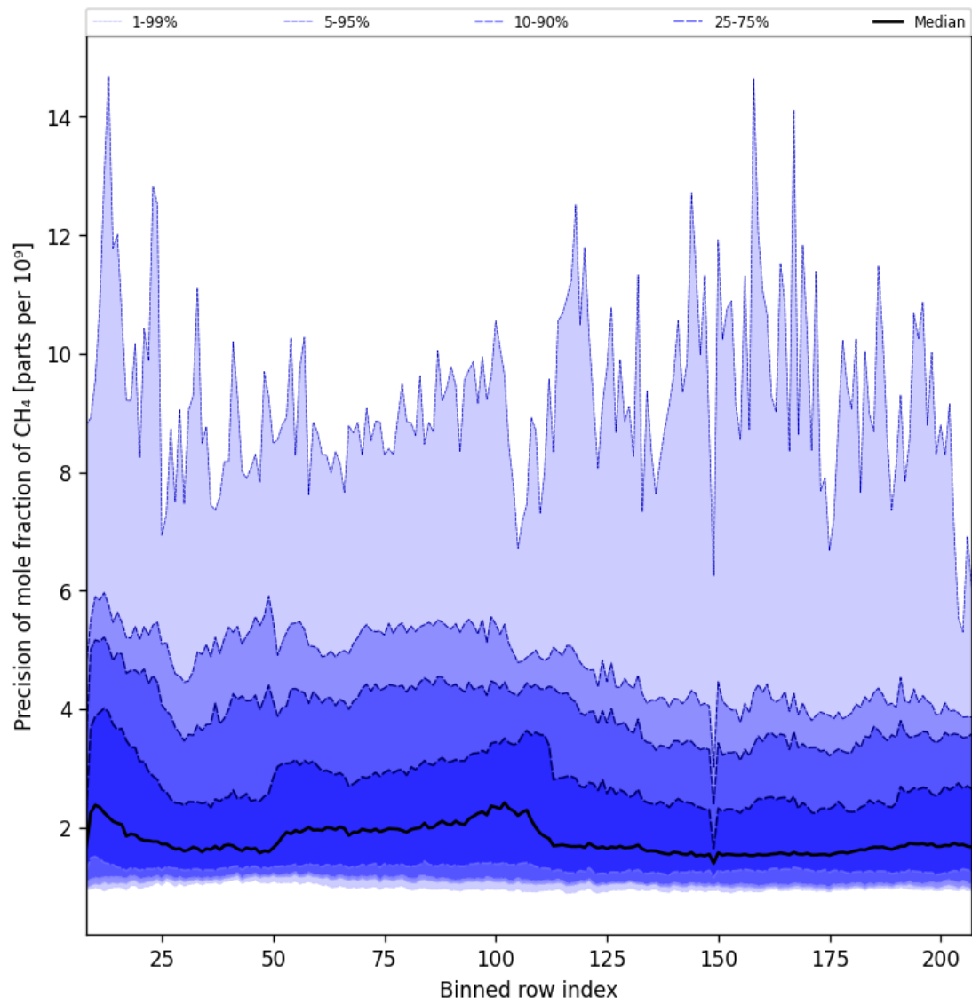
Figure 35: Along track statistics of “Precision of mole fraction of CH 4 ” for 2025-07-20 to 2025-07-22
