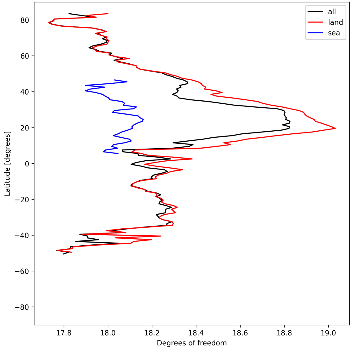
Figure 19: Zonal average of “Degrees of freedom” for 2025-07-20 to 2025-07-22.
