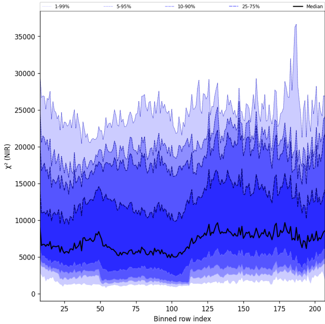
Figure 40: Along track statistics of “ \chi^2 (NIR)” for 2025-07-20 to 2025-07-22
