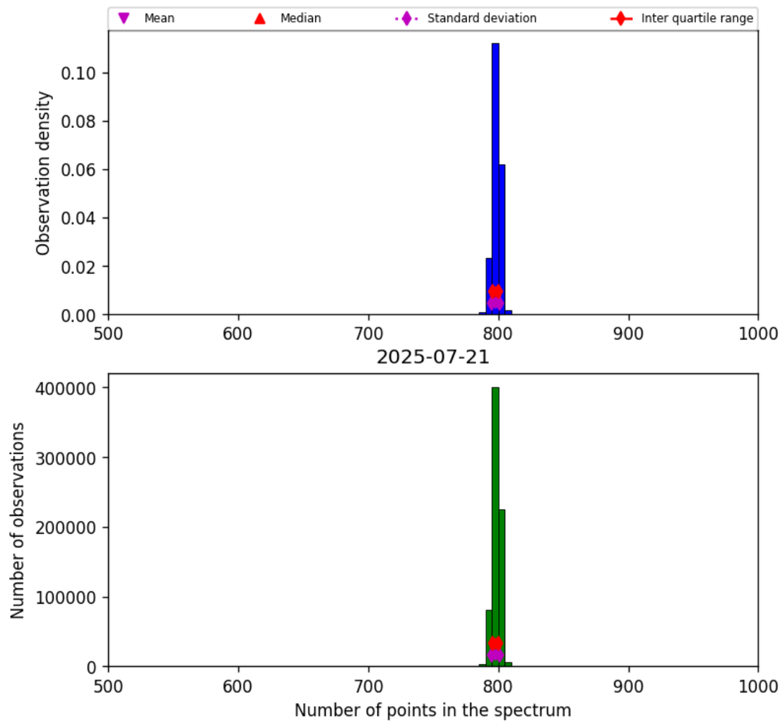
Figure 26: Histogram of “Number of points in the spectrum” for 2025-07-20 to 2025-07-22
