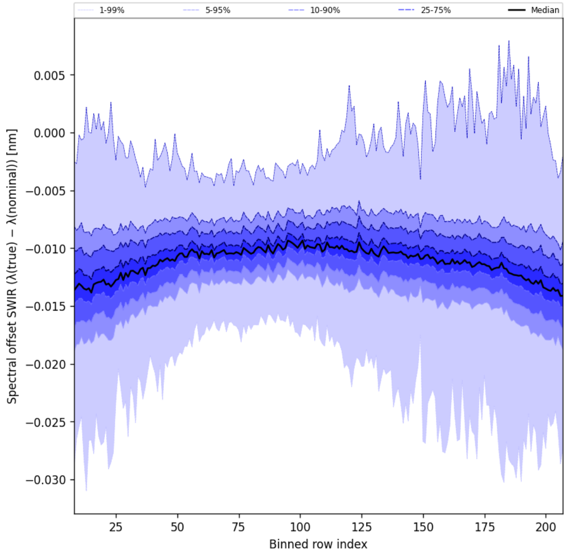
Figure 38: Along track statistics of “Spectral offset SWIR ( \lambda_{\text{true}} - \lambda_{\text{nominal}} )” for 2025-07-20 to 2025-07-22
