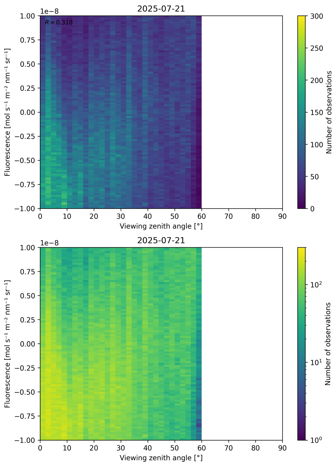
Figure 108: Scatter density plot of “Viewing zenith angle” against “Fluorescence” for 2025-07-20 to 2025-07-22.
