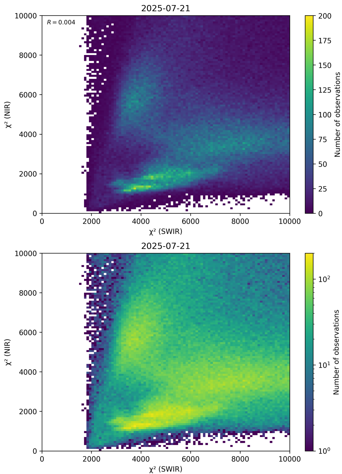
Figure 47: Scatter density plot of “ \chi^2 (SWIR)” against “ \chi^2 (NIR)” for 2025-07-20 to 2025-07-22.
