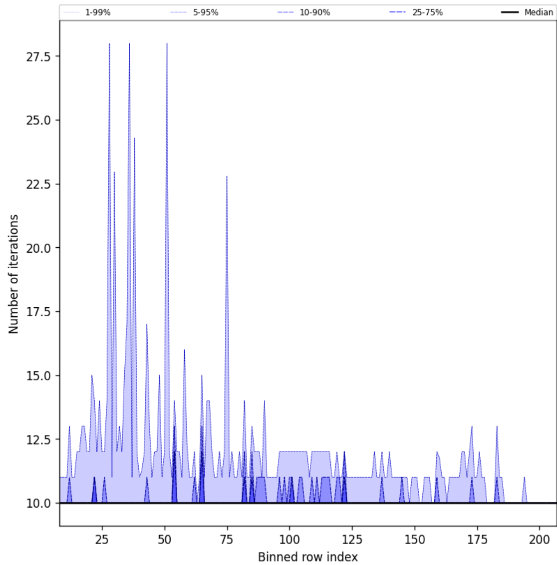
Figure 42: Along track statistics of “Number of iterations” for 2025-07-20 to 2025-07-22
