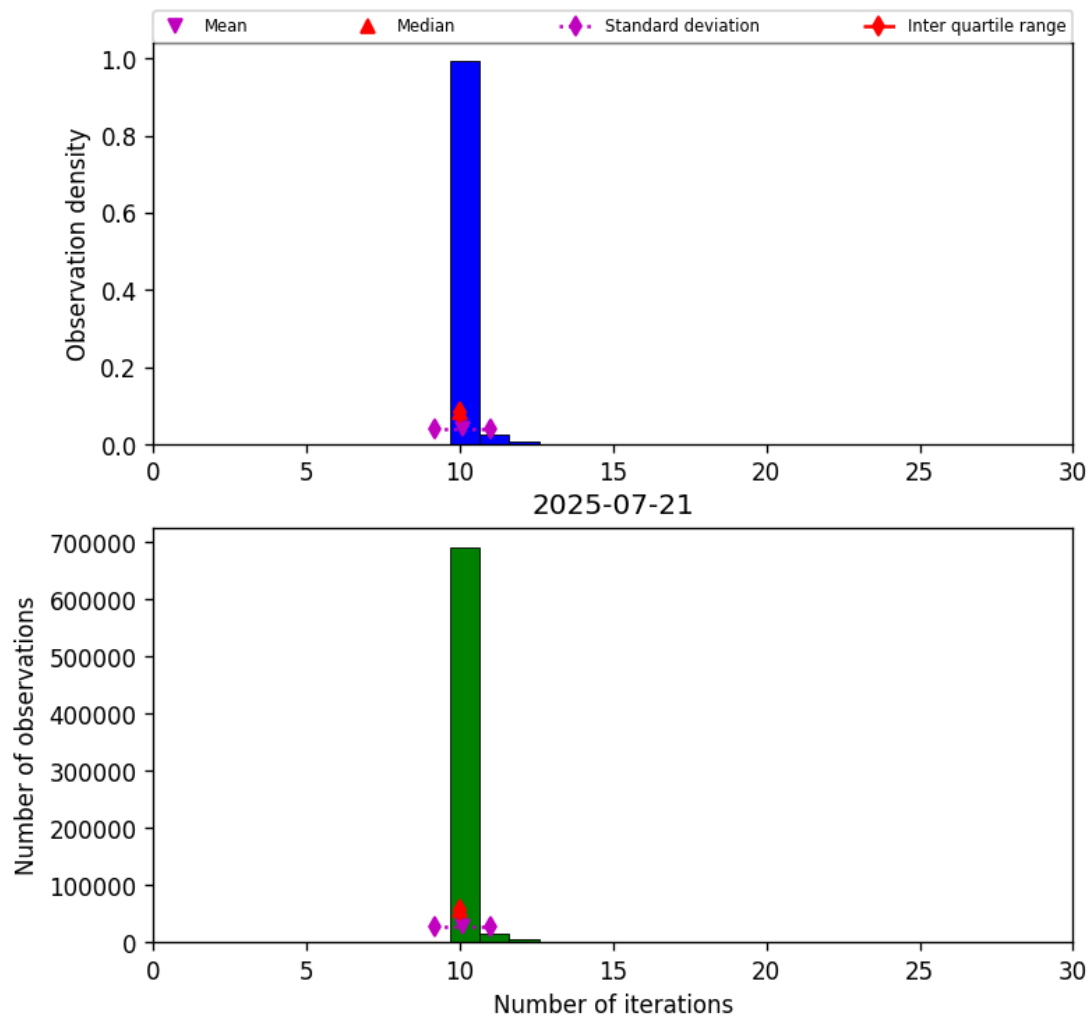
Figure 31: Histogram of "Number of iterations" for 2025-07-20 to 2025-07-22
