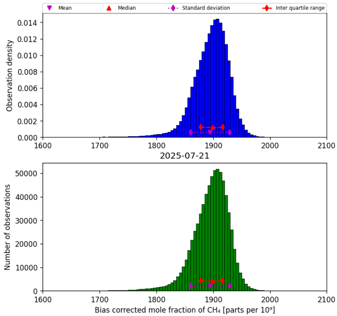
Figure 25: Histogram of “Bias corrected mole fraction of CH 4 ” for 2025-07-20 to 2025-07-22
