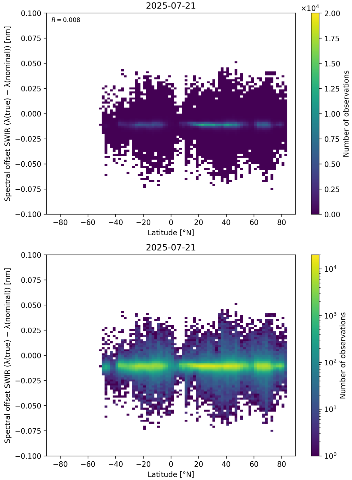
Figure 62: Scatter density plot of “Latitude” against “Spectral offset SWIR ( \lambda_{\text{true}} - \lambda_{\text{nominal}} )” for 2025-07-20 to 2025-07-22.
