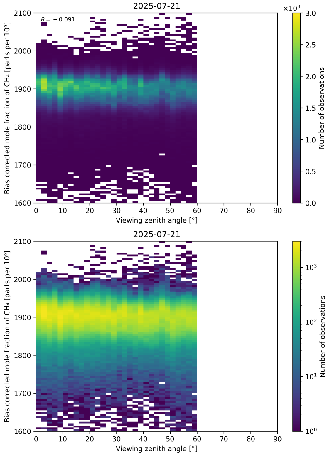
Figure 111: Scatter density plot of “Viewing zenith angle” against “Bias corrected mole fraction of CH 4 ” for 2025-07-20 to 2025-07-22.
