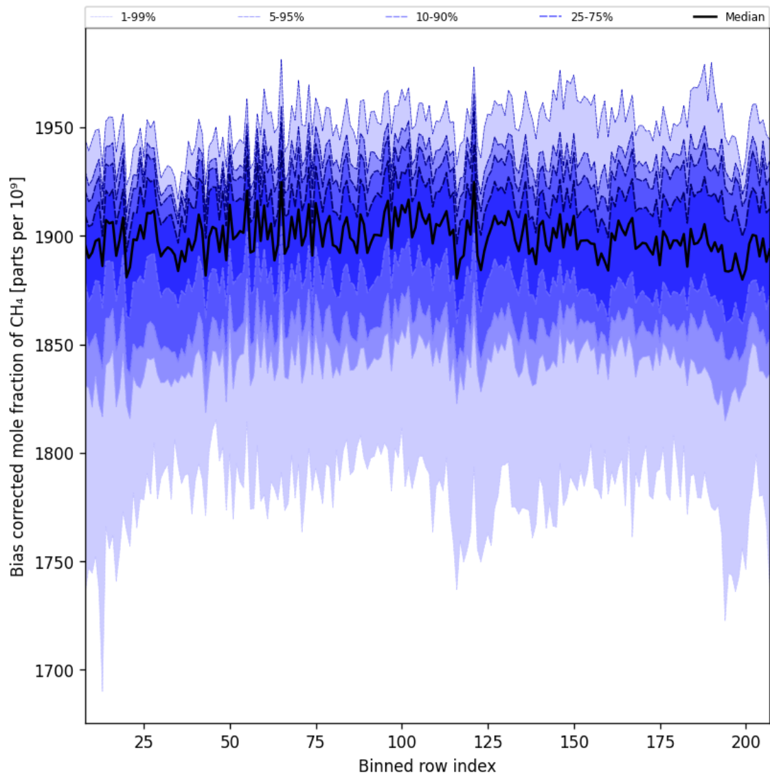
Figure 36: Along track statistics of “Bias corrected mole fraction of CH 4 ” for 2025-07-20 to 2025-07-22
