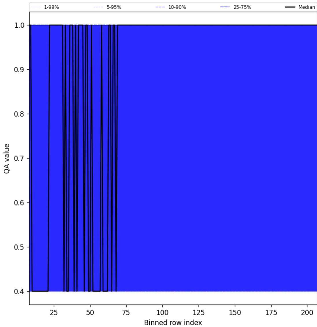
Figure 33: Along track statistics of “QA value” for 2025-07-20 to 2025-07-22
