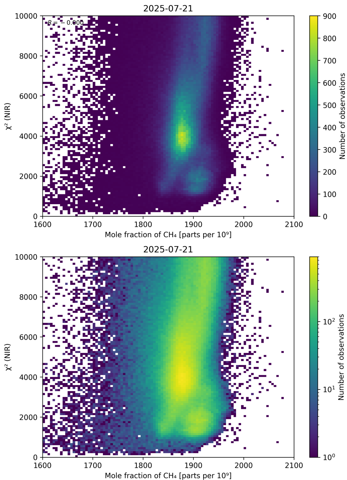
Figure 70: Scatter density plot of “Mole fraction of CH 4 ” against “ \chi^2 (NIR)” for 2025-07-20 to 2025-07-22.
