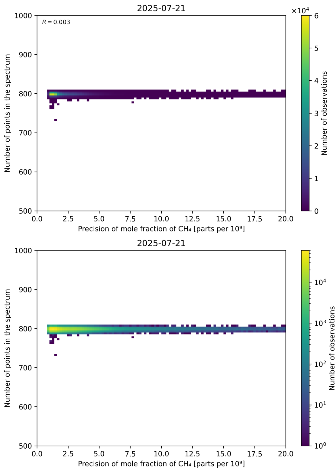
Figure 84: Scatter density plot of “Precision of mole fraction of CH 4 ” against “Number of points in the spectrum” for 2025-07-20 to 2025-07-22.
