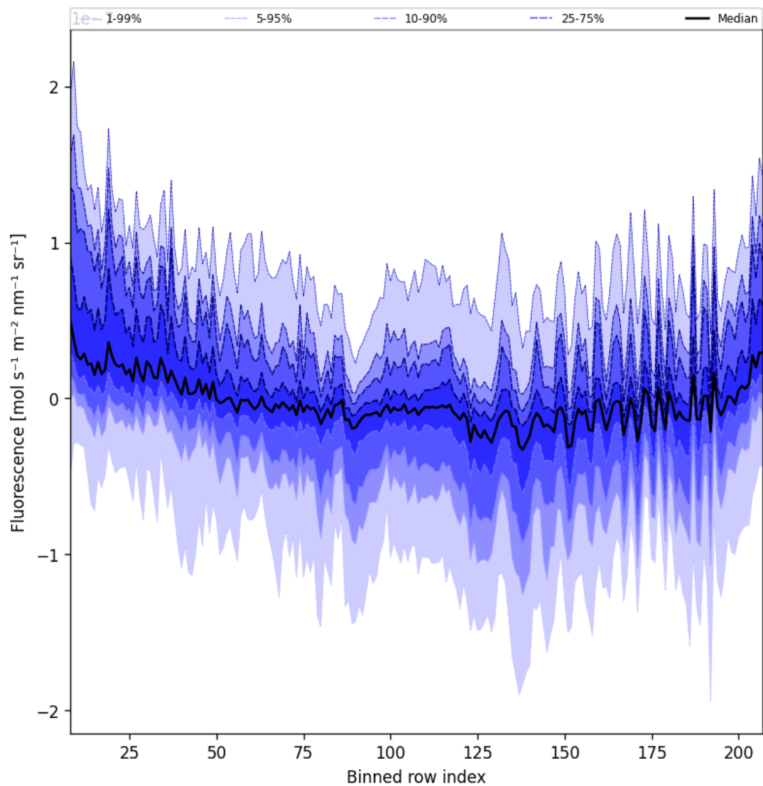
Figure 43: Along track statistics of “Fluorescence” for 2025-07-20 to 2025-07-22
