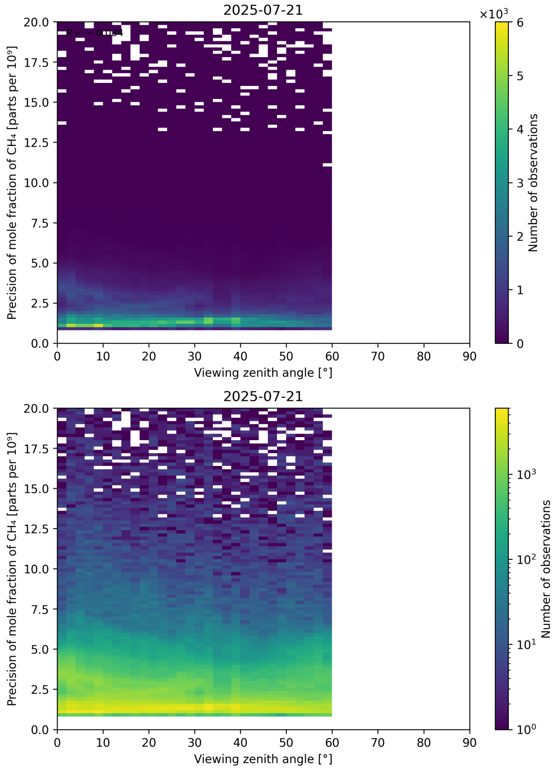
Figure 112: Scatter density plot of “Viewing zenith angle” against “Precision of mole fraction of \text{CH}_4 ” for 2025-07-20 to 2025-07-22.
