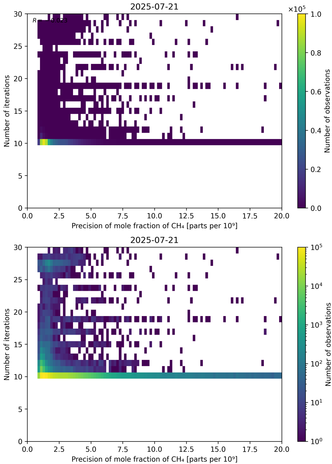
Figure 83: Scatter density plot of “Precision of mole fraction of CH 4 ” against “Number of iterations” for 2025-07-20 to 2025-07-22.
