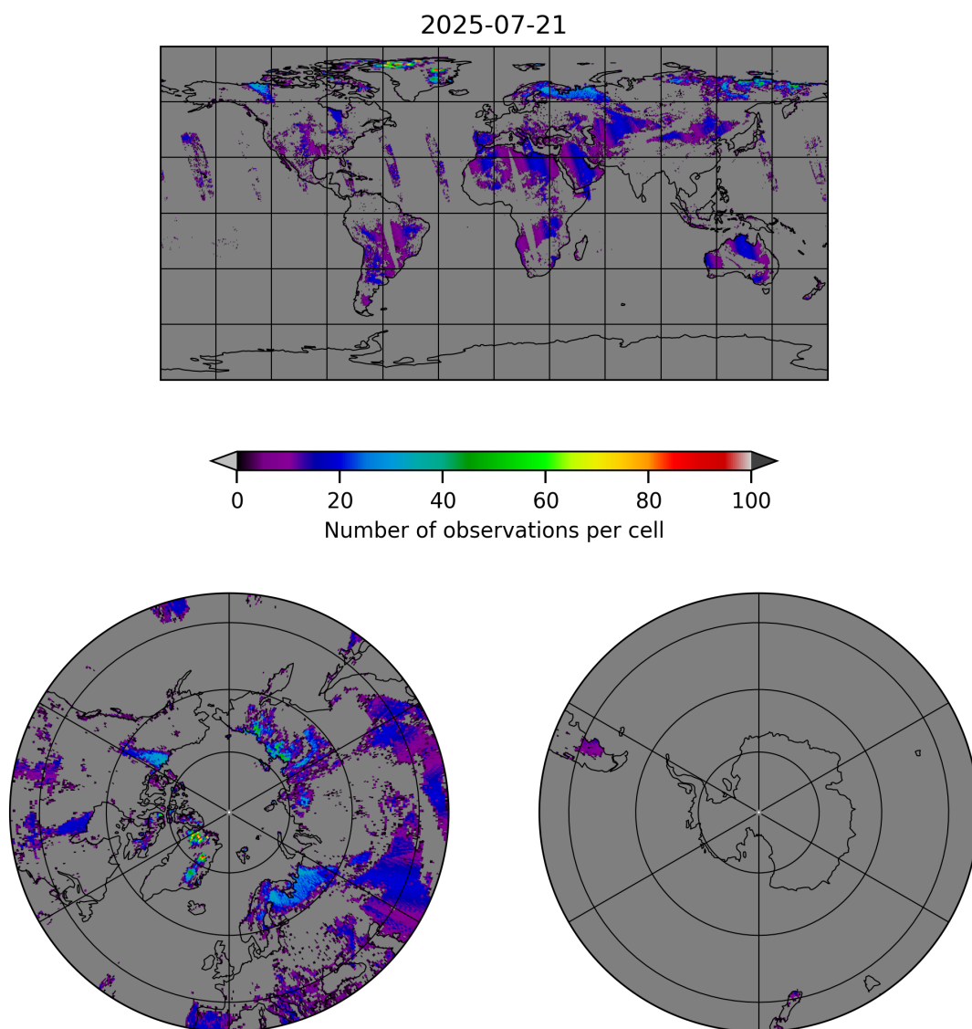
Figure 10: Map of the number of observations for 2025-07-20 to 2025-07-22
