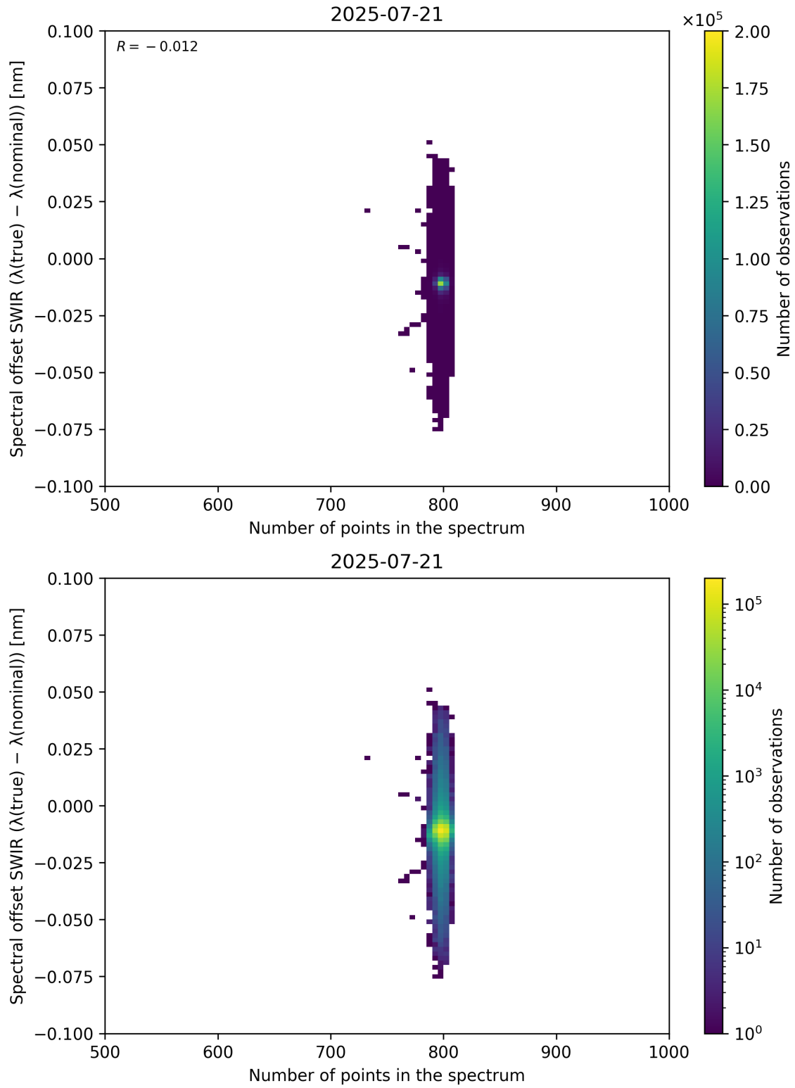
Figure 93: Scatter density plot of “Number of points in the spectrum” against “Spectral offset SWIR ( \lambda_{\text{true}} - \lambda_{\text{nominal}} )” for 2025-07-20 to 2025-07-22.
