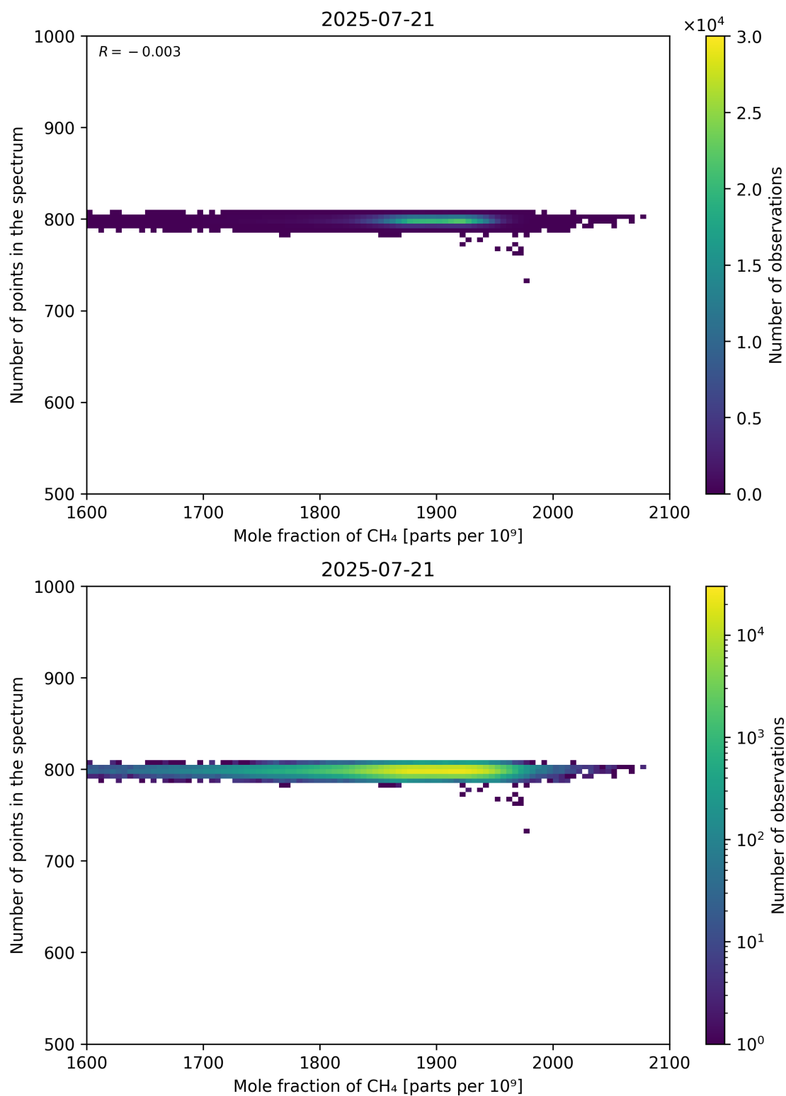
Figure 77: Scatter density plot of “Mole fraction of CH 4 ” against “Number of points in the spectrum” for 2025-07-20 to 2025-07-22.
