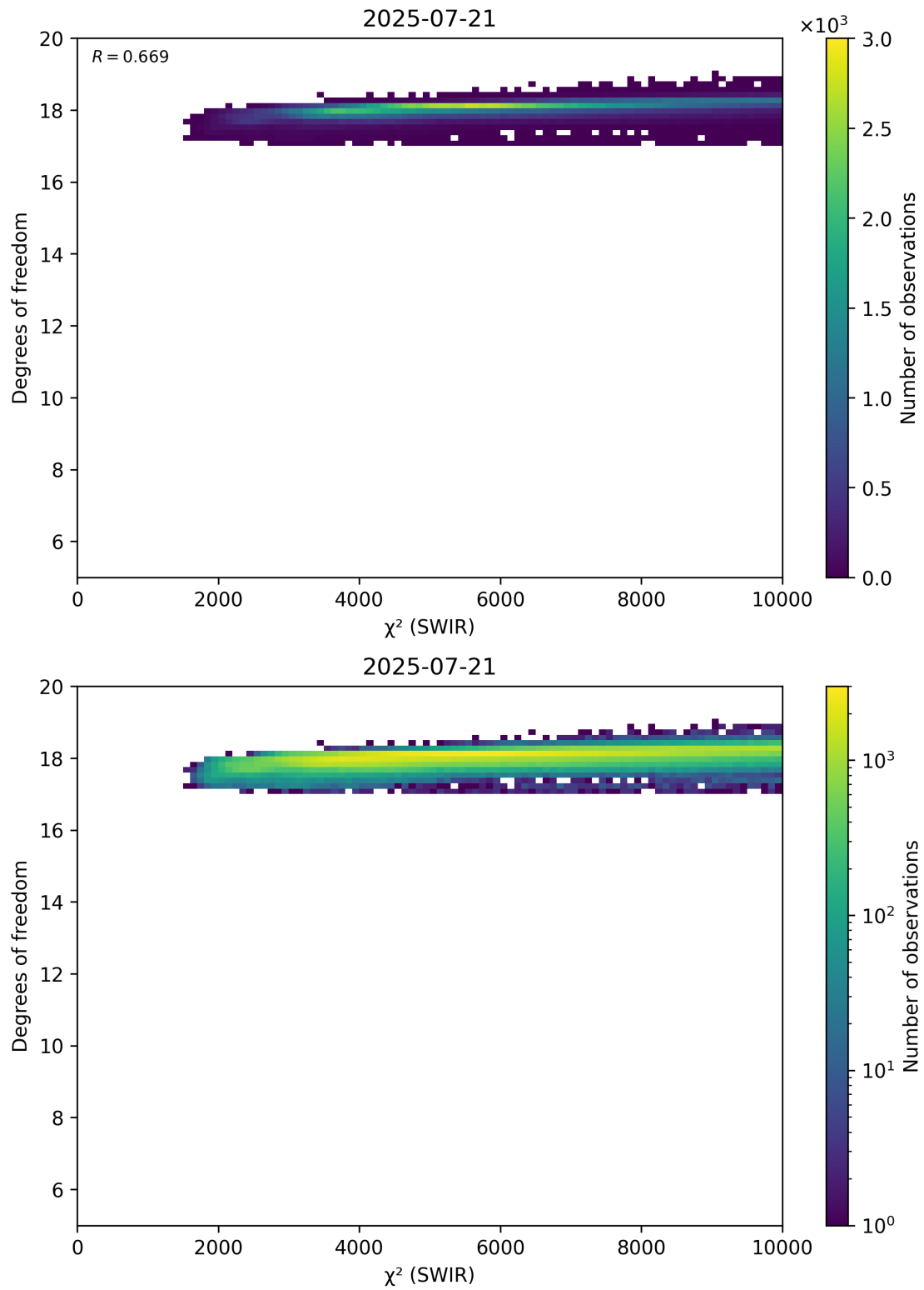
Figure 48: Scatter density plot of “ \chi^2 (SWIR)” against “Degrees of freedom” for 2025-07-20 to 2025-07-22.
