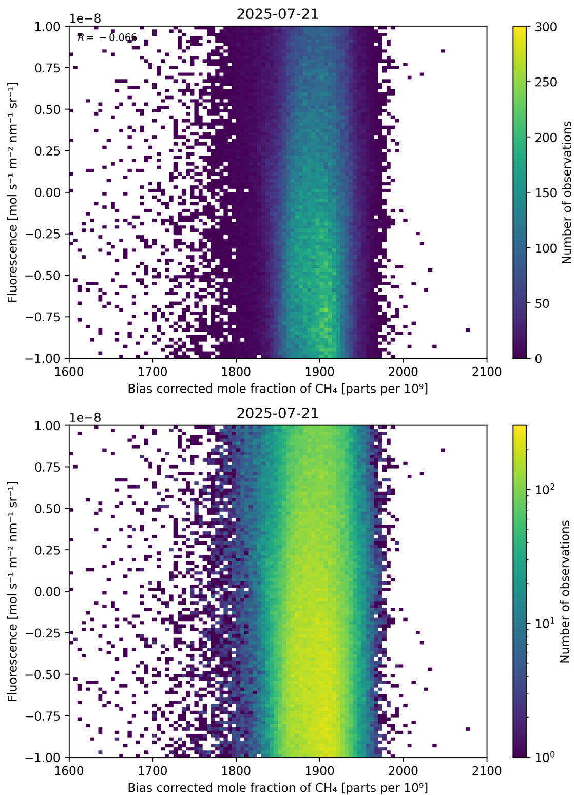
Figure 66: Scatter density plot of “Bias corrected mole fraction of \text{CH}_4 ” against “Fluorescence” for 2025-07-20 to 2025-07-22.
