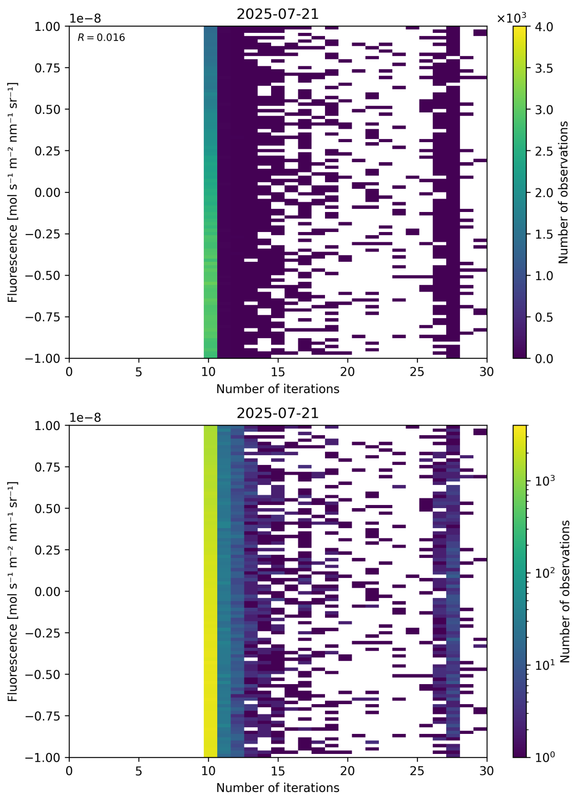
Figure 87: Scatter density plot of “Number of iterations” against “Fluorescence” for 2025-07-20 to 2025-07-22.
