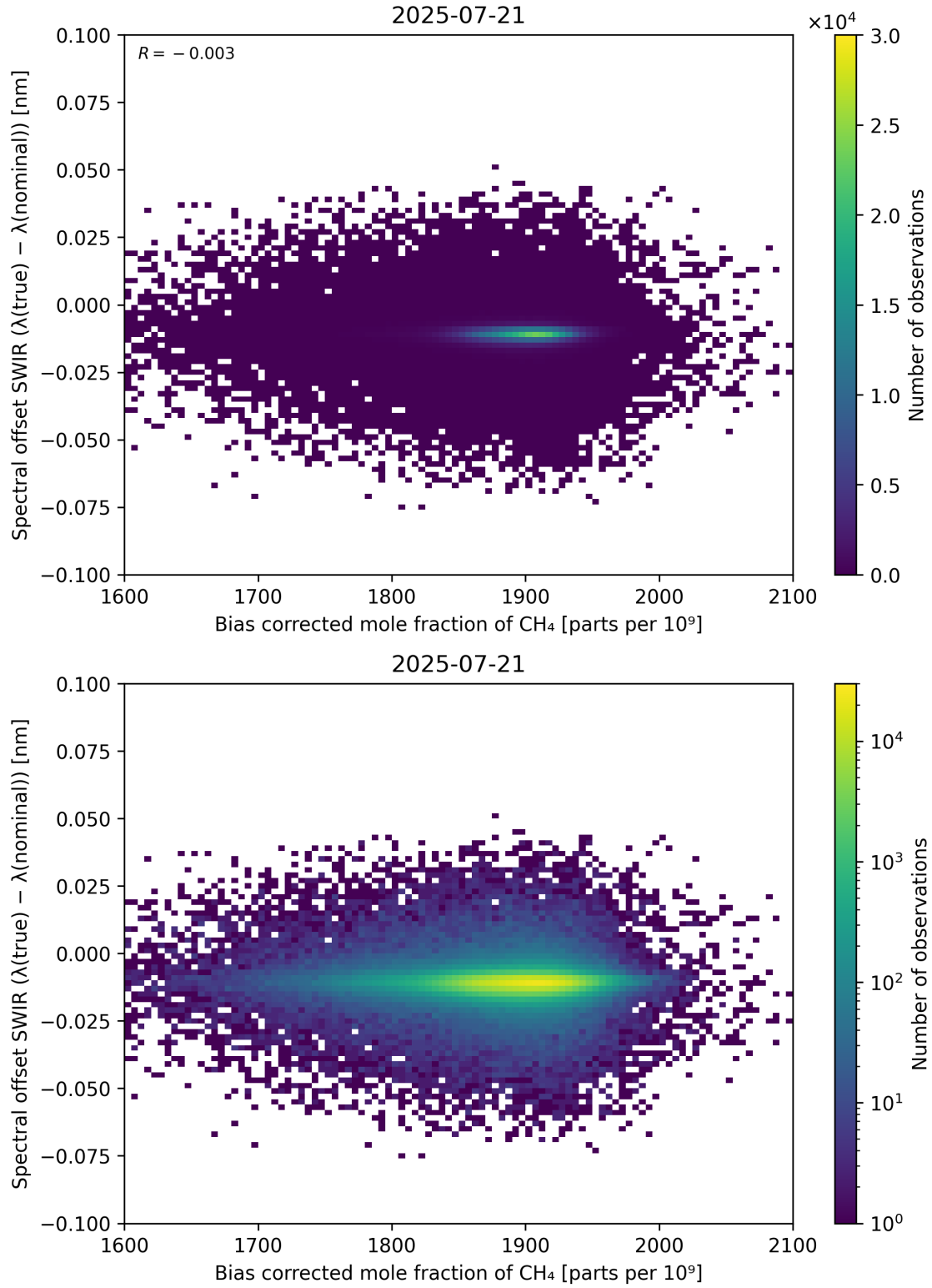
Figure 69: Scatter density plot of “Bias corrected mole fraction of \text{CH}_4 ” against “Spectral offset SWIR ( \lambda_{\text{true}} - \lambda_{\text{nominal}} )” for 2025-07-20 to 2025-07-22.
