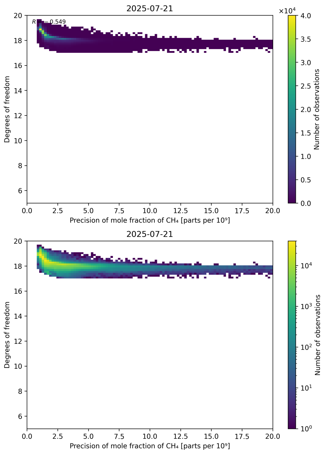
Figure 80: Scatter density plot of “Precision of mole fraction of CH 4 ” against “Degrees of freedom” for 2025-07-20 to 2025-07-22.
