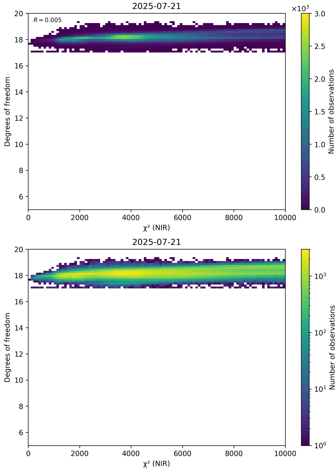
Figure 44: Scatter density plot of “ \chi^2 (NIR)” against “Degrees of freedom” for 2025-07-20 to 2025-07-22.
