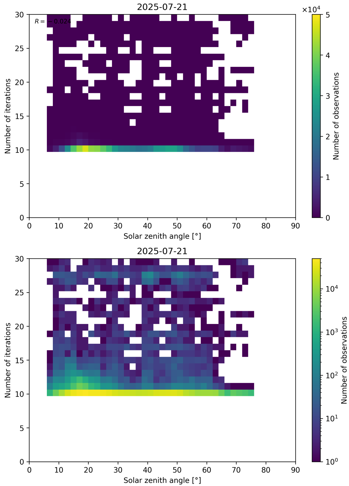
Figure 102: Scatter density plot of “Solar zenith angle” against “Number of iterations” for 2025-07-20 to 2025-07-22.
