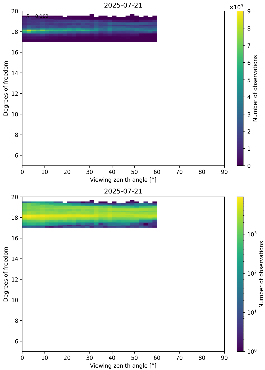
Figure 107: Scatter density plot of “Viewing zenith angle” against “Degrees of freedom” for 2025-07-20 to 2025-07-22.
