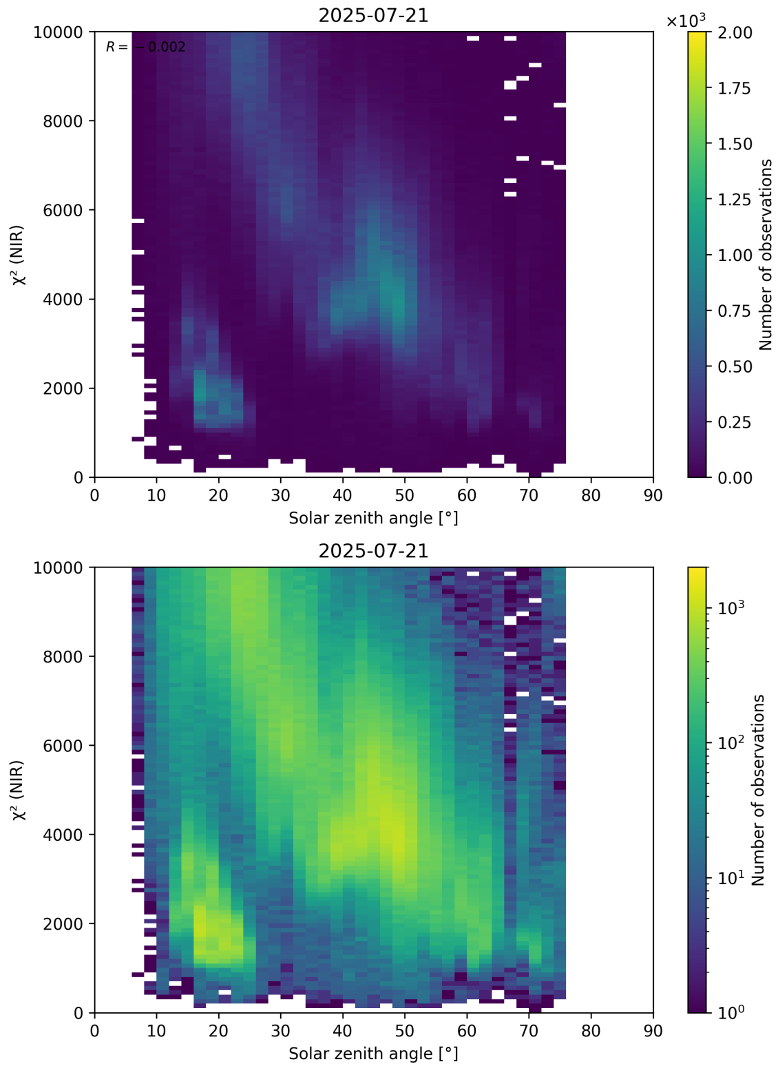
Figure 94: Scatter density plot of “Solar zenith angle” against “ \chi^2 (NIR)” for 2025-07-20 to 2025-07-22.
