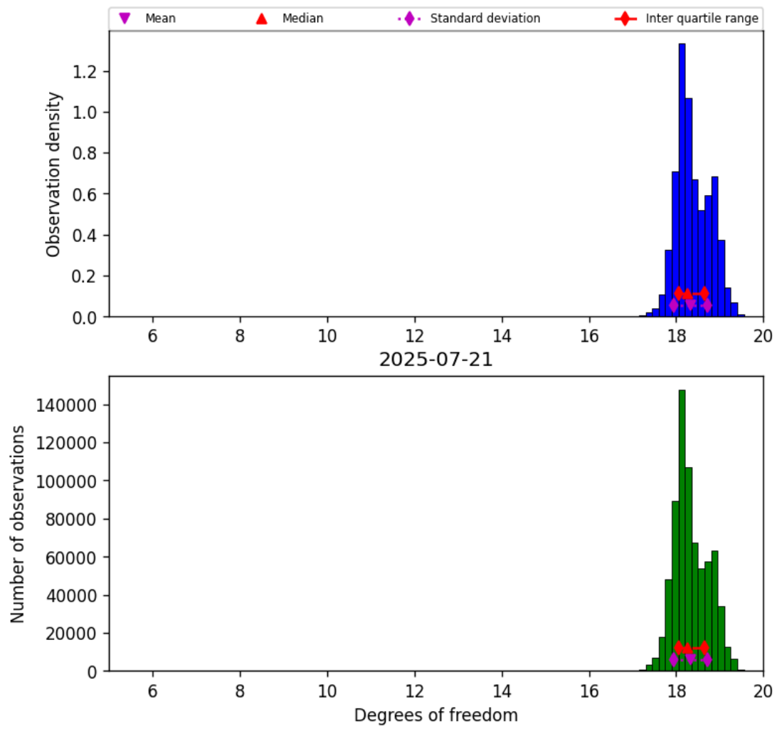
Figure 30: Histogram of “Degrees of freedom” for 2025-07-20 to 2025-07-22
