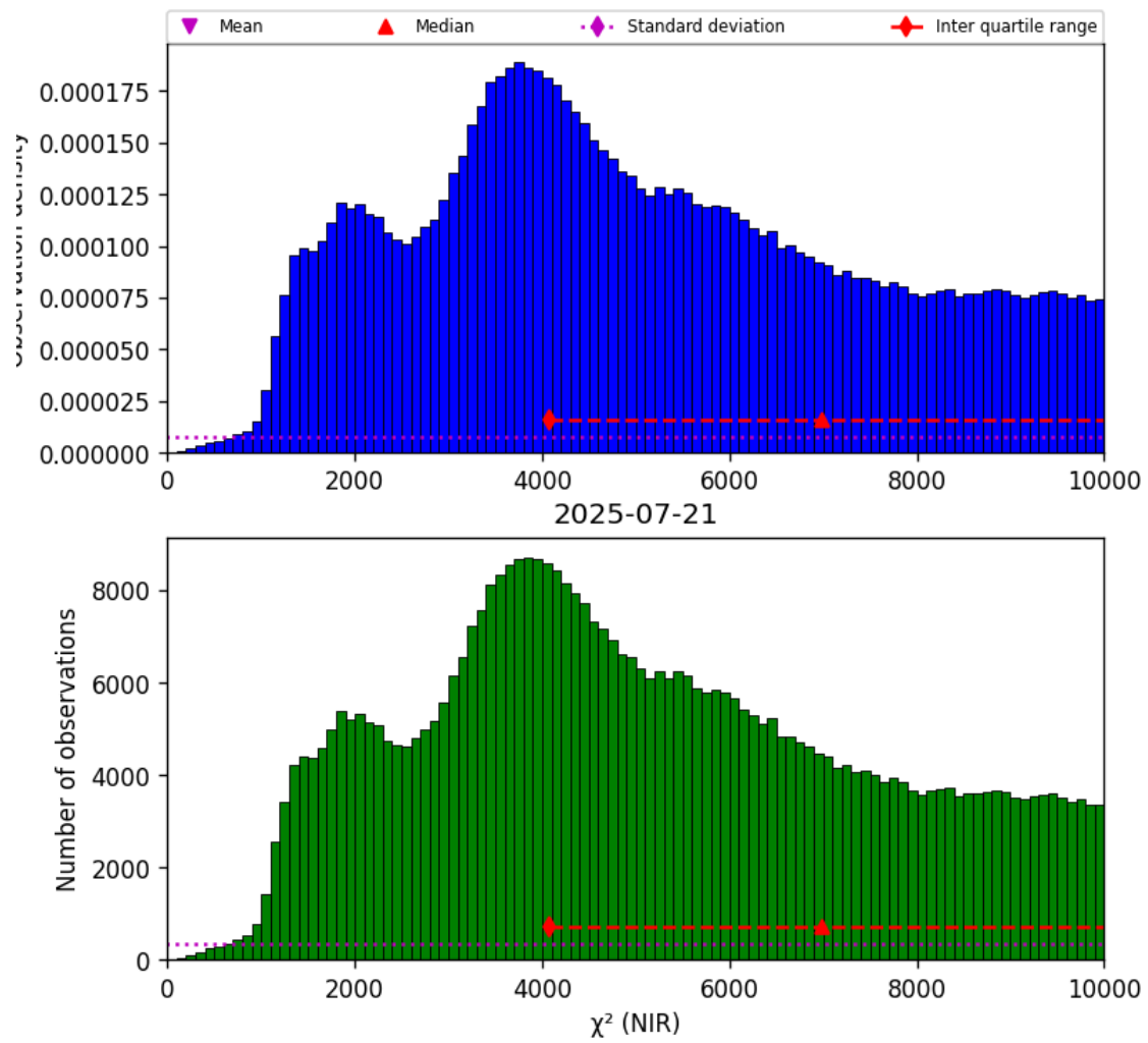
Figure 29: Histogram of “ \chi^2 (NIR)” for 2025-07-20 to 2025-07-22
