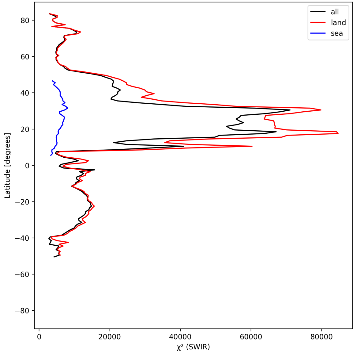
Figure 17: Zonal average of “ \chi^2 (SWIR)” for 2025-07-20 to 2025-07-22.
