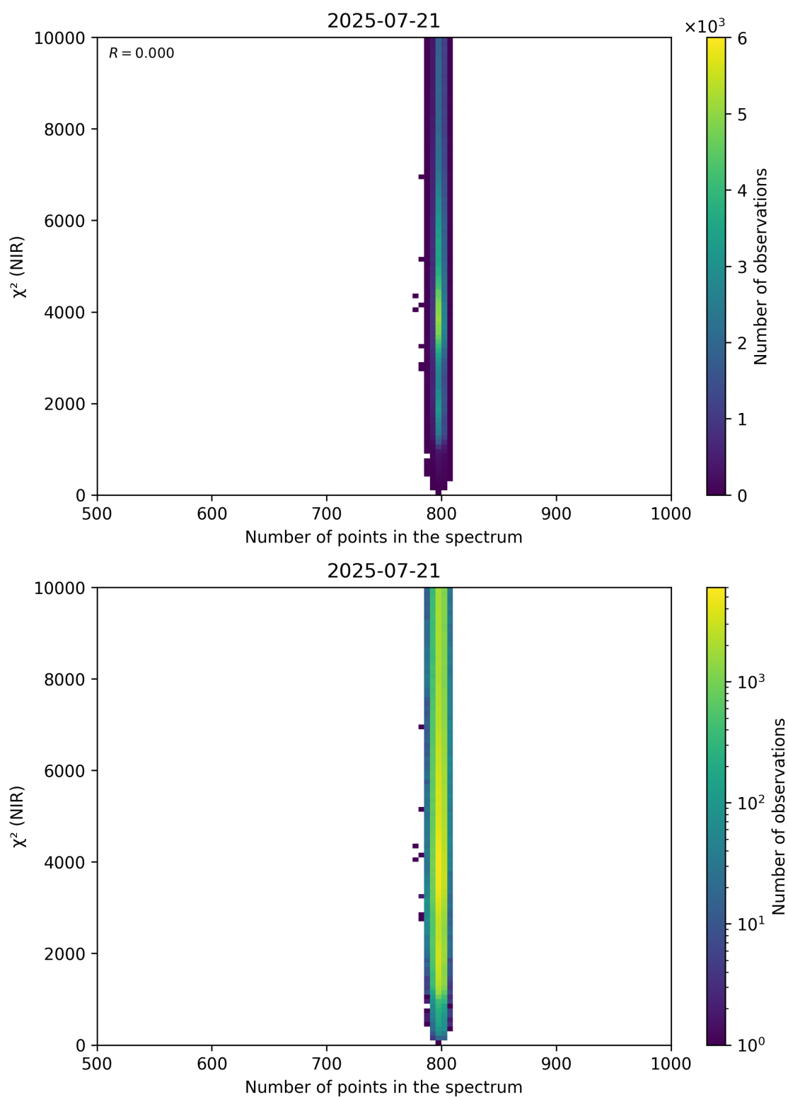
Figure 88: Scatter density plot of “Number of points in the spectrum” against “ \chi^2 (NIR)” for 2025-07-20 to 2025-07-22.
