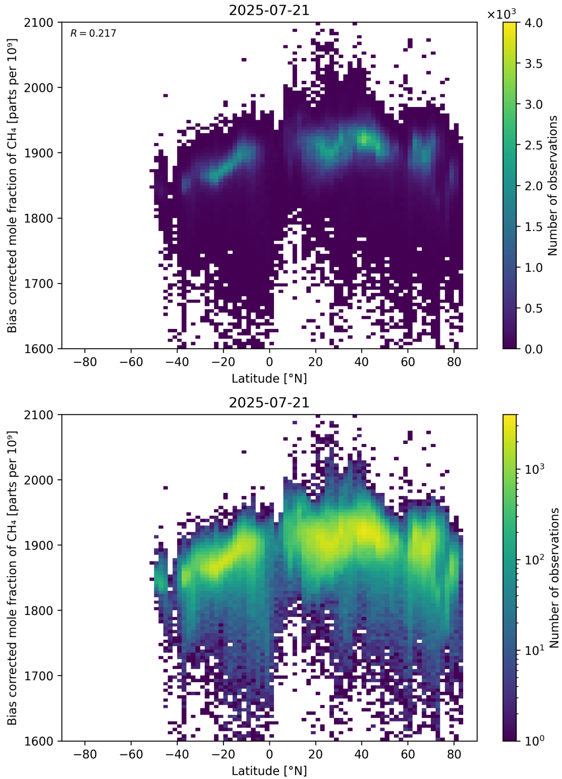
Figure 58: Scatter density plot of “Latitude” against “Bias corrected mole fraction of CH 4 ” for 2025-07-20 to 2025-07-22.
