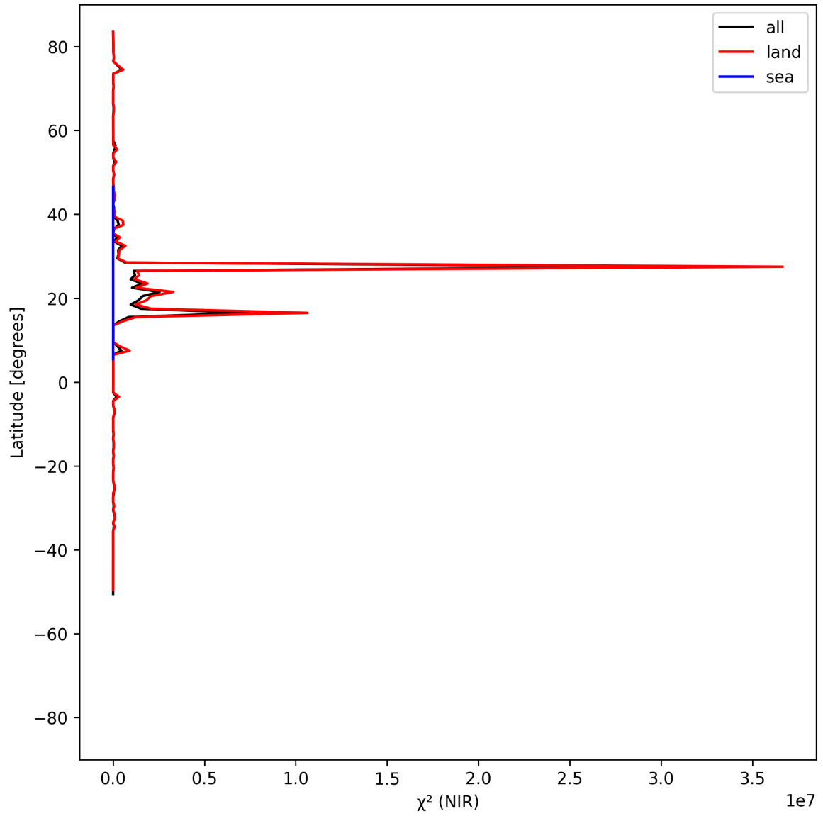
Figure 18: Zonal average of “ \chi^2 (NIR)” for 2025-07-20 to 2025-07-22.
