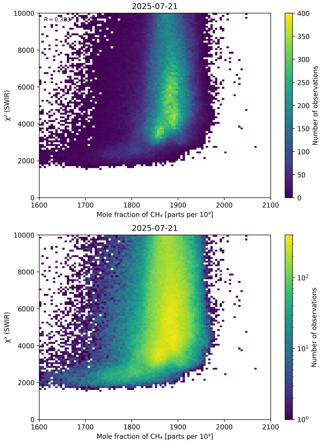
Figure 71: Scatter density plot of “Mole fraction of \text{CH}_4 ” against “ \chi^2 (SWIR)” for 2025-07-20 to 2025-07-22.
