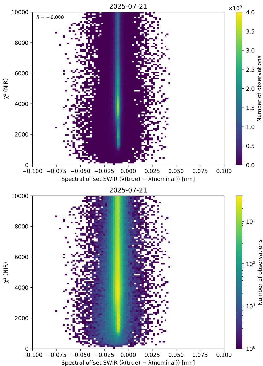
Figure 117: Scatter density plot of “Spectral offset SWIR ( \lambda_{\text{true}} - \lambda_{\text{nominal}} )” against “ \chi^2 (NIR)” for 2025-07-20 to 2025-07-22.
