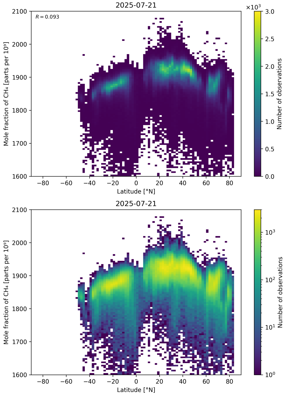
Figure 57: Scatter density plot of “Latitude” against “Mole fraction of \text{CH}_4 ” for 2025-07-20 to 2025-07-22.
