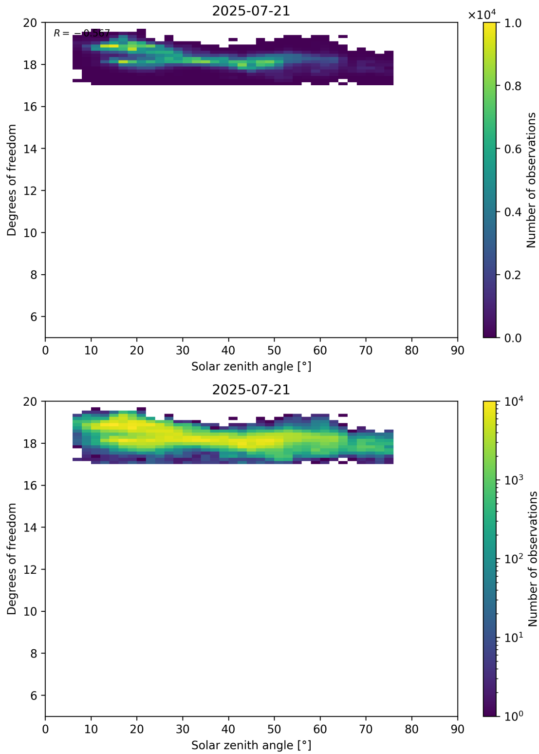
Figure 96: Scatter density plot of “Solar zenith angle” against “Degrees of freedom” for 2025-07-20 to 2025-07-22.
