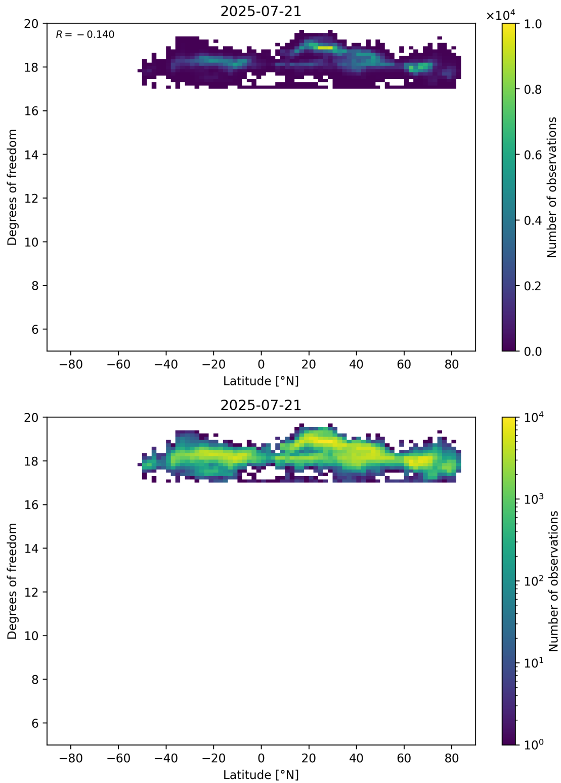
Figure 55: Scatter density plot of “Latitude” against “Degrees of freedom” for 2025-07-20 to 2025-07-22.
