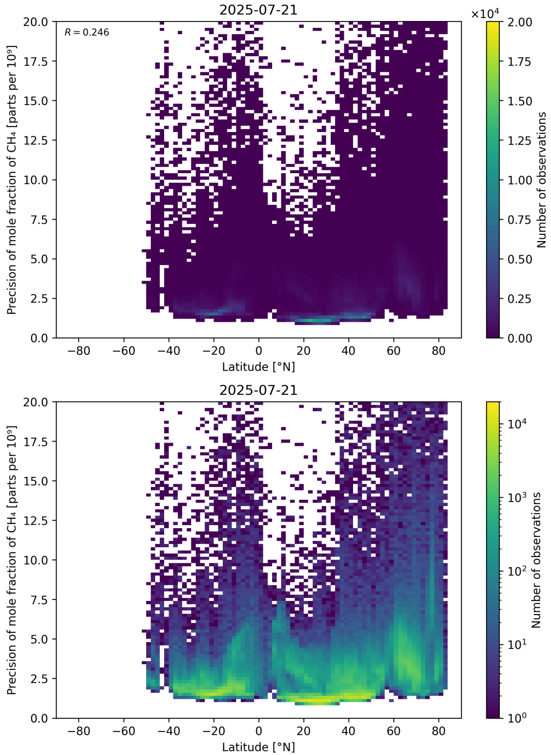
Figure 59: Scatter density plot of “Latitude” against “Precision of mole fraction of \text{CH}_4 ” for 2025-07-20 to 2025-07-22.
