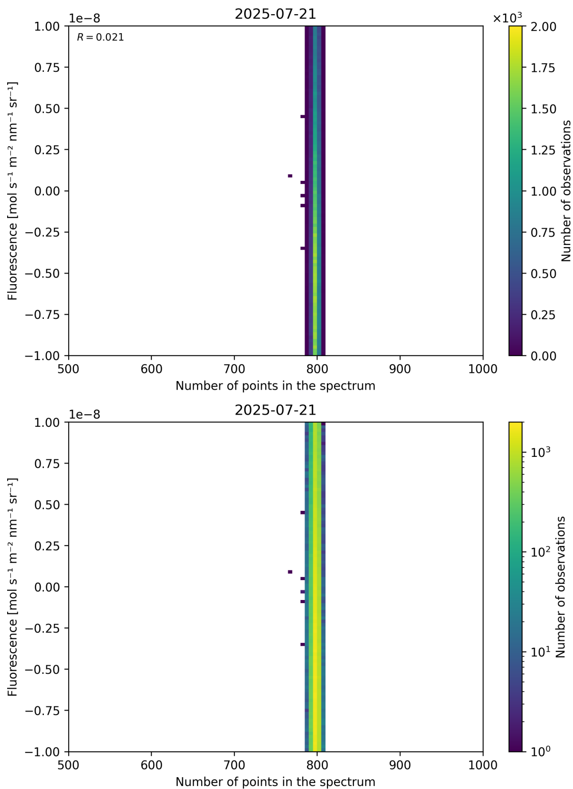
Figure 91: Scatter density plot of “Number of points in the spectrum” against “Fluorescence” for 2025-07-20 to 2025-07-22.
