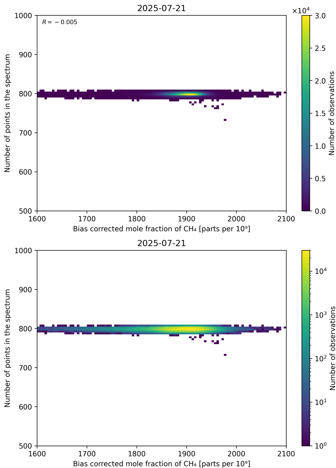
Figure 68: Scatter density plot of “Bias corrected mole fraction of CH 4 ” against “Number of points in the spectrum” for 2025-07-20 to 2025-07-22.
