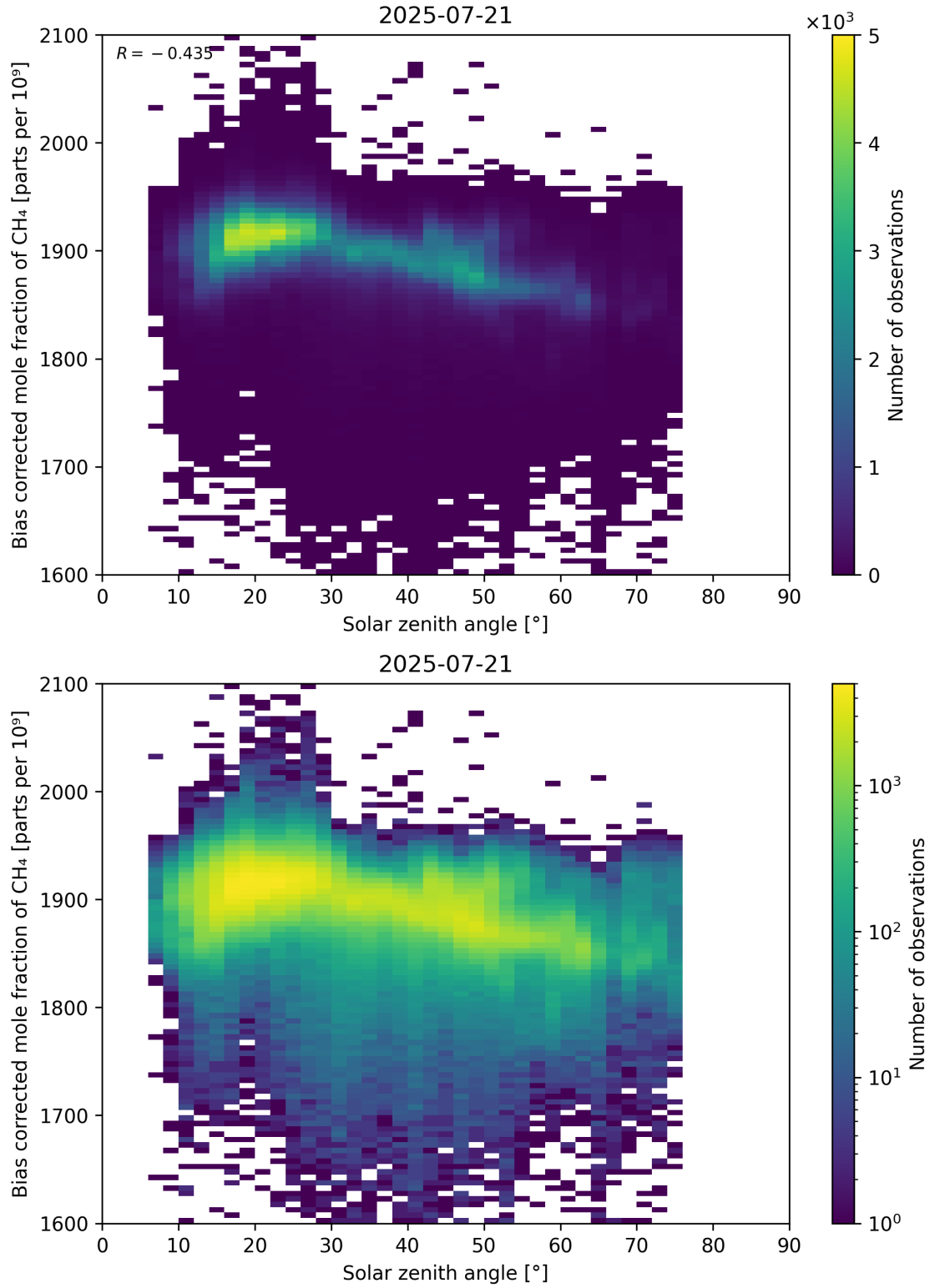
Figure 100: Scatter density plot of “Solar zenith angle” against “Bias corrected mole fraction of \text{CH}_4 ” for 2025-07-20 to 2025-07-22.
