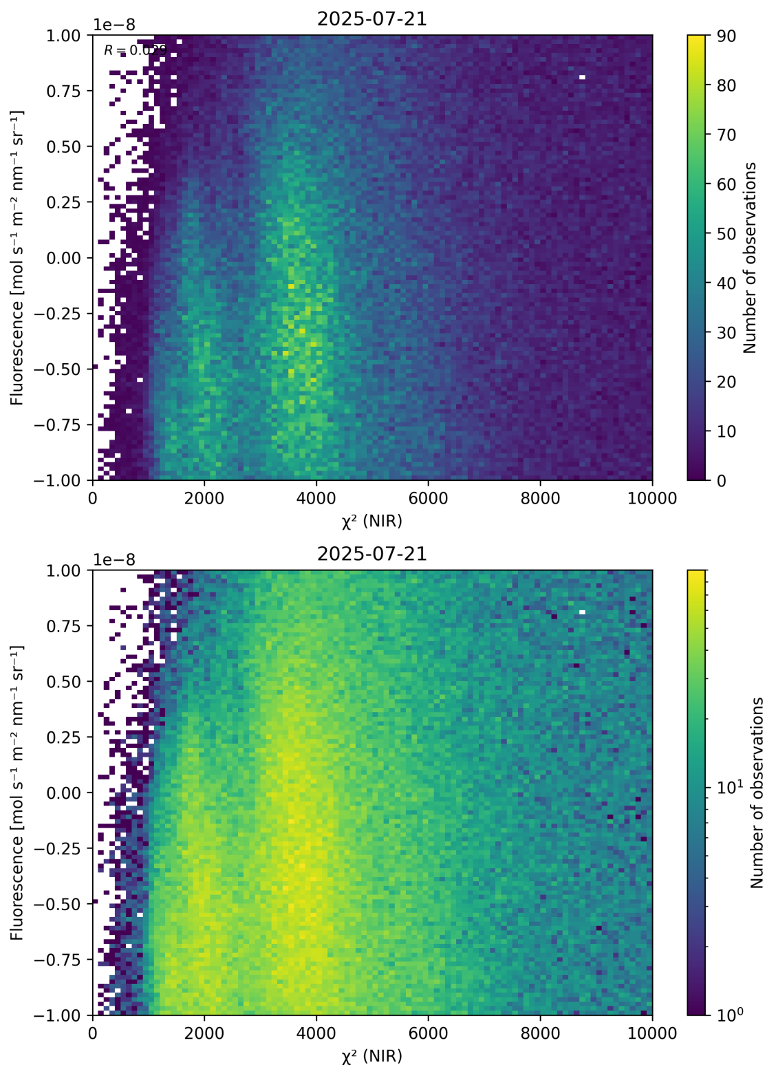
Figure 45: Scatter density plot of “ \chi^2 (NIR)” against “Fluorescence” for 2025-07-20 to 2025-07-22.
