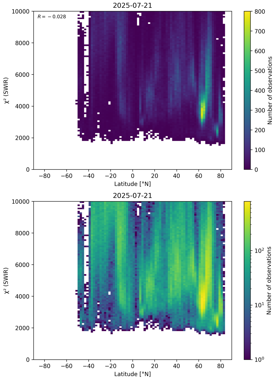
Figure 54: Scatter density plot of “Latitude” against “ \chi^2 (SWIR)” for 2025-07-20 to 2025-07-22.
