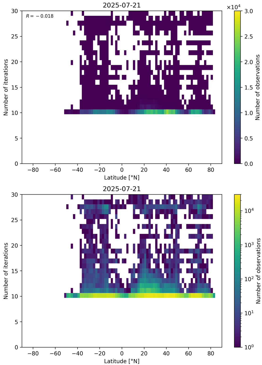
Figure 60: Scatter density plot of “Latitude” against “Number of iterations” for 2025-07-20 to 2025-07-22.
