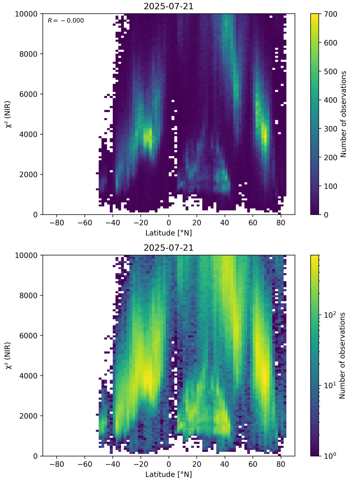
Figure 53: Scatter density plot of “Latitude” against “ \chi^2 (NIR)” for 2025-07-20 to 2025-07-22.
