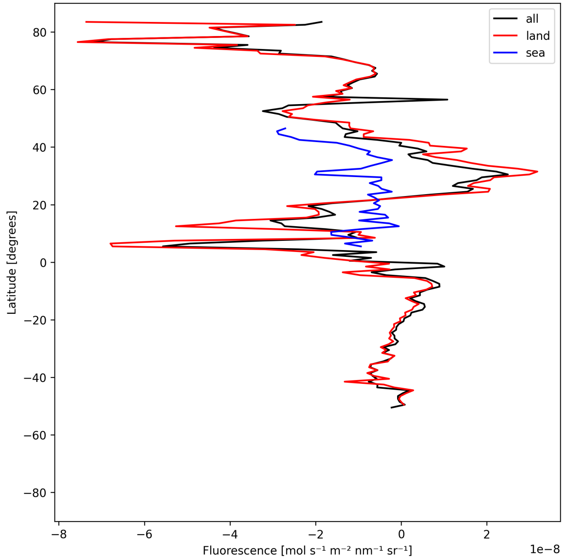
Figure 21: Zonal average of “Fluorescence” for 2025-07-20 to 2025-07-22.
