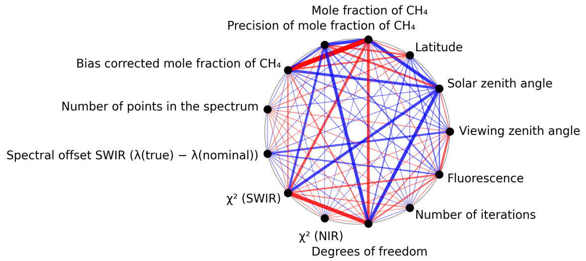
Figure 1: Map of correlation graph for 2025-07-20 to 2025-07-22.
