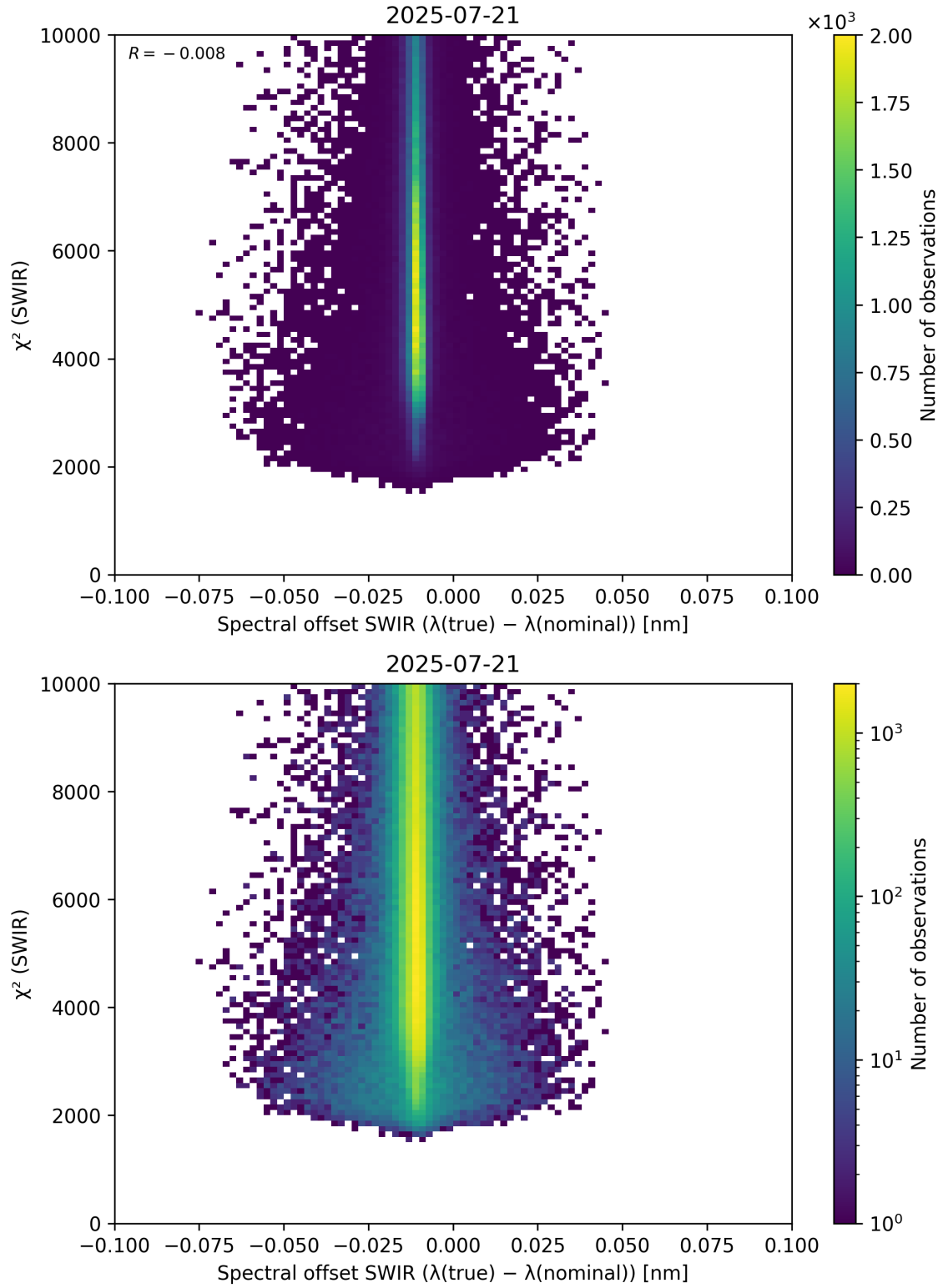
Figure 118: Scatter density plot of “Spectral offset SWIR ( \lambda_{\text{true}} - \lambda_{\text{nominal}} )” against “ \chi^2 (SWIR)” for 2025-07-20 to 2025-07-22.
