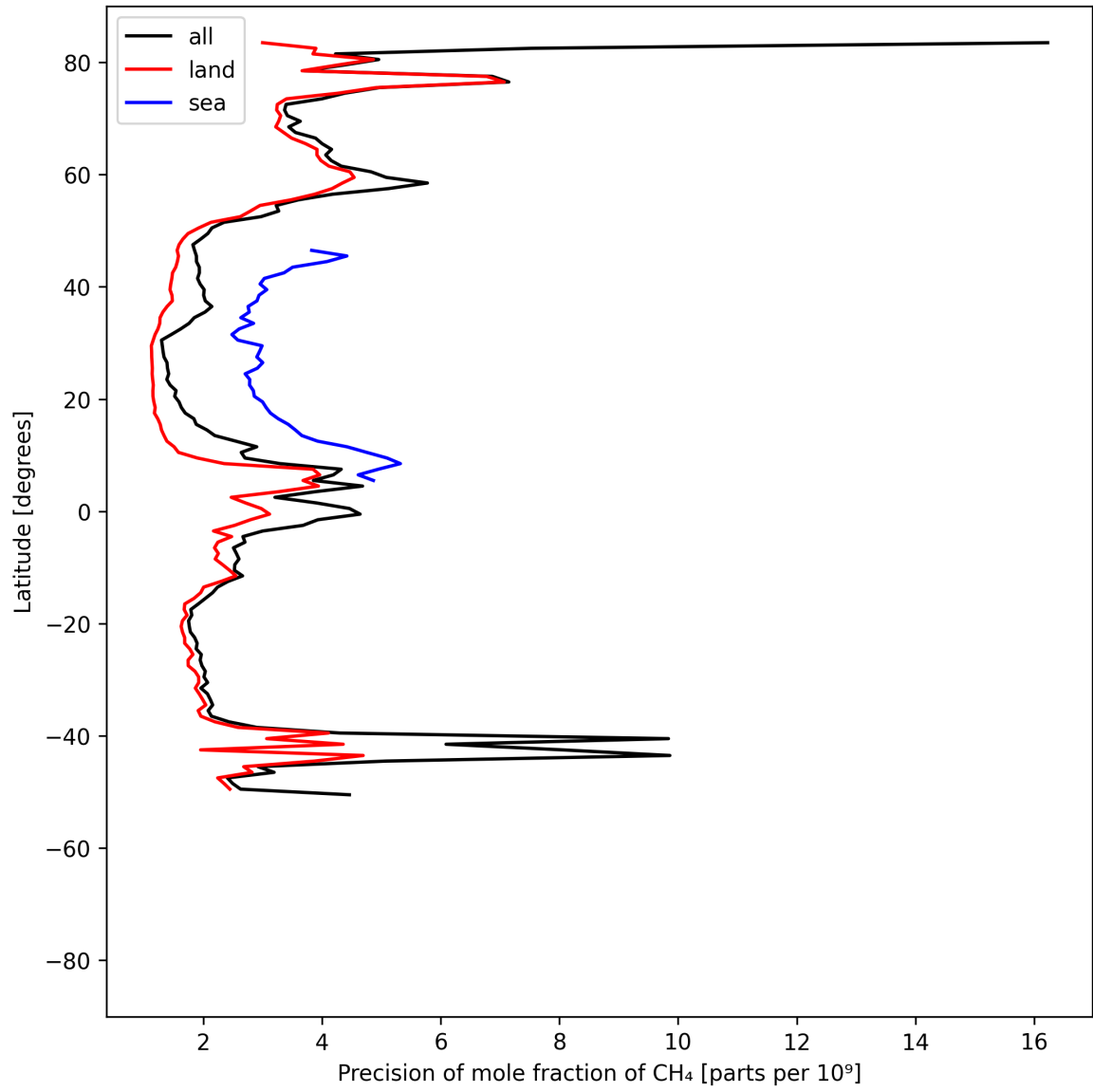
Figure 13: Zonal average of “Precision of mole fraction of CH 4 ” for 2025-07-20 to 2025-07-22.
