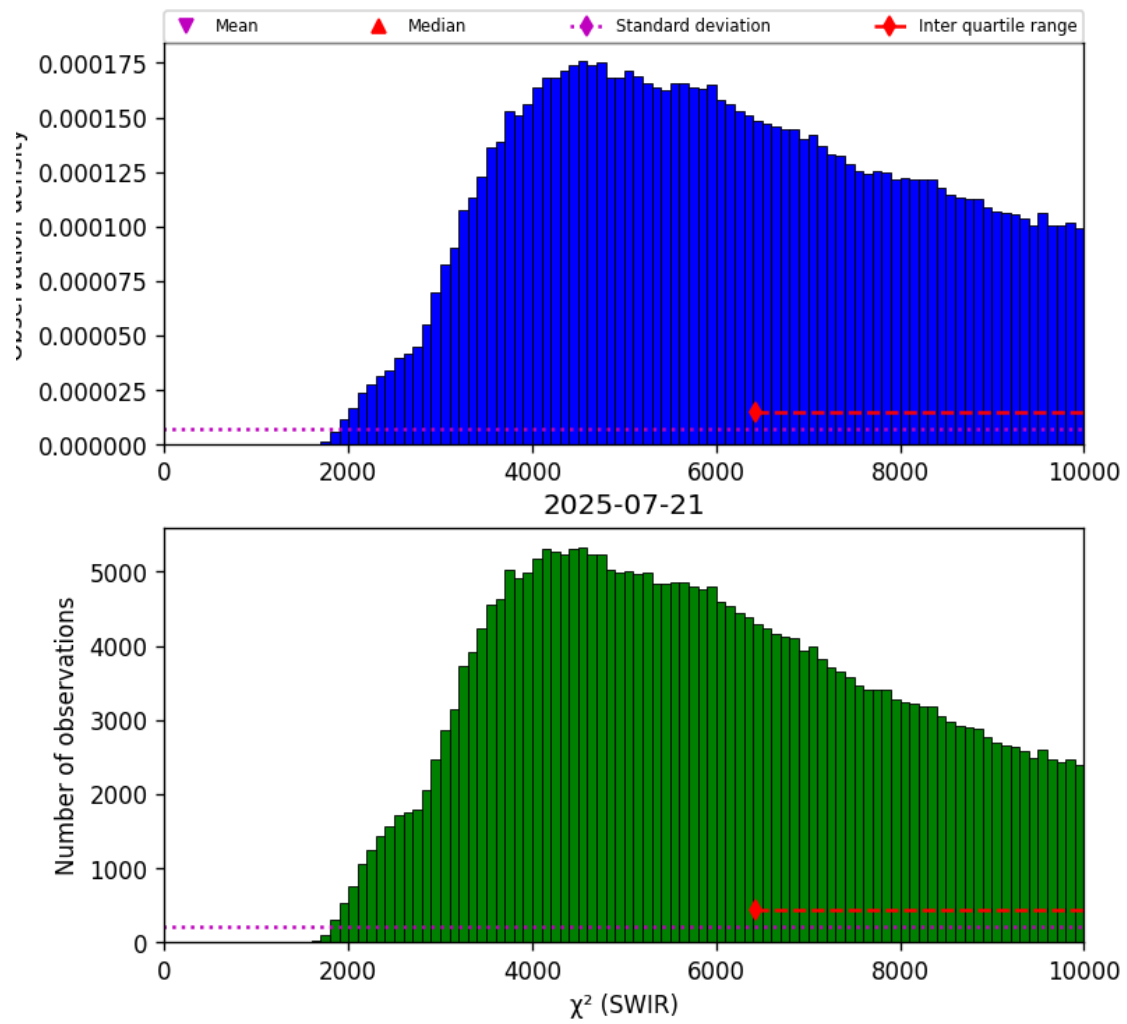
Figure 28: Histogram of “ \chi^2 (SWIR)” for 2025-07-20 to 2025-07-22
