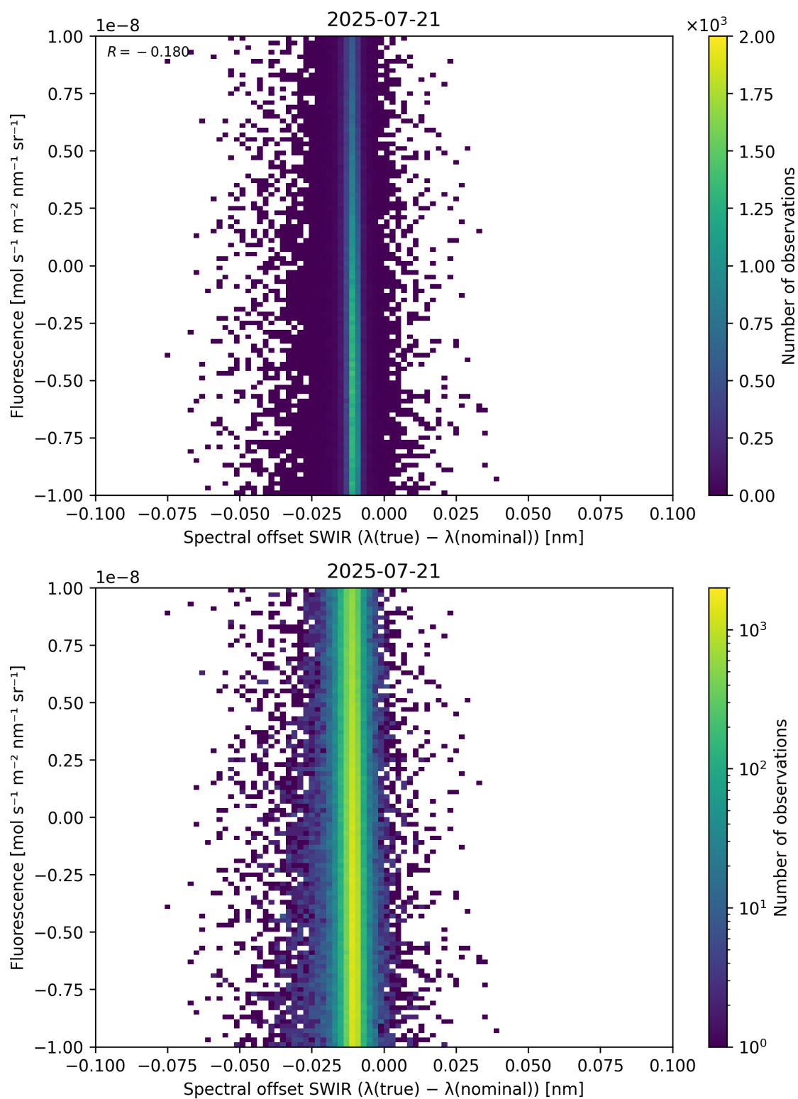
Figure 120: Scatter density plot of “Spectral offset SWIR ( \lambda_{\text{true}} - \lambda_{\text{nominal}} )” against “Fluorescence” for 2025-07-20 to 2025-07-22.
