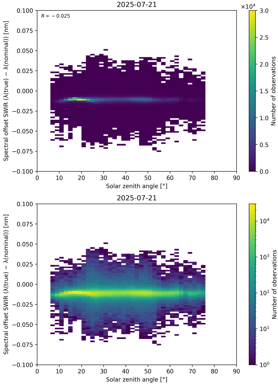
Figure 104: Scatter density plot of “Solar zenith angle” against “Spectral offset SWIR ( \lambda_{\text{true}} - \lambda_{\text{nominal}} )” for 2025-07-20 to 2025-07-22.
