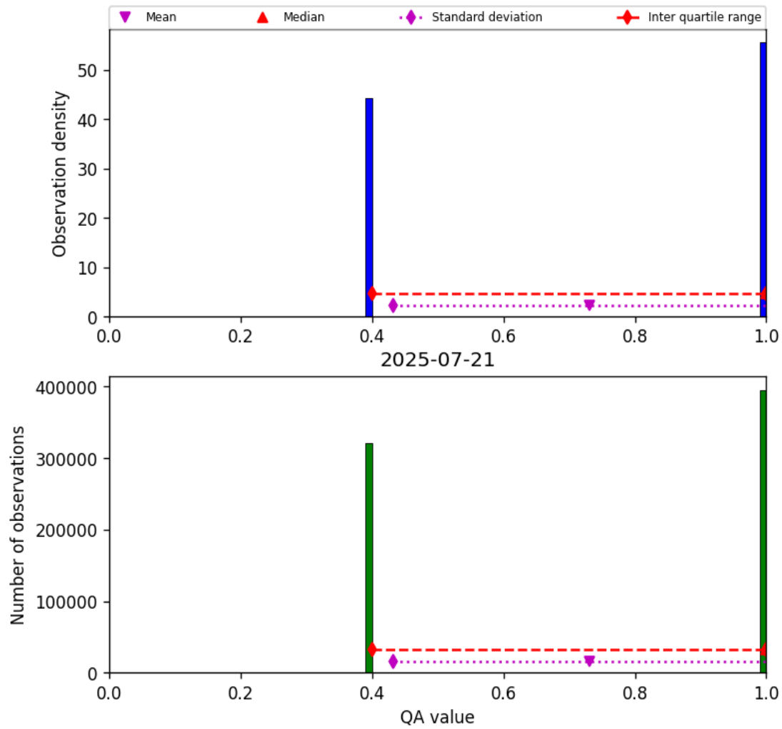
Figure 22: Histogram of “QA value” for 2025-07-20 to 2025-07-22
