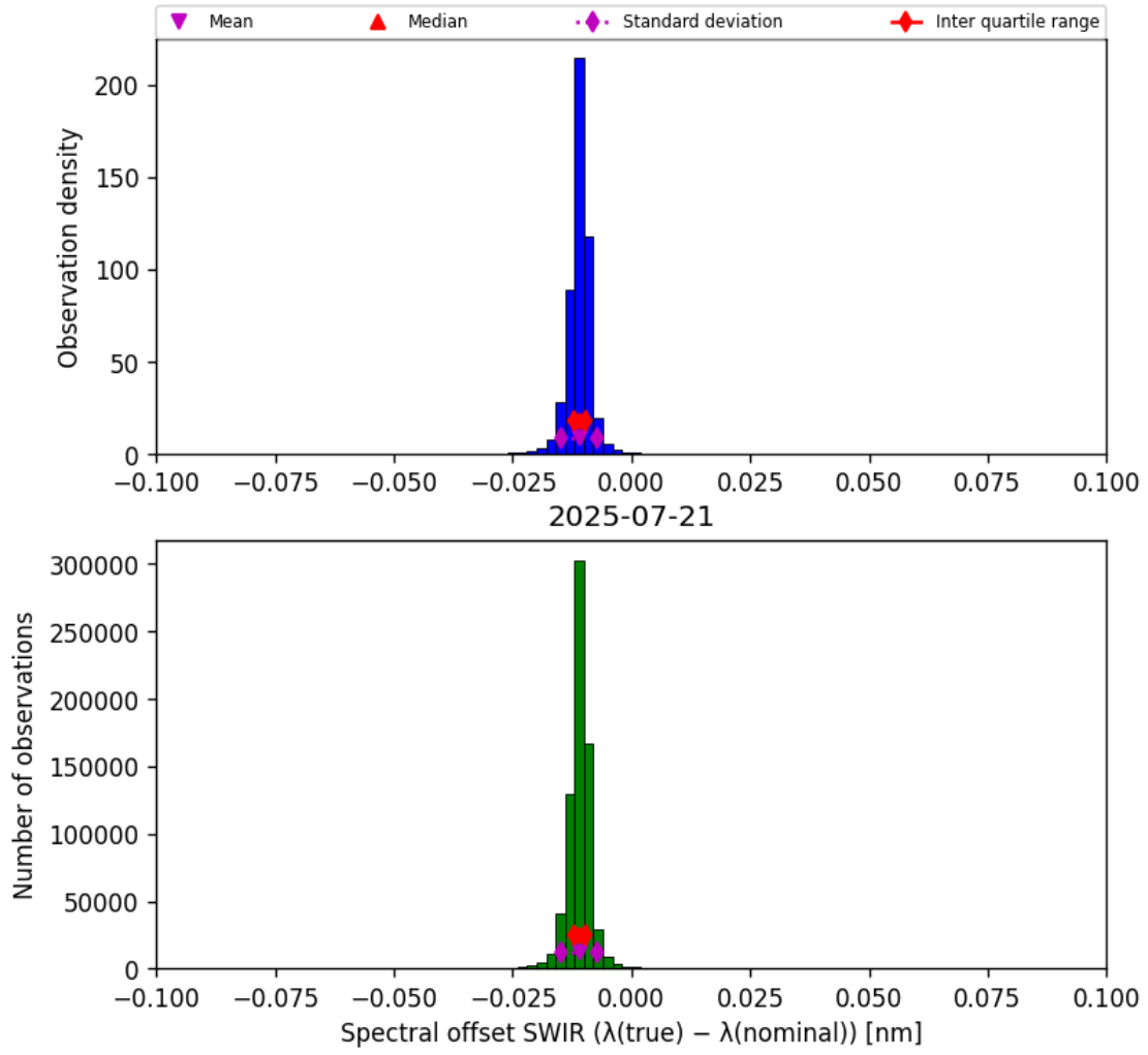
Figure 27: Histogram of “Spectral offset SWIR ( \lambda_{\text{true}} - \lambda_{\text{nominal}} )” for 2025-07-20 to 2025-07-22
