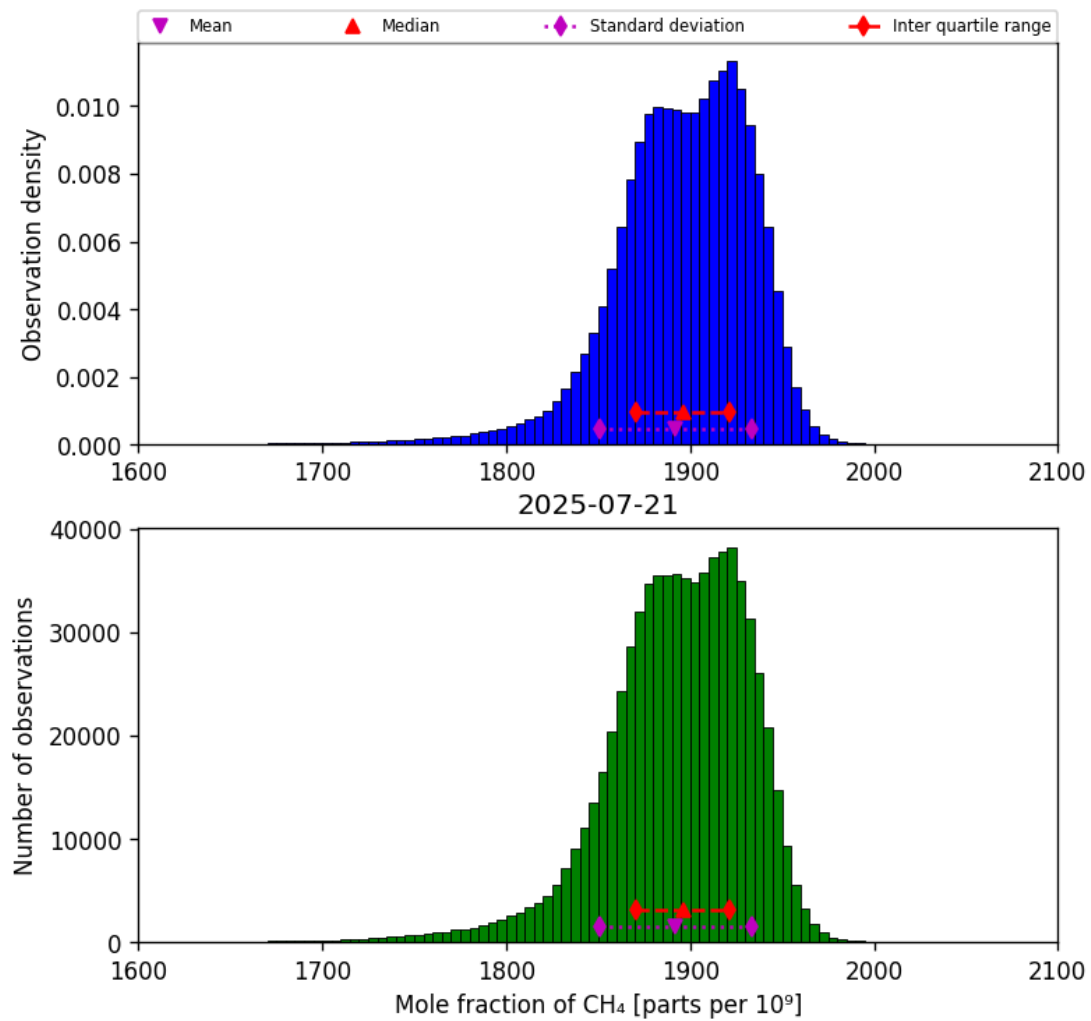
Figure 23: Histogram of “Mole fraction of CH 4 ” for 2025-07-20 to 2025-07-22
