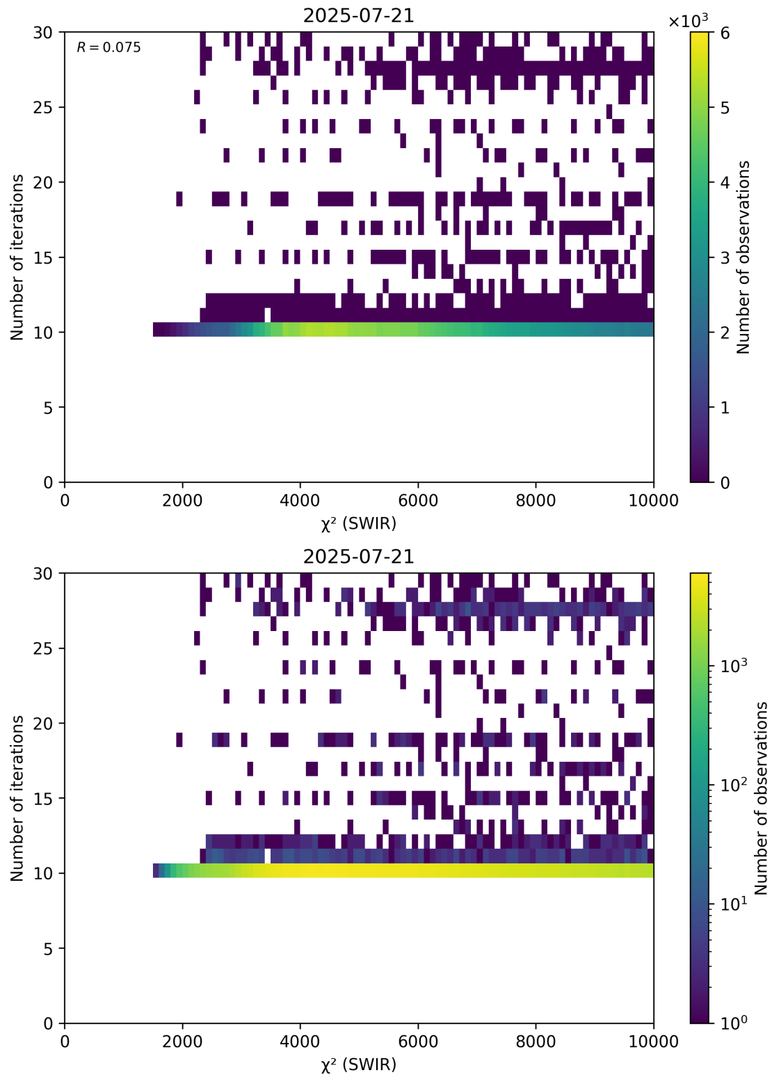
Figure 50: Scatter density plot of " \chi^2 (SWIR)" against "Number of iterations" for 2025-07-20 to 2025-07-22.
