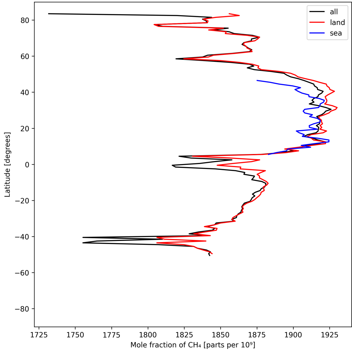
Figure 12: Zonal average of “Mole fraction of \text{CH}_4 ” for 2025-07-20 to 2025-07-22.
