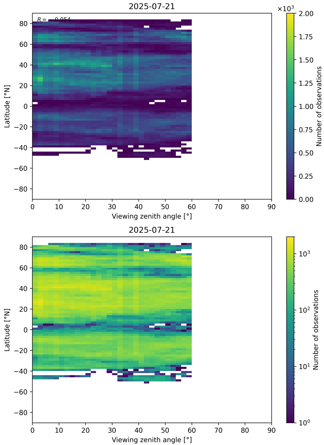
Figure 109: Scatter density plot of “Viewing zenith angle” against “Latitude” for 2025-07-20 to 2025-07-22.
