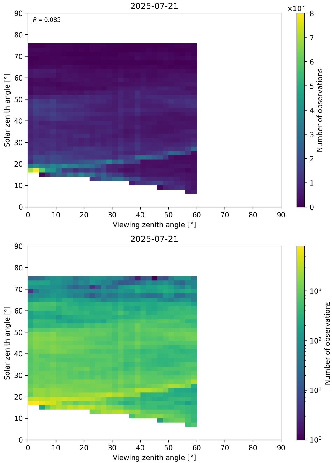
Figure 115: Scatter density plot of “Viewing zenith angle” against “Solar zenith angle” for 2025-07-20 to 2025-07-22.
