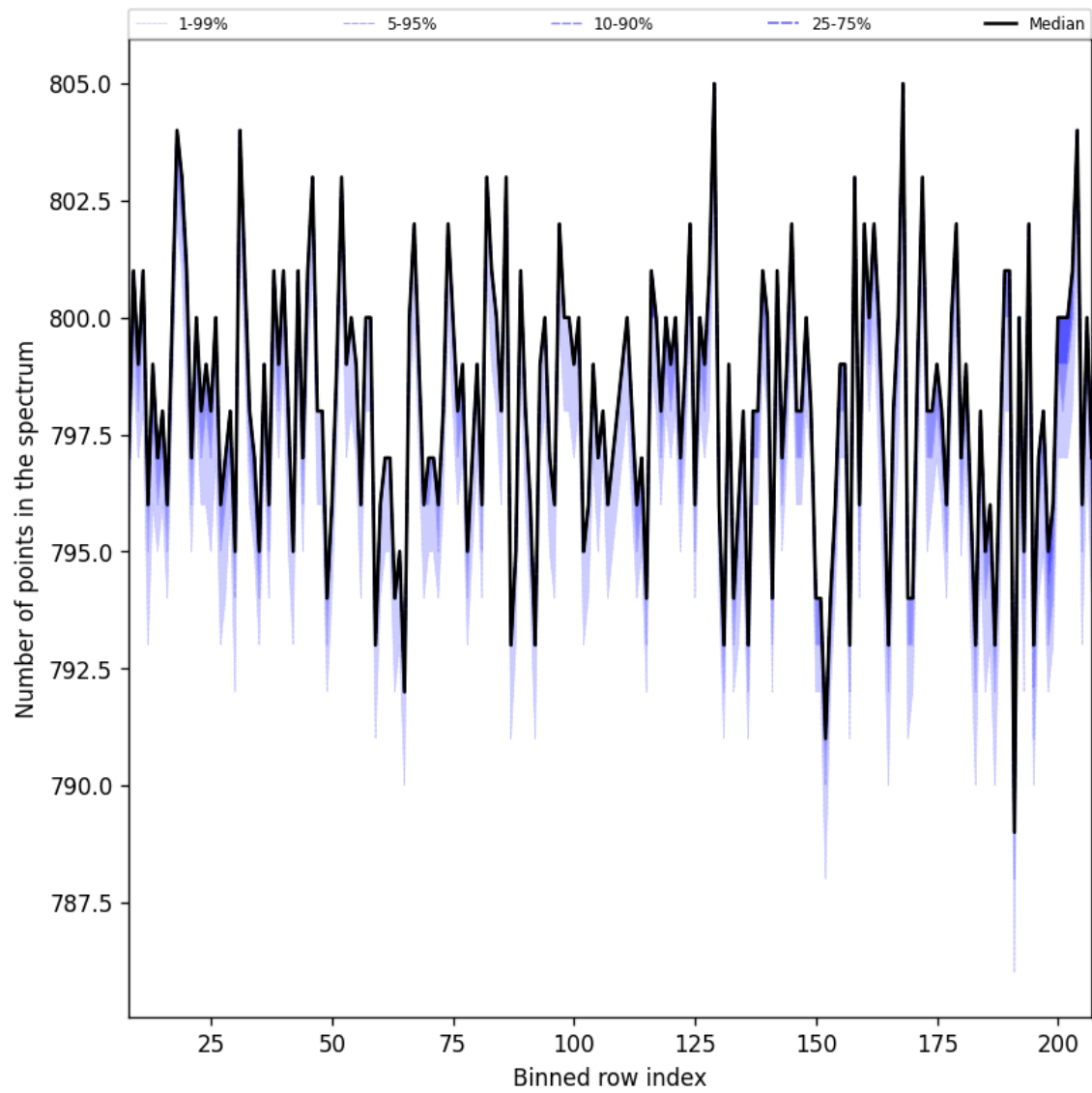
Figure 37: Along track statistics of “Number of points in the spectrum” for 2025-07-20 to 2025-07-22
