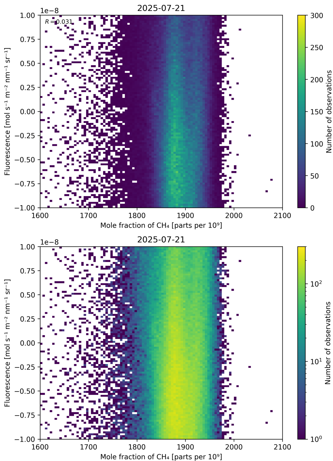
Figure 73: Scatter density plot of “Mole fraction of \text{CH}_4 ” against “Fluorescence” for 2025-07-20 to 2025-07-22.
