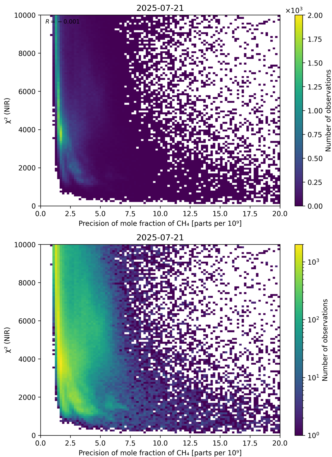
Figure 78: Scatter density plot of “Precision of mole fraction of \text{CH}_4 ” against “ \chi^2 (NIR)” for 2025-07-20 to 2025-07-22.
