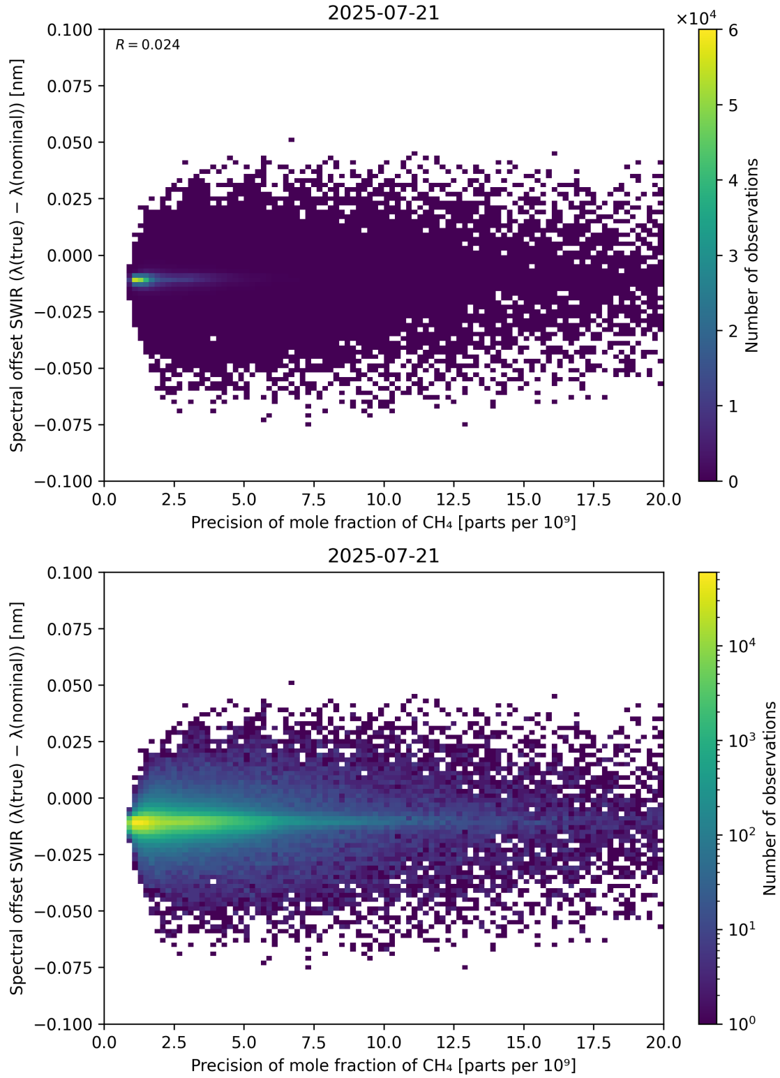
Figure 85: Scatter density plot of “Precision of mole fraction of CH 4 ” against “Spectral offset SWIR ( \lambda_{\text{true}} - \lambda_{\text{nominal}} )” for 2025-07-20 to 2025-07-22.
