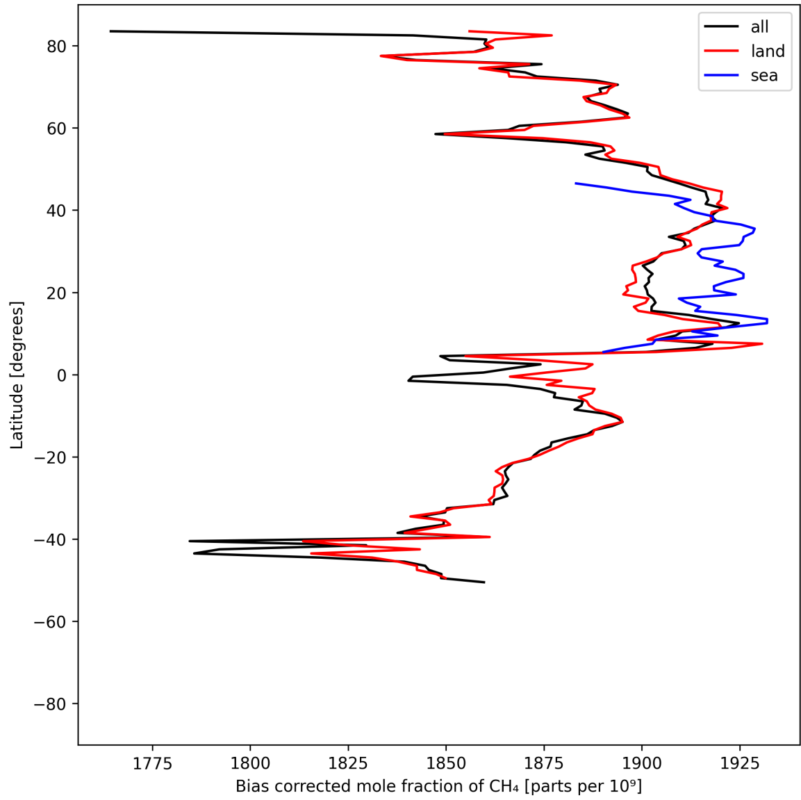
Figure 14: Zonal average of “Bias corrected mole fraction of CH 4 ” for 2025-07-20 to 2025-07-22.
