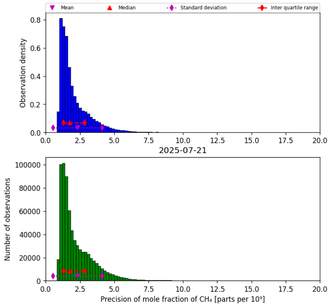
Figure 24: Histogram of “Precision of mole fraction of CH 4 ” for 2025-07-20 to 2025-07-22
