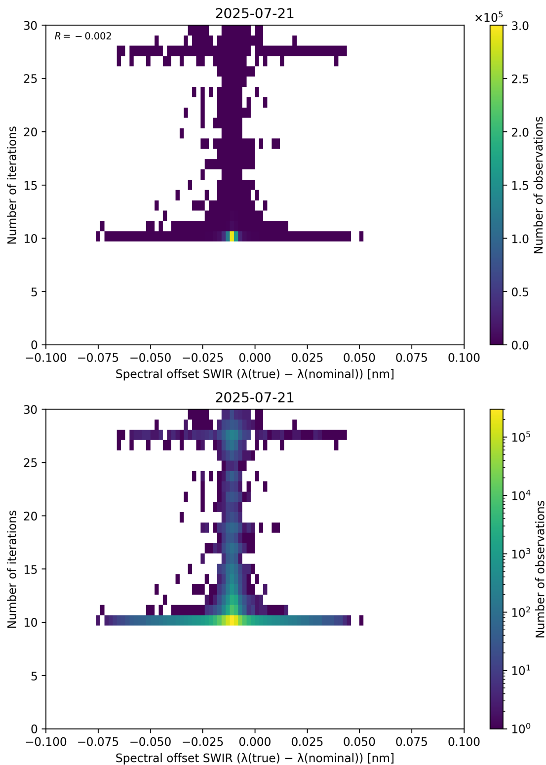
Figure 121: Scatter density plot of “Spectral offset SWIR ( \lambda_{\text{true}} - \lambda_{\text{nominal}} )” against “Number of iterations” for 2025-07-20 to 2025-07-22.
