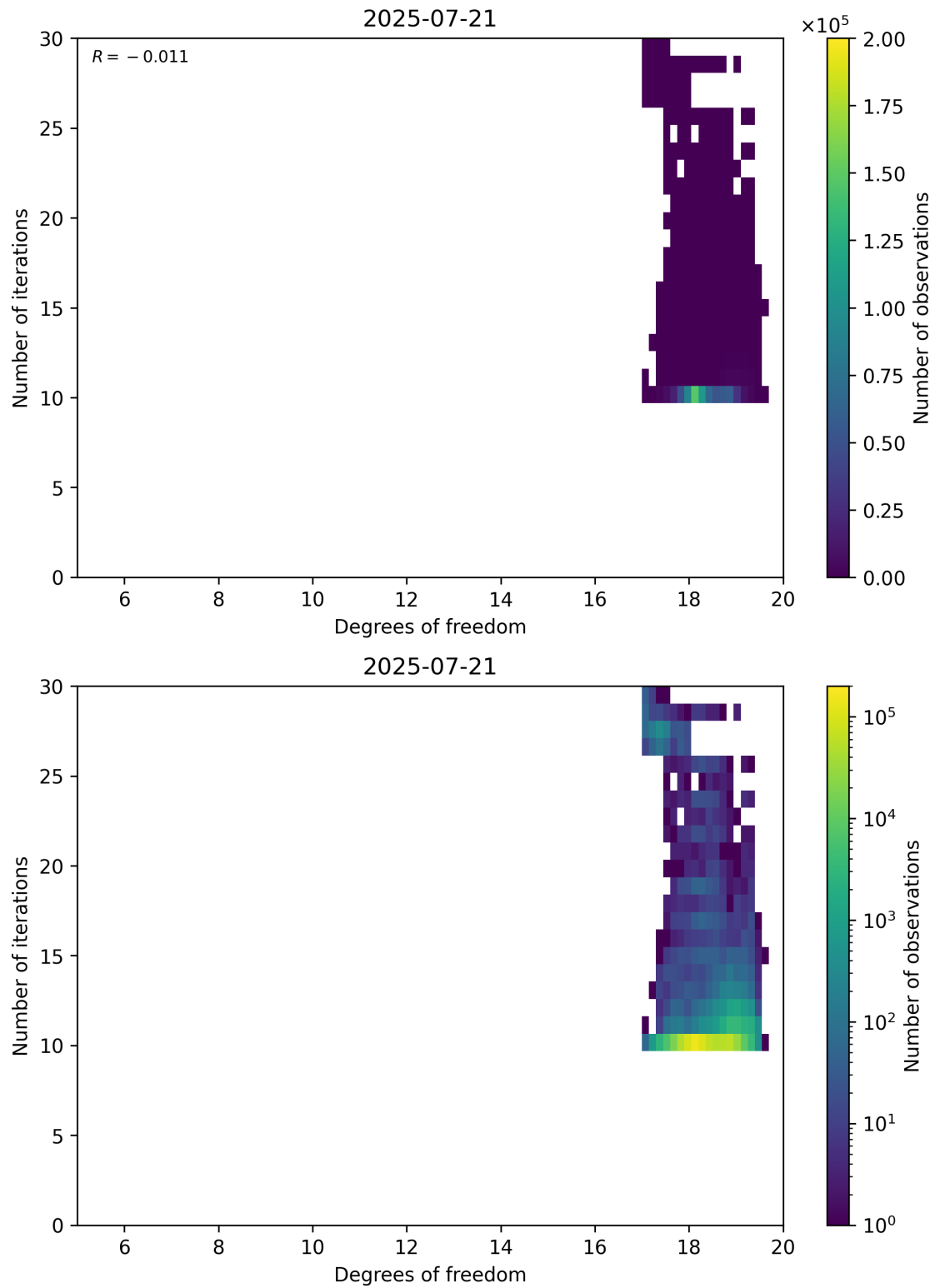
Figure 52: Scatter density plot of “Degrees of freedom” against “Number of iterations” for 2025-07-20 to 2025-07-22.
