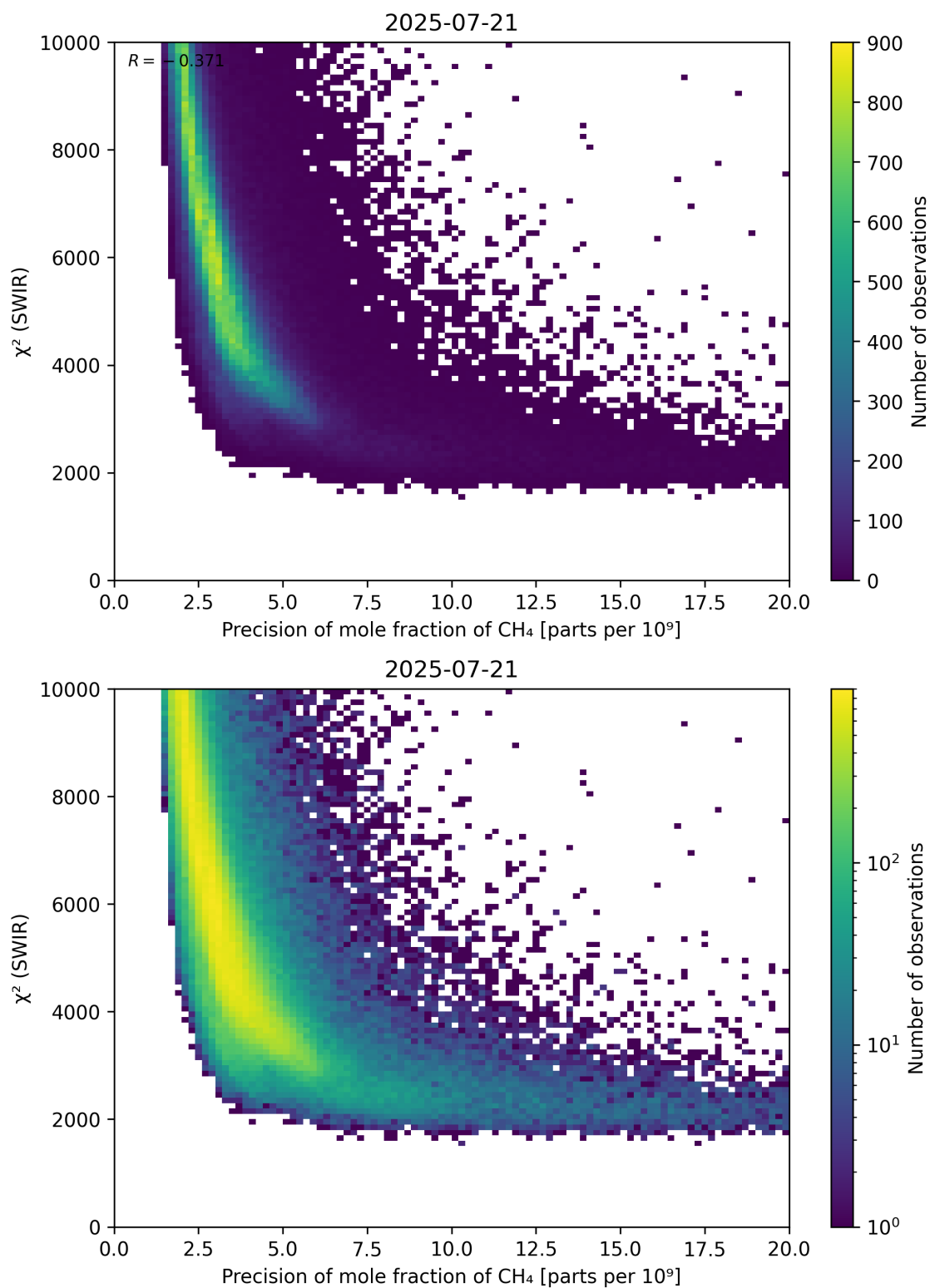
Figure 79: Scatter density plot of “Precision of mole fraction of \text{CH}_4 ” against “ \chi^2 (SWIR)” for 2025-07-20 to 2025-07-22.
