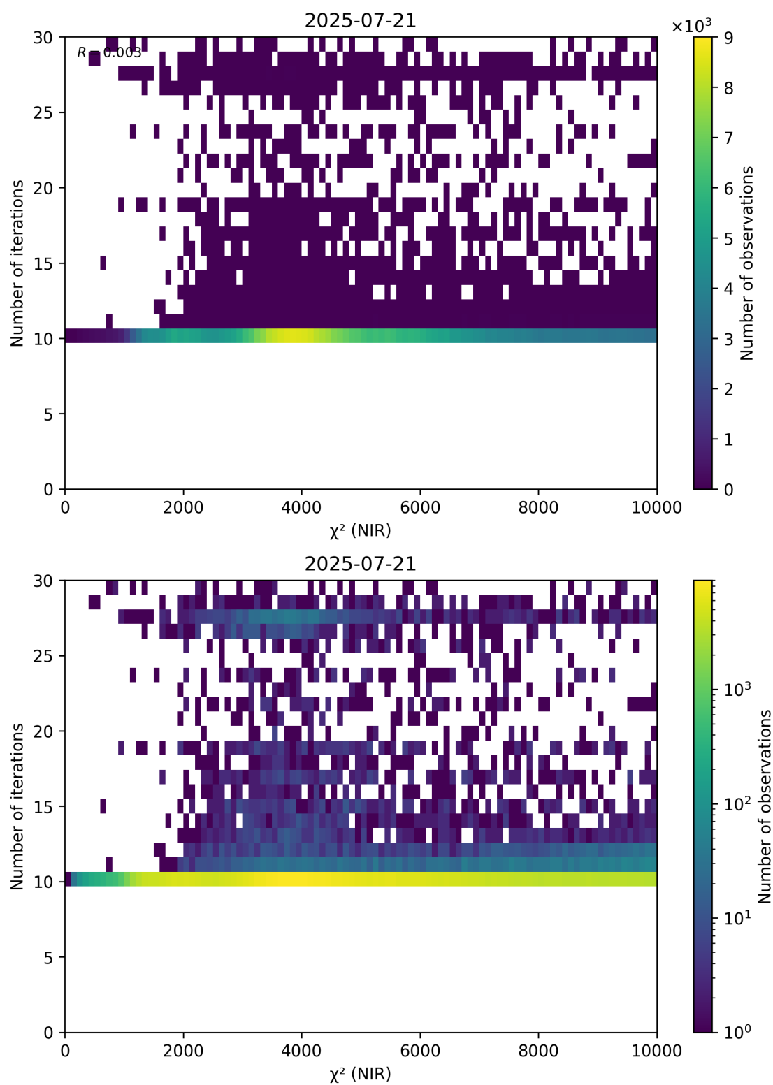
Figure 46: Scatter density plot of “ \chi^2 (NIR)” against “Number of iterations” for 2025-07-20 to 2025-07-22.
