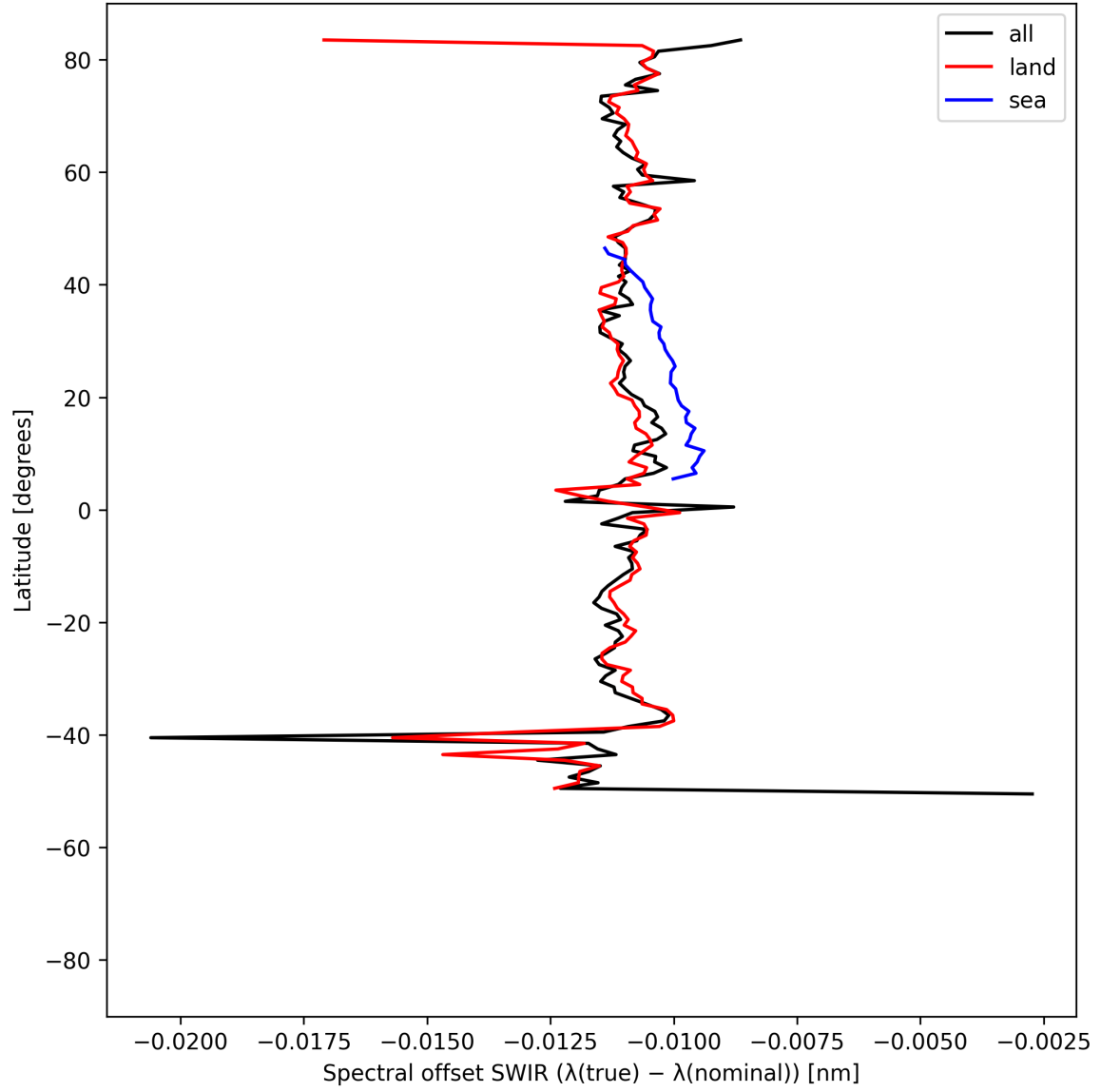
Figure 16: Zonal average of “Spectral offset SWIR ( \lambda_{\text{true}} - \lambda_{\text{nominal}} )” for 2025-07-20 to 2025-07-22.
