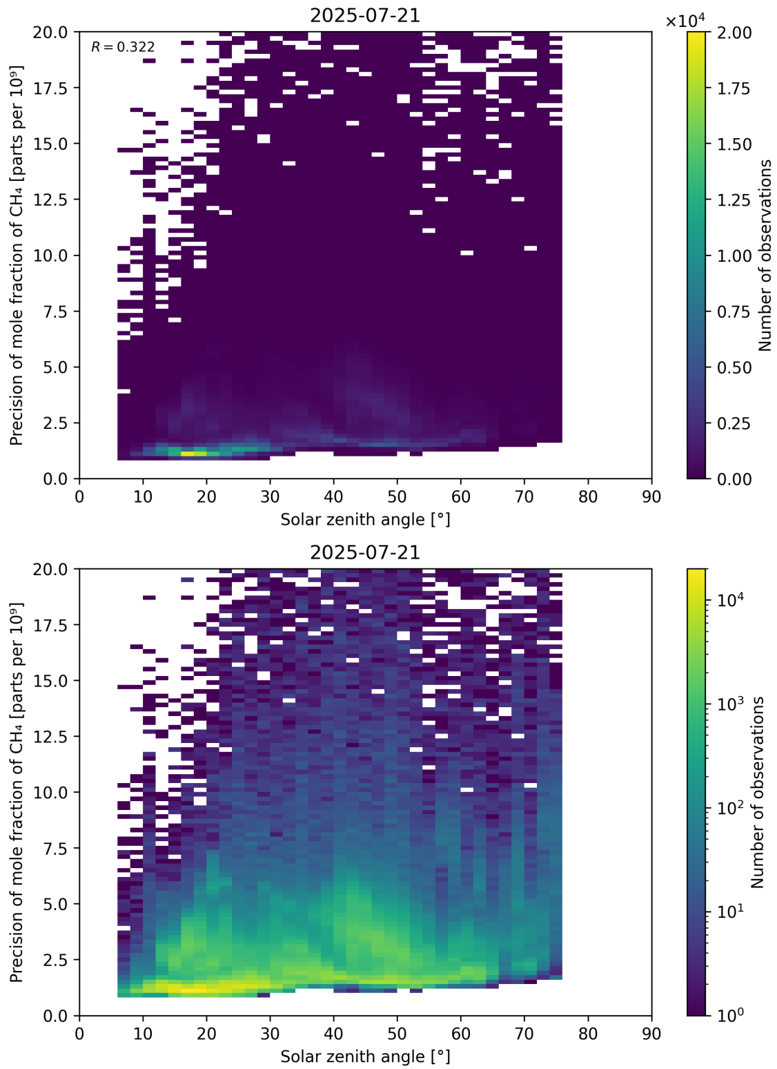
Figure 101: Scatter density plot of “Solar zenith angle” against “Precision of mole fraction of \text{CH}_4 ” for 2025-07-20 to 2025-07-22.
