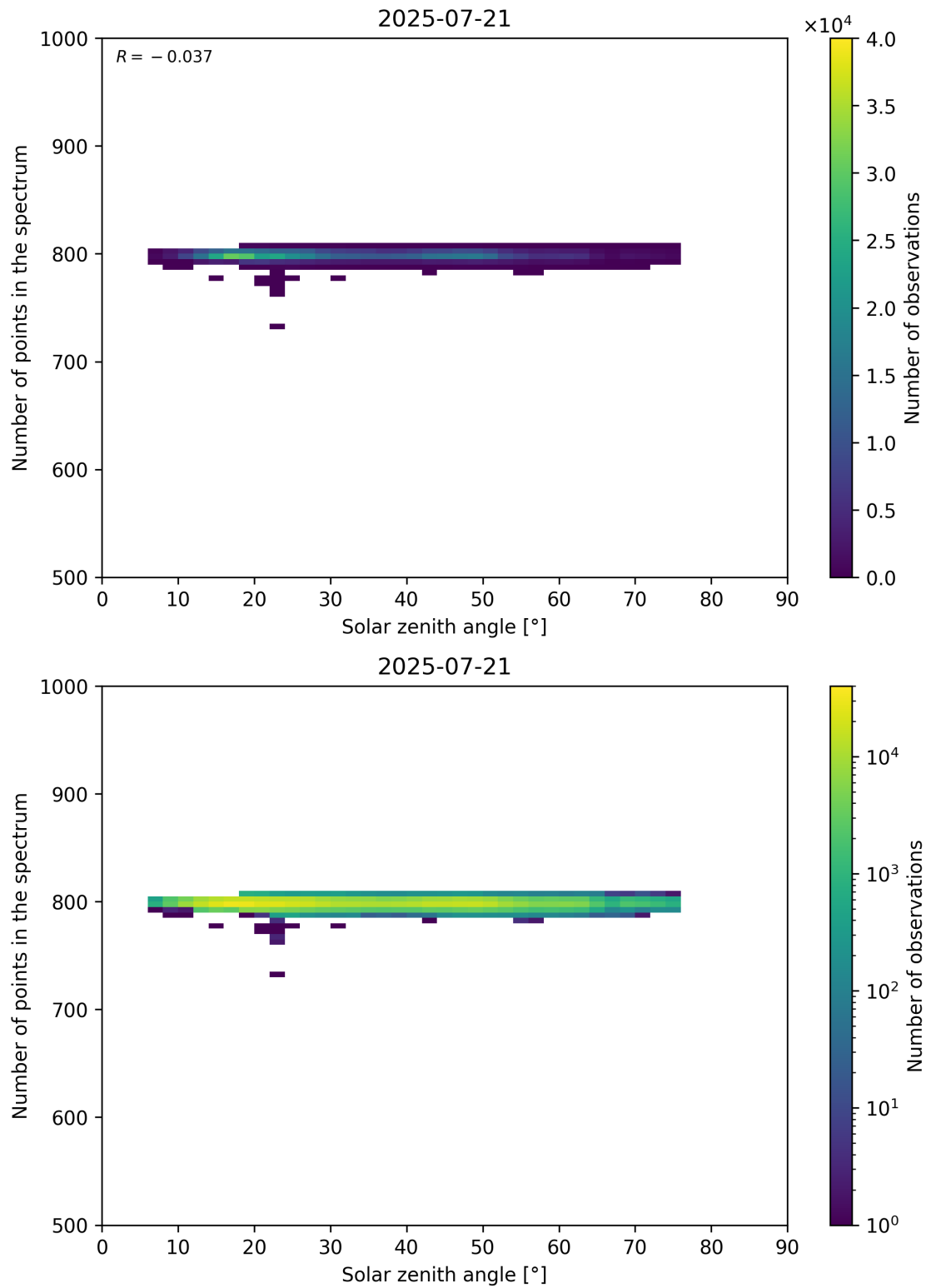
Figure 103: Scatter density plot of “Solar zenith angle” against “Number of points in the spectrum” for 2025-07-20 to 2025-07-22.
