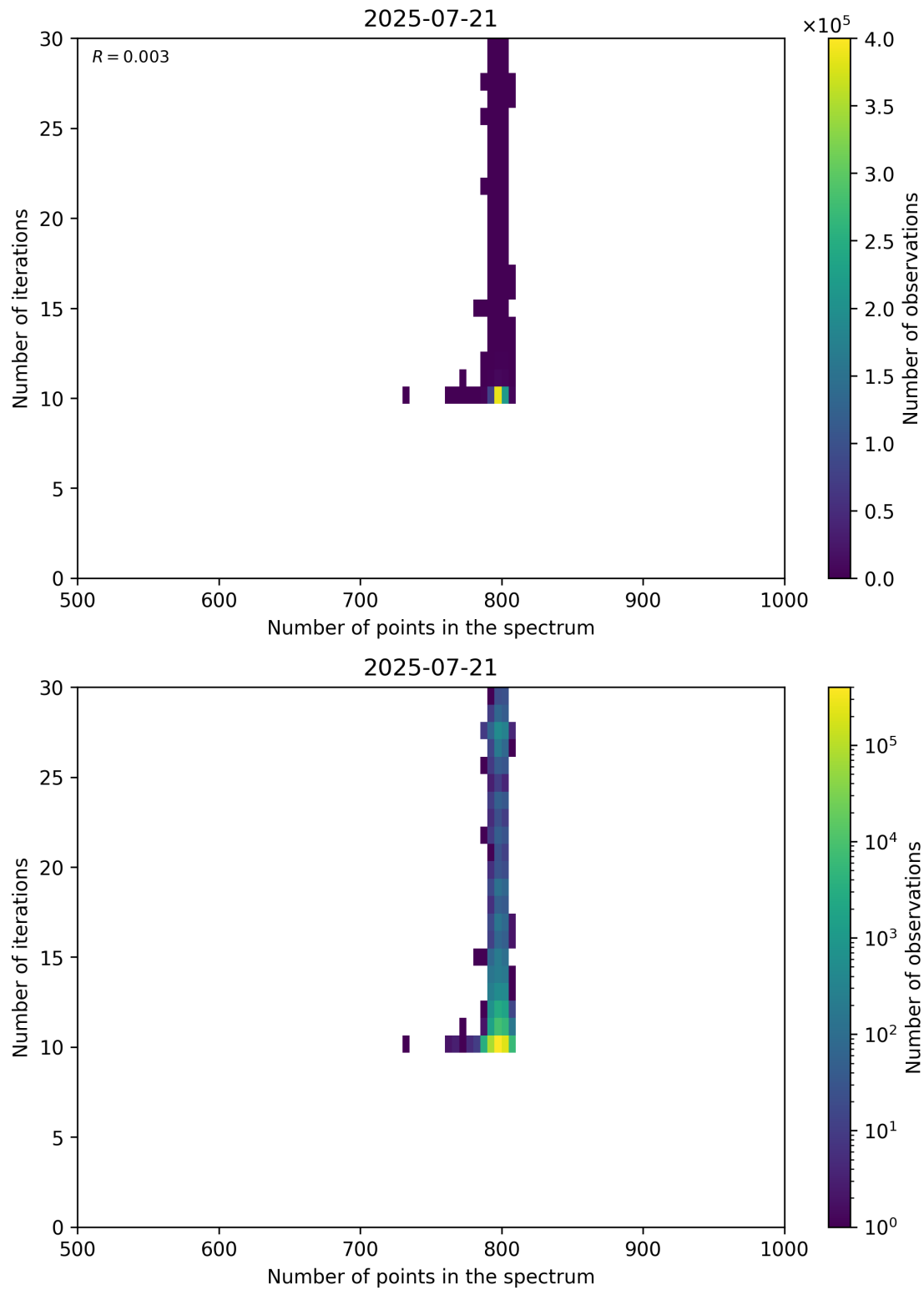
Figure 92: Scatter density plot of “Number of points in the spectrum” against “Number of iterations” for 2025-07-20 to 2025-07-22.
