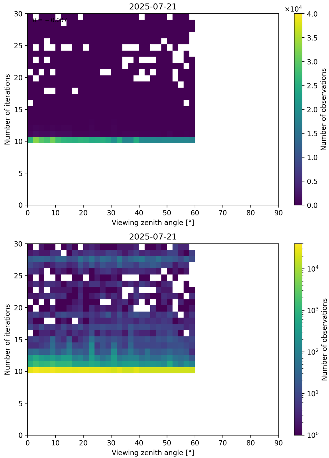
Figure 113: Scatter density plot of “Viewing zenith angle” against “Number of iterations” for 2025-07-20 to 2025-07-22.
