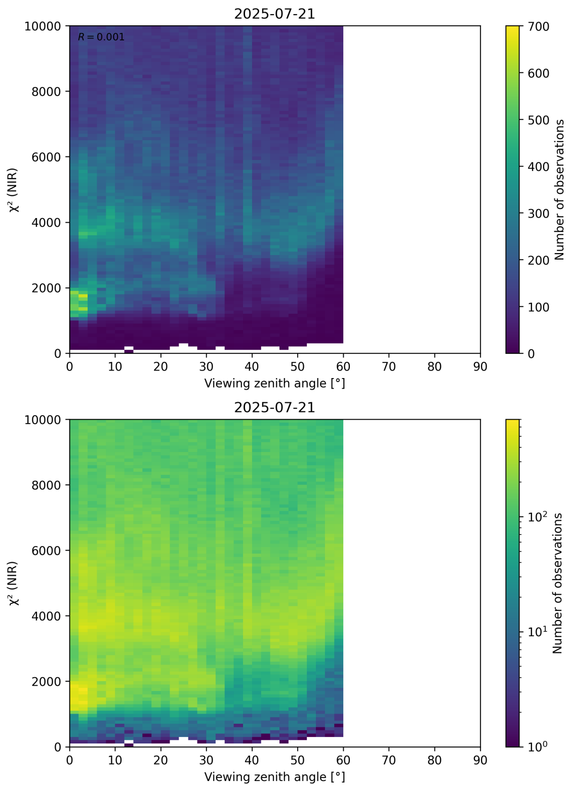
Figure 105: Scatter density plot of “Viewing zenith angle” against “ \chi^2 (NIR)” for 2025-07-20 to 2025-07-22.
