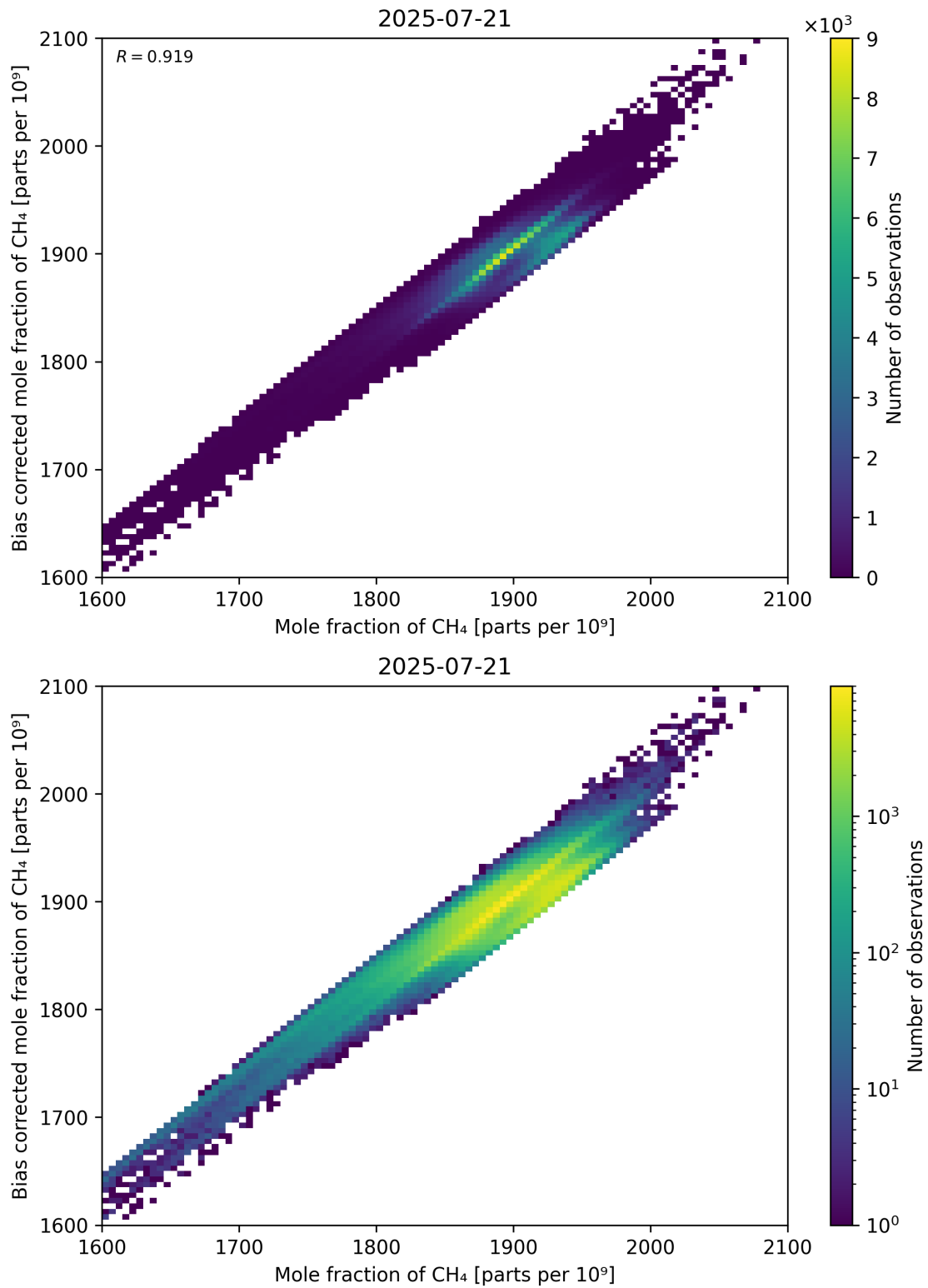
Figure 74: Scatter density plot of “Mole fraction of CH 4 ” against “Bias corrected mole fraction of CH 4 ” for 2025-07-20 to 2025-07-22.
