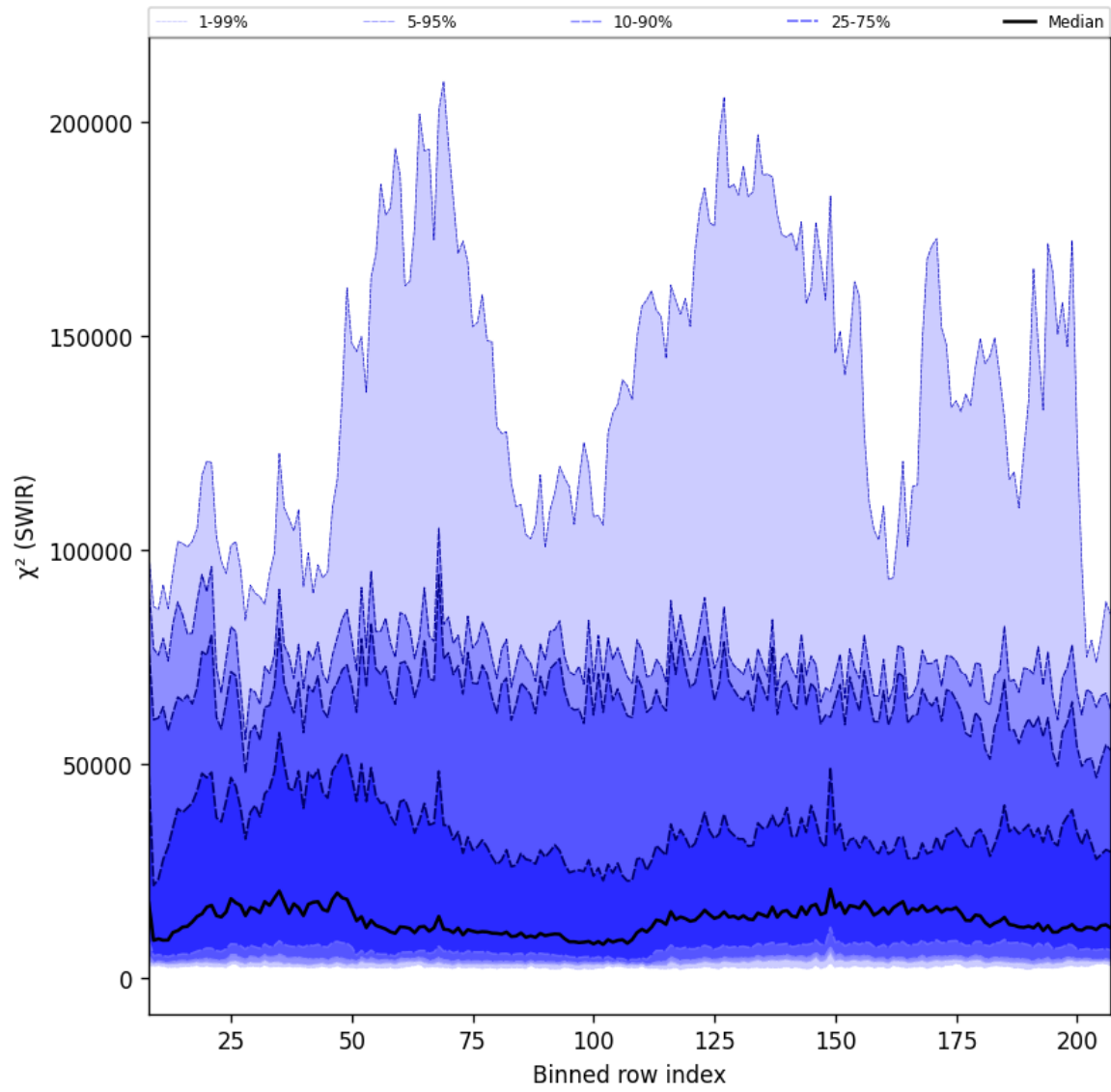
Figure 39: Along track statistics of “ \chi^2 (SWIR)” for 2025-07-20 to 2025-07-22
