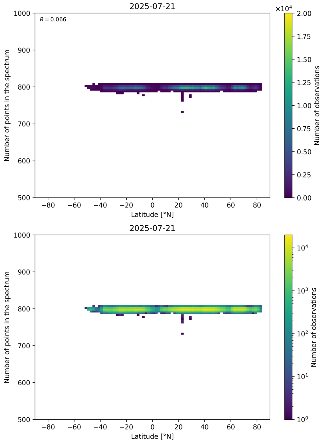
Figure 61: Scatter density plot of “Latitude” against “Number of points in the spectrum” for 2025-07-20 to 2025-07-22.
