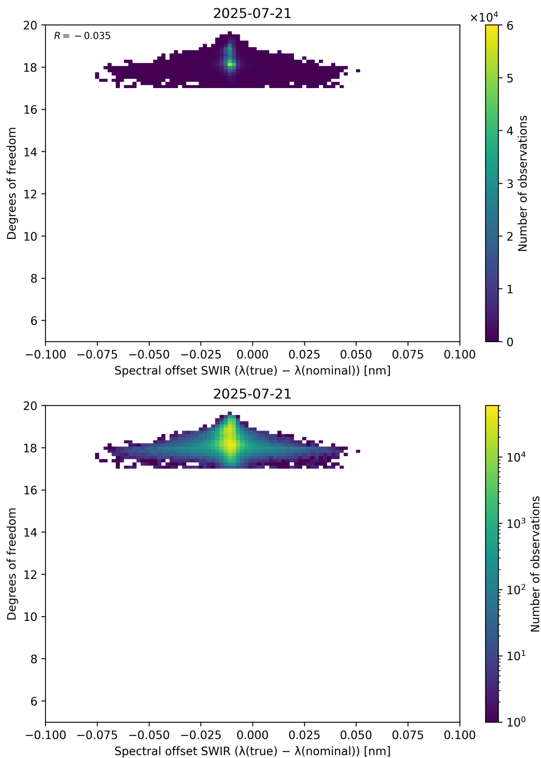
Figure 119: Scatter density plot of “Spectral offset SWIR ( \lambda_{\text{true}} - \lambda_{\text{nominal}} )” against “Degrees of freedom” for 2025-07-20 to 2025-07-22.
