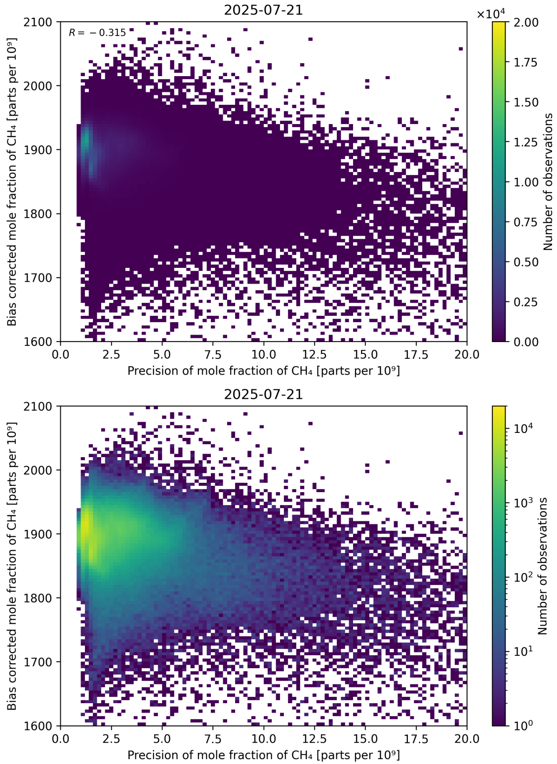
Figure 82: Scatter density plot of “Precision of mole fraction of CH 4 ” against “Bias corrected mole fraction of CH 4 ” for 2025-07-20 to 2025-07-22.
