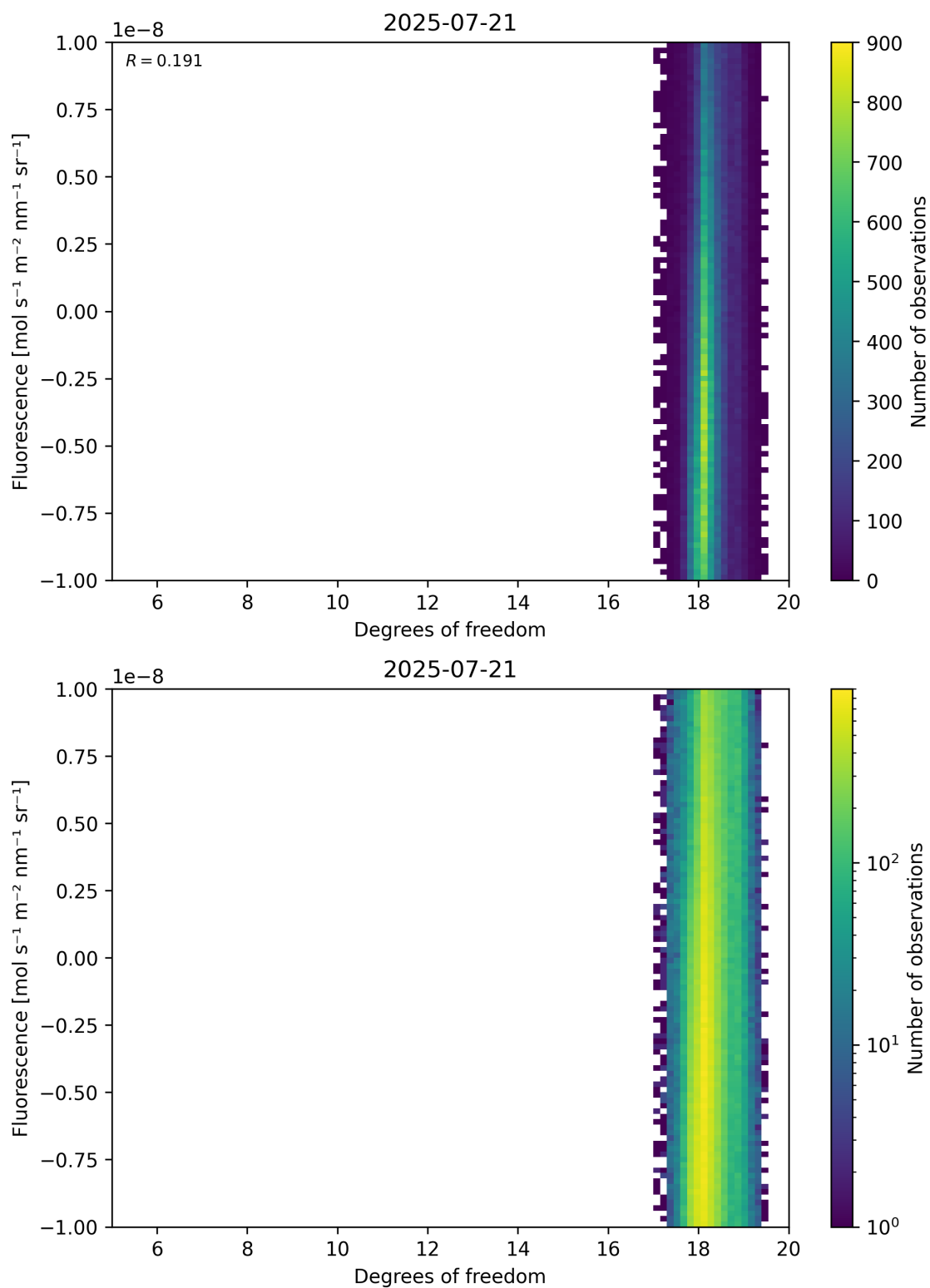
Figure 51: Scatter density plot of “Degrees of freedom” against “Fluorescence” for 2025-07-20 to 2025-07-22.
