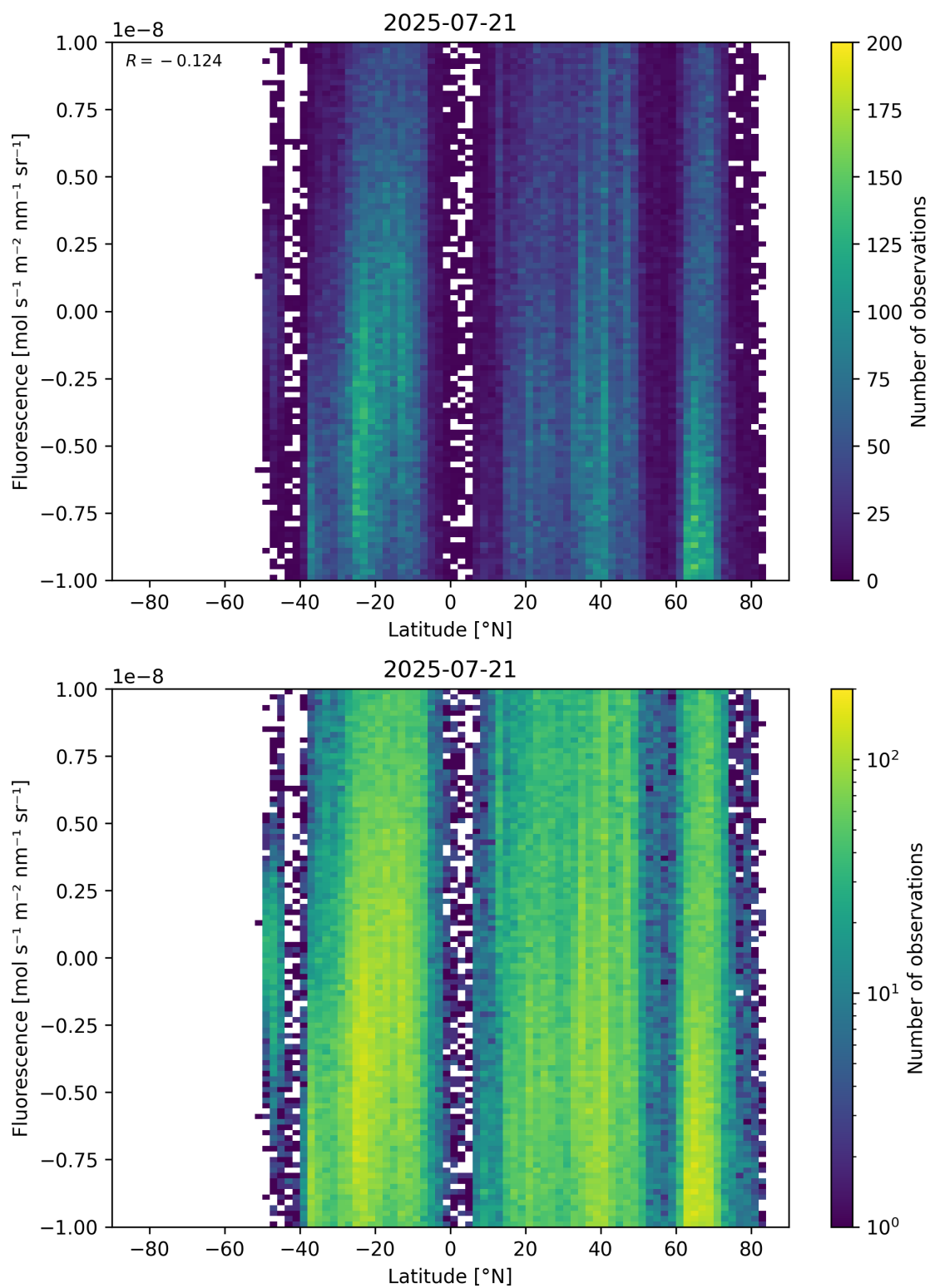
Figure 56: Scatter density plot of “Latitude” against “Fluorescence” for 2025-07-20 to 2025-07-22.
