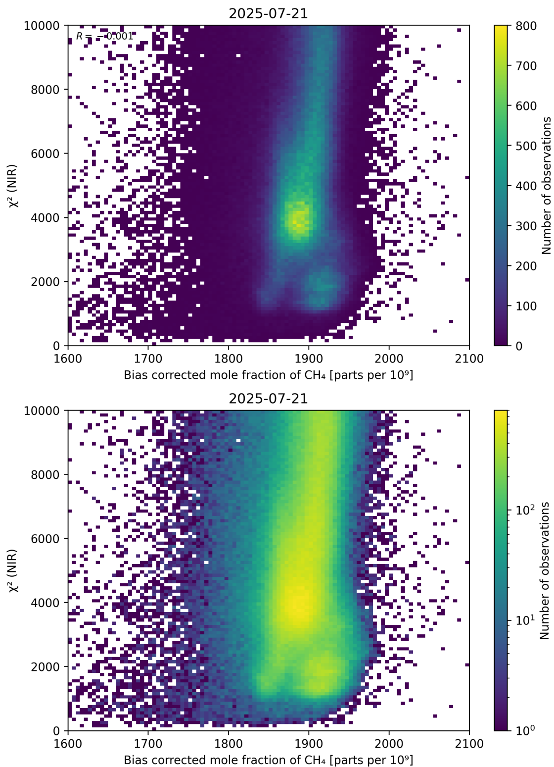
Figure 63: Scatter density plot of “Bias corrected mole fraction of \text{CH}_4 ” against “ \chi^2 (NIR)” for 2025-07-20 to 2025-07-22.
