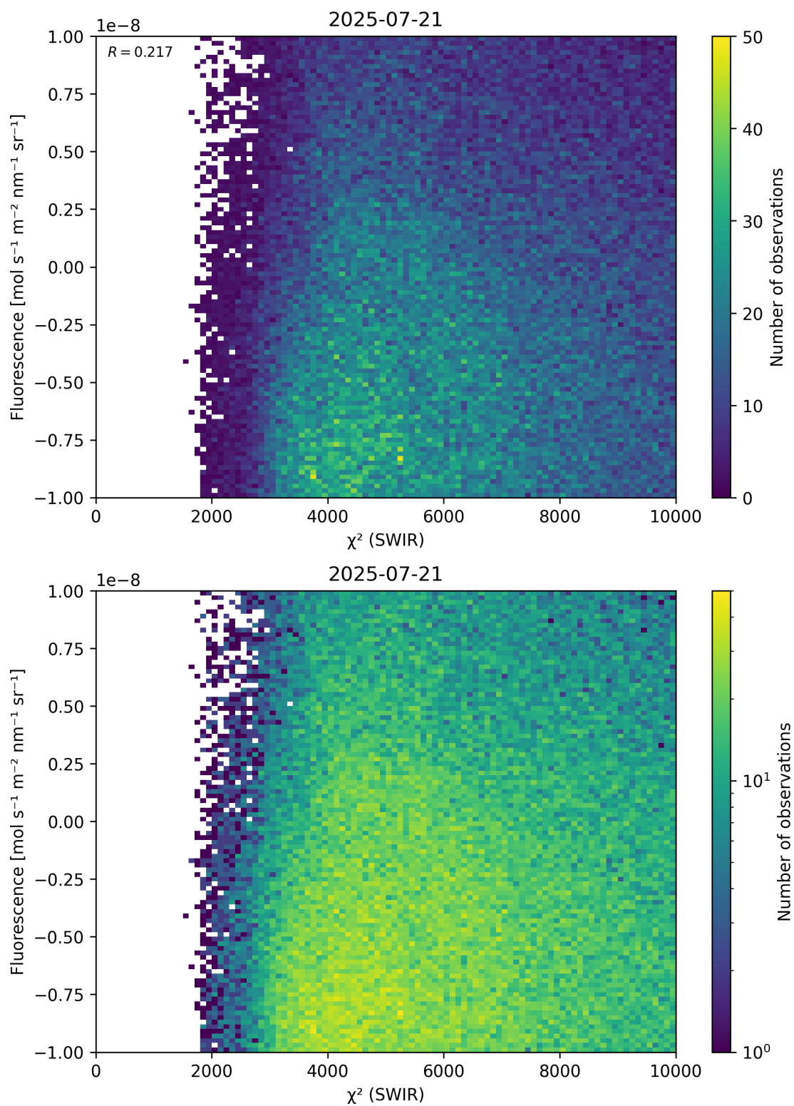
Figure 49: Scatter density plot of “ \chi^2 (SWIR)” against “Fluorescence” for 2025-07-20 to 2025-07-22.
