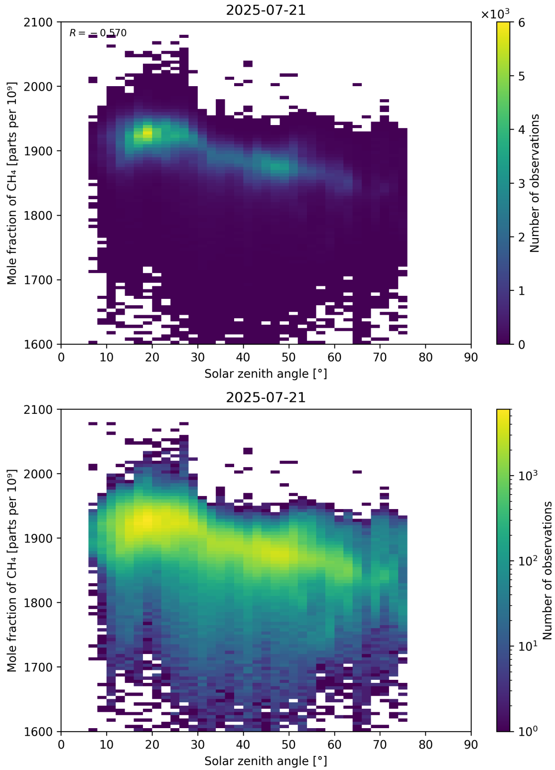
Figure 99: Scatter density plot of “Solar zenith angle” against “Mole fraction of \text{CH}_4 ” for 2025-07-20 to 2025-07-22.
