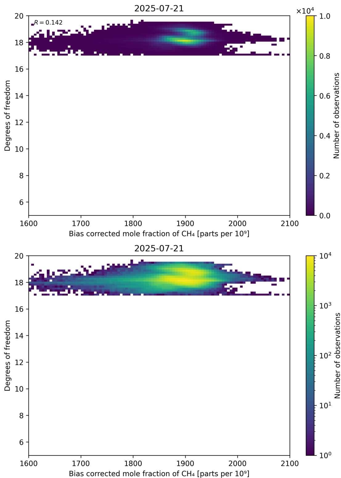
Figure 65: Scatter density plot of “Bias corrected mole fraction of CH 4 ” against “Degrees of freedom” for 2025-07-20 to 2025-07-22.
