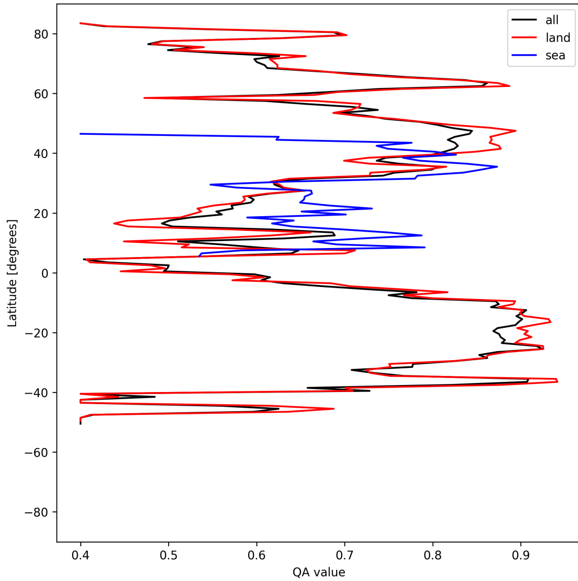
Figure 11: Zonal average of “QA value” for 2025-07-20 to 2025-07-22.
