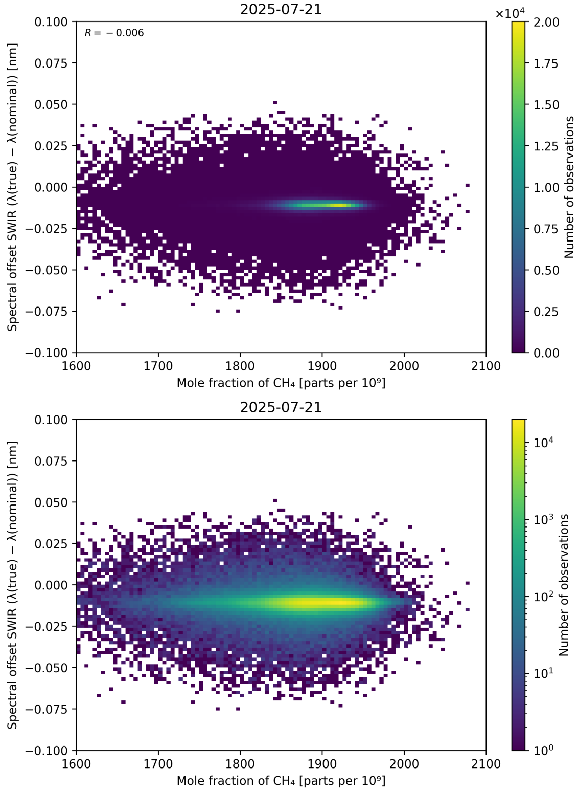
Figure 86: Scatter density plot of “Mole fraction of CH 4 ” against “Spectral offset SWIR ( \lambda_{\text{true}} - \lambda_{\text{nominal}} )” for 2025-07-20 to 2025-07-22.
