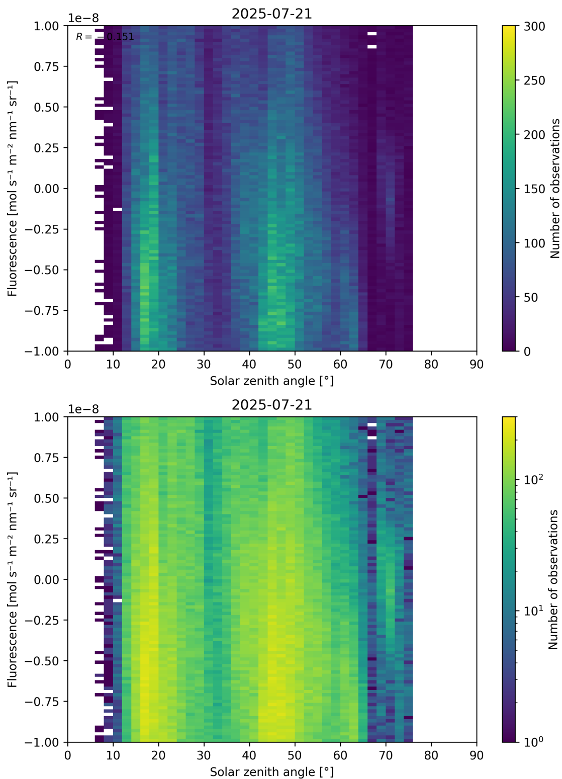
Figure 97: Scatter density plot of “Solar zenith angle” against “Fluorescence” for 2025-07-20 to 2025-07-22.
