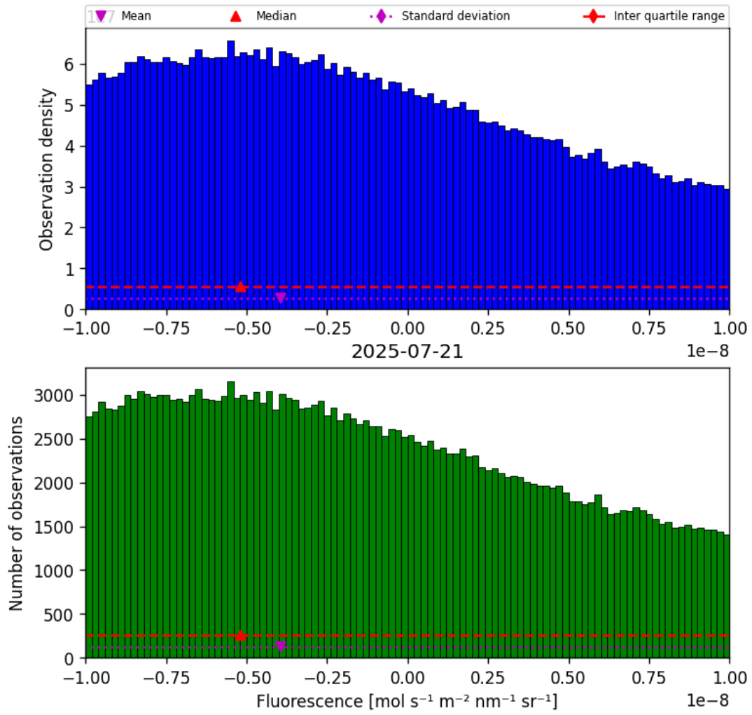
Figure 32: Histogram of “Fluorescence” for 2025-07-20 to 2025-07-22
