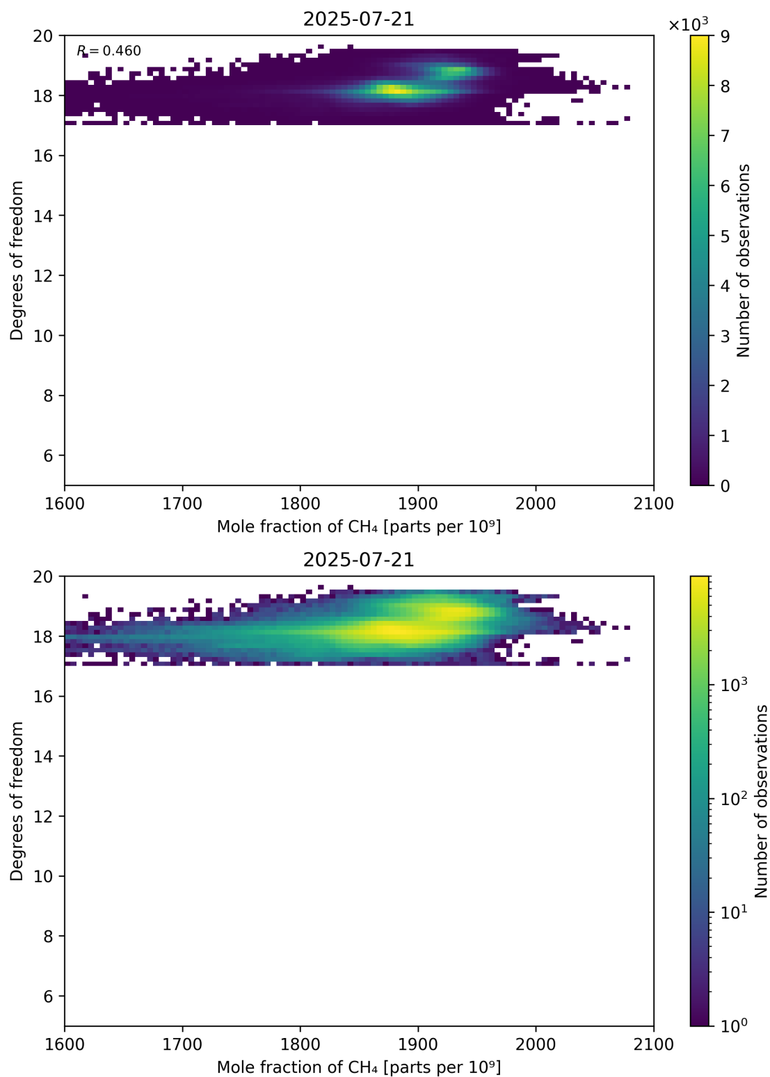
Figure 72: Scatter density plot of “Mole fraction of CH 4 ” against “Degrees of freedom” for 2025-07-20 to 2025-07-22.
