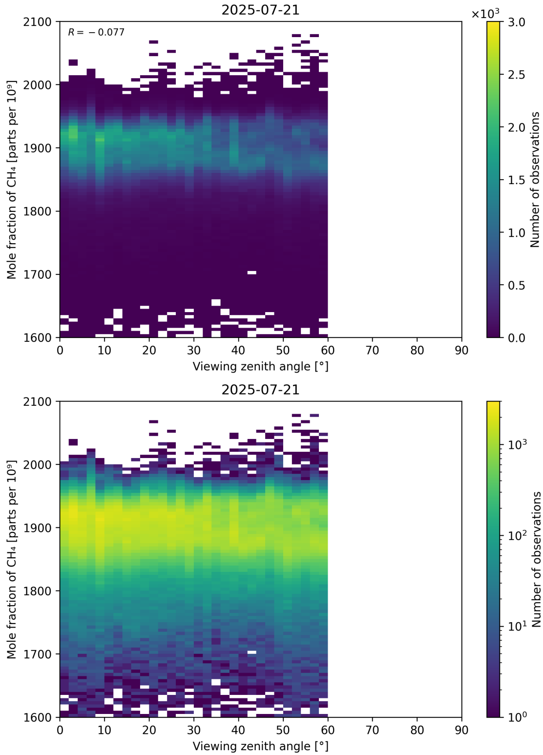
Figure 110: Scatter density plot of “Viewing zenith angle” against “Mole fraction of CH 4 ” for 2025-07-20 to 2025-07-22.
