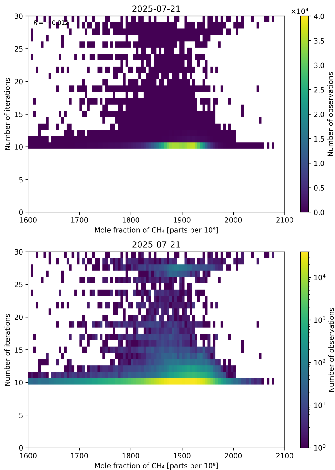
Figure 76: Scatter density plot of “Mole fraction of CH 4 ” against “Number of iterations” for 2025-07-20 to 2025-07-22.
