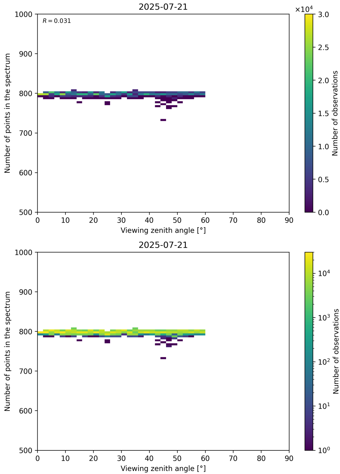
Figure 114: Scatter density plot of “Viewing zenith angle” against “Number of points in the spectrum” for 2025-07-20 to 2025-07-22.
