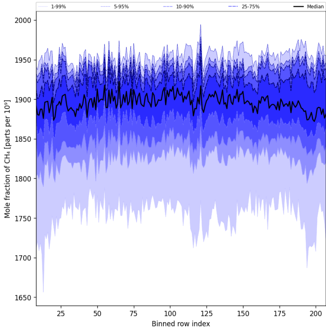
Figure 34: Along track statistics of “Mole fraction of CH 4 ” for 2025-07-20 to 2025-07-22
