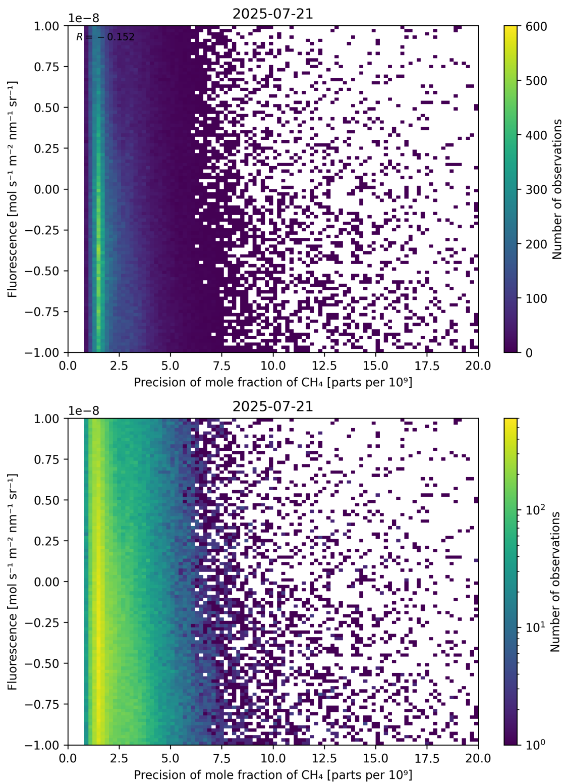
Figure 81: Scatter density plot of “Precision of mole fraction of \text{CH}_4 ” against “Fluorescence” for 2025-07-20 to 2025-07-22.
