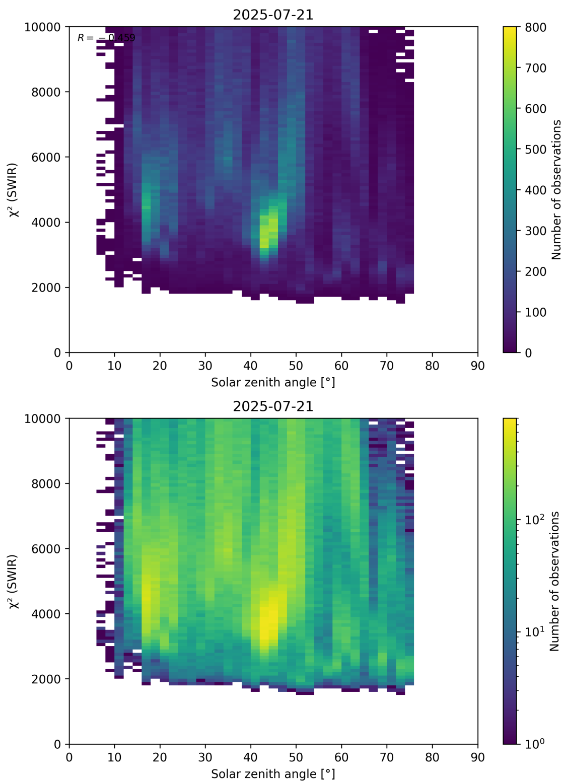
Figure 95: Scatter density plot of “Solar zenith angle” against “ \chi^2 (SWIR)” for 2025-07-20 to 2025-07-22.
