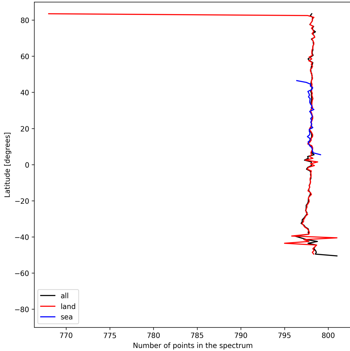
Figure 15: Zonal average of “Number of points in the spectrum” for 2025-07-20 to 2025-07-22.
