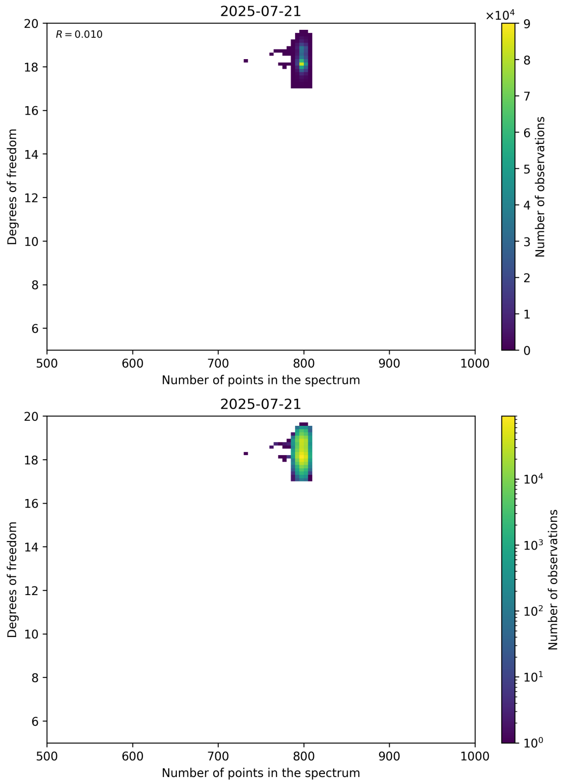
Figure 90: Scatter density plot of “Number of points in the spectrum” against “Degrees of freedom” for 2025-07-20 to 2025-07-22.
