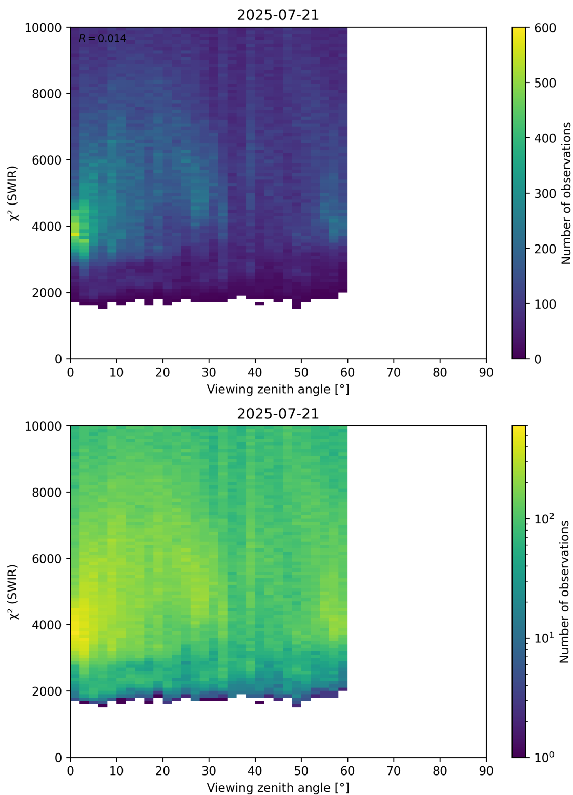
Figure 106: Scatter density plot of “Viewing zenith angle” against “ \chi^2 (SWIR)” for 2025-07-20 to 2025-07-22.
