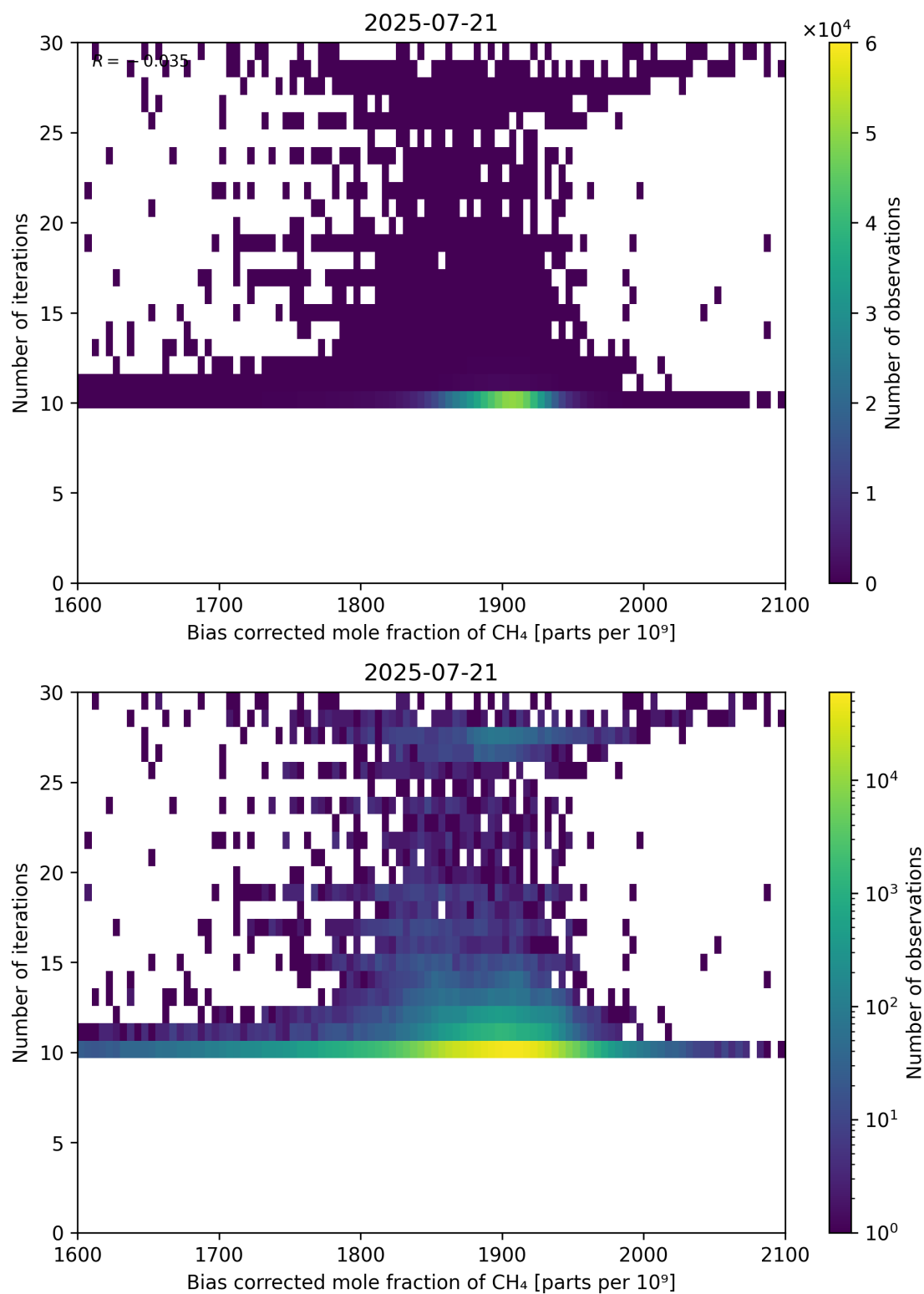
Figure 67: Scatter density plot of “Bias corrected mole fraction of CH 4 ” against “Number of iterations” for 2025-07-20 to 2025-07-22.
