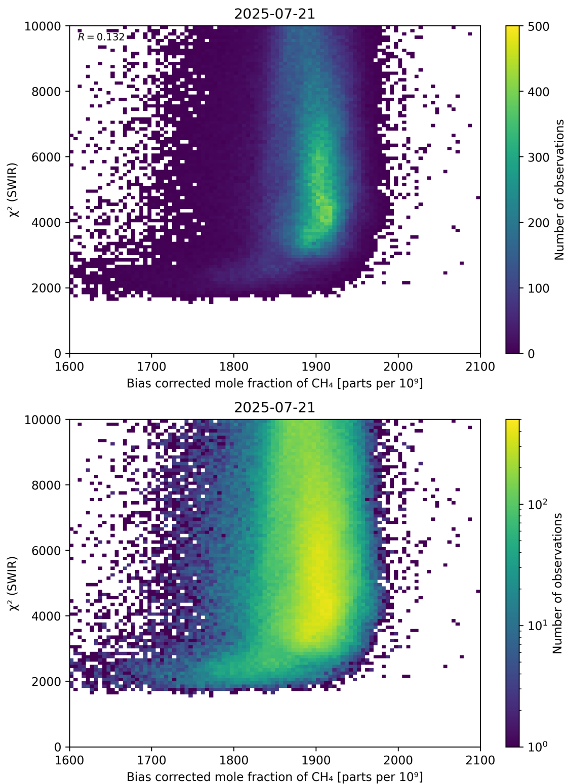
Figure 64: Scatter density plot of “Bias corrected mole fraction of \text{CH}_4 ” against “ \chi^2 (SWIR)” for 2025-07-20 to 2025-07-22.
