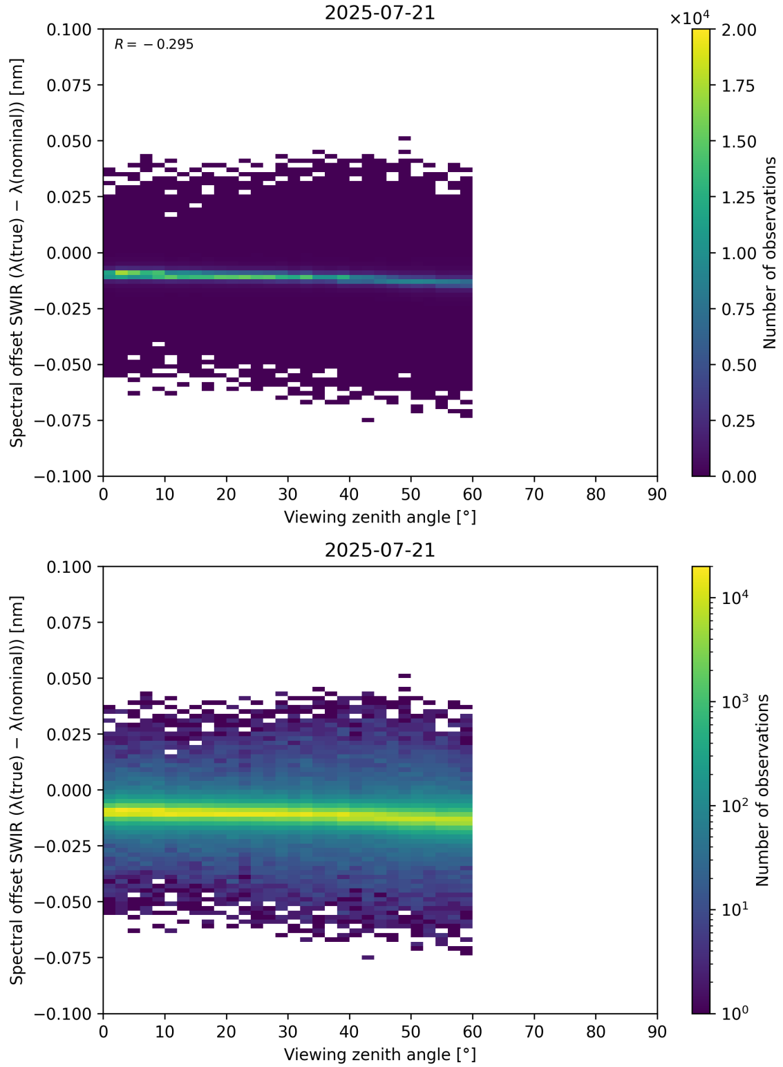
Figure 116: Scatter density plot of “Viewing zenith angle” against “Spectral offset SWIR ( \lambda_{\text{true}} - \lambda_{\text{nominal}} )” for 2025-07-20 to 2025-07-22.
