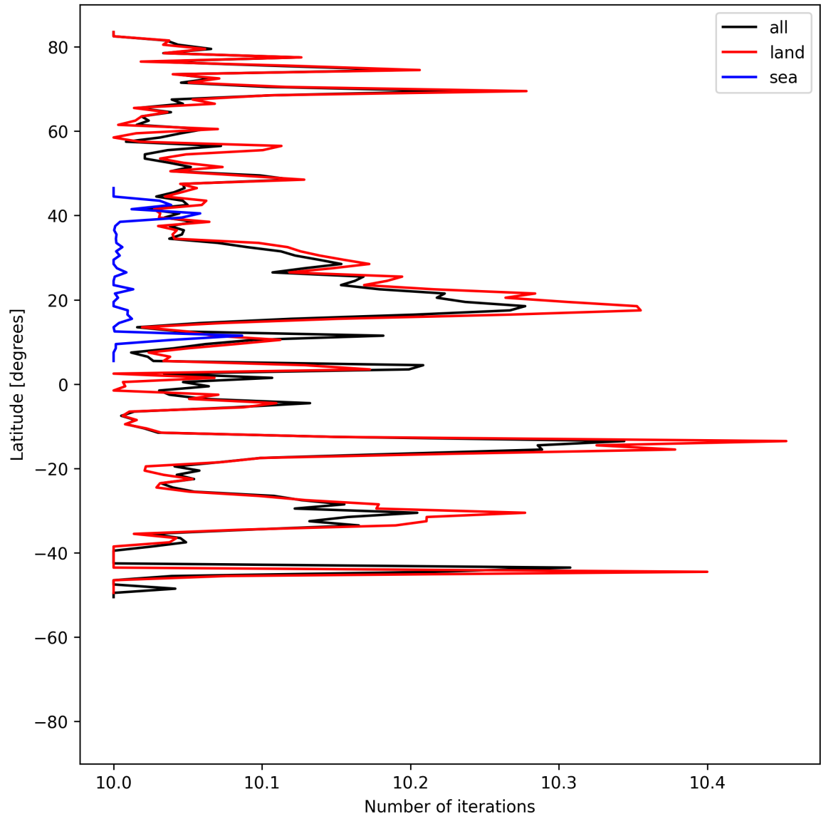
Figure 20: Zonal average of “Number of iterations” for 2025-07-20 to 2025-07-22.
