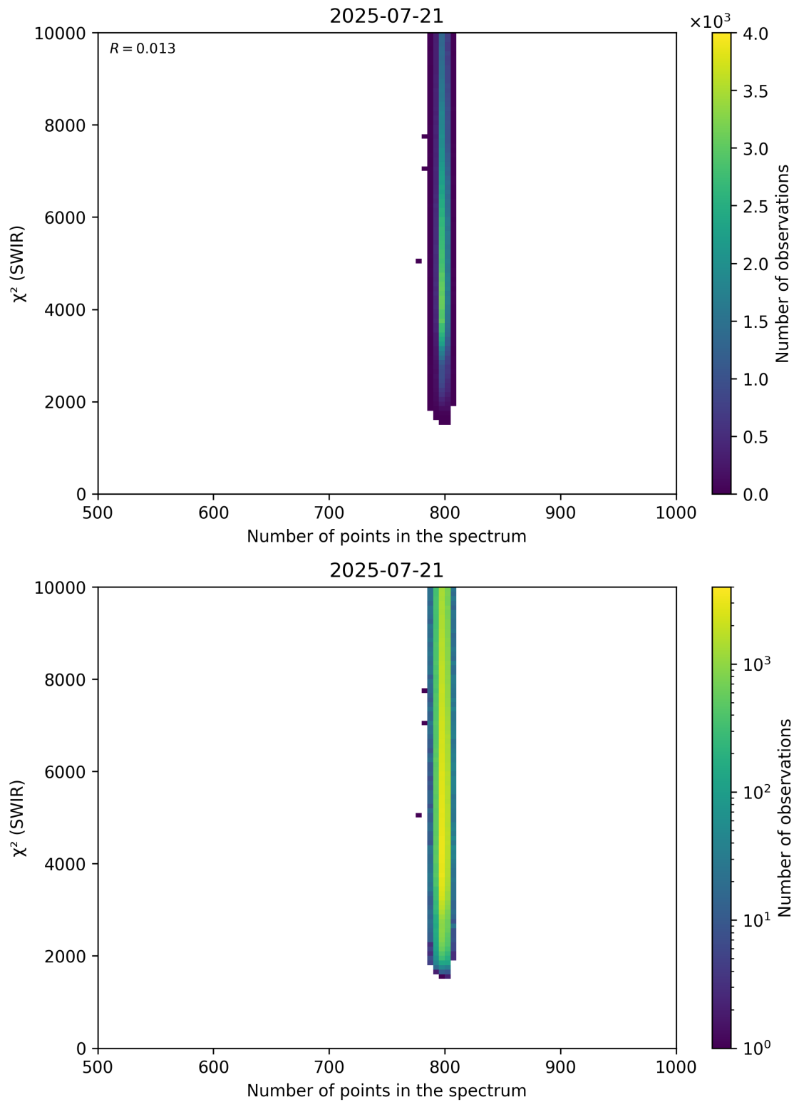
Figure 89: Scatter density plot of “Number of points in the spectrum” against “ \chi^2 (SWIR)” for 2025-07-20 to 2025-07-22.
