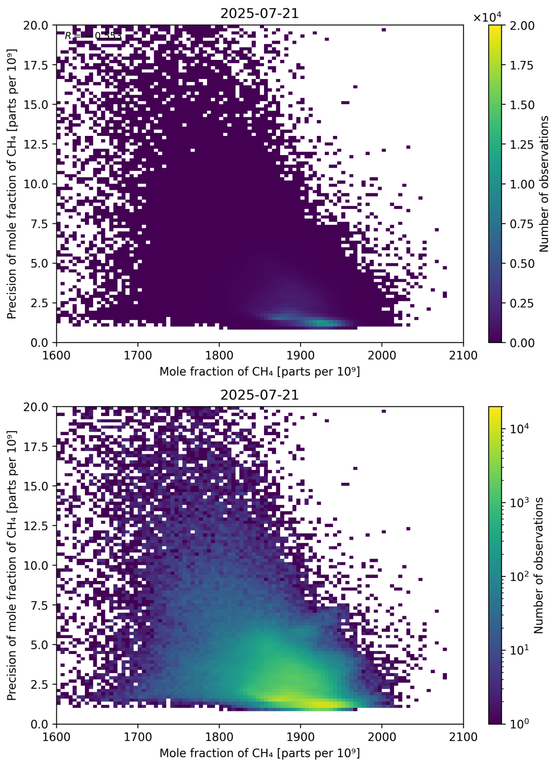
Figure 75: Scatter density plot of “Mole fraction of CH 4 ” against “Precision of mole fraction of CH 4 ” for 2025-07-20 to 2025-07-22.
