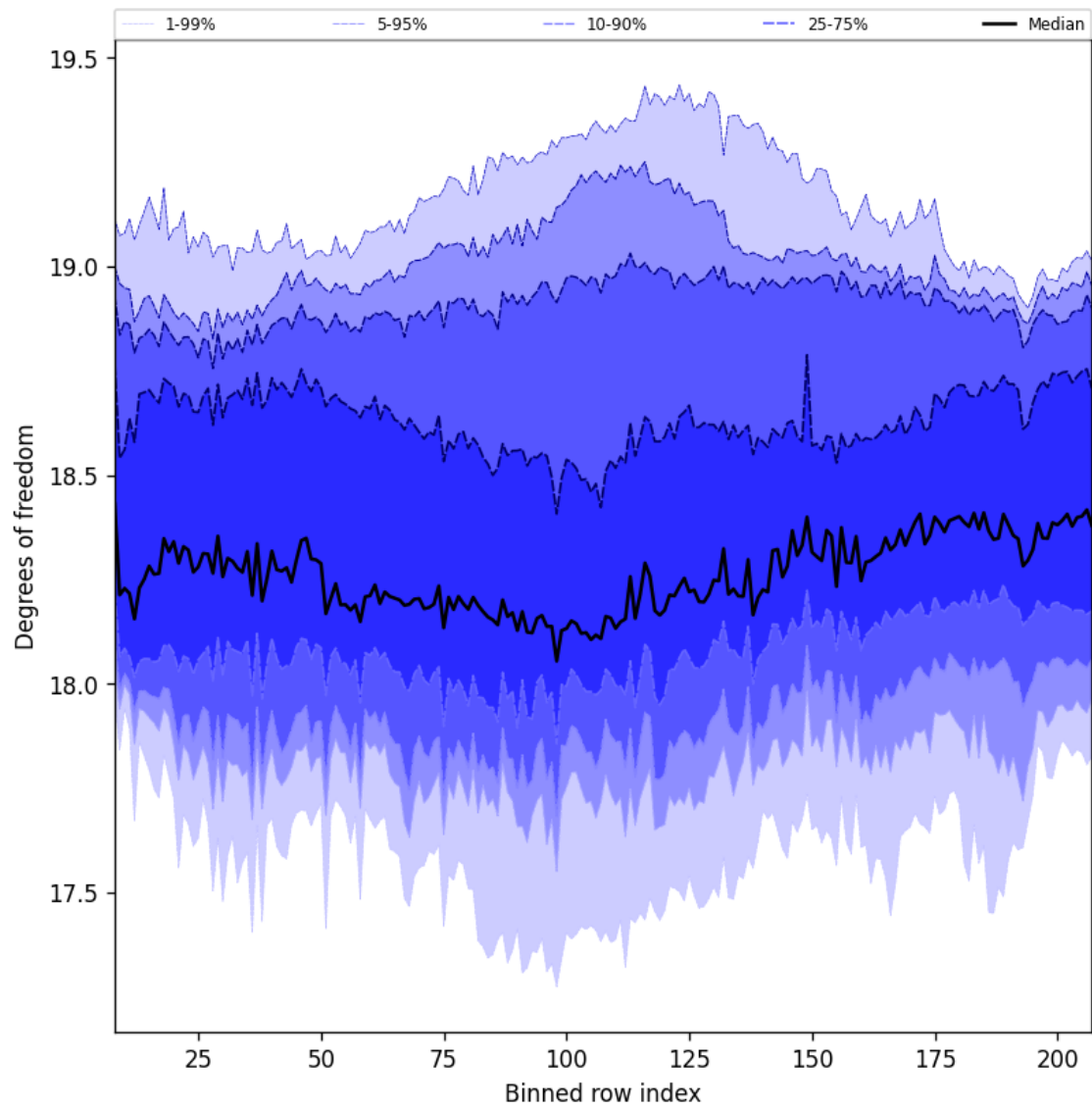
Figure 41: Along track statistics of “Degrees of freedom” for 2025-07-20 to 2025-07-22
