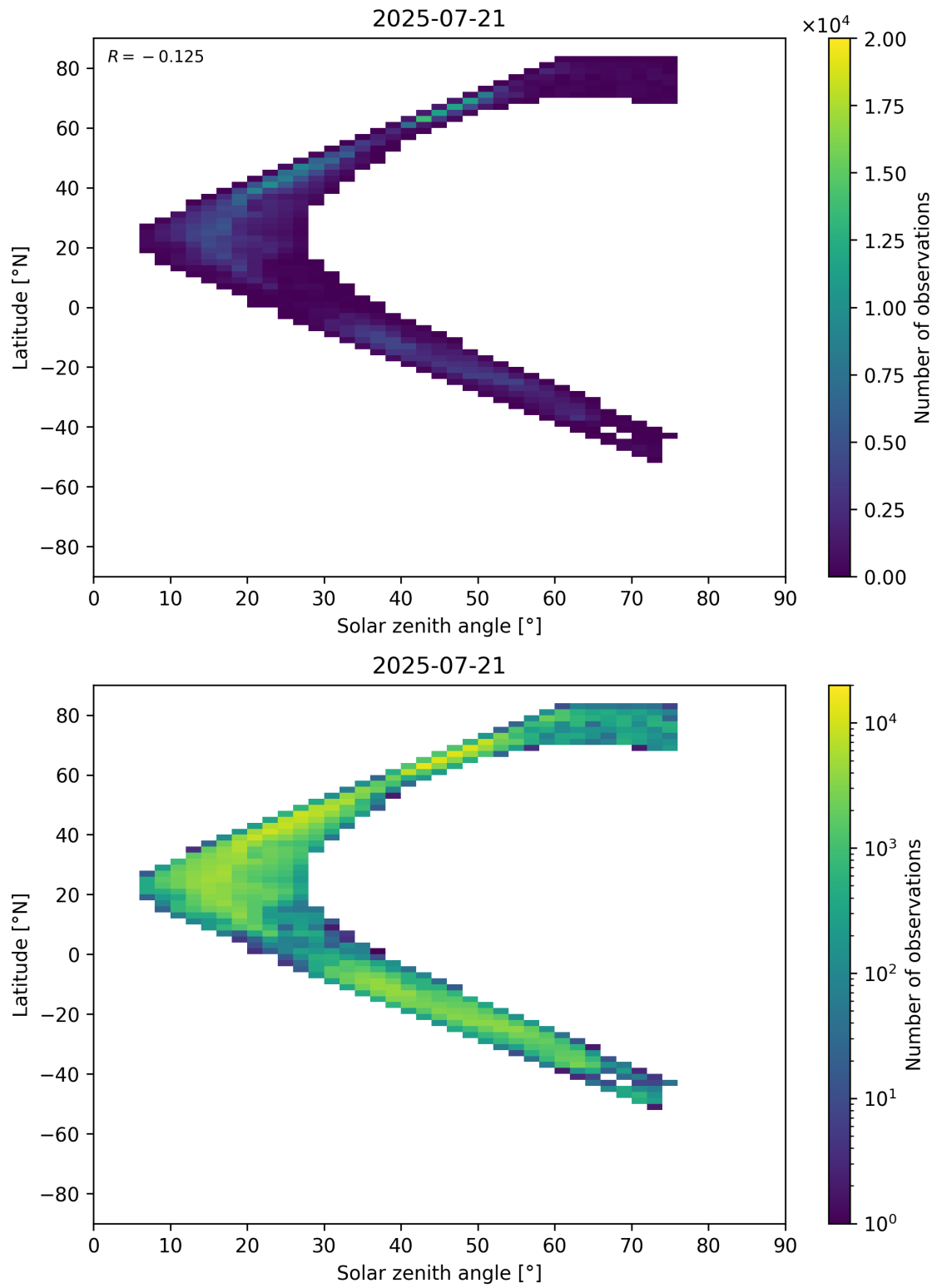
Figure 98: Scatter density plot of “Solar zenith angle” against “Latitude” for 2025-07-20 to 2025-07-22.
