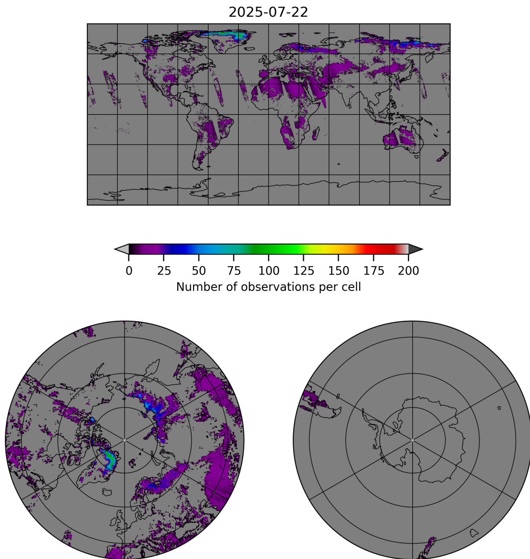
Figure 10: Map of the number of observations for 2025-07-21 to 2025-07-23
