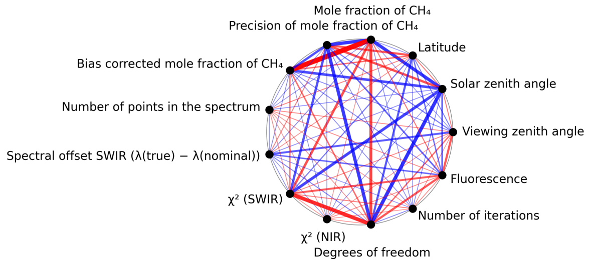
Figure 1: Map of correlation graph for 2025-07-21 to 2025-07-23.
