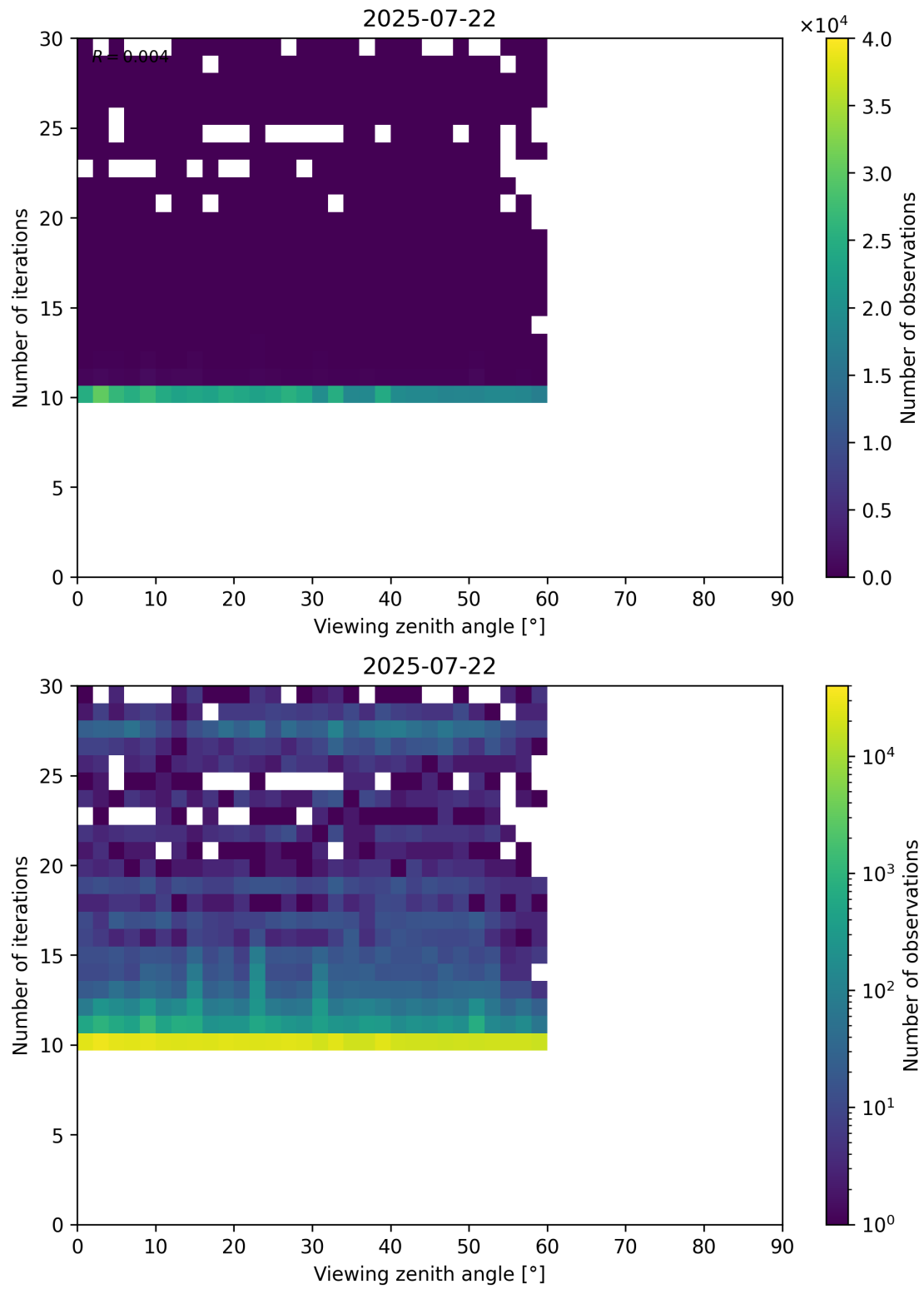
Figure 113: Scatter density plot of “Viewing zenith angle” against “Number of iterations” for 2025-07-21 to 2025-07-23.
