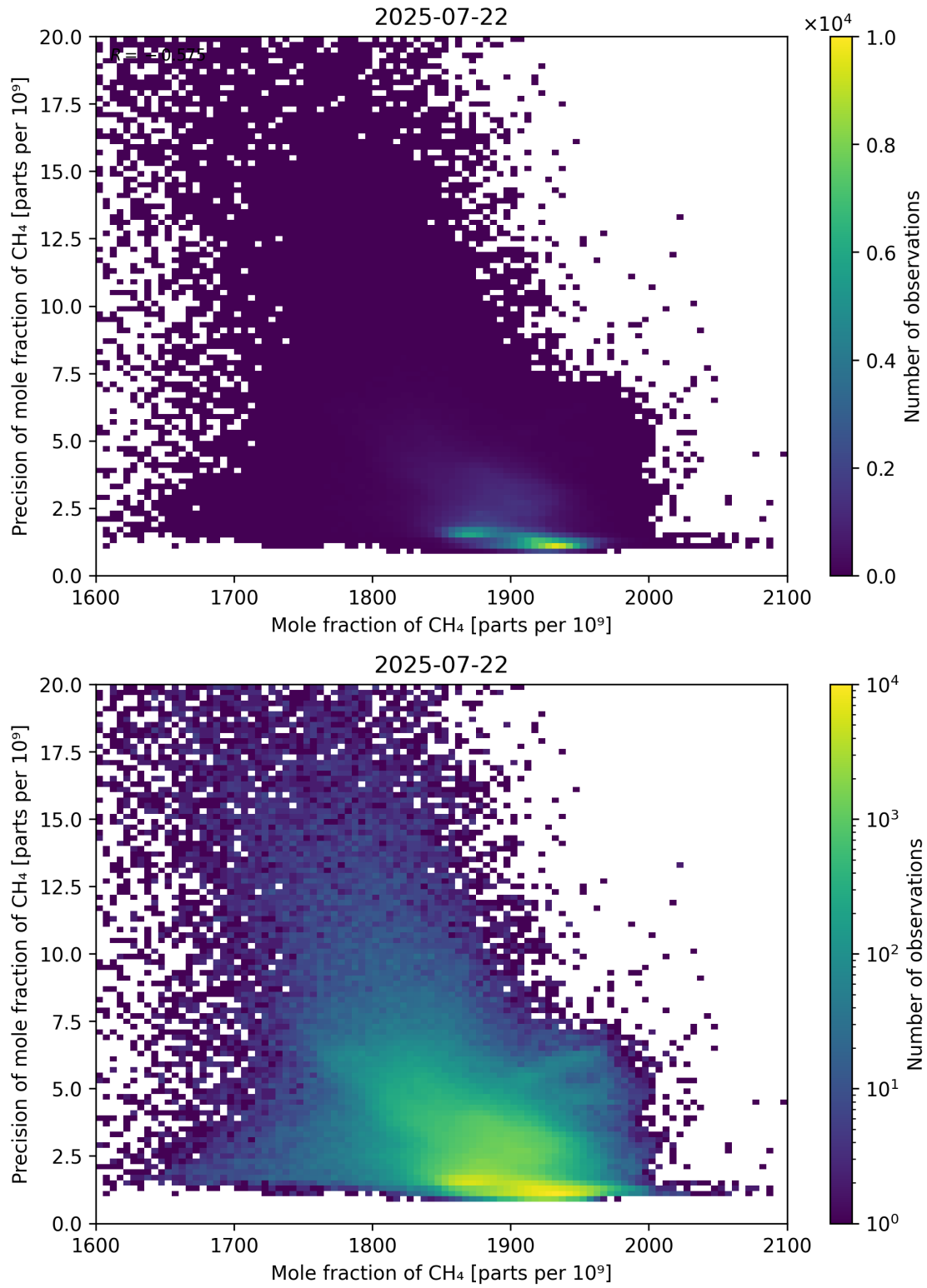
Figure 75: Scatter density plot of “Mole fraction of CH 4 ” against “Precision of mole fraction of CH 4 ” for 2025-07-21 to 2025-07-23.
