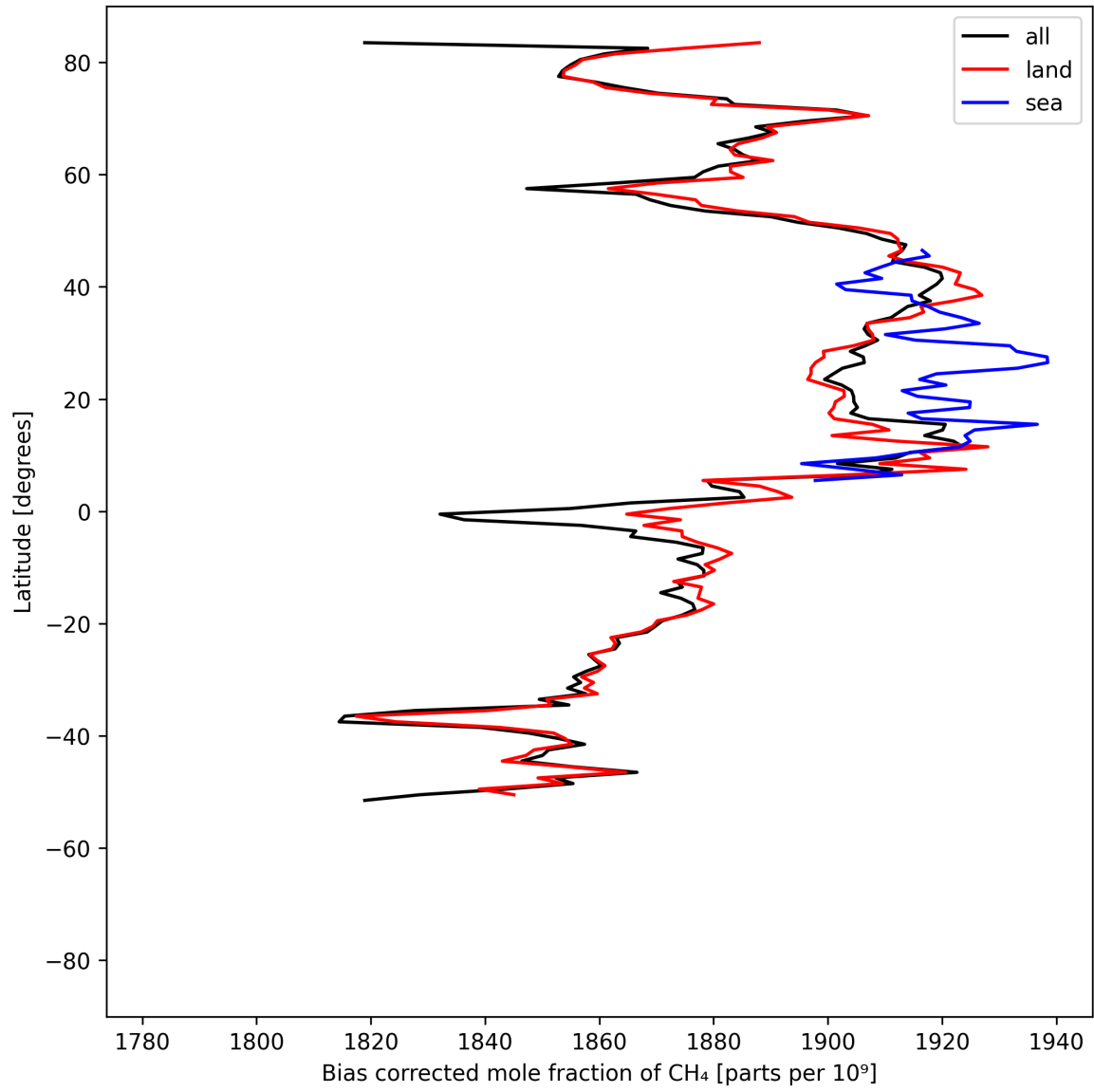
Figure 14: Zonal average of “Bias corrected mole fraction of CH 4 ” for 2025-07-21 to 2025-07-23.
