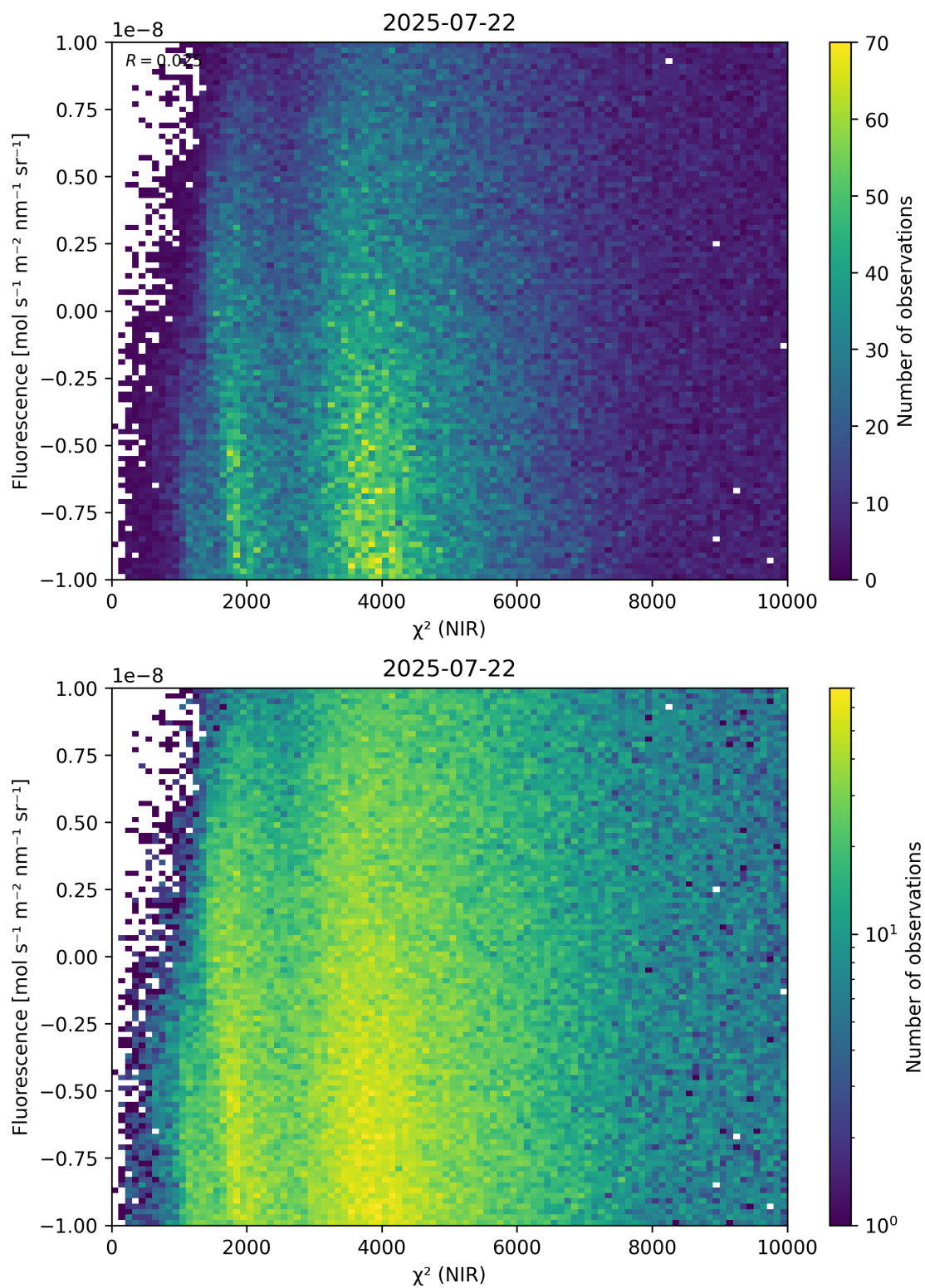
Figure 45: Scatter density plot of “ \chi^2 (NIR)” against “Fluorescence” for 2025-07-21 to 2025-07-23.
