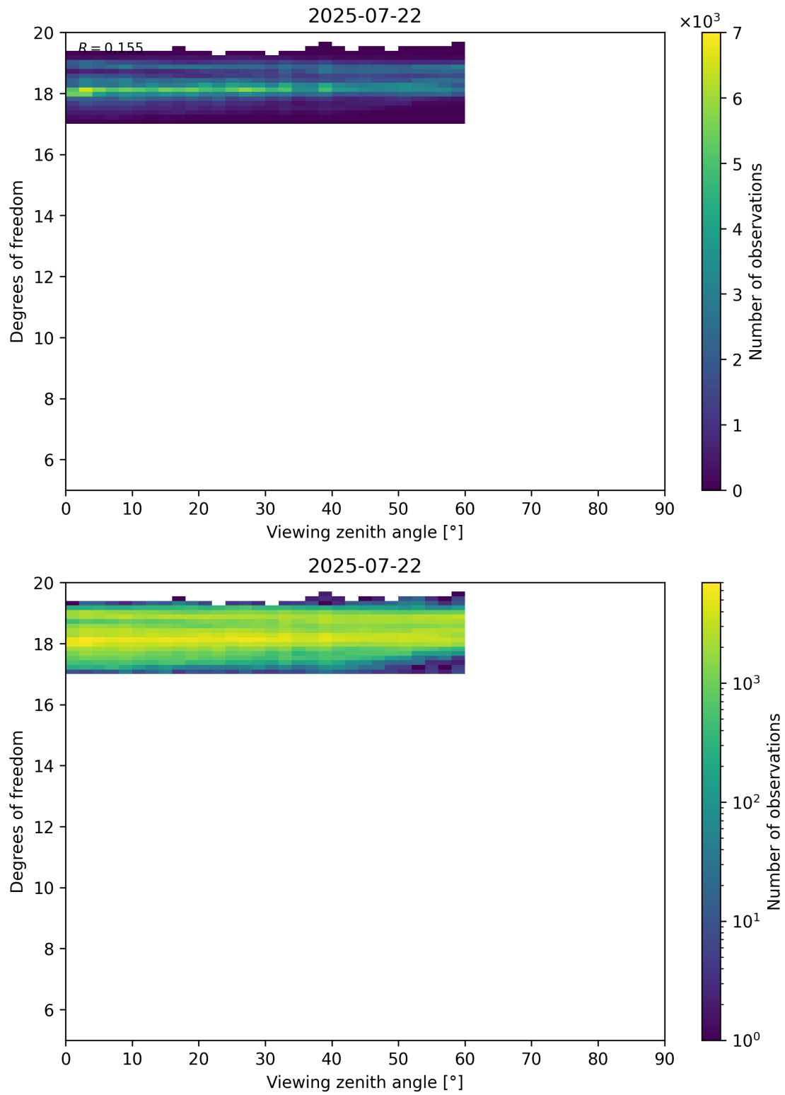
Figure 107: Scatter density plot of “Viewing zenith angle” against “Degrees of freedom” for 2025-07-21 to 2025-07-23.
