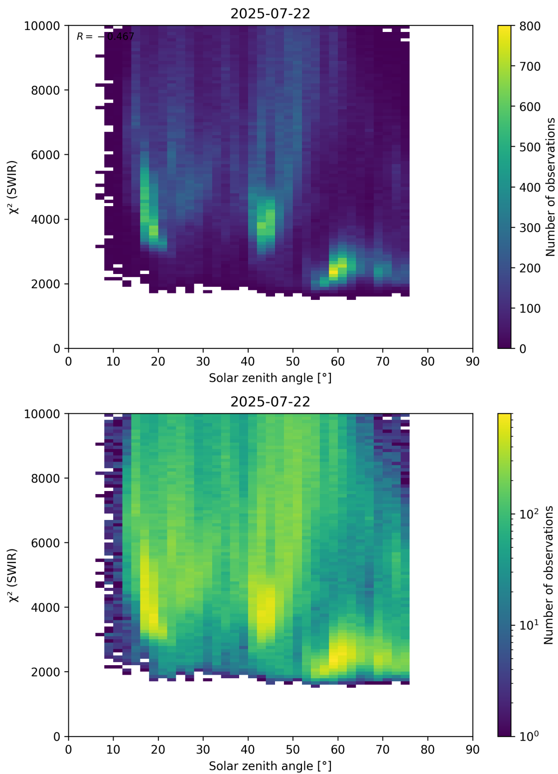
Figure 95: Scatter density plot of “Solar zenith angle” against “ \chi^2 (SWIR)” for 2025-07-21 to 2025-07-23.
