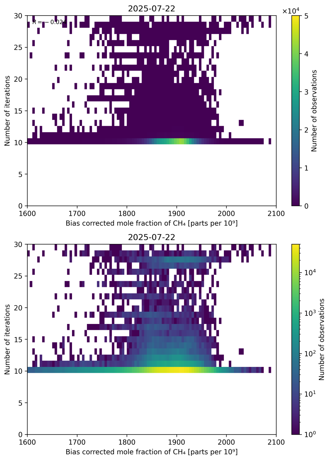
Figure 67: Scatter density plot of “Bias corrected mole fraction of CH 4 ” against “Number of iterations” for 2025-07-21 to 2025-07-23.
