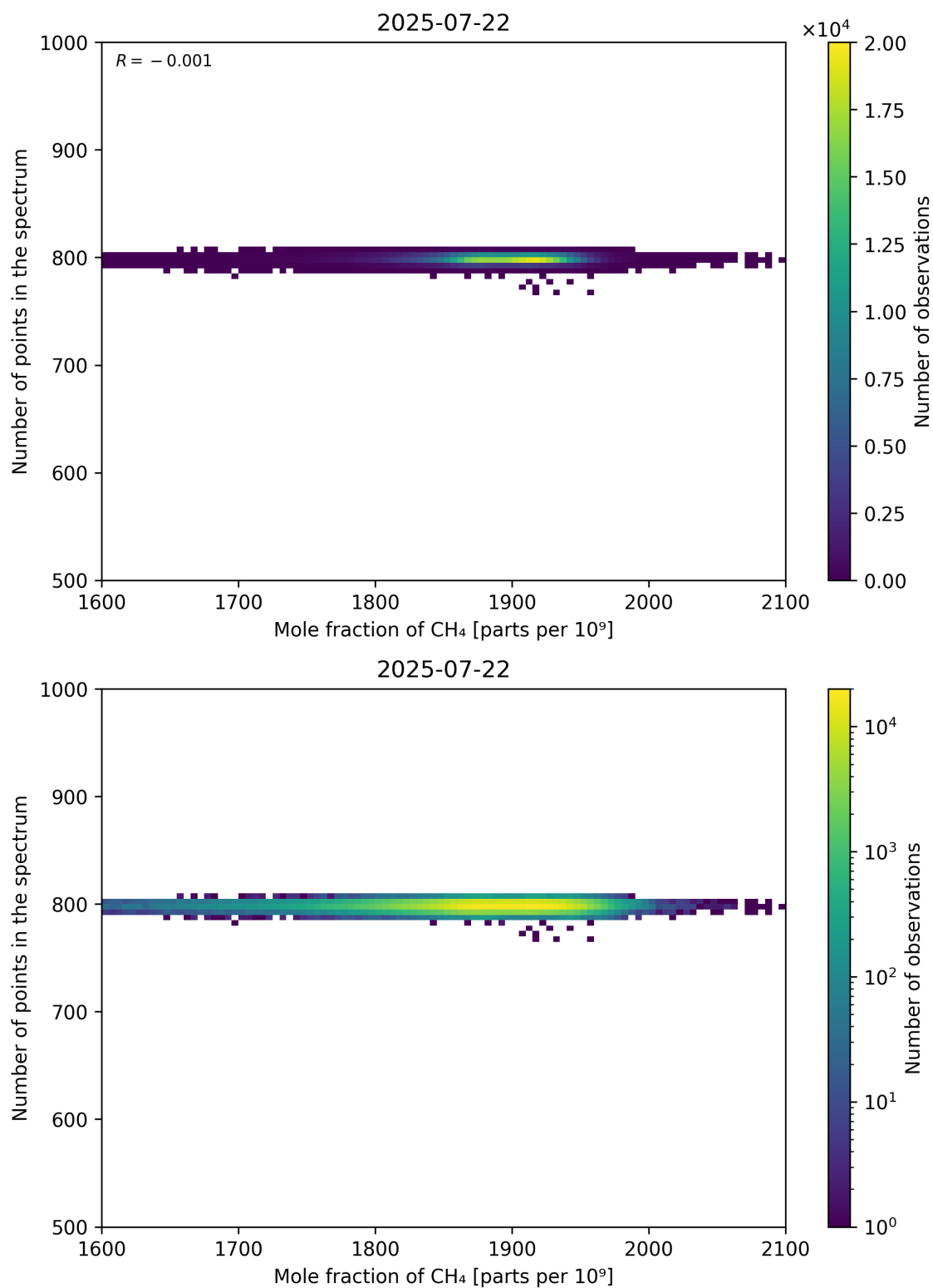
Figure 77: Scatter density plot of “Mole fraction of CH 4 ” against “Number of points in the spectrum” for 2025-07-21 to 2025-07-23.
