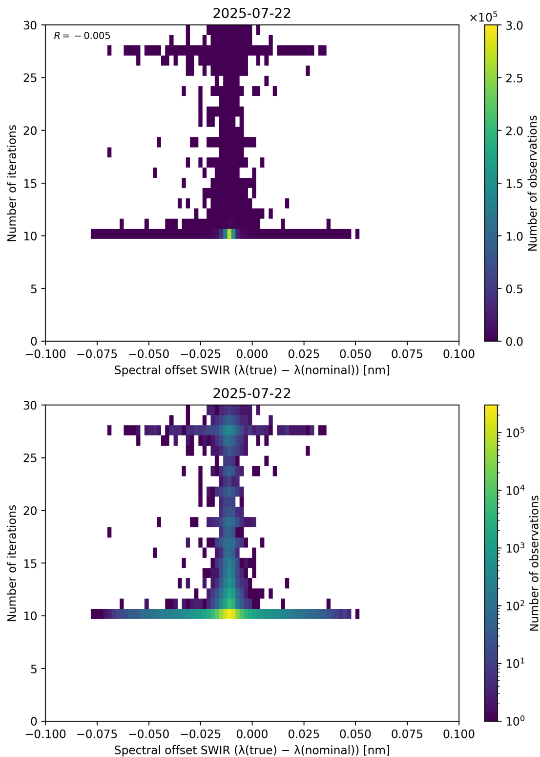
Figure 121: Scatter density plot of “Spectral offset SWIR ( \lambda_{\text{true}} - \lambda_{\text{nominal}} )” against “Number of iterations” for 2025-07-21 to 2025-07-23.
