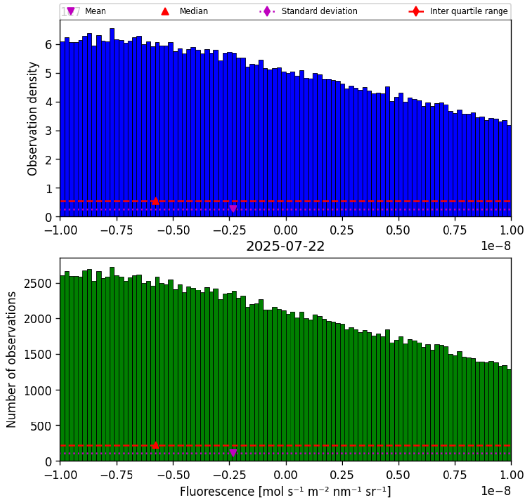
Figure 32: Histogram of “Fluorescence” for 2025-07-21 to 2025-07-23
