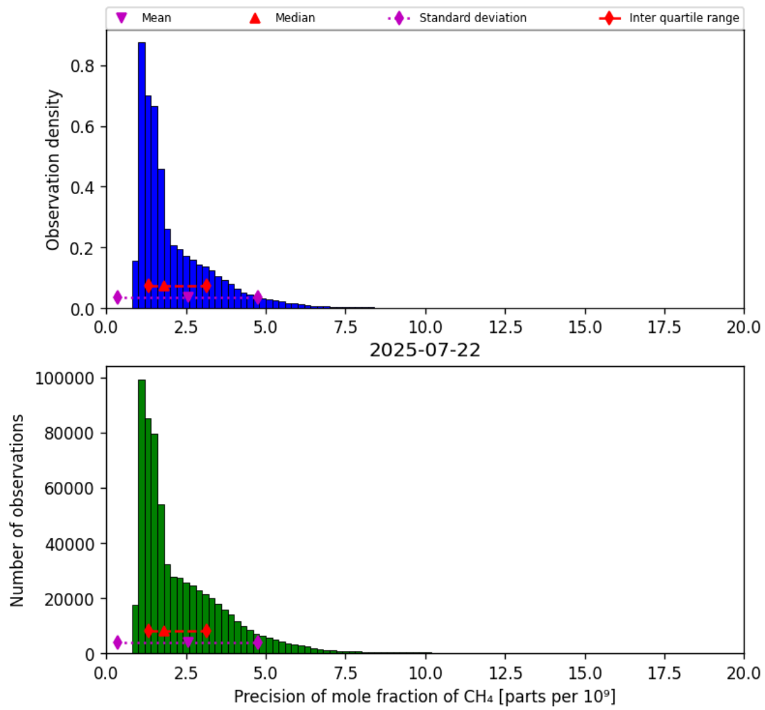
Figure 24: Histogram of “Precision of mole fraction of CH 4 ” for 2025-07-21 to 2025-07-23
