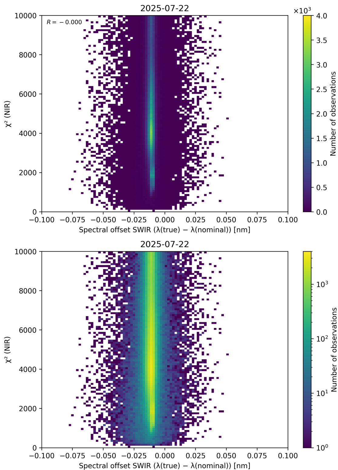
Figure 117: Scatter density plot of “Spectral offset SWIR ( \lambda_{\text{true}} - \lambda_{\text{nominal}} )” against “ \chi^2 (NIR)” for 2025-07-21 to 2025-07-23.
