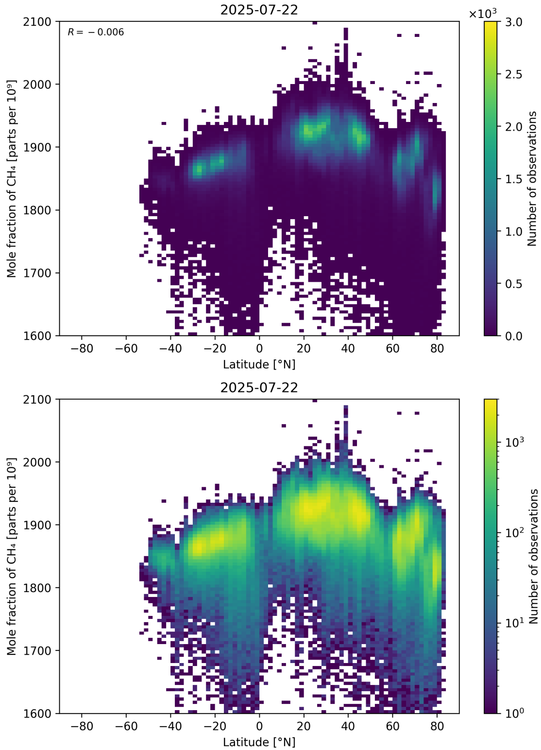
Figure 57: Scatter density plot of “Latitude” against “Mole fraction of \text{CH}_4 ” for 2025-07-21 to 2025-07-23.
