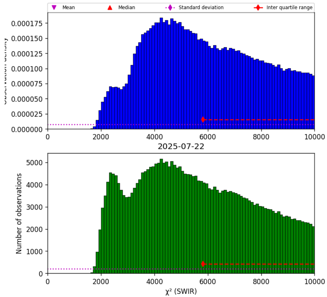
Figure 28: Histogram of “ \chi^2 (SWIR)” for 2025-07-21 to 2025-07-23
