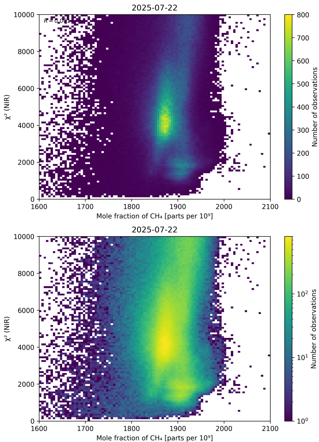
Figure 70: Scatter density plot of “Mole fraction of \text{CH}_4 ” against “ \chi^2 (NIR)” for 2025-07-21 to 2025-07-23.
