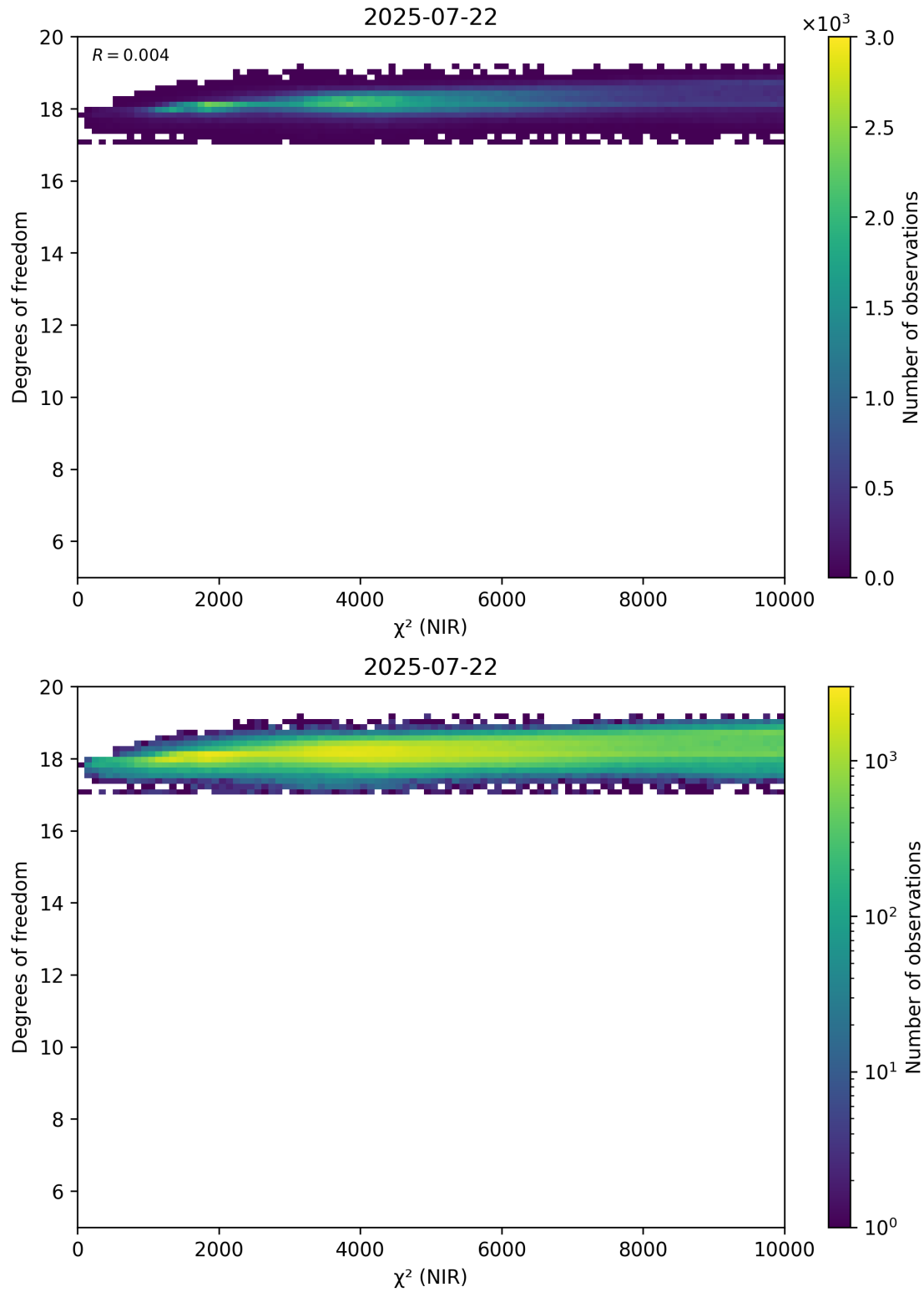
Figure 44: Scatter density plot of “ \chi^2 (NIR)” against “Degrees of freedom” for 2025-07-21 to 2025-07-23.
