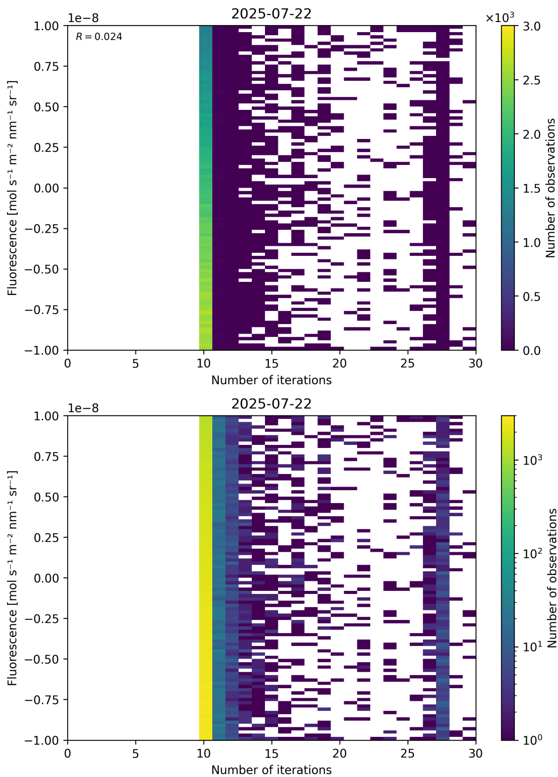
Figure 87: Scatter density plot of “Number of iterations” against “Fluorescence” for 2025-07-21 to 2025-07-23.
