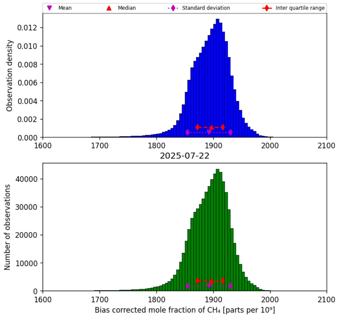
Figure 25: Histogram of “Bias corrected mole fraction of CH 4 ” for 2025-07-21 to 2025-07-23
