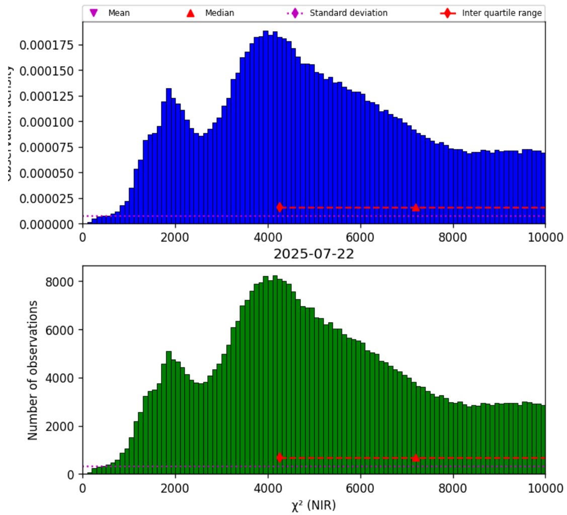
Figure 29: Histogram of “ \chi^2 (NIR)” for 2025-07-21 to 2025-07-23
