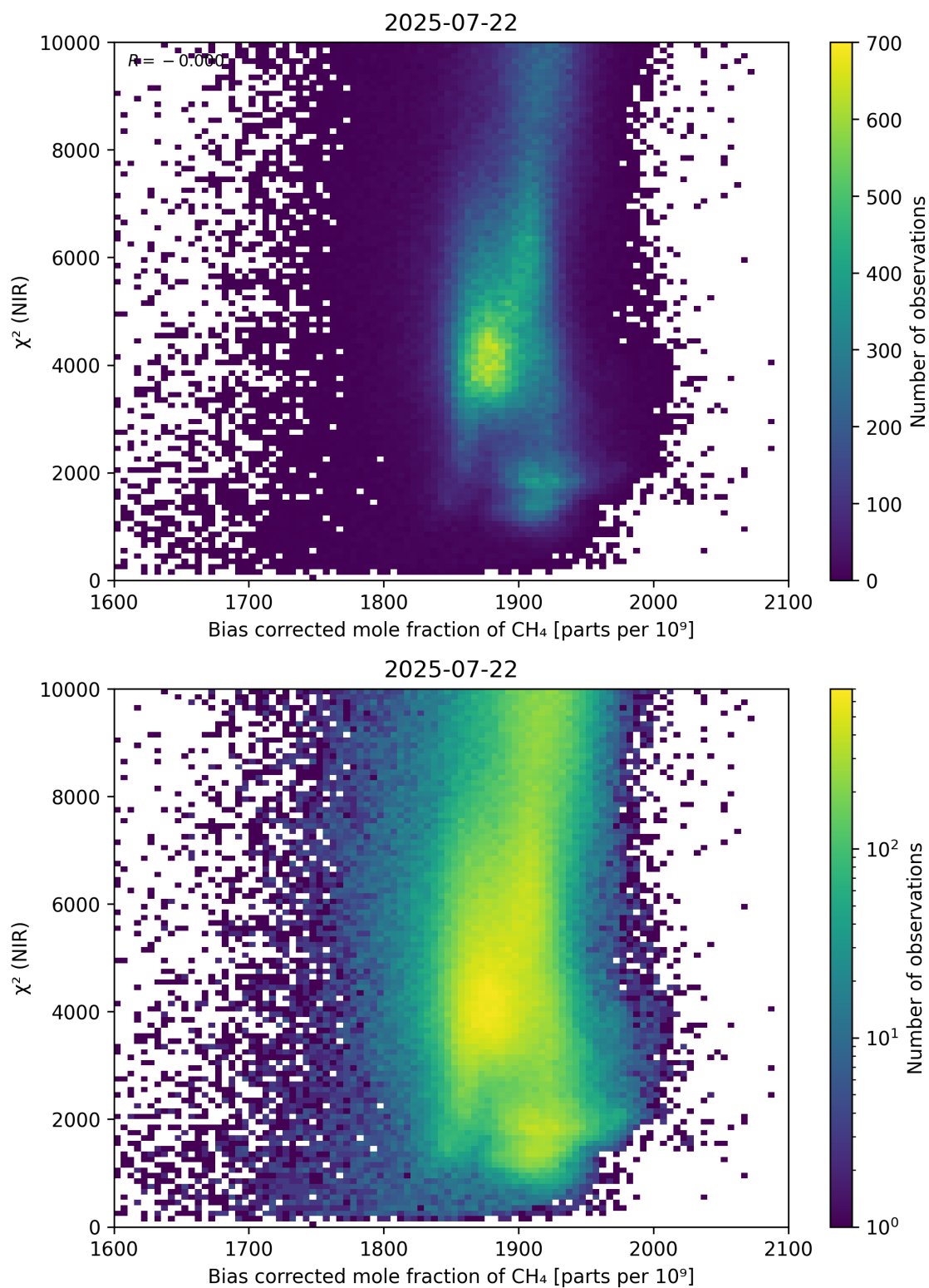
Figure 63: Scatter density plot of “Bias corrected mole fraction of \text{CH}_4 ” against “ \chi^2 (NIR)” for 2025-07-21 to 2025-07-23.
