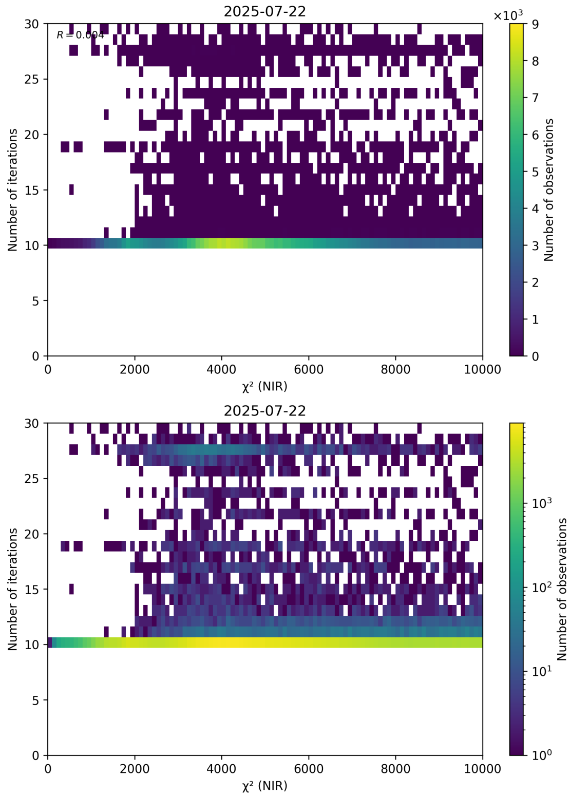
Figure 46: Scatter density plot of “ \chi^2 (NIR)” against “Number of iterations” for 2025-07-21 to 2025-07-23.
