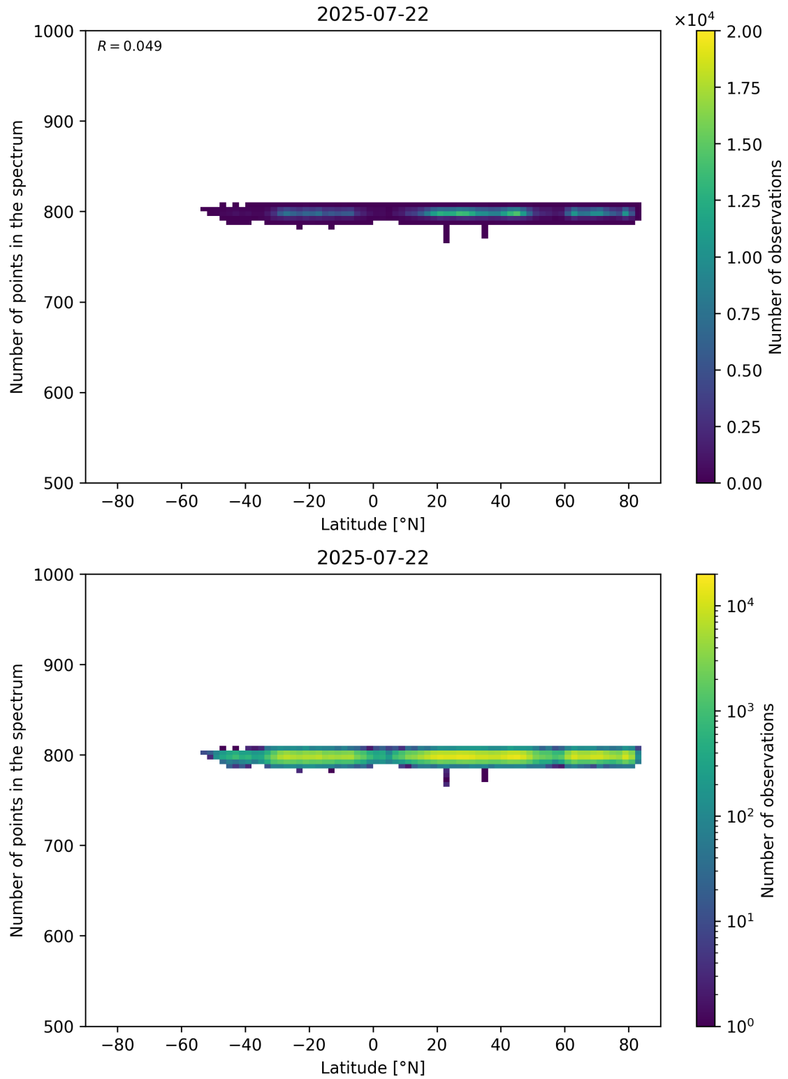
Figure 61: Scatter density plot of “Latitude” against “Number of points in the spectrum” for 2025-07-21 to 2025-07-23.
