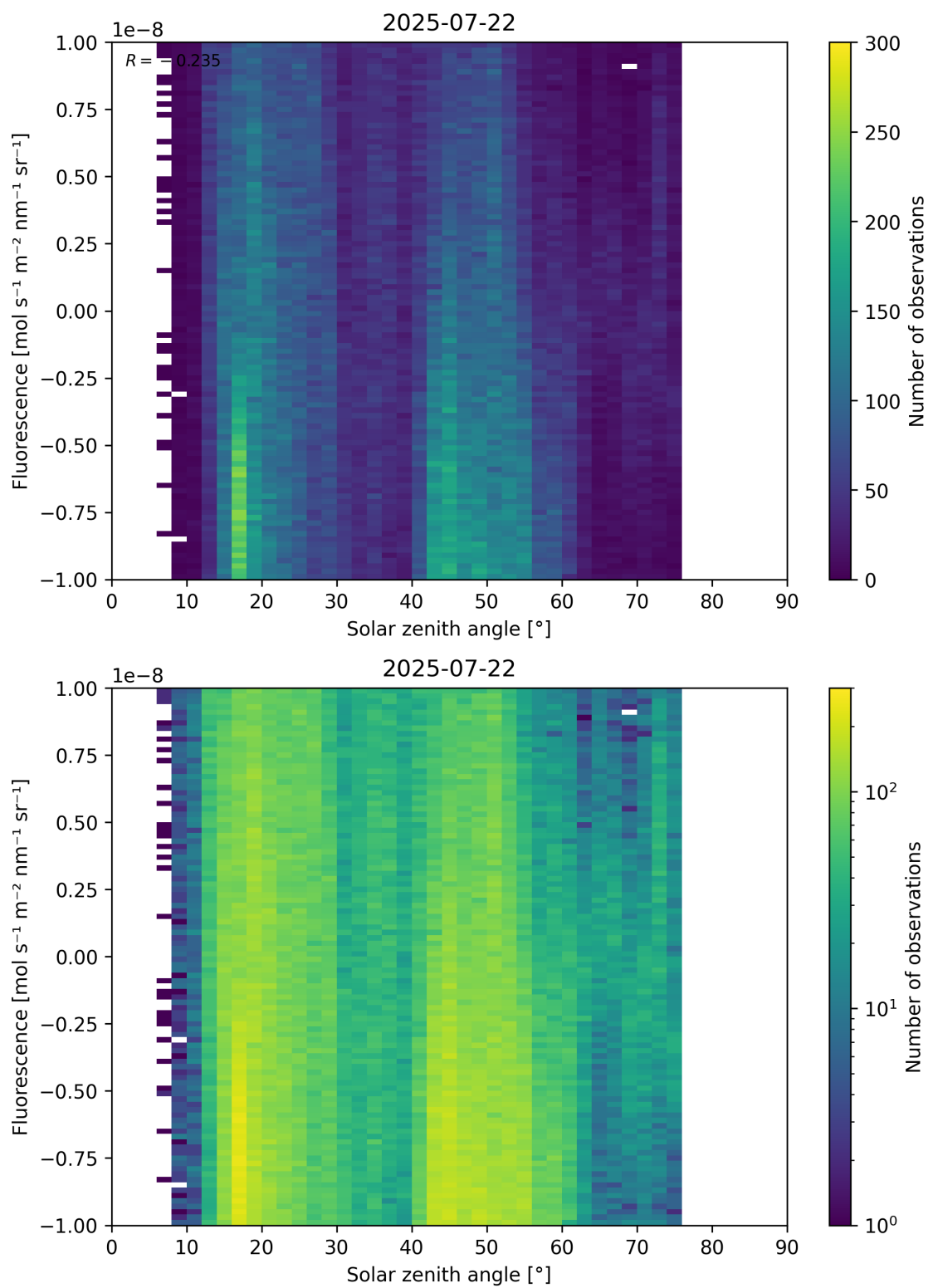
Figure 97: Scatter density plot of “Solar zenith angle” against “Fluorescence” for 2025-07-21 to 2025-07-23.
