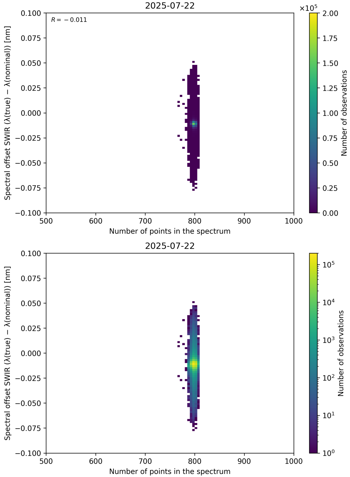
Figure 93: Scatter density plot of “Number of points in the spectrum” against “Spectral offset SWIR ( \lambda_{\text{true}} - \lambda_{\text{nominal}} )” for 2025-07-21 to 2025-07-23.
