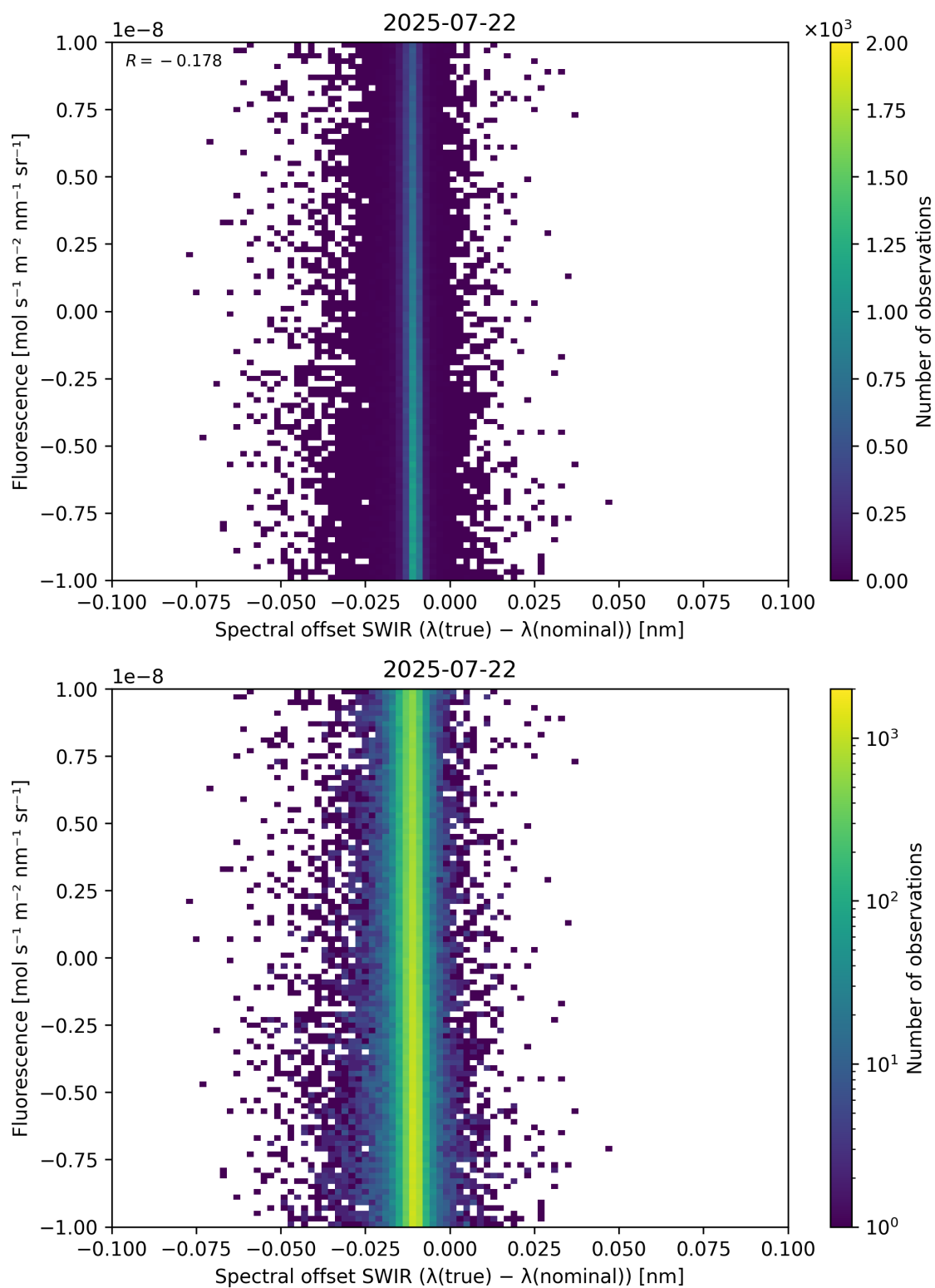
Figure 120: Scatter density plot of “Spectral offset SWIR ( \lambda_{\text{true}} - \lambda_{\text{nominal}} )” against “Fluorescence” for 2025-07-21 to 2025-07-23.
