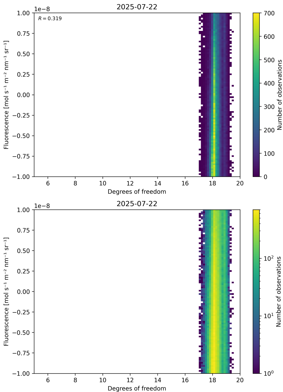
Figure 51: Scatter density plot of “Degrees of freedom” against “Fluorescence” for 2025-07-21 to 2025-07-23.
