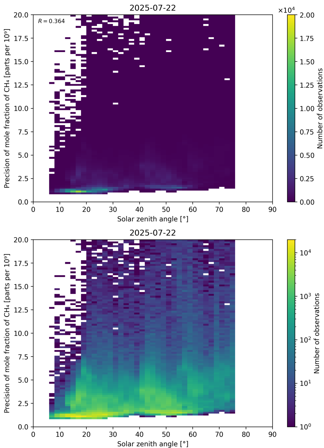
Figure 101: Scatter density plot of “Solar zenith angle” against “Precision of mole fraction of CH 4 ” for 2025-07-21 to 2025-07-23.
