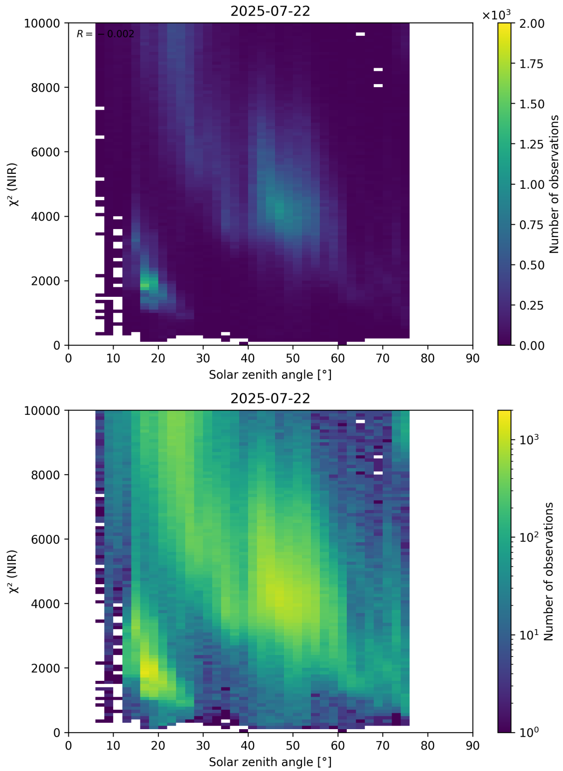
Figure 94: Scatter density plot of “Solar zenith angle” against “ \chi^2 (NIR)” for 2025-07-21 to 2025-07-23.
