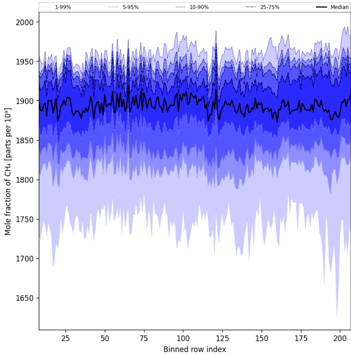
Figure 34: Along track statistics of “Mole fraction of CH 4 ” for 2025-07-21 to 2025-07-23
