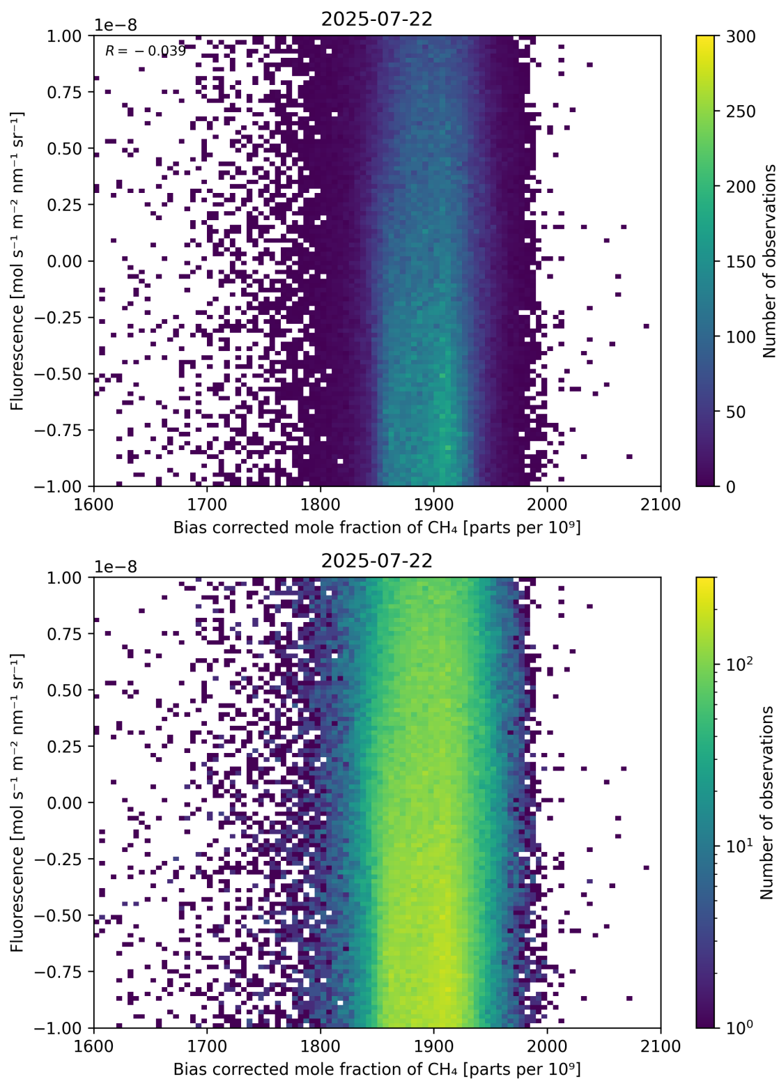
Figure 66: Scatter density plot of “Bias corrected mole fraction of \text{CH}_4 ” against “Fluorescence” for 2025-07-21 to 2025-07-23.
