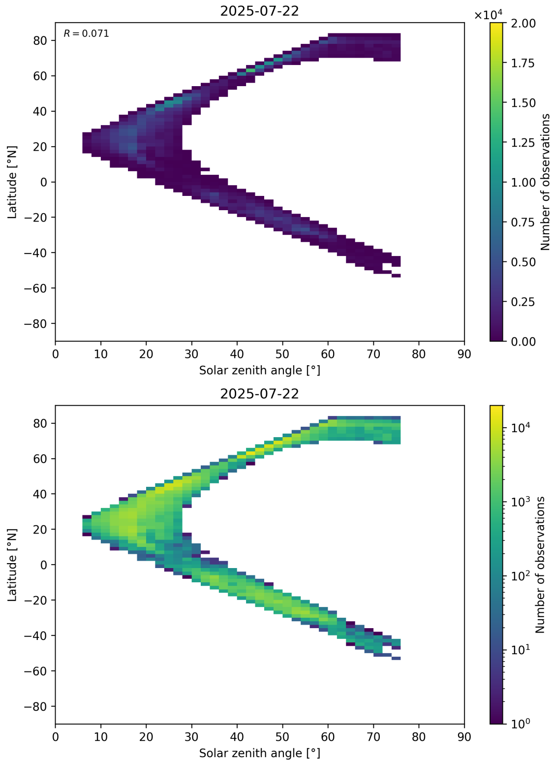
Figure 98: Scatter density plot of “Solar zenith angle” against “Latitude” for 2025-07-21 to 2025-07-23.
