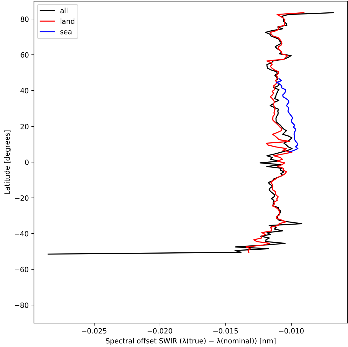
Figure 16: Zonal average of “Spectral offset SWIR ( \lambda_{\text{true}} - \lambda_{\text{nominal}} )” for 2025-07-21 to 2025-07-23.
