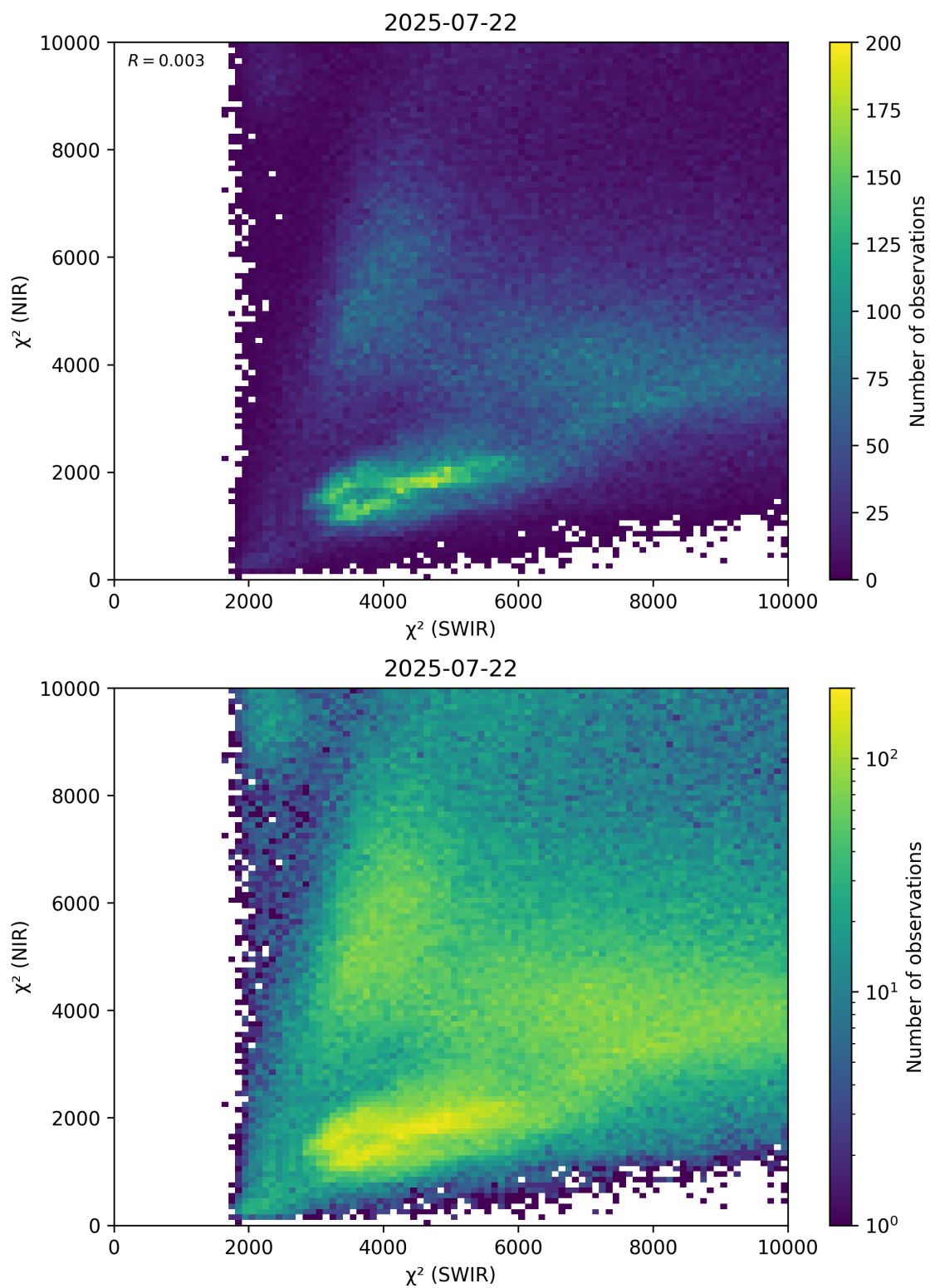
Figure 47: Scatter density plot of “ \chi^2 (SWIR)” against “ \chi^2 (NIR)” for 2025-07-21 to 2025-07-23.
