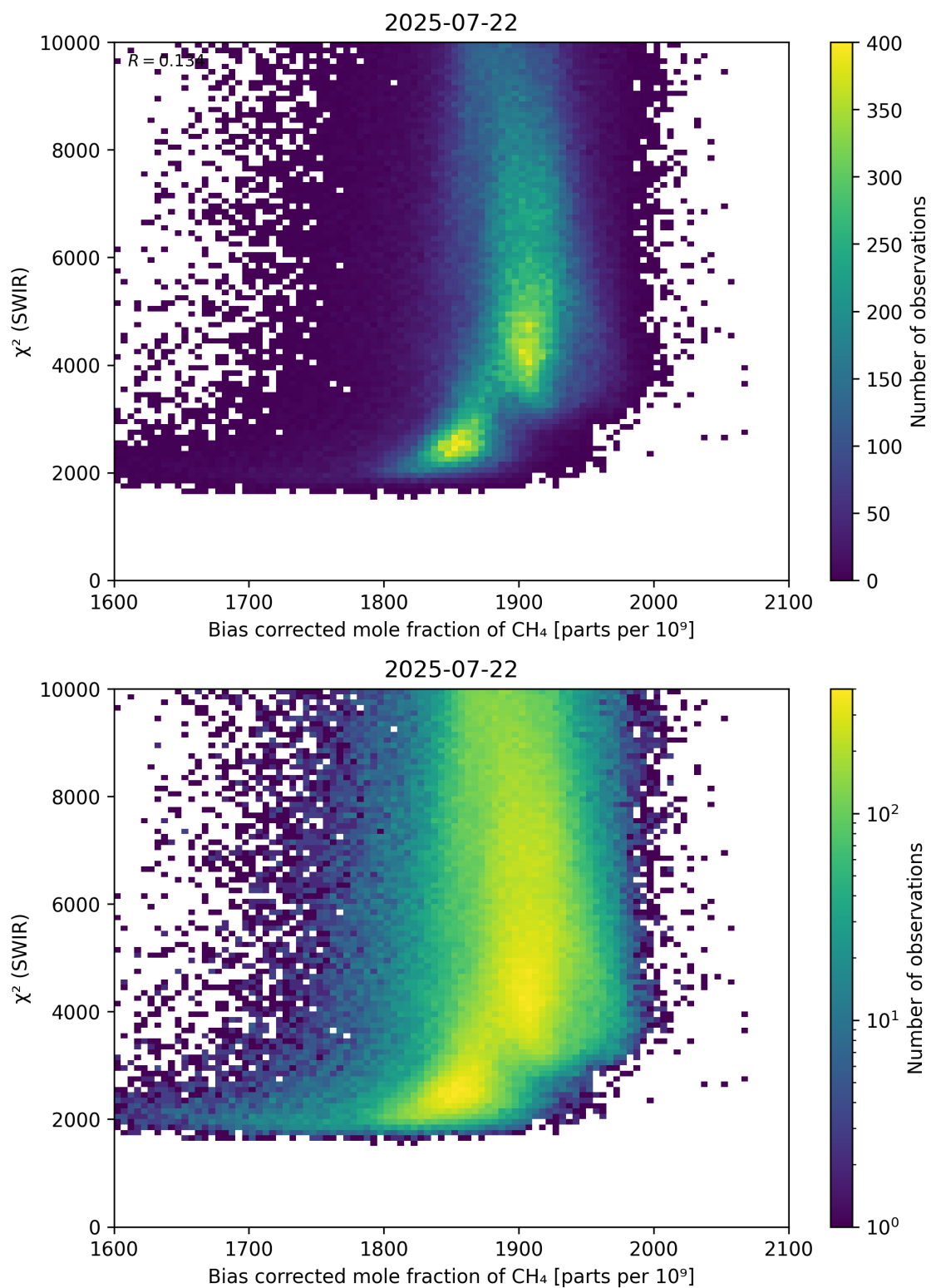
Figure 64: Scatter density plot of “Bias corrected mole fraction of \text{CH}_4 ” against “ \chi^2 (SWIR)” for 2025-07-21 to 2025-07-23.
