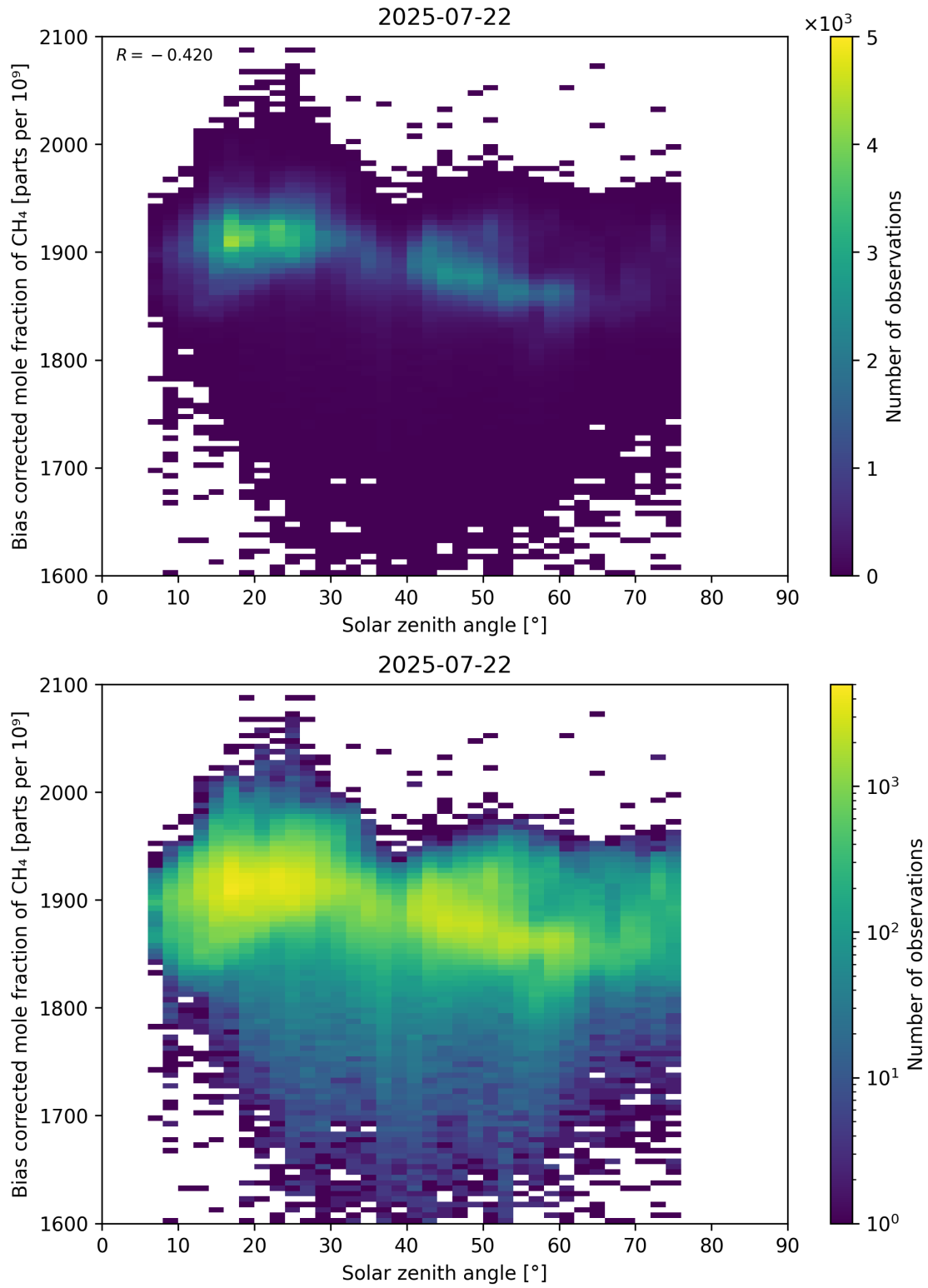
Figure 100: Scatter density plot of “Solar zenith angle” against “Bias corrected mole fraction of \text{CH}_4 ” for 2025-07-21 to 2025-07-23.
