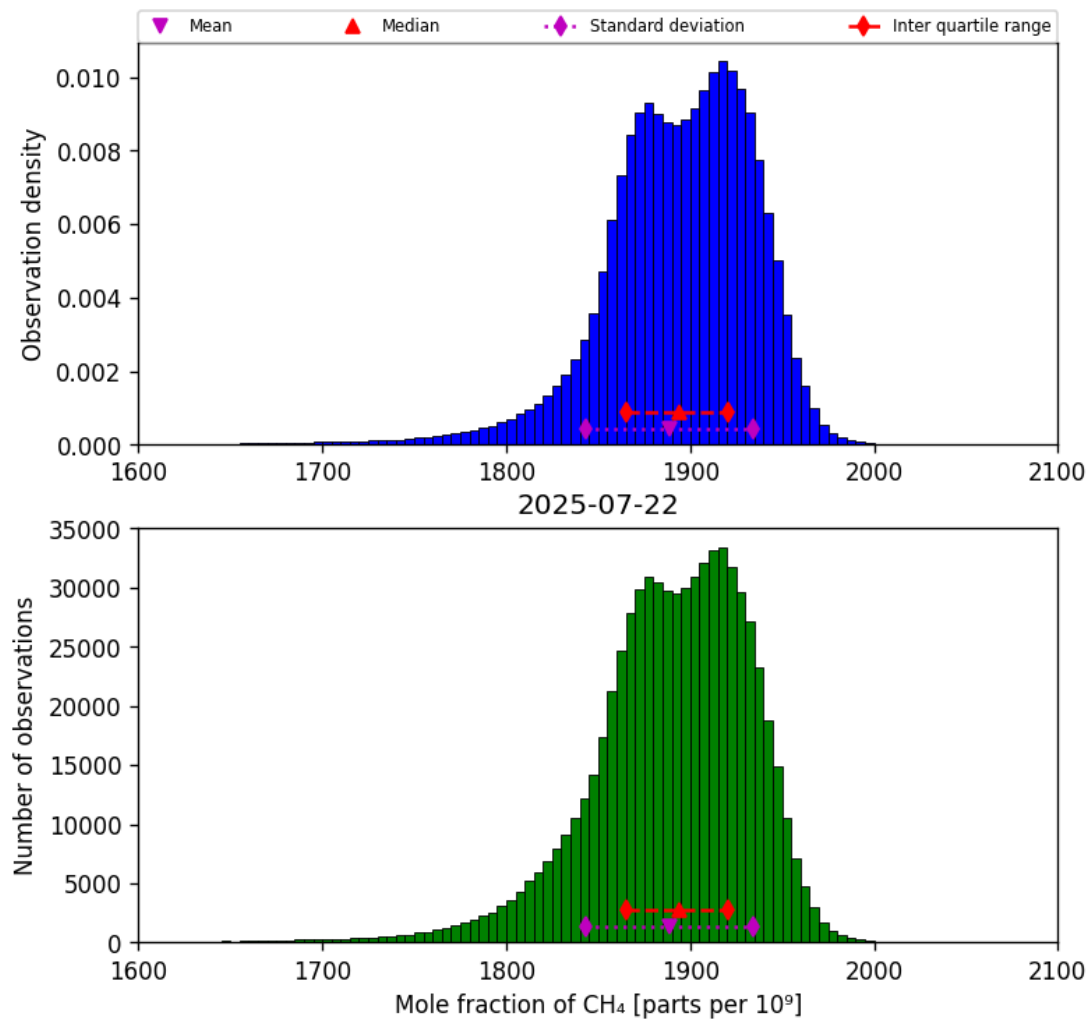
Figure 23: Histogram of “Mole fraction of CH 4 ” for 2025-07-21 to 2025-07-23
