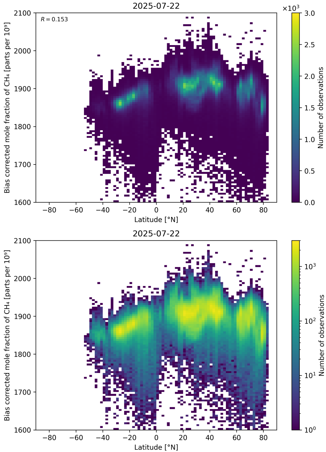
Figure 58: Scatter density plot of “Latitude” against “Bias corrected mole fraction of \text{CH}_4 ” for 2025-07-21 to 2025-07-23.
