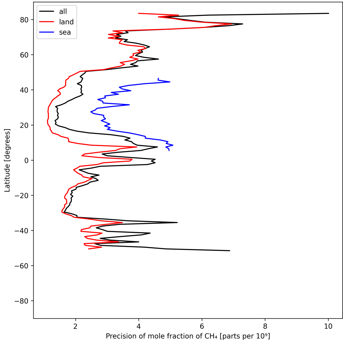
Figure 13: Zonal average of “Precision of mole fraction of CH 4 ” for 2025-07-21 to 2025-07-23.
