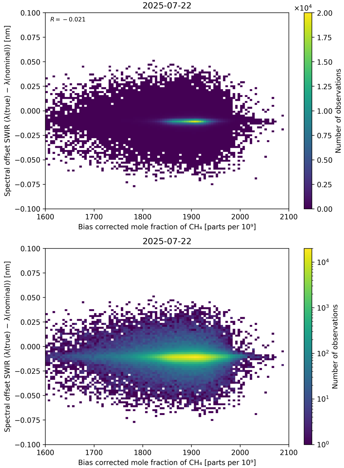
Figure 69: Scatter density plot of “Bias corrected mole fraction of \text{CH}_4 ” against “Spectral offset SWIR ( \lambda_{\text{true}} - \lambda_{\text{nominal}} )” for 2025-07-21 to 2025-07-23.
