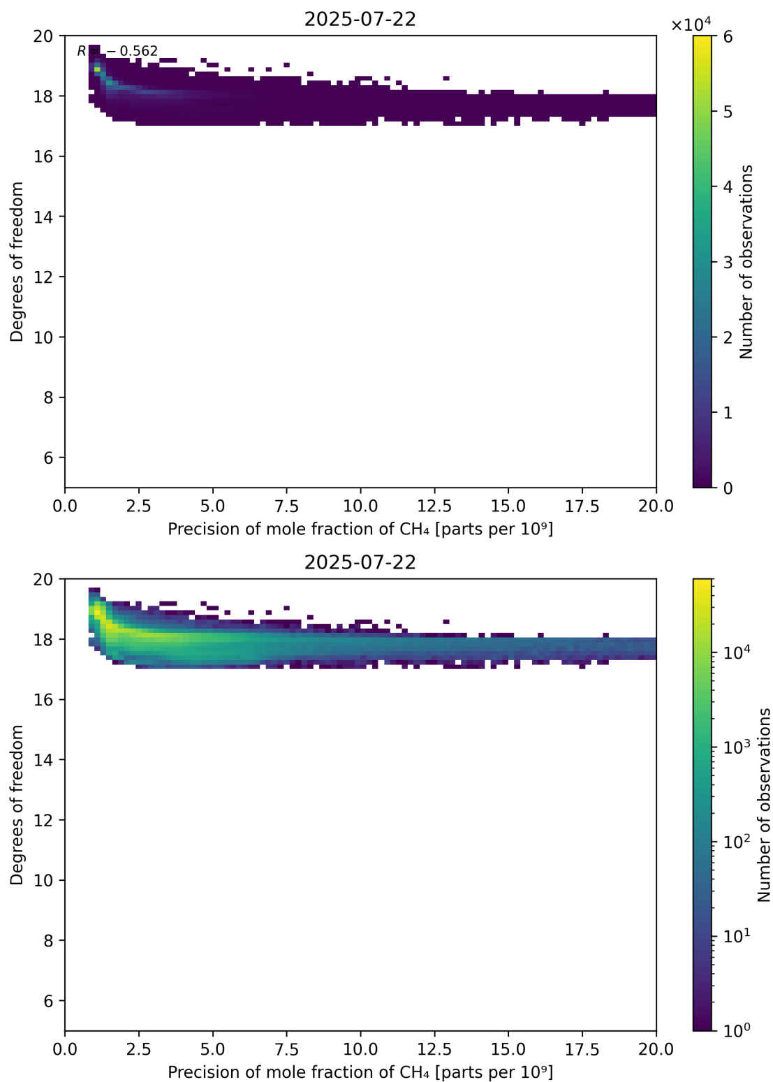
Figure 80: Scatter density plot of “Precision of mole fraction of CH 4 ” against “Degrees of freedom” for 2025-07-21 to 2025-07-23.
