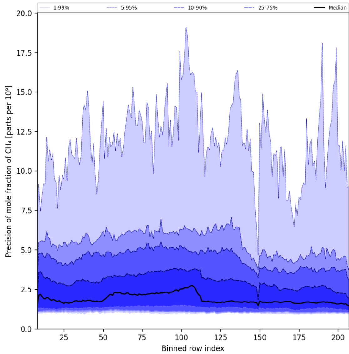
Figure 35: Along track statistics of “Precision of mole fraction of CH 4 ” for 2025-07-21 to 2025-07-23
