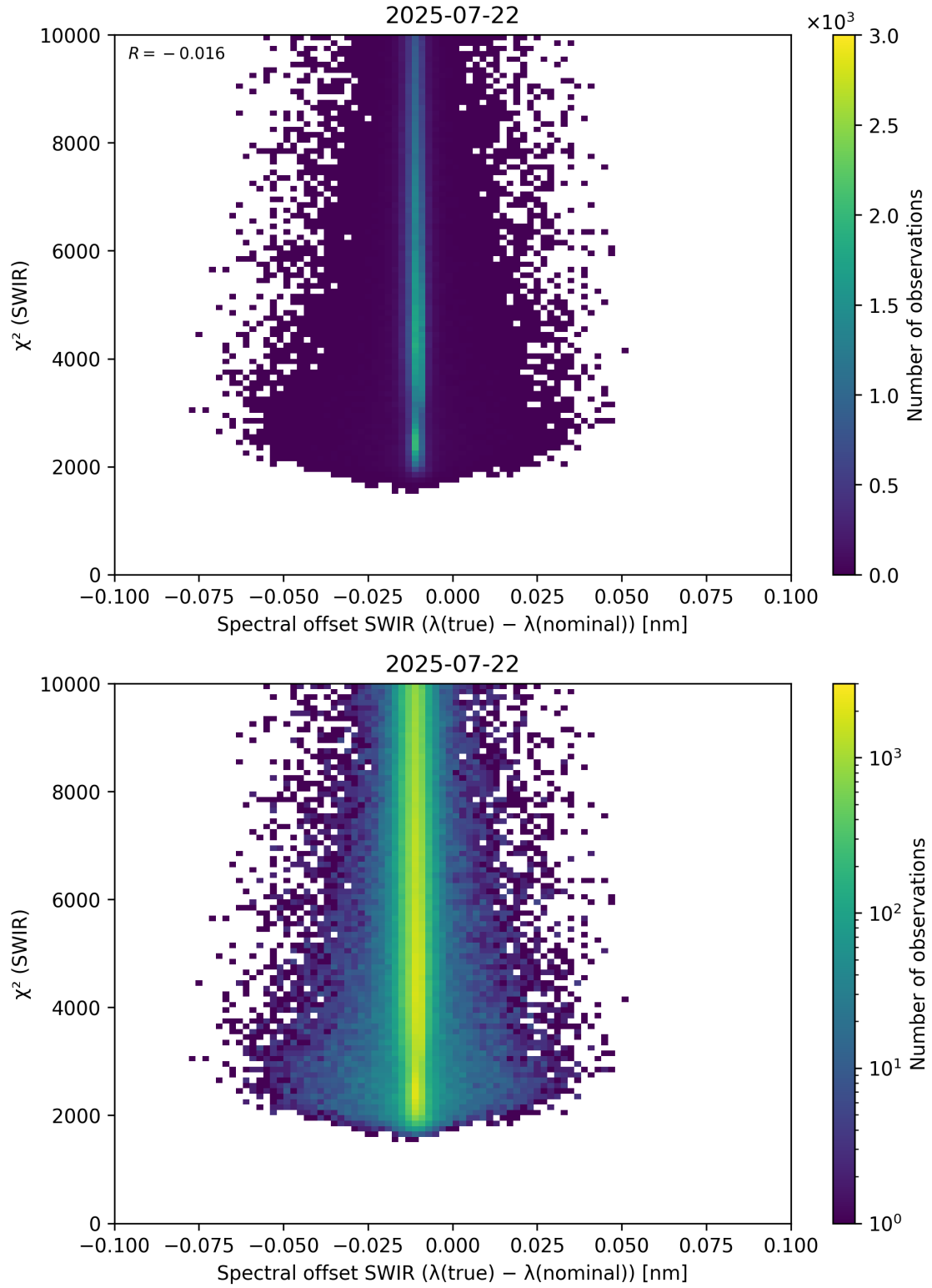
Figure 118: Scatter density plot of “Spectral offset SWIR ( \lambda_{\text{true}} - \lambda_{\text{nominal}} )” against “ \chi^2 (SWIR)” for 2025-07-21 to 2025-07-23.
