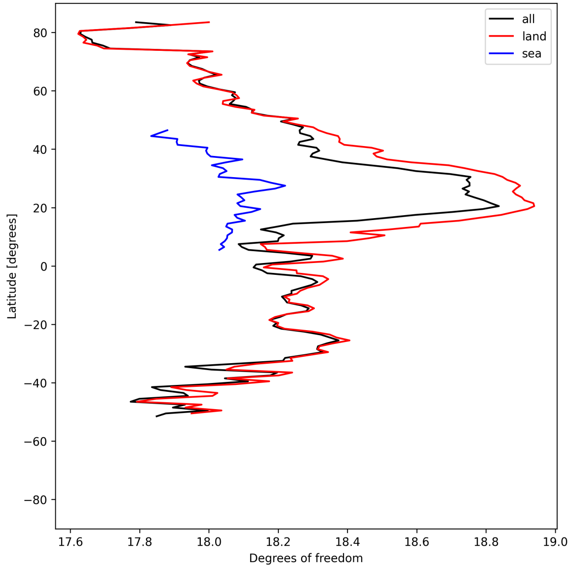
Figure 19: Zonal average of “Degrees of freedom” for 2025-07-21 to 2025-07-23.
