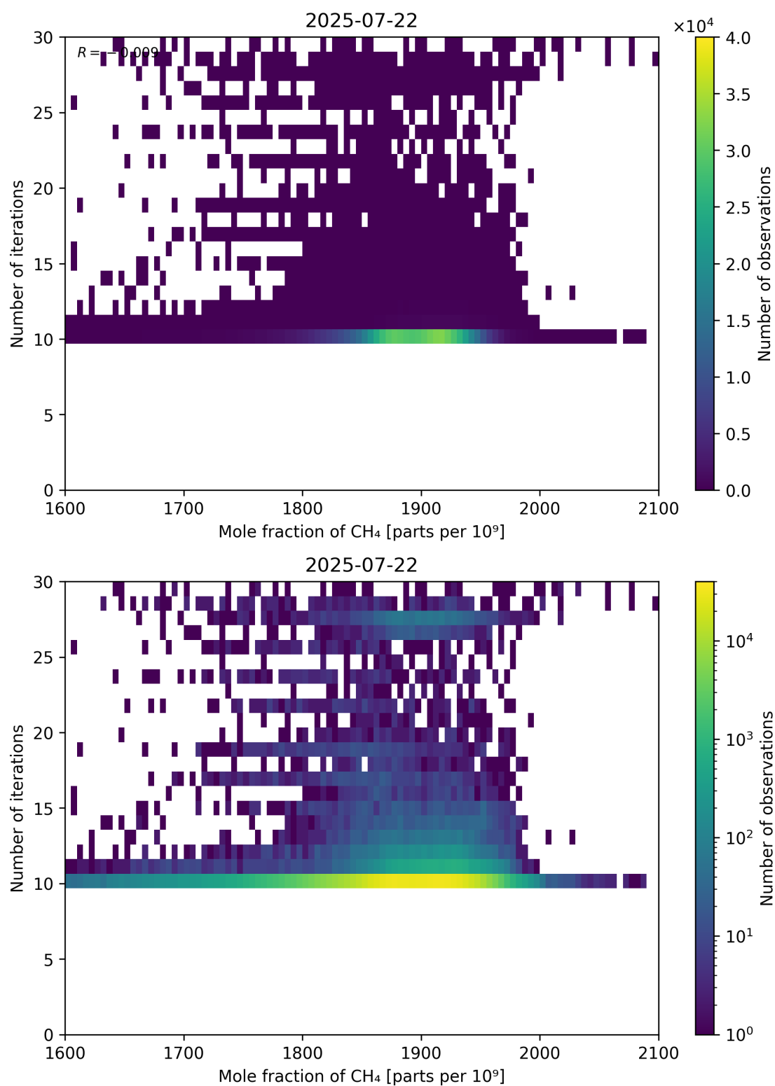
Figure 76: Scatter density plot of “Mole fraction of CH 4 ” against “Number of iterations” for 2025-07-21 to 2025-07-23.
