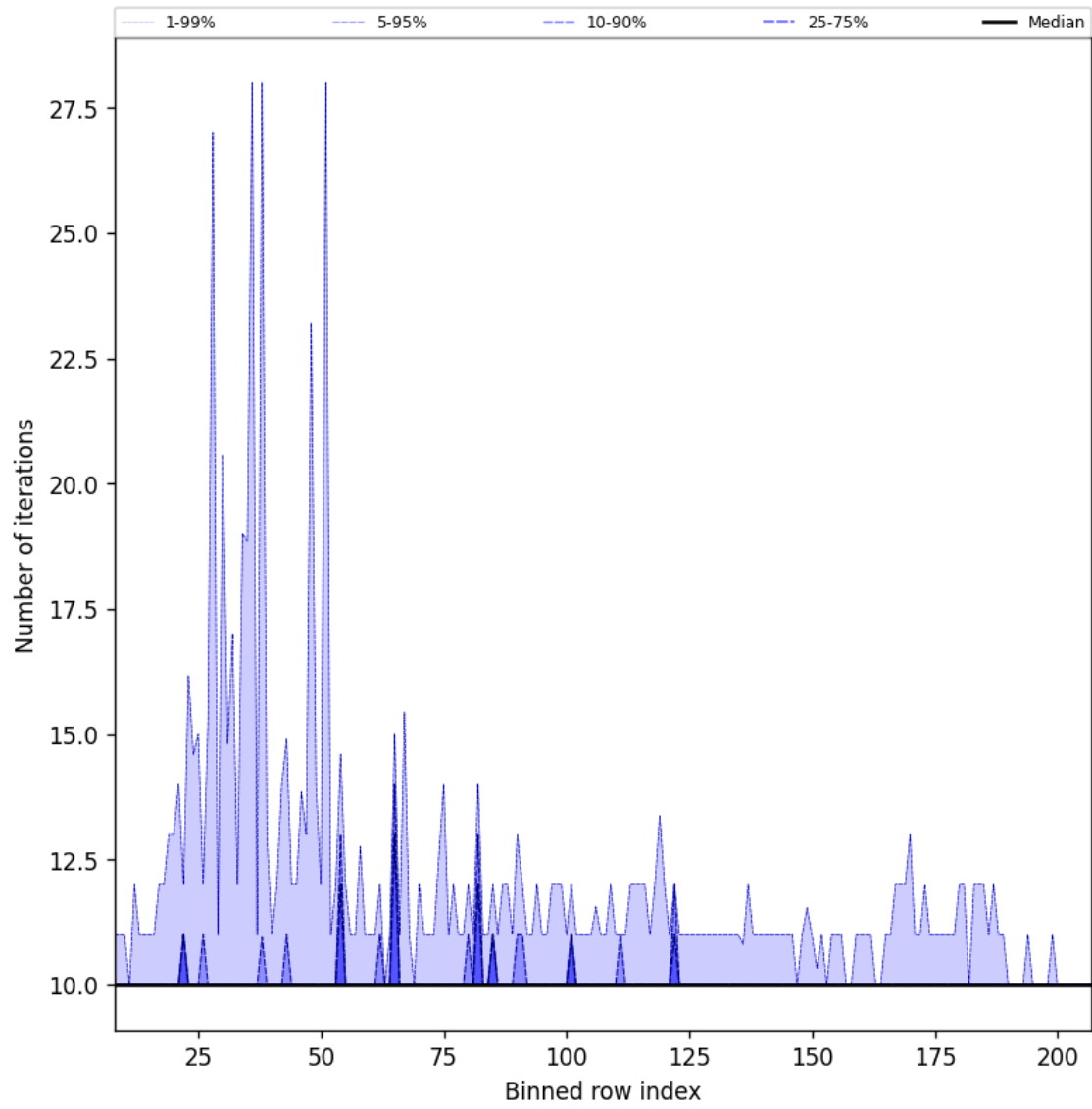
Figure 42: Along track statistics of “Number of iterations” for 2025-07-21 to 2025-07-23
