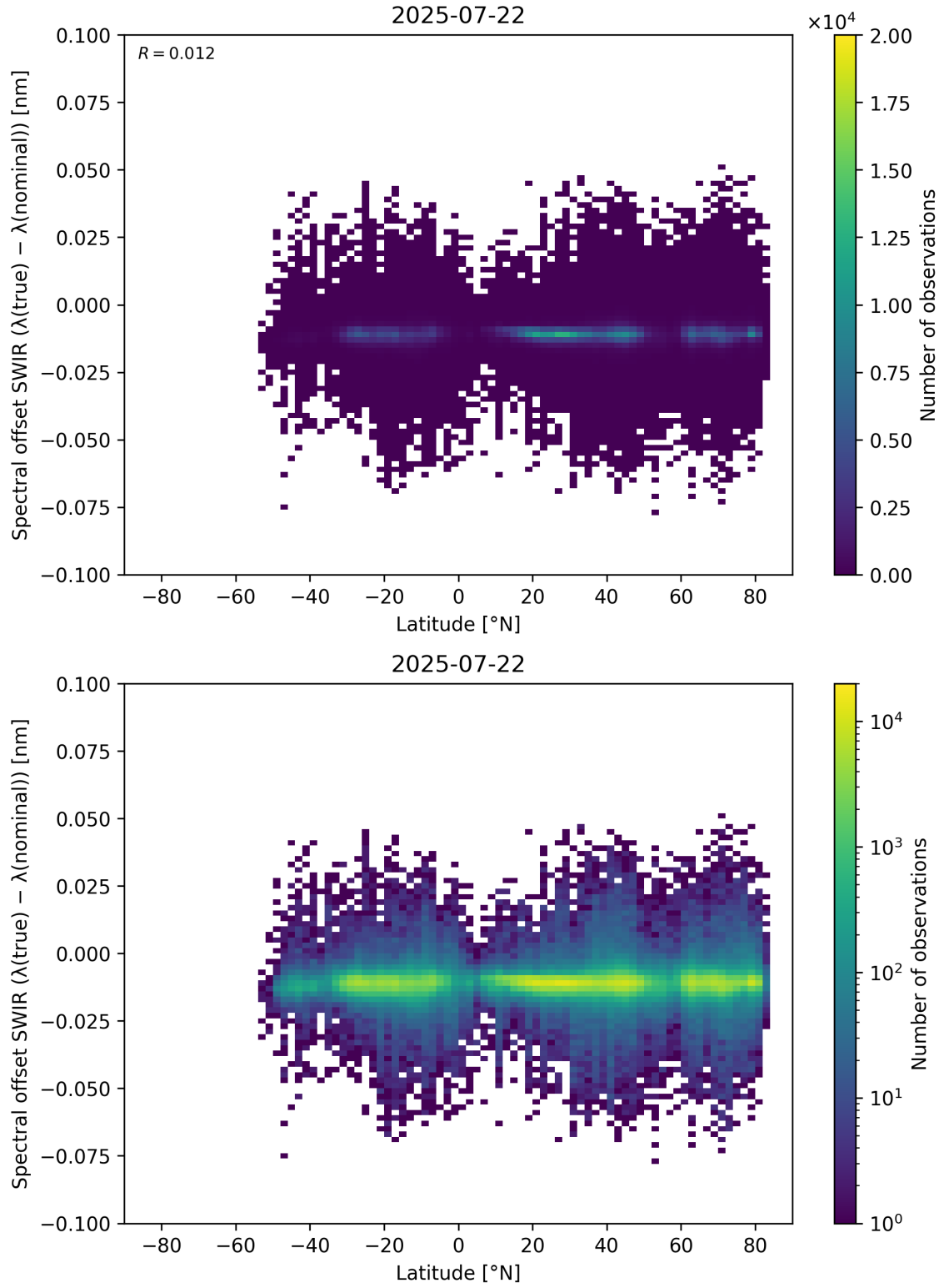
Figure 62: Scatter density plot of “Latitude” against “Spectral offset SWIR ( \lambda_{\text{true}} - \lambda_{\text{nominal}} )” for 2025-07-21 to 2025-07-23.
