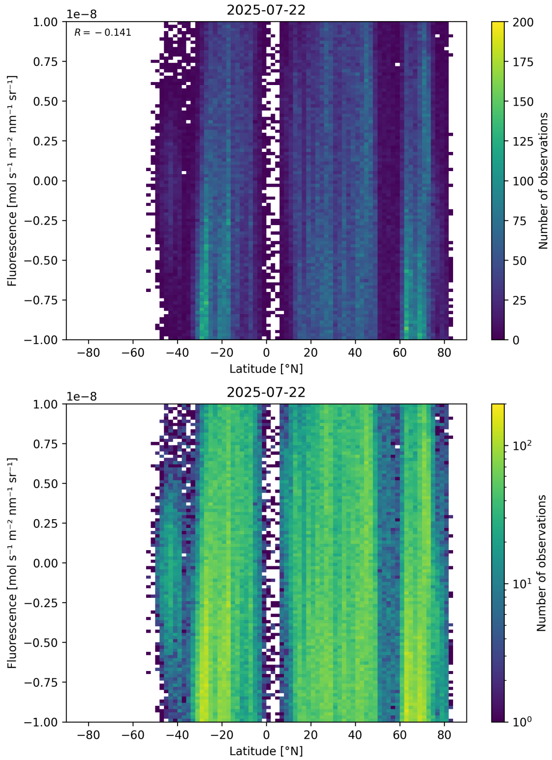
Figure 56: Scatter density plot of “Latitude” against “Fluorescence” for 2025-07-21 to 2025-07-23.
