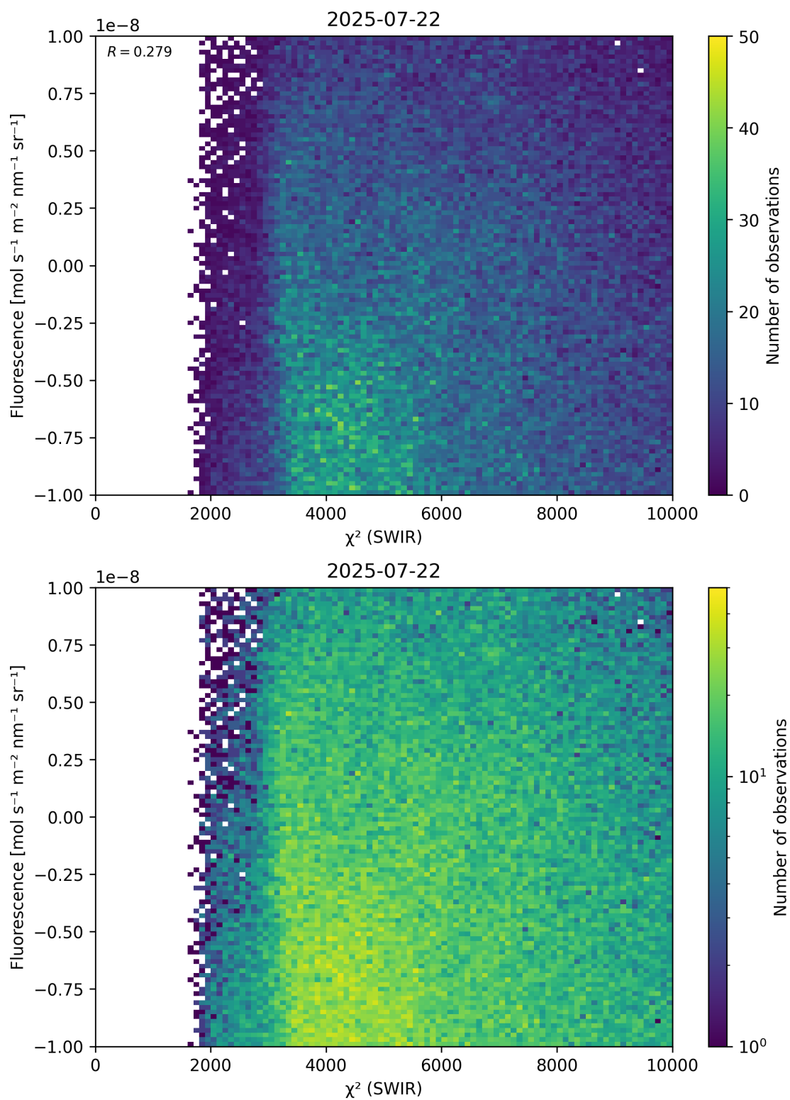
Figure 49: Scatter density plot of “ \chi^2 (SWIR)” against “Fluorescence” for 2025-07-21 to 2025-07-23.
