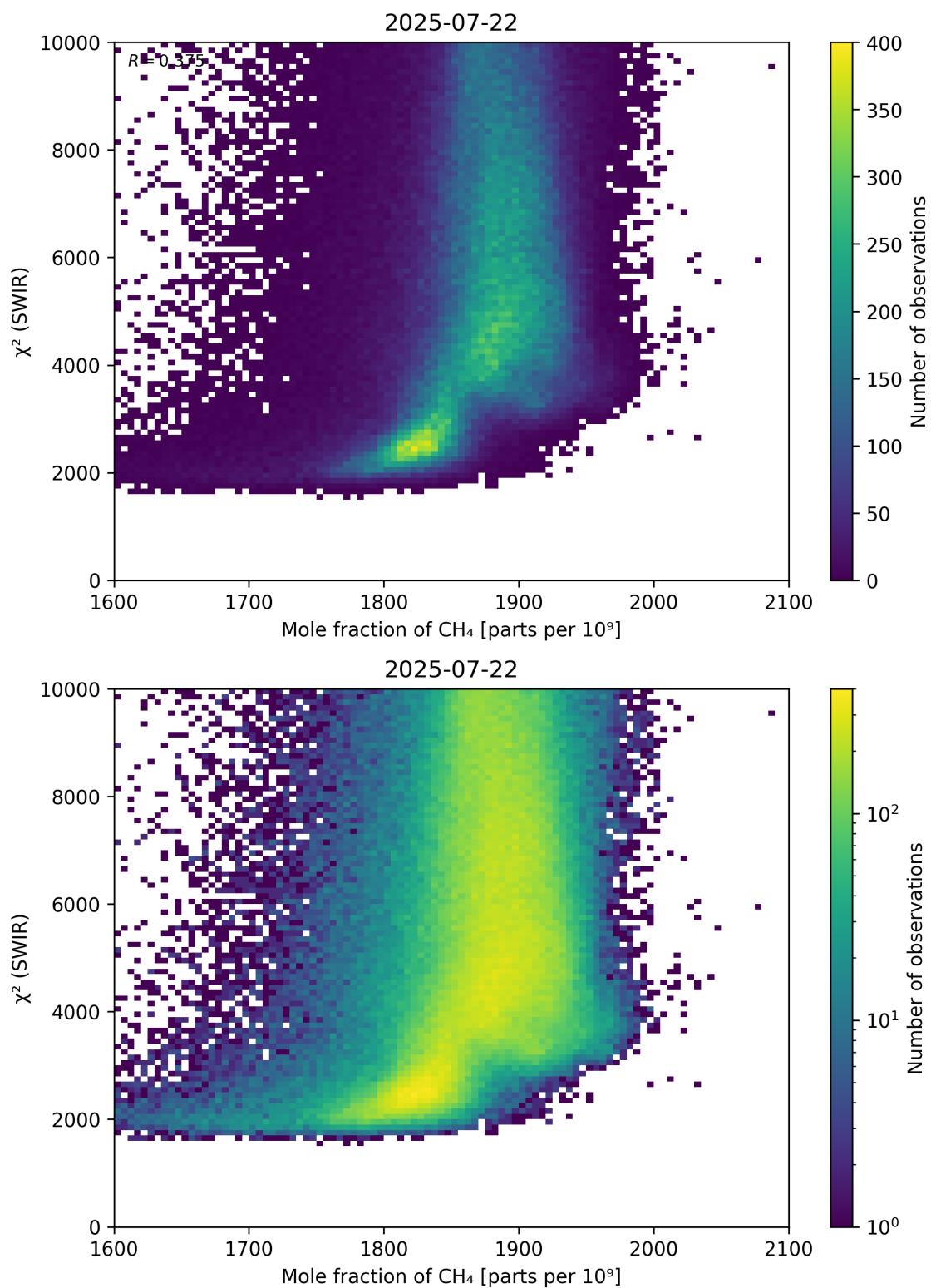
Figure 71: Scatter density plot of “Mole fraction of \text{CH}_4 ” against “ \chi^2 (SWIR)” for 2025-07-21 to 2025-07-23.
