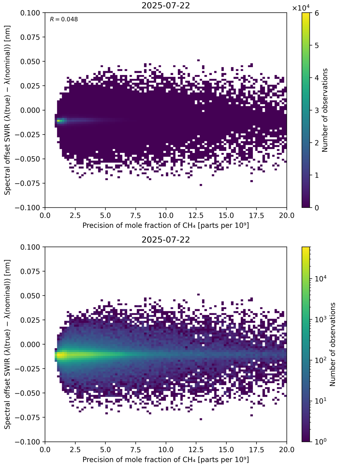
Figure 85: Scatter density plot of “Precision of mole fraction of CH 4 ” against “Spectral offset SWIR ( \lambda_{\text{true}} - \lambda_{\text{nominal}} )” for 2025-07-21 to 2025-07-23.
