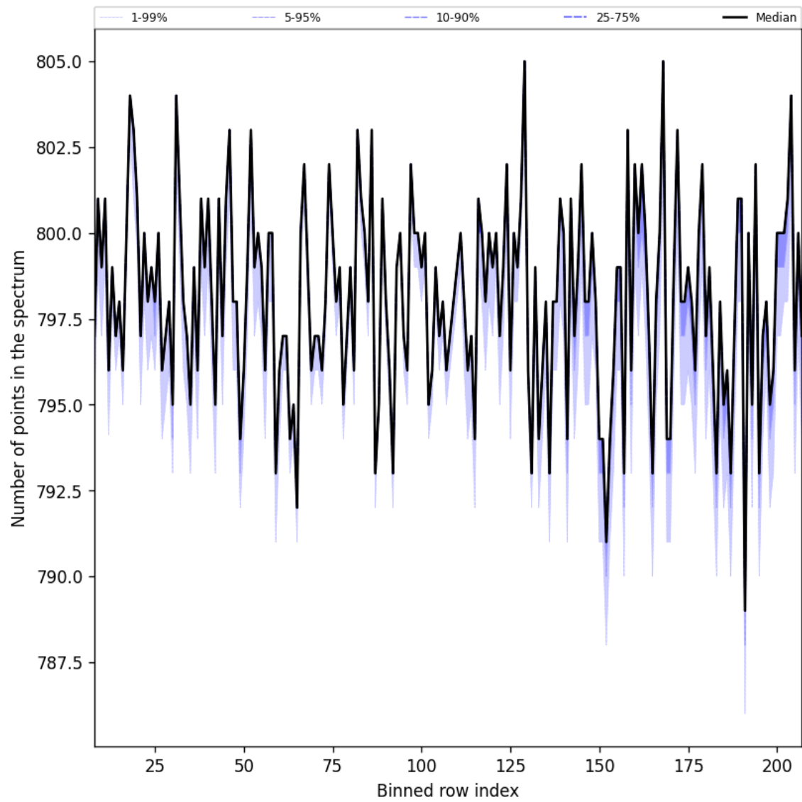
Figure 37: Along track statistics of “Number of points in the spectrum” for 2025-07-21 to 2025-07-23
