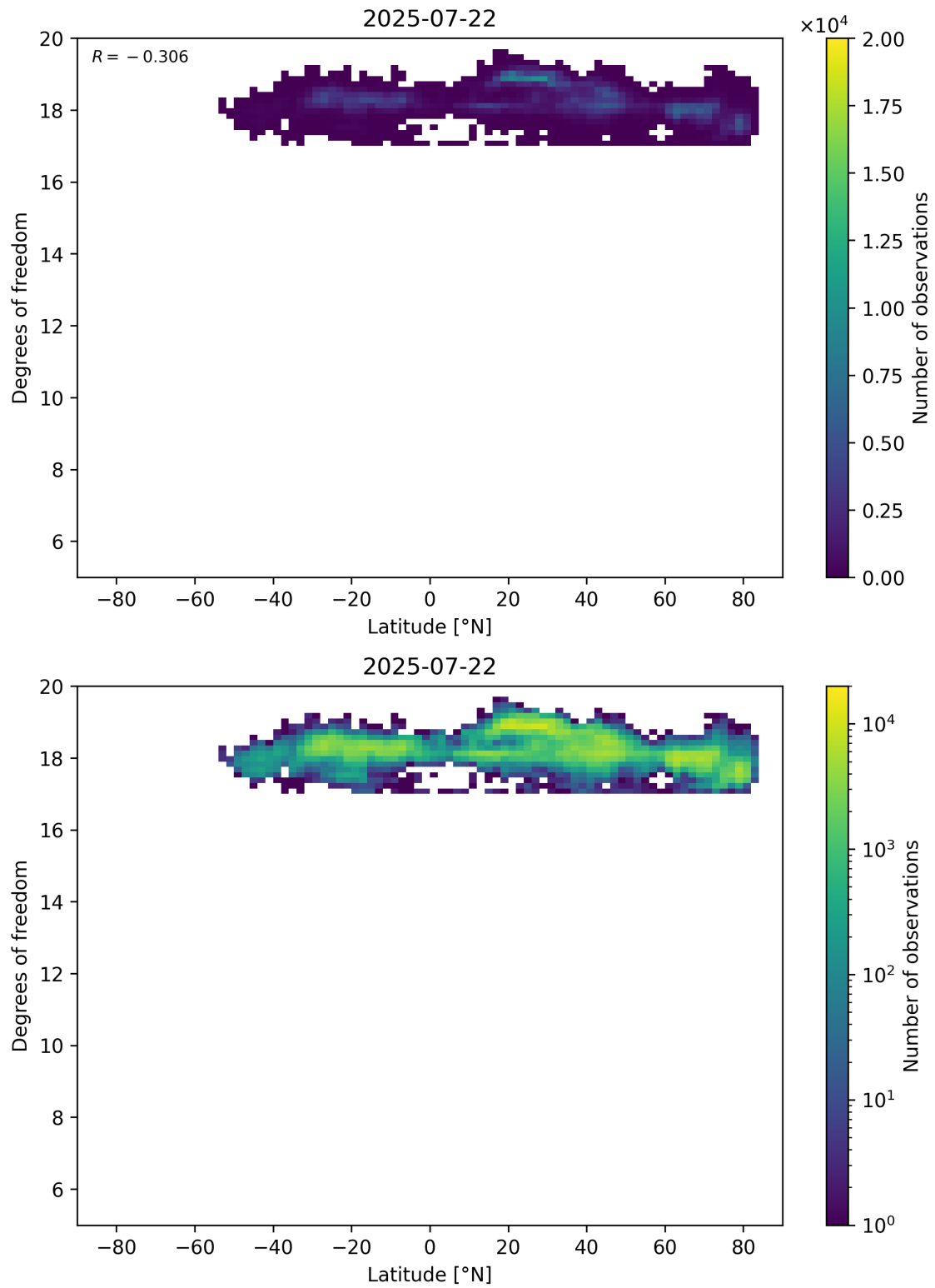
Figure 55: Scatter density plot of “Latitude” against “Degrees of freedom” for 2025-07-21 to 2025-07-23.
