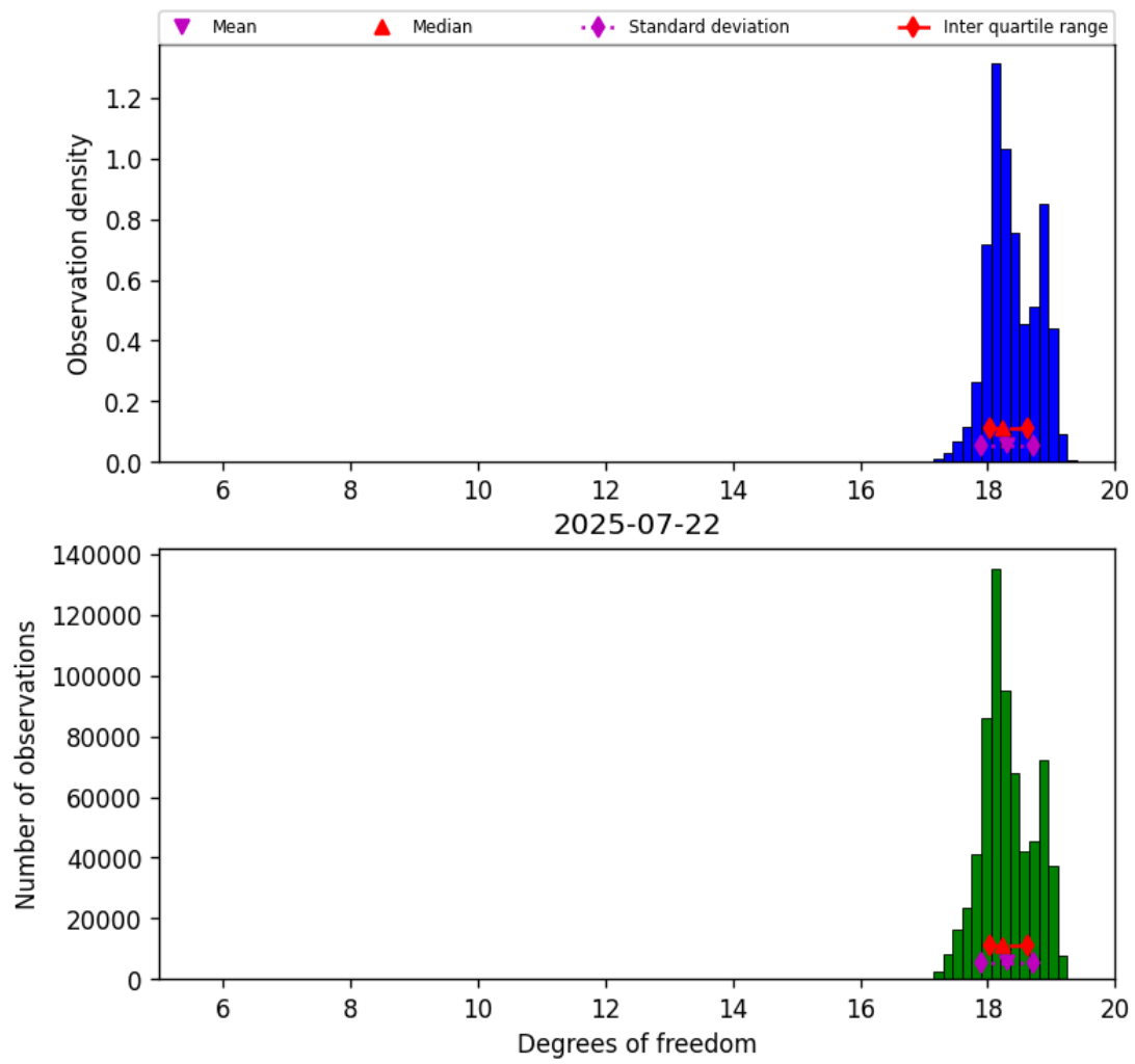
Figure 30: Histogram of “Degrees of freedom” for 2025-07-21 to 2025-07-23
