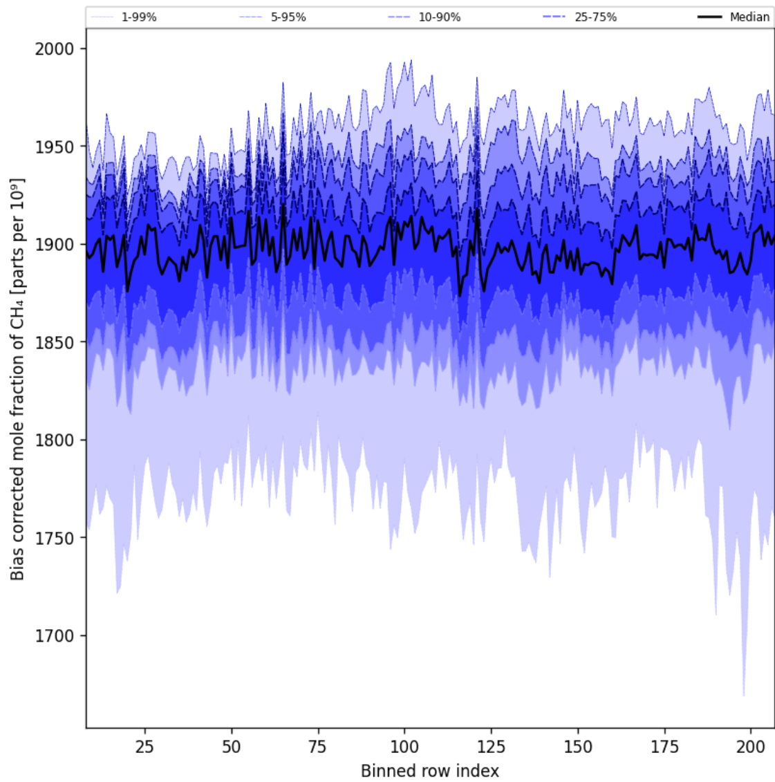
Figure 36: Along track statistics of “Bias corrected mole fraction of CH 4 ” for 2025-07-21 to 2025-07-23
