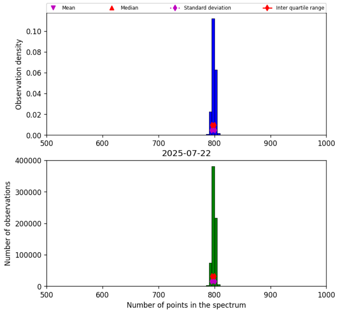
Figure 26: Histogram of “Number of points in the spectrum” for 2025-07-21 to 2025-07-23
