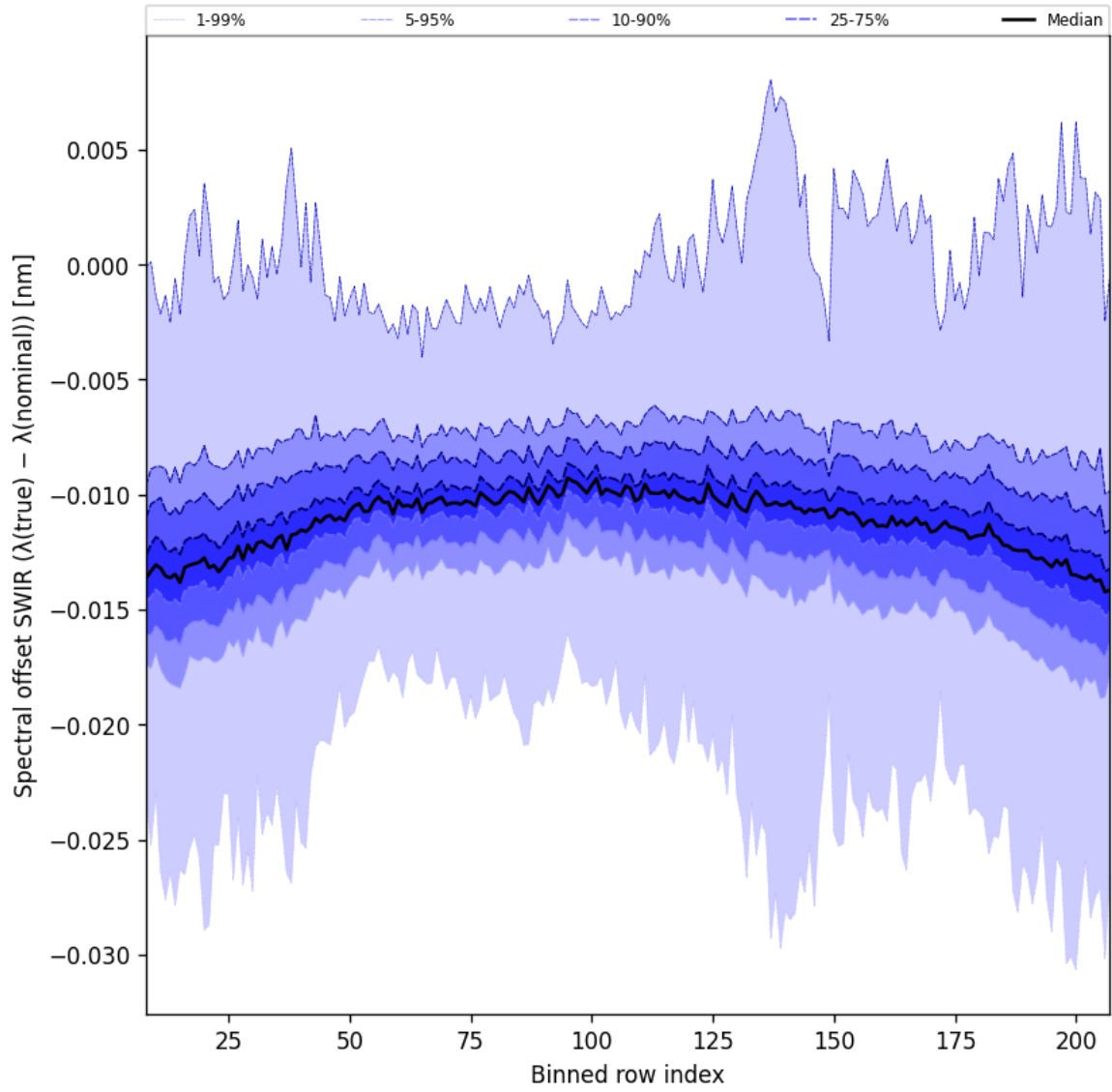
Figure 38: Along track statistics of “Spectral offset SWIR ( \lambda_{\text{true}} - \lambda_{\text{nominal}} )” for 2025-07-21 to 2025-07-23
