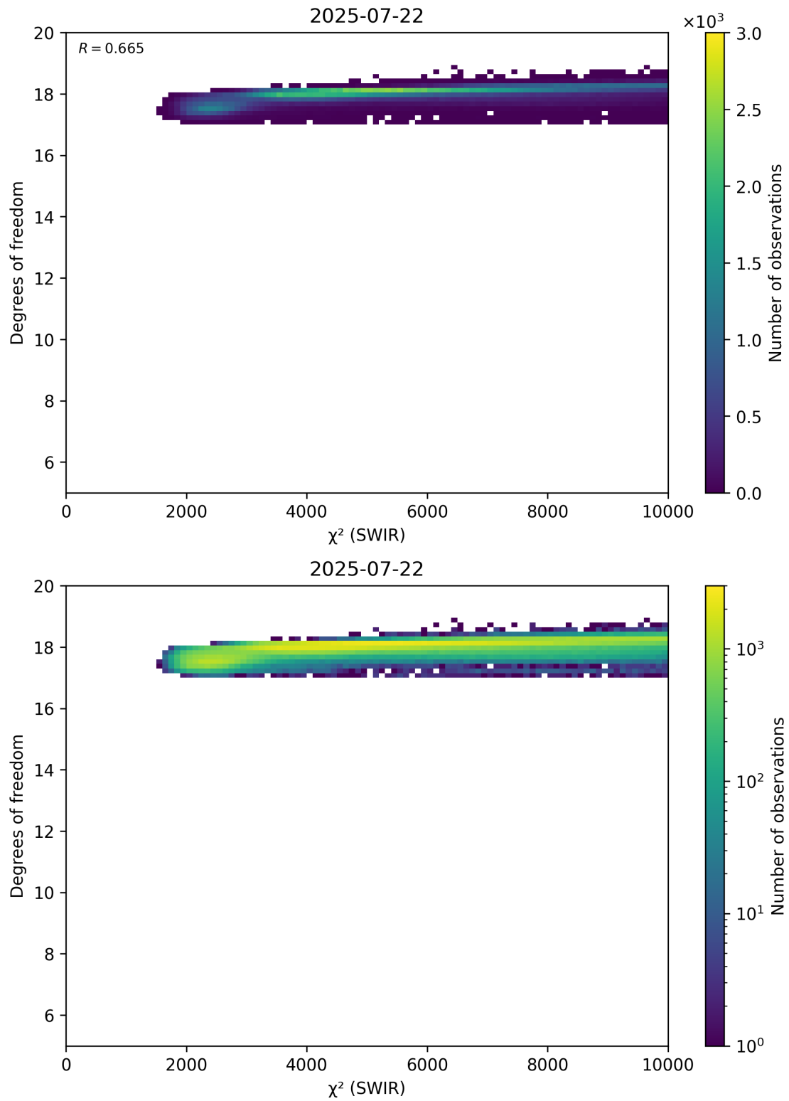
Figure 48: Scatter density plot of " \chi^2 (SWIR)" against "Degrees of freedom" for 2025-07-21 to 2025-07-23.
