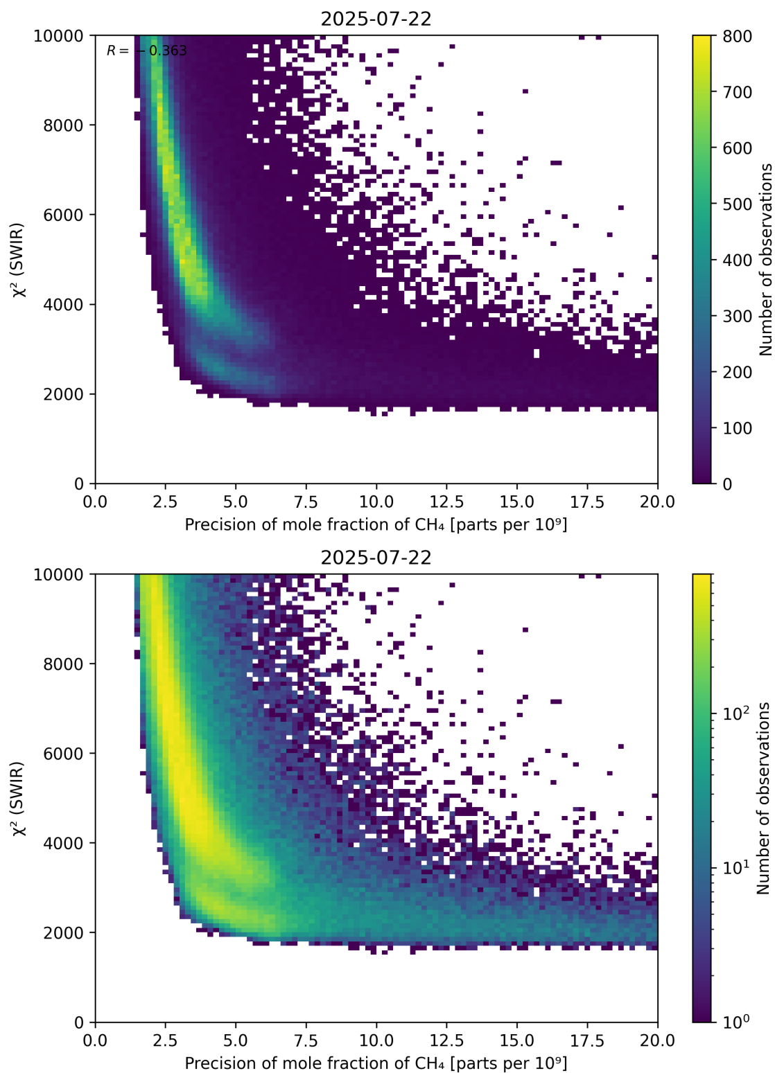
Figure 79: Scatter density plot of “Precision of mole fraction of \text{CH}_4 ” against “ \chi^2 (SWIR)” for 2025-07-21 to 2025-07-23.
