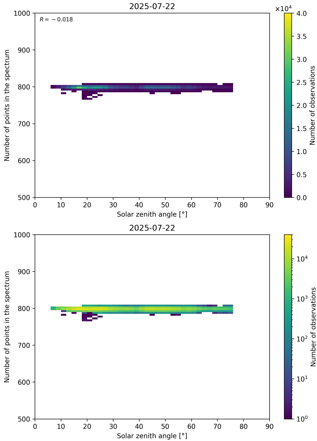
Figure 103: Scatter density plot of “Solar zenith angle” against “Number of points in the spectrum” for 2025-07-21 to 2025-07-23.
