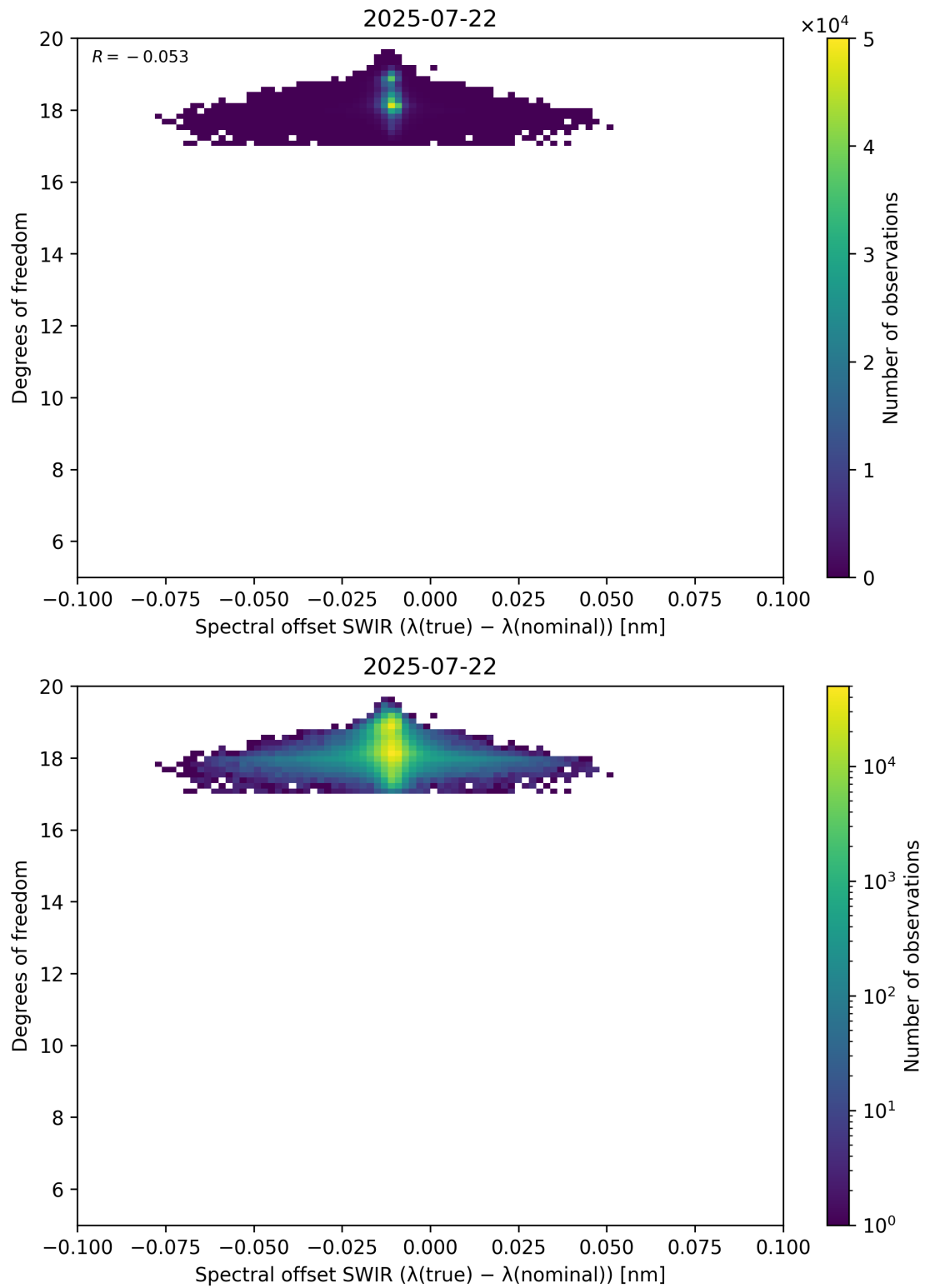
Figure 119: Scatter density plot of “Spectral offset SWIR ( \lambda_{\text{true}} - \lambda_{\text{nominal}} )” against “Degrees of freedom” for 2025-07-21 to 2025-07-23.
