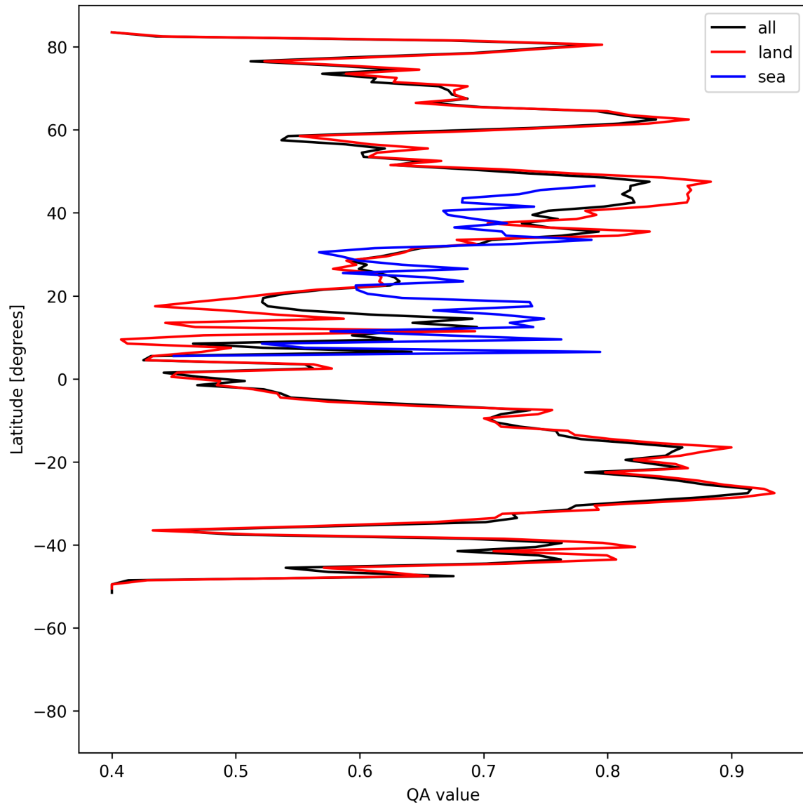
Figure 11: Zonal average of “QA value” for 2025-07-21 to 2025-07-23.
