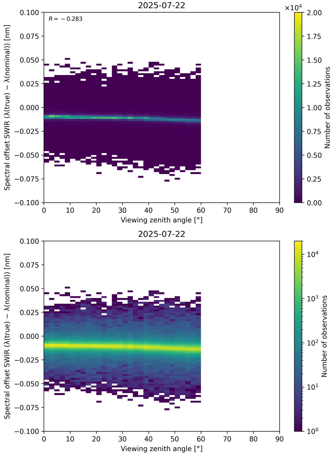
Figure 116: Scatter density plot of “Viewing zenith angle” against “Spectral offset SWIR ( \lambda_{\text{true}} - \lambda_{\text{nominal}} )” for 2025-07-21 to 2025-07-23.
