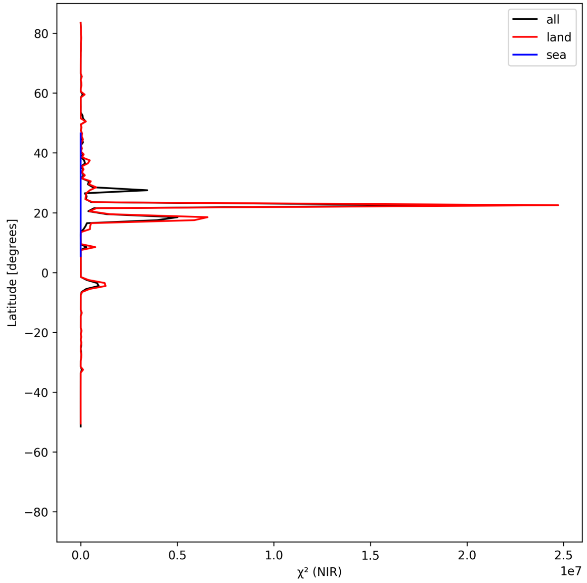
Figure 18: Zonal average of “ \chi^2 (NIR)” for 2025-07-21 to 2025-07-23.
