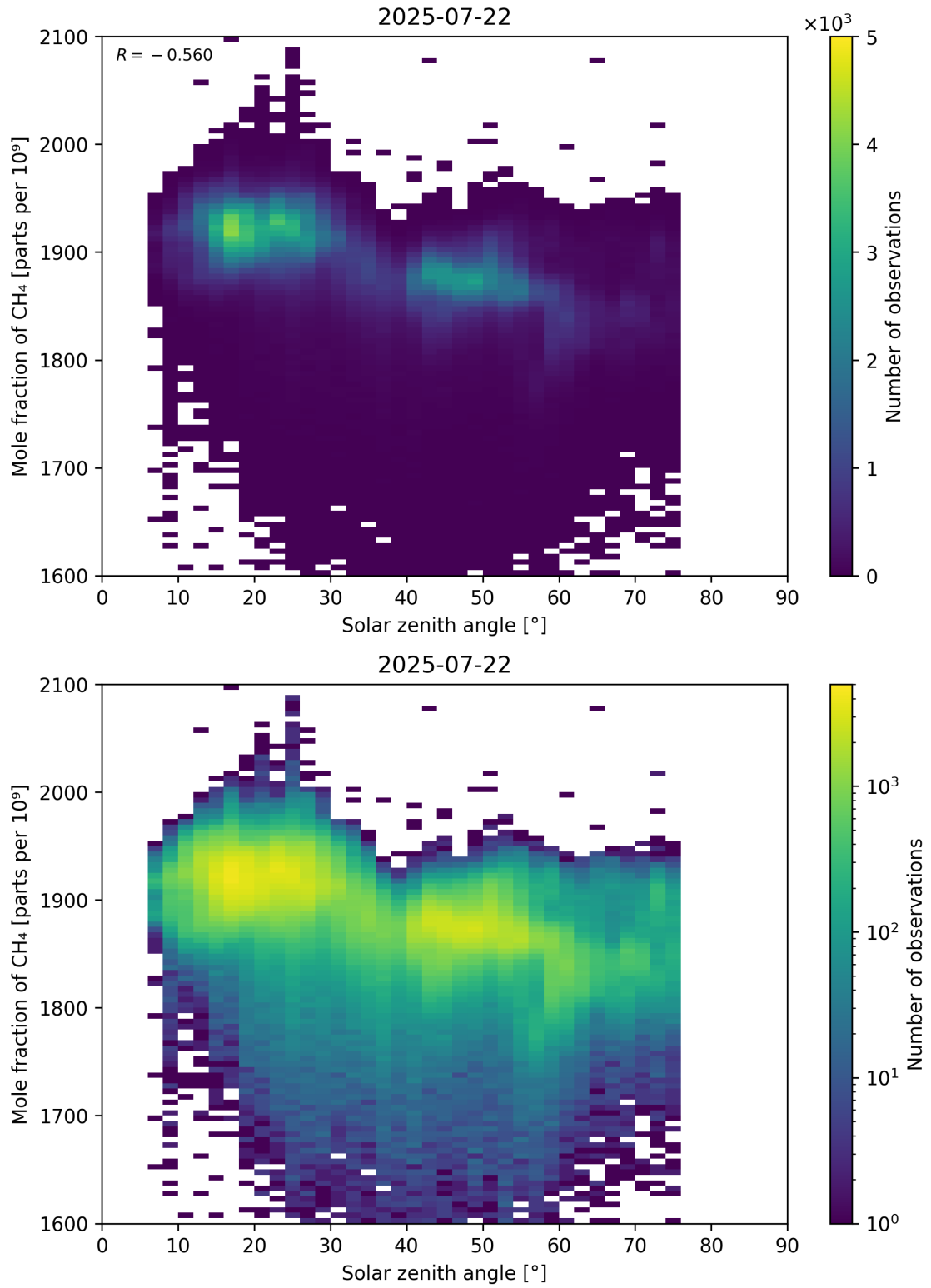
Figure 99: Scatter density plot of “Solar zenith angle” against “Mole fraction of CH 4 ” for 2025-07-21 to 2025-07-23.
