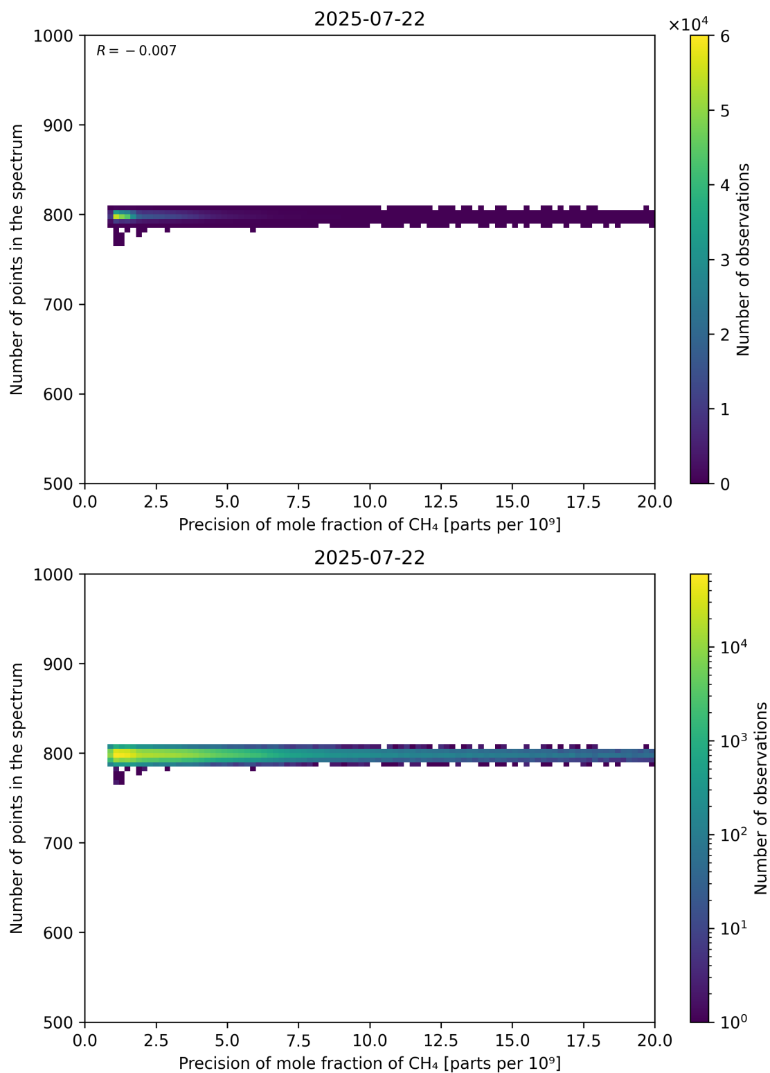
Figure 84: Scatter density plot of “Precision of mole fraction of CH 4 ” against “Number of points in the spectrum” for 2025-07-21 to 2025-07-23.
