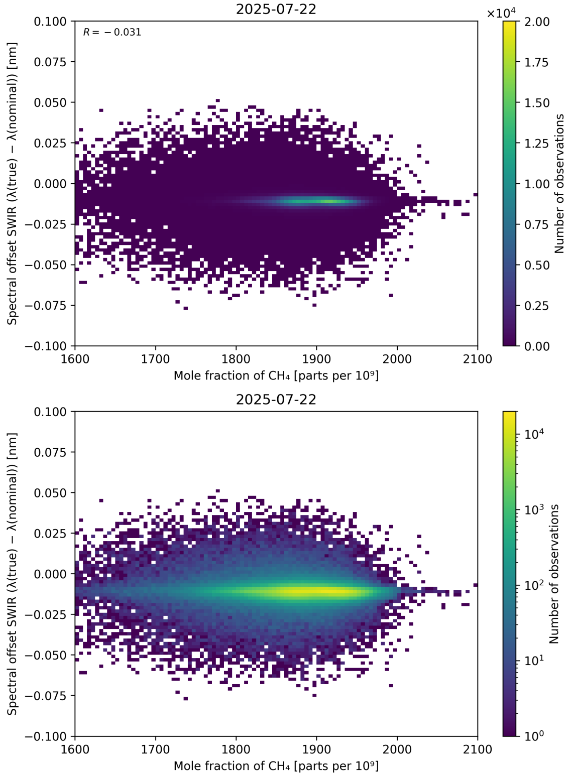
Figure 86: Scatter density plot of “Mole fraction of CH 4 ” against “Spectral offset SWIR ( \lambda_{\text{true}} - \lambda_{\text{nominal}} )” for 2025-07-21 to 2025-07-23.
