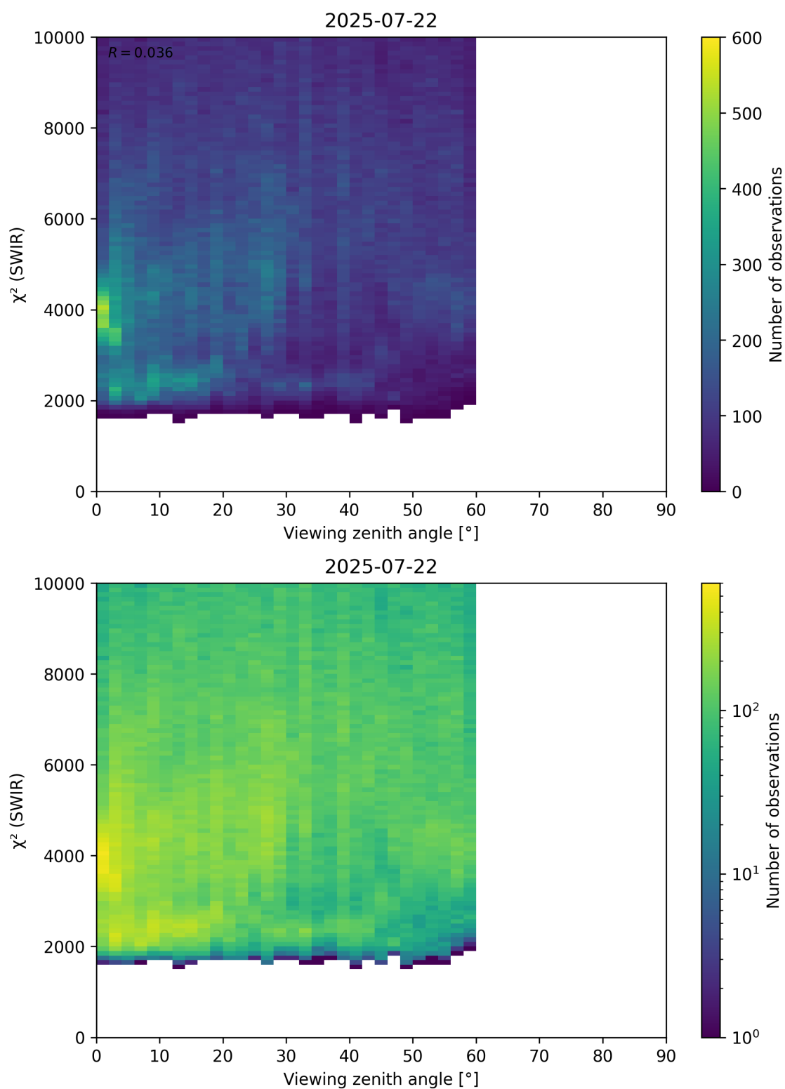
Figure 106: Scatter density plot of “Viewing zenith angle” against “ \chi^2 (SWIR)” for 2025-07-21 to 2025-07-23.
