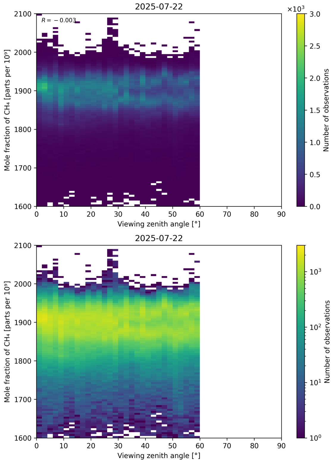
Figure 110: Scatter density plot of “Viewing zenith angle” against “Mole fraction of CH 4 ” for 2025-07-21 to 2025-07-23.
