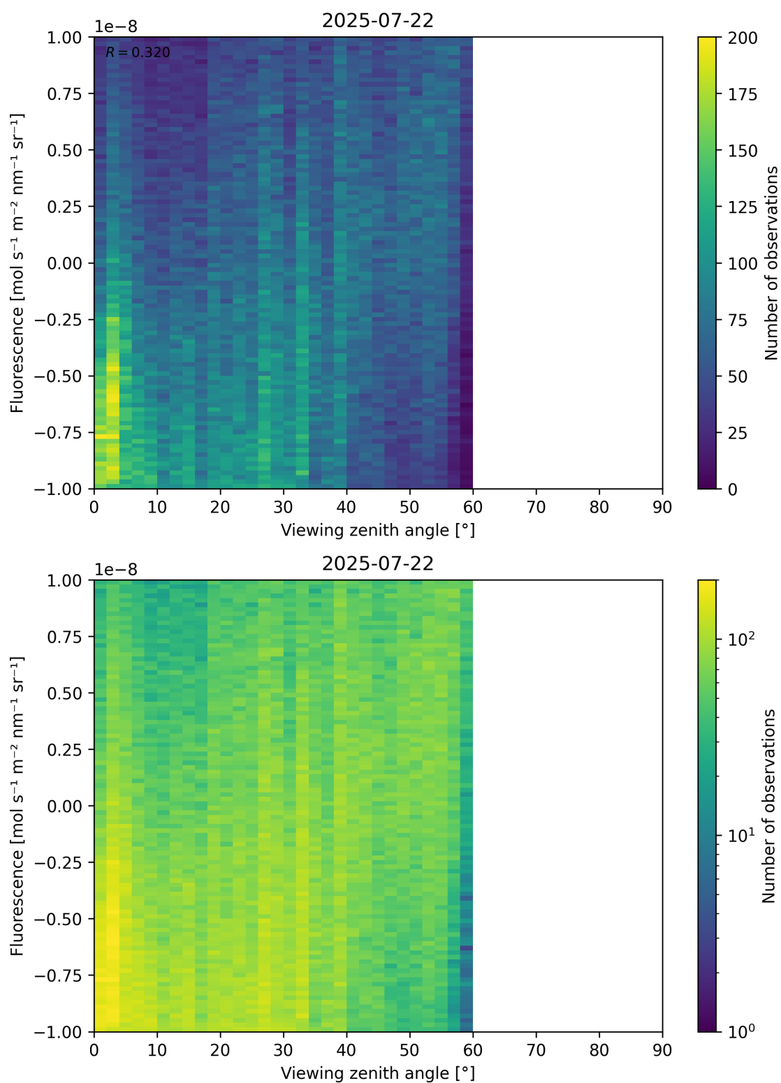
Figure 108: Scatter density plot of “Viewing zenith angle” against “Fluorescence” for 2025-07-21 to 2025-07-23.
