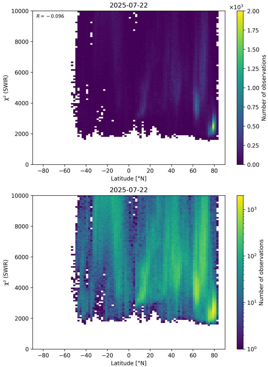
Figure 54: Scatter density plot of “Latitude” against “ \chi^2 (SWIR)” for 2025-07-21 to 2025-07-23.
