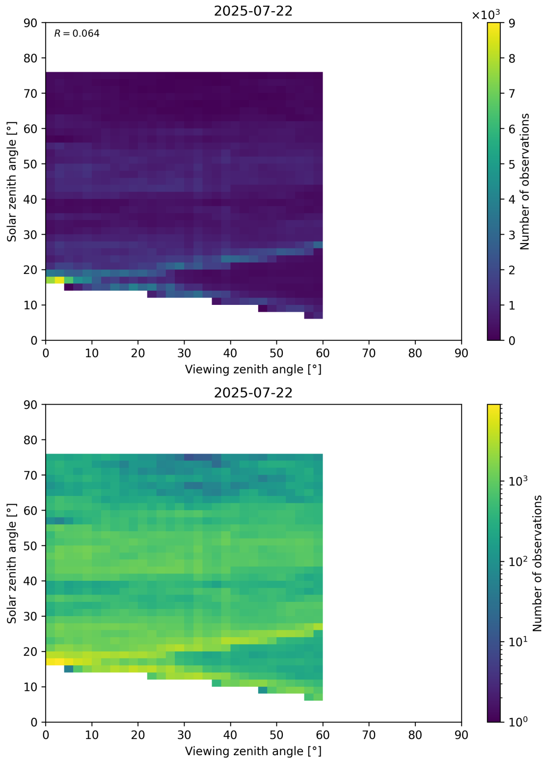
Figure 115: Scatter density plot of “Viewing zenith angle” against “Solar zenith angle” for 2025-07-21 to 2025-07-23.
