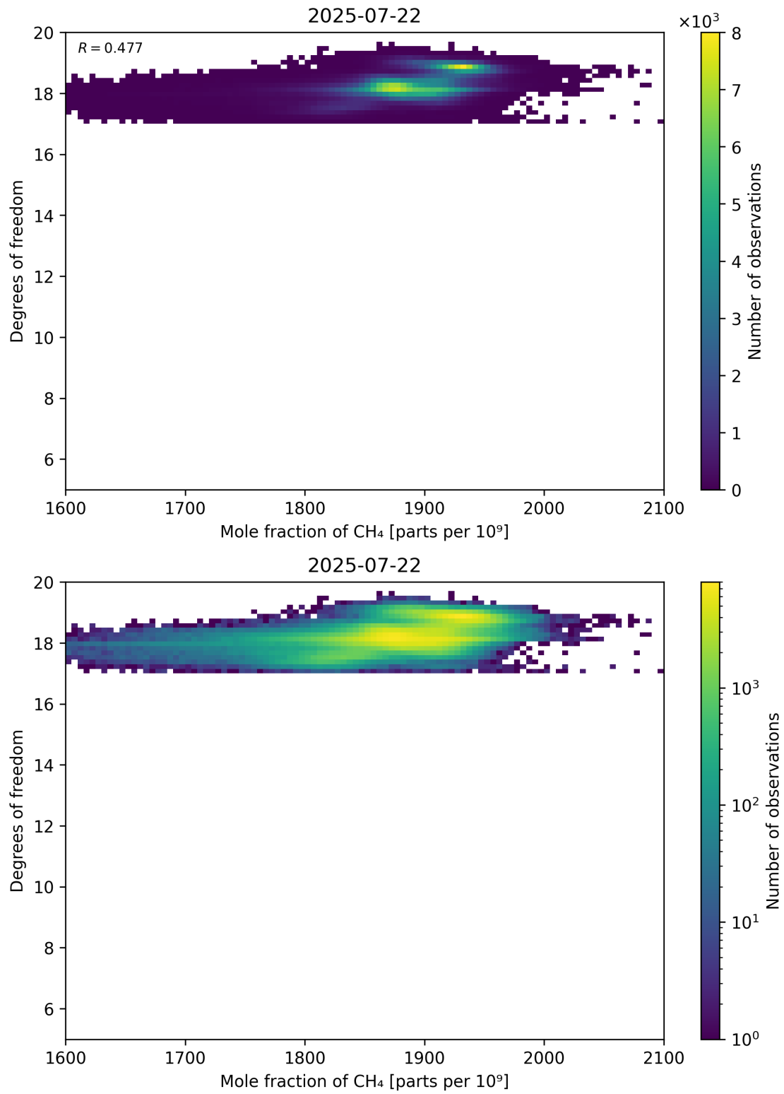
Figure 72: Scatter density plot of “Mole fraction of CH 4 ” against “Degrees of freedom” for 2025-07-21 to 2025-07-23.
