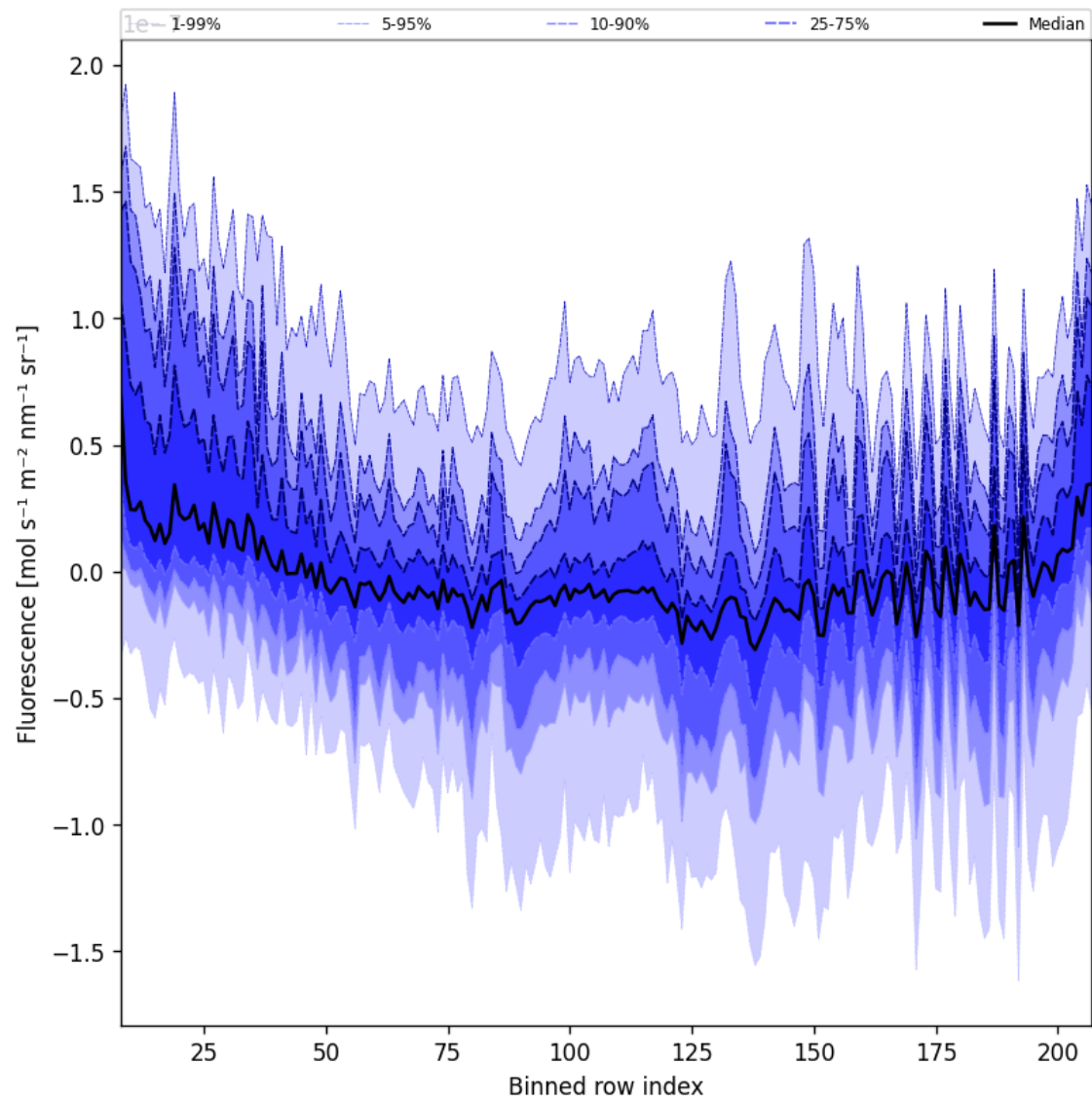
Figure 43: Along track statistics of “Fluorescence” for 2025-07-21 to 2025-07-23
