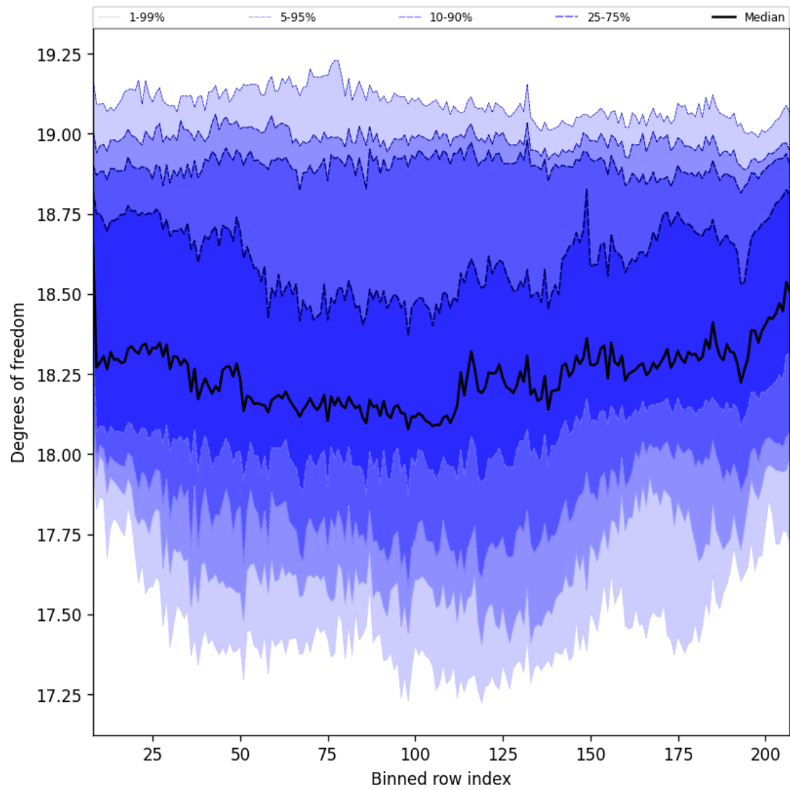
Figure 41: Along track statistics of “Degrees of freedom” for 2025-07-21 to 2025-07-23
