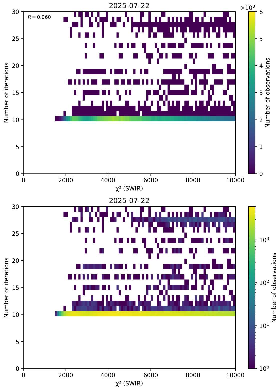
Figure 50: Scatter density plot of “ \chi^2 (SWIR)” against “Number of iterations” for 2025-07-21 to 2025-07-23.
