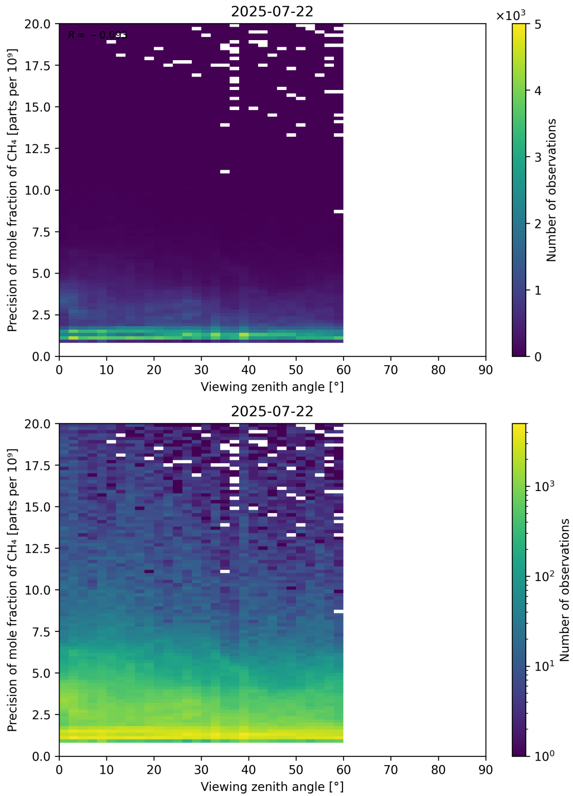
Figure 112: Scatter density plot of “Viewing zenith angle” against “Precision of mole fraction of CH 4 ” for 2025-07-21 to 2025-07-23.
