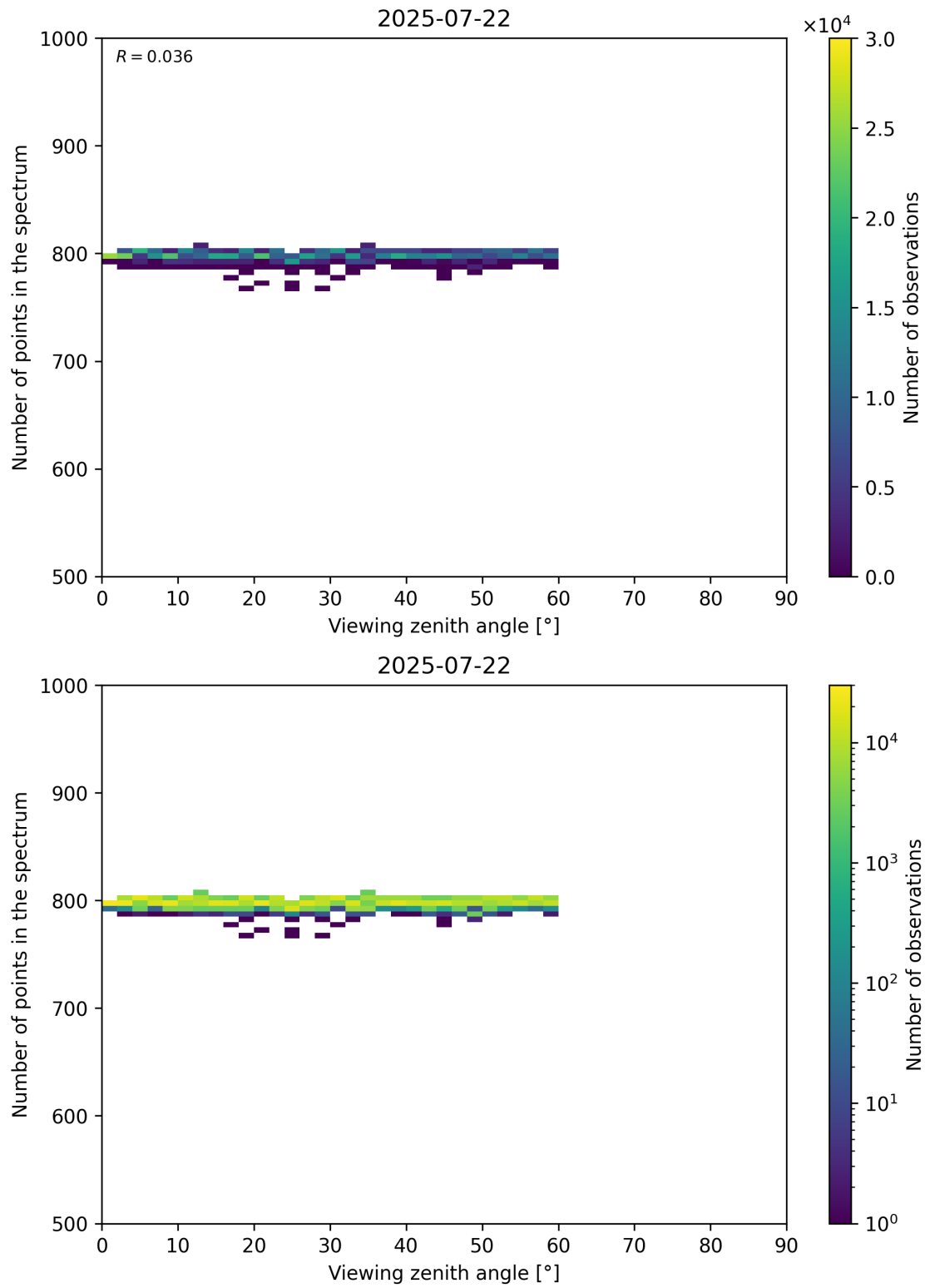
Figure 114: Scatter density plot of “Viewing zenith angle” against “Number of points in the spectrum” for 2025-07-21 to 2025-07-23.
