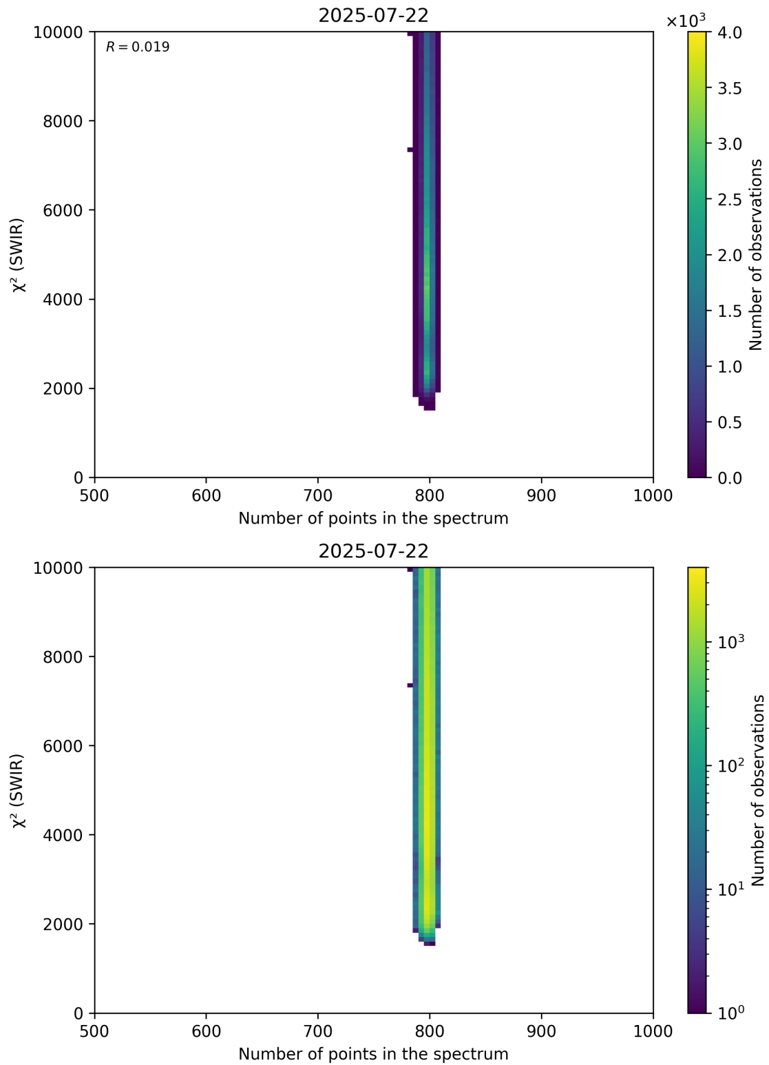
Figure 89: Scatter density plot of “Number of points in the spectrum” against “ \chi^2 (SWIR)” for 2025-07-21 to 2025-07-23.
