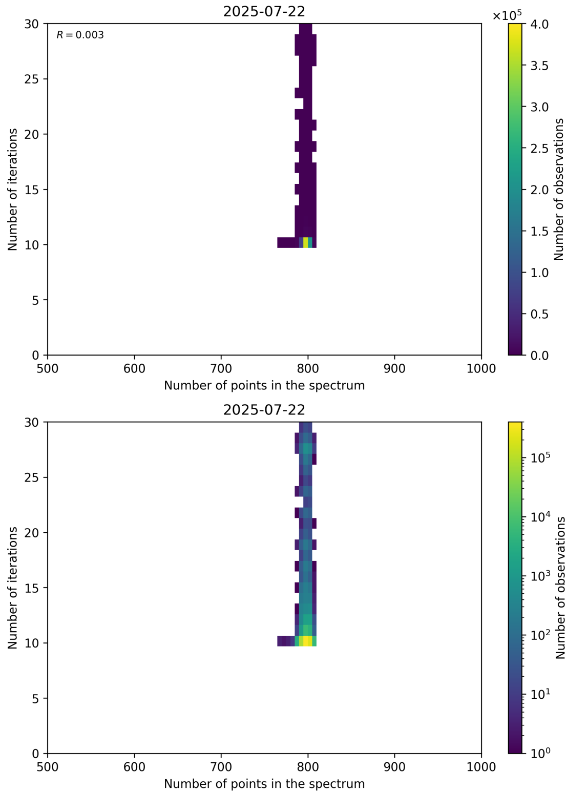
Figure 92: Scatter density plot of “Number of points in the spectrum” against “Number of iterations” for 2025-07-21 to 2025-07-23.
