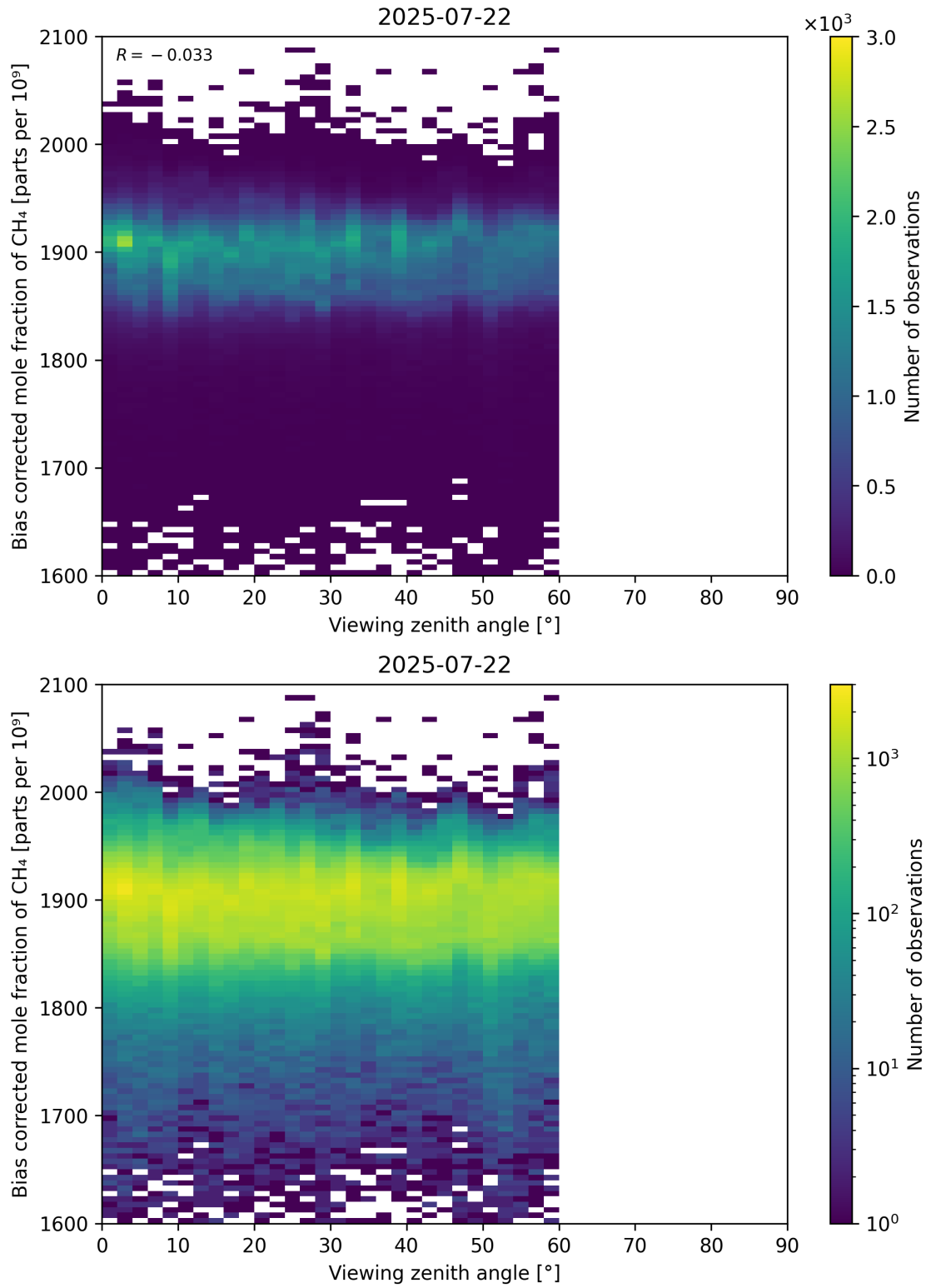
Figure 111: Scatter density plot of “Viewing zenith angle” against “Bias corrected mole fraction of CH 4 ” for 2025-07-21 to 2025-07-23.
