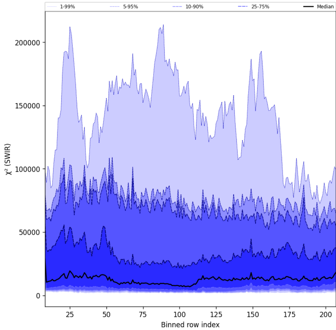
Figure 39: Along track statistics of “ \chi^2 (SWIR)” for 2025-07-21 to 2025-07-23
