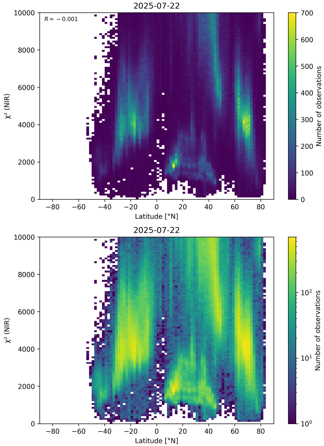
Figure 53: Scatter density plot of “Latitude” against “ \chi^2 (NIR)” for 2025-07-21 to 2025-07-23.
