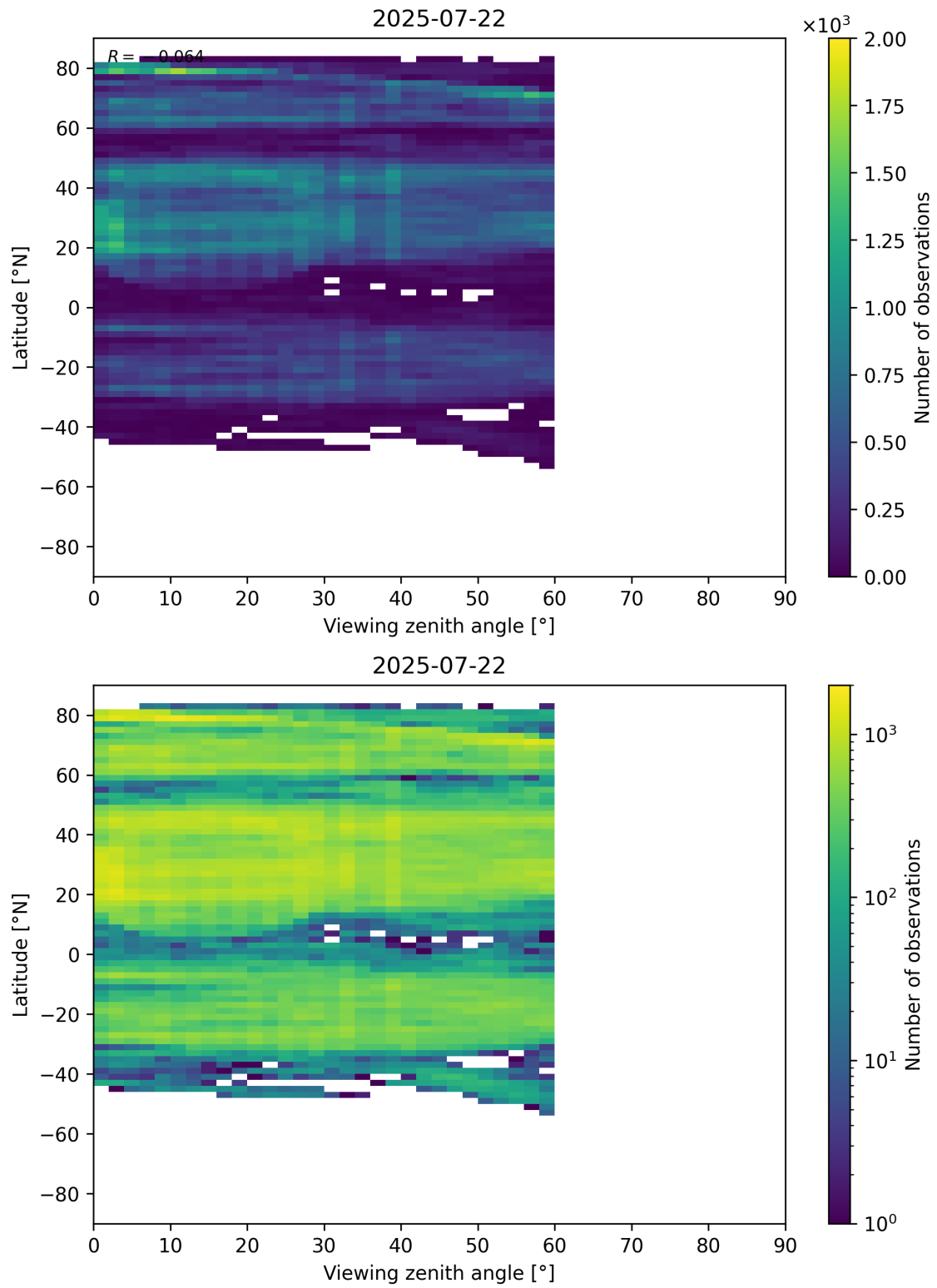
Figure 109: Scatter density plot of “Viewing zenith angle” against “Latitude” for 2025-07-21 to 2025-07-23.
