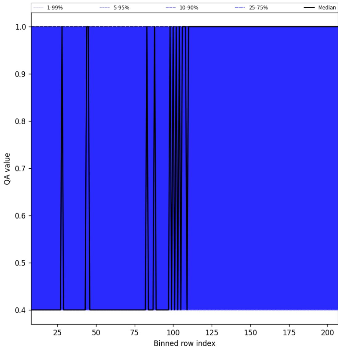
Figure 33: Along track statistics of “QA value” for 2025-07-21 to 2025-07-23
