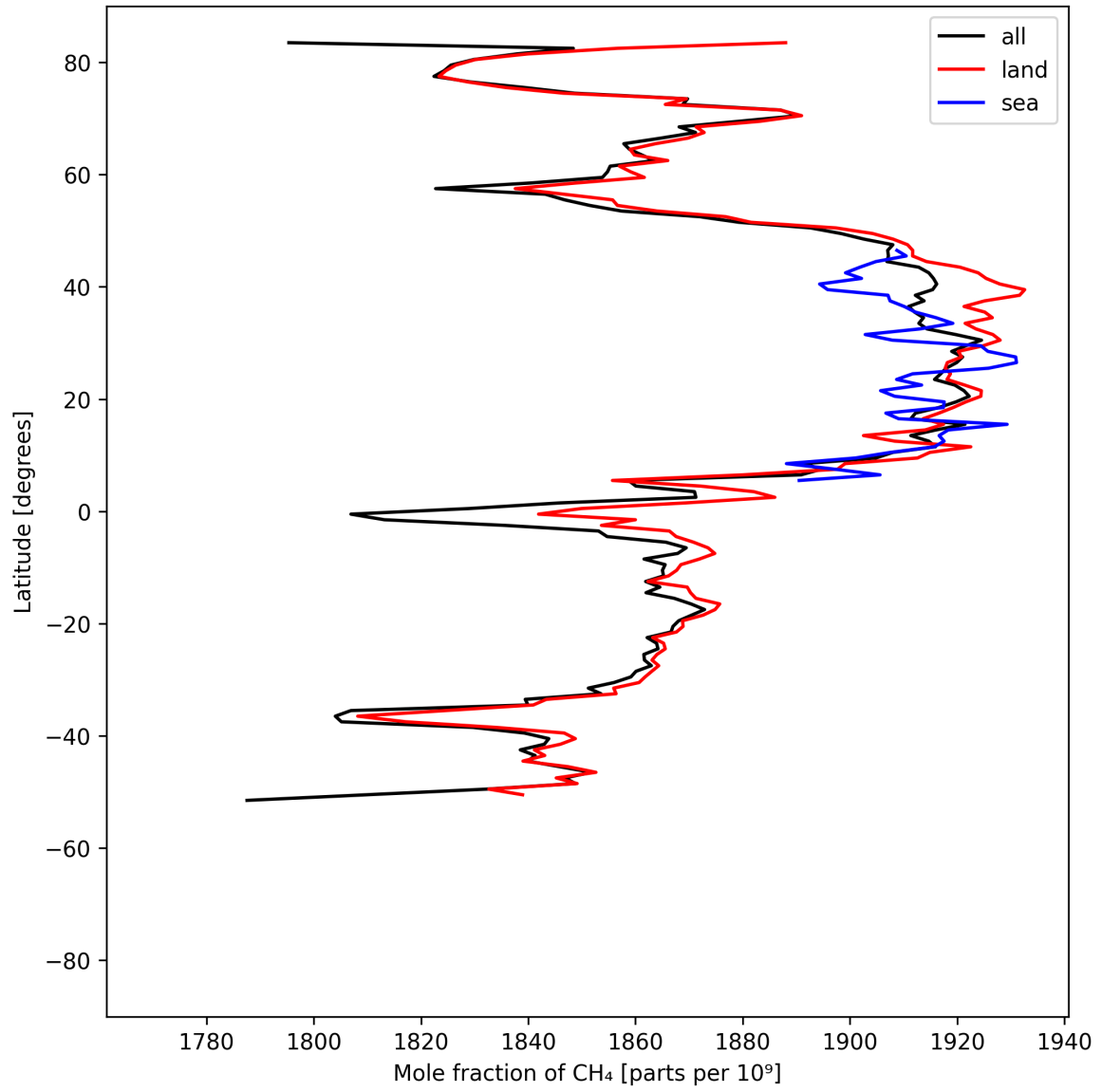
Figure 12: Zonal average of “Mole fraction of \text{CH}_4 ” for 2025-07-21 to 2025-07-23.
