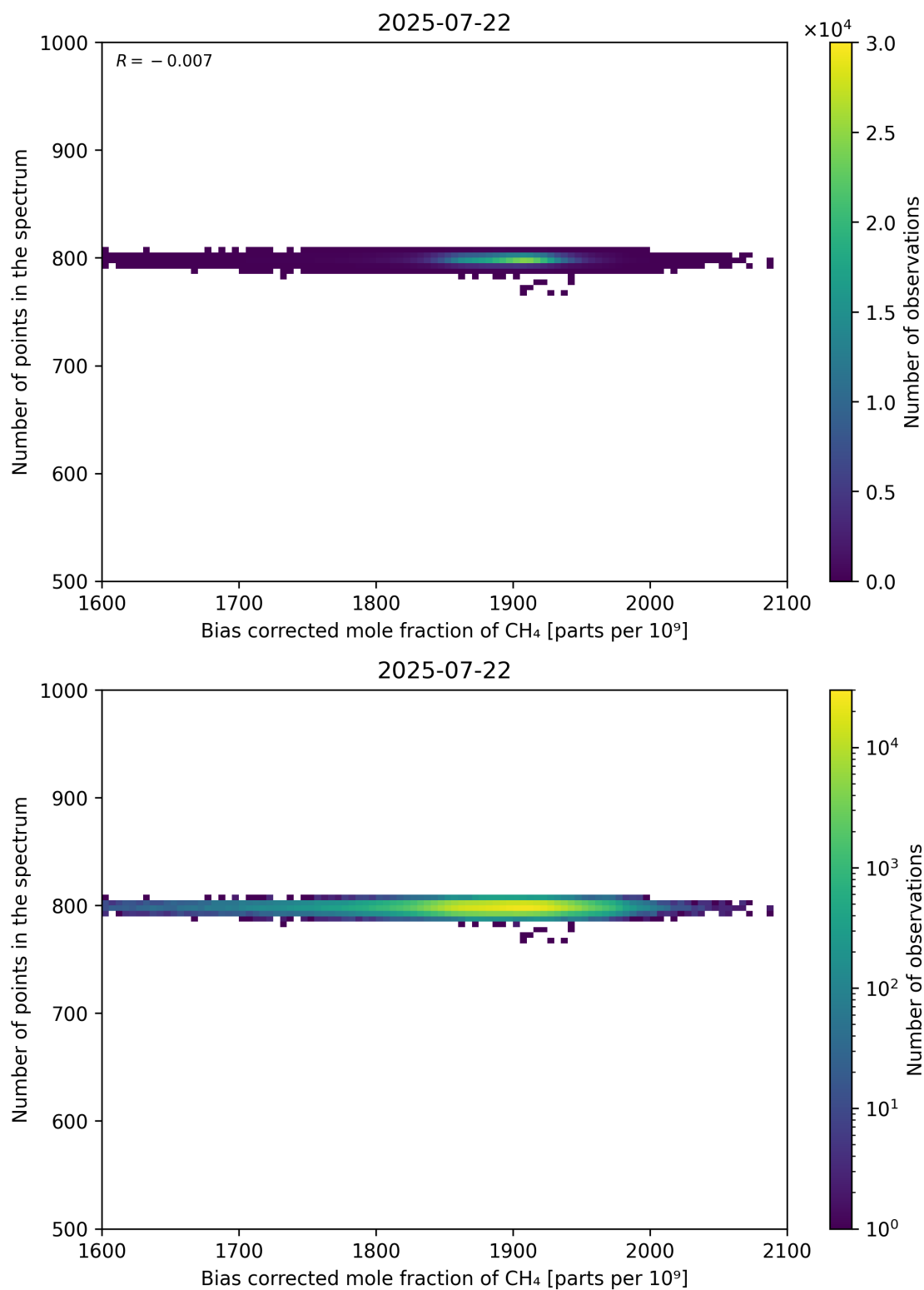
Figure 68: Scatter density plot of “Bias corrected mole fraction of CH 4 ” against “Number of points in the spectrum” for 2025-07-21 to 2025-07-23.
