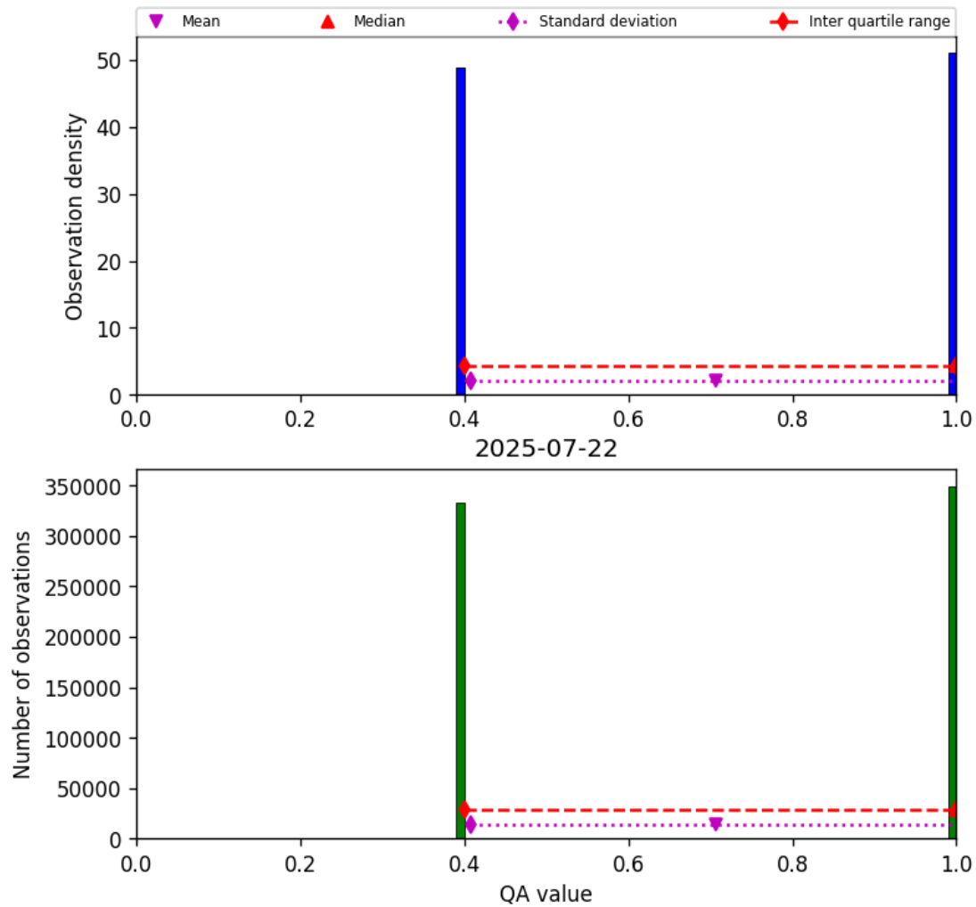
Figure 22: Histogram of “QA value” for 2025-07-21 to 2025-07-23
