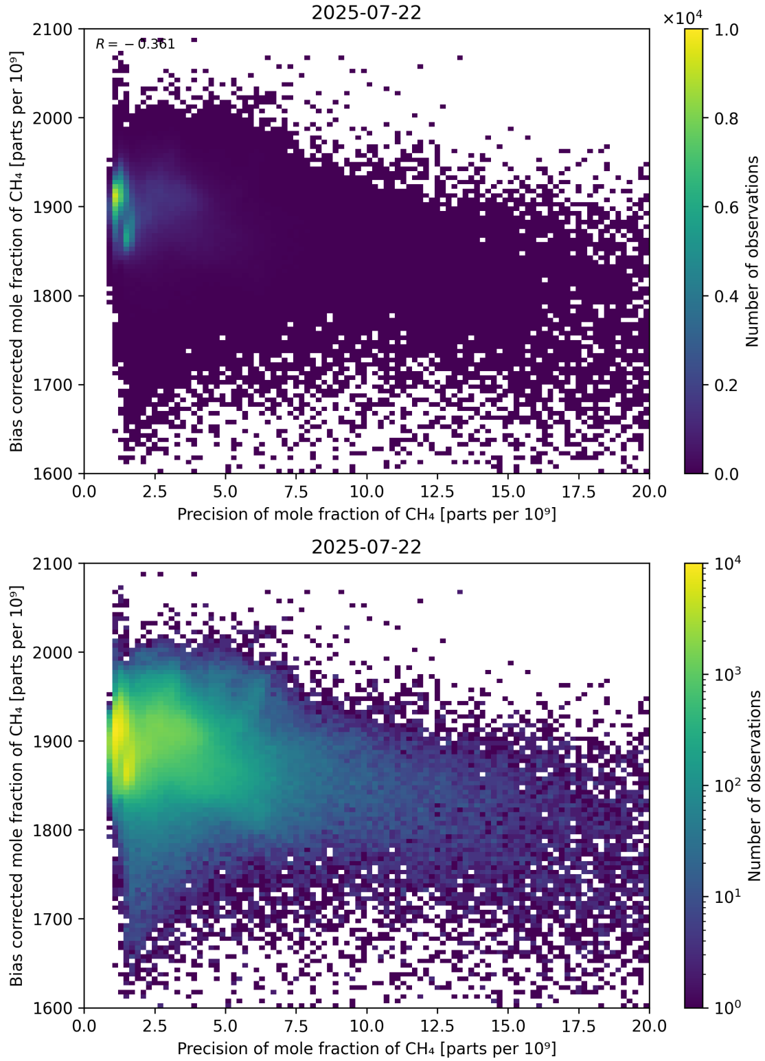
Figure 82: Scatter density plot of “Precision of mole fraction of CH 4 ” against “Bias corrected mole fraction of CH 4 ” for 2025-07-21 to 2025-07-23.
