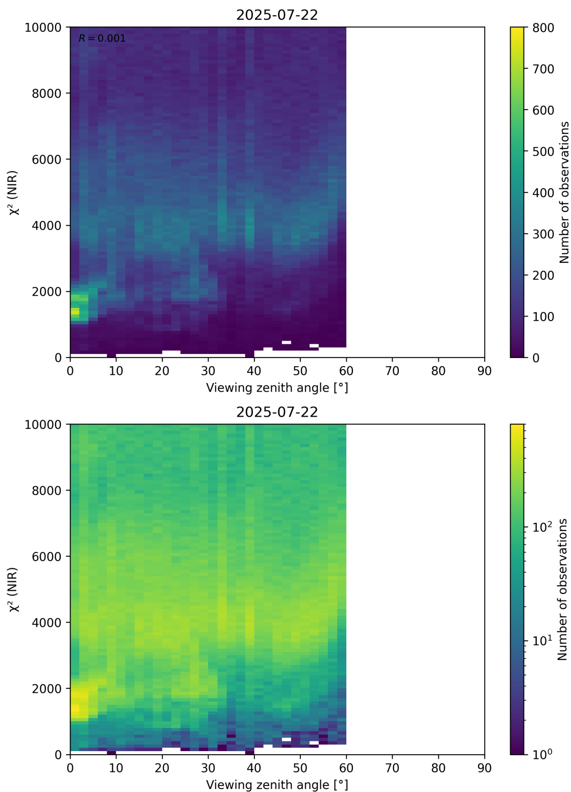
Figure 105: Scatter density plot of “Viewing zenith angle” against “ \chi^2 (NIR)” for 2025-07-21 to 2025-07-23.
