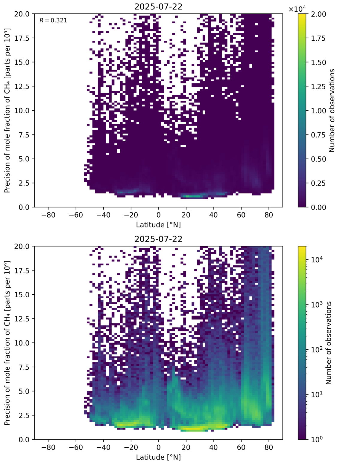
Figure 59: Scatter density plot of “Latitude” against “Precision of mole fraction of \text{CH}_4 ” for 2025-07-21 to 2025-07-23.
