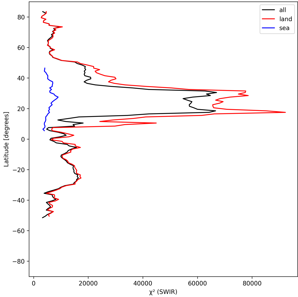
Figure 17: Zonal average of “ \chi^2 (SWIR)” for 2025-07-21 to 2025-07-23.
