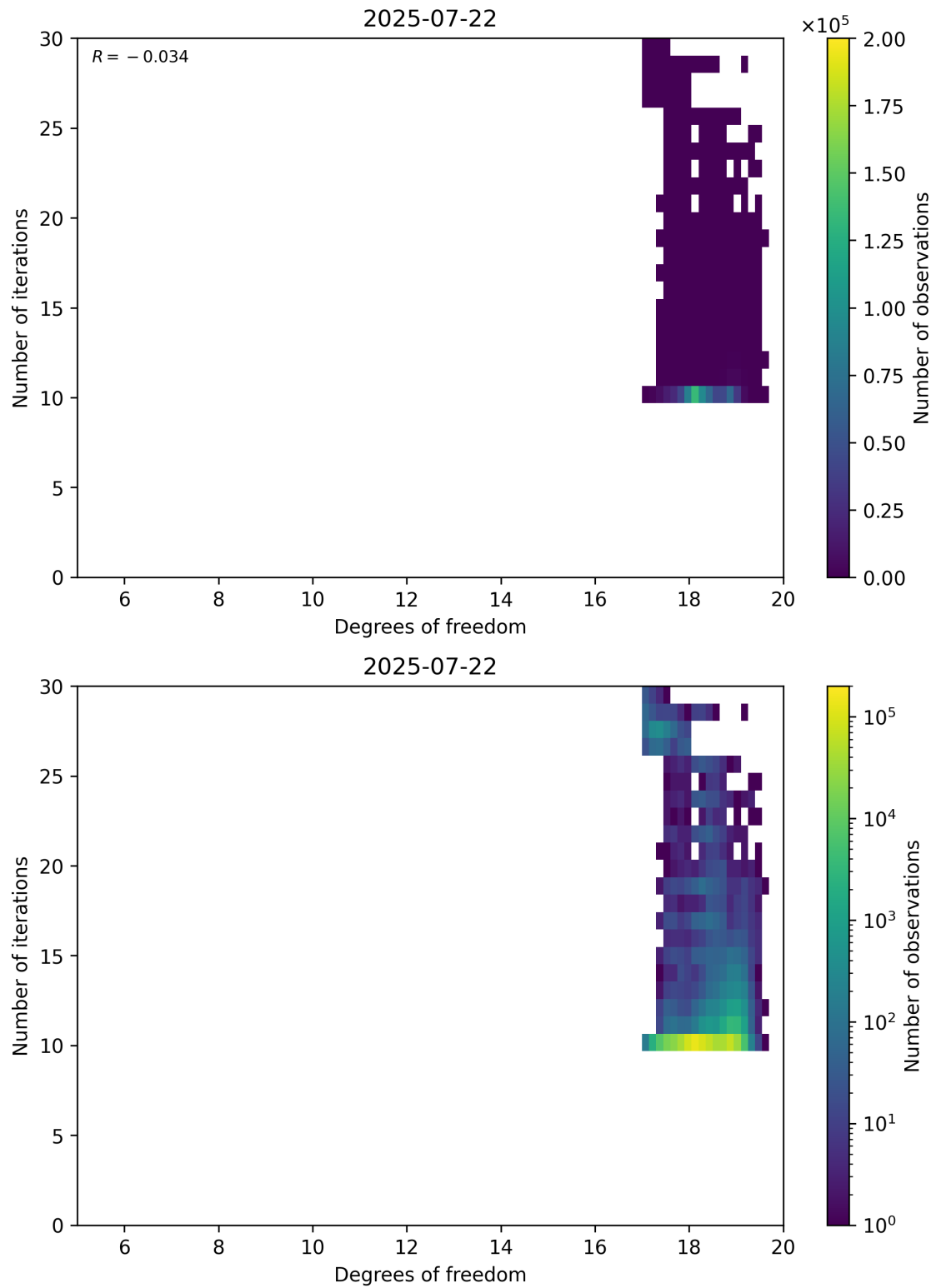
Figure 52: Scatter density plot of “Degrees of freedom” against “Number of iterations” for 2025-07-21 to 2025-07-23.
