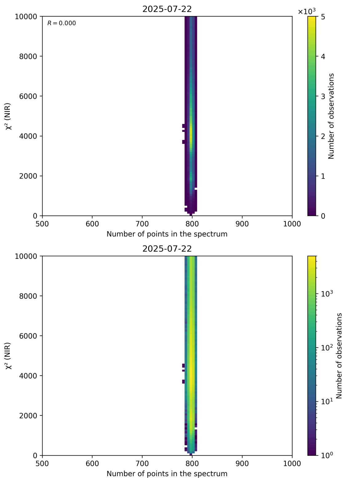
Figure 88: Scatter density plot of “Number of points in the spectrum” against “ \chi^2 (NIR)” for 2025-07-21 to 2025-07-23.
