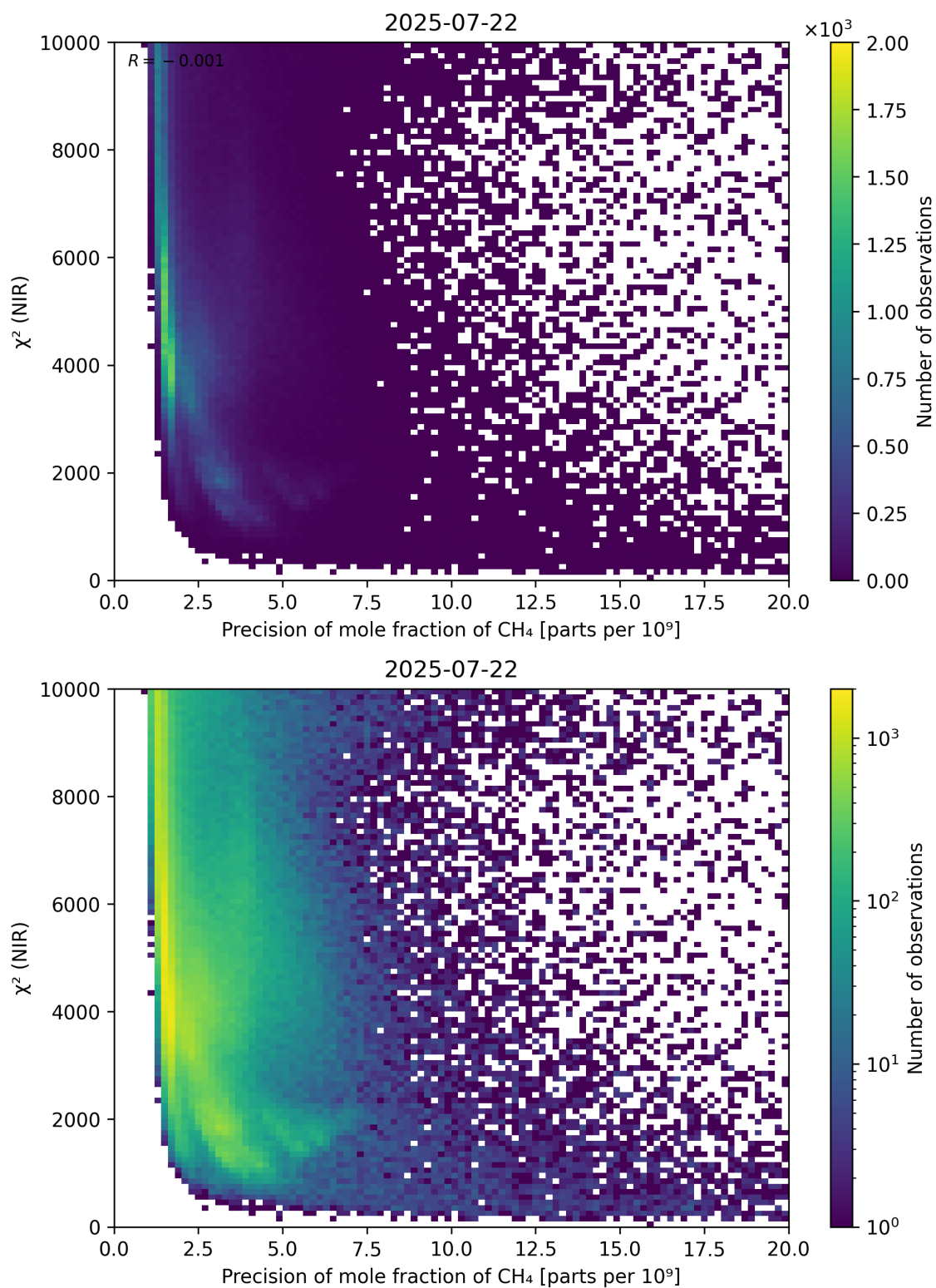
Figure 78: Scatter density plot of “Precision of mole fraction of \text{CH}_4 ” against “ \chi^2 (NIR)” for 2025-07-21 to 2025-07-23.
