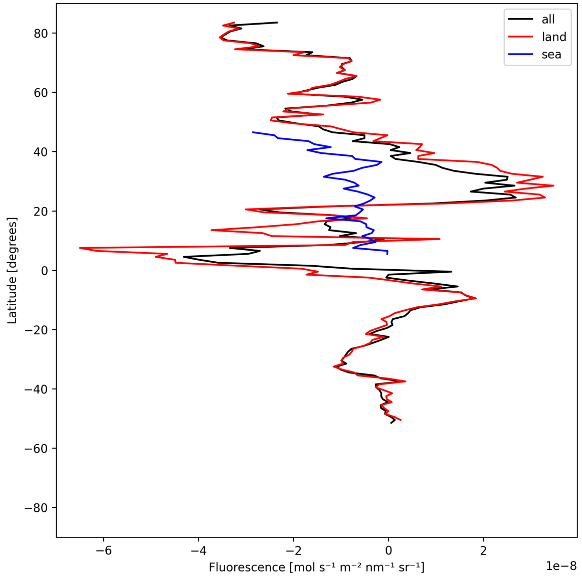
Figure 21: Zonal average of “Fluorescence” for 2025-07-21 to 2025-07-23.
