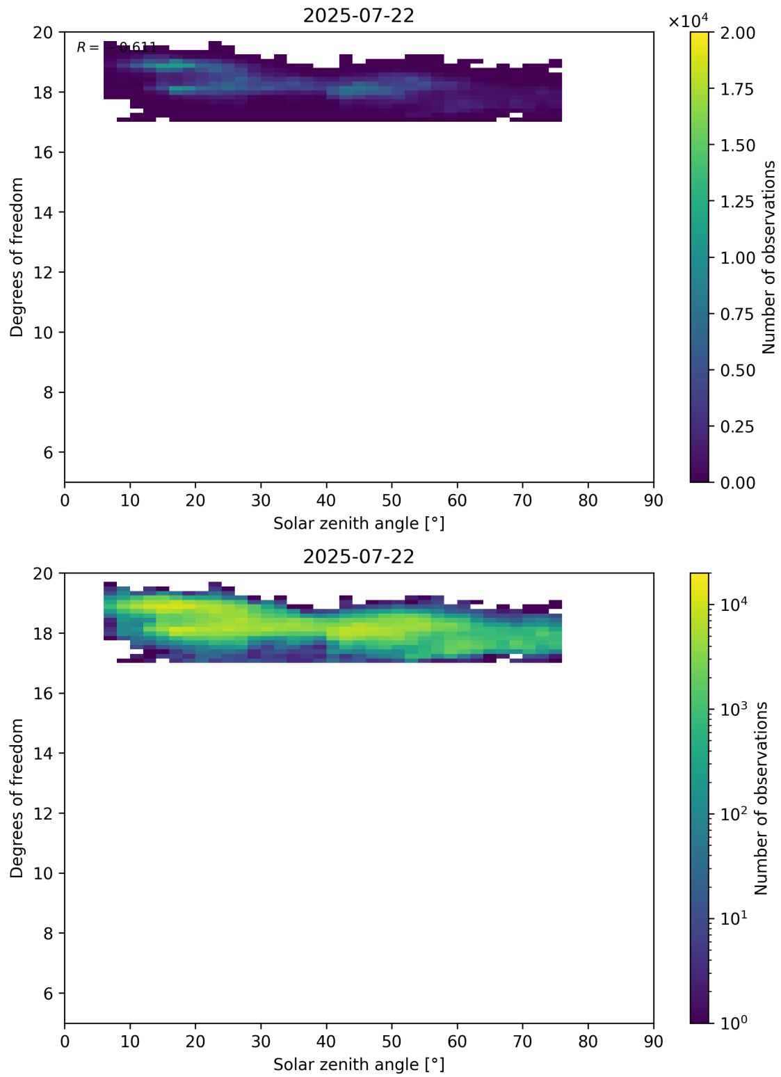
Figure 96: Scatter density plot of “Solar zenith angle” against “Degrees of freedom” for 2025-07-21 to 2025-07-23.
