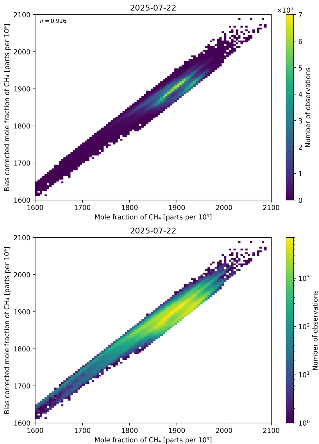
Figure 74: Scatter density plot of “Mole fraction of CH 4 ” against “Bias corrected mole fraction of CH 4 ” for 2025-07-21 to 2025-07-23.
