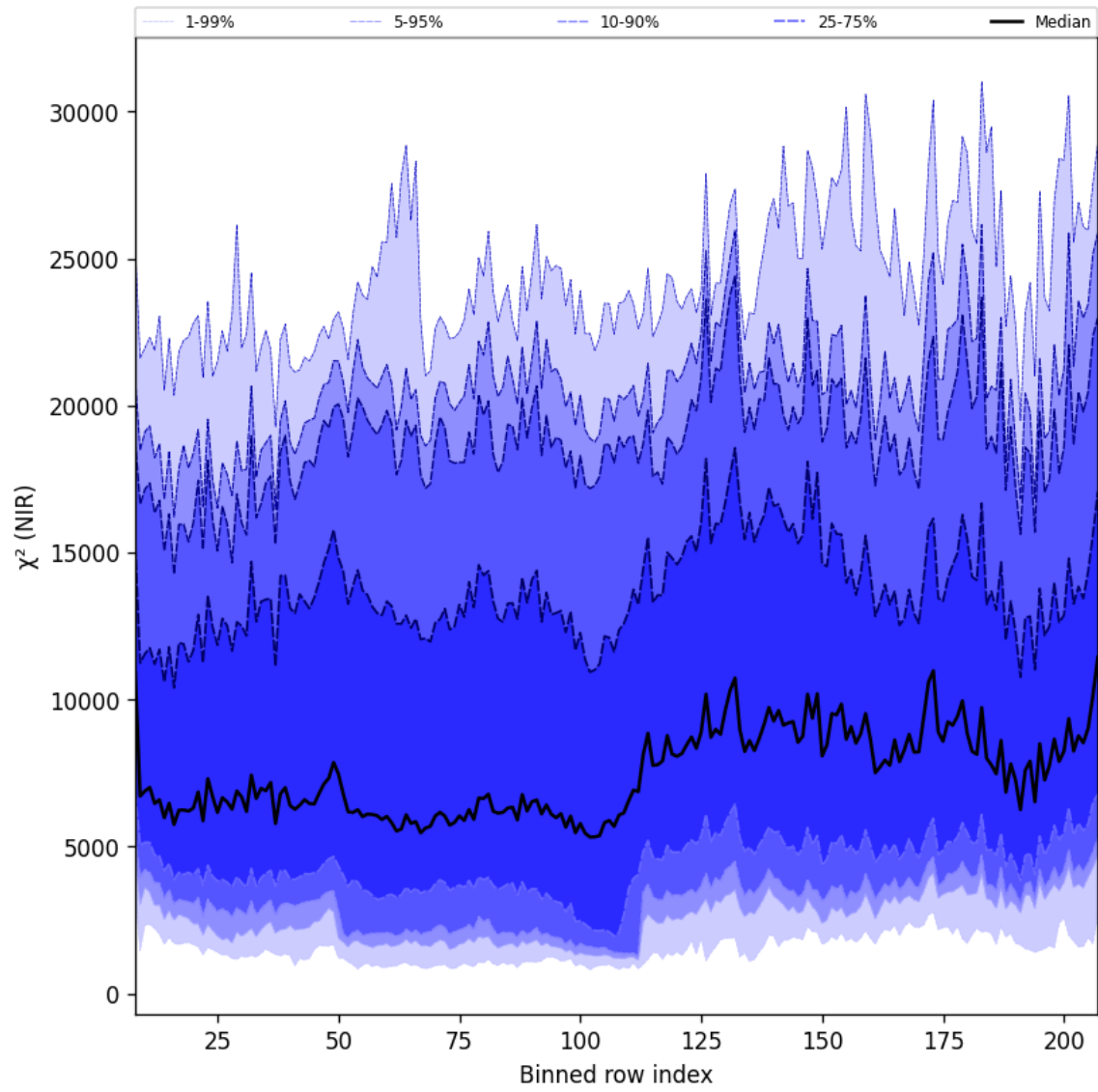
Figure 40: Along track statistics of “ \chi^2 (NIR)” for 2025-07-21 to 2025-07-23
