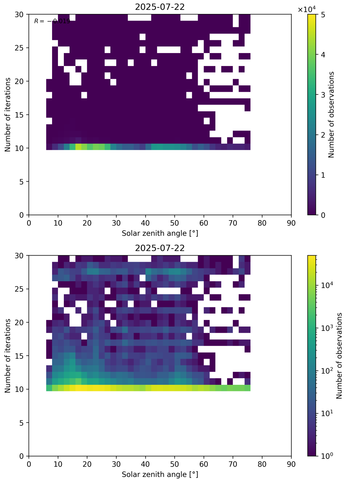
Figure 102: Scatter density plot of “Solar zenith angle” against “Number of iterations” for 2025-07-21 to 2025-07-23.
