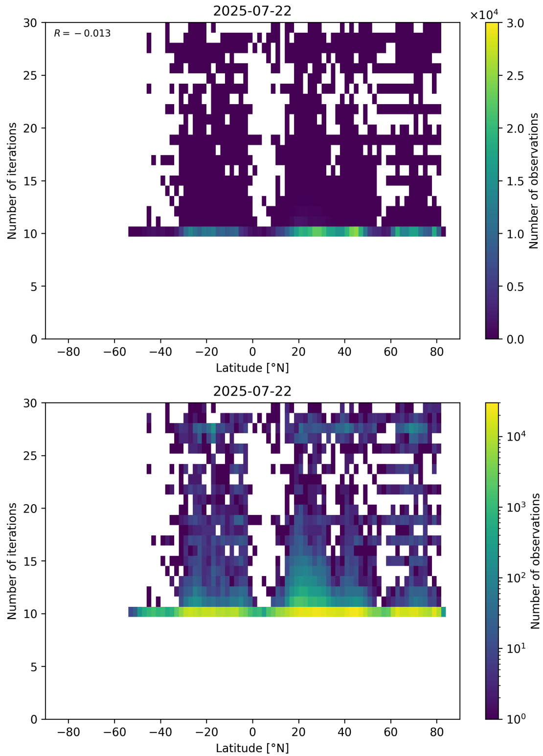
Figure 60: Scatter density plot of “Latitude” against “Number of iterations” for 2025-07-21 to 2025-07-23.
