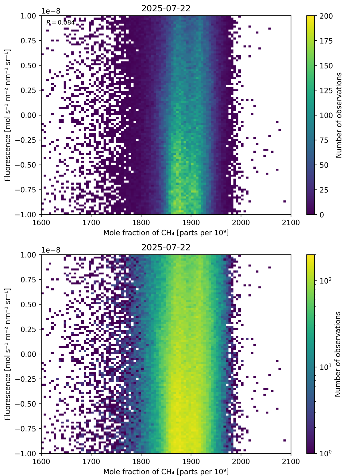
Figure 73: Scatter density plot of “Mole fraction of \text{CH}_4 ” against “Fluorescence” for 2025-07-21 to 2025-07-23.
