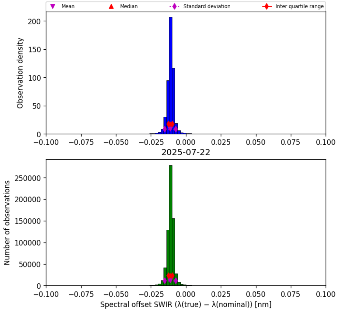
Figure 27: Histogram of “Spectral offset SWIR ( \lambda_{\text{true}} - \lambda_{\text{nominal}} )” for 2025-07-21 to 2025-07-23
