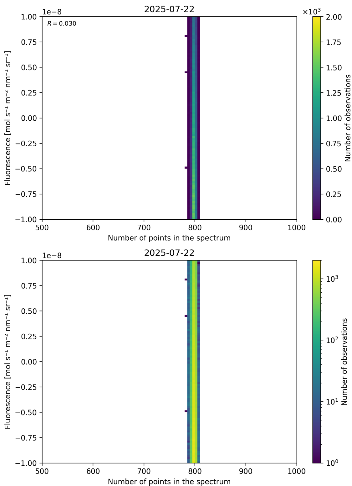
Figure 91: Scatter density plot of “Number of points in the spectrum” against “Fluorescence” for 2025-07-21 to 2025-07-23.
