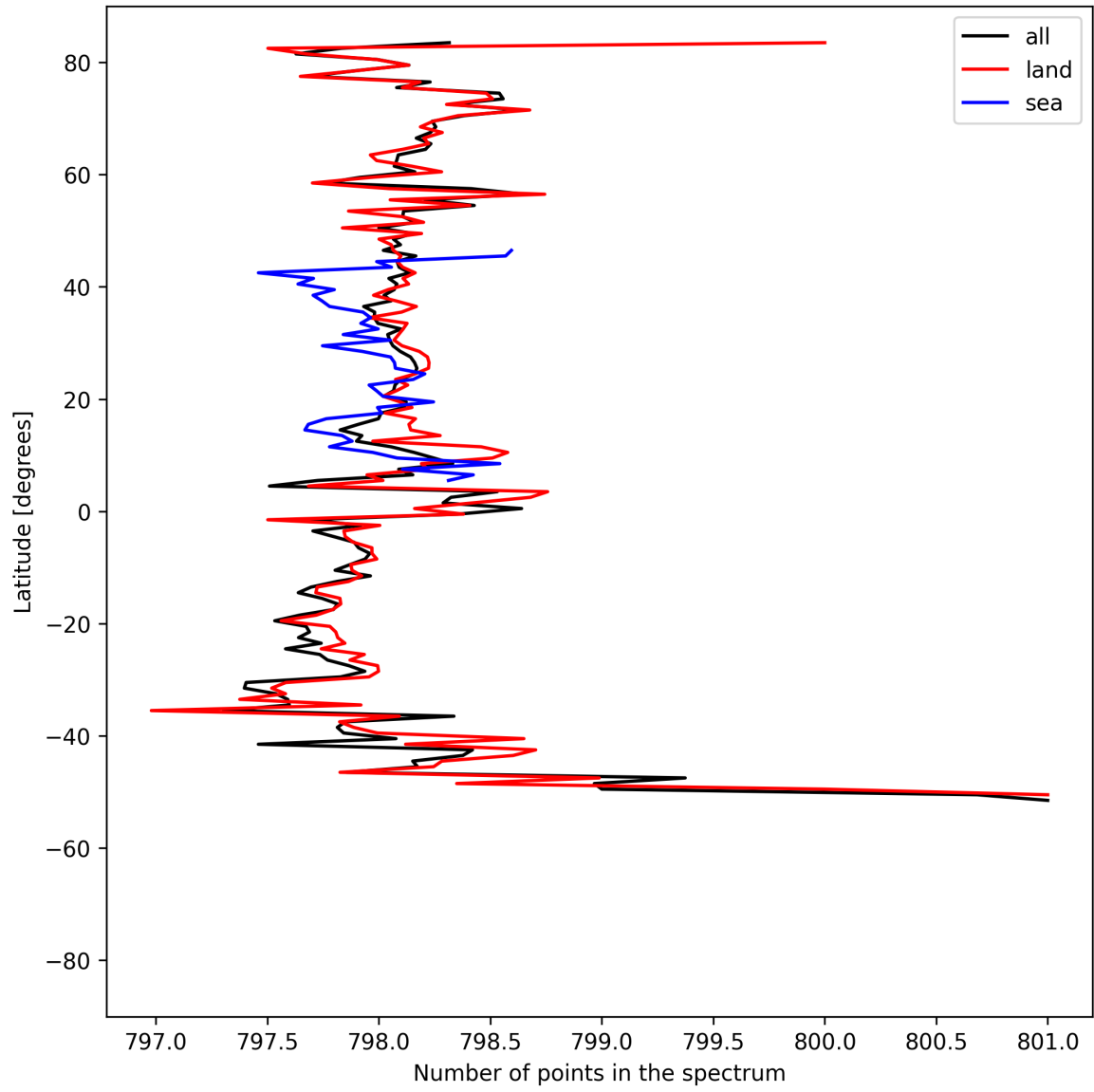
Figure 15: Zonal average of “Number of points in the spectrum” for 2025-07-21 to 2025-07-23.
