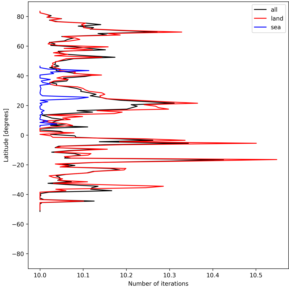
Figure 20: Zonal average of “Number of iterations” for 2025-07-21 to 2025-07-23.
