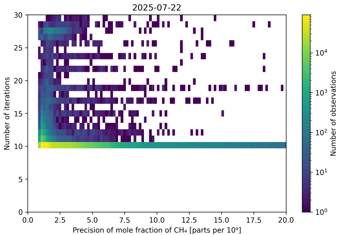
Figure 83: Scatter density plot of “Precision of mole fraction of \text{CH}_4 ” against “Number of iterations” for 2025-07-21 to 2025-07-23.
