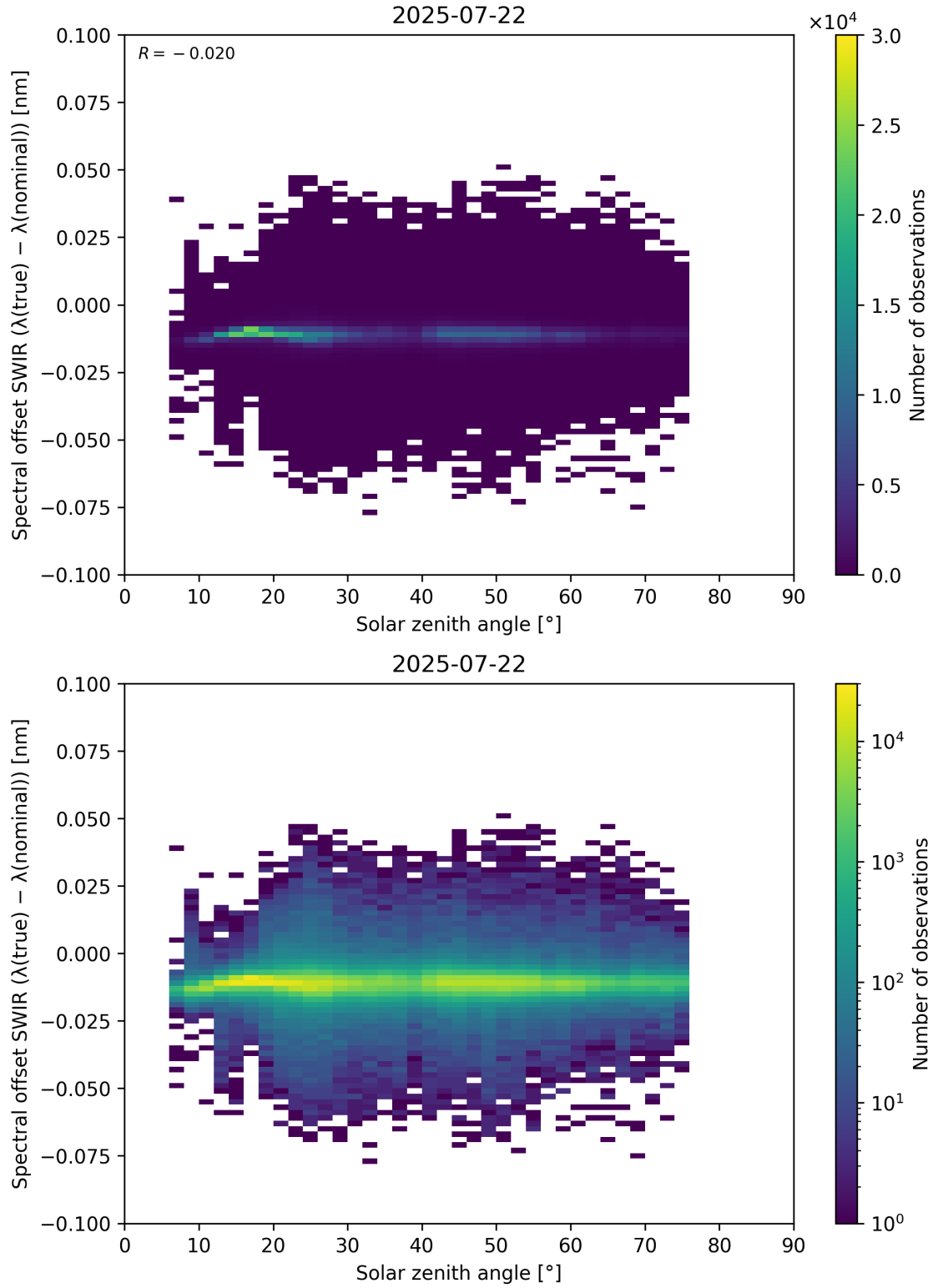
Figure 104: Scatter density plot of “Solar zenith angle” against “Spectral offset SWIR ( \lambda_{\text{true}} - \lambda_{\text{nominal}} )” for 2025-07-21 to 2025-07-23.
