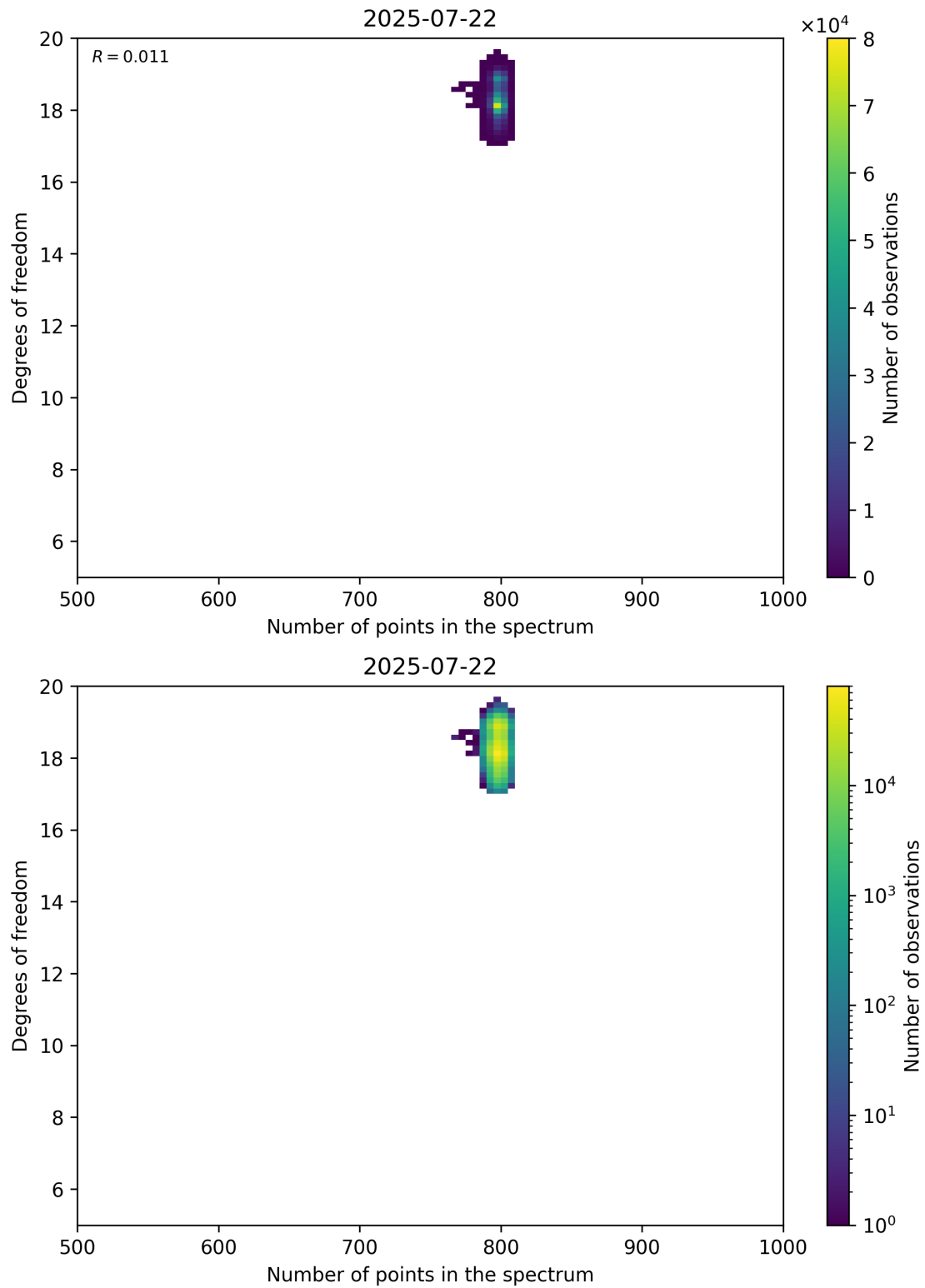
Figure 90: Scatter density plot of “Number of points in the spectrum” against “Degrees of freedom” for 2025-07-21 to 2025-07-23.
