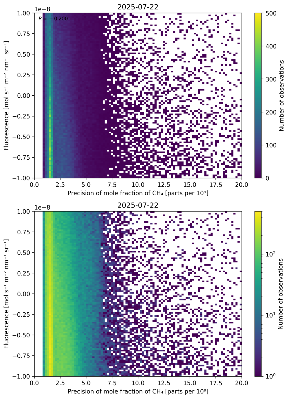
Figure 81: Scatter density plot of “Precision of mole fraction of \text{CH}_4 ” against “Fluorescence” for 2025-07-21 to 2025-07-23.
