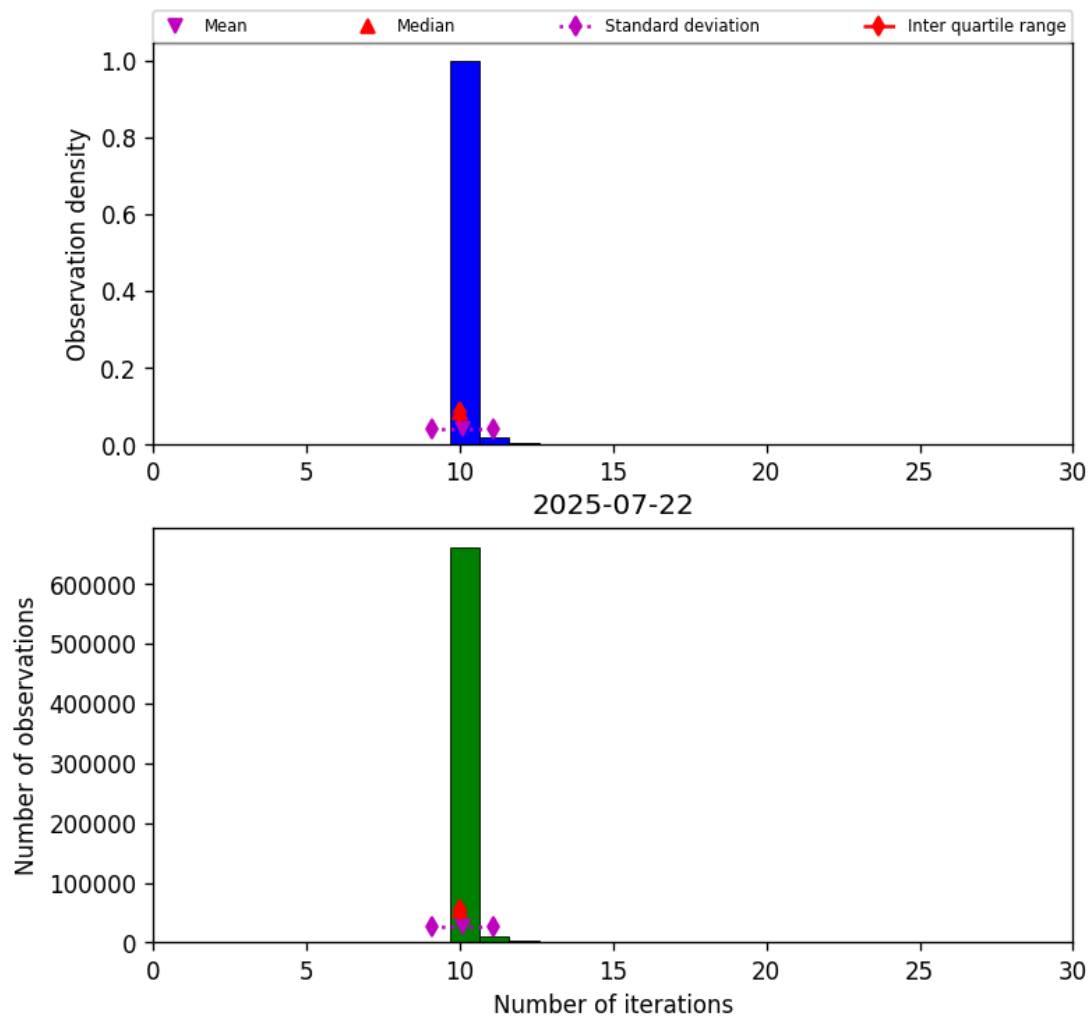
Figure 31: Histogram of “Number of iterations” for 2025-07-21 to 2025-07-23
