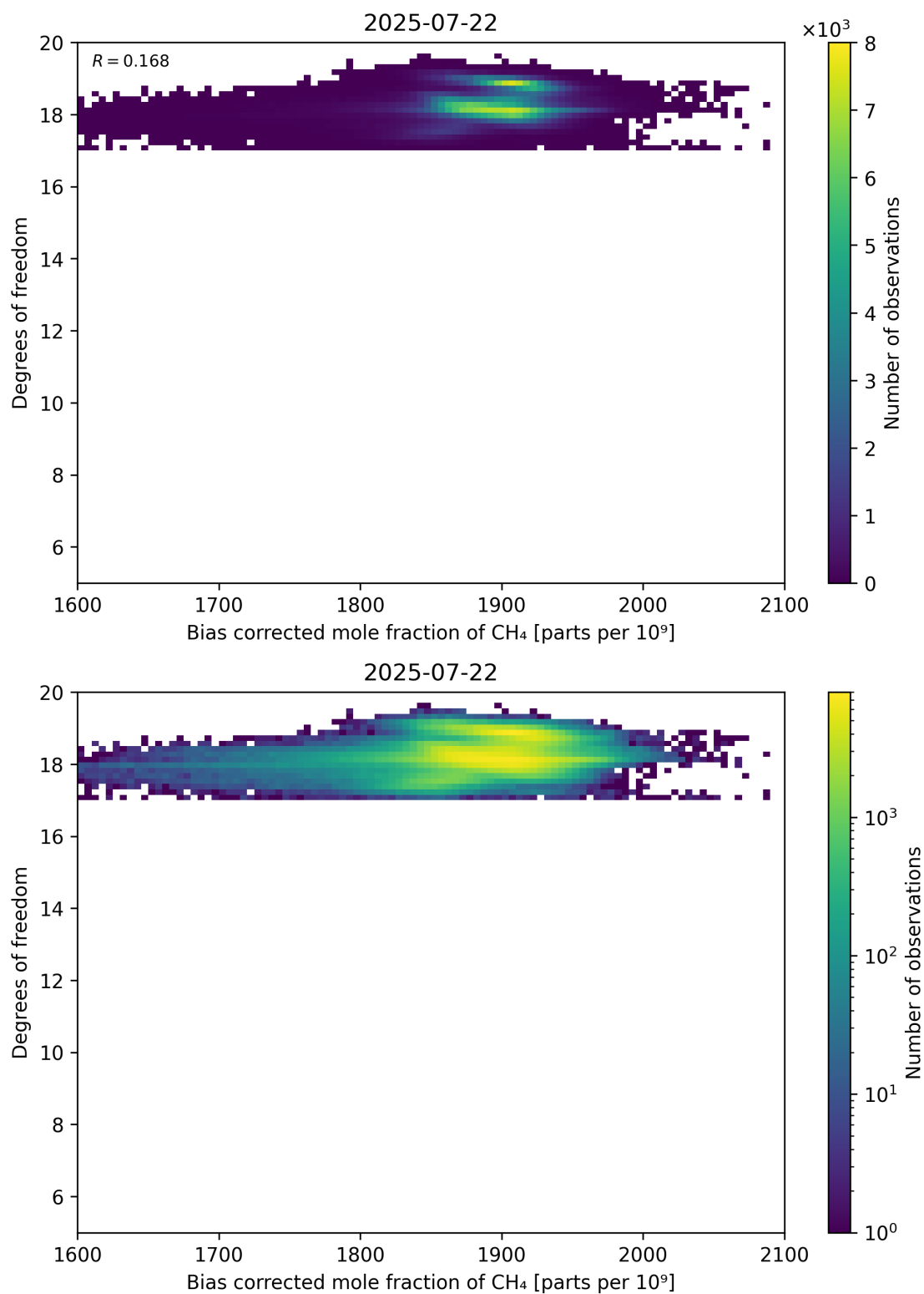
Figure 65: Scatter density plot of “Bias corrected mole fraction of CH 4 ” against “Degrees of freedom” for 2025-07-21 to 2025-07-23.
