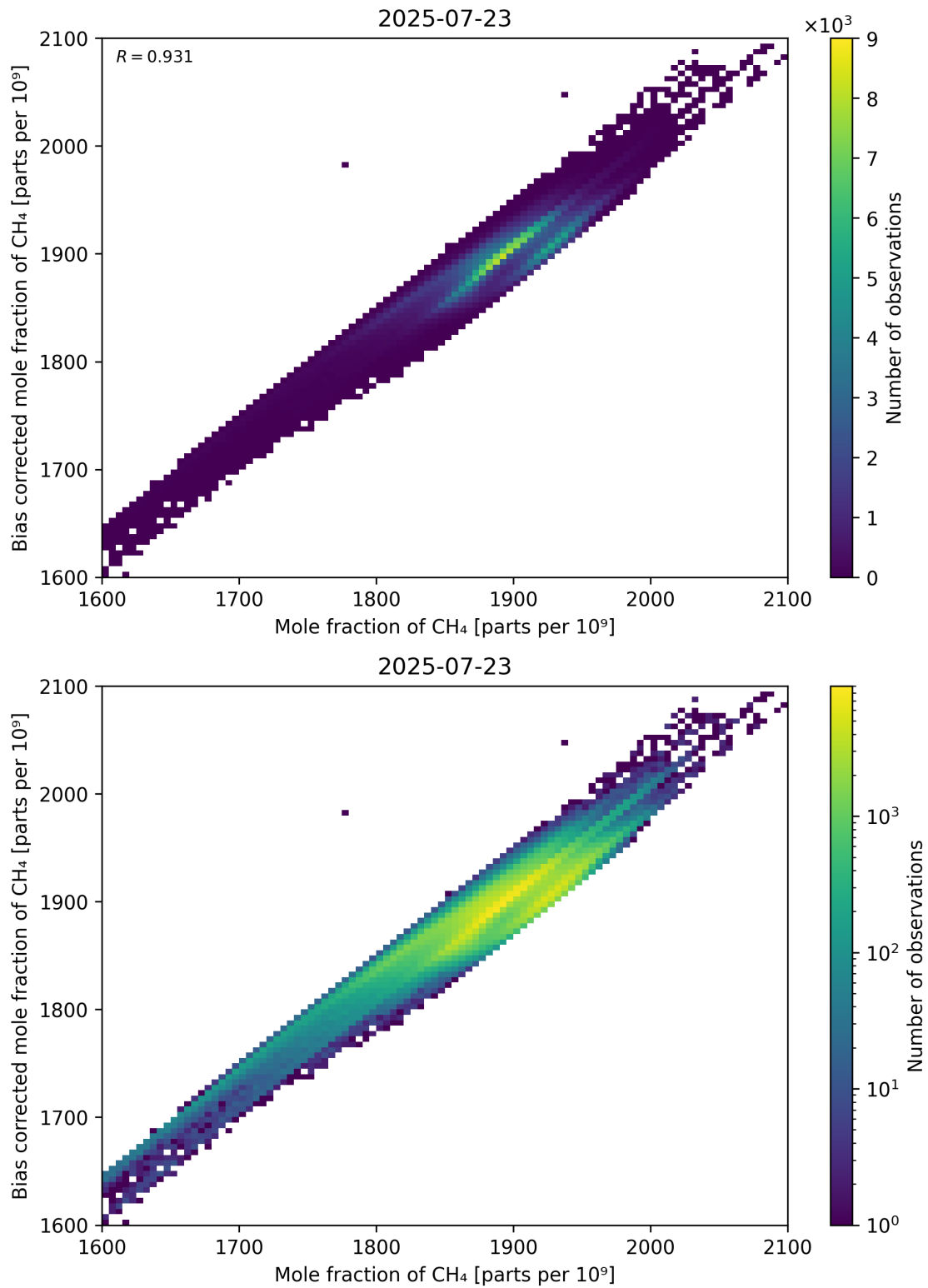
Figure 74: Scatter density plot of “Mole fraction of CH 4 ” against “Bias corrected mole fraction of CH 4 ” for 2025-07-22 to 2025-07-24.
