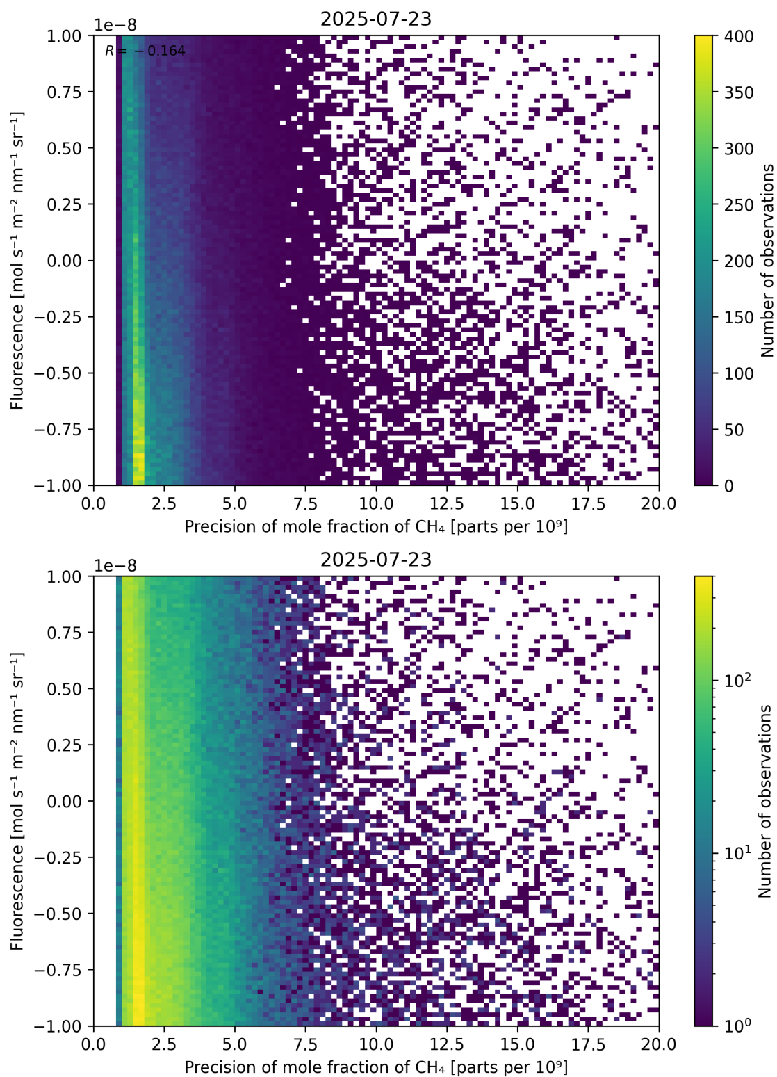
Figure 81: Scatter density plot of “Precision of mole fraction of \text{CH}_4 ” against “Fluorescence” for 2025-07-22 to 2025-07-24.
