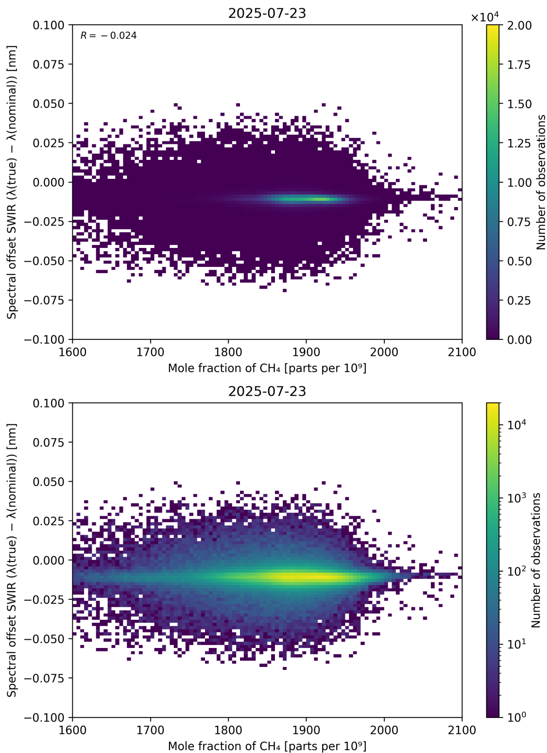
Figure 86: Scatter density plot of “Mole fraction of CH 4 ” against “Spectral offset SWIR ( \lambda_{\text{true}} - \lambda_{\text{nominal}} )” for 2025-07-22 to 2025-07-24.
