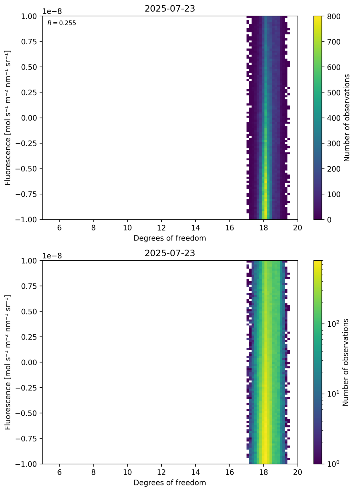
Figure 51: Scatter density plot of “Degrees of freedom” against “Fluorescence” for 2025-07-22 to 2025-07-24.
