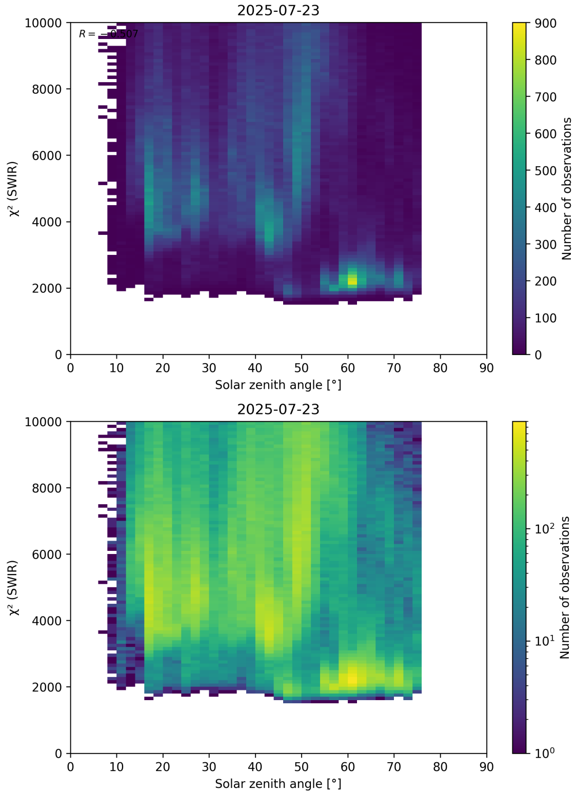
Figure 95: Scatter density plot of “Solar zenith angle” against “ \chi^2 (SWIR)” for 2025-07-22 to 2025-07-24.
