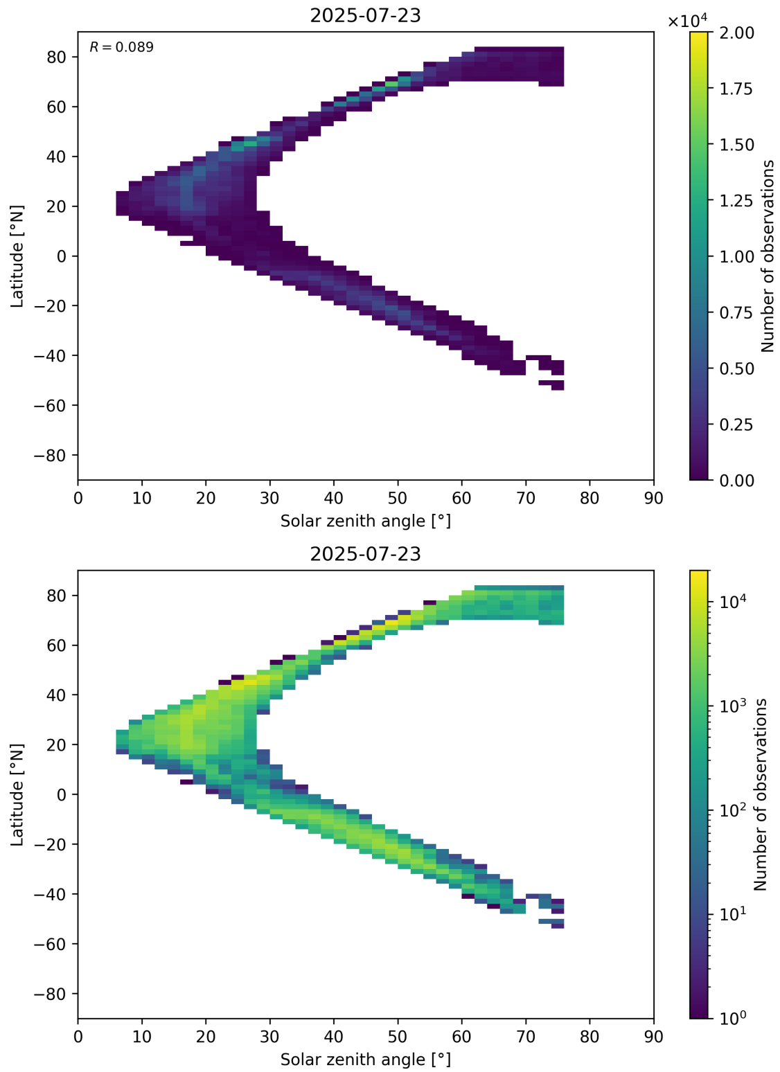
Figure 98: Scatter density plot of “Solar zenith angle” against “Latitude” for 2025-07-22 to 2025-07-24.
