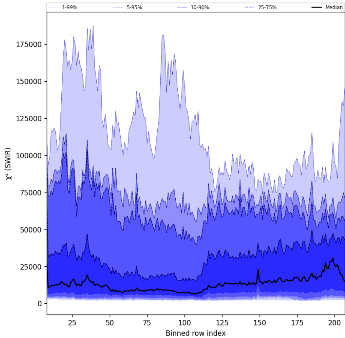
Figure 39: Along track statistics of “ \chi^2 (SWIR)” for 2025-07-22 to 2025-07-24
