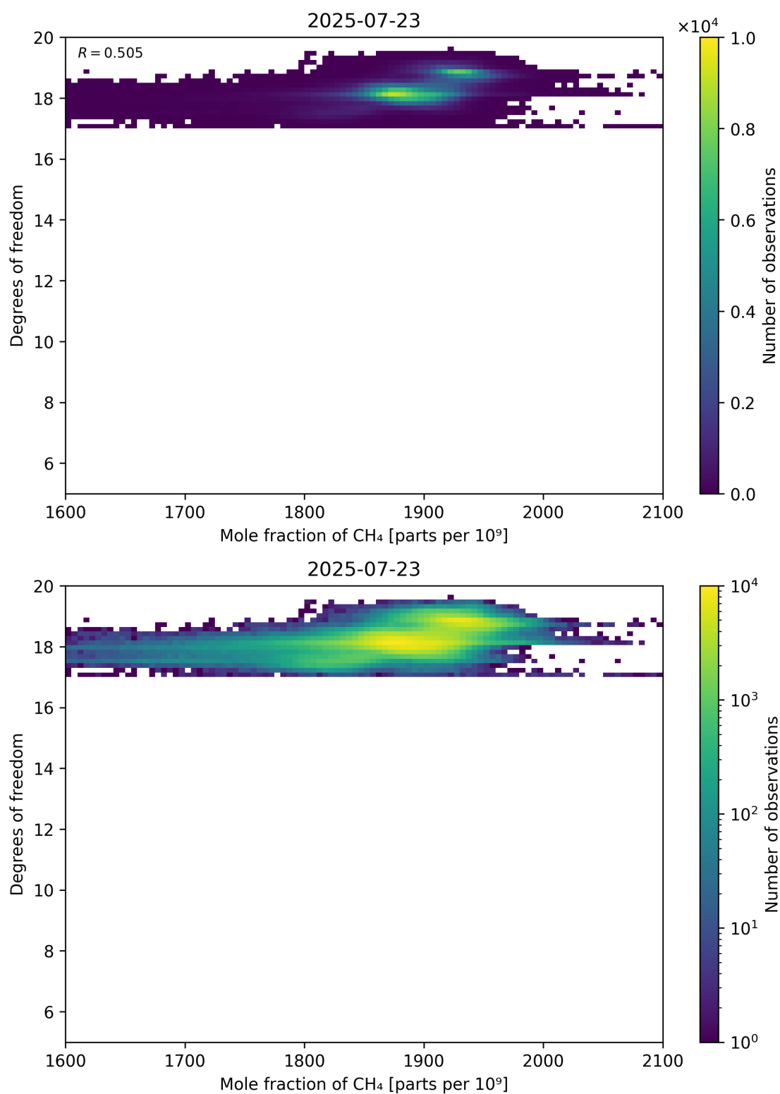
Figure 72: Scatter density plot of “Mole fraction of CH 4 ” against “Degrees of freedom” for 2025-07-22 to 2025-07-24.
