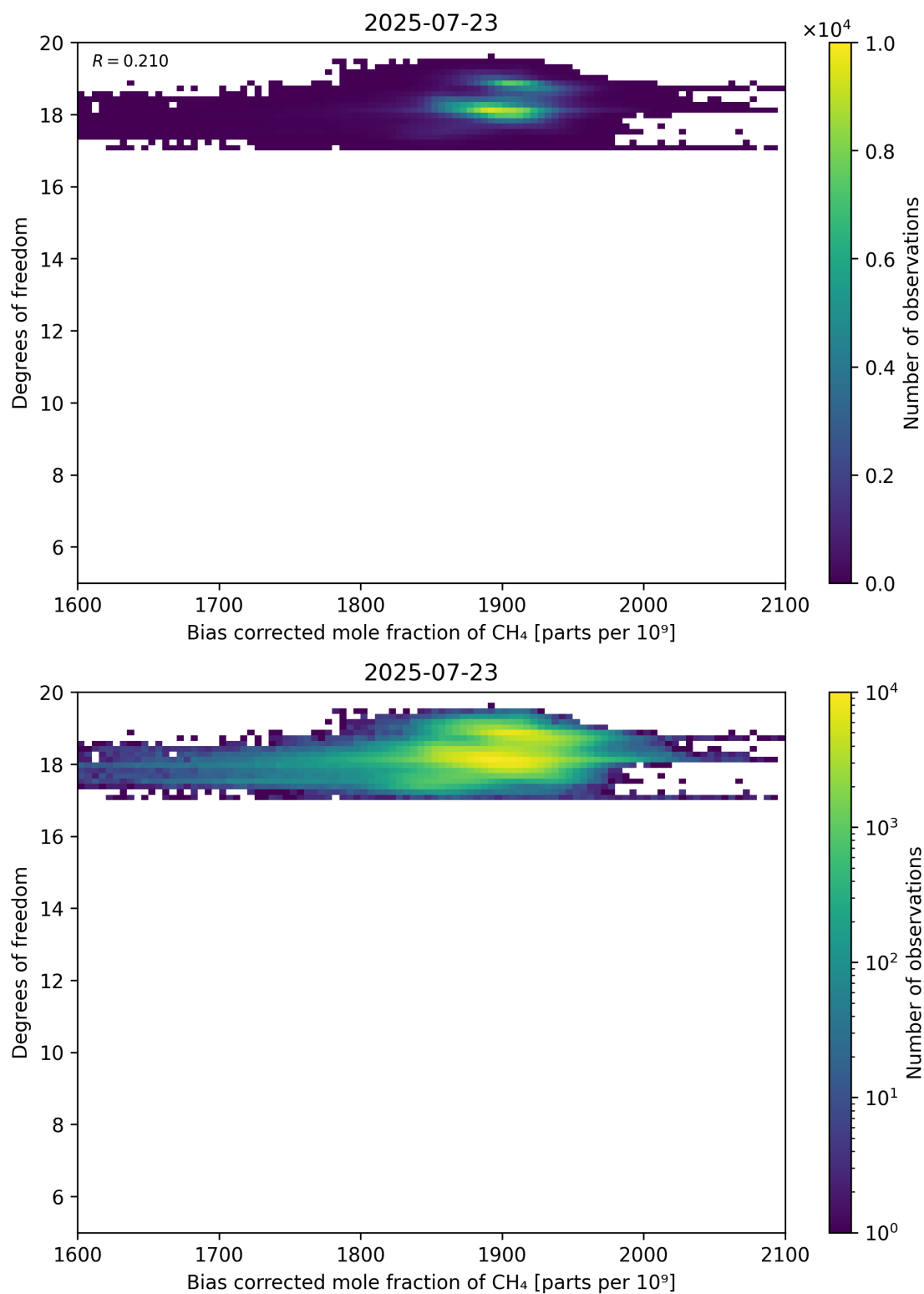
Figure 65: Scatter density plot of “Bias corrected mole fraction of \text{CH}_4 ” against “Degrees of freedom” for 2025-07-22 to 2025-07-24.
