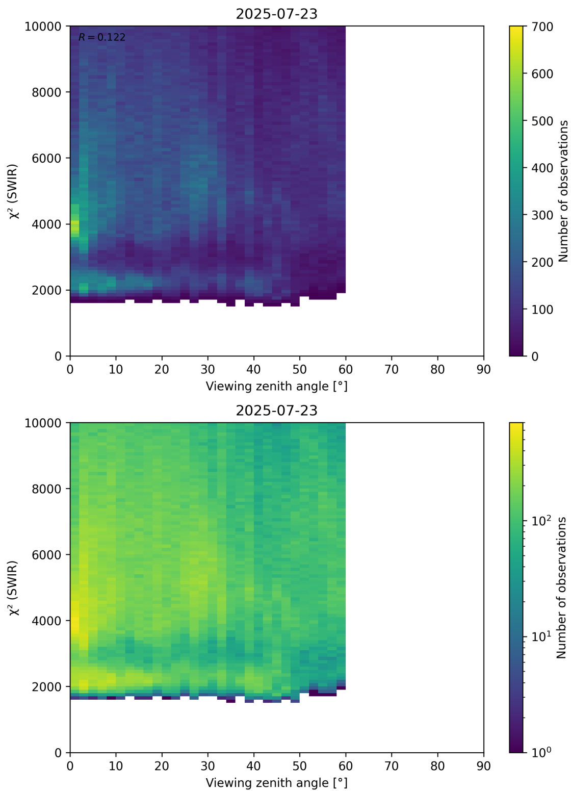
Figure 106: Scatter density plot of “Viewing zenith angle” against “ \chi^2 (SWIR)” for 2025-07-22 to 2025-07-24.
