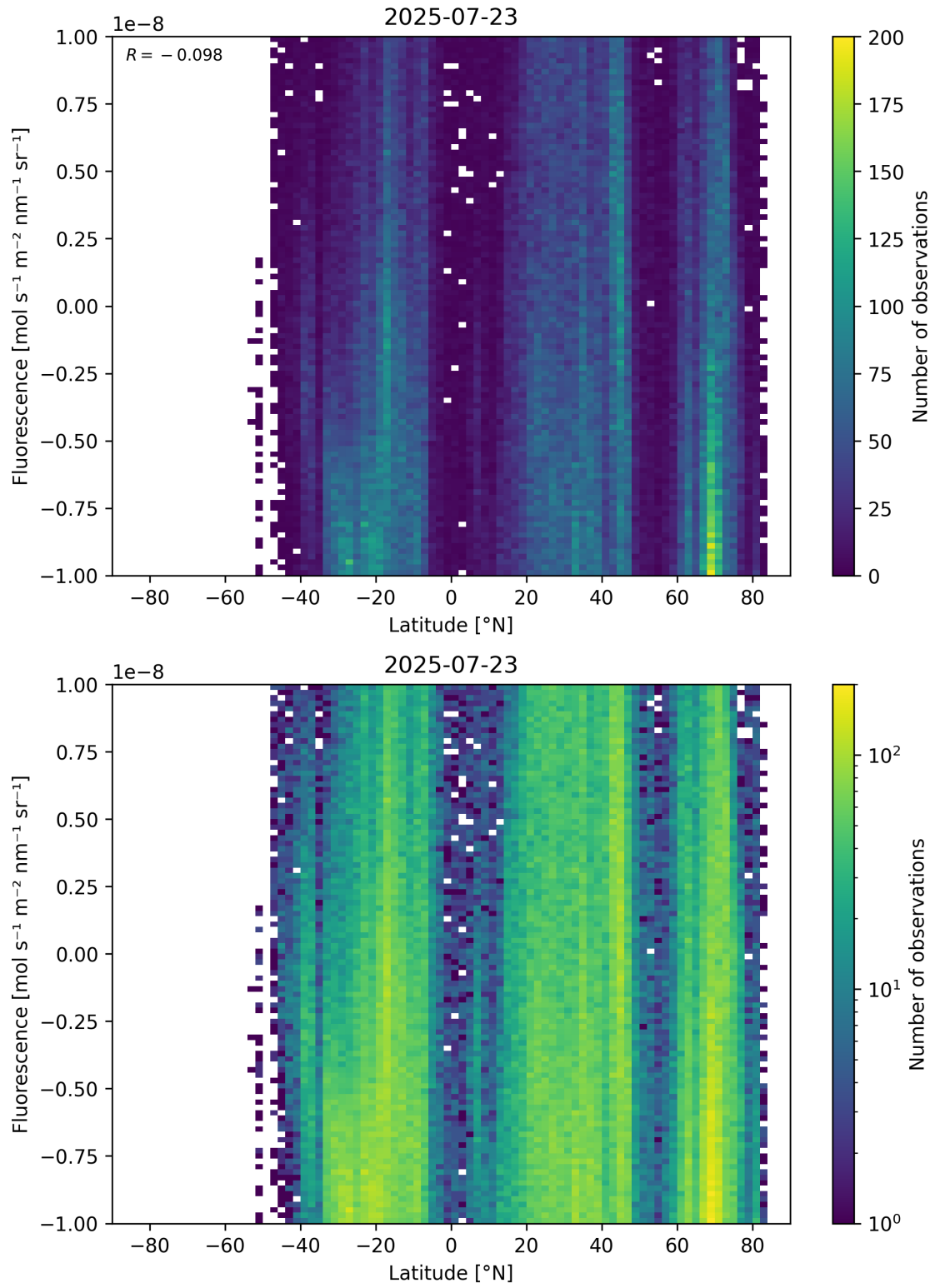
Figure 56: Scatter density plot of “Latitude” against “Fluorescence” for 2025-07-22 to 2025-07-24.
