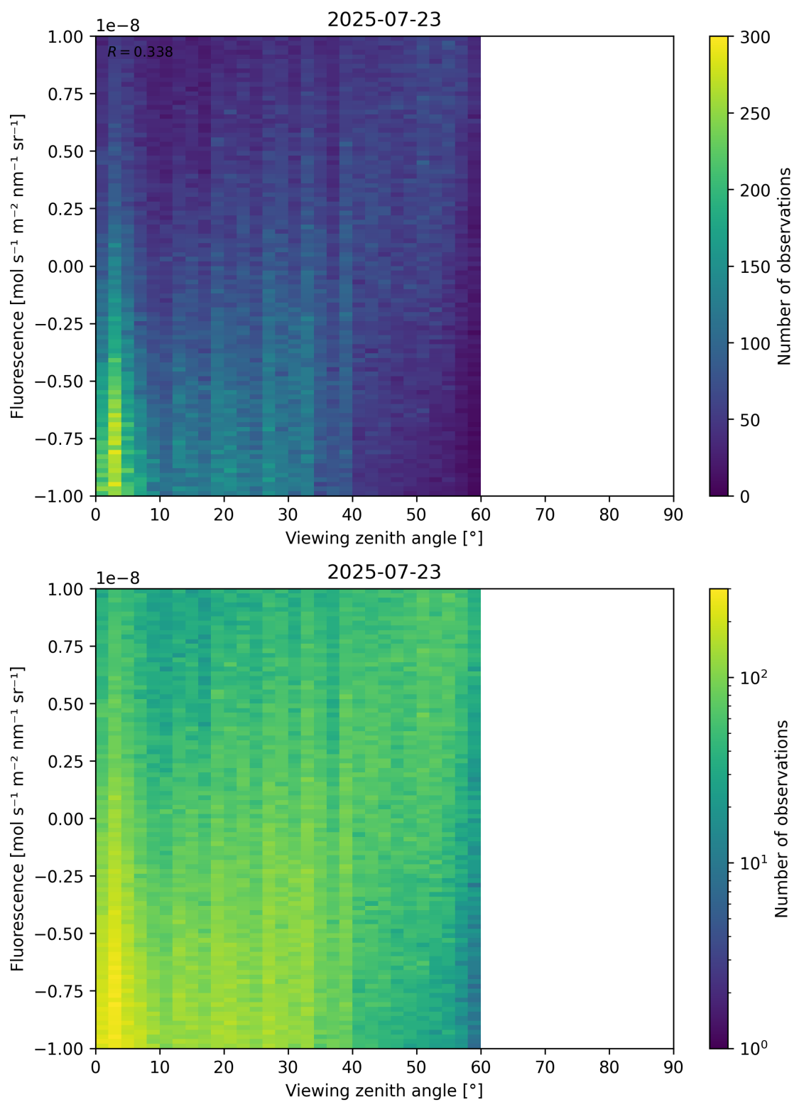
Figure 108: Scatter density plot of “Viewing zenith angle” against “Fluorescence” for 2025-07-22 to 2025-07-24.
