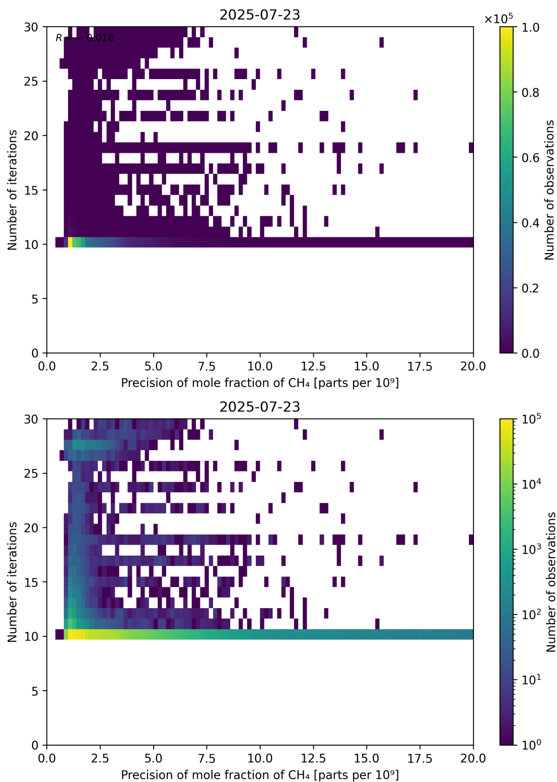
Figure 83: Scatter density plot of “Precision of mole fraction of CH 4 ” against “Number of iterations” for 2025-07-22 to 2025-07-24.
