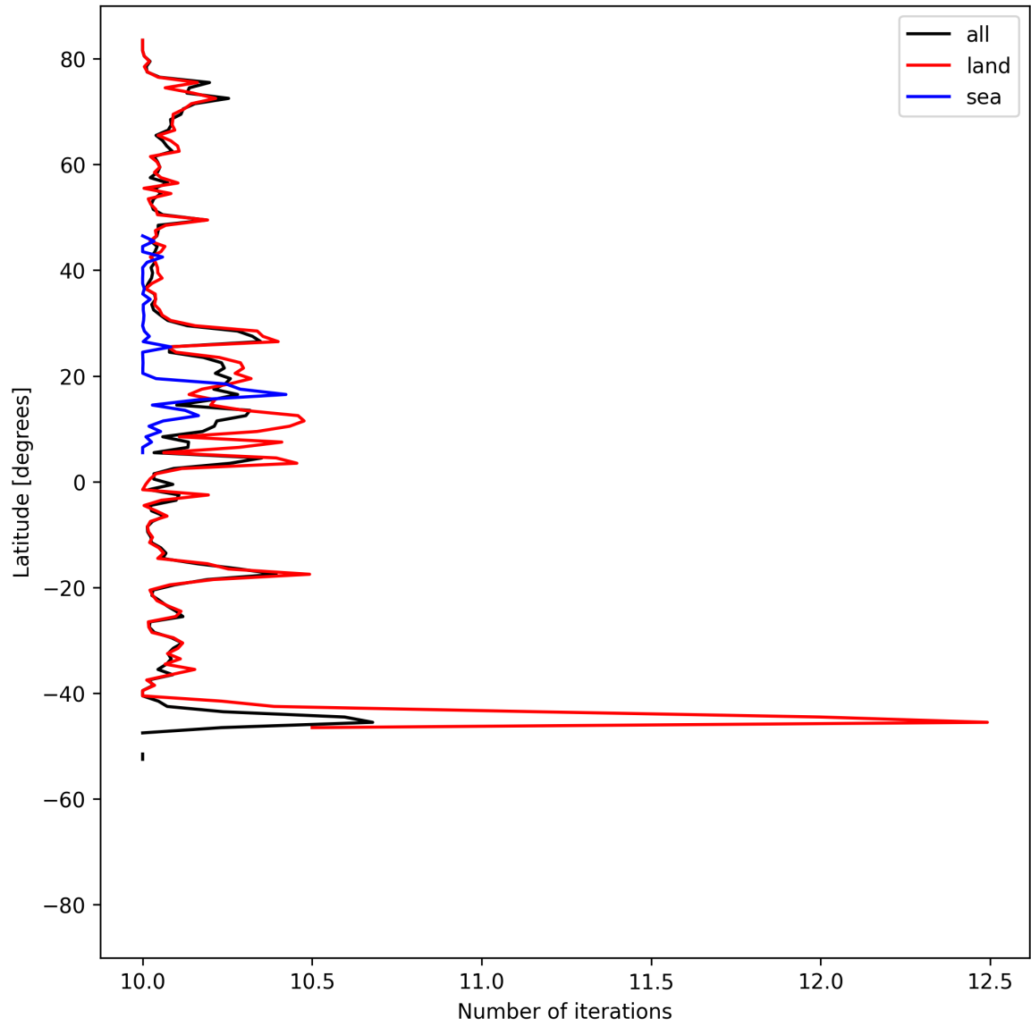
Figure 20: Zonal average of “Number of iterations” for 2025-07-22 to 2025-07-24.
