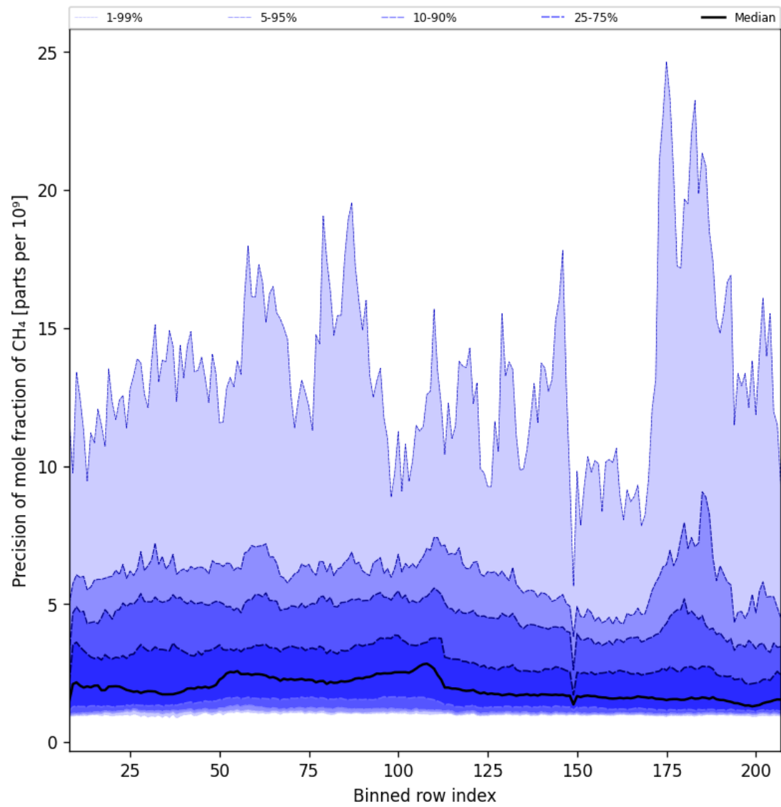
Figure 35: Along track statistics of “Precision of mole fraction of CH 4 ” for 2025-07-22 to 2025-07-24
