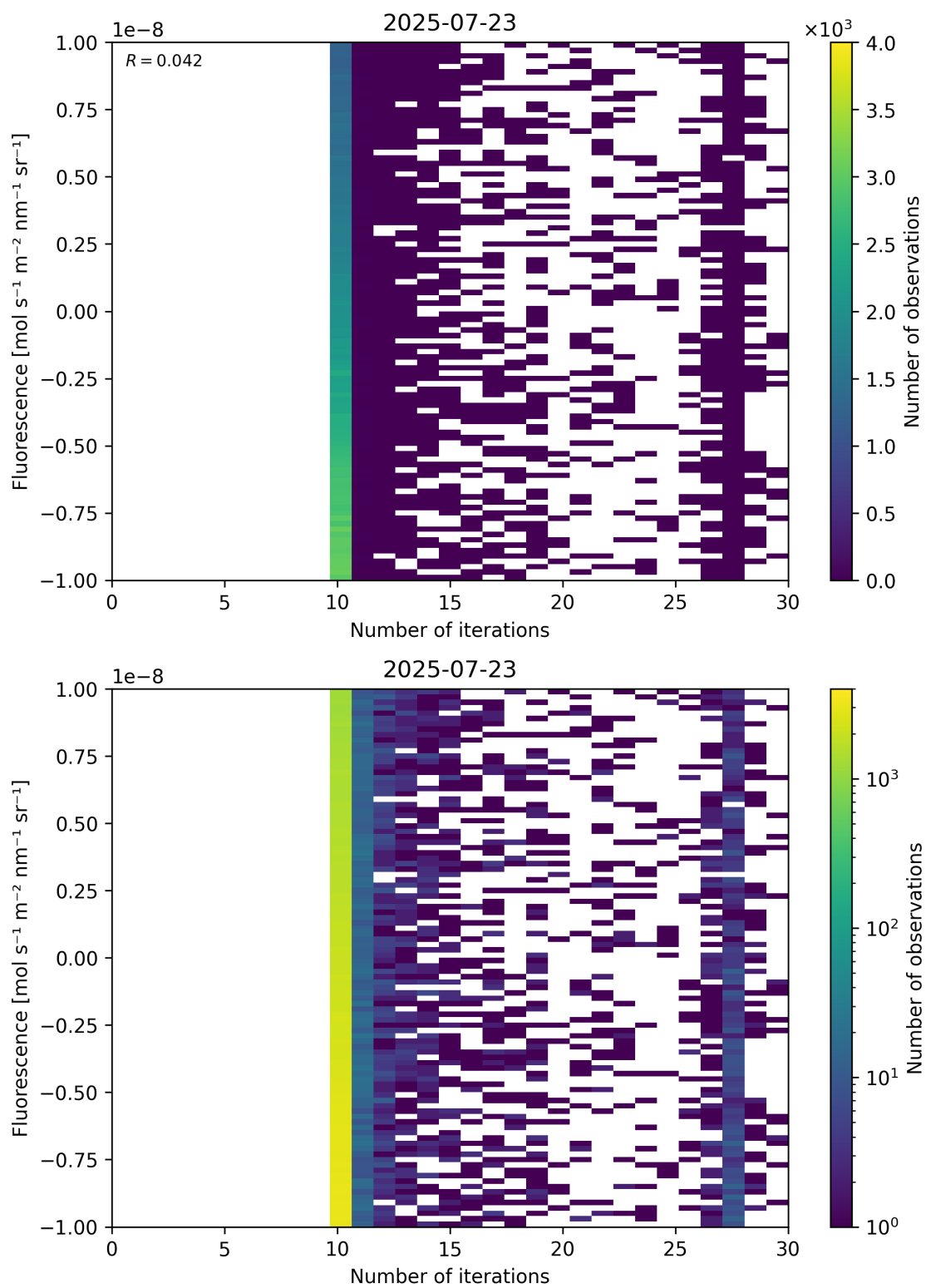
Figure 87: Scatter density plot of “Number of iterations” against “Fluorescence” for 2025-07-22 to 2025-07-24.
