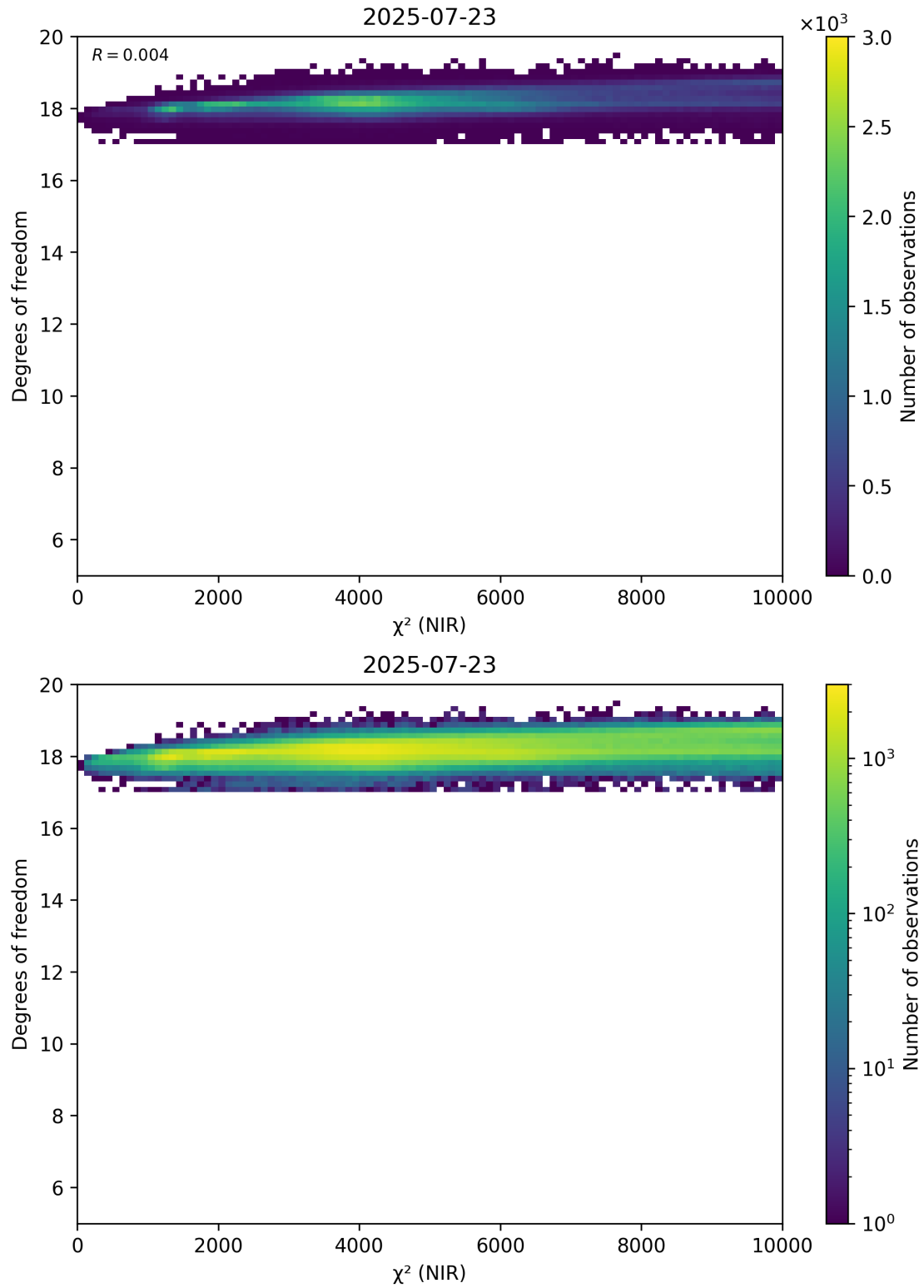
Figure 44: Scatter density plot of “ \chi^2 (NIR)” against “Degrees of freedom” for 2025-07-22 to 2025-07-24.
