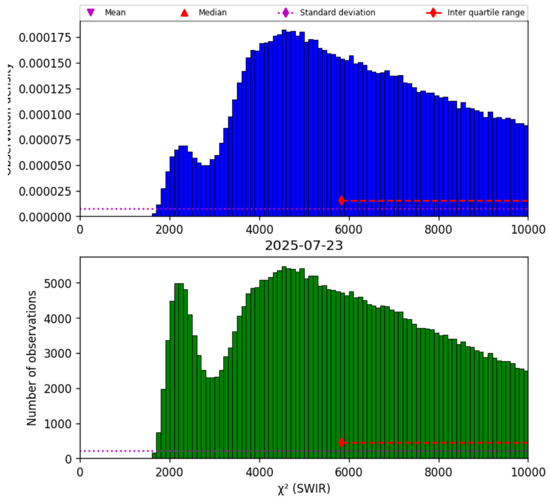
Figure 28: Histogram of “ \chi^2 (SWIR)” for 2025-07-22 to 2025-07-24
