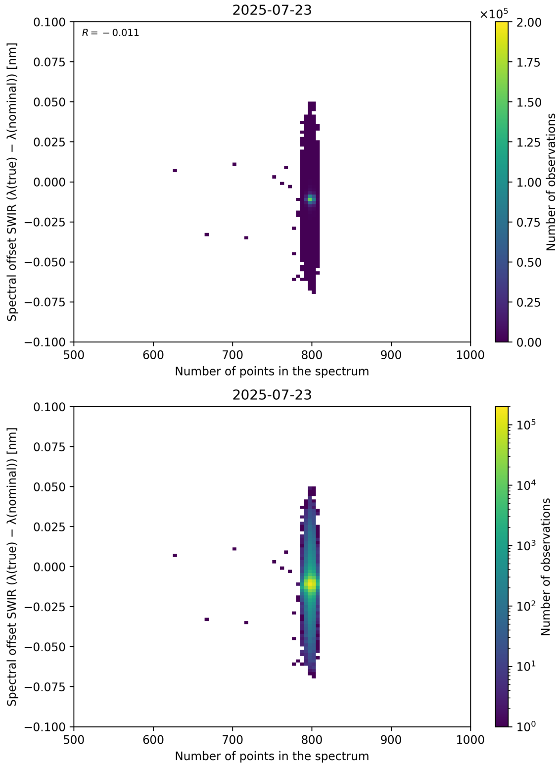
Figure 93: Scatter density plot of “Number of points in the spectrum” against “Spectral offset SWIR ( \lambda_{\text{true}} - \lambda_{\text{nominal}} )” for 2025-07-22 to 2025-07-24.
