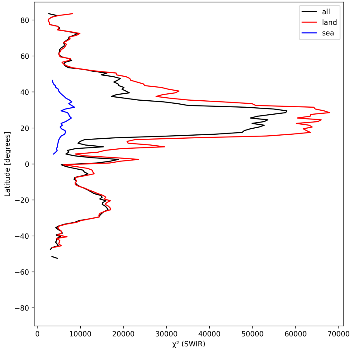
Figure 17: Zonal average of “ \chi^2 (SWIR)” for 2025-07-22 to 2025-07-24.
