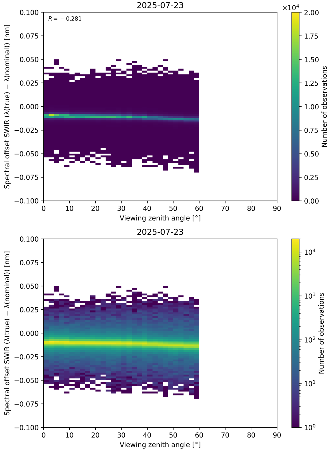
Figure 116: Scatter density plot of “Viewing zenith angle” against “Spectral offset SWIR ( \lambda_{\text{true}} - \lambda_{\text{nominal}} )” for 2025-07-22 to 2025-07-24.
