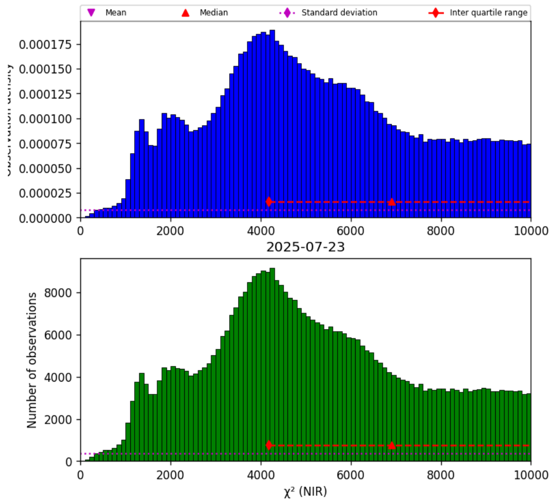
Figure 29: Histogram of “ \chi^2 (NIR)” for 2025-07-22 to 2025-07-24
