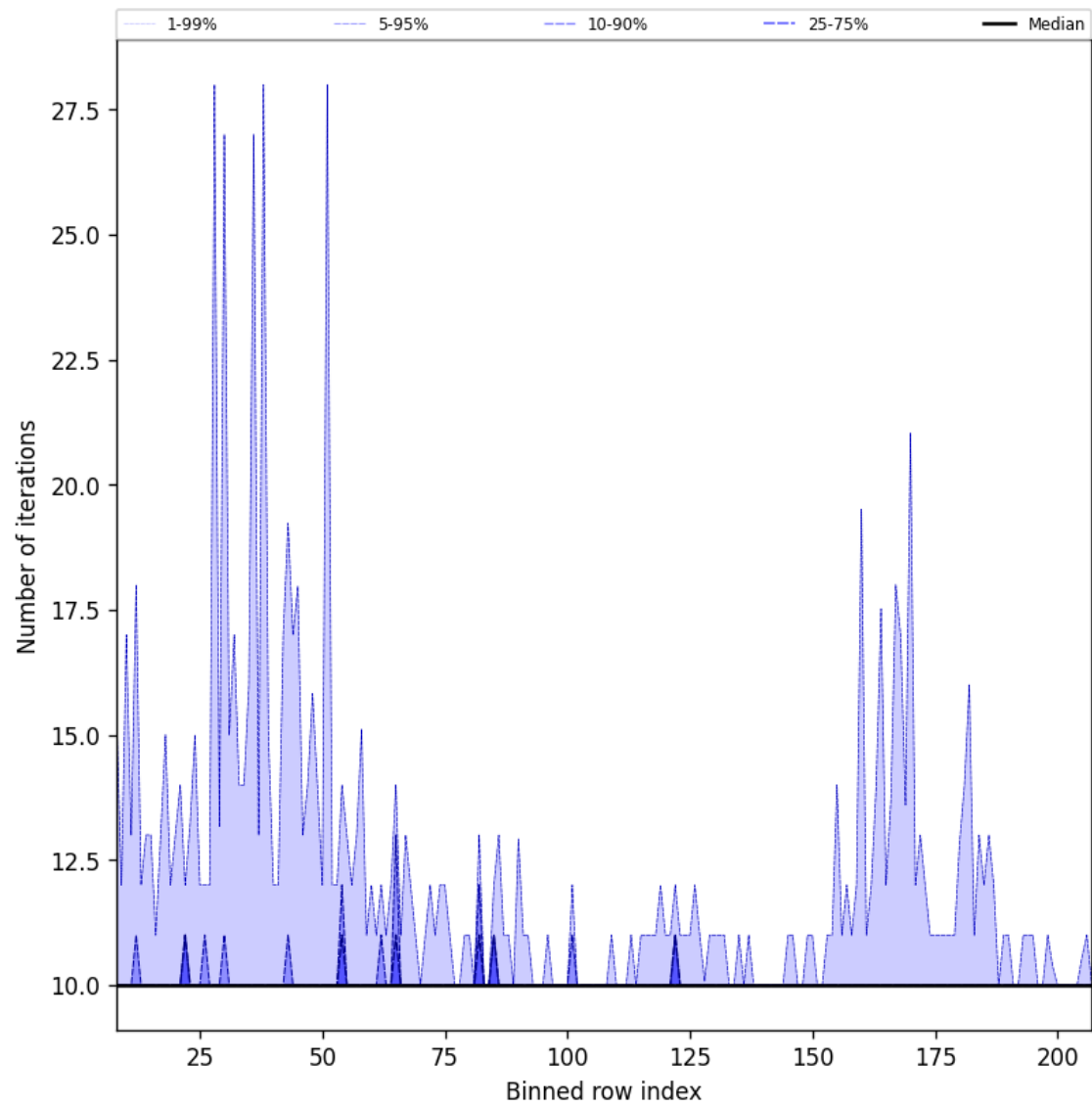
Figure 42: Along track statistics of “Number of iterations” for 2025-07-22 to 2025-07-24
