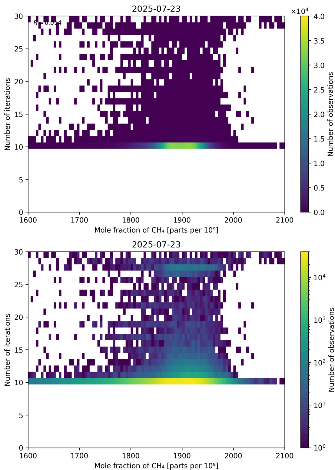
Figure 76: Scatter density plot of “Mole fraction of CH 4 ” against “Number of iterations” for 2025-07-22 to 2025-07-24.
