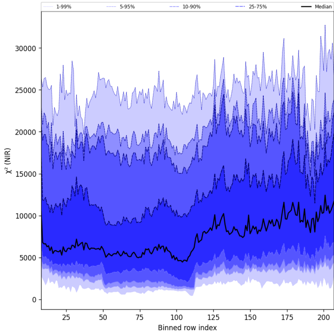
Figure 40: Along track statistics of “ \chi^2 (NIR)” for 2025-07-22 to 2025-07-24
