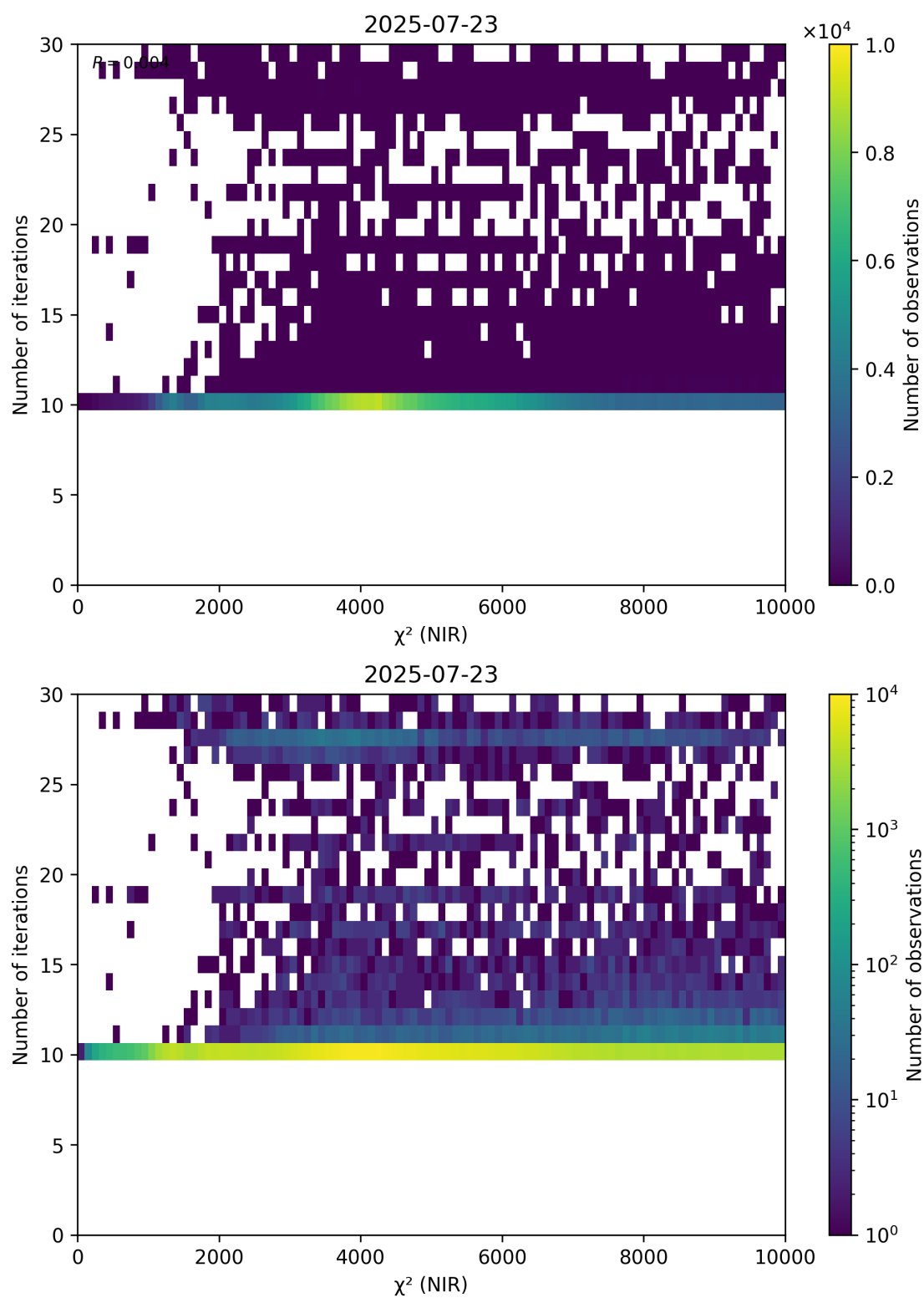
Figure 46: Scatter density plot of “ \chi^2 (NIR)” against “Number of iterations” for 2025-07-22 to 2025-07-24.
