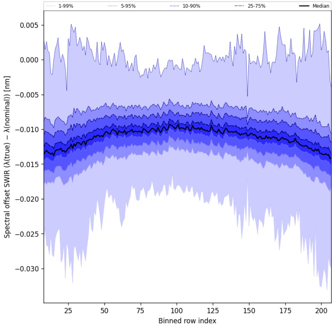
Figure 38: Along track statistics of “Spectral offset SWIR ( \lambda_{\text{true}} - \lambda_{\text{nominal}} )” for 2025-07-22 to 2025-07-24
