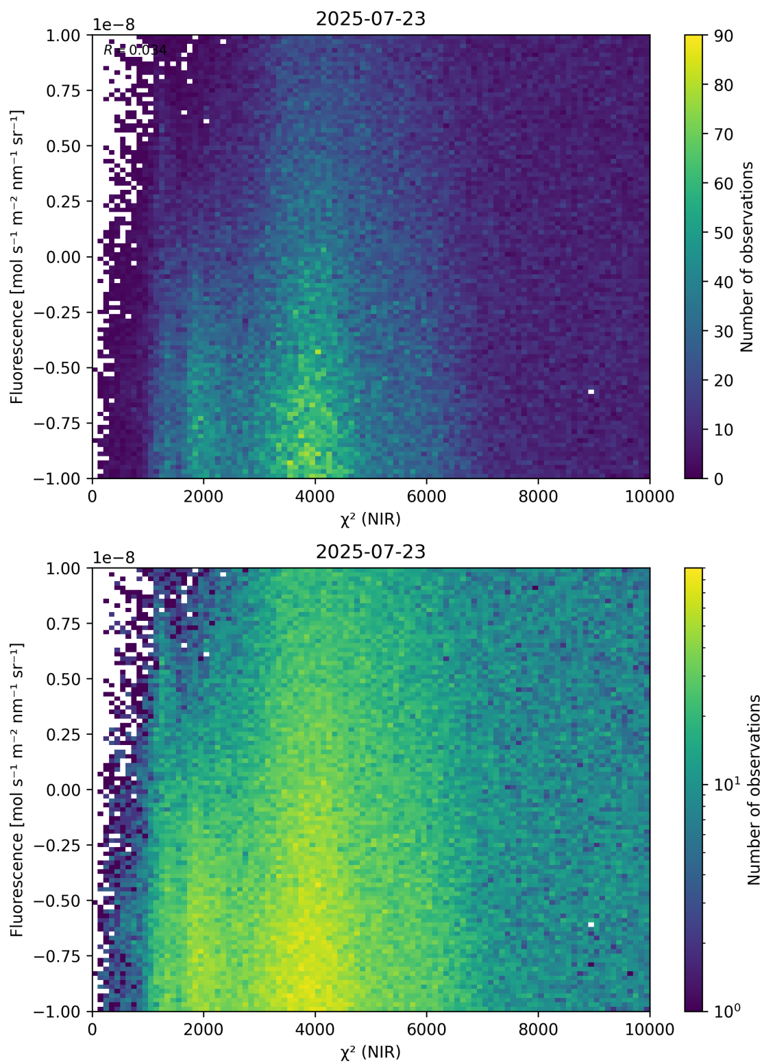
Figure 45: Scatter density plot of “ \chi^2 (NIR)” against “Fluorescence” for 2025-07-22 to 2025-07-24.
