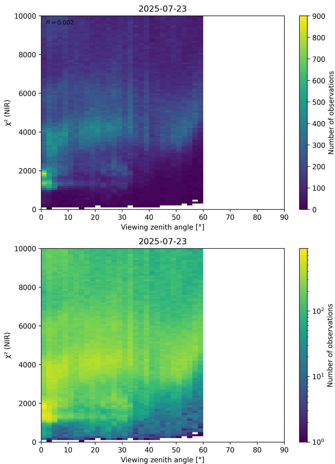
Figure 105: Scatter density plot of “Viewing zenith angle” against “ \chi^2 (NIR)” for 2025-07-22 to 2025-07-24.
