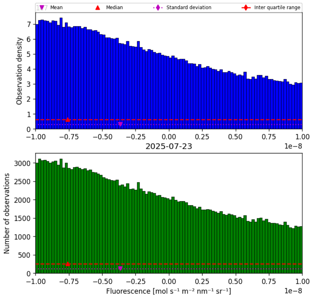
Figure 32: Histogram of “Fluorescence” for 2025-07-22 to 2025-07-24
