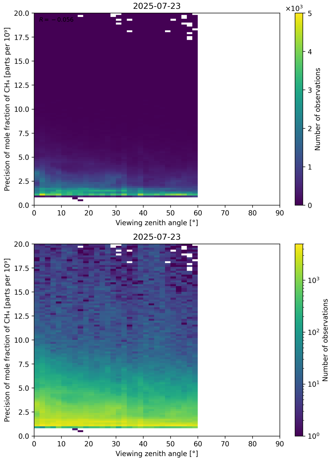
Figure 112: Scatter density plot of “Viewing zenith angle” against “Precision of mole fraction of CH 4 ” for 2025-07-22 to 2025-07-24.
