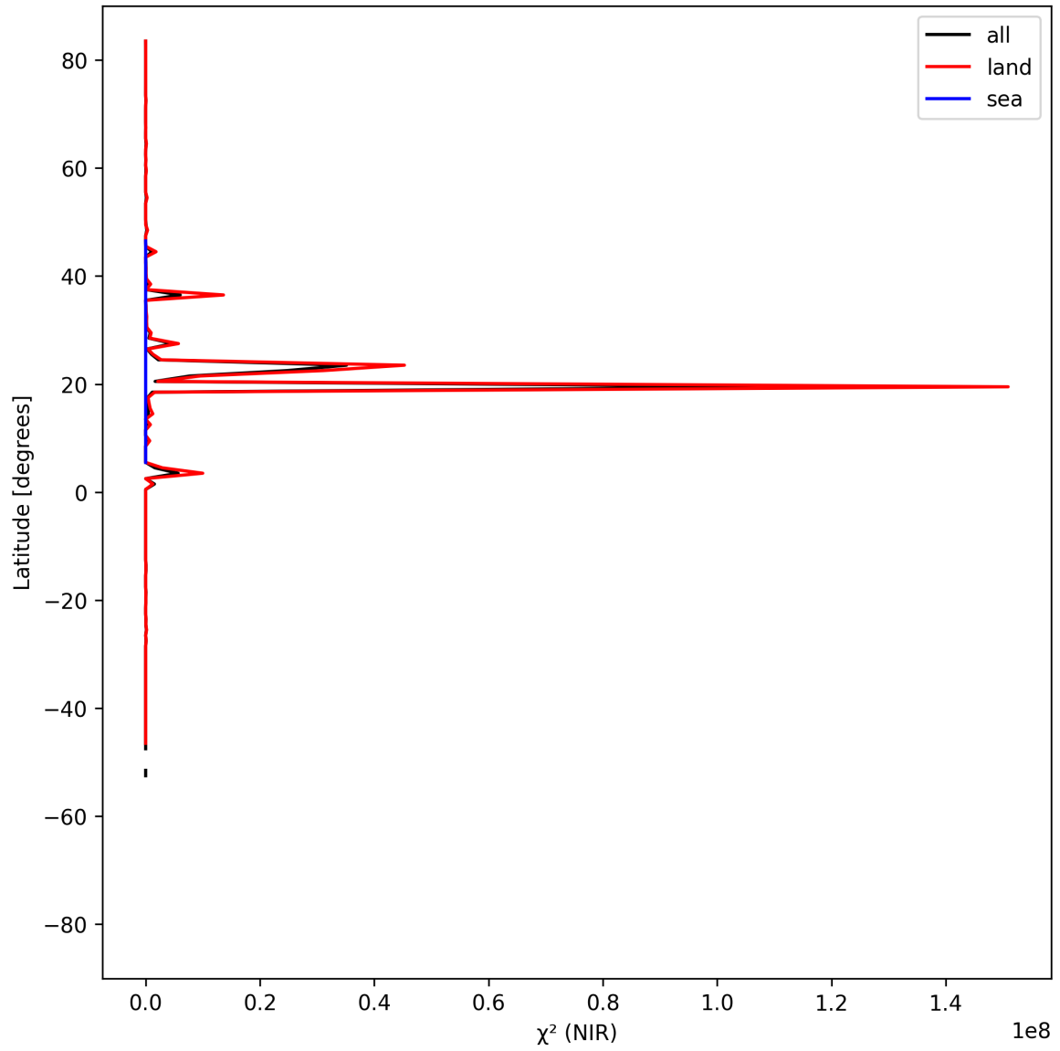
Figure 18: Zonal average of “ \chi^2 (NIR)” for 2025-07-22 to 2025-07-24.
