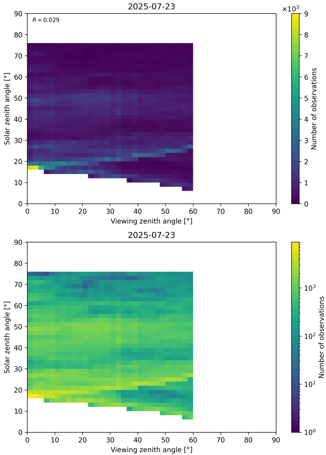
Figure 115: Scatter density plot of “Viewing zenith angle” against “Solar zenith angle” for 2025-07-22 to 2025-07-24.
