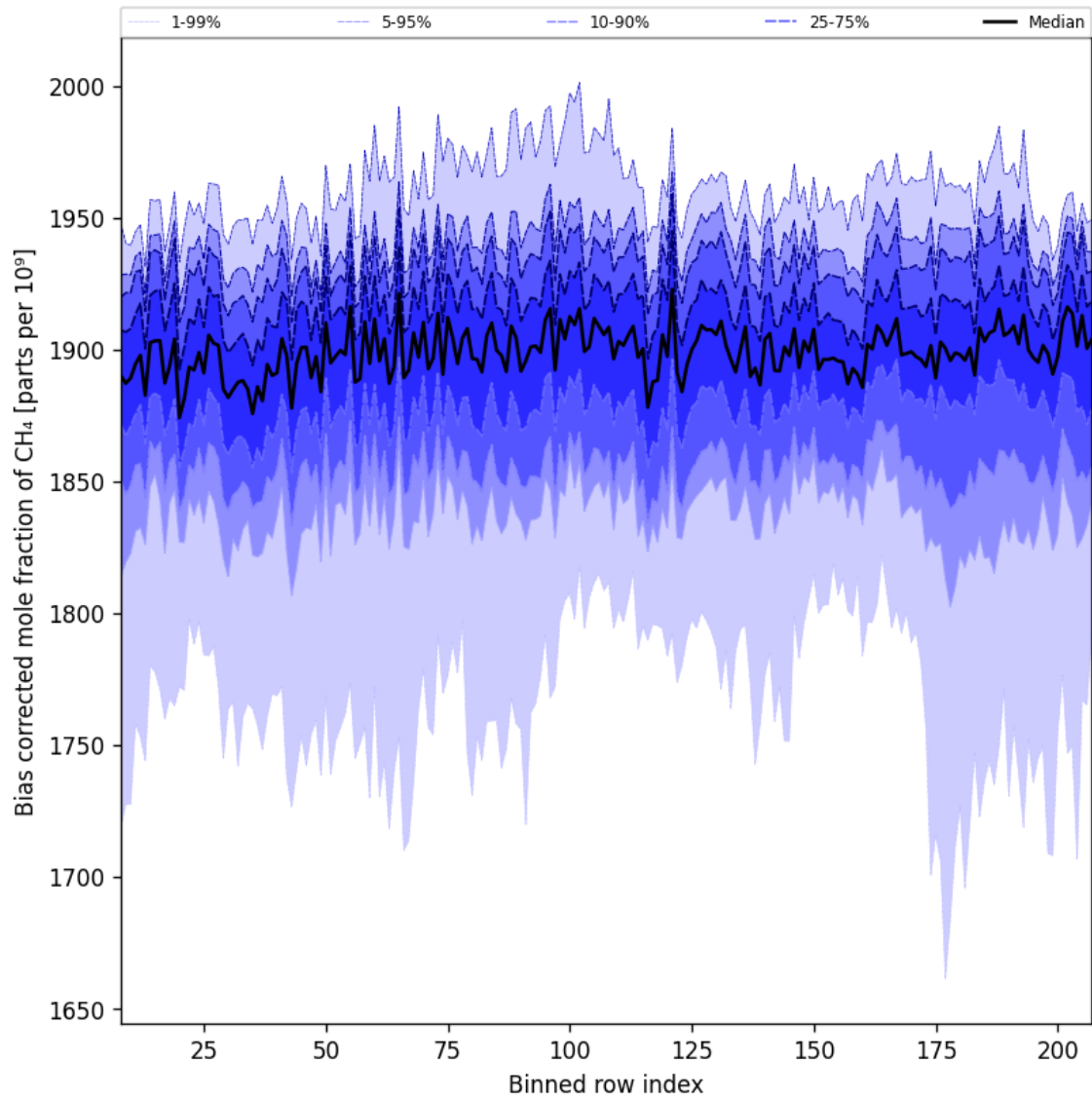
Figure 36: Along track statistics of “Bias corrected mole fraction of CH 4 ” for 2025-07-22 to 2025-07-24
