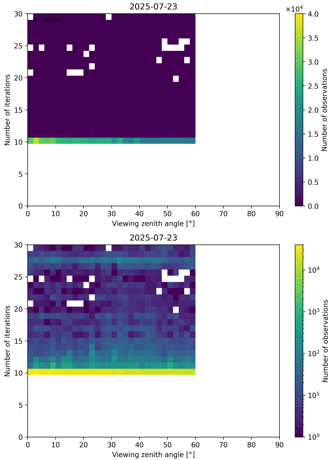
Figure 113: Scatter density plot of “Viewing zenith angle” against “Number of iterations” for 2025-07-22 to 2025-07-24.
