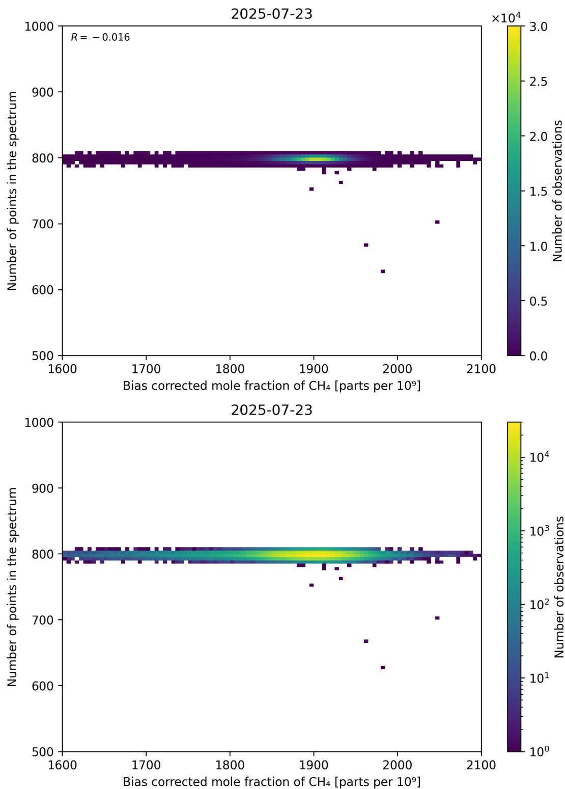
Figure 68: Scatter density plot of “Bias corrected mole fraction of CH 4 ” against “Number of points in the spectrum” for 2025-07-22 to 2025-07-24.
