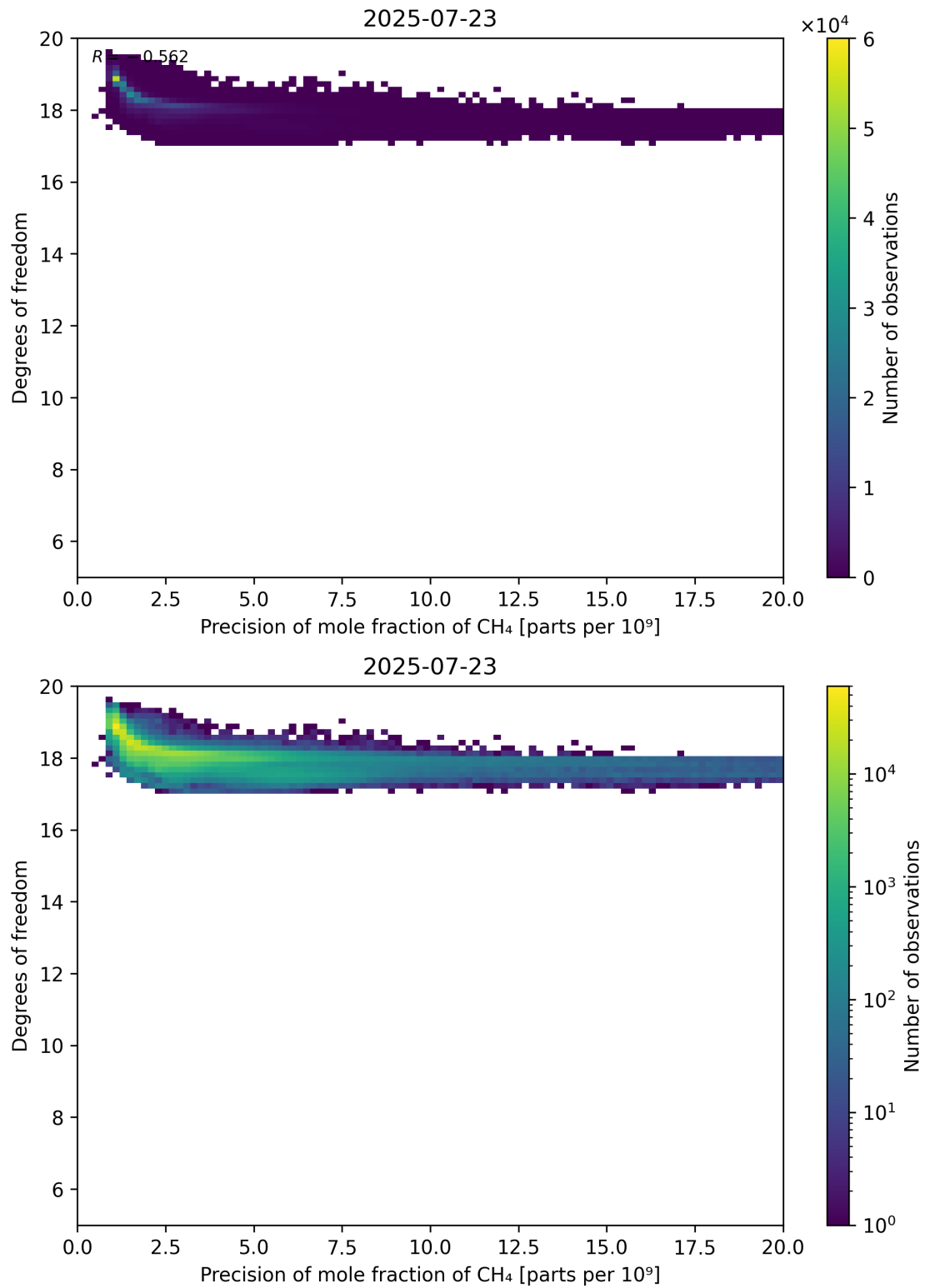
Figure 80: Scatter density plot of “Precision of mole fraction of CH 4 ” against “Degrees of freedom” for 2025-07-22 to 2025-07-24.
