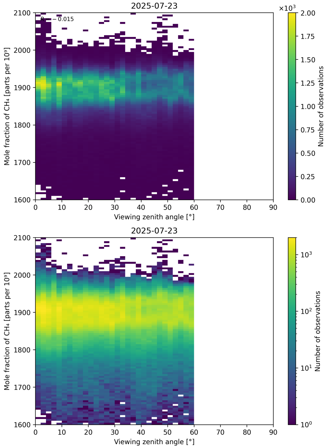
Figure 110: Scatter density plot of “Viewing zenith angle” against “Mole fraction of CH 4 ” for 2025-07-22 to 2025-07-24.
