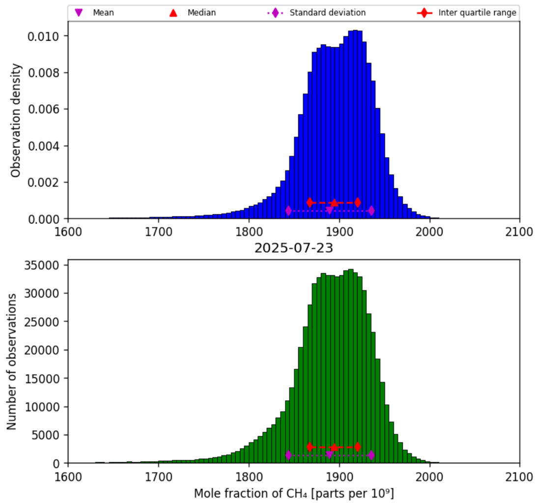
Figure 23: Histogram of “Mole fraction of CH 4 ” for 2025-07-22 to 2025-07-24
