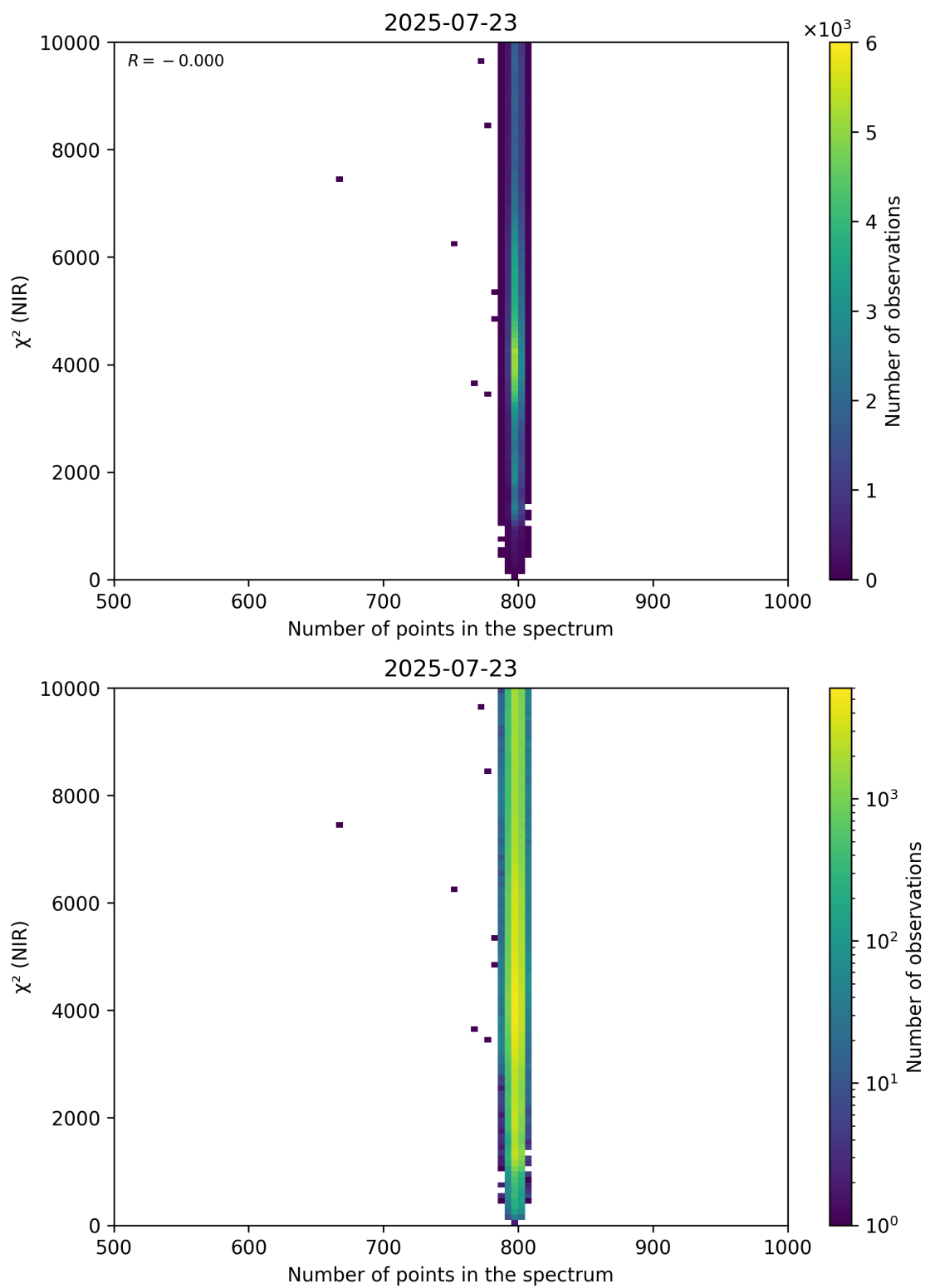
Figure 88: Scatter density plot of “Number of points in the spectrum” against “ \chi^2 (NIR)” for 2025-07-22 to 2025-07-24.
