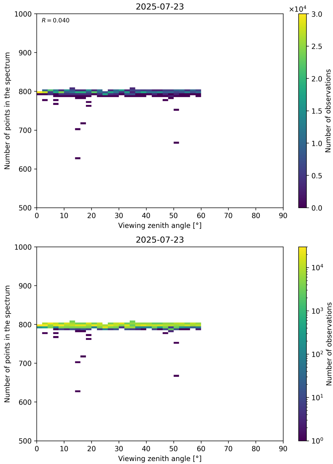
Figure 114: Scatter density plot of “Viewing zenith angle” against “Number of points in the spectrum” for 2025-07-22 to 2025-07-24.
