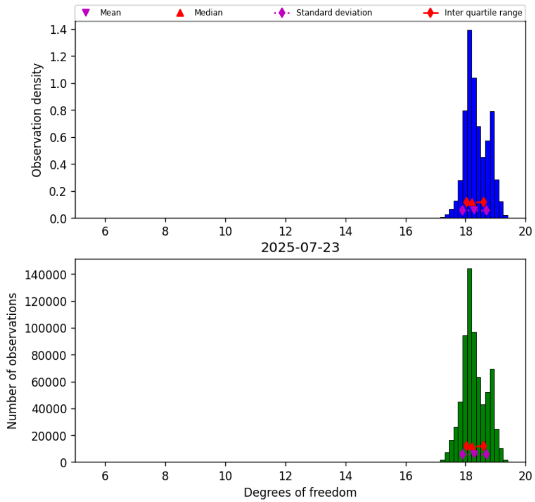
Figure 30: Histogram of “Degrees of freedom” for 2025-07-22 to 2025-07-24
