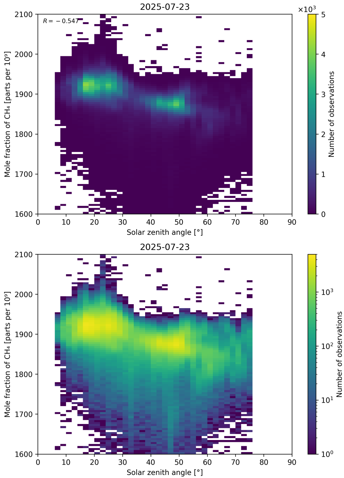
Figure 99: Scatter density plot of “Solar zenith angle” against “Mole fraction of CH 4 ” for 2025-07-22 to 2025-07-24.
