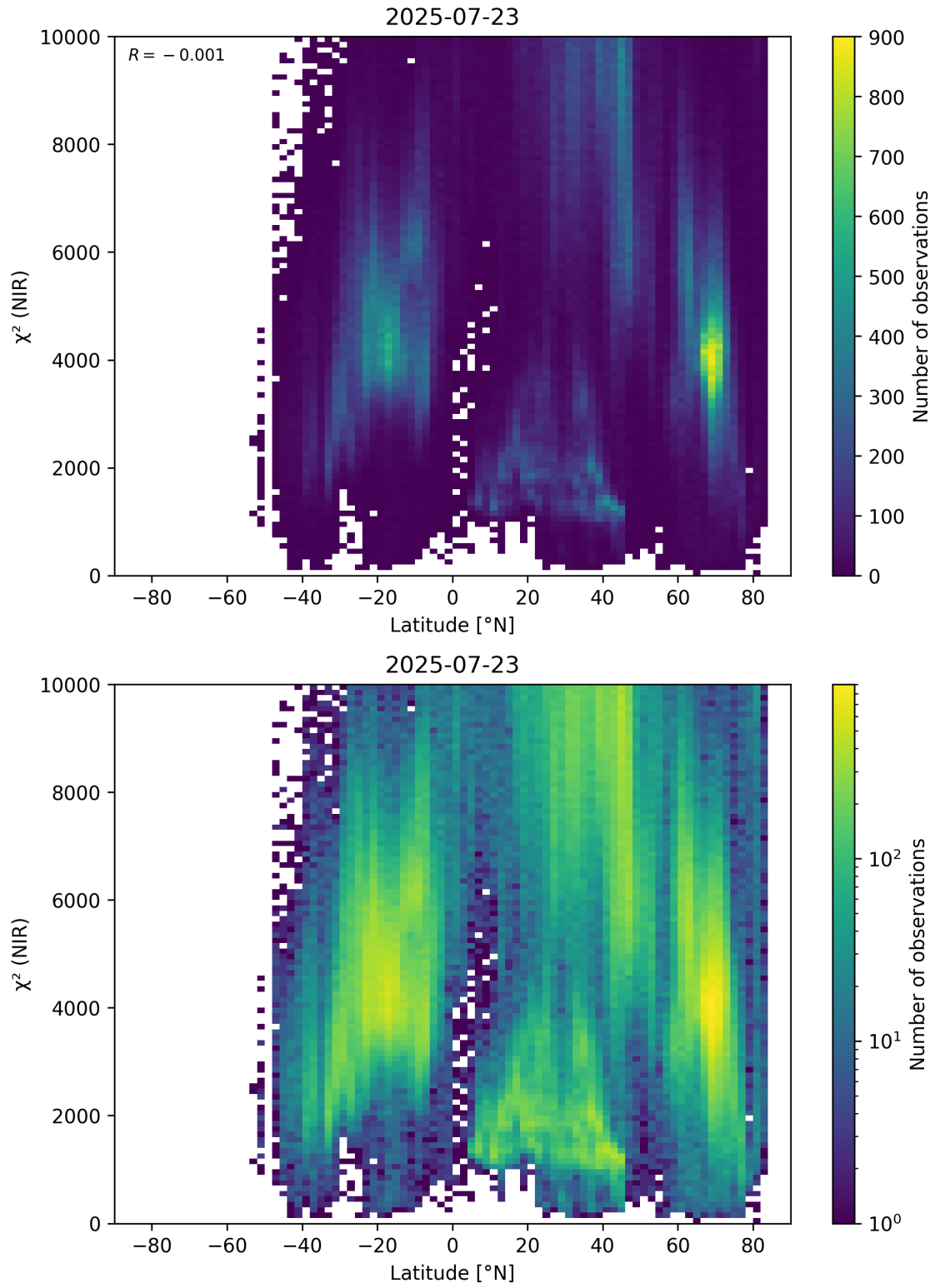
Figure 53: Scatter density plot of “Latitude” against “ \chi^2 (NIR)” for 2025-07-22 to 2025-07-24.
