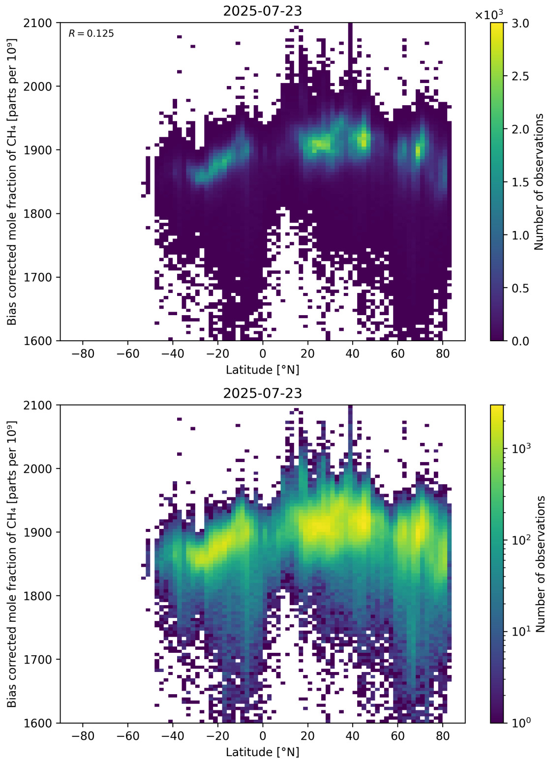
Figure 58: Scatter density plot of “Latitude” against “Bias corrected mole fraction of CH 4 ” for 2025-07-22 to 2025-07-24.
