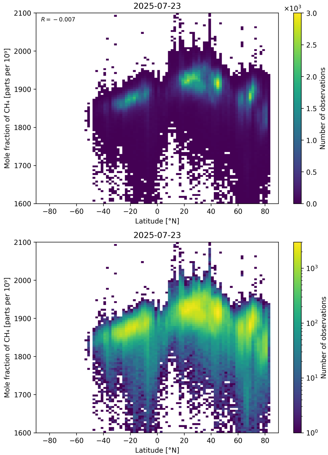
Figure 57: Scatter density plot of “Latitude” against “Mole fraction of \text{CH}_4 ” for 2025-07-22 to 2025-07-24.
