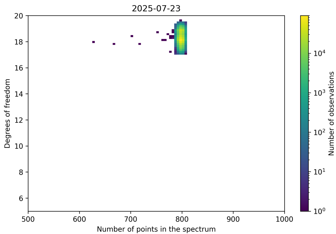
Figure 90: Scatter density plot of “Number of points in the spectrum” against “Degrees of freedom” for 2025-07-22 to 2025-07-24.
