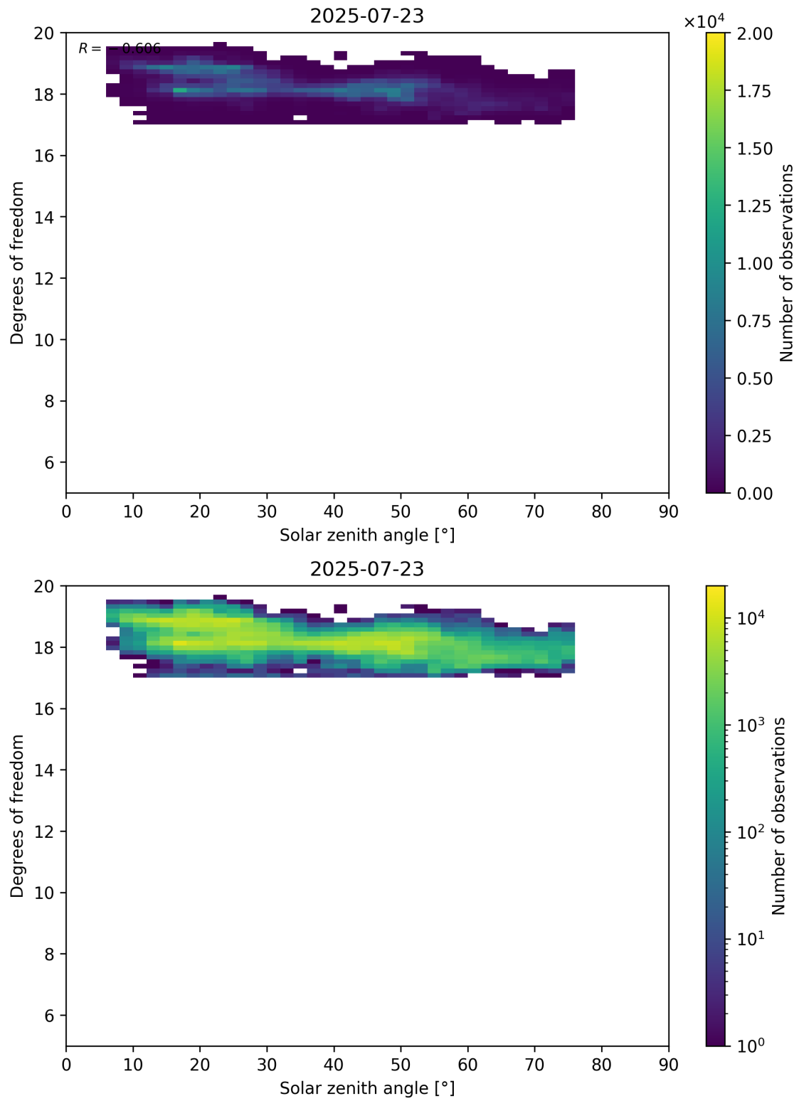
Figure 96: Scatter density plot of “Solar zenith angle” against “Degrees of freedom” for 2025-07-22 to 2025-07-24.
