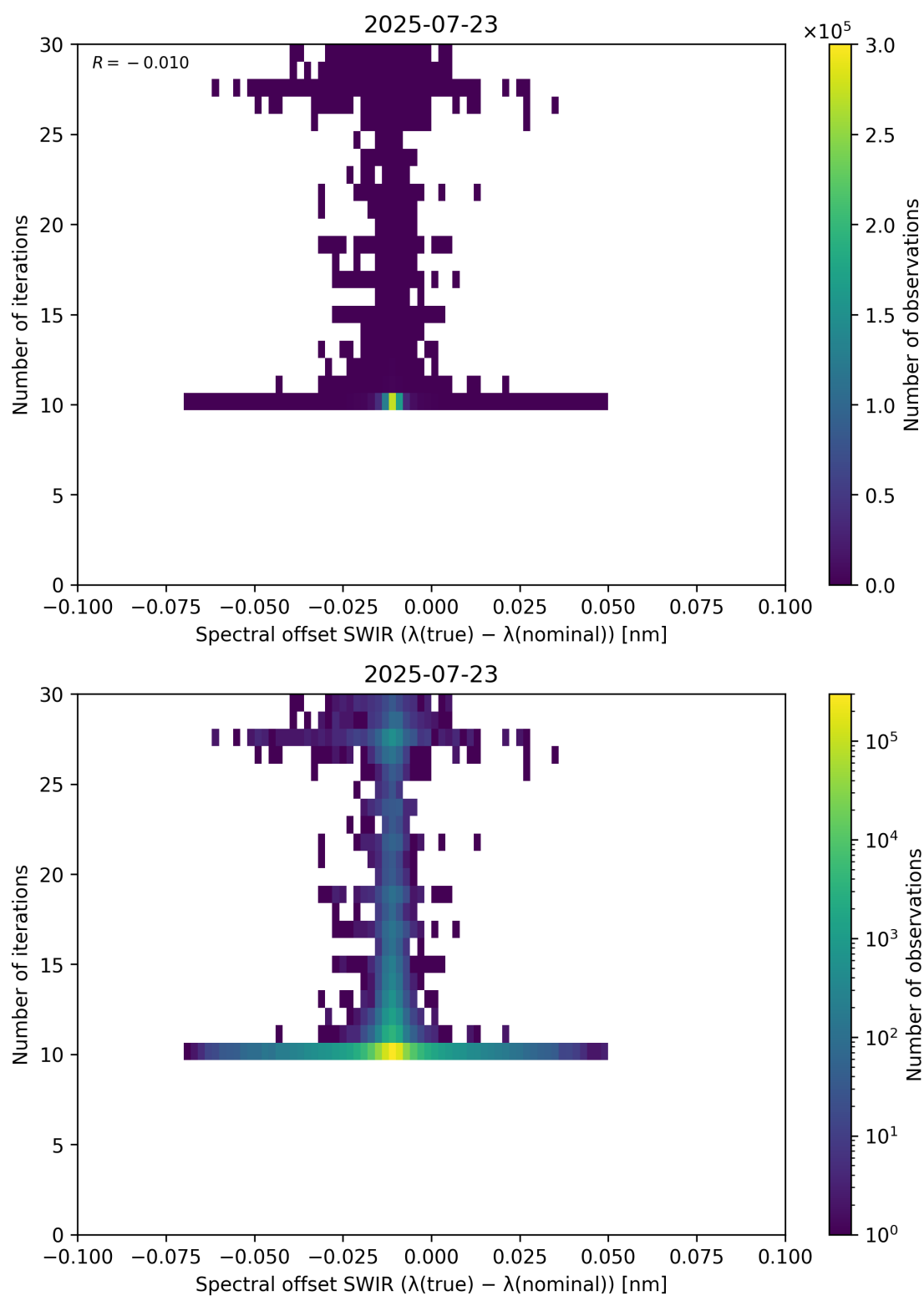
Figure 121: Scatter density plot of “Spectral offset SWIR ( \lambda_{\text{true}} - \lambda_{\text{nominal}} )” against “Number of iterations” for 2025-07-22 to 2025-07-24.
