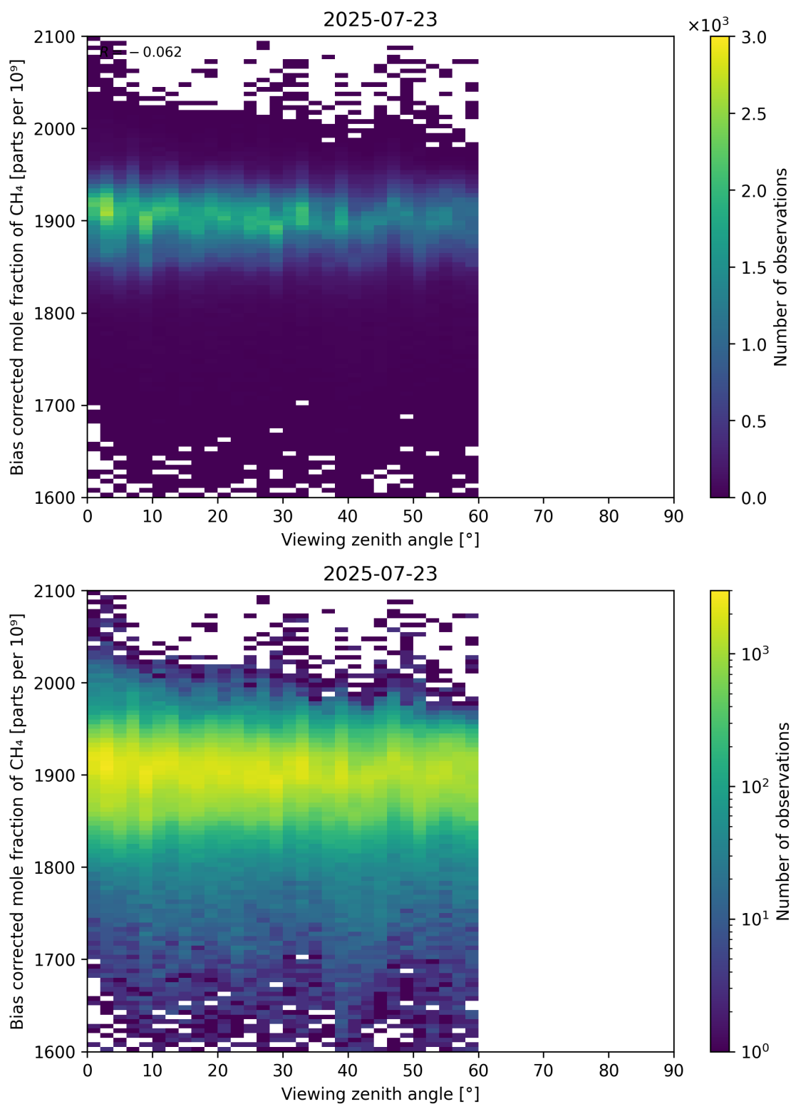
Figure 111: Scatter density plot of “Viewing zenith angle” against “Bias corrected mole fraction of CH 4 ” for 2025-07-22 to 2025-07-24.
