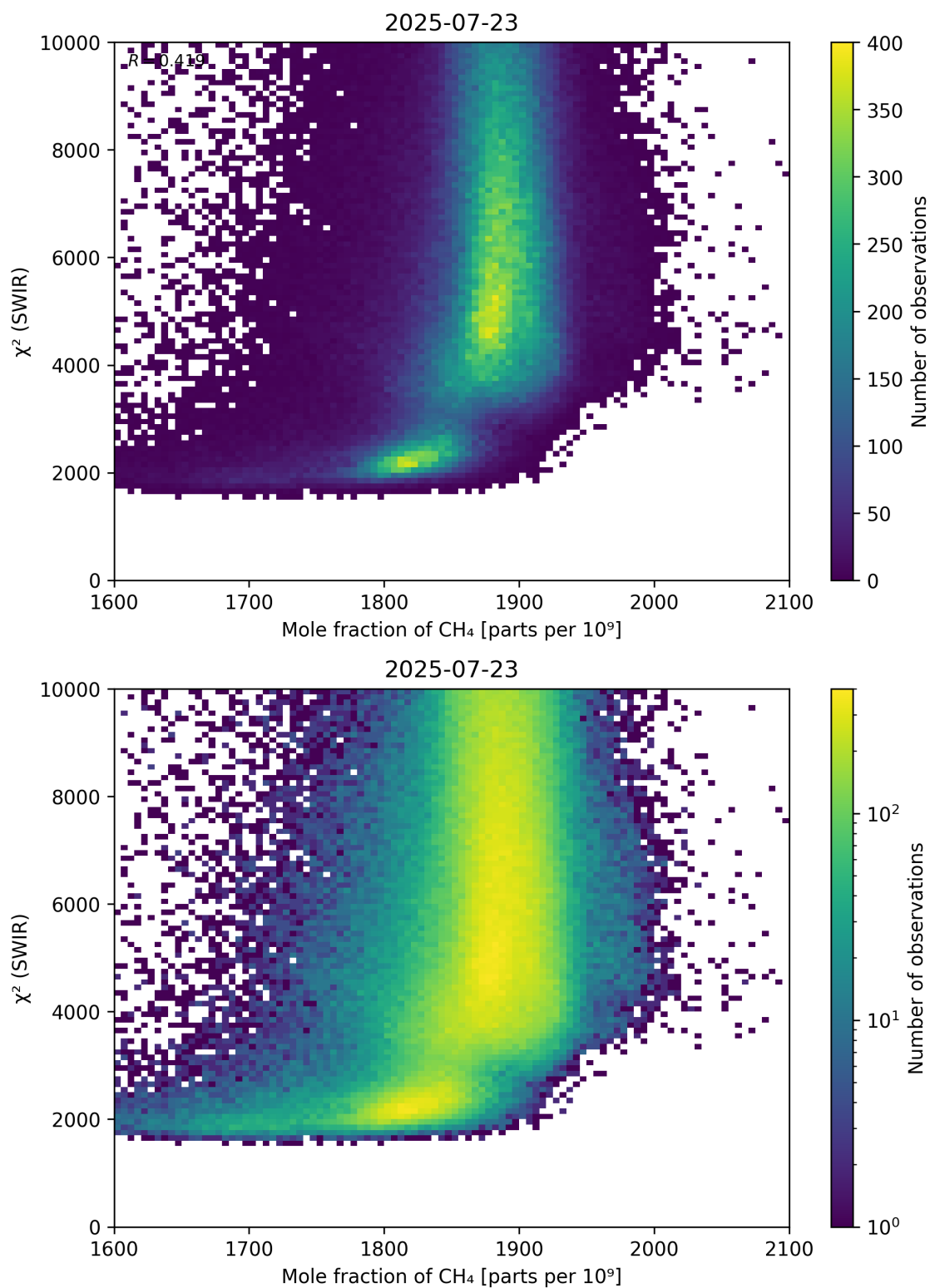
Figure 71: Scatter density plot of “Mole fraction of CH 4 ” against “ \chi^2 (SWIR)” for 2025-07-22 to 2025-07-24.
