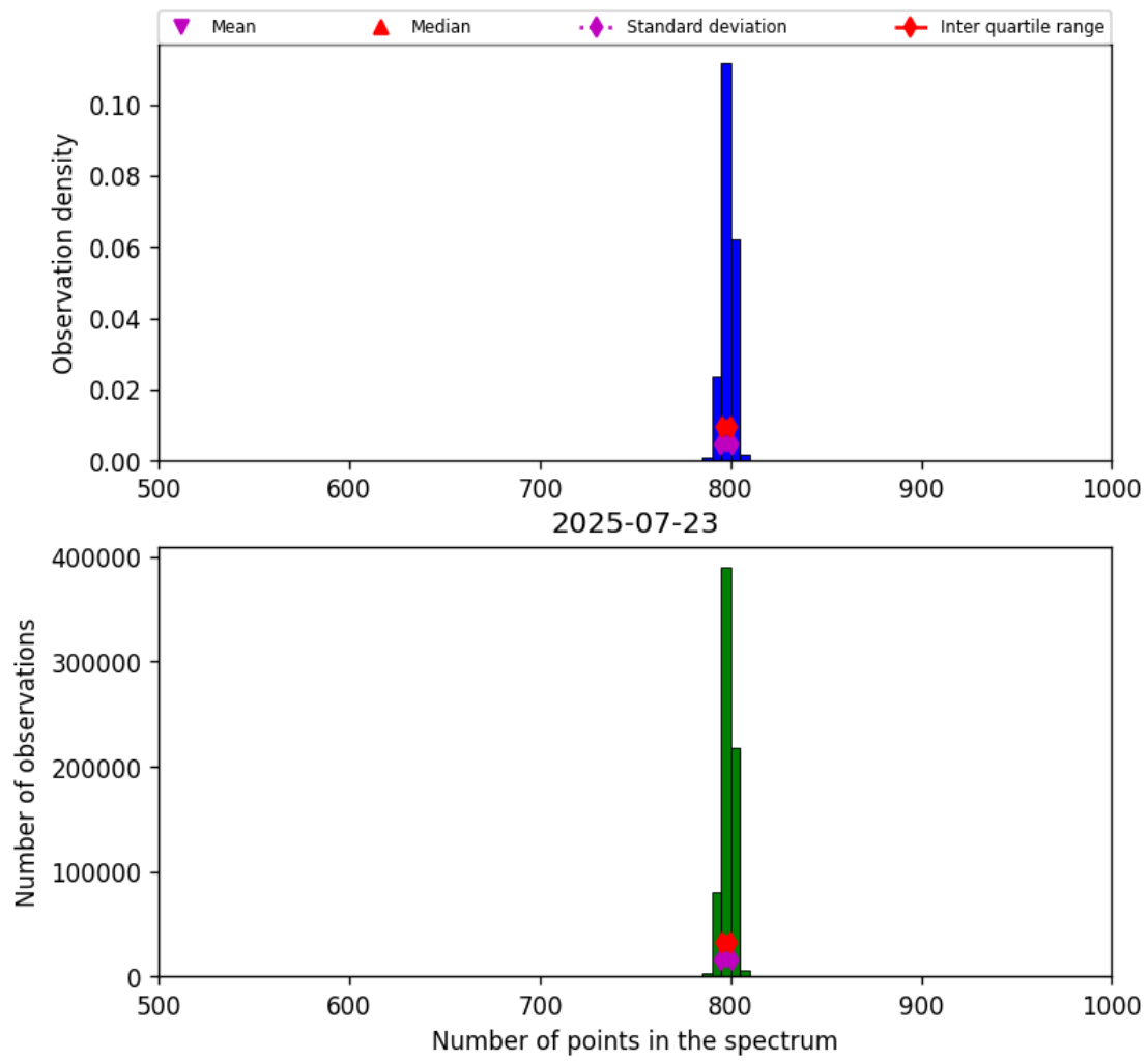
Figure 26: Histogram of “Number of points in the spectrum” for 2025-07-22 to 2025-07-24
