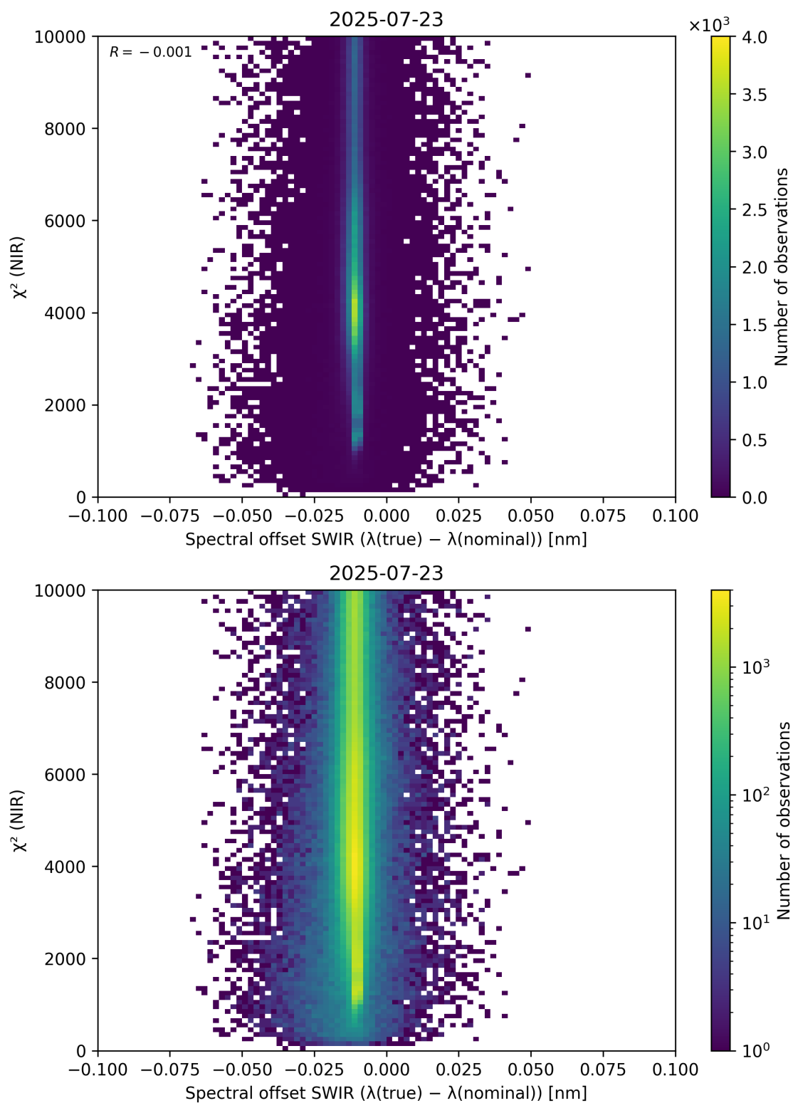
Figure 117: Scatter density plot of “Spectral offset SWIR ( \lambda_{\text{true}} - \lambda_{\text{nominal}} )” against “ \chi^2 (NIR)” for 2025-07-22 to 2025-07-24.
