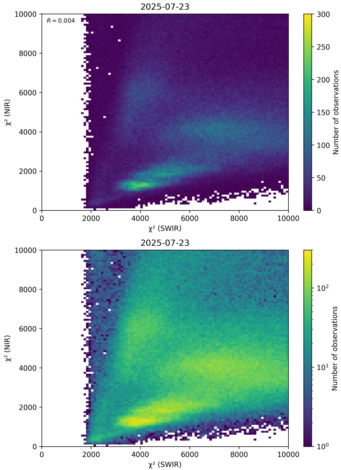
Figure 47: Scatter density plot of “ \chi^2 (SWIR)” against “ \chi^2 (NIR)” for 2025-07-22 to 2025-07-24.
