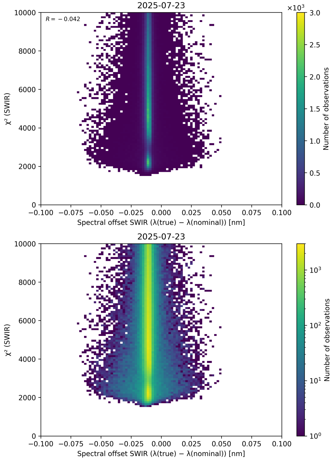
Figure 118: Scatter density plot of “Spectral offset SWIR ( \lambda_{\text{true}} - \lambda_{\text{nominal}} )” against “ \chi^2 (SWIR)” for 2025-07-22 to 2025-07-24.
