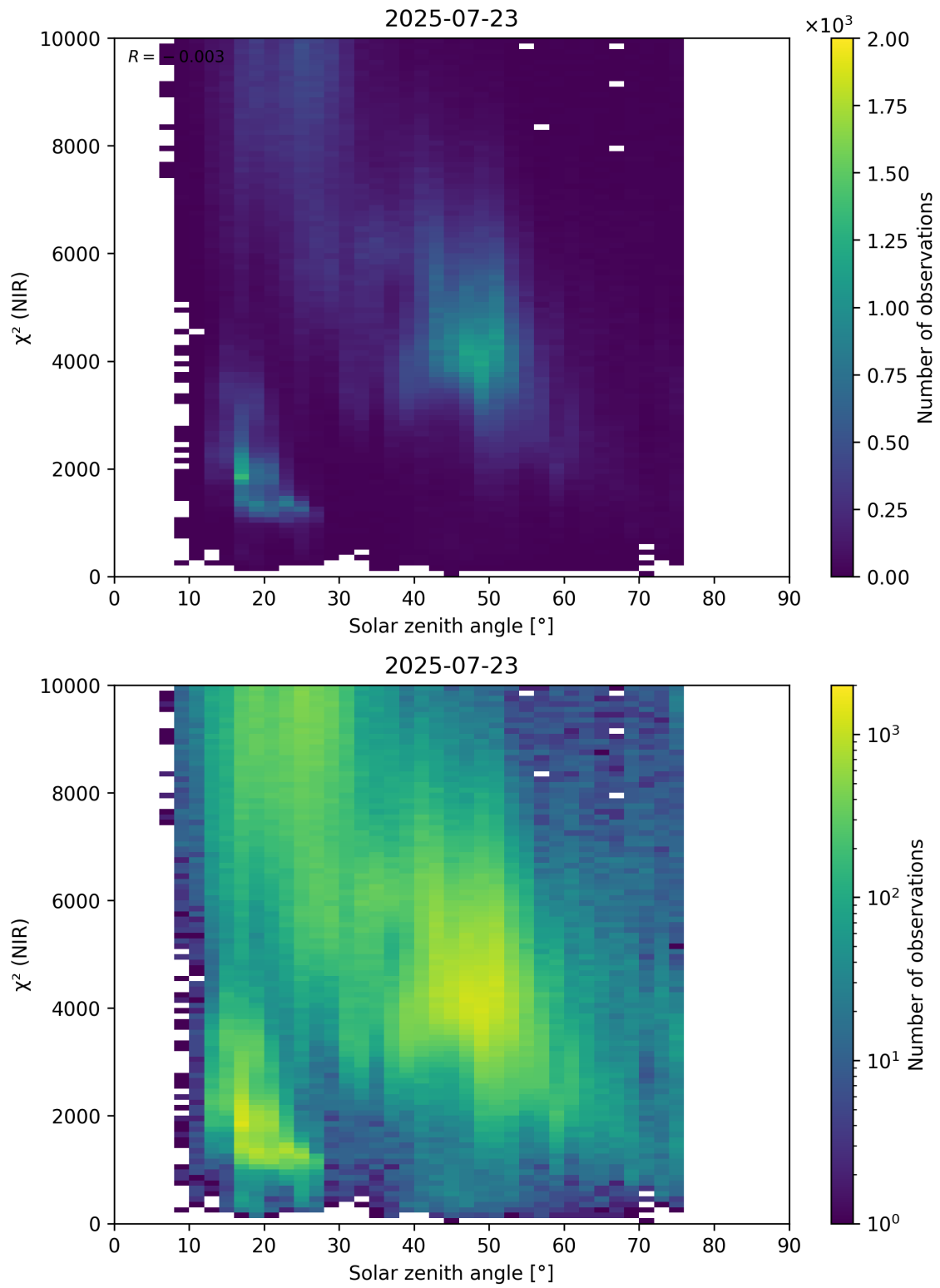
Figure 94: Scatter density plot of “Solar zenith angle” against “ \chi^2 (NIR)” for 2025-07-22 to 2025-07-24.
