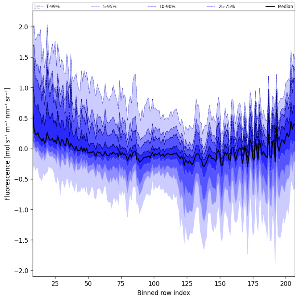
Figure 43: Along track statistics of “Fluorescence” for 2025-07-22 to 2025-07-24
