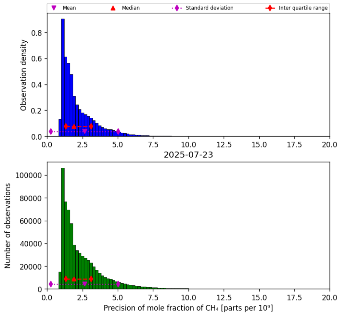
Figure 24: Histogram of “Precision of mole fraction of CH 4 ” for 2025-07-22 to 2025-07-24
