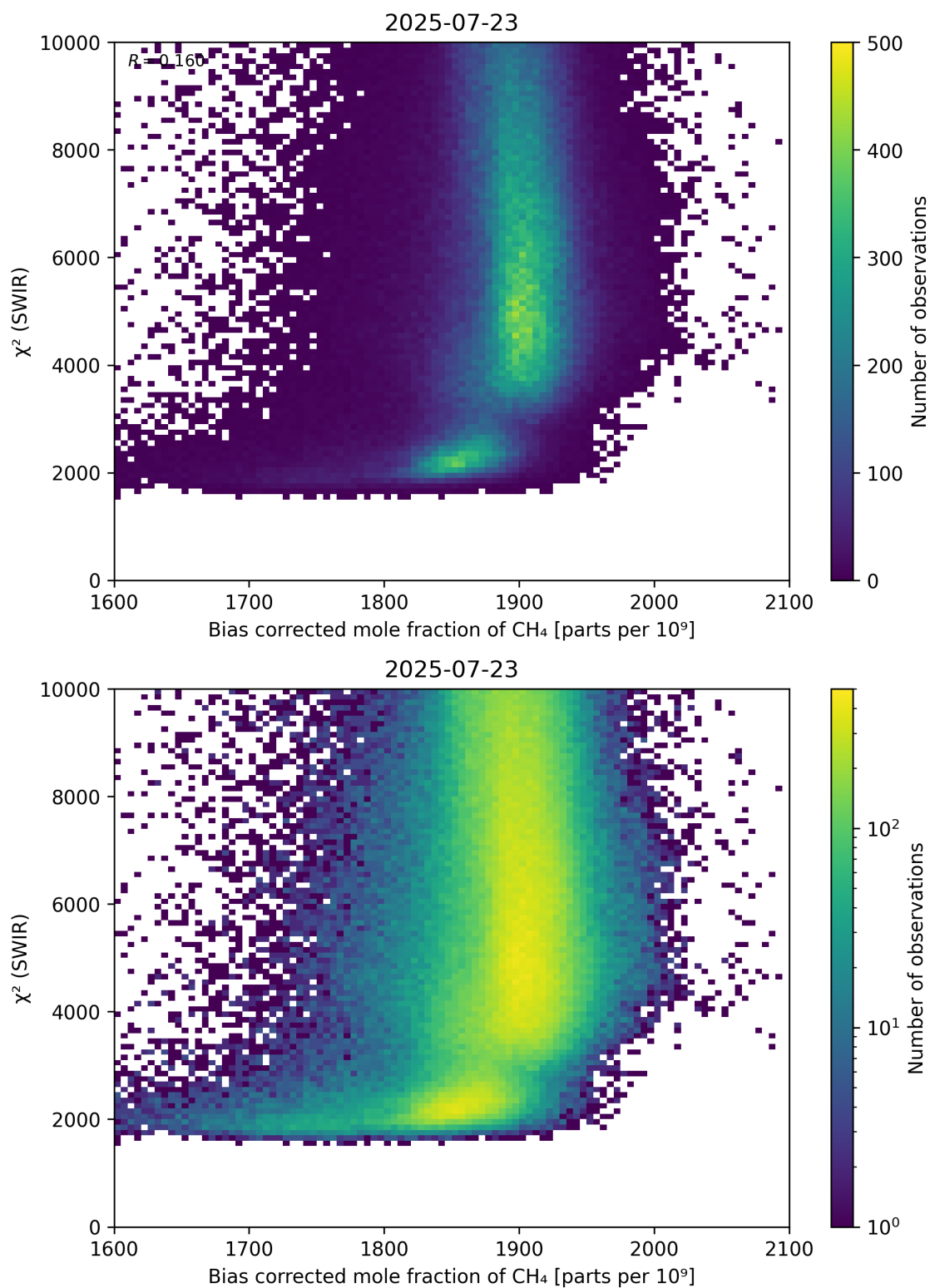
Figure 64: Scatter density plot of “Bias corrected mole fraction of \text{CH}_4 ” against “ \chi^2 (SWIR)” for 2025-07-22 to 2025-07-24.
