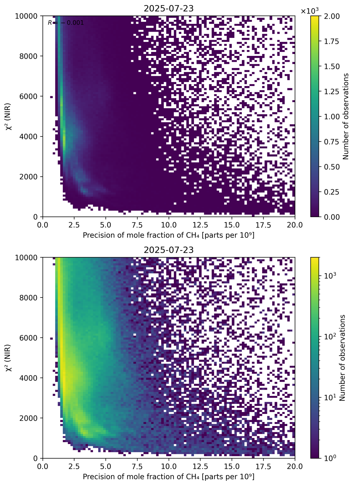
Figure 78: Scatter density plot of “Precision of mole fraction of CH 4 ” against “ \chi^2 (NIR)” for 2025-07-22 to 2025-07-24.
