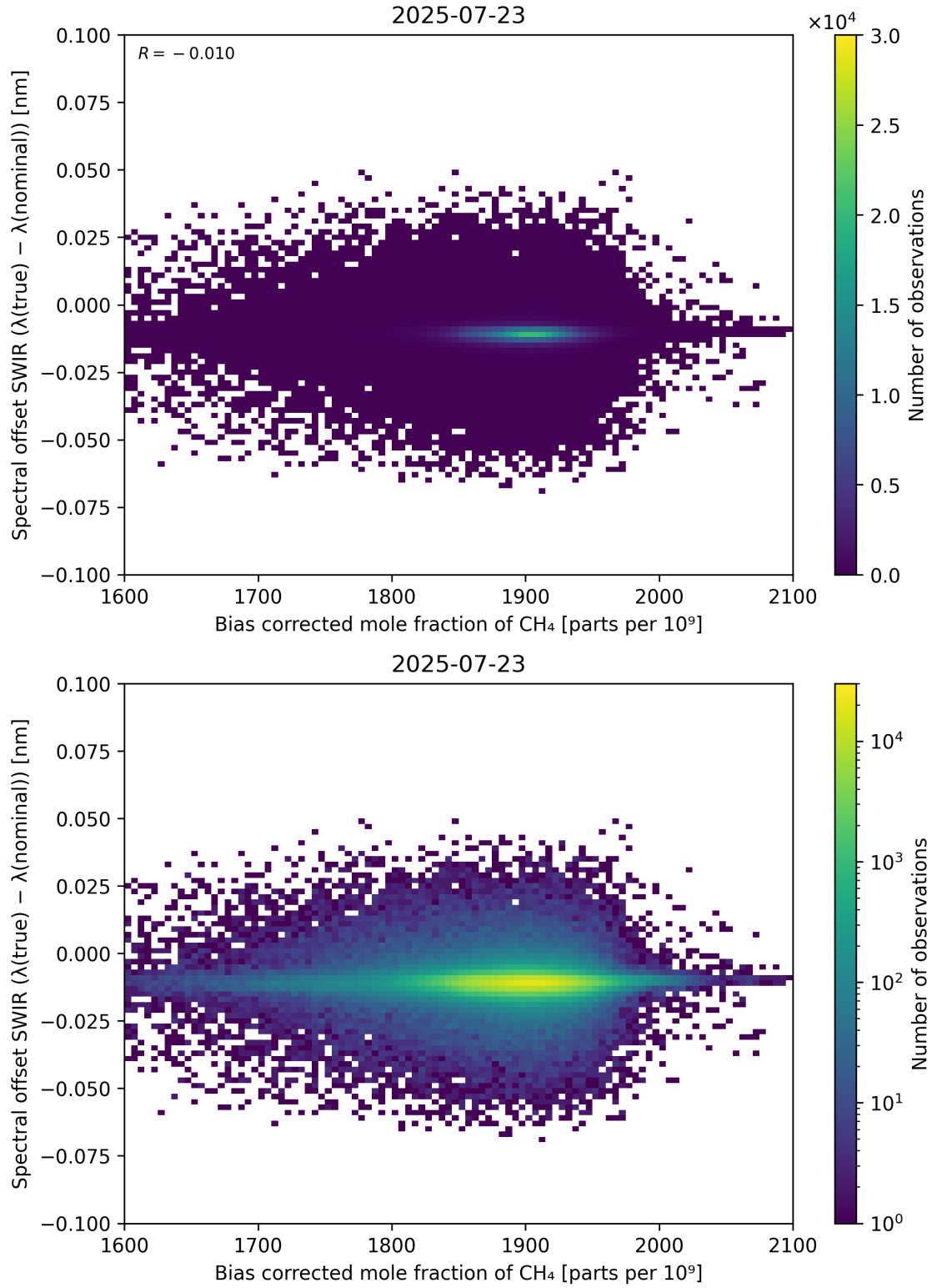
Figure 69: Scatter density plot of “Bias corrected mole fraction of CH 4 ” against “Spectral offset SWIR ( \lambda_{\text{true}} - \lambda_{\text{nominal}} )” for 2025-07-22 to 2025-07-24.
