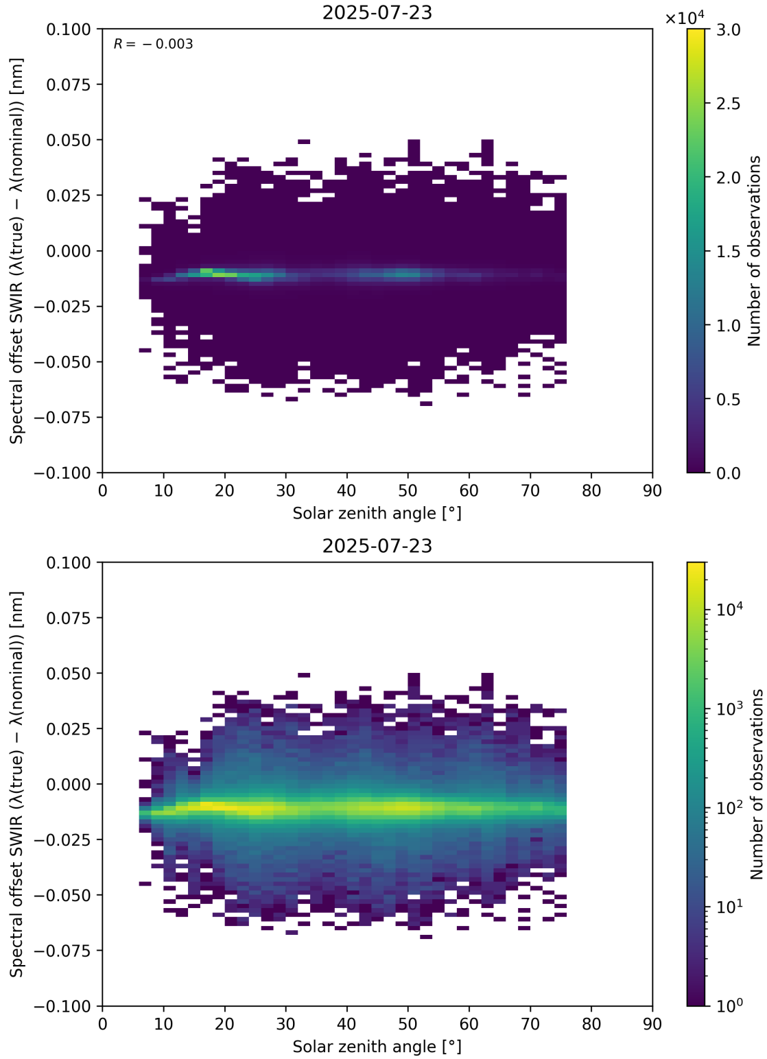
Figure 104: Scatter density plot of “Solar zenith angle” against “Spectral offset SWIR ( \lambda_{\text{true}} - \lambda_{\text{nominal}} )” for 2025-07-22 to 2025-07-24.
