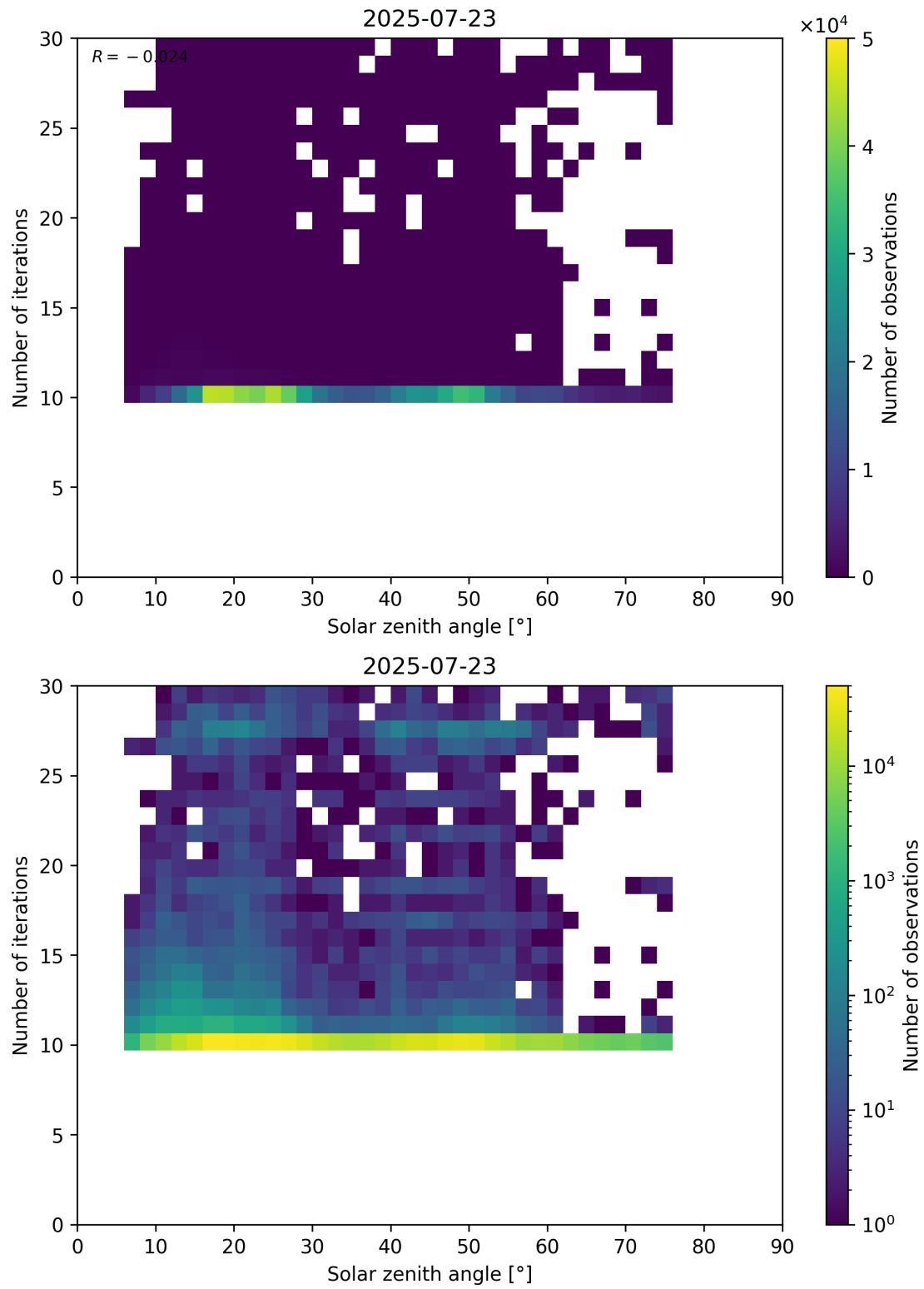
Figure 102: Scatter density plot of “Solar zenith angle” against “Number of iterations” for 2025-07-22 to 2025-07-24.
