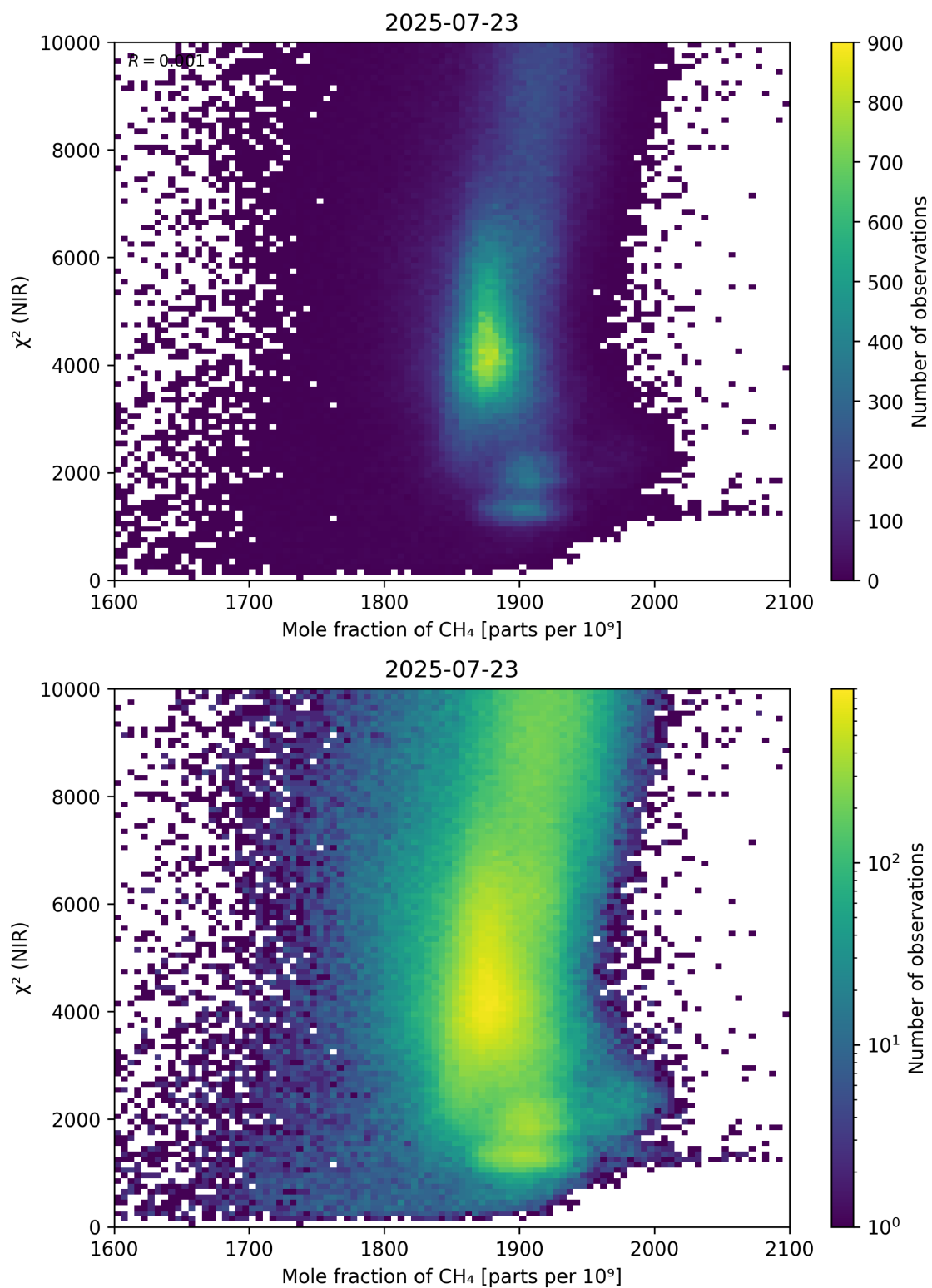
Figure 70: Scatter density plot of “Mole fraction of \text{CH}_4 ” against “ \chi^2 (NIR)” for 2025-07-22 to 2025-07-24.
