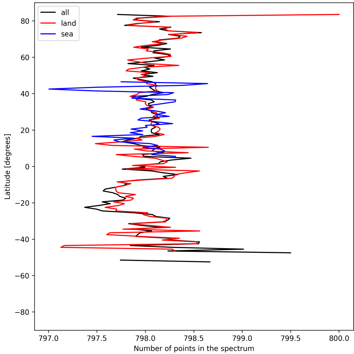
Figure 15: Zonal average of “Number of points in the spectrum” for 2025-07-22 to 2025-07-24.
