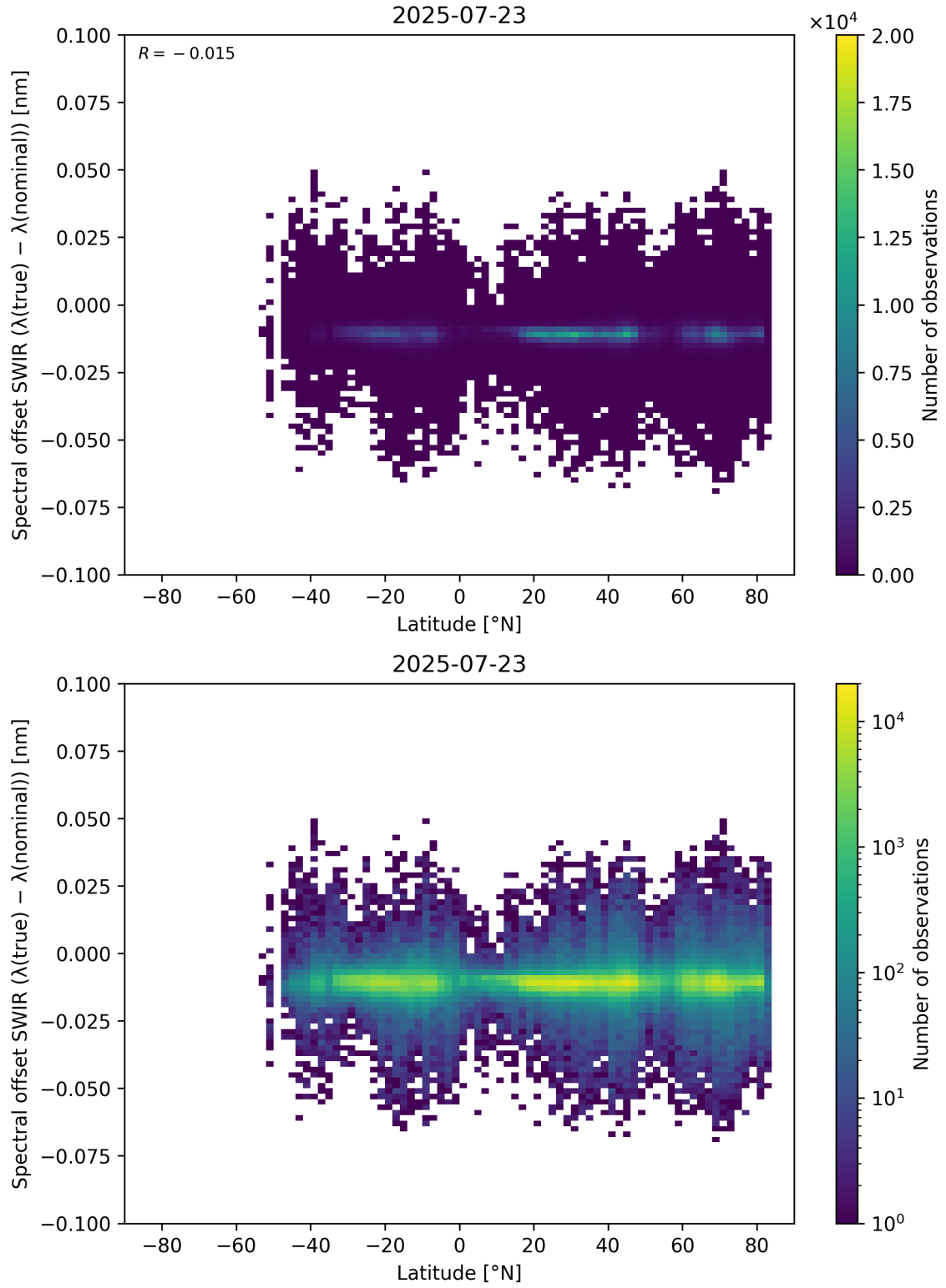
Figure 62: Scatter density plot of “Latitude” against “Spectral offset SWIR ( \lambda_{\text{true}} - \lambda_{\text{nominal}} )” for 2025-07-22 to 2025-07-24.
