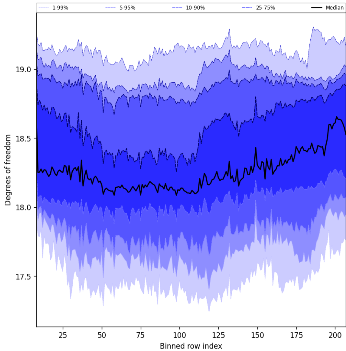
Figure 41: Along track statistics of “Degrees of freedom” for 2025-07-22 to 2025-07-24
