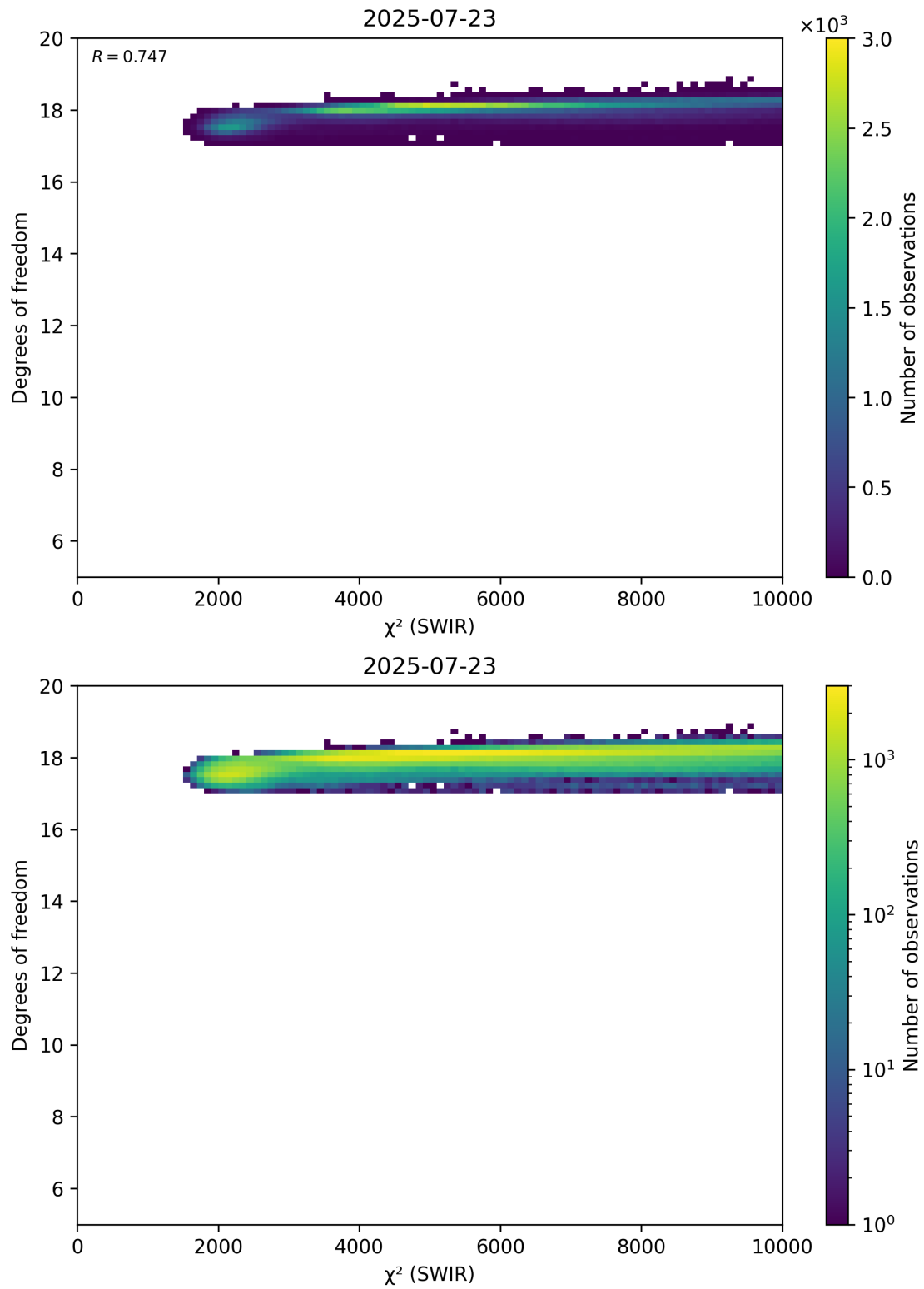
Figure 48: Scatter density plot of “ \chi^2 (SWIR)” against “Degrees of freedom” for 2025-07-22 to 2025-07-24.
