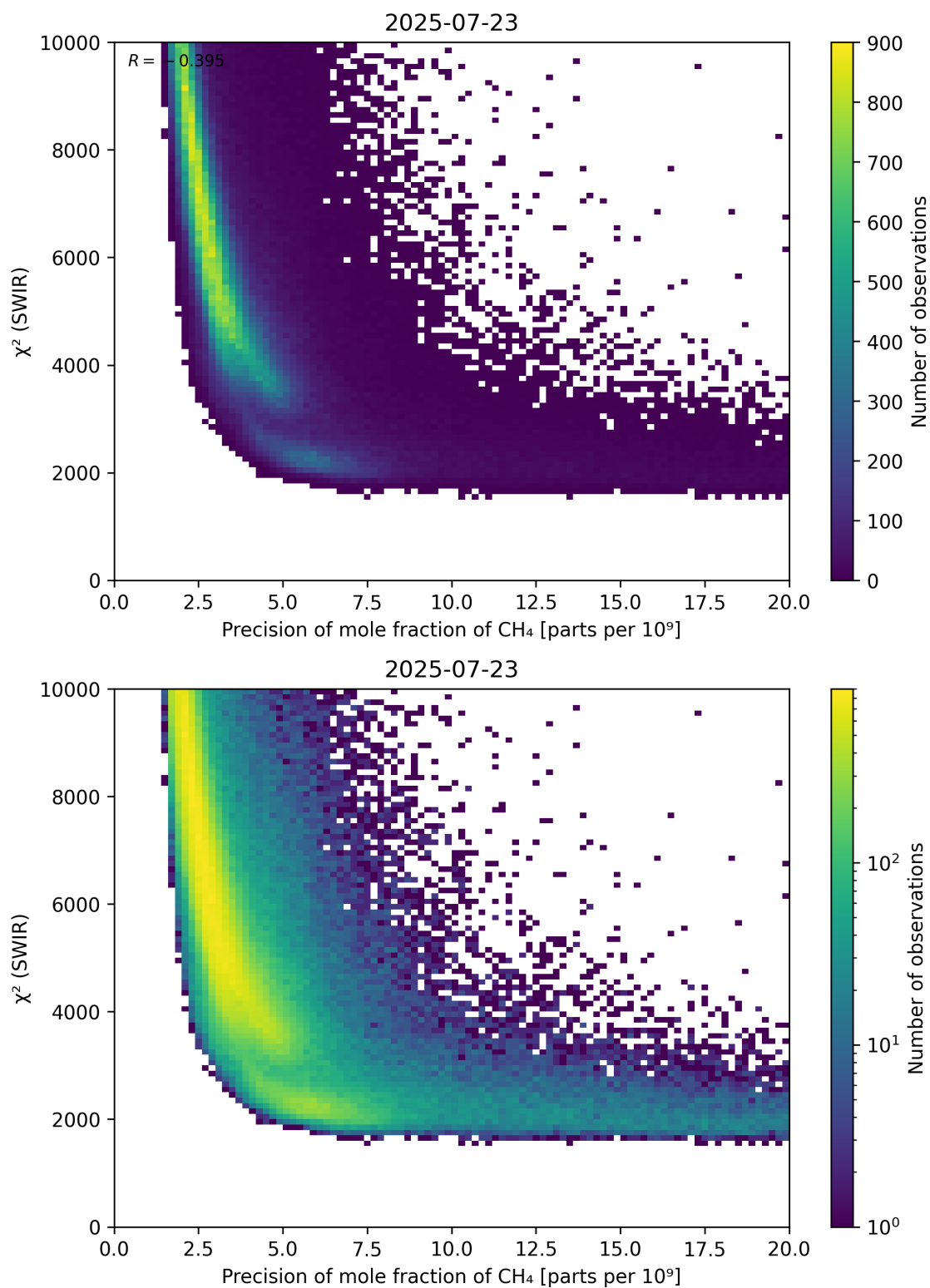
Figure 79: Scatter density plot of “Precision of mole fraction of \text{CH}_4 ” against “ \chi^2 (SWIR)” for 2025-07-22 to 2025-07-24.
