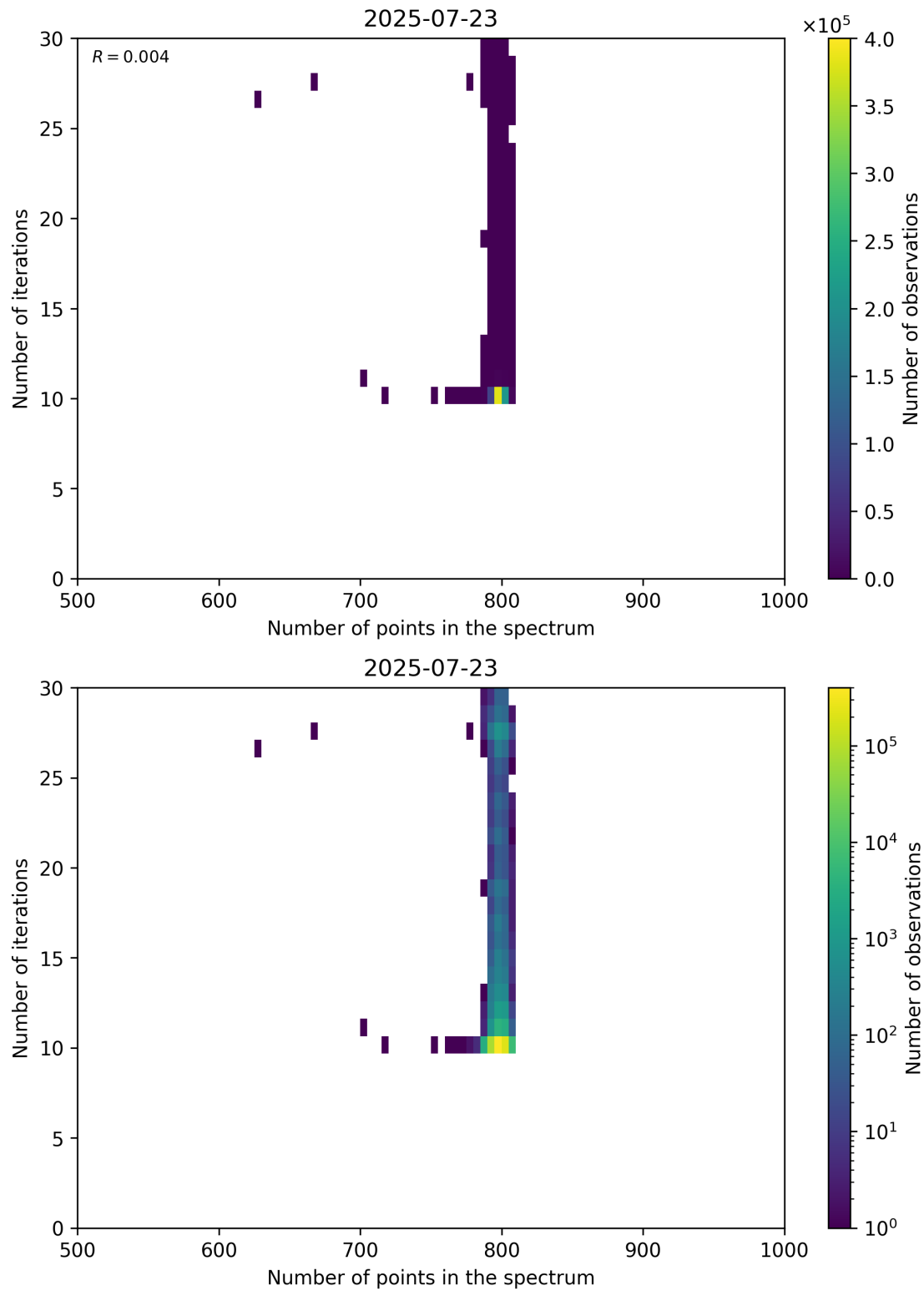
Figure 92: Scatter density plot of “Number of points in the spectrum” against “Number of iterations” for 2025-07-22 to 2025-07-24.
