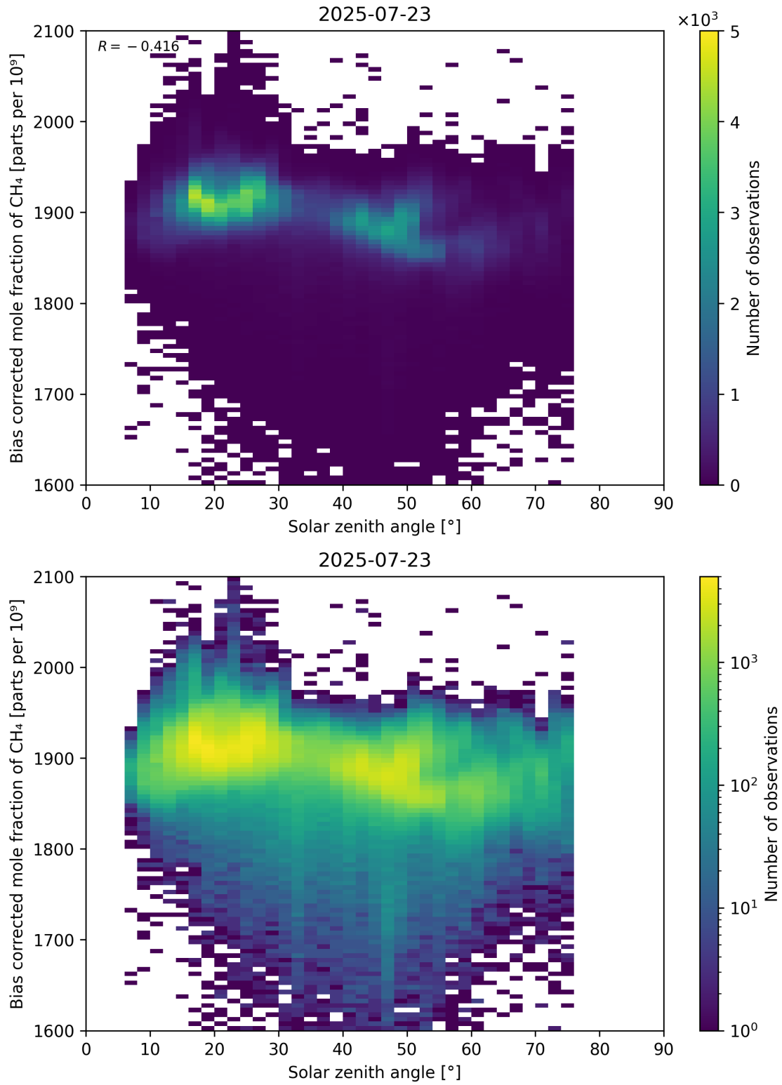
Figure 100: Scatter density plot of “Solar zenith angle” against “Bias corrected mole fraction of CH 4 ” for 2025-07-22 to 2025-07-24.
