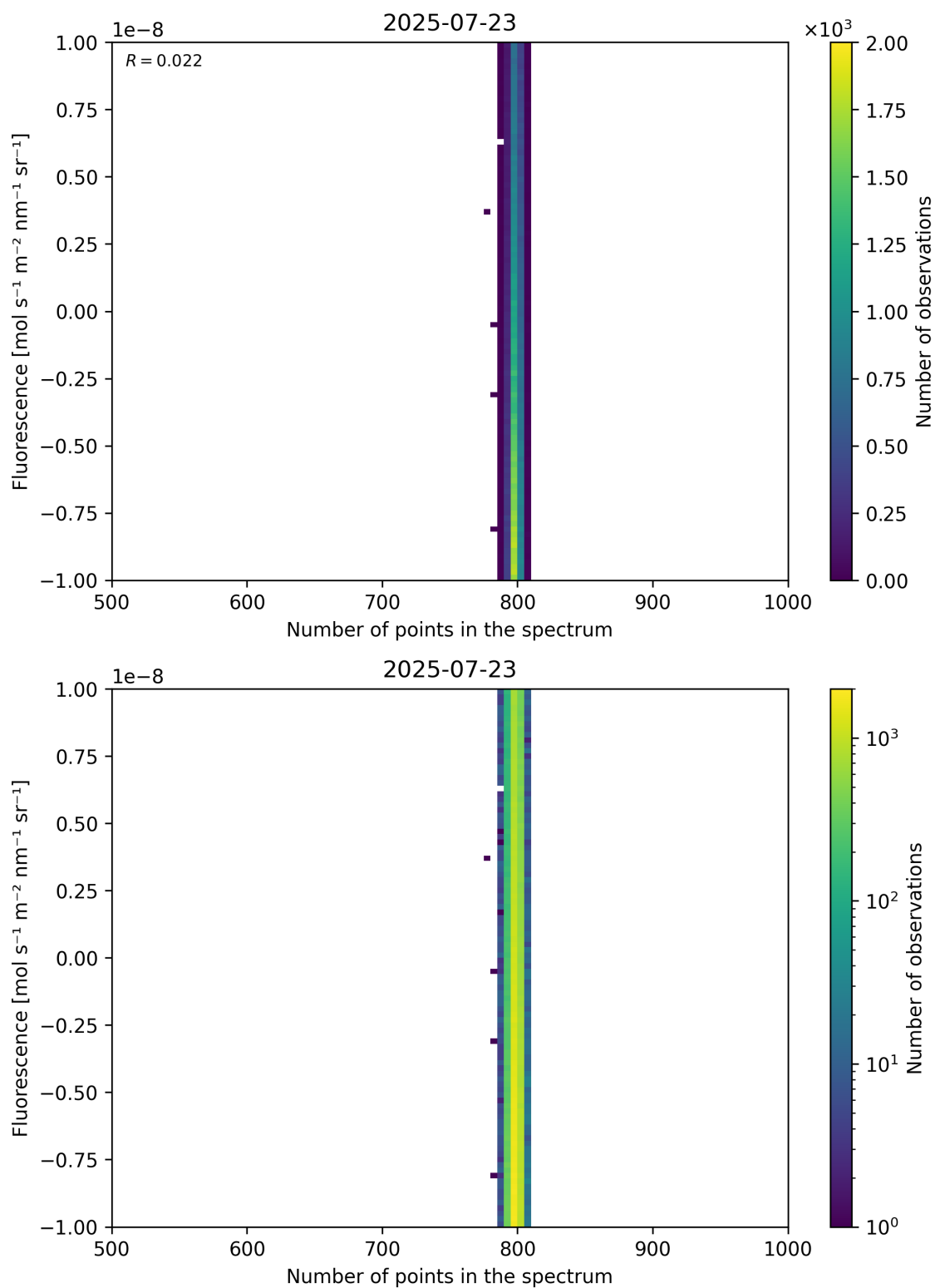
Figure 91: Scatter density plot of “Number of points in the spectrum” against “Fluorescence” for 2025-07-22 to 2025-07-24.
