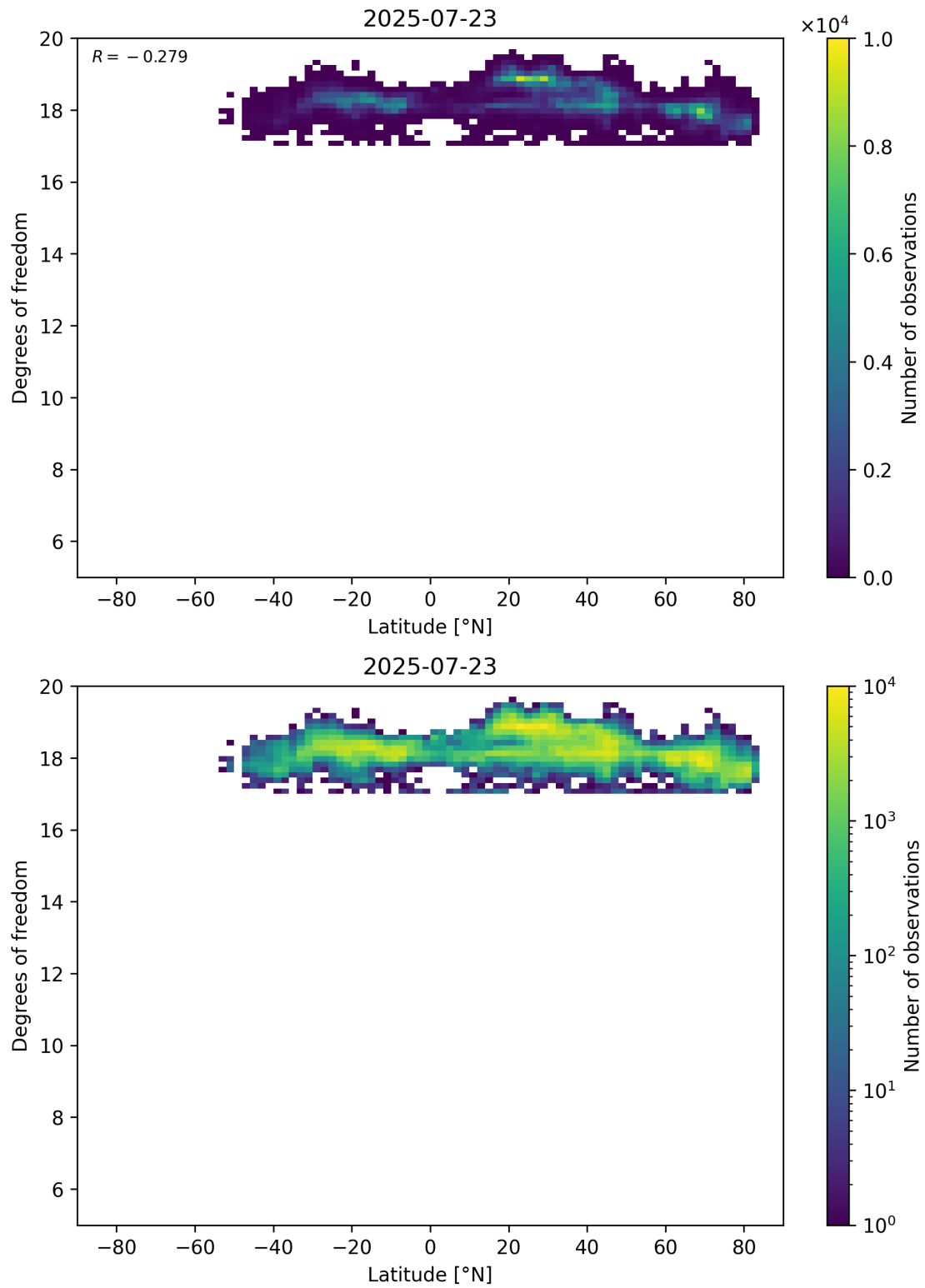
Figure 55: Scatter density plot of “Latitude” against “Degrees of freedom” for 2025-07-22 to 2025-07-24.
