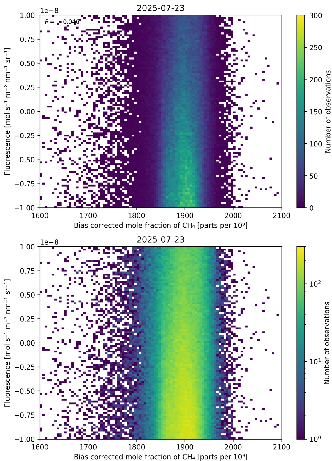
Figure 66: Scatter density plot of “Bias corrected mole fraction of \text{CH}_4 ” against “Fluorescence” for 2025-07-22 to 2025-07-24.
