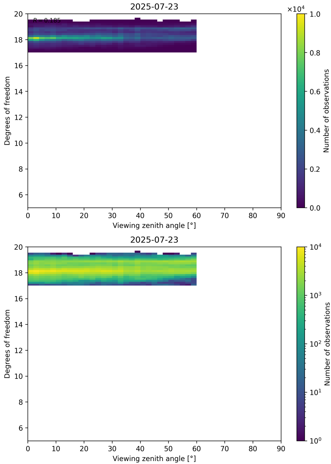
Figure 107: Scatter density plot of “Viewing zenith angle” against “Degrees of freedom” for 2025-07-22 to 2025-07-24.
