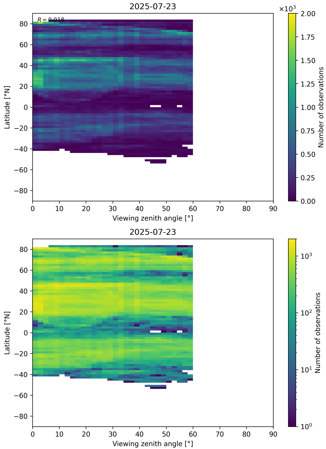
Figure 109: Scatter density plot of “Viewing zenith angle” against “Latitude” for 2025-07-22 to 2025-07-24.
