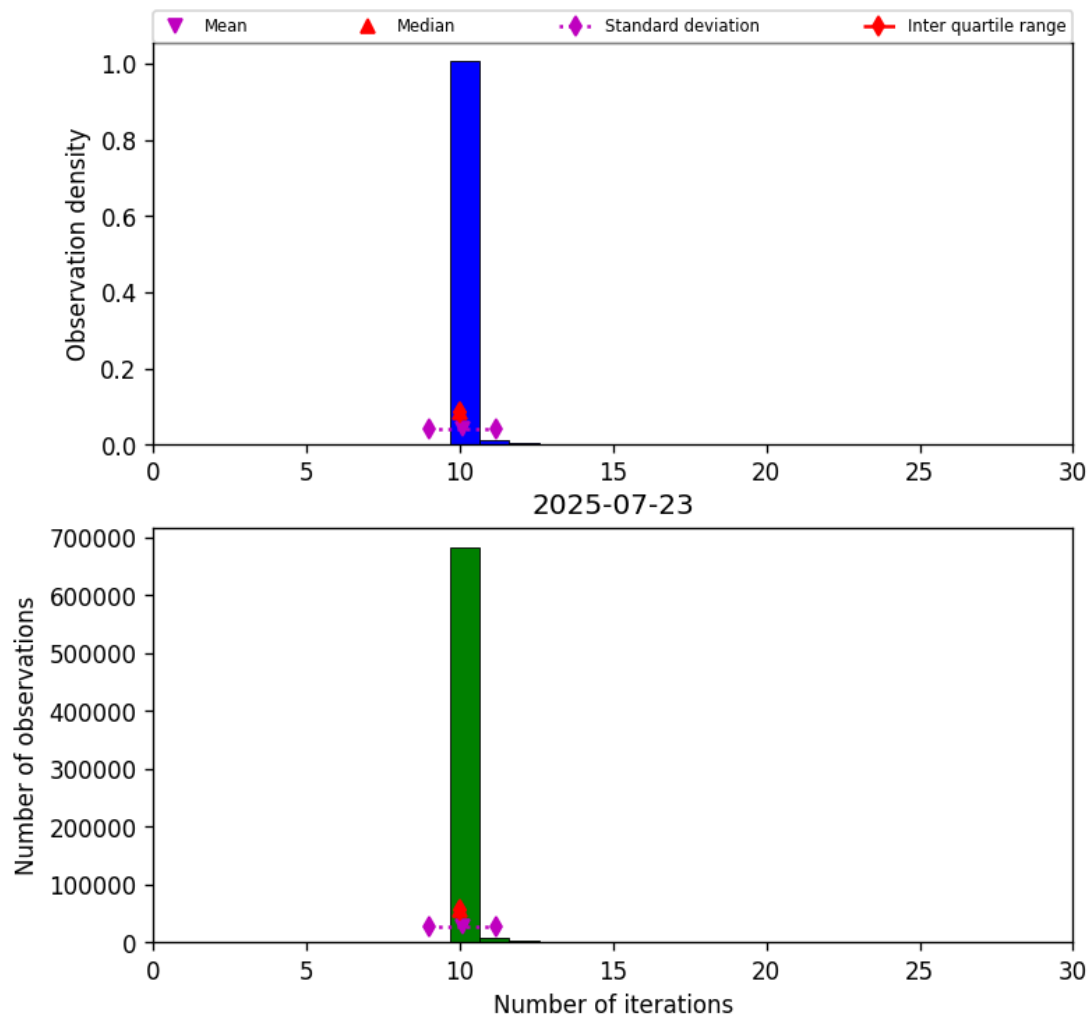
Figure 31: Histogram of “Number of iterations” for 2025-07-22 to 2025-07-24
