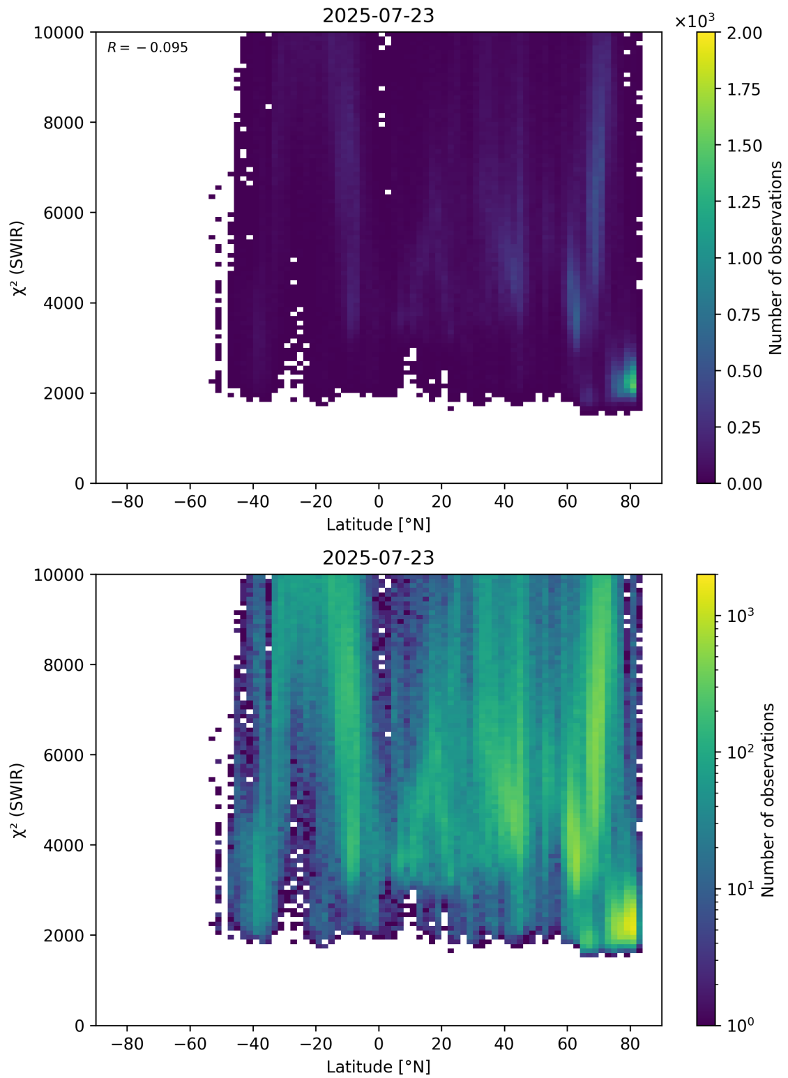
Figure 54: Scatter density plot of “Latitude” against “ \chi^2 (SWIR)” for 2025-07-22 to 2025-07-24.
