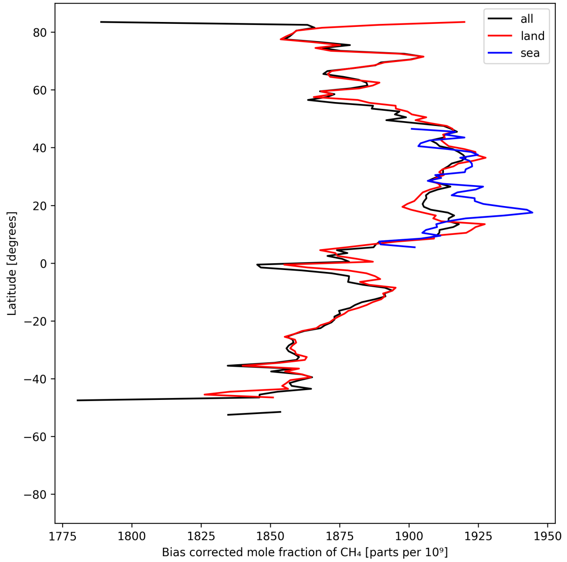
Figure 14: Zonal average of “Bias corrected mole fraction of CH 4 ” for 2025-07-22 to 2025-07-24.
