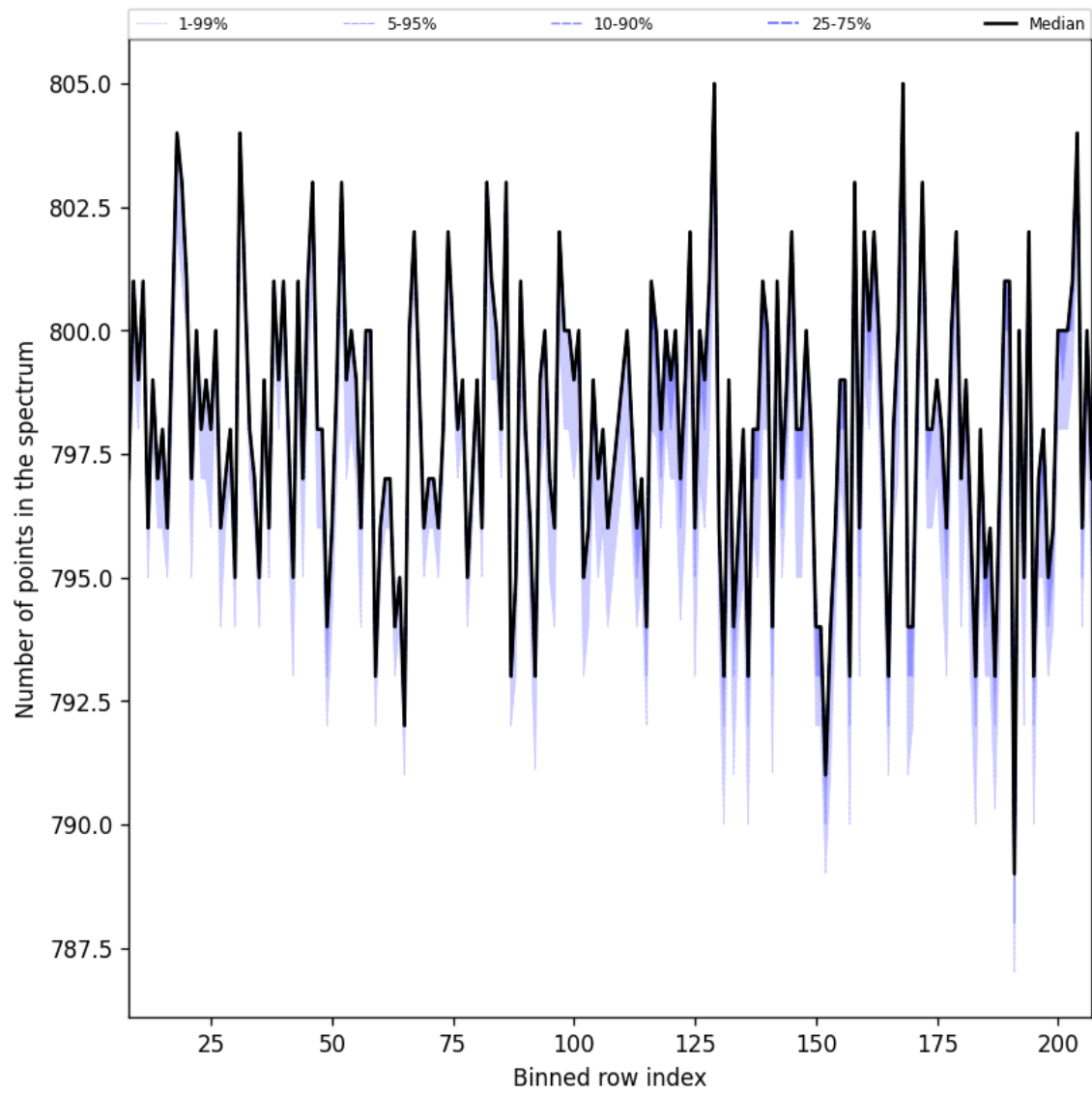
Figure 37: Along track statistics of “Number of points in the spectrum” for 2025-07-22 to 2025-07-24
