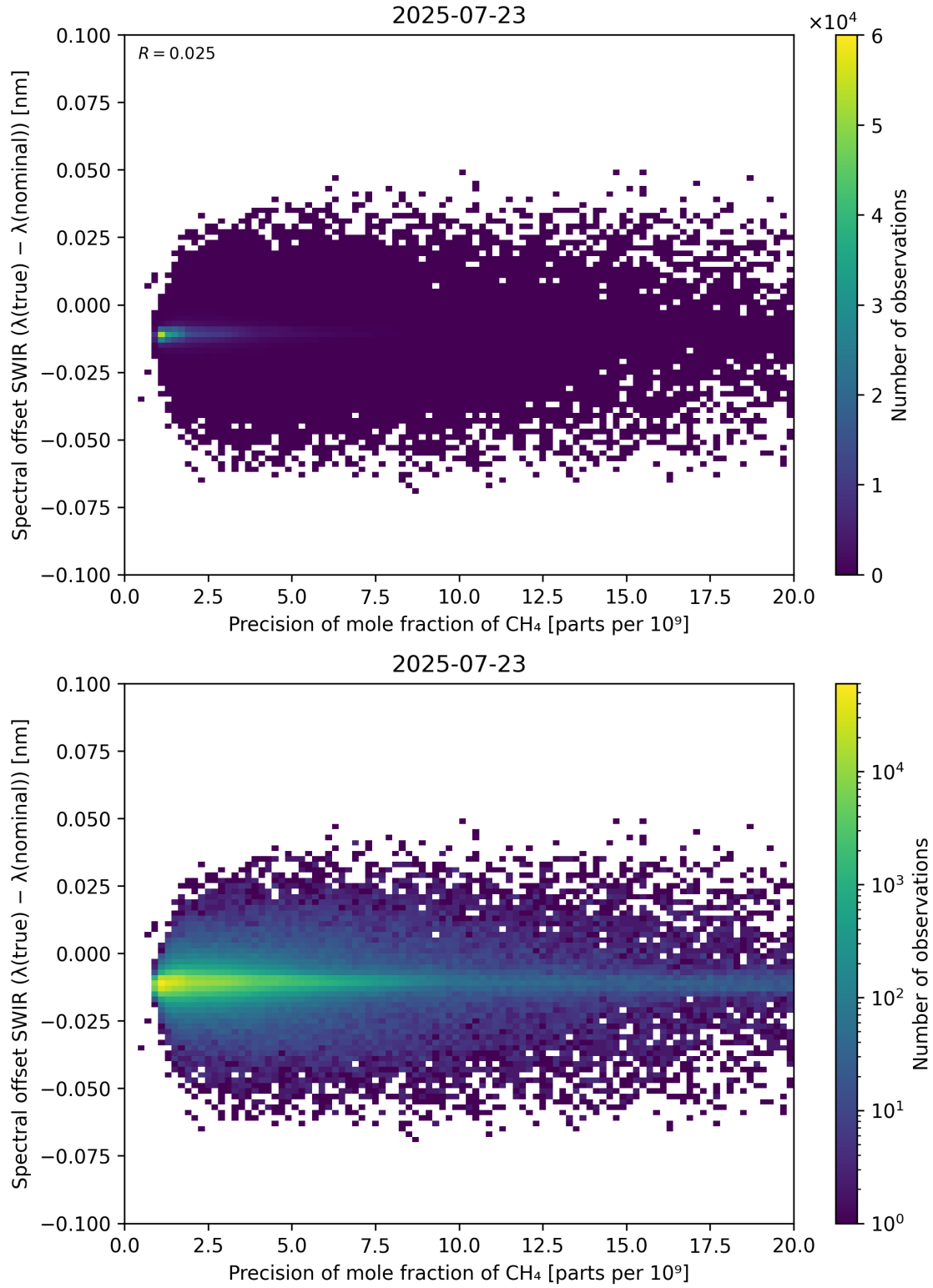
Figure 85: Scatter density plot of “Precision of mole fraction of CH 4 ” against “Spectral offset SWIR ( \lambda_{\text{true}} - \lambda_{\text{nominal}} )” for 2025-07-22 to 2025-07-24.
