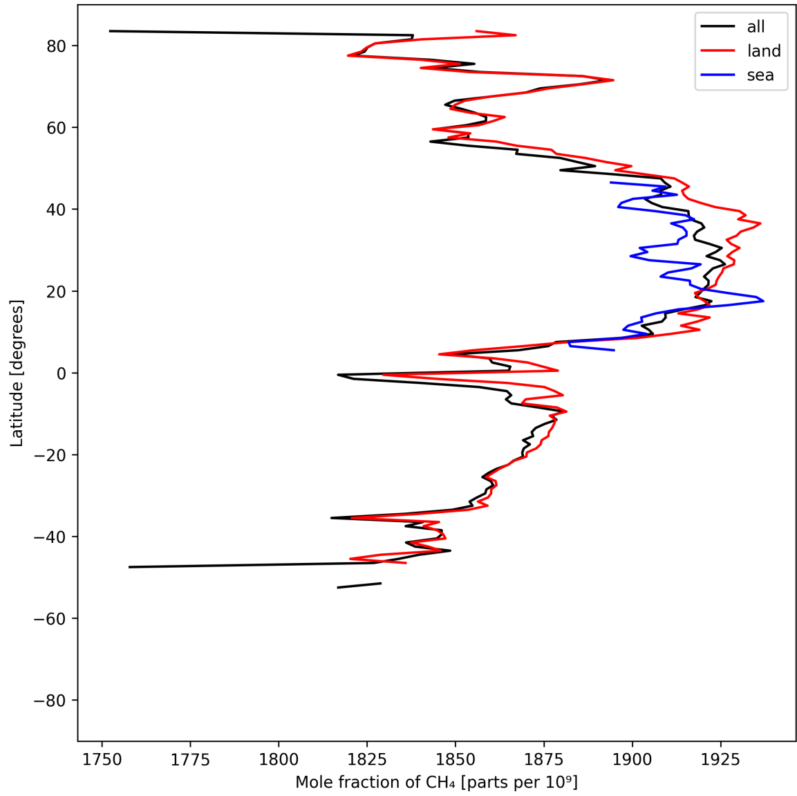
Figure 12: Zonal average of “Mole fraction of CH 4 ” for 2025-07-22 to 2025-07-24.
