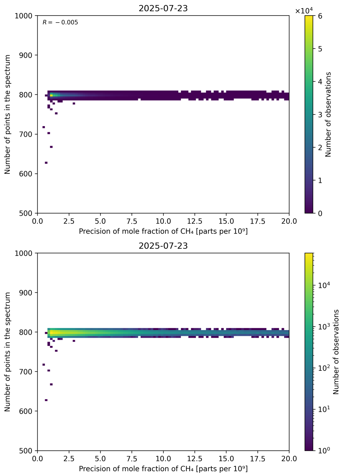
Figure 84: Scatter density plot of “Precision of mole fraction of CH 4 ” against “Number of points in the spectrum” for 2025-07-22 to 2025-07-24.
