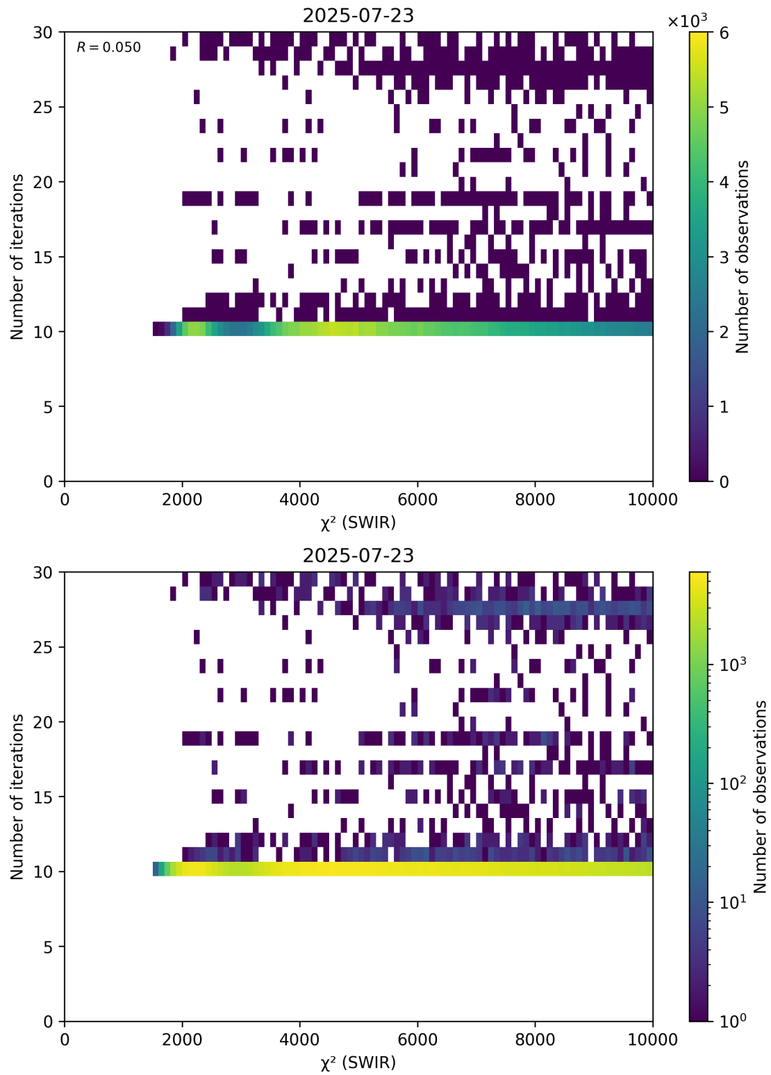
Figure 50: Scatter density plot of “ \chi^2 (SWIR)” against “Number of iterations” for 2025-07-22 to 2025-07-24.
