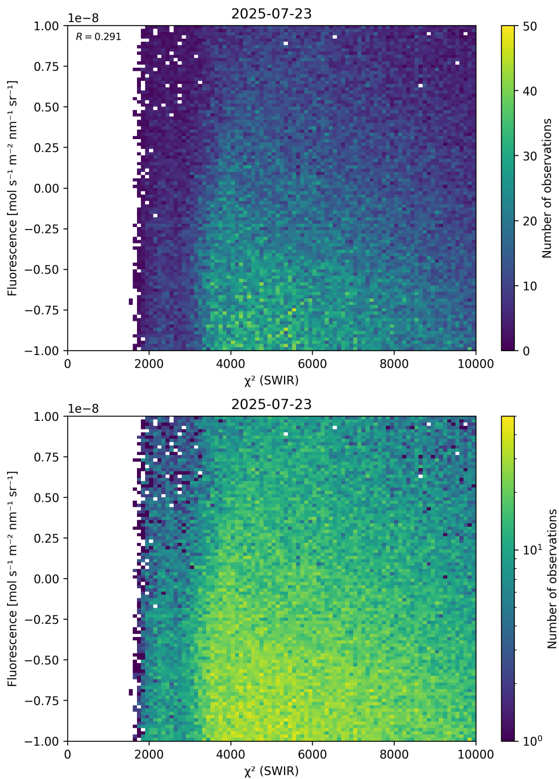
Figure 49: Scatter density plot of “ \chi^2 (SWIR)” against “Fluorescence” for 2025-07-22 to 2025-07-24.
