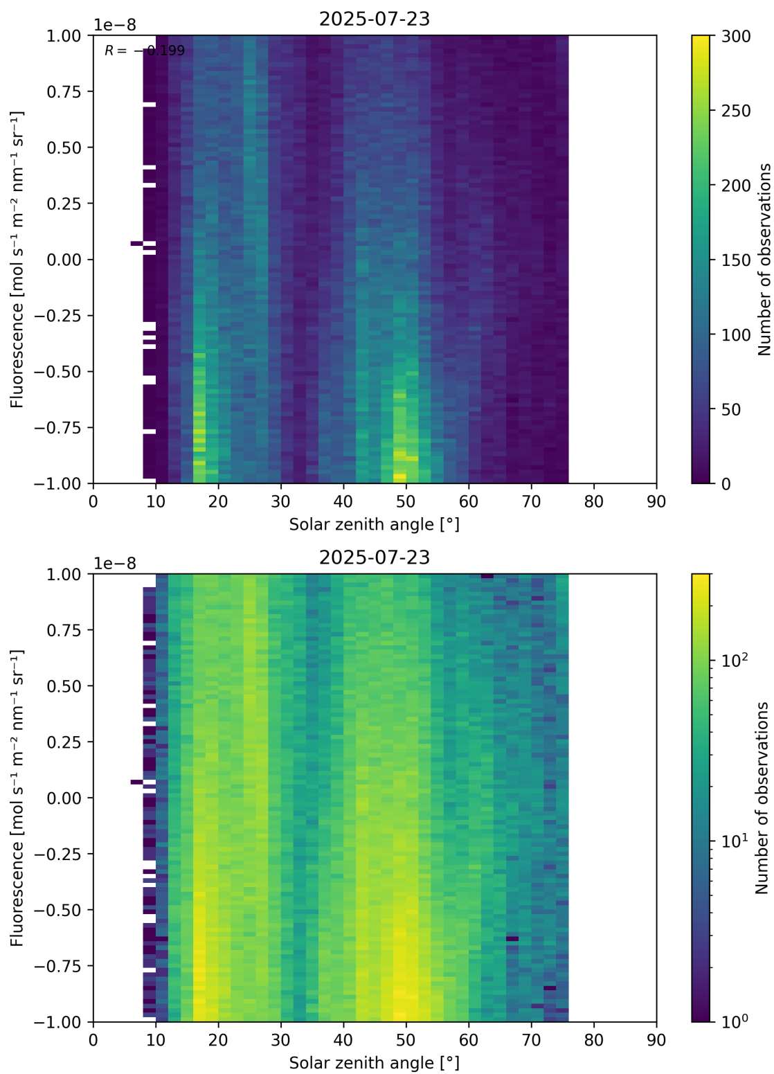
Figure 97: Scatter density plot of “Solar zenith angle” against “Fluorescence” for 2025-07-22 to 2025-07-24.
