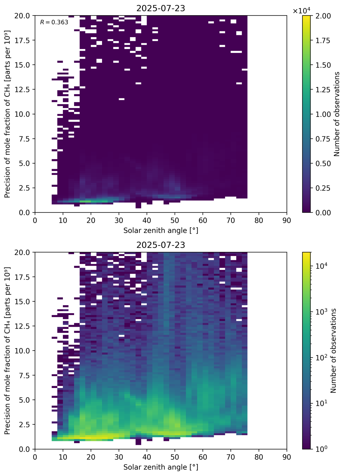
Figure 101: Scatter density plot of “Solar zenith angle” against “Precision of mole fraction of CH 4 ” for 2025-07-22 to 2025-07-24.
