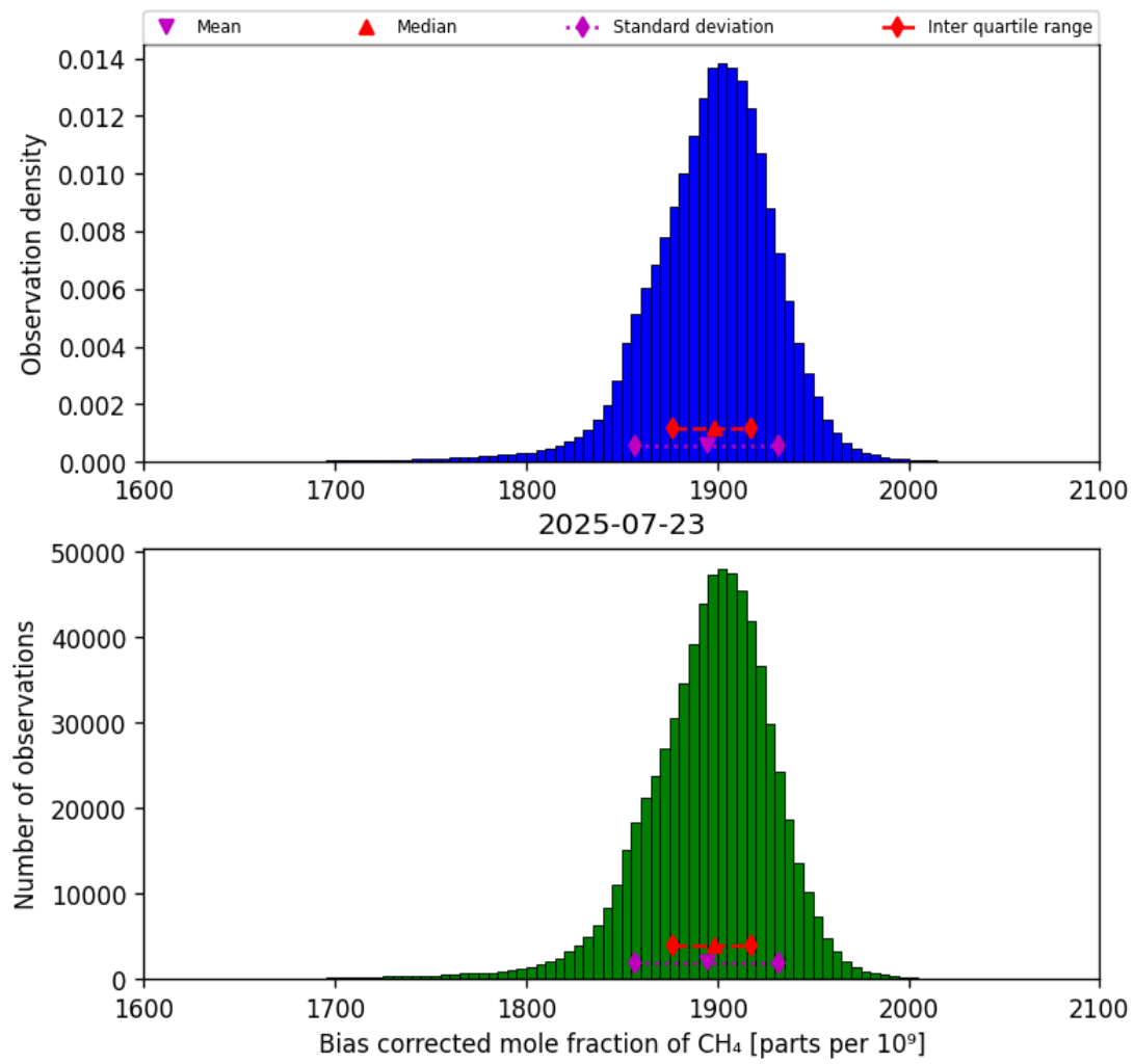
Figure 25: Histogram of “Bias corrected mole fraction of CH 4 ” for 2025-07-22 to 2025-07-24
