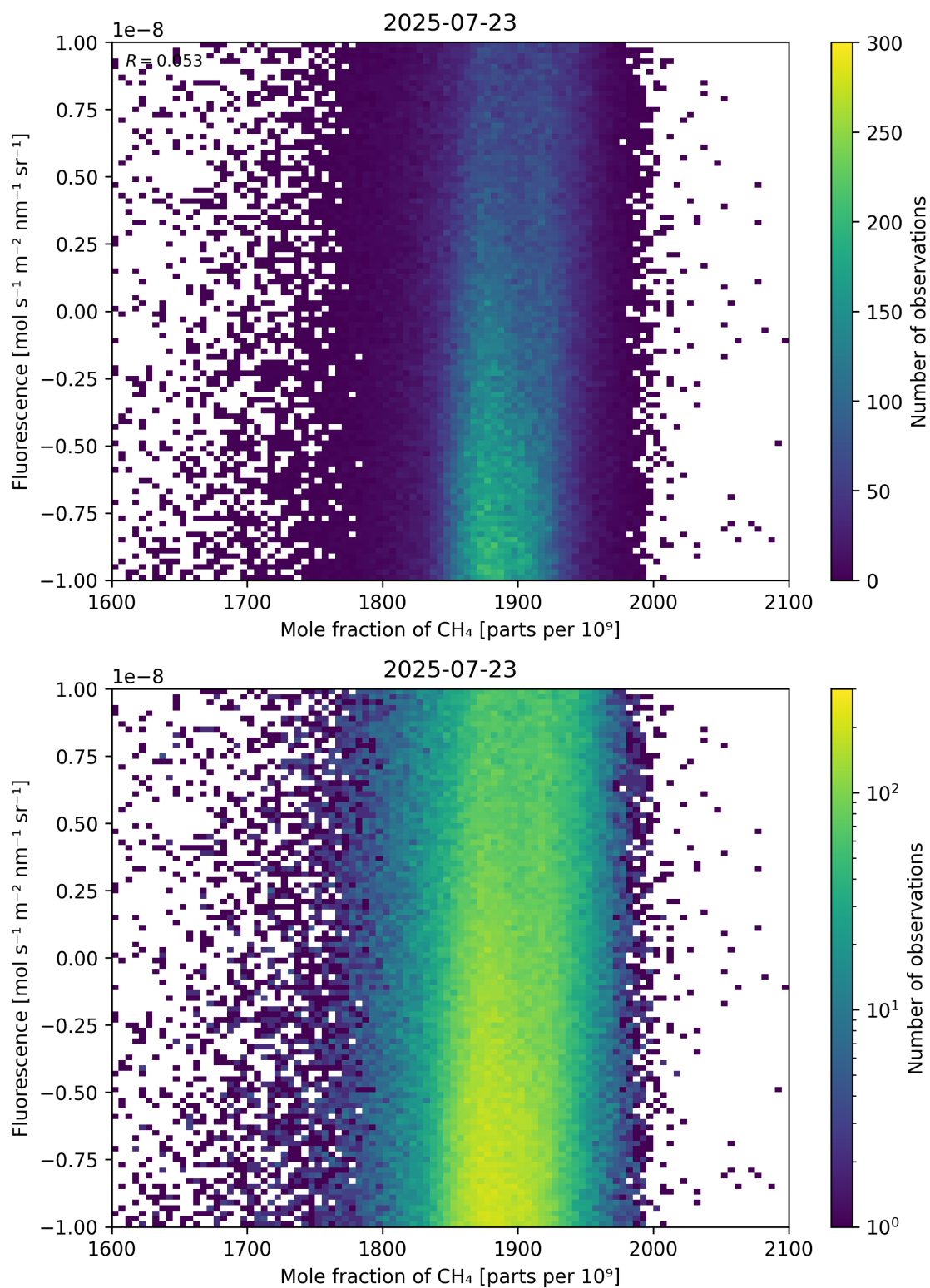
Figure 73: Scatter density plot of “Mole fraction of \text{CH}_4 ” against “Fluorescence” for 2025-07-22 to 2025-07-24.
