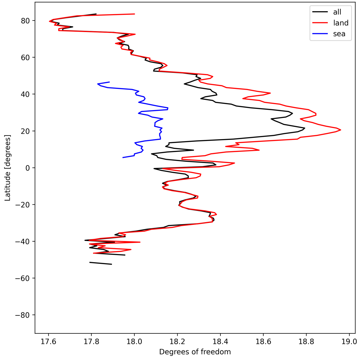
Figure 19: Zonal average of “Degrees of freedom” for 2025-07-22 to 2025-07-24.
