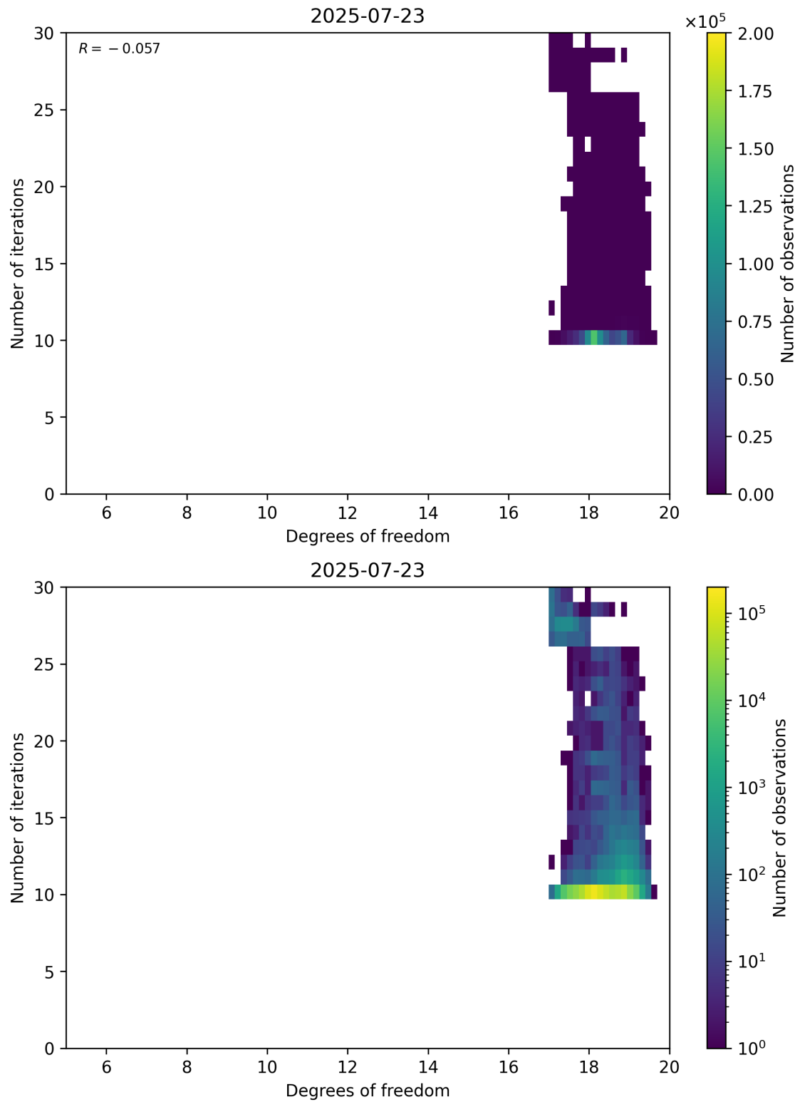
Figure 52: Scatter density plot of “Degrees of freedom” against “Number of iterations” for 2025-07-22 to 2025-07-24.
