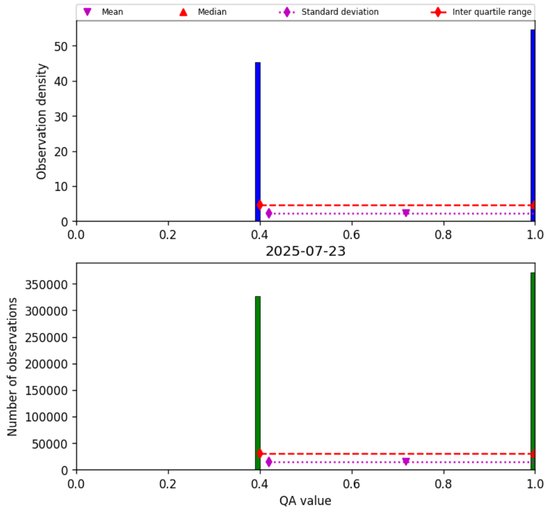
Figure 22: Histogram of “QA value” for 2025-07-22 to 2025-07-24
