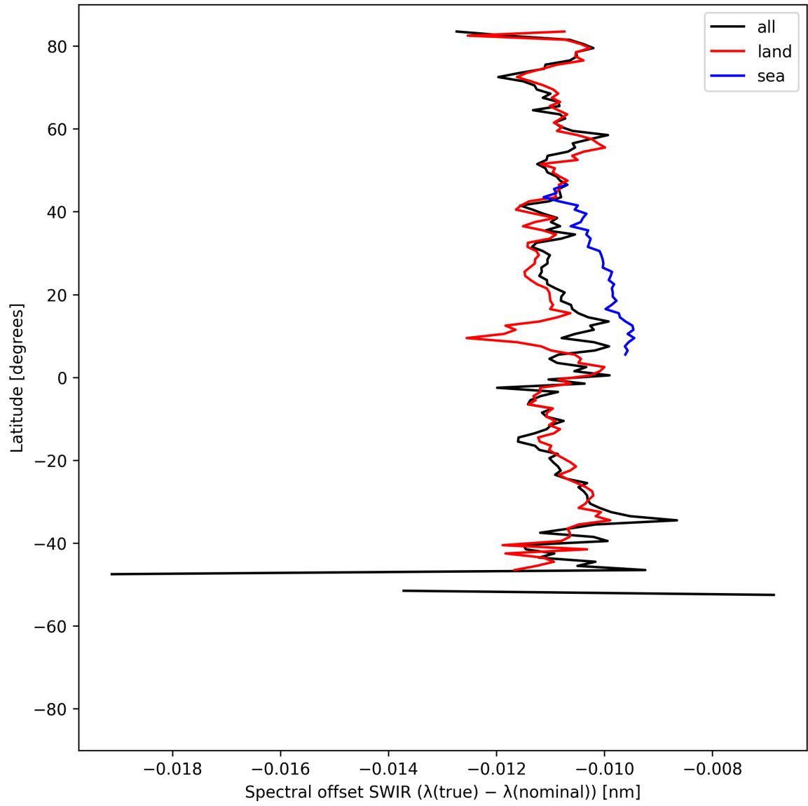
Figure 16: Zonal average of “Spectral offset SWIR ( \lambda_{\text{true}} - \lambda_{\text{nominal}} )” for 2025-07-22 to 2025-07-24.
