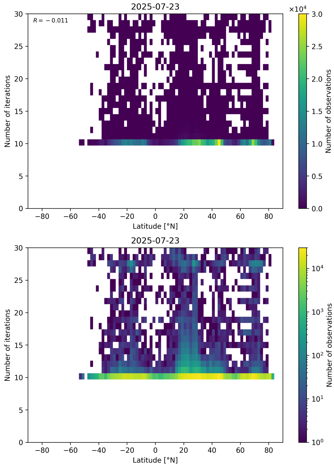
Figure 60: Scatter density plot of “Latitude” against “Number of iterations” for 2025-07-22 to 2025-07-24.
