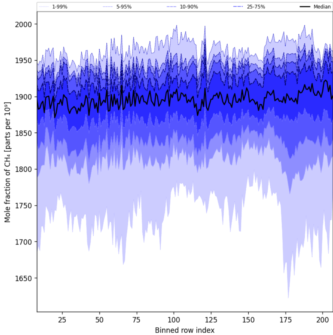
Figure 34: Along track statistics of “Mole fraction of CH 4 ” for 2025-07-22 to 2025-07-24
