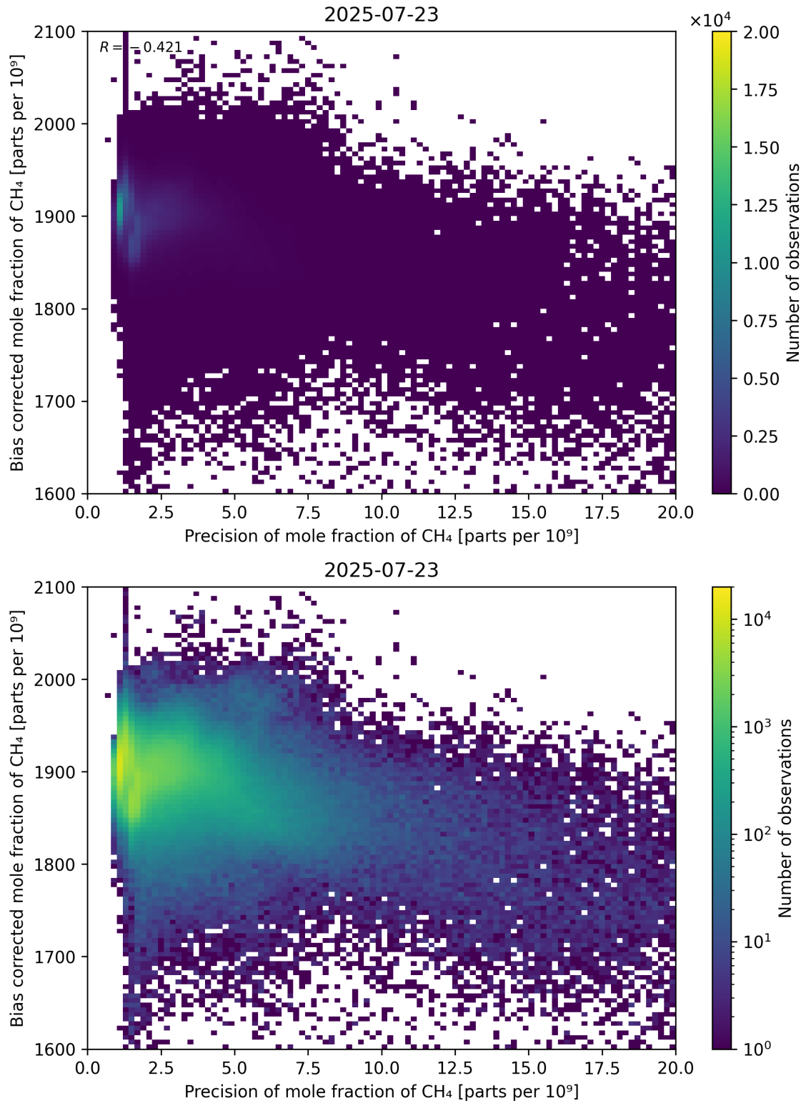
Figure 82: Scatter density plot of “Precision of mole fraction of CH 4 ” against “Bias corrected mole fraction of CH 4 ” for 2025-07-22 to 2025-07-24.
