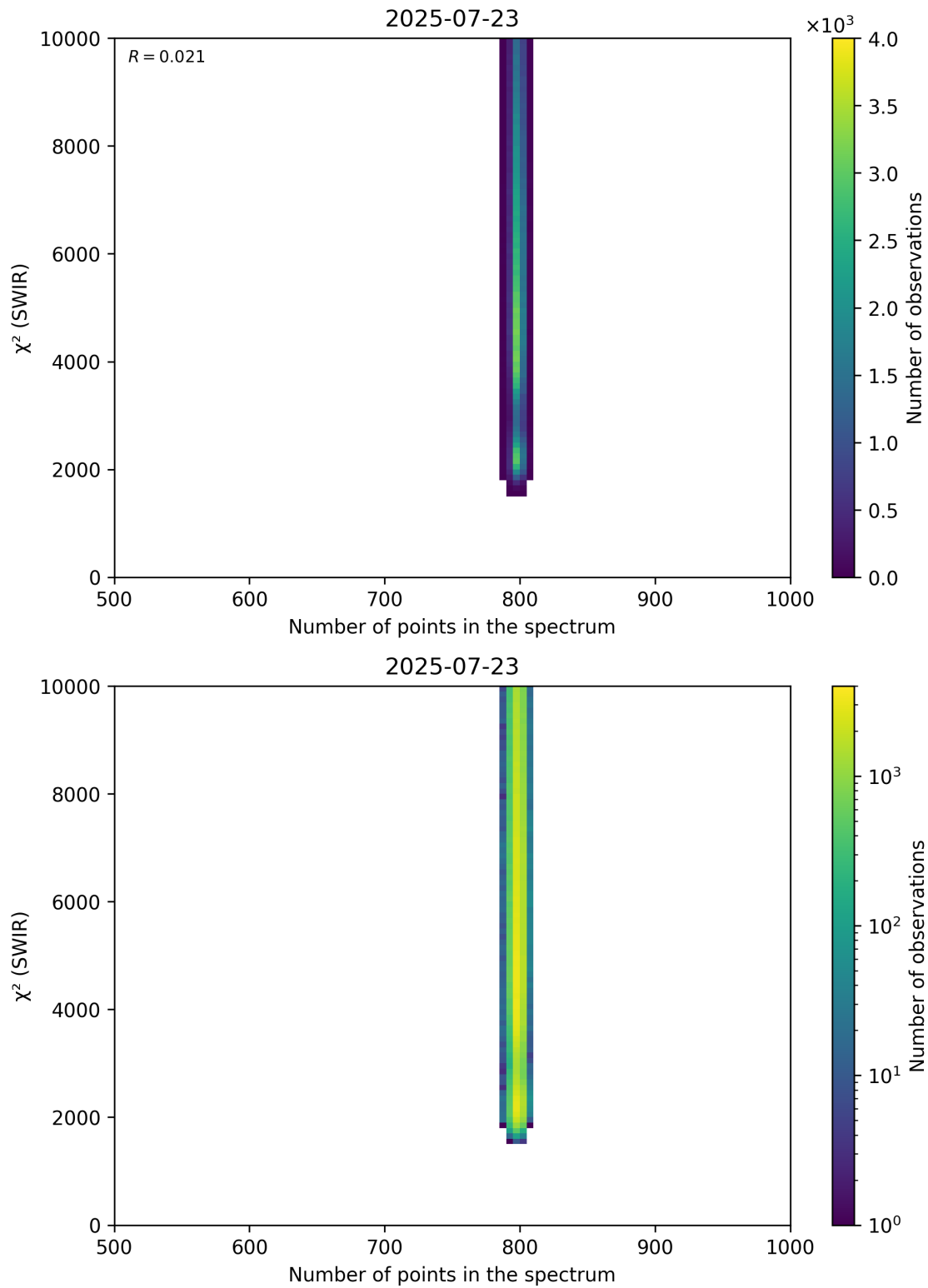
Figure 89: Scatter density plot of “Number of points in the spectrum” against “ \chi^2 (SWIR)” for 2025-07-22 to 2025-07-24.
