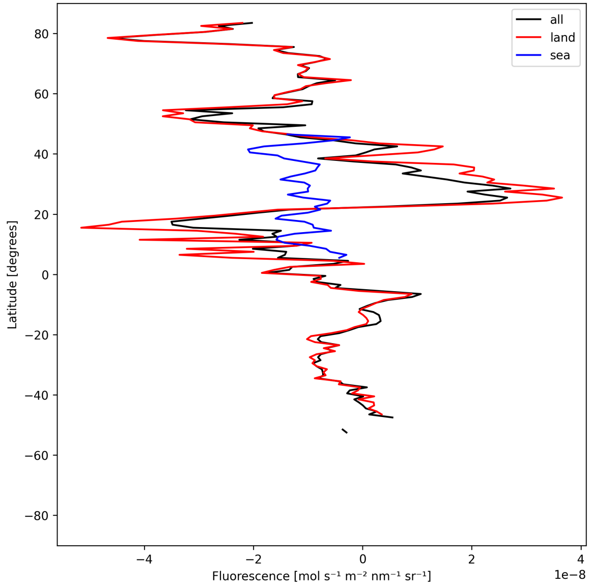
Figure 21: Zonal average of “Fluorescence” for 2025-07-22 to 2025-07-24.
