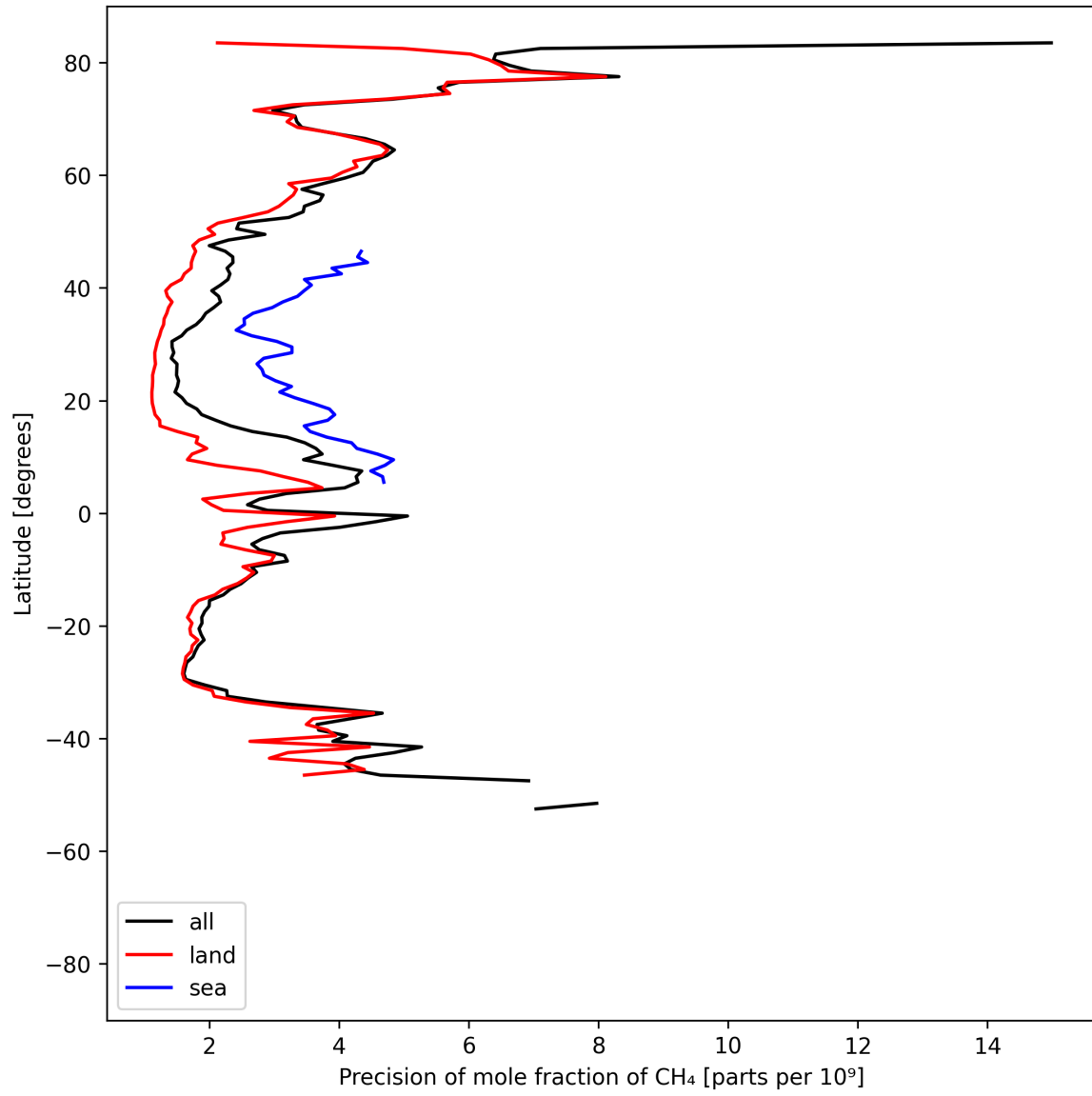
Figure 13: Zonal average of “Precision of mole fraction of CH 4 ” for 2025-07-22 to 2025-07-24.
