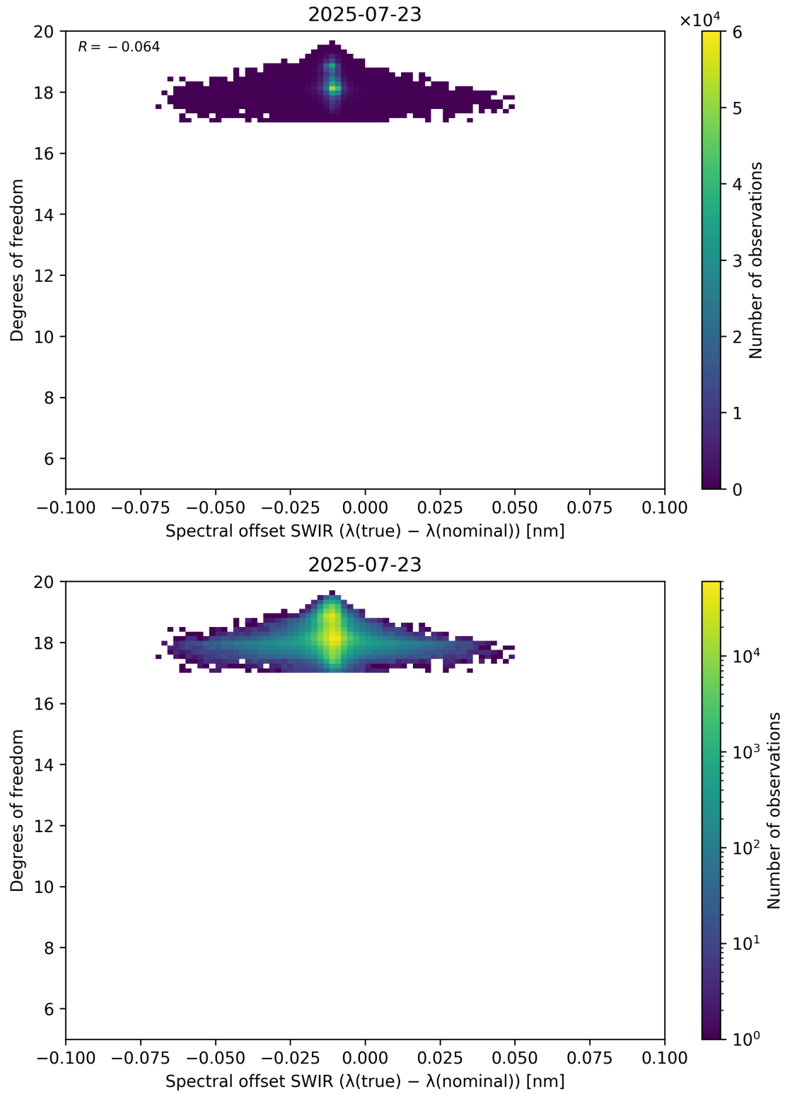
Figure 119: Scatter density plot of “Spectral offset SWIR ( \lambda_{\text{true}} - \lambda_{\text{nominal}} )” against “Degrees of freedom” for 2025-07-22 to 2025-07-24.
