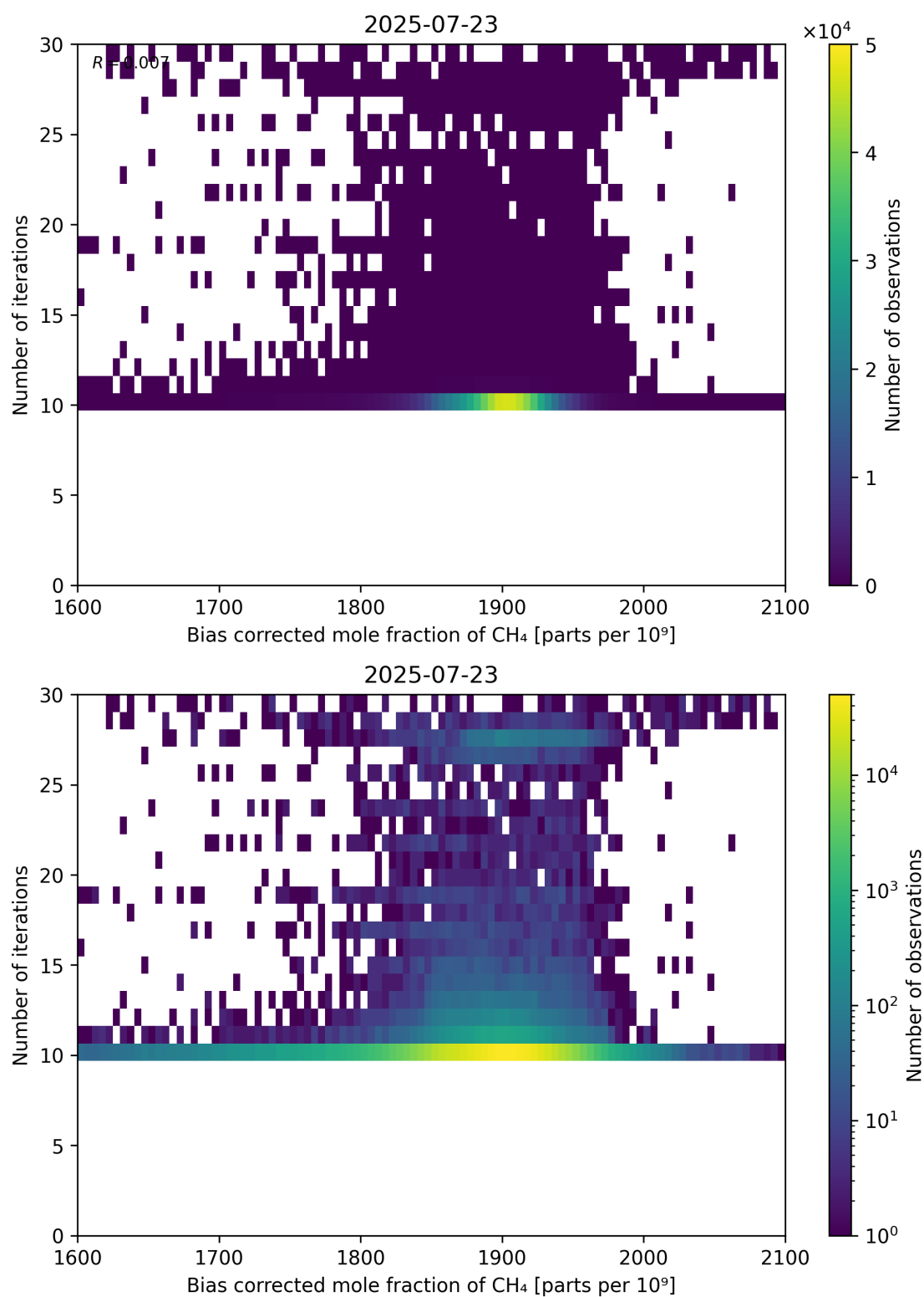
Figure 67: Scatter density plot of “Bias corrected mole fraction of \text{CH}_4 ” against “Number of iterations” for 2025-07-22 to 2025-07-24.
