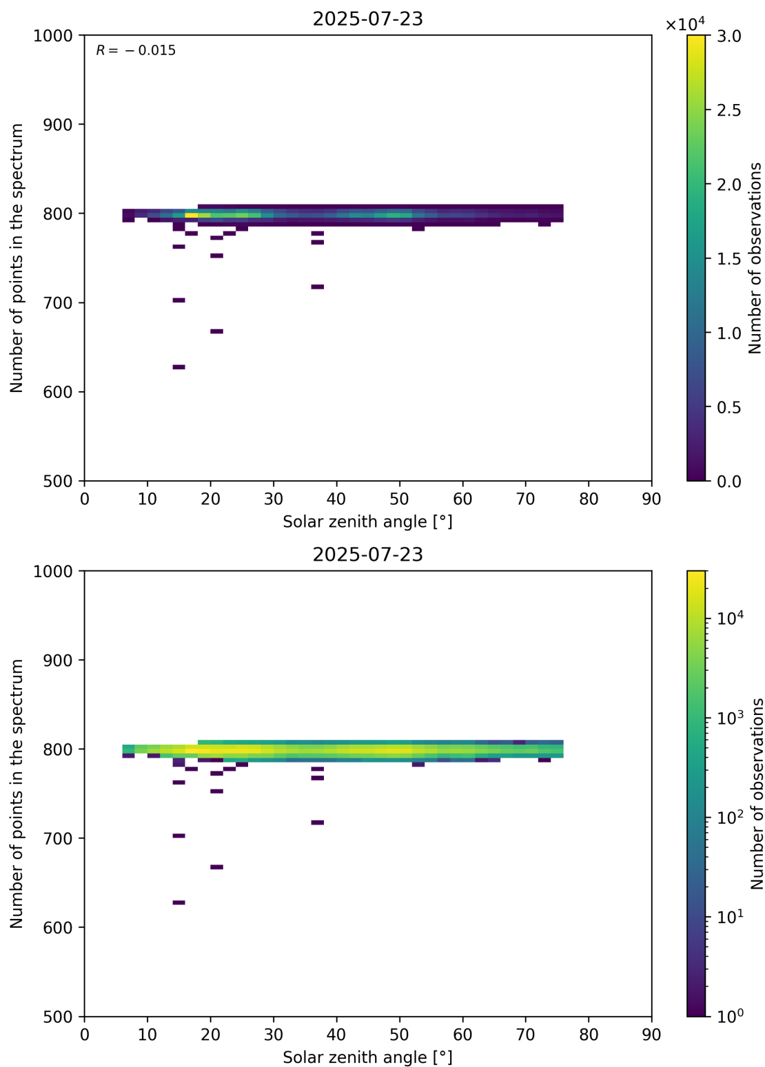
Figure 103: Scatter density plot of “Solar zenith angle” against “Number of points in the spectrum” for 2025-07-22 to 2025-07-24.
