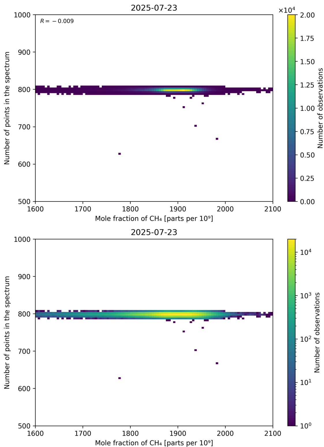
Figure 77: Scatter density plot of “Mole fraction of CH 4 ” against “Number of points in the spectrum” for 2025-07-22 to 2025-07-24.
