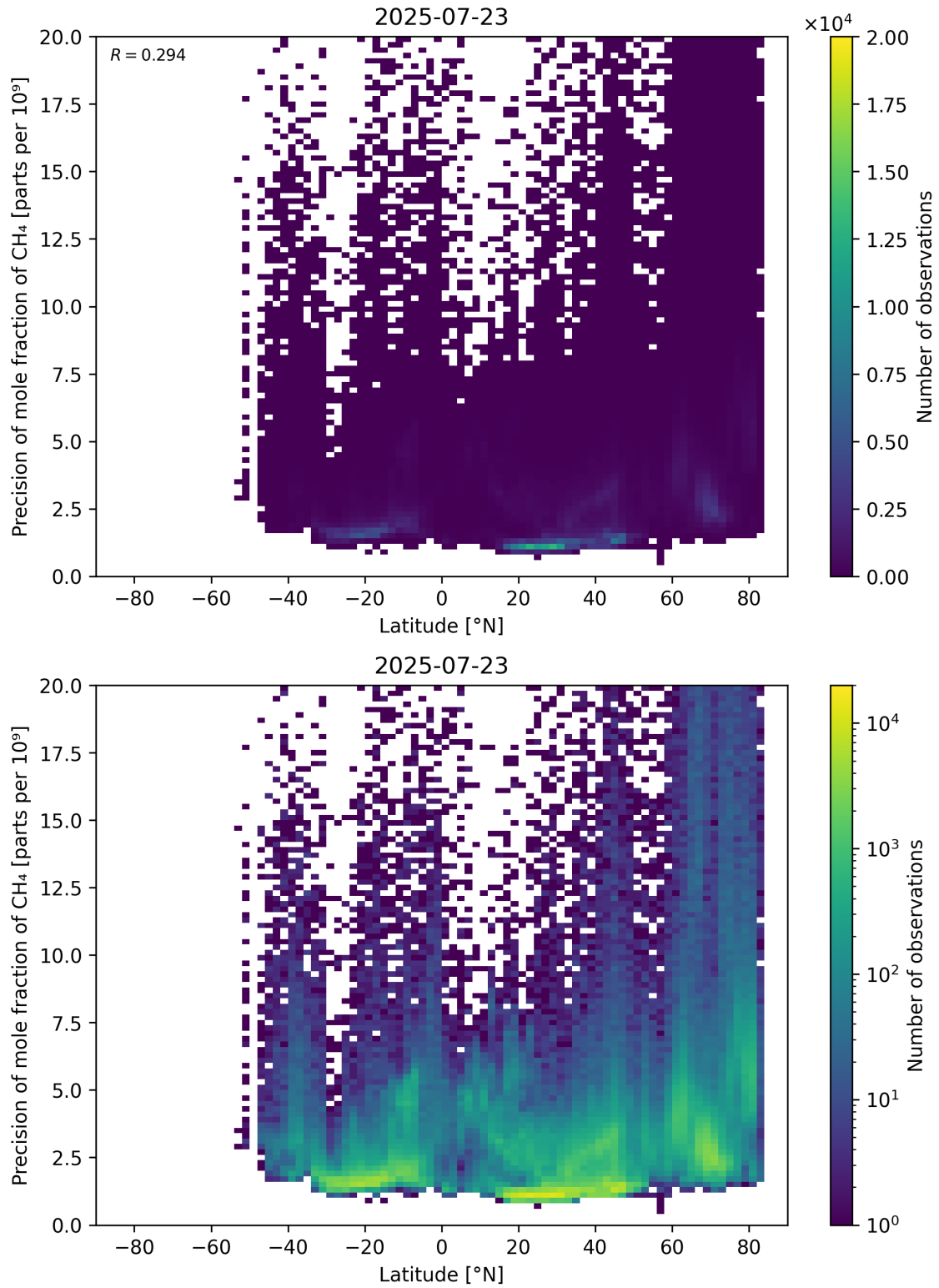
Figure 59: Scatter density plot of “Latitude” against “Precision of mole fraction of \text{CH}_4 ” for 2025-07-22 to 2025-07-24.
