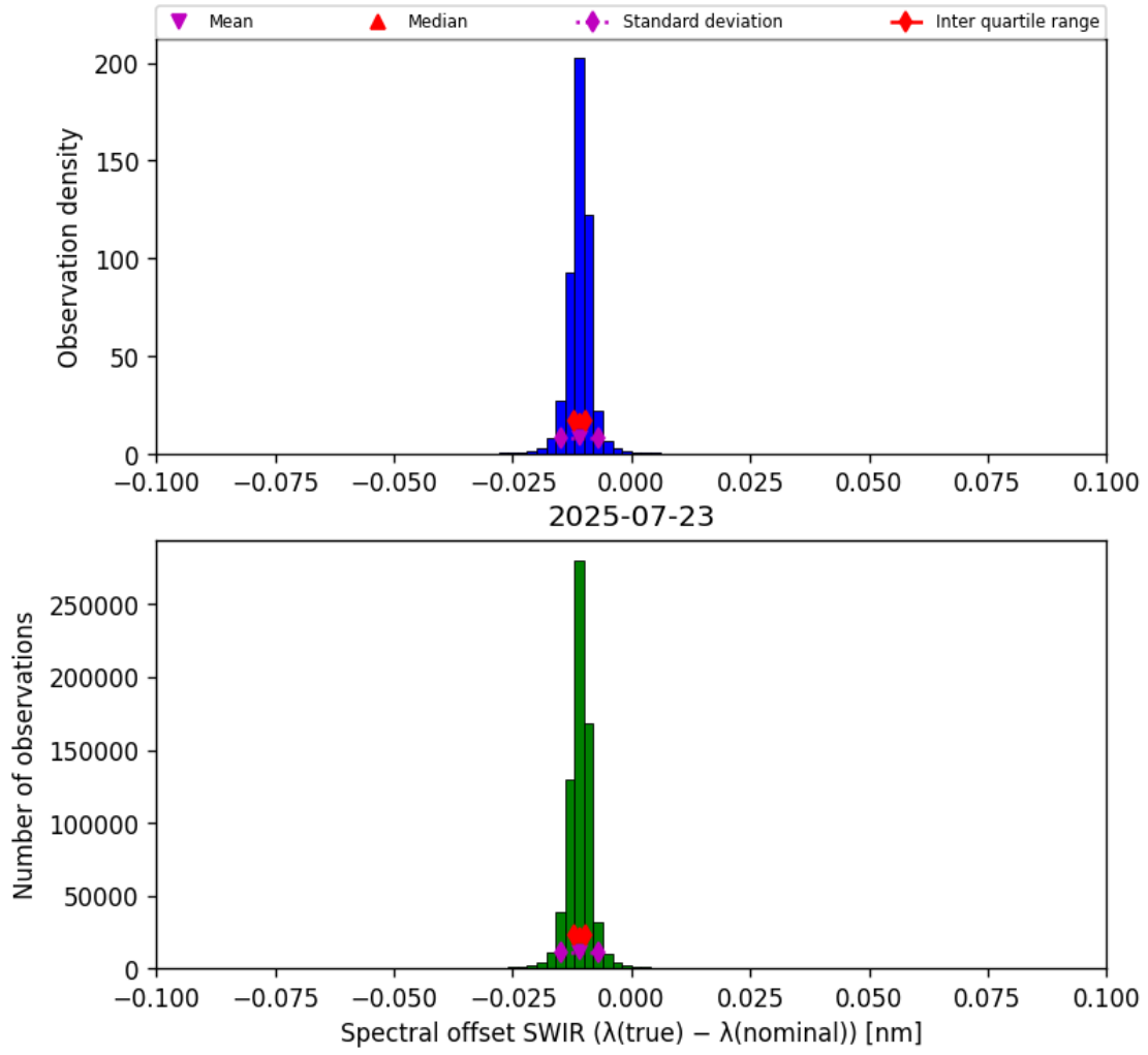
Figure 27: Histogram of “Spectral offset SWIR ( \lambda_{\text{true}} - \lambda_{\text{nominal}} )” for 2025-07-22 to 2025-07-24
