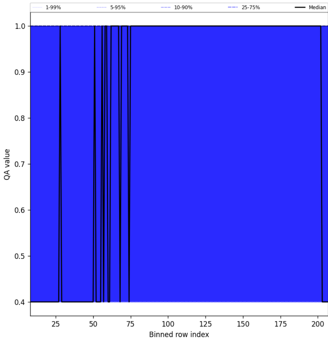
Figure 33: Along track statistics of “QA value” for 2025-07-22 to 2025-07-24
