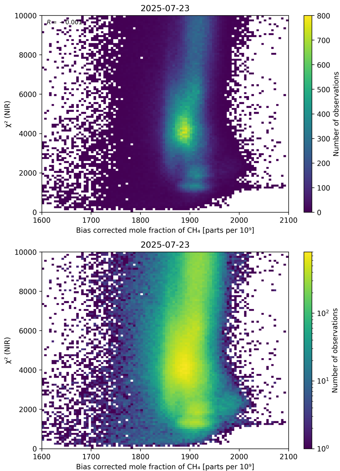
Figure 63: Scatter density plot of “Bias corrected mole fraction of \text{CH}_4 ” against “ \chi^2 (NIR)” for 2025-07-22 to 2025-07-24.
