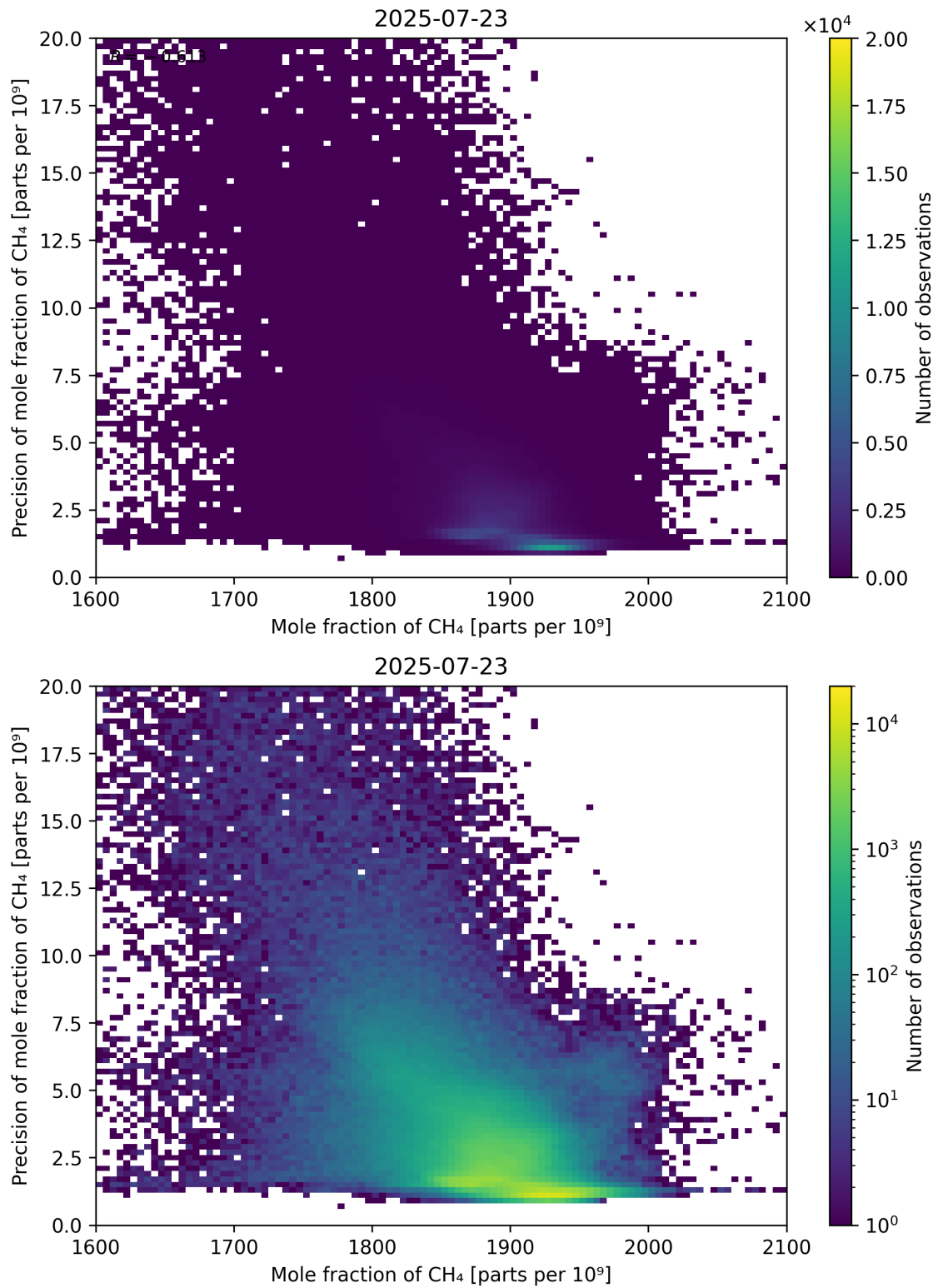
Figure 75: Scatter density plot of “Mole fraction of CH 4 ” against “Precision of mole fraction of CH 4 ” for 2025-07-22 to 2025-07-24.
