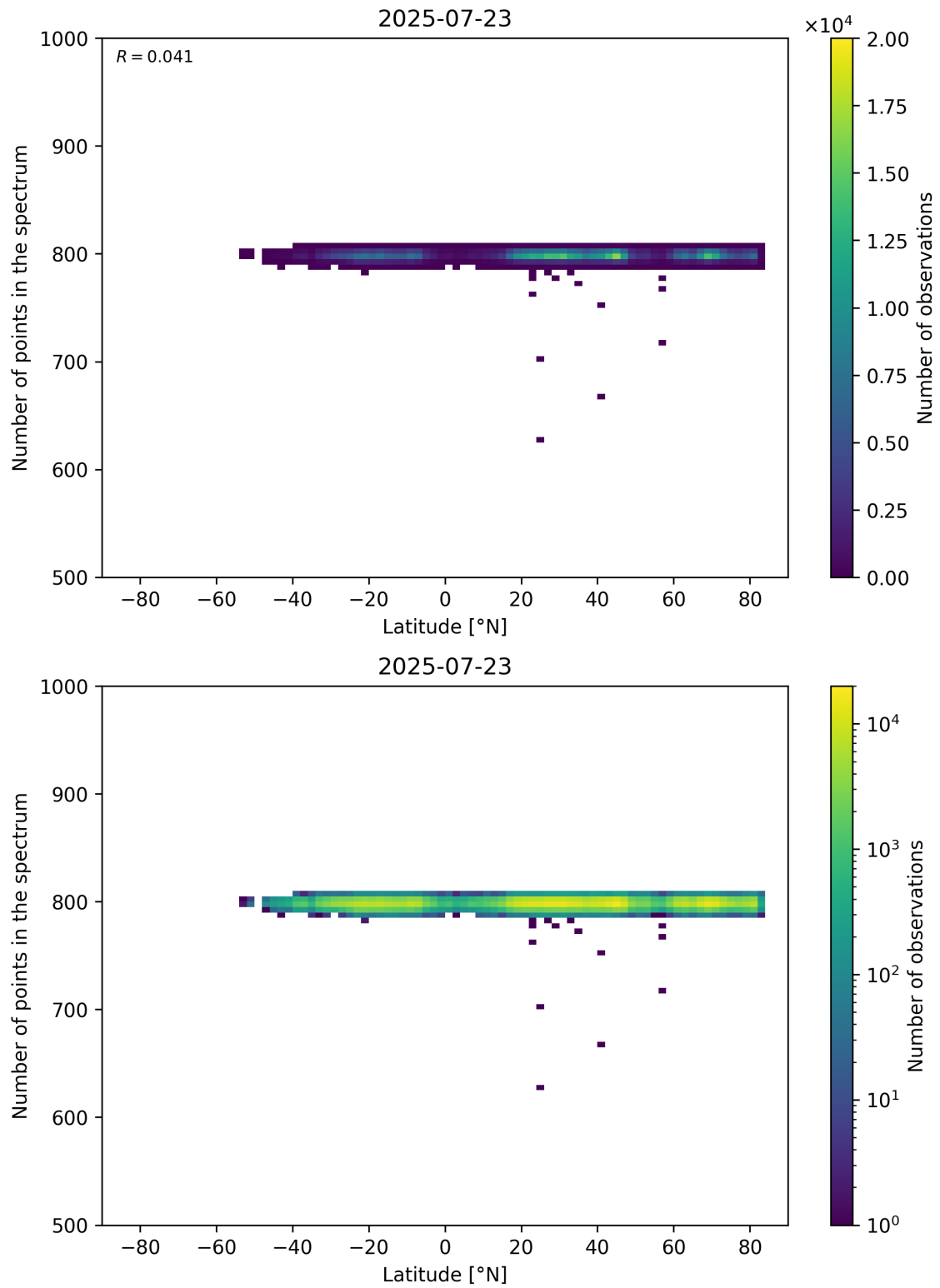
Figure 61: Scatter density plot of “Latitude” against “Number of points in the spectrum” for 2025-07-22 to 2025-07-24.
