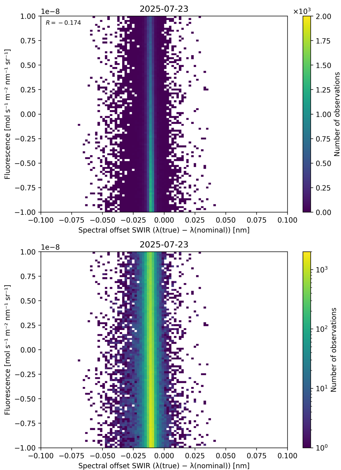
Figure 120: Scatter density plot of “Spectral offset SWIR ( \lambda_{\text{true}} - \lambda_{\text{nominal}} )” against “Fluorescence” for 2025-07-22 to 2025-07-24.
