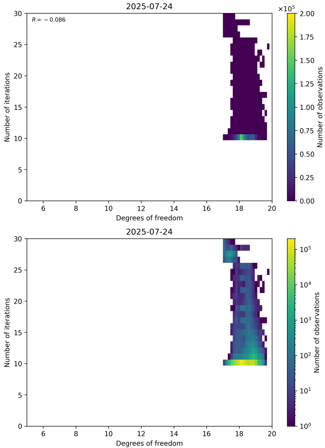
Figure 52: Scatter density plot of “Degrees of freedom” against “Number of iterations” for 2025-07-24 to 2025-07-25.
