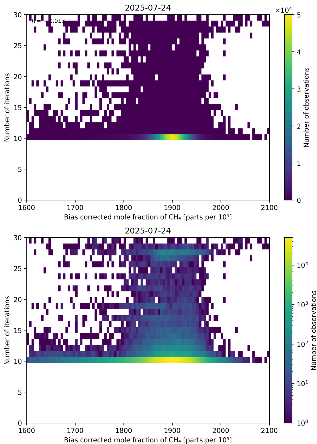
Figure 67: Scatter density plot of “Bias corrected mole fraction of \text{CH}_4 ” against “Number of iterations” for 2025-07-24 to 2025-07-25.
