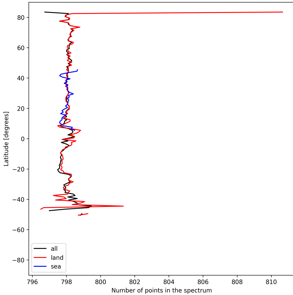
Figure 15: Zonal average of “Number of points in the spectrum” for 2025-07-24 to 2025-07-25.
