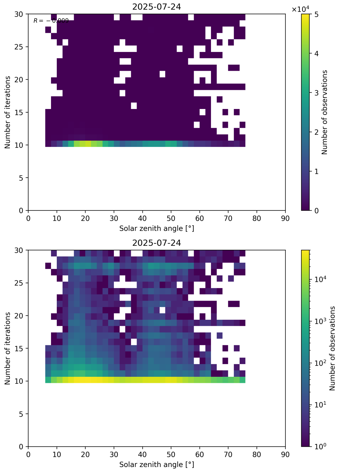
Figure 102: Scatter density plot of “Solar zenith angle” against “Number of iterations” for 2025-07-24 to 2025-07-25.
