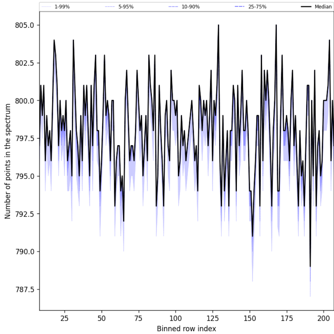
Figure 37: Along track statistics of “Number of points in the spectrum” for 2025-07-24 to 2025-07-25
