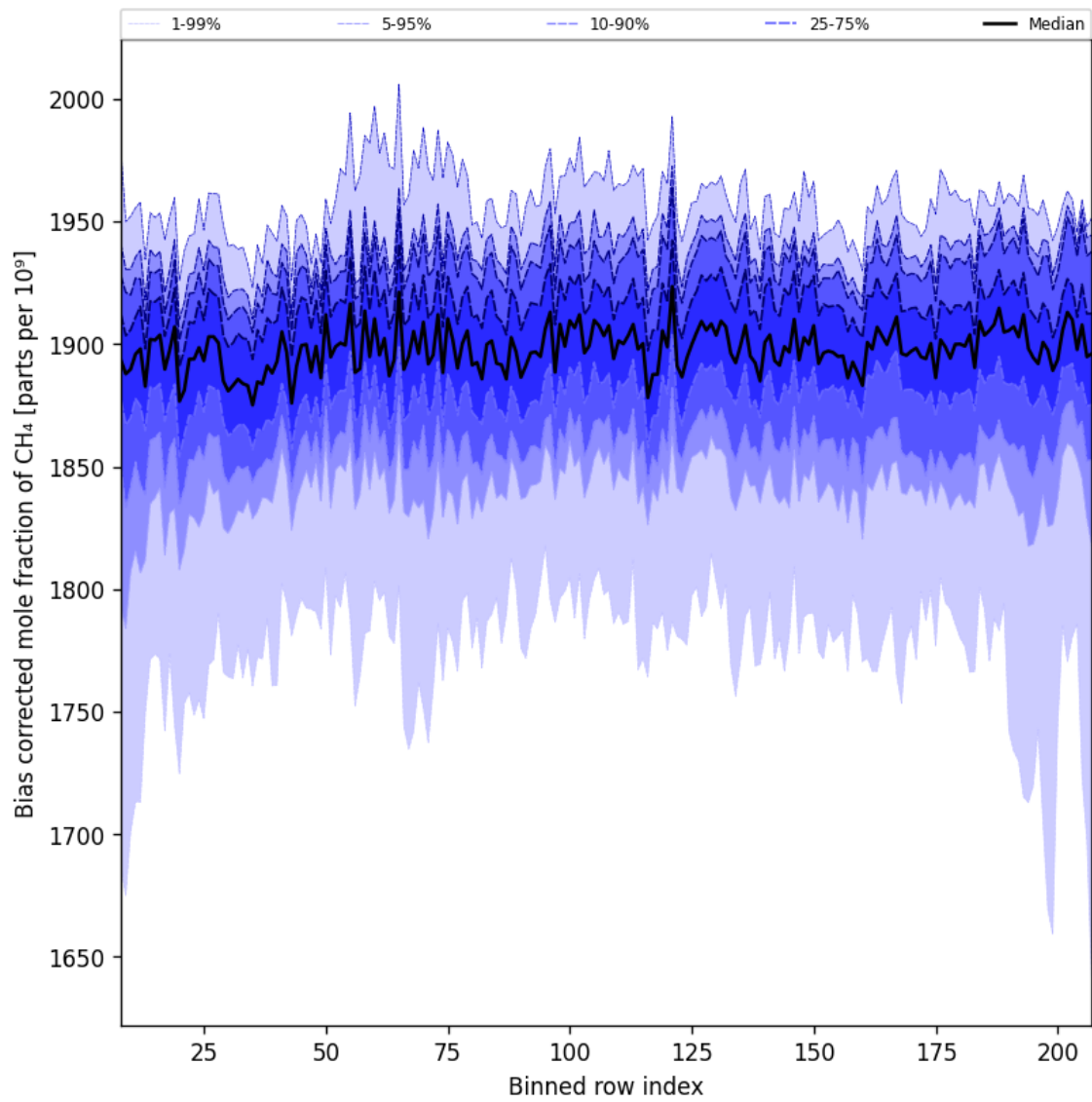
Figure 36: Along track statistics of “Bias corrected mole fraction of CH 4 ” for 2025-07-24 to 2025-07-25
