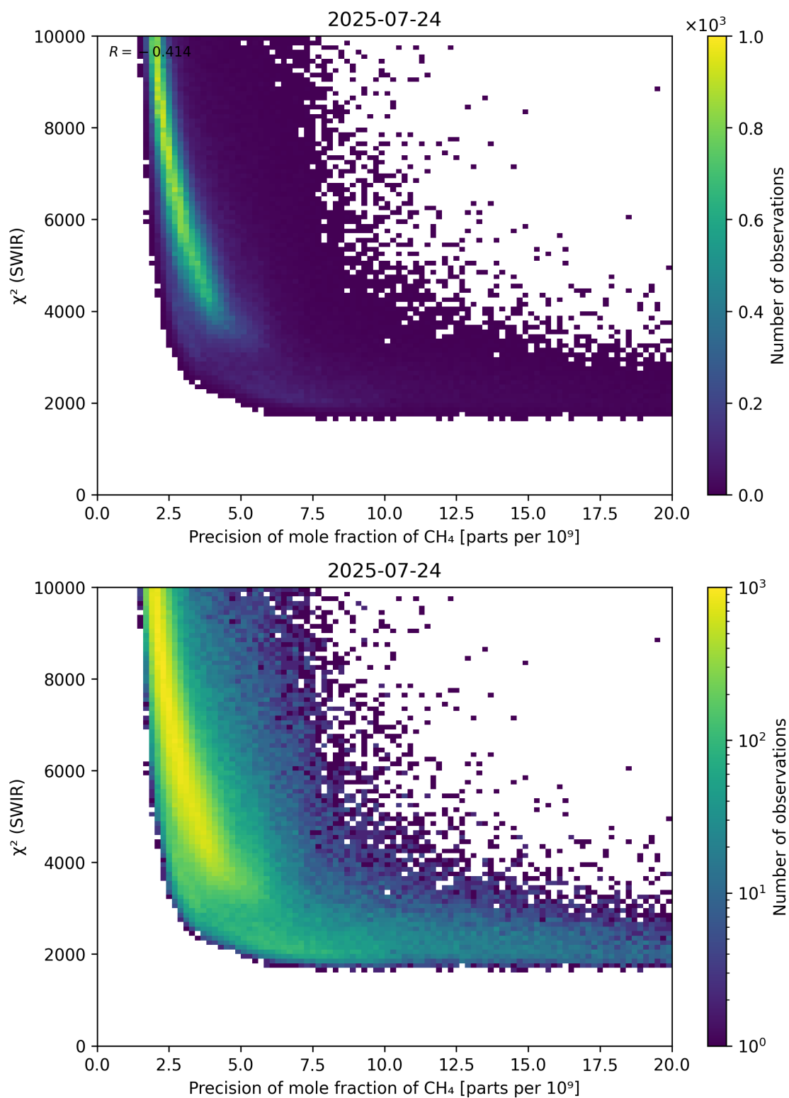
Figure 79: Scatter density plot of “Precision of mole fraction of \text{CH}_4 ” against “ \chi^2 (SWIR)” for 2025-07-24 to 2025-07-25.
