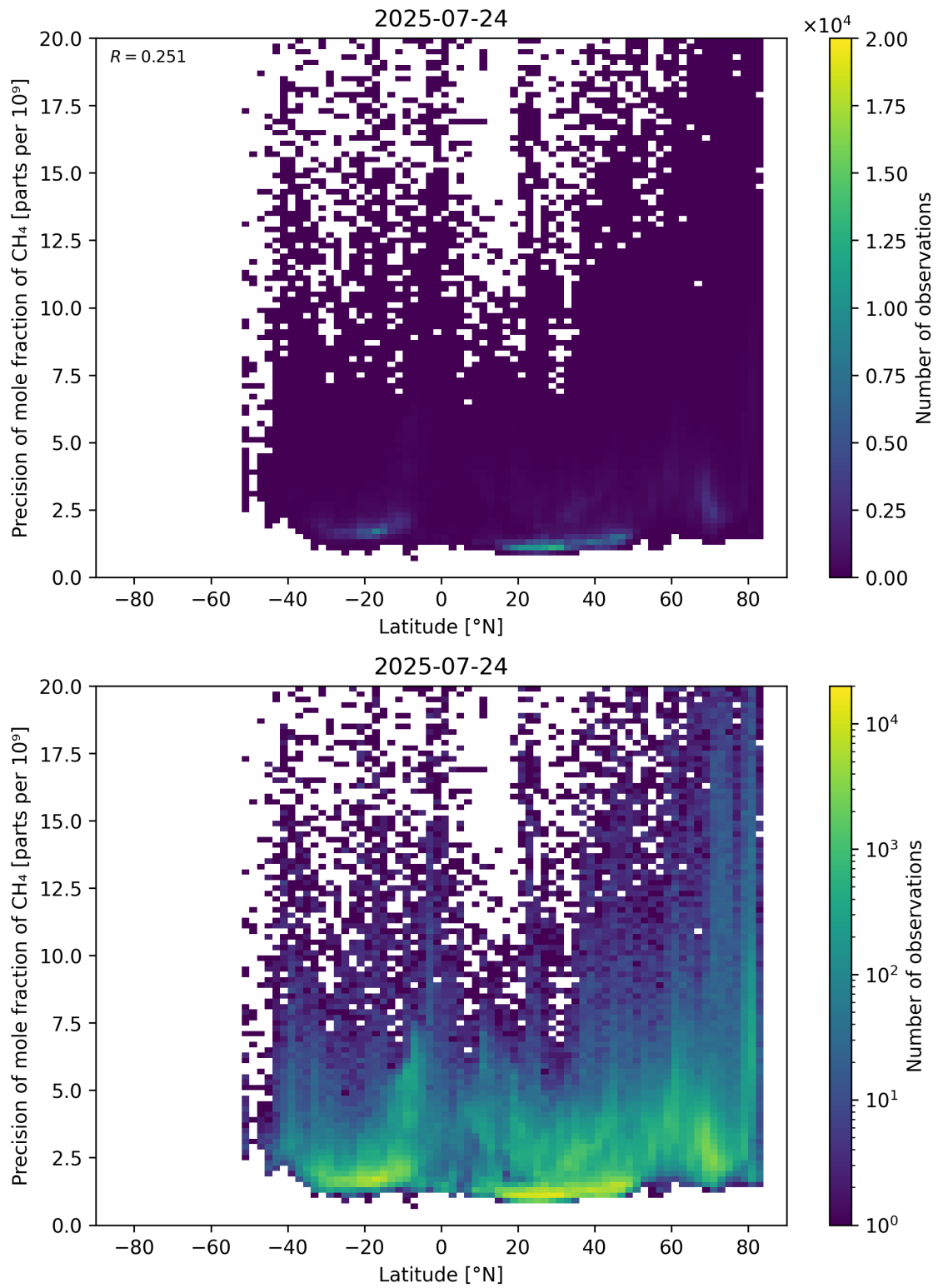
Figure 59: Scatter density plot of “Latitude” against “Precision of mole fraction of \text{CH}_4 ” for 2025-07-24 to 2025-07-25.
