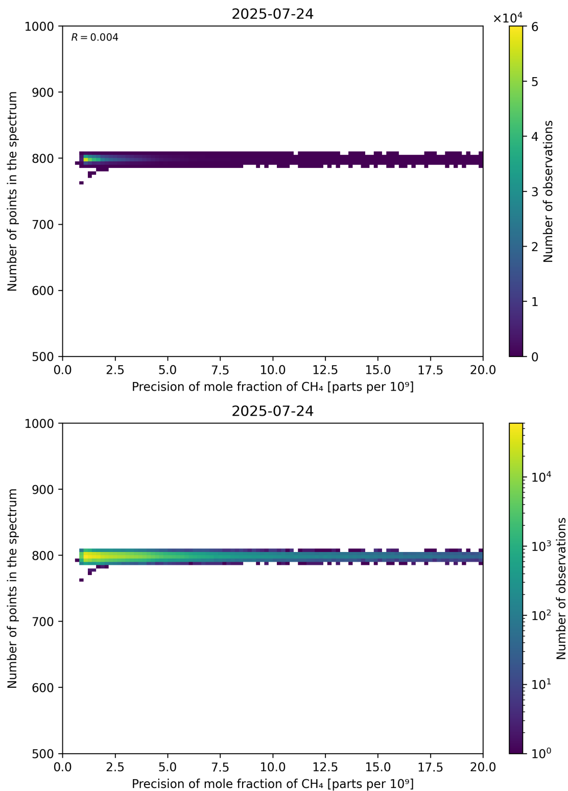
Figure 84: Scatter density plot of “Precision of mole fraction of CH 4 ” against “Number of points in the spectrum” for 2025-07-24 to 2025-07-25.
