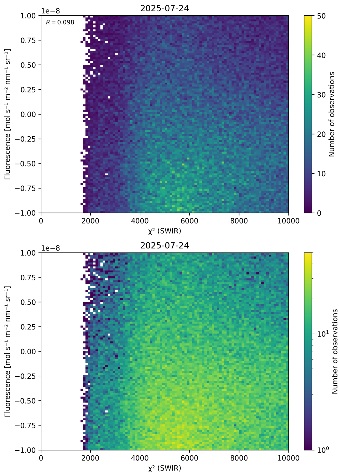
Figure 49: Scatter density plot of “ \chi^2 (SWIR)” against “Fluorescence” for 2025-07-24 to 2025-07-25.
