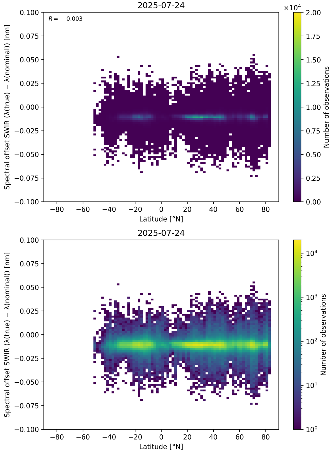
Figure 62: Scatter density plot of “Latitude” against “Spectral offset SWIR ( \lambda_{\text{true}} - \lambda_{\text{nominal}} )” for 2025-07-24 to 2025-07-25.
