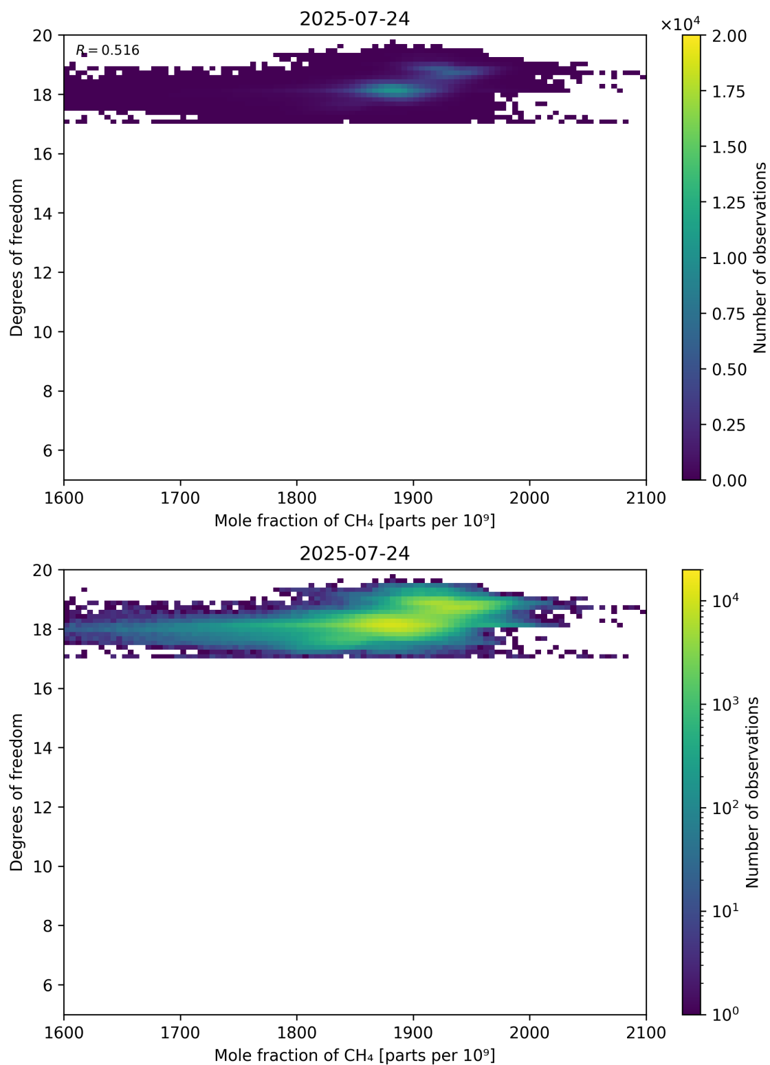
Figure 72: Scatter density plot of “Mole fraction of CH 4 ” against “Degrees of freedom” for 2025-07-24 to 2025-07-25.
