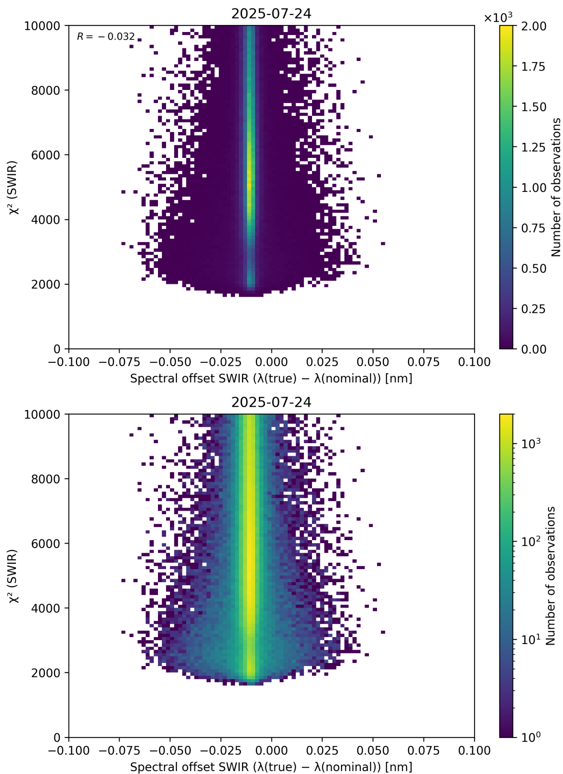
Figure 118: Scatter density plot of “Spectral offset SWIR ( \lambda_{\text{true}} - \lambda_{\text{nominal}} )” against “ \chi^2 (SWIR)” for 2025-07-24 to 2025-07-25.
