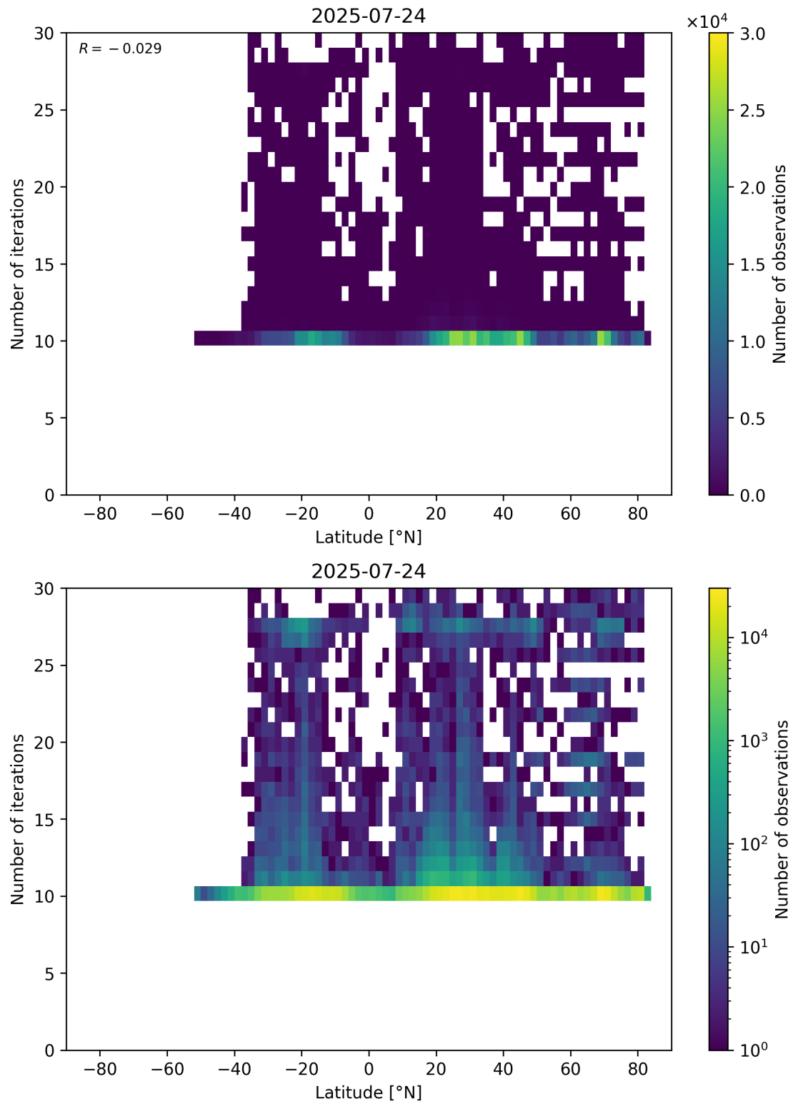
Figure 60: Scatter density plot of “Latitude” against “Number of iterations” for 2025-07-24 to 2025-07-25.
