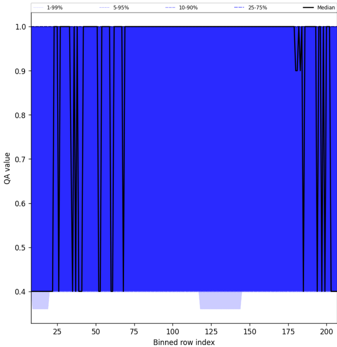
Figure 33: Along track statistics of “QA value” for 2025-07-24 to 2025-07-25
