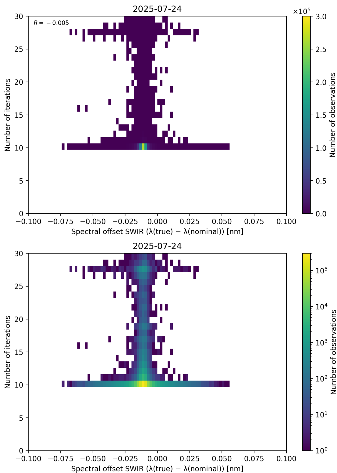
Figure 121: Scatter density plot of “Spectral offset SWIR ( \lambda_{\text{true}} - \lambda_{\text{nominal}} )” against “Number of iterations” for 2025-07-24 to 2025-07-25.
