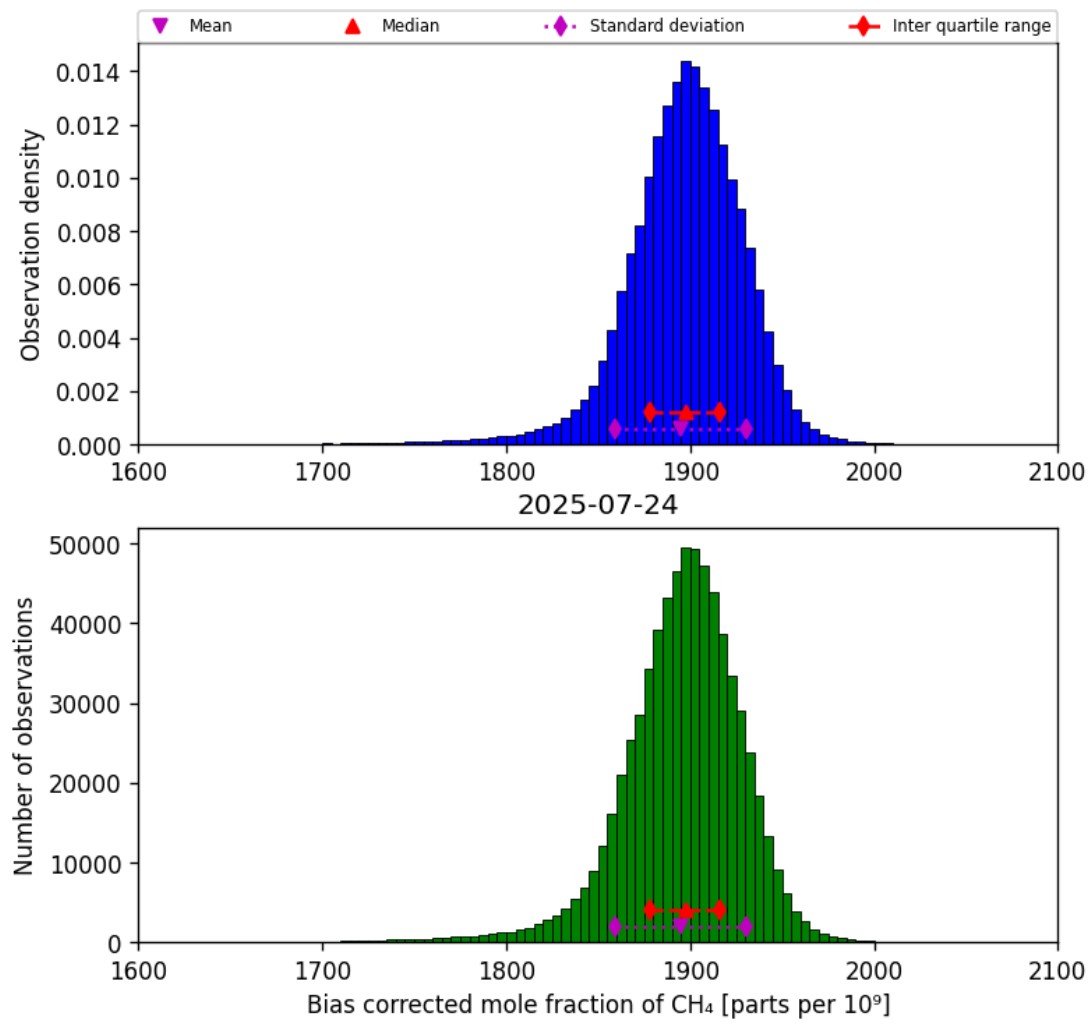
Figure 25: Histogram of “Bias corrected mole fraction of CH 4 ” for 2025-07-24 to 2025-07-25
