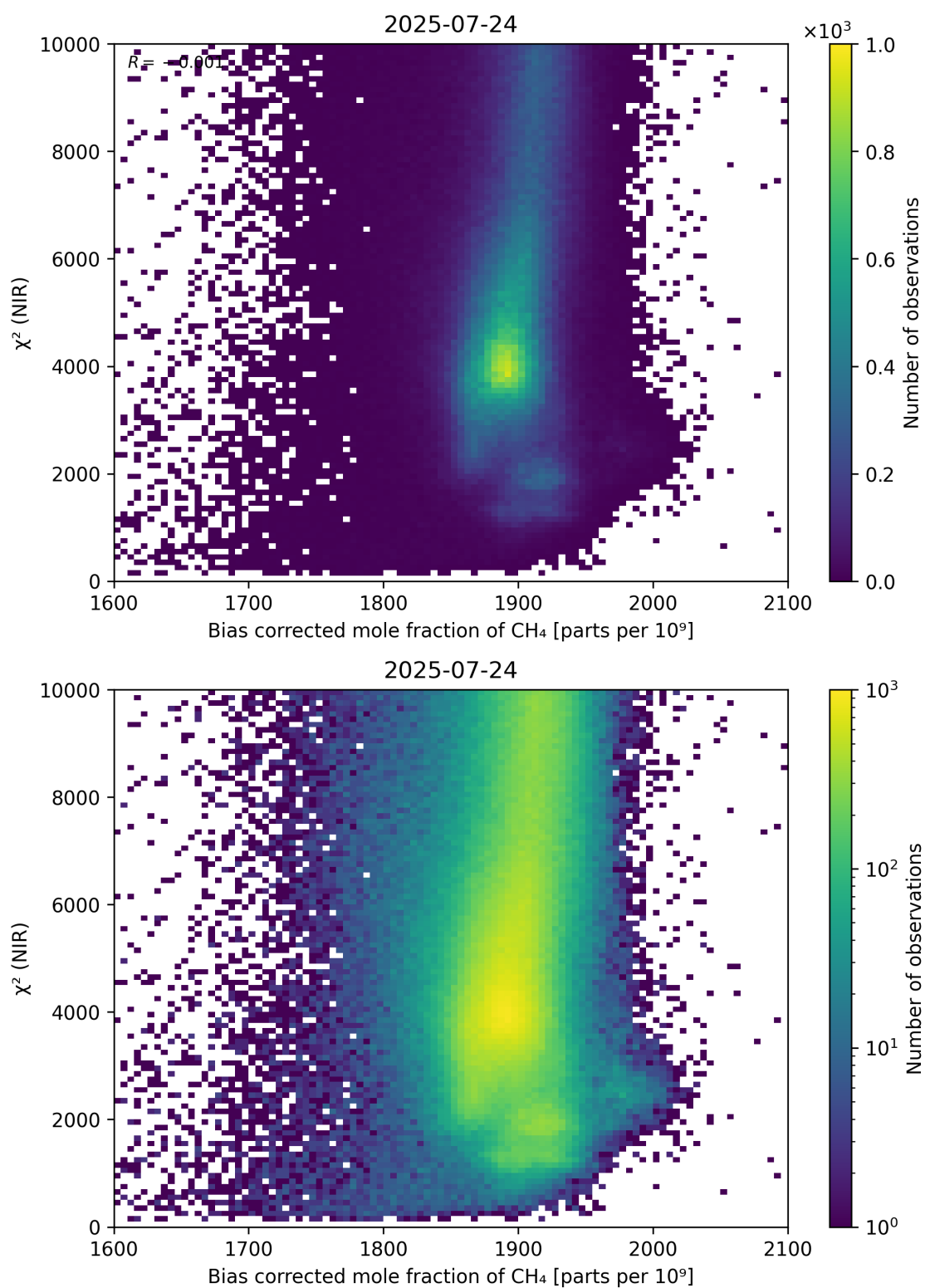
Figure 63: Scatter density plot of “Bias corrected mole fraction of CH 4 ” against “ \chi^2 (NIR)” for 2025-07-24 to 2025-07-25.
