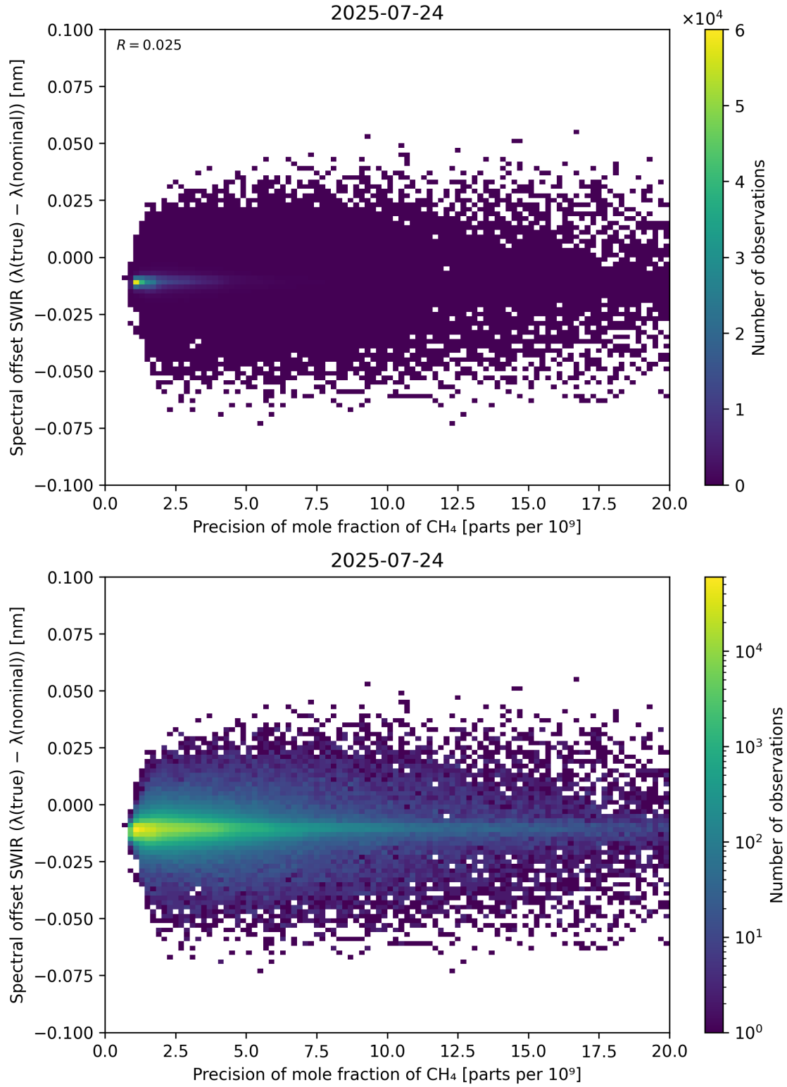
Figure 85: Scatter density plot of “Precision of mole fraction of \text{CH}_4 ” against “Spectral offset SWIR ( \lambda_{\text{true}} - \lambda_{\text{nominal}} )” for 2025-07-24 to 2025-07-25.
