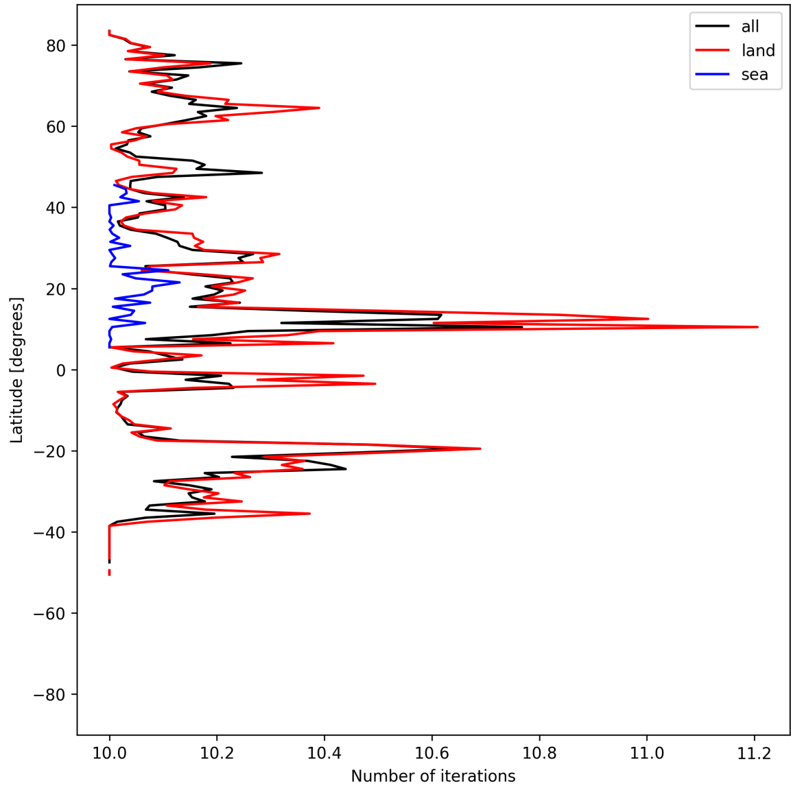
Figure 20: Zonal average of “Number of iterations” for 2025-07-24 to 2025-07-25.
