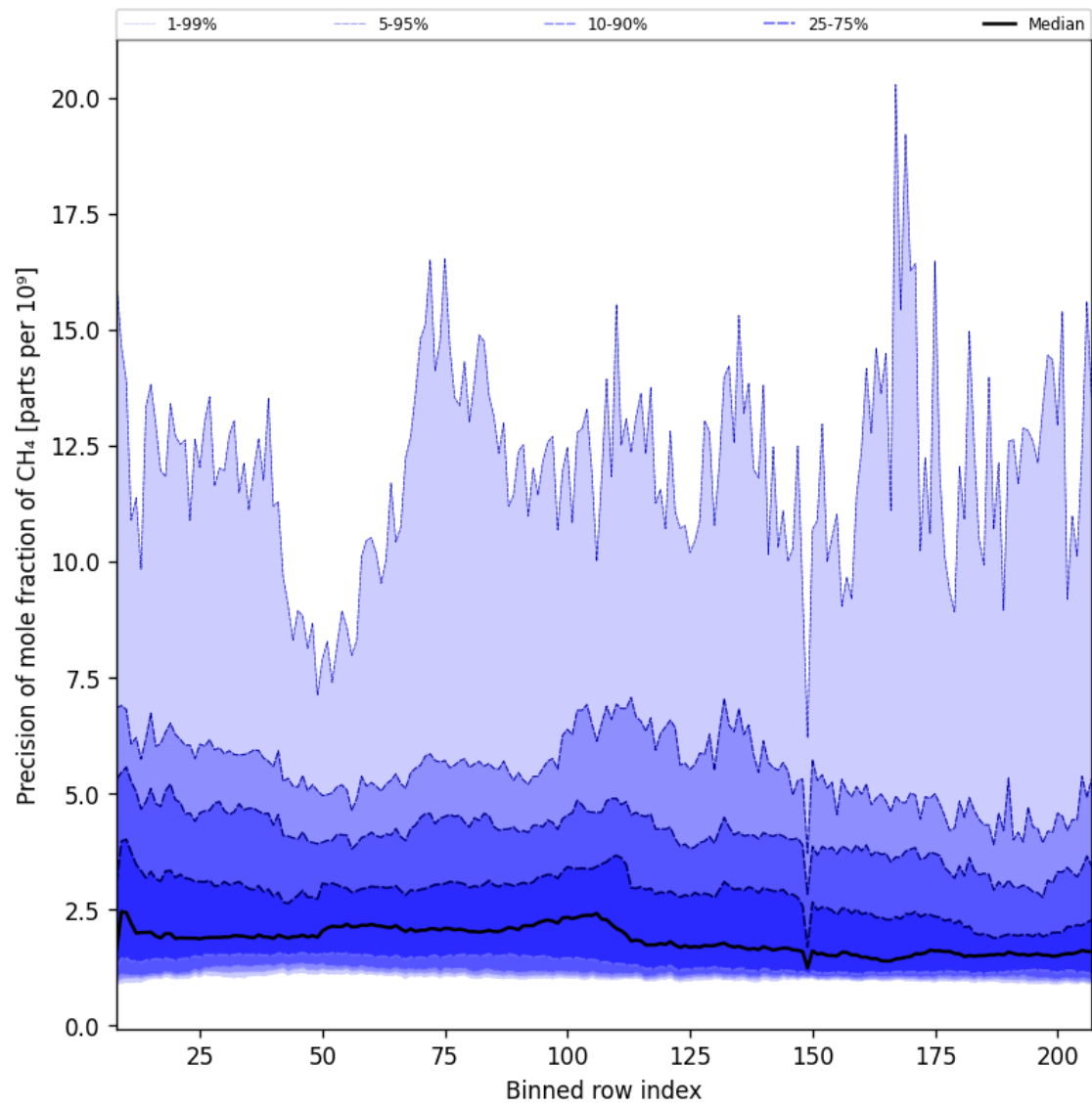
Figure 35: Along track statistics of “Precision of mole fraction of CH 4 ” for 2025-07-24 to 2025-07-25
