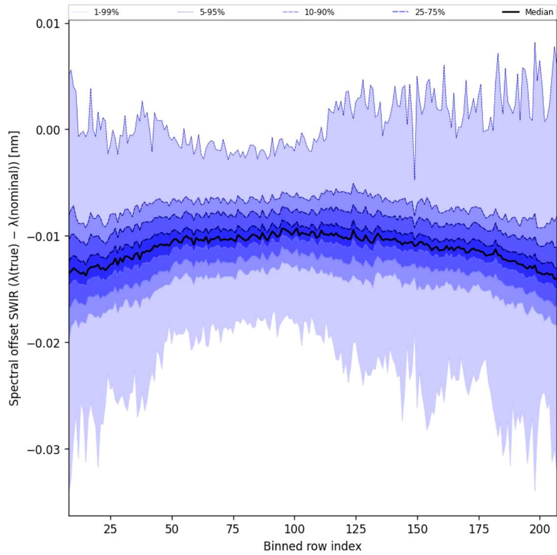
Figure 38: Along track statistics of “Spectral offset SWIR ( \lambda_{\text{true}} - \lambda_{\text{nominal}} )” for 2025-07-24 to 2025-07-25
