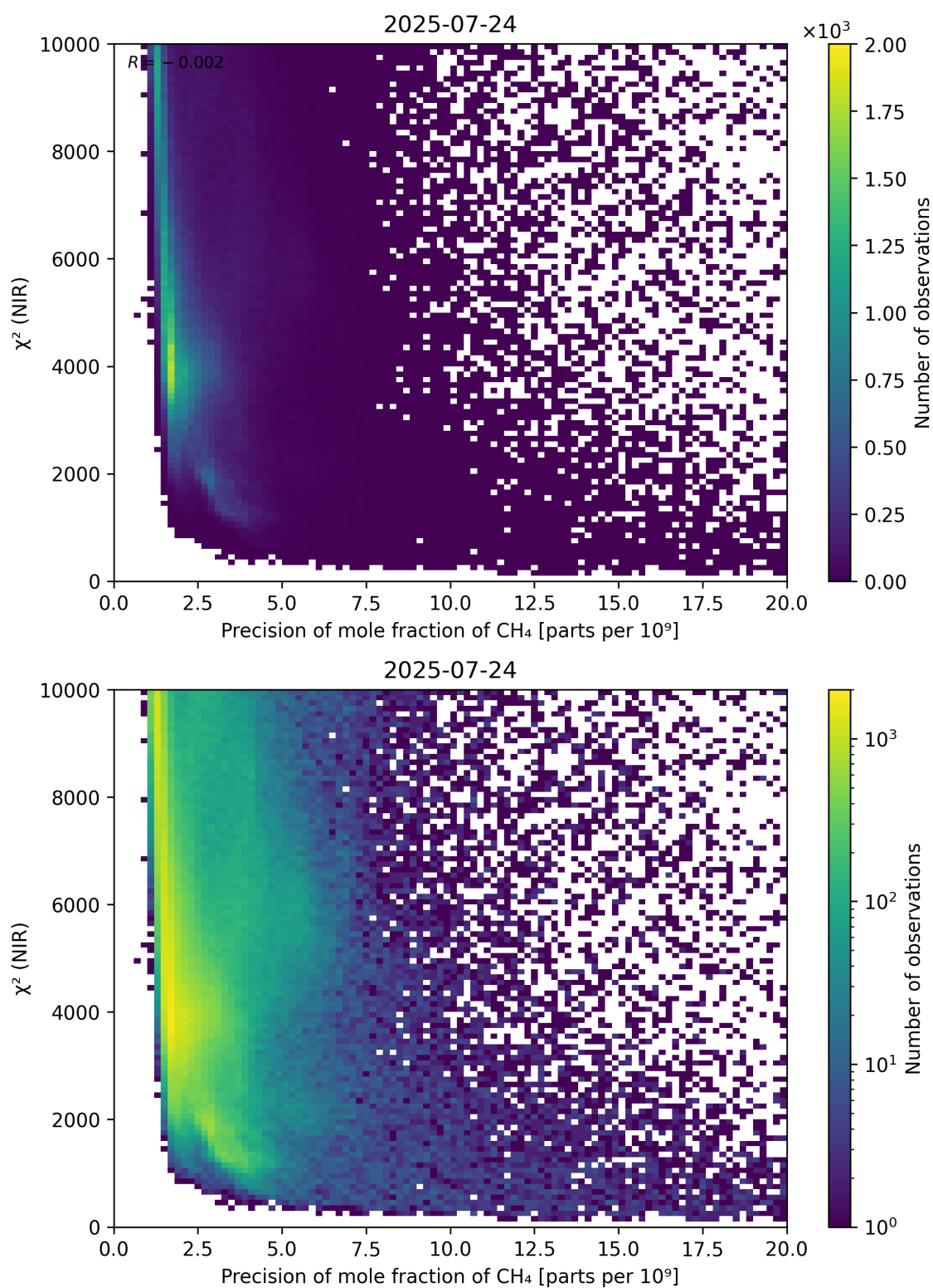
Figure 78: Scatter density plot of “Precision of mole fraction of \text{CH}_4 ” against “ \chi^2 (NIR)” for 2025-07-24 to 2025-07-25.
