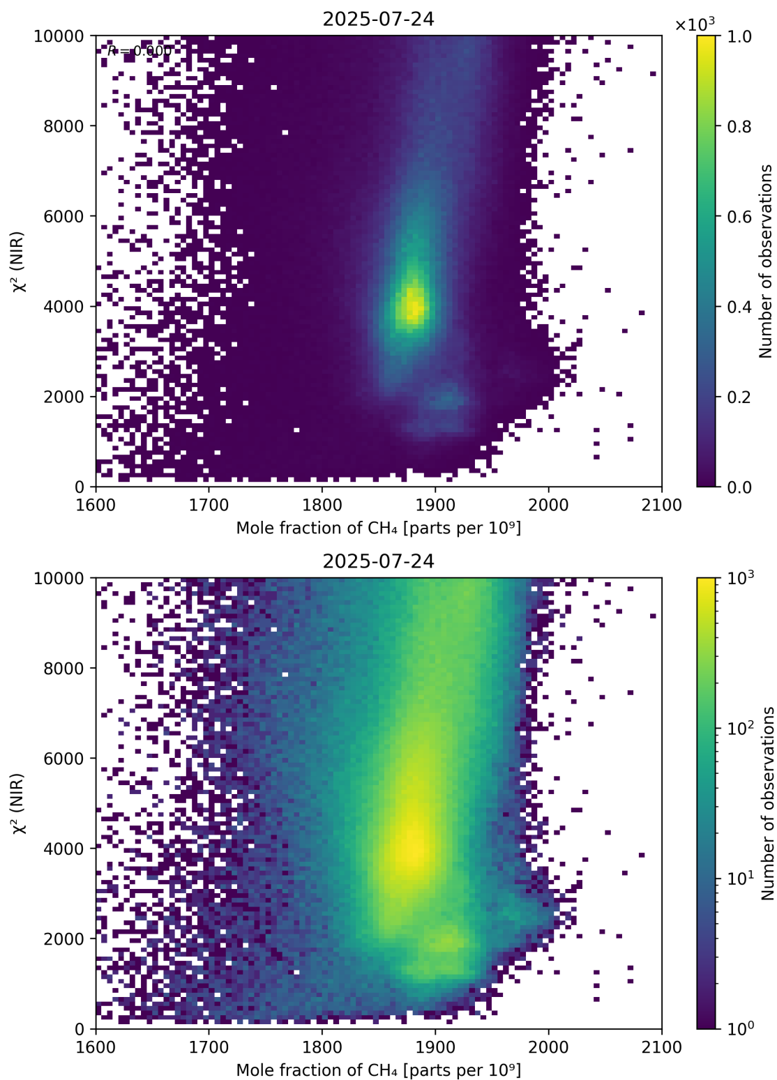
Figure 70: Scatter density plot of “Mole fraction of \text{CH}_4 ” against “ \chi^2 (NIR)” for 2025-07-24 to 2025-07-25.
