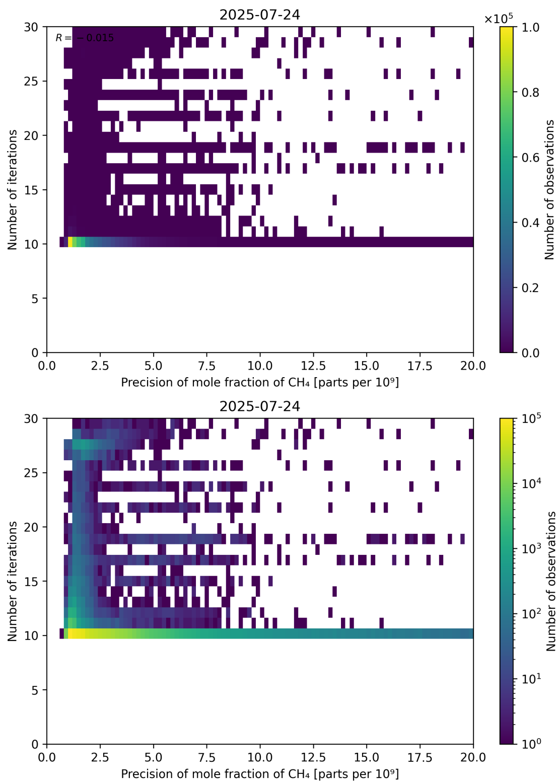
Figure 83: Scatter density plot of “Precision of mole fraction of CH 4 ” against “Number of iterations” for 2025-07-24 to 2025-07-25.
