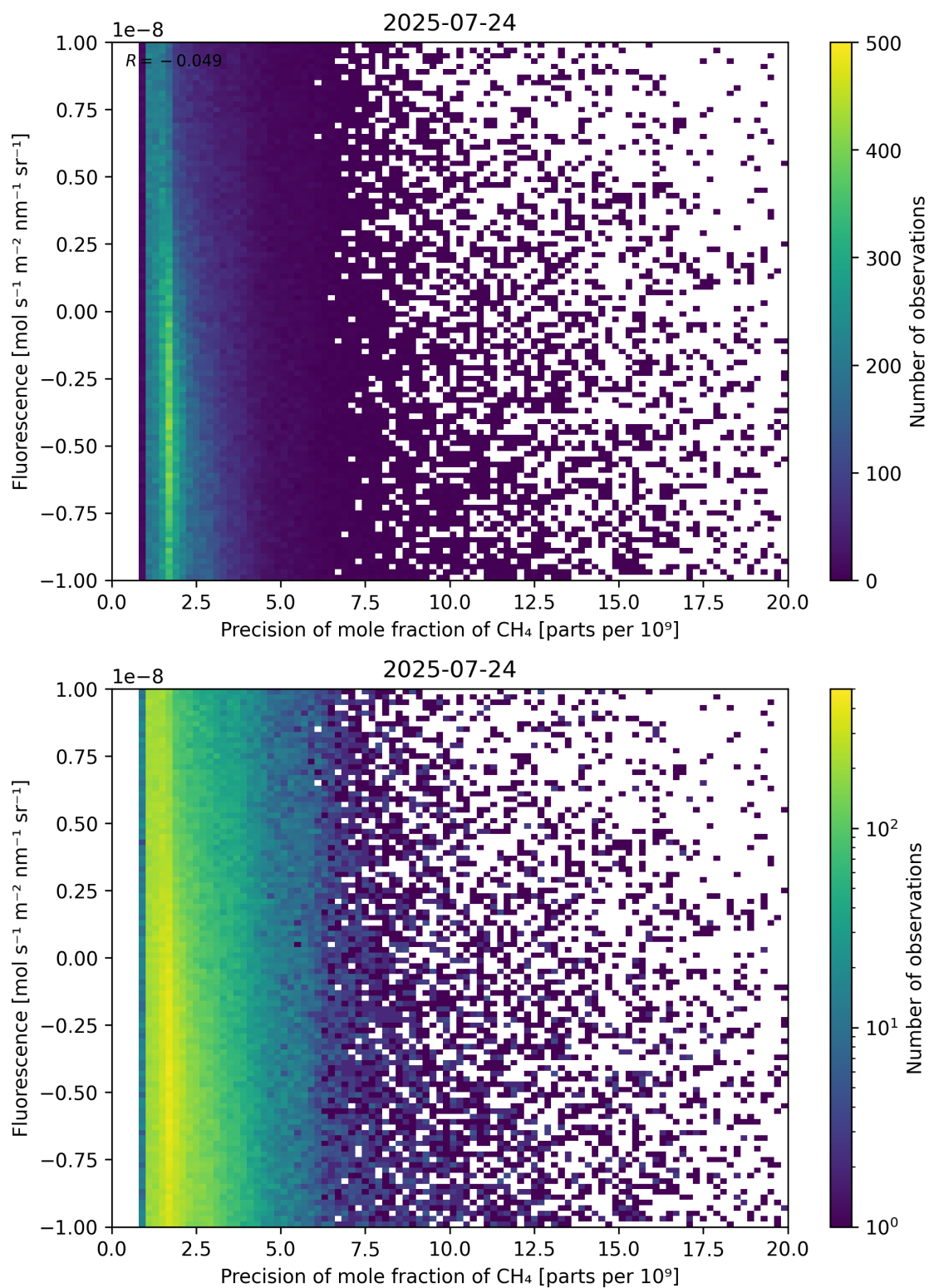
Figure 81: Scatter density plot of “Precision of mole fraction of \text{CH}_4 ” against “Fluorescence” for 2025-07-24 to 2025-07-25.
