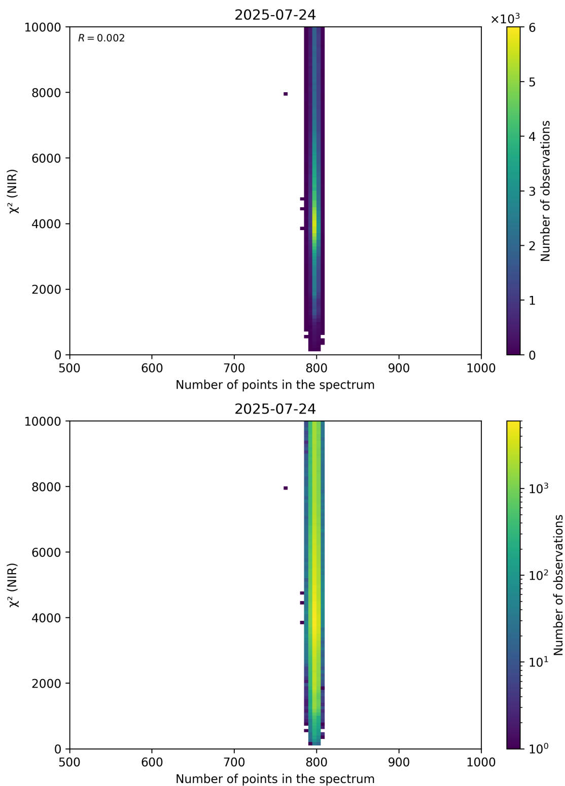
Figure 88: Scatter density plot of “Number of points in the spectrum” against “ \chi^2 (NIR)” for 2025-07-24 to 2025-07-25.
