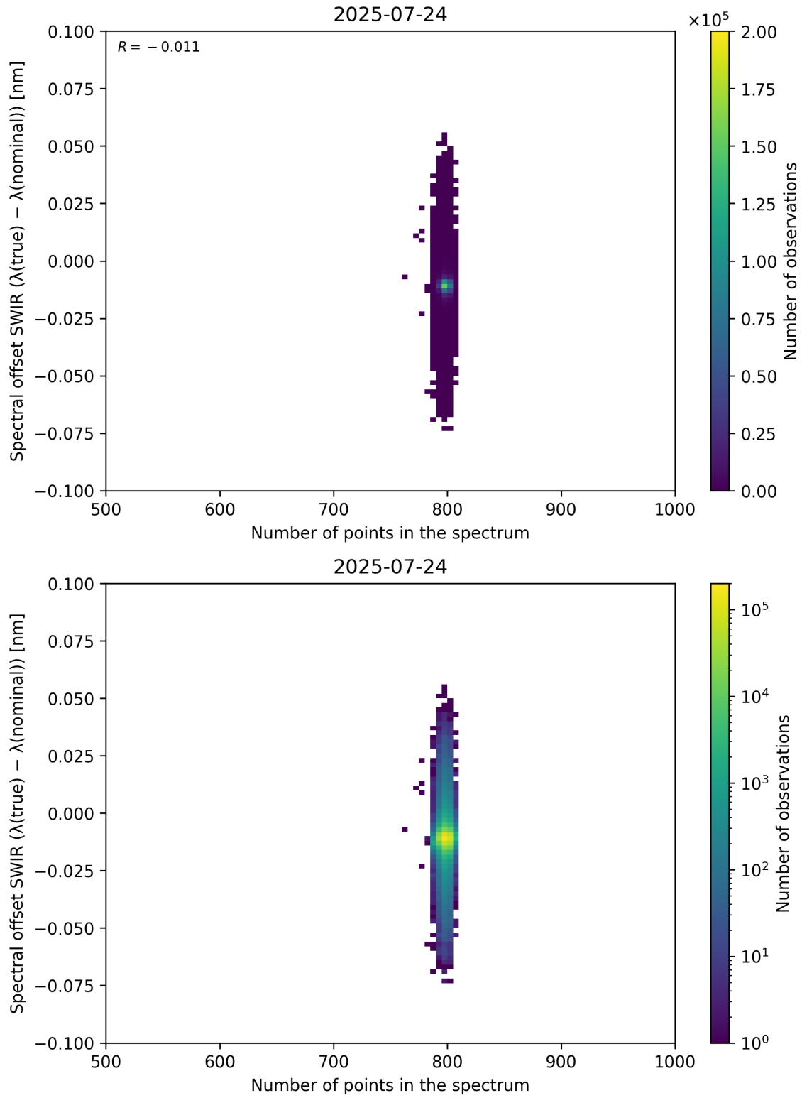
Figure 93: Scatter density plot of “Number of points in the spectrum” against “Spectral offset SWIR ( \lambda_{\text{true}} - \lambda_{\text{nominal}} )” for 2025-07-24 to 2025-07-25.
