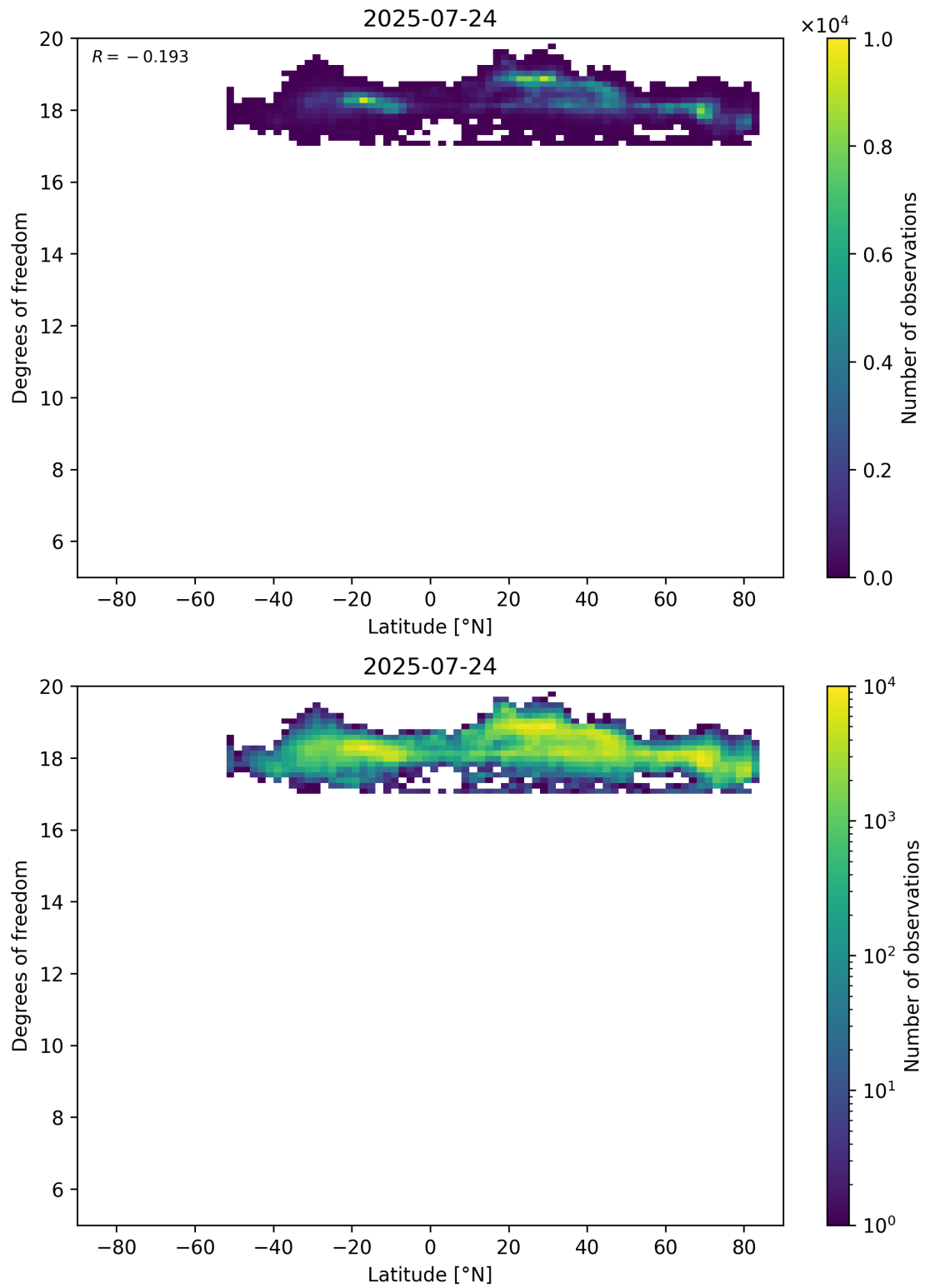
Figure 55: Scatter density plot of “Latitude” against “Degrees of freedom” for 2025-07-24 to 2025-07-25.
