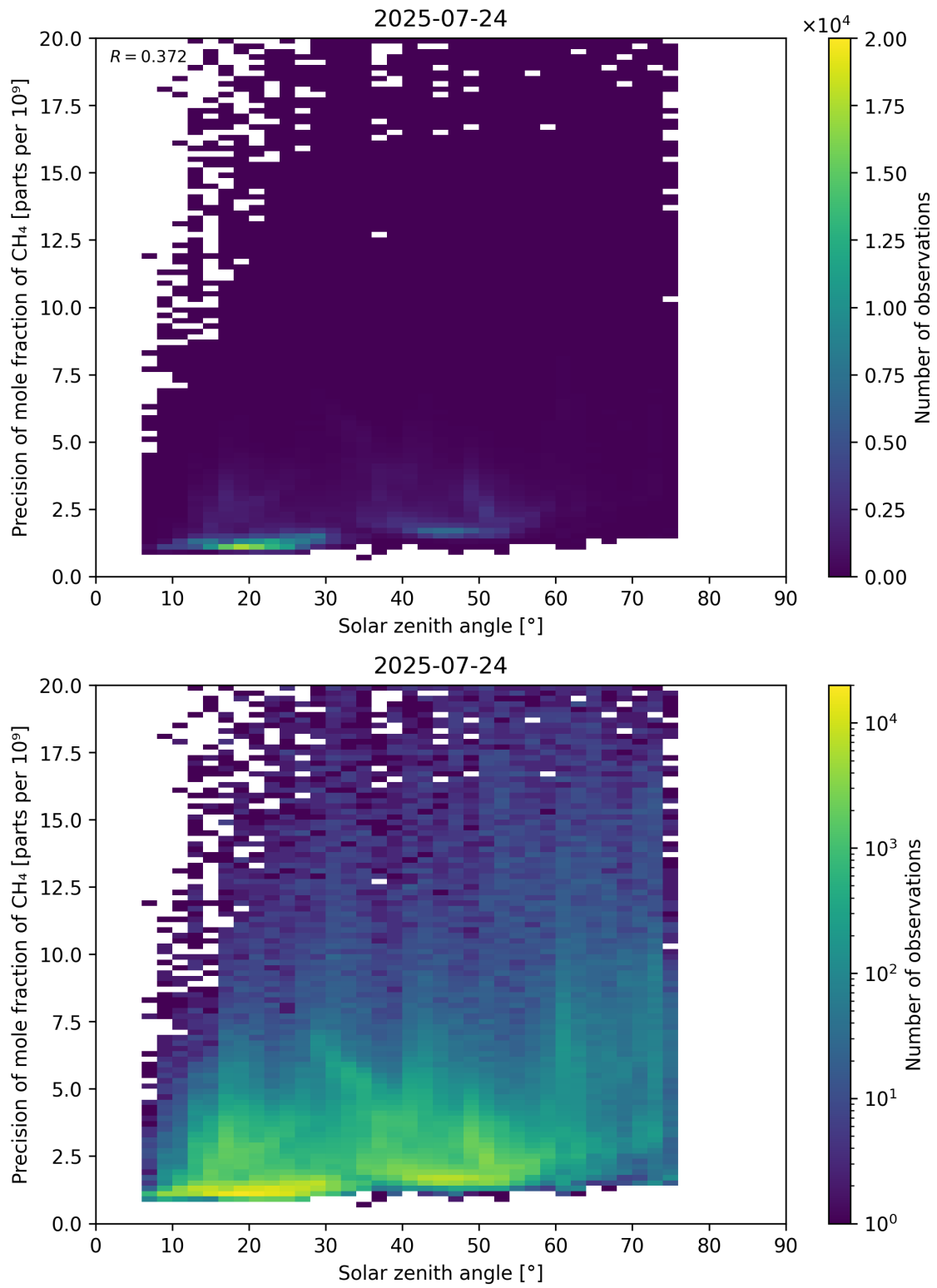
Figure 101: Scatter density plot of “Solar zenith angle” against “Precision of mole fraction of CH 4 ” for 2025-07-24 to 2025-07-25.
