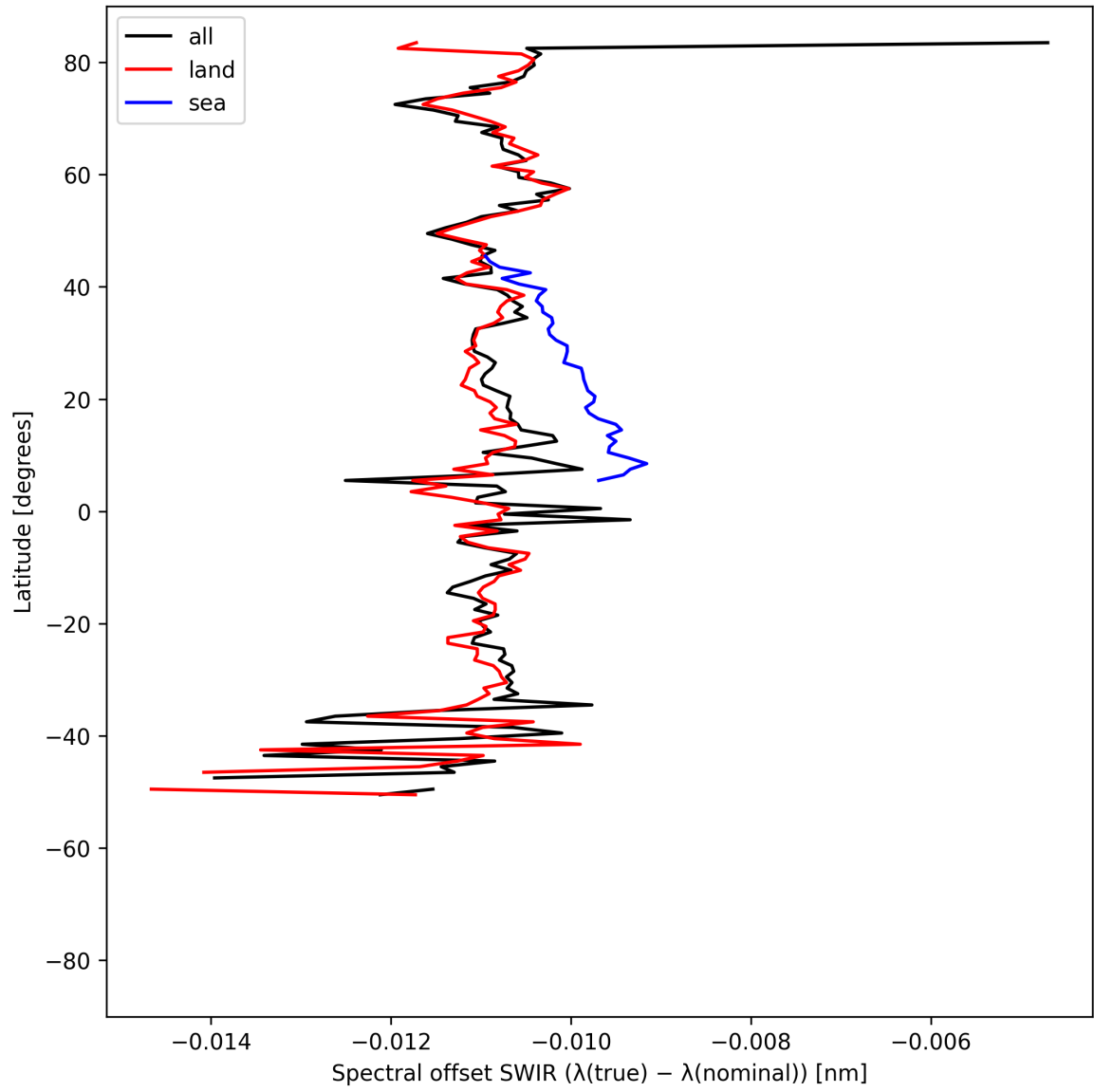
Figure 16: Zonal average of “Spectral offset SWIR ( \lambda_{\text{true}} - \lambda_{\text{nominal}} )” for 2025-07-24 to 2025-07-25.
