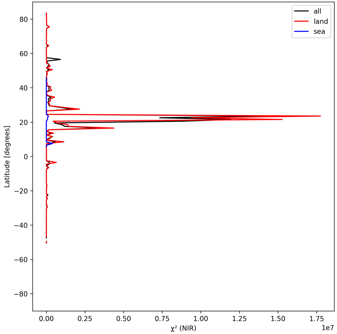
Figure 18: Zonal average of “ \chi^2 (NIR)” for 2025-07-24 to 2025-07-25.
