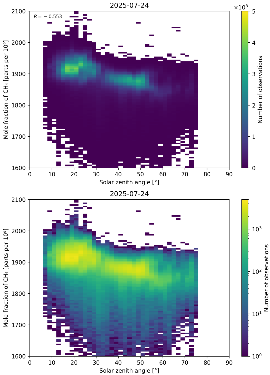
Figure 99: Scatter density plot of “Solar zenith angle” against “Mole fraction of \text{CH}_4 ” for 2025-07-24 to 2025-07-25.
