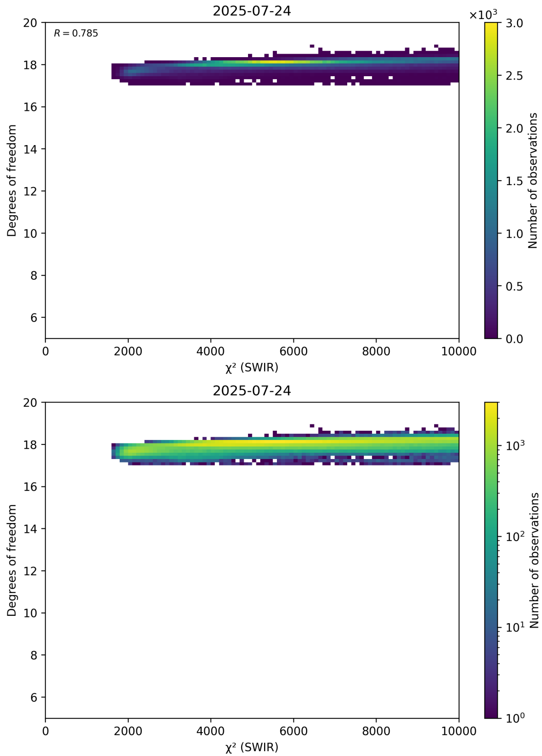
Figure 48: Scatter density plot of “ \chi^2 (SWIR)” against “Degrees of freedom” for 2025-07-24 to 2025-07-25.
