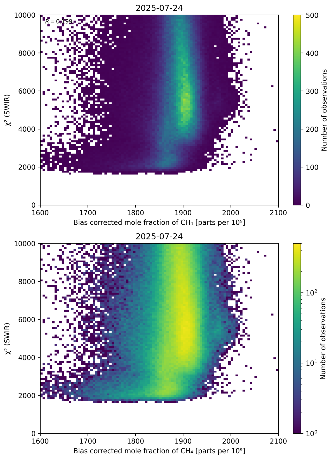
Figure 64: Scatter density plot of “Bias corrected mole fraction of \text{CH}_4 ” against “ \chi^2 (SWIR)” for 2025-07-24 to 2025-07-25.
