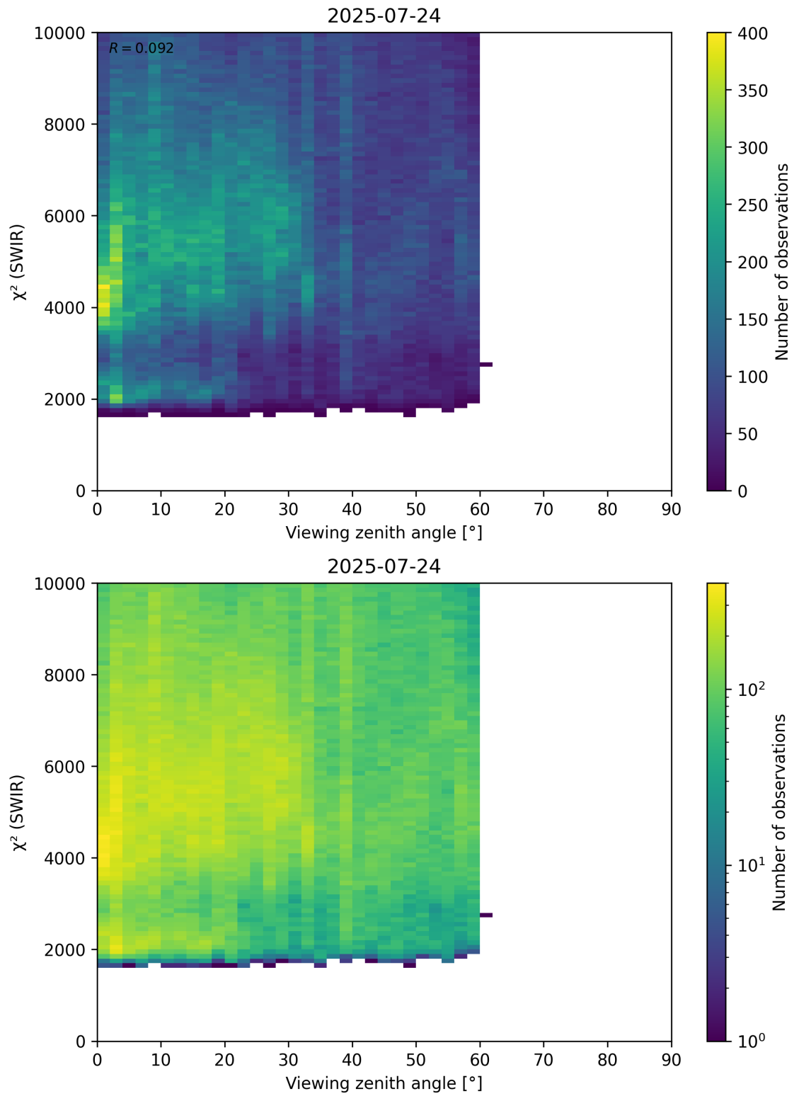
Figure 106: Scatter density plot of “Viewing zenith angle” against “ \chi^2 (SWIR)” for 2025-07-24 to 2025-07-25.
