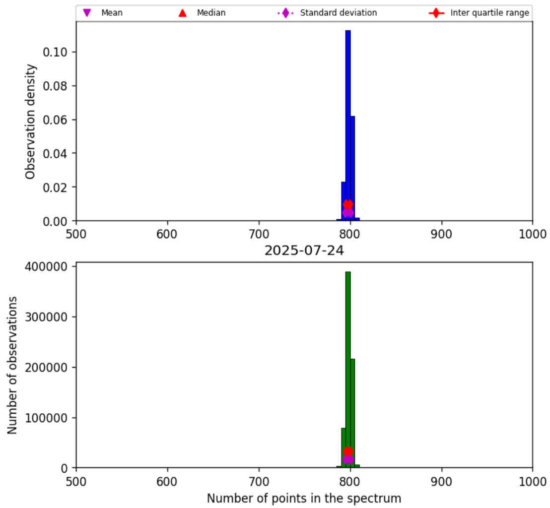
Figure 26: Histogram of “Number of points in the spectrum” for 2025-07-24 to 2025-07-25
