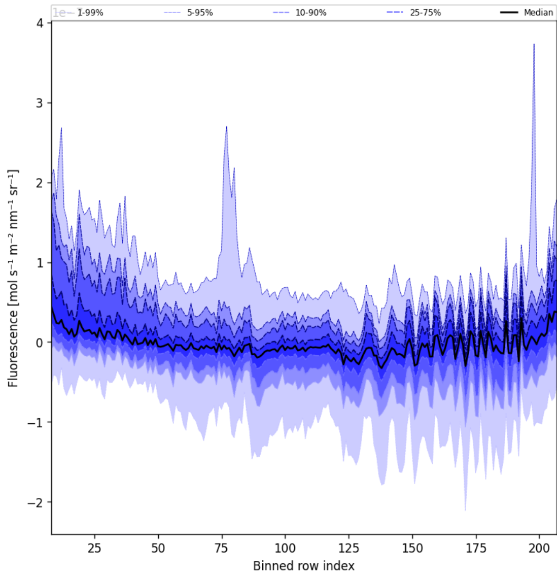
Figure 43: Along track statistics of “Fluorescence” for 2025-07-24 to 2025-07-25
