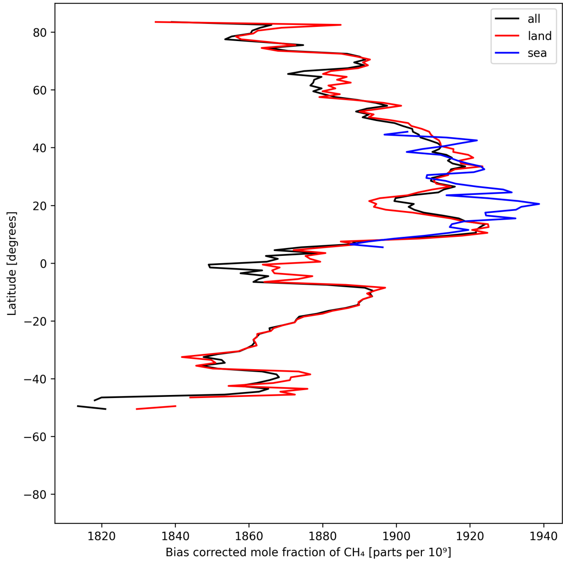
Figure 14: Zonal average of “Bias corrected mole fraction of CH 4 ” for 2025-07-24 to 2025-07-25.
