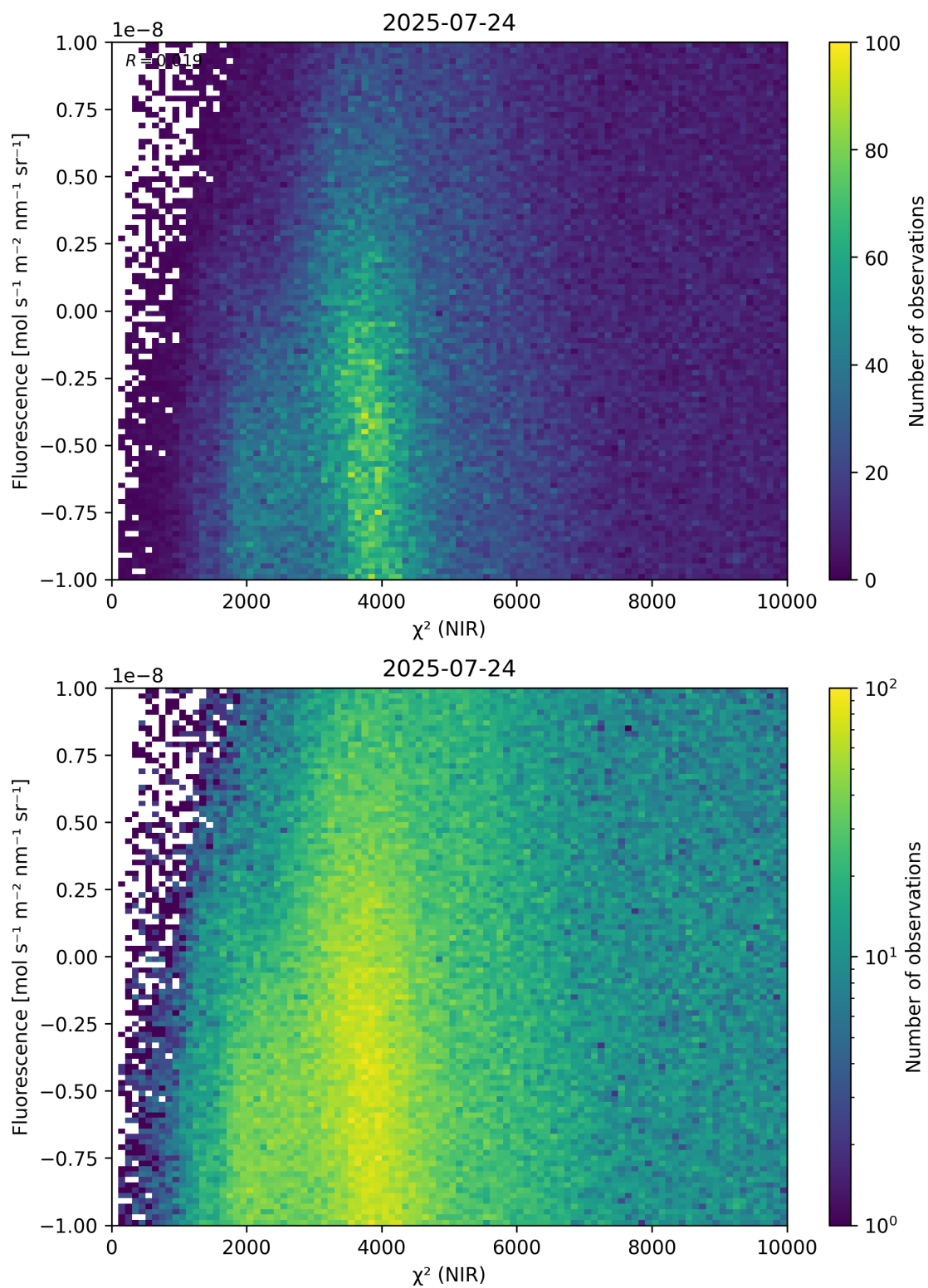
Figure 45: Scatter density plot of “ \chi^2 (NIR)” against “Fluorescence” for 2025-07-24 to 2025-07-25.
