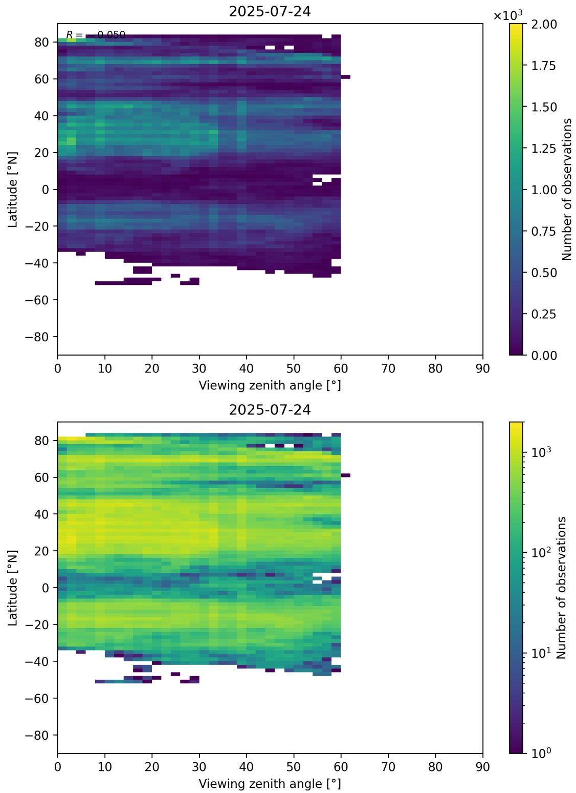
Figure 109: Scatter density plot of “Viewing zenith angle” against “Latitude” for 2025-07-24 to 2025-07-25.
