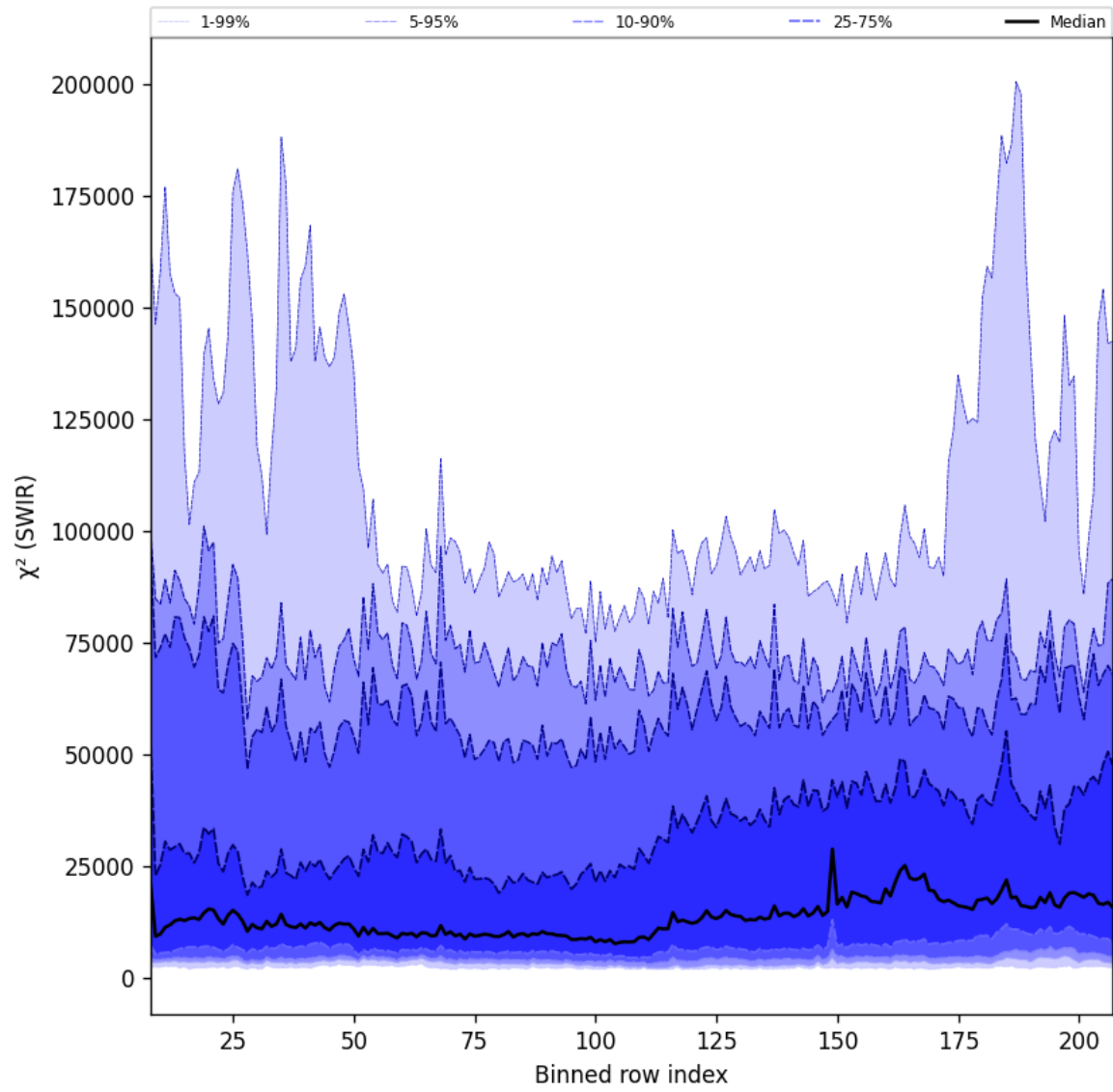
Figure 39: Along track statistics of " \chi^2 (SWIR)" for 2025-07-24 to 2025-07-25
