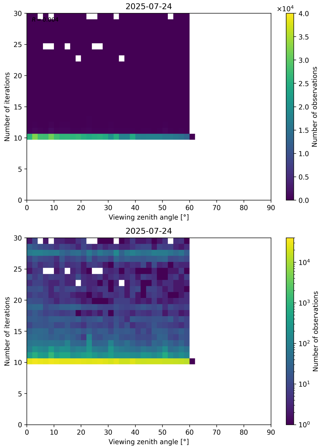
Figure 113: Scatter density plot of “Viewing zenith angle” against “Number of iterations” for 2025-07-24 to 2025-07-25.
