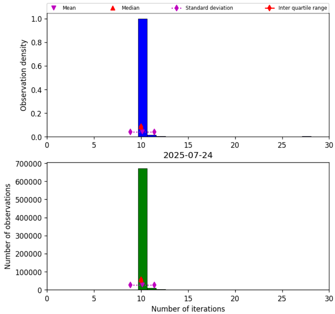
Figure 31: Histogram of “Number of iterations” for 2025-07-24 to 2025-07-25
