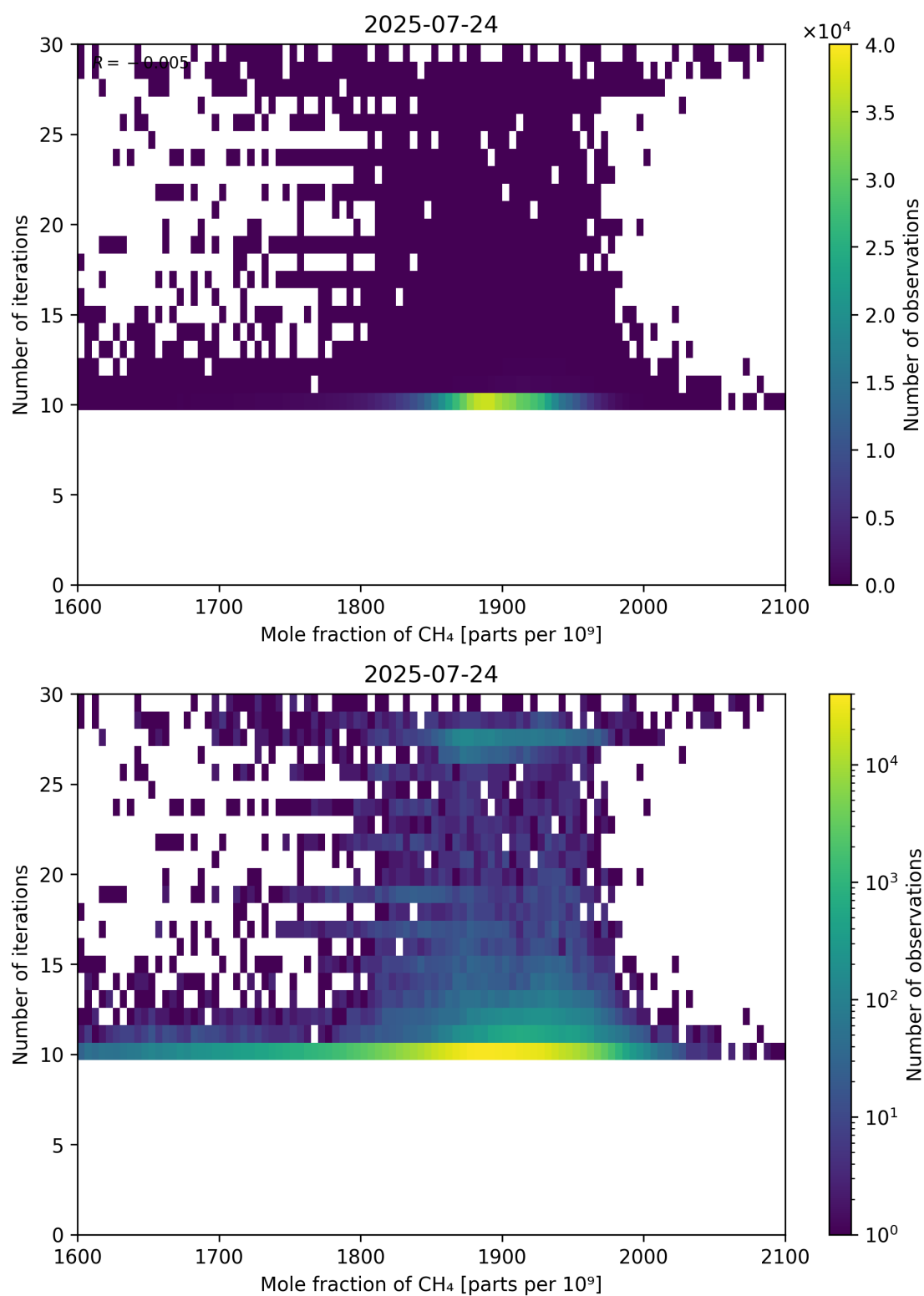
Figure 76: Scatter density plot of “Mole fraction of CH 4 ” against “Number of iterations” for 2025-07-24 to 2025-07-25.
