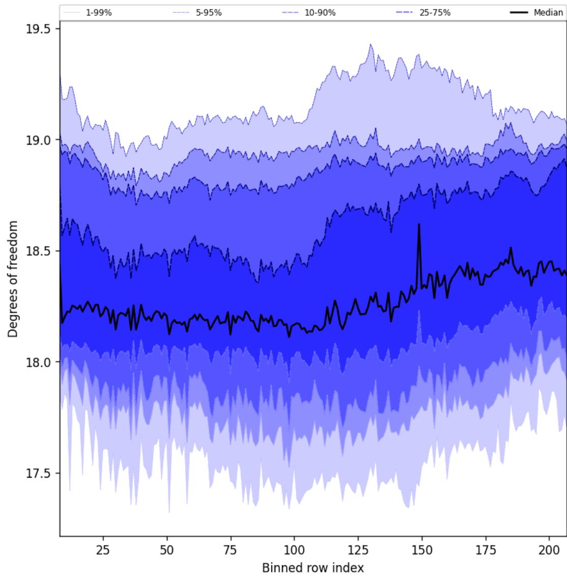
Figure 41: Along track statistics of “Degrees of freedom” for 2025-07-24 to 2025-07-25
