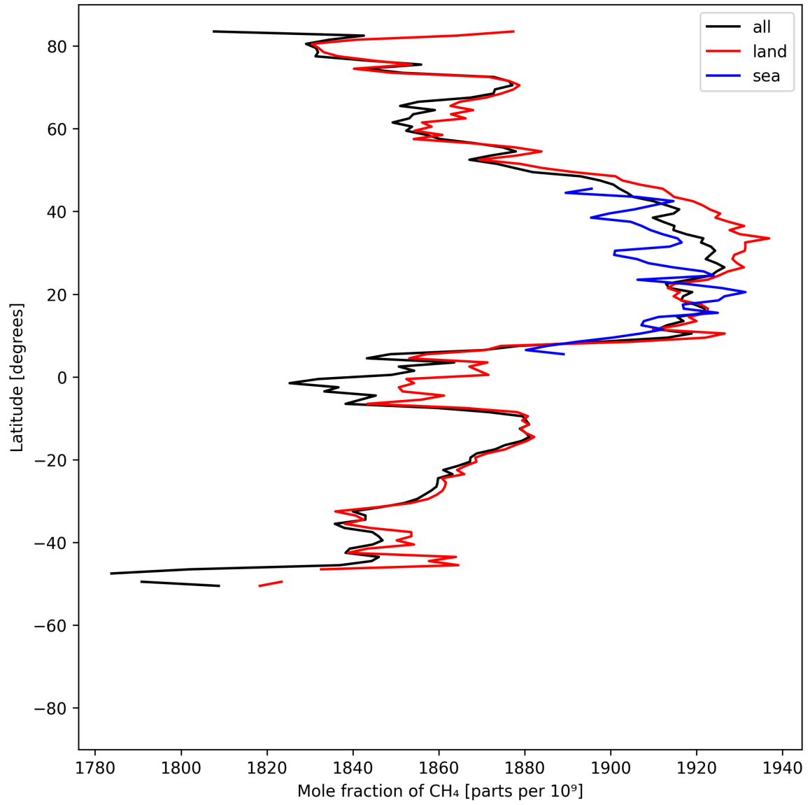
Figure 12: Zonal average of “Mole fraction of \text{CH}_4 ” for 2025-07-24 to 2025-07-25.
