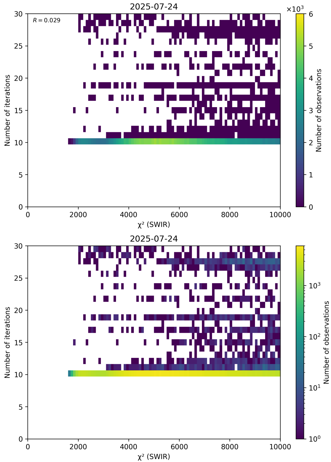
Figure 50: Scatter density plot of “ \chi^2 (SWIR)” against “Number of iterations” for 2025-07-24 to 2025-07-25.
