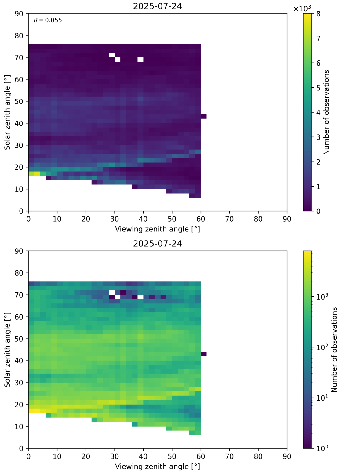
Figure 115: Scatter density plot of “Viewing zenith angle” against “Solar zenith angle” for 2025-07-24 to 2025-07-25.
