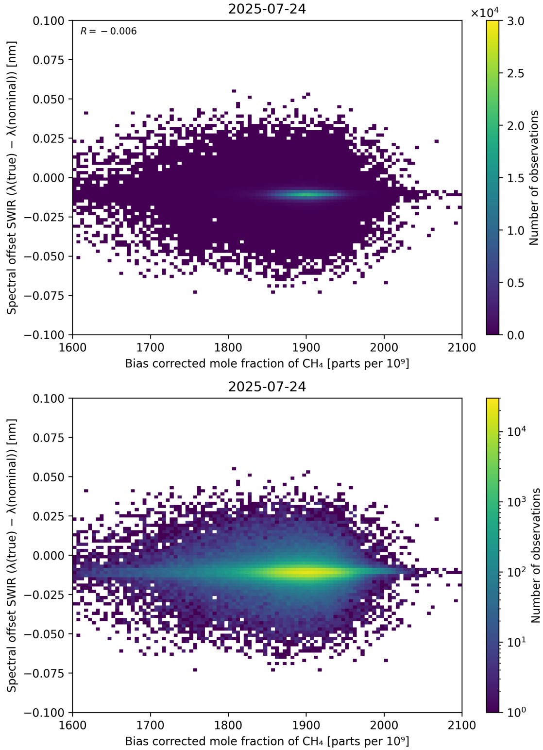
Figure 69: Scatter density plot of “Bias corrected mole fraction of \text{CH}_4 ” against “Spectral offset SWIR ( \lambda_{\text{true}} - \lambda_{\text{nominal}} )” for 2025-07-24 to 2025-07-25.
