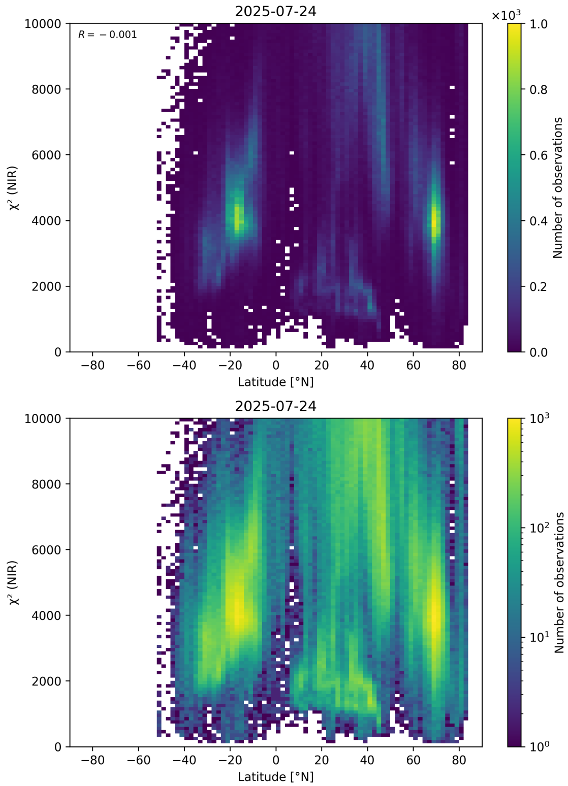
Figure 53: Scatter density plot of “Latitude” against “ \chi^2 (NIR)” for 2025-07-24 to 2025-07-25.
