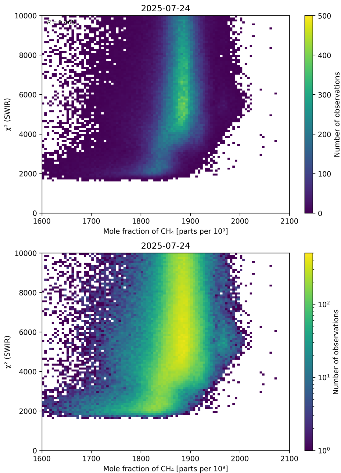
Figure 71: Scatter density plot of “Mole fraction of \text{CH}_4 ” against “ \chi^2 (SWIR)” for 2025-07-24 to 2025-07-25.
