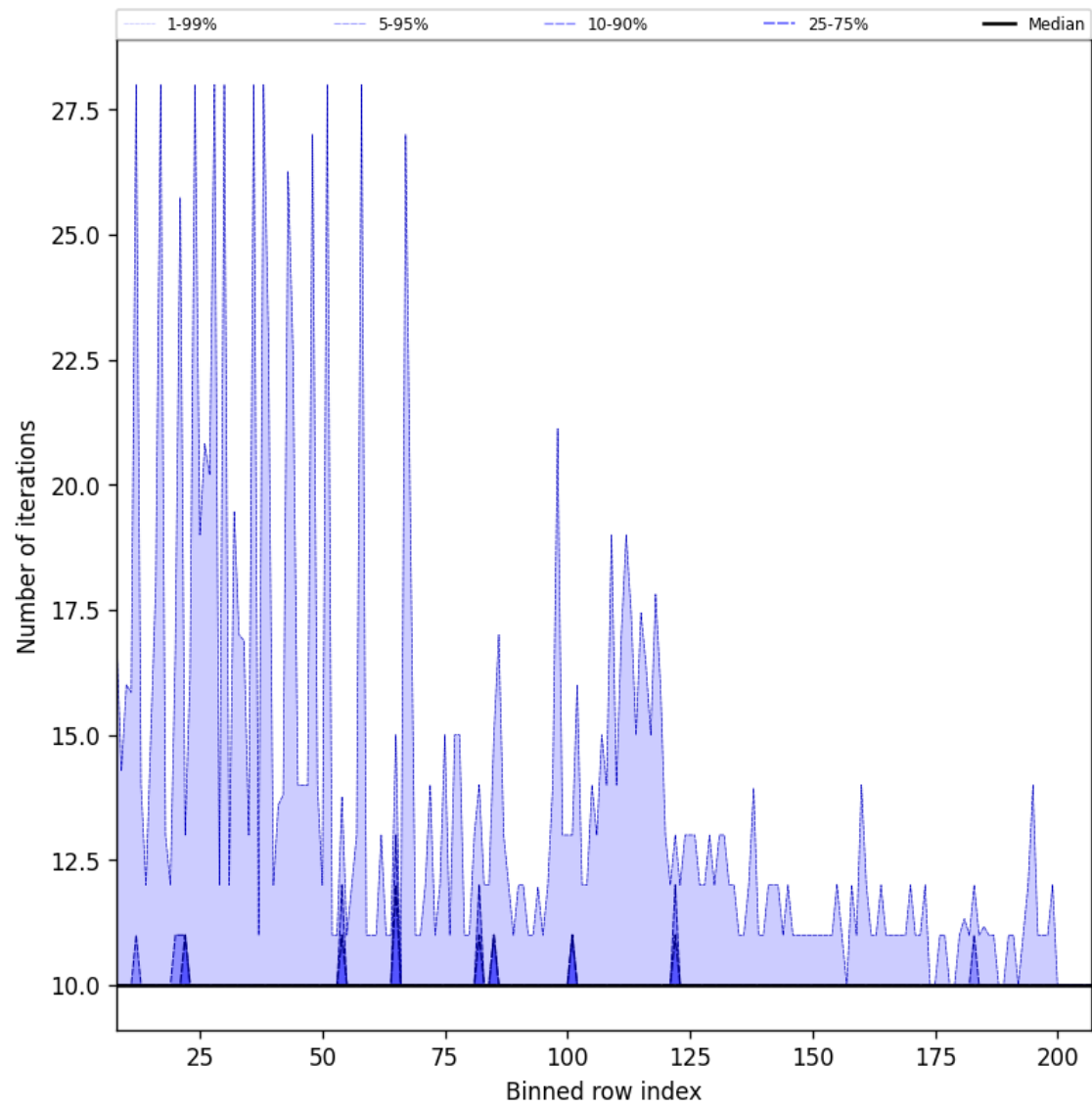
Figure 42: Along track statistics of “Number of iterations” for 2025-07-24 to 2025-07-25
