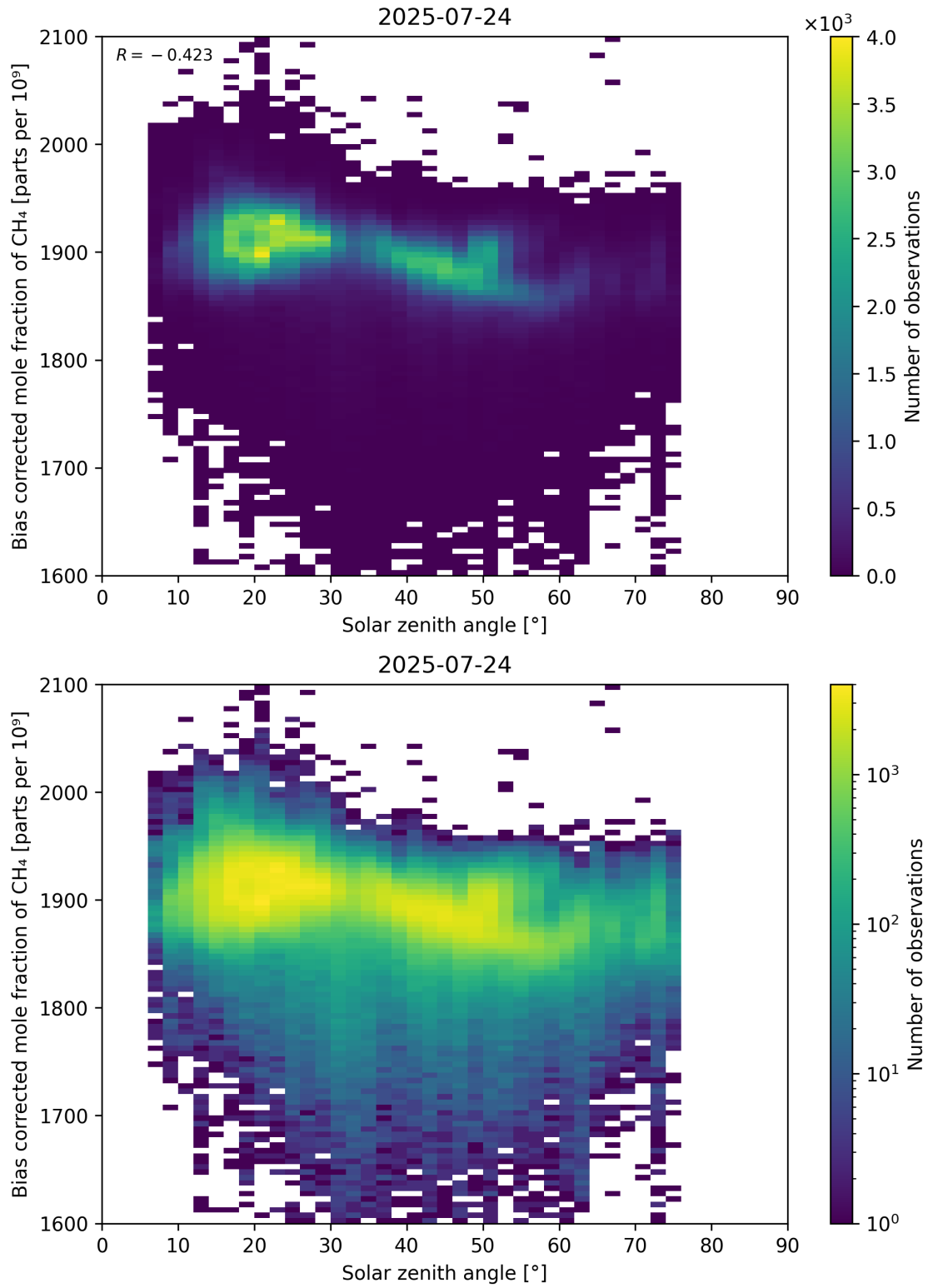
Figure 100: Scatter density plot of “Solar zenith angle” against “Bias corrected mole fraction of CH 4 ” for 2025-07-24 to 2025-07-25.
