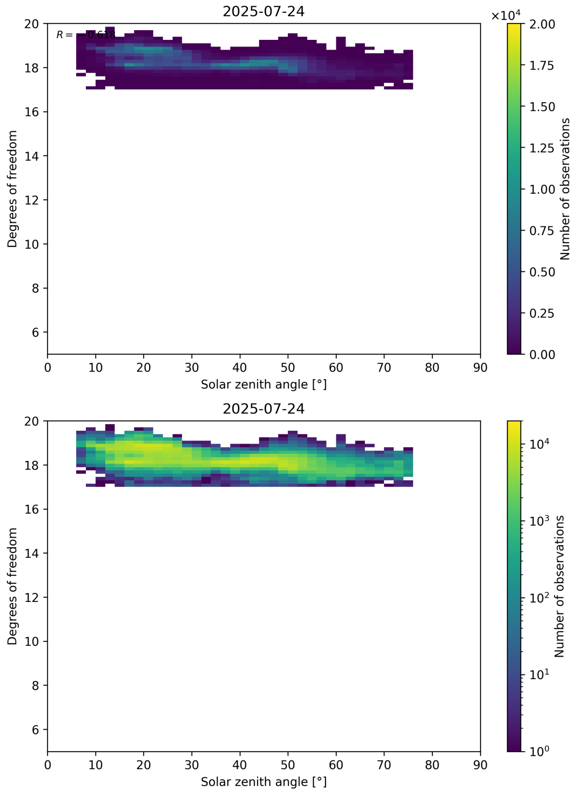
Figure 96: Scatter density plot of “Solar zenith angle” against “Degrees of freedom” for 2025-07-24 to 2025-07-25.
