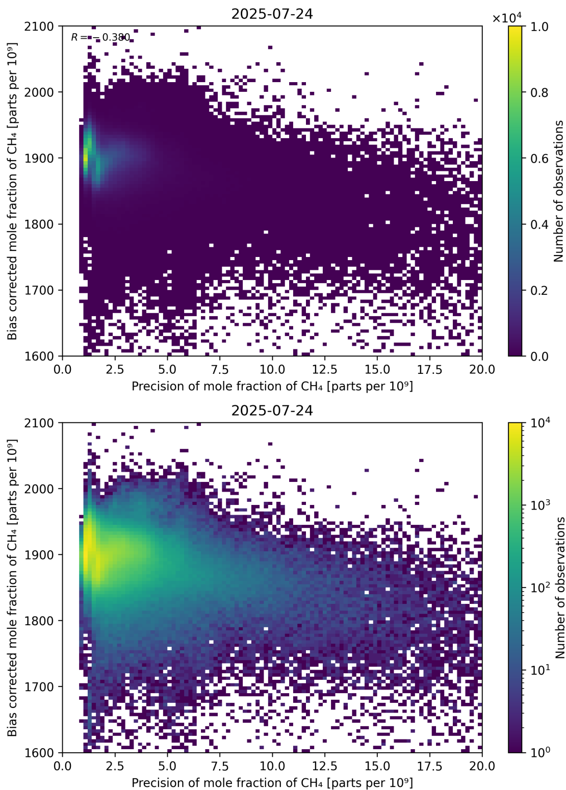
Figure 82: Scatter density plot of “Precision of mole fraction of CH 4 ” against “Bias corrected mole fraction of CH 4 ” for 2025-07-24 to 2025-07-25.
