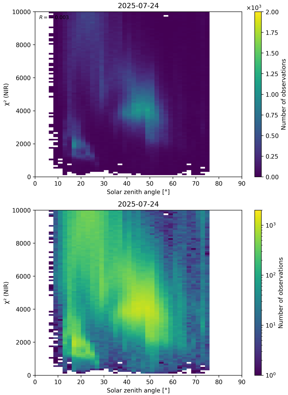
Figure 94: Scatter density plot of “Solar zenith angle” against “ \chi^2 (NIR)” for 2025-07-24 to 2025-07-25.
