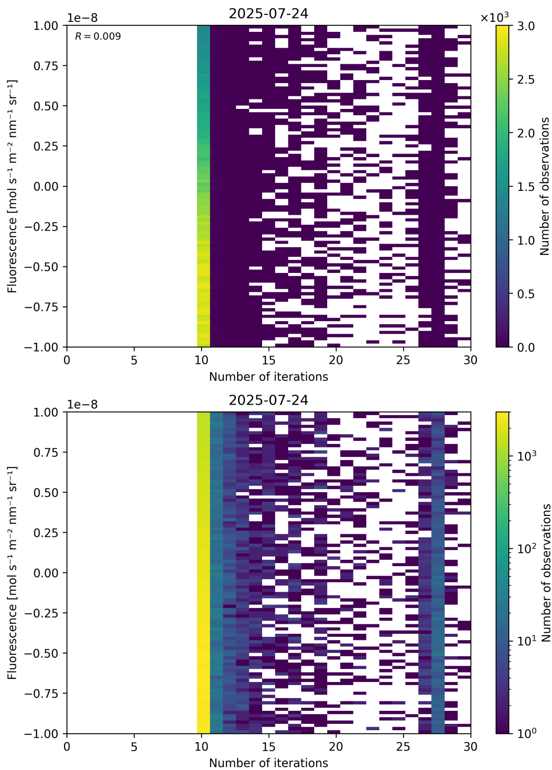
Figure 87: Scatter density plot of “Number of iterations” against “Fluorescence” for 2025-07-24 to 2025-07-25.
