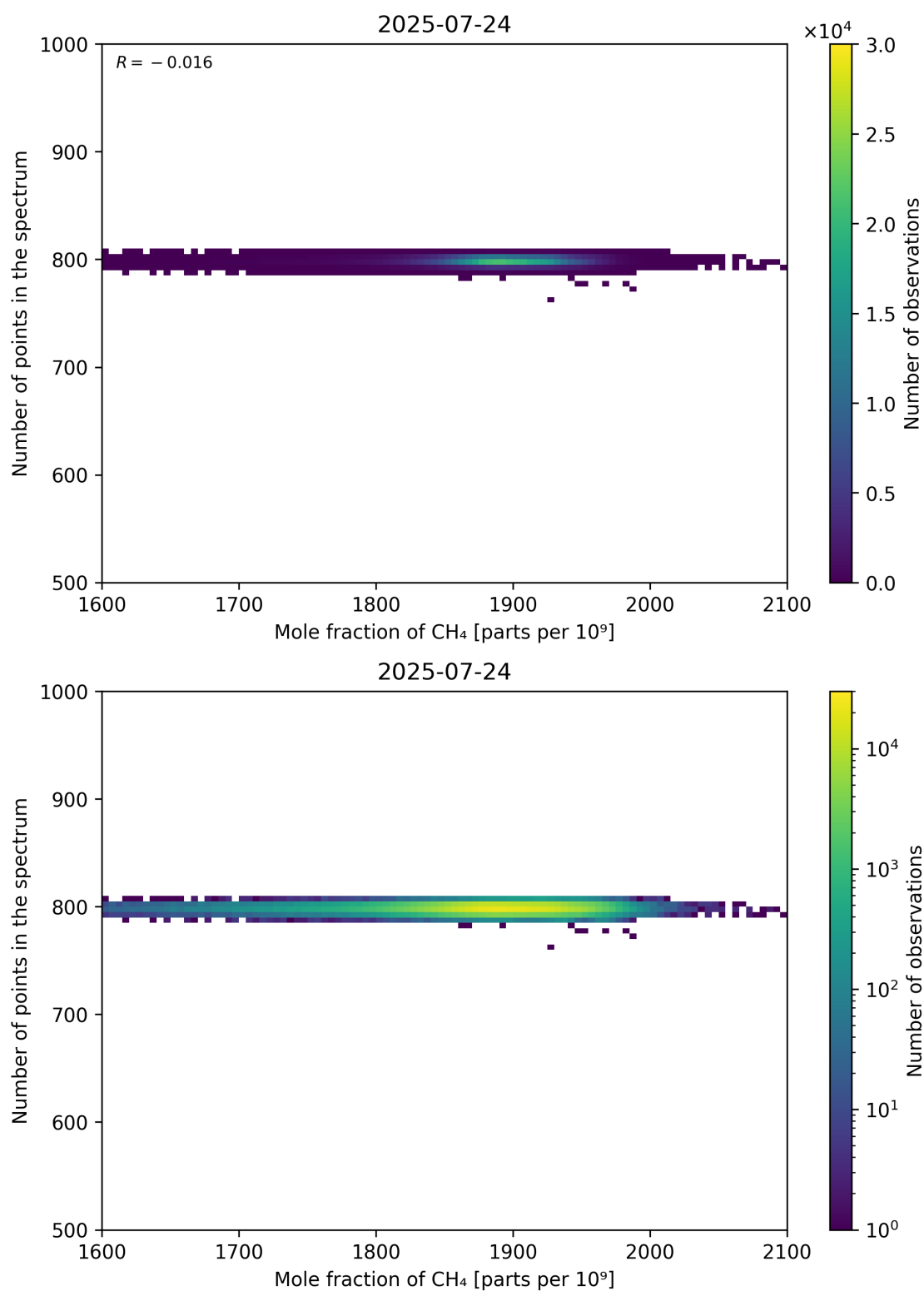
Figure 77: Scatter density plot of “Mole fraction of CH 4 ” against “Number of points in the spectrum” for 2025-07-24 to 2025-07-25.
