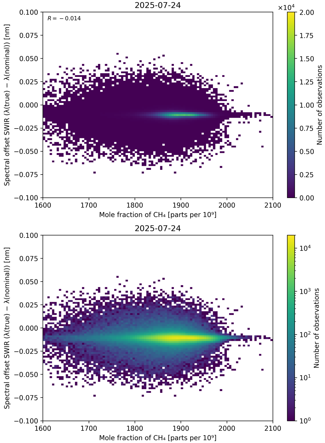
Figure 86: Scatter density plot of “Mole fraction of CH 4 ” against “Spectral offset SWIR ( \lambda_{\text{true}} - \lambda_{\text{nominal}} )” for 2025-07-24 to 2025-07-25.
