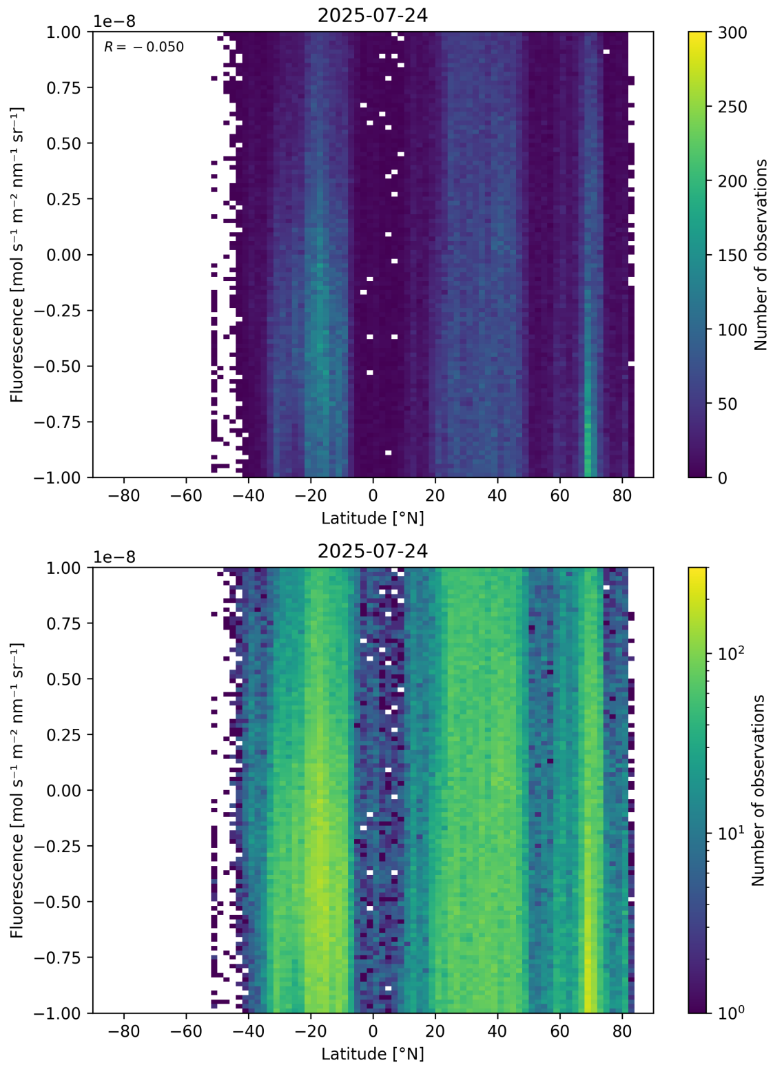
Figure 56: Scatter density plot of “Latitude” against “Fluorescence” for 2025-07-24 to 2025-07-25.
