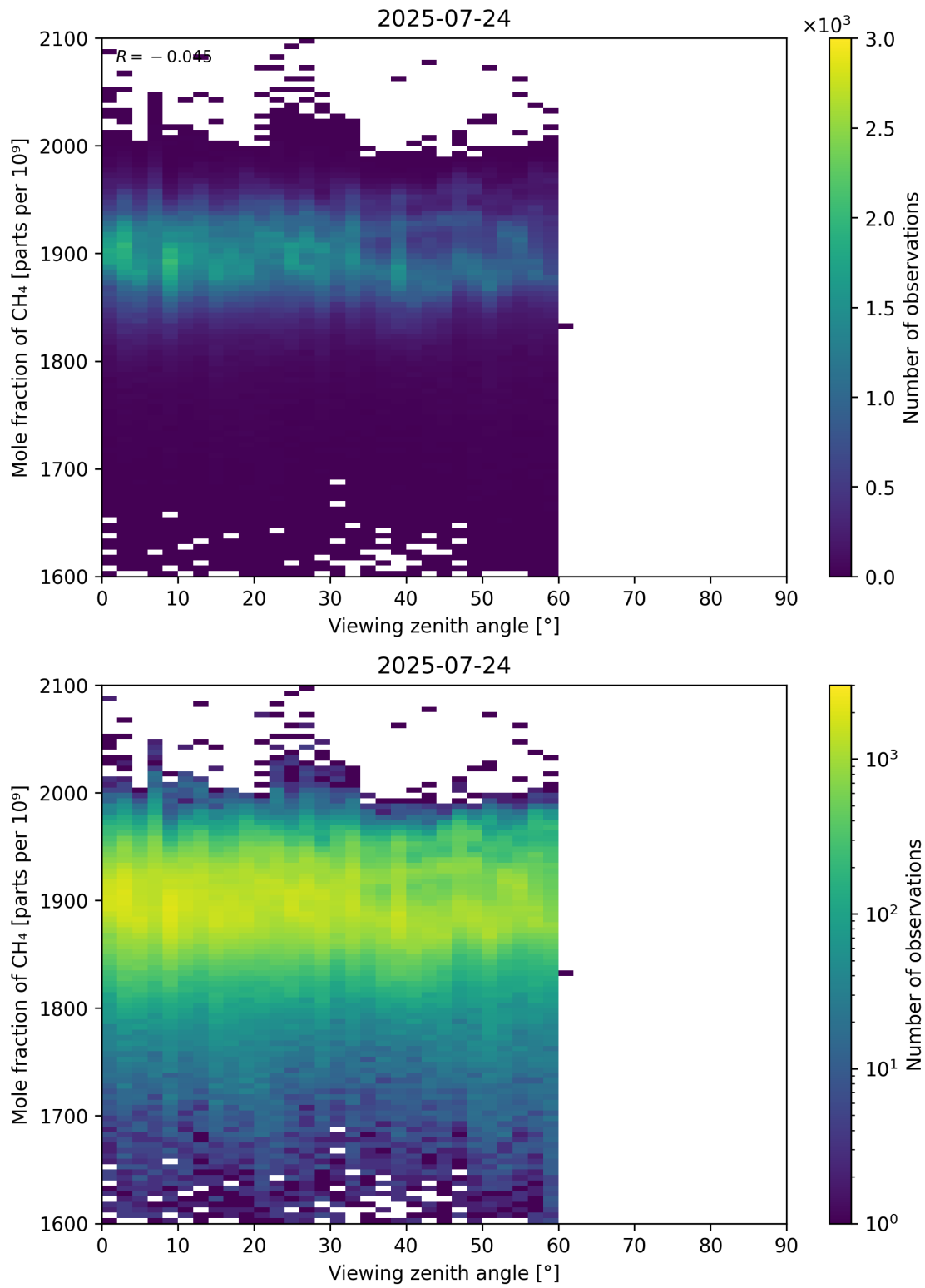
Figure 110: Scatter density plot of “Viewing zenith angle” against “Mole fraction of CH 4 ” for 2025-07-24 to 2025-07-25.
