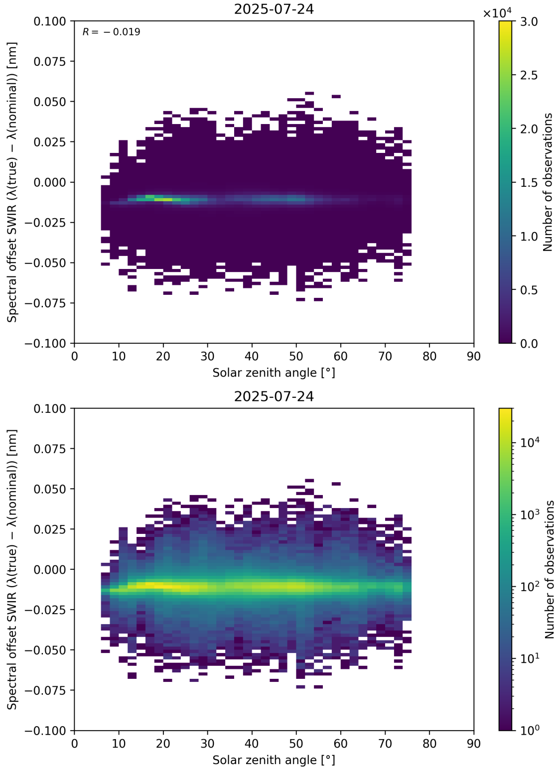
Figure 104: Scatter density plot of “Solar zenith angle” against “Spectral offset SWIR ( \lambda_{\text{true}} - \lambda_{\text{nominal}} )” for 2025-07-24 to 2025-07-25.
