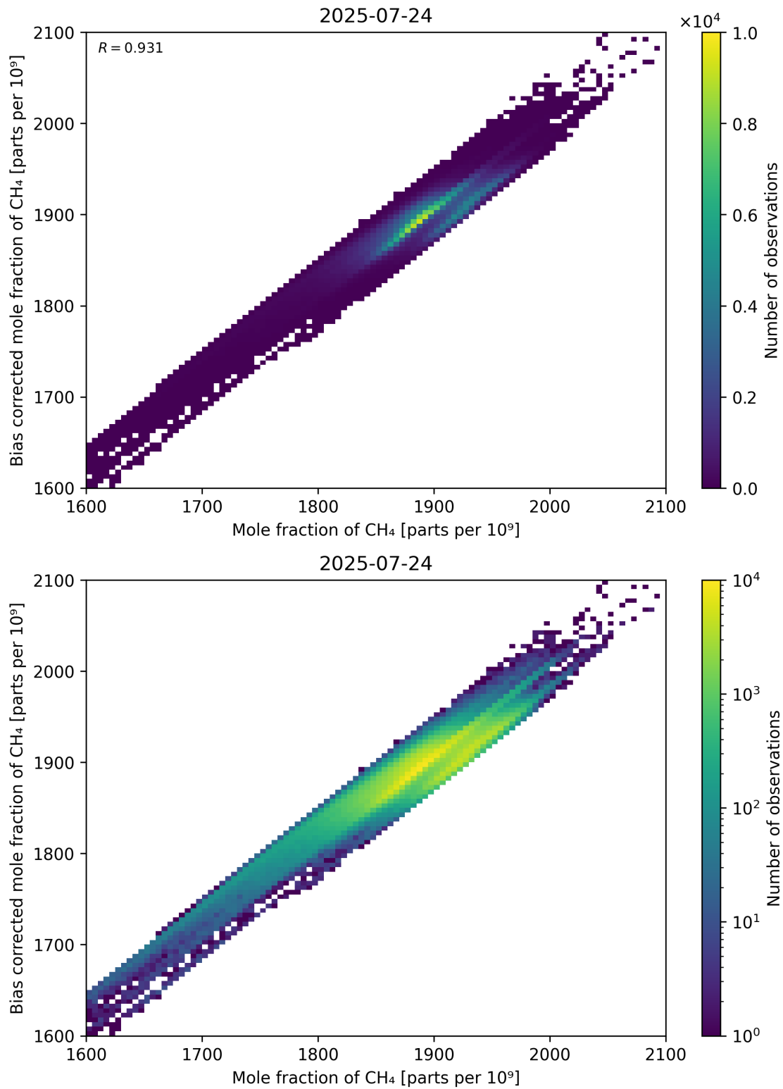
Figure 74: Scatter density plot of “Mole fraction of \text{CH}_4 ” against “Bias corrected mole fraction of \text{CH}_4 ” for 2025-07-24 to 2025-07-25.
