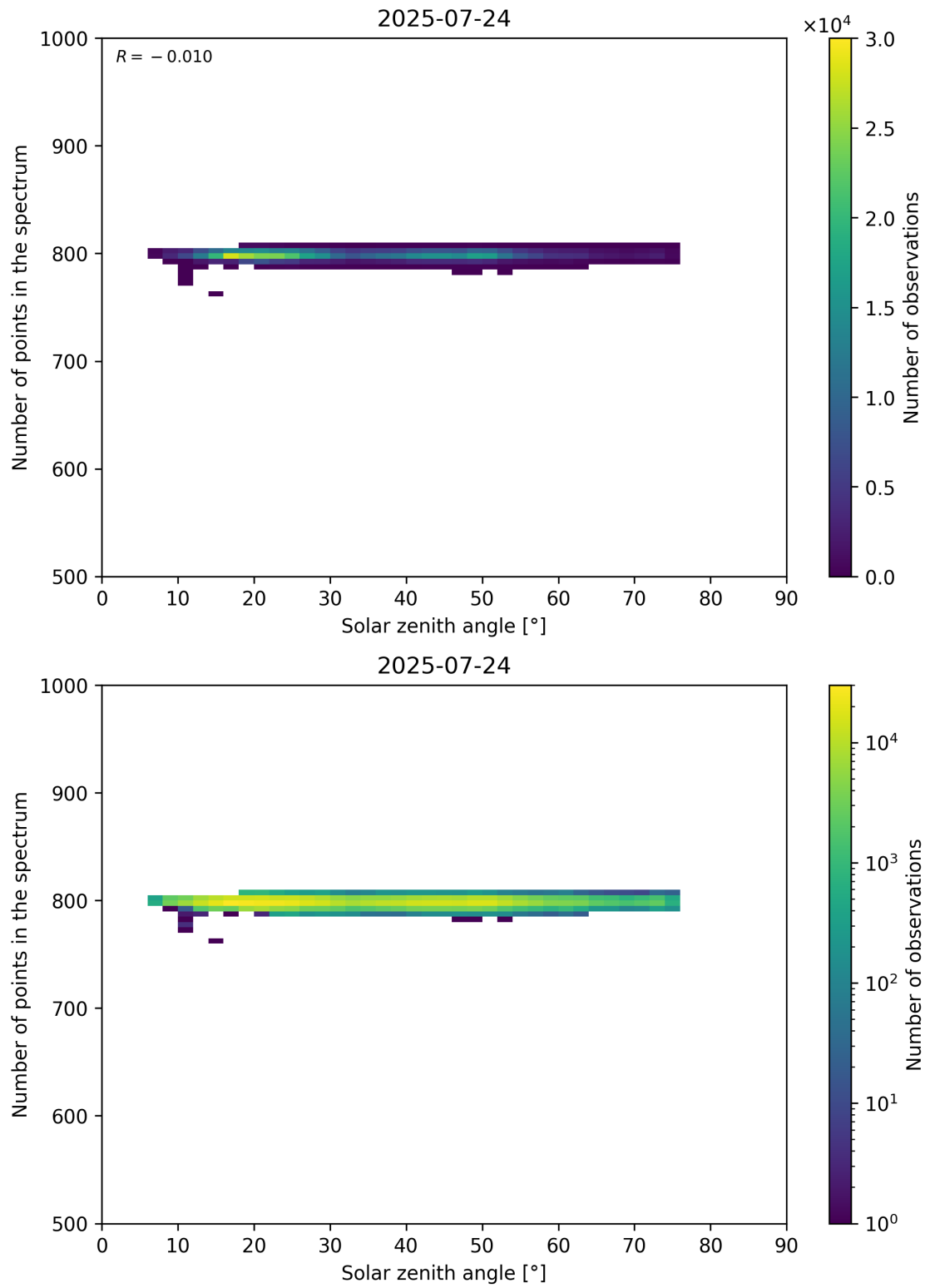
Figure 103: Scatter density plot of “Solar zenith angle” against “Number of points in the spectrum” for 2025-07-24 to 2025-07-25.
