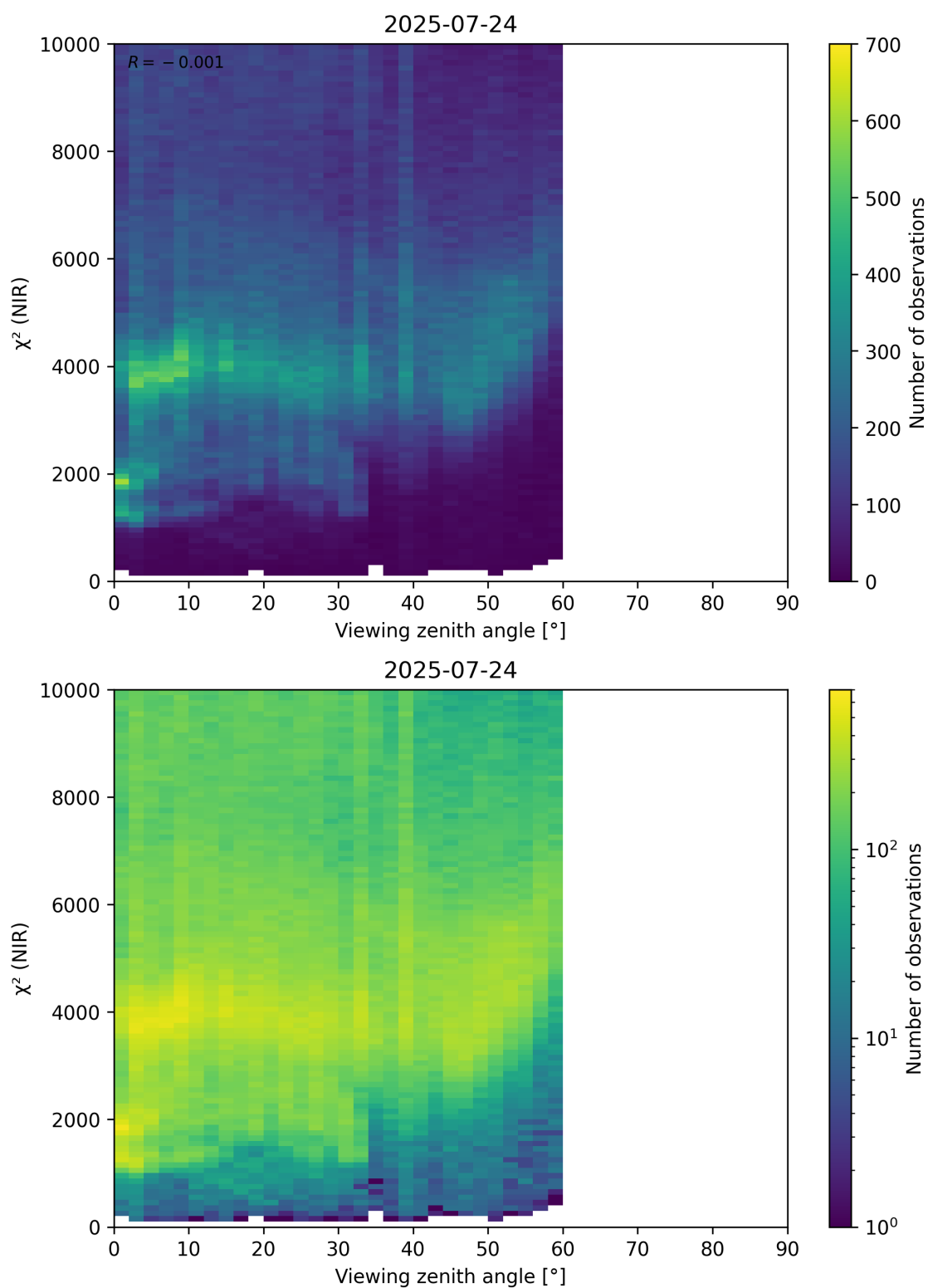
Figure 105: Scatter density plot of “Viewing zenith angle” against “ \chi^2 (NIR)” for 2025-07-24 to 2025-07-25.
