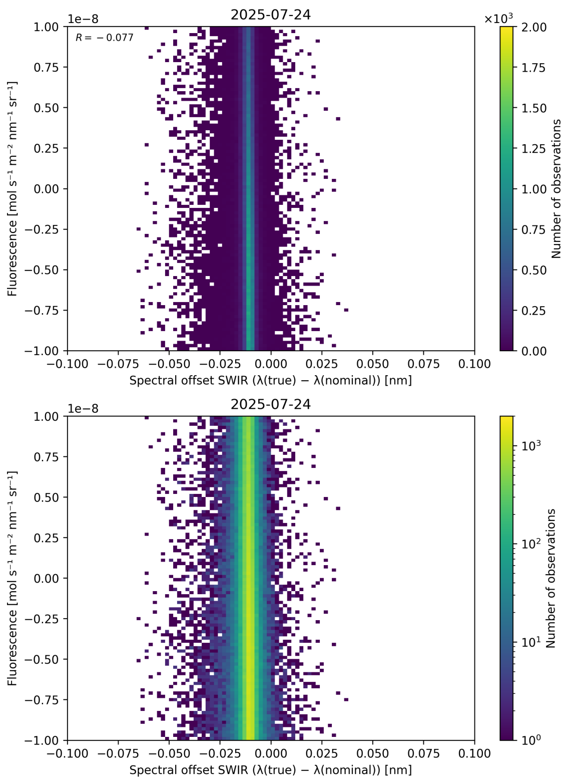
Figure 120: Scatter density plot of “Spectral offset SWIR ( \lambda_{\text{true}} - \lambda_{\text{nominal}} )” against “Fluorescence” for 2025-07-24 to 2025-07-25.
