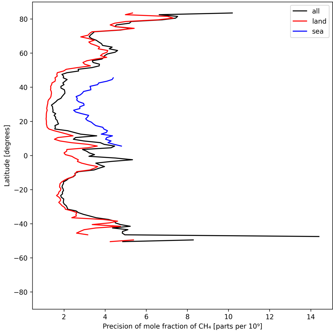
Figure 13: Zonal average of “Precision of mole fraction of CH 4 ” for 2025-07-24 to 2025-07-25.
