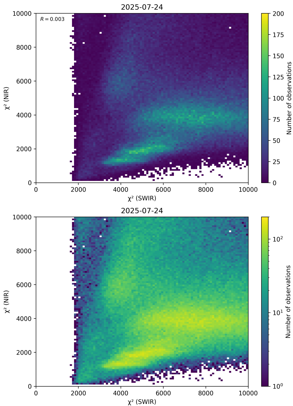
Figure 47: Scatter density plot of “ \chi^2 (SWIR)” against “ \chi^2 (NIR)” for 2025-07-24 to 2025-07-25.
