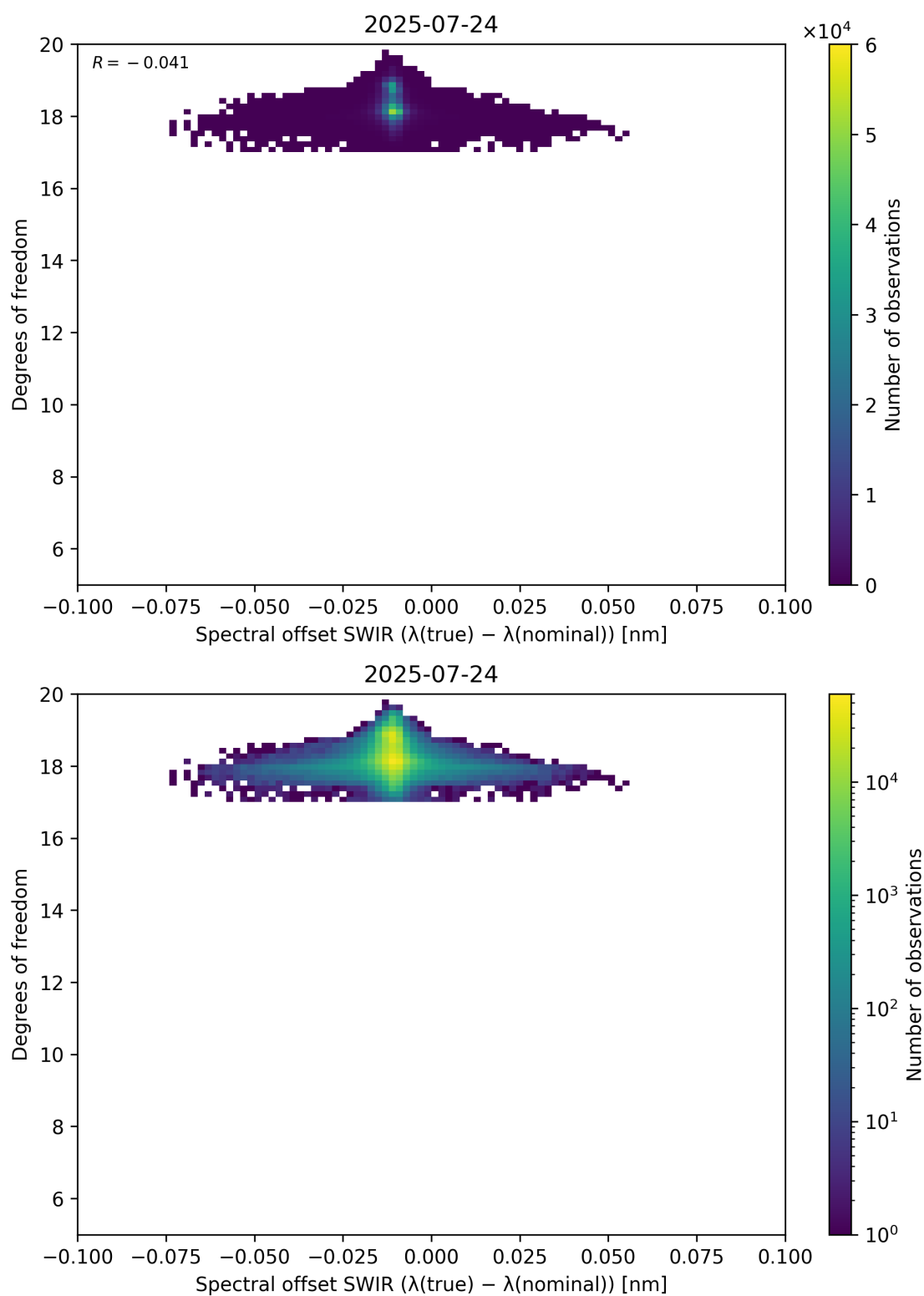
Figure 119: Scatter density plot of “Spectral offset SWIR ( \lambda_{\text{true}} - \lambda_{\text{nominal}} )” against “Degrees of freedom” for 2025-07-24 to 2025-07-25.
