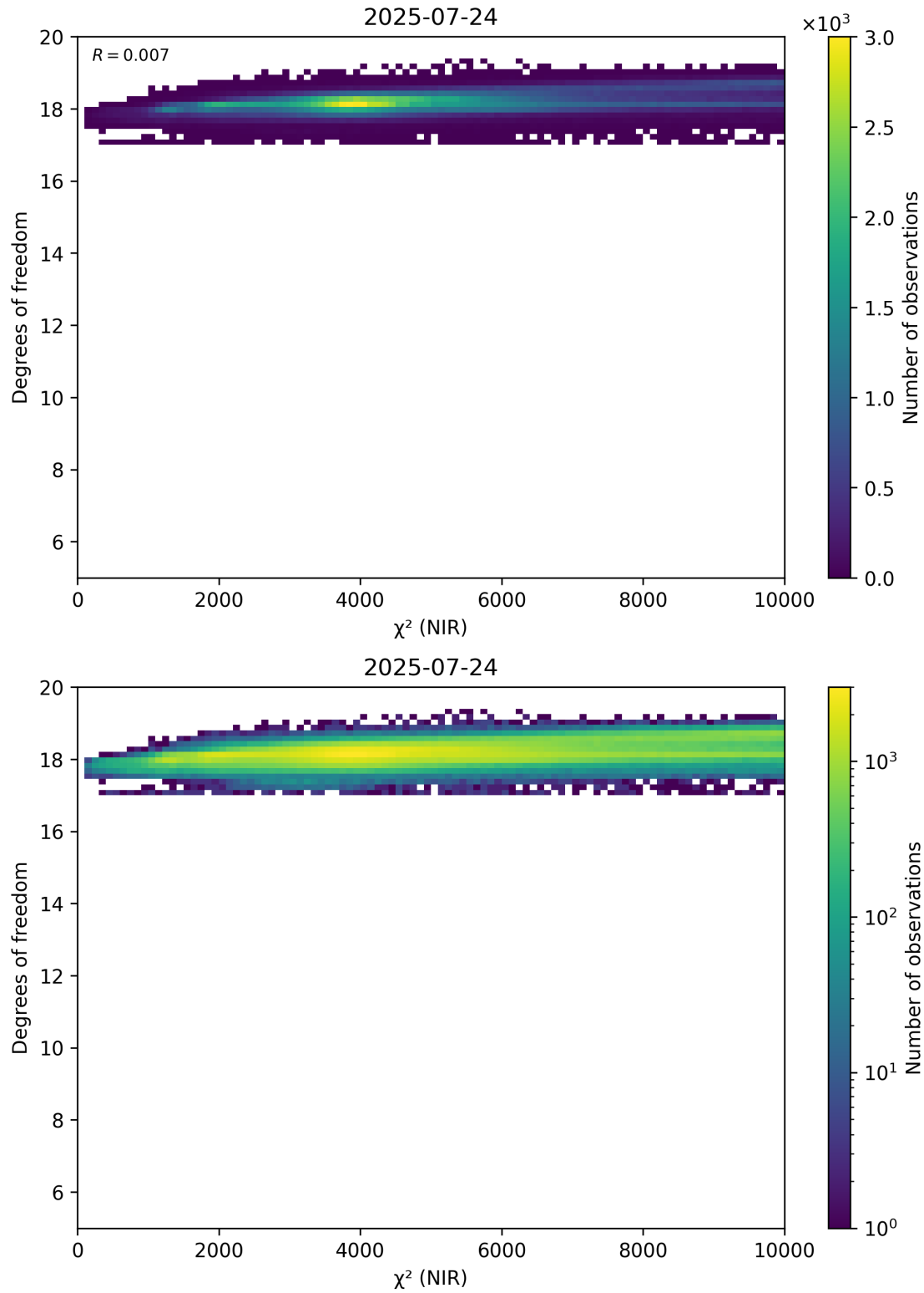
Figure 44: Scatter density plot of “ \chi^2 (NIR)” against “Degrees of freedom” for 2025-07-24 to 2025-07-25.
