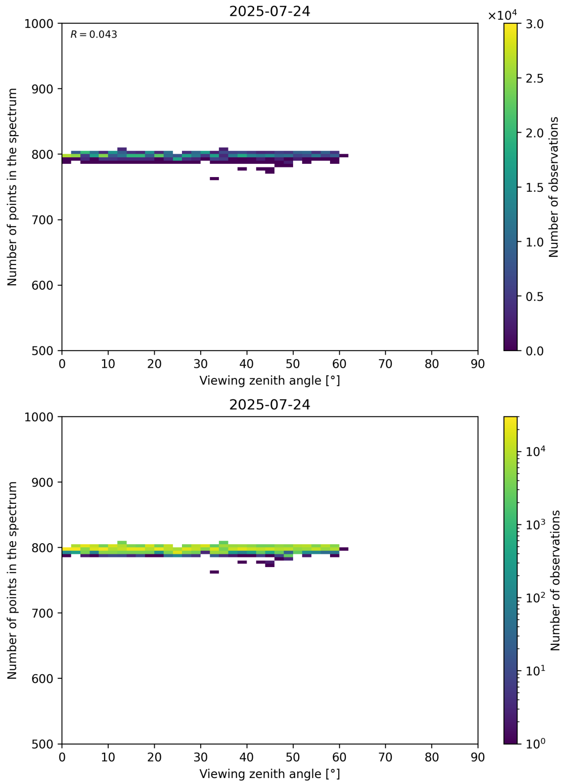
Figure 114: Scatter density plot of “Viewing zenith angle” against “Number of points in the spectrum” for 2025-07-24 to 2025-07-25.
