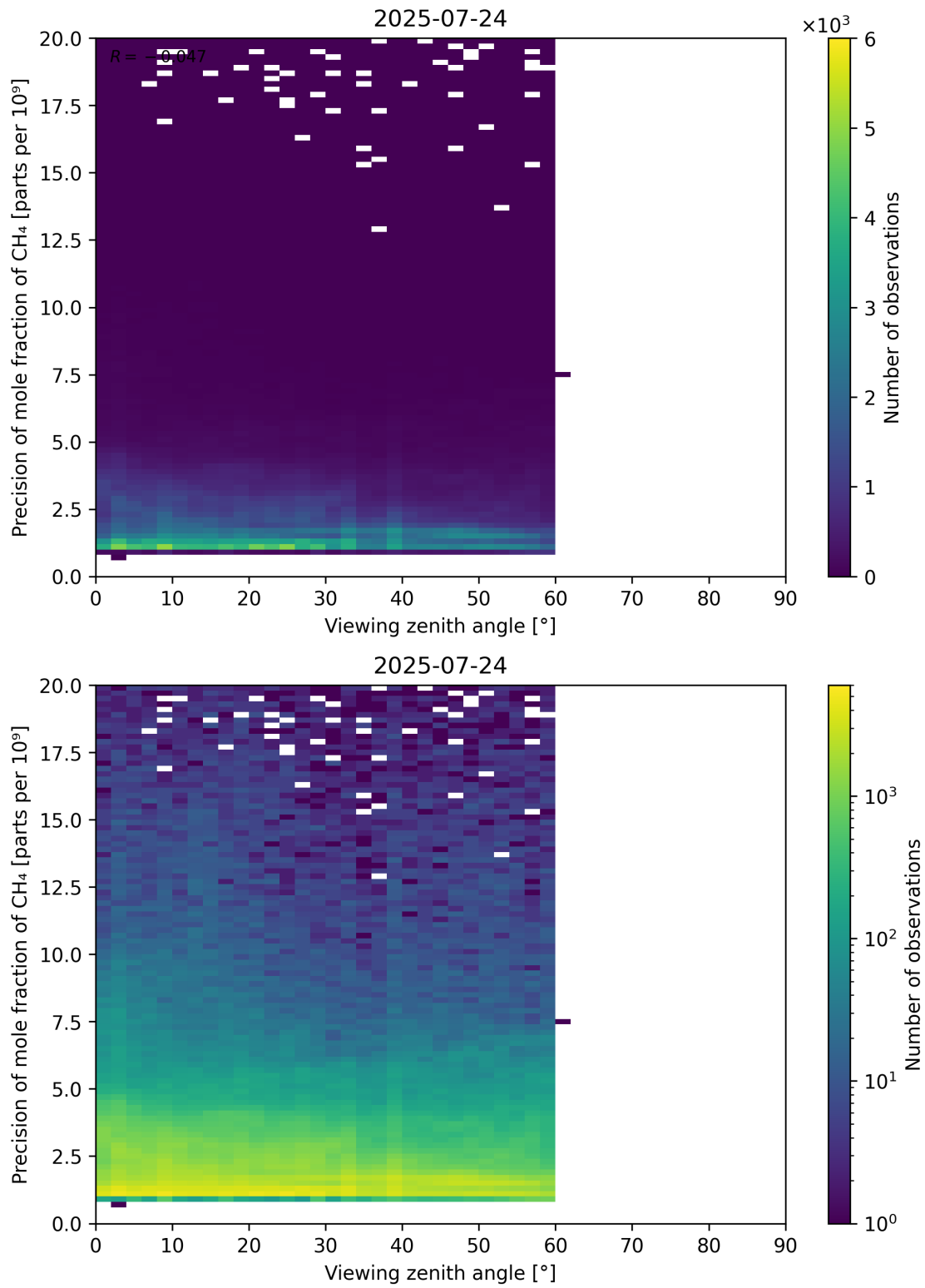
Figure 112: Scatter density plot of “Viewing zenith angle” against “Precision of mole fraction of CH 4 ” for 2025-07-24 to 2025-07-25.
