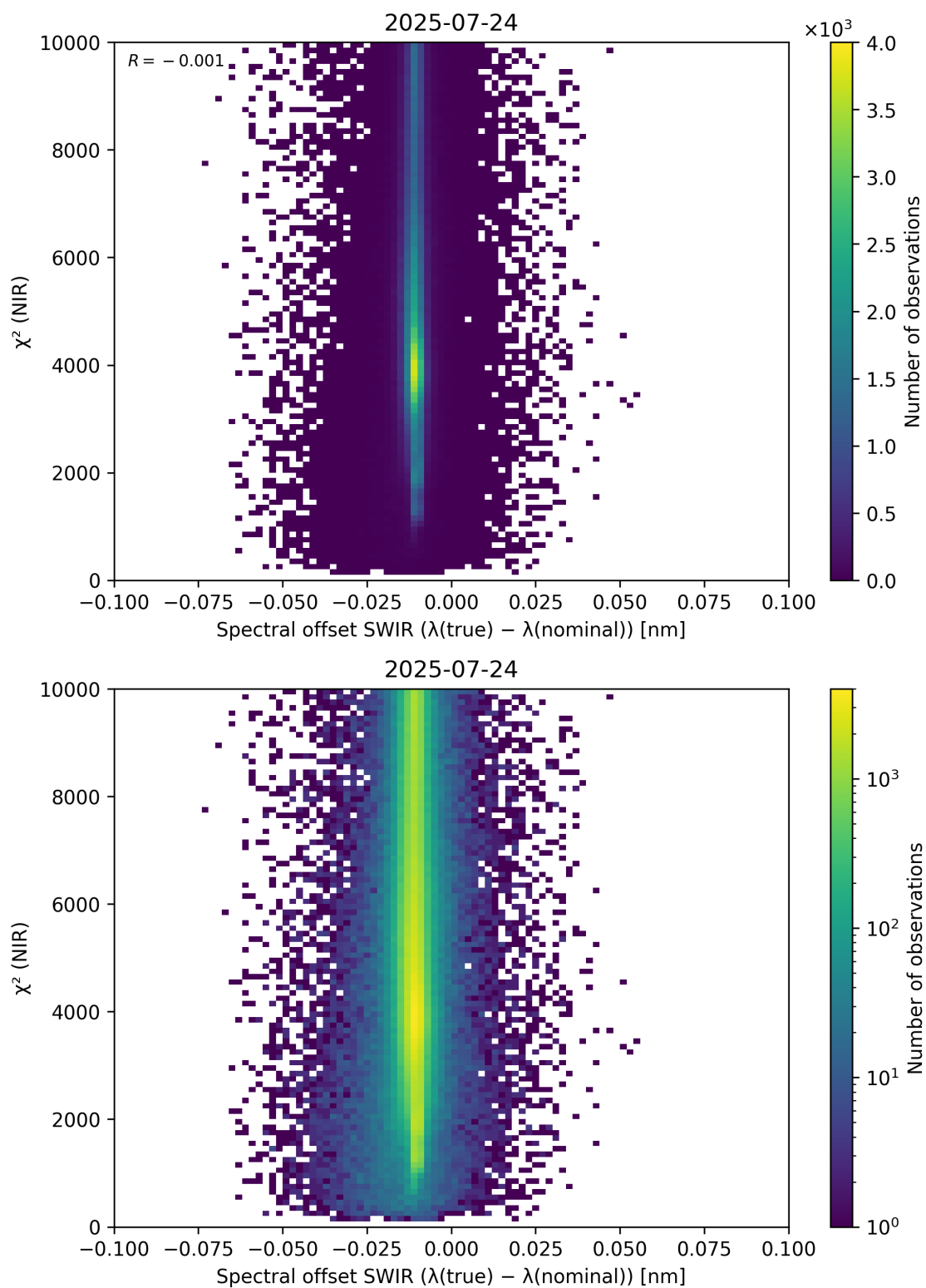
Figure 117: Scatter density plot of “Spectral offset SWIR ( \lambda_{\text{true}} - \lambda_{\text{nominal}} )” against “ \chi^2 (NIR)” for 2025-07-24 to 2025-07-25.
