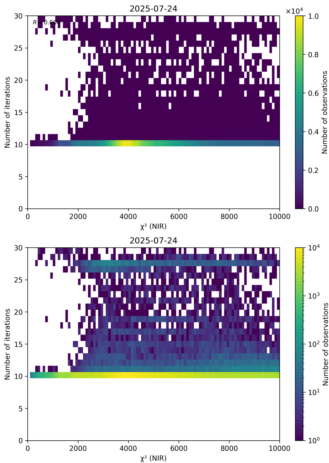
Figure 46: Scatter density plot of “ \chi^2 (NIR)” against “Number of iterations” for 2025-07-24 to 2025-07-25.
