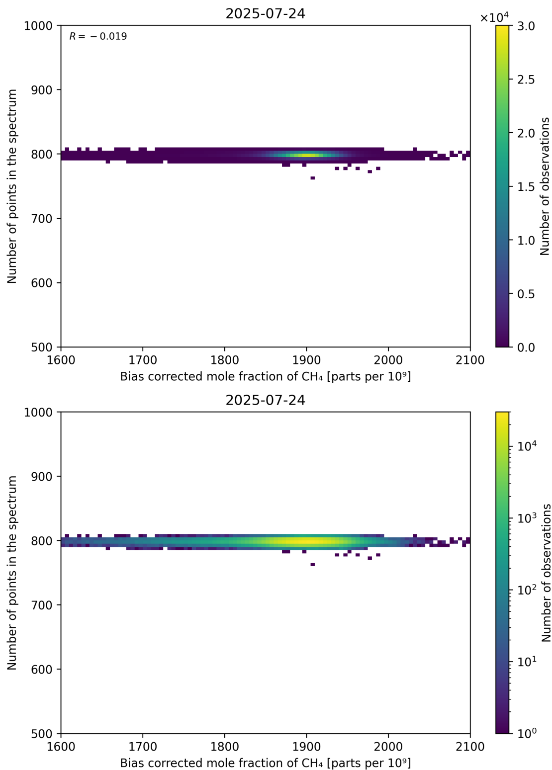
Figure 68: Scatter density plot of “Bias corrected mole fraction of CH 4 ” against “Number of points in the spectrum” for 2025-07-24 to 2025-07-25.
