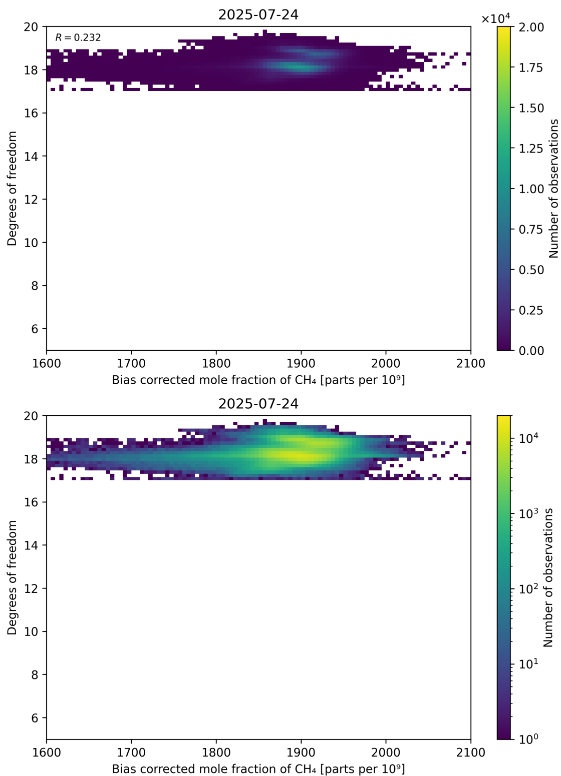
Figure 65: Scatter density plot of “Bias corrected mole fraction of CH 4 ” against “Degrees of freedom” for 2025-07-24 to 2025-07-25.
