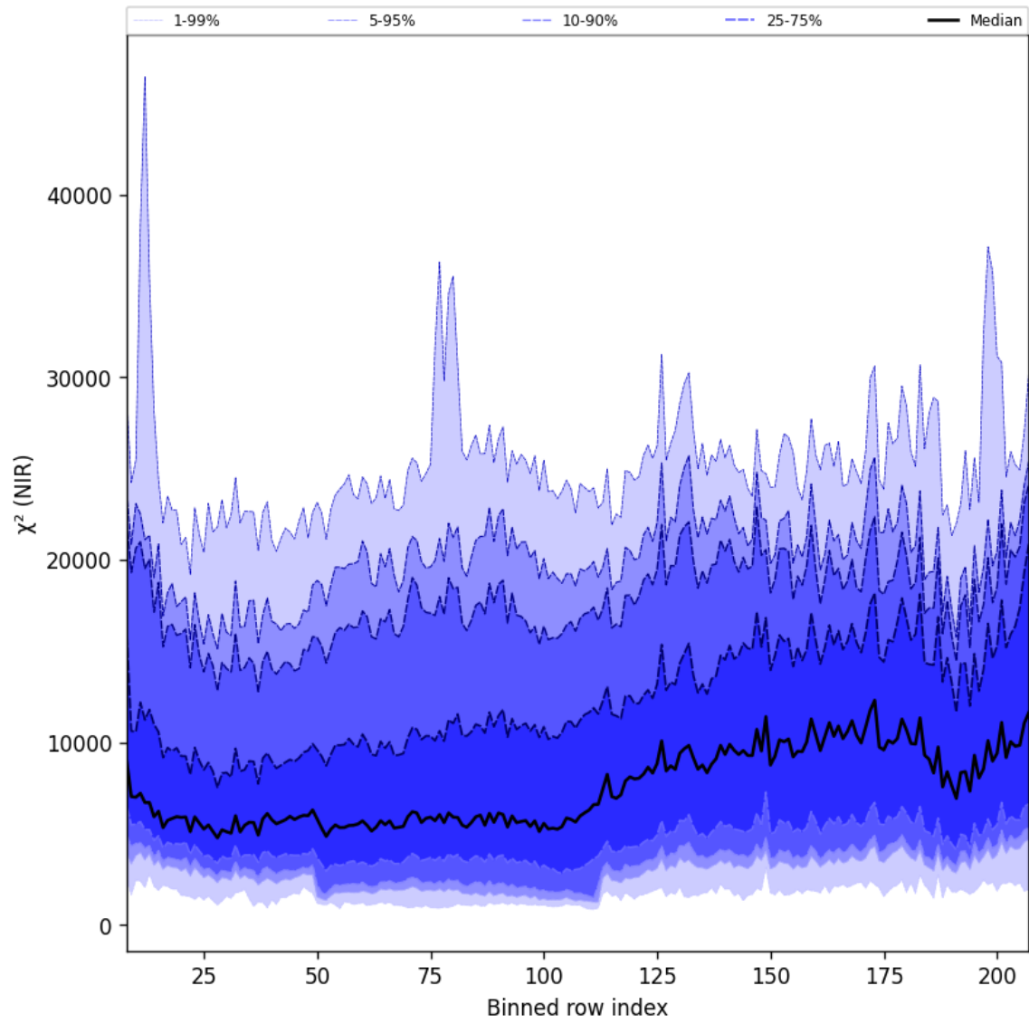
Figure 40: Along track statistics of “ \chi^2 (NIR)” for 2025-07-24 to 2025-07-25
