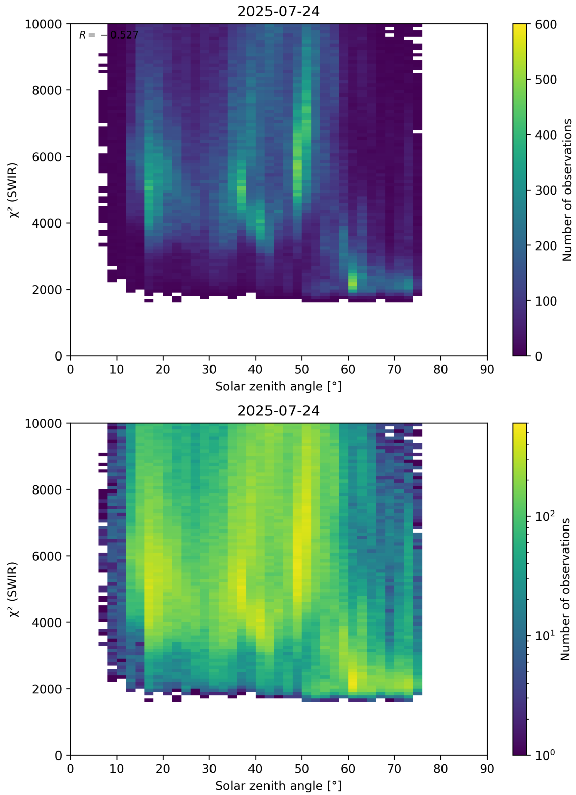
Figure 95: Scatter density plot of “Solar zenith angle” against “ \chi^2 (SWIR)” for 2025-07-24 to 2025-07-25.
