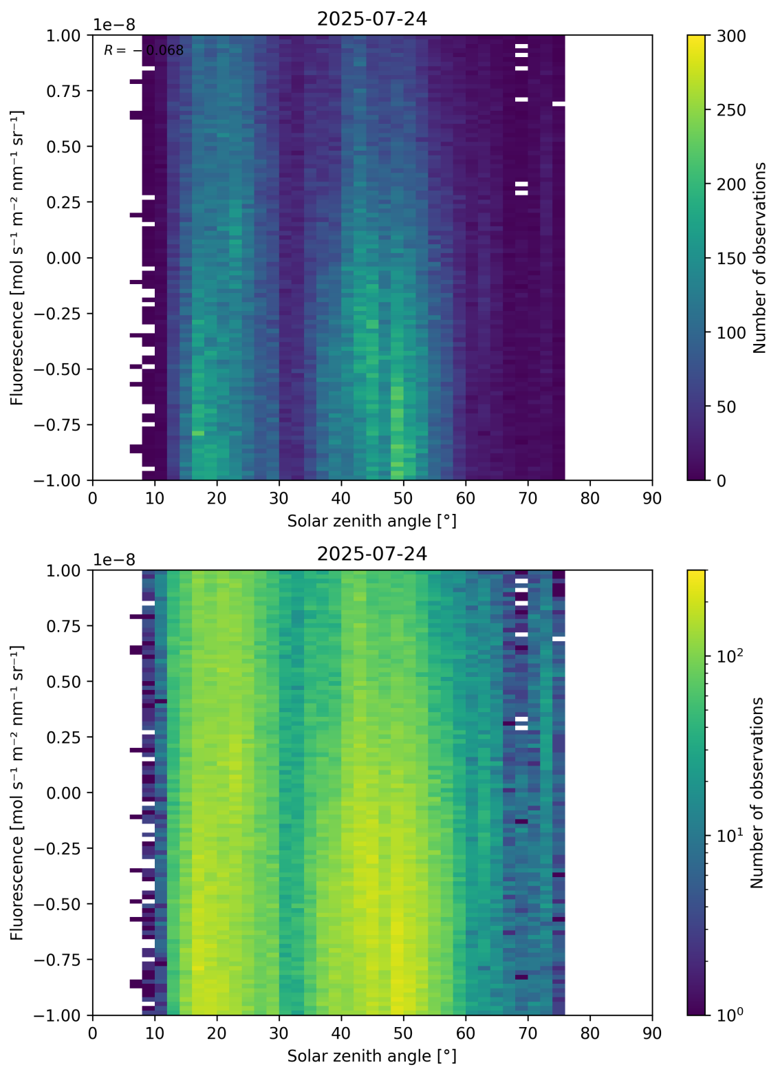
Figure 97: Scatter density plot of “Solar zenith angle” against “Fluorescence” for 2025-07-24 to 2025-07-25.
