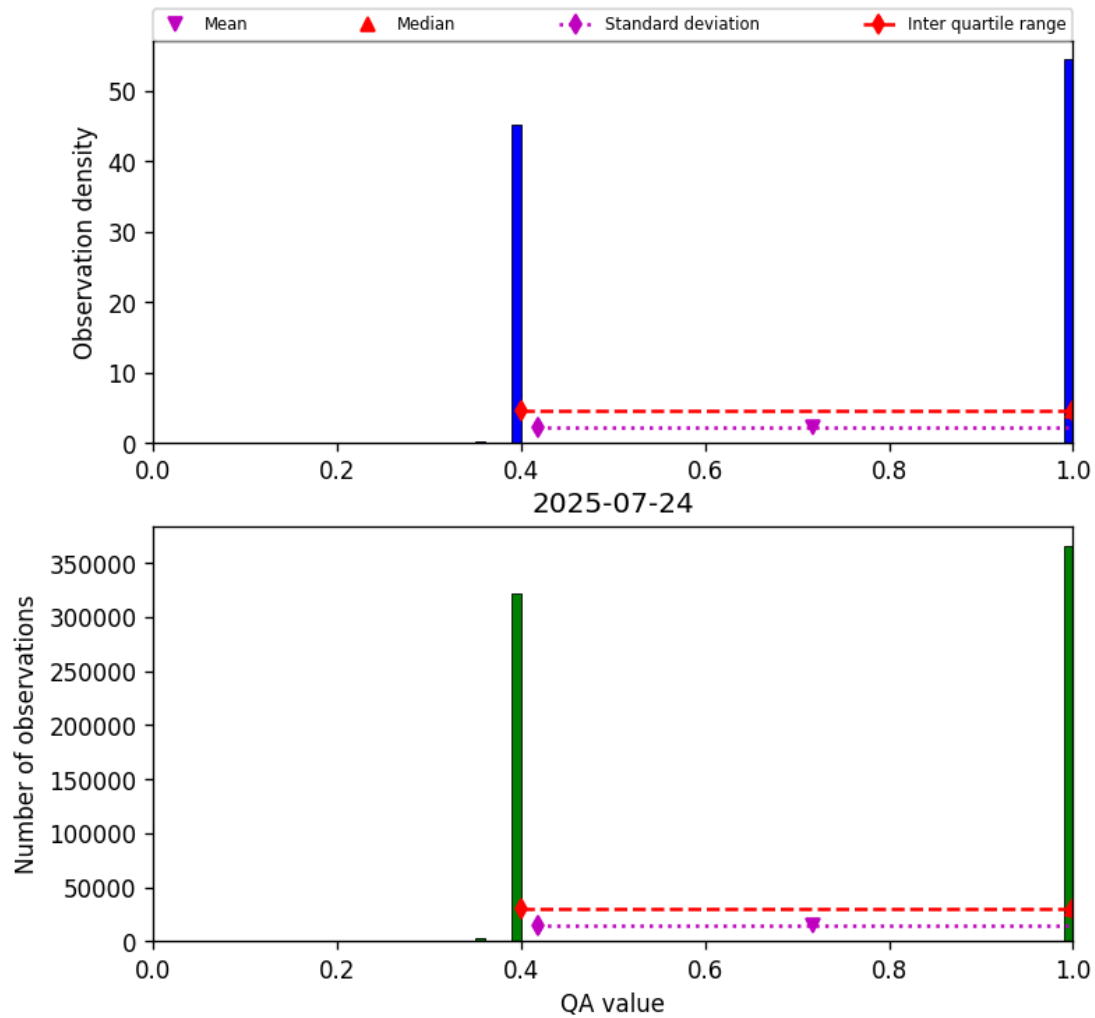
Figure 22: Histogram of “QA value” for 2025-07-24 to 2025-07-25
