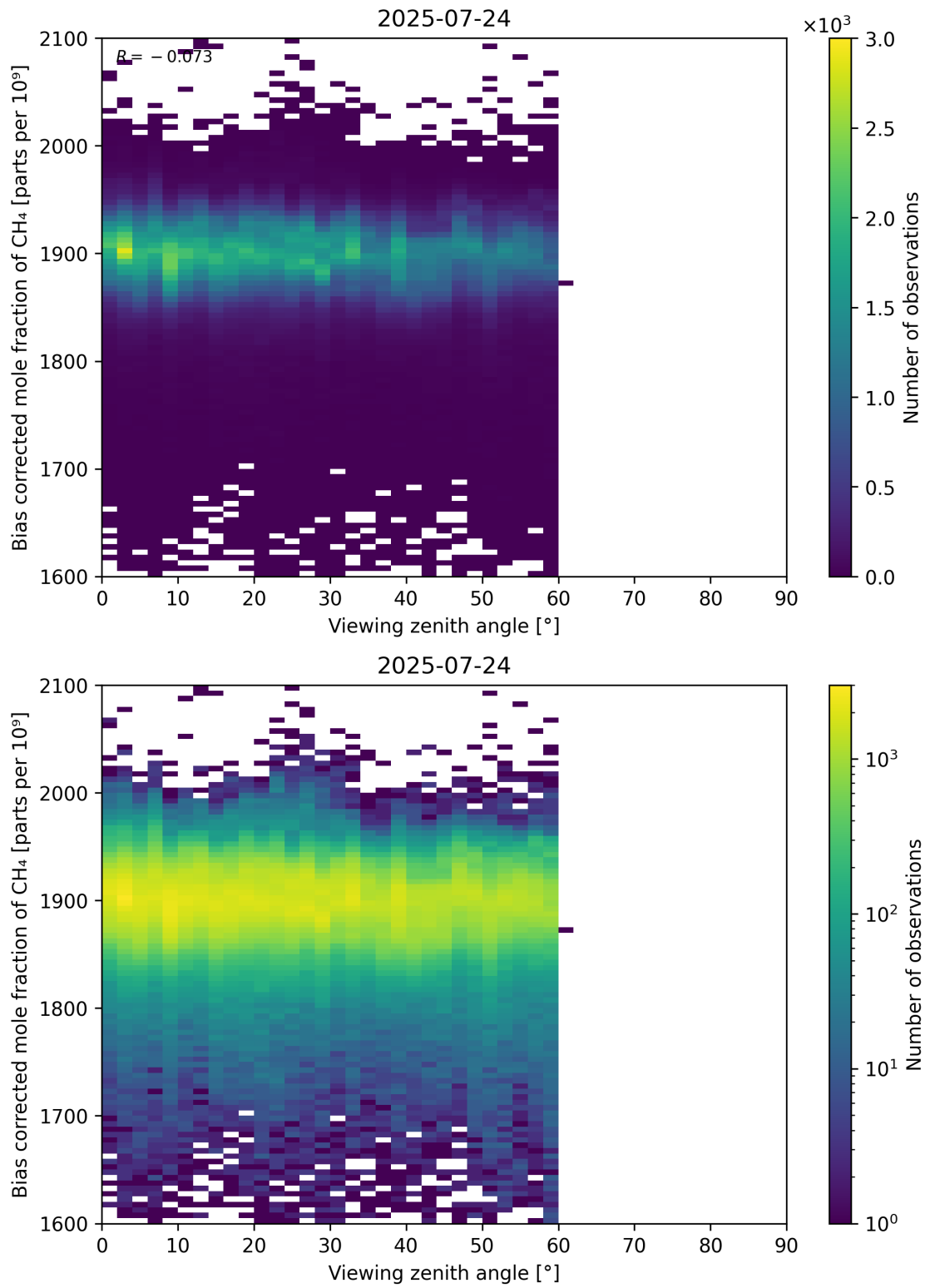
Figure 111: Scatter density plot of “Viewing zenith angle” against “Bias corrected mole fraction of CH 4 ” for 2025-07-24 to 2025-07-25.
