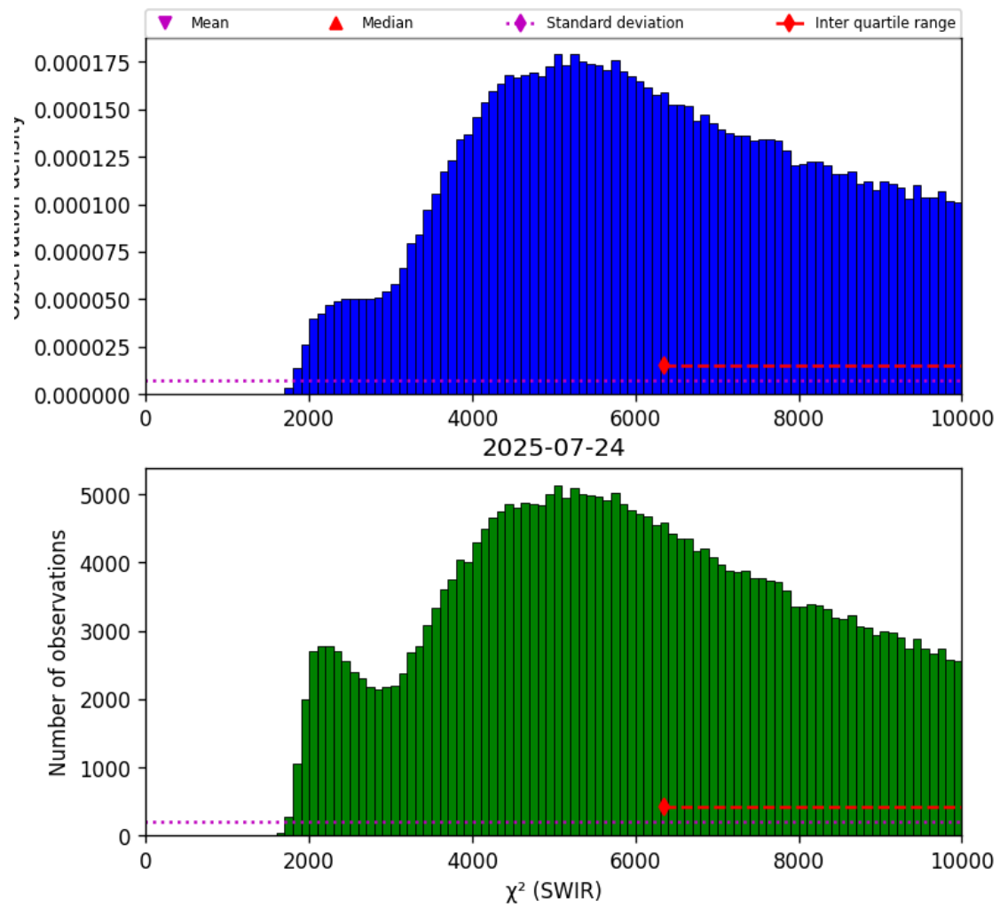
Figure 28: Histogram of “ \chi^2 (SWIR)” for 2025-07-24 to 2025-07-25
