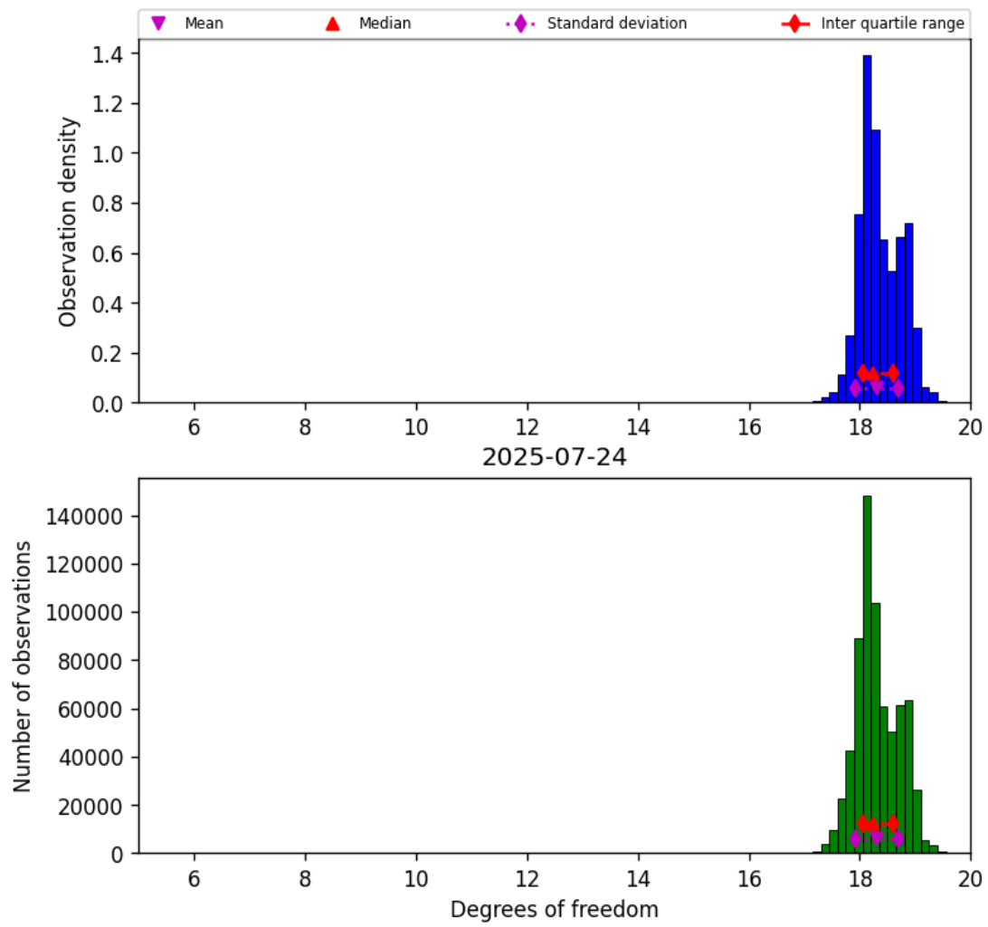
Figure 30: Histogram of “Degrees of freedom” for 2025-07-24 to 2025-07-25
