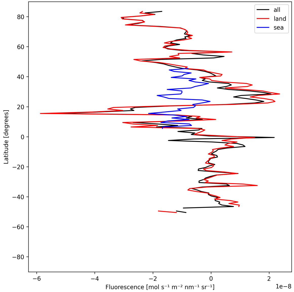
Figure 21: Zonal average of “Fluorescence” for 2025-07-24 to 2025-07-25.
