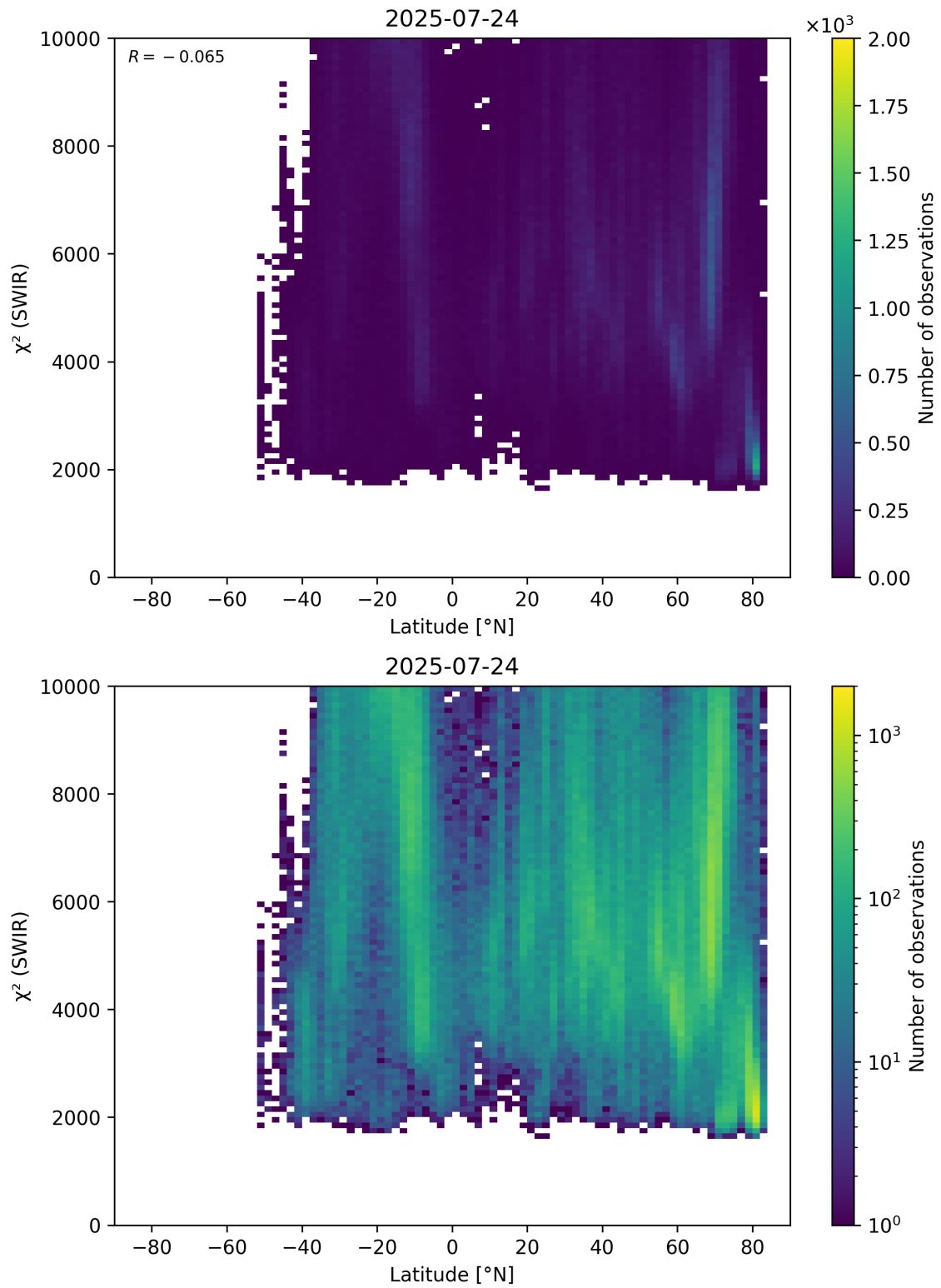
Figure 54: Scatter density plot of “Latitude” against “ \chi^2 (SWIR)” for 2025-07-24 to 2025-07-25.
