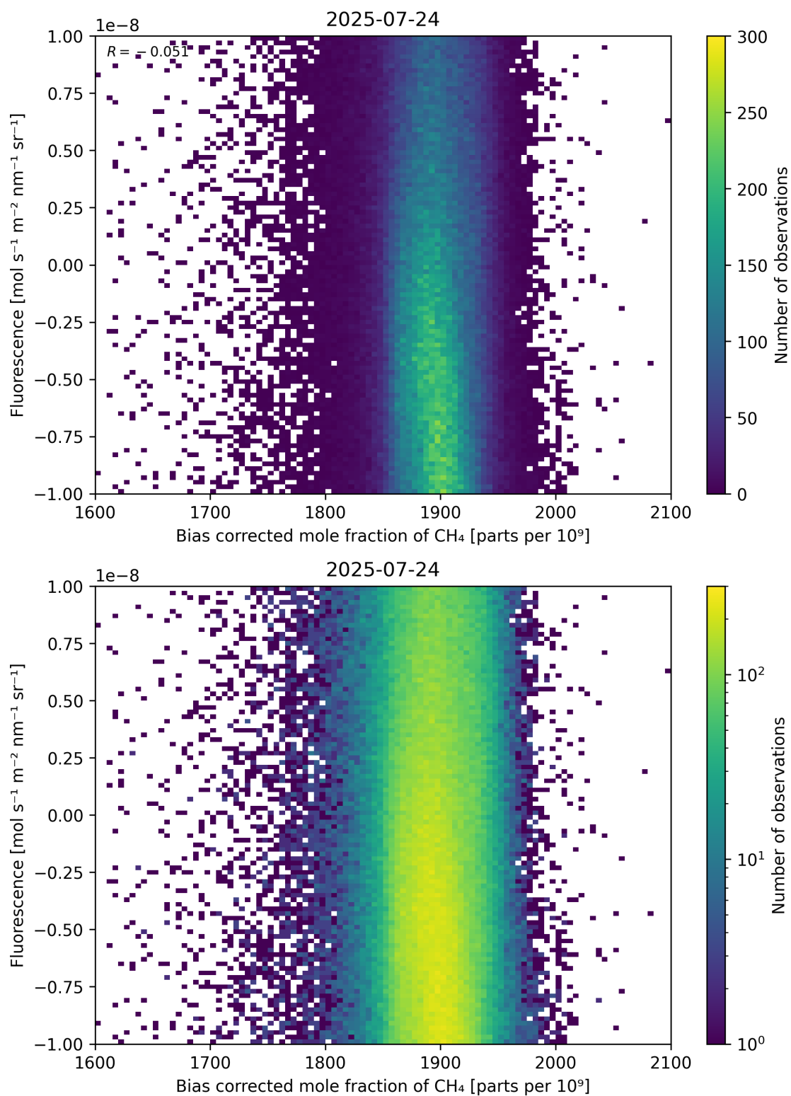
Figure 66: Scatter density plot of “Bias corrected mole fraction of \text{CH}_4 ” against “Fluorescence” for 2025-07-24 to 2025-07-25.
