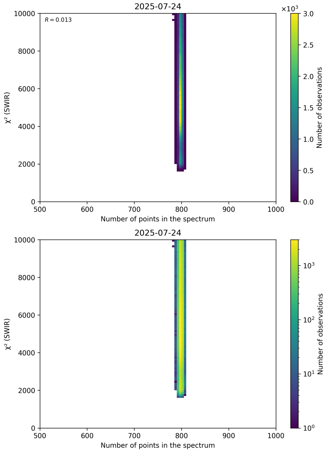
Figure 89: Scatter density plot of “Number of points in the spectrum” against “ \chi^2 (SWIR)” for 2025-07-24 to 2025-07-25.
