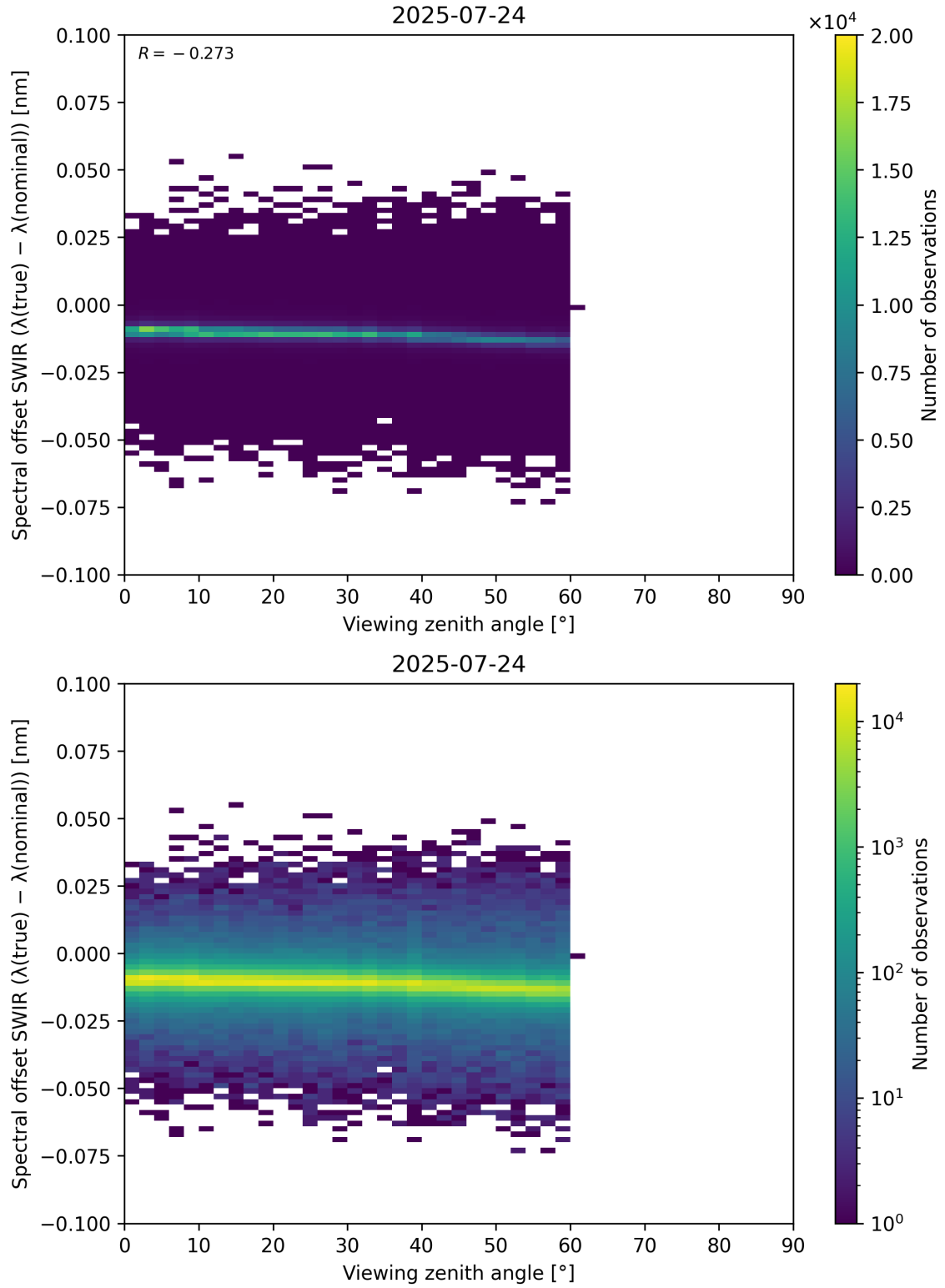
Figure 116: Scatter density plot of “Viewing zenith angle” against “Spectral offset SWIR ( \lambda_{\text{true}} - \lambda_{\text{nominal}} )” for 2025-07-24 to 2025-07-25.
