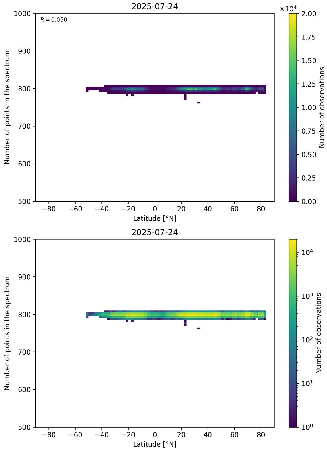
Figure 61: Scatter density plot of “Latitude” against “Number of points in the spectrum” for 2025-07-24 to 2025-07-25.
