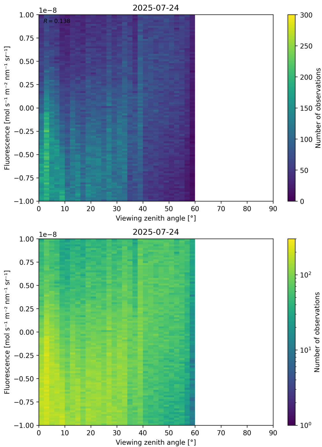
Figure 108: Scatter density plot of “Viewing zenith angle” against “Fluorescence” for 2025-07-24 to 2025-07-25.
