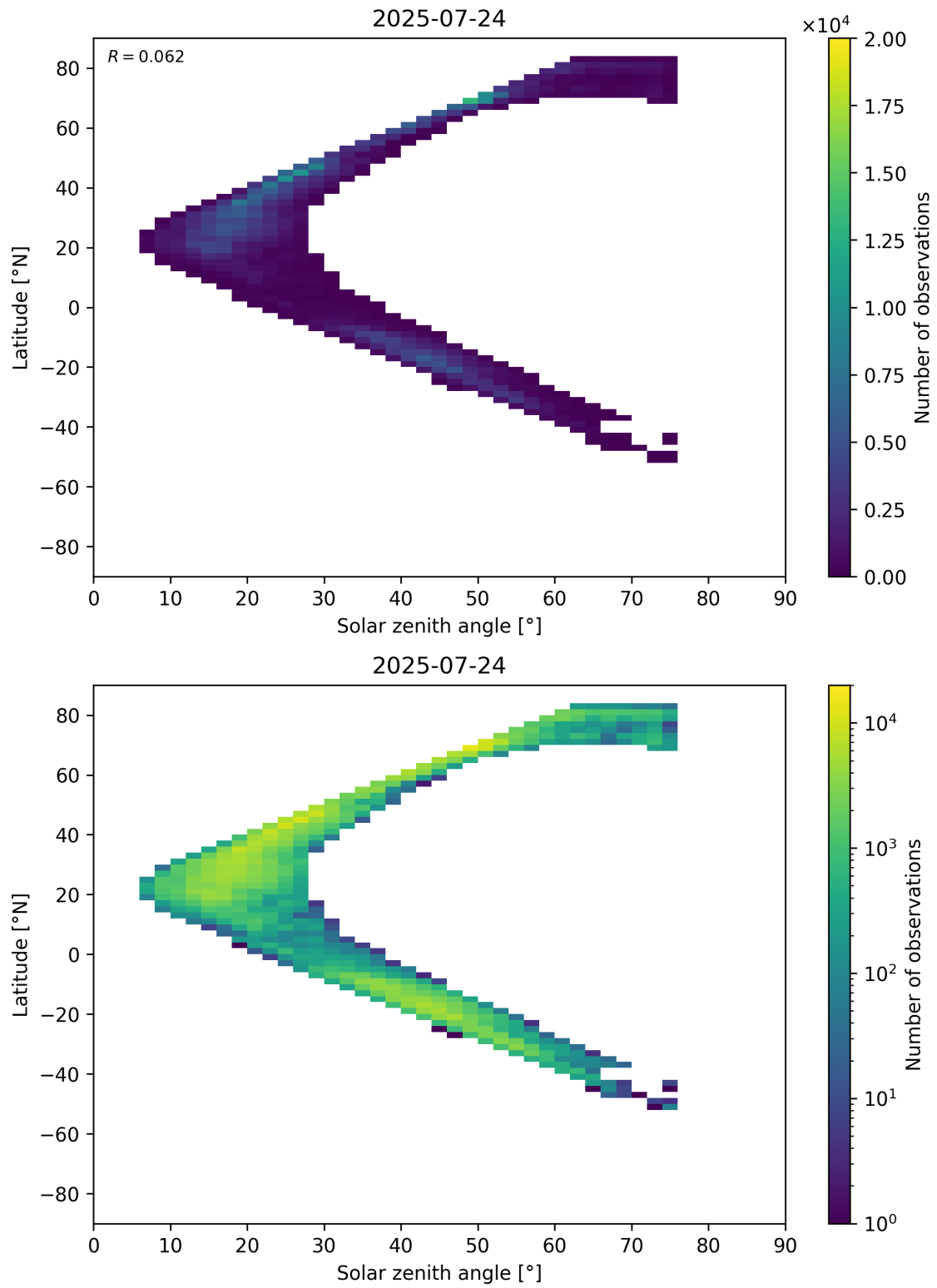
Figure 98: Scatter density plot of “Solar zenith angle” against “Latitude” for 2025-07-24 to 2025-07-25.
