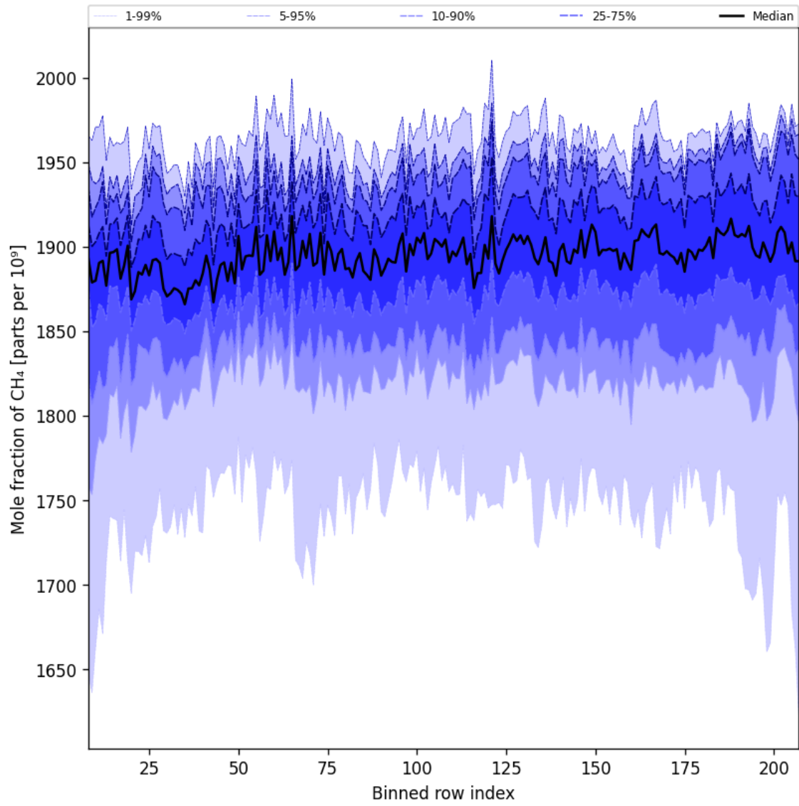
Figure 34: Along track statistics of “Mole fraction of CH 4 ” for 2025-07-24 to 2025-07-25
