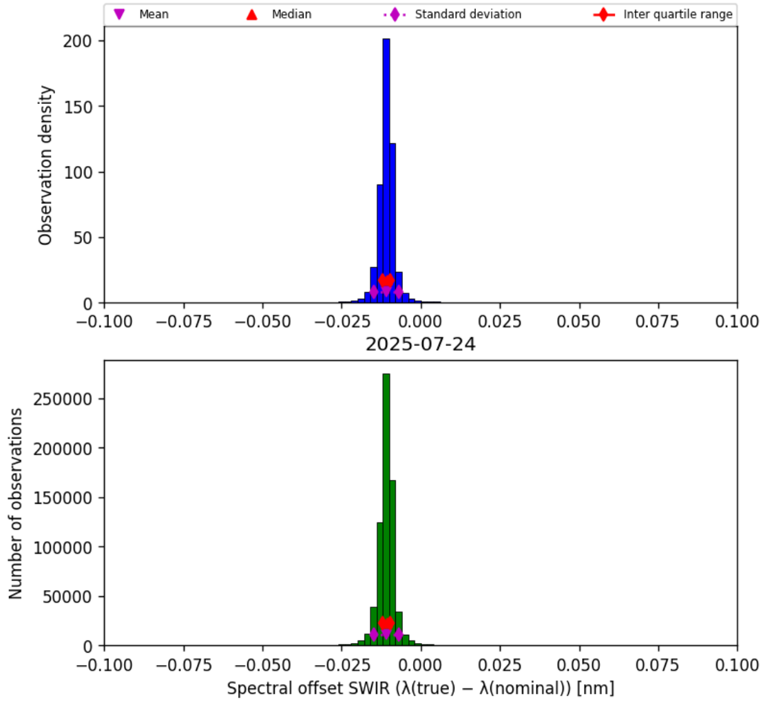
Figure 27: Histogram of “Spectral offset SWIR ( \lambda_{\text{true}} - \lambda_{\text{nominal}} )” for 2025-07-24 to 2025-07-25
