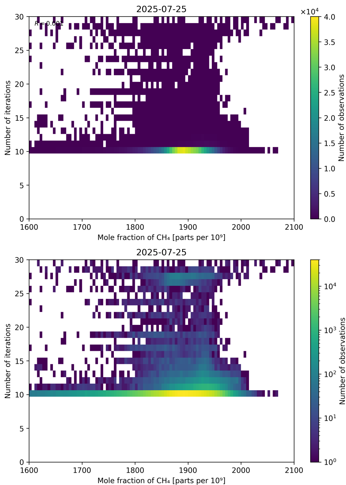
Figure 76: Scatter density plot of “Mole fraction of CH 4 ” against “Number of iterations” for 2025-07-24 to 2025-07-26.
