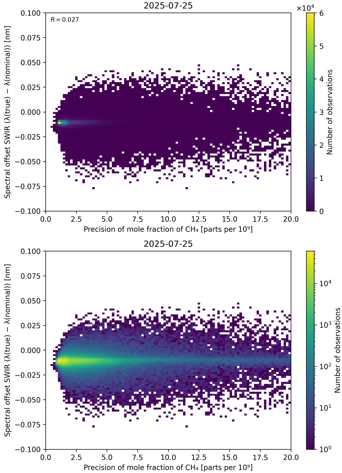
Figure 85: Scatter density plot of “Precision of mole fraction of CH 4 ” against “Spectral offset SWIR ( \lambda_{\text{true}} - \lambda_{\text{nominal}} )” for 2025-07-24 to 2025-07-26.
