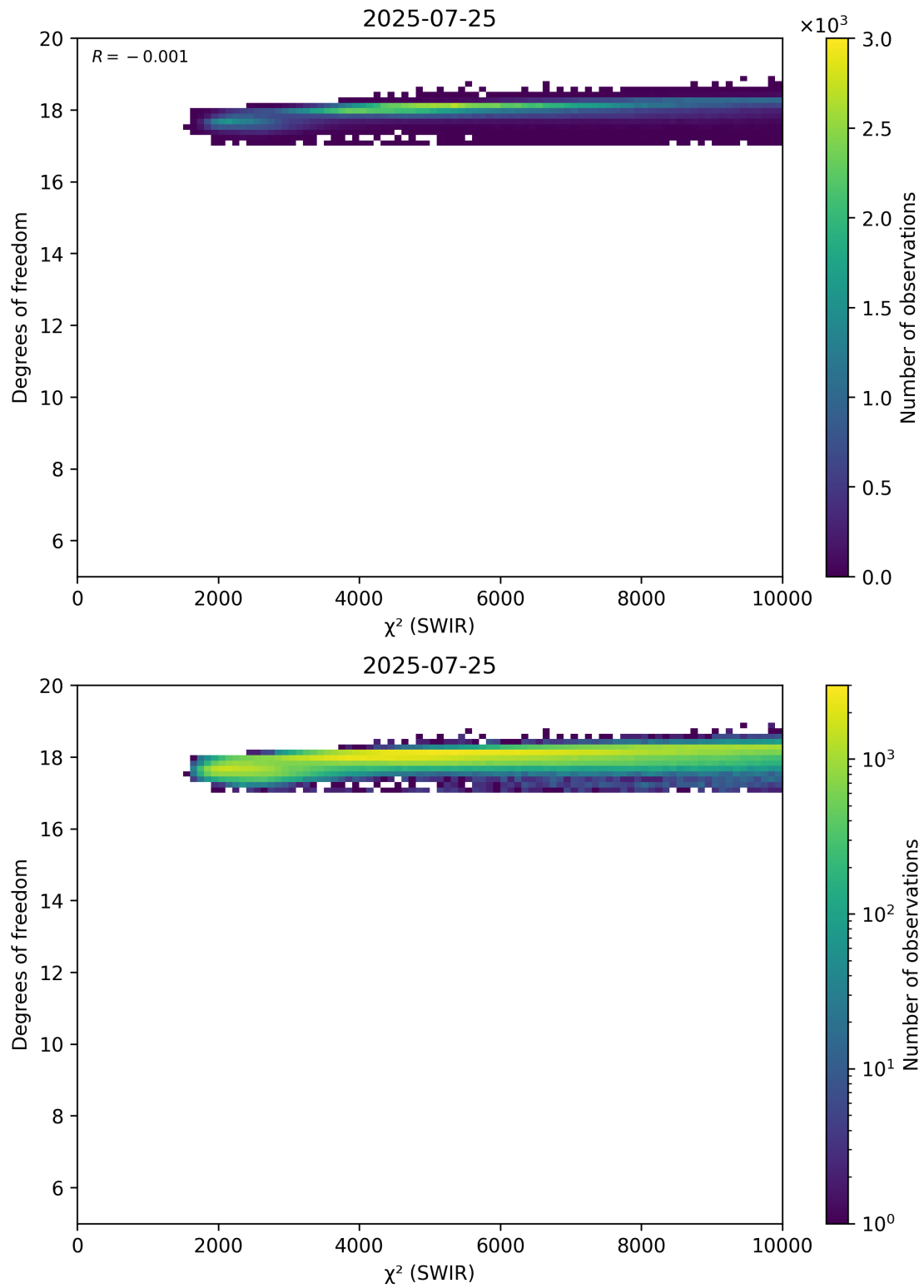
Figure 48: Scatter density plot of “ \chi^2 (SWIR)” against “Degrees of freedom” for 2025-07-24 to 2025-07-26.
