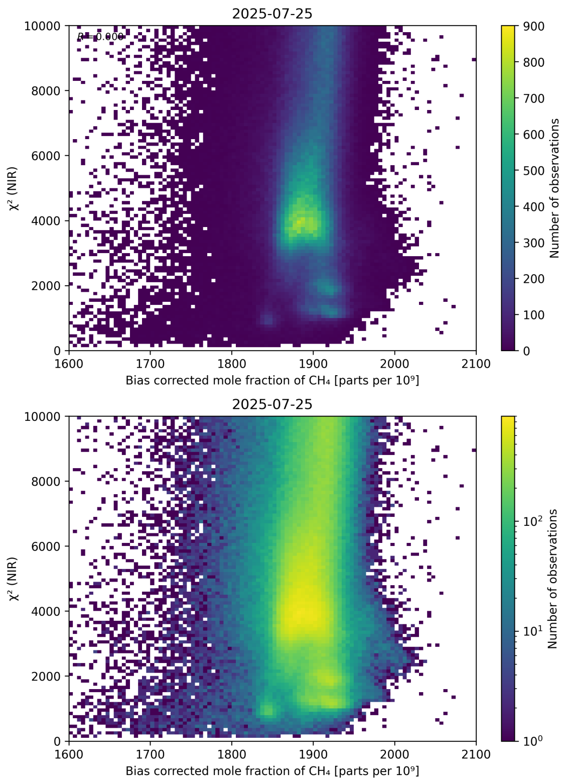
Figure 63: Scatter density plot of “Bias corrected mole fraction of \text{CH}_4 ” against “ \chi^2 (NIR)” for 2025-07-24 to 2025-07-26.
