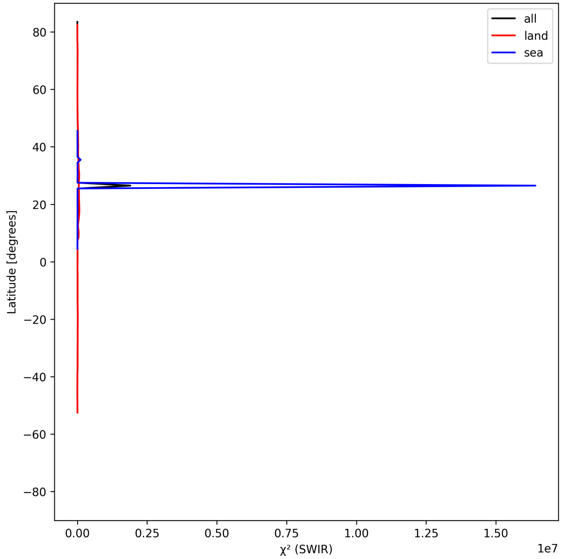
Figure 17: Zonal average of “ \chi^2 (SWIR)” for 2025-07-24 to 2025-07-26.
