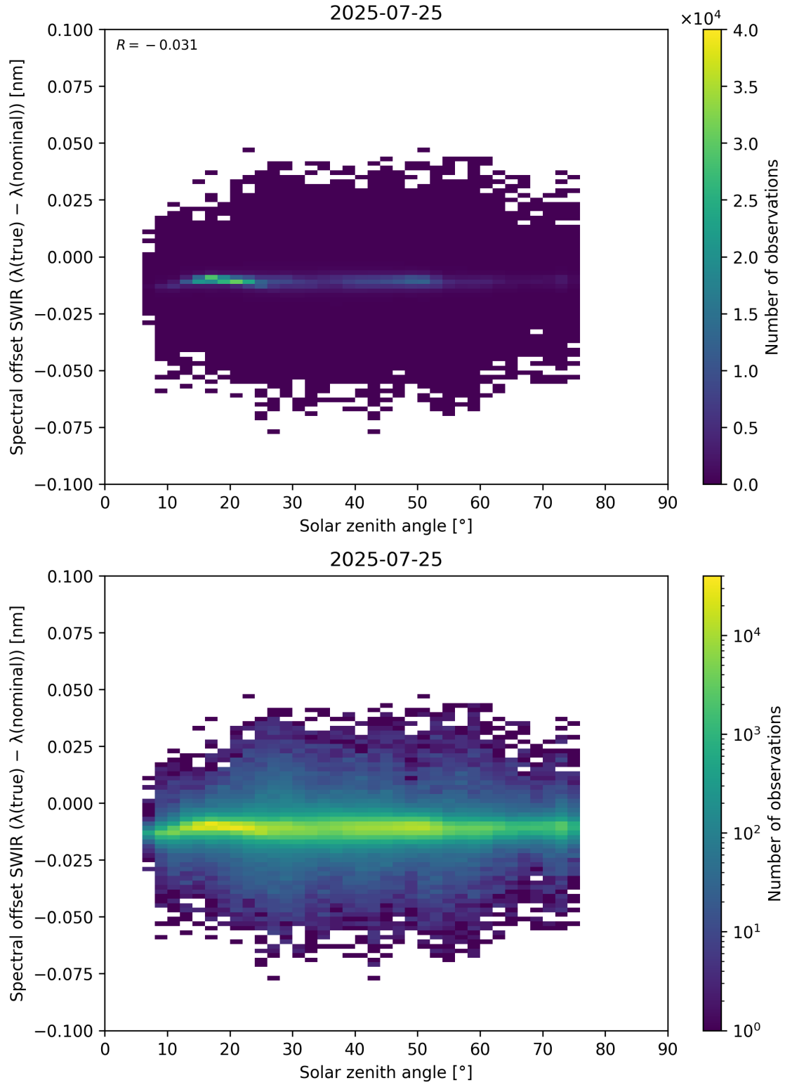
Figure 104: Scatter density plot of “Solar zenith angle” against “Spectral offset SWIR ( \lambda_{\text{true}} - \lambda_{\text{nominal}} )” for 2025-07-24 to 2025-07-26.
