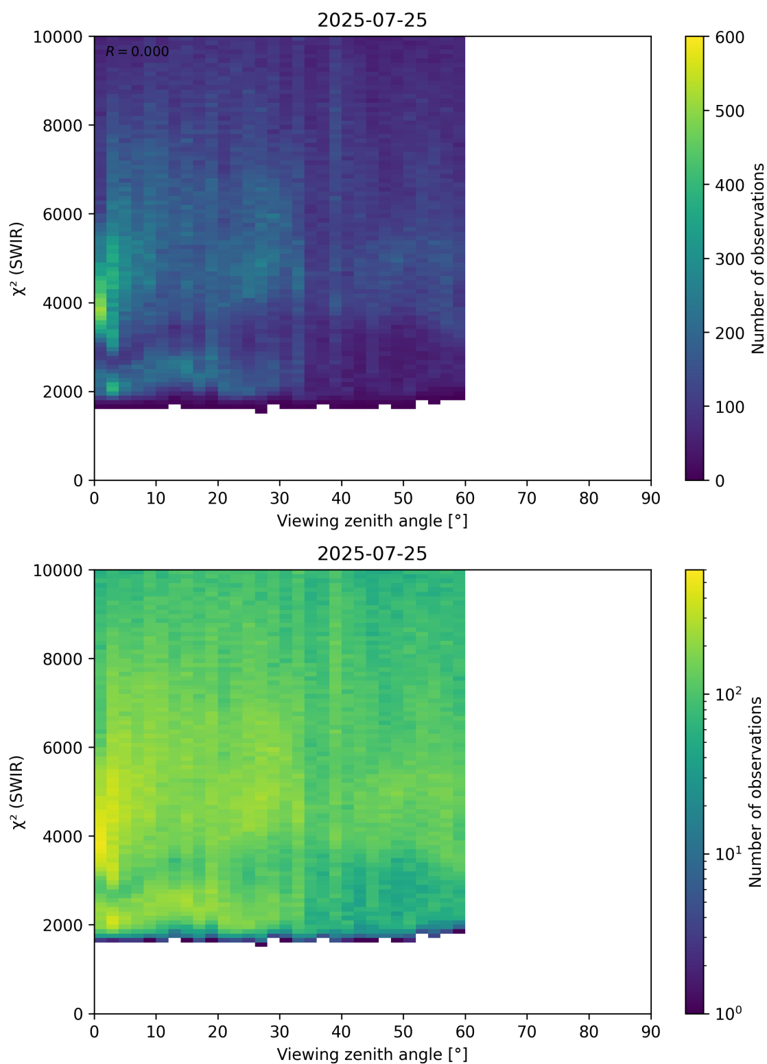
Figure 106: Scatter density plot of “Viewing zenith angle” against “ \chi^2 (SWIR)” for 2025-07-24 to 2025-07-26.
