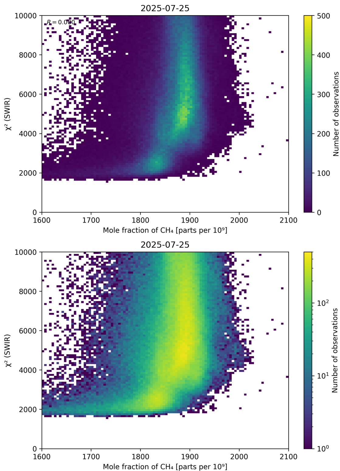
Figure 71: Scatter density plot of “Mole fraction of CH 4 ” against “ \chi^2 (SWIR)” for 2025-07-24 to 2025-07-26.
