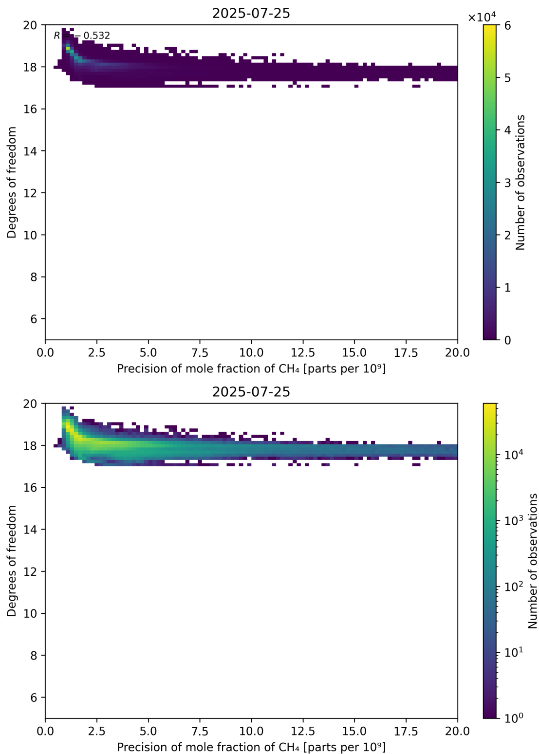
Figure 80: Scatter density plot of “Precision of mole fraction of CH 4 ” against “Degrees of freedom” for 2025-07-24 to 2025-07-26.
