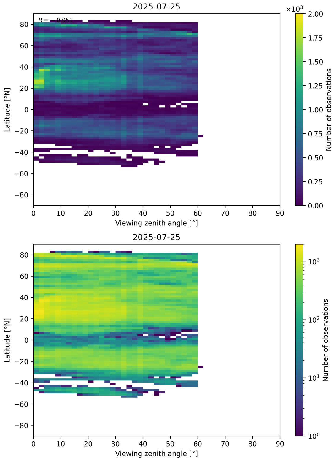
Figure 109: Scatter density plot of “Viewing zenith angle” against “Latitude” for 2025-07-24 to 2025-07-26.
