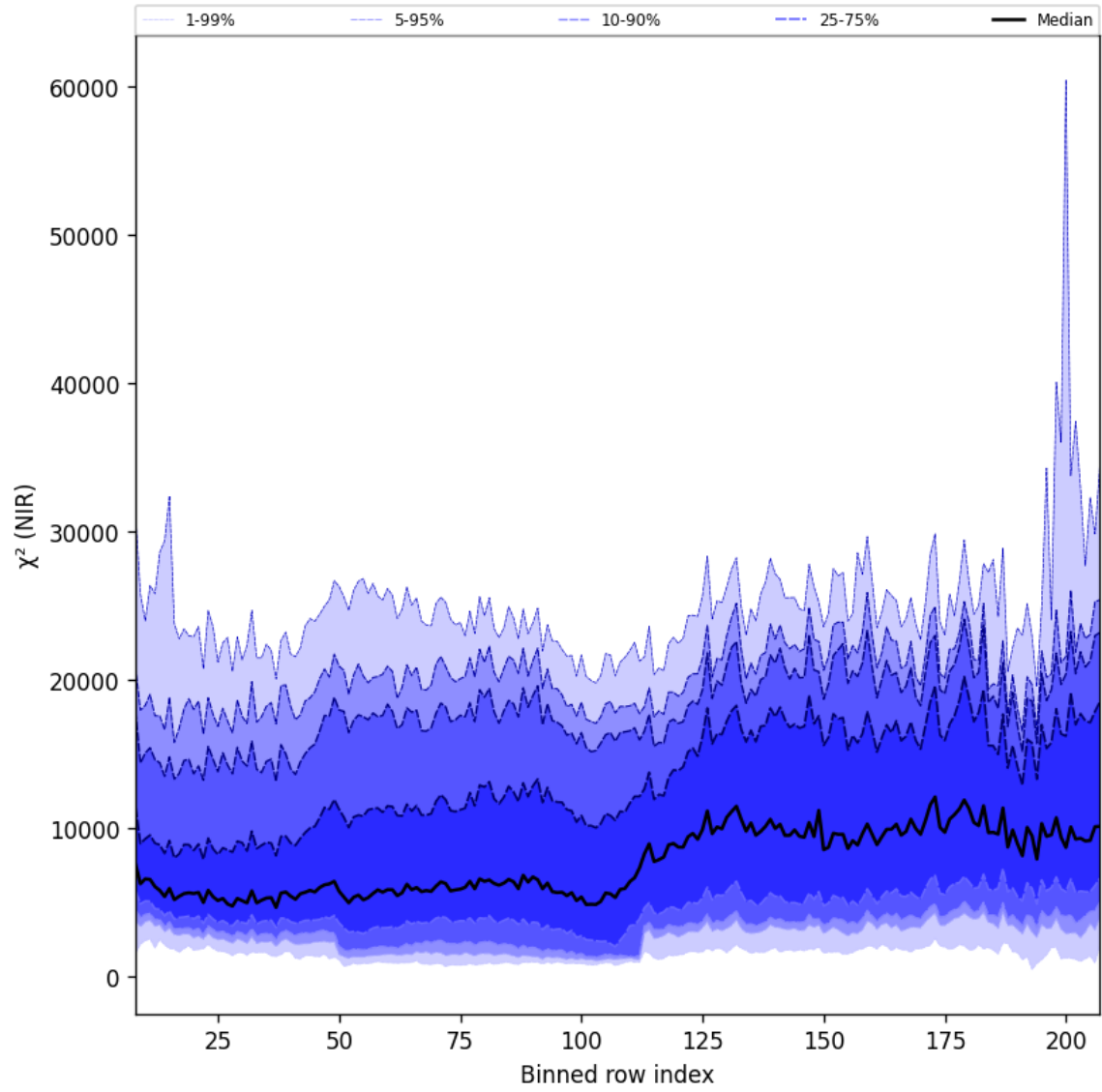
Figure 40: Along track statistics of " \chi^2 (NIR)" for 2025-07-24 to 2025-07-26
