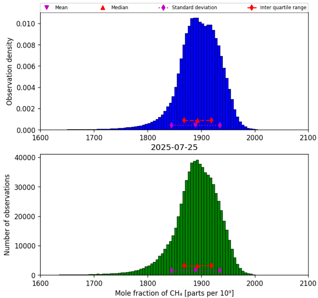
Figure 23: Histogram of “Mole fraction of CH 4 ” for 2025-07-24 to 2025-07-26
