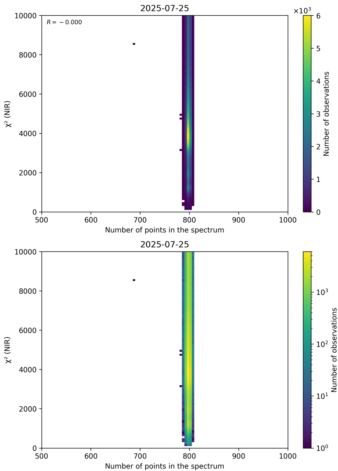
Figure 88: Scatter density plot of “Number of points in the spectrum” against “ \chi^2 (NIR)” for 2025-07-24 to 2025-07-26.
