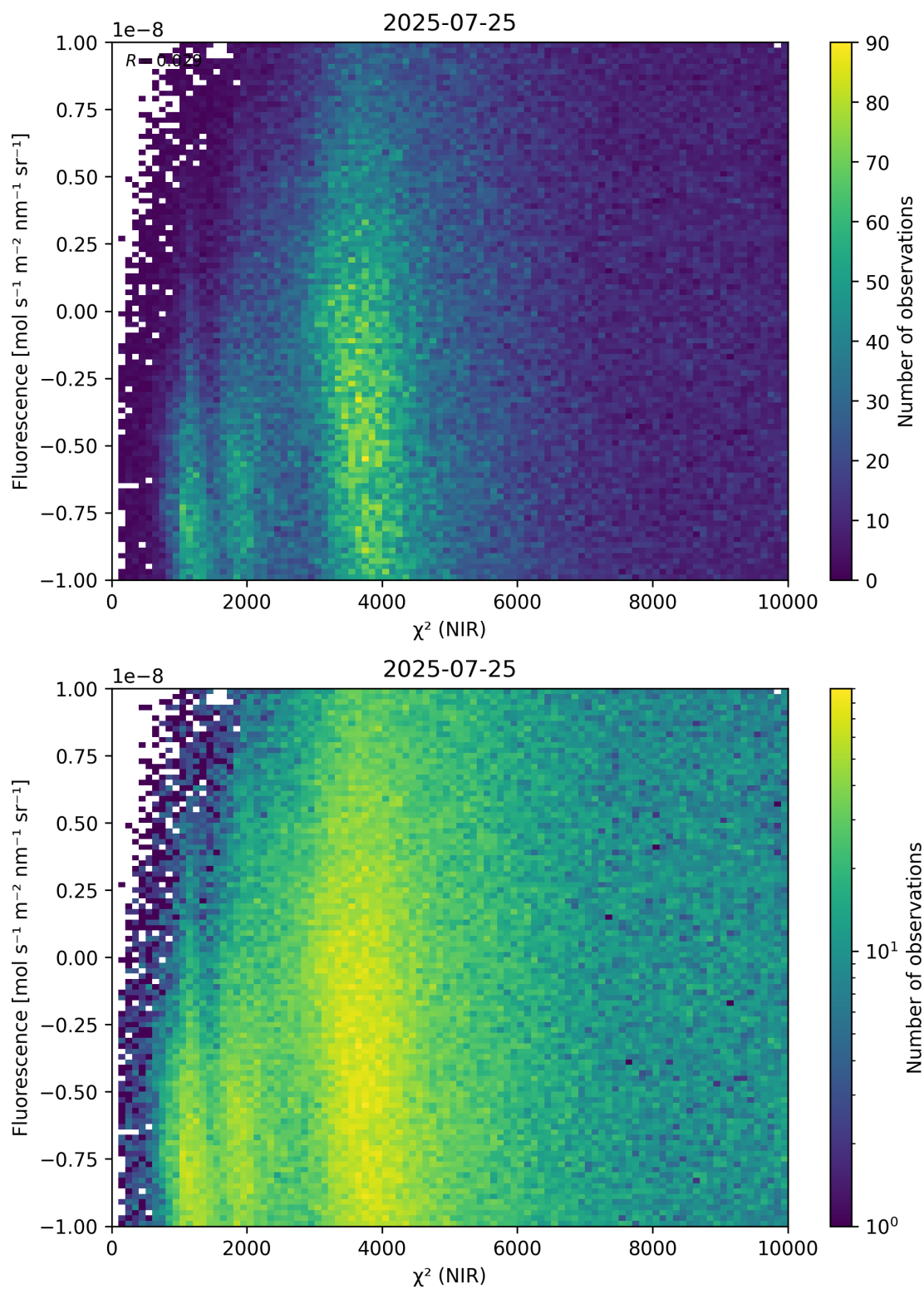
Figure 45: Scatter density plot of “ \chi^2 (NIR)” against “Fluorescence” for 2025-07-24 to 2025-07-26.
