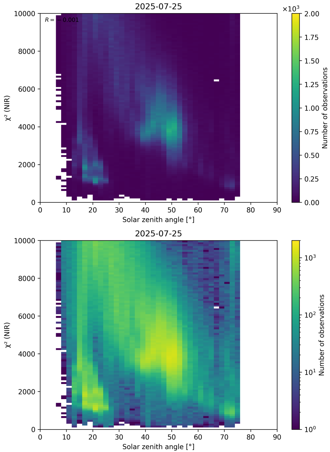
Figure 94: Scatter density plot of “Solar zenith angle” against “ \chi^2 (NIR)” for 2025-07-24 to 2025-07-26.
