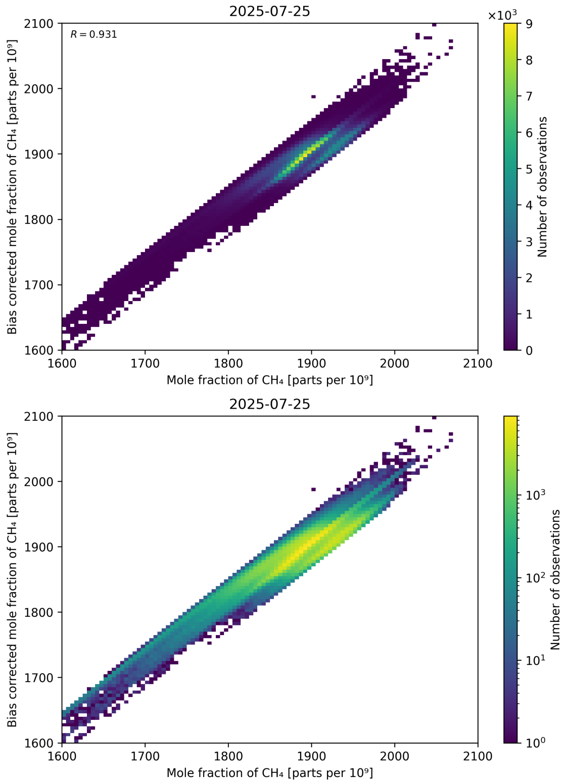
Figure 74: Scatter density plot of “Mole fraction of CH 4 ” against “Bias corrected mole fraction of CH 4 ” for 2025-07-24 to 2025-07-26.
