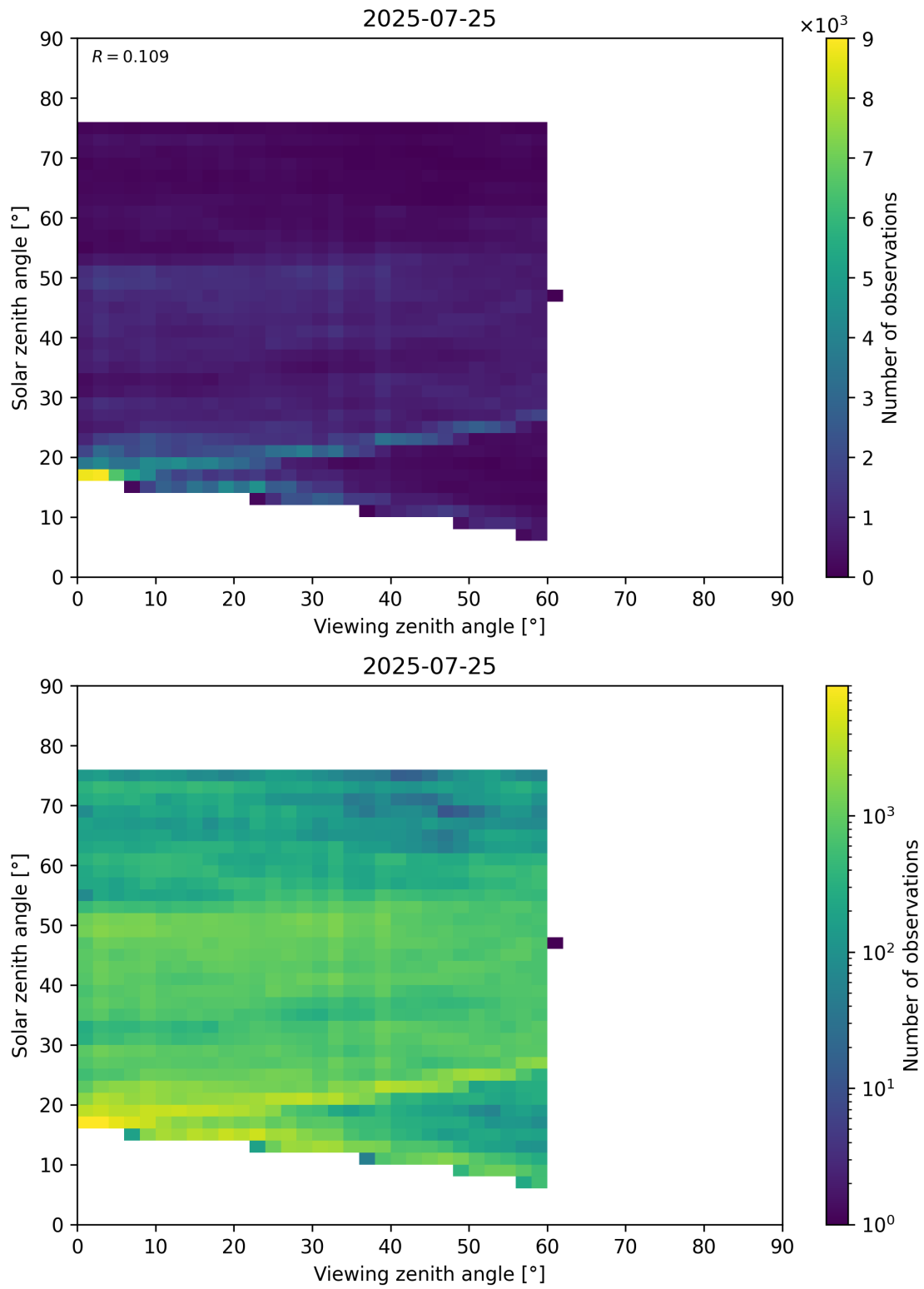
Figure 115: Scatter density plot of “Viewing zenith angle” against “Solar zenith angle” for 2025-07-24 to 2025-07-26.
