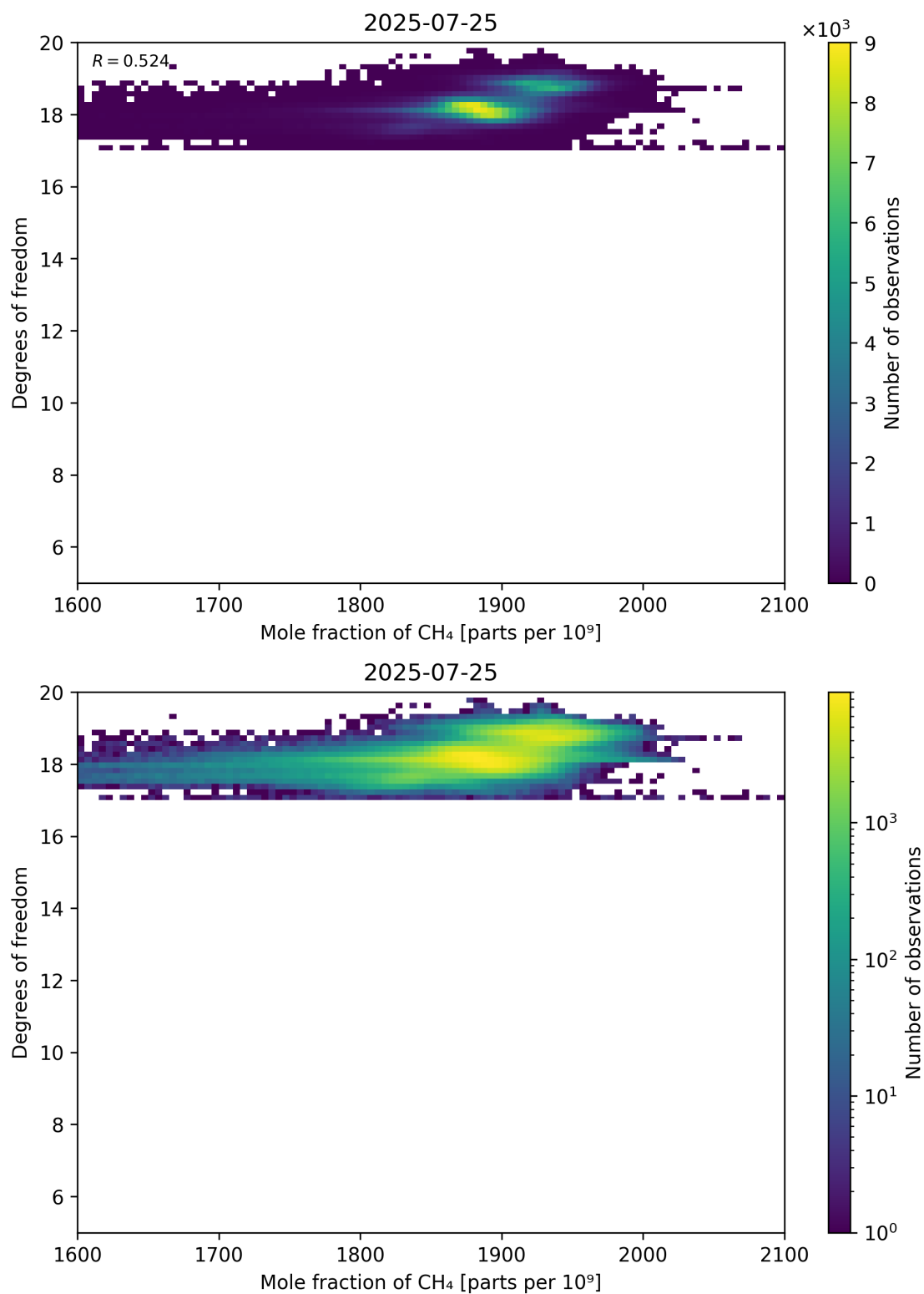
Figure 72: Scatter density plot of “Mole fraction of CH 4 ” against “Degrees of freedom” for 2025-07-24 to 2025-07-26.
