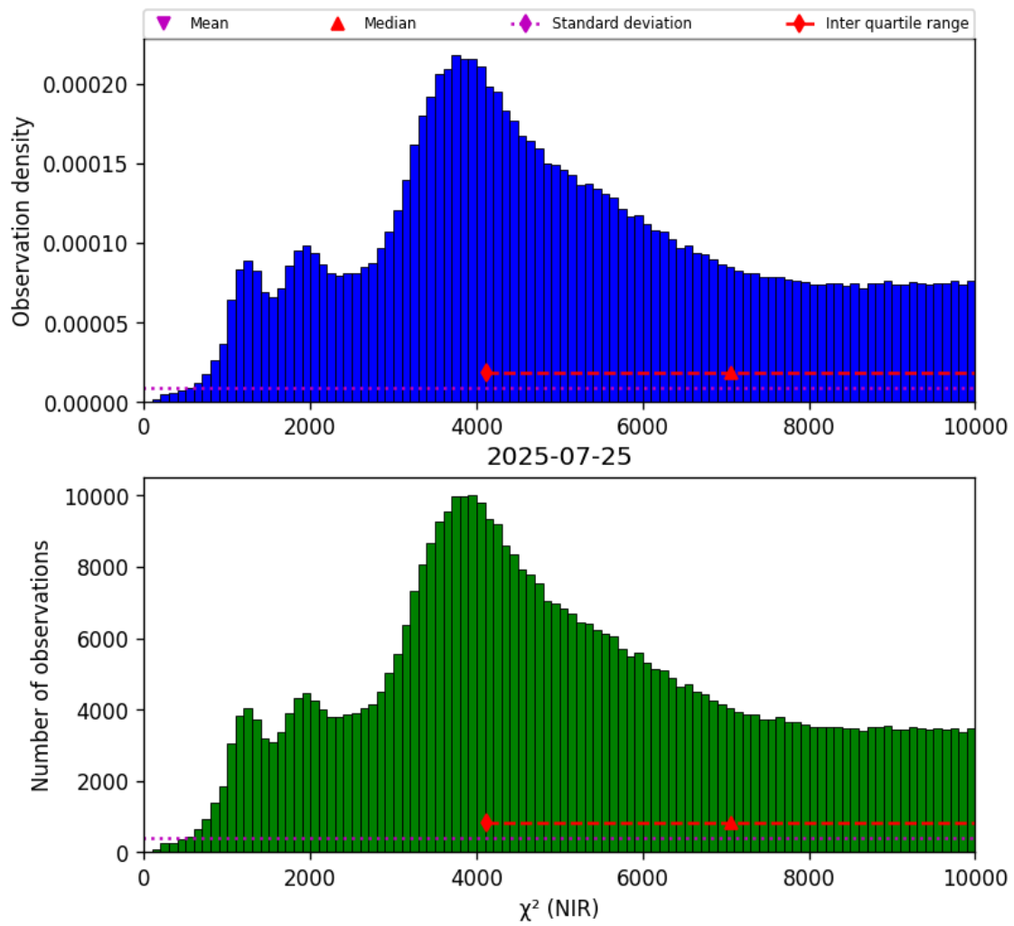
Figure 29: Histogram of “ \chi^2 (NIR)” for 2025-07-24 to 2025-07-26
