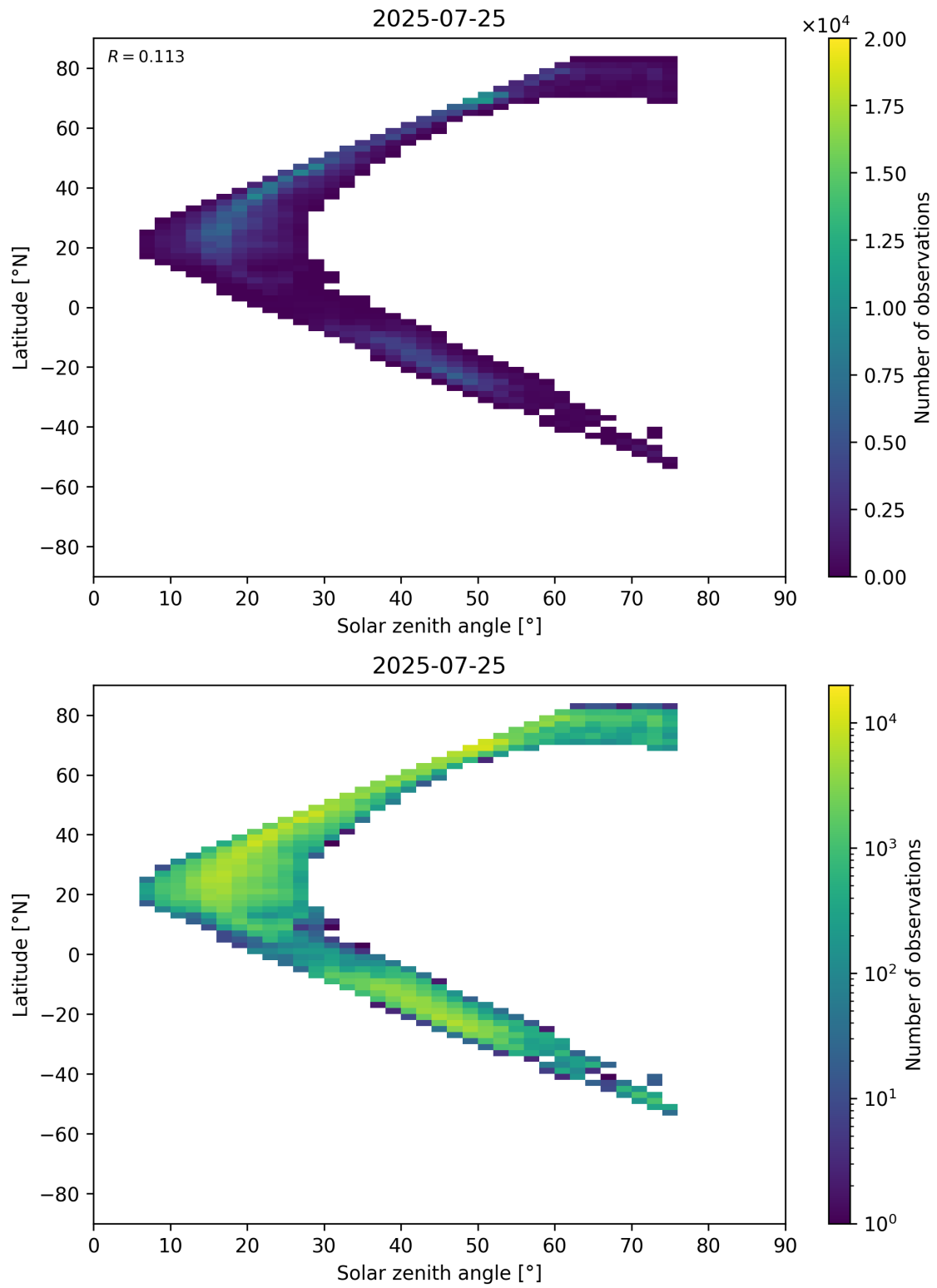
Figure 98: Scatter density plot of “Solar zenith angle” against “Latitude” for 2025-07-24 to 2025-07-26.
