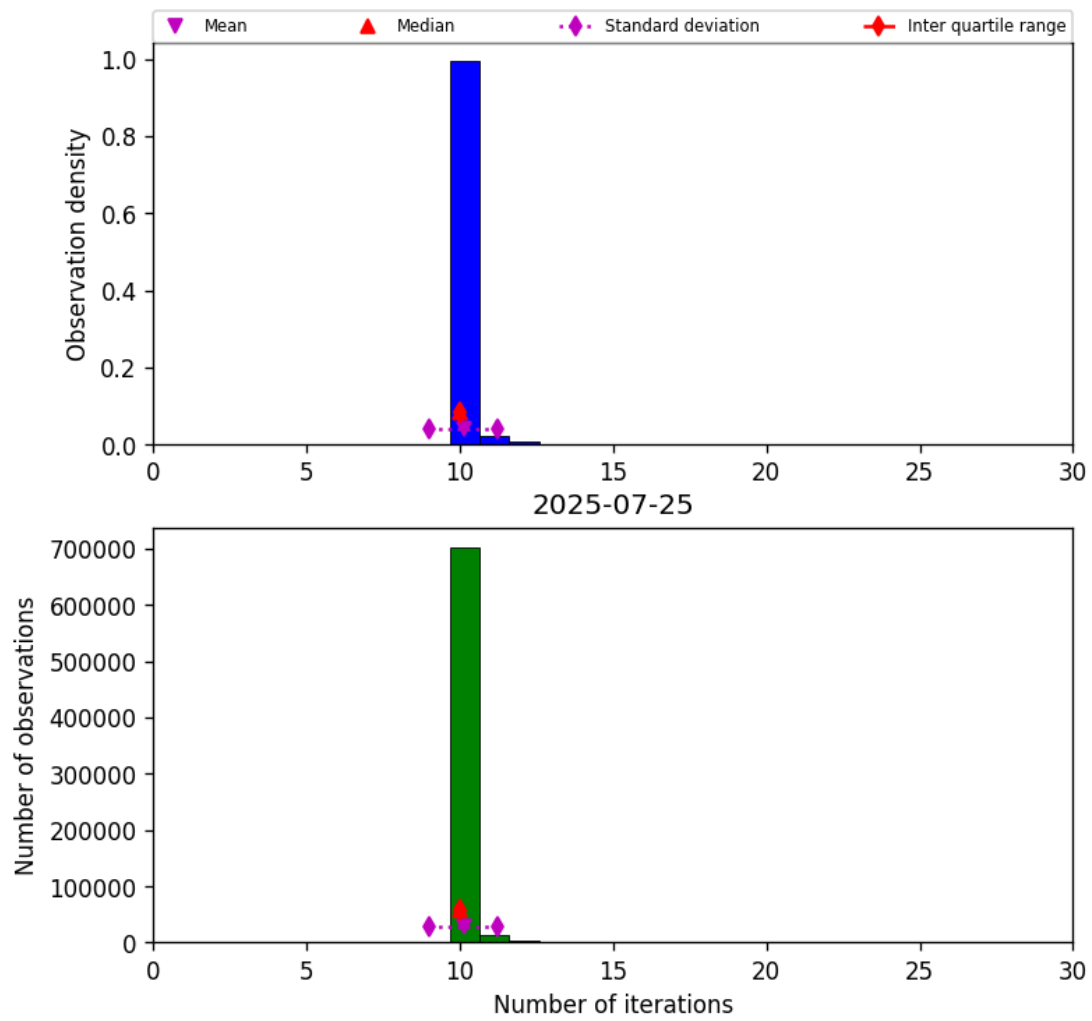
Figure 31: Histogram of “Number of iterations” for 2025-07-24 to 2025-07-26
