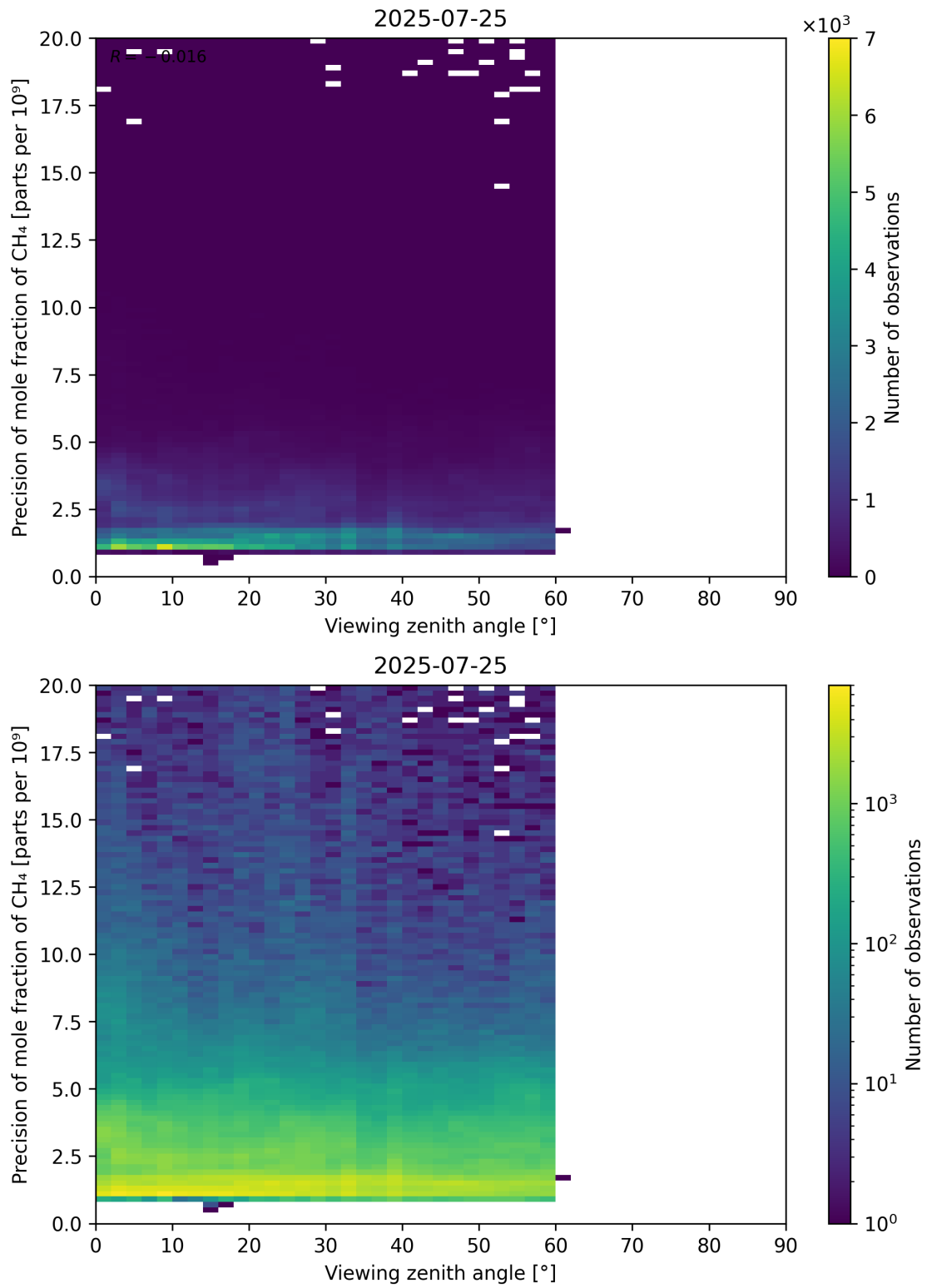
Figure 112: Scatter density plot of “Viewing zenith angle” against “Precision of mole fraction of CH 4 ” for 2025-07-24 to 2025-07-26.
