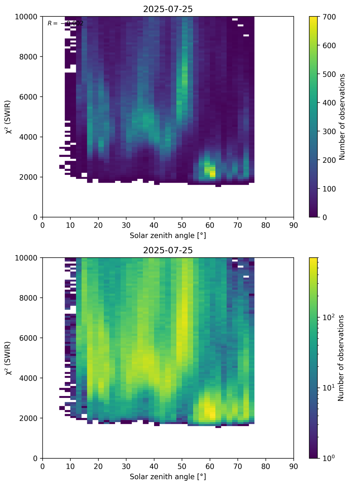
Figure 95: Scatter density plot of “Solar zenith angle” against “ \chi^2 (SWIR)” for 2025-07-24 to 2025-07-26.
