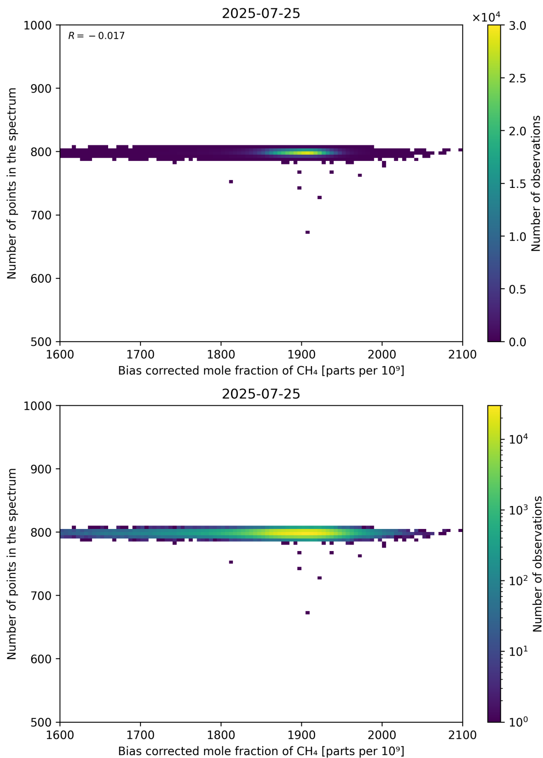
Figure 68: Scatter density plot of “Bias corrected mole fraction of \text{CH}_4 ” against “Number of points in the spectrum” for 2025-07-24 to 2025-07-26.
