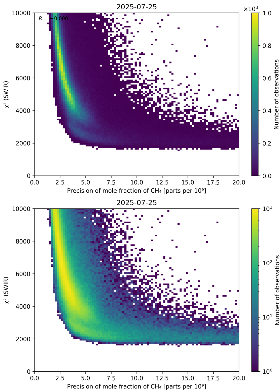
Figure 79: Scatter density plot of “Precision of mole fraction of \text{CH}_4 ” against “ \chi^2 (SWIR)” for 2025-07-24 to 2025-07-26.
