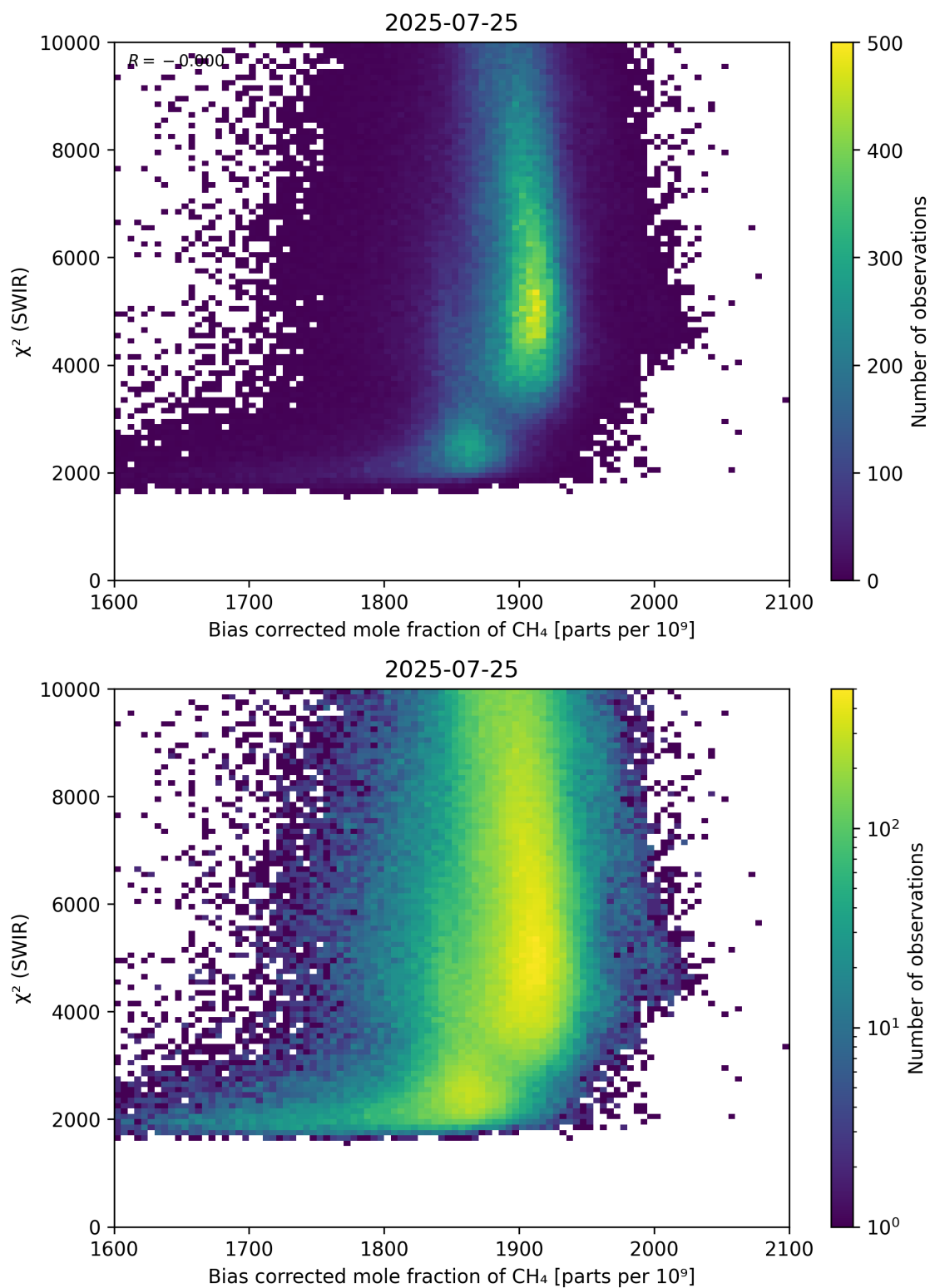
Figure 64: Scatter density plot of “Bias corrected mole fraction of CH 4 ” against “ \chi^2 (SWIR)” for 2025-07-24 to 2025-07-26.
