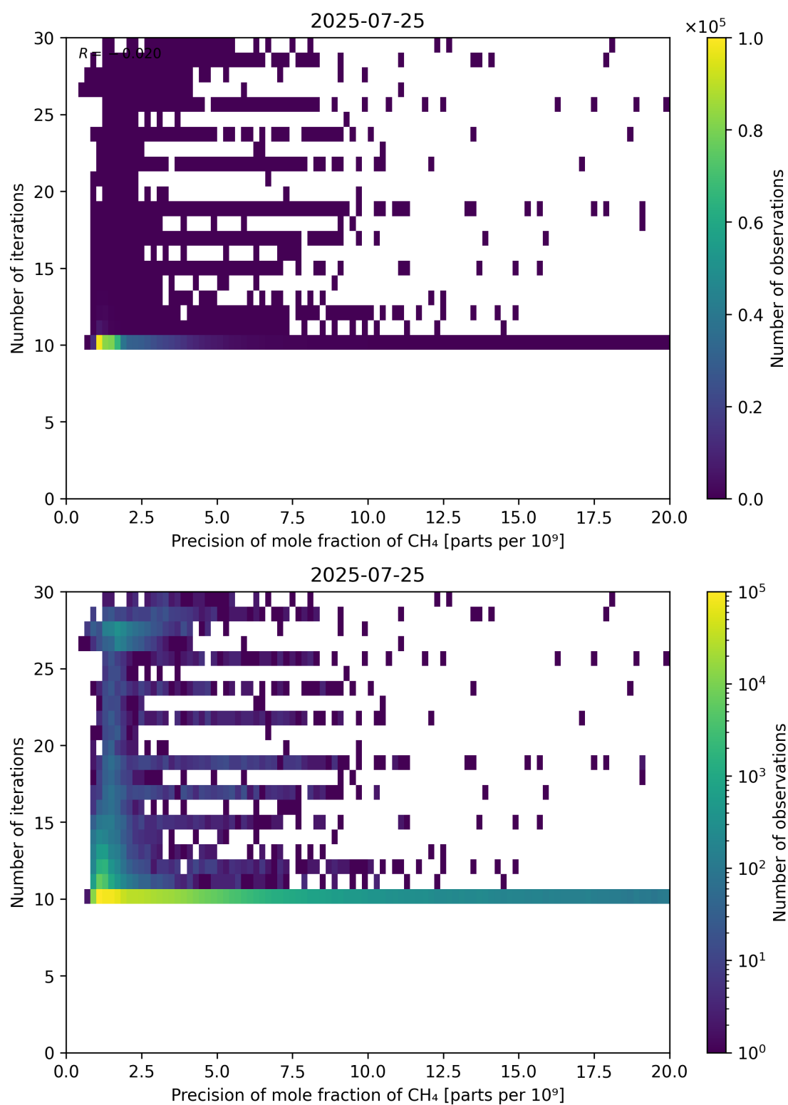
Figure 83: Scatter density plot of “Precision of mole fraction of \text{CH}_4 ” against “Number of iterations” for 2025-07-24 to 2025-07-26.
