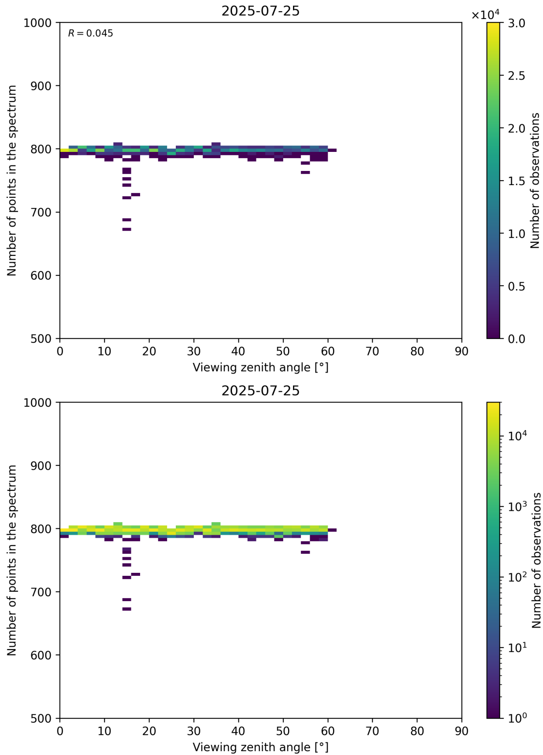
Figure 114: Scatter density plot of “Viewing zenith angle” against “Number of points in the spectrum” for 2025-07-24 to 2025-07-26.
