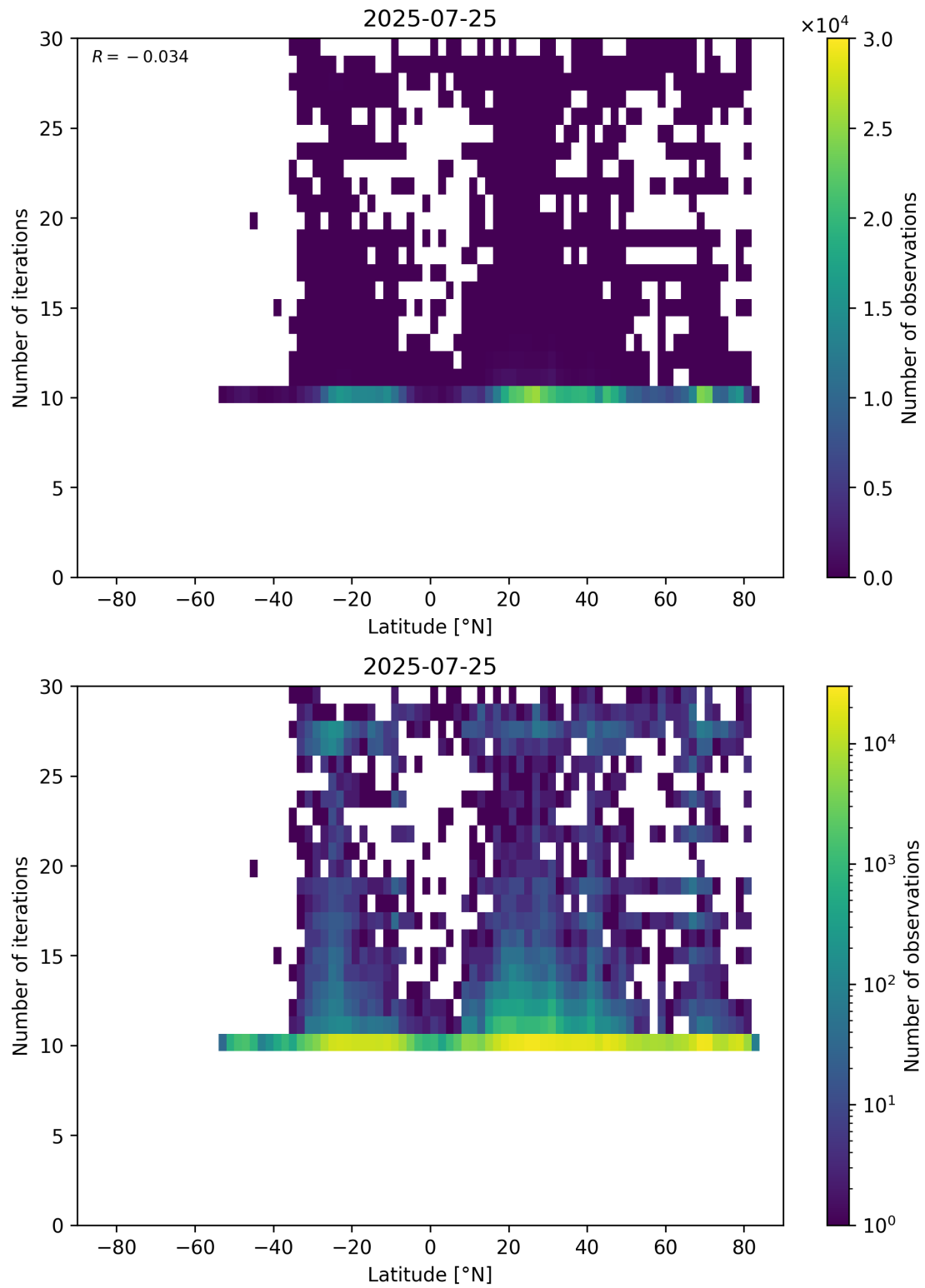
Figure 60: Scatter density plot of “Latitude” against “Number of iterations” for 2025-07-24 to 2025-07-26.
