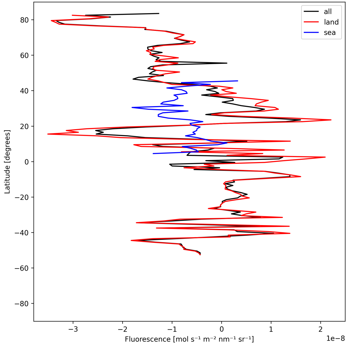
Figure 21: Zonal average of “Fluorescence” for 2025-07-24 to 2025-07-26.
