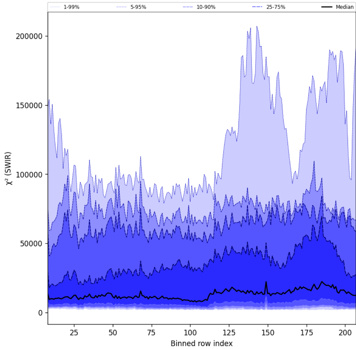
Figure 39: Along track statistics of " \chi^2 (SWIR)" for 2025-07-24 to 2025-07-26
