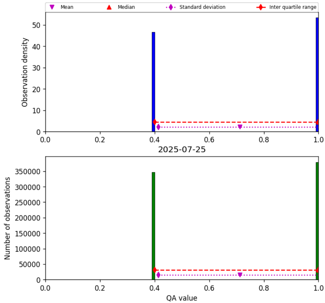
Figure 22: Histogram of “QA value” for 2025-07-24 to 2025-07-26
