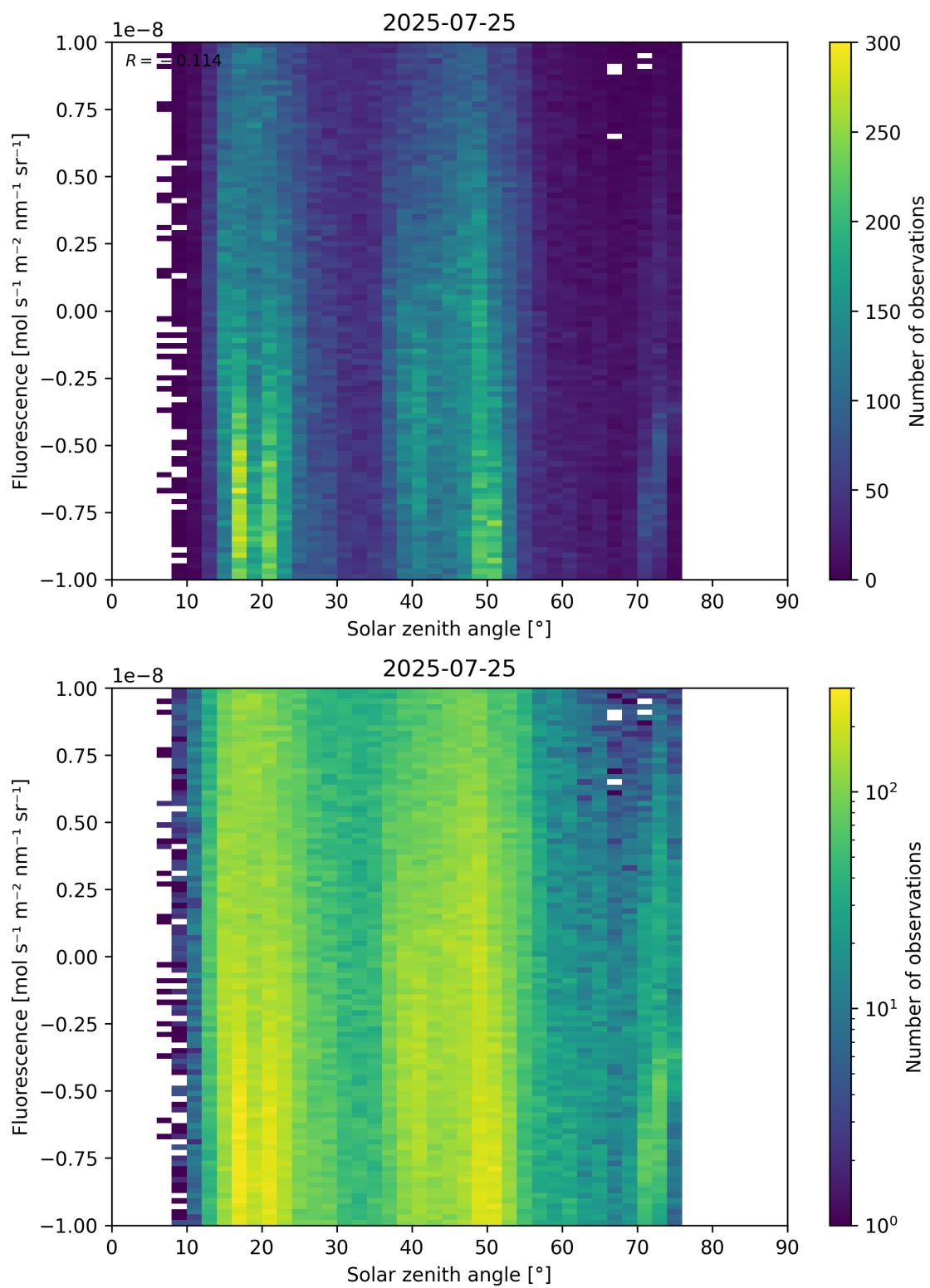
Figure 97: Scatter density plot of “Solar zenith angle” against “Fluorescence” for 2025-07-24 to 2025-07-26.
