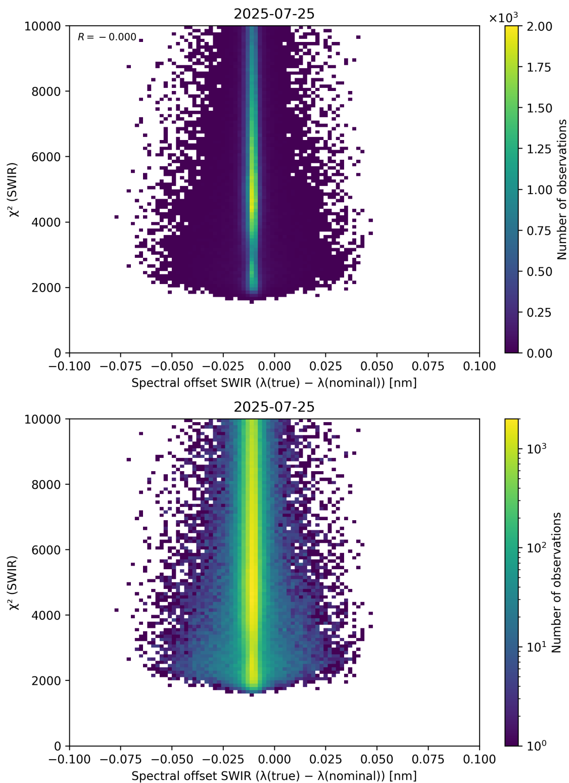
Figure 118: Scatter density plot of “Spectral offset SWIR ( \lambda_{\text{true}} - \lambda_{\text{nominal}} )” against “ \chi^2 (SWIR)” for 2025-07-24 to 2025-07-26.
