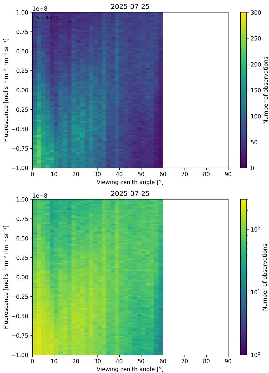
Figure 108: Scatter density plot of “Viewing zenith angle” against “Fluorescence” for 2025-07-24 to 2025-07-26.
