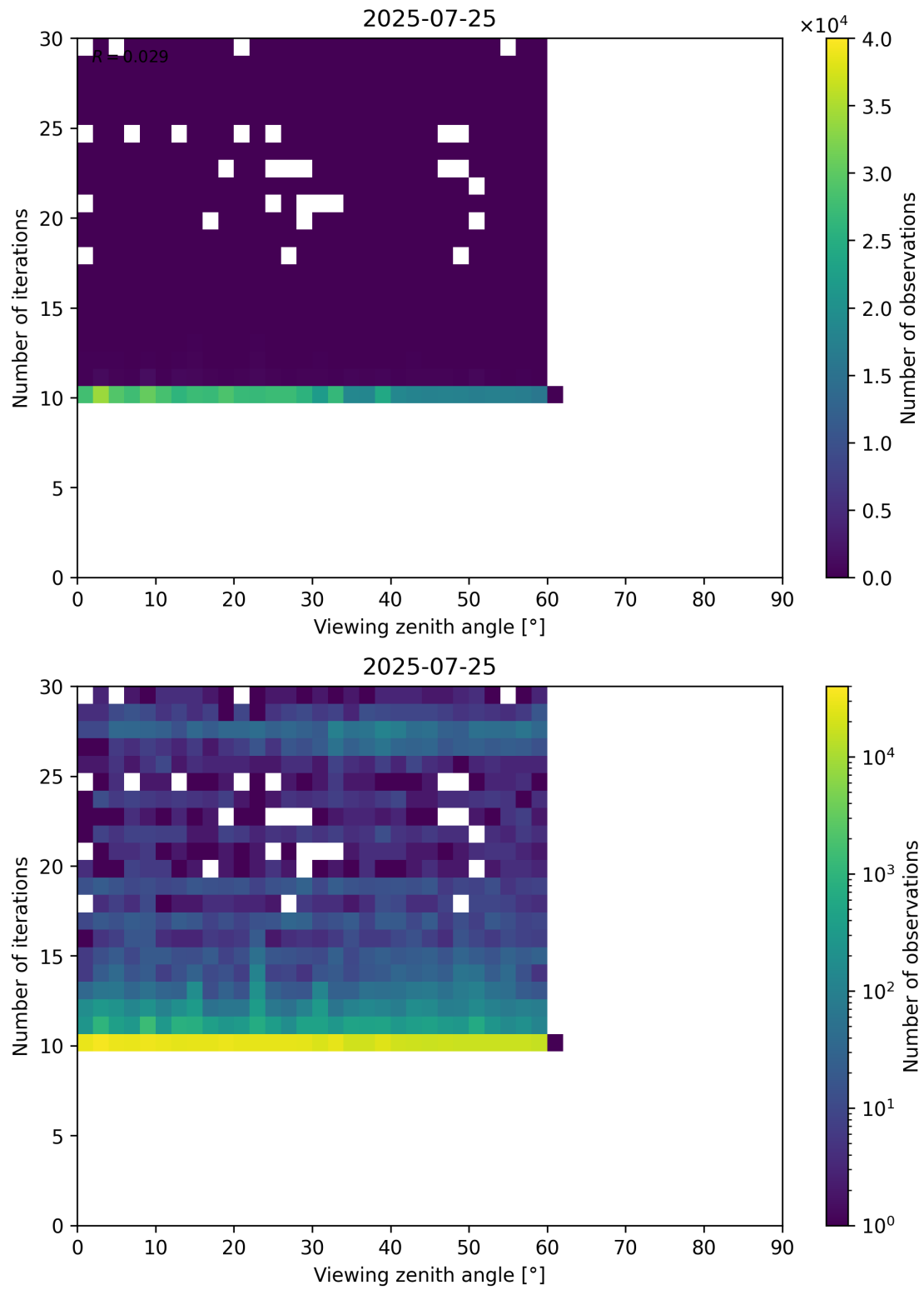
Figure 113: Scatter density plot of “Viewing zenith angle” against “Number of iterations” for 2025-07-24 to 2025-07-26.
