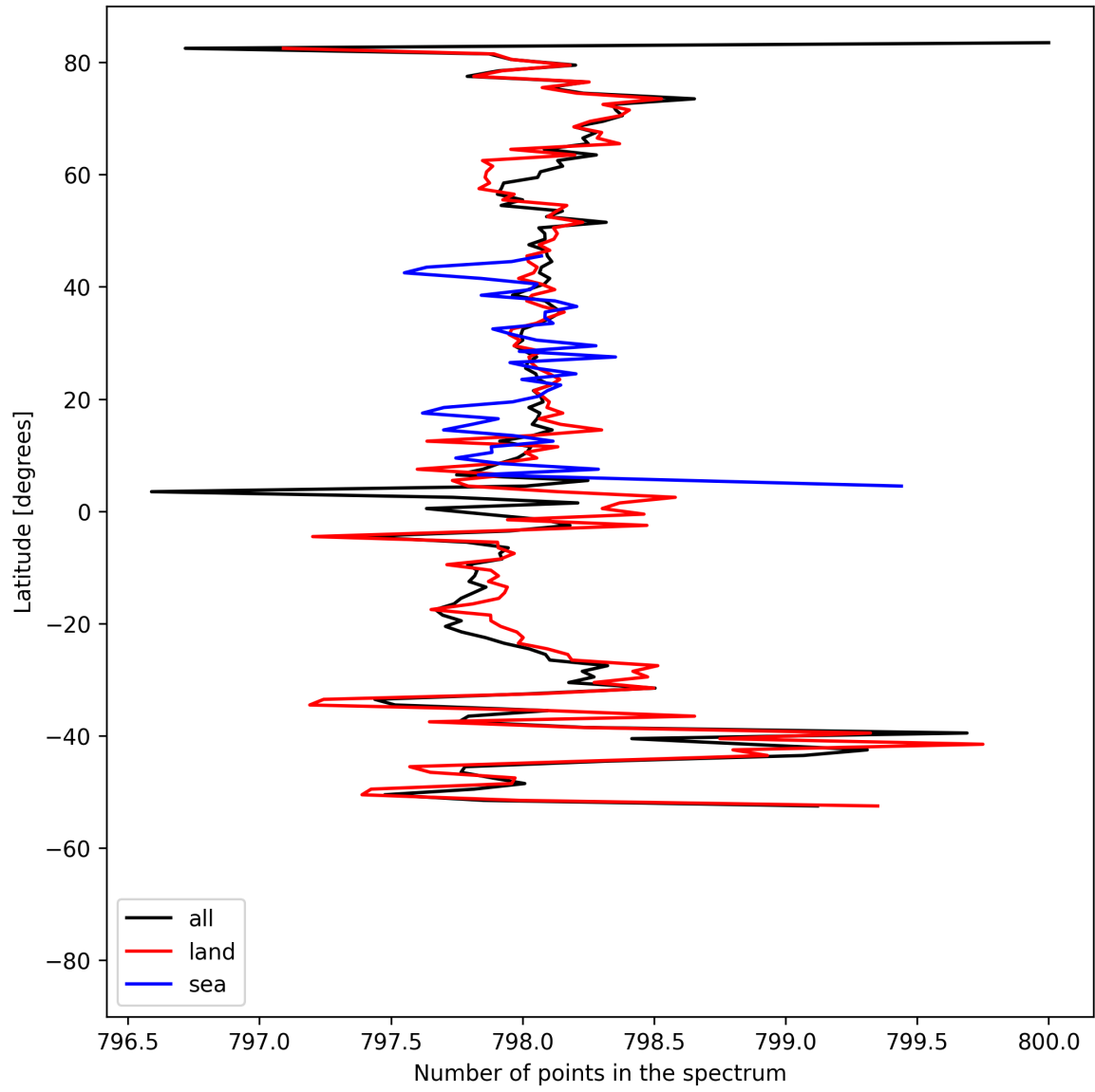
Figure 15: Zonal average of “Number of points in the spectrum” for 2025-07-24 to 2025-07-26.
