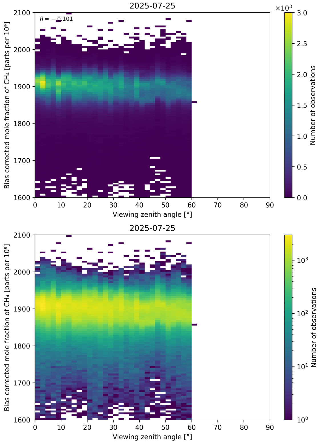
Figure 111: Scatter density plot of “Viewing zenith angle” against “Bias corrected mole fraction of CH 4 ” for 2025-07-24 to 2025-07-26.
