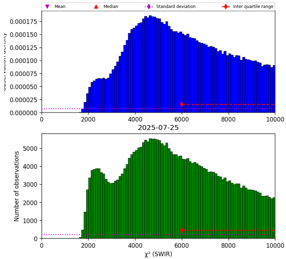
Figure 28: Histogram of “ \chi^2 (SWIR)” for 2025-07-24 to 2025-07-26
