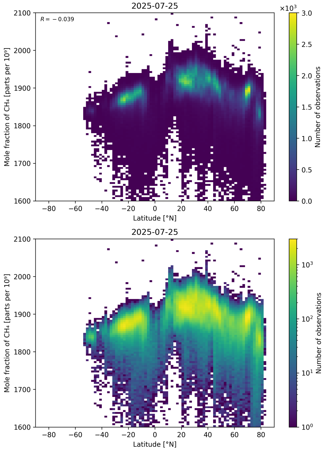
Figure 57: Scatter density plot of “Latitude” against “Mole fraction of CH 4 ” for 2025-07-24 to 2025-07-26.
