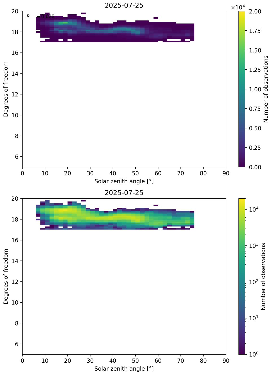
Figure 96: Scatter density plot of “Solar zenith angle” against “Degrees of freedom” for 2025-07-24 to 2025-07-26.
