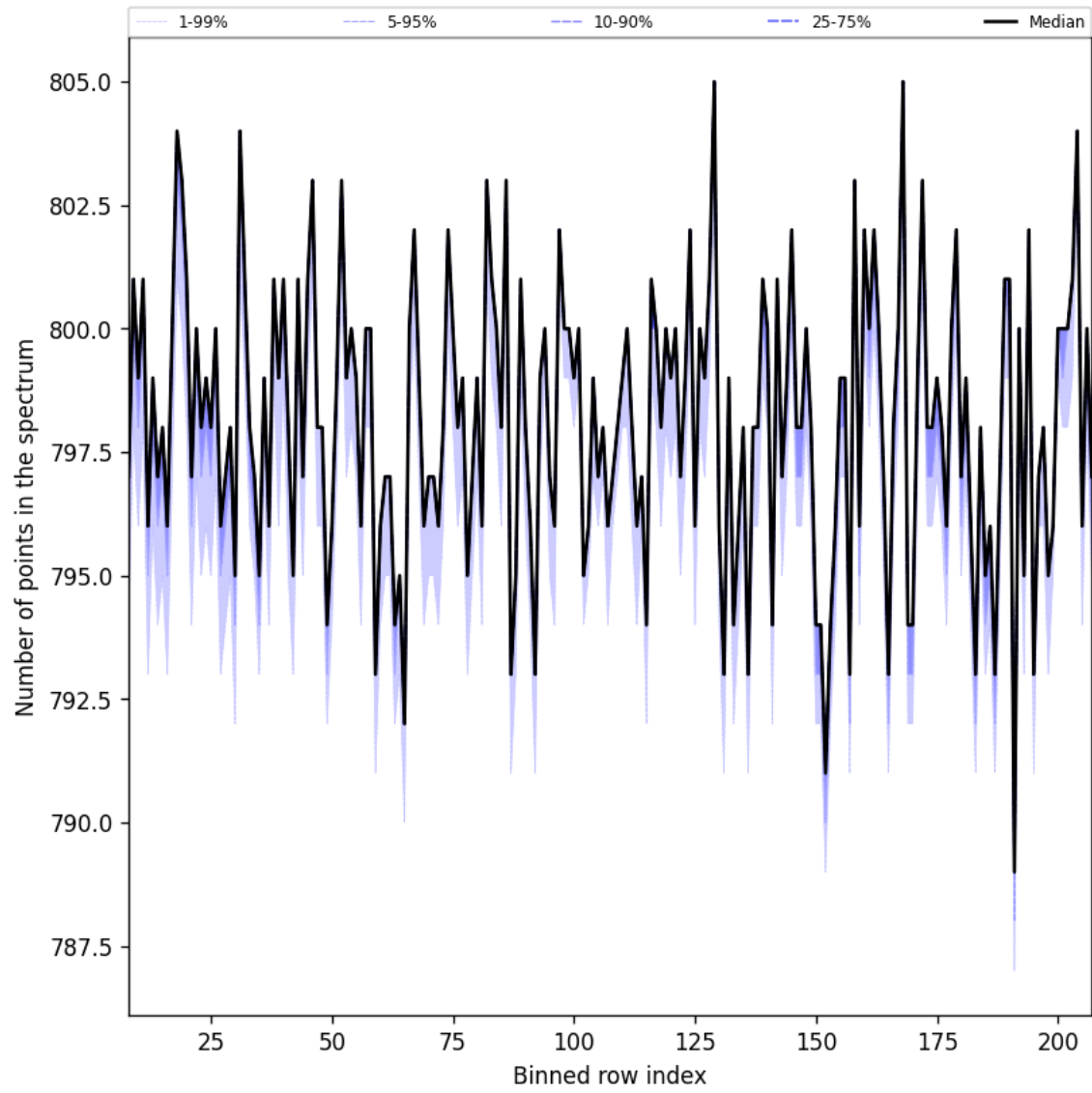
Figure 37: Along track statistics of “Number of points in the spectrum” for 2025-07-24 to 2025-07-26
