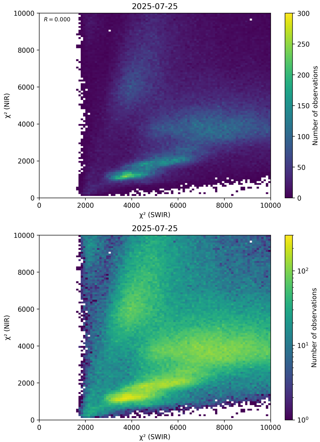
Figure 47: Scatter density plot of “ \chi^2 (SWIR)” against “ \chi^2 (NIR)” for 2025-07-24 to 2025-07-26.
