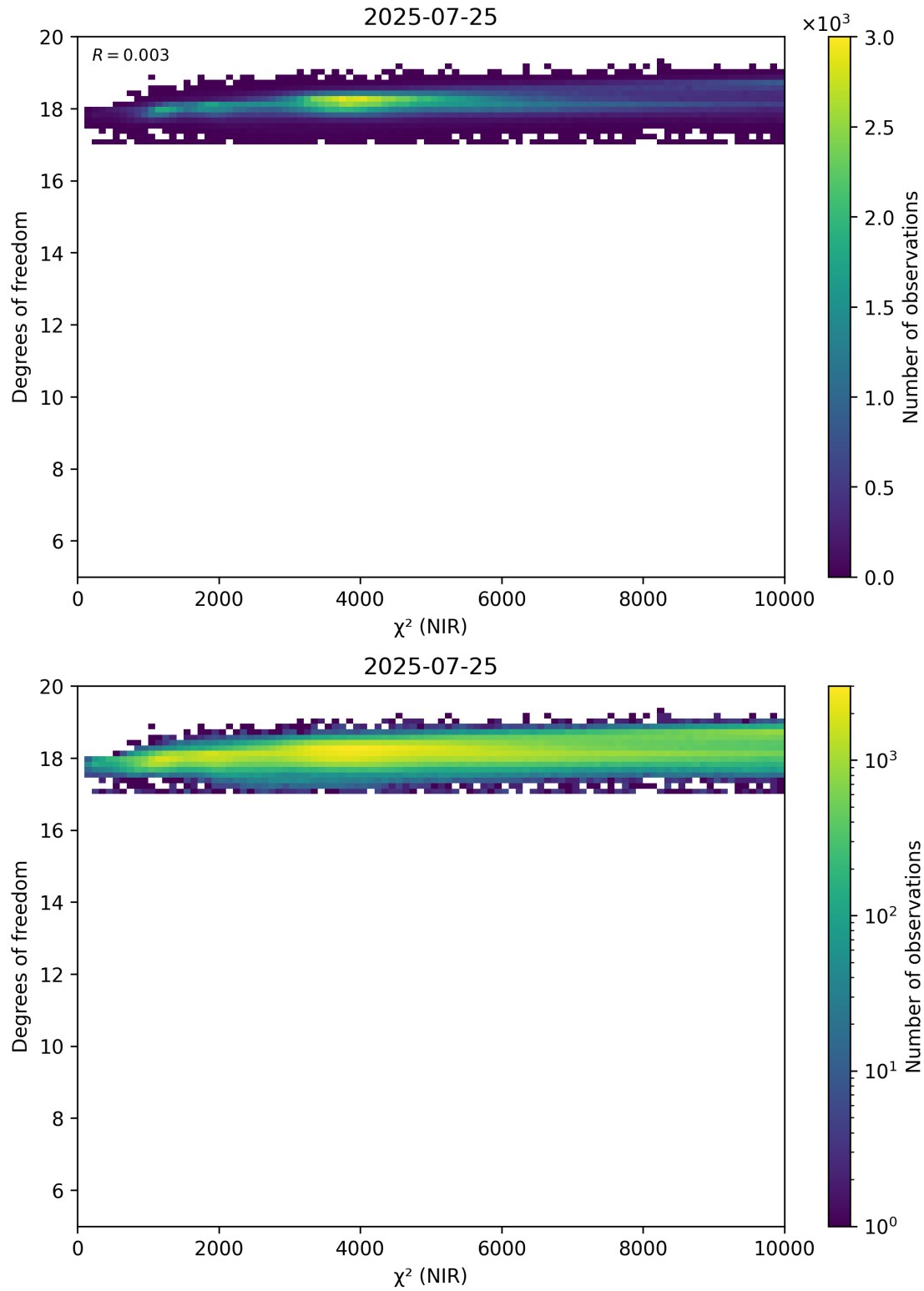
Figure 44: Scatter density plot of “ \chi^2 (NIR)” against “Degrees of freedom” for 2025-07-24 to 2025-07-26.
