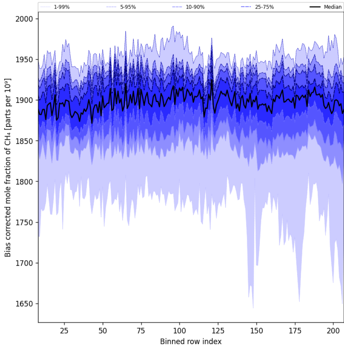
Figure 36: Along track statistics of “Bias corrected mole fraction of CH 4 ” for 2025-07-24 to 2025-07-26
