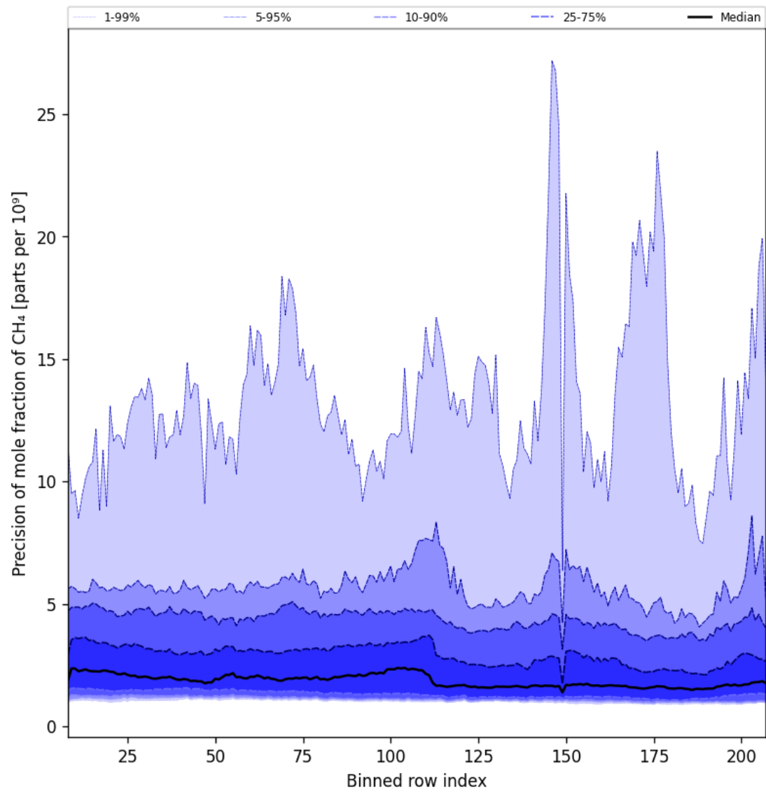
Figure 35: Along track statistics of “Precision of mole fraction of CH 4 ” for 2025-07-24 to 2025-07-26
