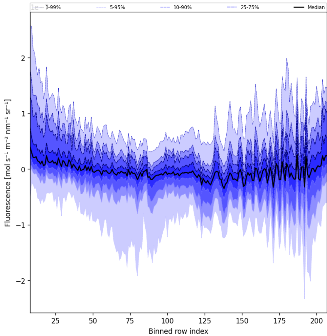
Figure 43: Along track statistics of “Fluorescence” for 2025-07-24 to 2025-07-26
