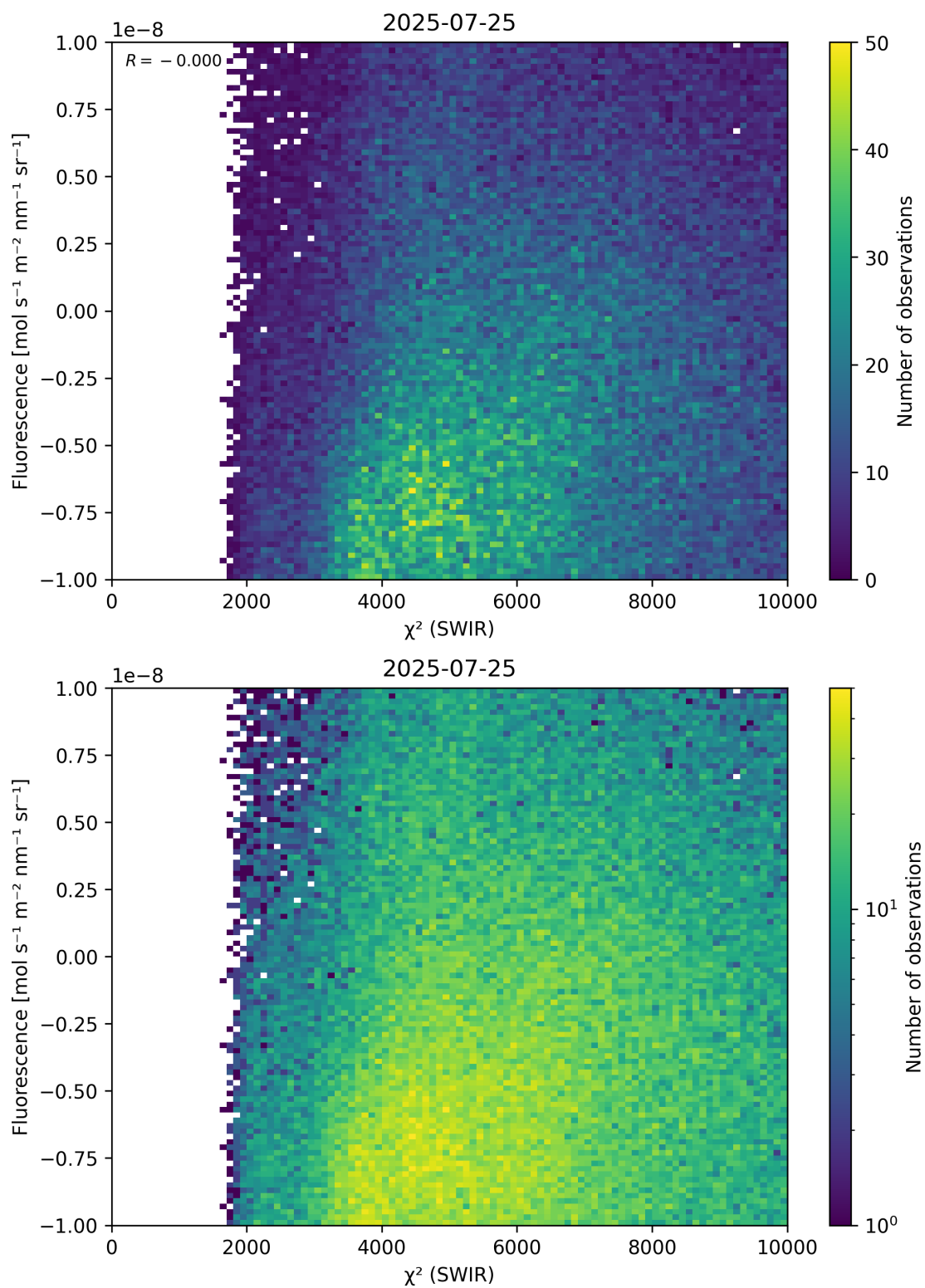
Figure 49: Scatter density plot of “ \chi^2 (SWIR)” against “Fluorescence” for 2025-07-24 to 2025-07-26.
