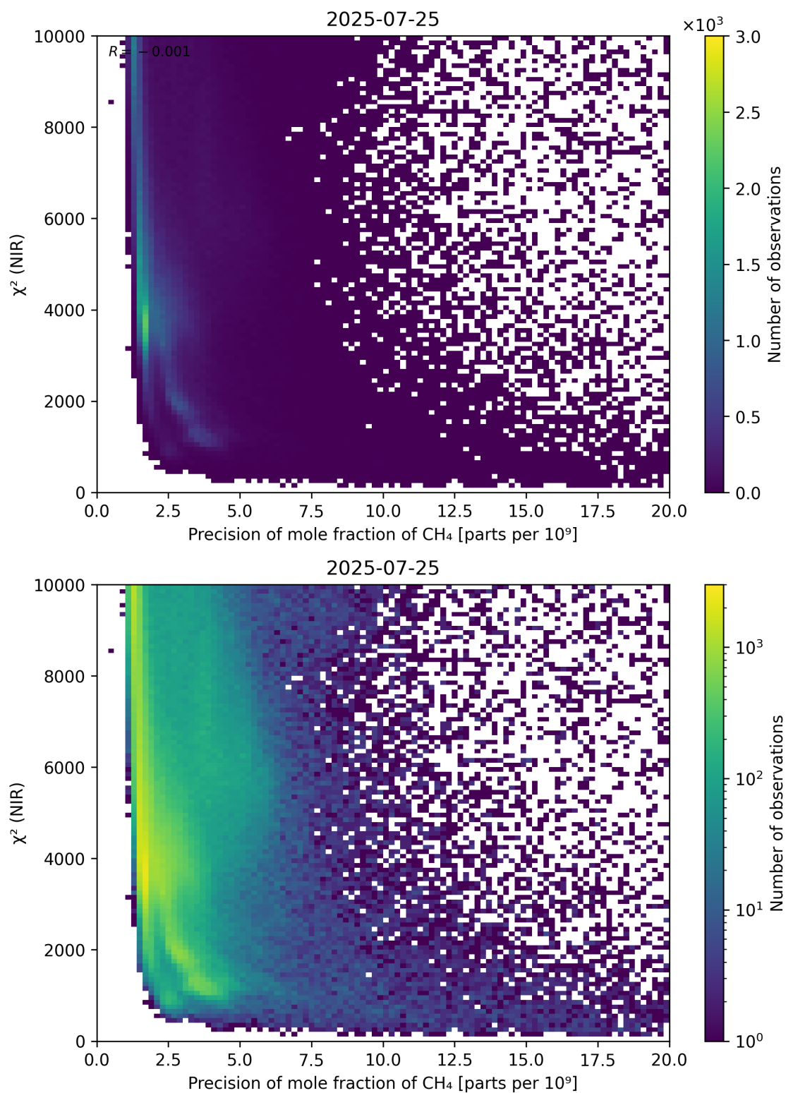
Figure 78: Scatter density plot of “Precision of mole fraction of CH 4 ” against “ \chi^2 (NIR)” for 2025-07-24 to 2025-07-26.
