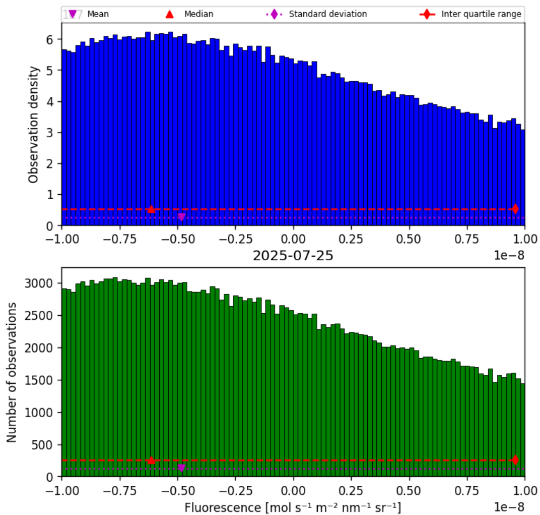
Figure 32: Histogram of “Fluorescence” for 2025-07-24 to 2025-07-26
