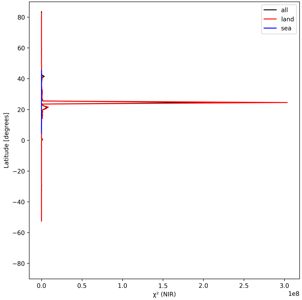
Figure 18: Zonal average of “ \chi^2 (NIR)” for 2025-07-24 to 2025-07-26.
