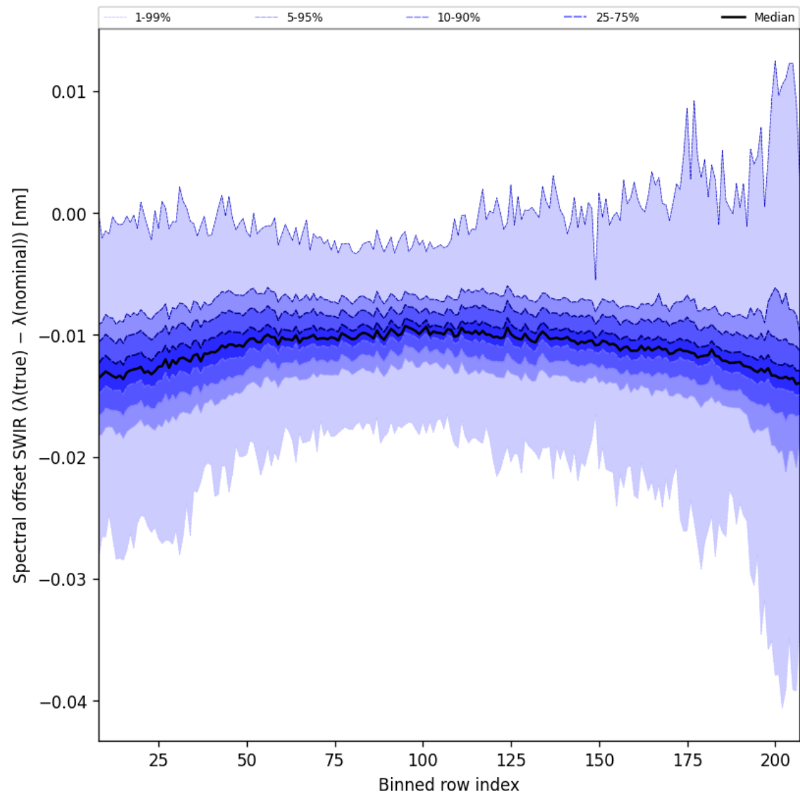
Figure 38: Along track statistics of “Spectral offset SWIR ( \lambda_{\text{true}} - \lambda_{\text{nominal}} )” for 2025-07-24 to 2025-07-26
