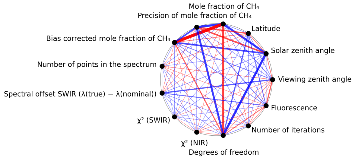
Figure 1: Map of correlation graph for 2025-07-24 to 2025-07-26.
