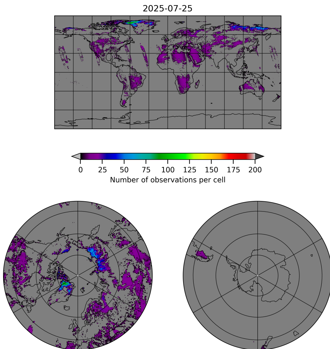
Figure 10: Map of the number of observations for 2025-07-24 to 2025-07-26
