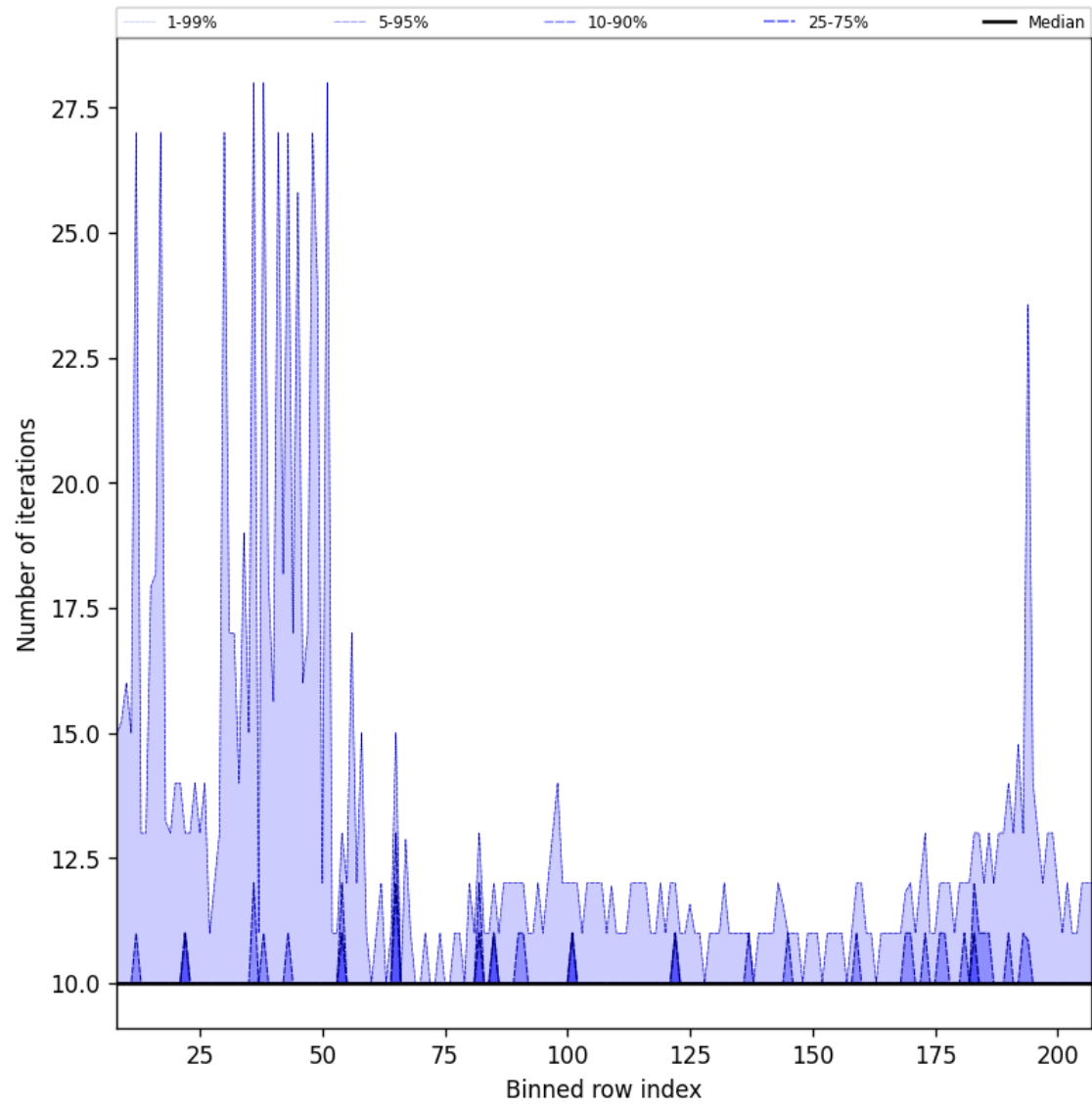
Figure 42: Along track statistics of “Number of iterations” for 2025-07-24 to 2025-07-26
