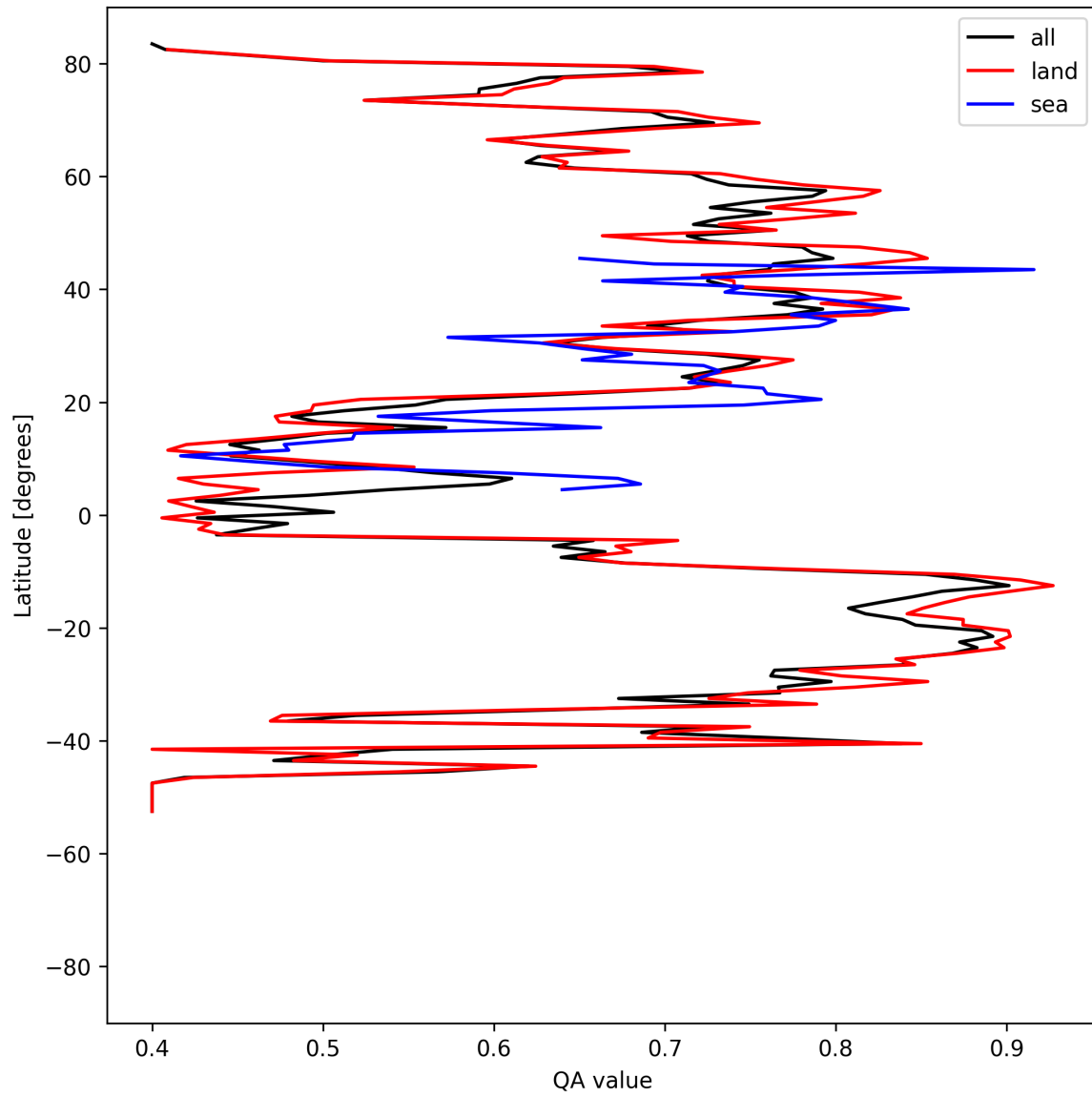
Figure 11: Zonal average of “QA value” for 2025-07-24 to 2025-07-26.
