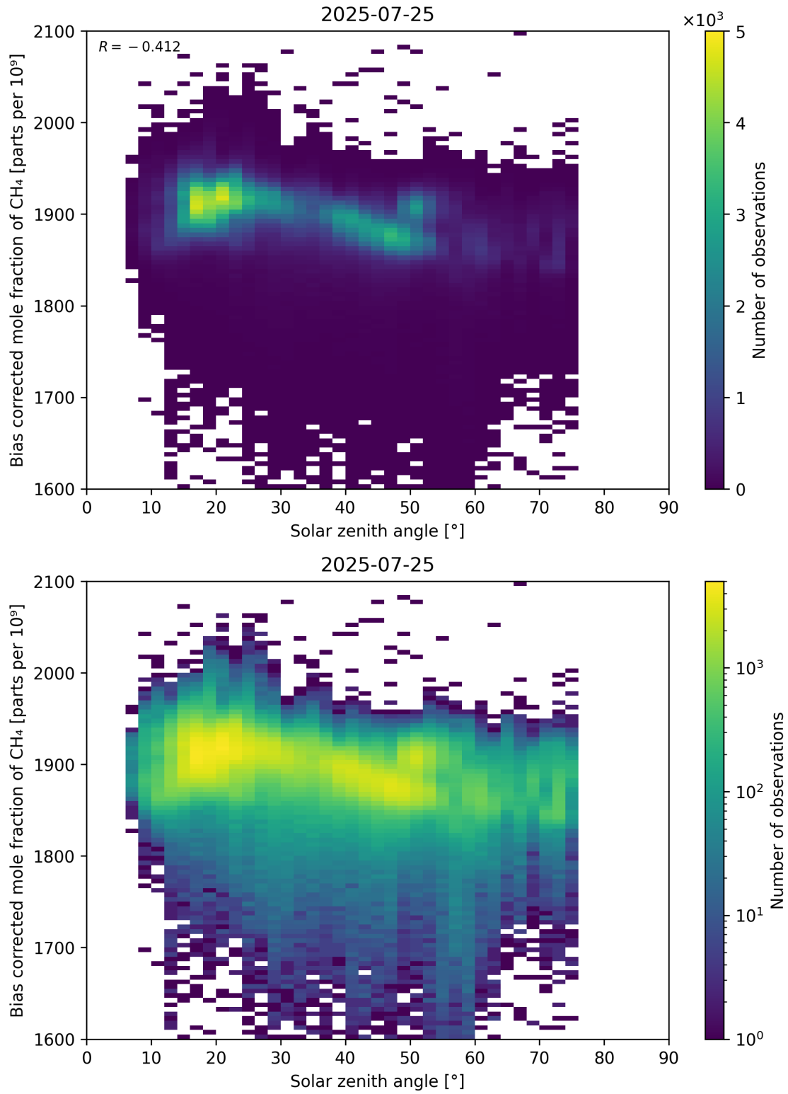
Figure 100: Scatter density plot of “Solar zenith angle” against “Bias corrected mole fraction of \text{CH}_4 ” for 2025-07-24 to 2025-07-26.
