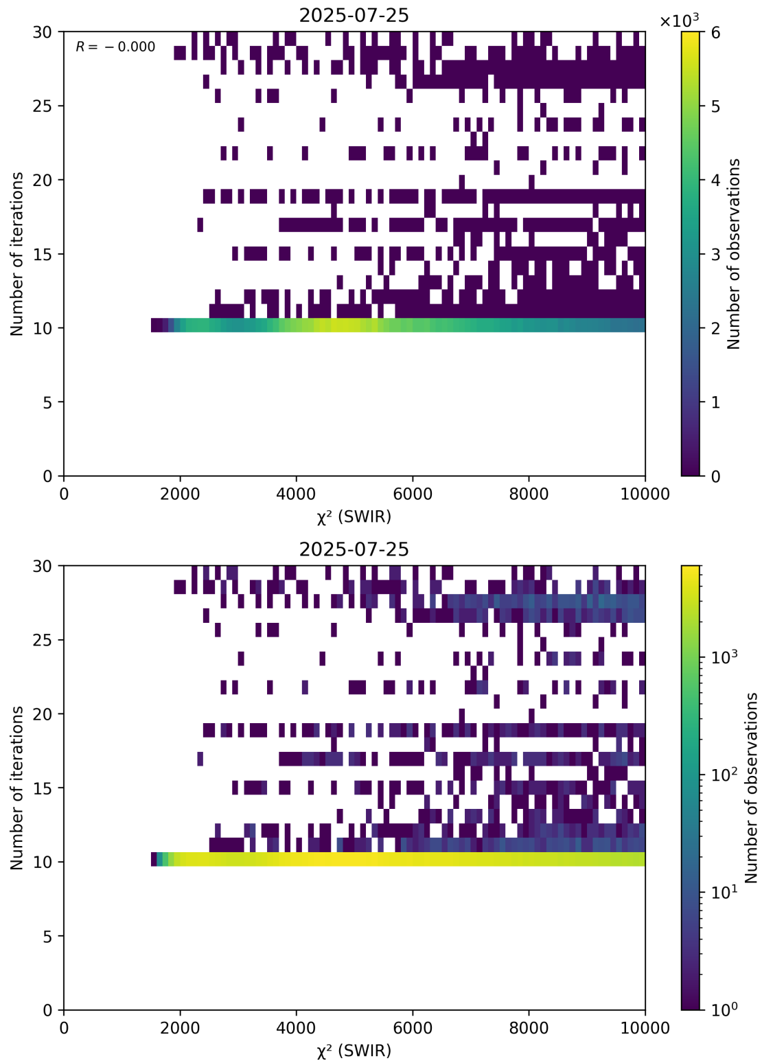
Figure 50: Scatter density plot of “ \chi^2 (SWIR)” against “Number of iterations” for 2025-07-24 to 2025-07-26.
