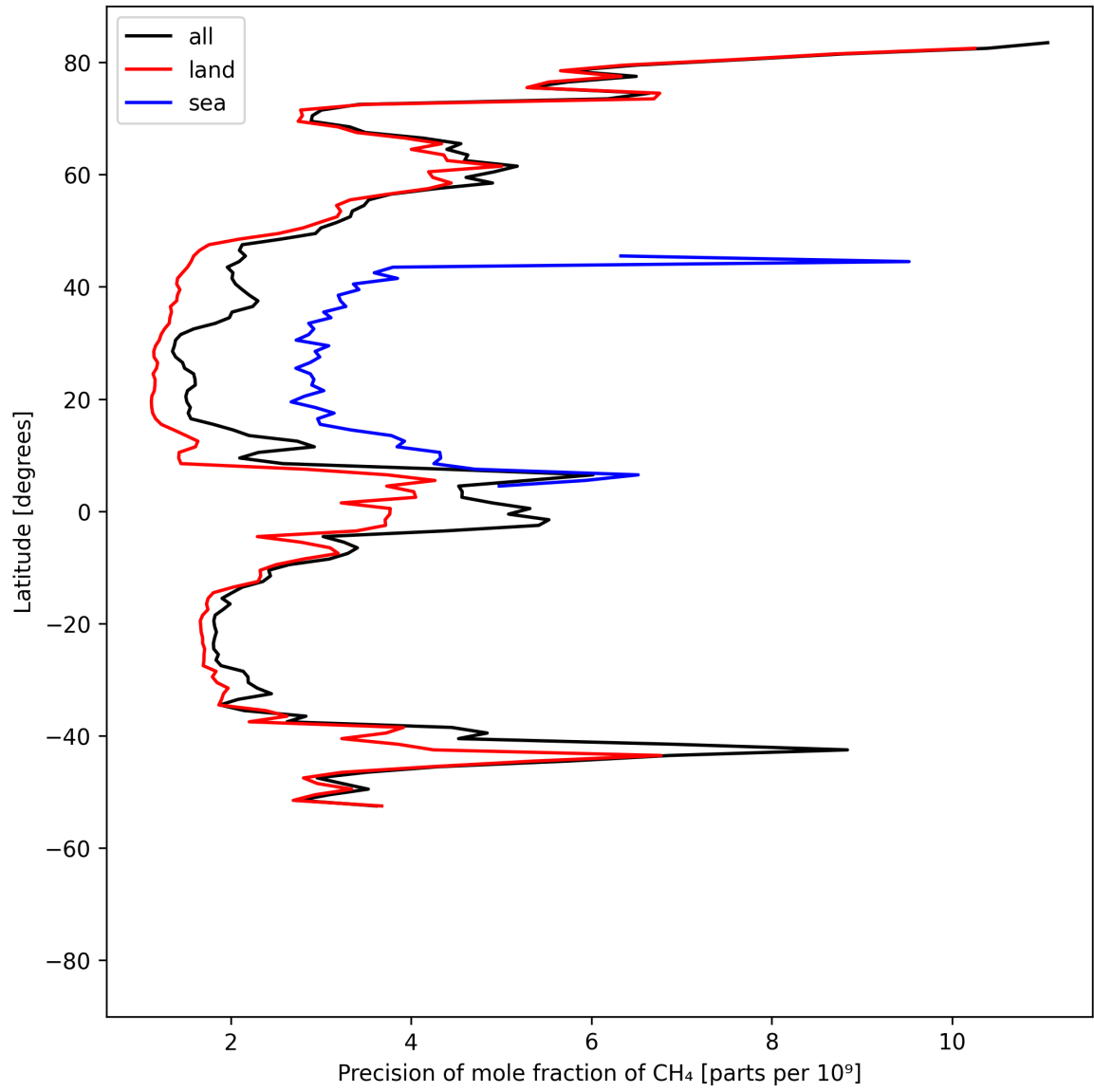
Figure 13: Zonal average of “Precision of mole fraction of CH 4 ” for 2025-07-24 to 2025-07-26.
