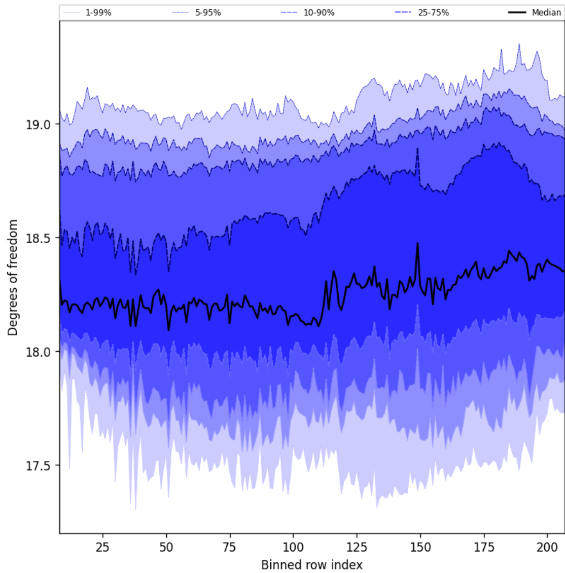
Figure 41: Along track statistics of “Degrees of freedom” for 2025-07-24 to 2025-07-26
