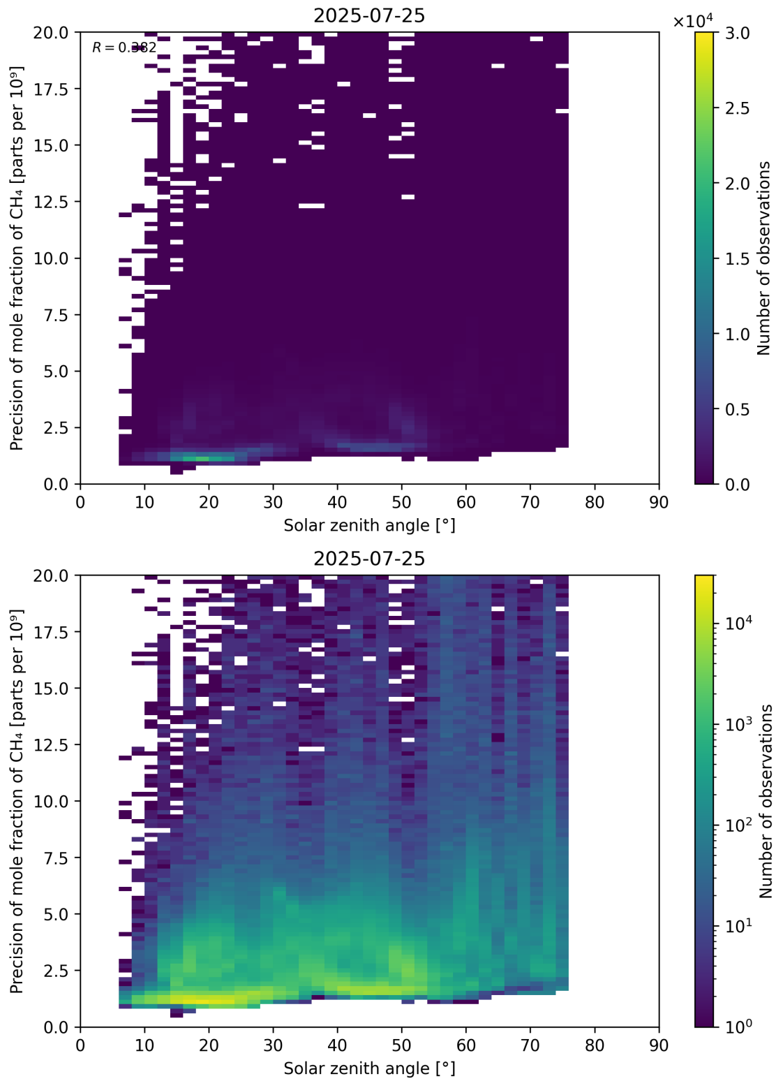
Figure 101: Scatter density plot of “Solar zenith angle” against “Precision of mole fraction of CH 4 ” for 2025-07-24 to 2025-07-26.
