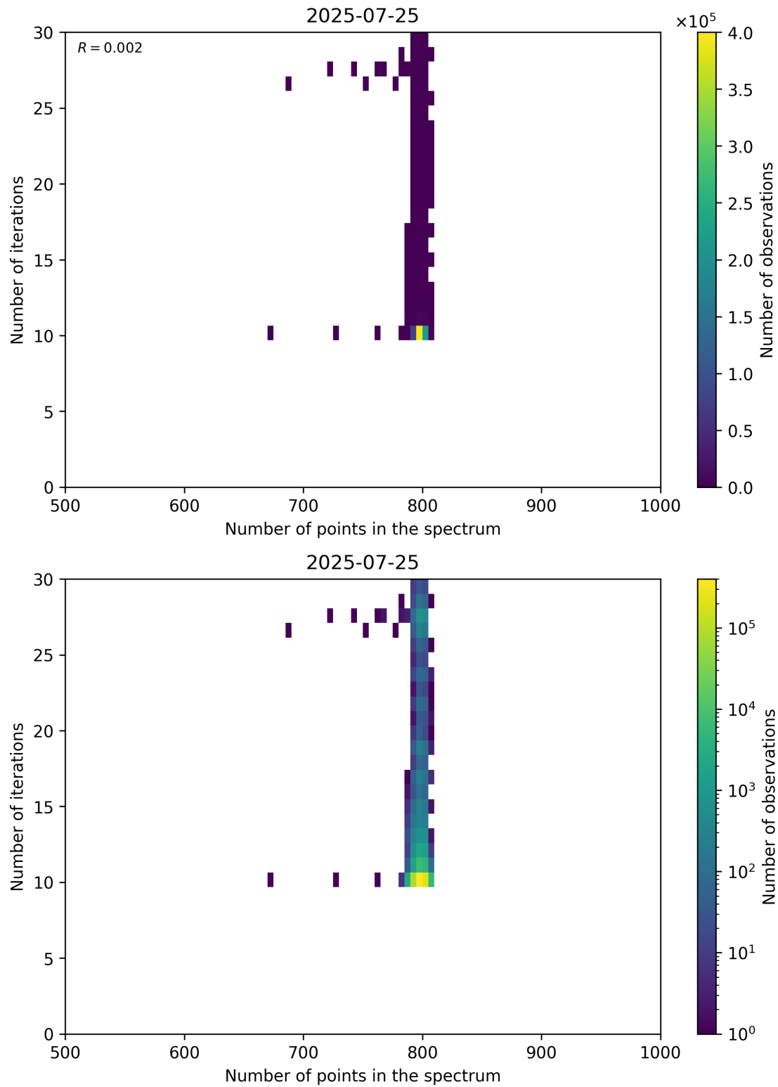
Figure 92: Scatter density plot of “Number of points in the spectrum” against “Number of iterations” for 2025-07-24 to 2025-07-26.
