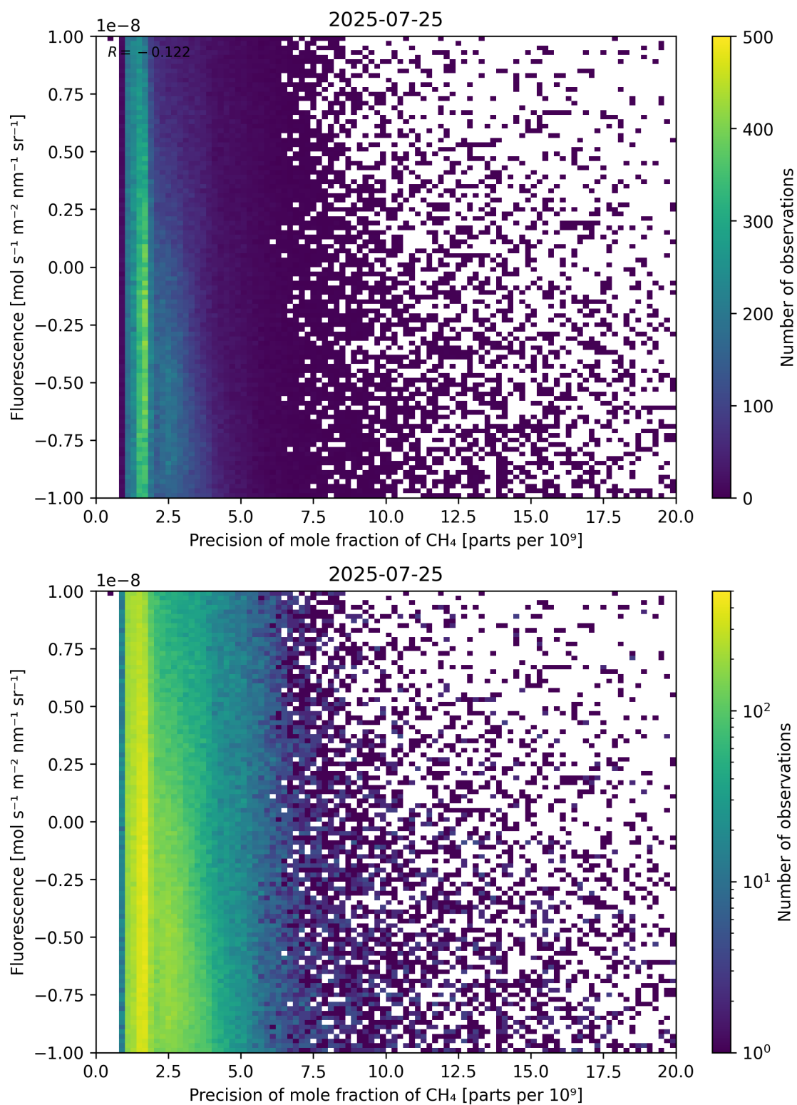
Figure 81: Scatter density plot of “Precision of mole fraction of \text{CH}_4 ” against “Fluorescence” for 2025-07-24 to 2025-07-26.
