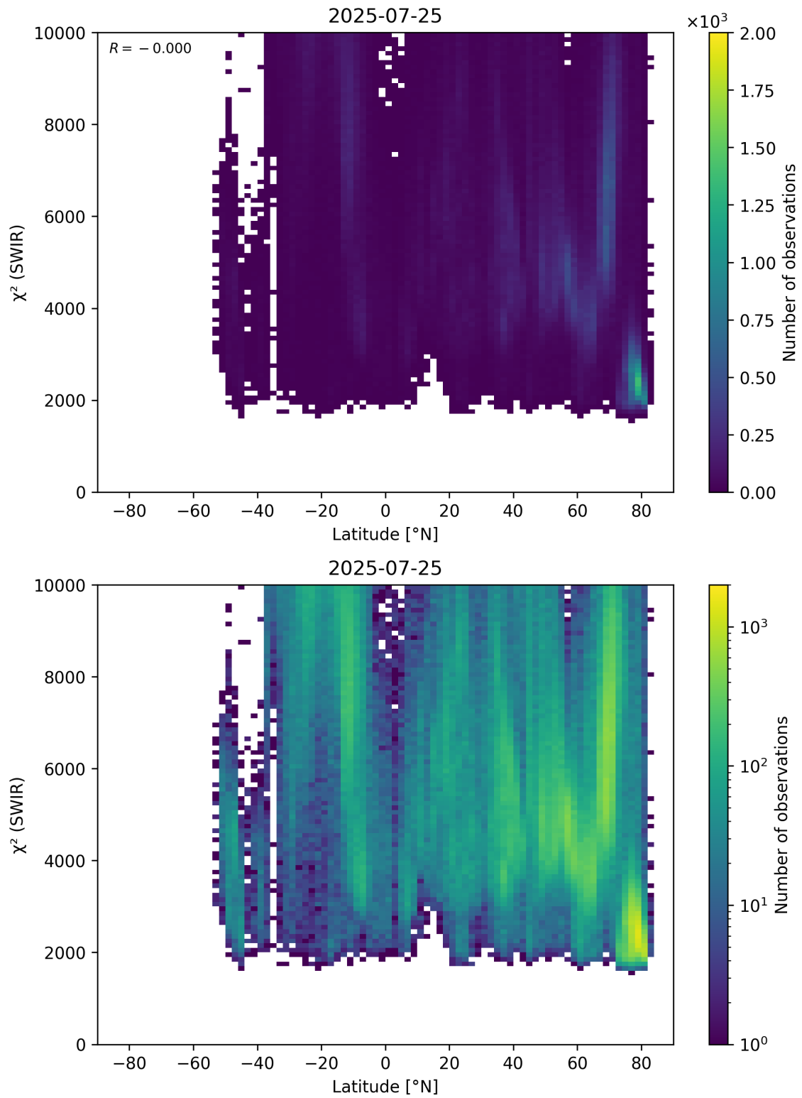
Figure 54: Scatter density plot of “Latitude” against “ \chi^2 (SWIR)” for 2025-07-24 to 2025-07-26.
