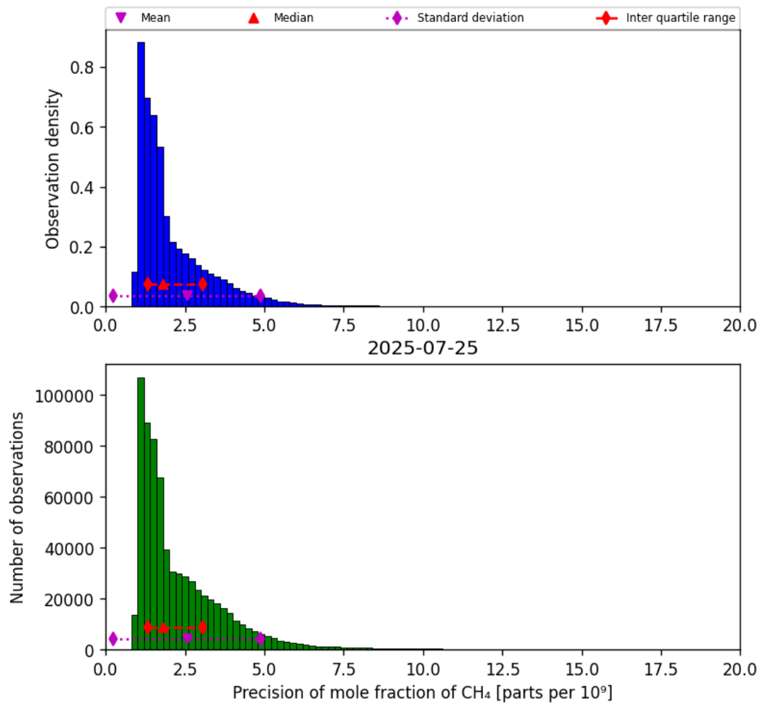
Figure 24: Histogram of “Precision of mole fraction of CH 4 ” for 2025-07-24 to 2025-07-26
