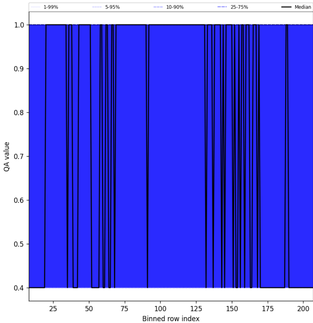
Figure 33: Along track statistics of “QA value” for 2025-07-24 to 2025-07-26
