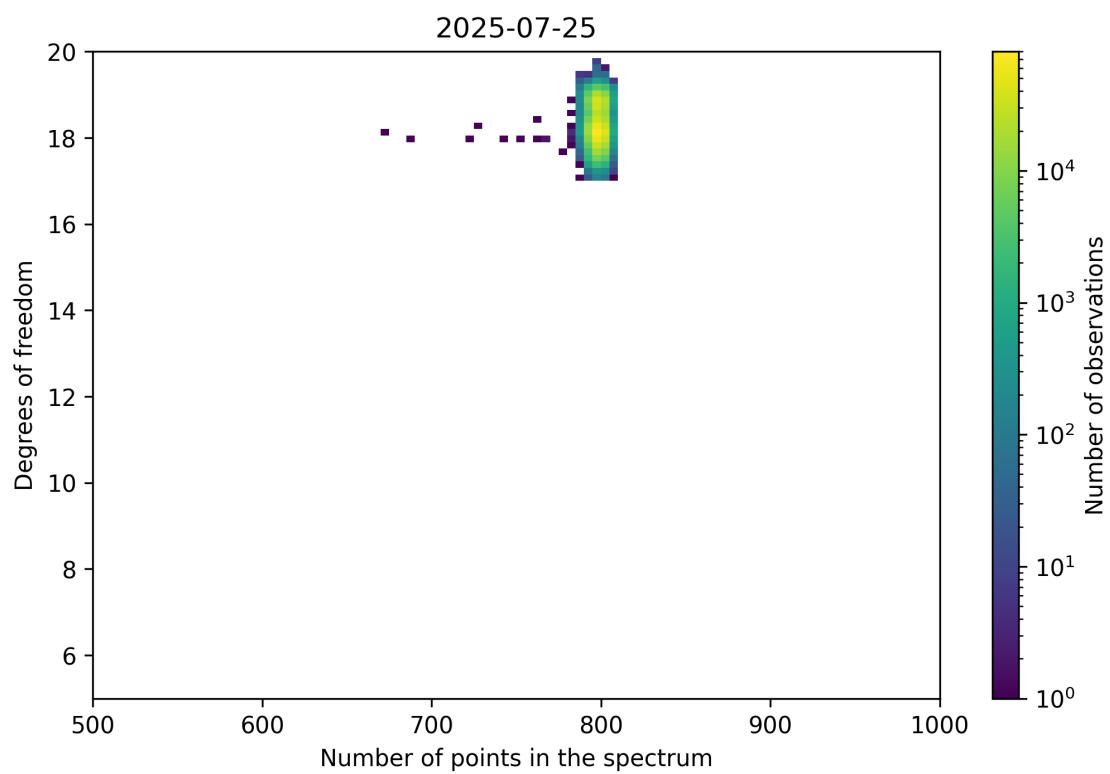
Figure 90: Scatter density plot of “Number of points in the spectrum” against “Degrees of freedom” for 2025-07-24 to 2025-07-26.
