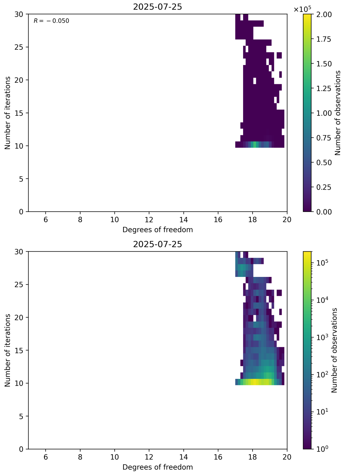
Figure 52: Scatter density plot of “Degrees of freedom” against “Number of iterations” for 2025-07-24 to 2025-07-26.
