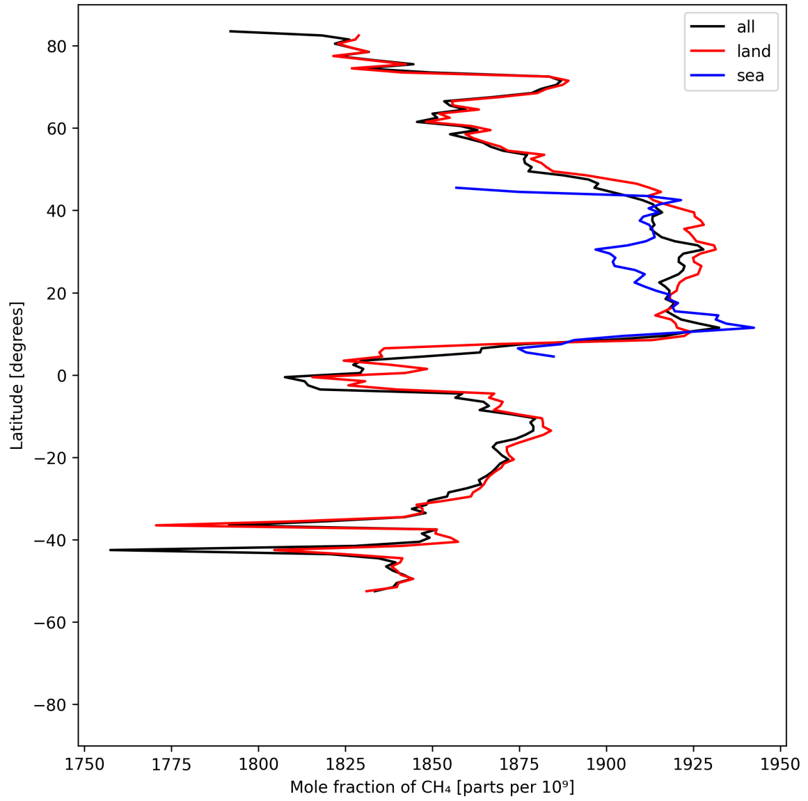
Figure 12: Zonal average of “Mole fraction of \text{CH}_4 ” for 2025-07-24 to 2025-07-26.
