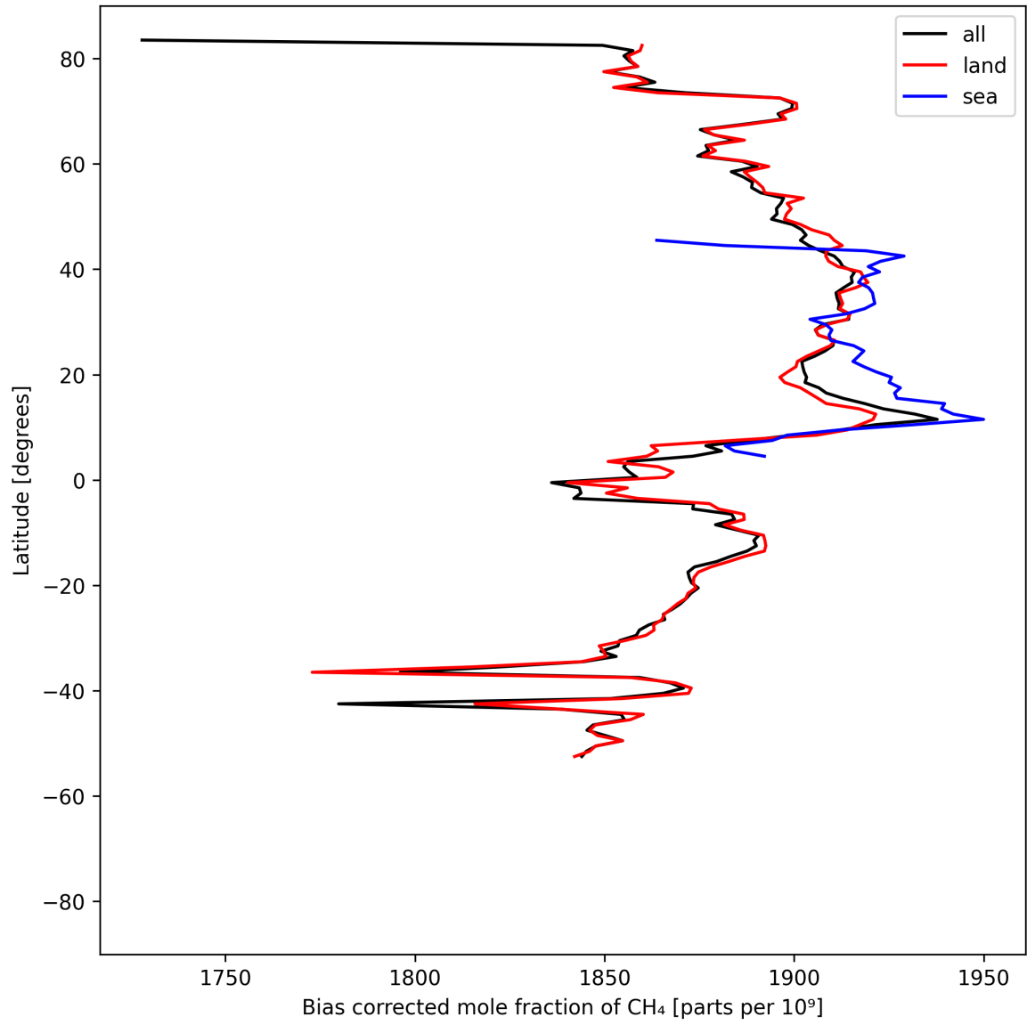
Figure 14: Zonal average of “Bias corrected mole fraction of CH 4 ” for 2025-07-24 to 2025-07-26.
