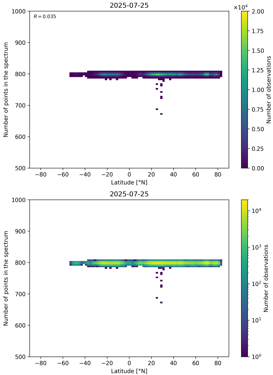
Figure 61: Scatter density plot of “Latitude” against “Number of points in the spectrum” for 2025-07-24 to 2025-07-26.
