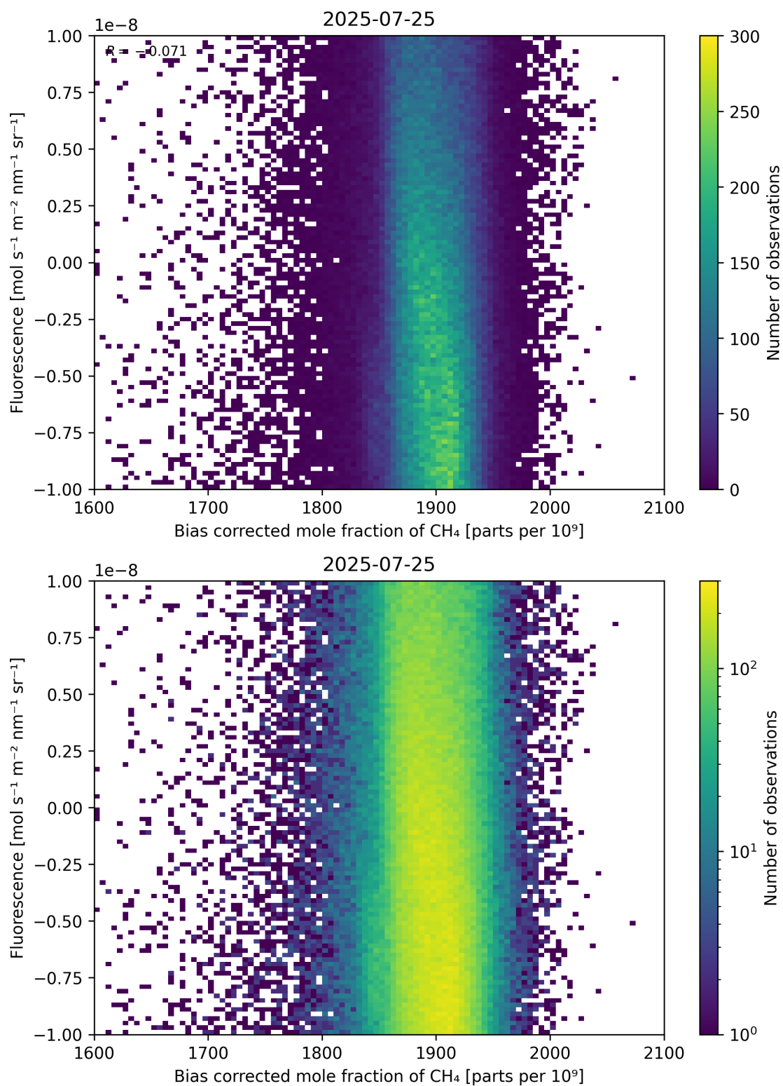
Figure 66: Scatter density plot of “Bias corrected mole fraction of \text{CH}_4 ” against “Fluorescence” for 2025-07-24 to 2025-07-26.
