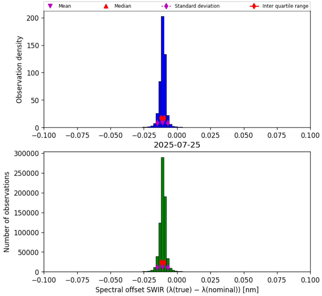
Figure 27: Histogram of “Spectral offset SWIR ( \lambda_{\text{true}} - \lambda_{\text{nominal}} )” for 2025-07-24 to 2025-07-26
