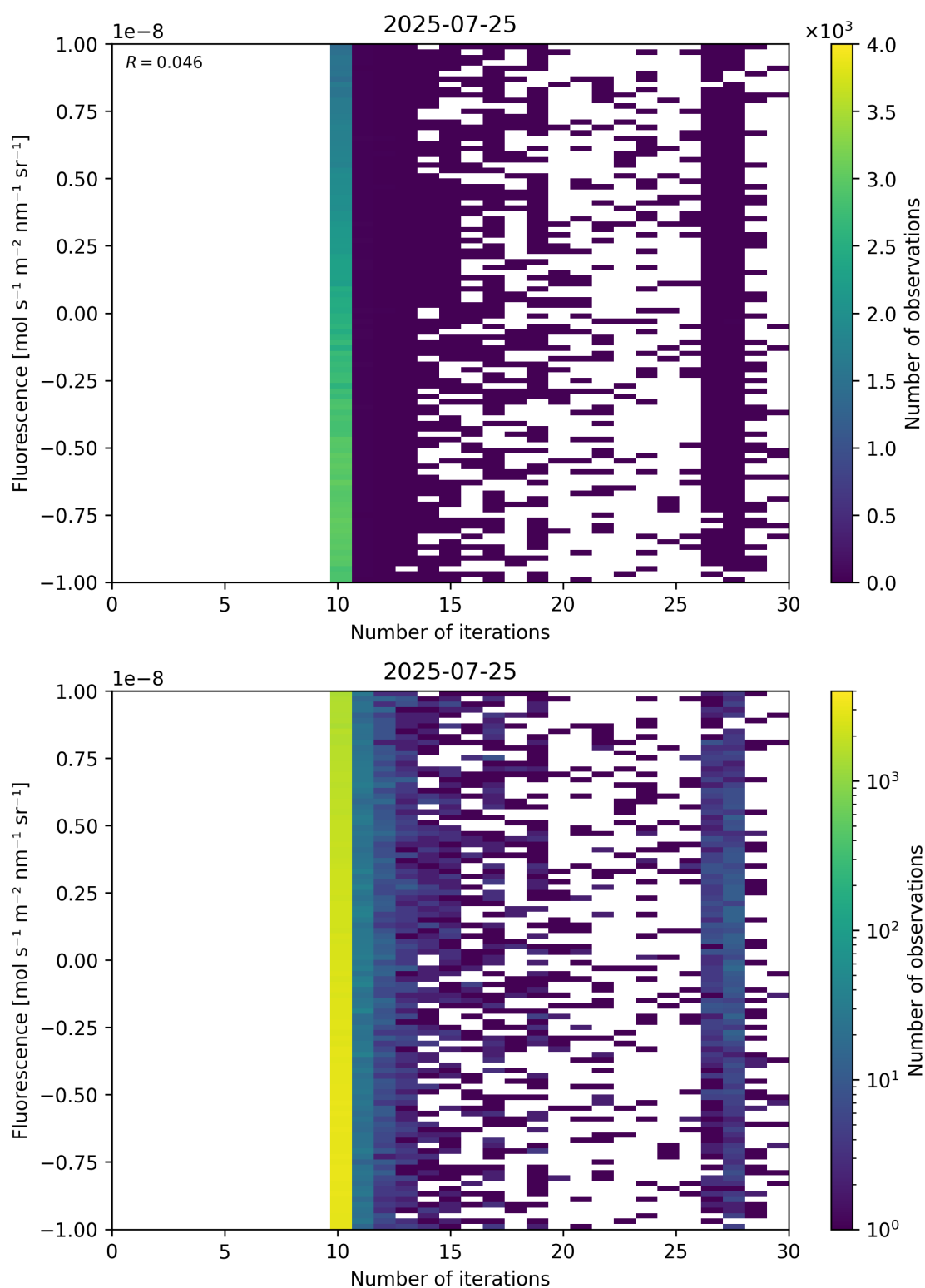
Figure 87: Scatter density plot of “Number of iterations” against “Fluorescence” for 2025-07-24 to 2025-07-26.
