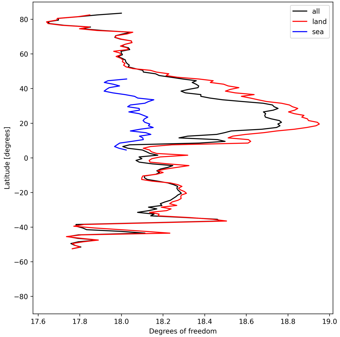
Figure 19: Zonal average of “Degrees of freedom” for 2025-07-24 to 2025-07-26.
