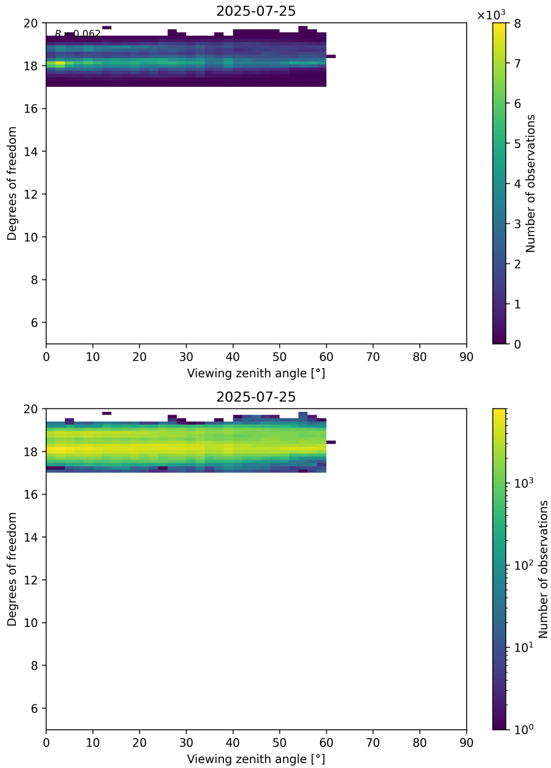
Figure 107: Scatter density plot of “Viewing zenith angle” against “Degrees of freedom” for 2025-07-24 to 2025-07-26.
