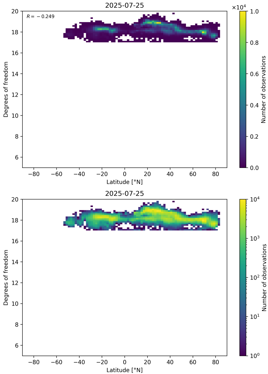
Figure 55: Scatter density plot of “Latitude” against “Degrees of freedom” for 2025-07-24 to 2025-07-26.
