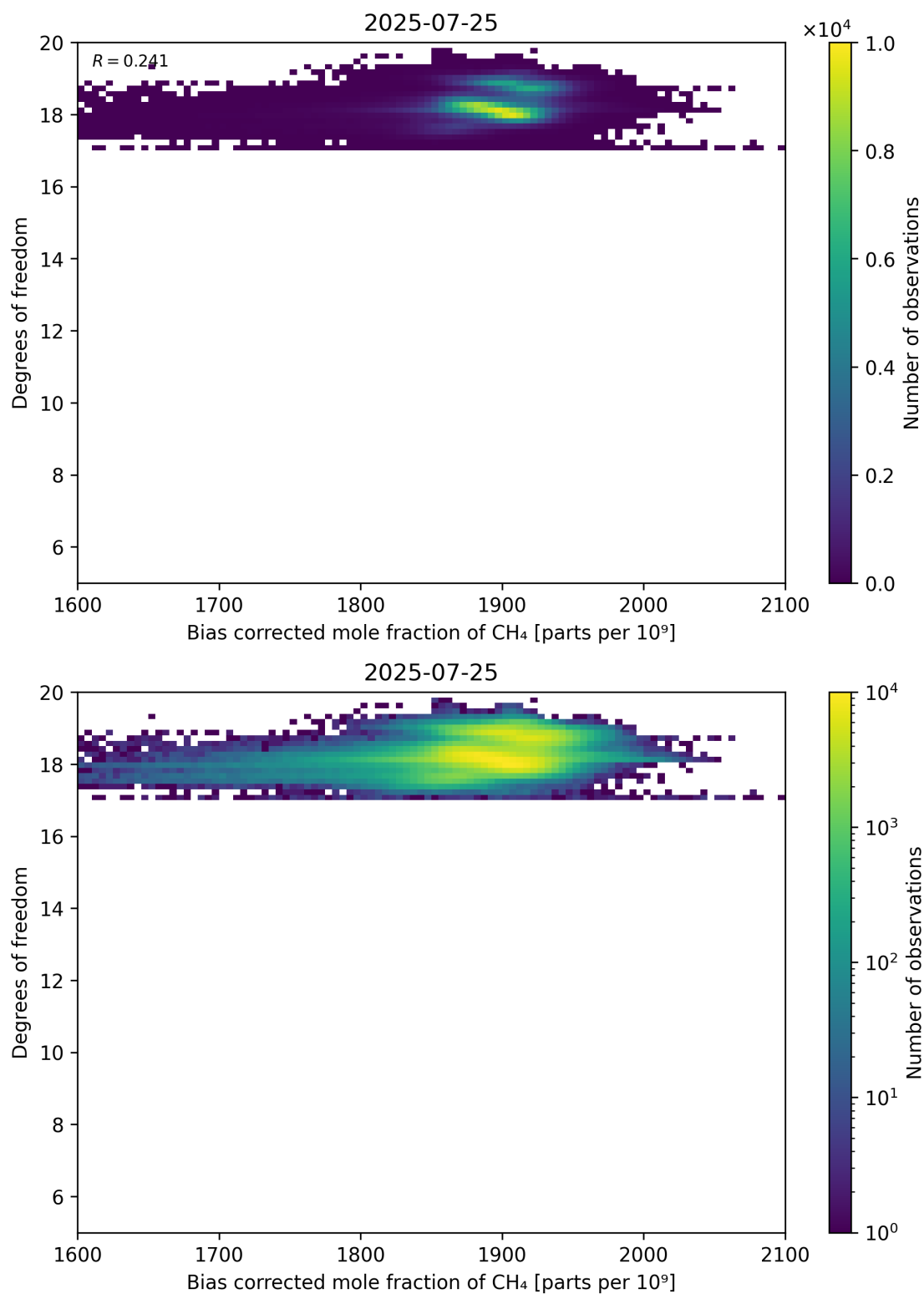
Figure 65: Scatter density plot of “Bias corrected mole fraction of CH 4 ” against “Degrees of freedom” for 2025-07-24 to 2025-07-26.
