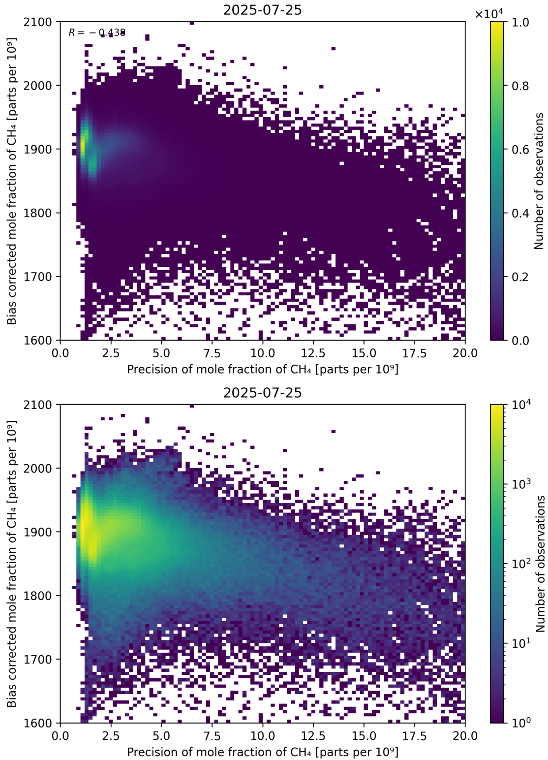
Figure 82: Scatter density plot of “Precision of mole fraction of CH 4 ” against “Bias corrected mole fraction of CH 4 ” for 2025-07-24 to 2025-07-26.
