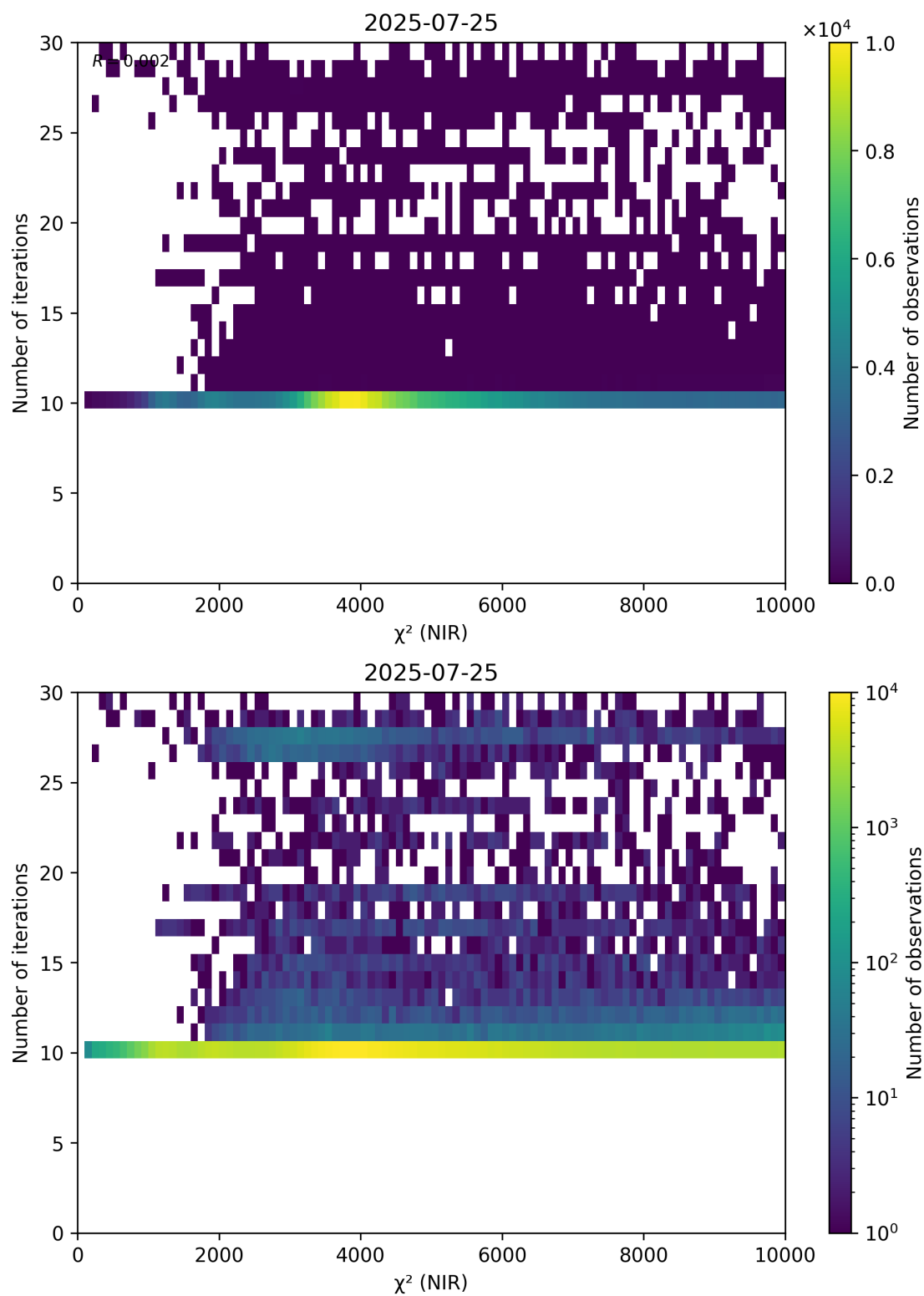
Figure 46: Scatter density plot of “ \chi^2 (NIR)” against “Number of iterations” for 2025-07-24 to 2025-07-26.
