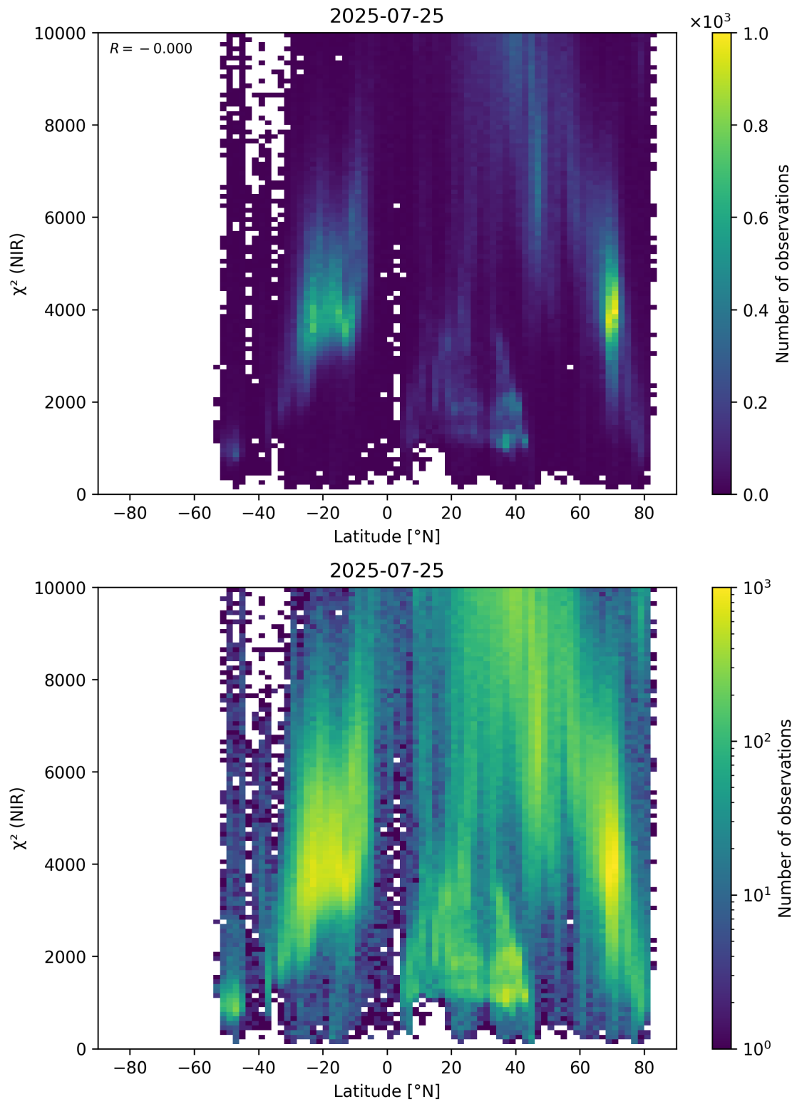
Figure 53: Scatter density plot of “Latitude” against “ \chi^2 (NIR)” for 2025-07-24 to 2025-07-26.
