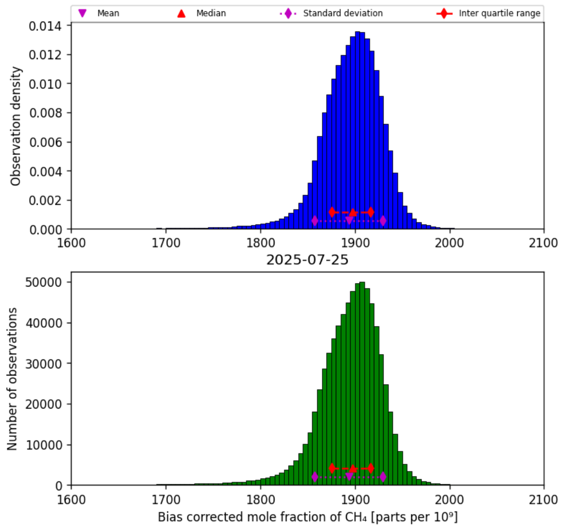
Figure 25: Histogram of “Bias corrected mole fraction of CH 4 ” for 2025-07-24 to 2025-07-26
