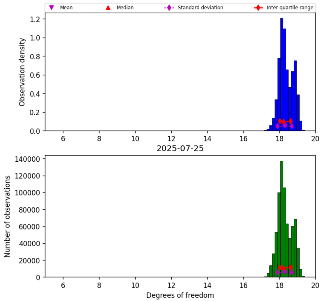
Figure 30: Histogram of “Degrees of freedom” for 2025-07-24 to 2025-07-26
