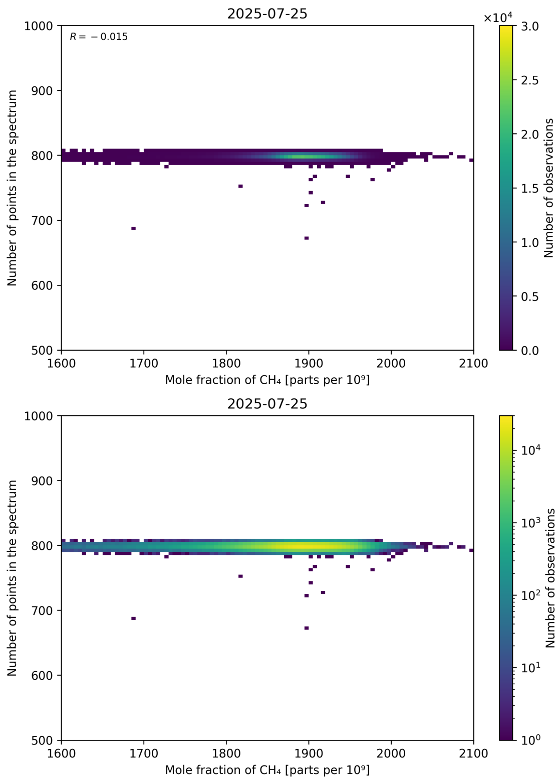
Figure 77: Scatter density plot of “Mole fraction of CH 4 ” against “Number of points in the spectrum” for 2025-07-24 to 2025-07-26.
