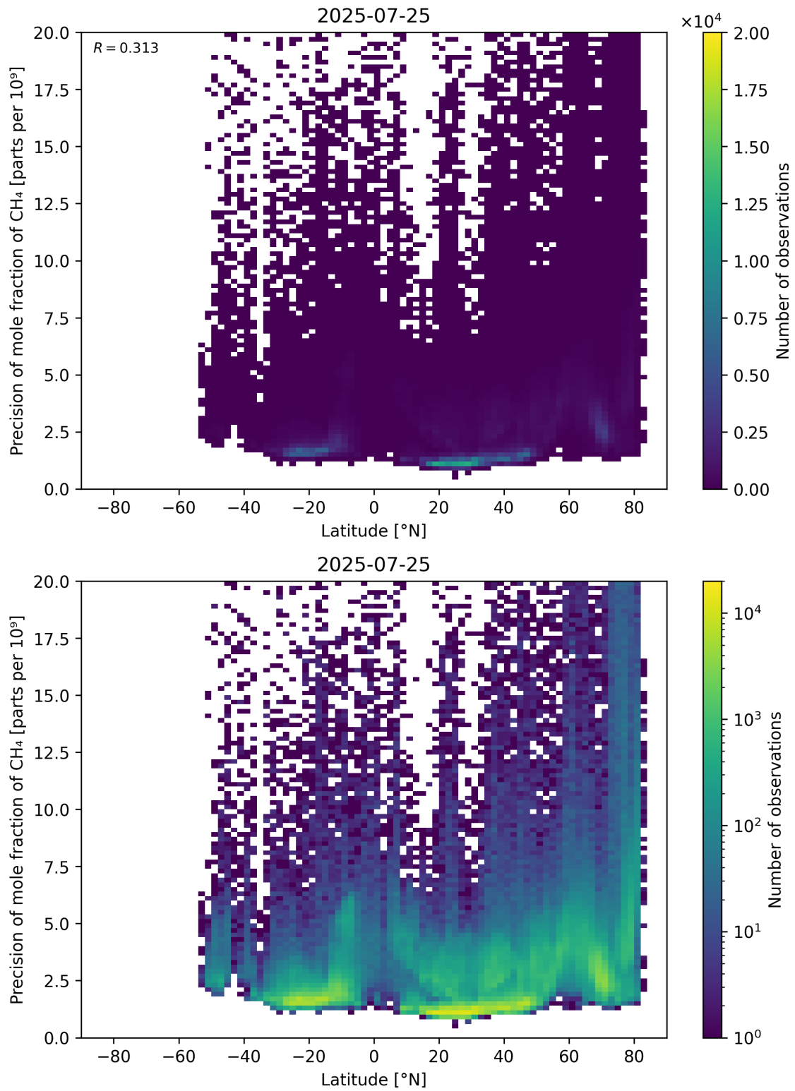
Figure 59: Scatter density plot of “Latitude” against “Precision of mole fraction of \text{CH}_4 ” for 2025-07-24 to 2025-07-26.
