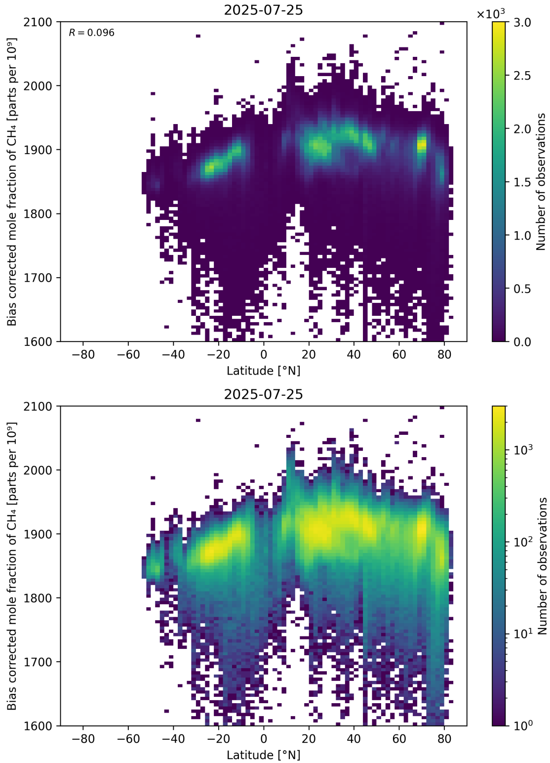
Figure 58: Scatter density plot of “Latitude” against “Bias corrected mole fraction of \text{CH}_4 ” for 2025-07-24 to 2025-07-26.
