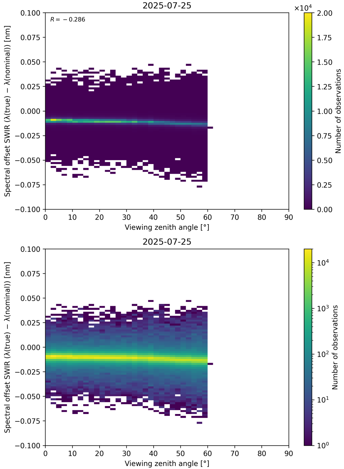
Figure 116: Scatter density plot of “Viewing zenith angle” against “Spectral offset SWIR ( \lambda_{\text{true}} - \lambda_{\text{nominal}} )” for 2025-07-24 to 2025-07-26.
