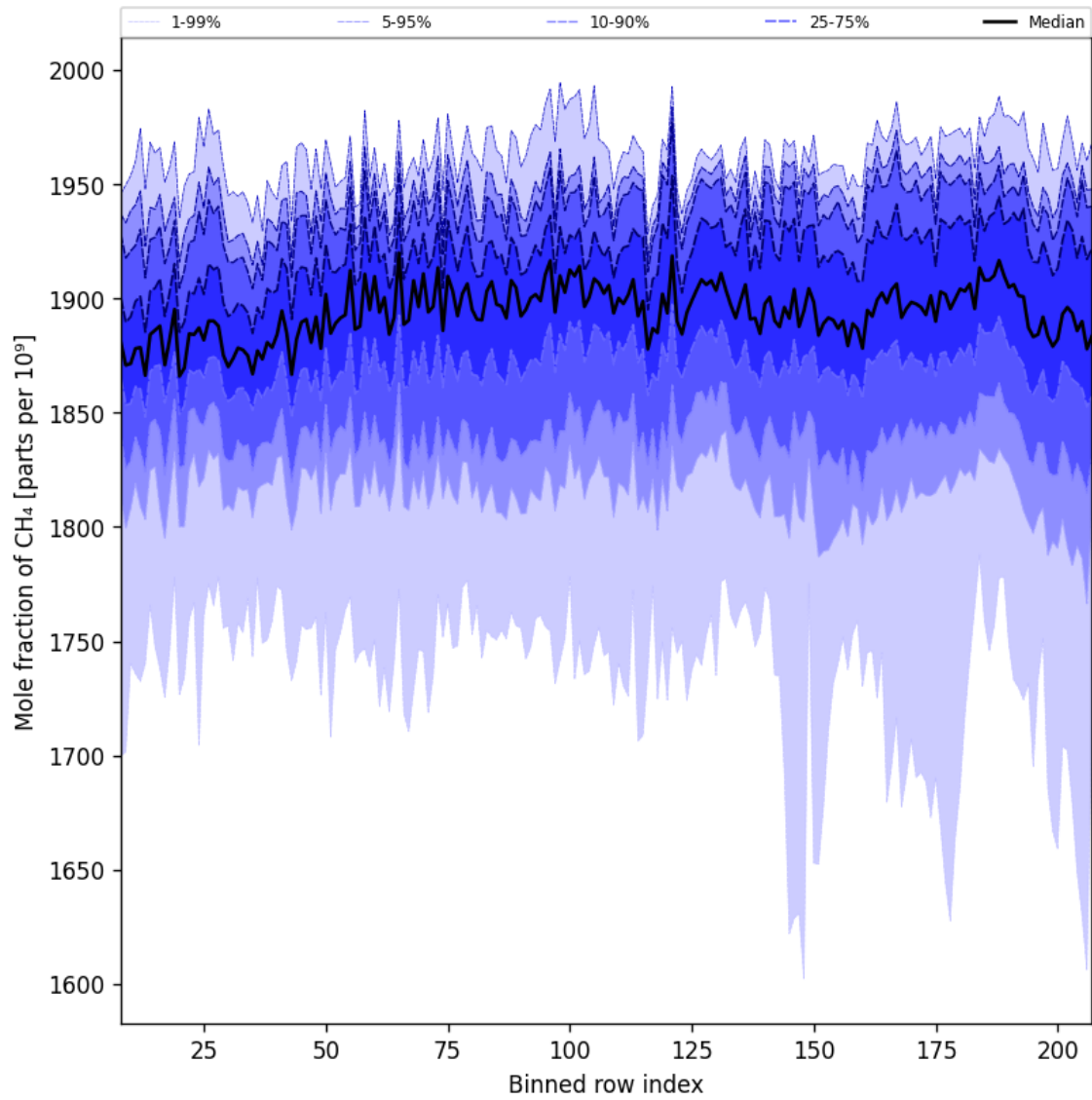
Figure 34: Along track statistics of “Mole fraction of CH 4 ” for 2025-07-24 to 2025-07-26
