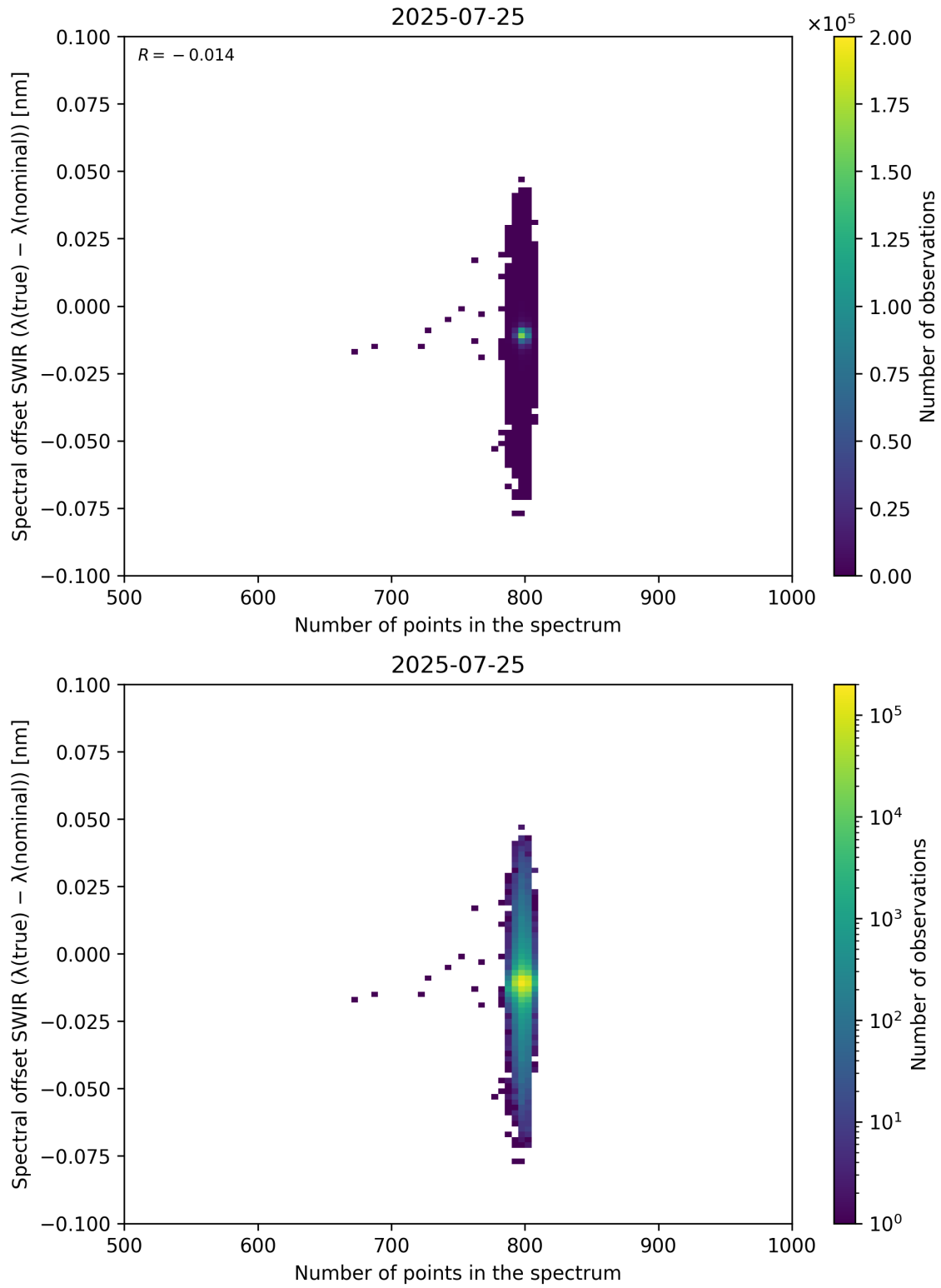
Figure 93: Scatter density plot of “Number of points in the spectrum” against “Spectral offset SWIR ( \lambda_{\text{true}} - \lambda_{\text{nominal}} )” for 2025-07-24 to 2025-07-26.
