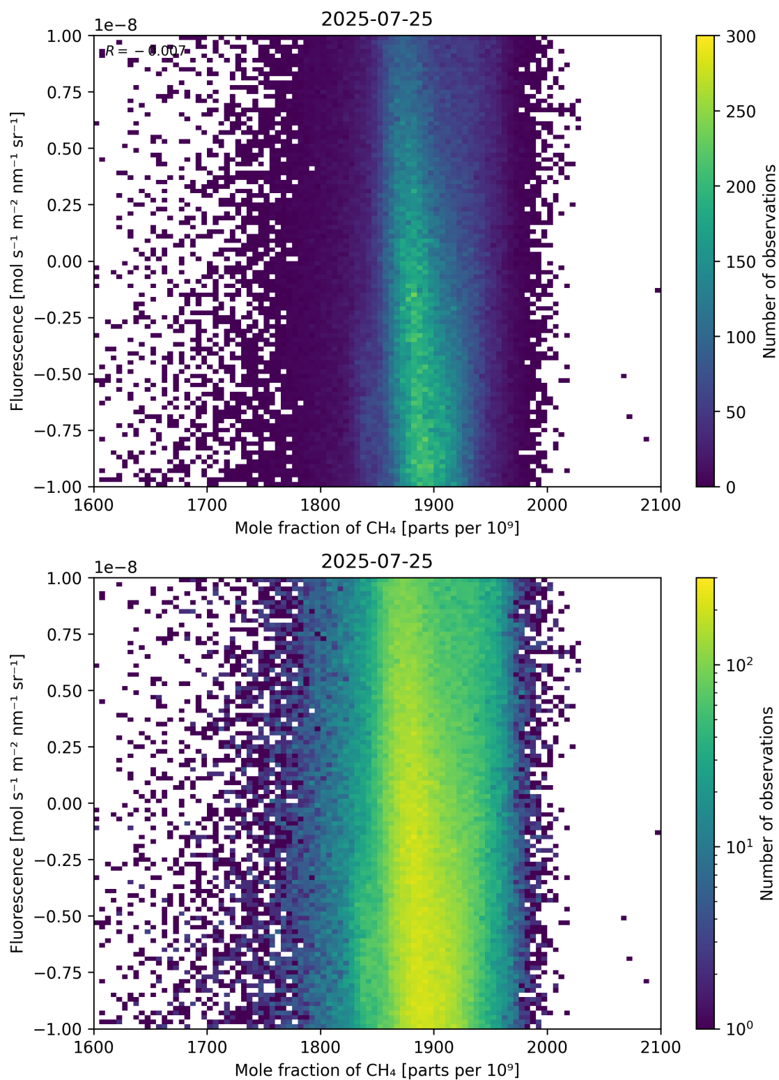
Figure 73: Scatter density plot of “Mole fraction of \text{CH}_4 ” against “Fluorescence” for 2025-07-24 to 2025-07-26.
