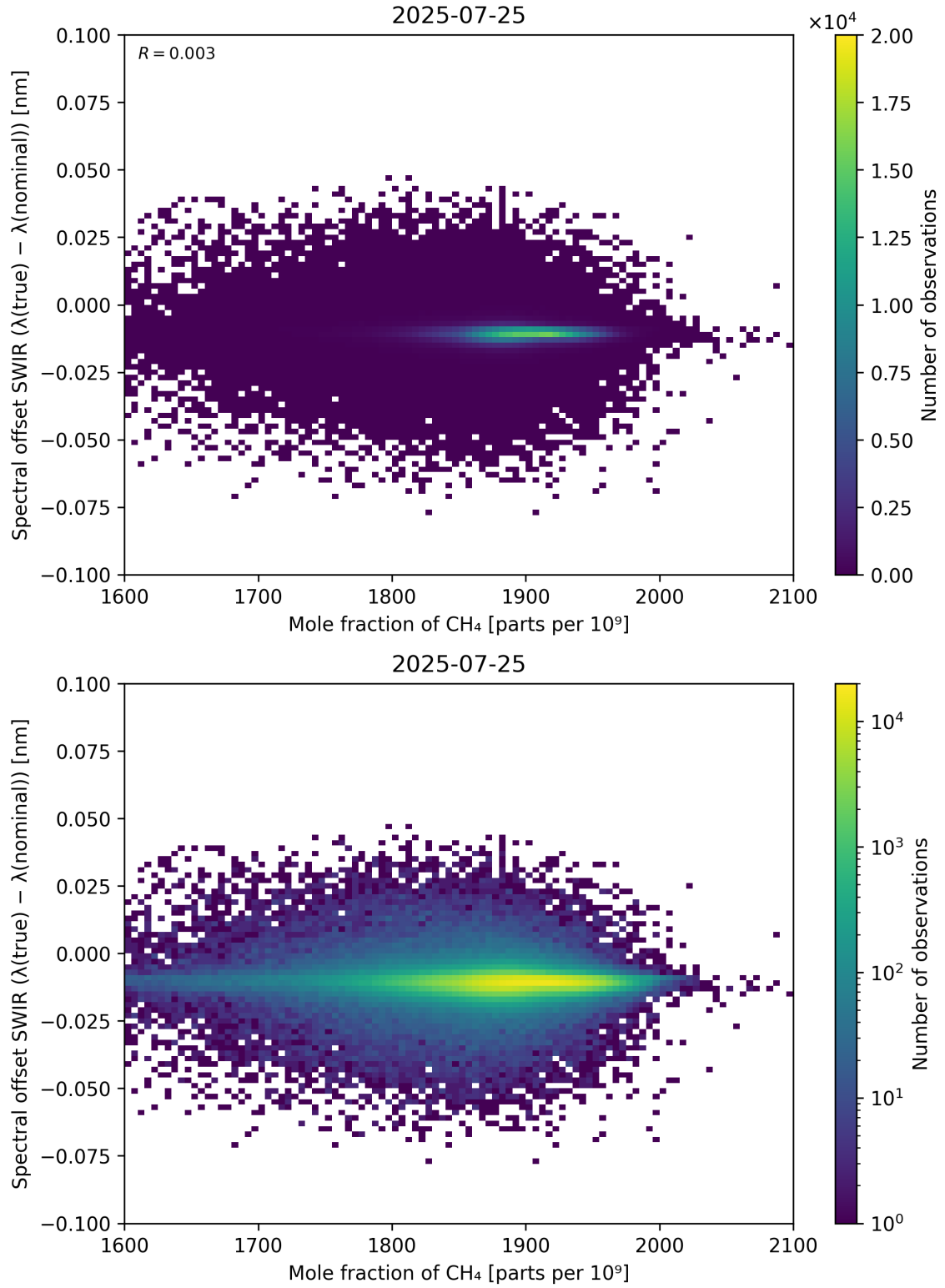
Figure 86: Scatter density plot of “Mole fraction of CH 4 ” against “Spectral offset SWIR ( \lambda_{\text{true}} - \lambda_{\text{nominal}} )” for 2025-07-24 to 2025-07-26.
