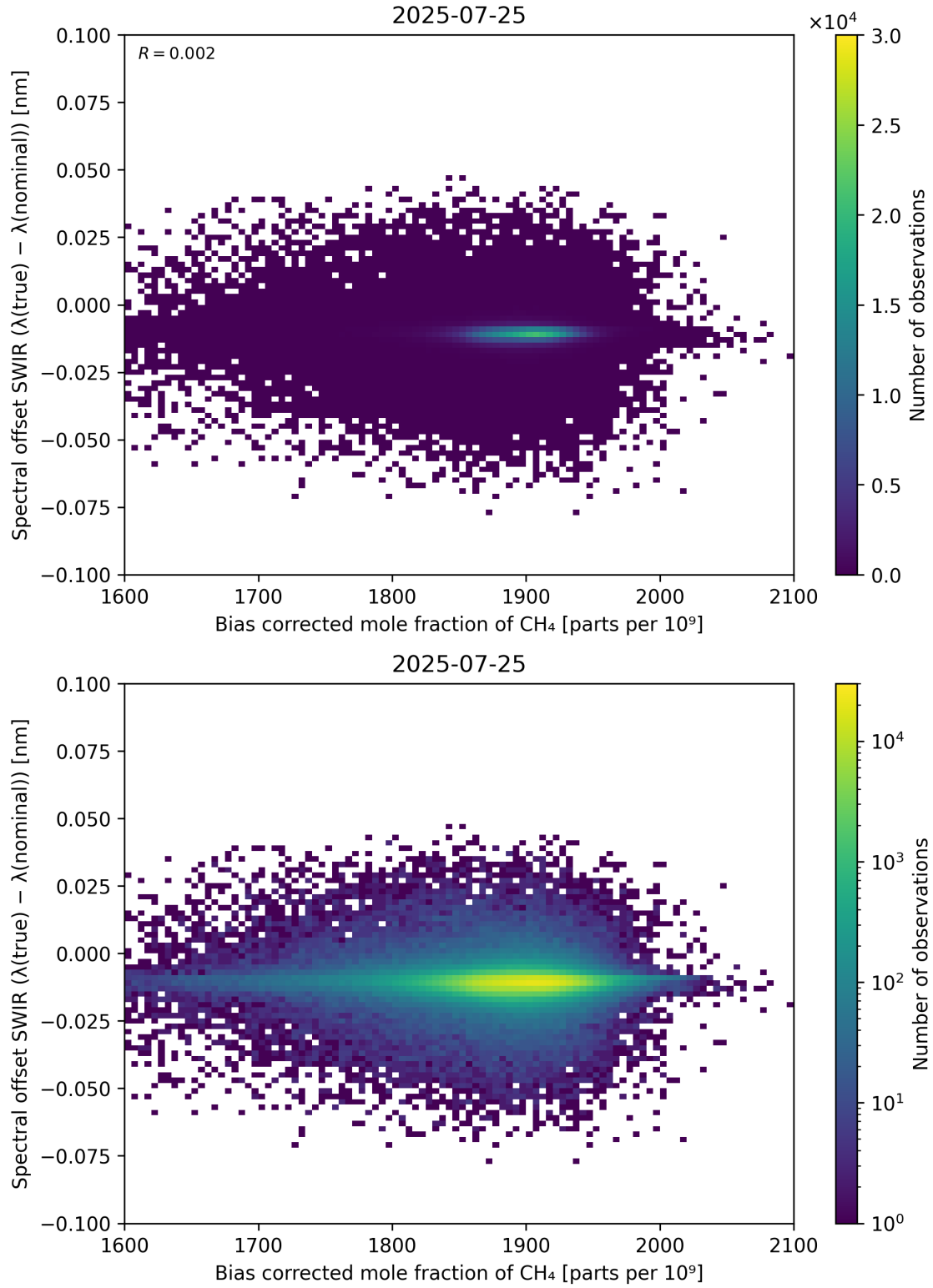
Figure 69: Scatter density plot of “Bias corrected mole fraction of \text{CH}_4 ” against “Spectral offset SWIR ( \lambda_{\text{true}} - \lambda_{\text{nominal}} )” for 2025-07-24 to 2025-07-26.
