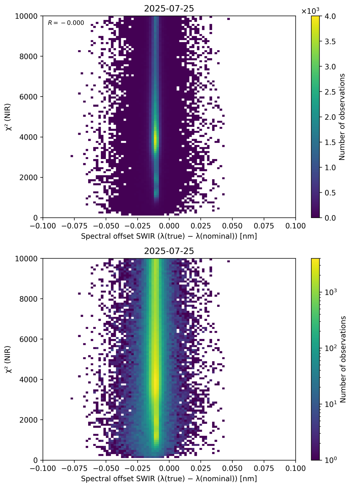
Figure 117: Scatter density plot of “Spectral offset SWIR ( \lambda_{\text{true}} - \lambda_{\text{nominal}} )” against “ \chi^2 (NIR)” for 2025-07-24 to 2025-07-26.
