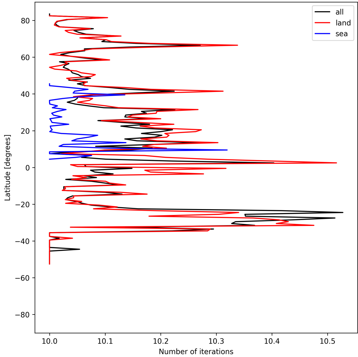
Figure 20: Zonal average of “Number of iterations” for 2025-07-24 to 2025-07-26.
