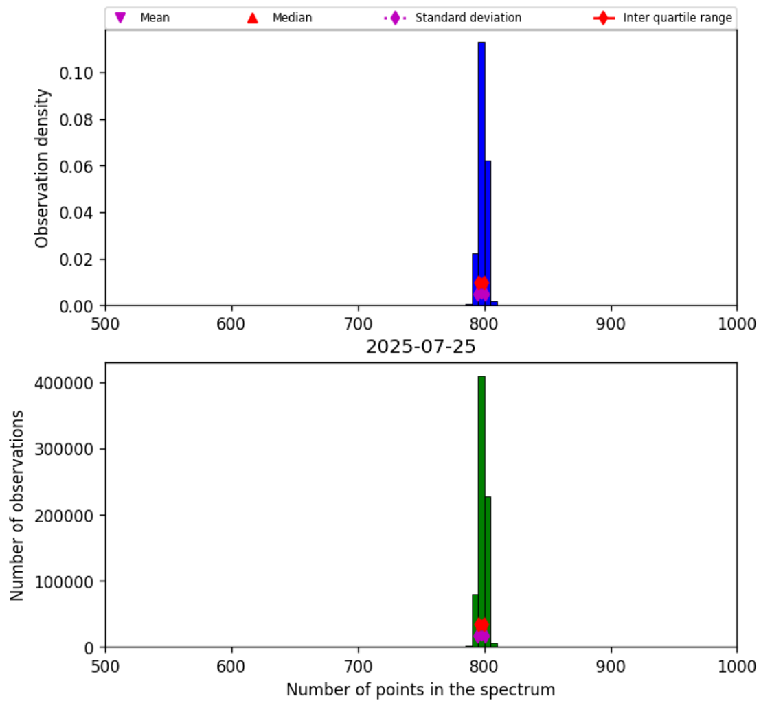
Figure 26: Histogram of “Number of points in the spectrum” for 2025-07-24 to 2025-07-26
