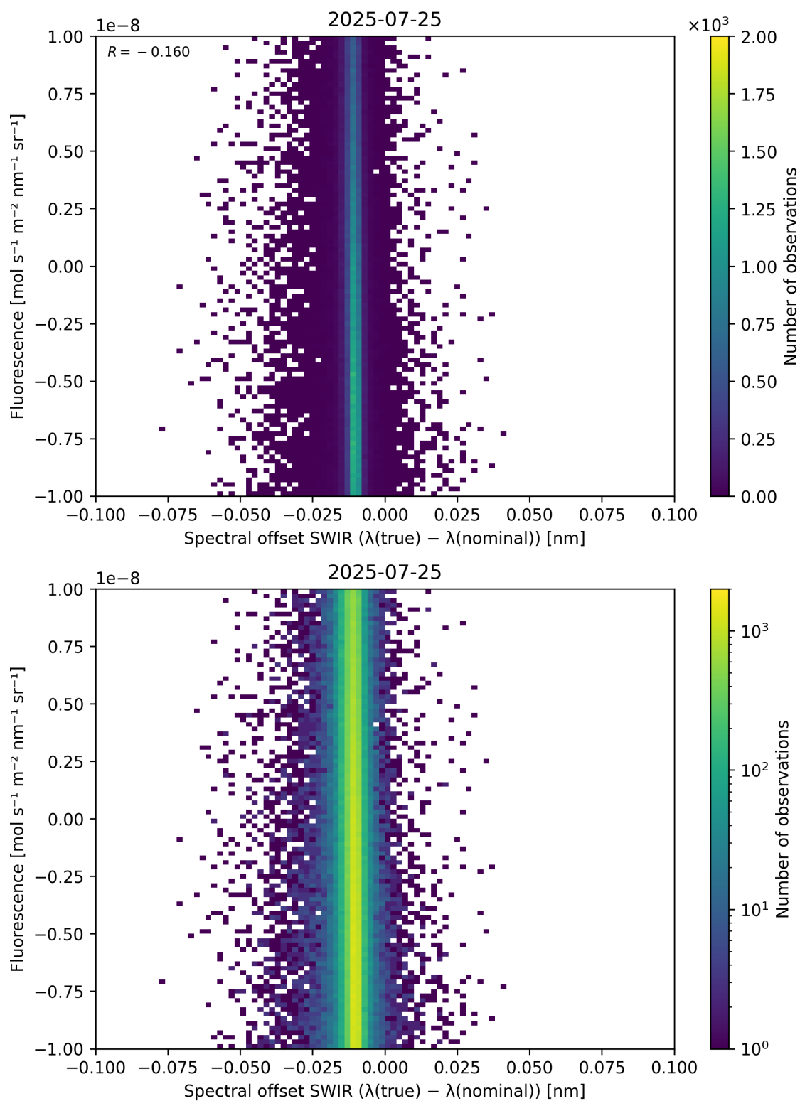
Figure 120: Scatter density plot of “Spectral offset SWIR ( \lambda_{\text{true}} - \lambda_{\text{nominal}} )” against “Fluorescence” for 2025-07-24 to 2025-07-26.
