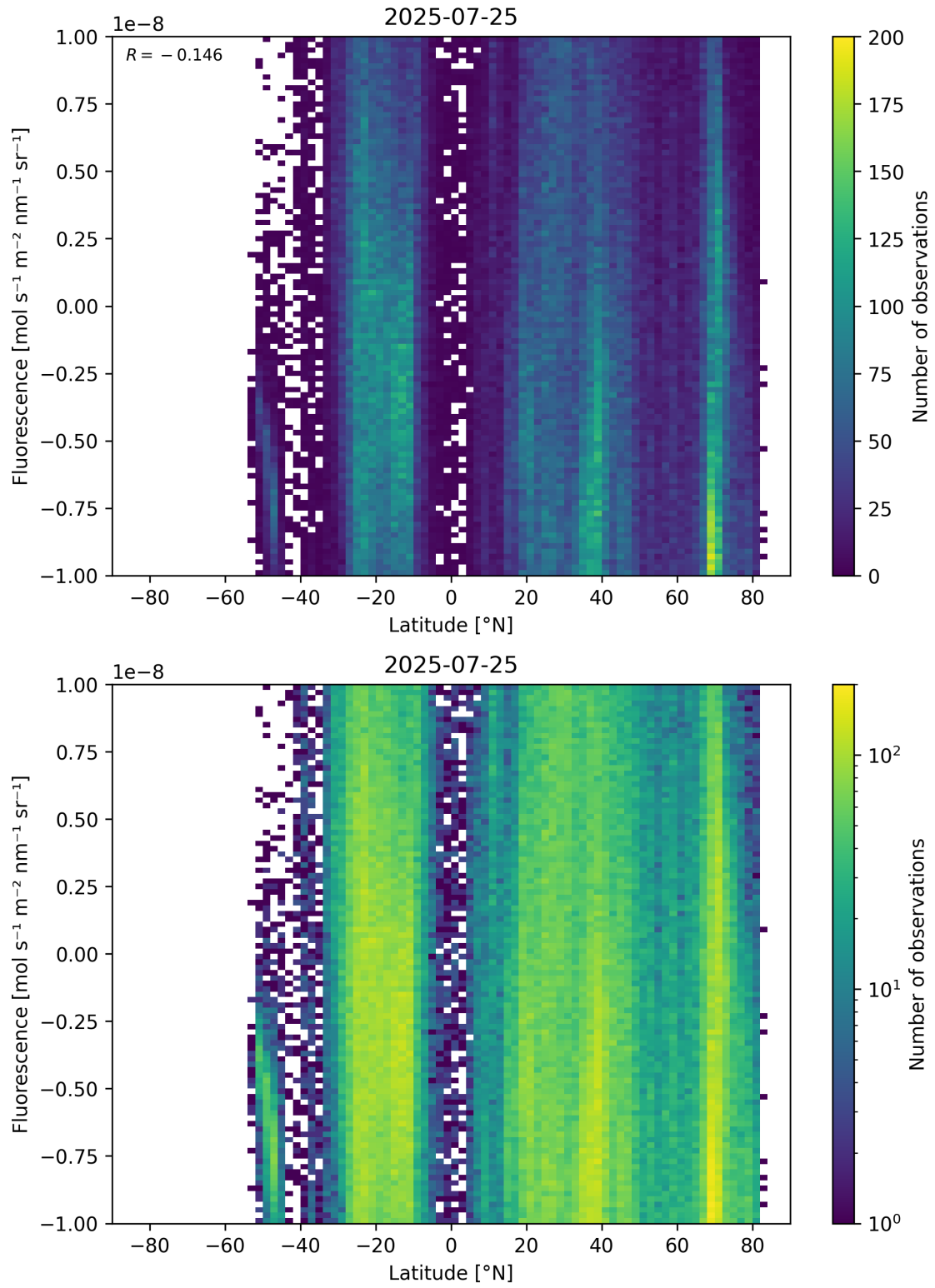
Figure 56: Scatter density plot of “Latitude” against “Fluorescence” for 2025-07-24 to 2025-07-26.
