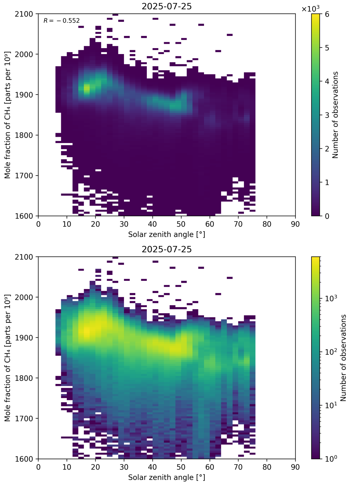
Figure 99: Scatter density plot of “Solar zenith angle” against “Mole fraction of CH 4 ” for 2025-07-24 to 2025-07-26.
