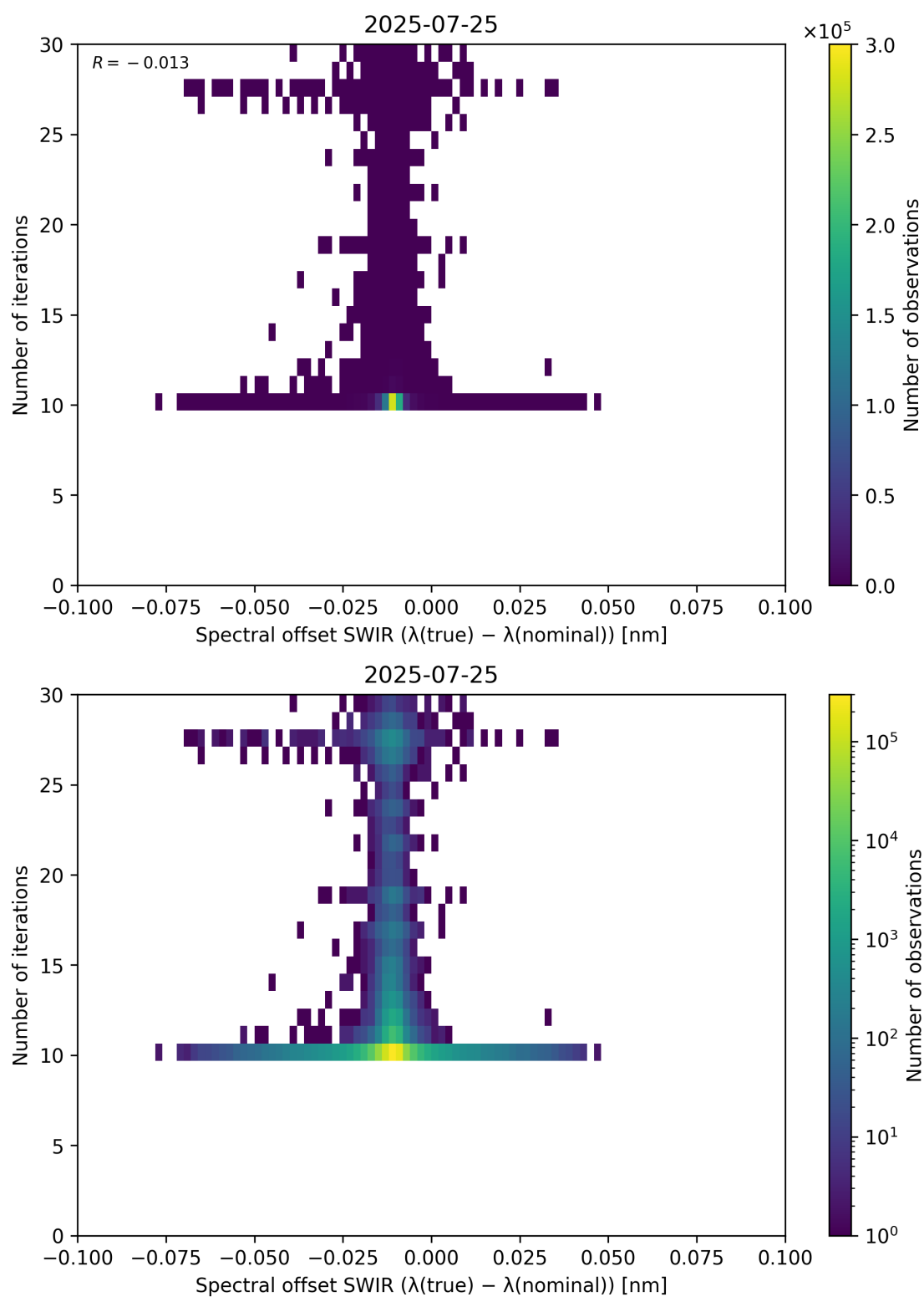
Figure 121: Scatter density plot of “Spectral offset SWIR ( \lambda_{\text{true}} - \lambda_{\text{nominal}} )” against “Number of iterations” for 2025-07-24 to 2025-07-26.
