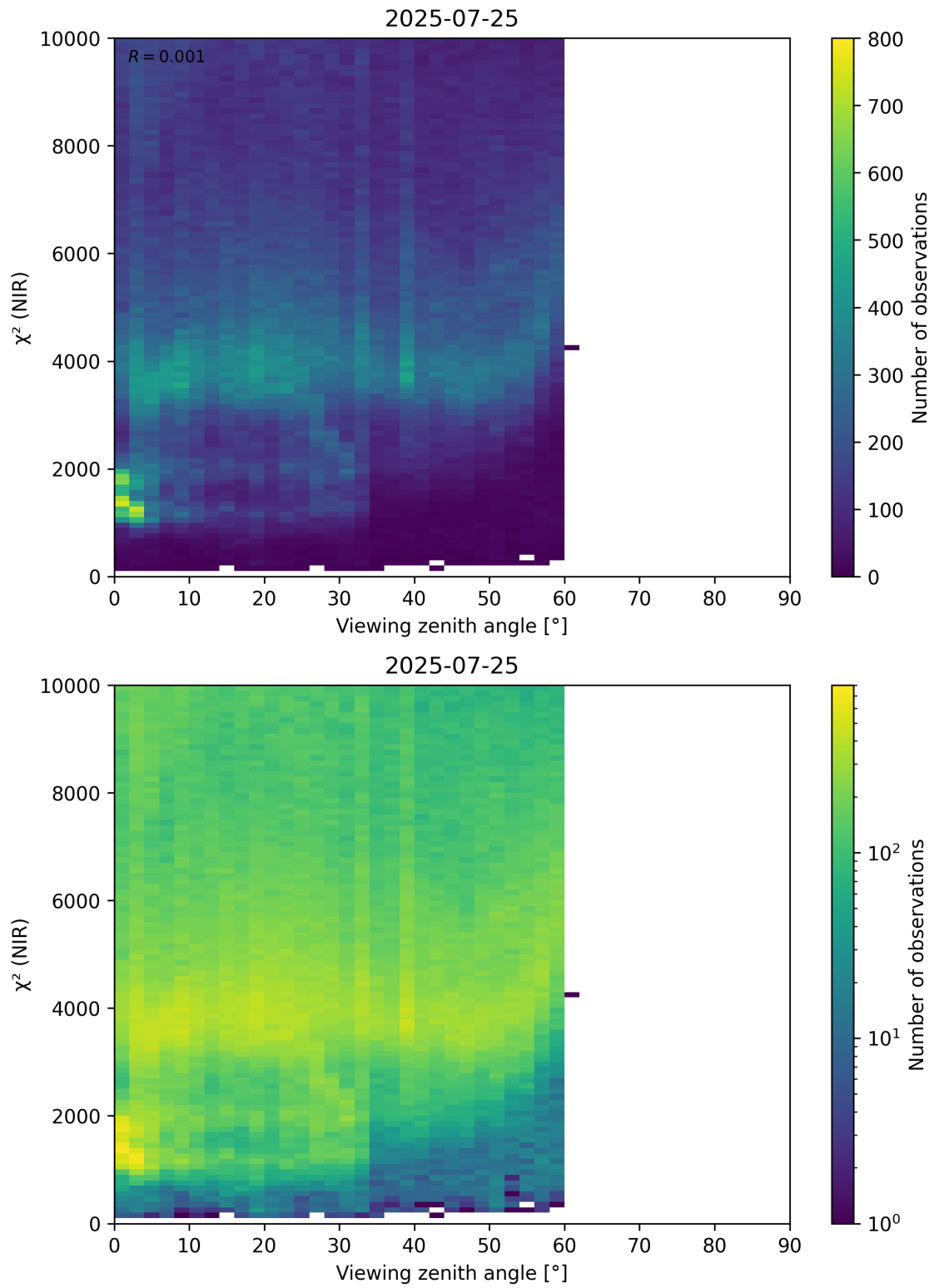
Figure 105: Scatter density plot of “Viewing zenith angle” against “ \chi^2 (NIR)” for 2025-07-24 to 2025-07-26.
