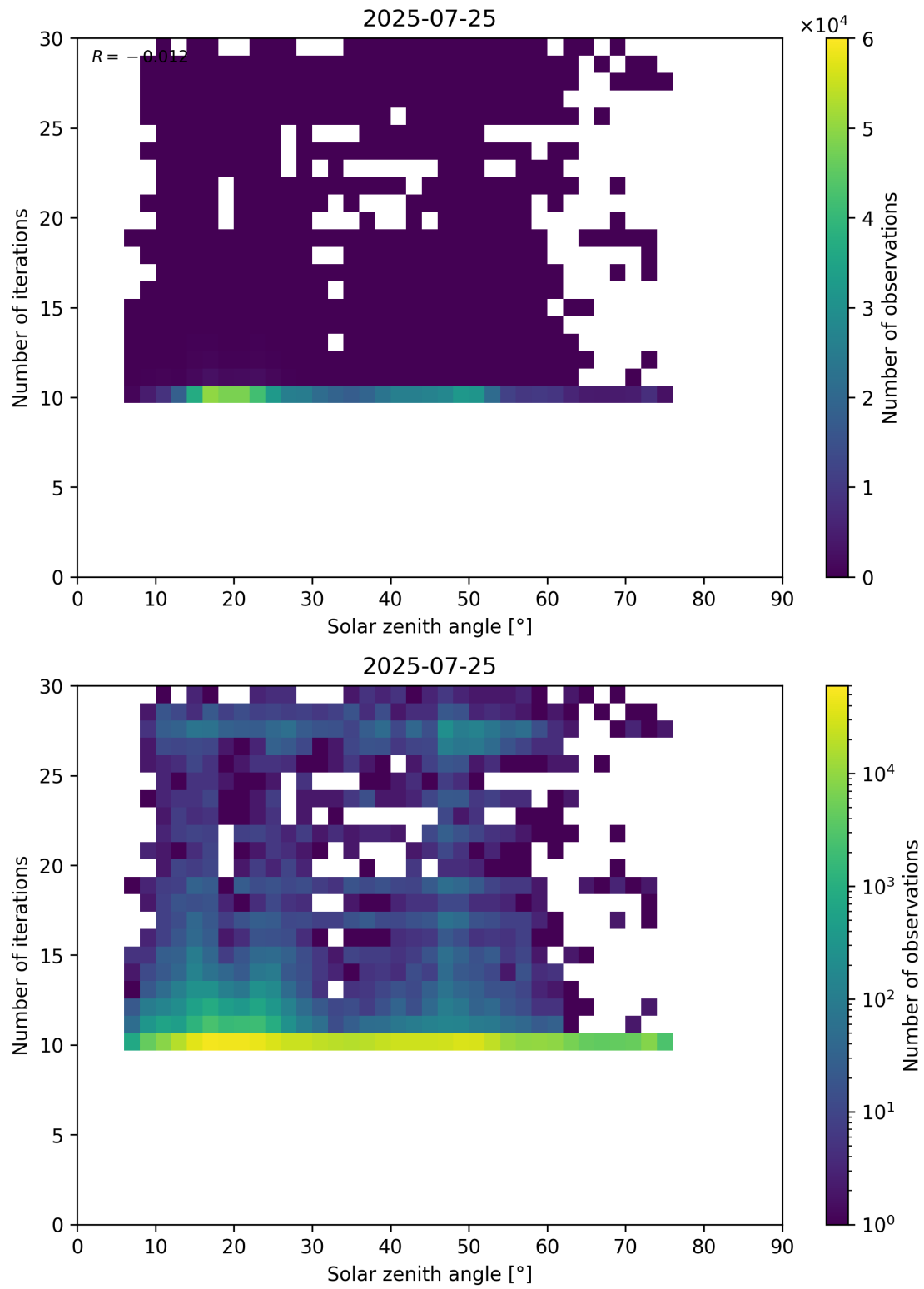
Figure 102: Scatter density plot of “Solar zenith angle” against “Number of iterations” for 2025-07-24 to 2025-07-26.
