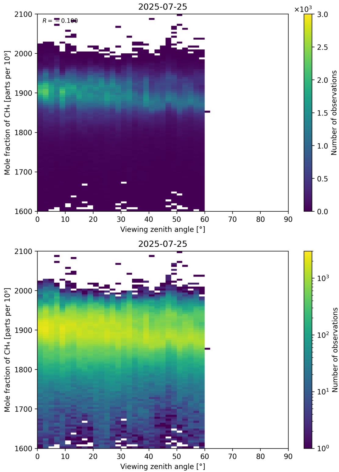
Figure 110: Scatter density plot of “Viewing zenith angle” against “Mole fraction of CH 4 ” for 2025-07-24 to 2025-07-26.
