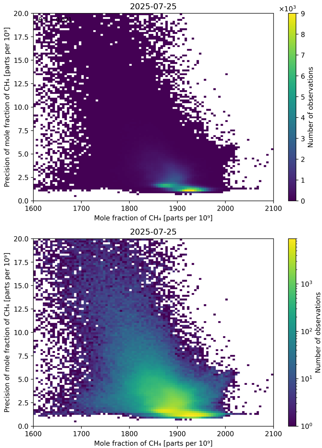
Figure 75: Scatter density plot of “Mole fraction of CH 4 ” against “Precision of mole fraction of CH 4 ” for 2025-07-24 to 2025-07-26.
