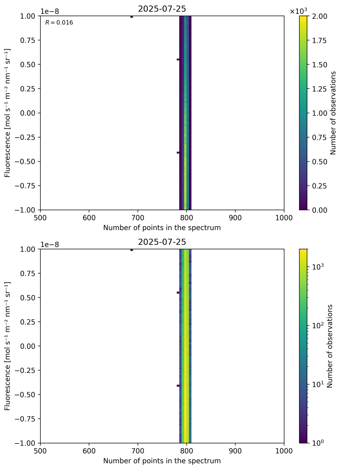
Figure 91: Scatter density plot of “Number of points in the spectrum” against “Fluorescence” for 2025-07-24 to 2025-07-26.
