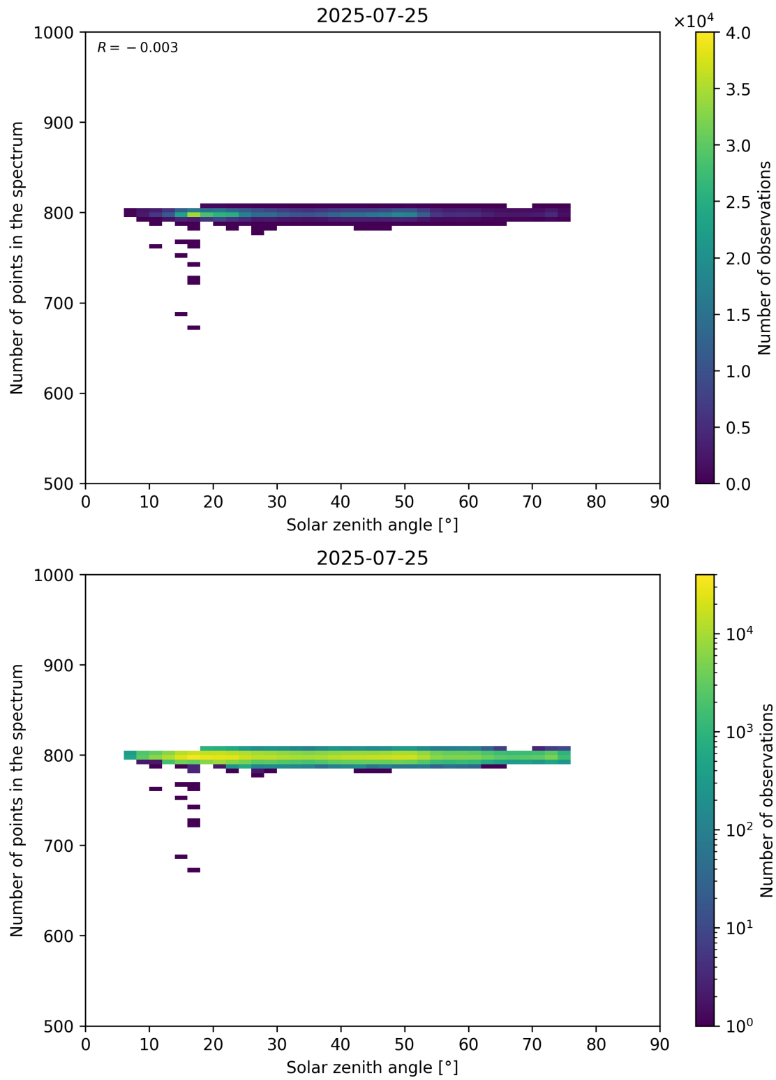
Figure 103: Scatter density plot of “Solar zenith angle” against “Number of points in the spectrum” for 2025-07-24 to 2025-07-26.
