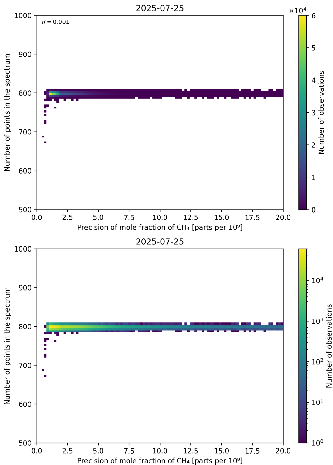
Figure 84: Scatter density plot of “Precision of mole fraction of CH 4 ” against “Number of points in the spectrum” for 2025-07-24 to 2025-07-26.
