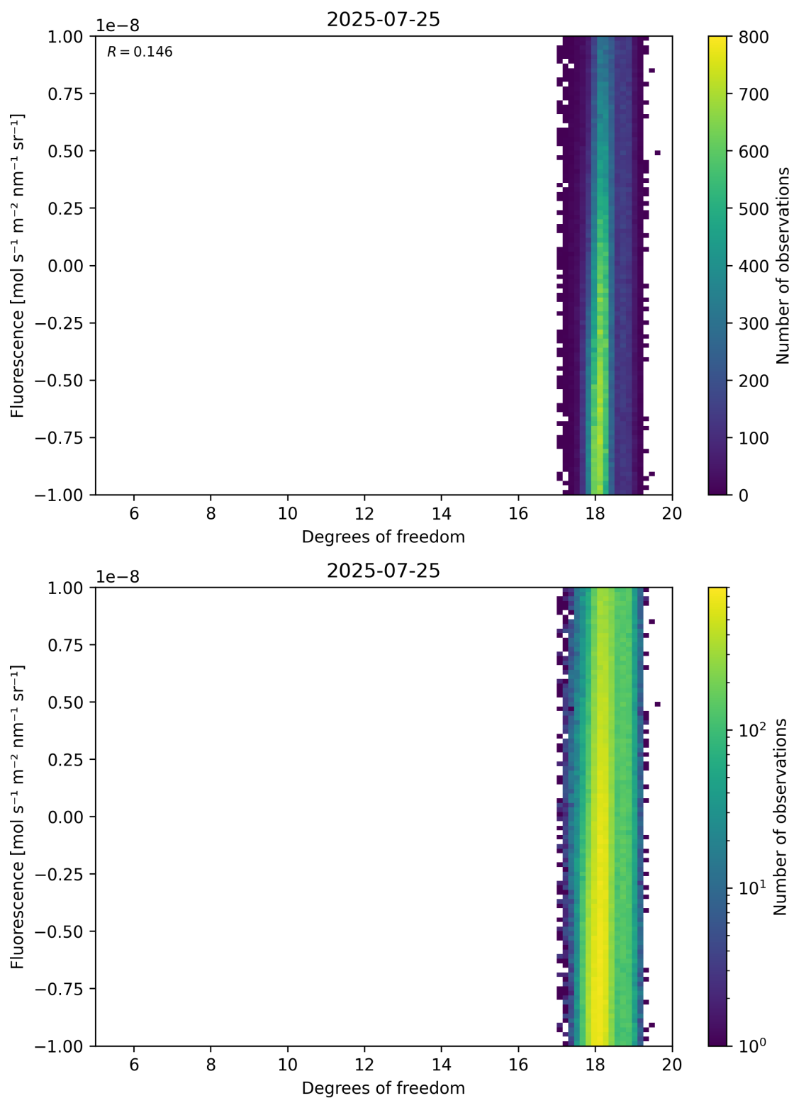
Figure 51: Scatter density plot of “Degrees of freedom” against “Fluorescence” for 2025-07-24 to 2025-07-26.
