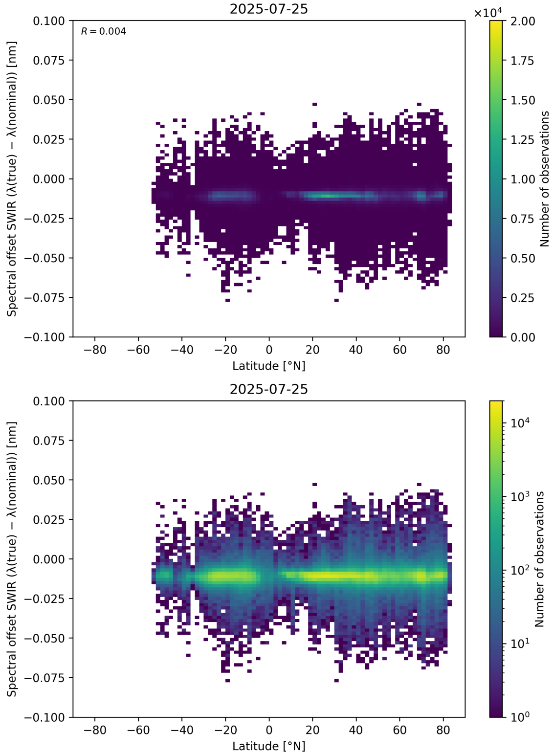
Figure 62: Scatter density plot of “Latitude” against “Spectral offset SWIR ( \lambda_{\text{true}} - \lambda_{\text{nominal}} )” for 2025-07-24 to 2025-07-26.
