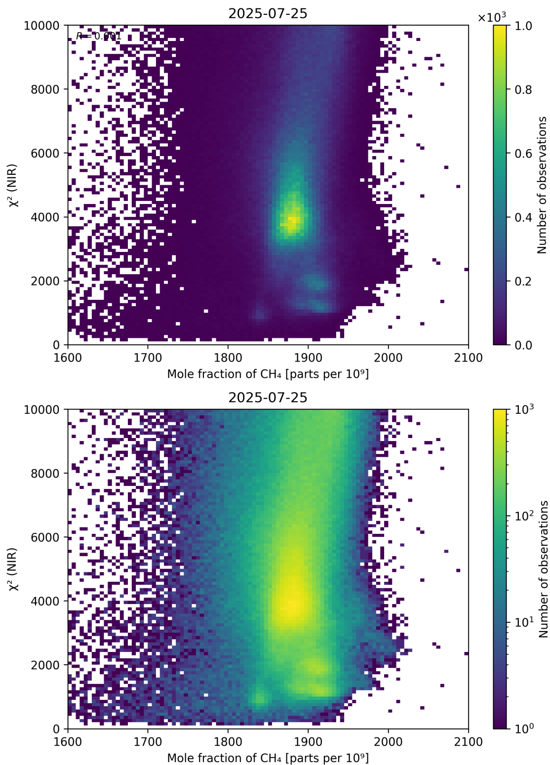
Figure 70: Scatter density plot of “Mole fraction of \text{CH}_4 ” against “ \chi^2 (NIR)” for 2025-07-24 to 2025-07-26.
