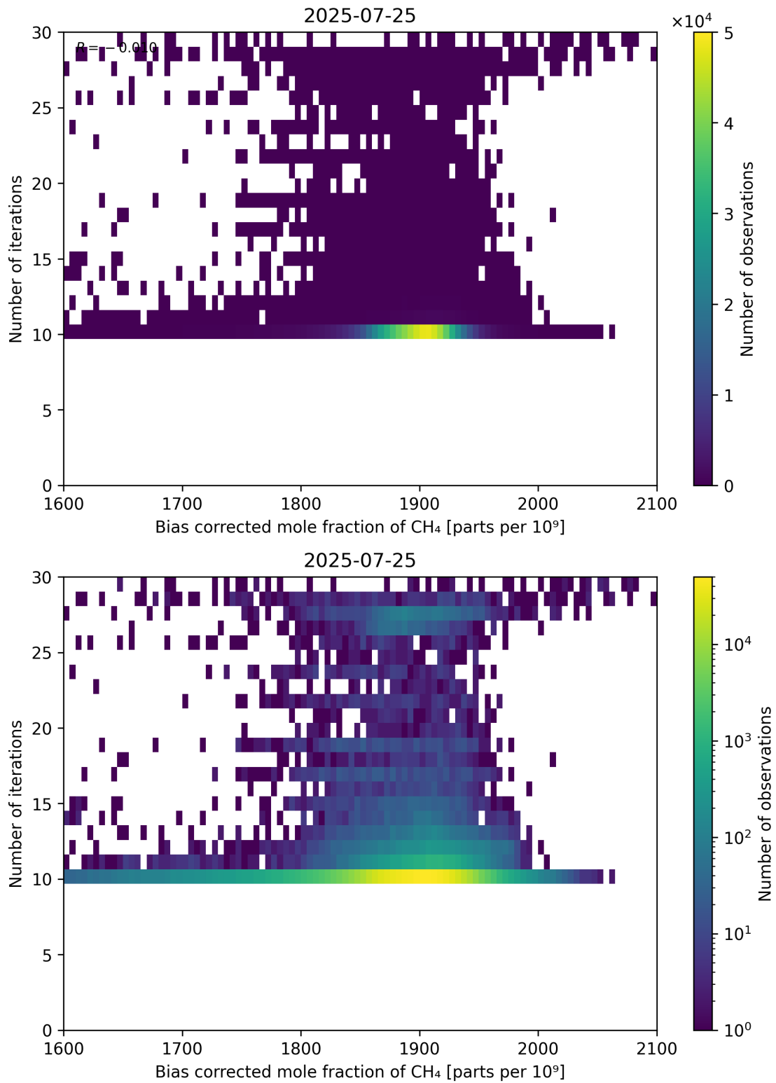
Figure 67: Scatter density plot of “Bias corrected mole fraction of CH 4 ” against “Number of iterations” for 2025-07-24 to 2025-07-26.
