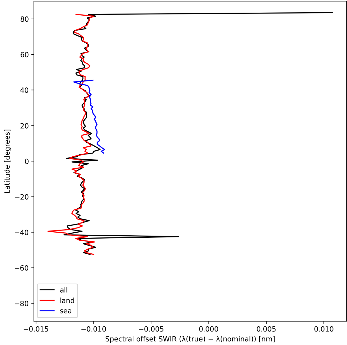
Figure 16: Zonal average of “Spectral offset SWIR ( \lambda_{\text{true}} - \lambda_{\text{nominal}} )” for 2025-07-24 to 2025-07-26.
