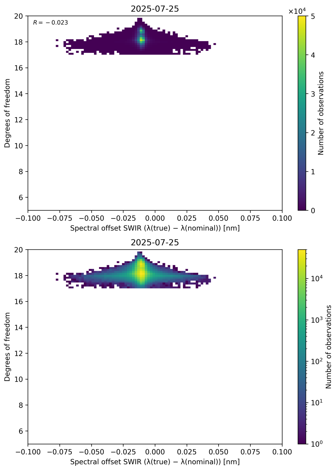
Figure 119: Scatter density plot of “Spectral offset SWIR ( \lambda_{\text{true}} - \lambda_{\text{nominal}} )” against “Degrees of freedom” for 2025-07-24 to 2025-07-26.
