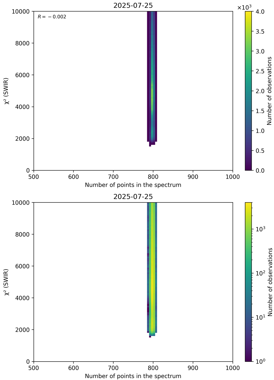
Figure 89: Scatter density plot of “Number of points in the spectrum” against “ \chi^2 (SWIR)” for 2025-07-24 to 2025-07-26.
