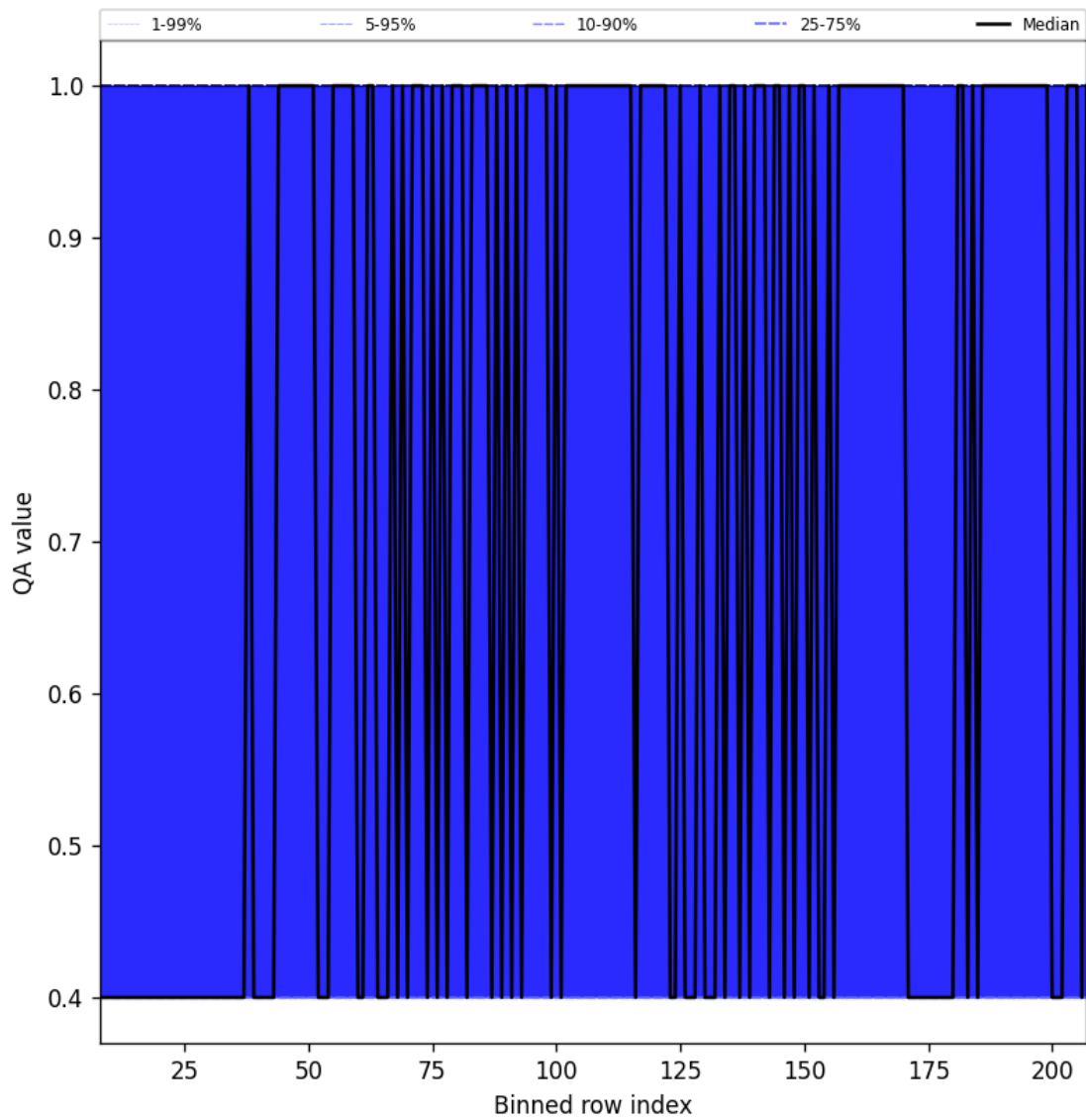
Figure 33: Along track statistics of “QA value” for 2025-07-25 to 2025-07-27
