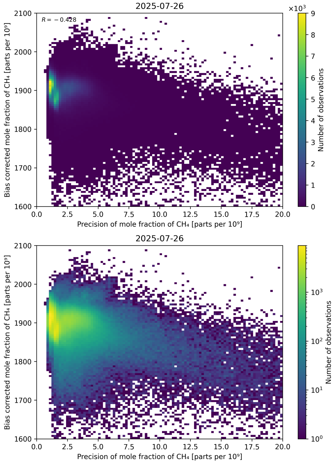
Figure 82: Scatter density plot of “Precision of mole fraction of CH 4 ” against “Bias corrected mole fraction of CH 4 ” for 2025-07-25 to 2025-07-27.
