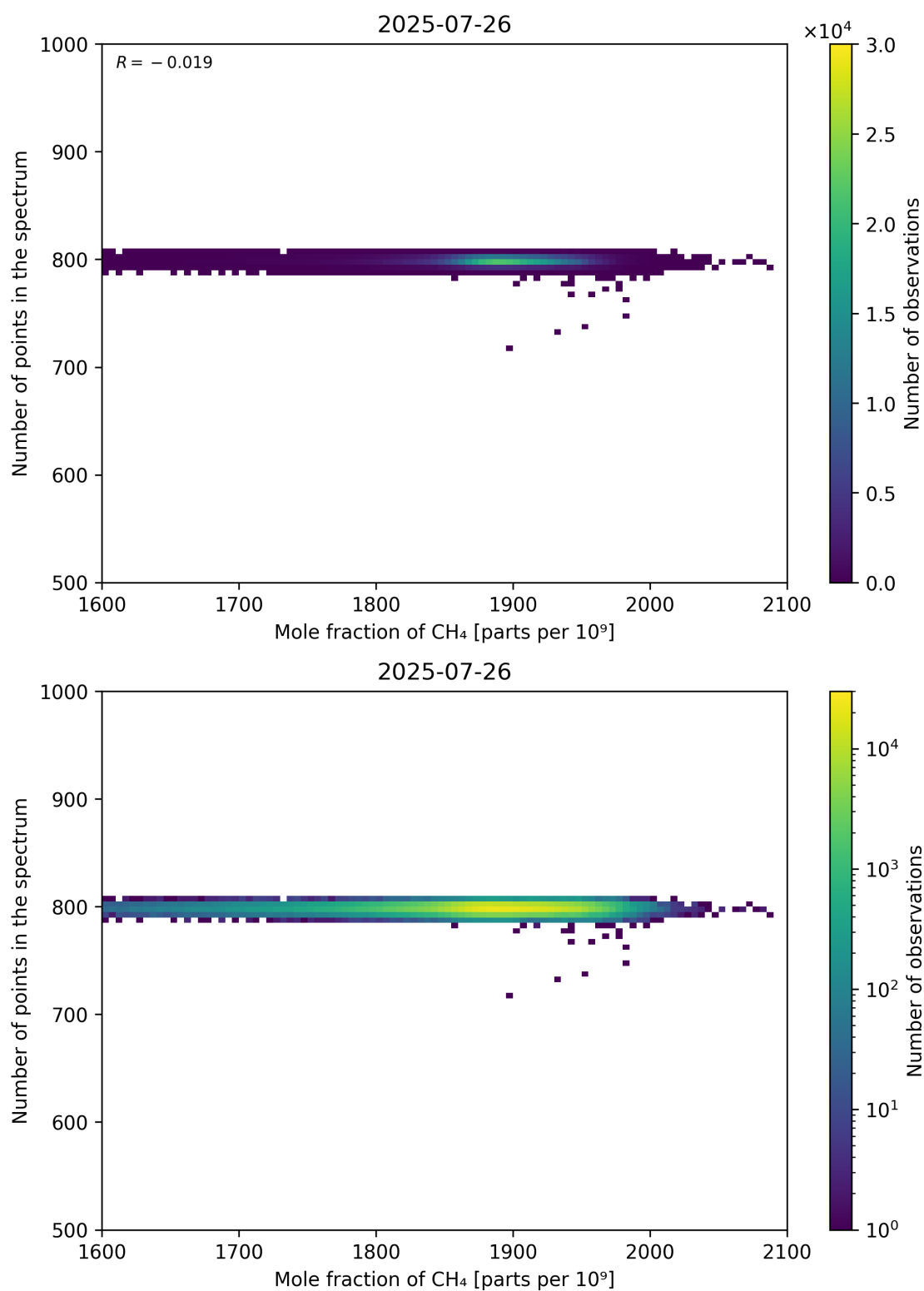
Figure 77: Scatter density plot of “Mole fraction of CH 4 ” against “Number of points in the spectrum” for 2025-07-25 to 2025-07-27.
