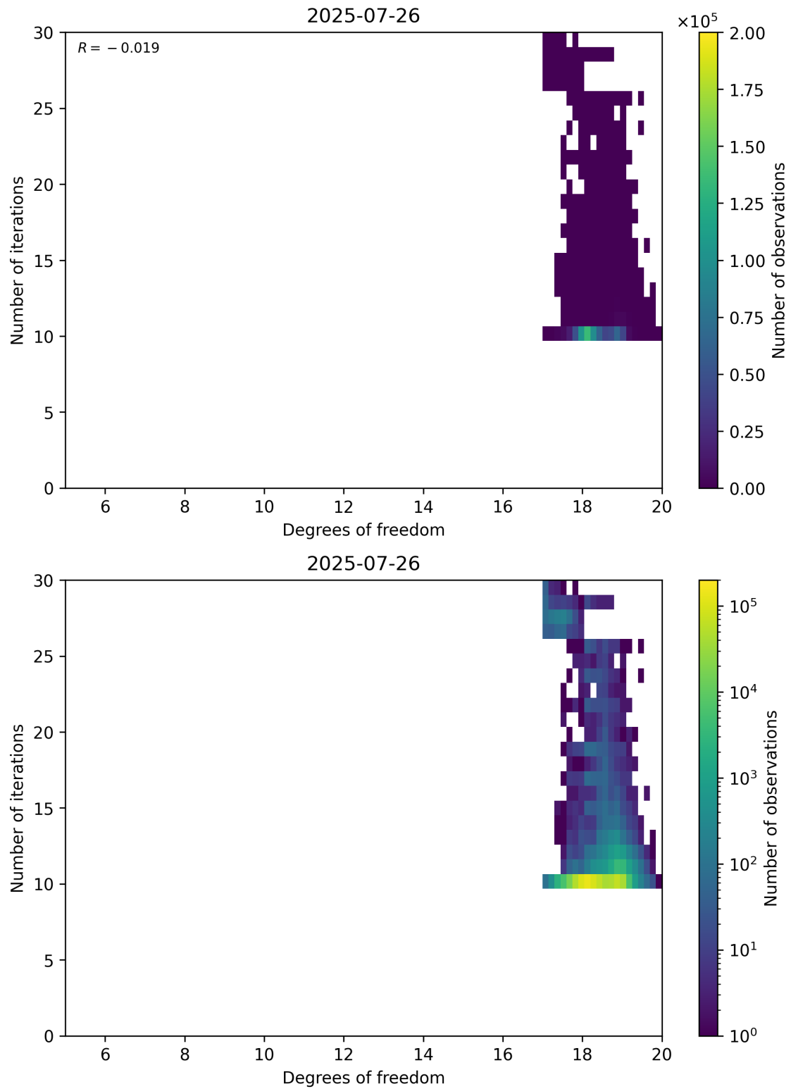
Figure 52: Scatter density plot of “Degrees of freedom” against “Number of iterations” for 2025-07-25 to 2025-07-27.
