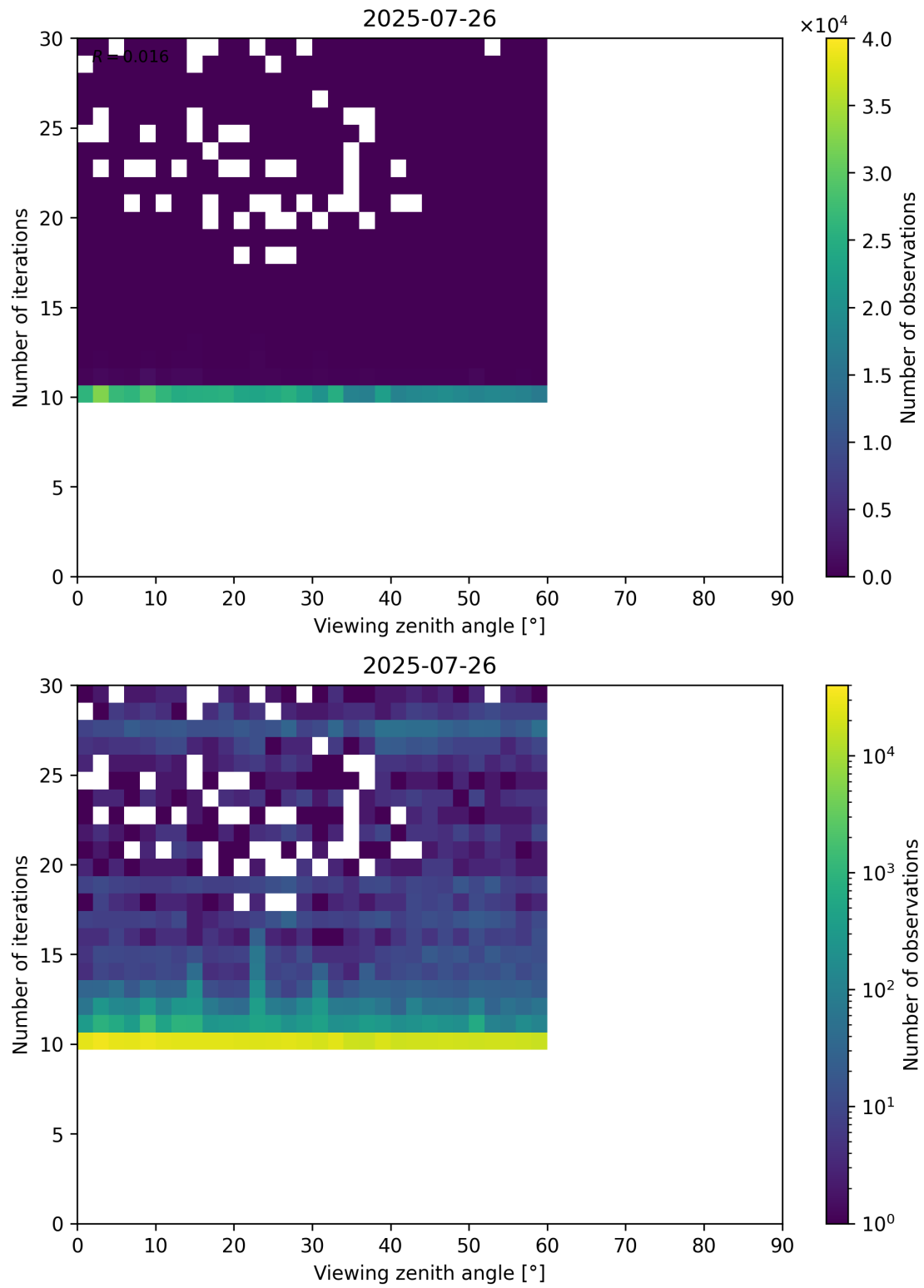
Figure 113: Scatter density plot of “Viewing zenith angle” against “Number of iterations” for 2025-07-25 to 2025-07-27.
