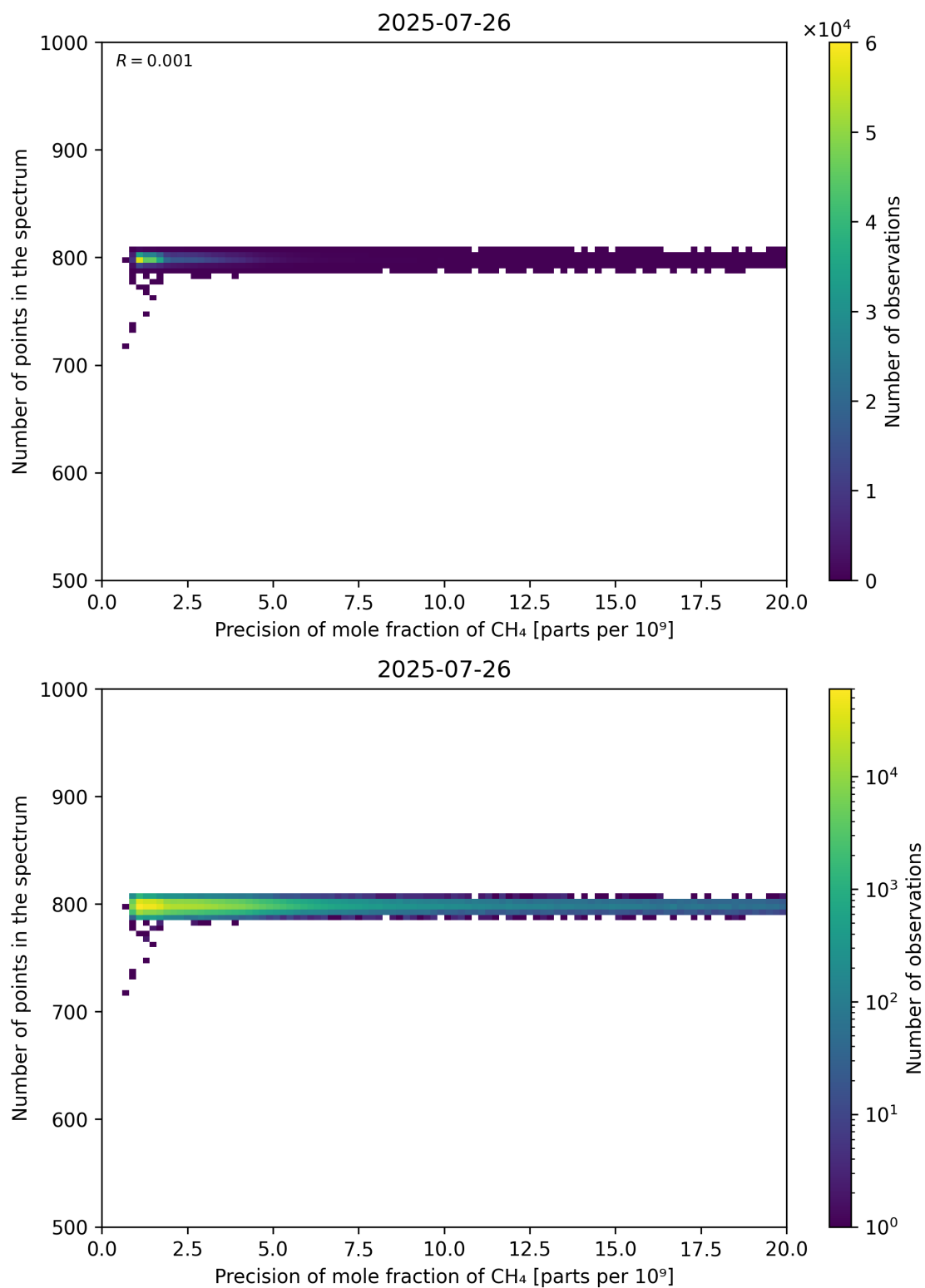
Figure 84: Scatter density plot of “Precision of mole fraction of CH 4 ” against “Number of points in the spectrum” for 2025-07-25 to 2025-07-27.
