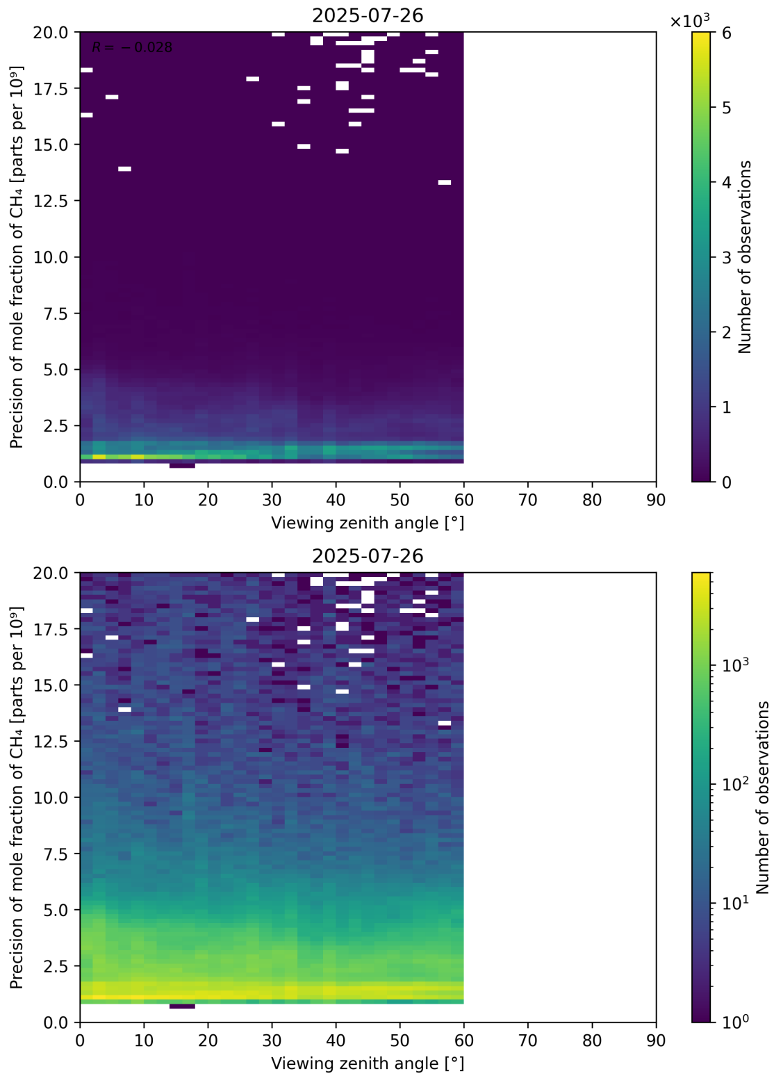
Figure 112: Scatter density plot of “Viewing zenith angle” against “Precision of mole fraction of CH 4 ” for 2025-07-25 to 2025-07-27.
