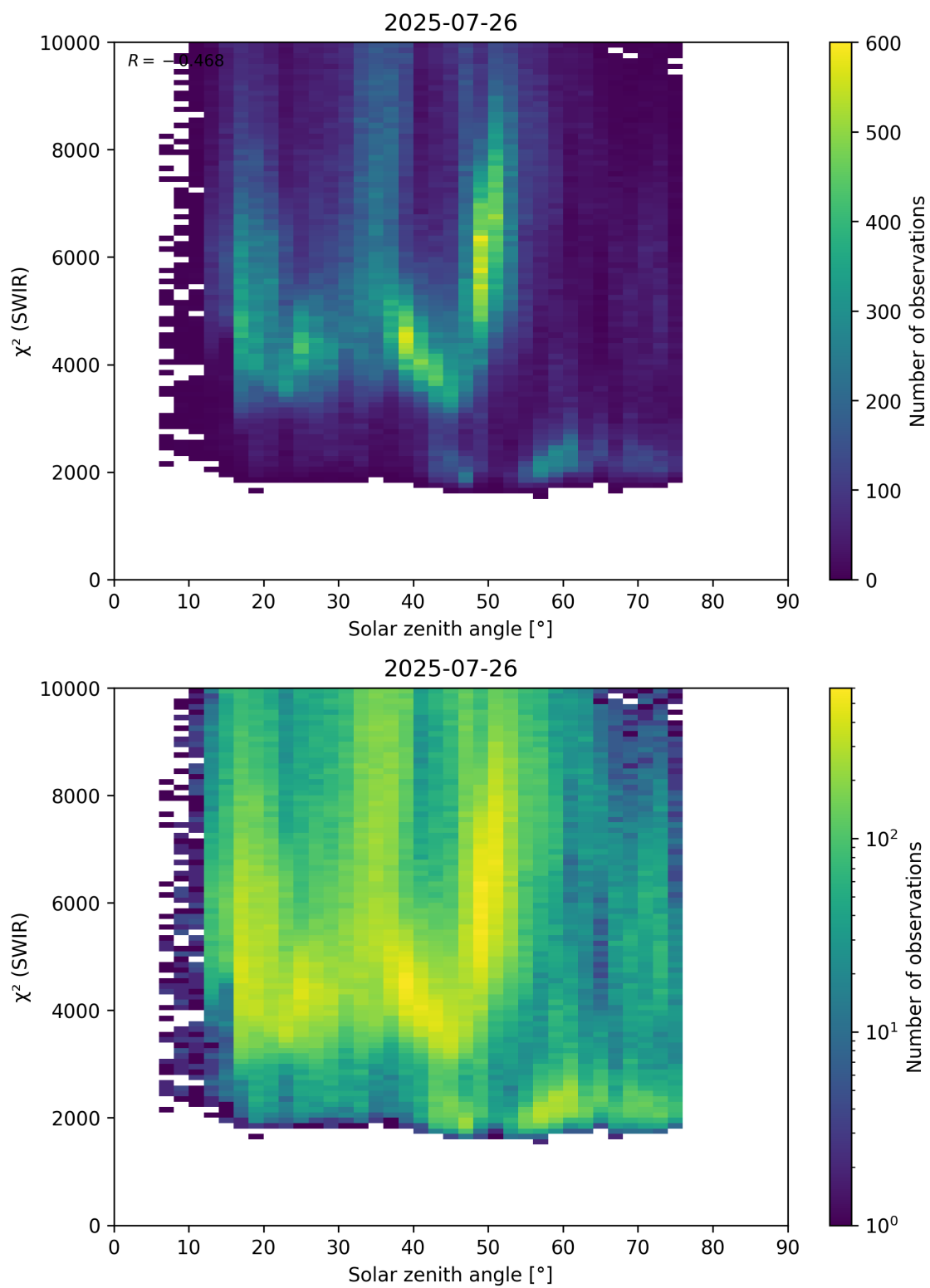
Figure 95: Scatter density plot of “Solar zenith angle” against “ \chi^2 (SWIR)” for 2025-07-25 to 2025-07-27.
