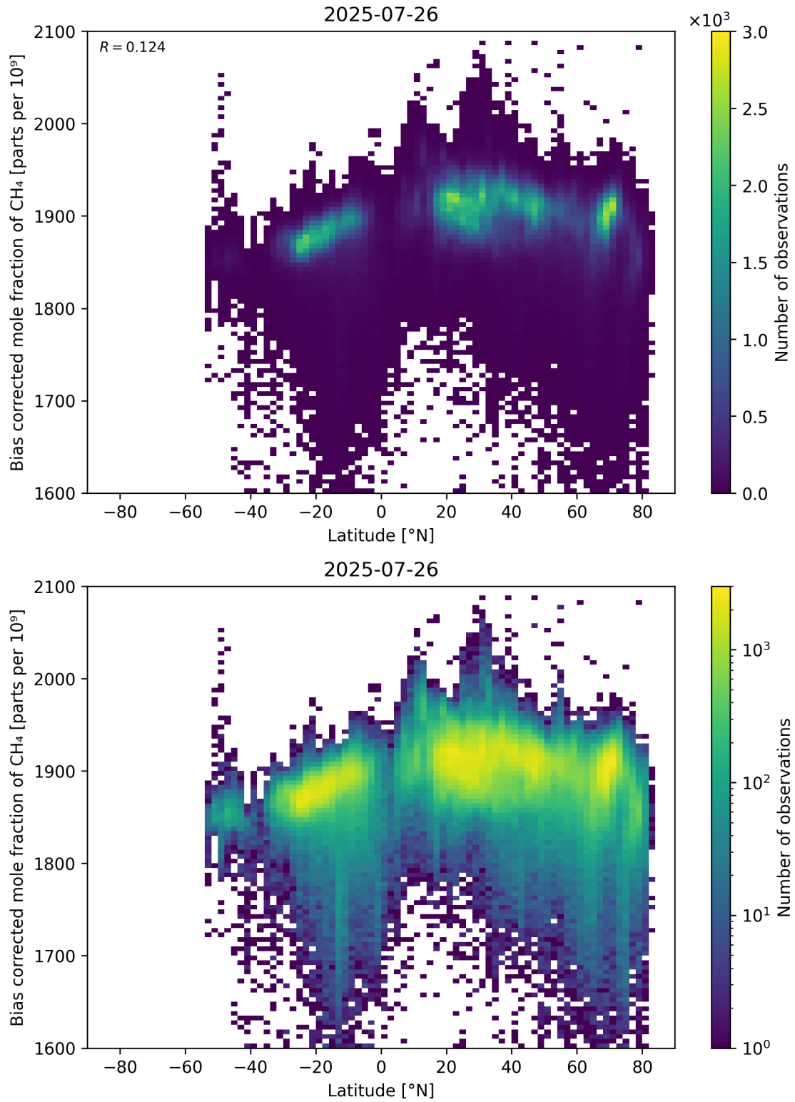
Figure 58: Scatter density plot of “Latitude” against “Bias corrected mole fraction of CH 4 ” for 2025-07-25 to 2025-07-27.
