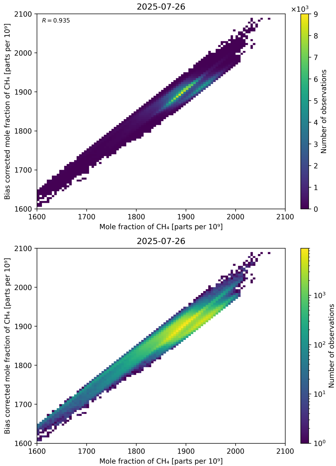
Figure 74: Scatter density plot of “Mole fraction of CH 4 ” against “Bias corrected mole fraction of CH 4 ” for 2025-07-25 to 2025-07-27.
