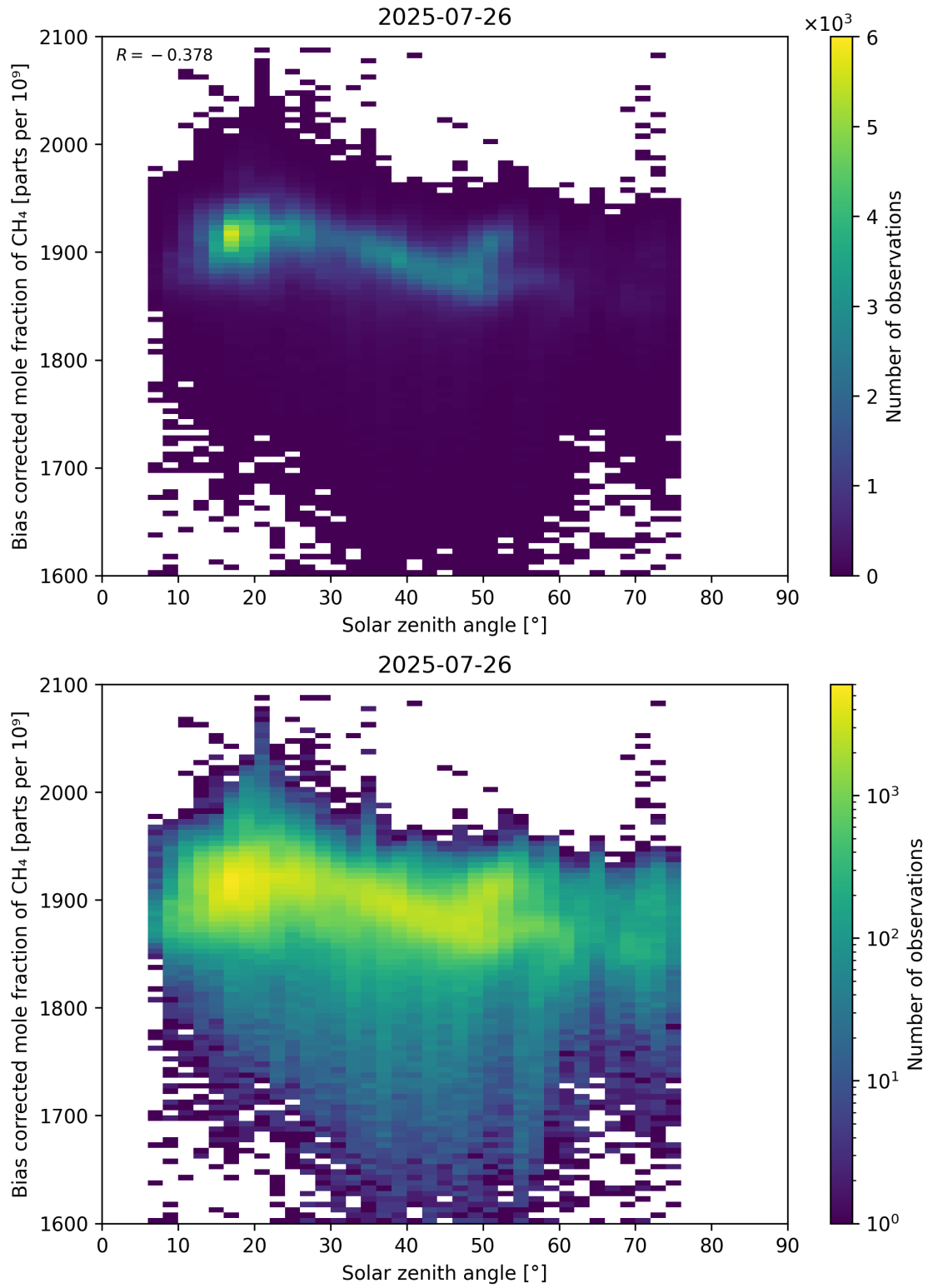
Figure 100: Scatter density plot of “Solar zenith angle” against “Bias corrected mole fraction of CH 4 ” for 2025-07-25 to 2025-07-27.
