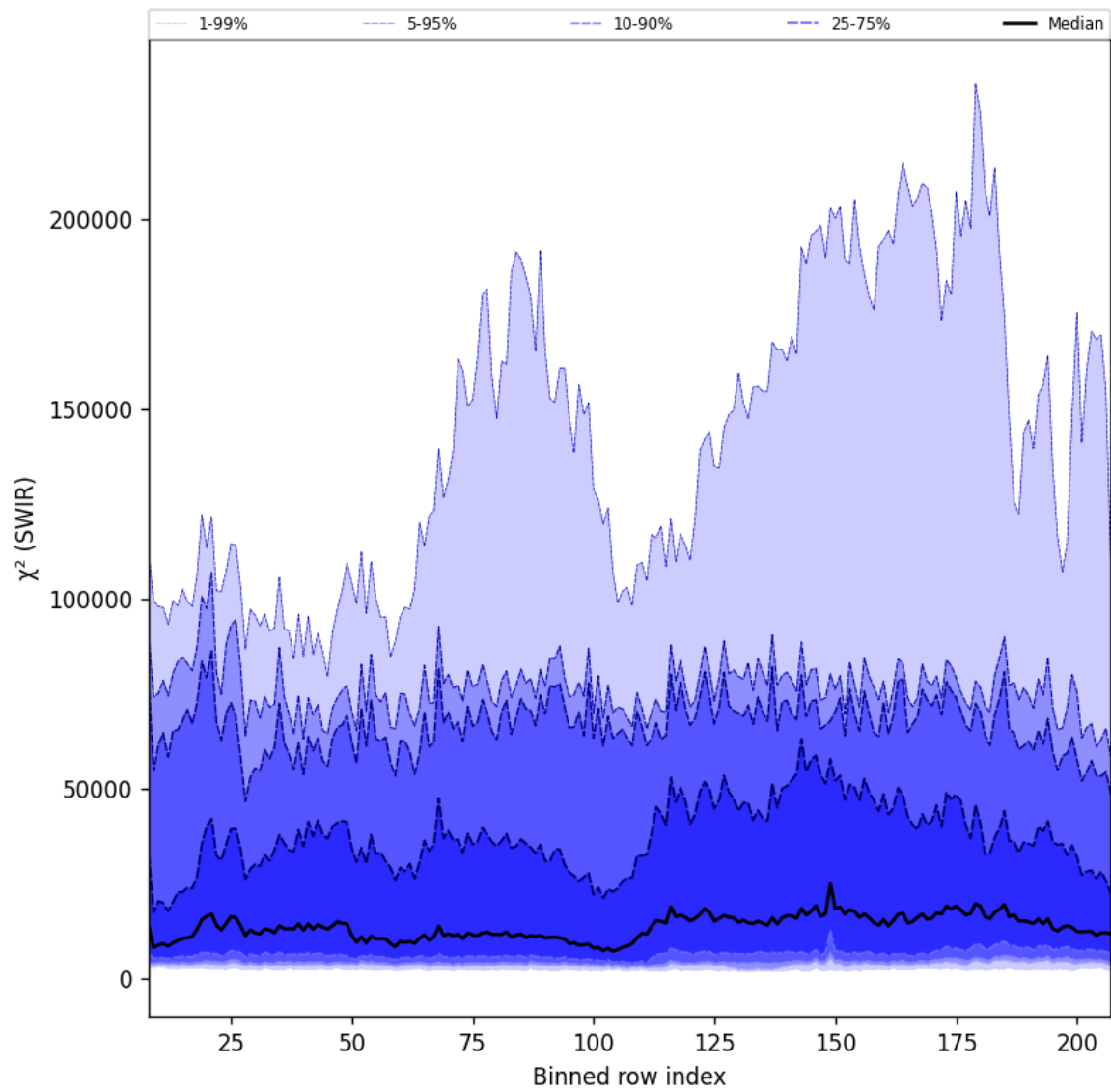
Figure 39: Along track statistics of “ \chi^2 (SWIR)” for 2025-07-25 to 2025-07-27
