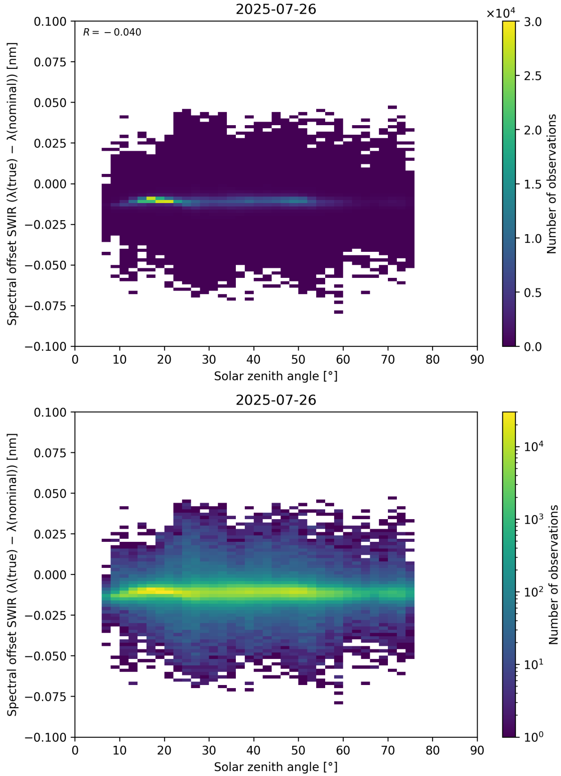
Figure 104: Scatter density plot of “Solar zenith angle” against “Spectral offset SWIR ( \lambda_{\text{true}} - \lambda_{\text{nominal}} )” for 2025-07-25 to 2025-07-27.
