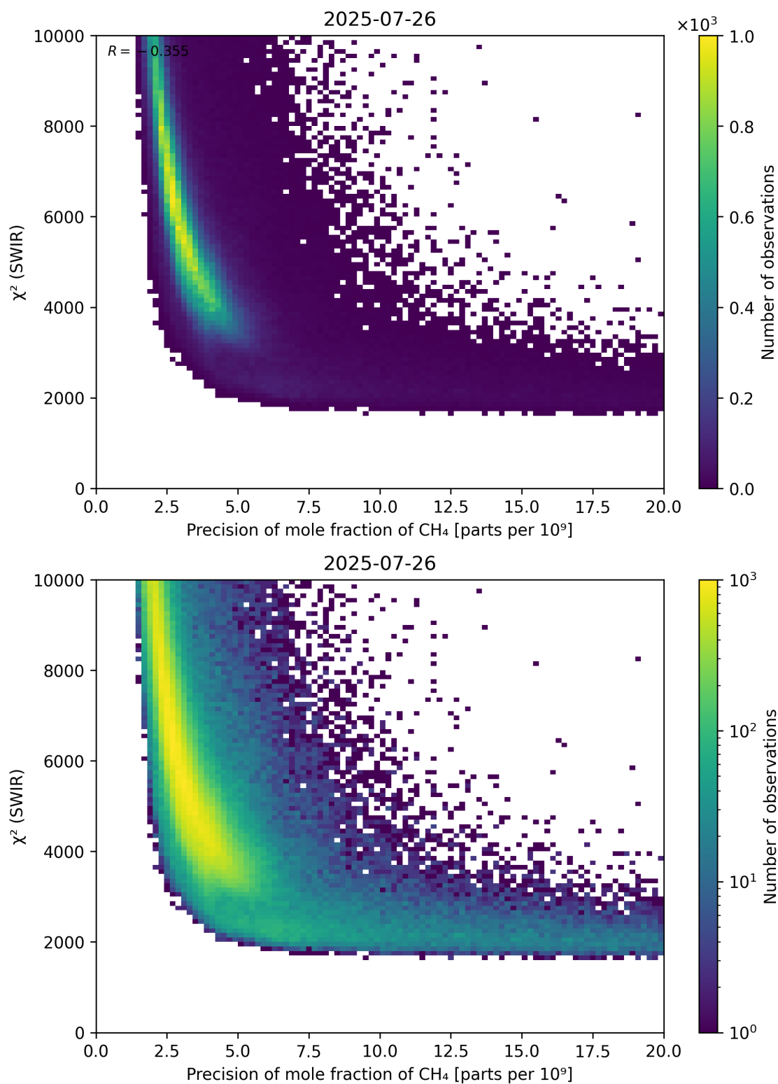
Figure 79: Scatter density plot of “Precision of mole fraction of \text{CH}_4 ” against “ \chi^2 (SWIR)” for 2025-07-25 to 2025-07-27.
