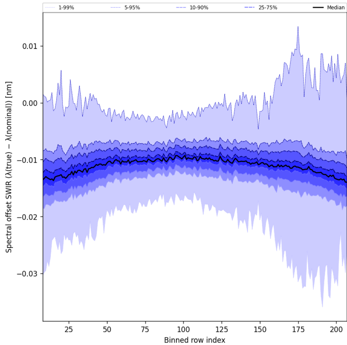
Figure 38: Along track statistics of “Spectral offset SWIR ( \lambda_{\text{true}} - \lambda_{\text{nominal}} )” for 2025-07-25 to 2025-07-27
