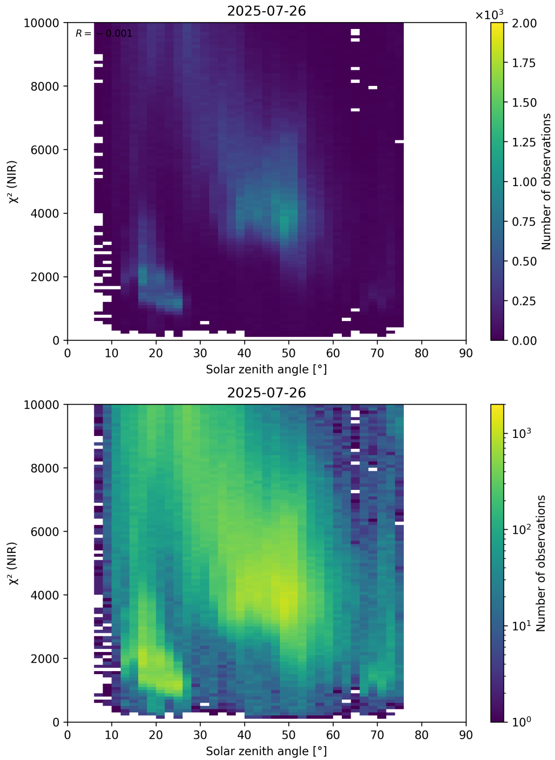
Figure 94: Scatter density plot of “Solar zenith angle” against “ \chi^2 (NIR)” for 2025-07-25 to 2025-07-27.
