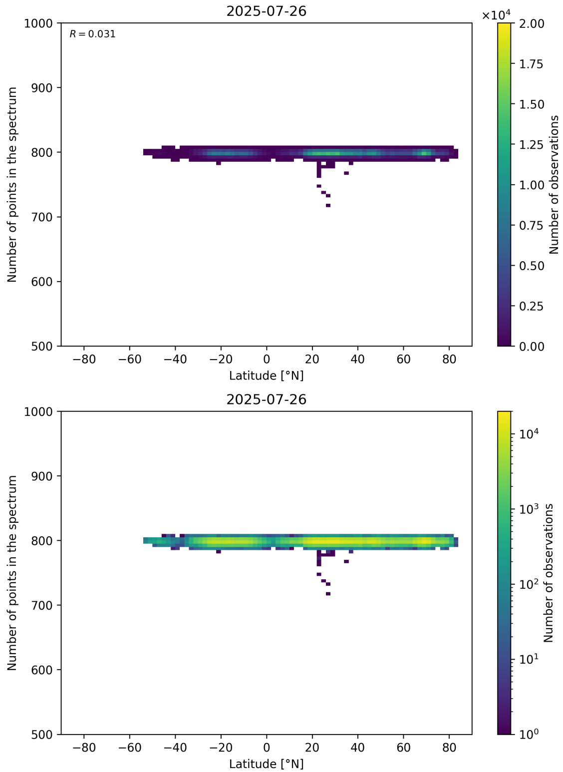
Figure 61: Scatter density plot of “Latitude” against “Number of points in the spectrum” for 2025-07-25 to 2025-07-27.
