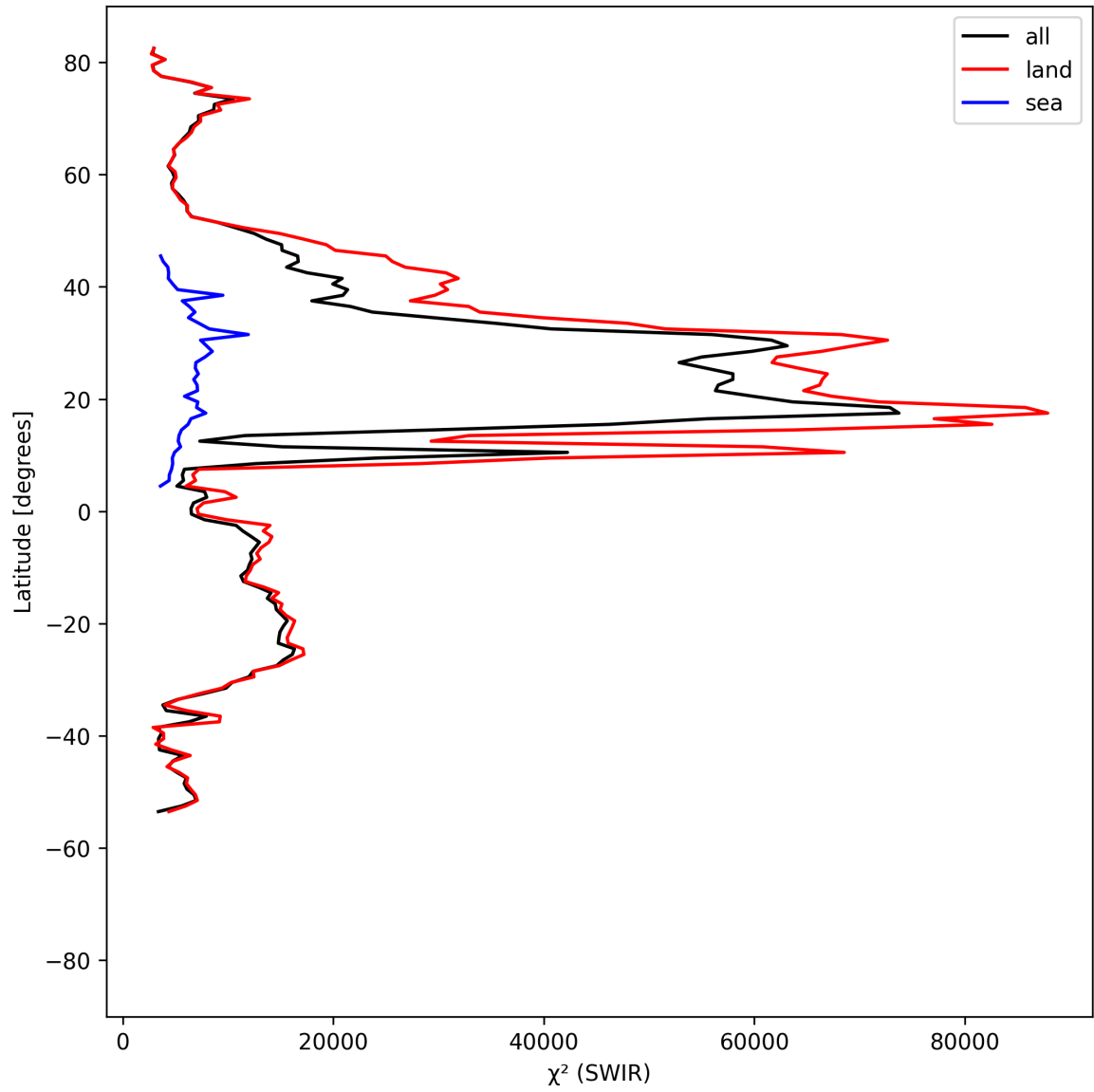
Figure 17: Zonal average of “ \chi^2 (SWIR)” for 2025-07-25 to 2025-07-27.
