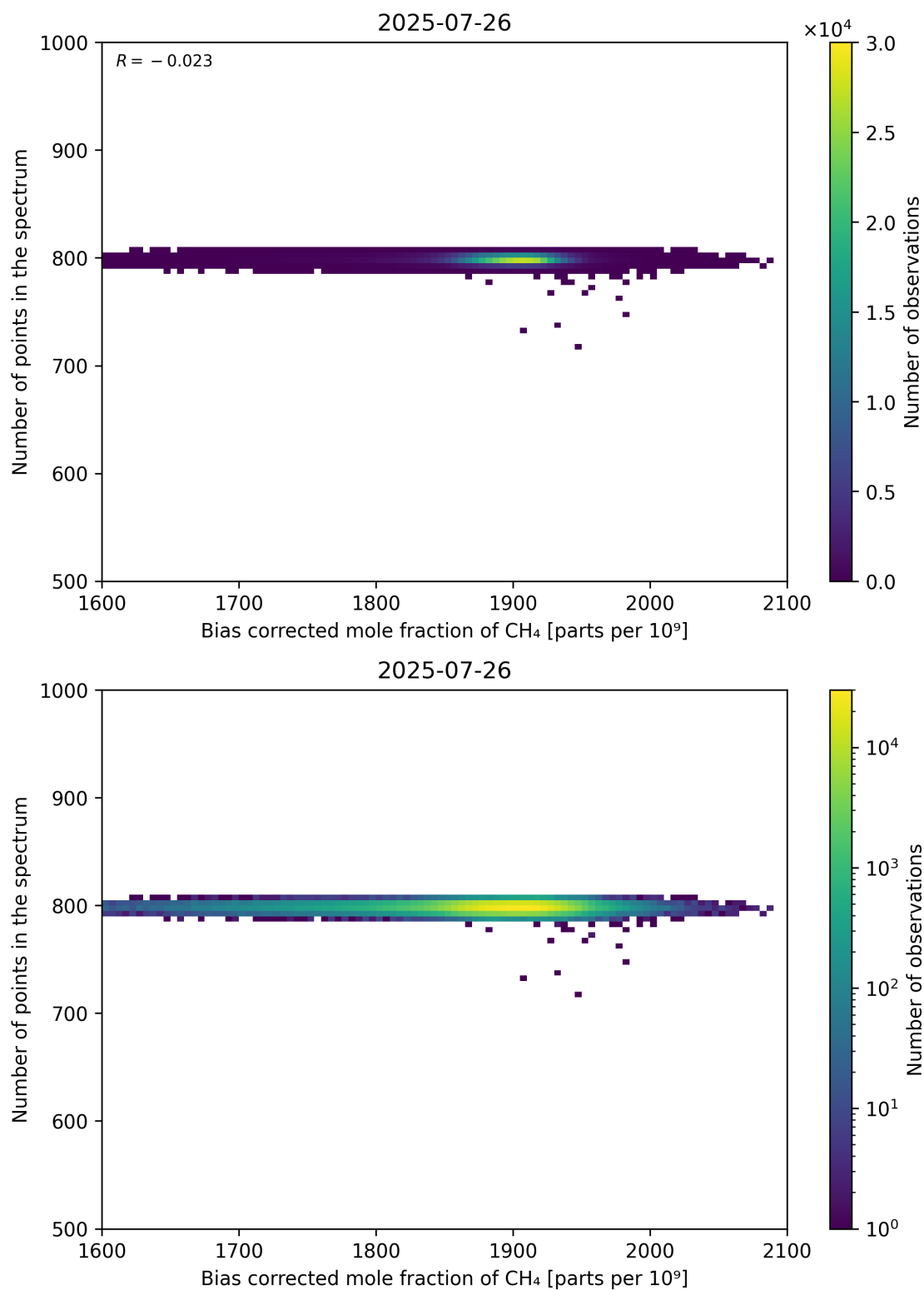
Figure 68: Scatter density plot of “Bias corrected mole fraction of CH 4 ” against “Number of points in the spectrum” for 2025-07-25 to 2025-07-27.
