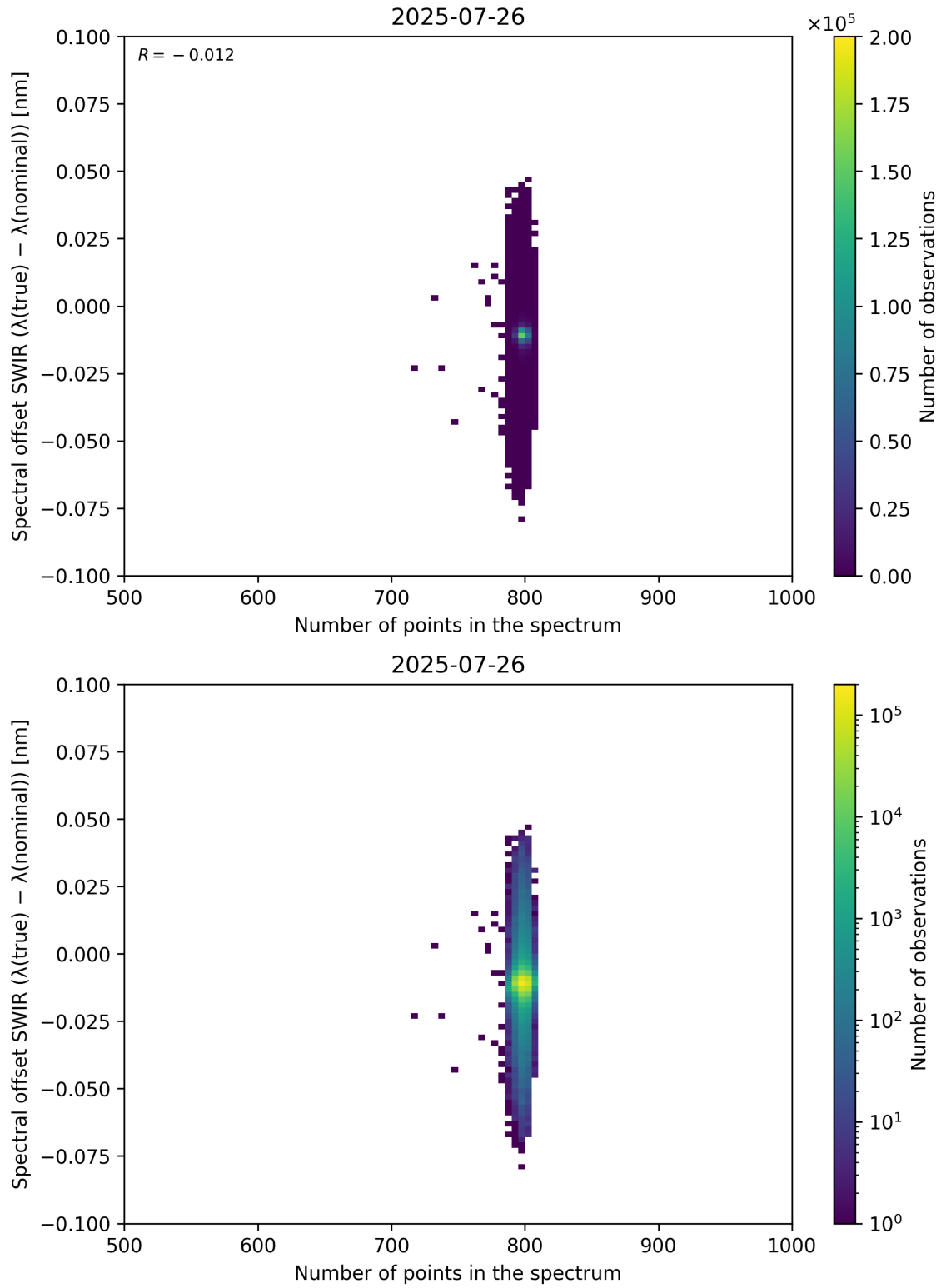
Figure 93: Scatter density plot of “Number of points in the spectrum” against “Spectral offset SWIR ( \lambda_{\text{true}} - \lambda_{\text{nominal}} )” for 2025-07-25 to 2025-07-27.
