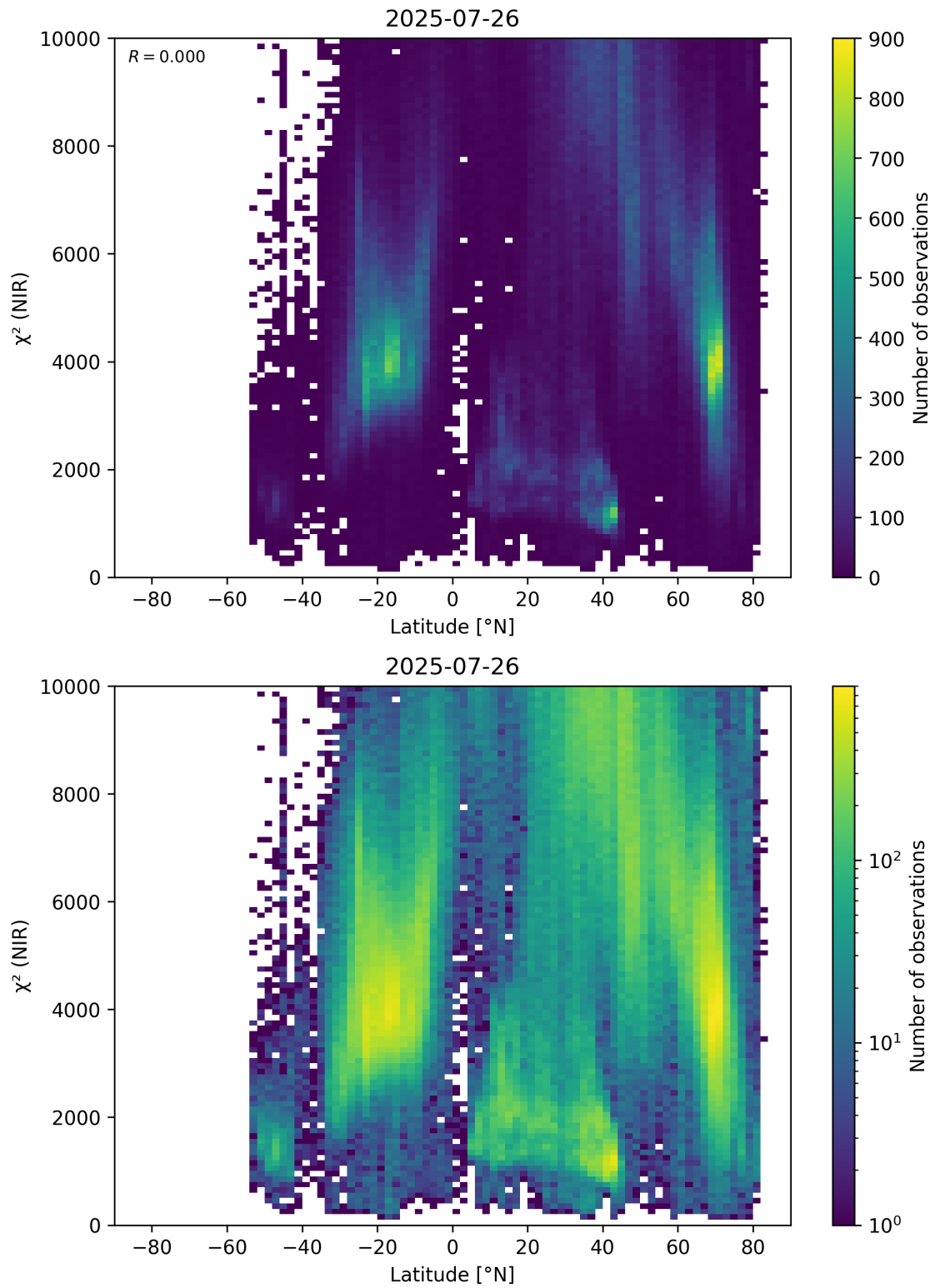
Figure 53: Scatter density plot of “Latitude” against “ \chi^2 (NIR)” for 2025-07-25 to 2025-07-27.
