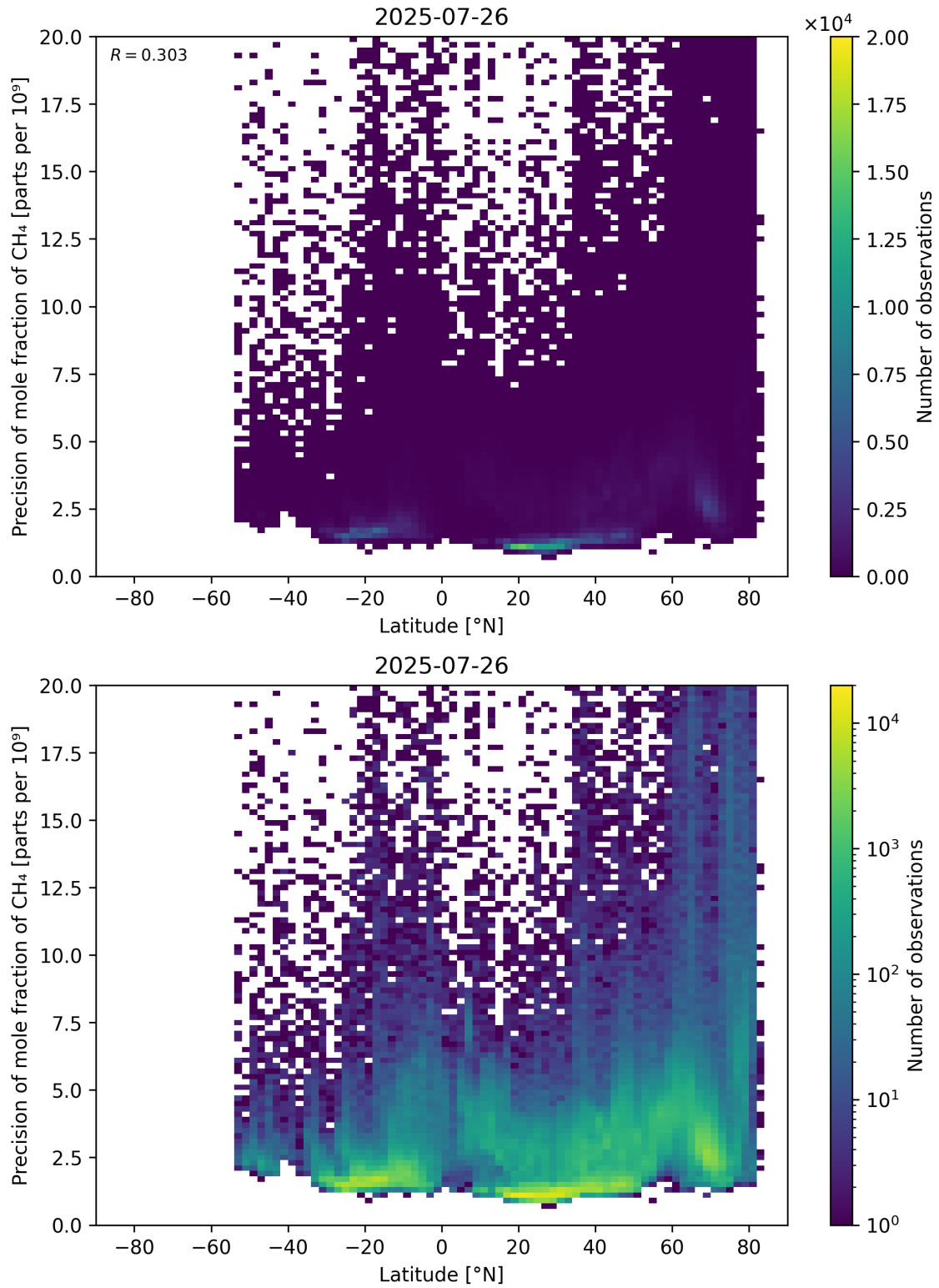
Figure 59: Scatter density plot of “Latitude” against “Precision of mole fraction of \text{CH}_4 ” for 2025-07-25 to 2025-07-27.
