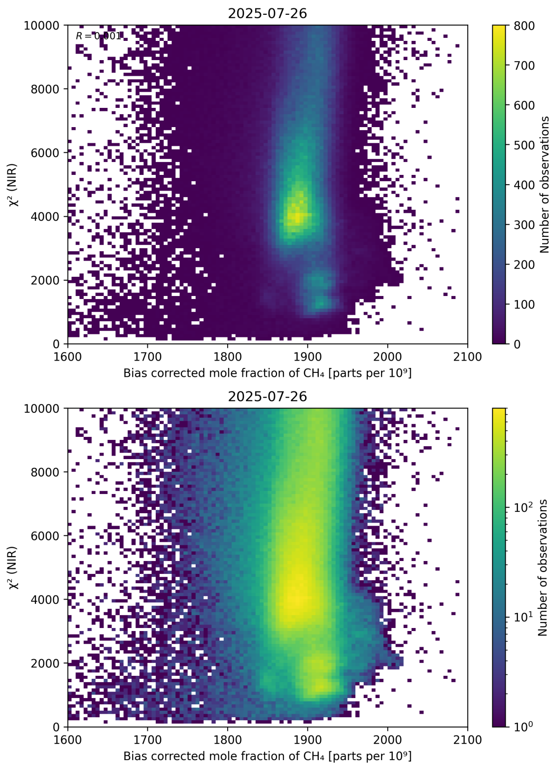
Figure 63: Scatter density plot of “Bias corrected mole fraction of \text{CH}_4 ” against “ \chi^2 (NIR)” for 2025-07-25 to 2025-07-27.
