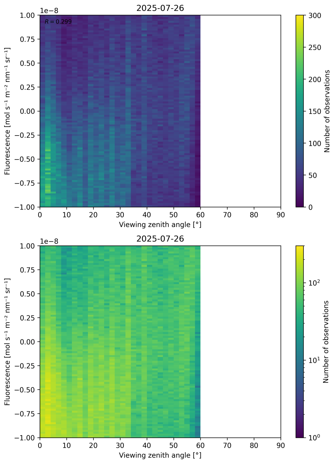
Figure 108: Scatter density plot of “Viewing zenith angle” against “Fluorescence” for 2025-07-25 to 2025-07-27.
