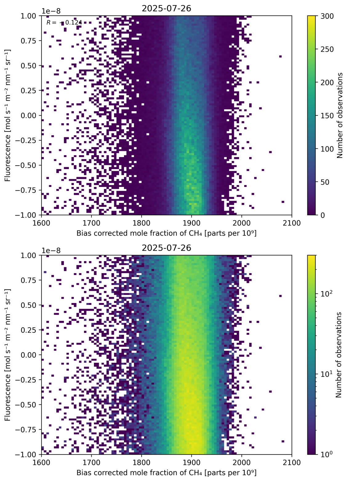
Figure 66: Scatter density plot of “Bias corrected mole fraction of \text{CH}_4 ” against “Fluorescence” for 2025-07-25 to 2025-07-27.
