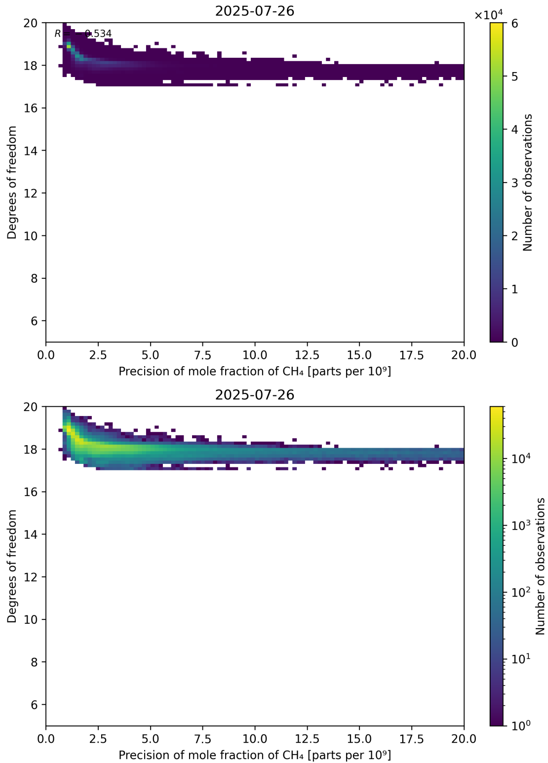
Figure 80: Scatter density plot of “Precision of mole fraction of CH 4 ” against “Degrees of freedom” for 2025-07-25 to 2025-07-27.
