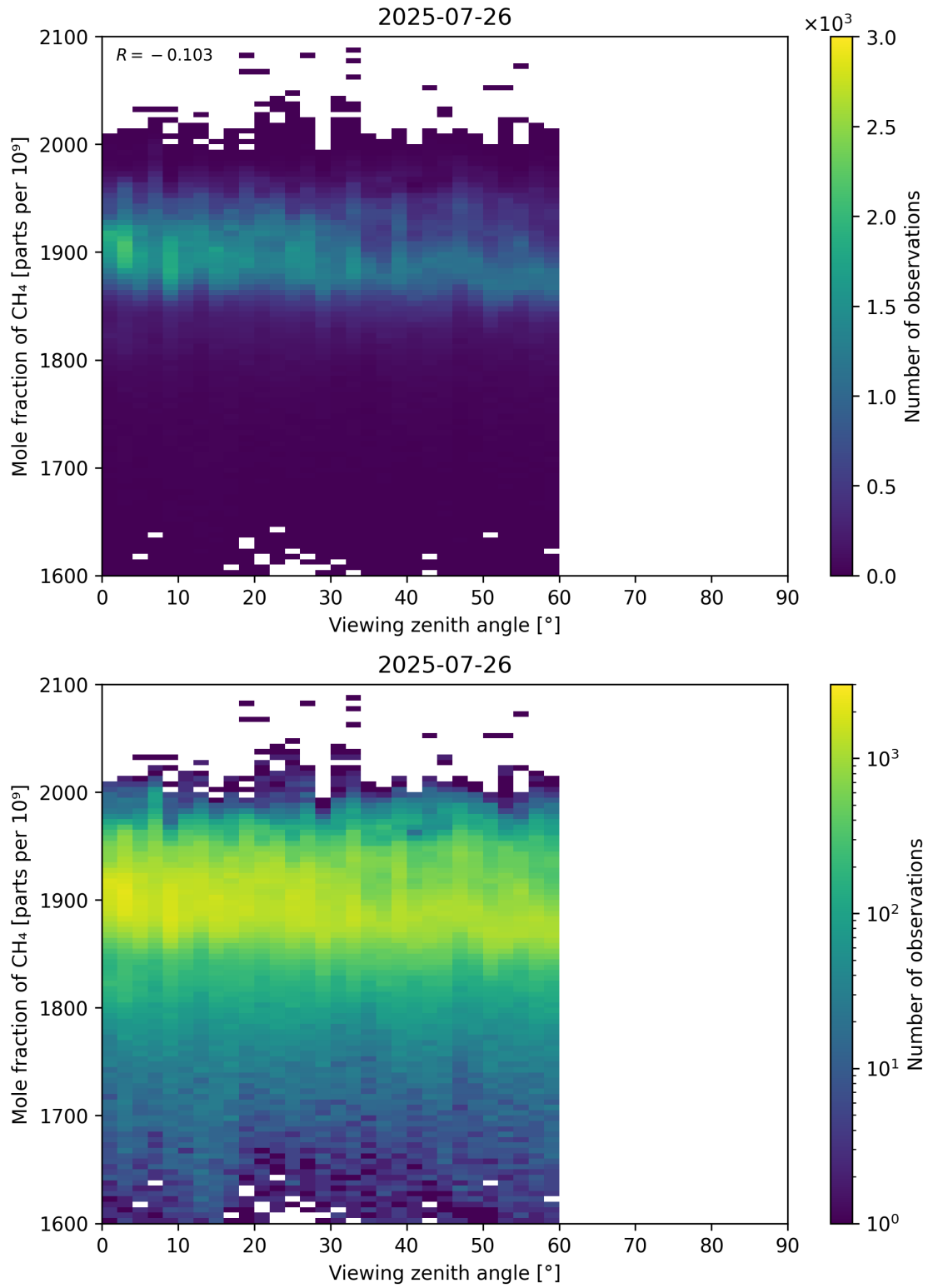
Figure 110: Scatter density plot of “Viewing zenith angle” against “Mole fraction of CH 4 ” for 2025-07-25 to 2025-07-27.
