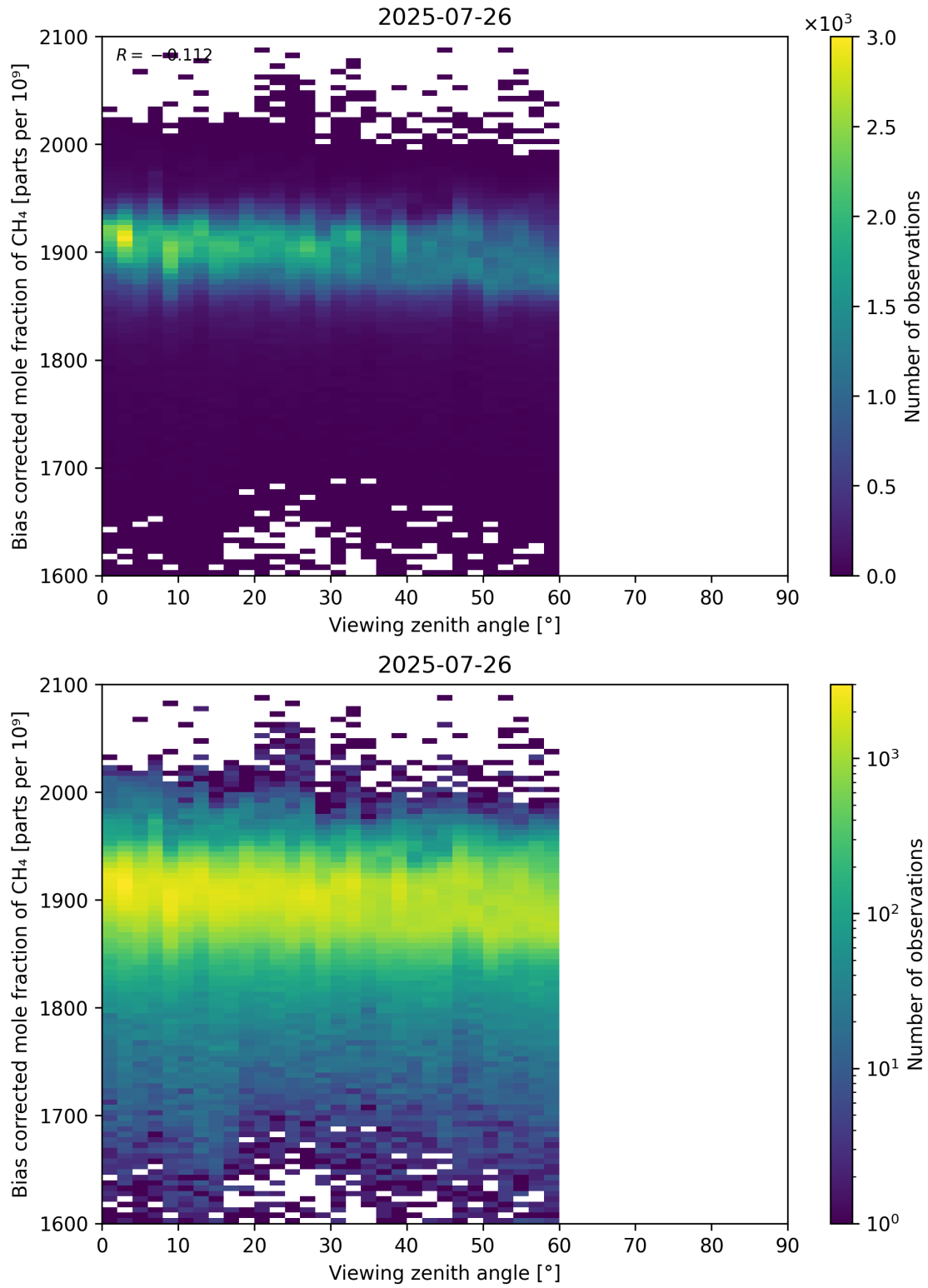
Figure 111: Scatter density plot of “Viewing zenith angle” against “Bias corrected mole fraction of CH 4 ” for 2025-07-25 to 2025-07-27.
