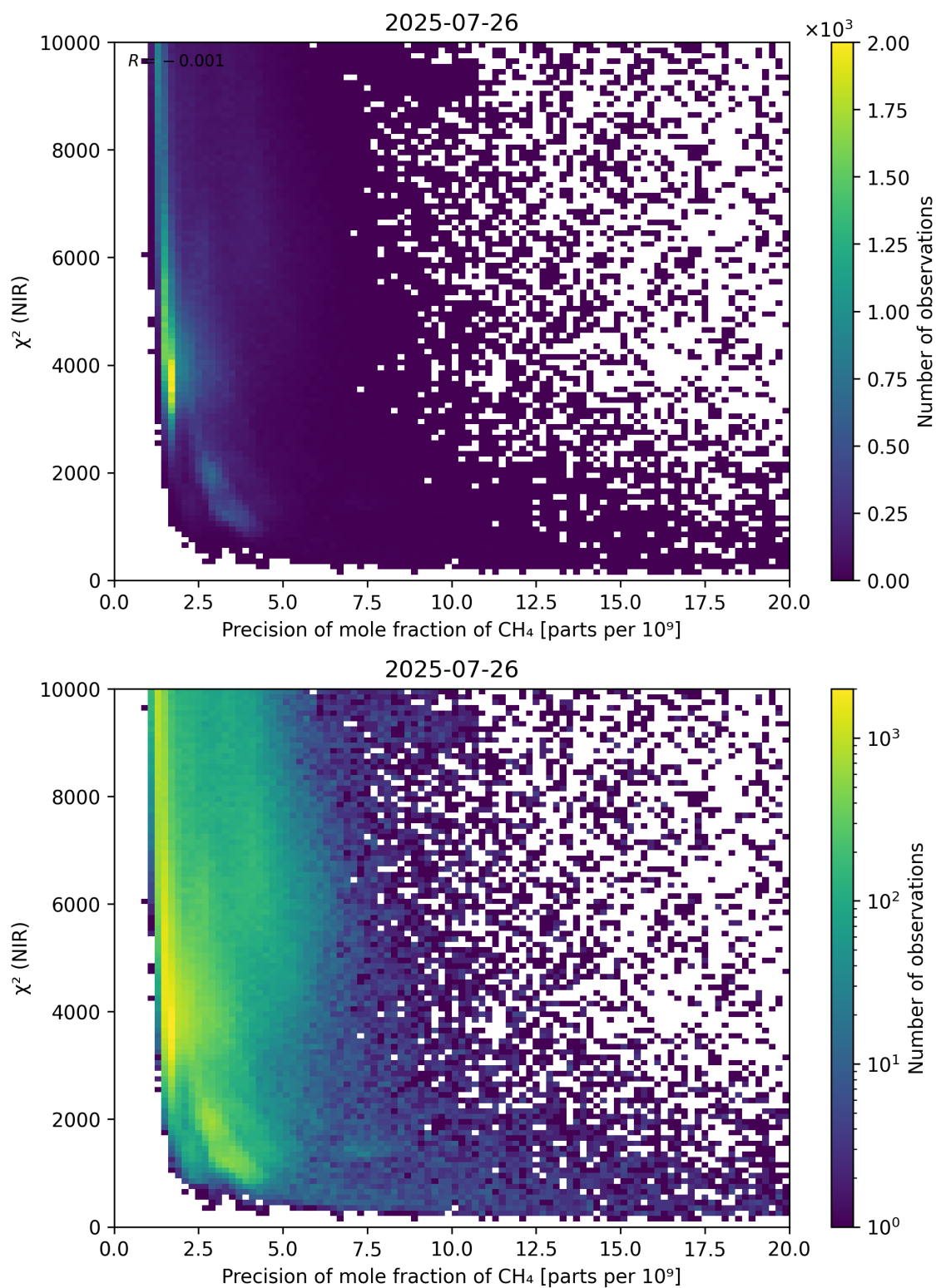
Figure 78: Scatter density plot of “Precision of mole fraction of CH 4 ” against “ \chi^2 (NIR)” for 2025-07-25 to 2025-07-27.
