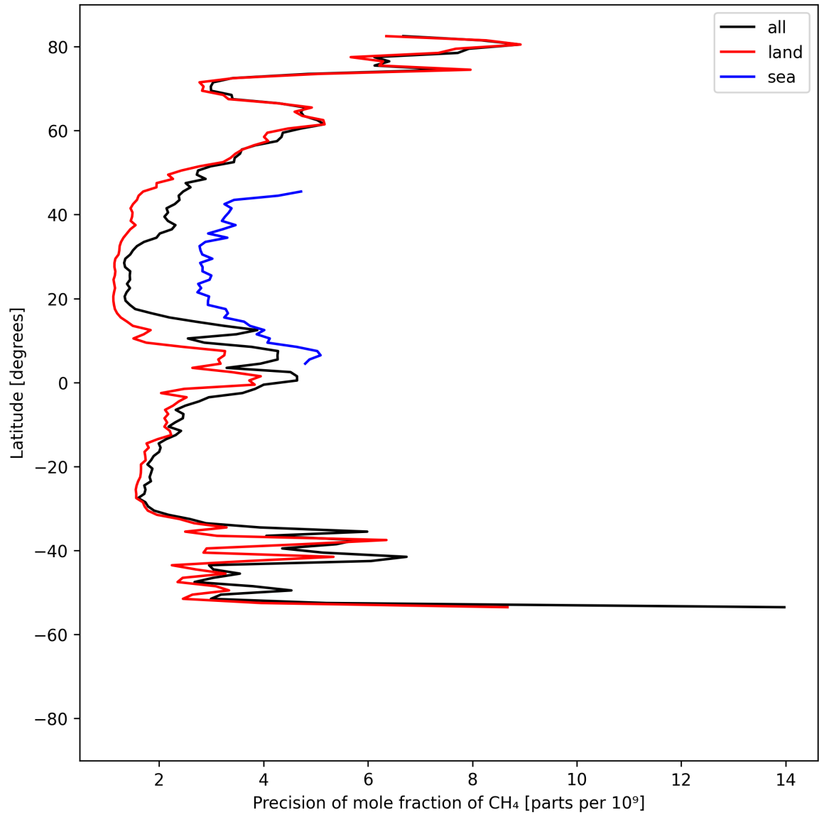
Figure 13: Zonal average of “Precision of mole fraction of CH 4 ” for 2025-07-25 to 2025-07-27.
