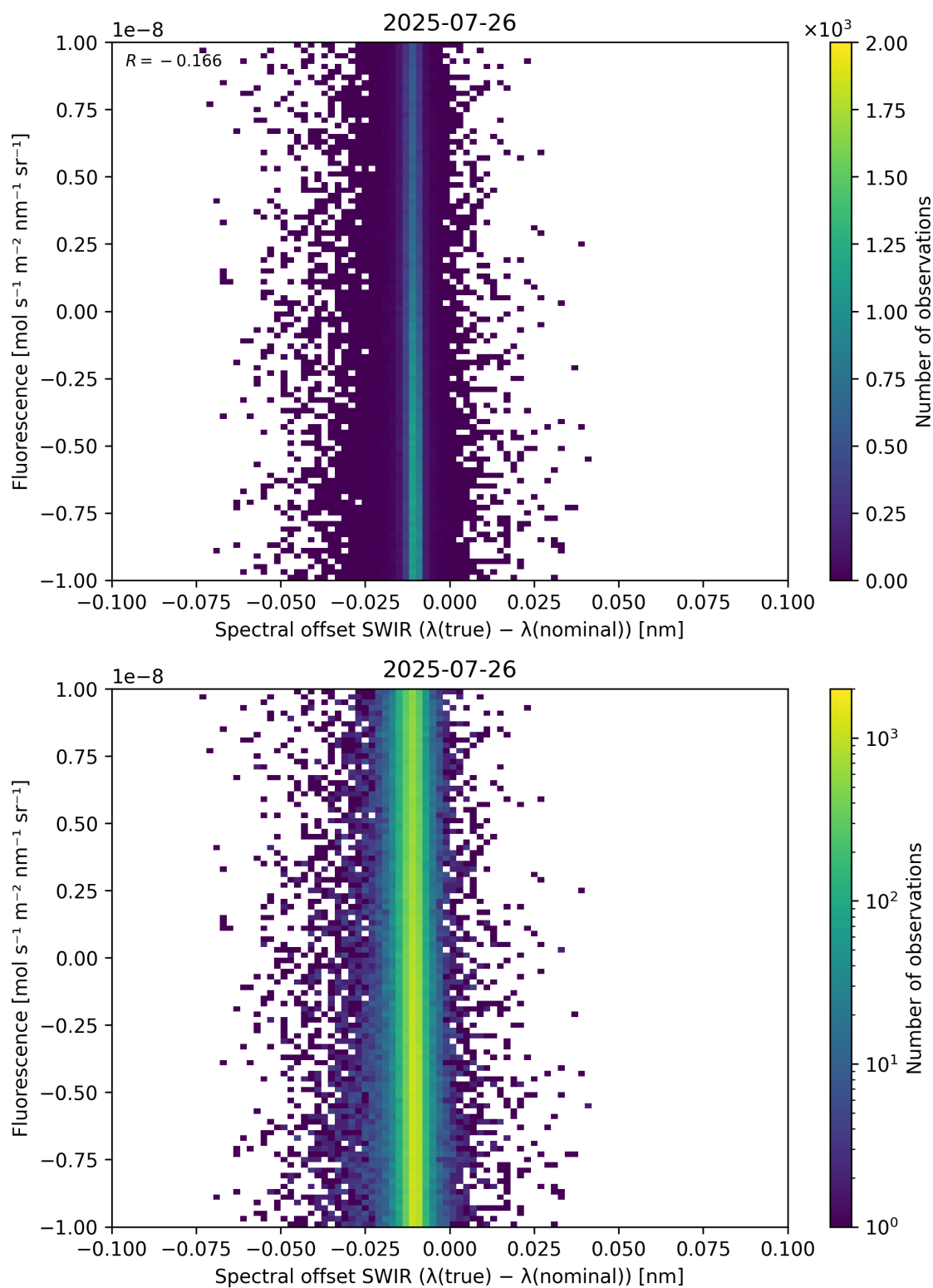
Figure 120: Scatter density plot of “Spectral offset SWIR ( \lambda_{\text{true}} - \lambda_{\text{nominal}} )” against “Fluorescence” for 2025-07-25 to 2025-07-27.
