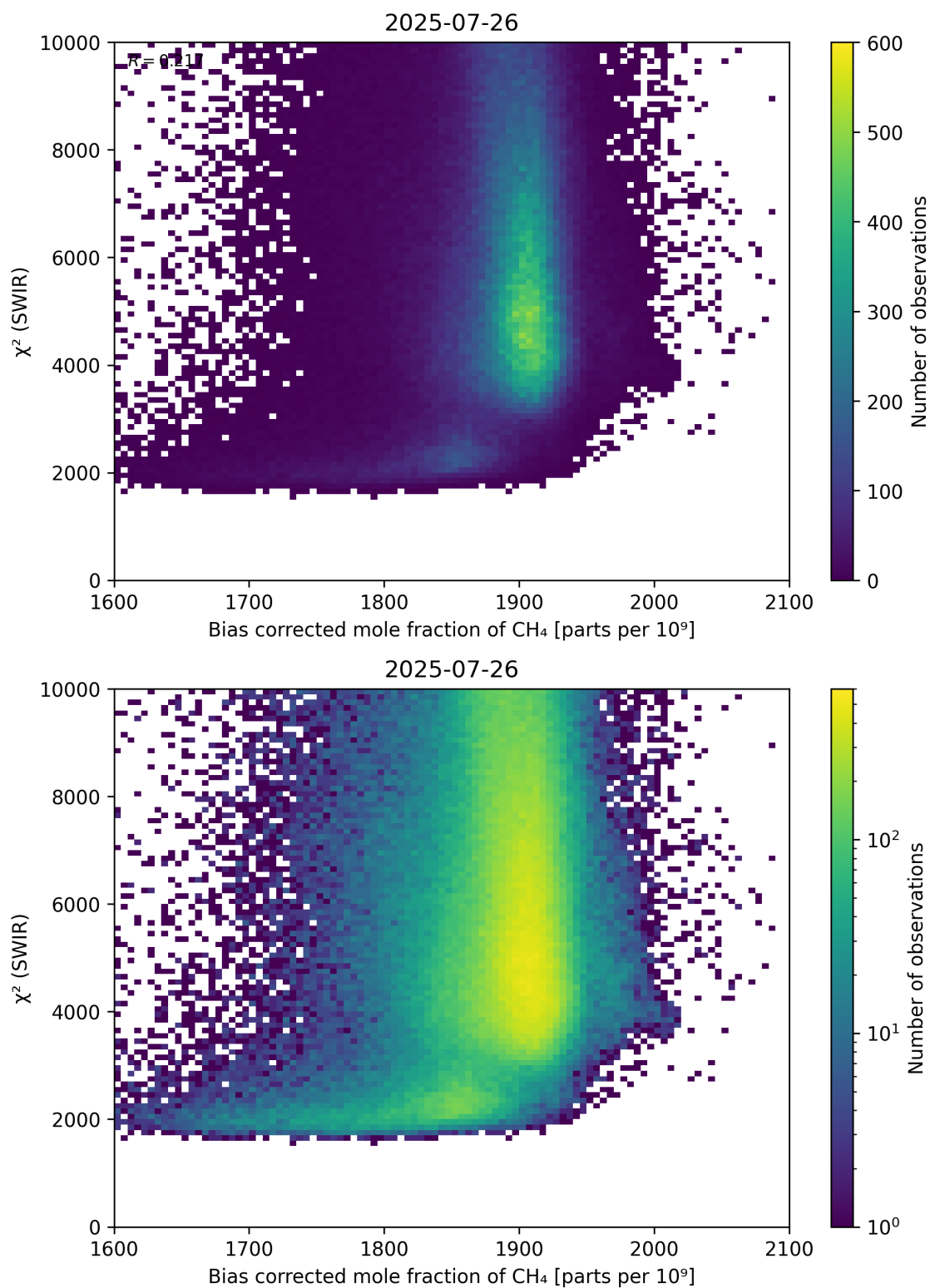
Figure 64: Scatter density plot of “Bias corrected mole fraction of CH 4 ” against “ \chi^2 (SWIR)” for 2025-07-25 to 2025-07-27.
