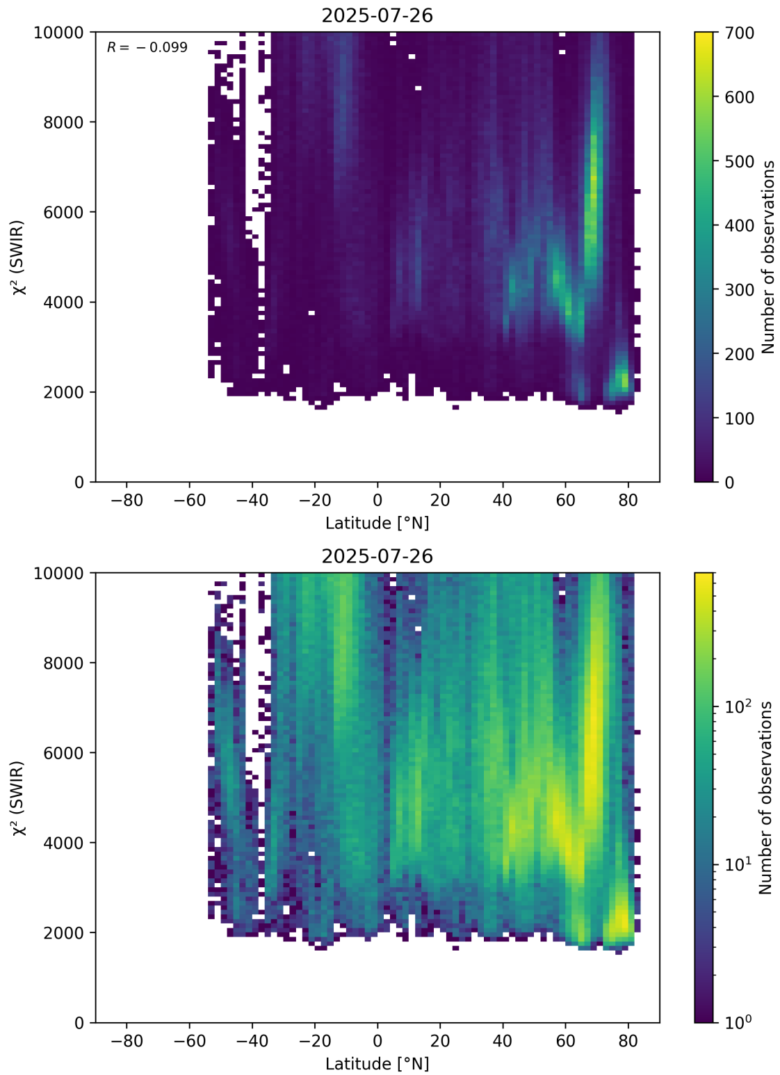
Figure 54: Scatter density plot of “Latitude” against “ \chi^2 (SWIR)” for 2025-07-25 to 2025-07-27.
