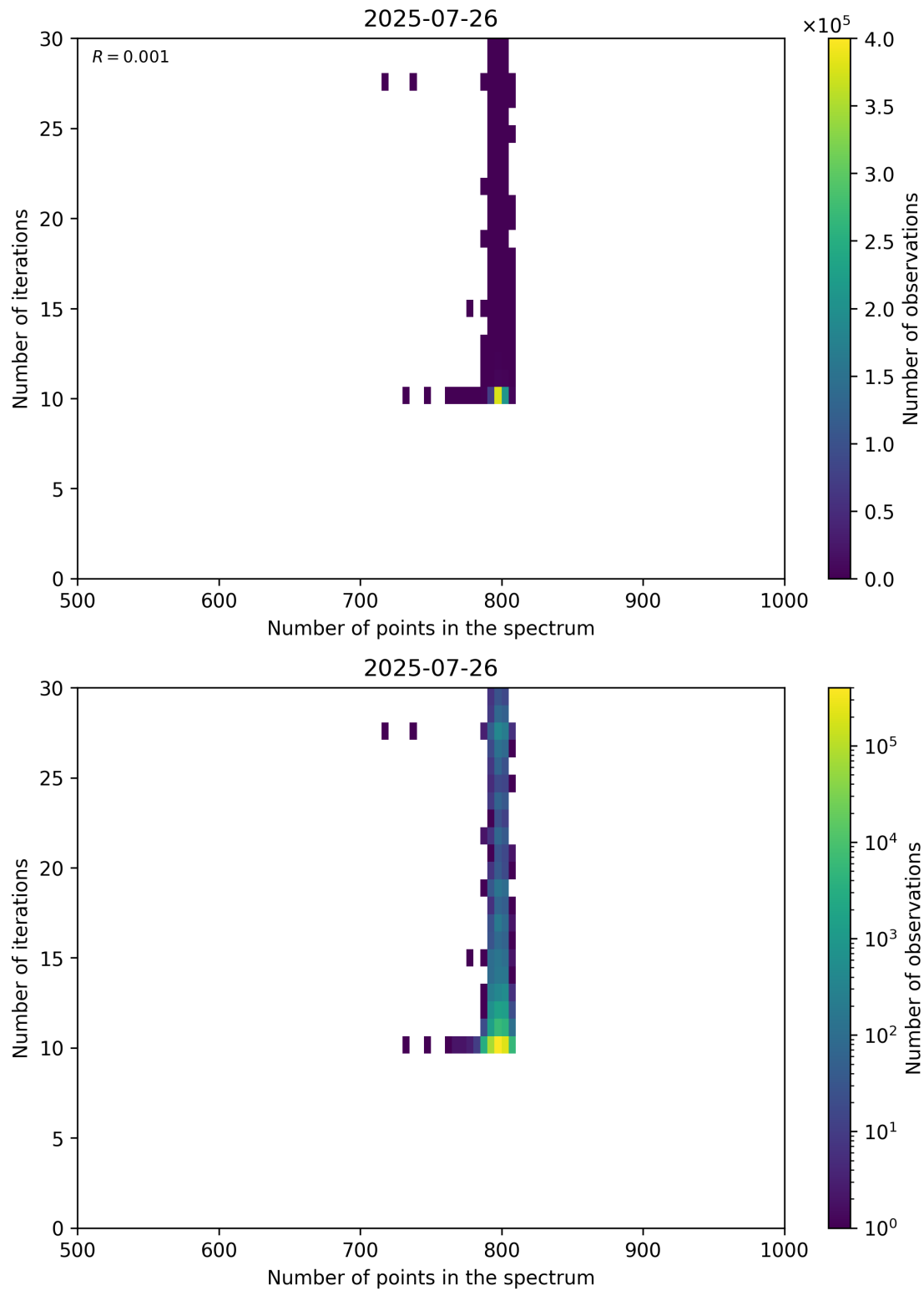
Figure 92: Scatter density plot of “Number of points in the spectrum” against “Number of iterations” for 2025-07-25 to 2025-07-27.
