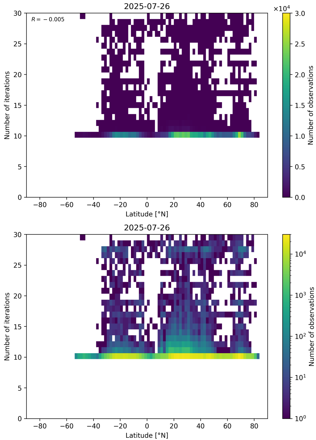
Figure 60: Scatter density plot of “Latitude” against “Number of iterations” for 2025-07-25 to 2025-07-27.
