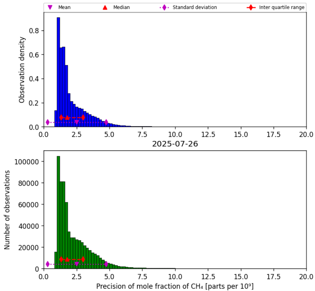
Figure 24: Histogram of “Precision of mole fraction of CH 4 ” for 2025-07-25 to 2025-07-27
