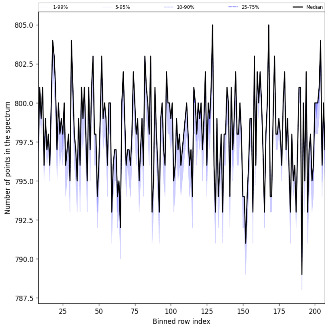
Figure 37: Along track statistics of “Number of points in the spectrum” for 2025-07-25 to 2025-07-27
