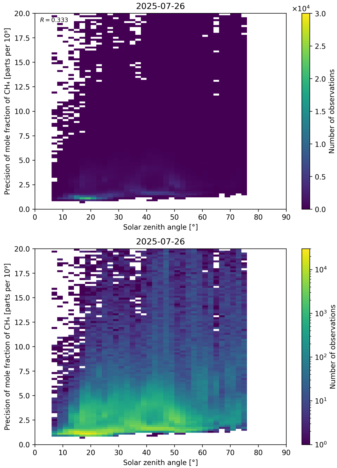
Figure 101: Scatter density plot of “Solar zenith angle” against “Precision of mole fraction of CH 4 ” for 2025-07-25 to 2025-07-27.
