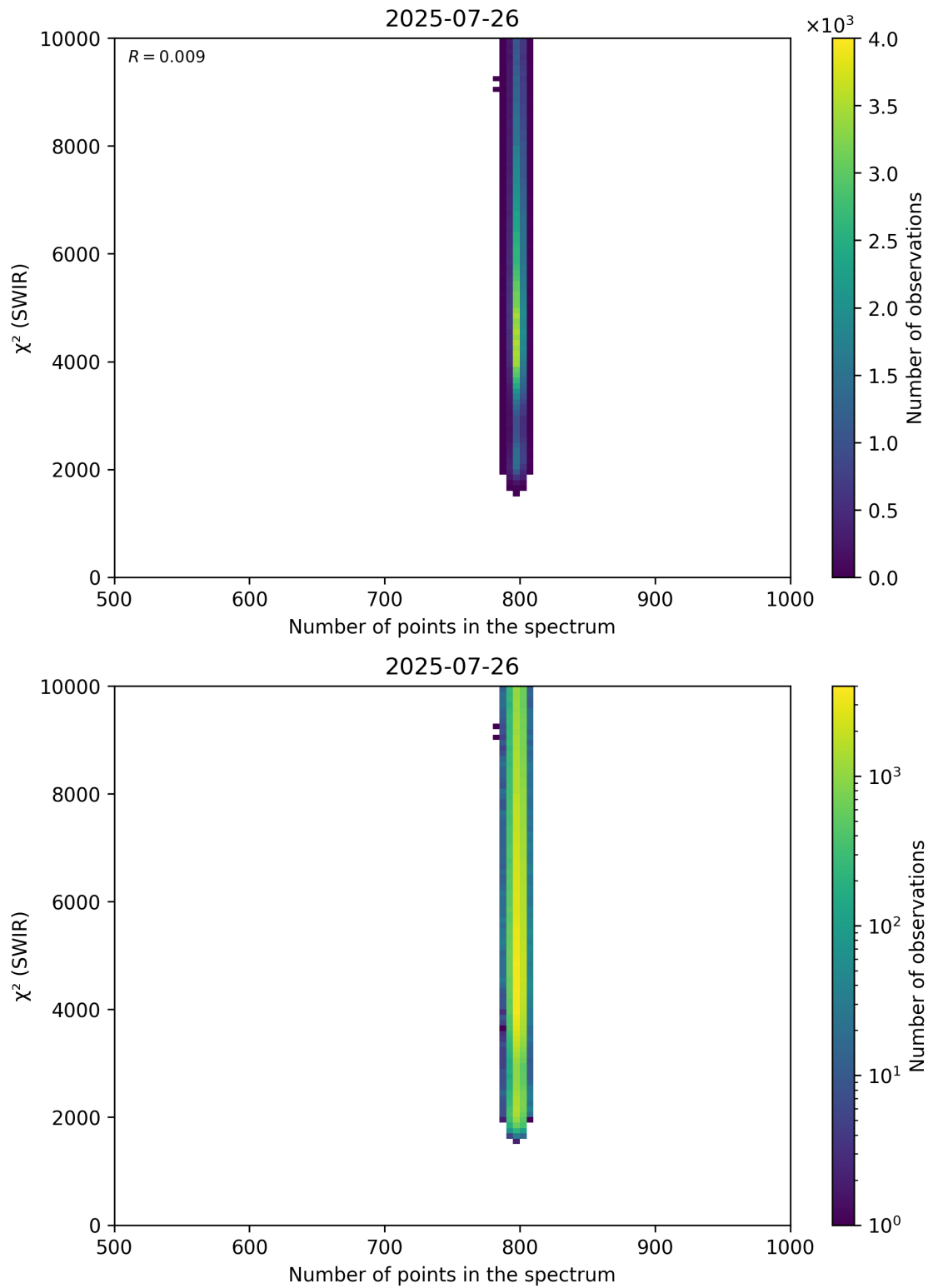
Figure 89: Scatter density plot of “Number of points in the spectrum” against “ \chi^2 (SWIR)” for 2025-07-25 to 2025-07-27.
