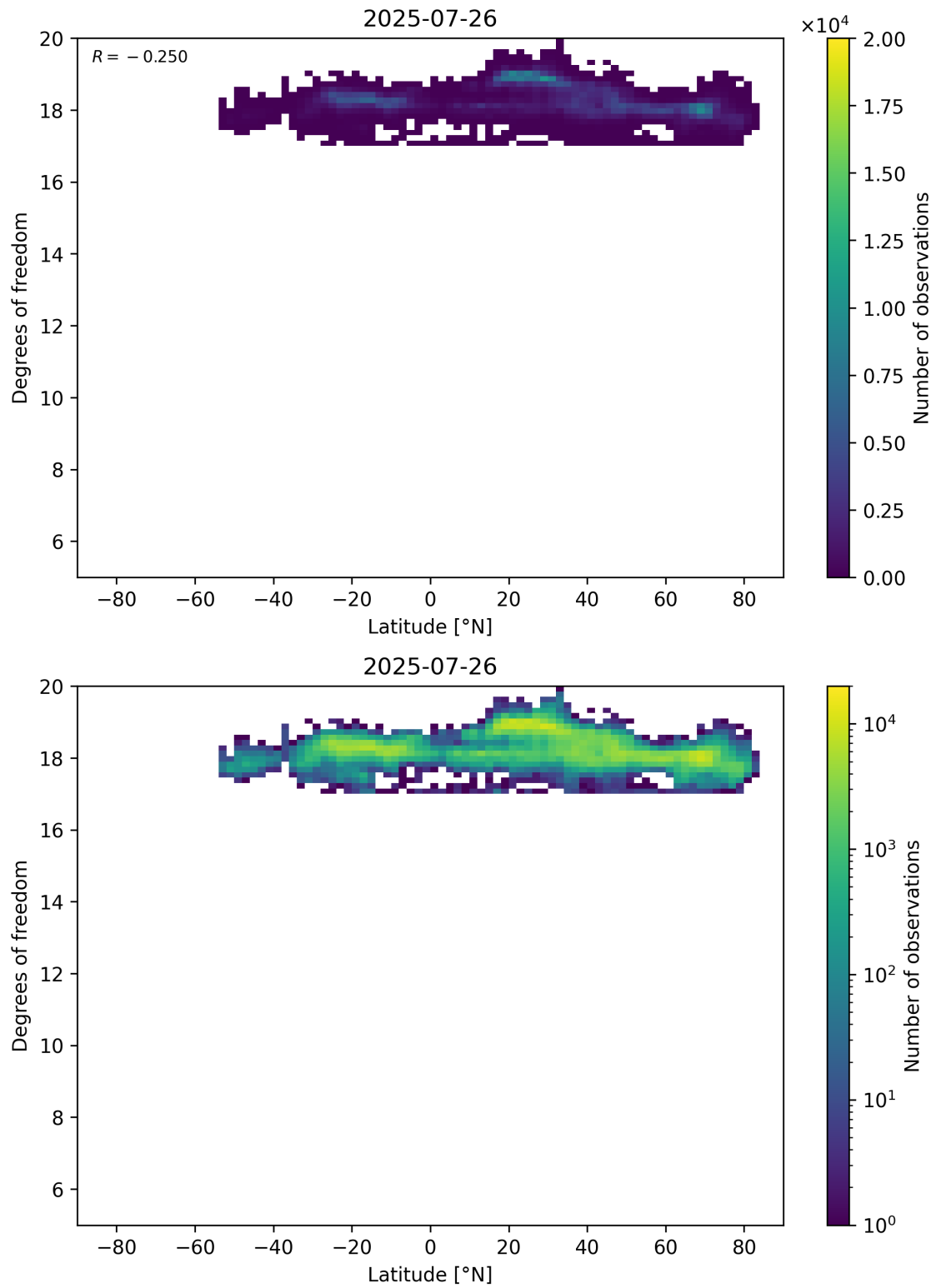
Figure 55: Scatter density plot of “Latitude” against “Degrees of freedom” for 2025-07-25 to 2025-07-27.
