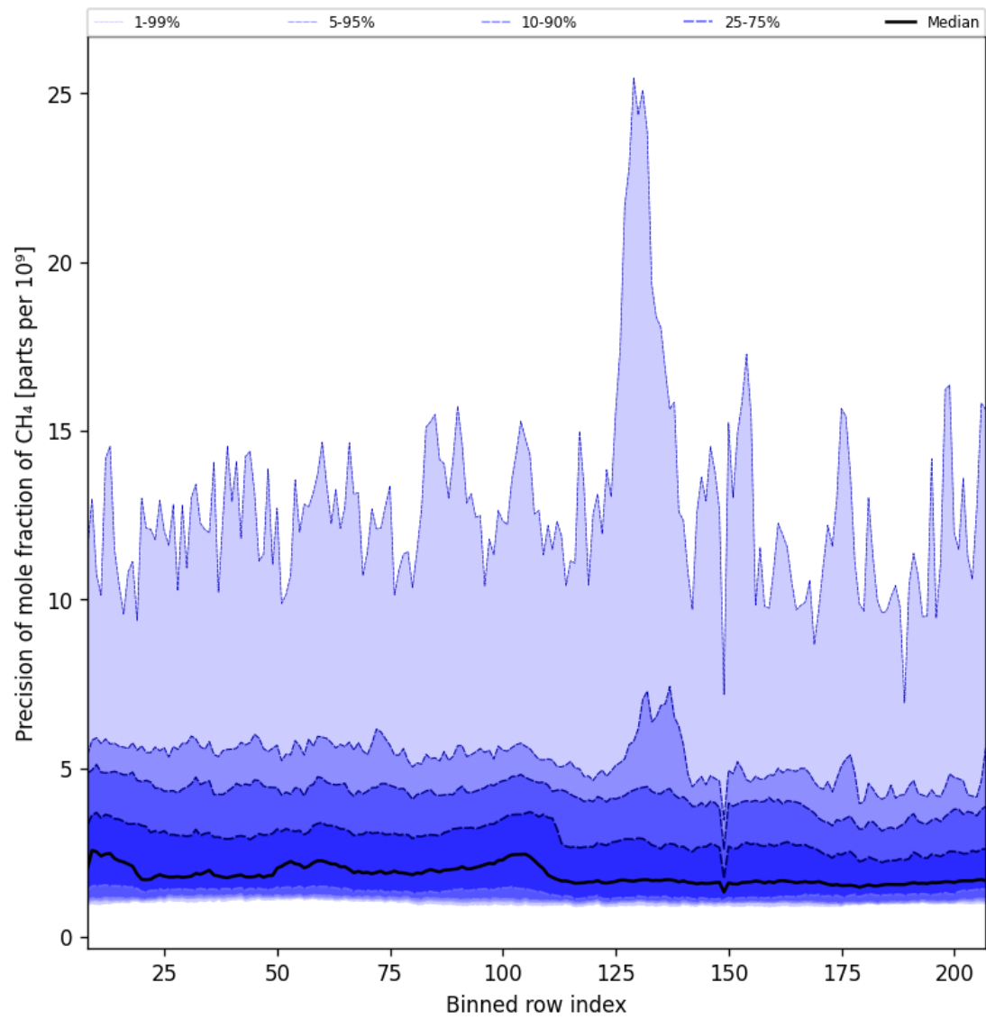
Figure 35: Along track statistics of “Precision of mole fraction of CH 4 ” for 2025-07-25 to 2025-07-27
