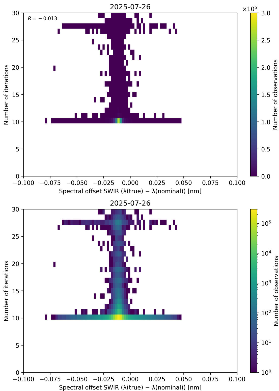
Figure 121: Scatter density plot of “Spectral offset SWIR ( \lambda_{\text{true}} - \lambda_{\text{nominal}} )” against “Number of iterations” for 2025-07-25 to 2025-07-27.
