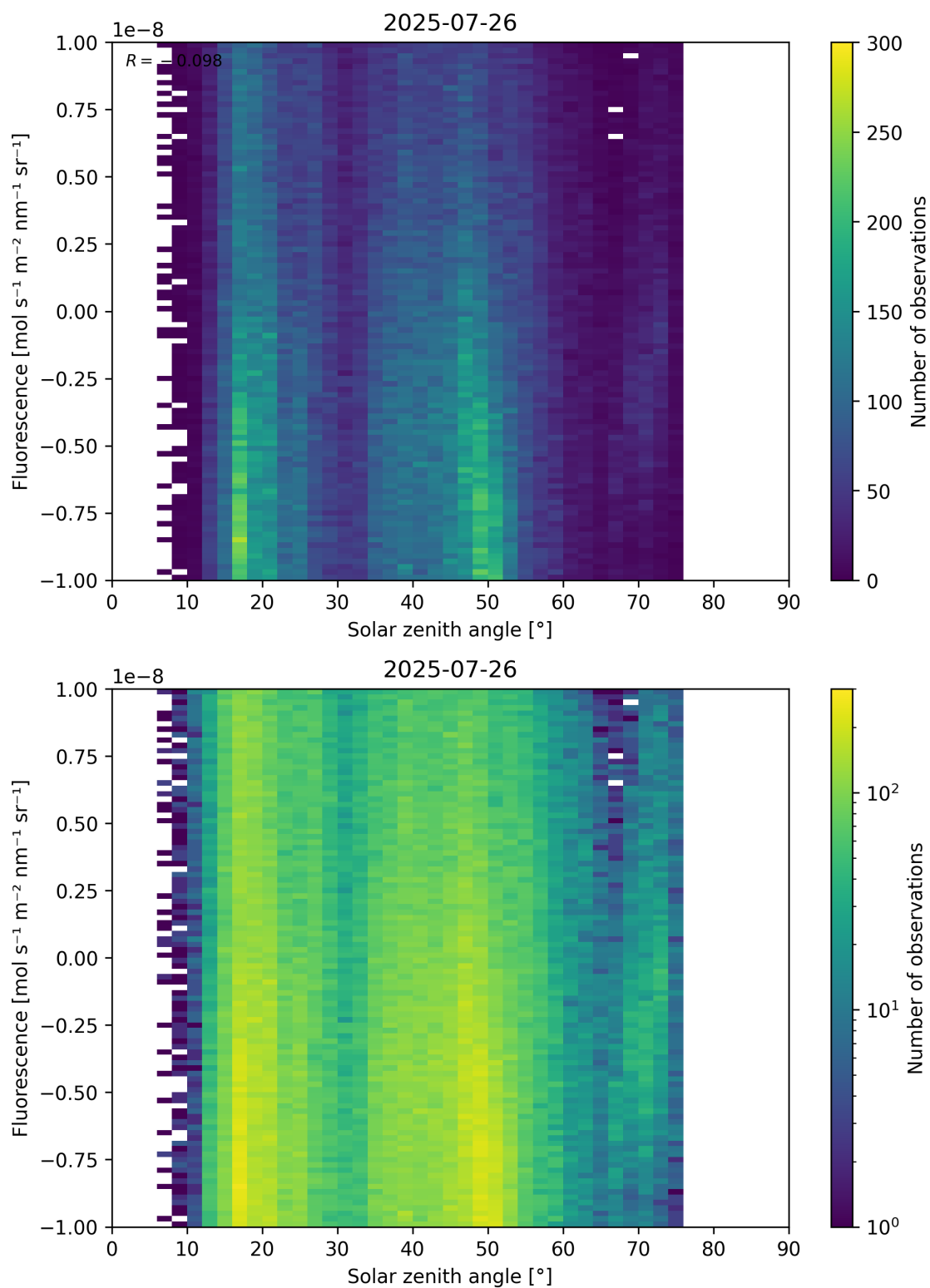
Figure 97: Scatter density plot of “Solar zenith angle” against “Fluorescence” for 2025-07-25 to 2025-07-27.
