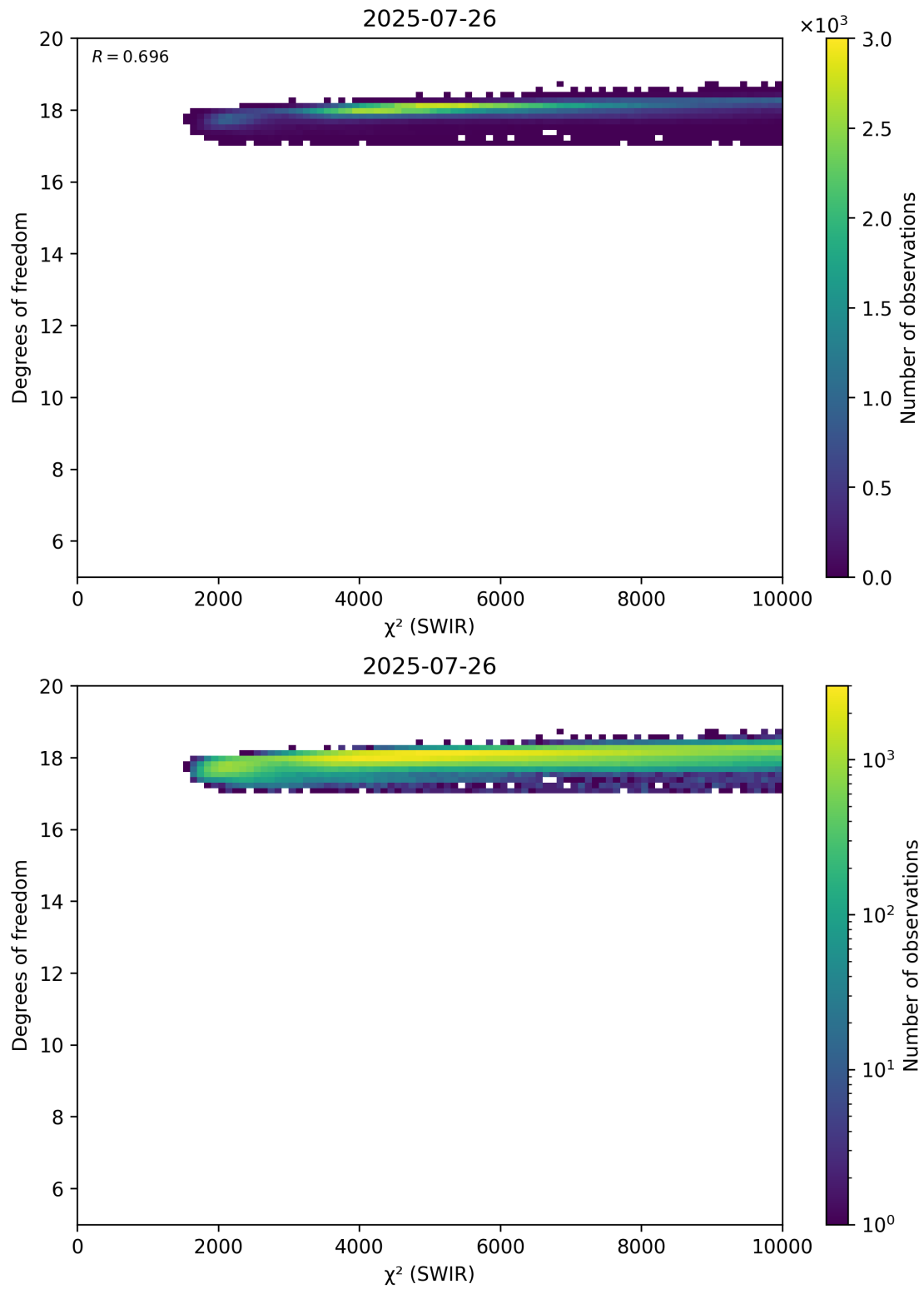
Figure 48: Scatter density plot of " \chi^2 (SWIR)" against "Degrees of freedom" for 2025-07-25 to 2025-07-27.
