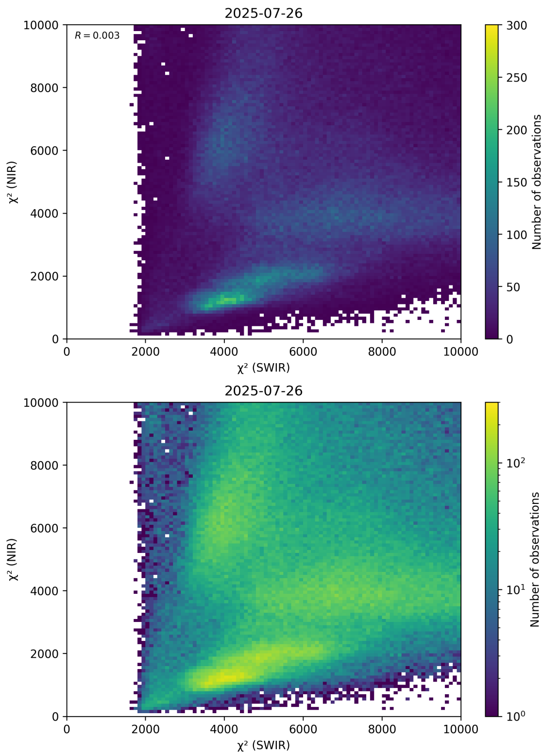
Figure 47: Scatter density plot of “ \chi^2 (SWIR)” against “ \chi^2 (NIR)” for 2025-07-25 to 2025-07-27.
