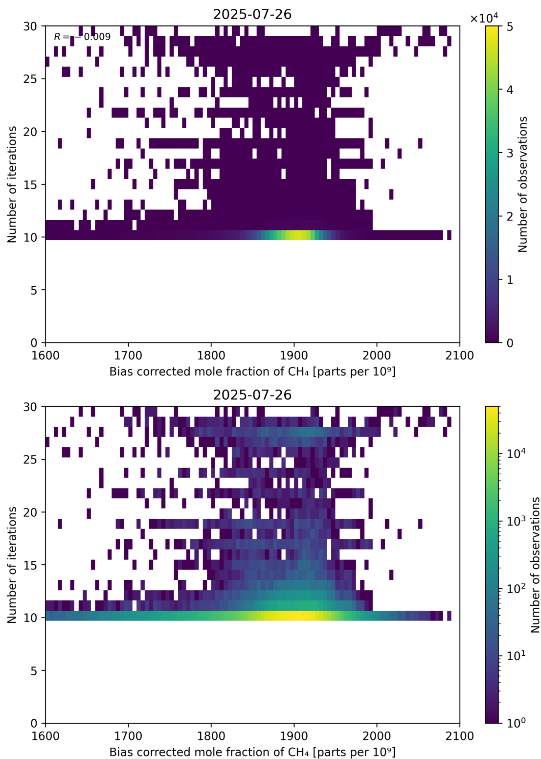
Figure 67: Scatter density plot of “Bias corrected mole fraction of CH 4 ” against “Number of iterations” for 2025-07-25 to 2025-07-27.
