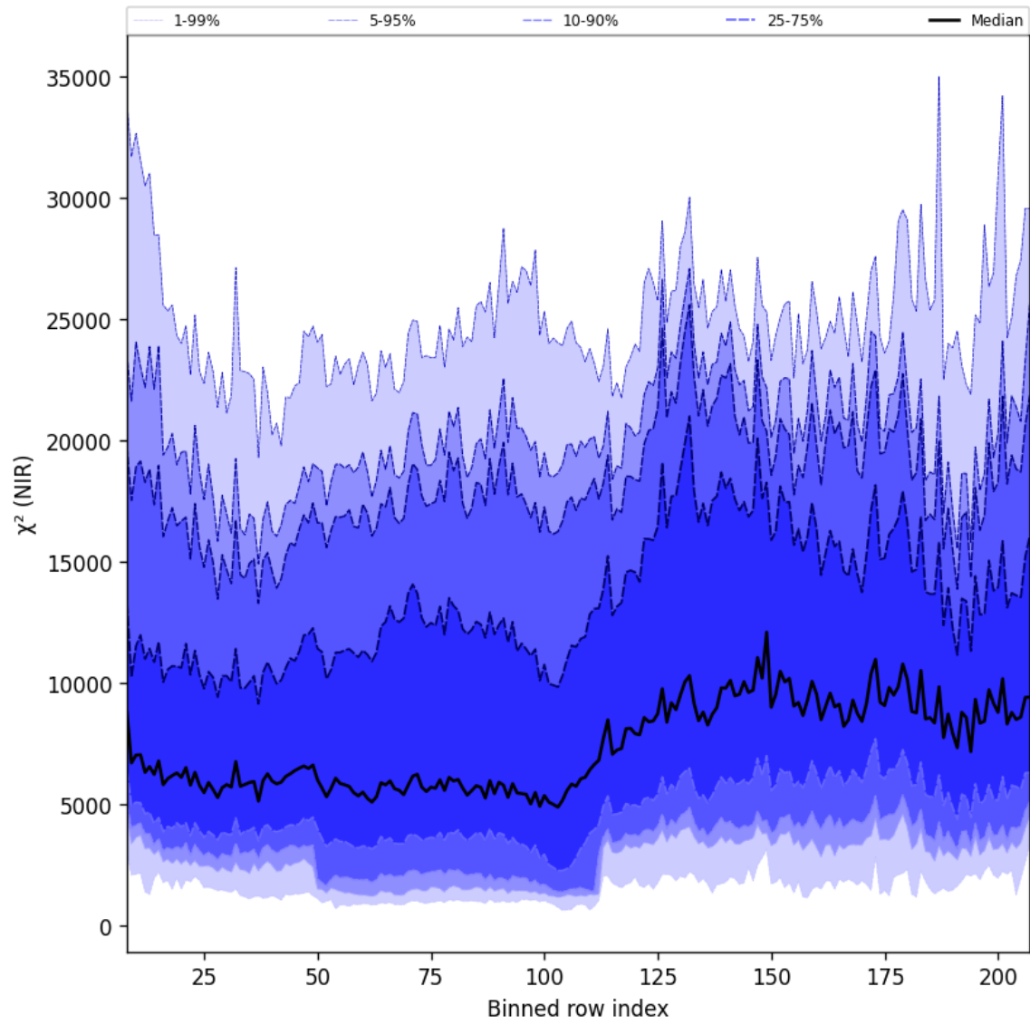
Figure 40: Along track statistics of " \chi^2 (NIR)" for 2025-07-25 to 2025-07-27
