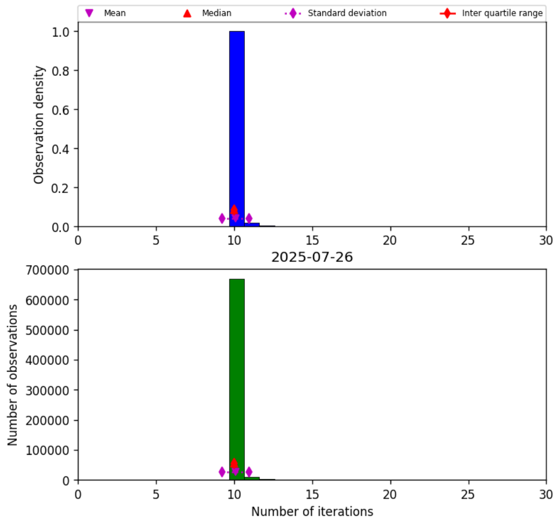
Figure 31: Histogram of “Number of iterations” for 2025-07-25 to 2025-07-27
