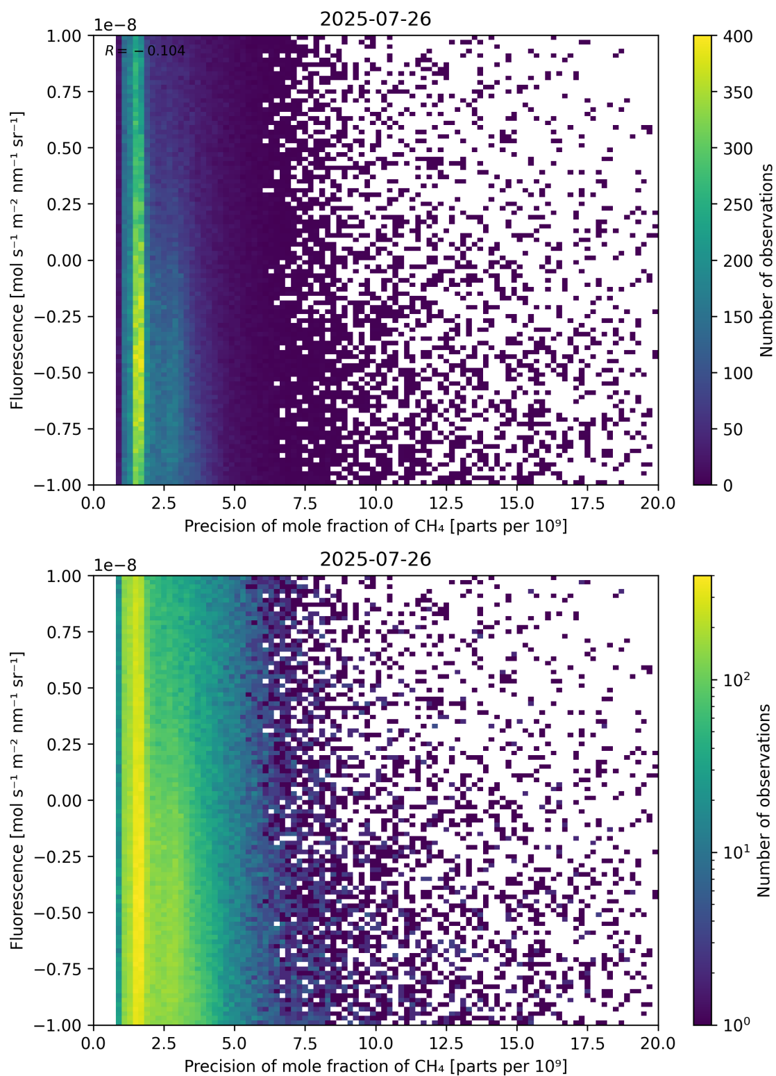
Figure 81: Scatter density plot of “Precision of mole fraction of \text{CH}_4 ” against “Fluorescence” for 2025-07-25 to 2025-07-27.
