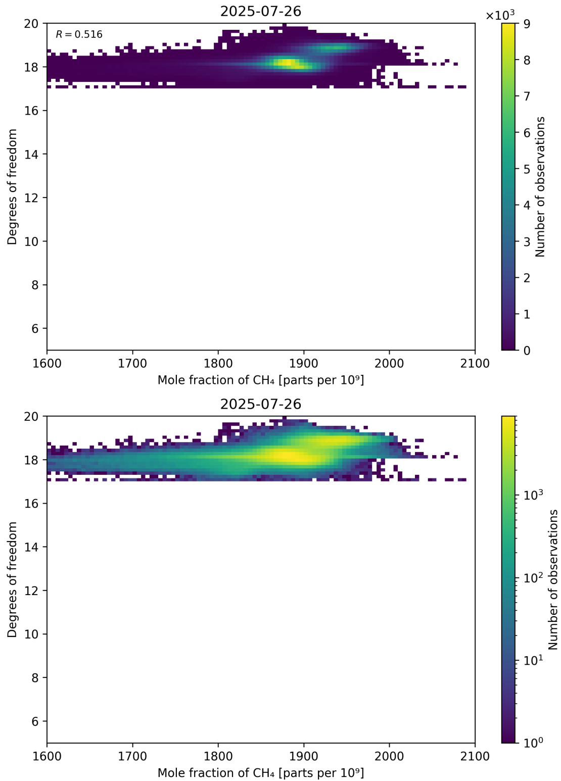
Figure 72: Scatter density plot of “Mole fraction of CH 4 ” against “Degrees of freedom” for 2025-07-25 to 2025-07-27.
