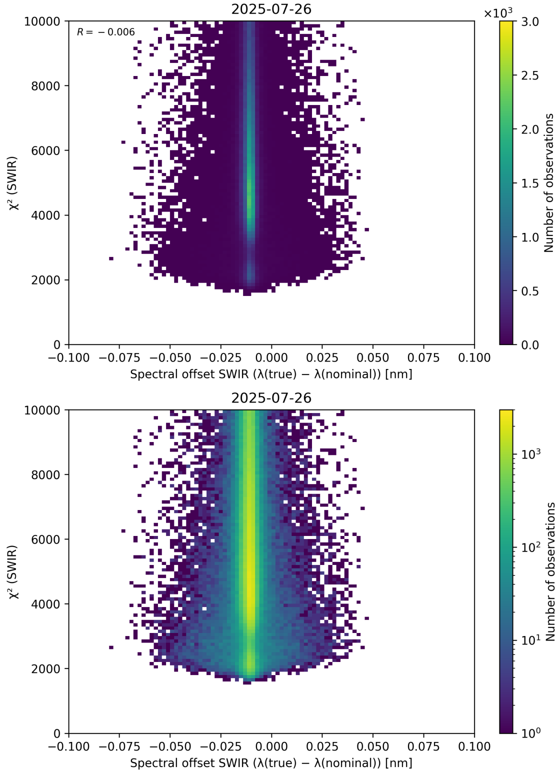
Figure 118: Scatter density plot of “Spectral offset SWIR ( \lambda_{\text{true}} - \lambda_{\text{nominal}} )” against “ \chi^2 (SWIR)” for 2025-07-25 to 2025-07-27.
