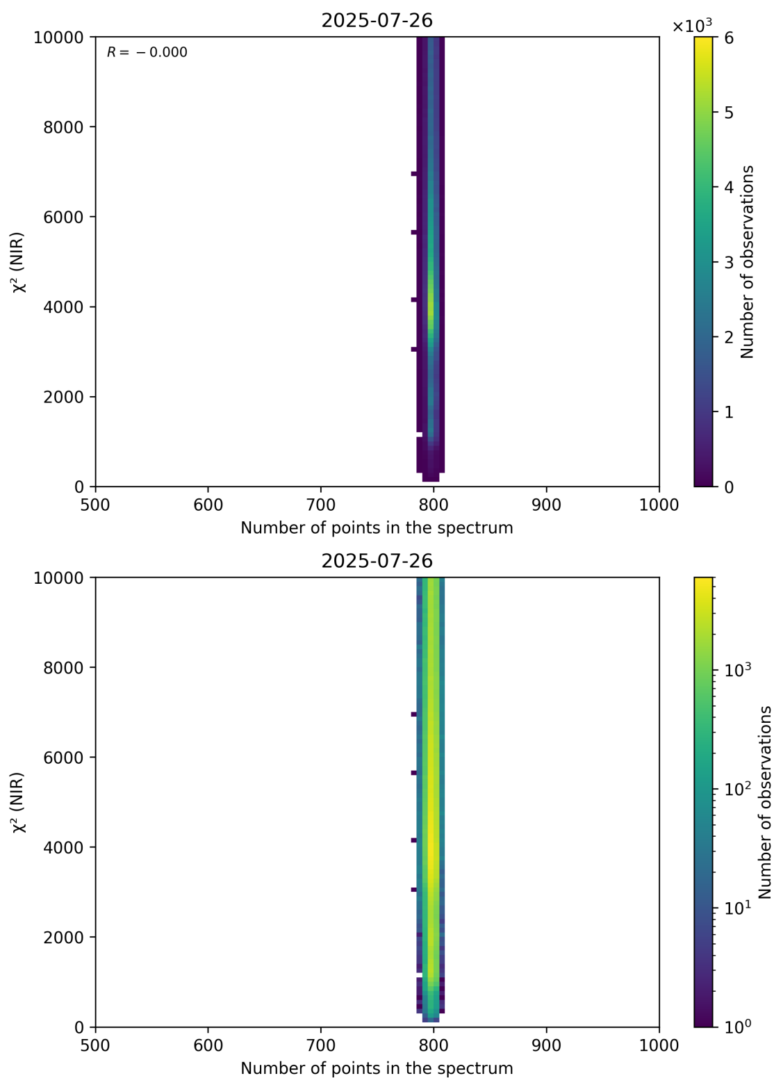
Figure 88: Scatter density plot of “Number of points in the spectrum” against “ \chi^2 (NIR)” for 2025-07-25 to 2025-07-27.
