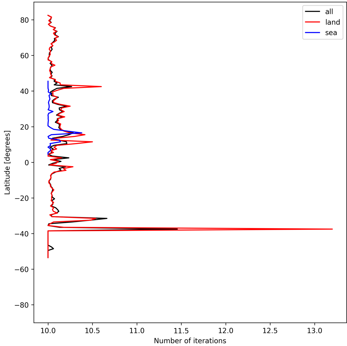
Figure 20: Zonal average of “Number of iterations” for 2025-07-25 to 2025-07-27.
