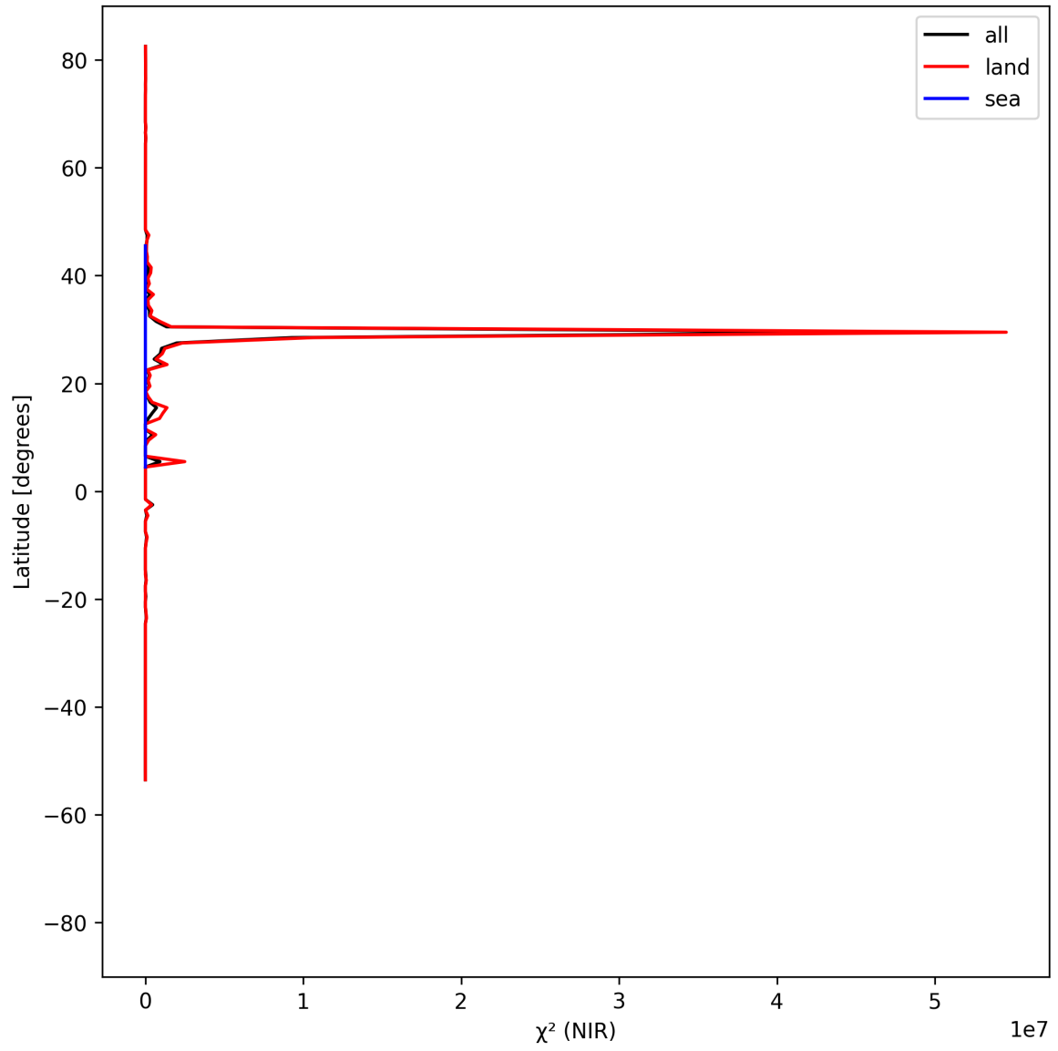
Figure 18: Zonal average of “ \chi^2 (NIR)” for 2025-07-25 to 2025-07-27.
