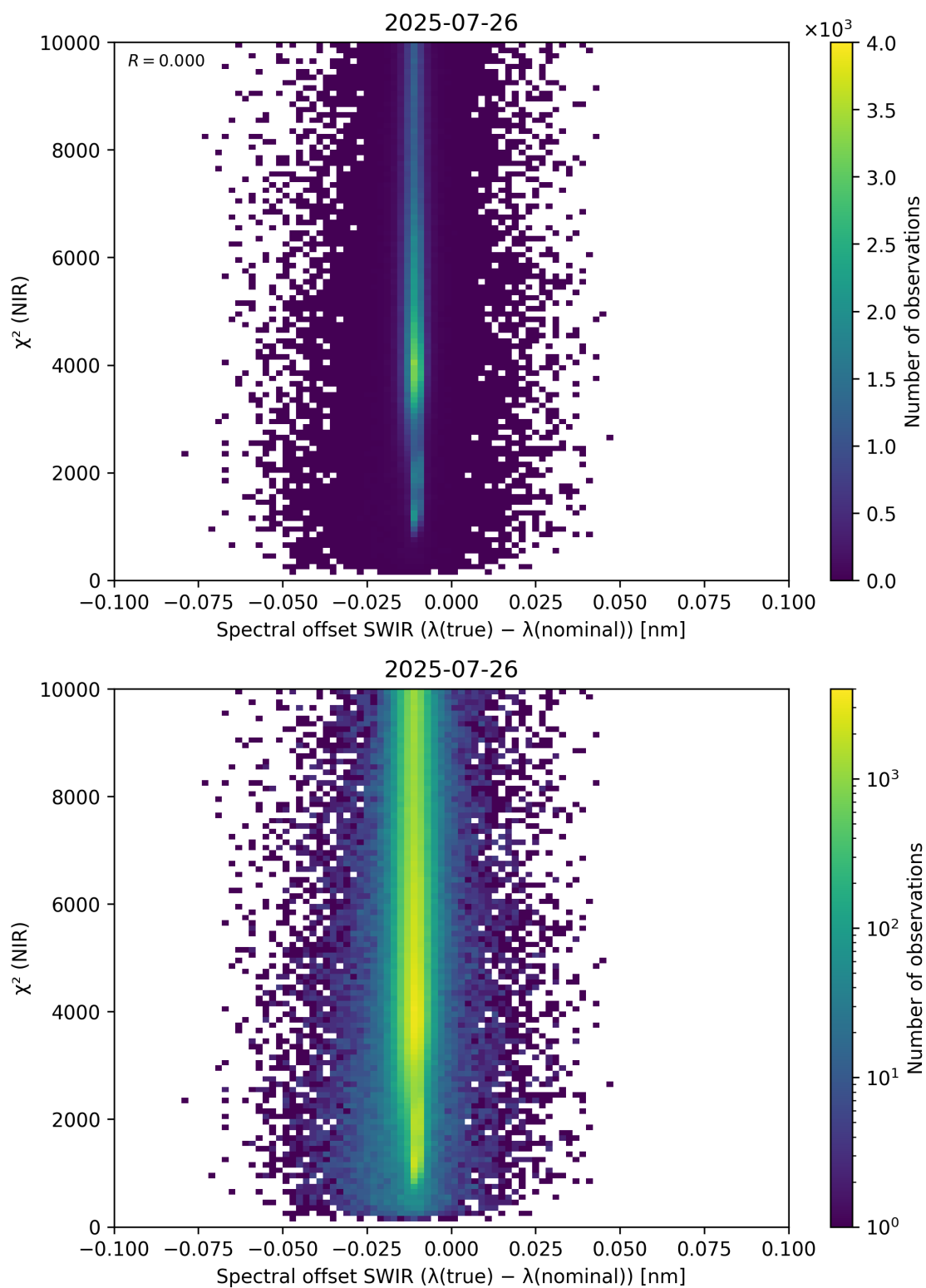
Figure 117: Scatter density plot of “Spectral offset SWIR ( \lambda_{\text{true}} - \lambda_{\text{nominal}} )” against “ \chi^2 (NIR)” for 2025-07-25 to 2025-07-27.
