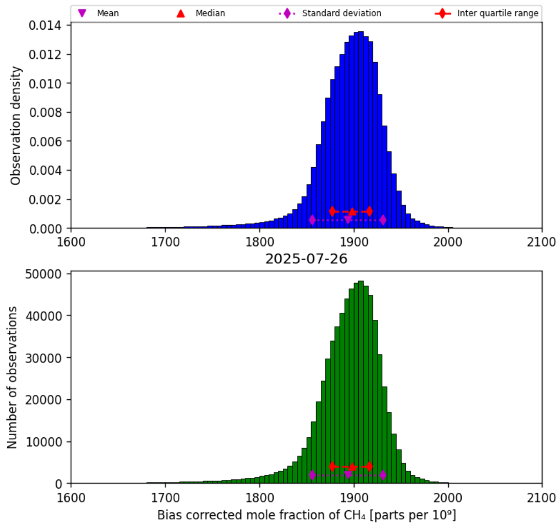
Figure 25: Histogram of “Bias corrected mole fraction of CH 4 ” for 2025-07-25 to 2025-07-27
