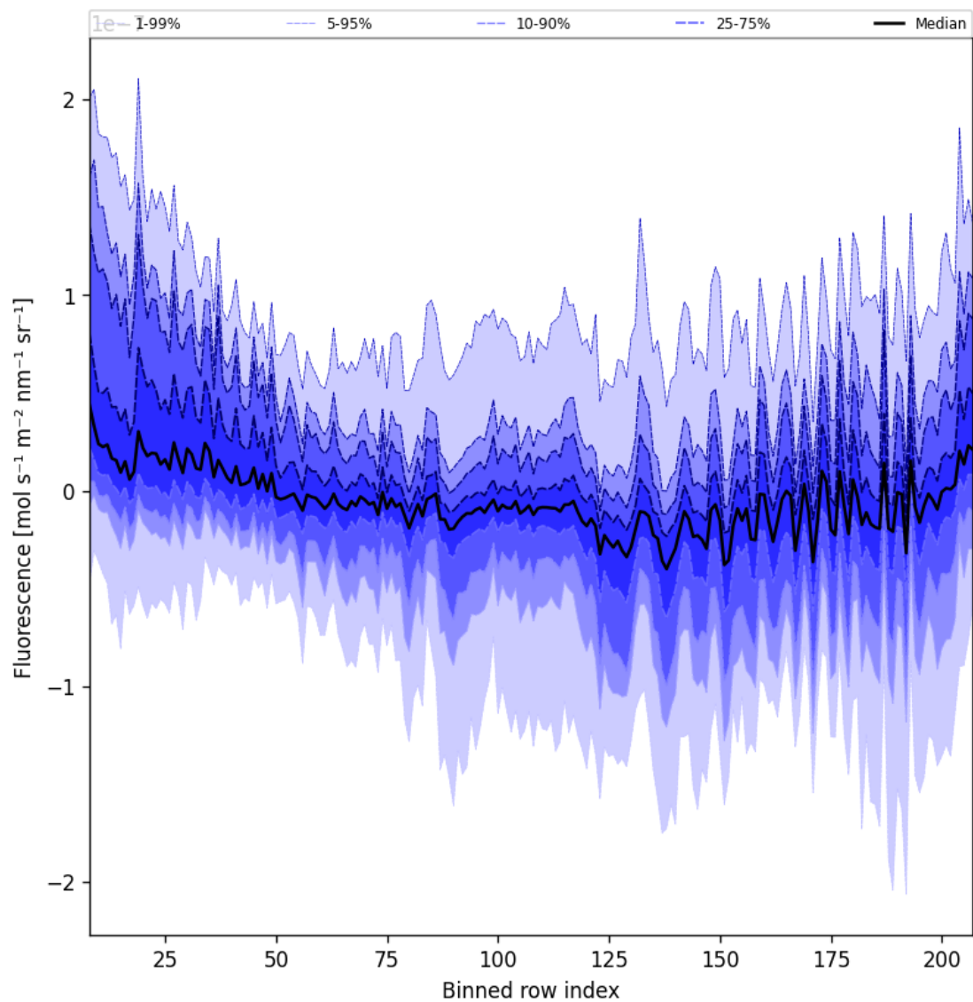
Figure 43: Along track statistics of “Fluorescence” for 2025-07-25 to 2025-07-27
