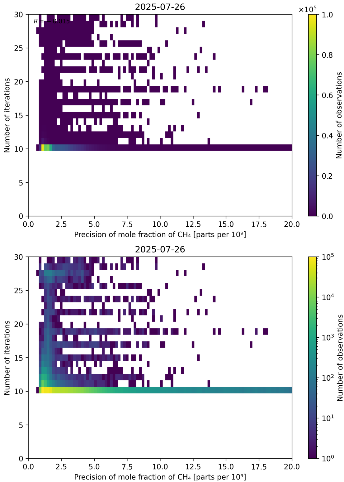
Figure 83: Scatter density plot of “Precision of mole fraction of CH 4 ” against “Number of iterations” for 2025-07-25 to 2025-07-27.
