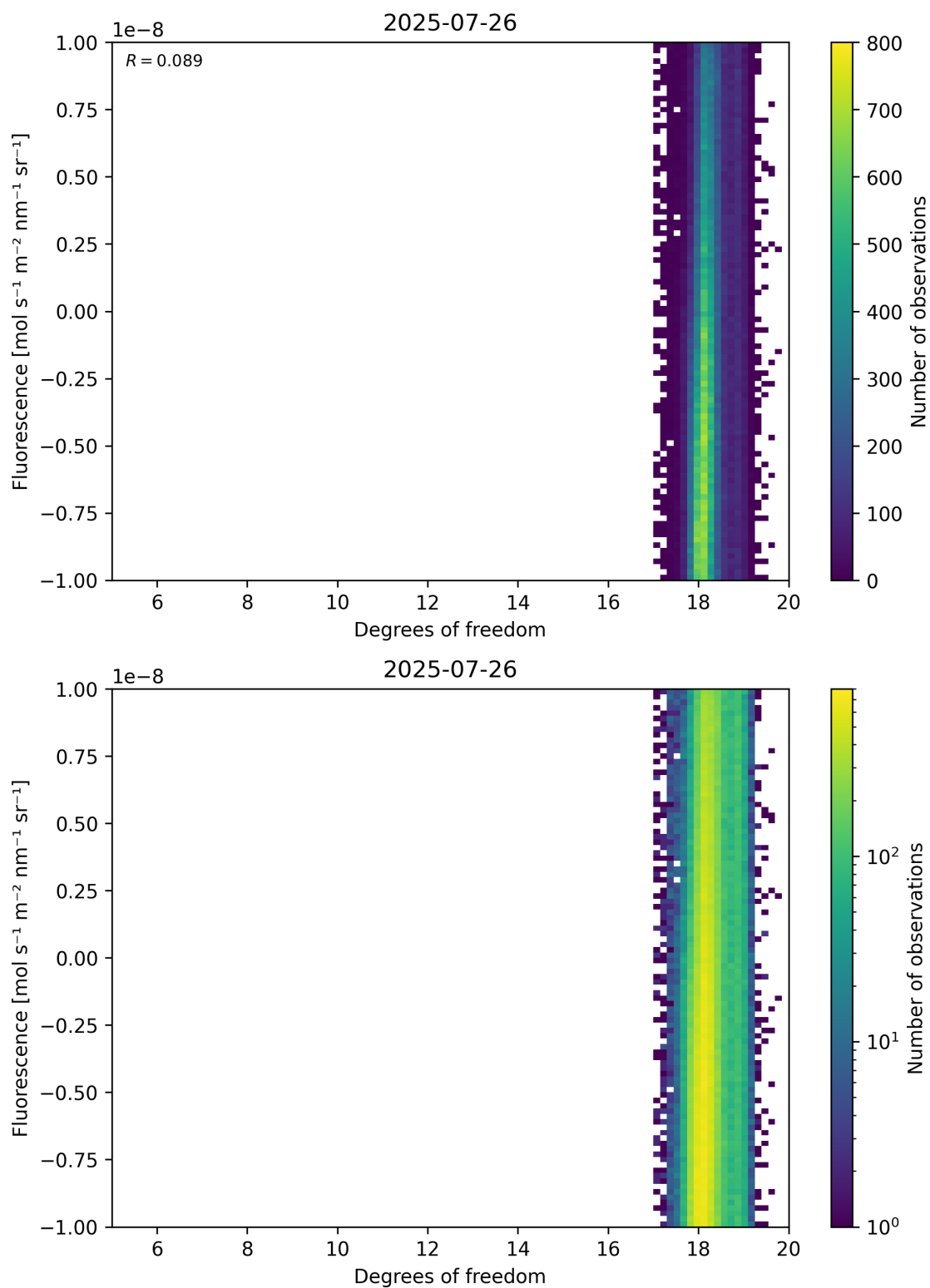
Figure 51: Scatter density plot of “Degrees of freedom” against “Fluorescence” for 2025-07-25 to 2025-07-27.
