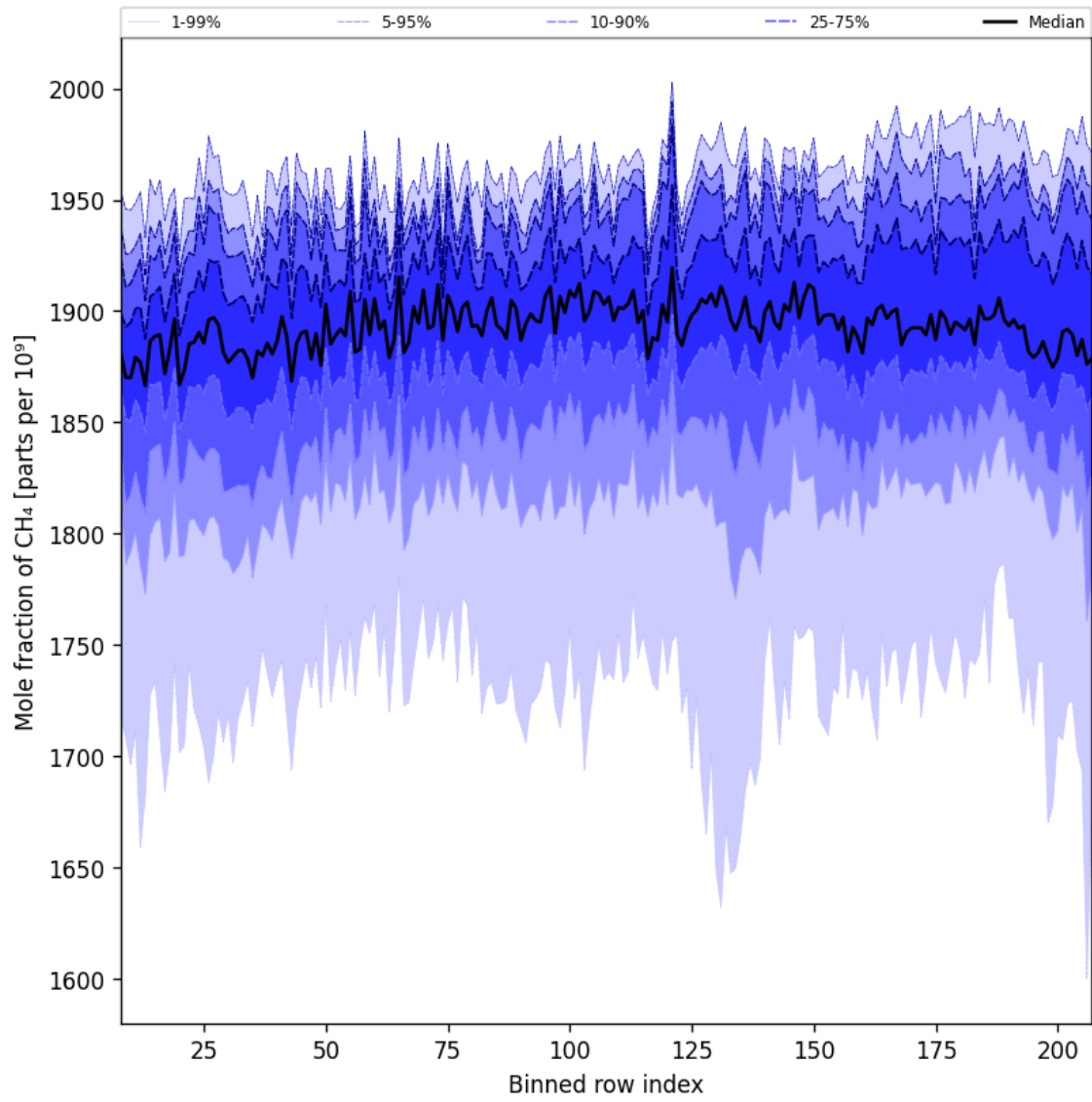
Figure 34: Along track statistics of “Mole fraction of CH 4 ” for 2025-07-25 to 2025-07-27
