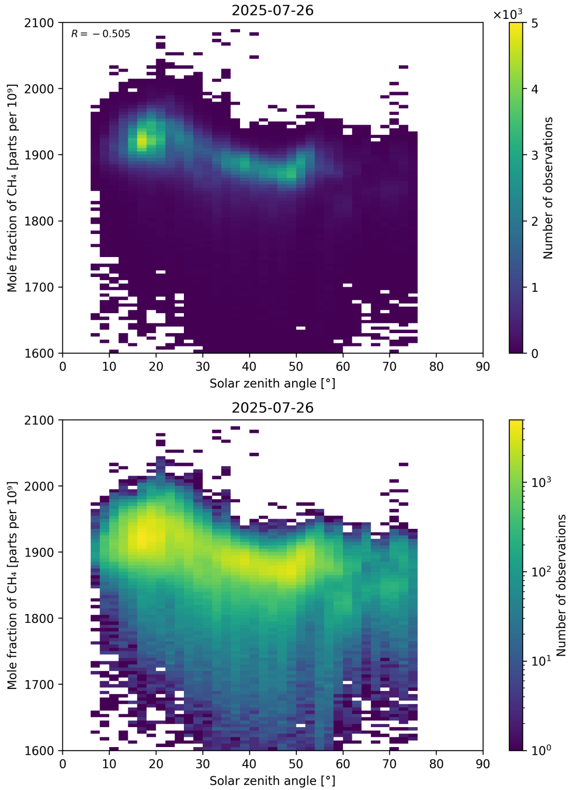
Figure 99: Scatter density plot of “Solar zenith angle” against “Mole fraction of \text{CH}_4 ” for 2025-07-25 to 2025-07-27.
