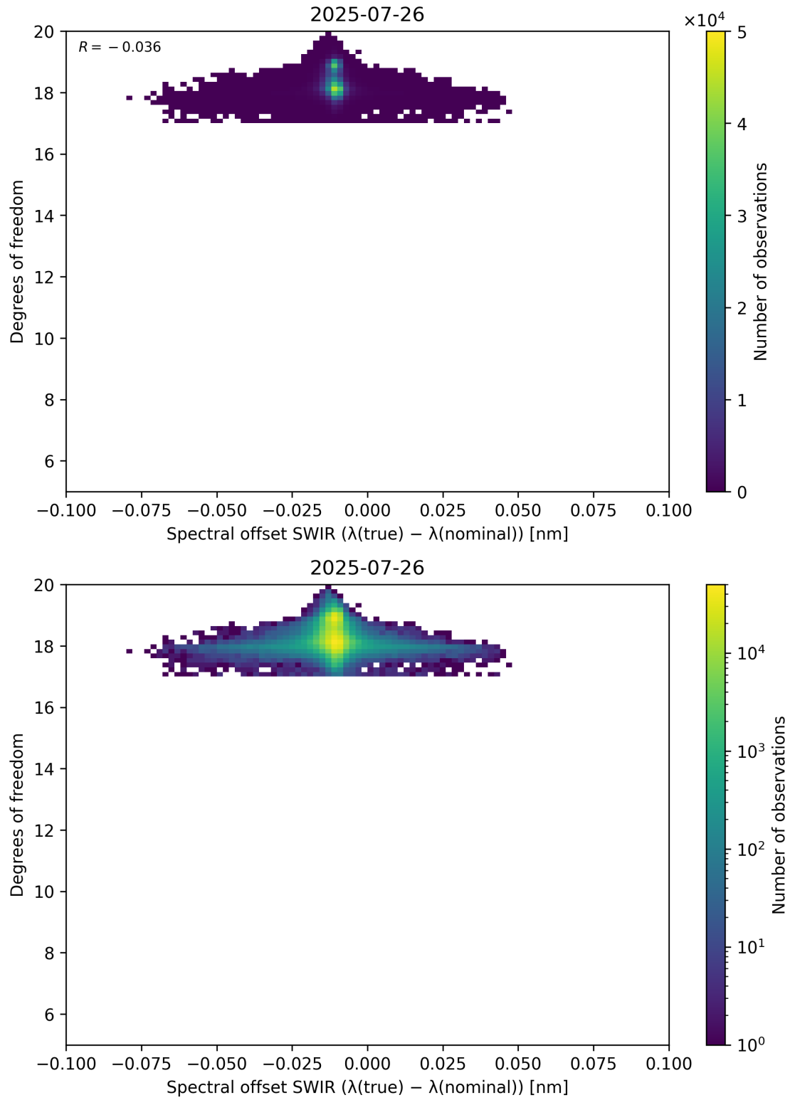
Figure 119: Scatter density plot of “Spectral offset SWIR ( \lambda_{\text{true}} - \lambda_{\text{nominal}} )” against “Degrees of freedom” for 2025-07-25 to 2025-07-27.
