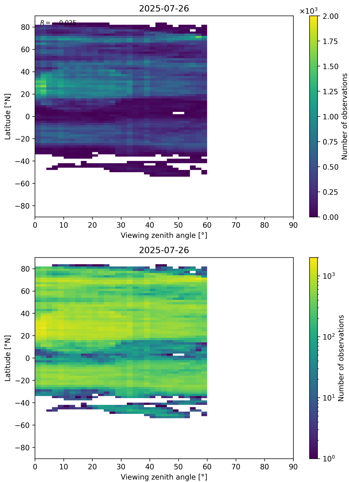
Figure 109: Scatter density plot of “Viewing zenith angle” against “Latitude” for 2025-07-25 to 2025-07-27.
