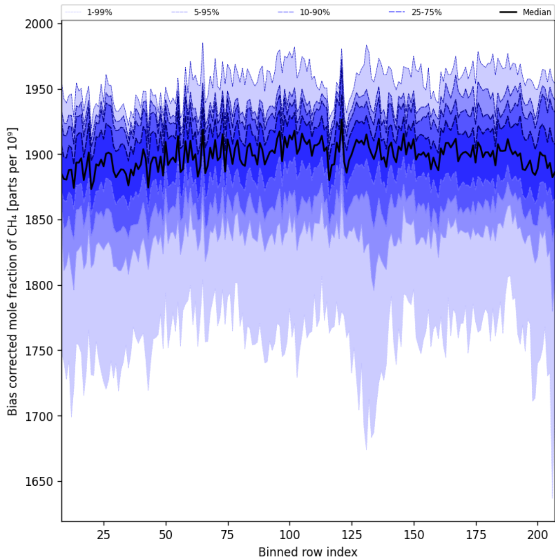
Figure 36: Along track statistics of “Bias corrected mole fraction of CH 4 ” for 2025-07-25 to 2025-07-27
