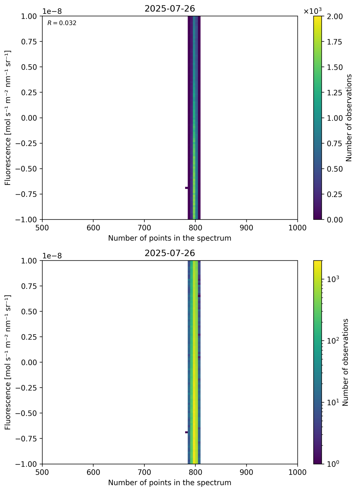
Figure 91: Scatter density plot of “Number of points in the spectrum” against “Fluorescence” for 2025-07-25 to 2025-07-27.
