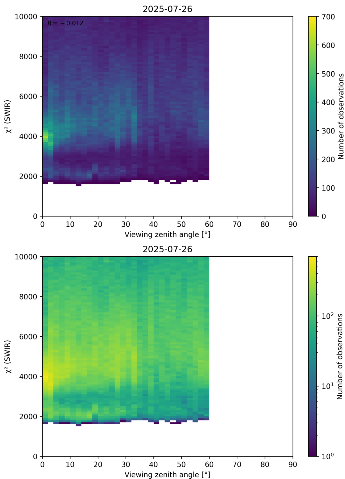
Figure 106: Scatter density plot of “Viewing zenith angle” against “ \chi^2 (SWIR)” for 2025-07-25 to 2025-07-27.
