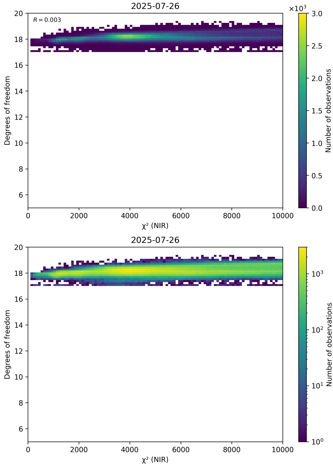
Figure 44: Scatter density plot of “ \chi^2 (NIR)” against “Degrees of freedom” for 2025-07-25 to 2025-07-27.
