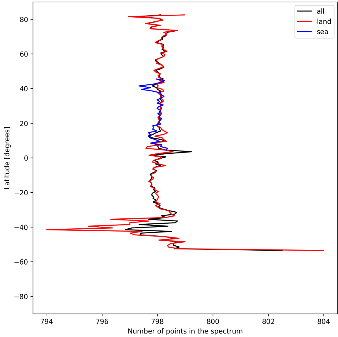
Figure 15: Zonal average of “Number of points in the spectrum” for 2025-07-25 to 2025-07-27.
