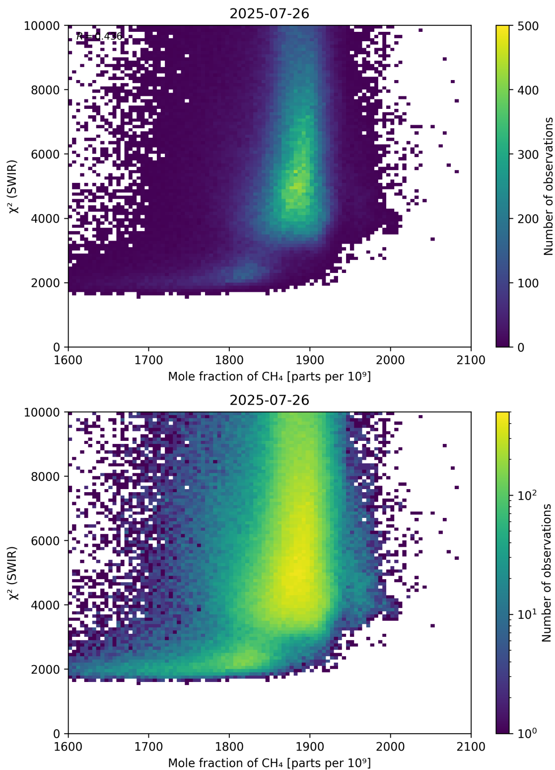
Figure 71: Scatter density plot of “Mole fraction of \text{CH}_4 ” against “ \chi^2 (SWIR)” for 2025-07-25 to 2025-07-27.
