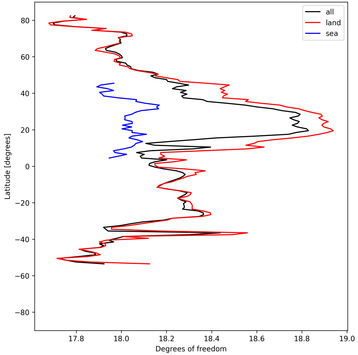
Figure 19: Zonal average of “Degrees of freedom” for 2025-07-25 to 2025-07-27.
