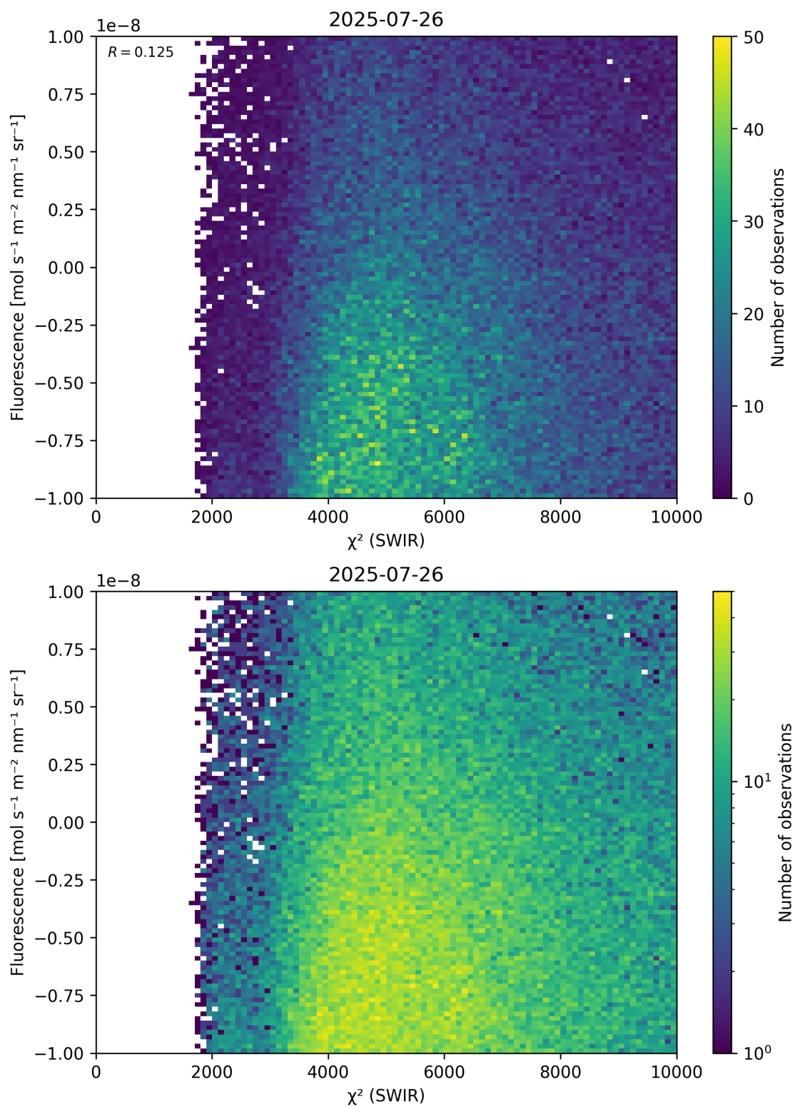
Figure 49: Scatter density plot of “ \chi^2 (SWIR)” against “Fluorescence” for 2025-07-25 to 2025-07-27.
