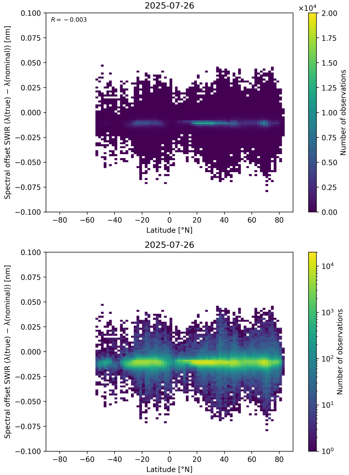
Figure 62: Scatter density plot of “Latitude” against “Spectral offset SWIR ( \lambda_{\text{true}} - \lambda_{\text{nominal}} )” for 2025-07-25 to 2025-07-27.
