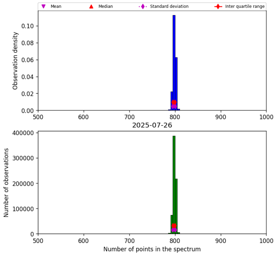
Figure 26: Histogram of “Number of points in the spectrum” for 2025-07-25 to 2025-07-27
