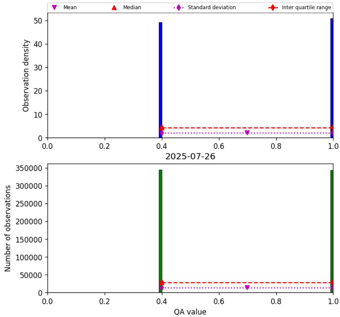
Figure 22: Histogram of “QA value” for 2025-07-25 to 2025-07-27
