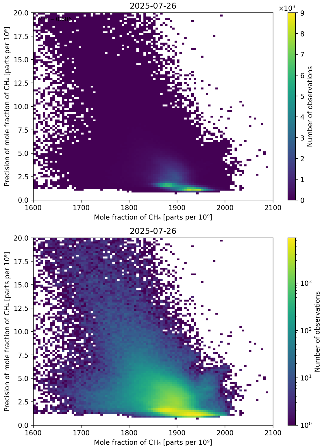
Figure 75: Scatter density plot of “Mole fraction of CH 4 ” against “Precision of mole fraction of CH 4 ” for 2025-07-25 to 2025-07-27.
