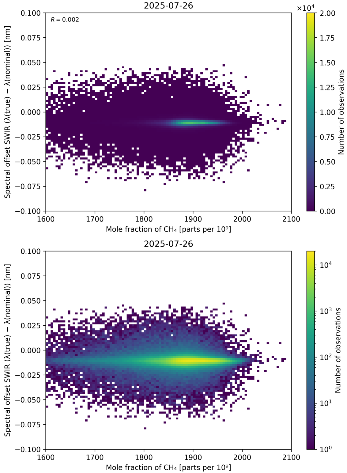
Figure 86: Scatter density plot of “Mole fraction of CH 4 ” against “Spectral offset SWIR ( \lambda_{\text{true}} - \lambda_{\text{nominal}} )” for 2025-07-25 to 2025-07-27.
