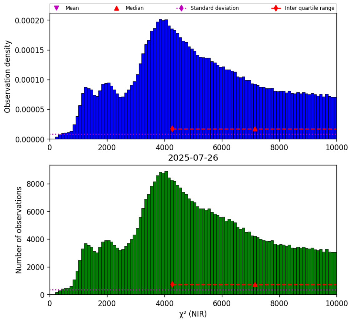
Figure 29: Histogram of “ \chi^2 (NIR)” for 2025-07-25 to 2025-07-27
