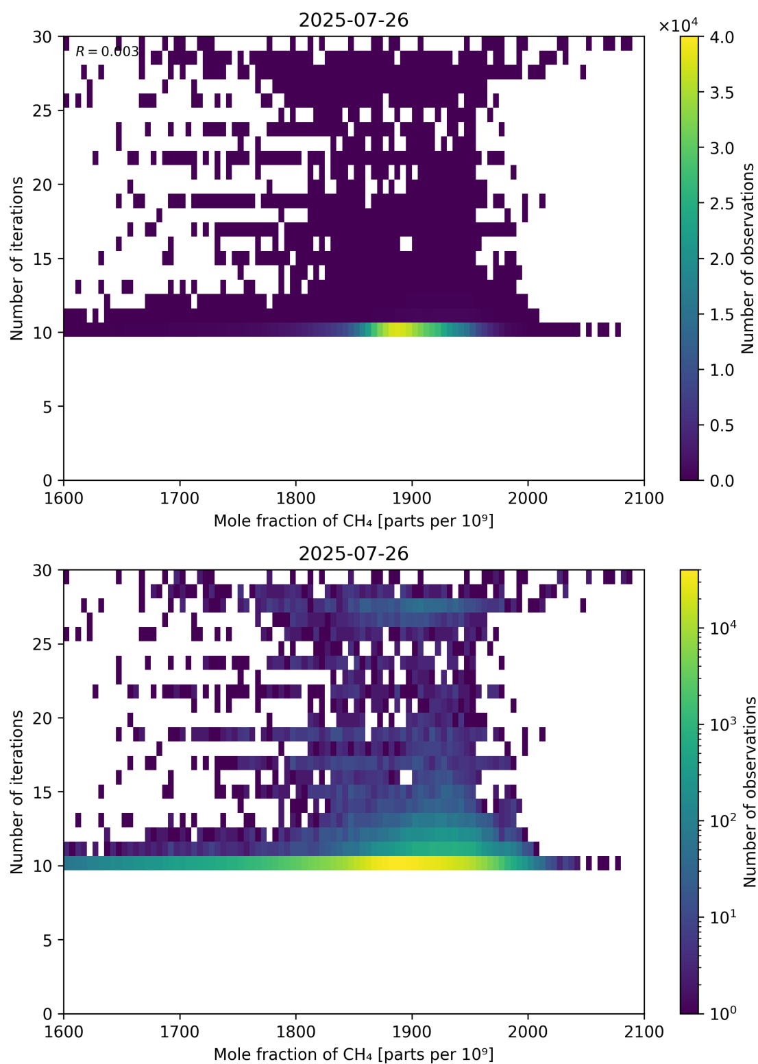
Figure 76: Scatter density plot of “Mole fraction of CH 4 ” against “Number of iterations” for 2025-07-25 to 2025-07-27.
