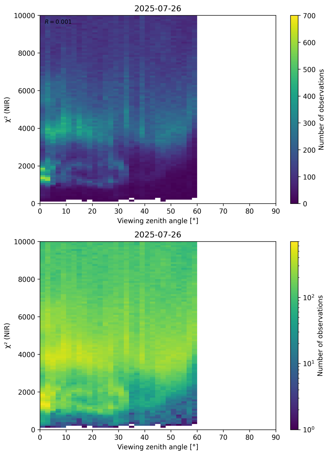
Figure 105: Scatter density plot of “Viewing zenith angle” against “ \chi^2 (NIR)” for 2025-07-25 to 2025-07-27.
