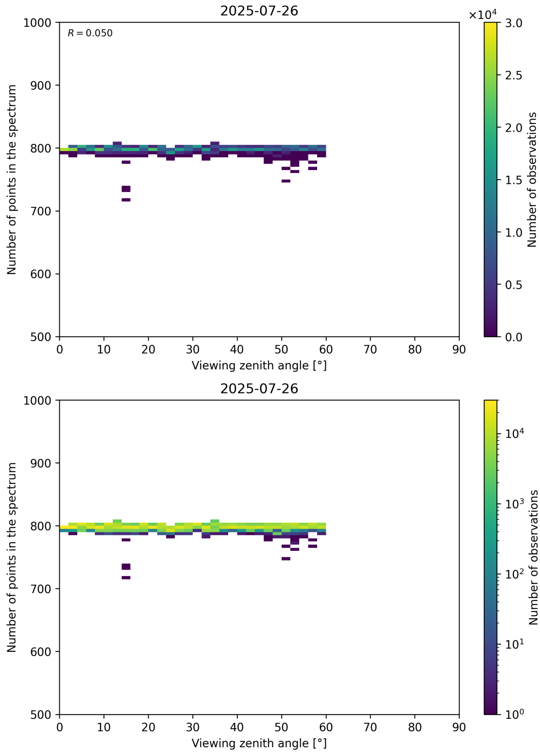
Figure 114: Scatter density plot of “Viewing zenith angle” against “Number of points in the spectrum” for 2025-07-25 to 2025-07-27.
