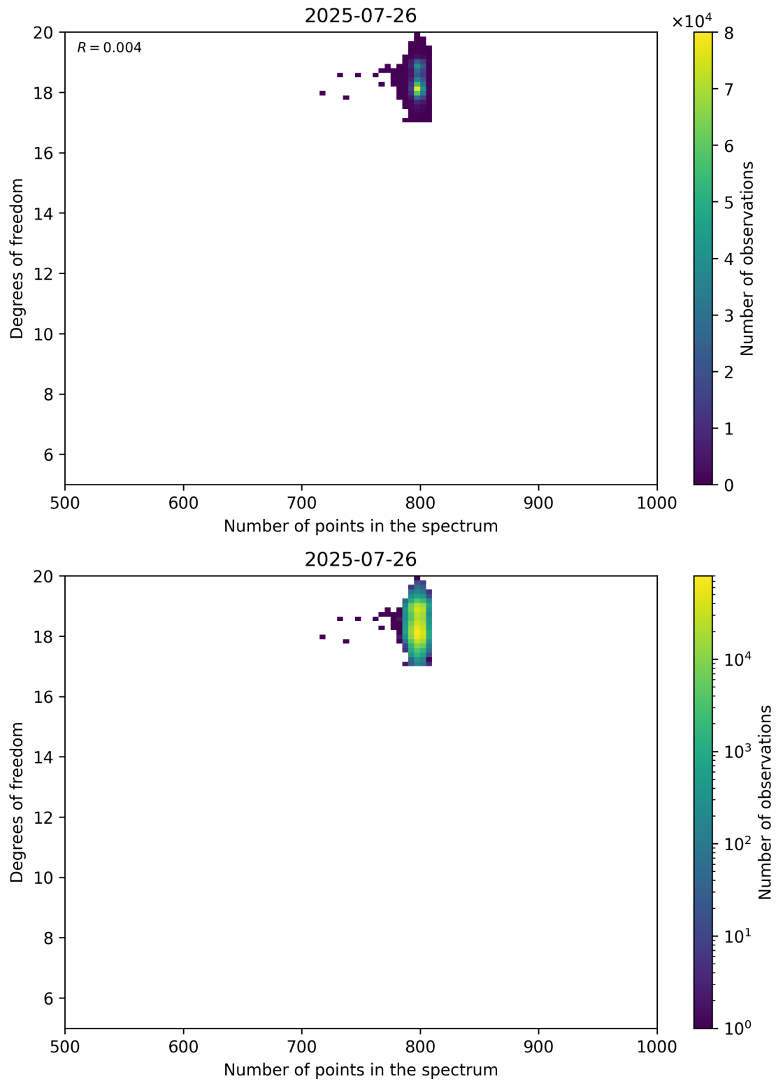
Figure 90: Scatter density plot of “Number of points in the spectrum” against “Degrees of freedom” for 2025-07-25 to 2025-07-27.
