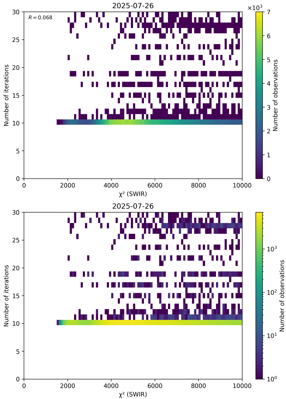
Figure 50: Scatter density plot of “ \chi^2 (SWIR)” against “Number of iterations” for 2025-07-25 to 2025-07-27.
