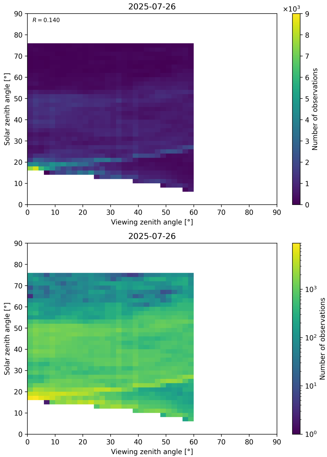
Figure 115: Scatter density plot of “Viewing zenith angle” against “Solar zenith angle” for 2025-07-25 to 2025-07-27.
