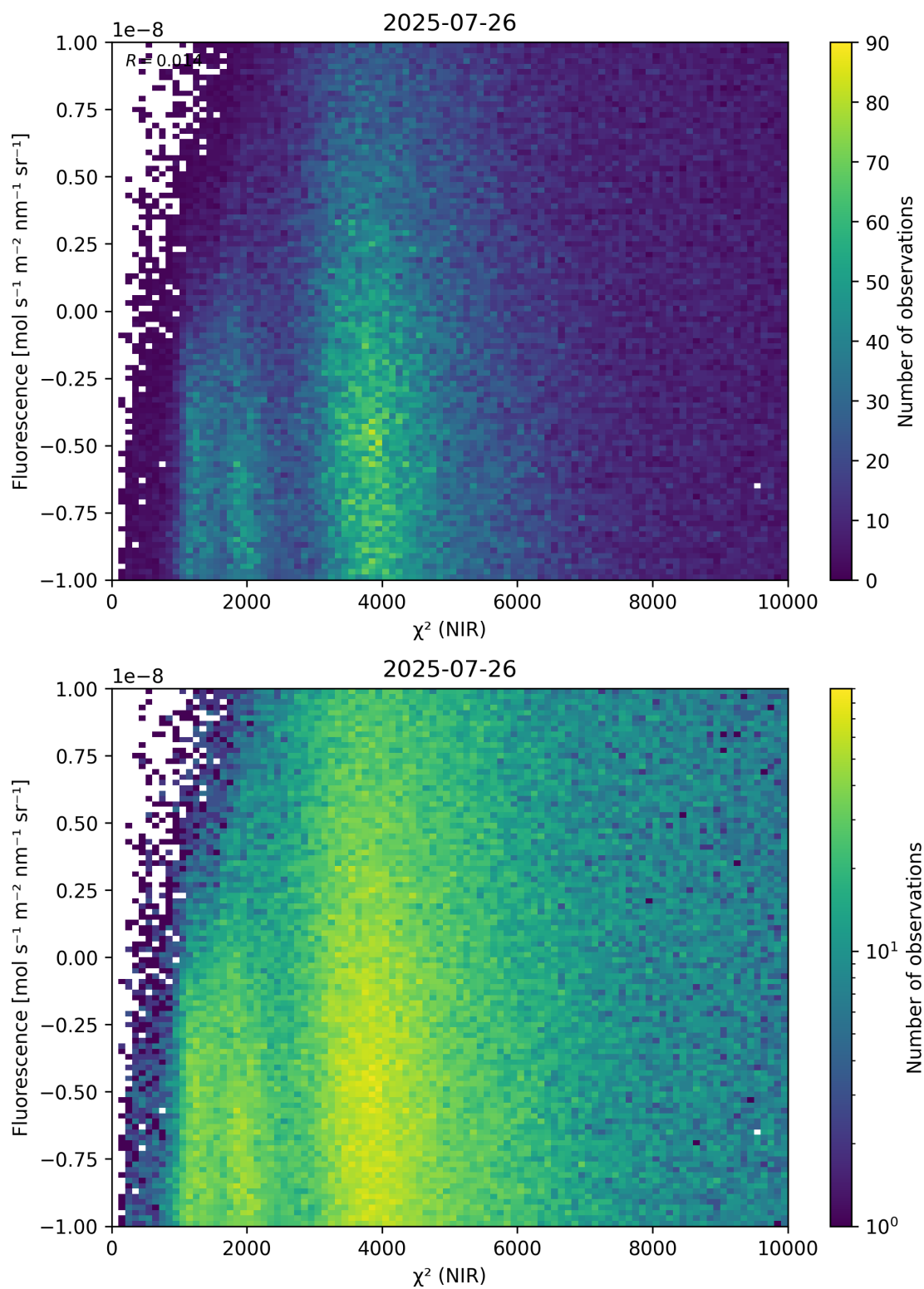
Figure 45: Scatter density plot of “ \chi^2 (NIR)” against “Fluorescence” for 2025-07-25 to 2025-07-27.
