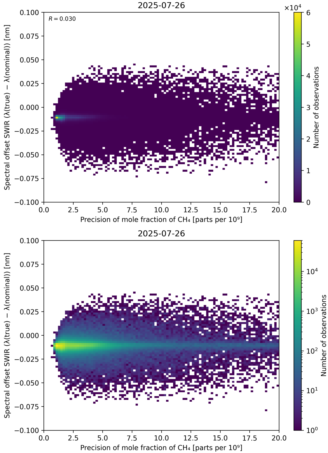
Figure 85: Scatter density plot of “Precision of mole fraction of CH 4 ” against “Spectral offset SWIR ( \lambda_{\text{true}} - \lambda_{\text{nominal}} )” for 2025-07-25 to 2025-07-27.
