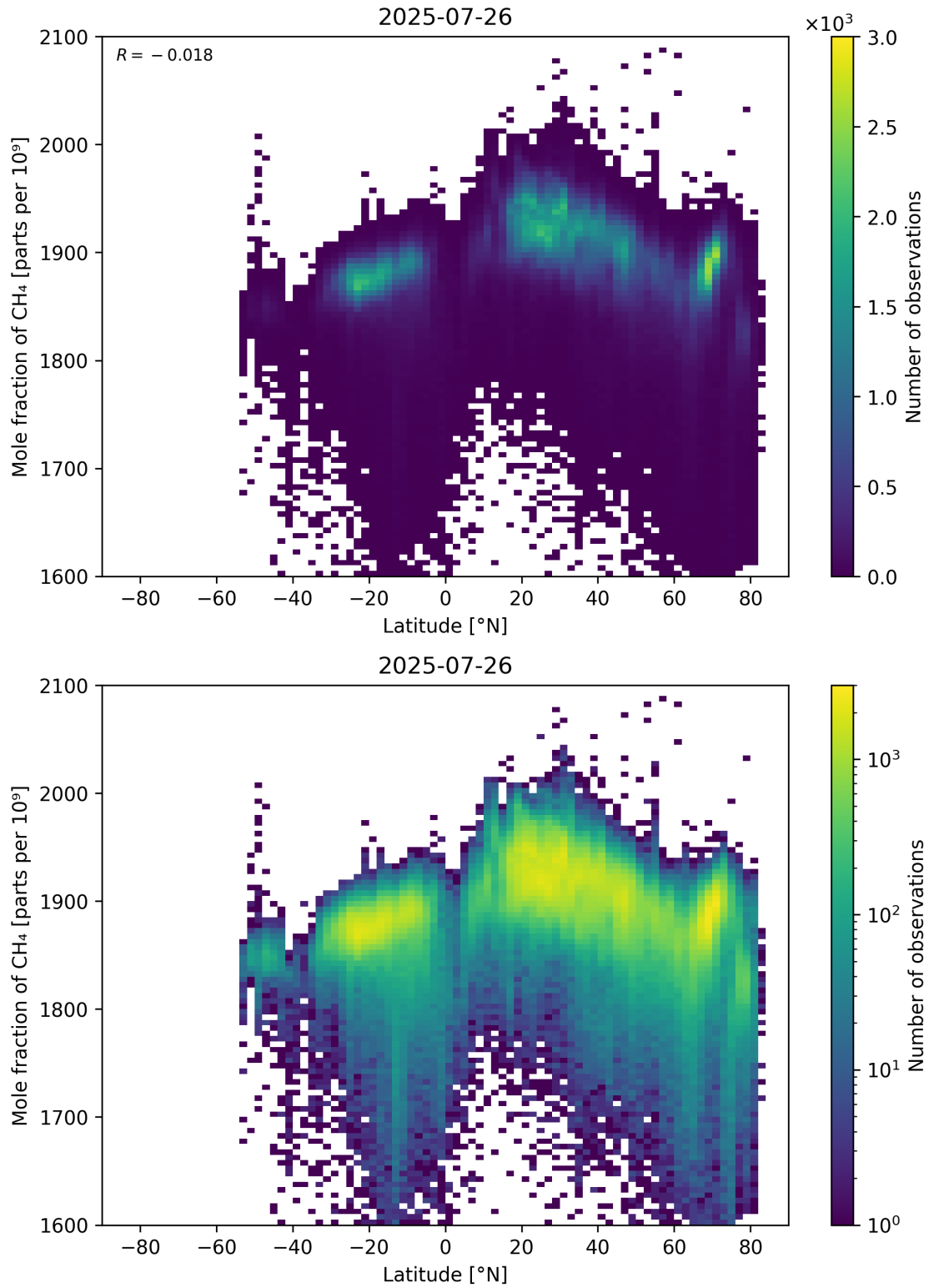
Figure 57: Scatter density plot of “Latitude” against “Mole fraction of CH 4 ” for 2025-07-25 to 2025-07-27.
