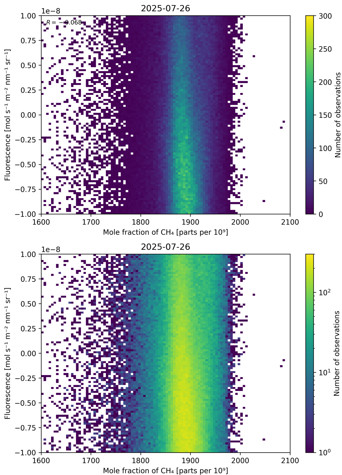
Figure 73: Scatter density plot of “Mole fraction of \text{CH}_4 ” against “Fluorescence” for 2025-07-25 to 2025-07-27.
