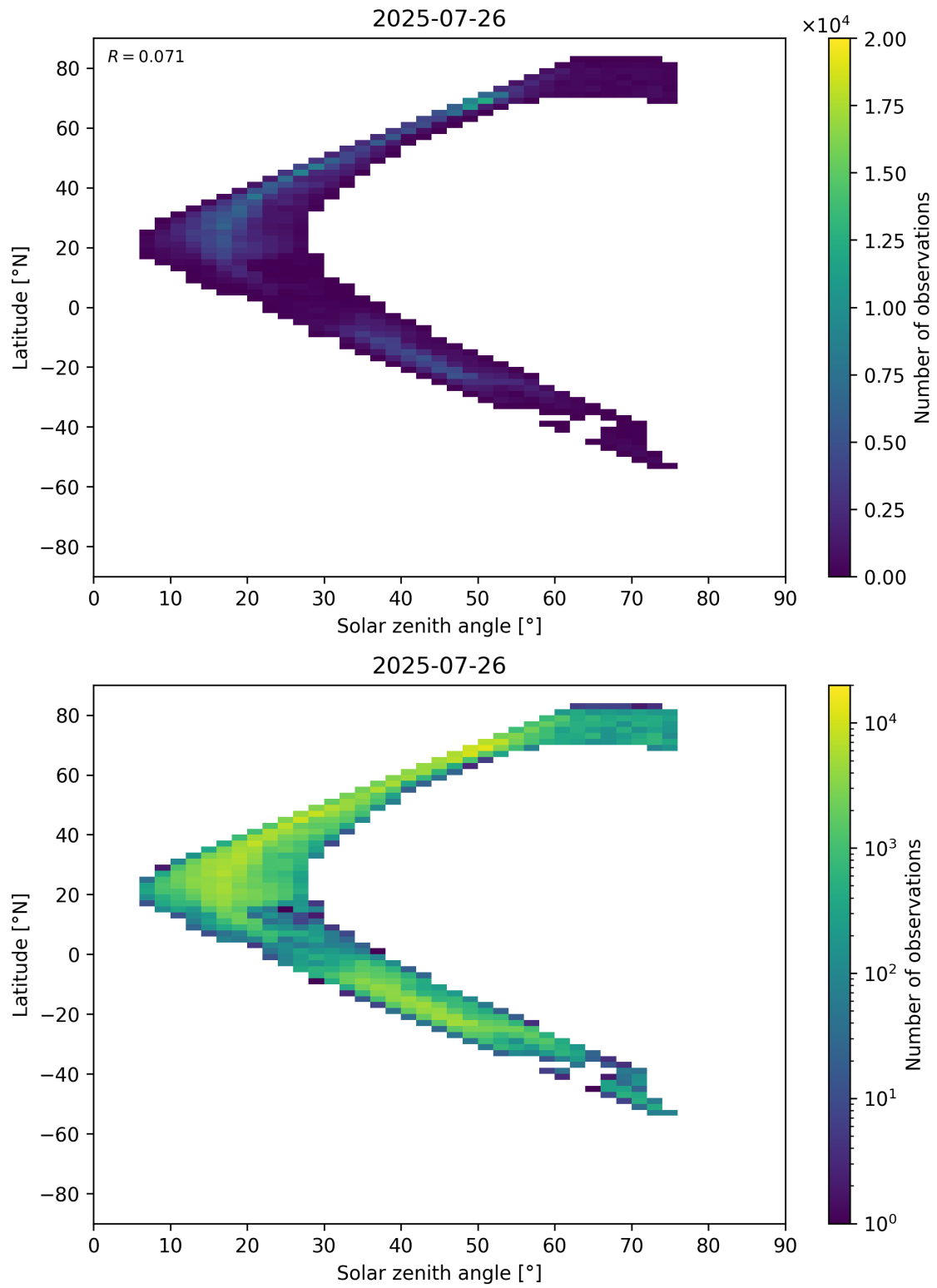
Figure 98: Scatter density plot of “Solar zenith angle” against “Latitude” for 2025-07-25 to 2025-07-27.
