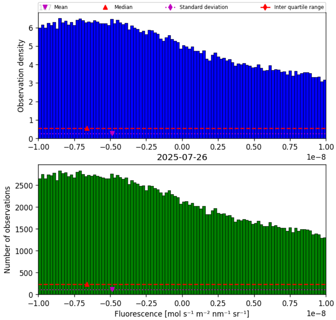
Figure 32: Histogram of “Fluorescence” for 2025-07-25 to 2025-07-27
