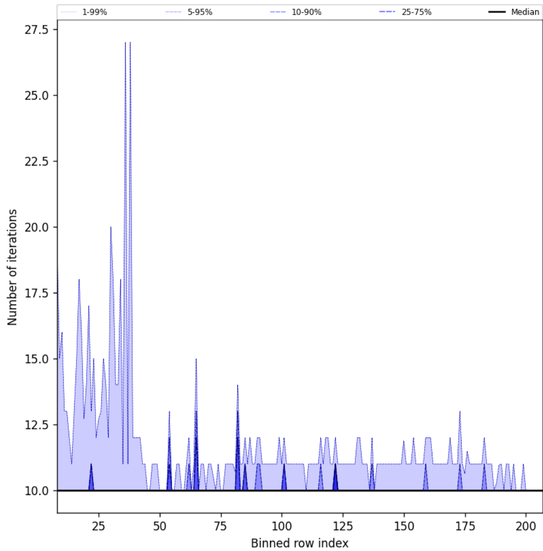
Figure 42: Along track statistics of “Number of iterations” for 2025-07-25 to 2025-07-27
