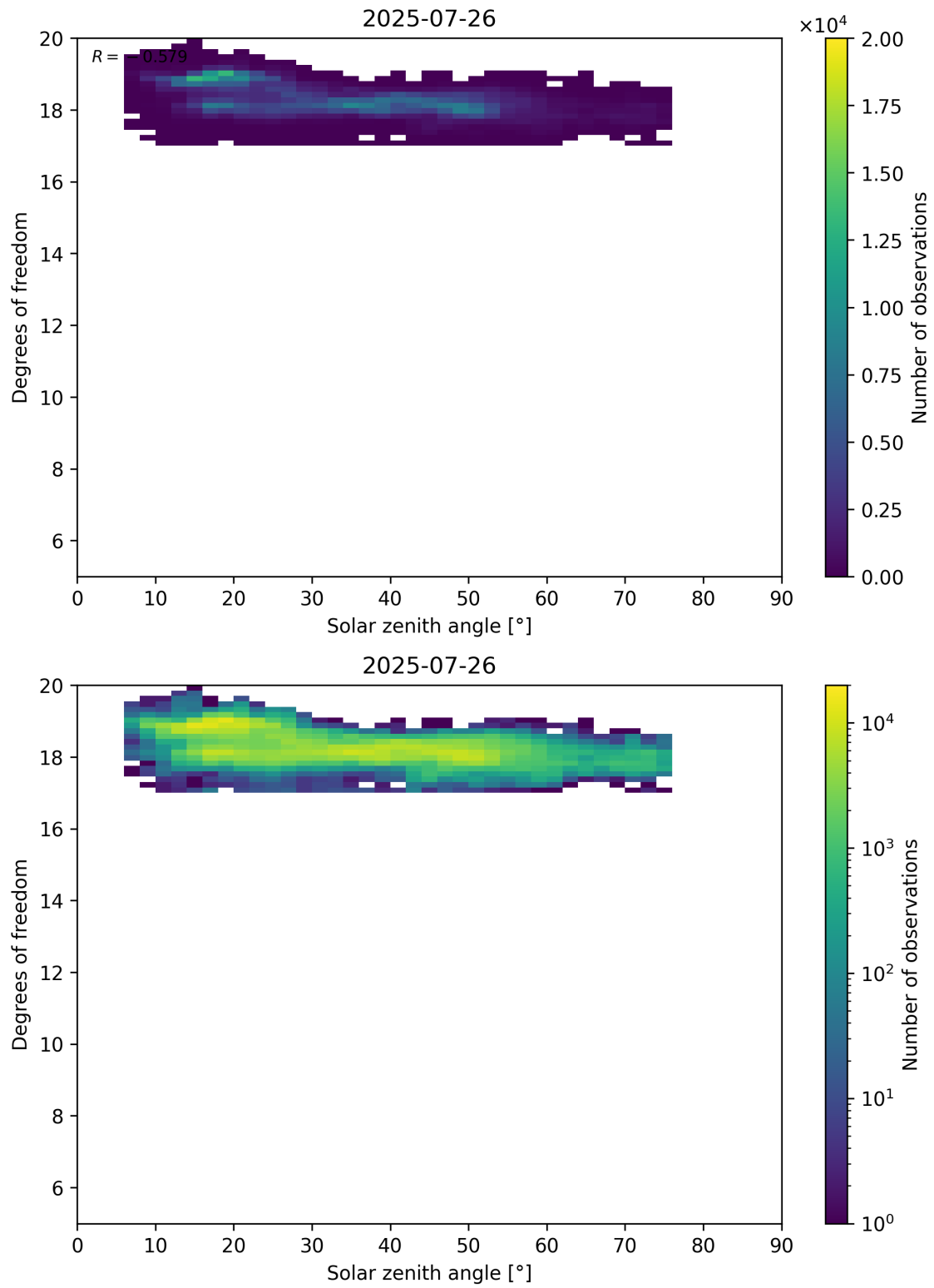
Figure 96: Scatter density plot of “Solar zenith angle” against “Degrees of freedom” for 2025-07-25 to 2025-07-27.
