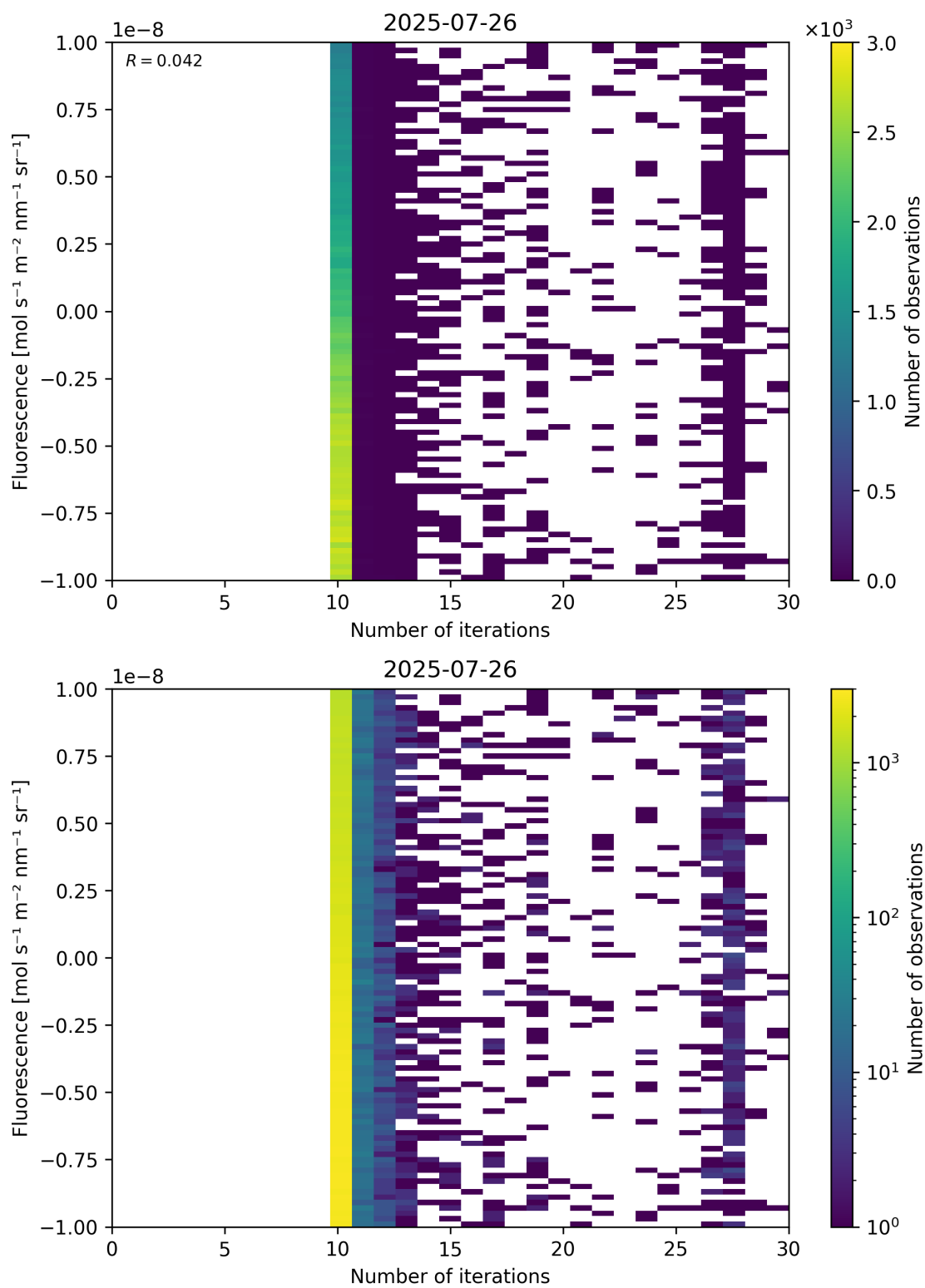
Figure 87: Scatter density plot of "Number of iterations" against "Fluorescence" for 2025-07-25 to 2025-07-27.
