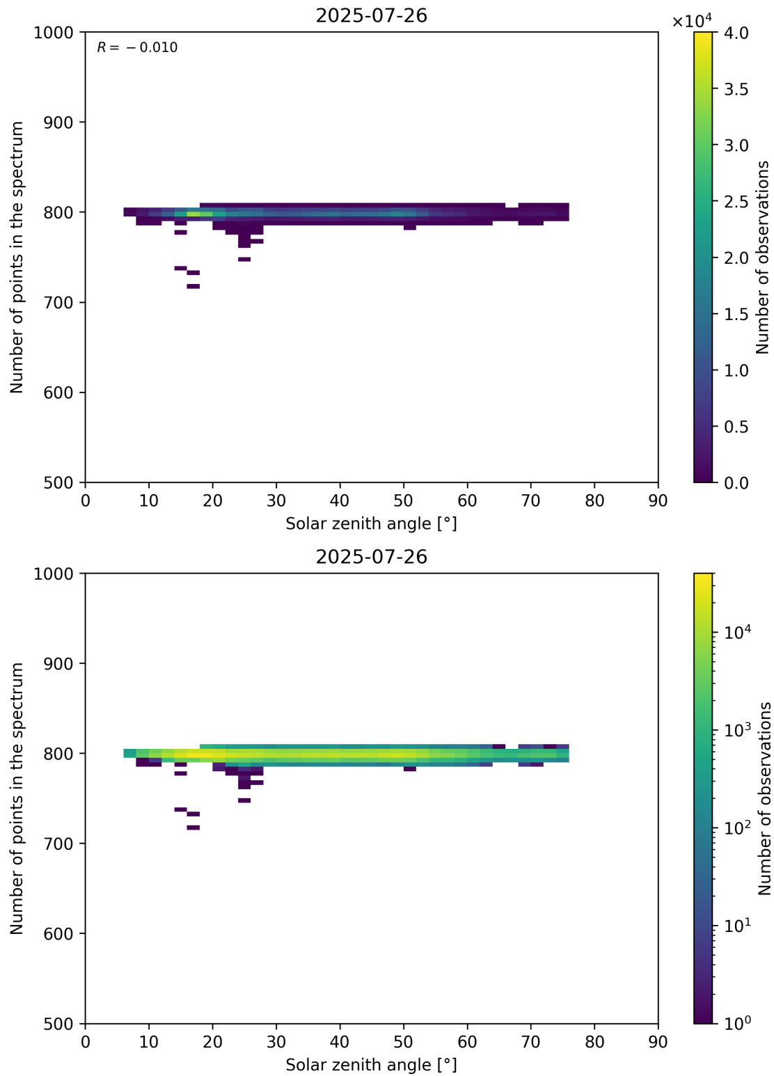
Figure 103: Scatter density plot of “Solar zenith angle” against “Number of points in the spectrum” for 2025-07-25 to 2025-07-27.
