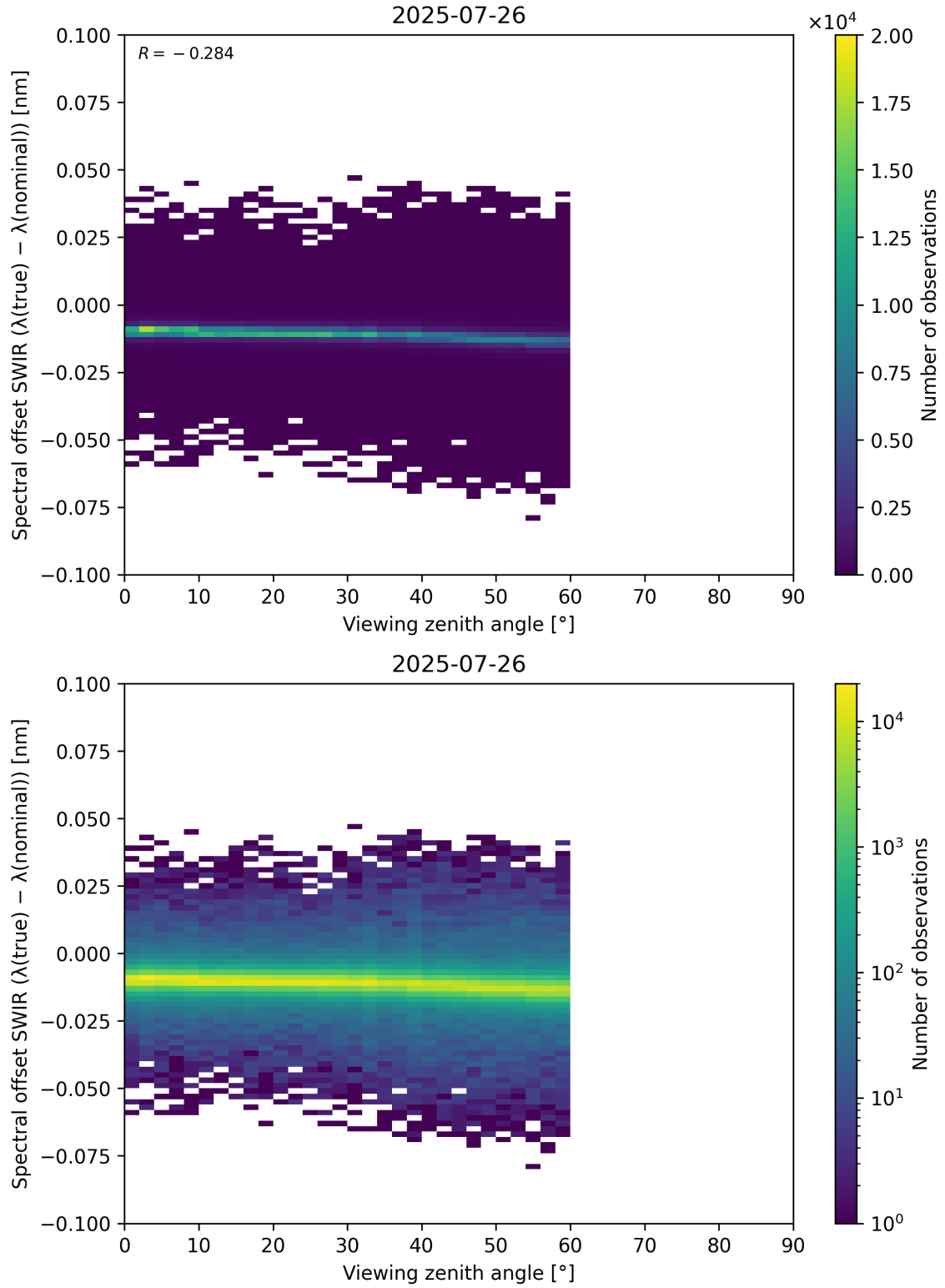
Figure 116: Scatter density plot of “Viewing zenith angle” against “Spectral offset SWIR ( \lambda_{\text{true}} - \lambda_{\text{nominal}} )” for 2025-07-25 to 2025-07-27.
