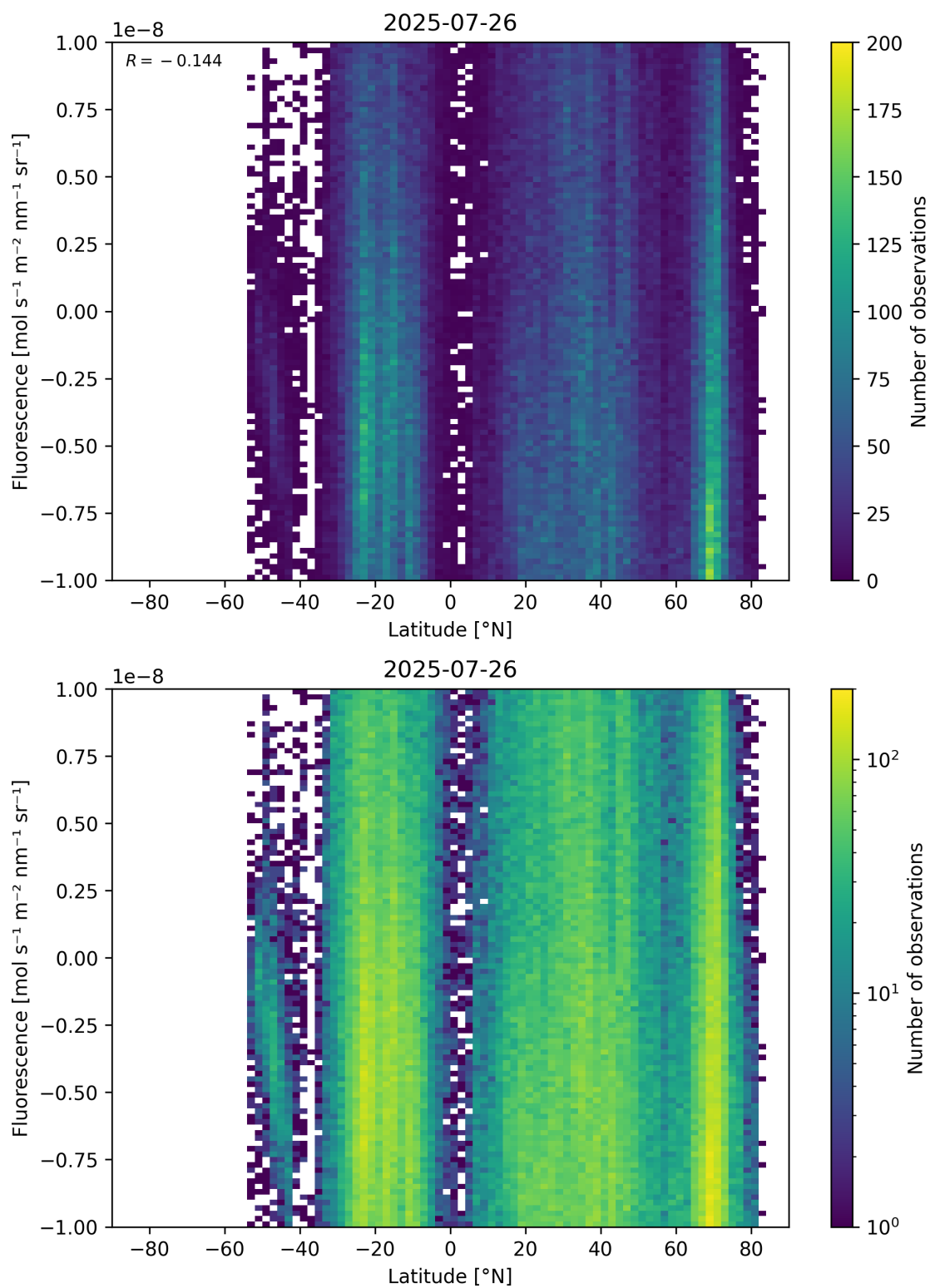
Figure 56: Scatter density plot of “Latitude” against “Fluorescence” for 2025-07-25 to 2025-07-27.
