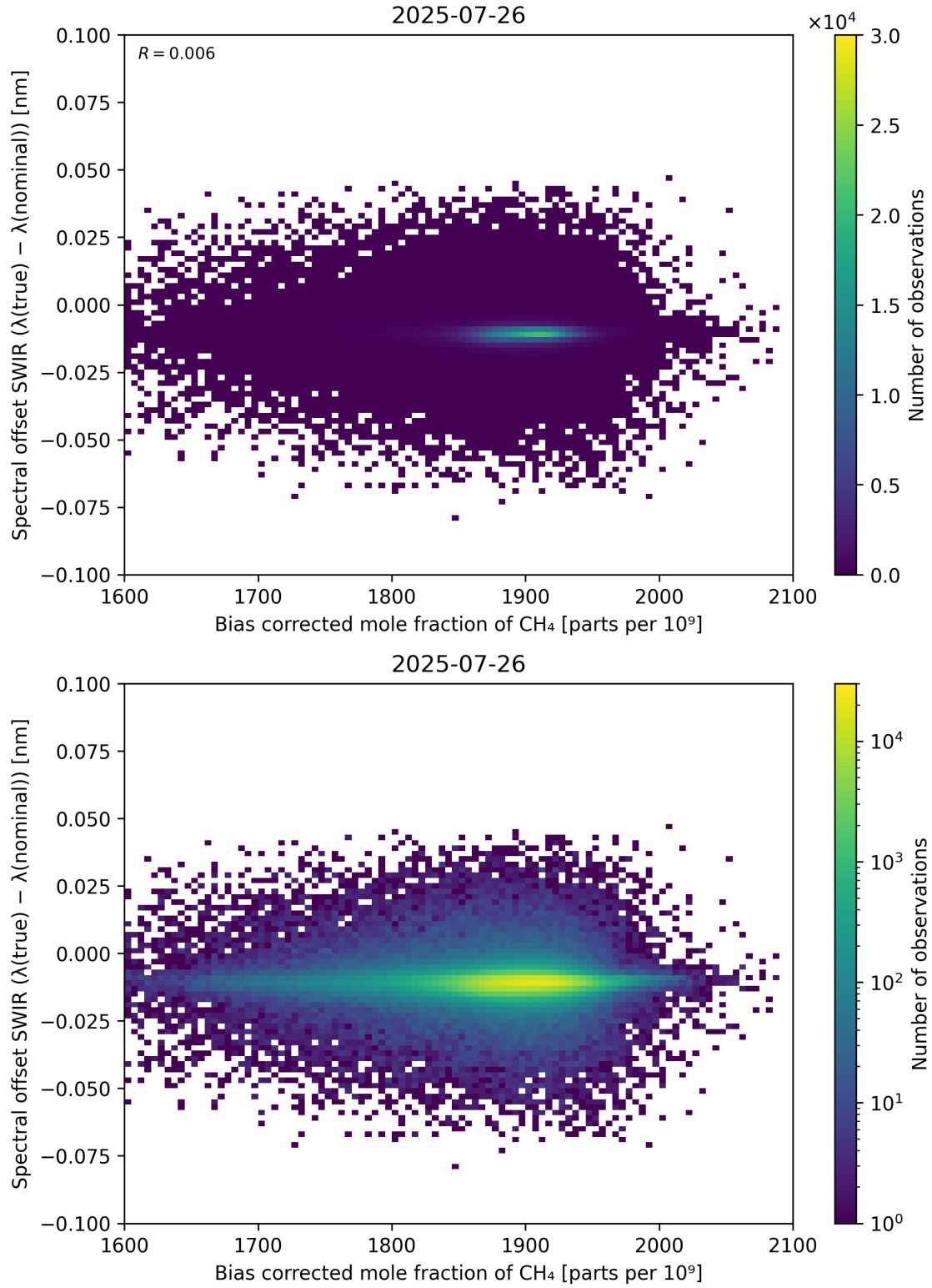
Figure 69: Scatter density plot of “Bias corrected mole fraction of CH 4 ” against “Spectral offset SWIR ( \lambda_{\text{true}} - \lambda_{\text{nominal}} )” for 2025-07-25 to 2025-07-27.
