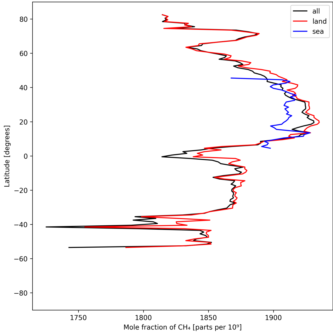
Figure 12: Zonal average of “Mole fraction of \text{CH}_4 ” for 2025-07-25 to 2025-07-27.
