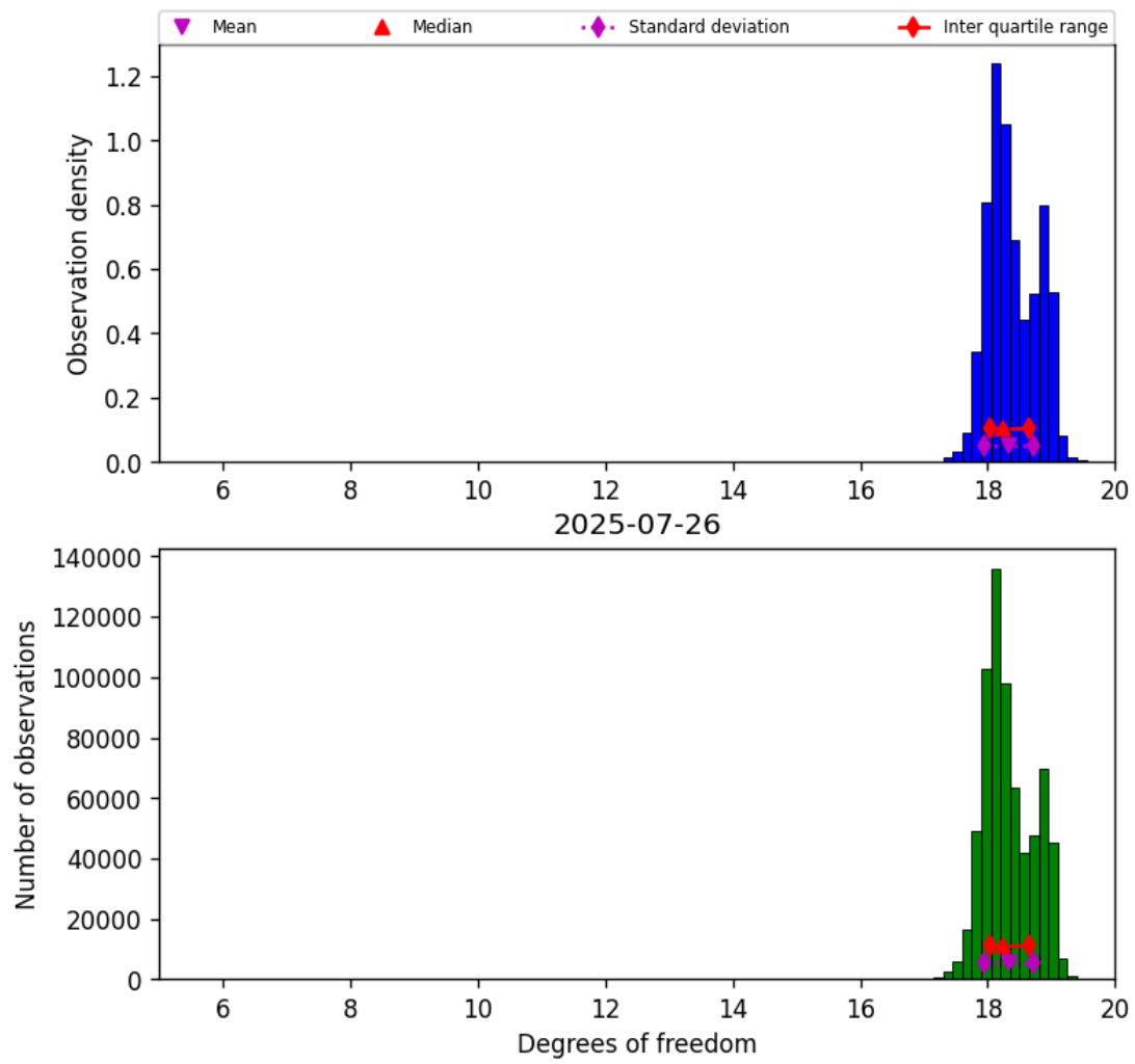
Figure 30: Histogram of “Degrees of freedom” for 2025-07-25 to 2025-07-27
