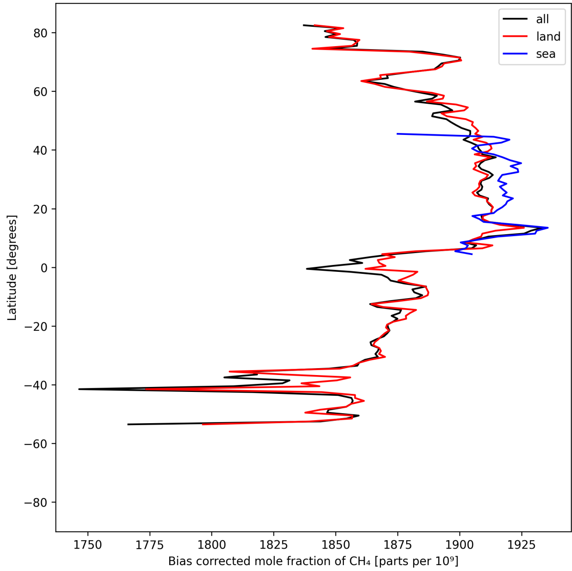
Figure 14: Zonal average of “Bias corrected mole fraction of CH 4 ” for 2025-07-25 to 2025-07-27.
