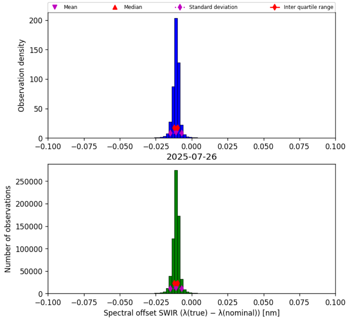
Figure 27: Histogram of “Spectral offset SWIR ( \lambda_{\text{true}} - \lambda_{\text{nominal}} )” for 2025-07-25 to 2025-07-27
