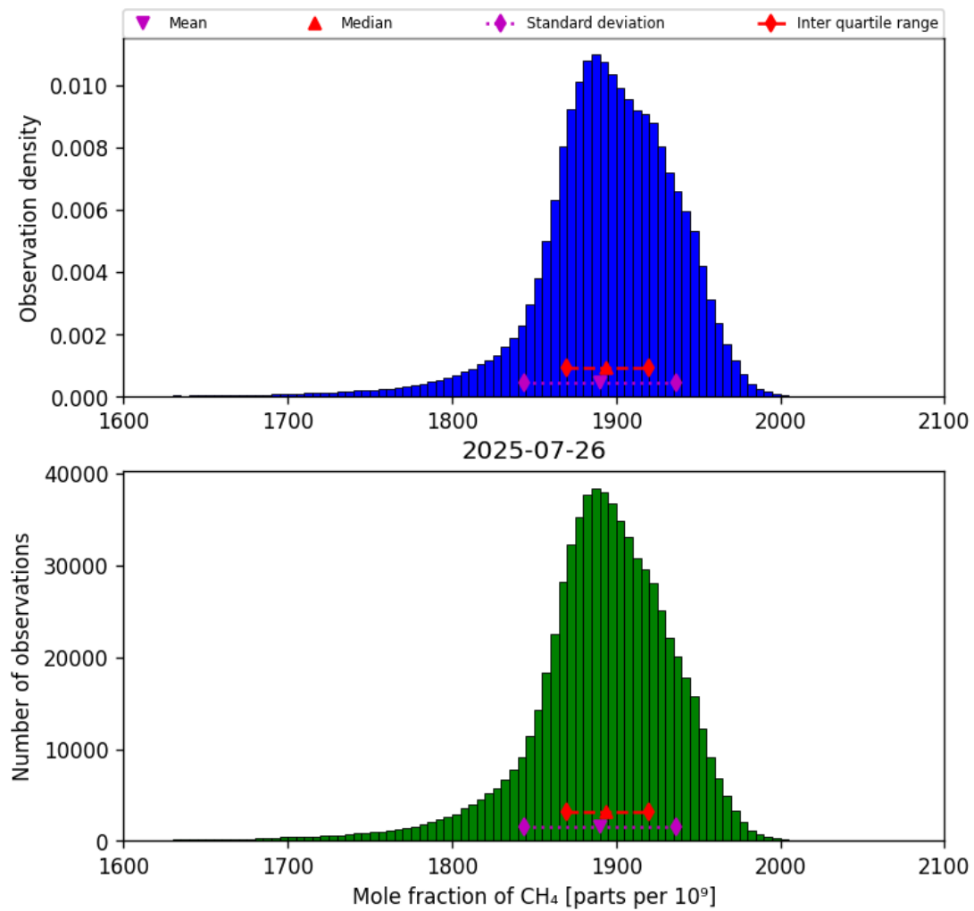
Figure 23: Histogram of “Mole fraction of CH 4 ” for 2025-07-25 to 2025-07-27
