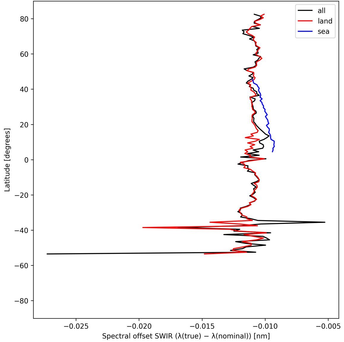
Figure 16: Zonal average of “Spectral offset SWIR ( \lambda_{\text{true}} - \lambda_{\text{nominal}} )” for 2025-07-25 to 2025-07-27.
