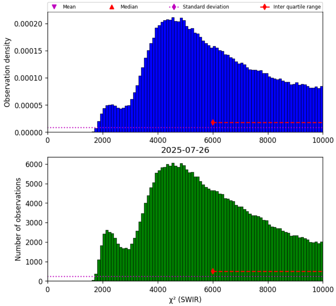
Figure 28: Histogram of “ \chi^2 (SWIR)” for 2025-07-25 to 2025-07-27
