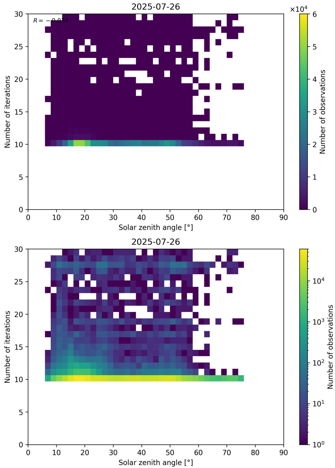
Figure 102: Scatter density plot of “Solar zenith angle” against “Number of iterations” for 2025-07-25 to 2025-07-27.
