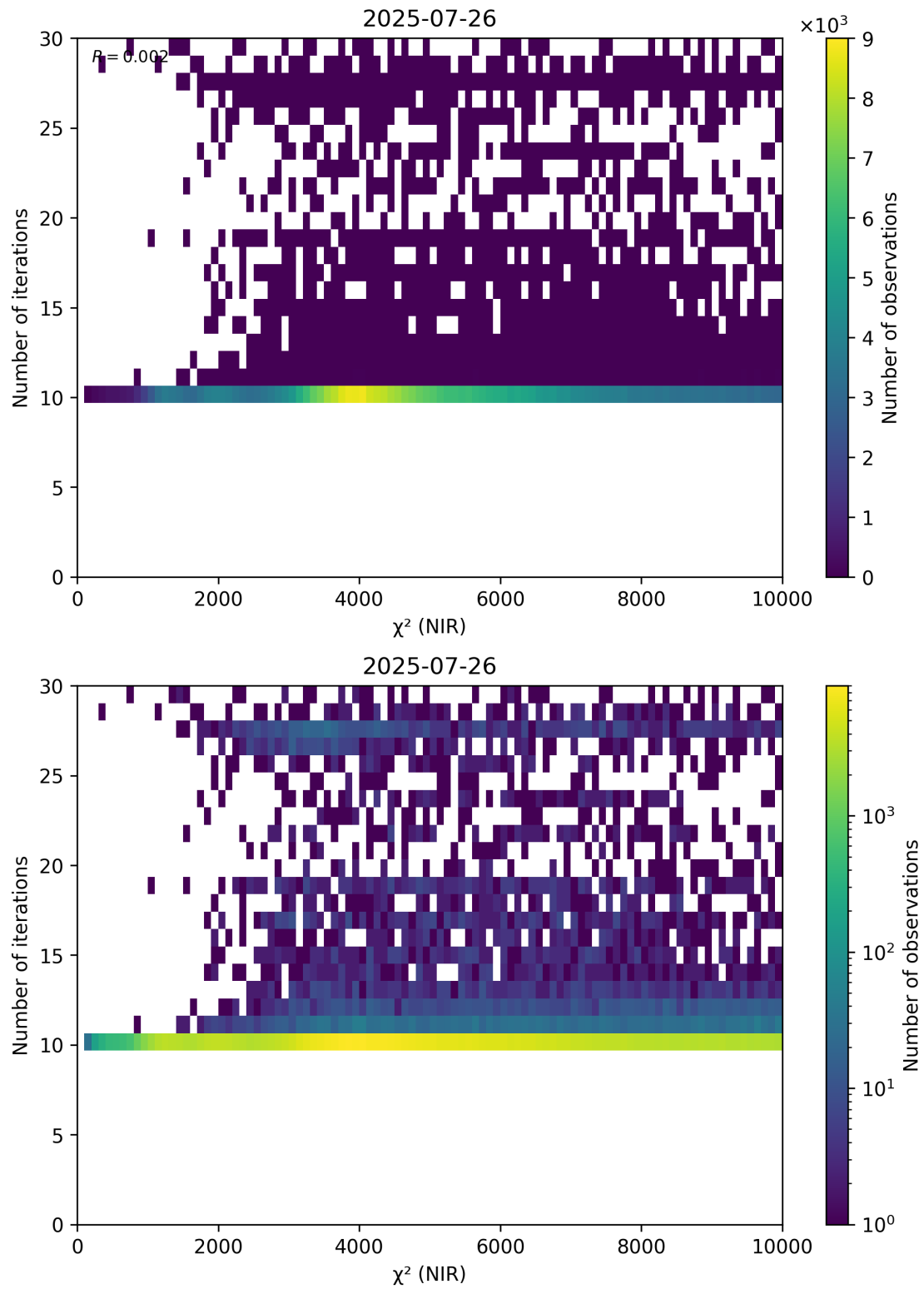
Figure 46: Scatter density plot of “ \chi^2 (NIR)” against “Number of iterations” for 2025-07-25 to 2025-07-27.
