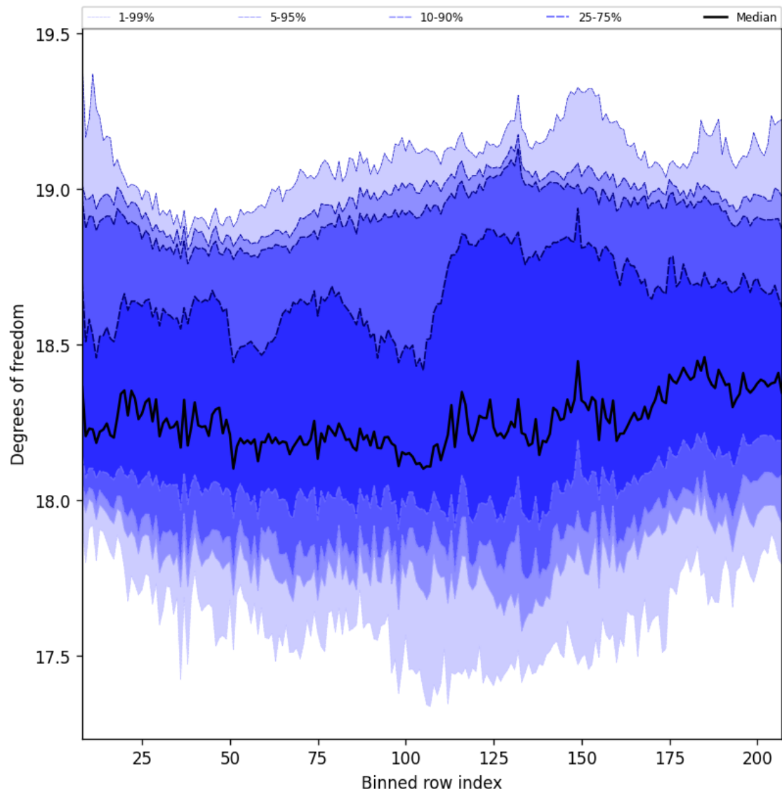
Figure 41: Along track statistics of “Degrees of freedom” for 2025-07-25 to 2025-07-27
