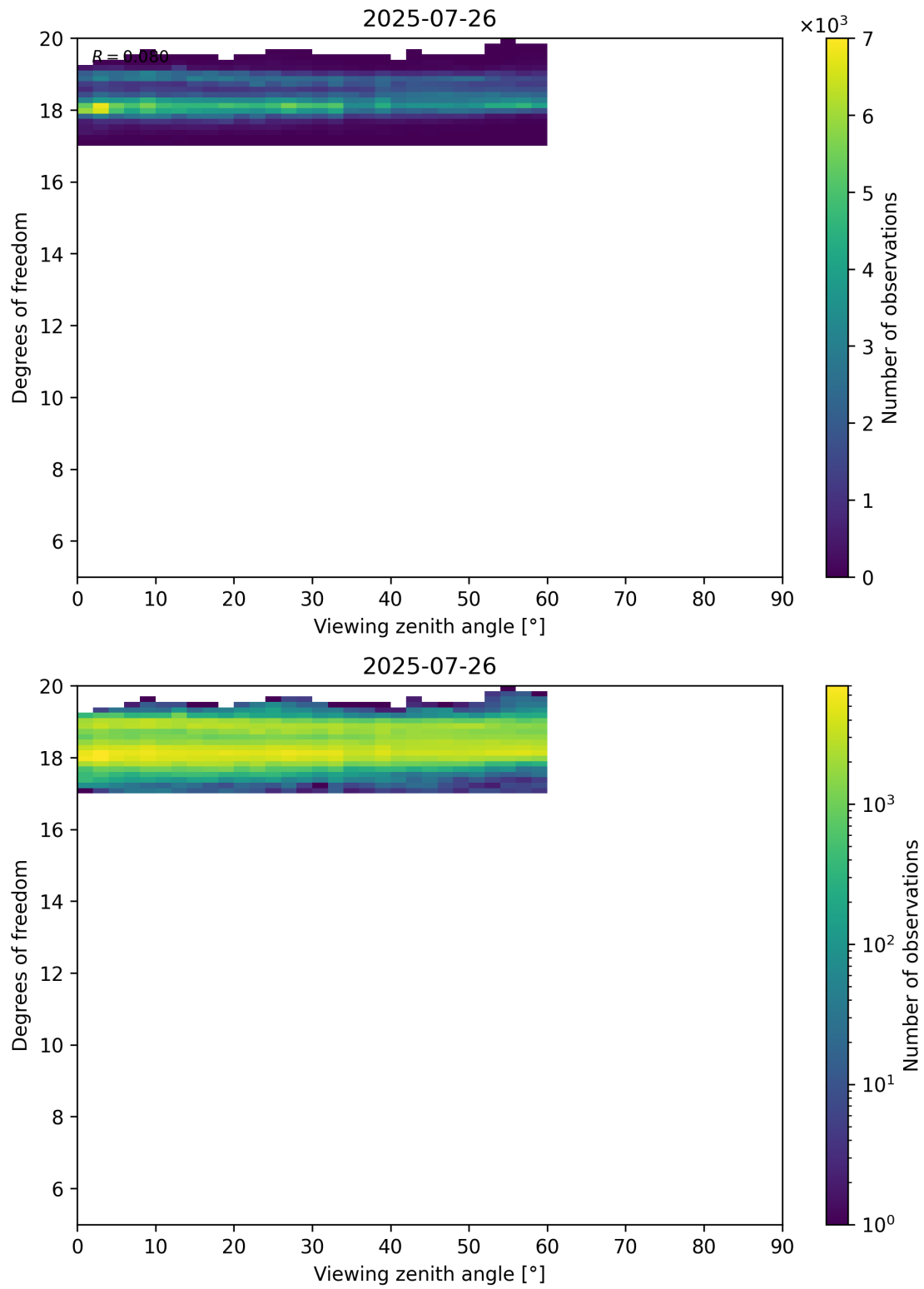
Figure 107: Scatter density plot of “Viewing zenith angle” against “Degrees of freedom” for 2025-07-25 to 2025-07-27.
