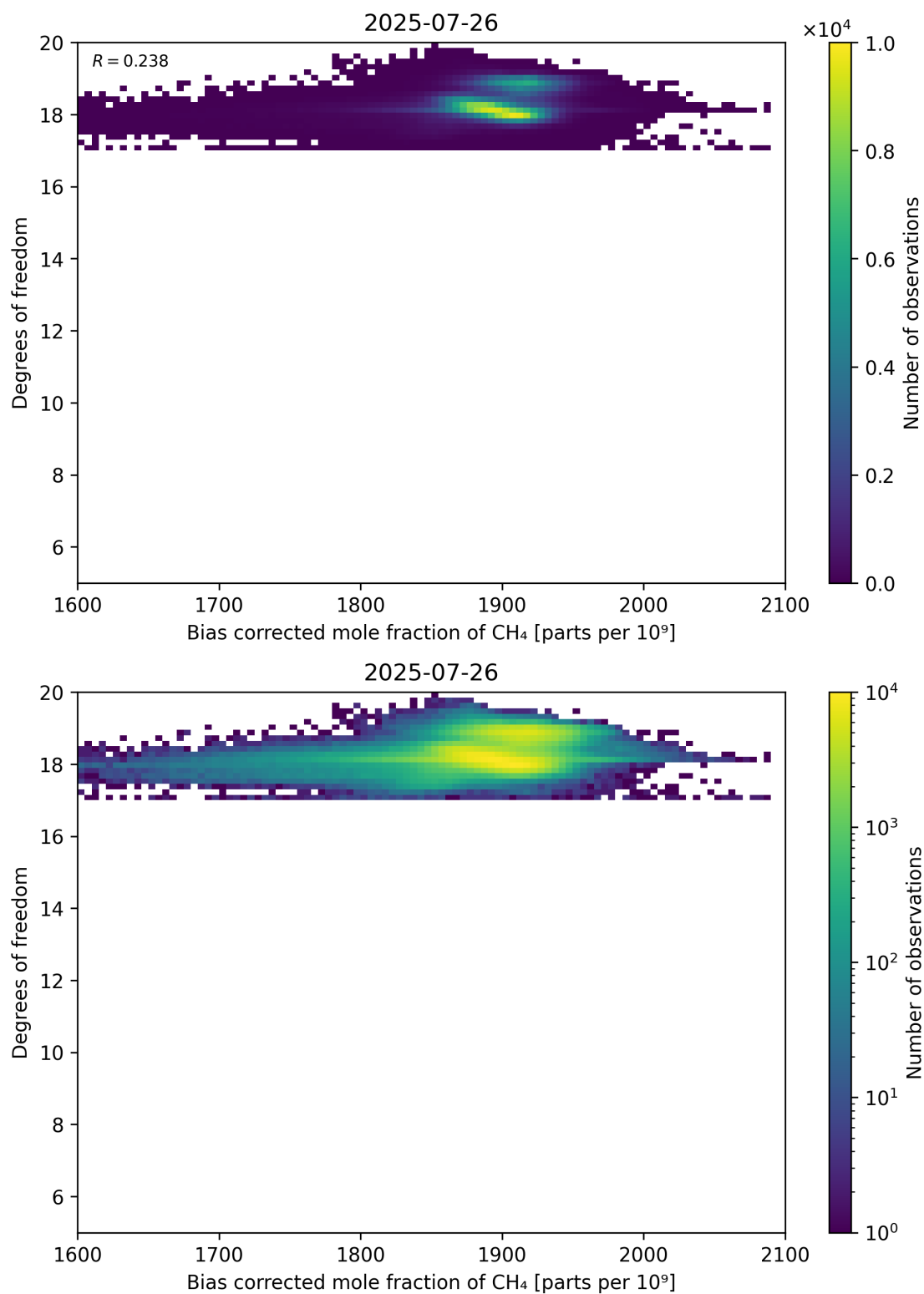
Figure 65: Scatter density plot of “Bias corrected mole fraction of CH 4 ” against “Degrees of freedom” for 2025-07-25 to 2025-07-27.
