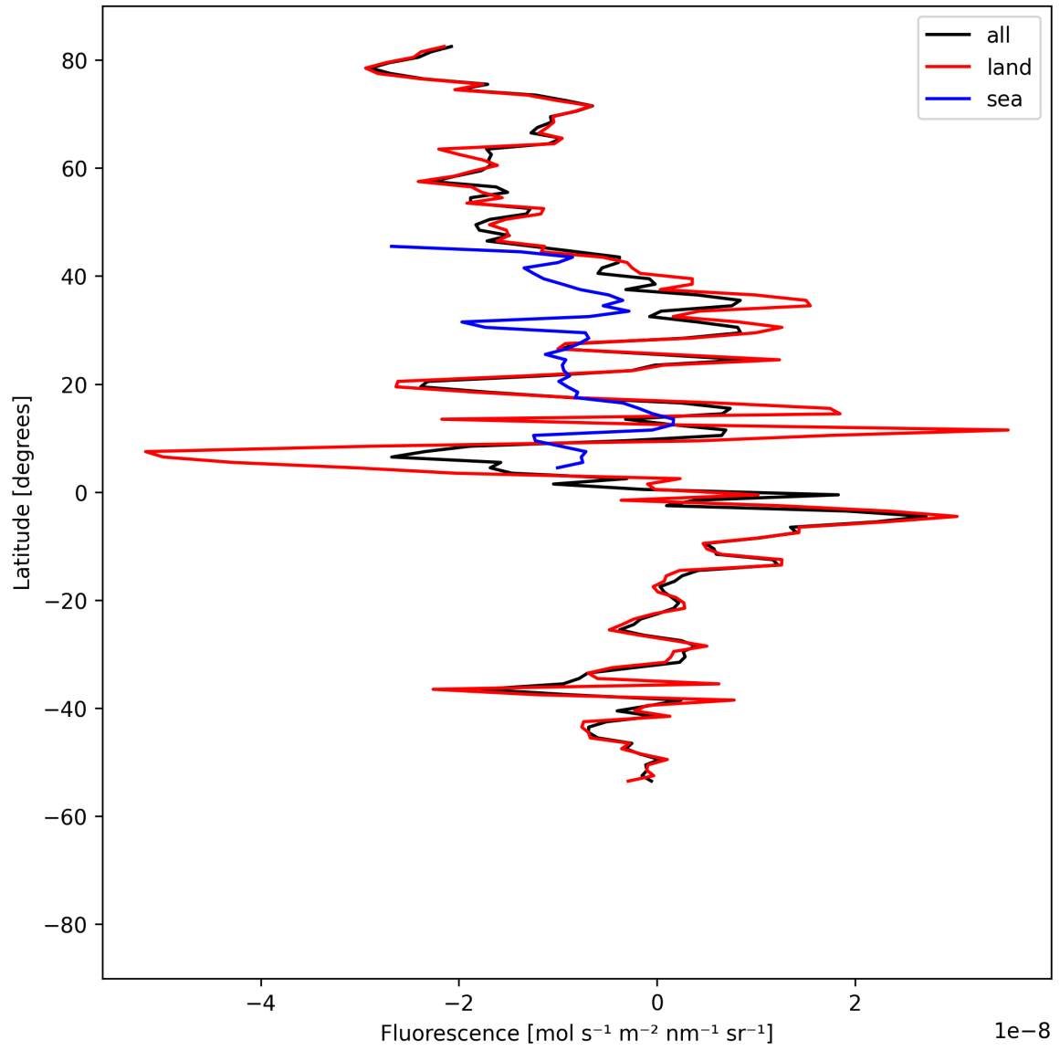
Figure 21: Zonal average of “Fluorescence” for 2025-07-25 to 2025-07-27.
