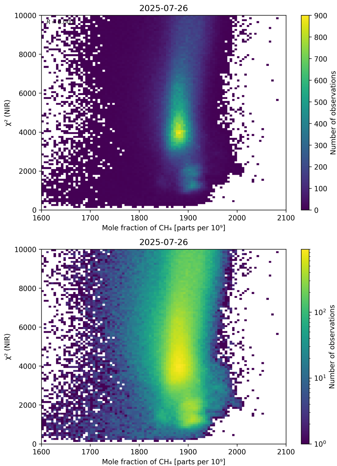
Figure 70: Scatter density plot of “Mole fraction of CH 4 ” against “ \chi^2 (NIR)” for 2025-07-25 to 2025-07-27.
