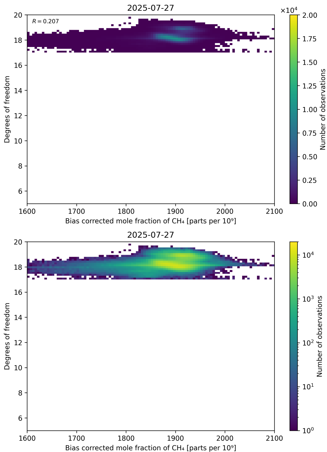
Figure 65: Scatter density plot of “Bias corrected mole fraction of CH 4 ” against “Degrees of freedom” for 2025-07-26 to 2025-07-28.
