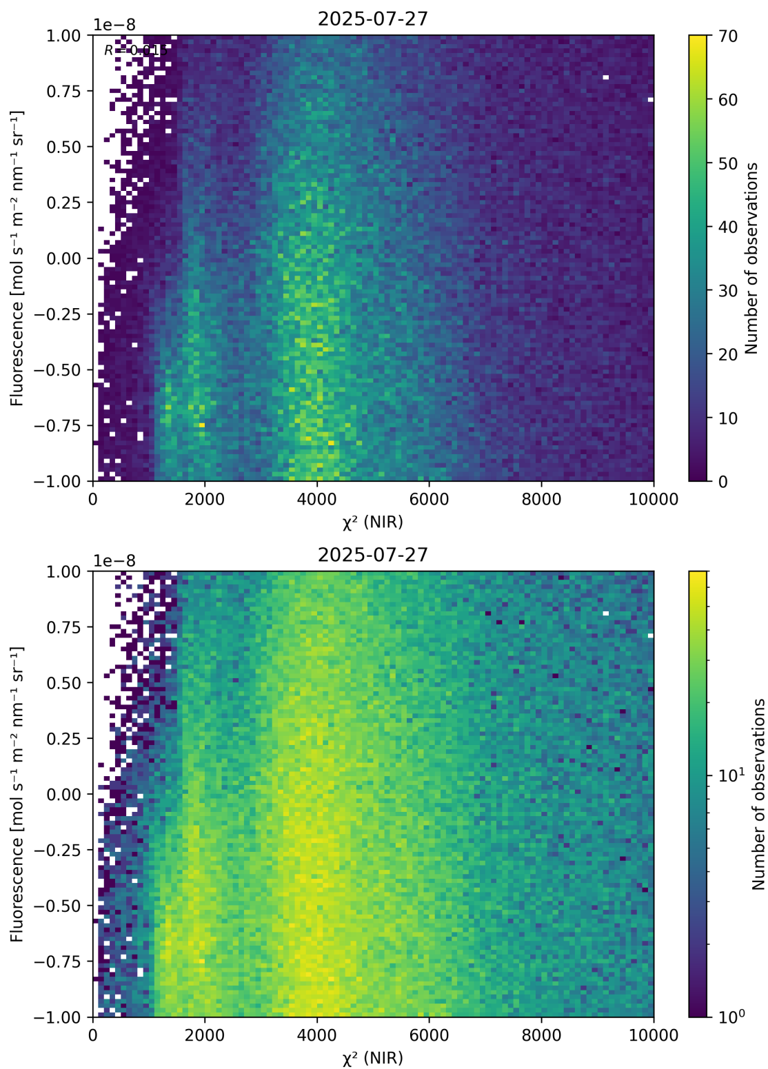
Figure 45: Scatter density plot of “ \chi^2 (NIR)” against “Fluorescence” for 2025-07-26 to 2025-07-28.
