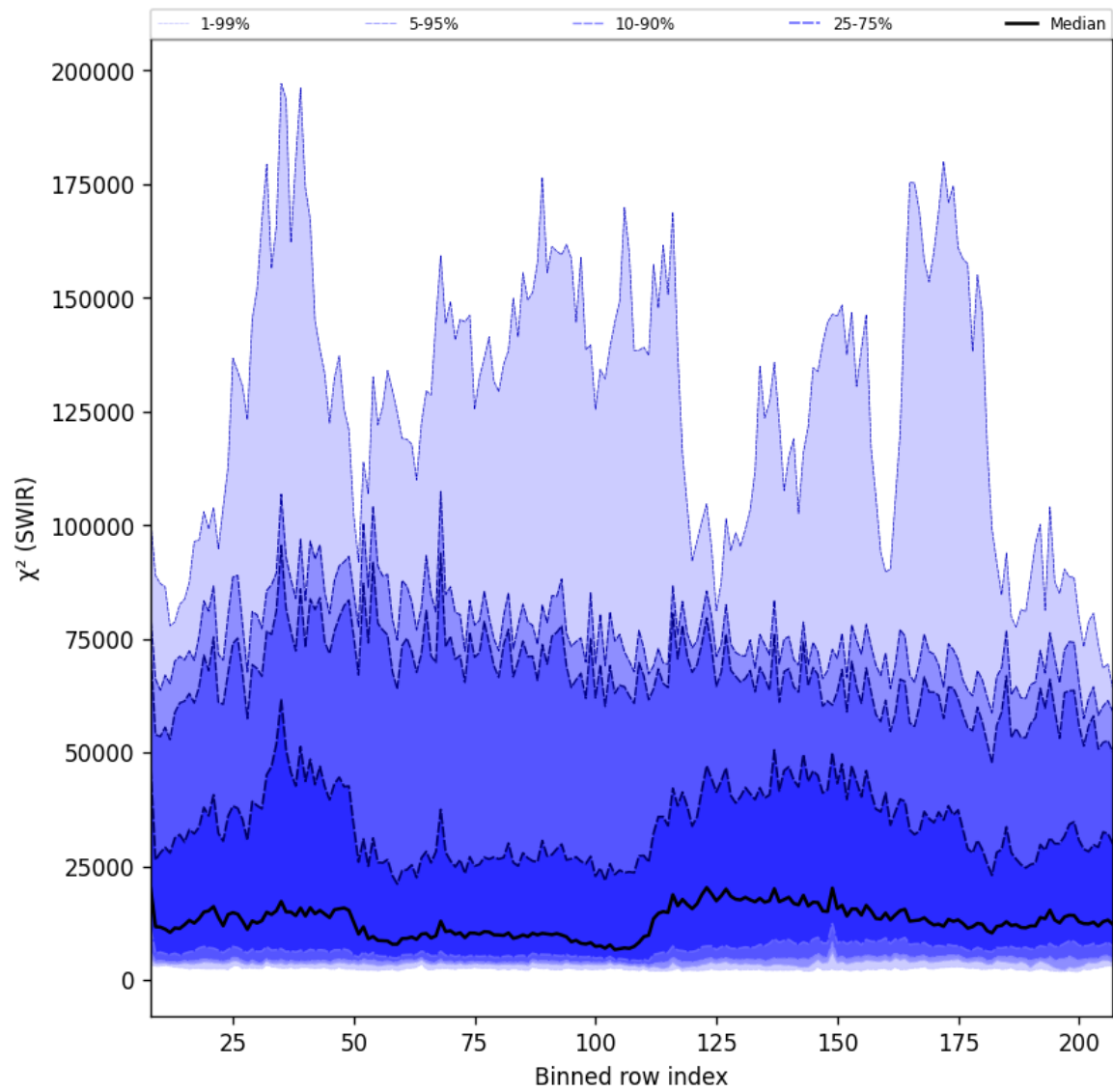
Figure 39: Along track statistics of “ \chi^2 (SWIR)” for 2025-07-26 to 2025-07-28
