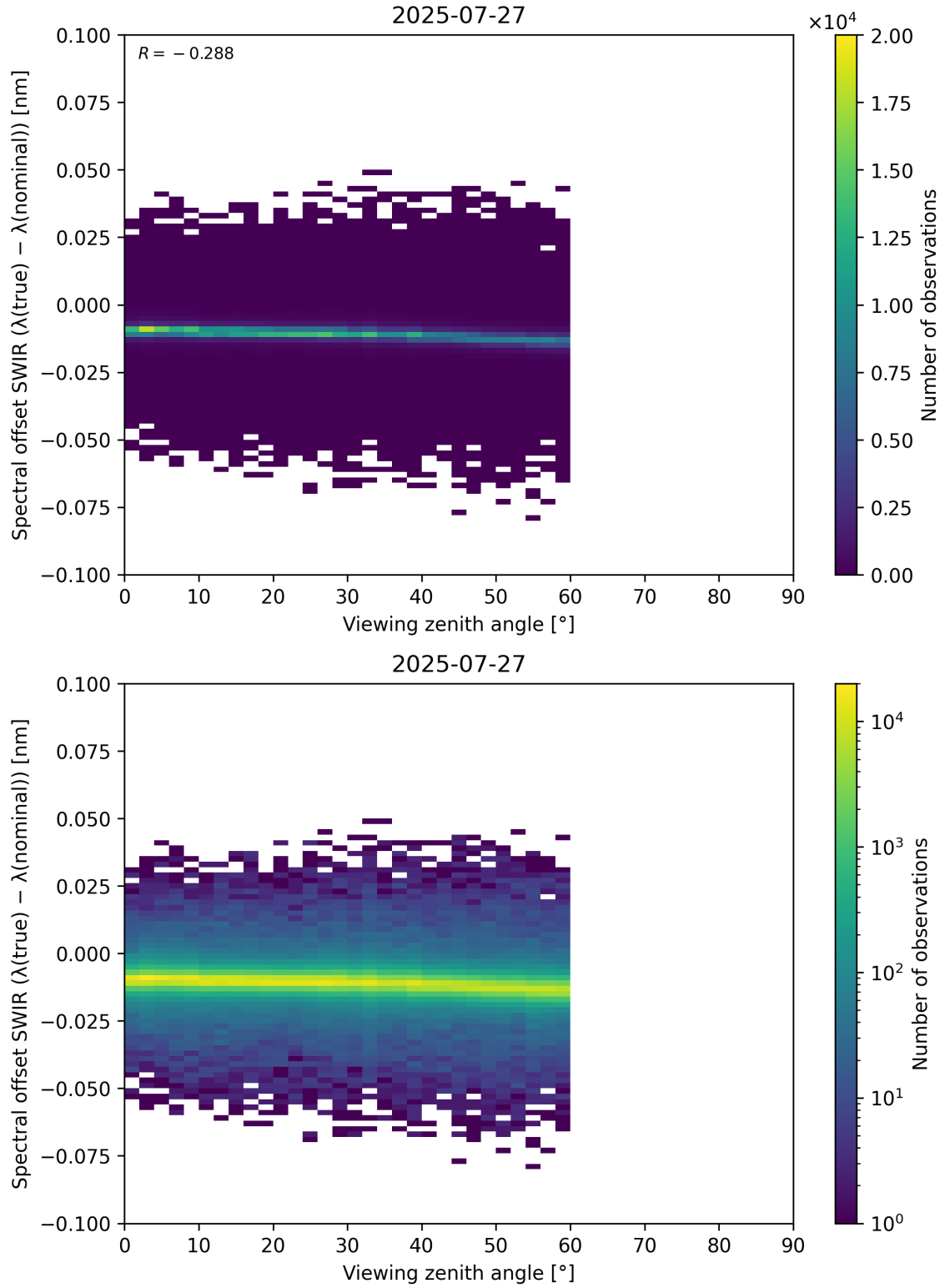
Figure 116: Scatter density plot of “Viewing zenith angle” against “Spectral offset SWIR ( \lambda_{\text{true}} - \lambda_{\text{nominal}} )” for 2025-07-26 to 2025-07-28.
