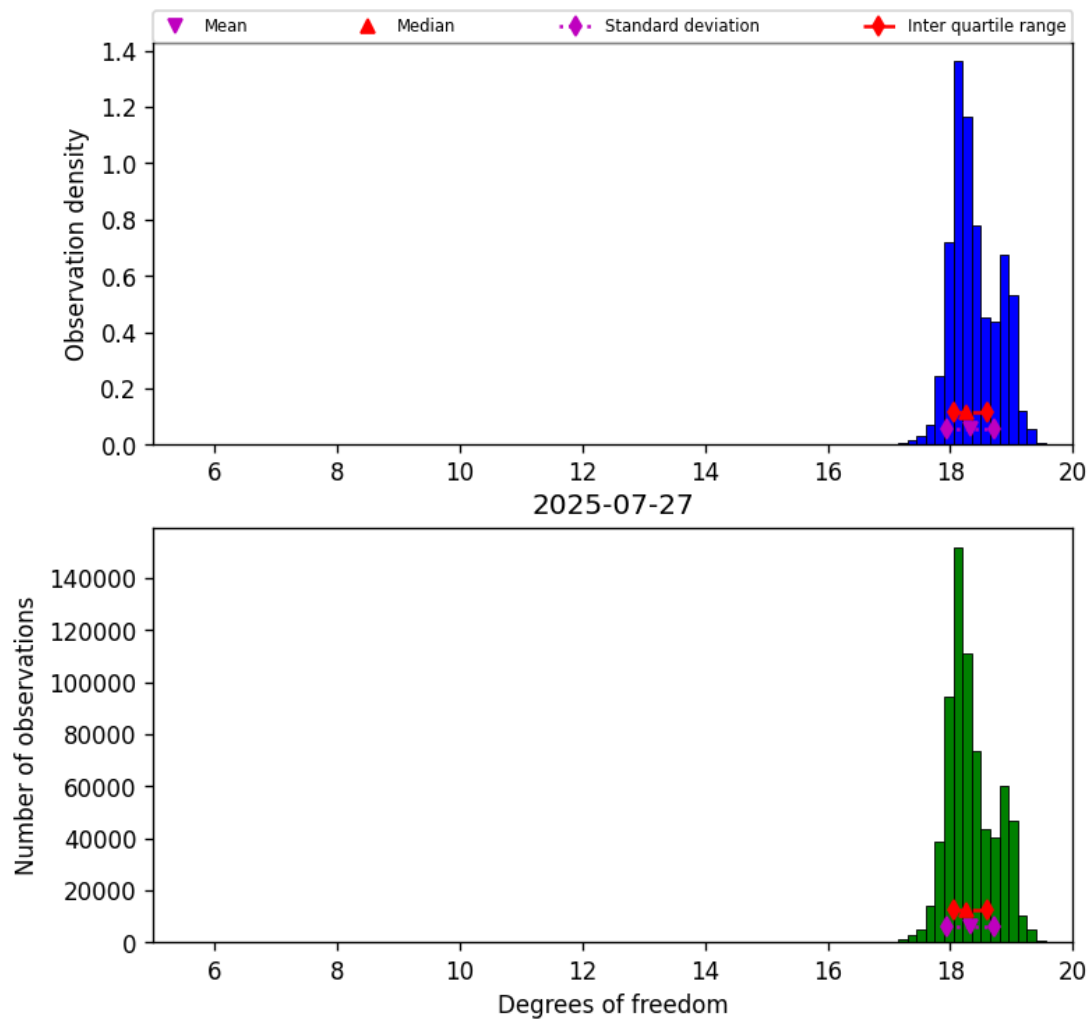
Figure 30: Histogram of “Degrees of freedom” for 2025-07-26 to 2025-07-28
