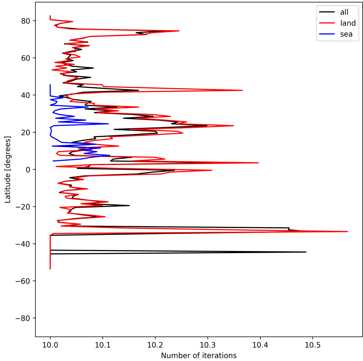
Figure 20: Zonal average of “Number of iterations” for 2025-07-26 to 2025-07-28.
