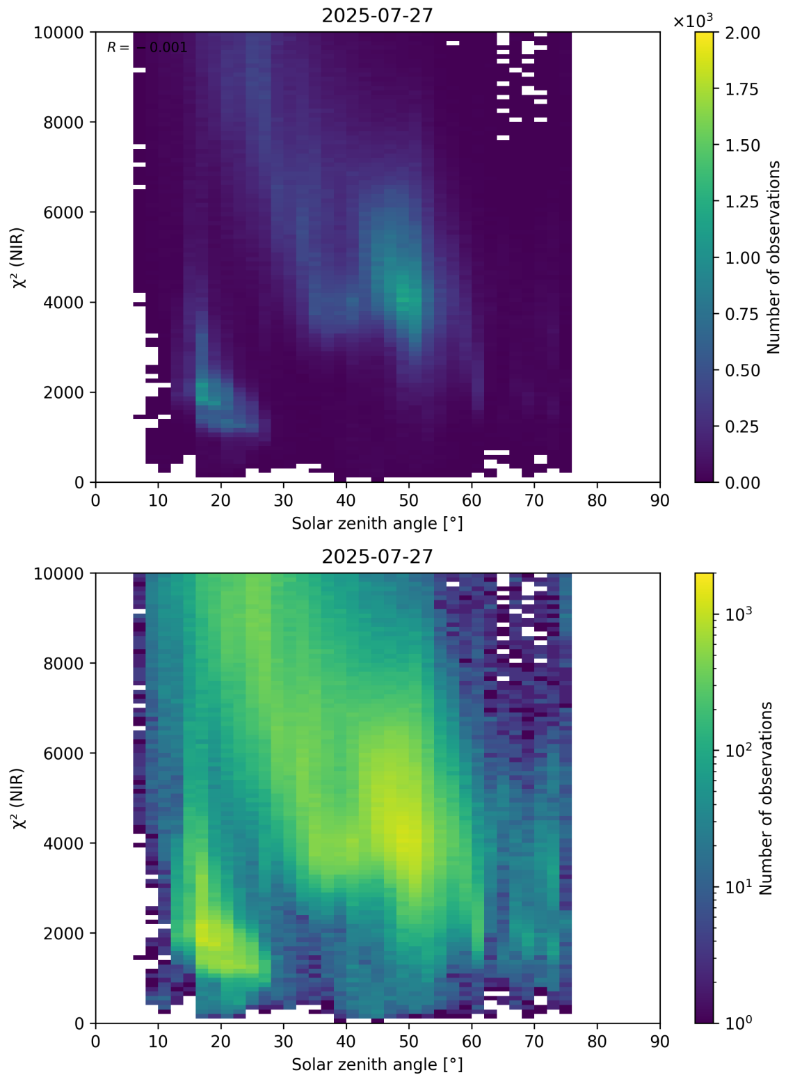
Figure 94: Scatter density plot of “Solar zenith angle” against “ \chi^2 (NIR)” for 2025-07-26 to 2025-07-28.
