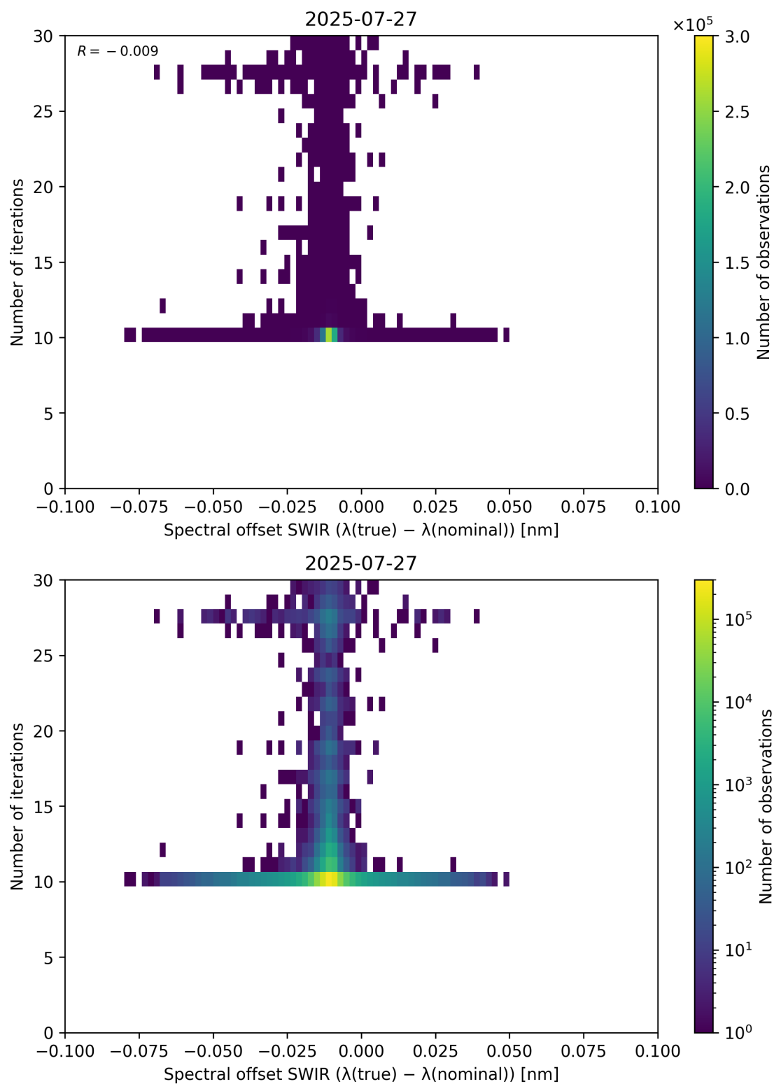
Figure 121: Scatter density plot of “Spectral offset SWIR ( \lambda_{\text{true}} - \lambda_{\text{nominal}} )” against “Number of iterations” for 2025-07-26 to 2025-07-28.
