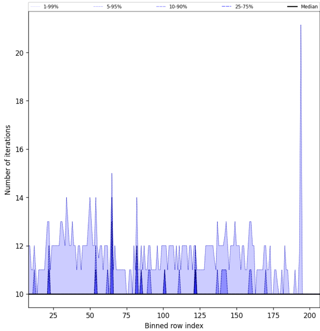
Figure 42: Along track statistics of “Number of iterations” for 2025-07-26 to 2025-07-28
