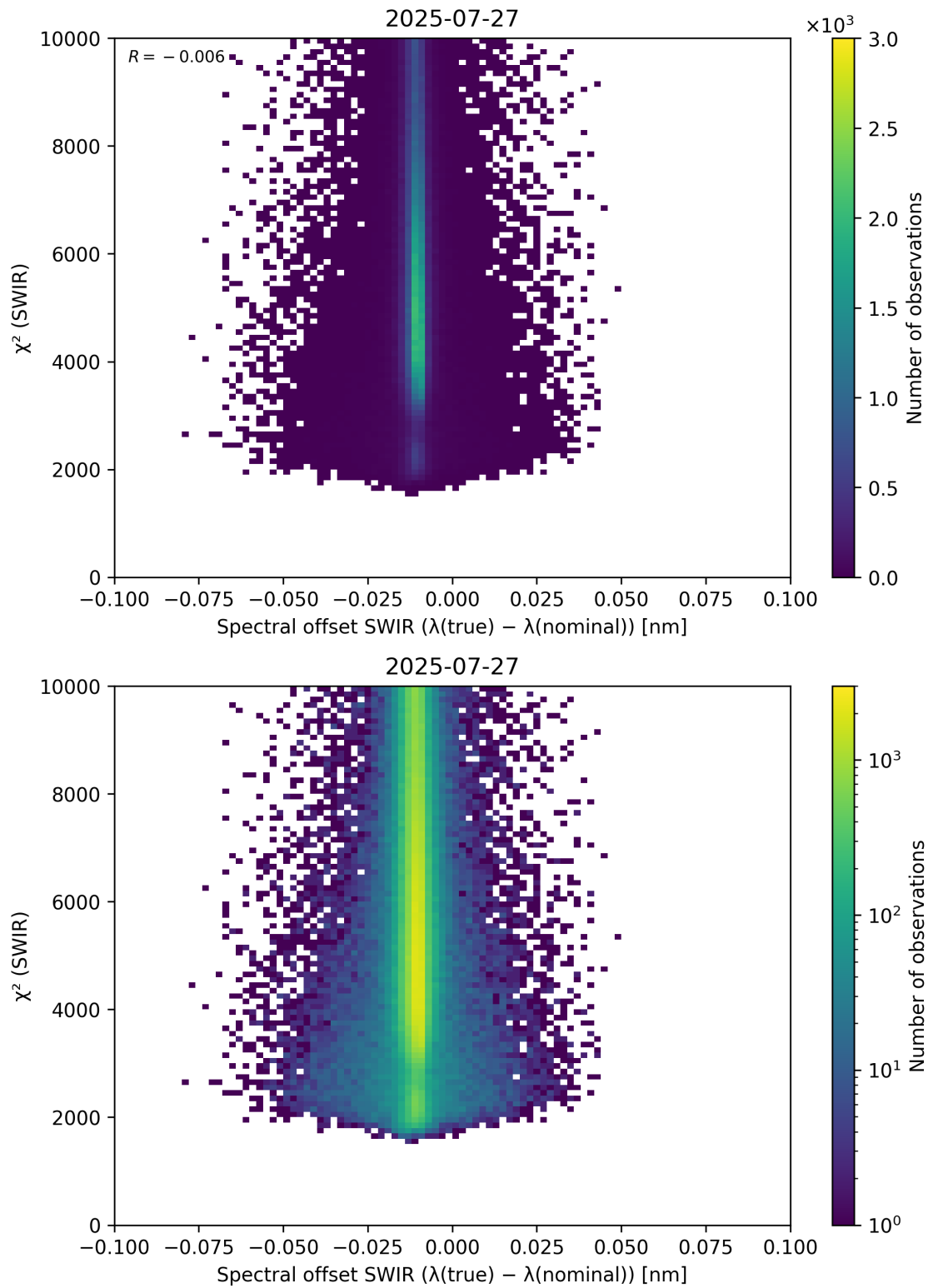
Figure 118: Scatter density plot of “Spectral offset SWIR ( \lambda_{\text{true}} - \lambda_{\text{nominal}} )” against “ \chi^2 (SWIR)” for 2025-07-26 to 2025-07-28.
