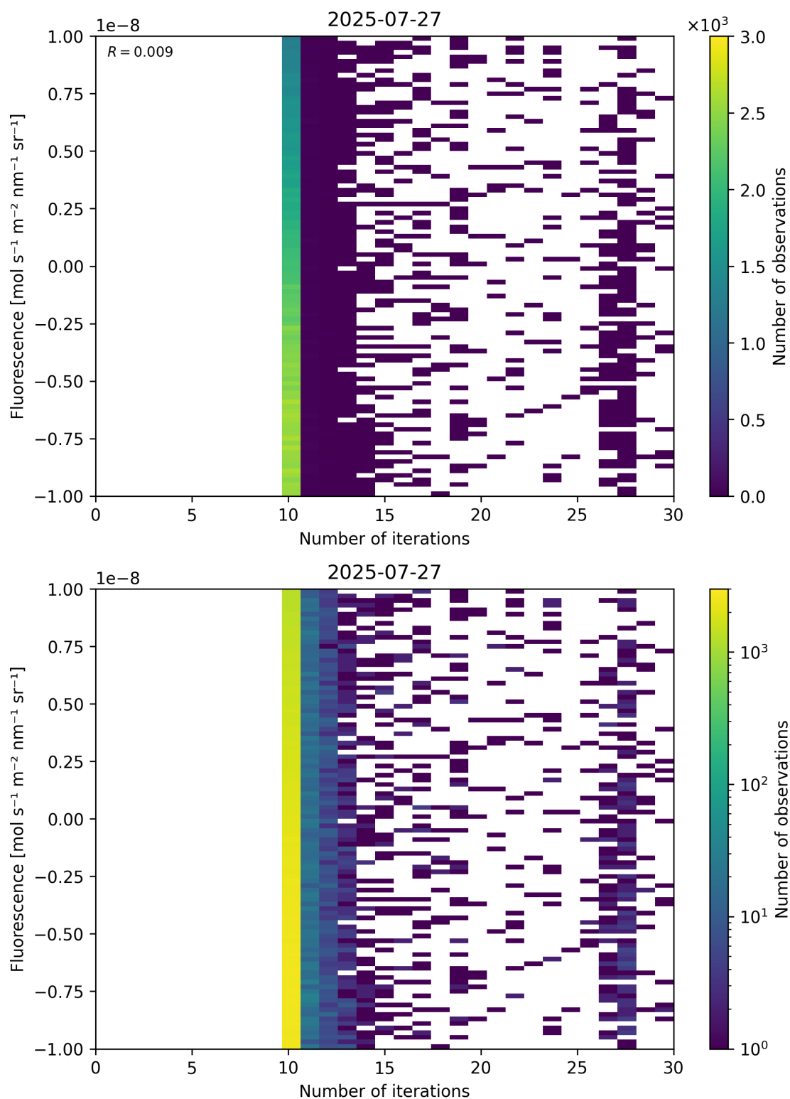
Figure 87: Scatter density plot of “Number of iterations” against “Fluorescence” for 2025-07-26 to 2025-07-28.
