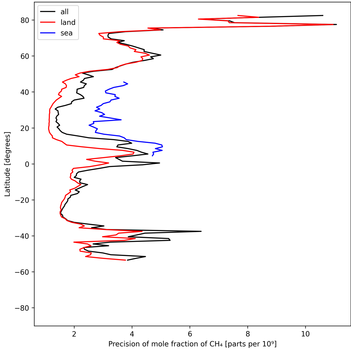
Figure 13: Zonal average of “Precision of mole fraction of CH 4 ” for 2025-07-26 to 2025-07-28.
