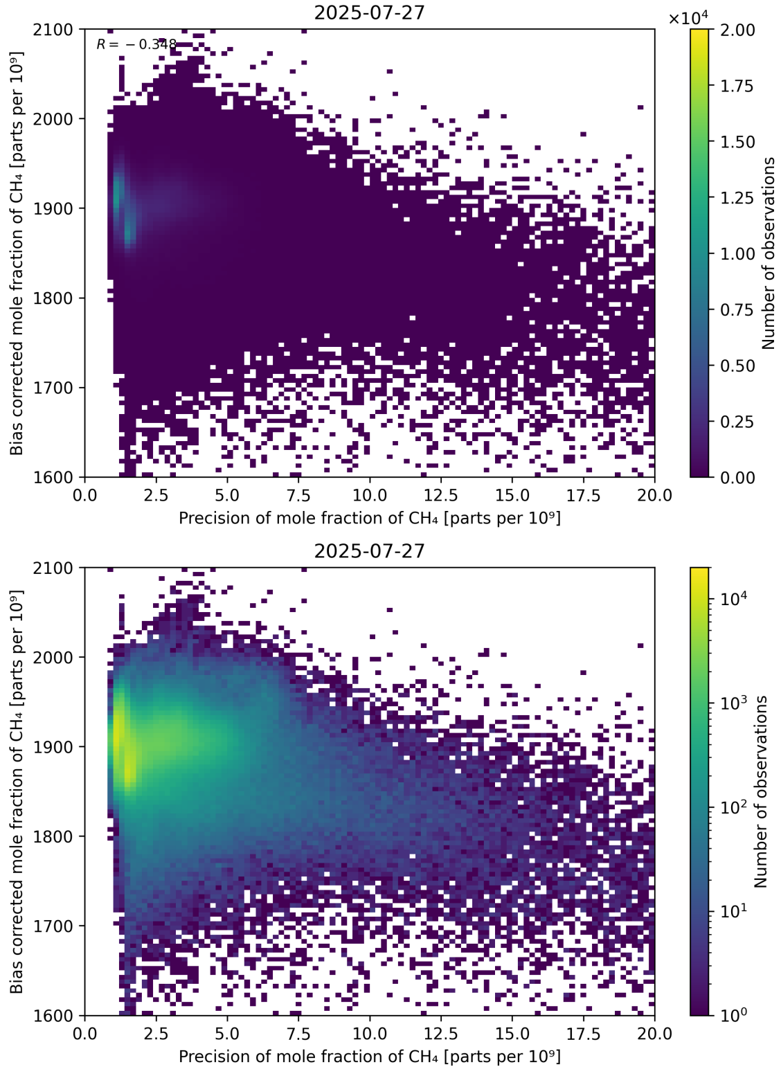
Figure 82: Scatter density plot of “Precision of mole fraction of CH 4 ” against “Bias corrected mole fraction of CH 4 ” for 2025-07-26 to 2025-07-28.
