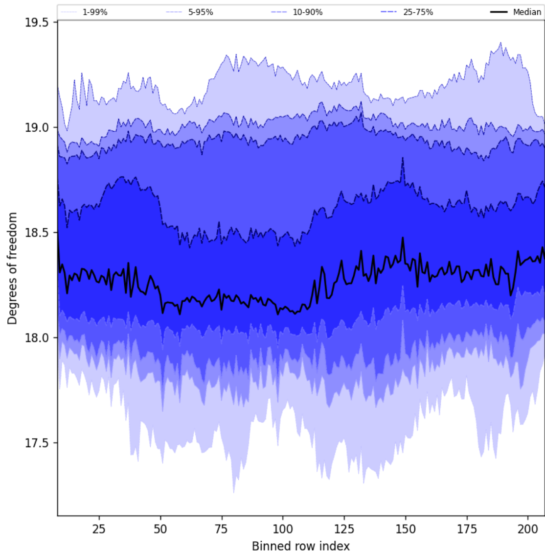
Figure 41: Along track statistics of “Degrees of freedom” for 2025-07-26 to 2025-07-28
