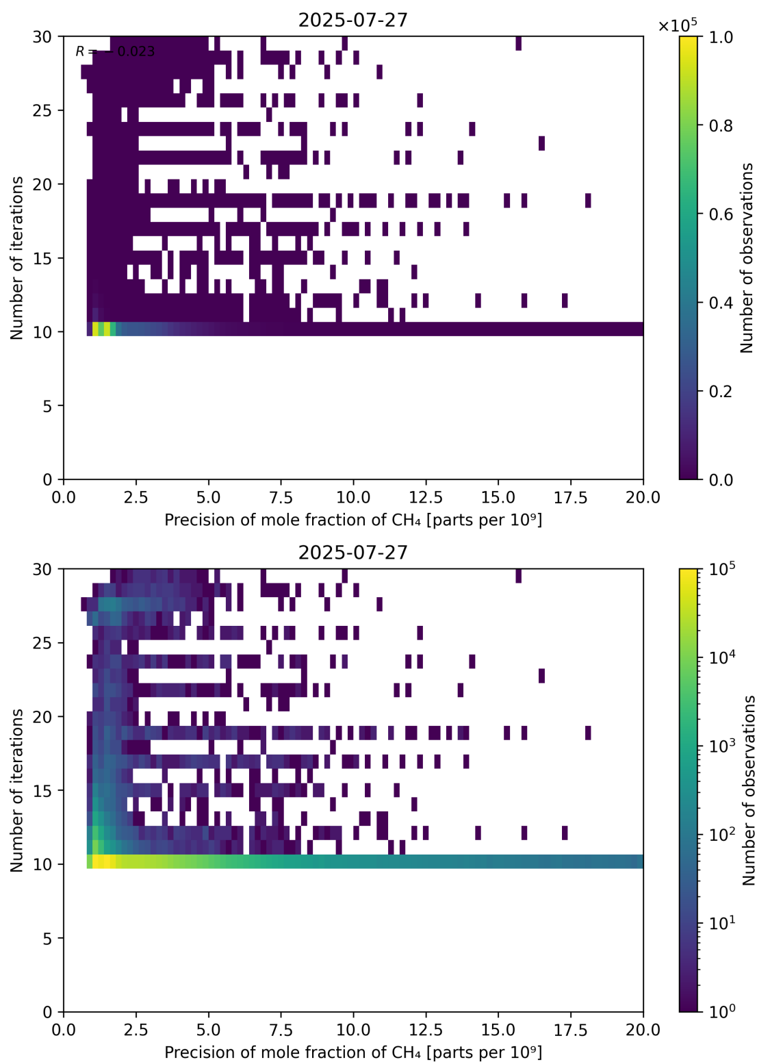
Figure 83: Scatter density plot of “Precision of mole fraction of \text{CH}_4 ” against “Number of iterations” for 2025-07-26 to 2025-07-28.
