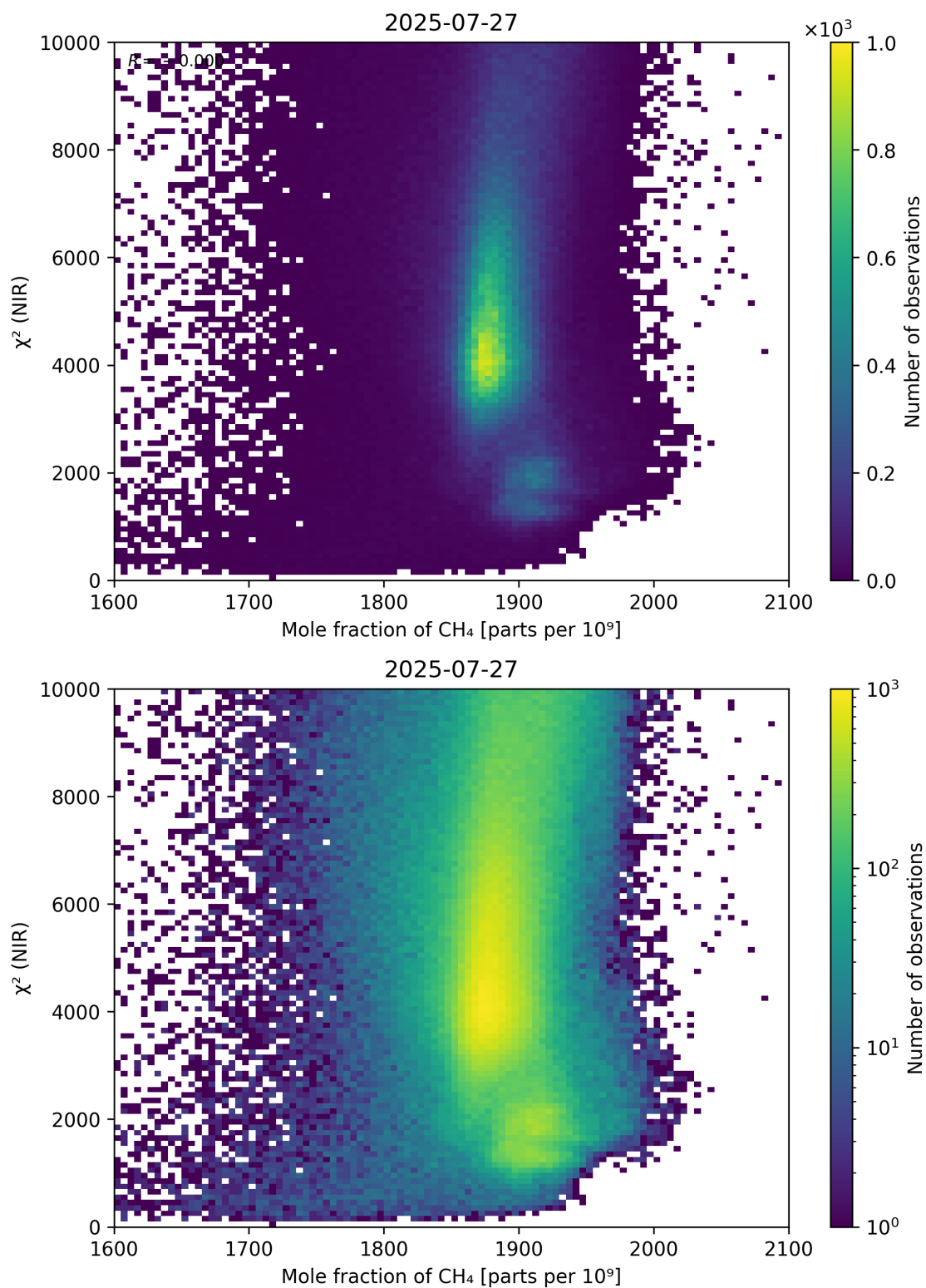
Figure 70: Scatter density plot of “Mole fraction of CH 4 ” against “ \chi^2 (NIR)” for 2025-07-26 to 2025-07-28.
