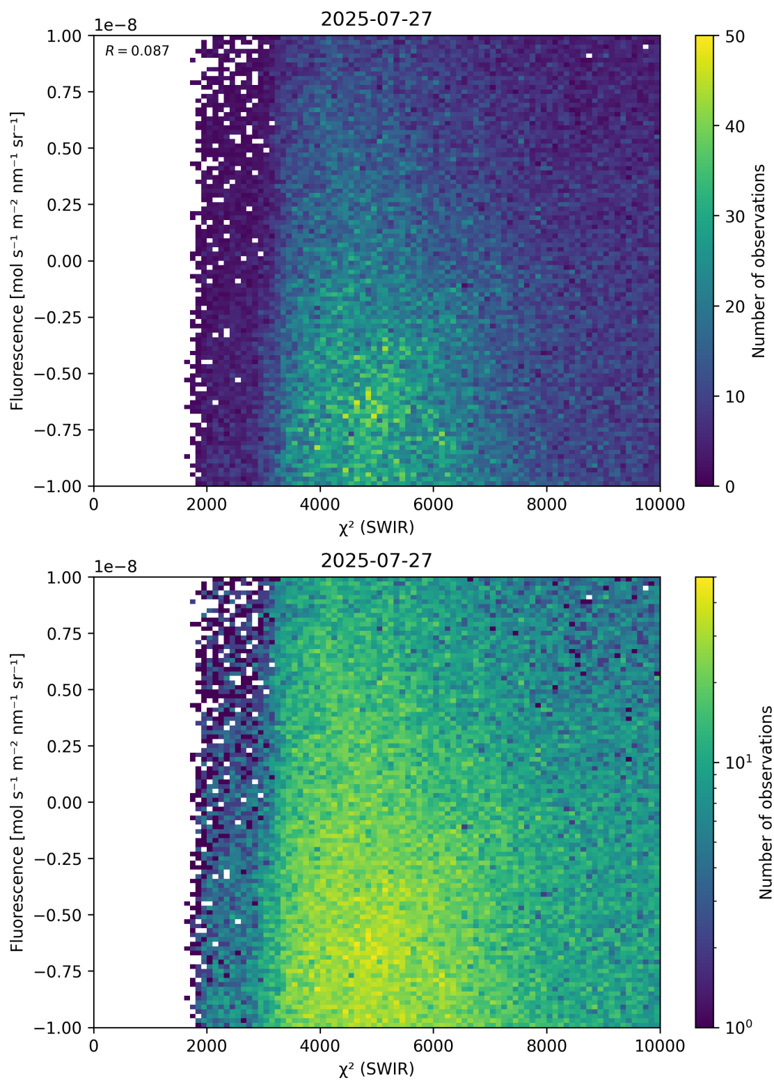
Figure 49: Scatter density plot of “ \chi^2 (SWIR)” against “Fluorescence” for 2025-07-26 to 2025-07-28.
