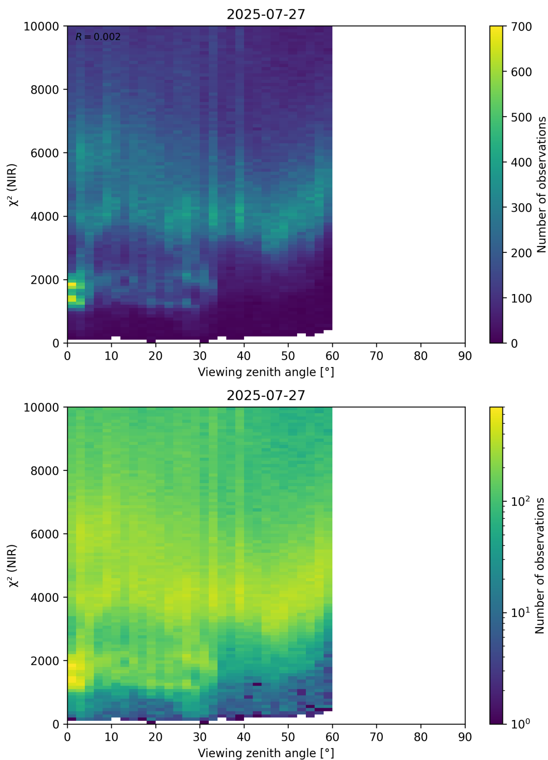
Figure 105: Scatter density plot of “Viewing zenith angle” against “ \chi^2 (NIR)” for 2025-07-26 to 2025-07-28.
