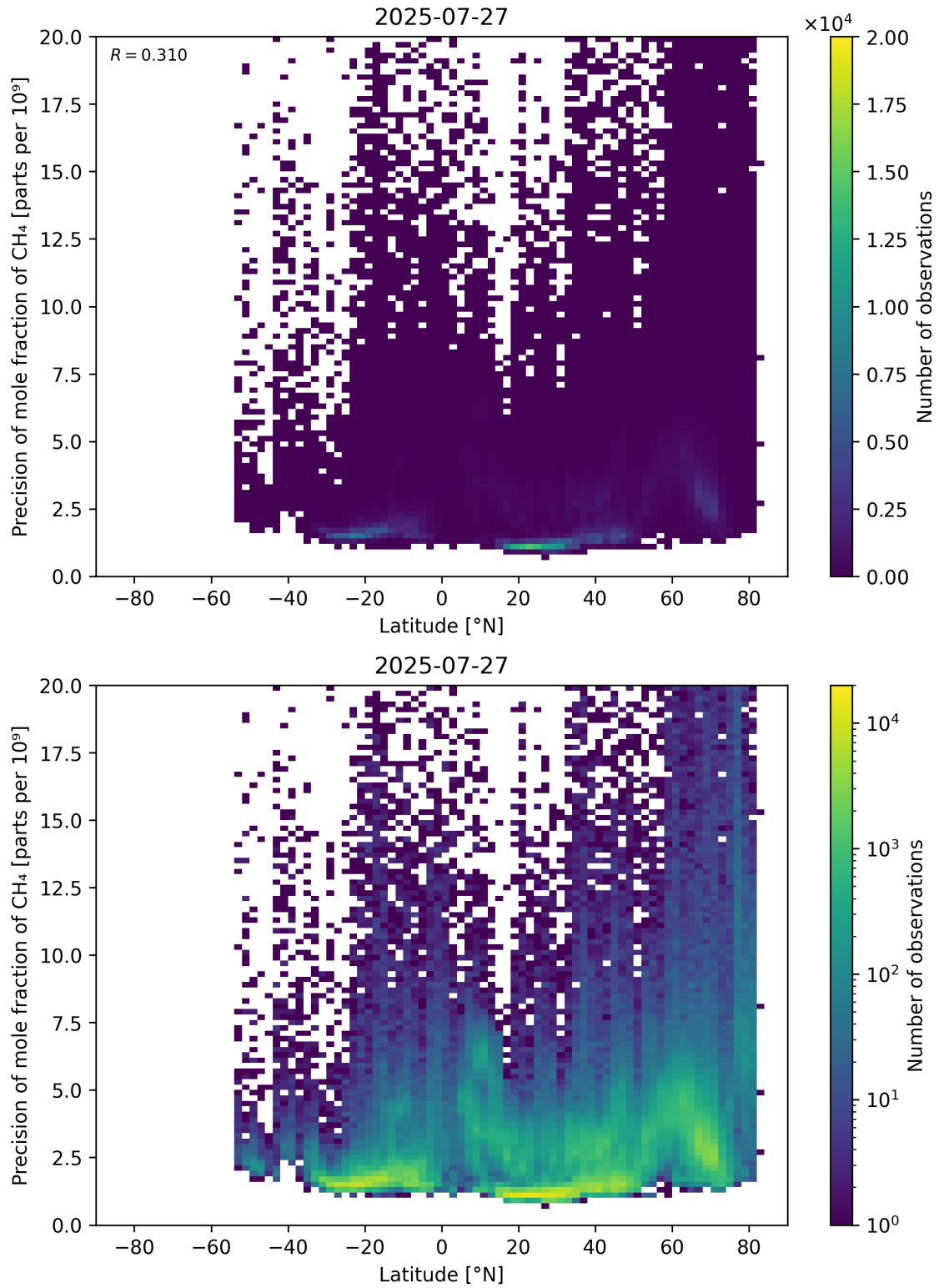
Figure 59: Scatter density plot of “Latitude” against “Precision of mole fraction of \text{CH}_4 ” for 2025-07-26 to 2025-07-28.
