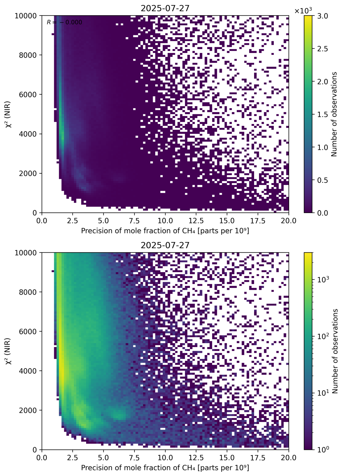
Figure 78: Scatter density plot of “Precision of mole fraction of CH 4 ” against “ \chi^2 (NIR)” for 2025-07-26 to 2025-07-28.
