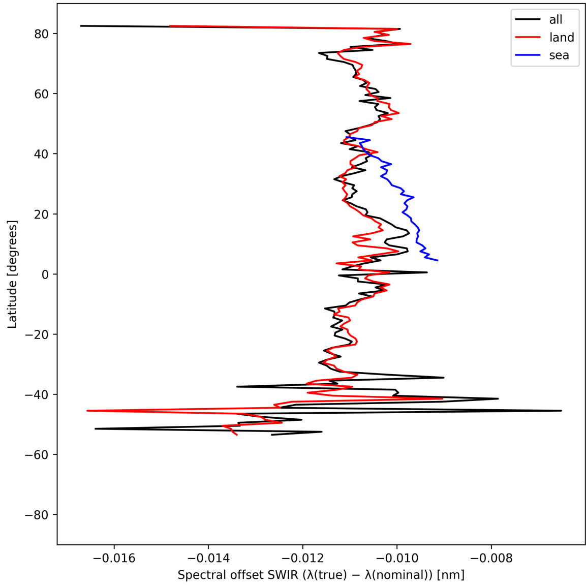
Figure 16: Zonal average of “Spectral offset SWIR ( \lambda_{\text{true}} - \lambda_{\text{nominal}} )” for 2025-07-26 to 2025-07-28.
