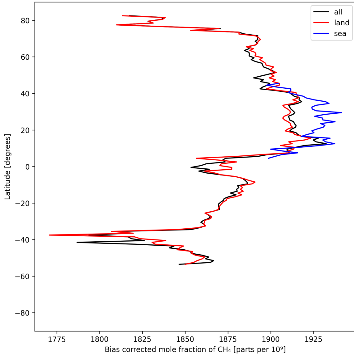
Figure 14: Zonal average of “Bias corrected mole fraction of CH 4 ” for 2025-07-26 to 2025-07-28.
