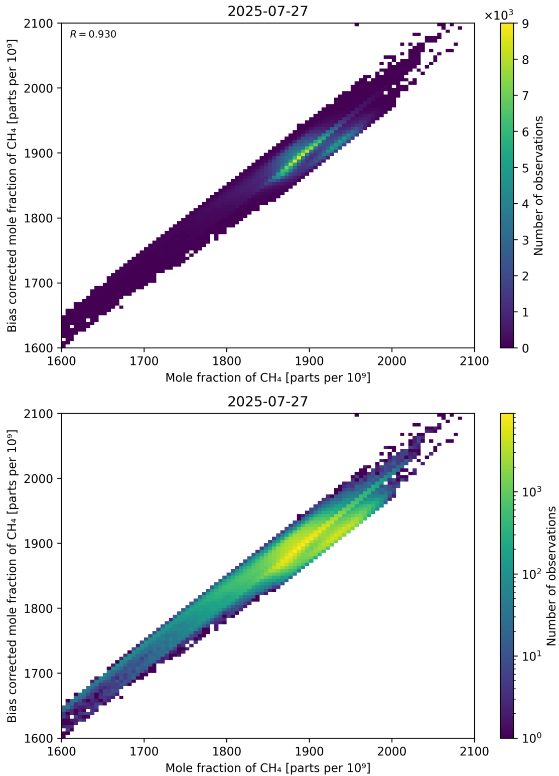
Figure 74: Scatter density plot of “Mole fraction of CH 4 ” against “Bias corrected mole fraction of CH 4 ” for 2025-07-26 to 2025-07-28.
