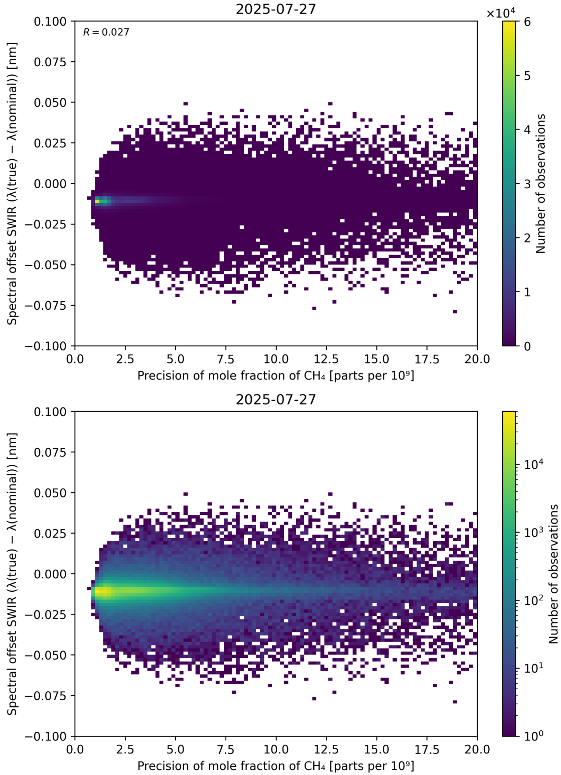
Figure 85: Scatter density plot of “Precision of mole fraction of \text{CH}_4 ” against “Spectral offset SWIR ( \lambda_{\text{true}} - \lambda_{\text{nominal}} )” for 2025-07-26 to 2025-07-28.
