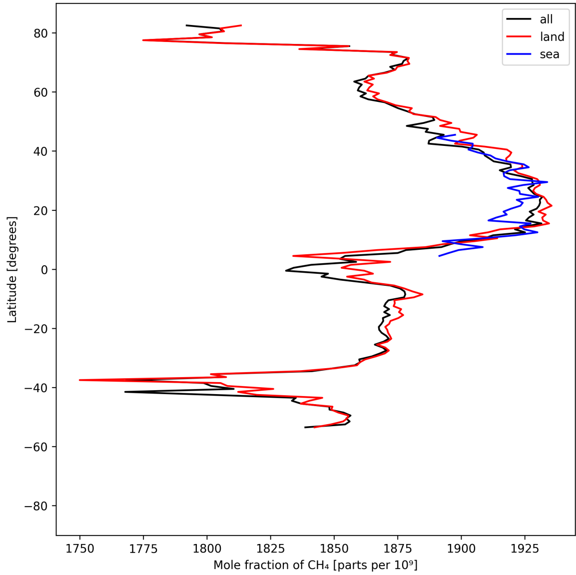
Figure 12: Zonal average of “Mole fraction of CH 4 ” for 2025-07-26 to 2025-07-28.
