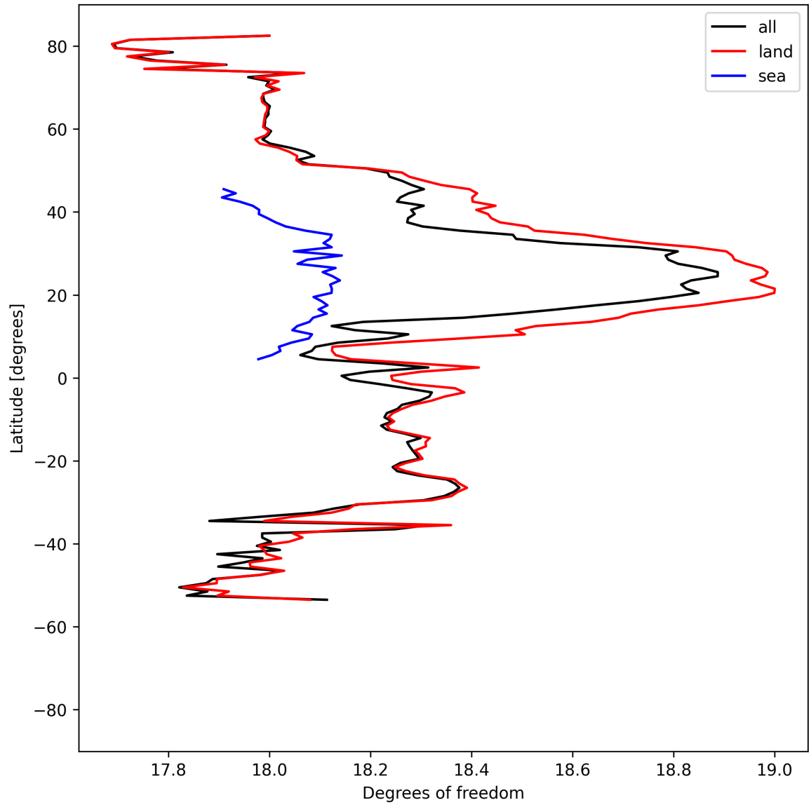
Figure 19: Zonal average of “Degrees of freedom” for 2025-07-26 to 2025-07-28.
