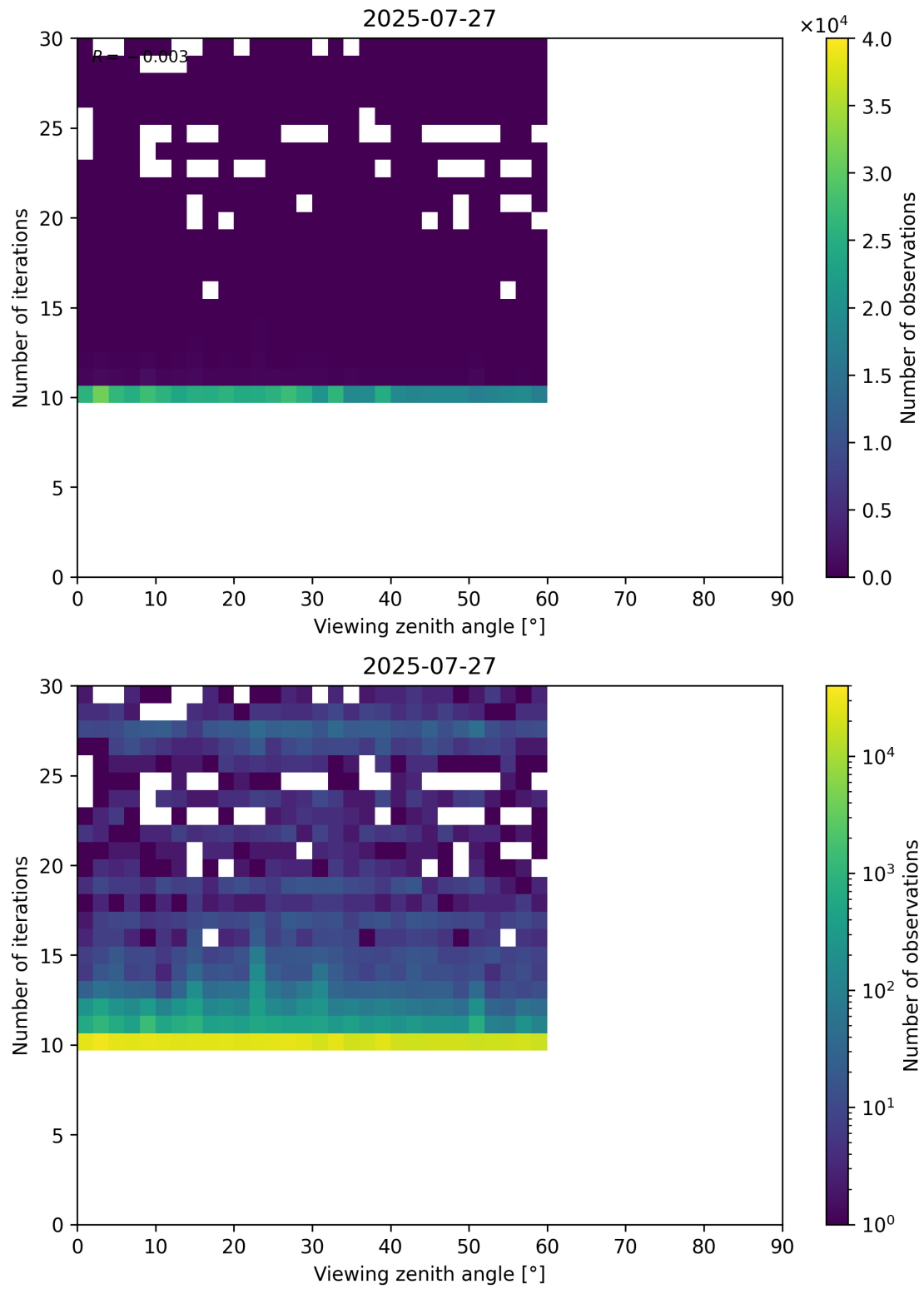
Figure 113: Scatter density plot of “Viewing zenith angle” against “Number of iterations” for 2025-07-26 to 2025-07-28.
