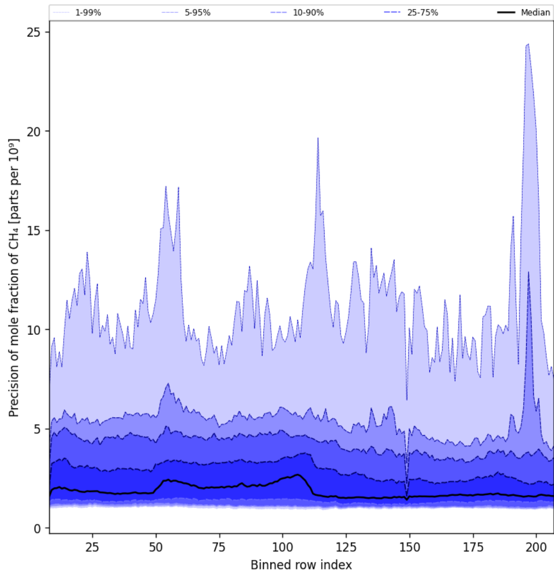
Figure 35: Along track statistics of “Precision of mole fraction of CH 4 ” for 2025-07-26 to 2025-07-28
