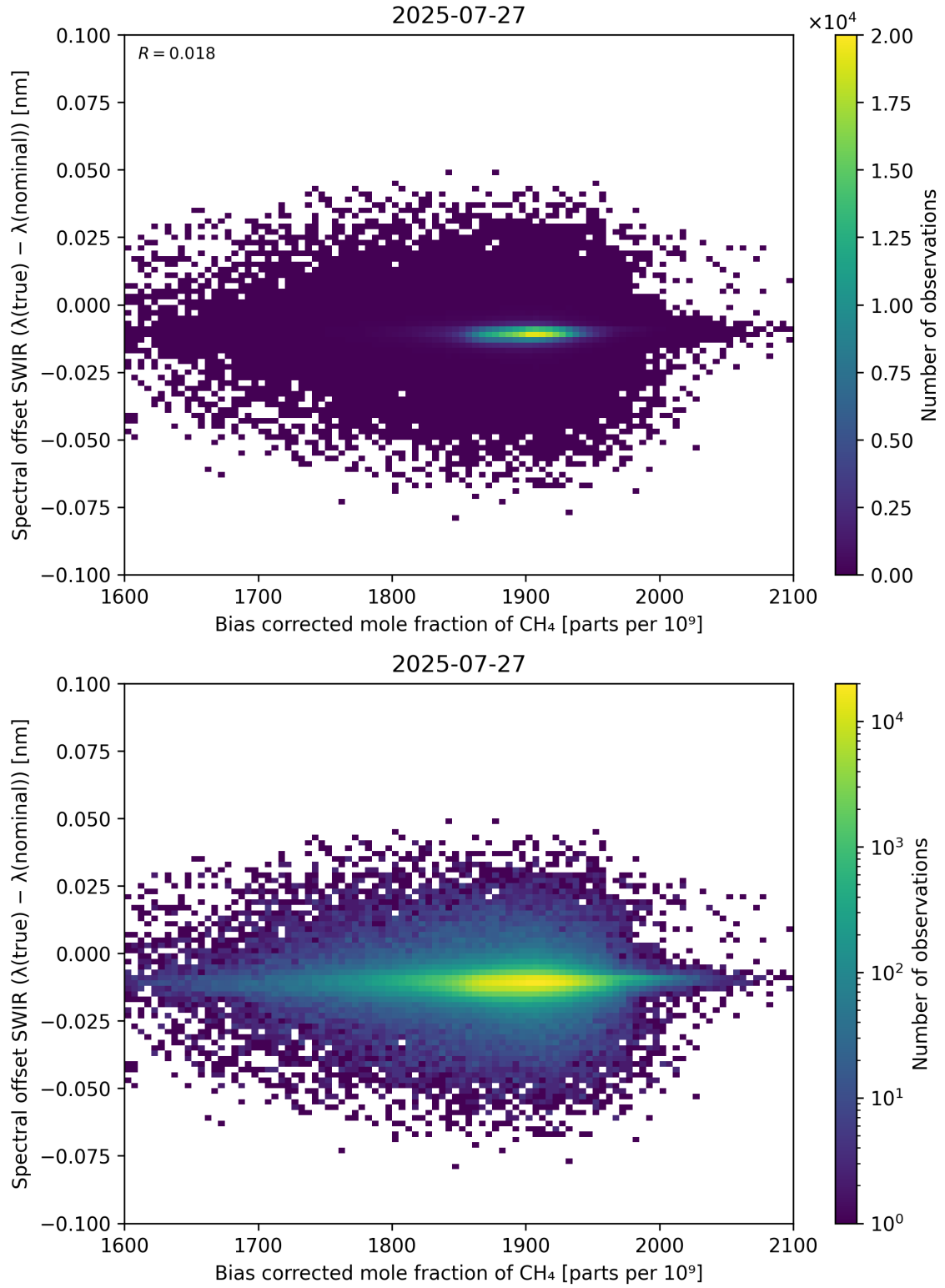
Figure 69: Scatter density plot of “Bias corrected mole fraction of \text{CH}_4 ” against “Spectral offset SWIR ( \lambda_{\text{true}} - \lambda_{\text{nominal}} )” for 2025-07-26 to 2025-07-28.
