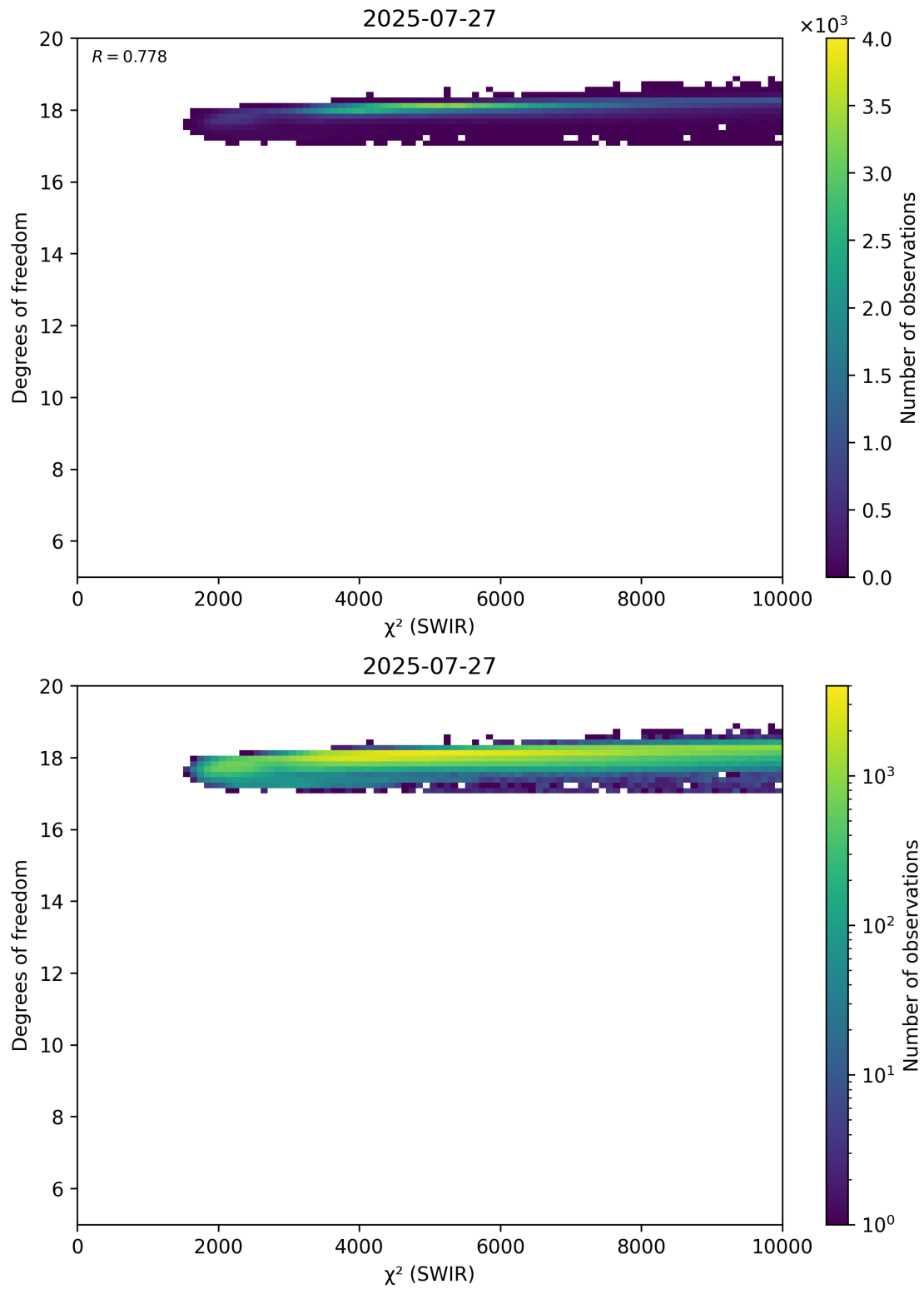
Figure 48: Scatter density plot of “ \chi^2 (SWIR)” against “Degrees of freedom” for 2025-07-26 to 2025-07-28.
