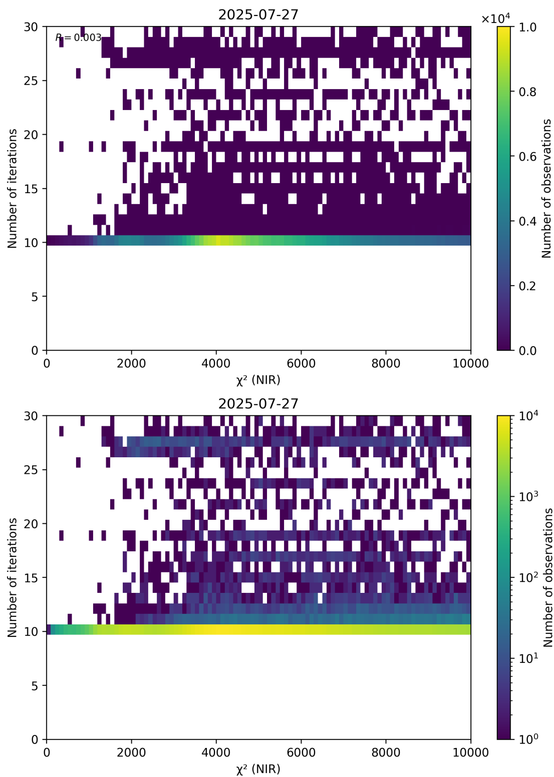
Figure 46: Scatter density plot of “ \chi^2 (NIR)” against “Number of iterations” for 2025-07-26 to 2025-07-28.
