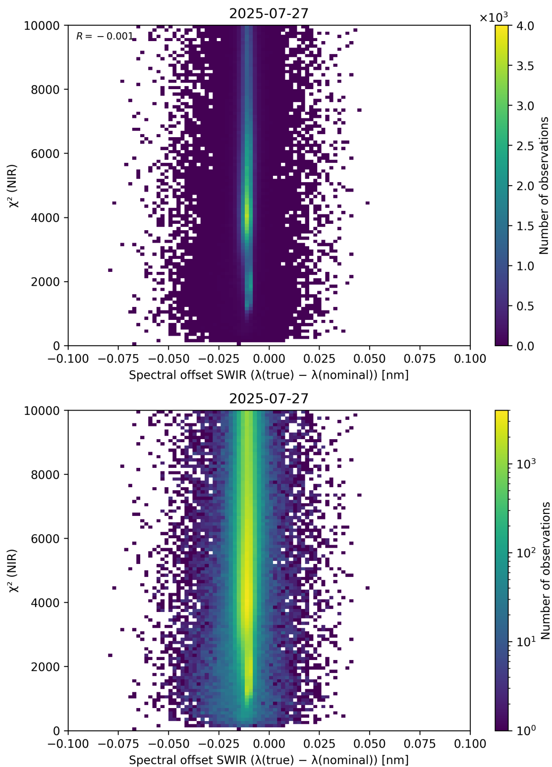
Figure 117: Scatter density plot of “Spectral offset SWIR ( \lambda_{\text{true}} - \lambda_{\text{nominal}} )” against “ \chi^2 (NIR)” for 2025-07-26 to 2025-07-28.
