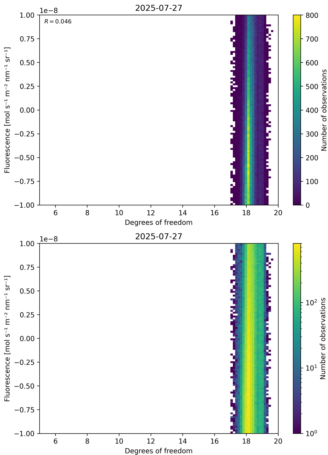
Figure 51: Scatter density plot of “Degrees of freedom” against “Fluorescence” for 2025-07-26 to 2025-07-28.
