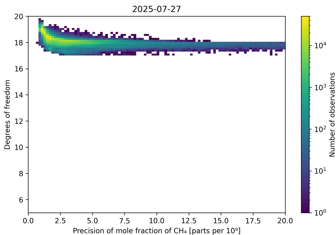
Figure 80: Scatter density plot of “Precision of mole fraction of CH 4 ” against “Degrees of freedom” for 2025-07-26 to 2025-07-28.
