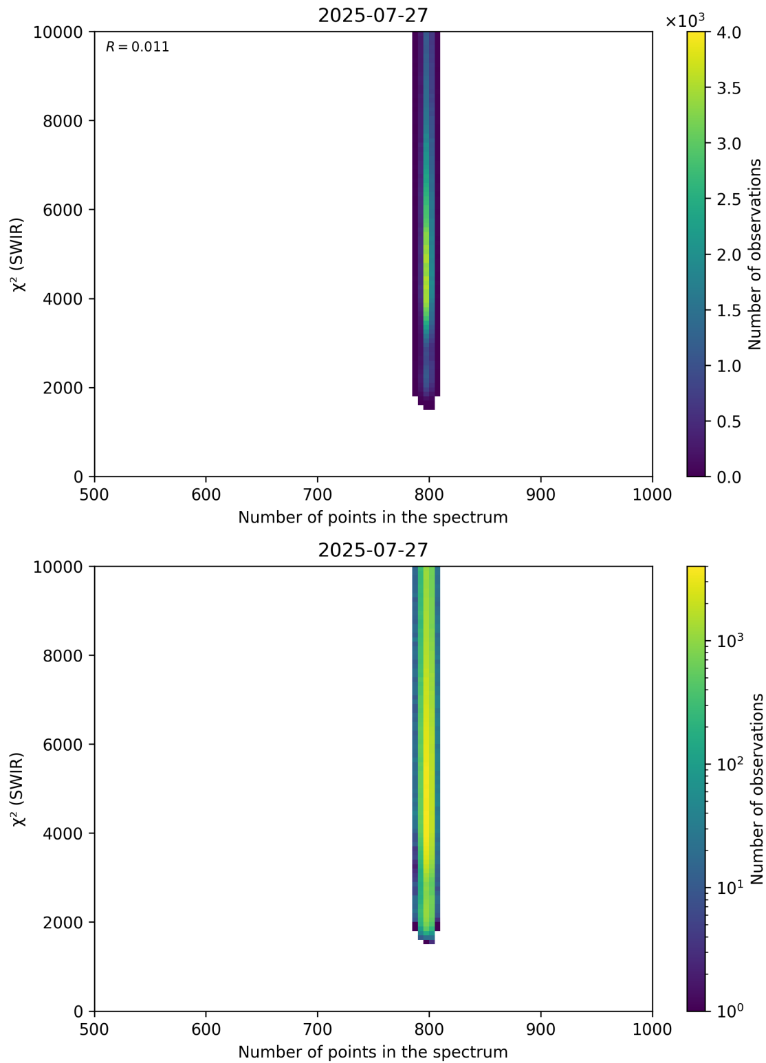
Figure 89: Scatter density plot of “Number of points in the spectrum” against “ \chi^2 (SWIR)” for 2025-07-26 to 2025-07-28.
