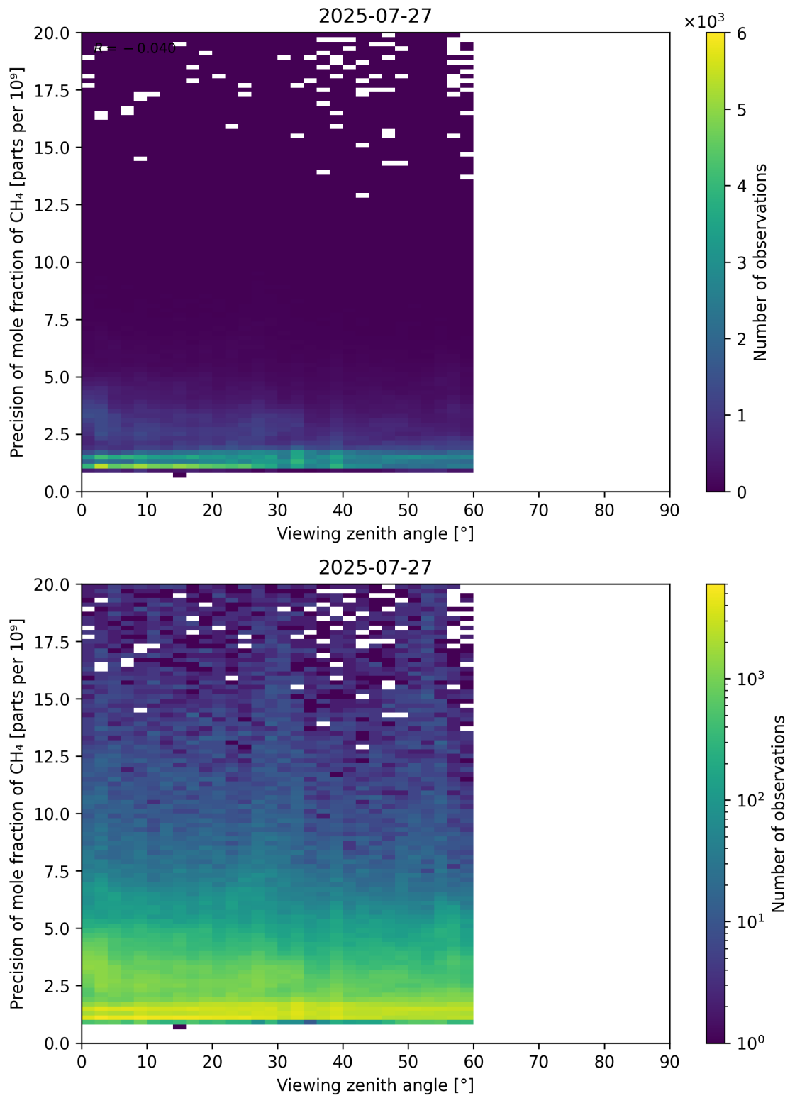
Figure 112: Scatter density plot of “Viewing zenith angle” against “Precision of mole fraction of CH 4 ” for 2025-07-26 to 2025-07-28.
