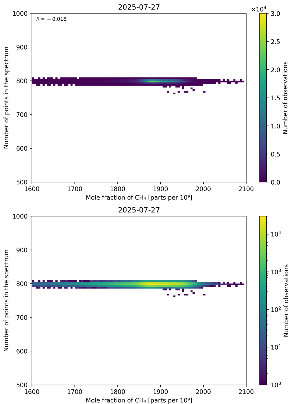
Figure 77: Scatter density plot of “Mole fraction of CH 4 ” against “Number of points in the spectrum” for 2025-07-26 to 2025-07-28.
