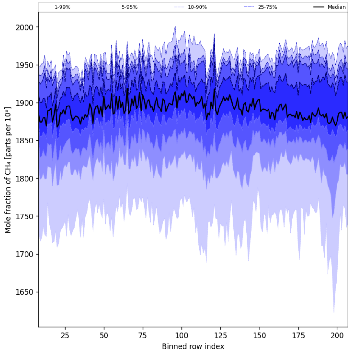
Figure 34: Along track statistics of “Mole fraction of CH 4 ” for 2025-07-26 to 2025-07-28
