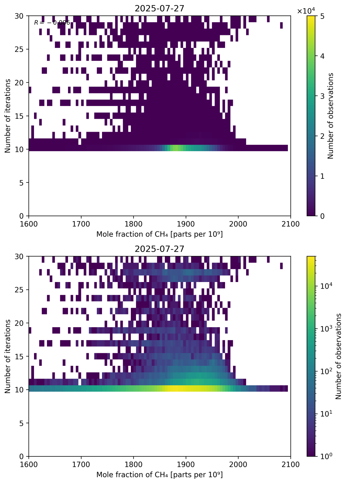
Figure 76: Scatter density plot of “Mole fraction of CH 4 ” against “Number of iterations” for 2025-07-26 to 2025-07-28.
