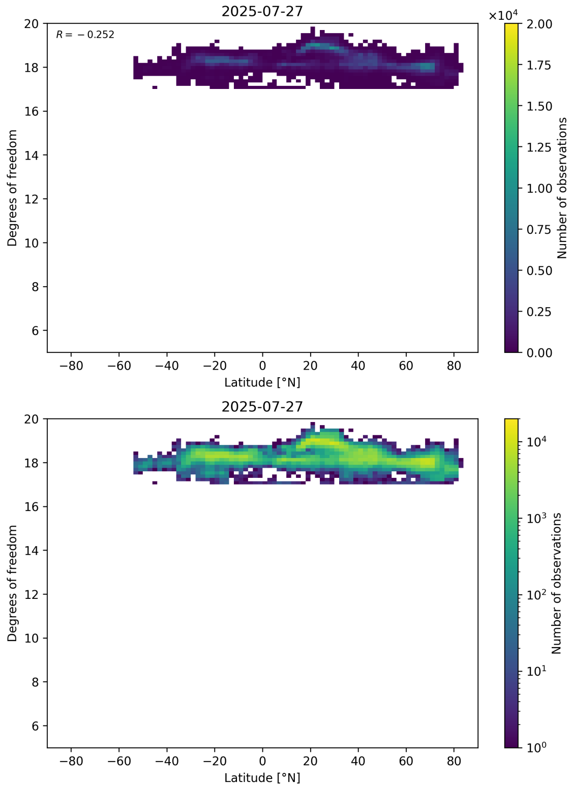
Figure 55: Scatter density plot of “Latitude” against “Degrees of freedom” for 2025-07-26 to 2025-07-28.
