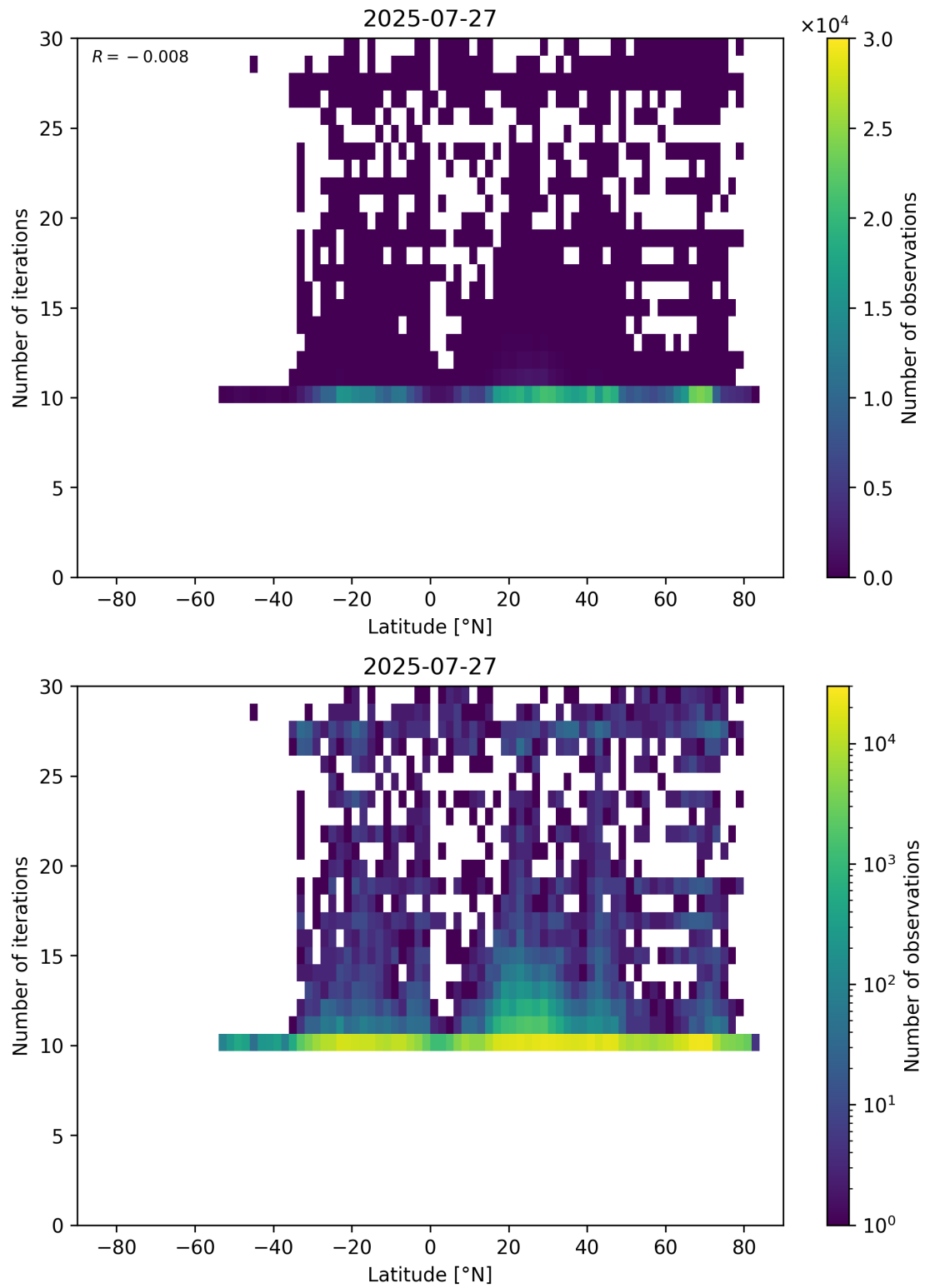
Figure 60: Scatter density plot of “Latitude” against “Number of iterations” for 2025-07-26 to 2025-07-28.
