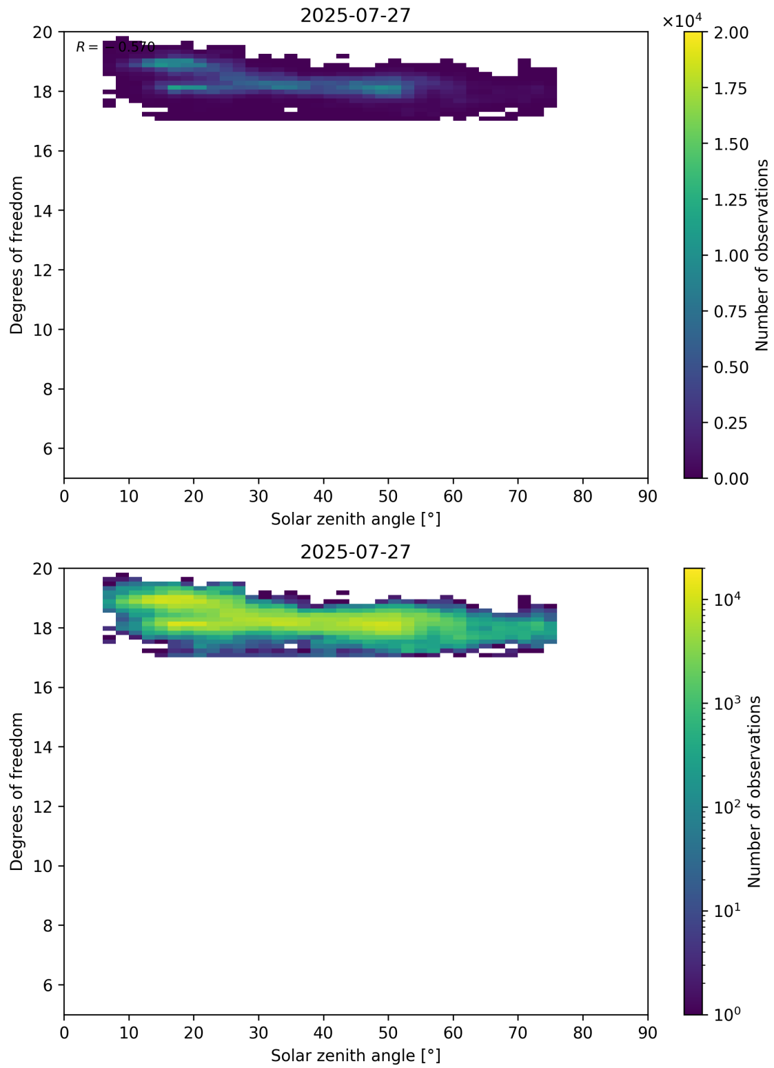
Figure 96: Scatter density plot of “Solar zenith angle” against “Degrees of freedom” for 2025-07-26 to 2025-07-28.
