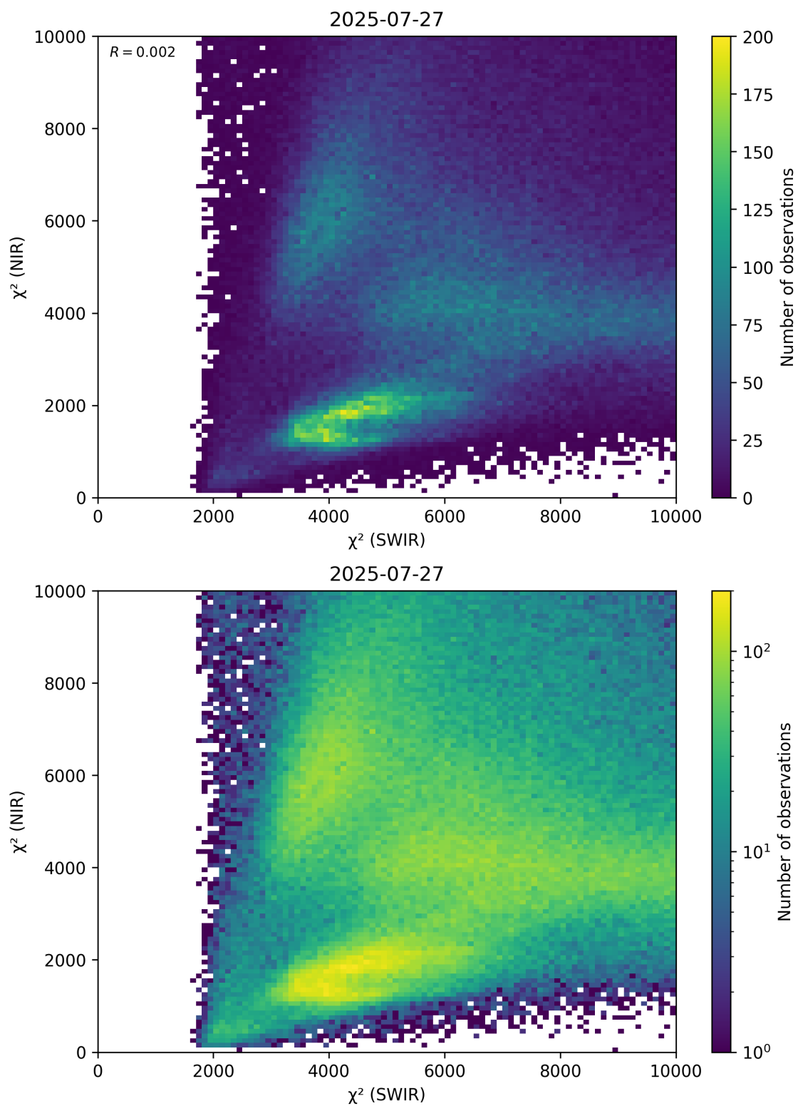
Figure 47: Scatter density plot of “ \chi^2 (SWIR)” against “ \chi^2 (NIR)” for 2025-07-26 to 2025-07-28.
