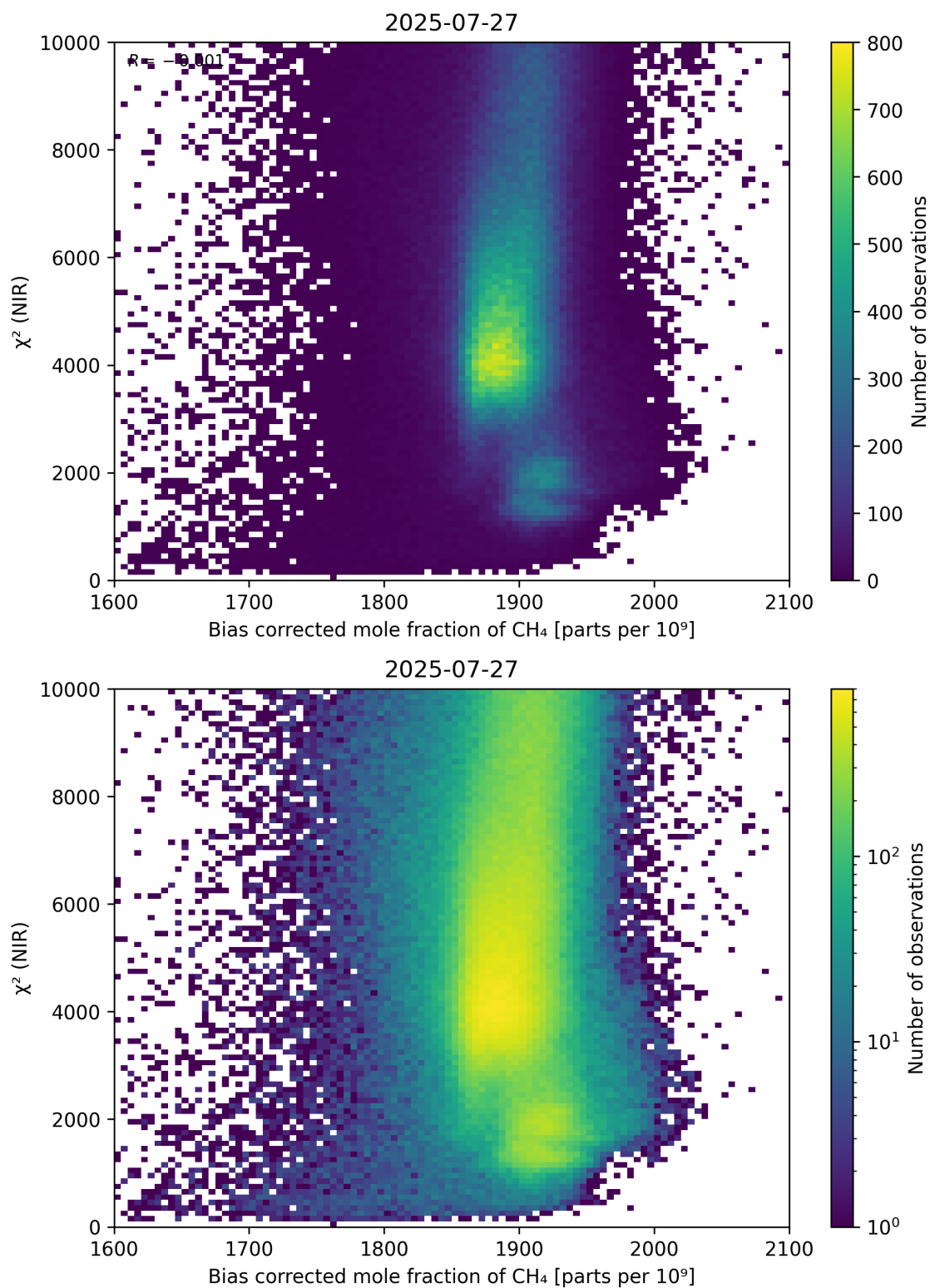
Figure 63: Scatter density plot of “Bias corrected mole fraction of \text{CH}_4 ” against “ \chi^2 (NIR)” for 2025-07-26 to 2025-07-28.
