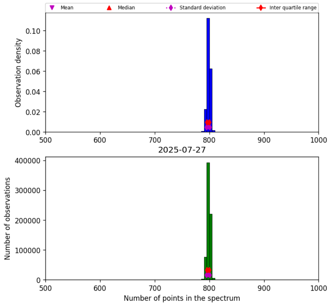
Figure 26: Histogram of “Number of points in the spectrum” for 2025-07-26 to 2025-07-28
