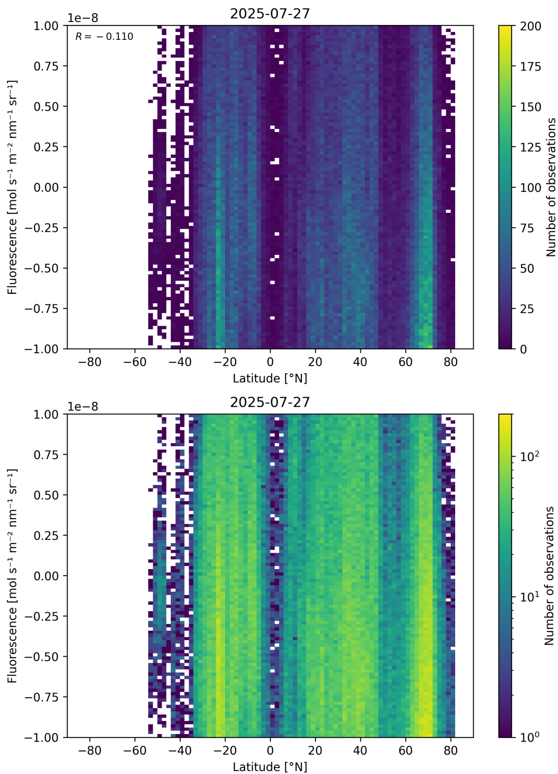
Figure 56: Scatter density plot of “Latitude” against “Fluorescence” for 2025-07-26 to 2025-07-28.
