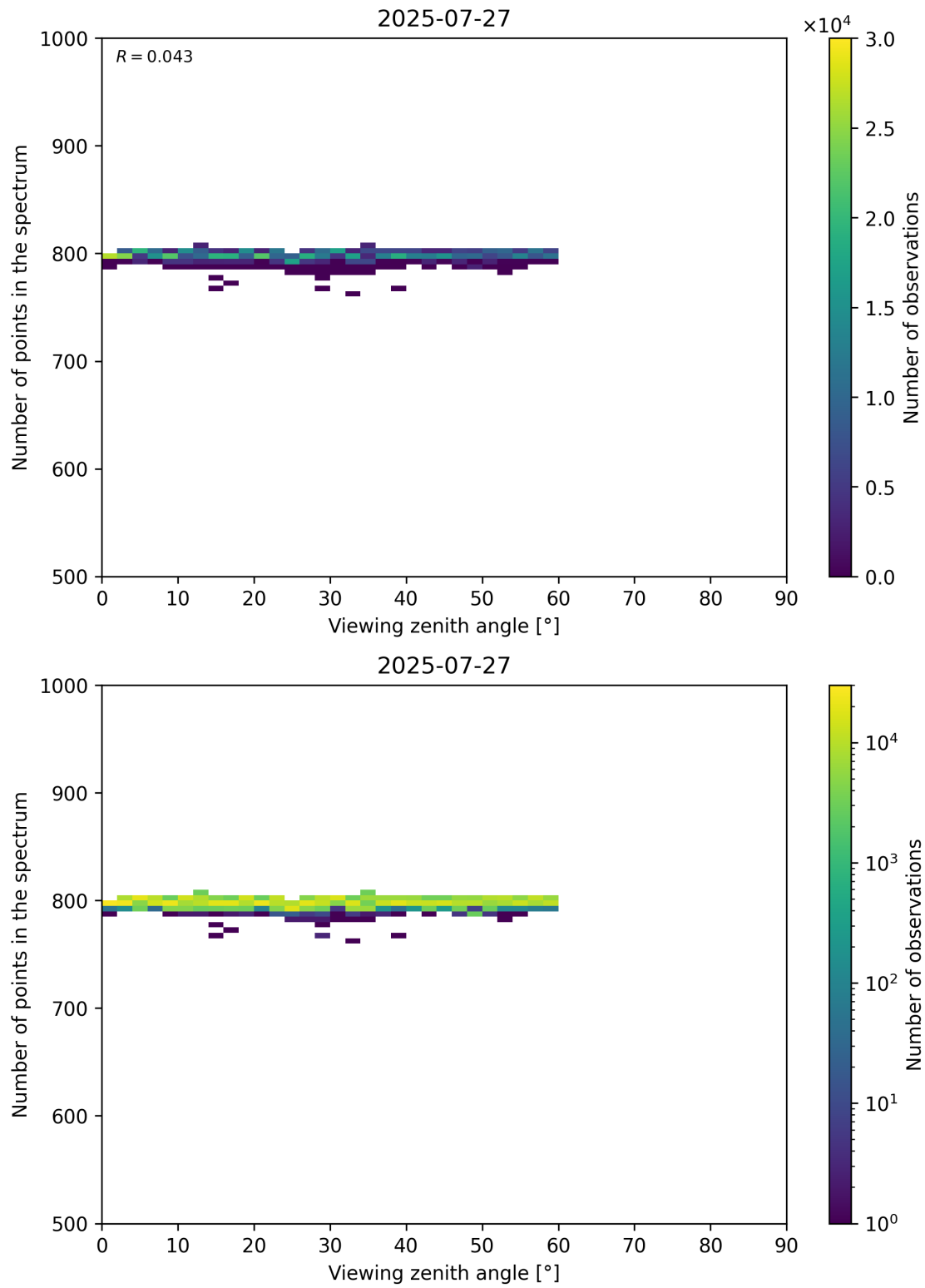
Figure 114: Scatter density plot of “Viewing zenith angle” against “Number of points in the spectrum” for 2025-07-26 to 2025-07-28.
