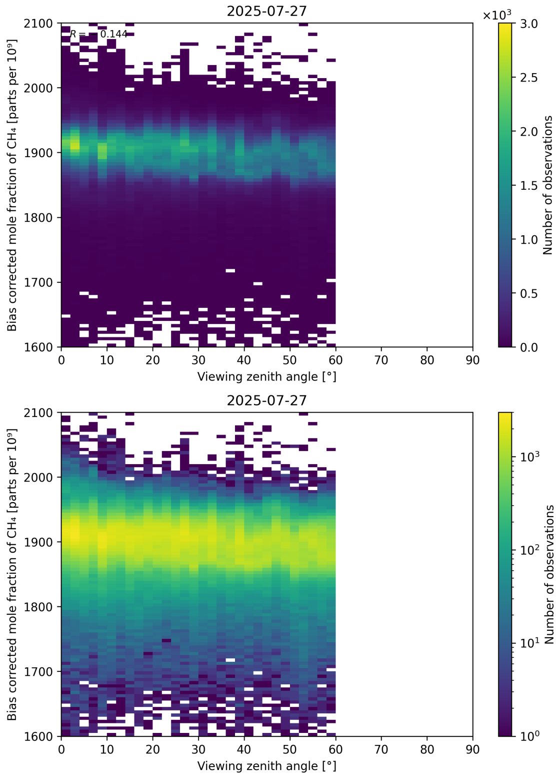
Figure 111: Scatter density plot of “Viewing zenith angle” against “Bias corrected mole fraction of CH 4 ” for 2025-07-26 to 2025-07-28.
