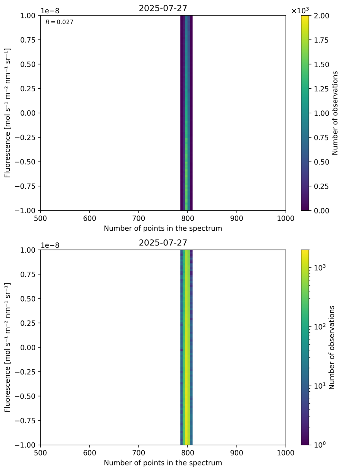
Figure 91: Scatter density plot of “Number of points in the spectrum” against “Fluorescence” for 2025-07-26 to 2025-07-28.
