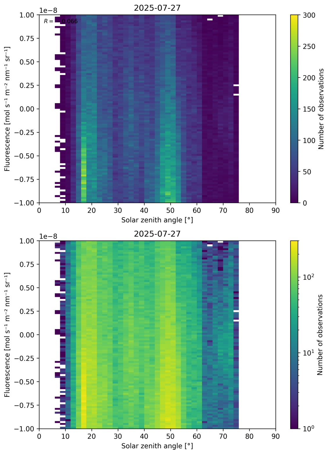
Figure 97: Scatter density plot of “Solar zenith angle” against “Fluorescence” for 2025-07-26 to 2025-07-28.
