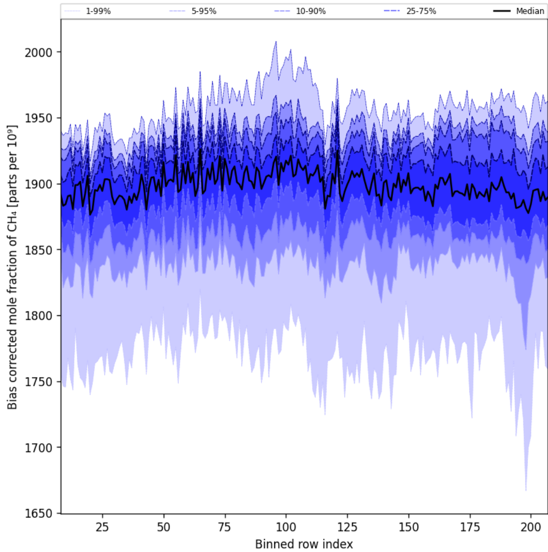
Figure 36: Along track statistics of “Bias corrected mole fraction of CH 4 ” for 2025-07-26 to 2025-07-28
