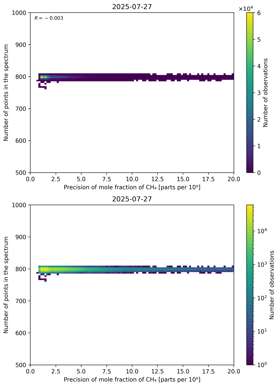
Figure 84: Scatter density plot of “Precision of mole fraction of CH 4 ” against “Number of points in the spectrum” for 2025-07-26 to 2025-07-28.
