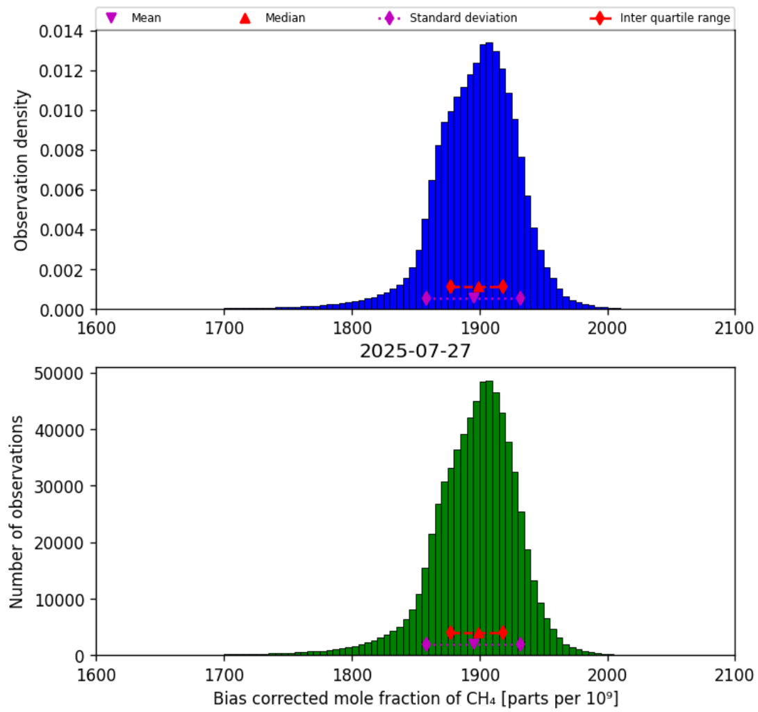
Figure 25: Histogram of “Bias corrected mole fraction of CH 4 ” for 2025-07-26 to 2025-07-28
