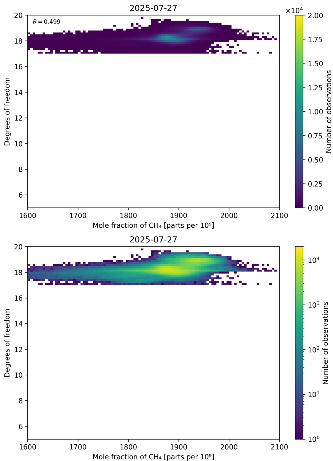
Figure 72: Scatter density plot of “Mole fraction of CH 4 ” against “Degrees of freedom” for 2025-07-26 to 2025-07-28.
