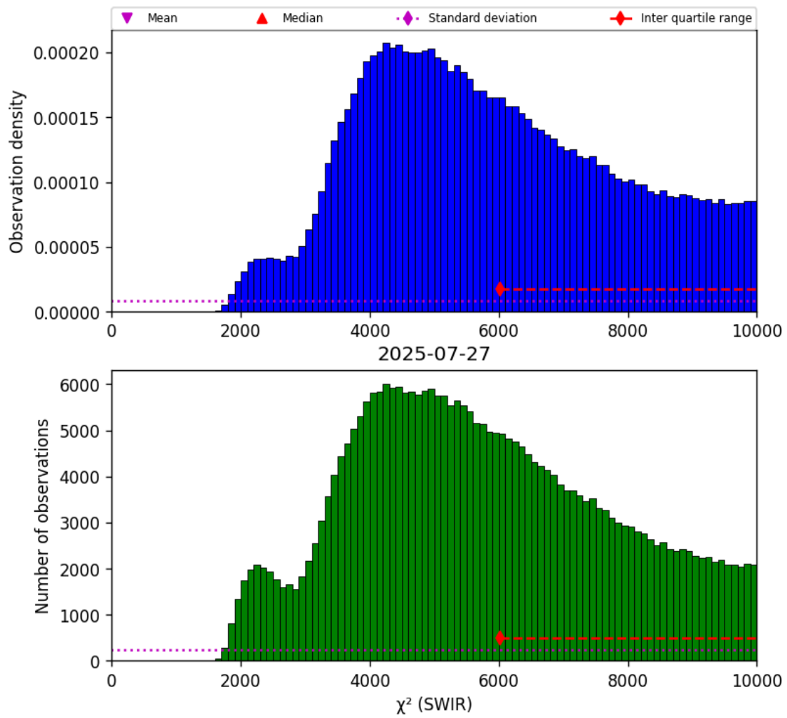
Figure 28: Histogram of “ \chi^2 (SWIR)” for 2025-07-26 to 2025-07-28
