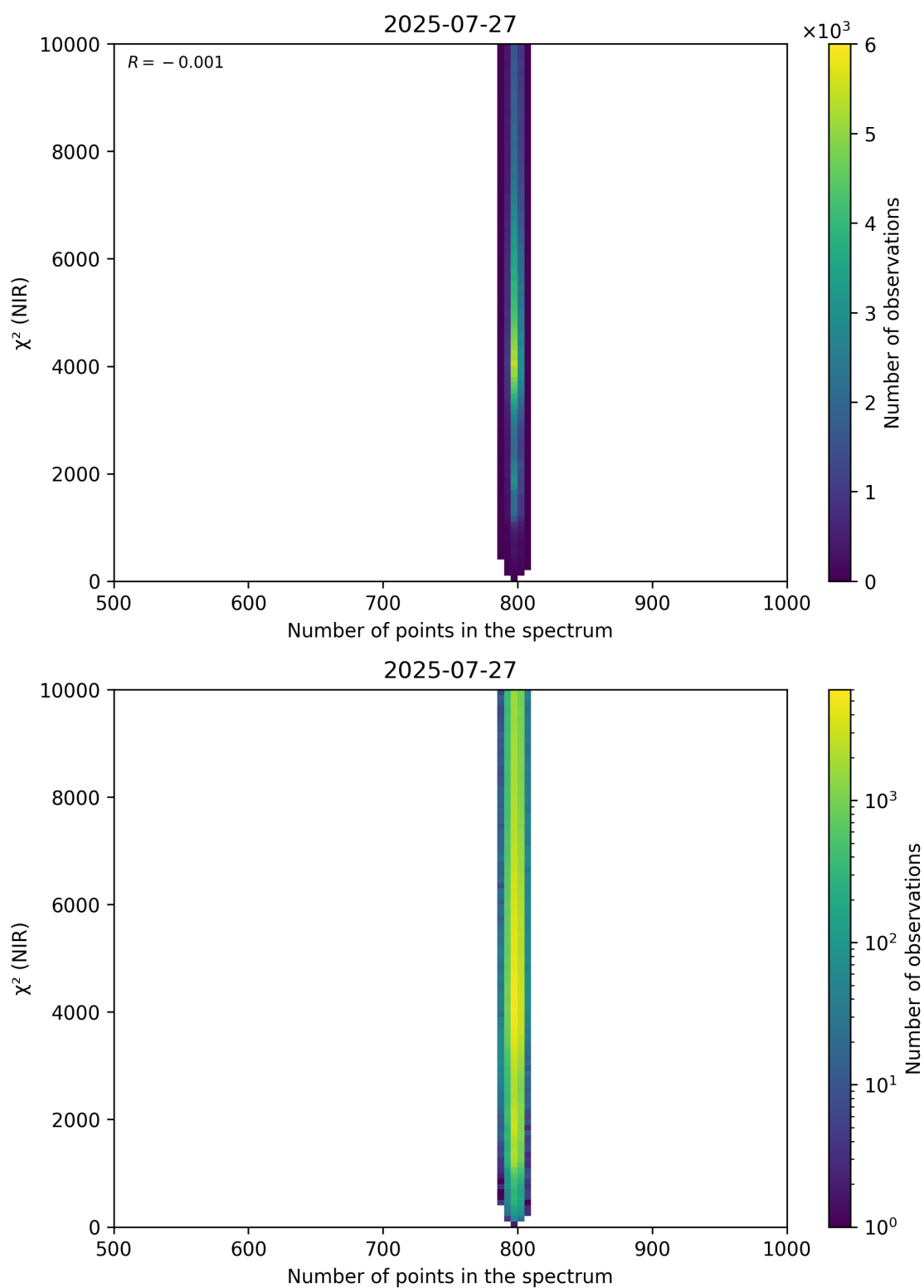
Figure 88: Scatter density plot of “Number of points in the spectrum” against “ \chi^2 (NIR)” for 2025-07-26 to 2025-07-28.
