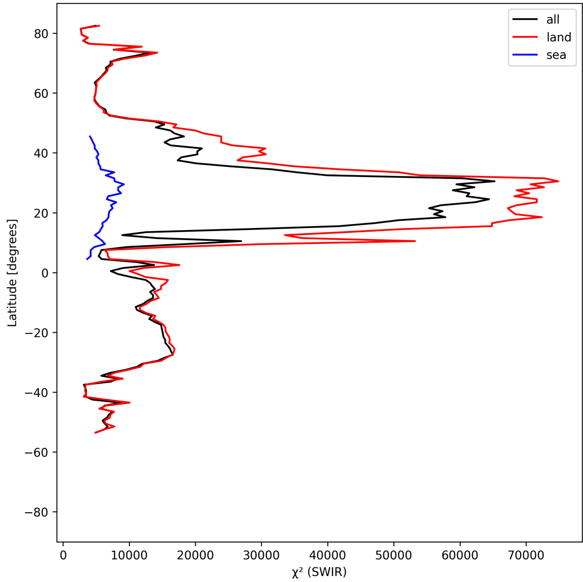
Figure 17: Zonal average of “ \chi^2 (SWIR)” for 2025-07-26 to 2025-07-28.
