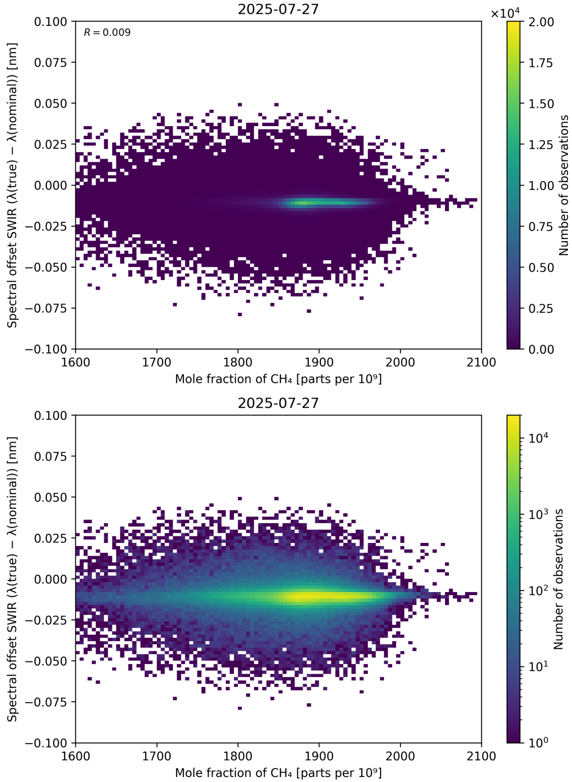
Figure 86: Scatter density plot of “Mole fraction of \text{CH}_4 ” against “Spectral offset SWIR ( \lambda_{\text{true}} - \lambda_{\text{nominal}} )” for 2025-07-26 to 2025-07-28.
