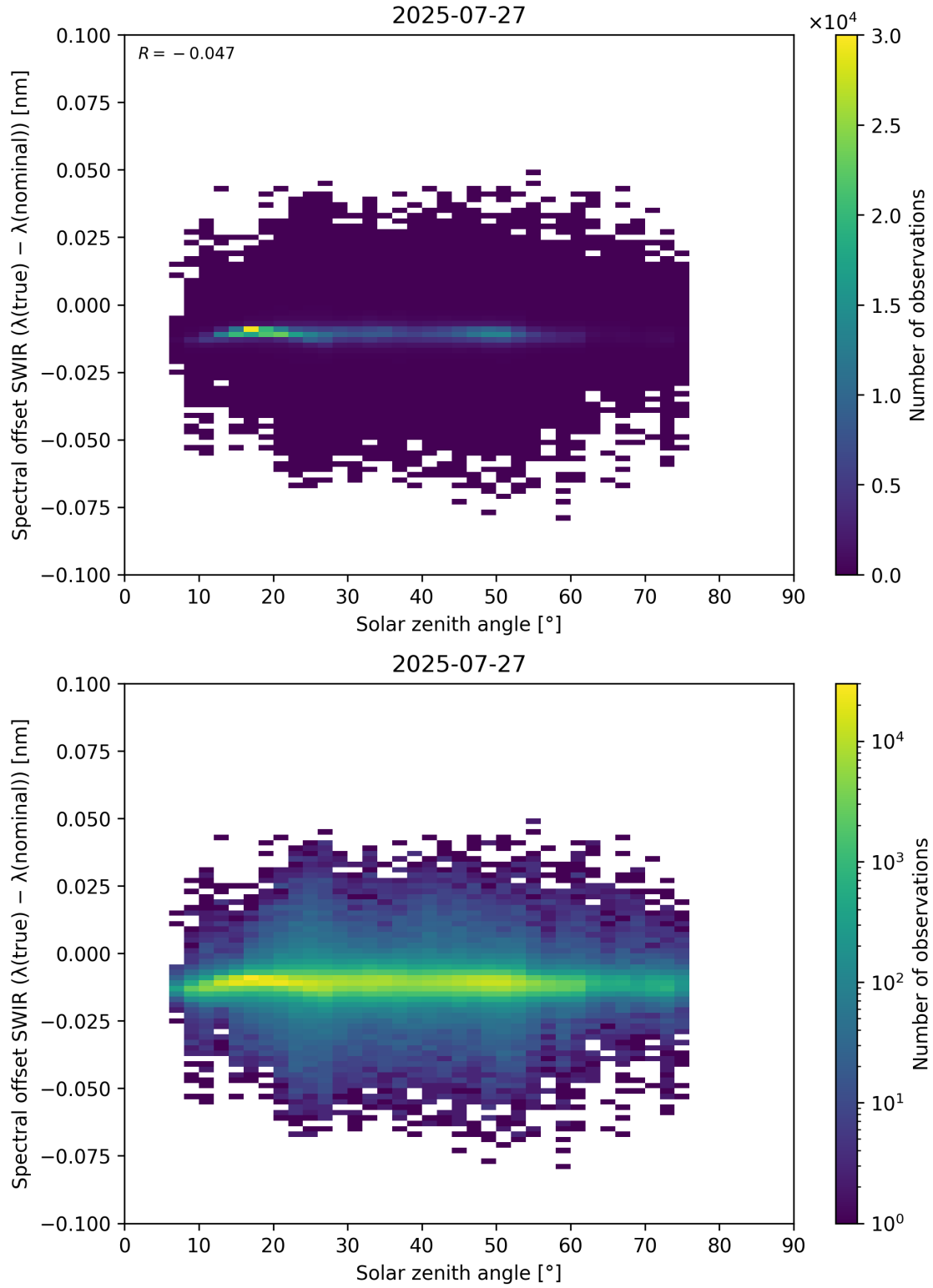
Figure 104: Scatter density plot of “Solar zenith angle” against “Spectral offset SWIR ( \lambda_{\text{true}} - \lambda_{\text{nominal}} )” for 2025-07-26 to 2025-07-28.
