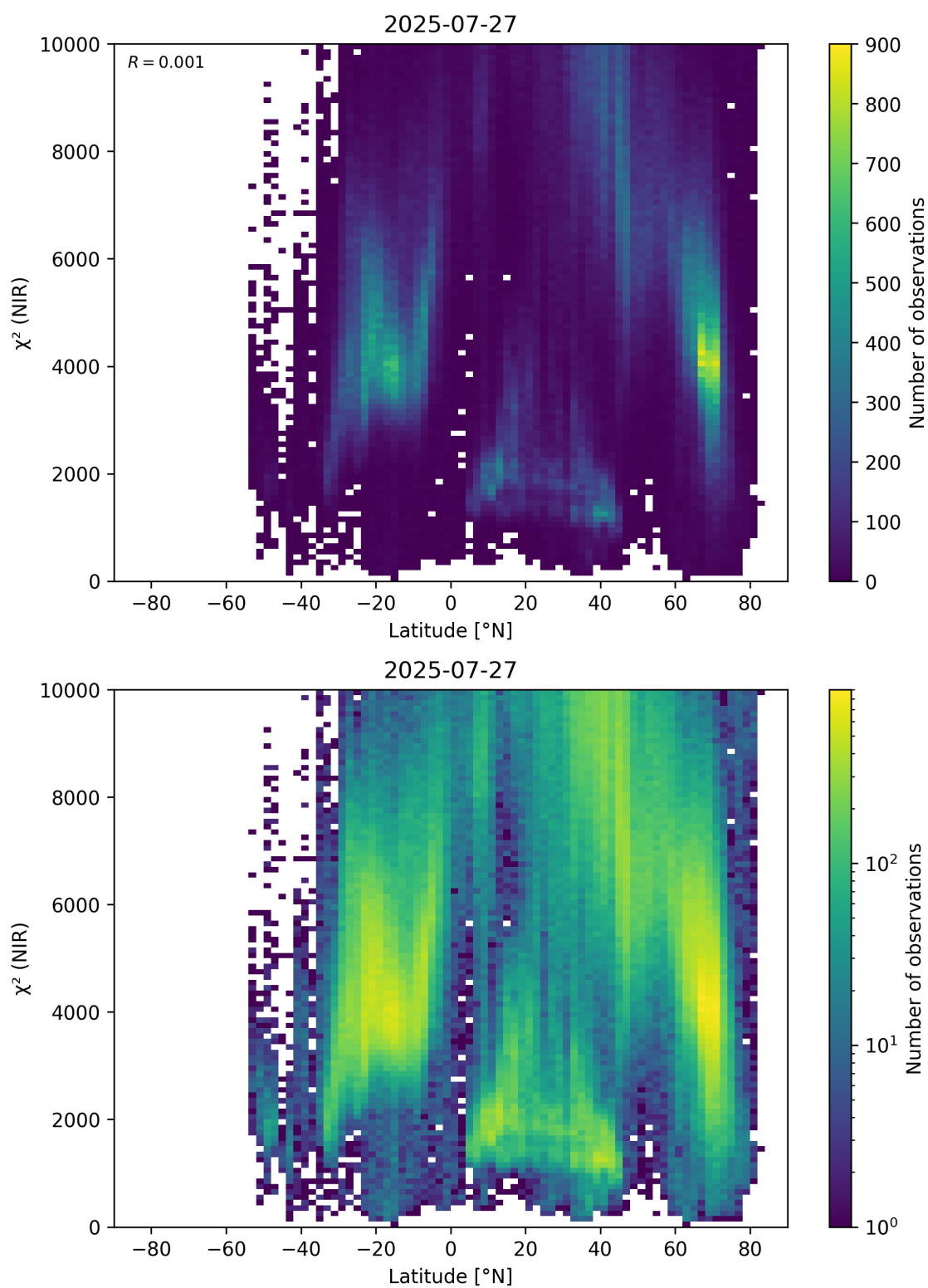
Figure 53: Scatter density plot of “Latitude” against “ \chi^2 (NIR)” for 2025-07-26 to 2025-07-28.
