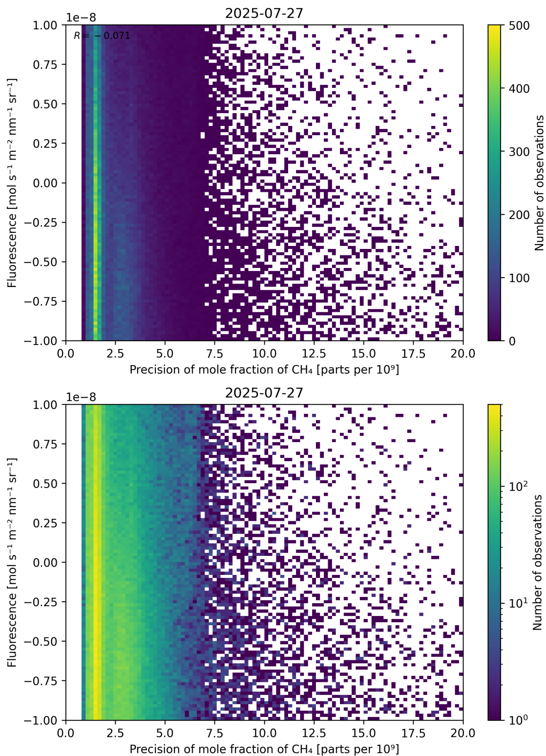
Figure 81: Scatter density plot of “Precision of mole fraction of CH 4 ” against “Fluorescence” for 2025-07-26 to 2025-07-28.
