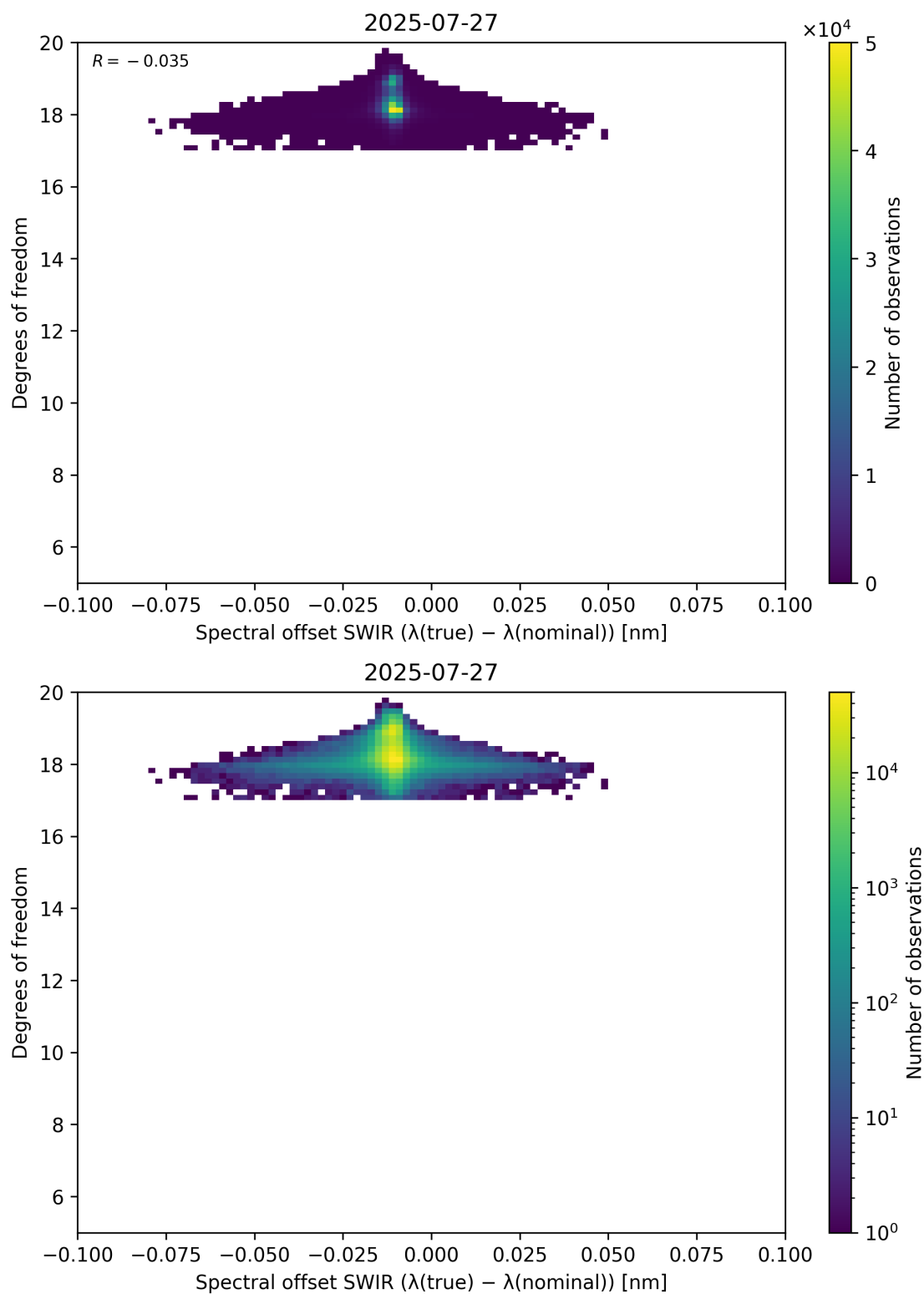
Figure 119: Scatter density plot of “Spectral offset SWIR ( \lambda_{\text{true}} - \lambda_{\text{nominal}} )” against “Degrees of freedom” for 2025-07-26 to 2025-07-28.
