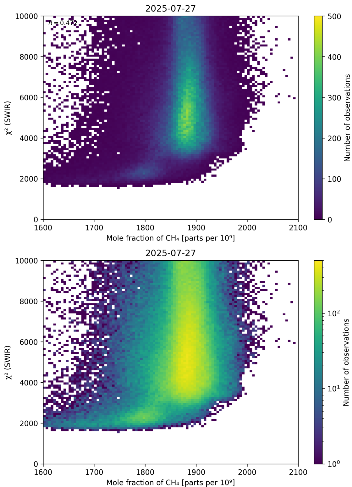
Figure 71: Scatter density plot of “Mole fraction of \text{CH}_4 ” against “ \chi^2 (SWIR)” for 2025-07-26 to 2025-07-28.
