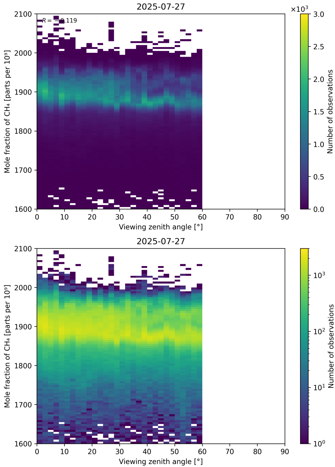
Figure 110: Scatter density plot of “Viewing zenith angle” against “Mole fraction of CH 4 ” for 2025-07-26 to 2025-07-28.
