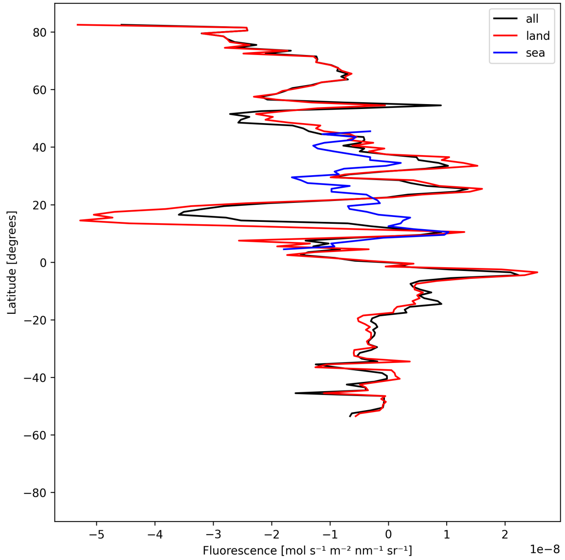
Figure 21: Zonal average of “Fluorescence” for 2025-07-26 to 2025-07-28.
