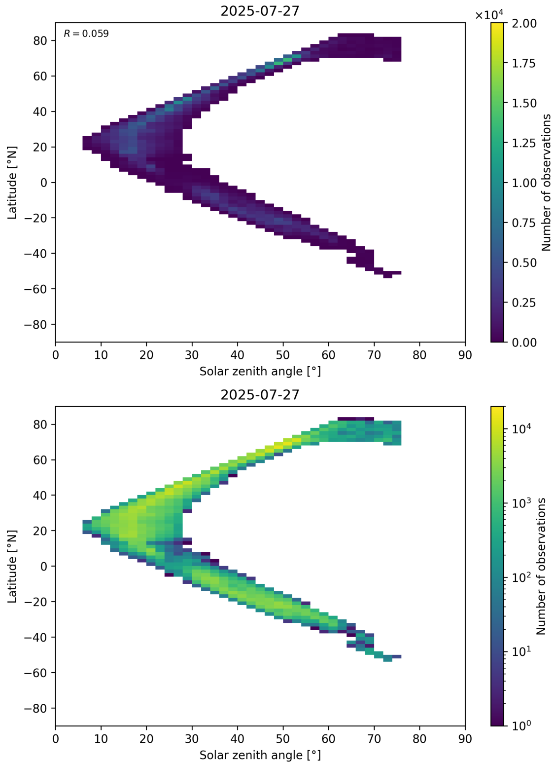
Figure 98: Scatter density plot of “Solar zenith angle” against “Latitude” for 2025-07-26 to 2025-07-28.
