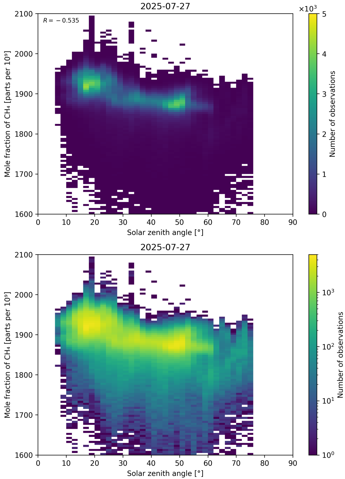
Figure 99: Scatter density plot of “Solar zenith angle” against “Mole fraction of CH 4 ” for 2025-07-26 to 2025-07-28.
