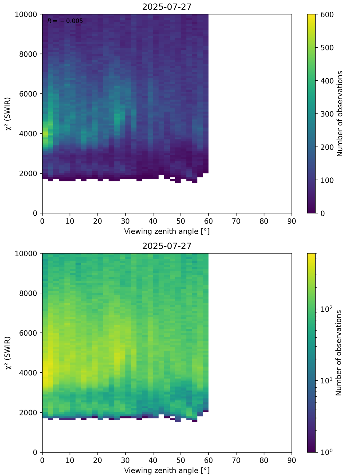
Figure 106: Scatter density plot of “Viewing zenith angle” against “ \chi^2 (SWIR)” for 2025-07-26 to 2025-07-28.
