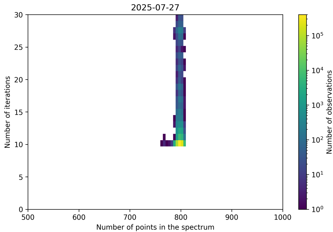
Figure 92: Scatter density plot of “Number of points in the spectrum” against “Number of iterations” for 2025-07-26 to 2025-07-28.
