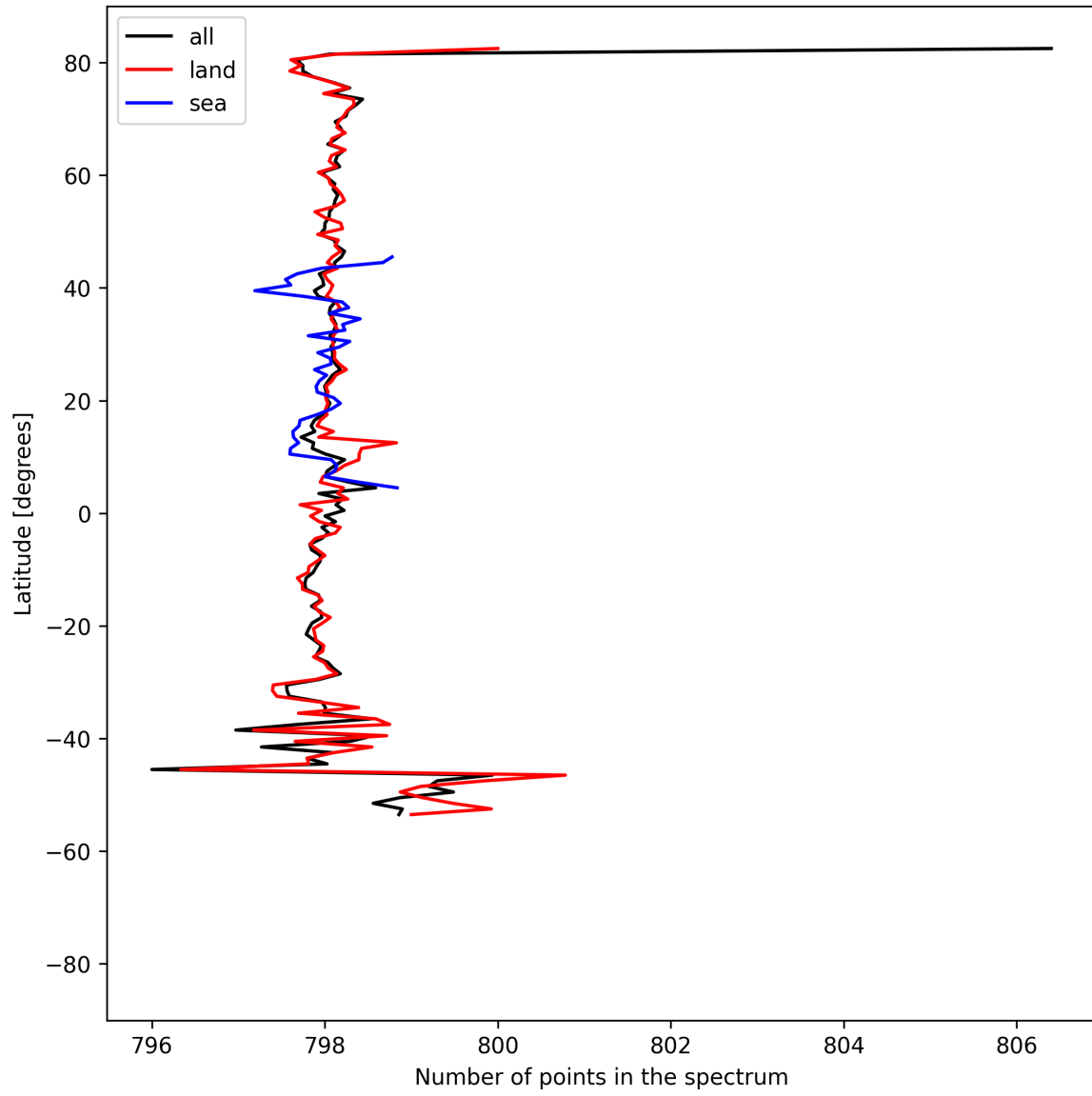
Figure 15: Zonal average of “Number of points in the spectrum” for 2025-07-26 to 2025-07-28.
