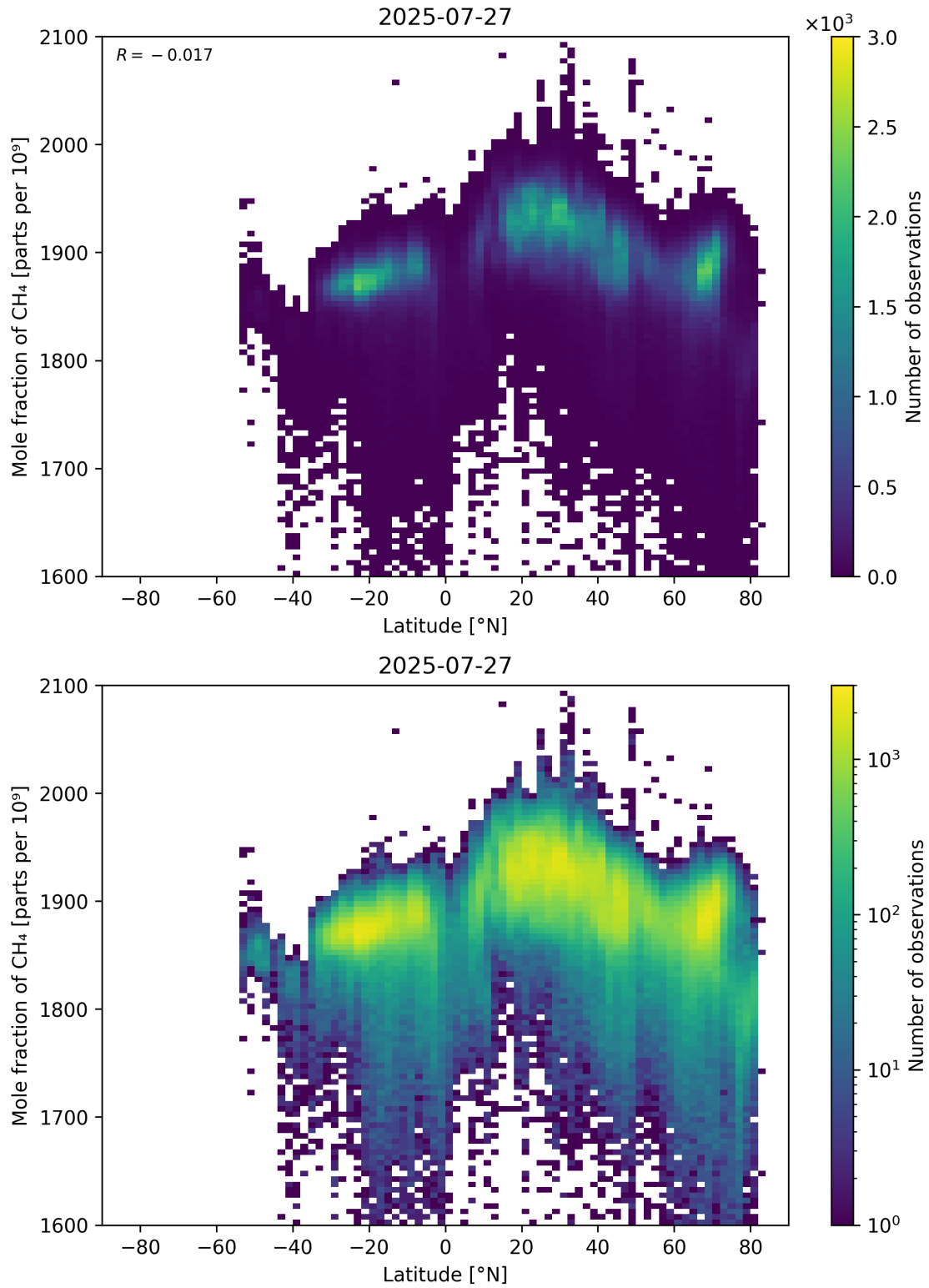
Figure 57: Scatter density plot of “Latitude” against “Mole fraction of CH 4 ” for 2025-07-26 to 2025-07-28.
