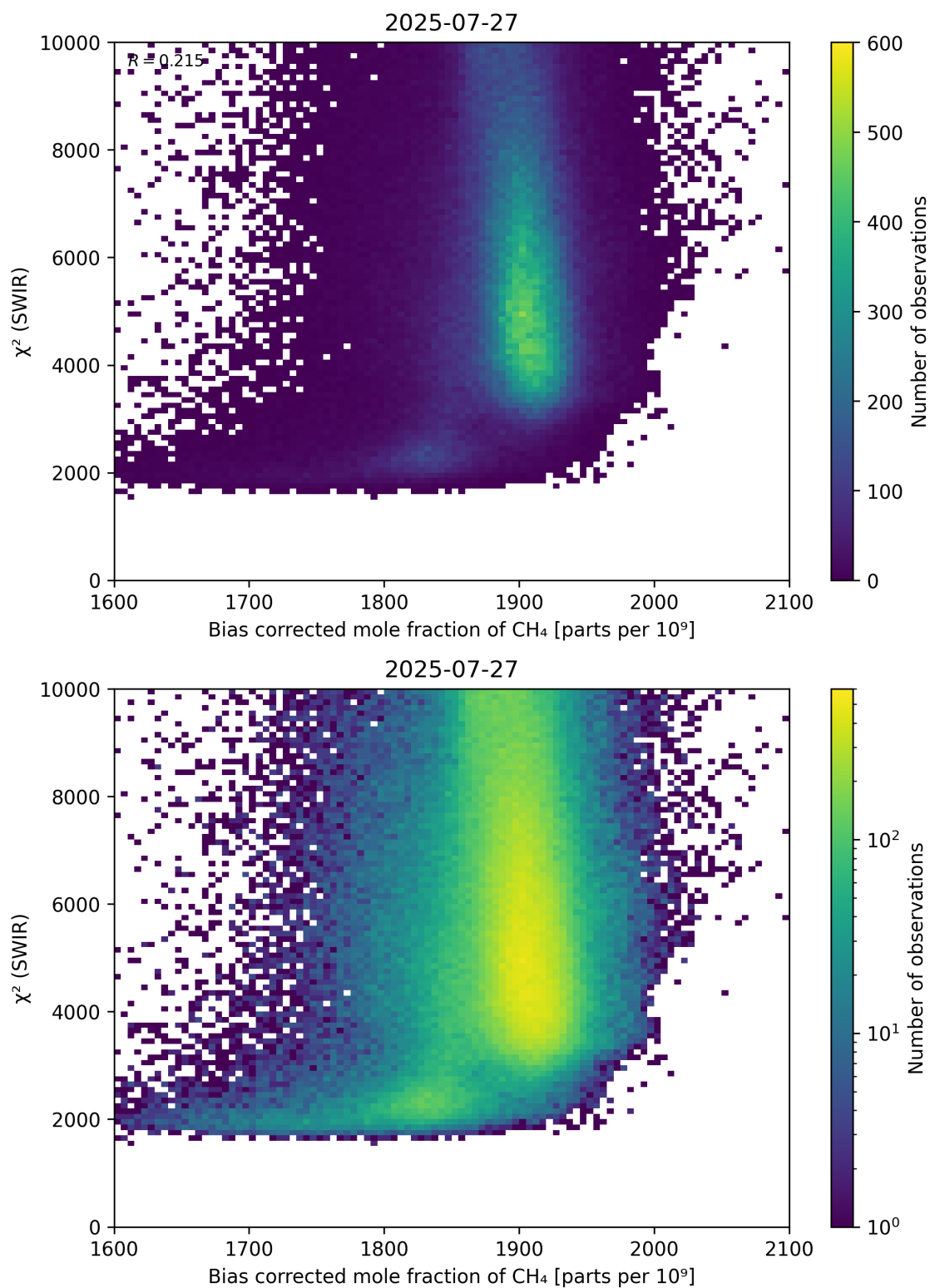
Figure 64: Scatter density plot of “Bias corrected mole fraction of \text{CH}_4 ” against “ \chi^2 (SWIR)” for 2025-07-26 to 2025-07-28.
