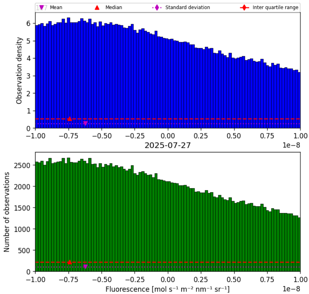
Figure 32: Histogram of “Fluorescence” for 2025-07-26 to 2025-07-28
