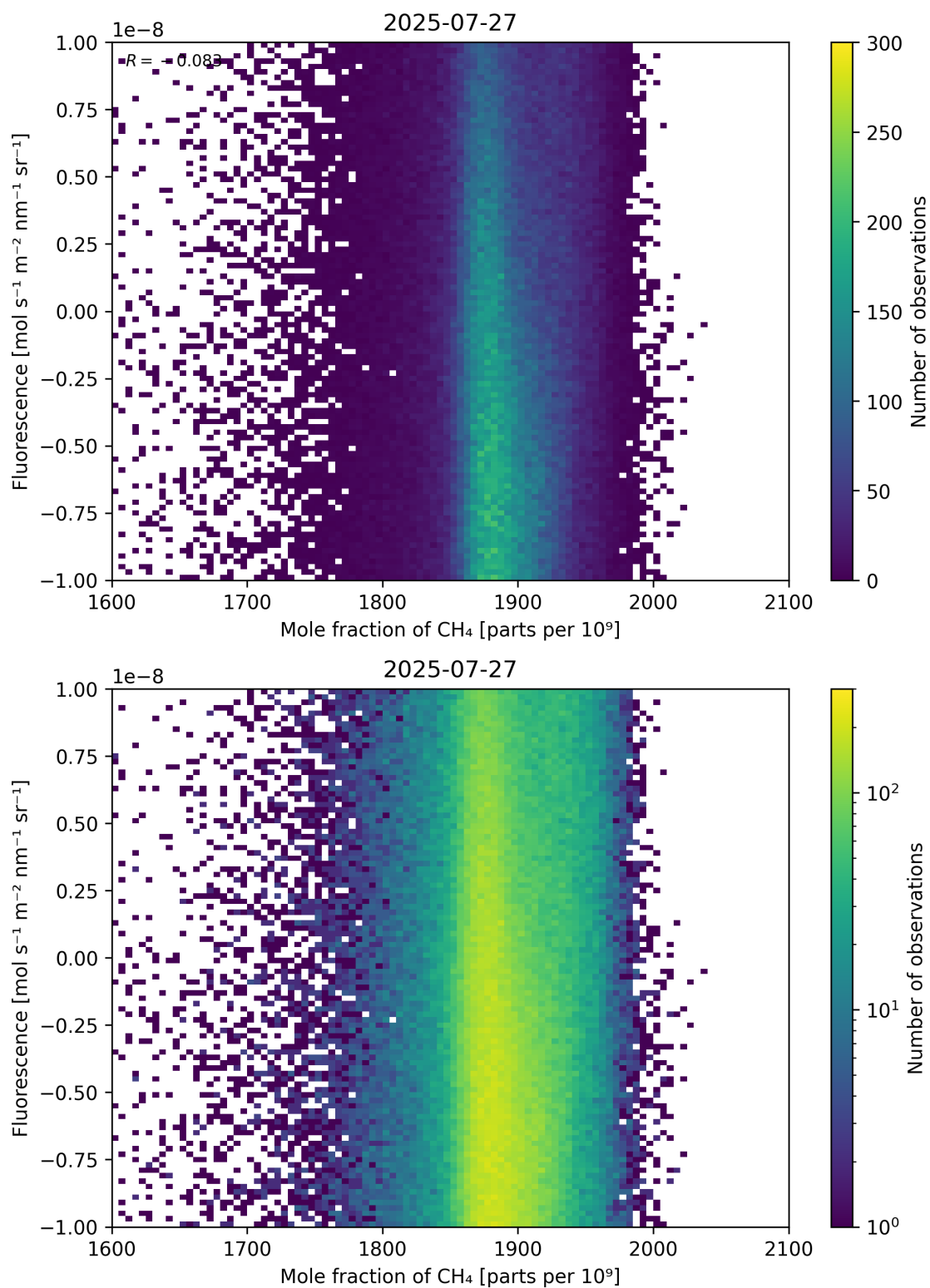
Figure 73: Scatter density plot of “Mole fraction of CH 4 ” against “Fluorescence” for 2025-07-26 to 2025-07-28.
