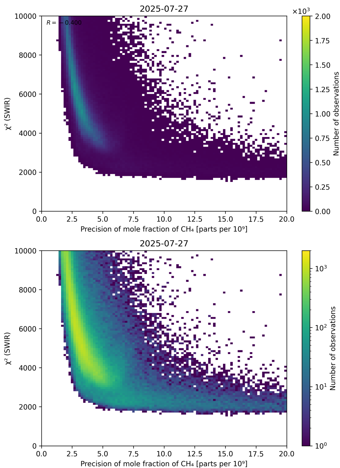
Figure 79: Scatter density plot of “Precision of mole fraction of CH 4 ” against “ \chi^2 (SWIR)” for 2025-07-26 to 2025-07-28.
