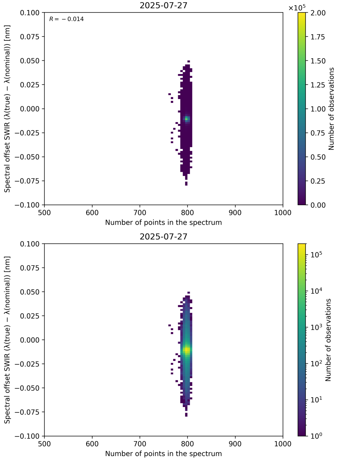
Figure 93: Scatter density plot of “Number of points in the spectrum” against “Spectral offset SWIR ( \lambda_{\text{true}} - \lambda_{\text{nominal}} )” for 2025-07-26 to 2025-07-28.
