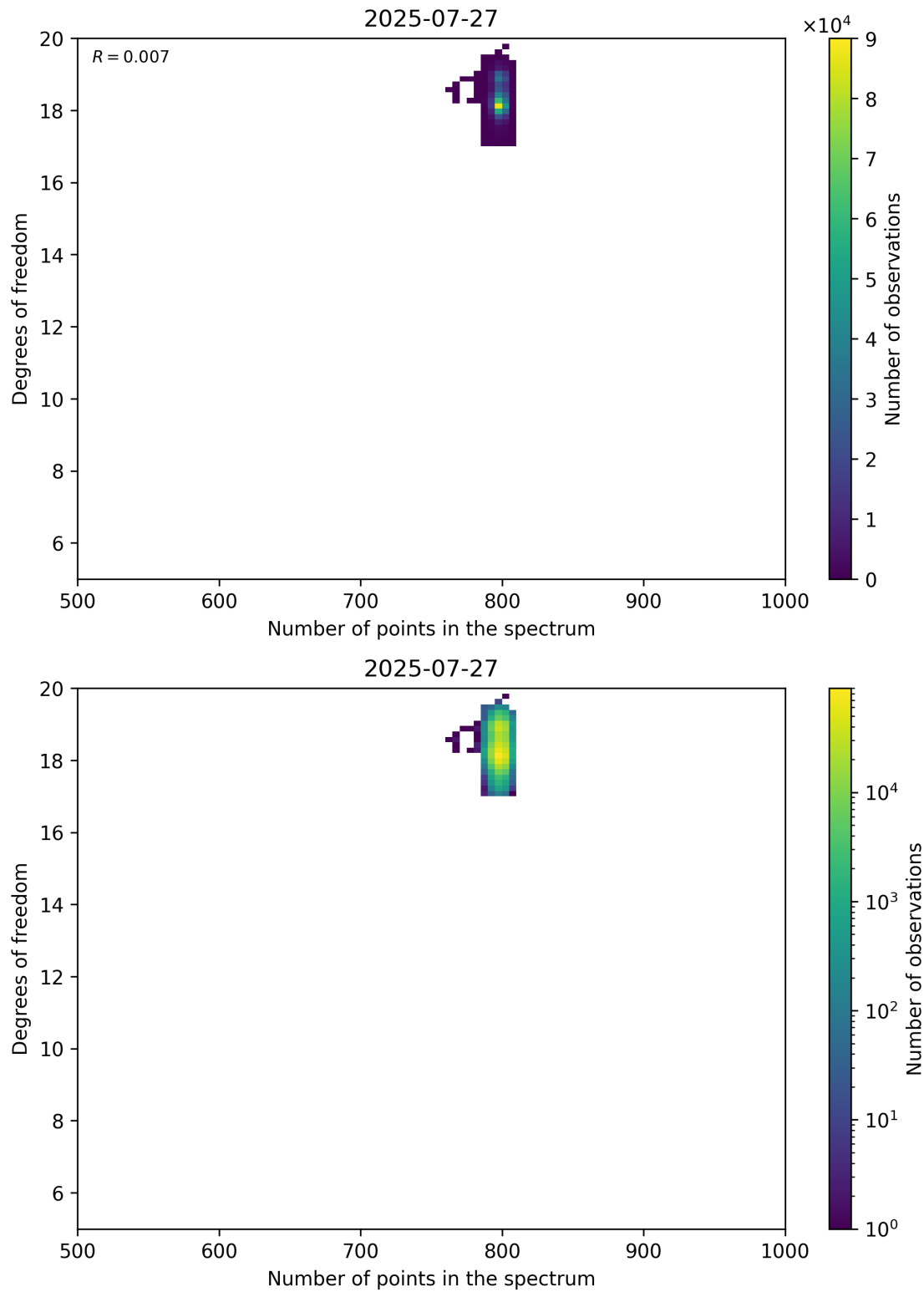
Figure 90: Scatter density plot of “Number of points in the spectrum” against “Degrees of freedom” for 2025-07-26 to 2025-07-28.
