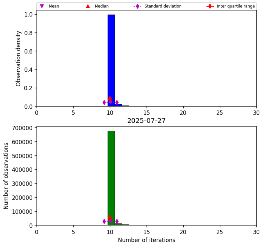
Figure 31: Histogram of “Number of iterations” for 2025-07-26 to 2025-07-28
