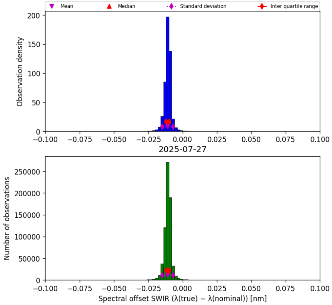
Figure 27: Histogram of “Spectral offset SWIR ( \lambda_{\text{true}} - \lambda_{\text{nominal}} )” for 2025-07-26 to 2025-07-28
