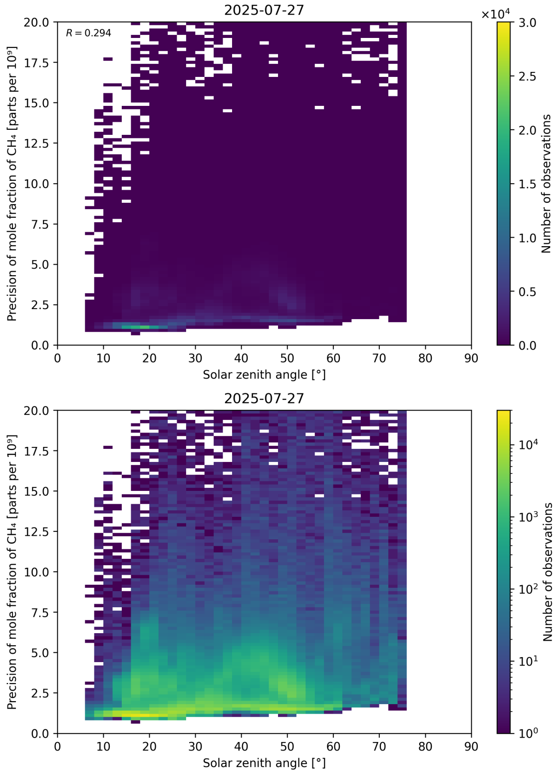
Figure 101: Scatter density plot of “Solar zenith angle” against “Precision of mole fraction of \text{CH}_4 ” for 2025-07-26 to 2025-07-28.
