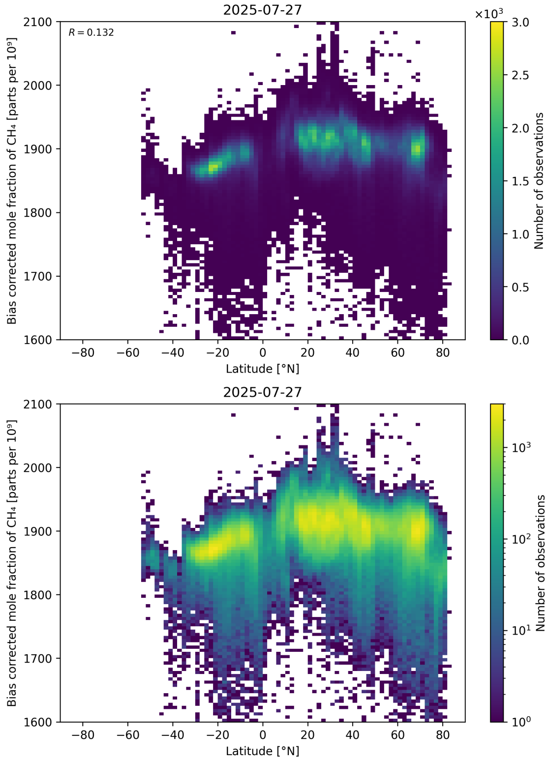
Figure 58: Scatter density plot of “Latitude” against “Bias corrected mole fraction of CH 4 ” for 2025-07-26 to 2025-07-28.
