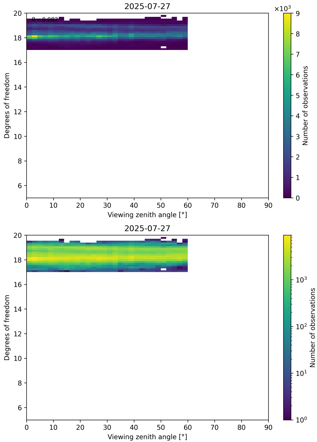
Figure 107: Scatter density plot of “Viewing zenith angle” against “Degrees of freedom” for 2025-07-26 to 2025-07-28.
