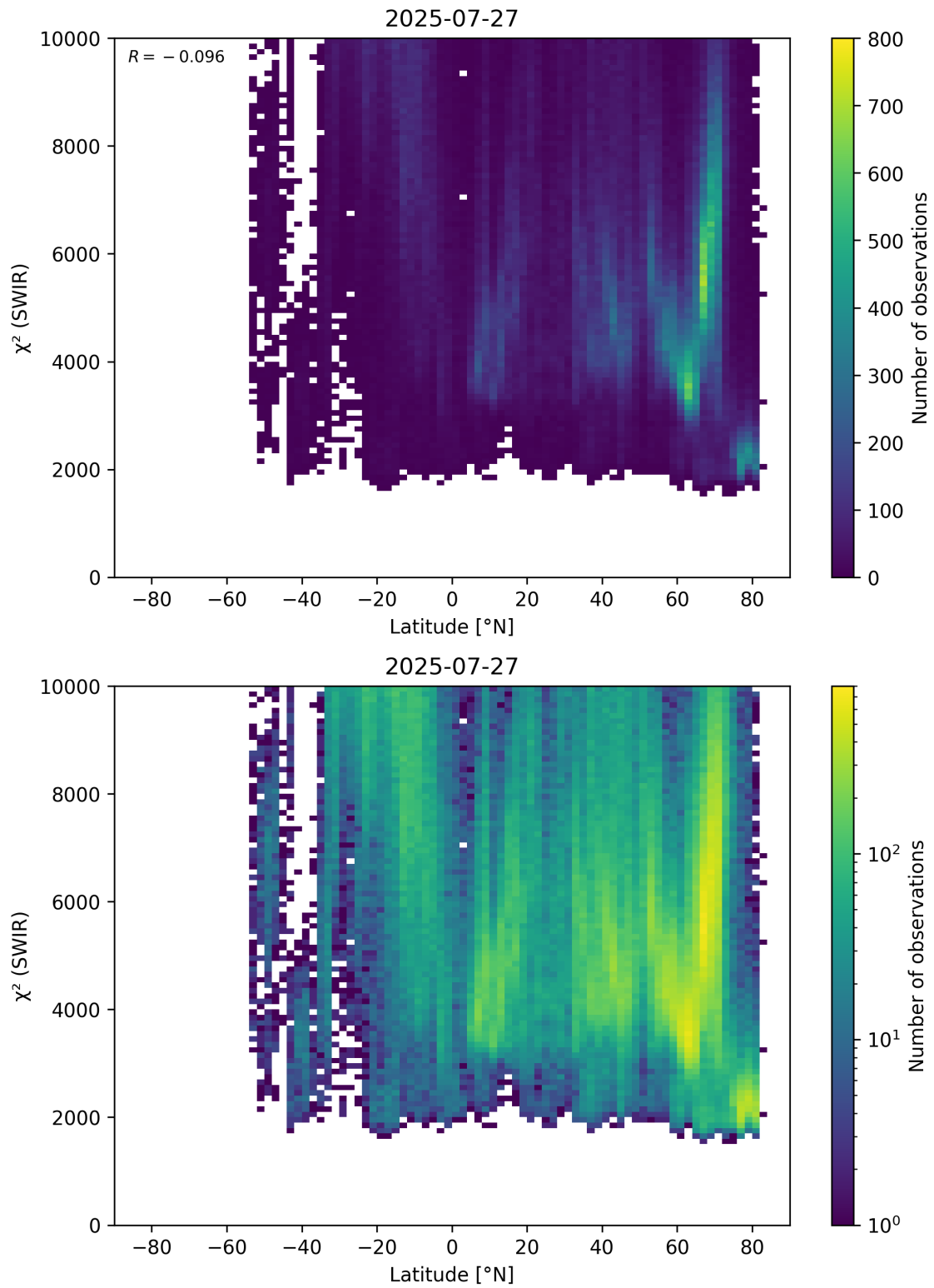
Figure 54: Scatter density plot of “Latitude” against “ \chi^2 (SWIR)” for 2025-07-26 to 2025-07-28.
