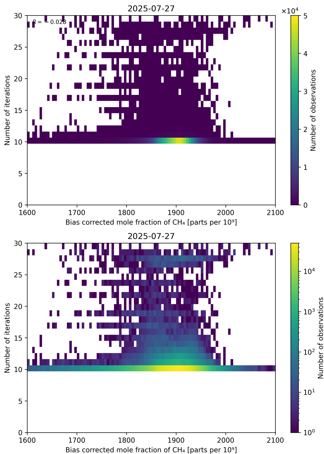
Figure 67: Scatter density plot of “Bias corrected mole fraction of CH 4 ” against “Number of iterations” for 2025-07-26 to 2025-07-28.
