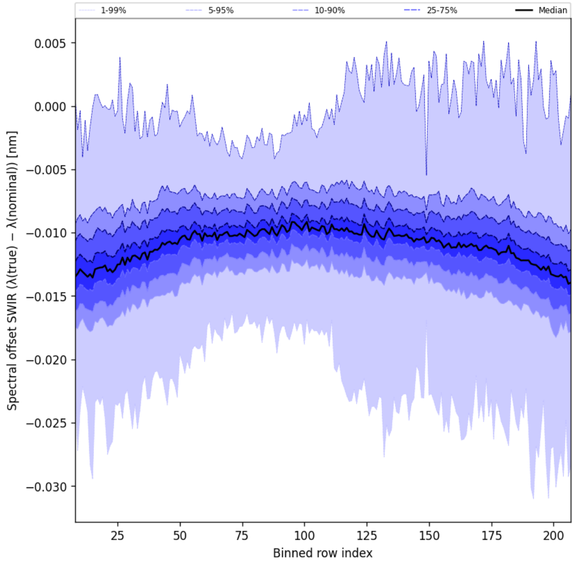
Figure 38: Along track statistics of “Spectral offset SWIR ( \lambda_{\text{true}} - \lambda_{\text{nominal}} )” for 2025-07-26 to 2025-07-28
