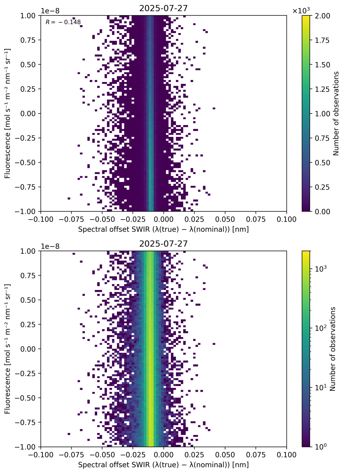
Figure 120: Scatter density plot of “Spectral offset SWIR ( \lambda_{\text{true}} - \lambda_{\text{nominal}} )” against “Fluorescence” for 2025-07-26 to 2025-07-28.
