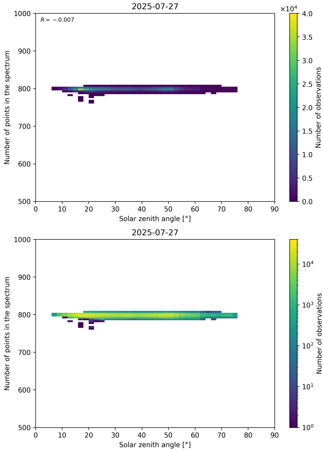
Figure 103: Scatter density plot of “Solar zenith angle” against “Number of points in the spectrum” for 2025-07-26 to 2025-07-28.
