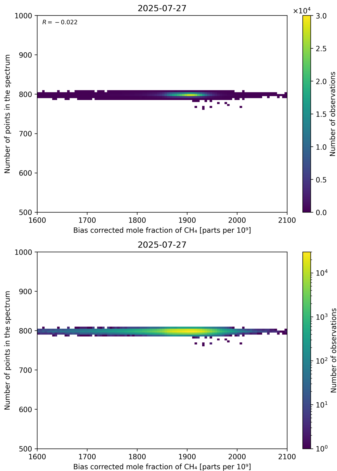
Figure 68: Scatter density plot of “Bias corrected mole fraction of CH 4 ” against “Number of points in the spectrum” for 2025-07-26 to 2025-07-28.
