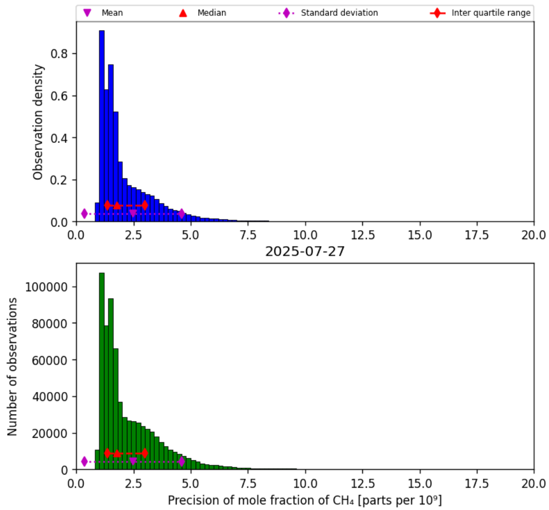
Figure 24: Histogram of “Precision of mole fraction of CH 4 ” for 2025-07-26 to 2025-07-28
