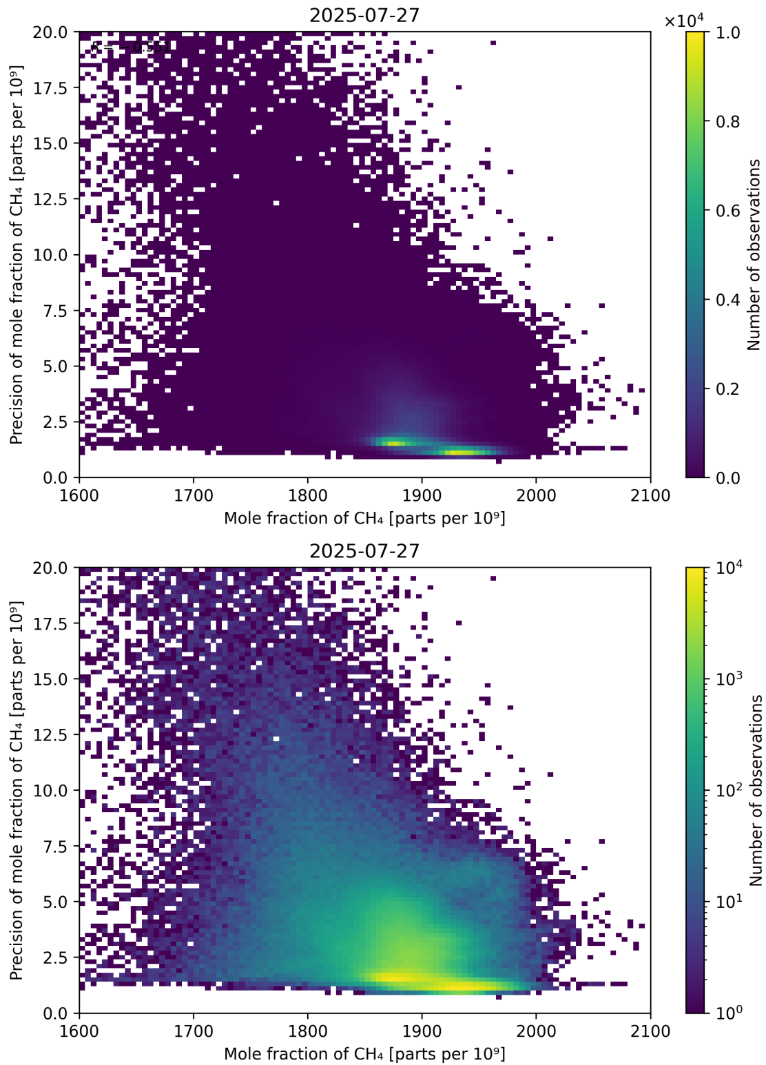
Figure 75: Scatter density plot of “Mole fraction of CH 4 ” against “Precision of mole fraction of CH 4 ” for 2025-07-26 to 2025-07-28.
