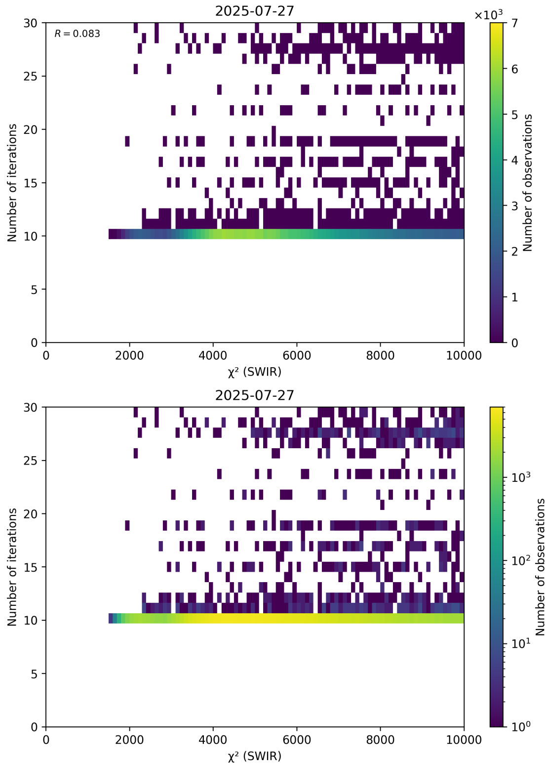
Figure 50: Scatter density plot of “ \chi^2 (SWIR)” against “Number of iterations” for 2025-07-26 to 2025-07-28.
