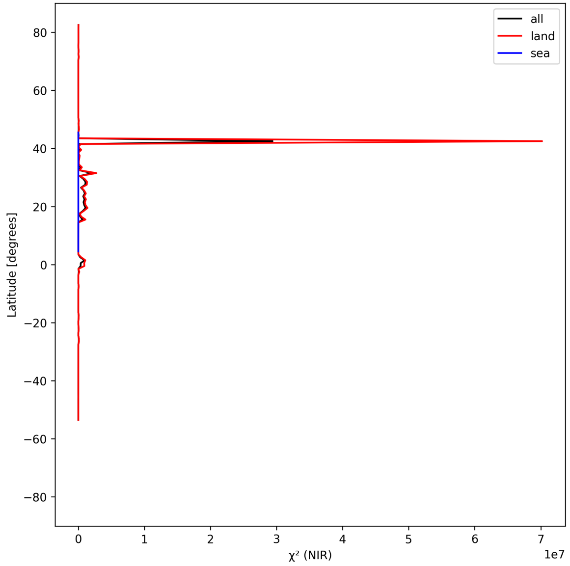
Figure 18: Zonal average of “ \chi^2 (NIR)” for 2025-07-26 to 2025-07-28.
