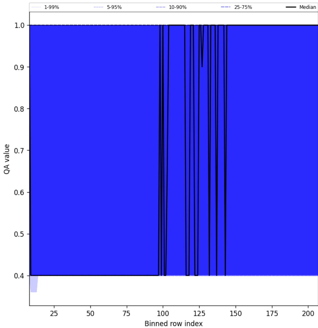
Figure 33: Along track statistics of “QA value” for 2025-07-26 to 2025-07-28
