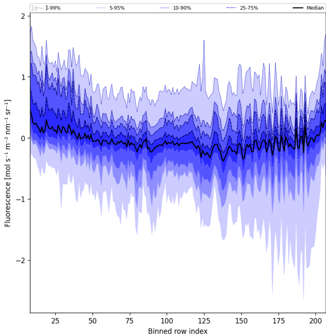
Figure 43: Along track statistics of “Fluorescence” for 2025-07-26 to 2025-07-28
