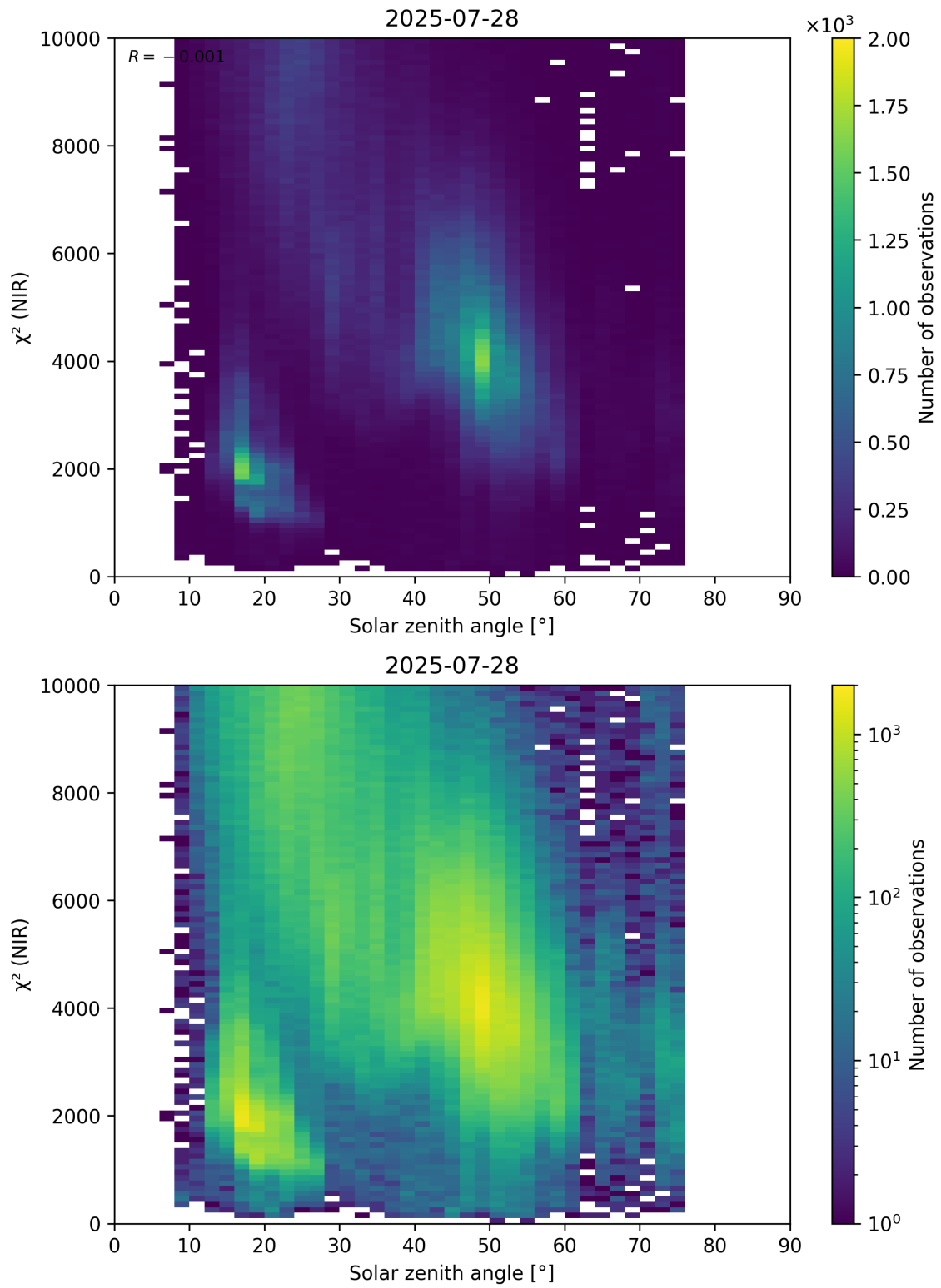
Figure 94: Scatter density plot of “Solar zenith angle” against “ \chi^2 (NIR)” for 2025-07-27 to 2025-07-29.
