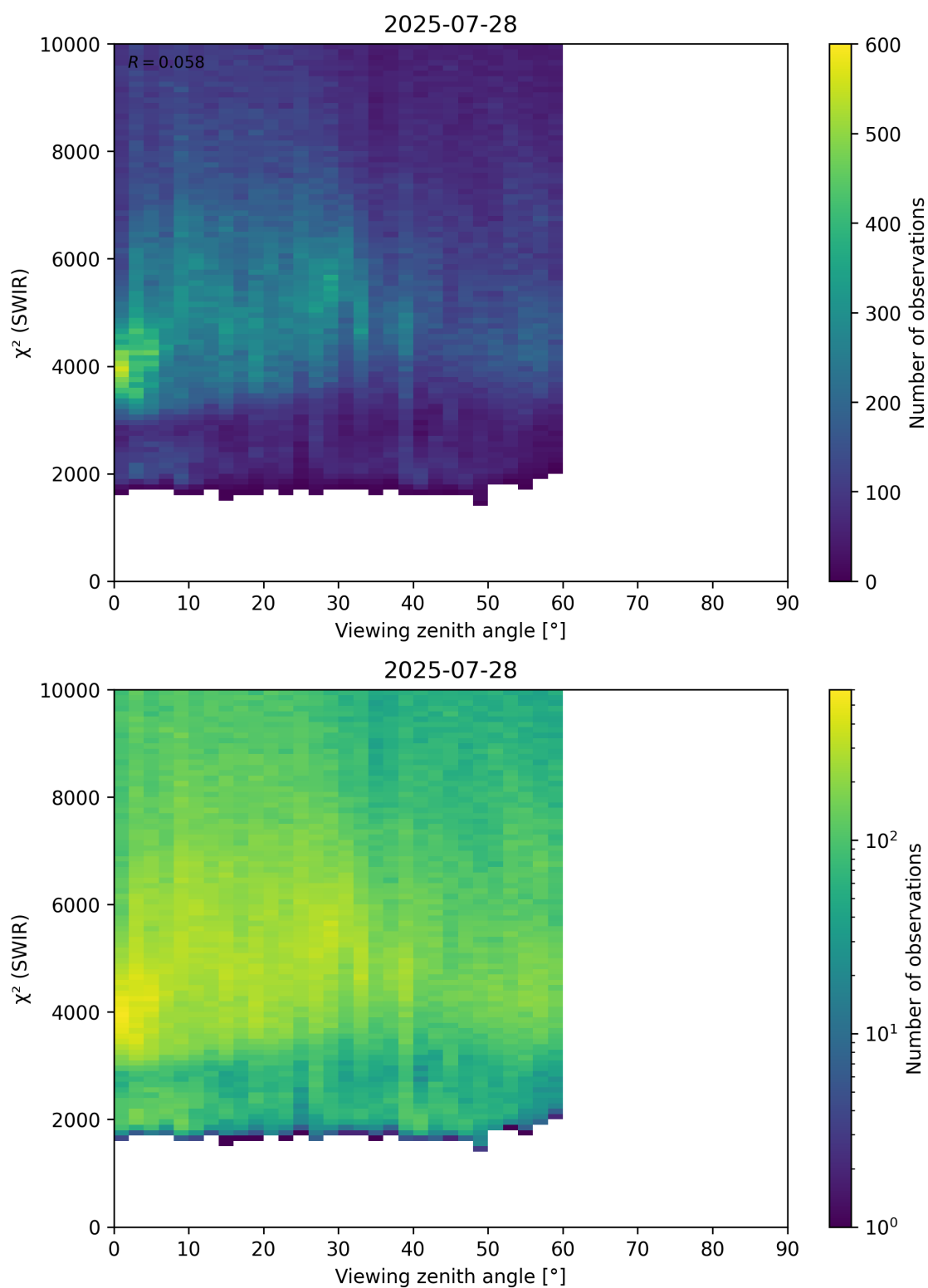
Figure 106: Scatter density plot of “Viewing zenith angle” against “ \chi^2 (SWIR)” for 2025-07-27 to 2025-07-29.
