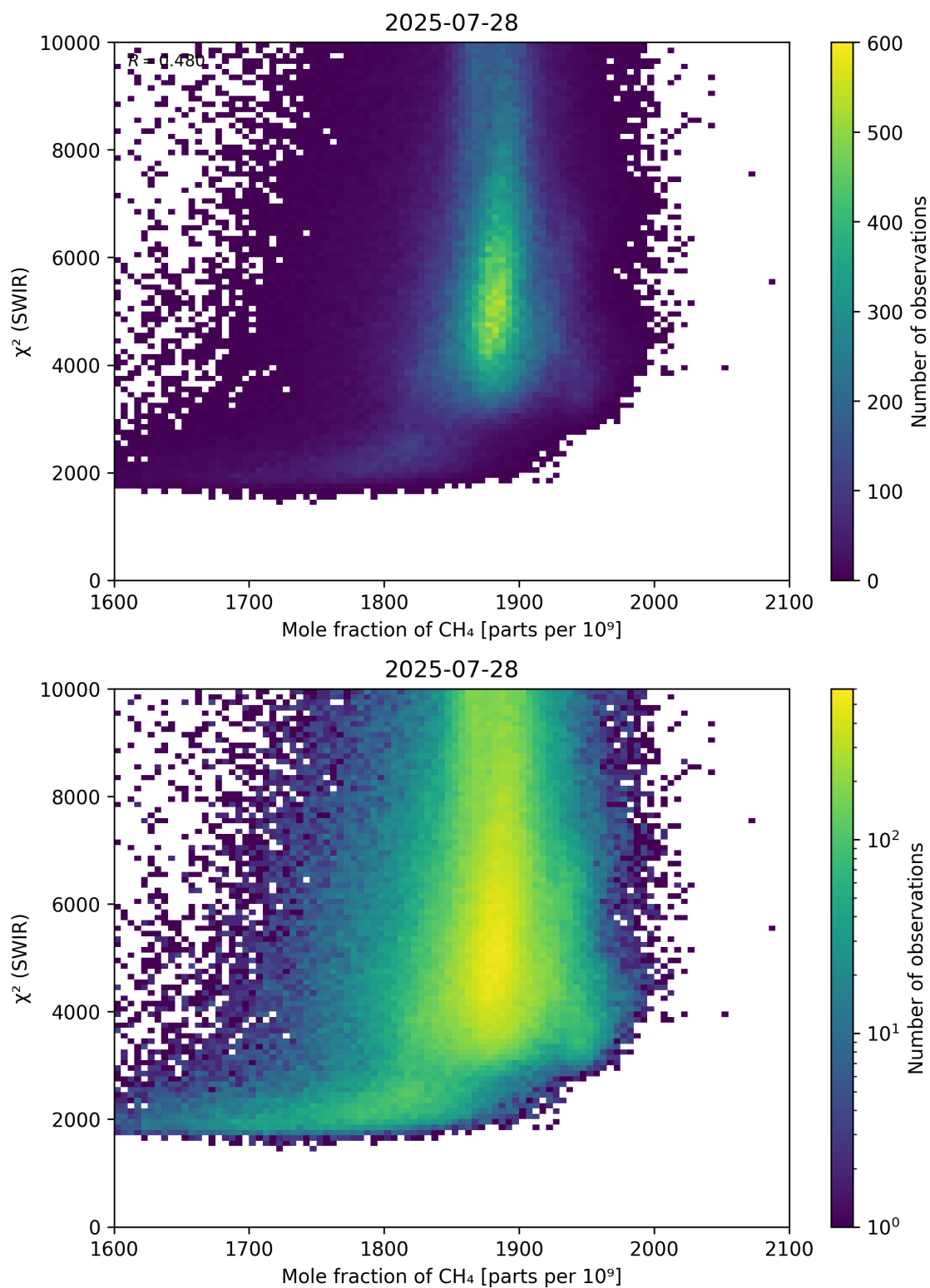
Figure 71: Scatter density plot of “Mole fraction of \text{CH}_4 ” against “ \chi^2 (SWIR)” for 2025-07-27 to 2025-07-29.
