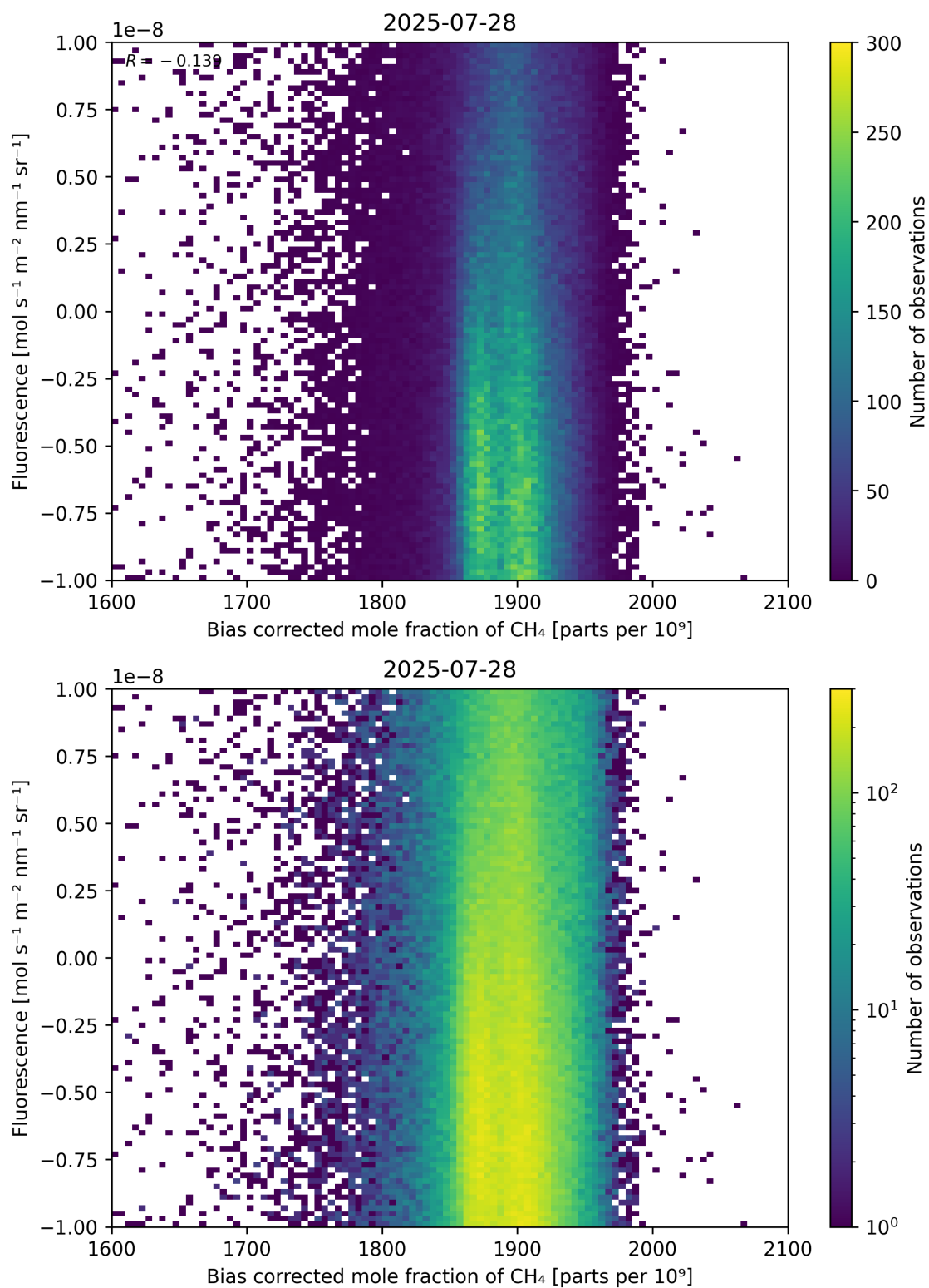
Figure 66: Scatter density plot of “Bias corrected mole fraction of \text{CH}_4 ” against “Fluorescence” for 2025-07-27 to 2025-07-29.
