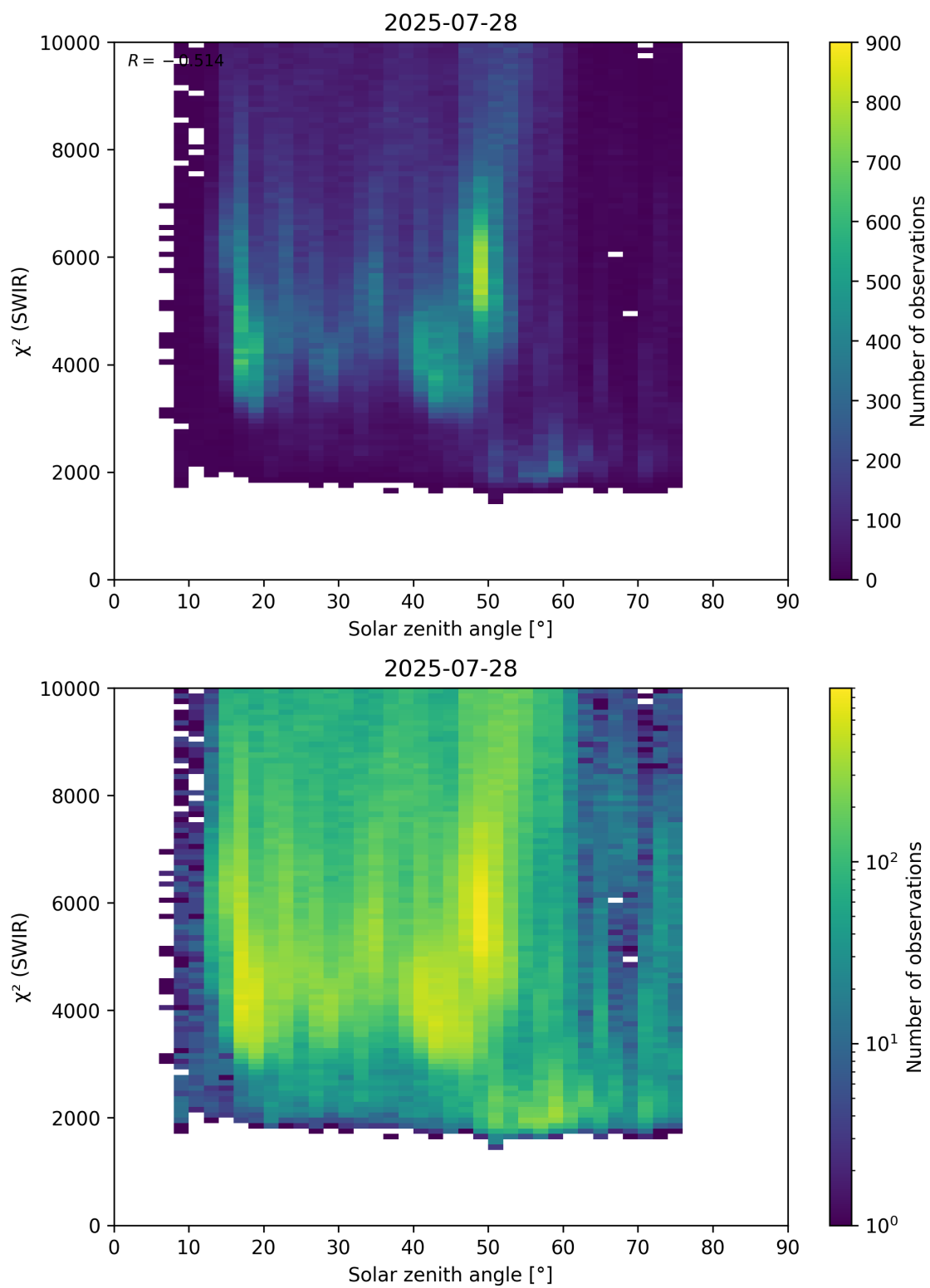
Figure 95: Scatter density plot of “Solar zenith angle” against “ \chi^2 (SWIR)” for 2025-07-27 to 2025-07-29.
