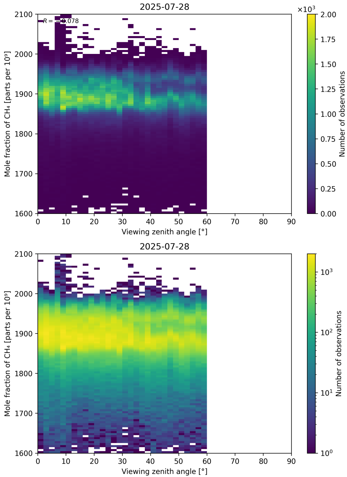
Figure 110: Scatter density plot of “Viewing zenith angle” against “Mole fraction of CH 4 ” for 2025-07-27 to 2025-07-29.
