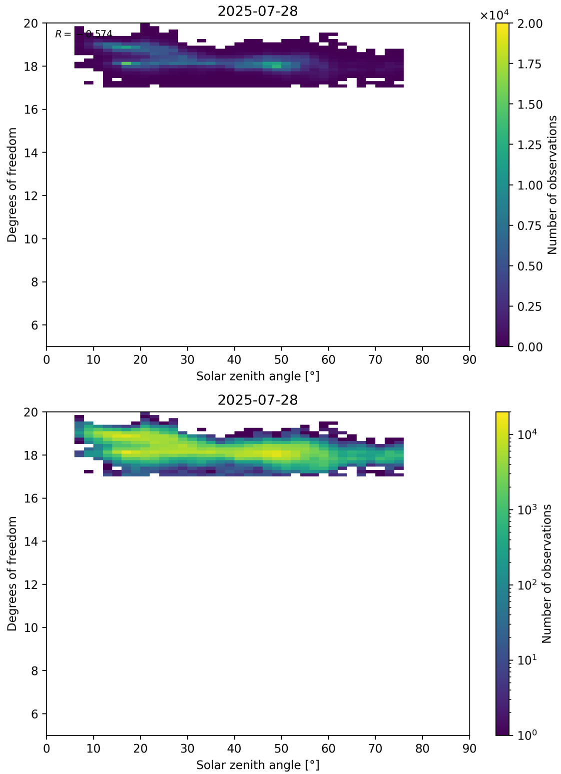
Figure 96: Scatter density plot of “Solar zenith angle” against “Degrees of freedom” for 2025-07-27 to 2025-07-29.
