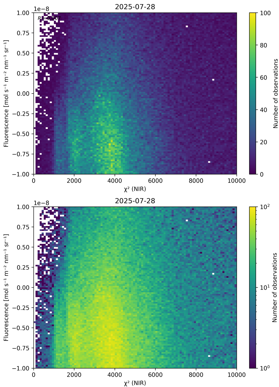
Figure 45: Scatter density plot of “ \chi^2 (NIR)” against “Fluorescence” for 2025-07-27 to 2025-07-29.
