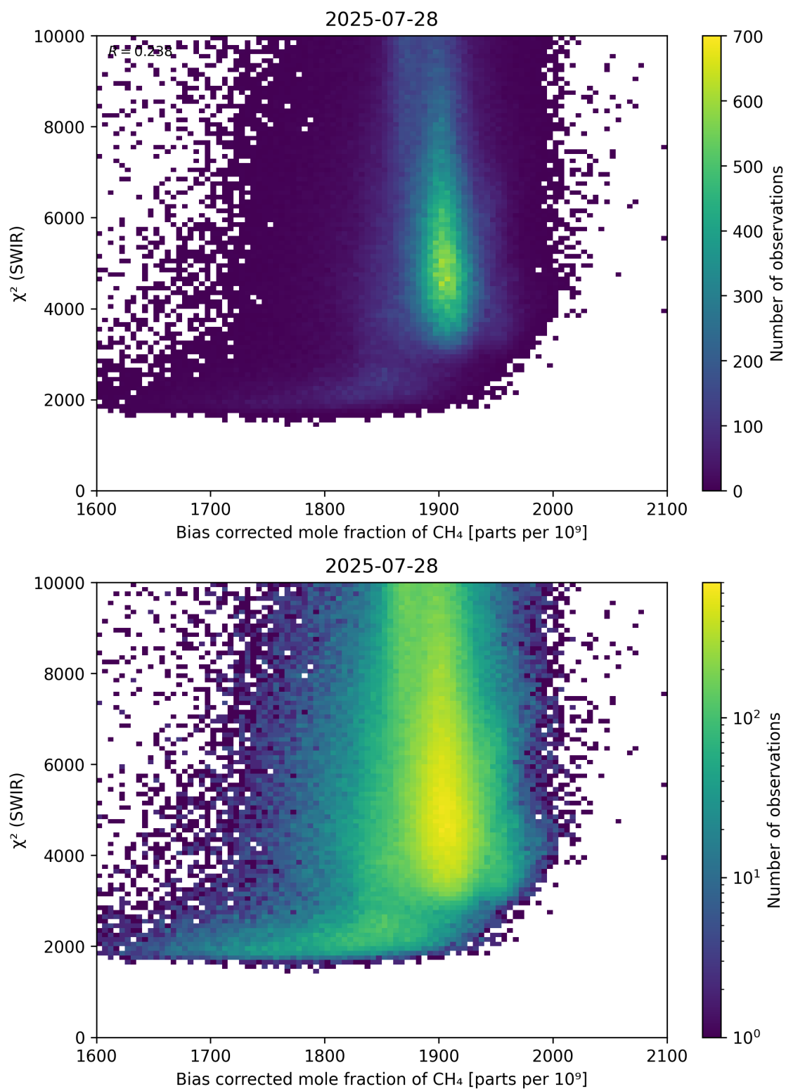
Figure 64: Scatter density plot of “Bias corrected mole fraction of \text{CH}_4 ” against “ \chi^2 (SWIR)” for 2025-07-27 to 2025-07-29.
