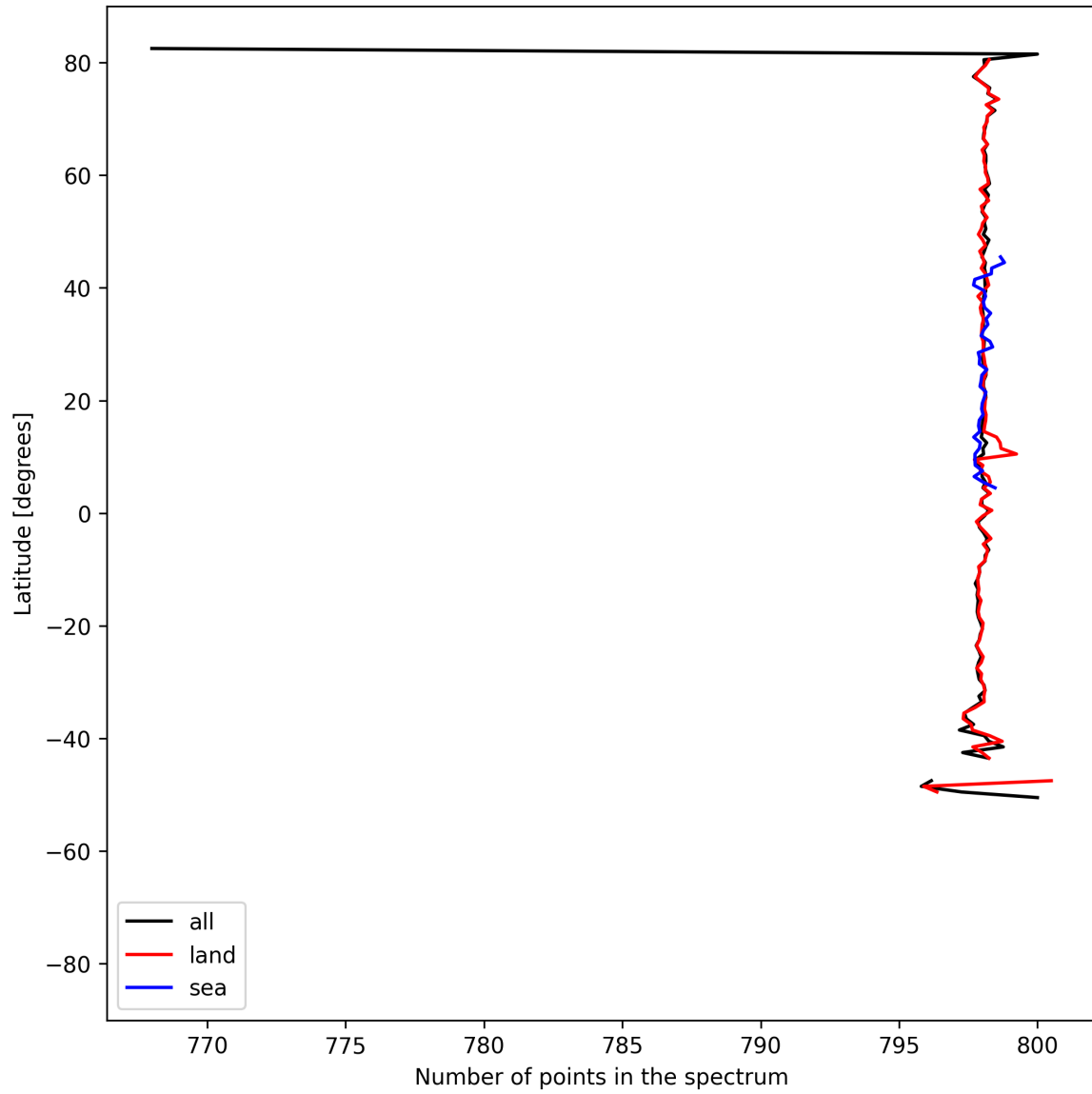
Figure 15: Zonal average of “Number of points in the spectrum” for 2025-07-27 to 2025-07-29.
