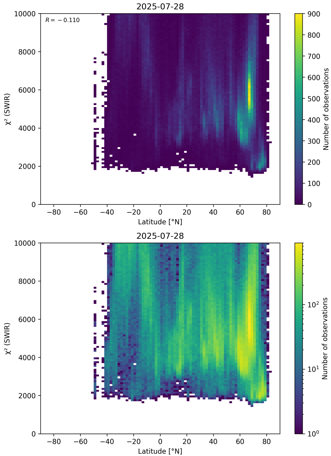
Figure 54: Scatter density plot of “Latitude” against “ \chi^2 (SWIR)” for 2025-07-27 to 2025-07-29.
