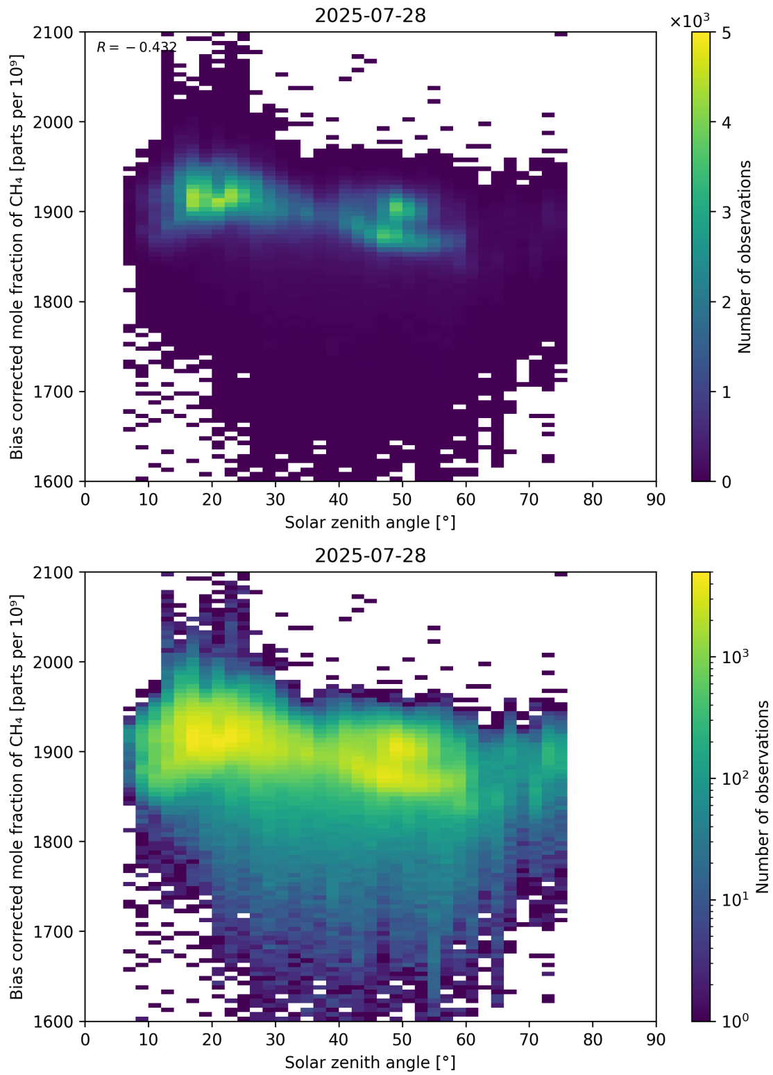
Figure 100: Scatter density plot of “Solar zenith angle” against “Bias corrected mole fraction of \text{CH}_4 ” for 2025-07-27 to 2025-07-29.
