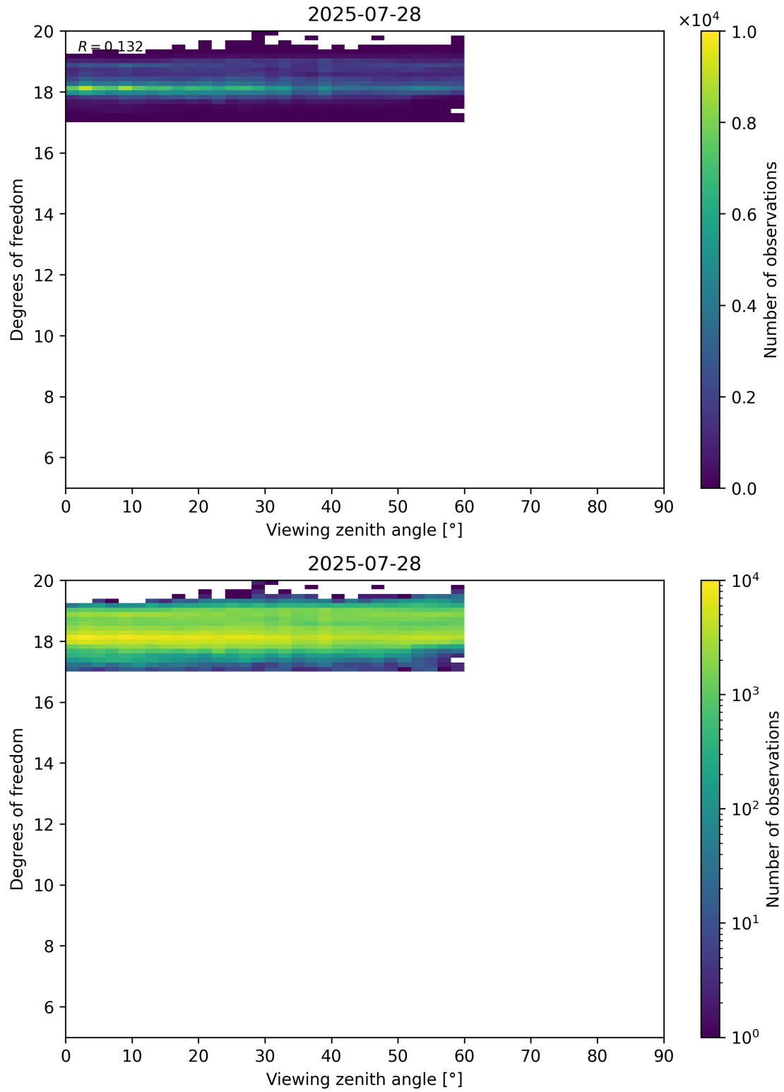
Figure 107: Scatter density plot of “Viewing zenith angle” against “Degrees of freedom” for 2025-07-27 to 2025-07-29.
