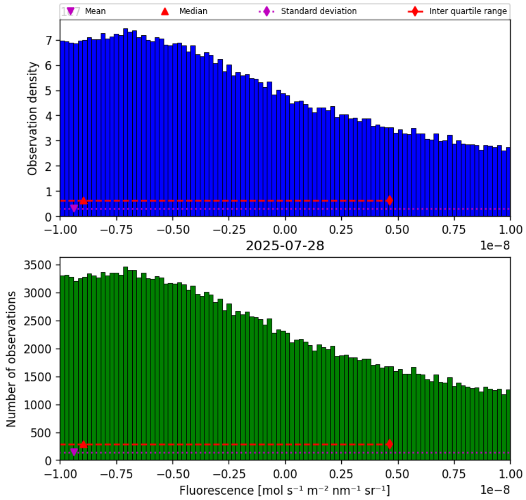
Figure 32: Histogram of “Fluorescence” for 2025-07-27 to 2025-07-29
