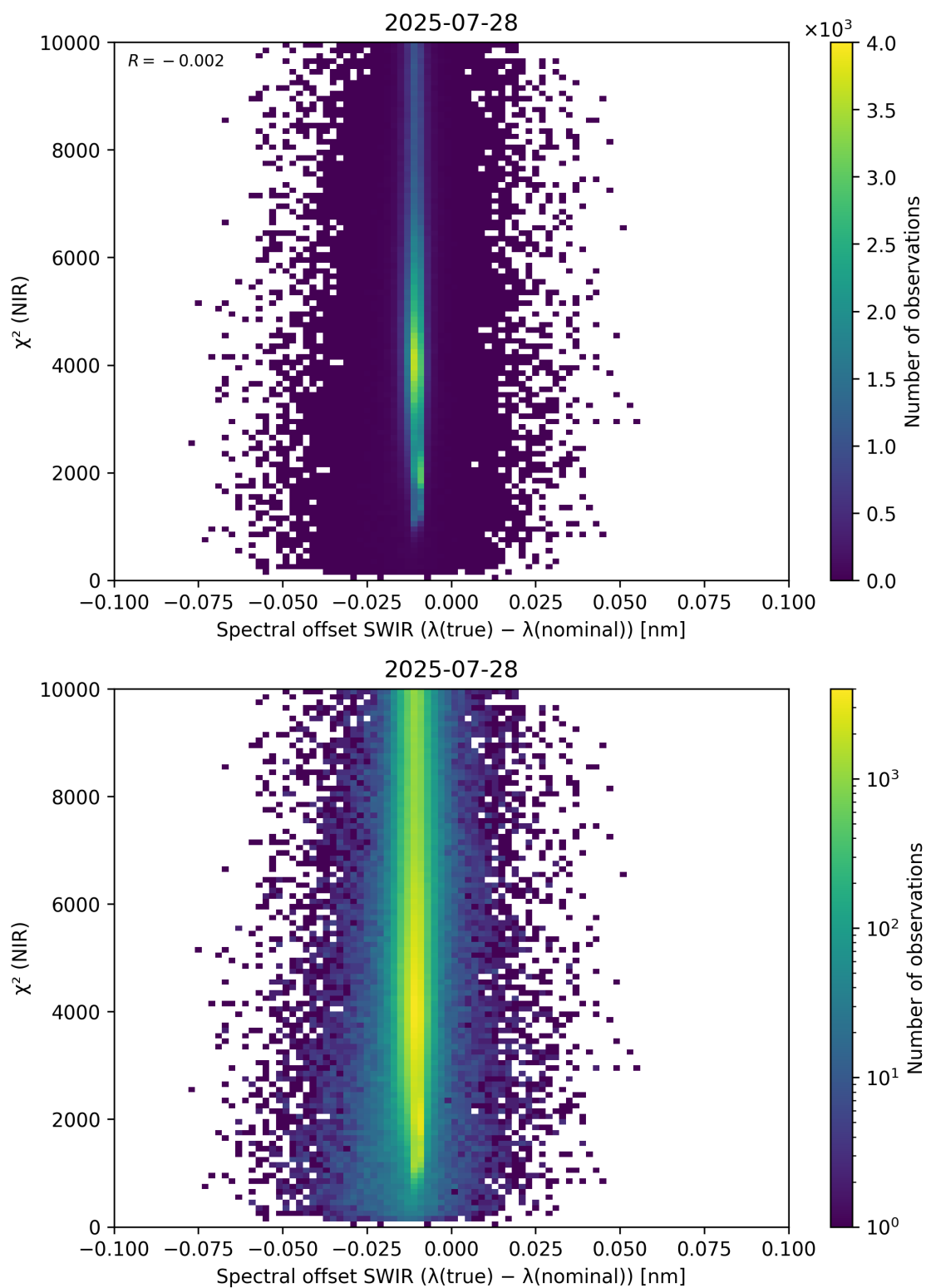
Figure 117: Scatter density plot of “Spectral offset SWIR ( \lambda_{\text{true}} - \lambda_{\text{nominal}} )” against “ \chi^2 (NIR)” for 2025-07-27 to 2025-07-29.
