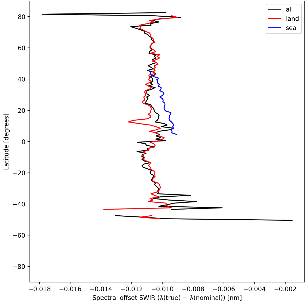
Figure 16: Zonal average of “Spectral offset SWIR ( \lambda_{\text{true}} - \lambda_{\text{nominal}} )” for 2025-07-27 to 2025-07-29.
