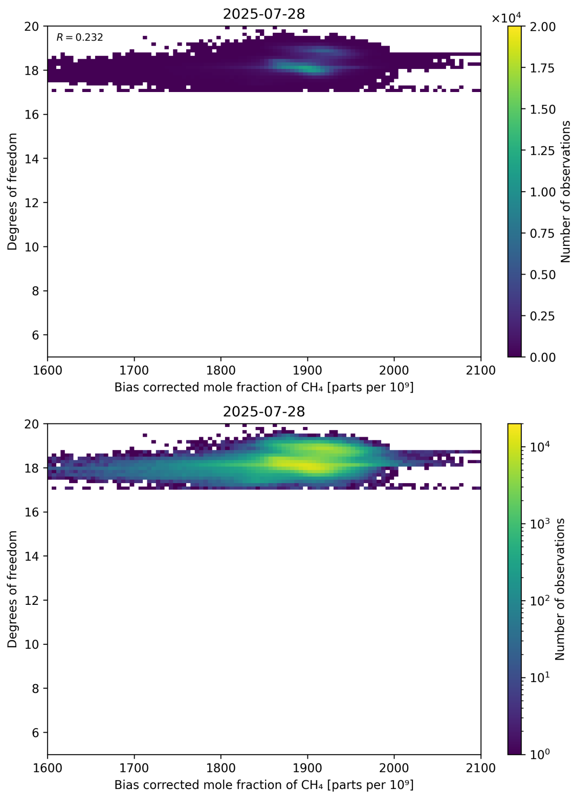
Figure 65: Scatter density plot of “Bias corrected mole fraction of CH 4 ” against “Degrees of freedom” for 2025-07-27 to 2025-07-29.
