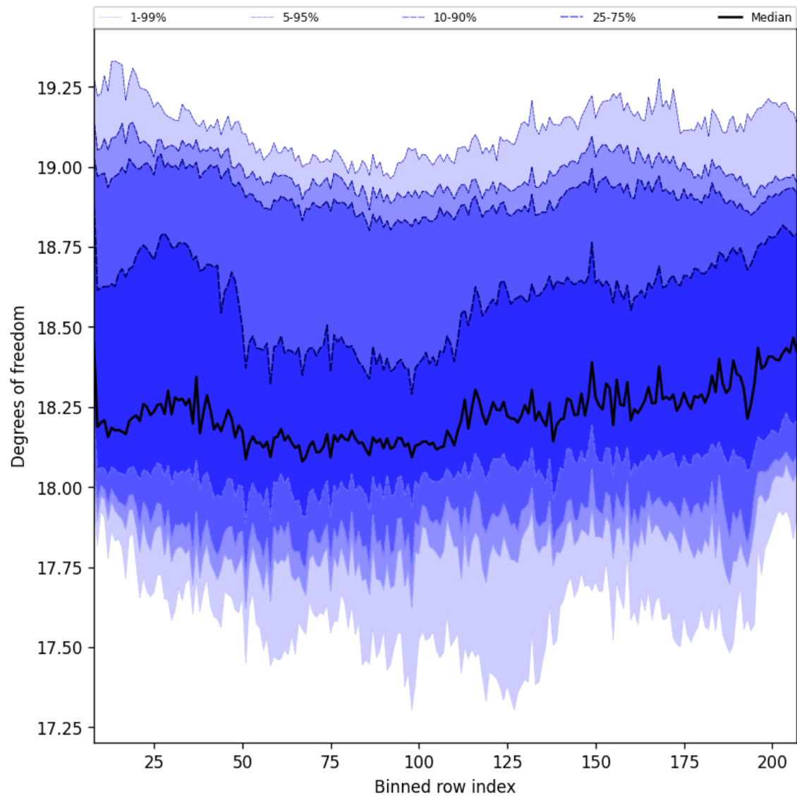
Figure 41: Along track statistics of “Degrees of freedom” for 2025-07-27 to 2025-07-29
