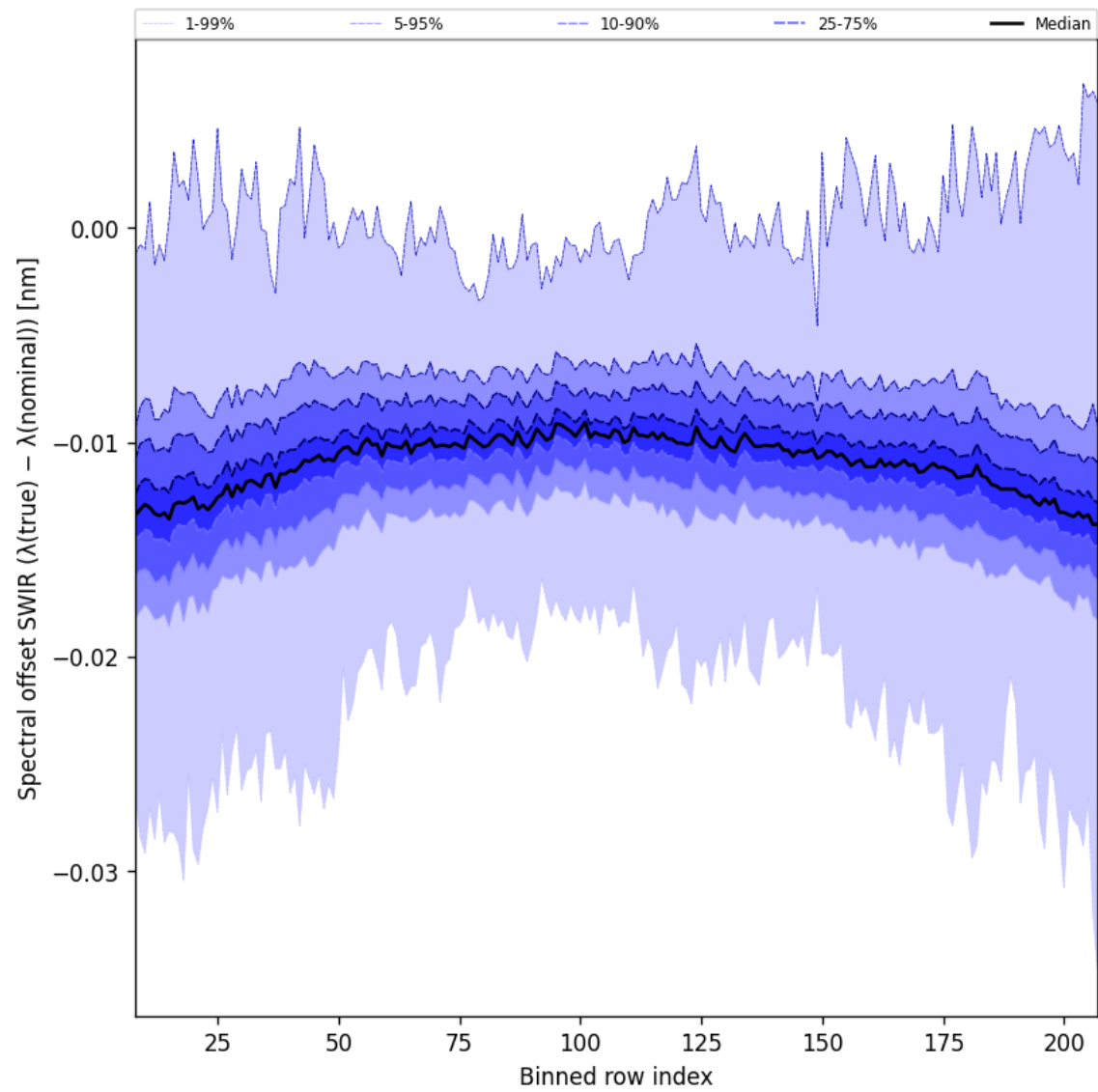
Figure 38: Along track statistics of “Spectral offset SWIR ( \lambda_{\text{true}} - \lambda_{\text{nominal}} )” for 2025-07-27 to 2025-07-29
