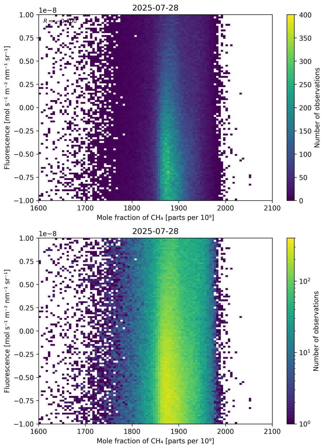
Figure 73: Scatter density plot of “Mole fraction of \text{CH}_4 ” against “Fluorescence” for 2025-07-27 to 2025-07-29.
