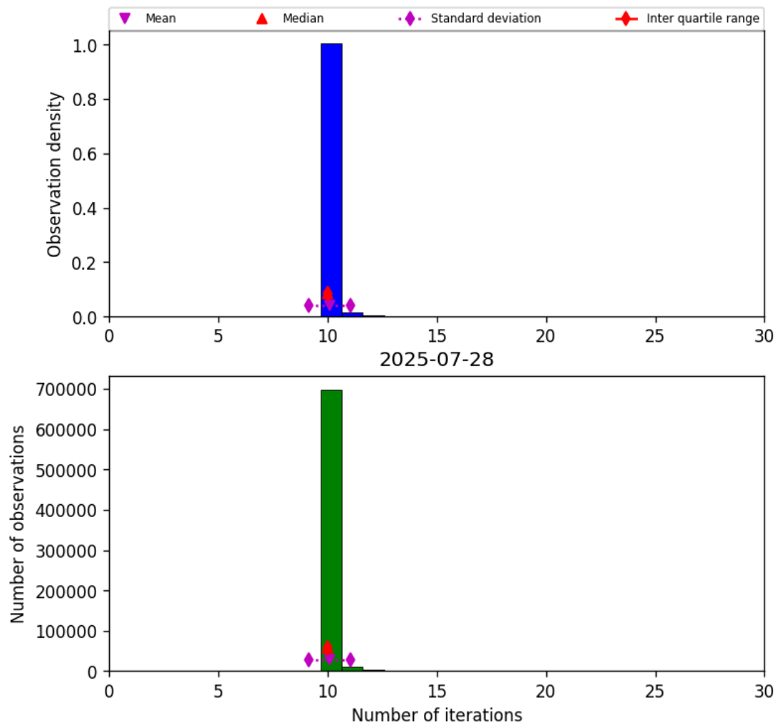
Figure 31: Histogram of “Number of iterations” for 2025-07-27 to 2025-07-29
