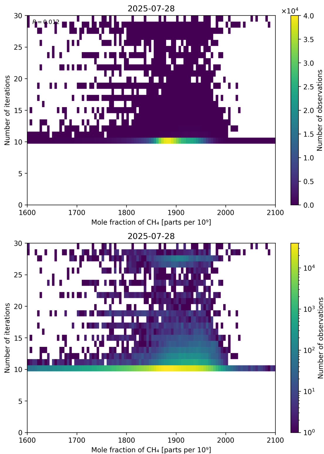
Figure 76: Scatter density plot of “Mole fraction of CH 4 ” against “Number of iterations” for 2025-07-27 to 2025-07-29.
