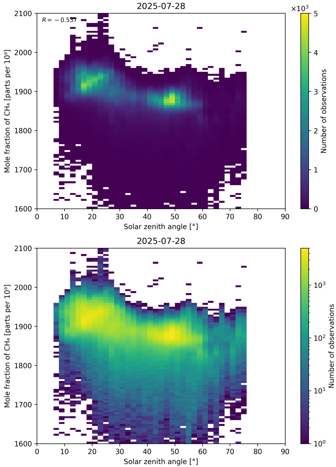
Figure 99: Scatter density plot of “Solar zenith angle” against “Mole fraction of CH 4 ” for 2025-07-27 to 2025-07-29.
