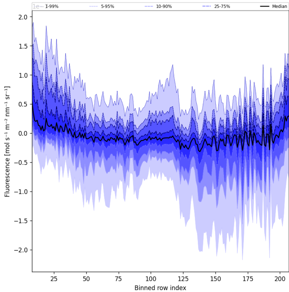
Figure 43: Along track statistics of “Fluorescence” for 2025-07-27 to 2025-07-29
