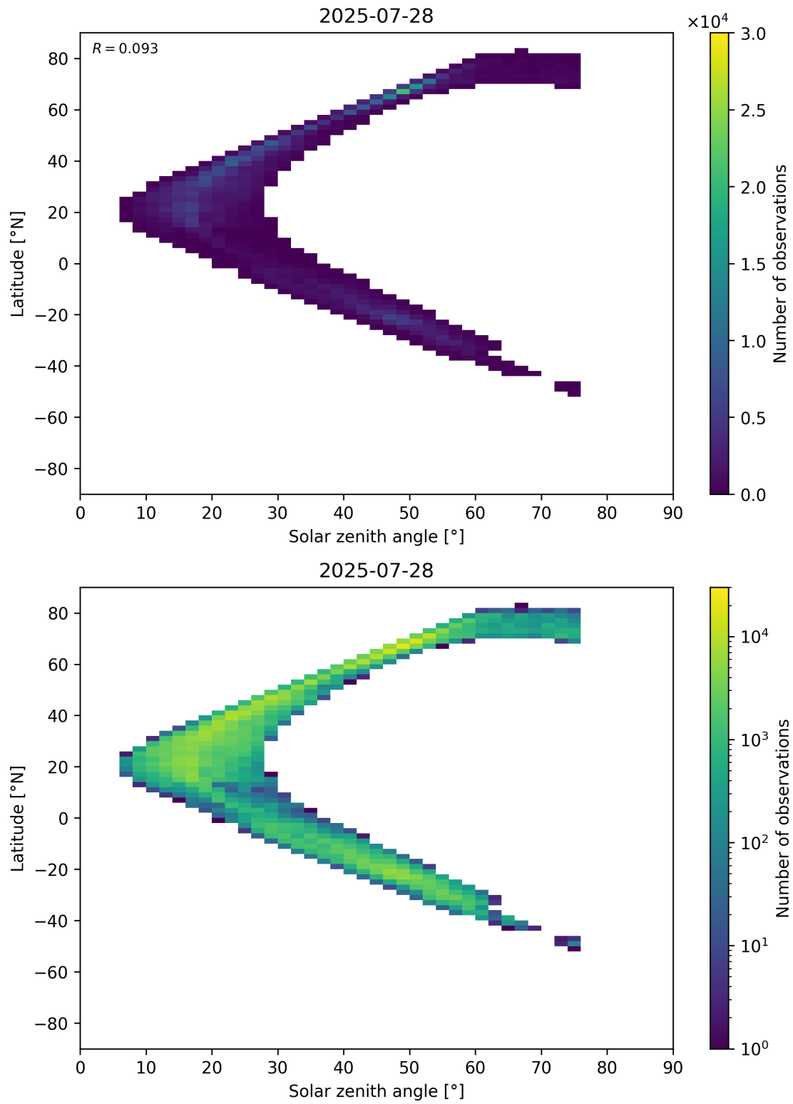
Figure 98: Scatter density plot of “Solar zenith angle” against “Latitude” for 2025-07-27 to 2025-07-29.
