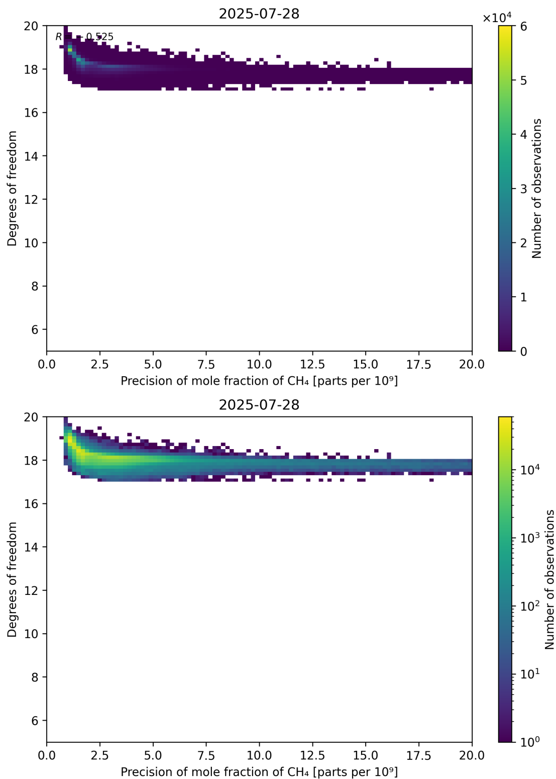
Figure 80: Scatter density plot of “Precision of mole fraction of CH 4 ” against “Degrees of freedom” for 2025-07-27 to 2025-07-29.
