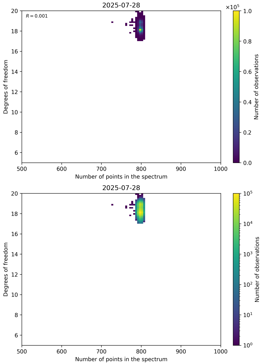
Figure 90: Scatter density plot of “Number of points in the spectrum” against “Degrees of freedom” for 2025-07-27 to 2025-07-29.
