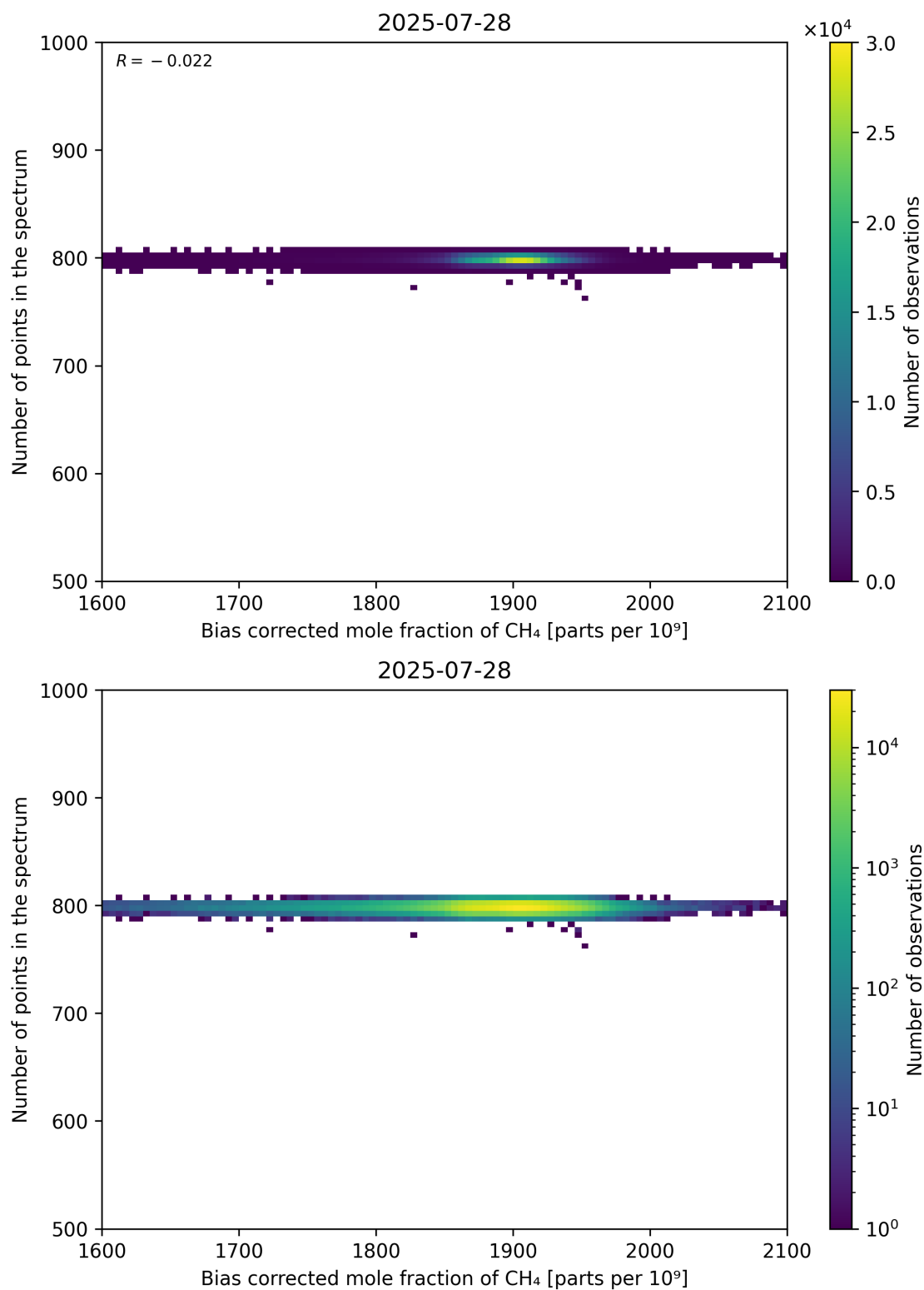
Figure 68: Scatter density plot of “Bias corrected mole fraction of CH 4 ” against “Number of points in the spectrum” for 2025-07-27 to 2025-07-29.
