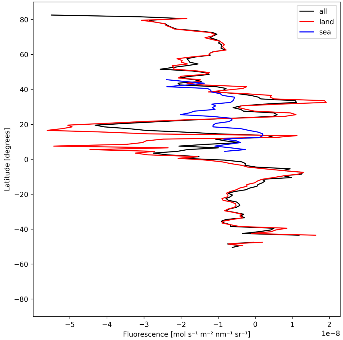
Figure 21: Zonal average of “Fluorescence” for 2025-07-27 to 2025-07-29.
