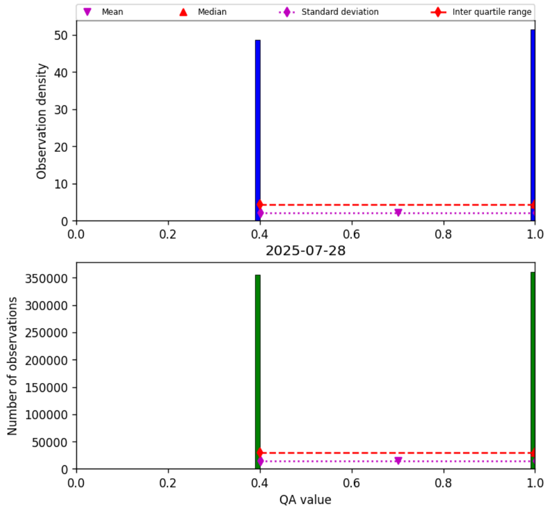
Figure 22: Histogram of “QA value” for 2025-07-27 to 2025-07-29
