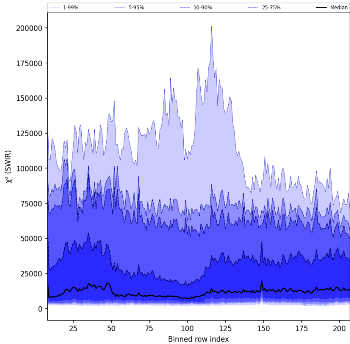
Figure 39: Along track statistics of “ \chi^2 (SWIR)” for 2025-07-27 to 2025-07-29
