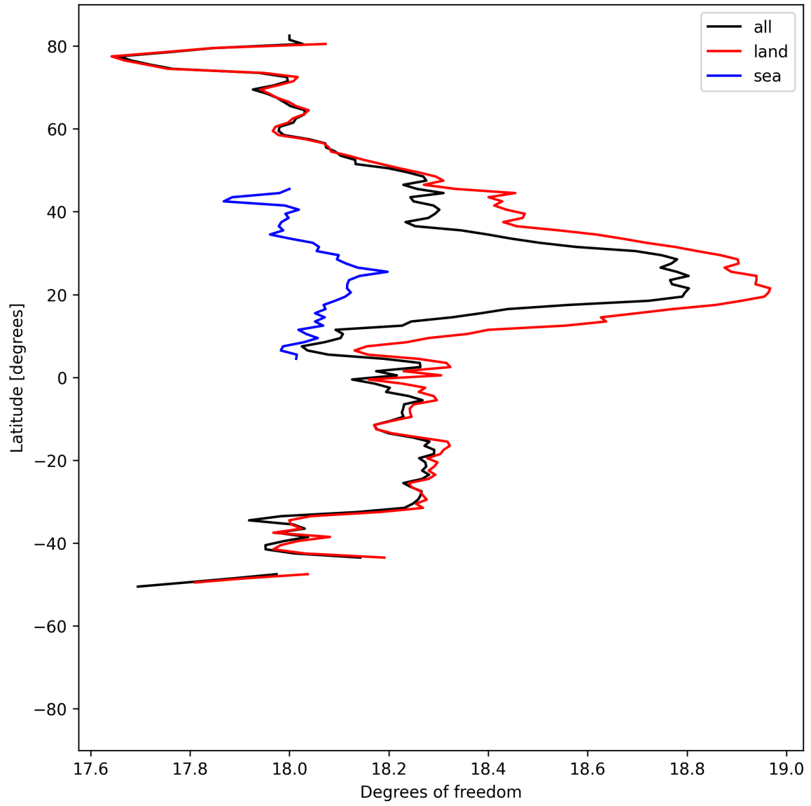
Figure 19: Zonal average of “Degrees of freedom” for 2025-07-27 to 2025-07-29.
