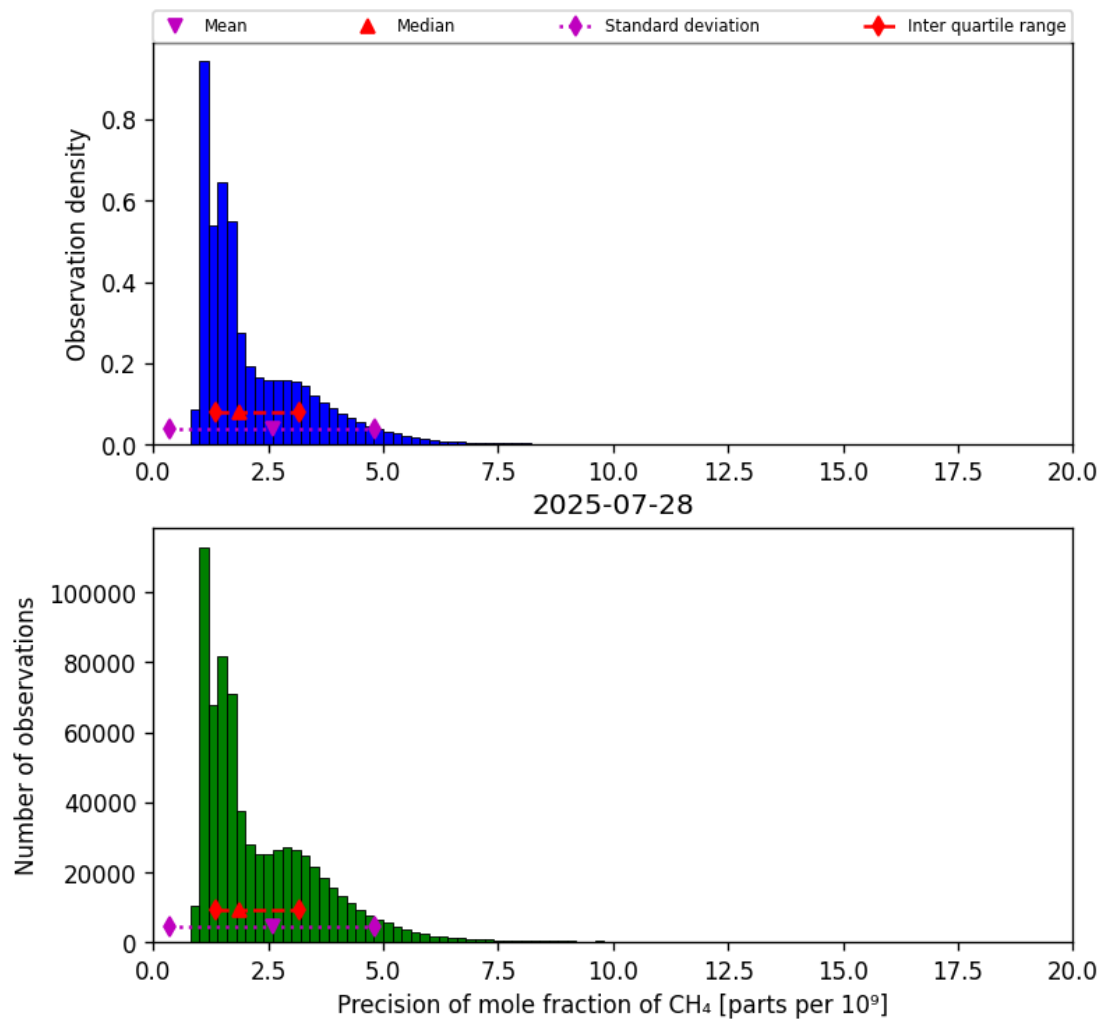
Figure 24: Histogram of “Precision of mole fraction of CH 4 ” for 2025-07-27 to 2025-07-29
