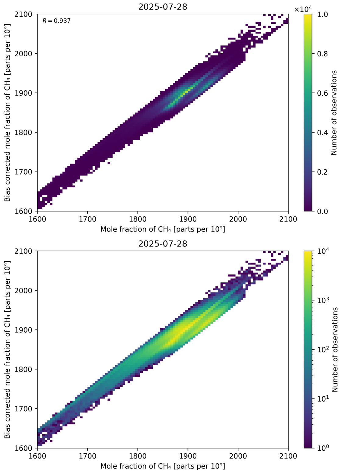
Figure 74: Scatter density plot of “Mole fraction of \text{CH}_4 ” against “Bias corrected mole fraction of \text{CH}_4 ” for 2025-07-27 to 2025-07-29.
