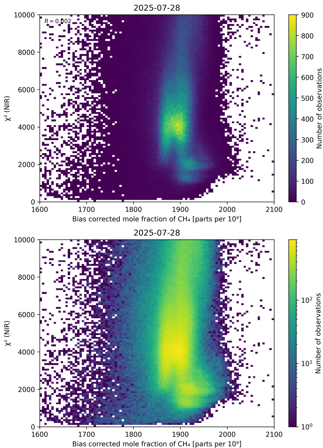
Figure 63: Scatter density plot of “Bias corrected mole fraction of CH 4 ” against “ \chi^2 (NIR)” for 2025-07-27 to 2025-07-29.
