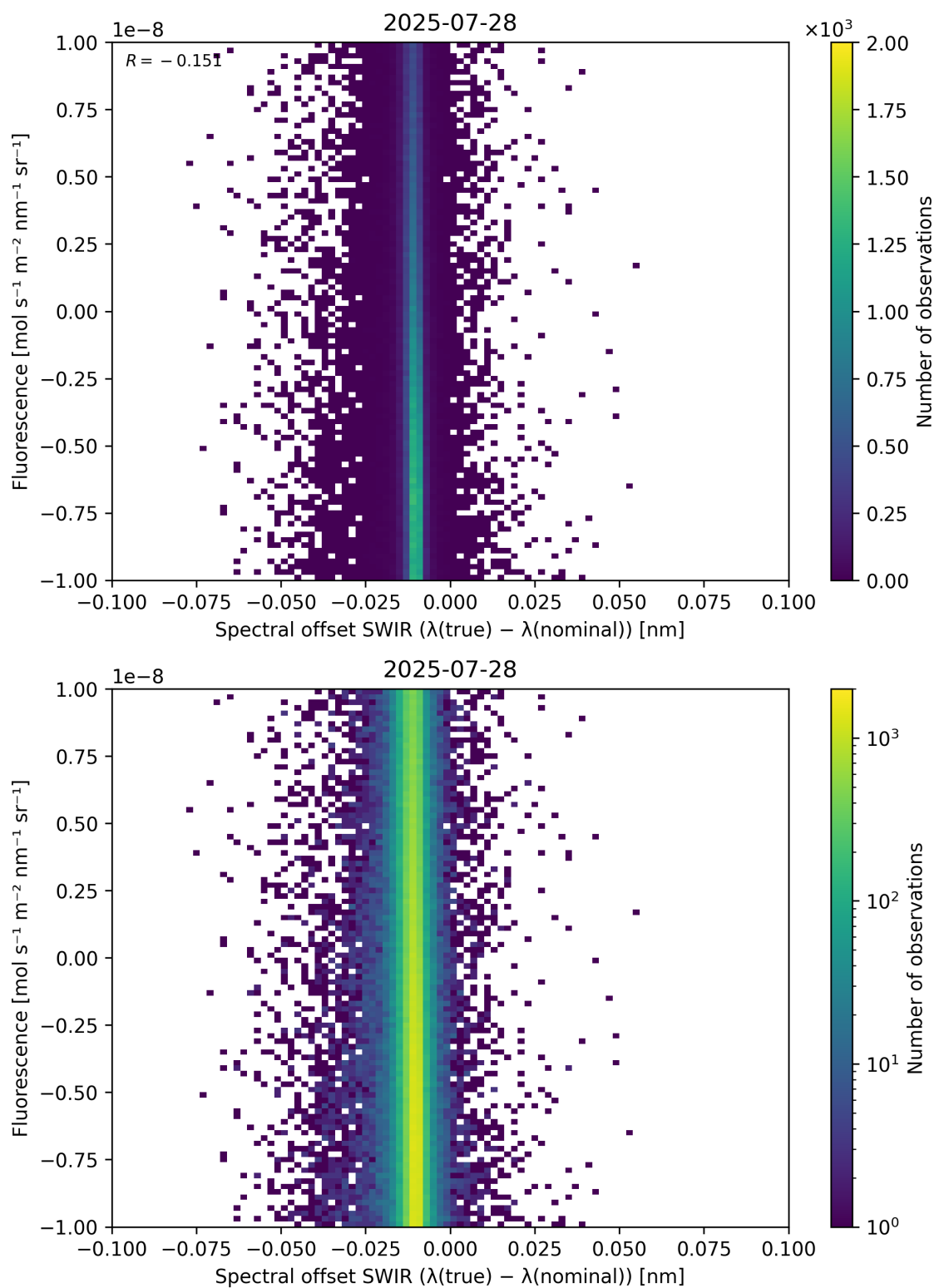
Figure 120: Scatter density plot of “Spectral offset SWIR ( \lambda_{\text{true}} - \lambda_{\text{nominal}} )” against “Fluorescence” for 2025-07-27 to 2025-07-29.
