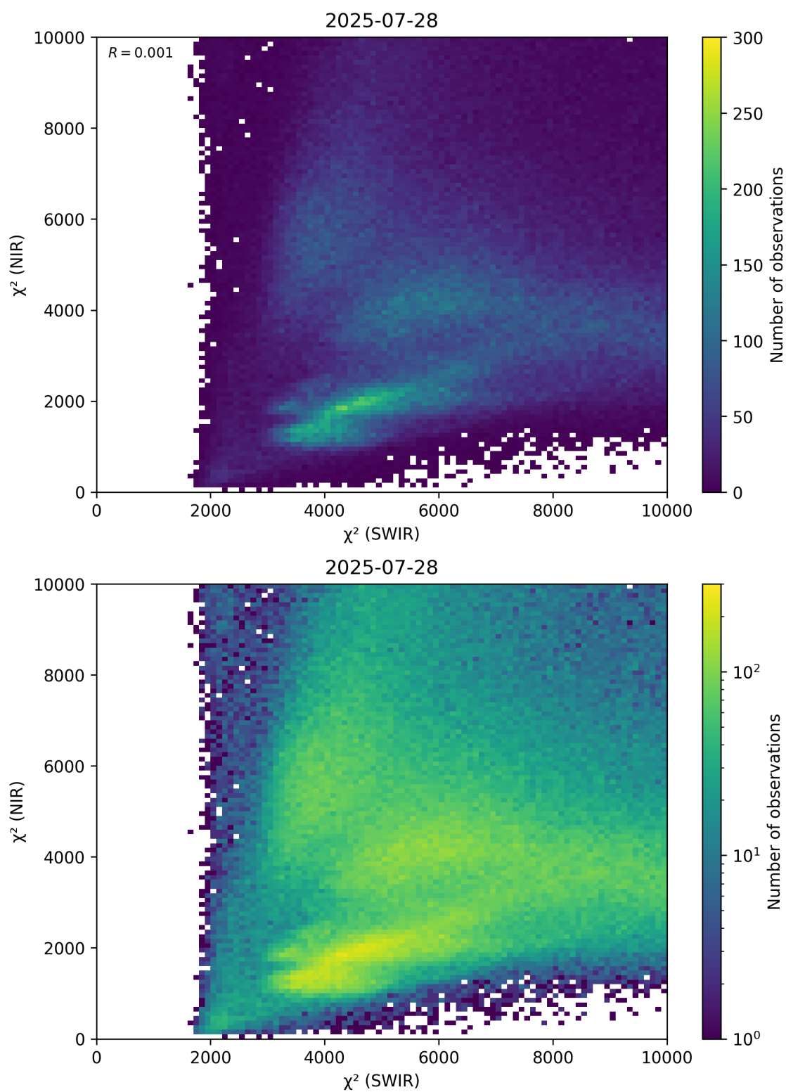
Figure 47: Scatter density plot of “ \chi^2 (SWIR)” against “ \chi^2 (NIR)” for 2025-07-27 to 2025-07-29.
