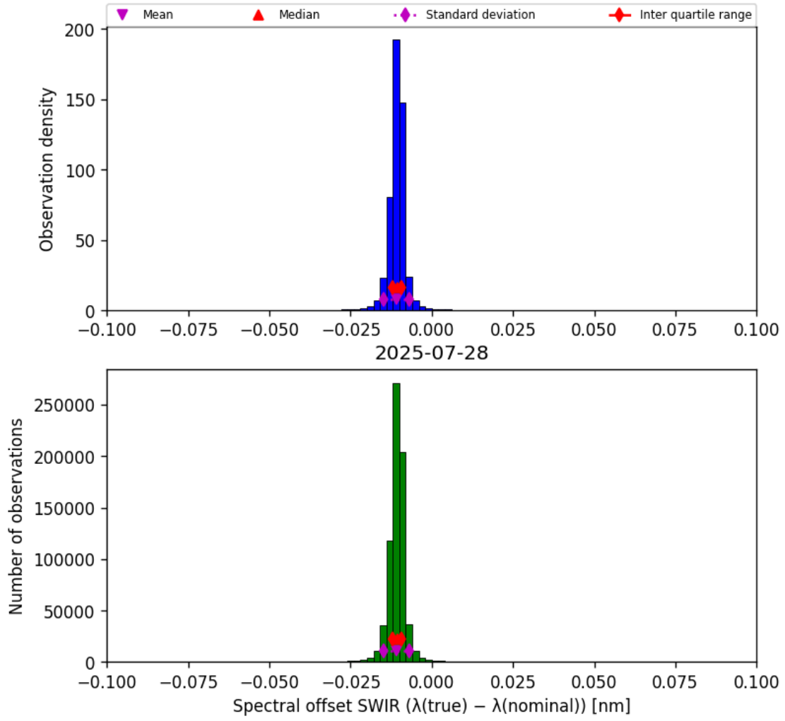
Figure 27: Histogram of “Spectral offset SWIR ( \lambda_{\text{true}} - \lambda_{\text{nominal}} )” for 2025-07-27 to 2025-07-29
