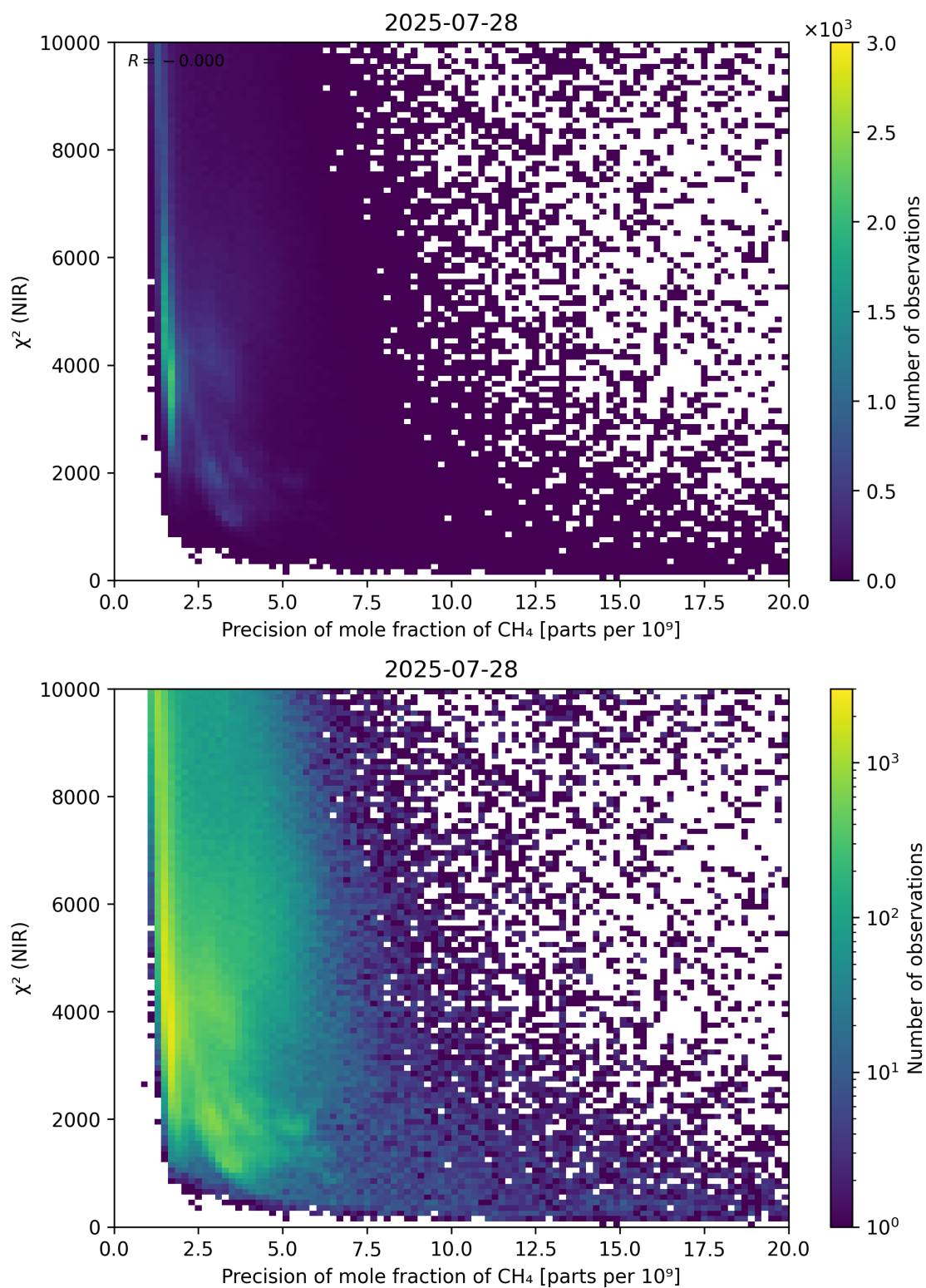
Figure 78: Scatter density plot of “Precision of mole fraction of CH 4 ” against “ \chi^2 (NIR)” for 2025-07-27 to 2025-07-29.
