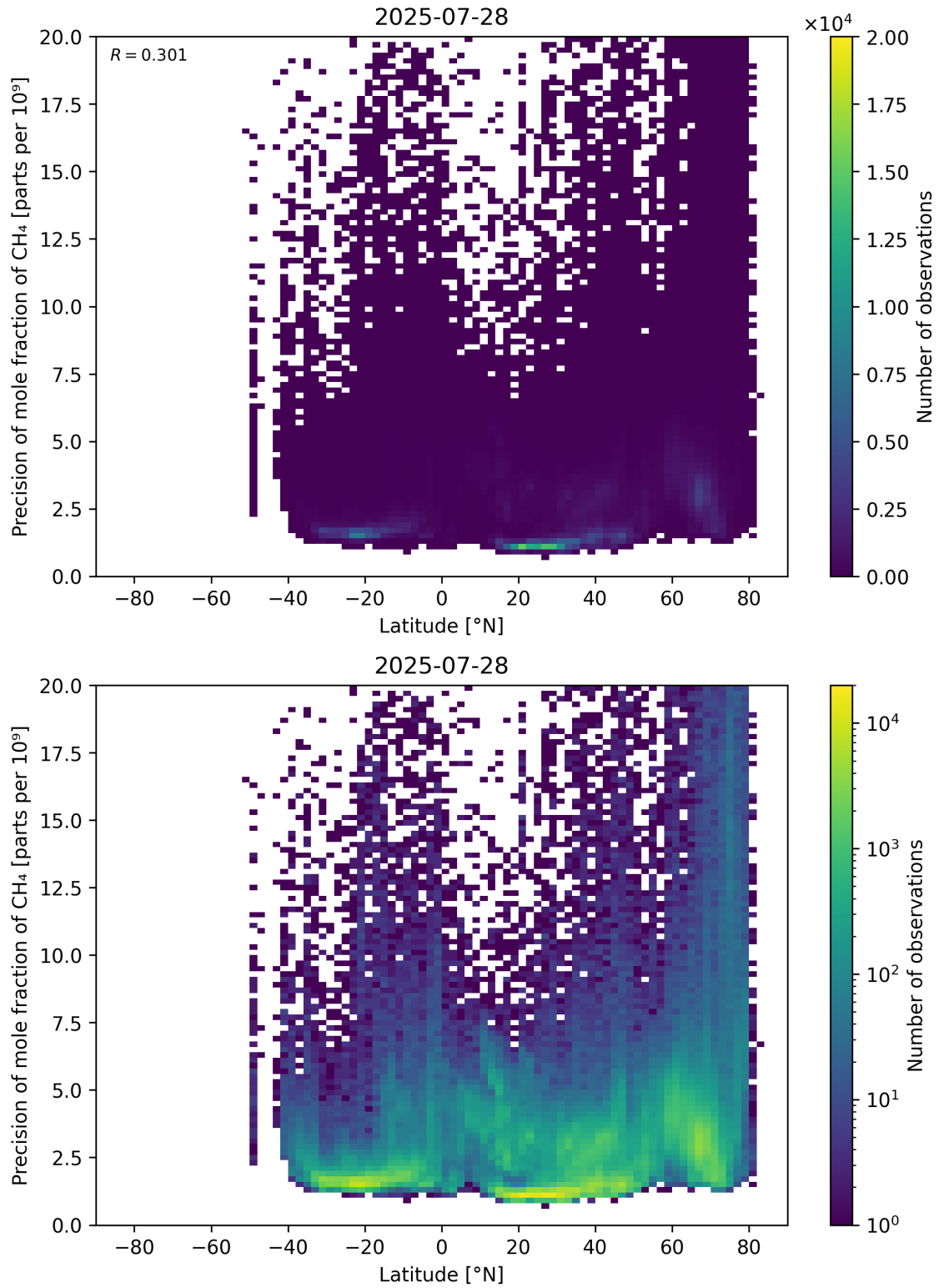
Figure 59: Scatter density plot of “Latitude” against “Precision of mole fraction of \text{CH}_4 ” for 2025-07-27 to 2025-07-29.
