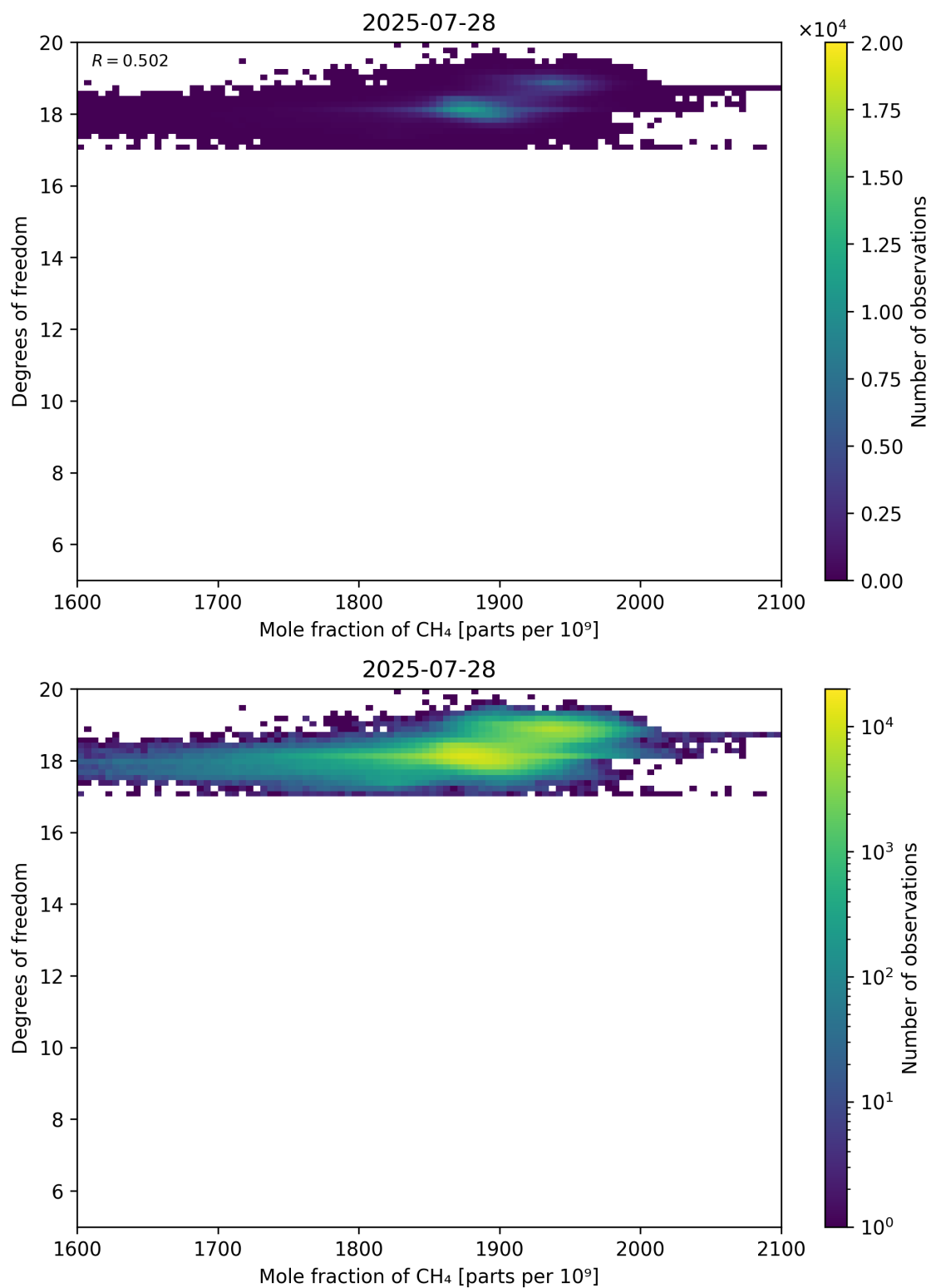
Figure 72: Scatter density plot of “Mole fraction of CH 4 ” against “Degrees of freedom” for 2025-07-27 to 2025-07-29.
