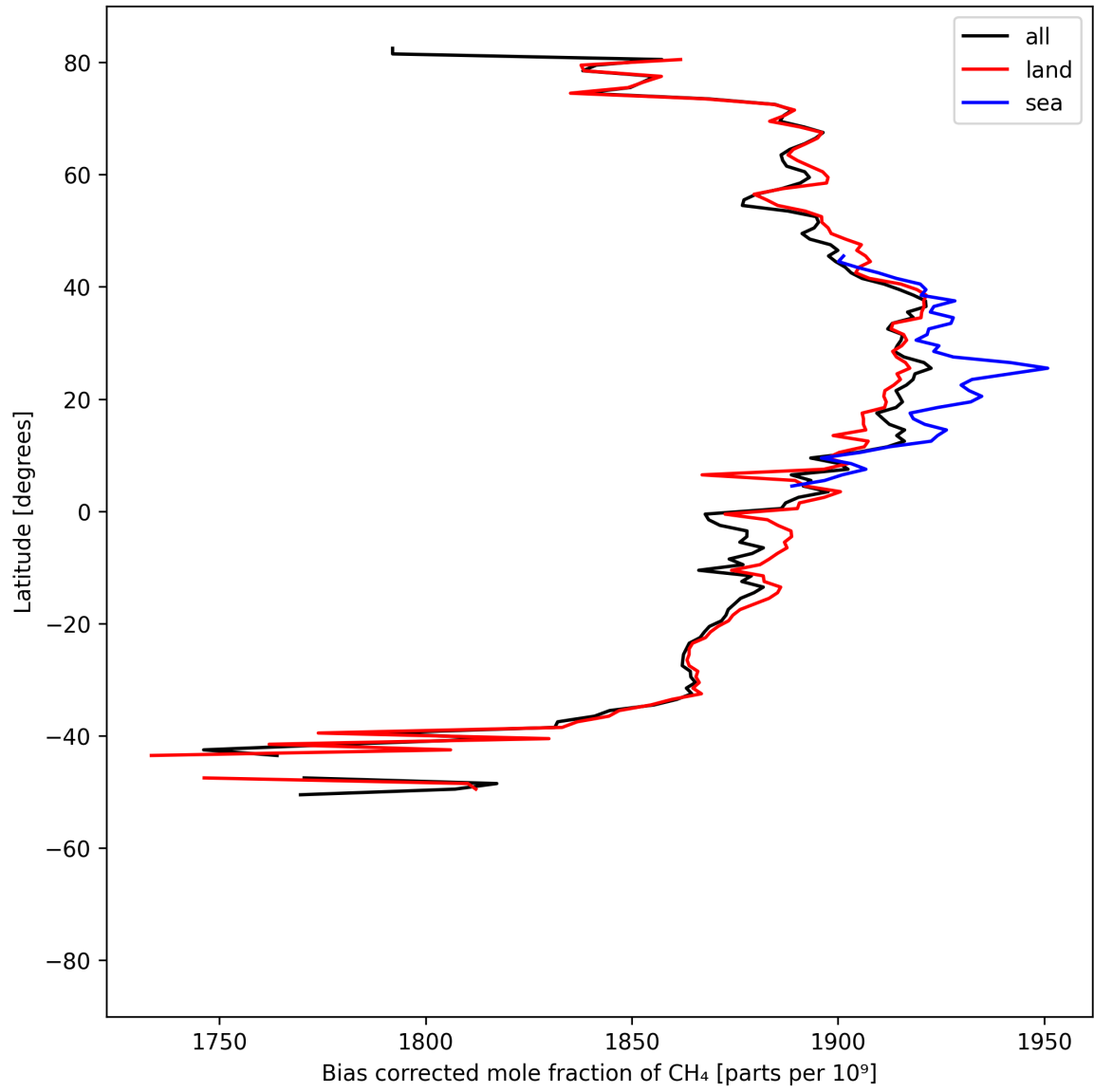
Figure 14: Zonal average of “Bias corrected mole fraction of CH 4 ” for 2025-07-27 to 2025-07-29.
