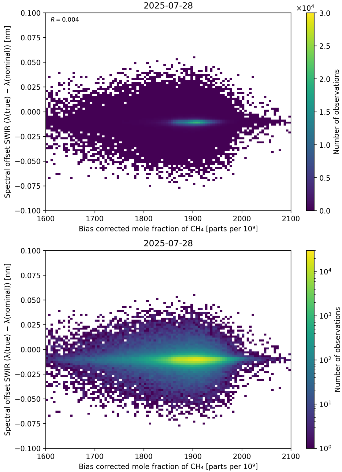
Figure 69: Scatter density plot of “Bias corrected mole fraction of \text{CH}_4 ” against “Spectral offset SWIR ( \lambda_{\text{true}} - \lambda_{\text{nominal}} )” for 2025-07-27 to 2025-07-29.
