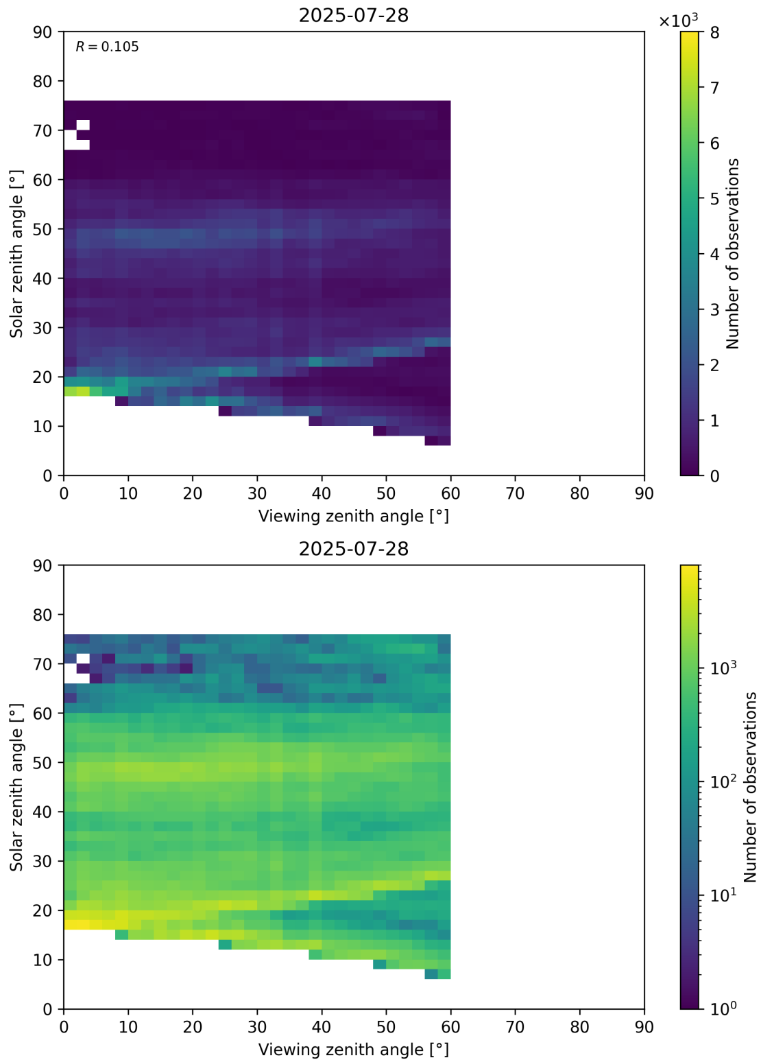
Figure 115: Scatter density plot of “Viewing zenith angle” against “Solar zenith angle” for 2025-07-27 to 2025-07-29.
