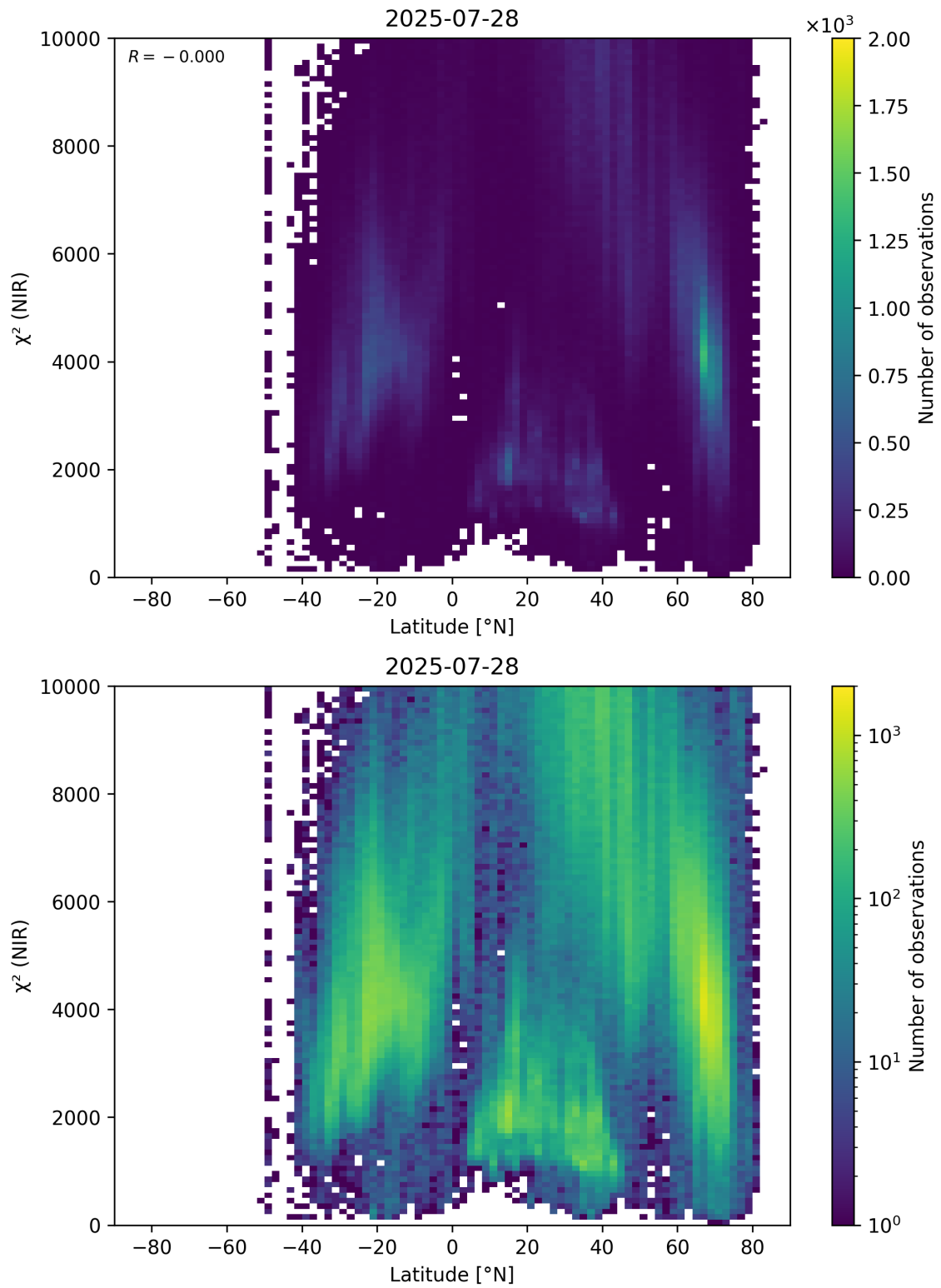
Figure 53: Scatter density plot of “Latitude” against “ \chi^2 (NIR)” for 2025-07-27 to 2025-07-29.
