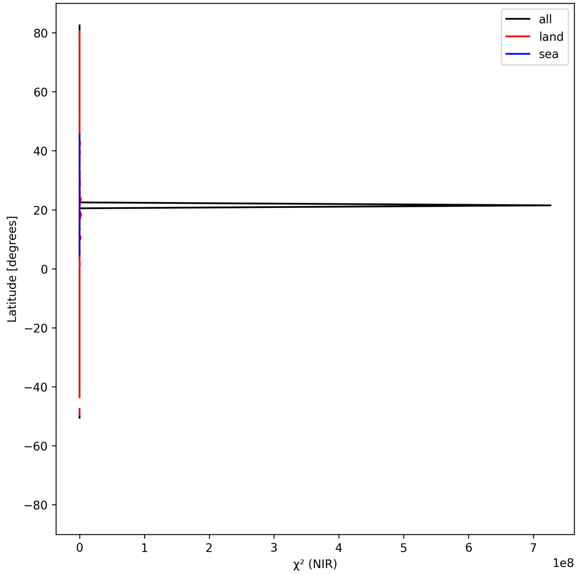
Figure 18: Zonal average of “ \chi^2 (NIR)” for 2025-07-27 to 2025-07-29.
