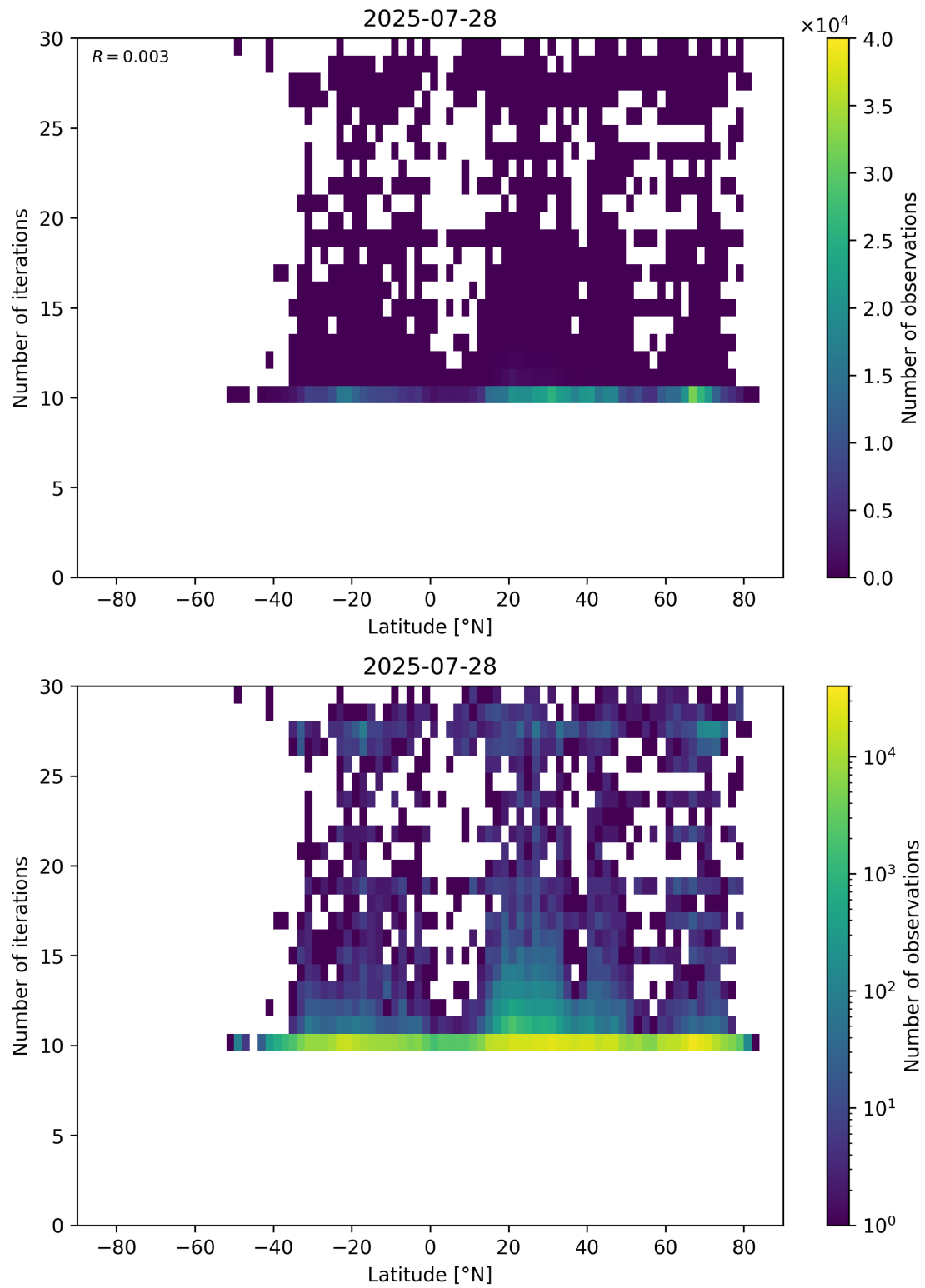
Figure 60: Scatter density plot of “Latitude” against “Number of iterations” for 2025-07-27 to 2025-07-29.
