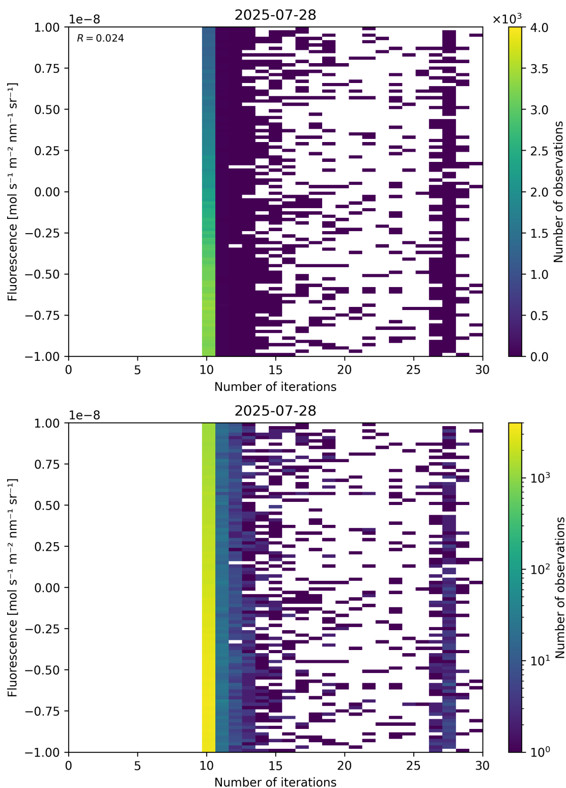
Figure 87: Scatter density plot of “Number of iterations” against “Fluorescence” for 2025-07-27 to 2025-07-29.
