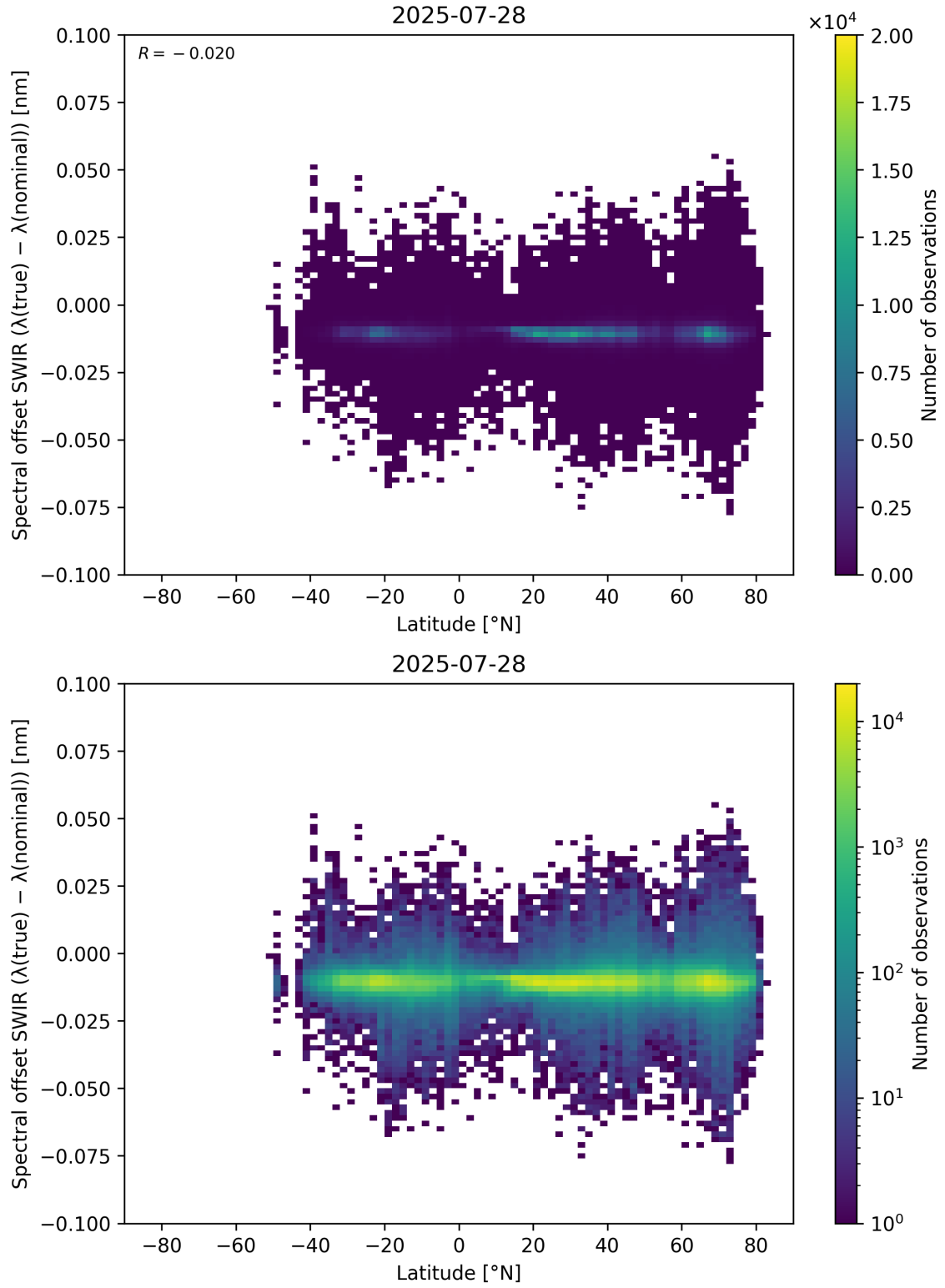
Figure 62: Scatter density plot of “Latitude” against “Spectral offset SWIR ( \lambda_{\text{true}} - \lambda_{\text{nominal}} )” for 2025-07-27 to 2025-07-29.
