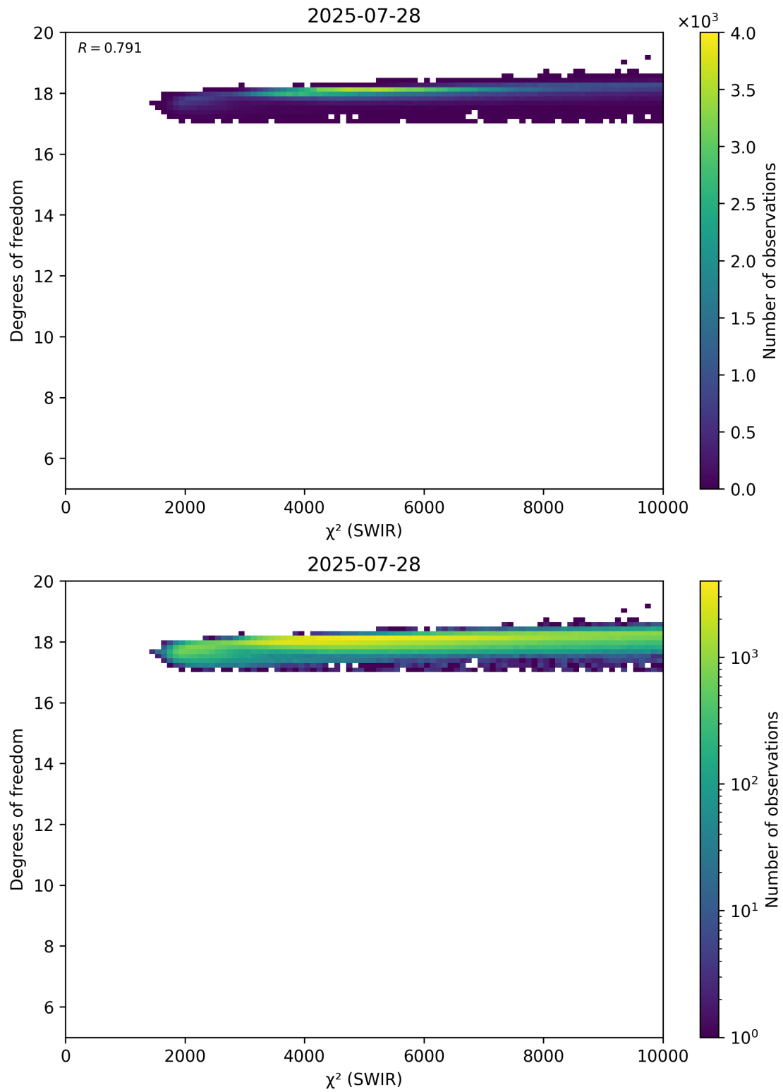
Figure 48: Scatter density plot of “ \chi^2 (SWIR)” against “Degrees of freedom” for 2025-07-27 to 2025-07-29.
