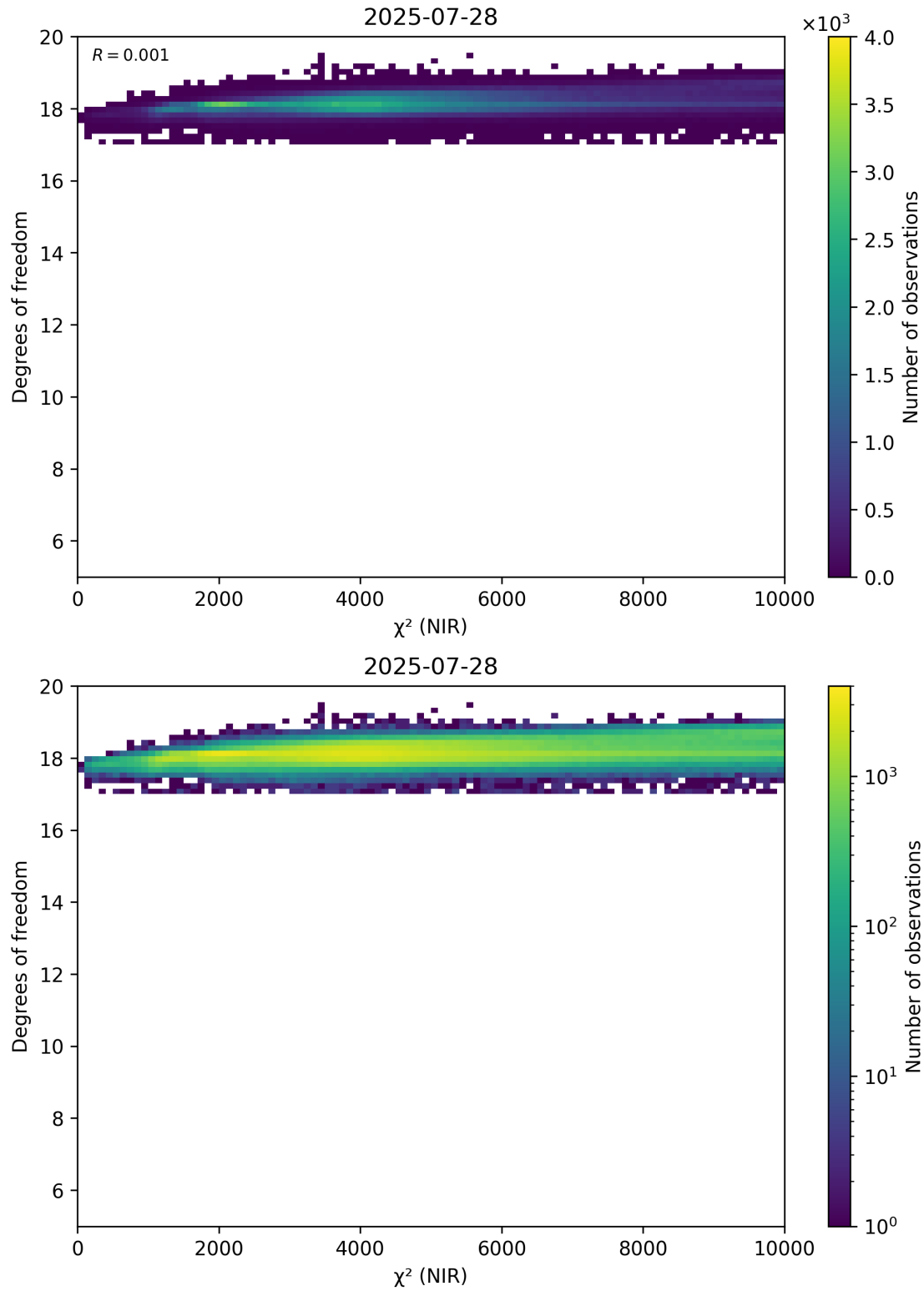
Figure 44: Scatter density plot of “ \chi^2 (NIR)” against “Degrees of freedom” for 2025-07-27 to 2025-07-29.
