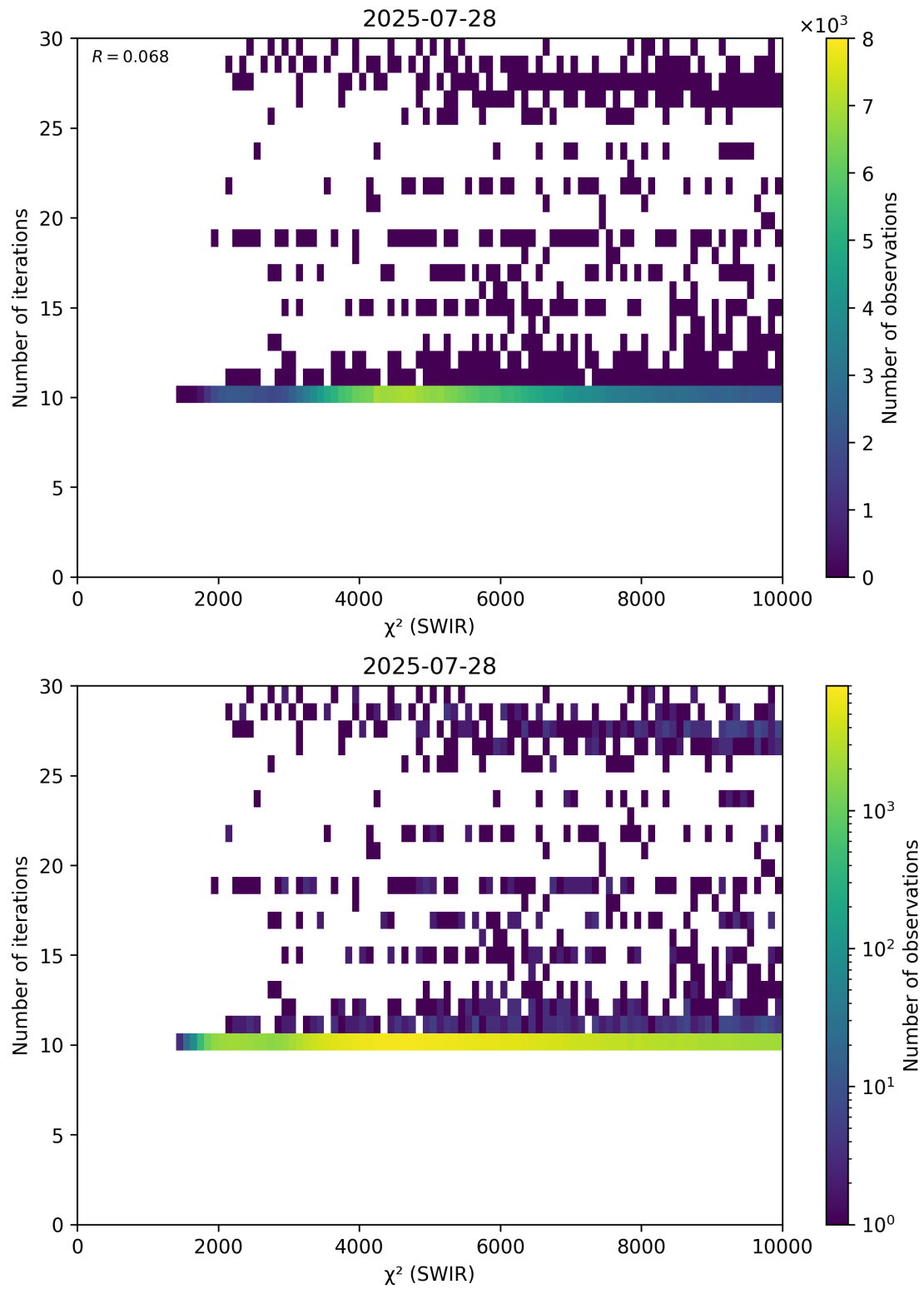
Figure 50: Scatter density plot of “ \chi^2 (SWIR)” against “Number of iterations” for 2025-07-27 to 2025-07-29.
