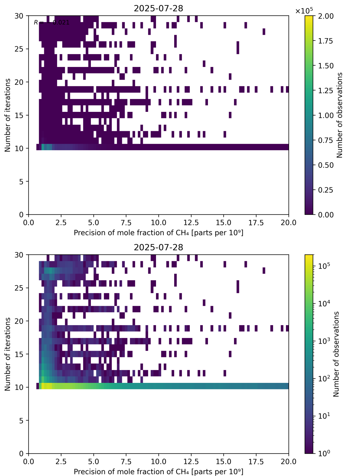
Figure 83: Scatter density plot of “Precision of mole fraction of CH 4 ” against “Number of iterations” for 2025-07-27 to 2025-07-29.
