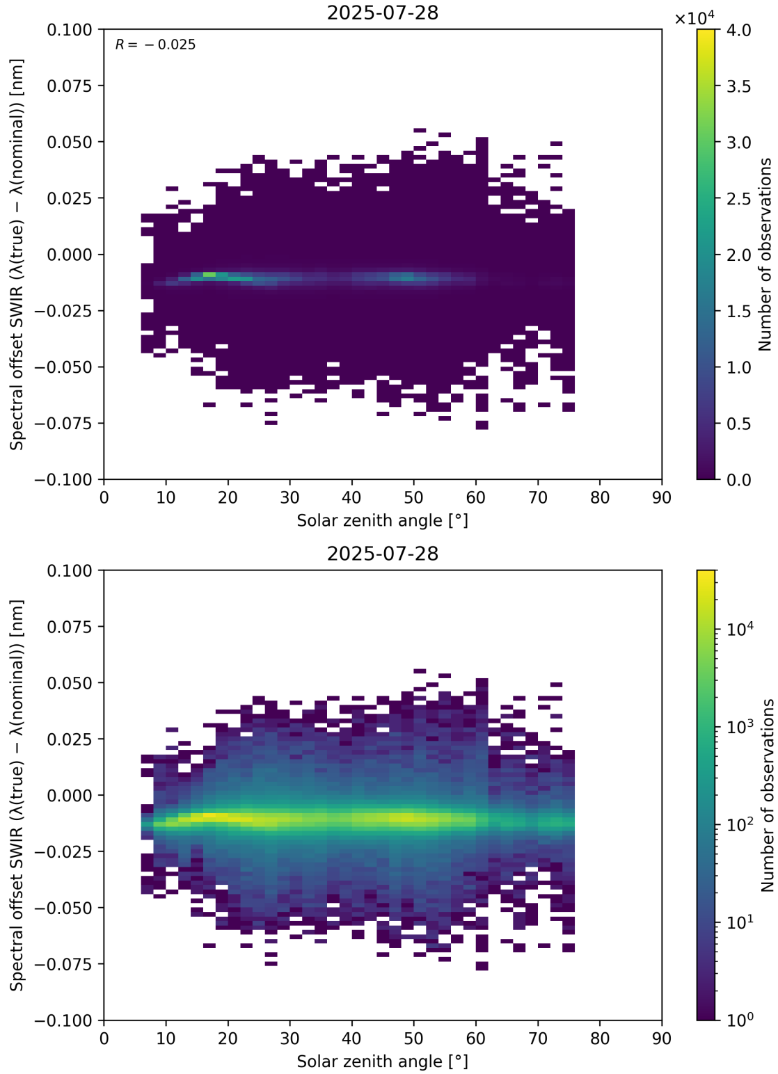
Figure 104: Scatter density plot of “Solar zenith angle” against “Spectral offset SWIR ( \lambda_{\text{true}} - \lambda_{\text{nominal}} )” for 2025-07-27 to 2025-07-29.
