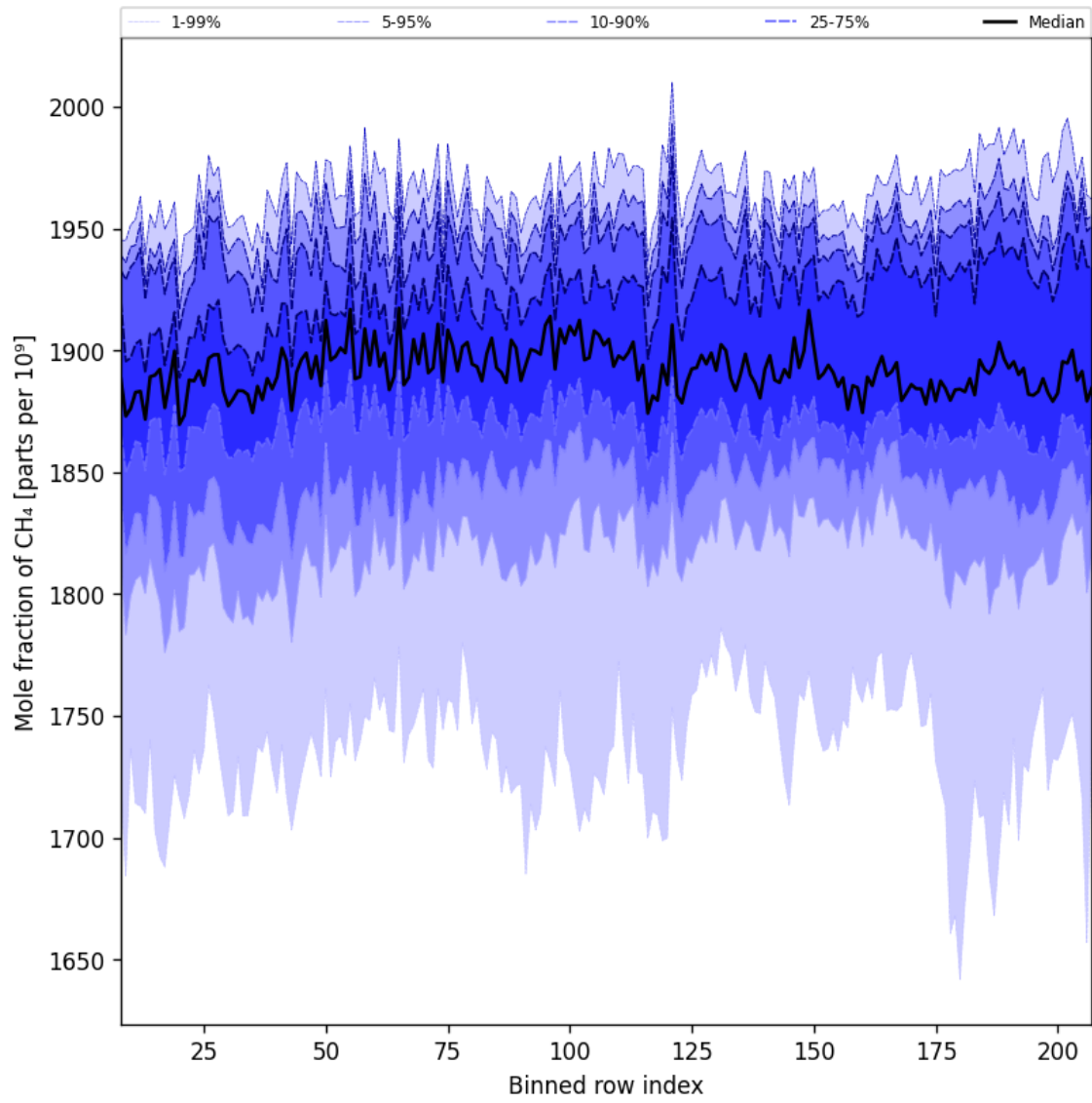
Figure 34: Along track statistics of “Mole fraction of CH 4 ” for 2025-07-27 to 2025-07-29
