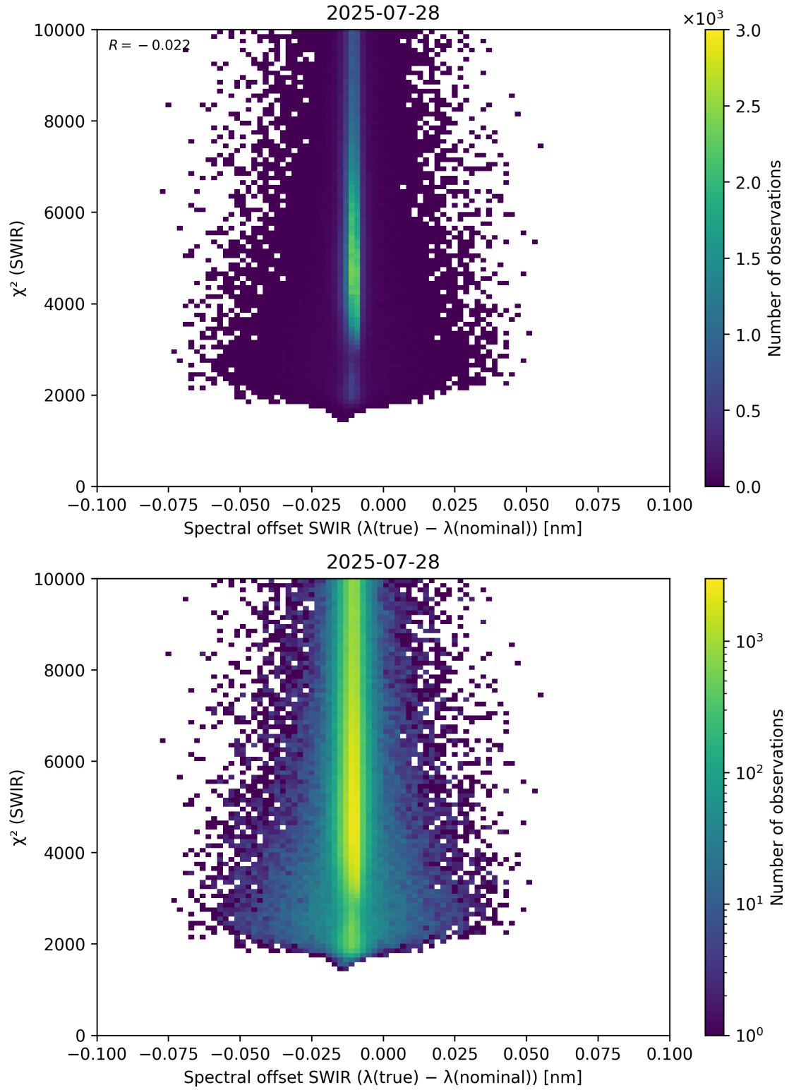
Figure 118: Scatter density plot of “Spectral offset SWIR ( \lambda_{\text{true}} - \lambda_{\text{nominal}} )” against “ \chi^2 (SWIR)” for 2025-07-27 to 2025-07-29.
