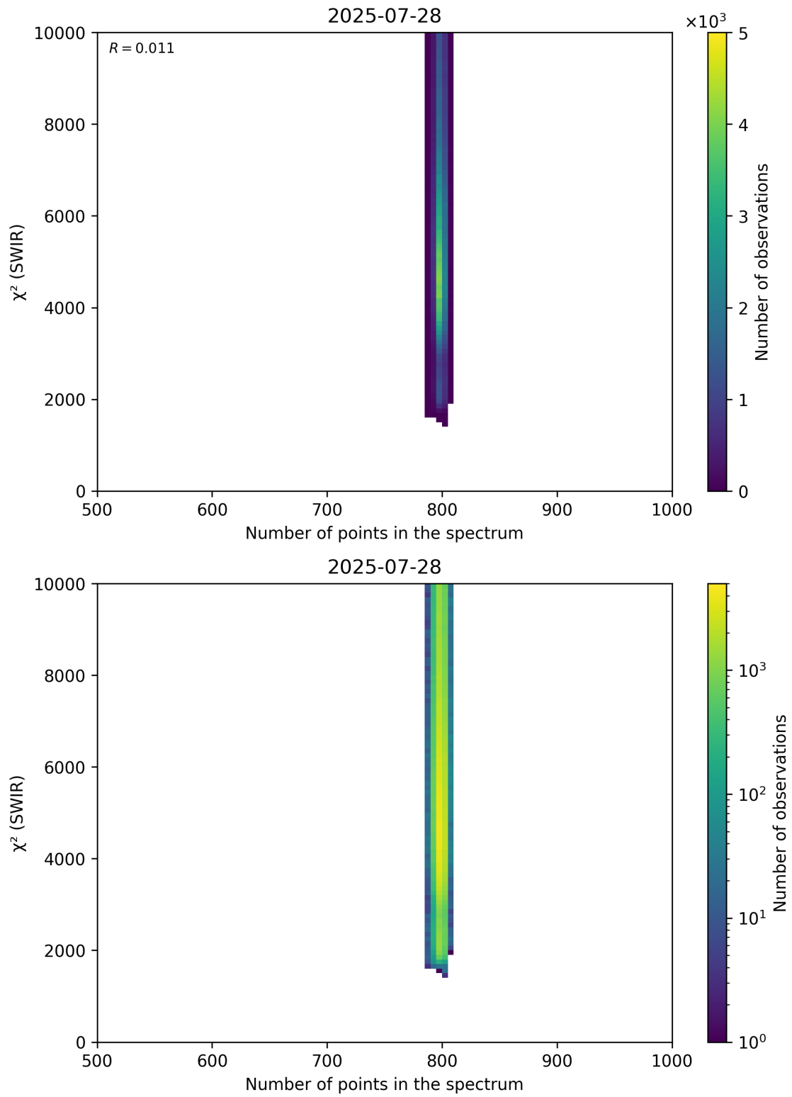
Figure 89: Scatter density plot of “Number of points in the spectrum” against “ \chi^2 (SWIR)” for 2025-07-27 to 2025-07-29.
