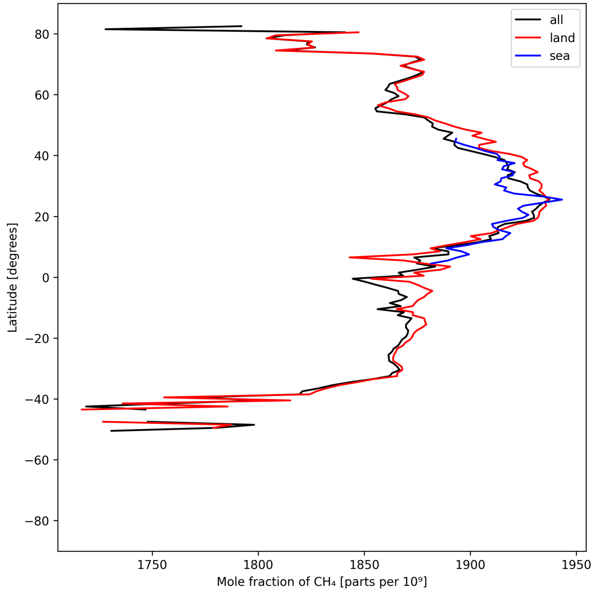
Figure 12: Zonal average of “Mole fraction of \text{CH}_4 ” for 2025-07-27 to 2025-07-29.
