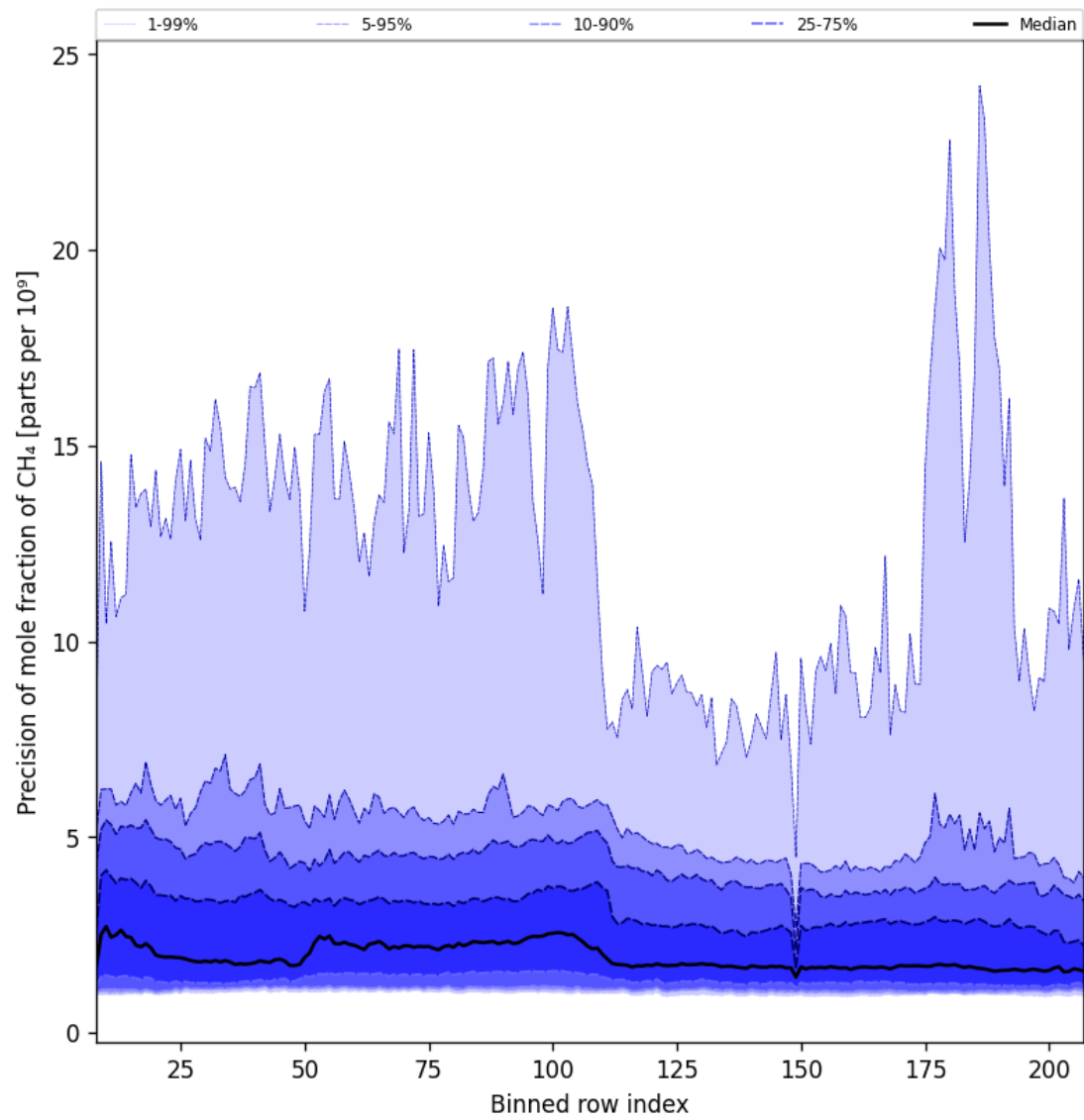
Figure 35: Along track statistics of “Precision of mole fraction of CH 4 ” for 2025-07-27 to 2025-07-29
