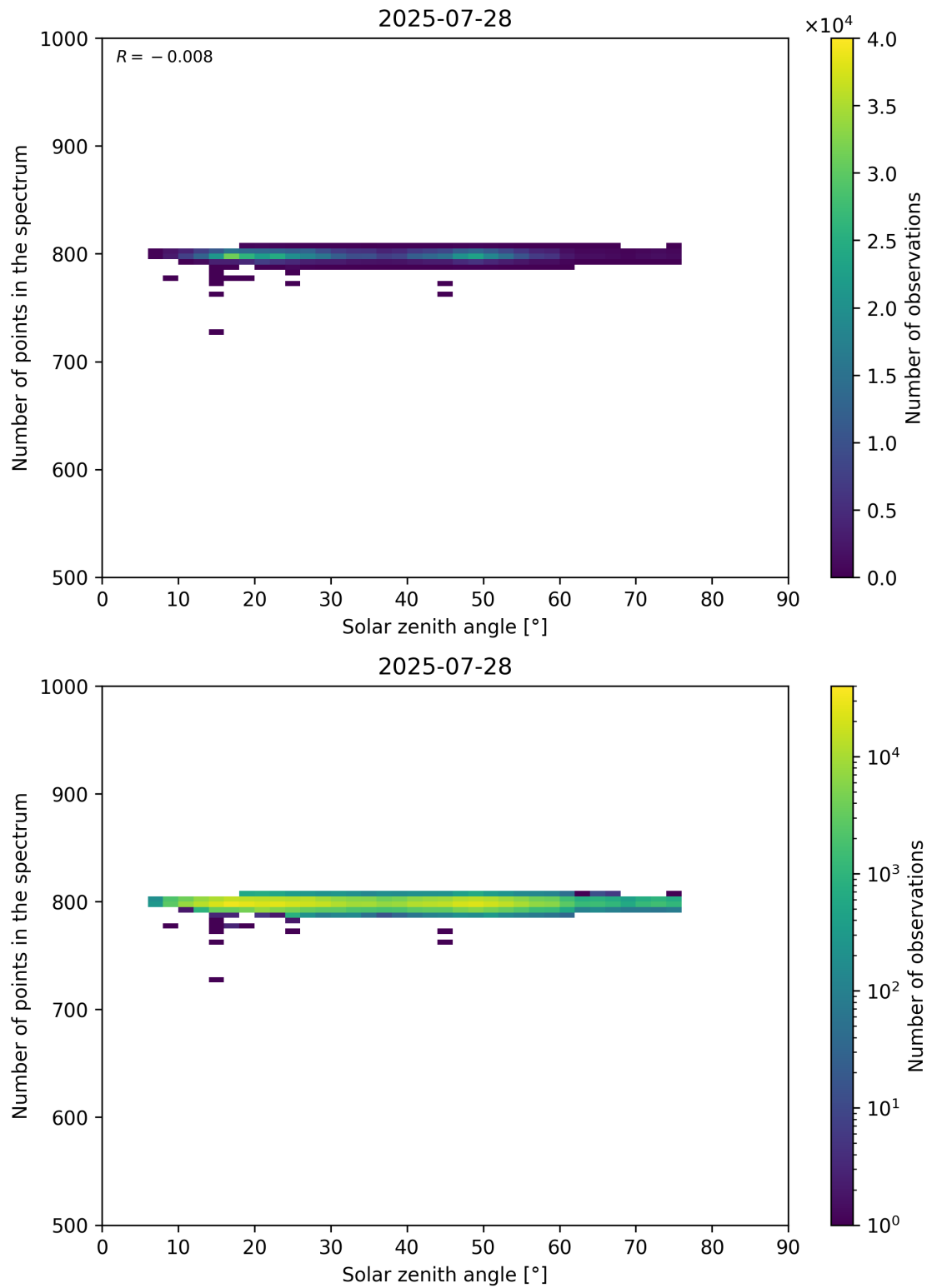
Figure 103: Scatter density plot of “Solar zenith angle” against “Number of points in the spectrum” for 2025-07-27 to 2025-07-29.
