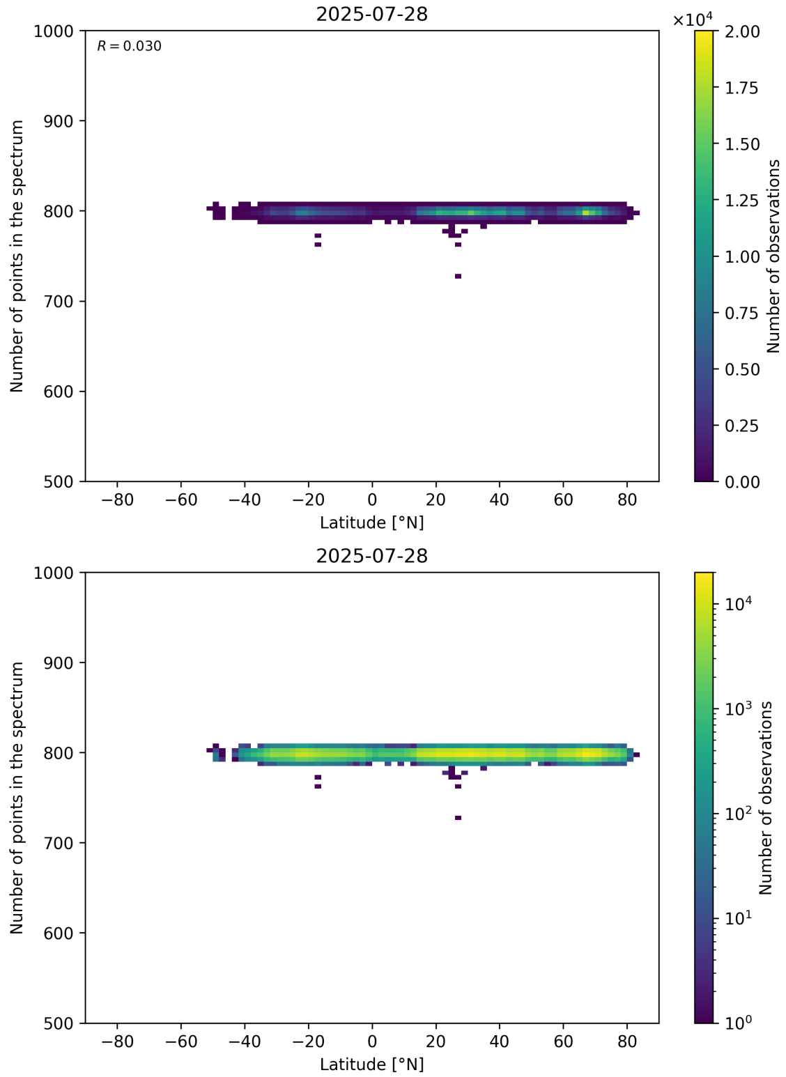
Figure 61: Scatter density plot of “Latitude” against “Number of points in the spectrum” for 2025-07-27 to 2025-07-29.
