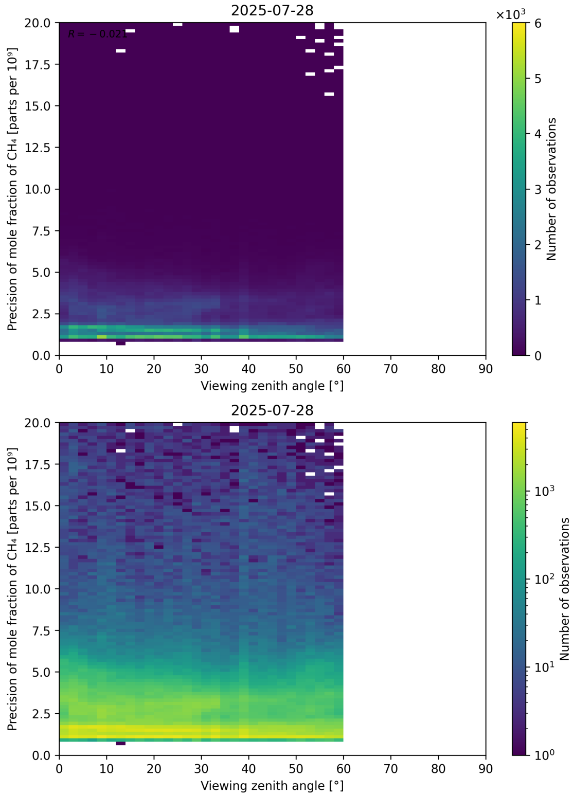
Figure 112: Scatter density plot of “Viewing zenith angle” against “Precision of mole fraction of CH 4 ” for 2025-07-27 to 2025-07-29.
