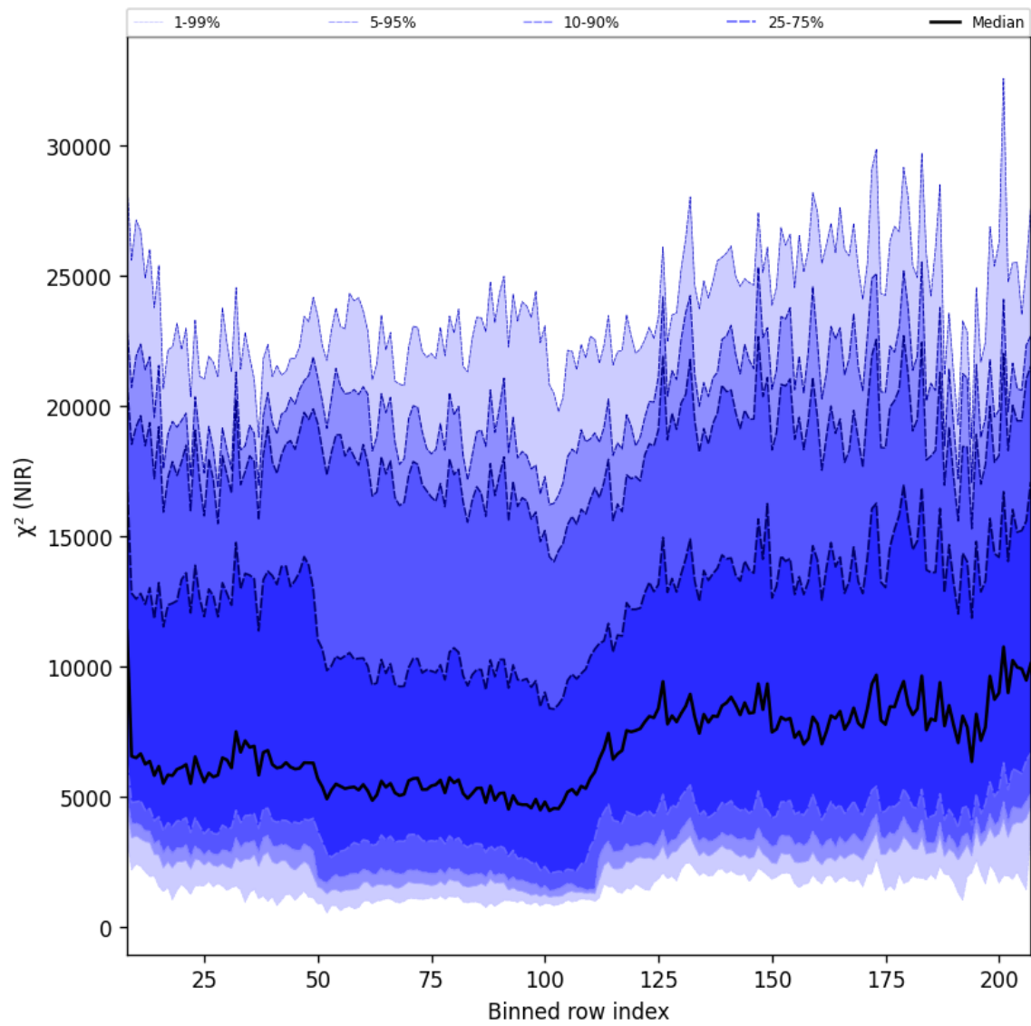
Figure 40: Along track statistics of “ \chi^2 (NIR)” for 2025-07-27 to 2025-07-29
