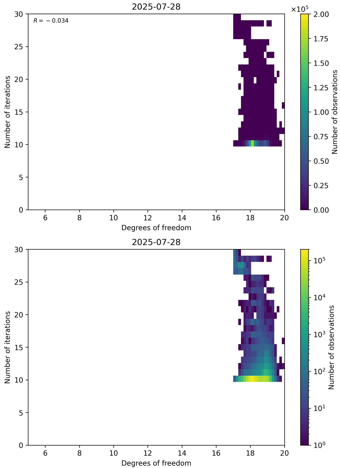
Figure 52: Scatter density plot of “Degrees of freedom” against “Number of iterations” for 2025-07-27 to 2025-07-29.
