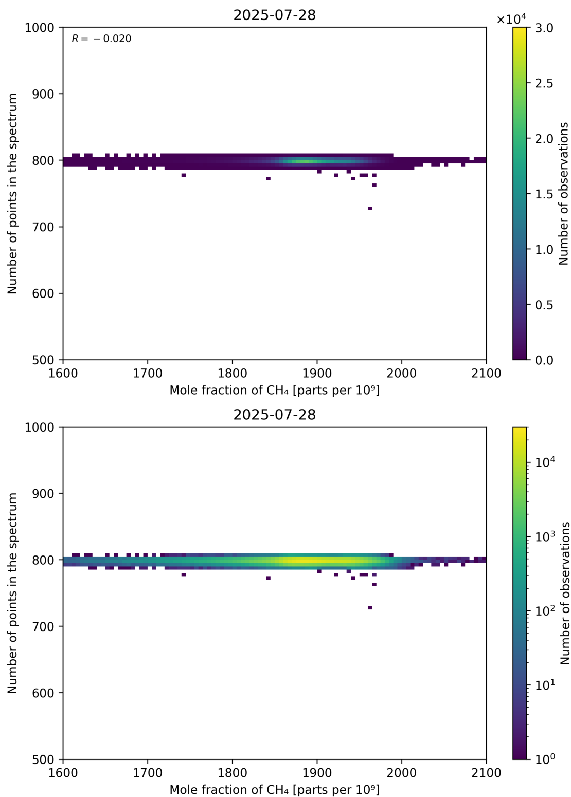
Figure 77: Scatter density plot of “Mole fraction of CH 4 ” against “Number of points in the spectrum” for 2025-07-27 to 2025-07-29.
