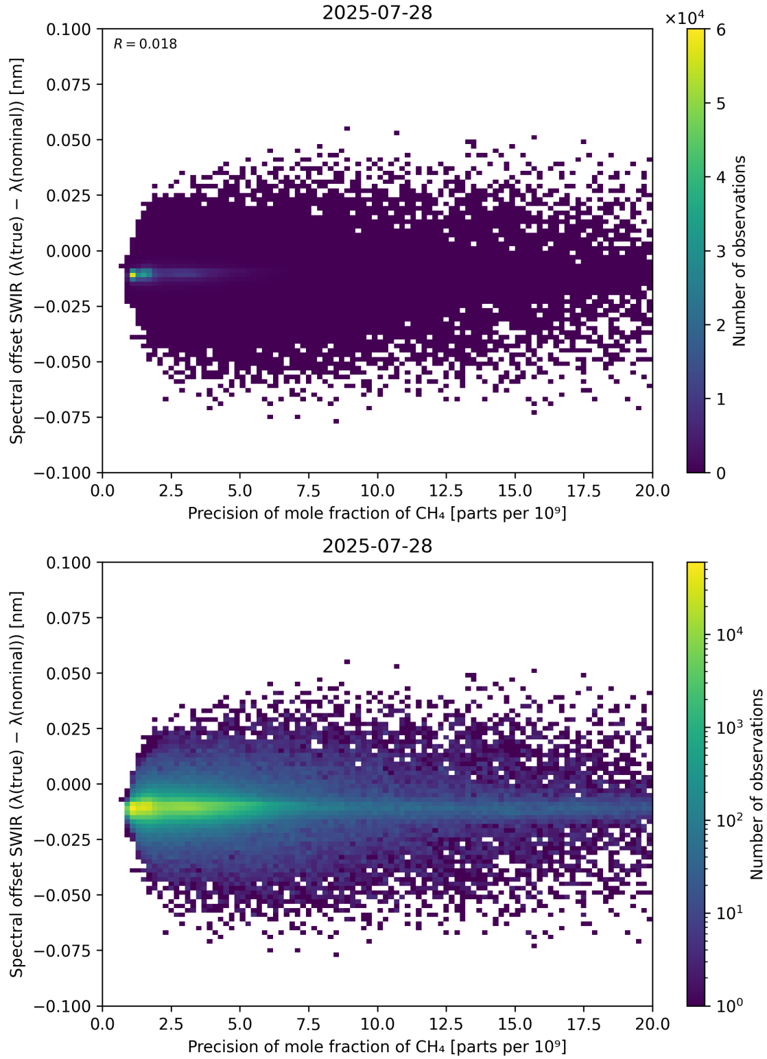
Figure 85: Scatter density plot of “Precision of mole fraction of CH 4 ” against “Spectral offset SWIR ( \lambda_{\text{true}} - \lambda_{\text{nominal}} )” for 2025-07-27 to 2025-07-29.
