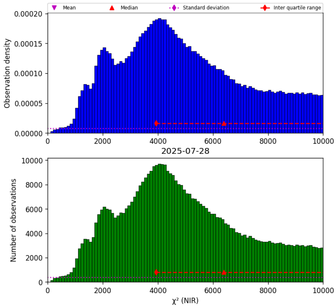
Figure 29: Histogram of “ \chi^2 (NIR)” for 2025-07-27 to 2025-07-29
