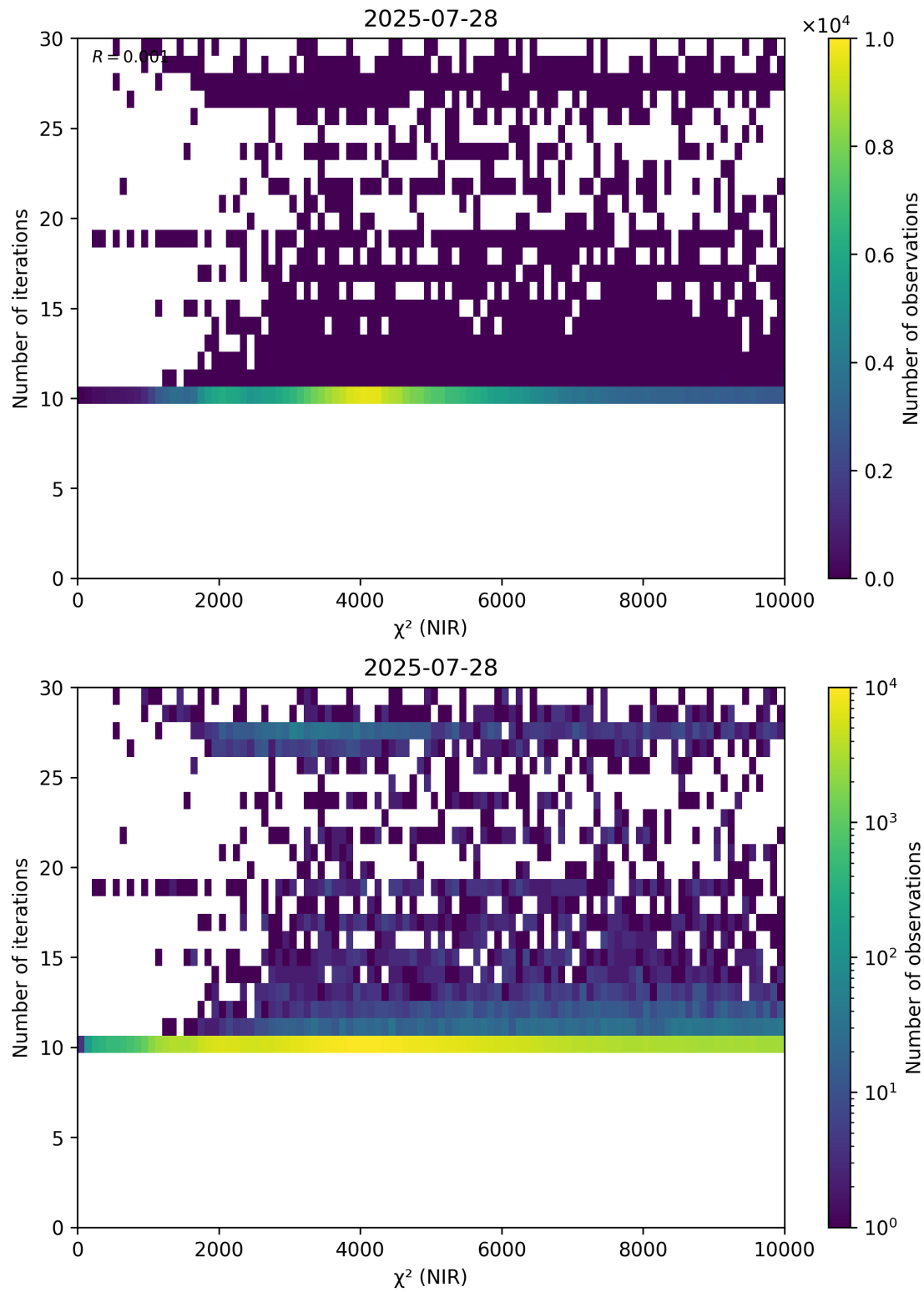
Figure 46: Scatter density plot of “ \chi^2 (NIR)” against “Number of iterations” for 2025-07-27 to 2025-07-29.
