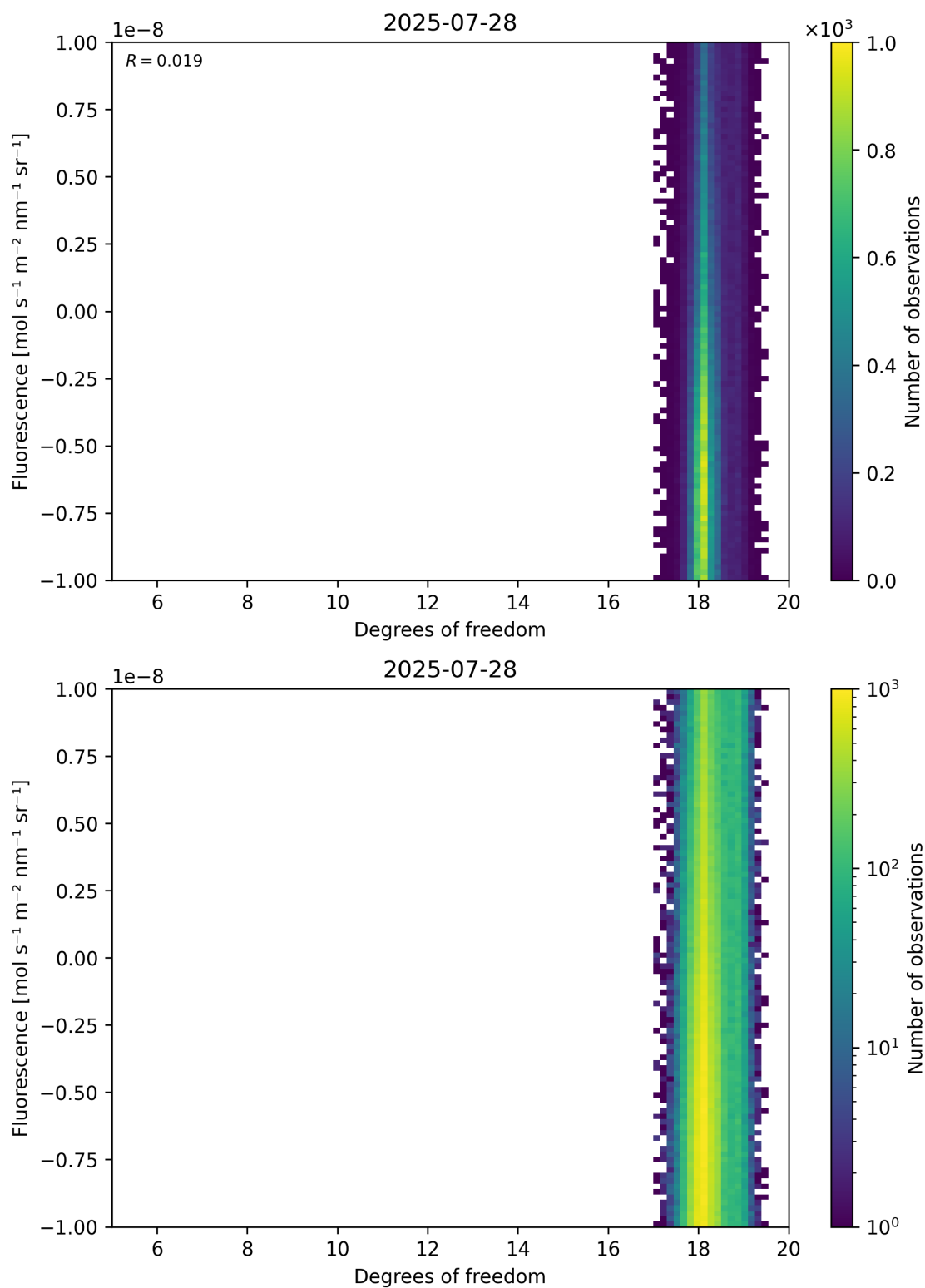
Figure 51: Scatter density plot of “Degrees of freedom” against “Fluorescence” for 2025-07-27 to 2025-07-29.
