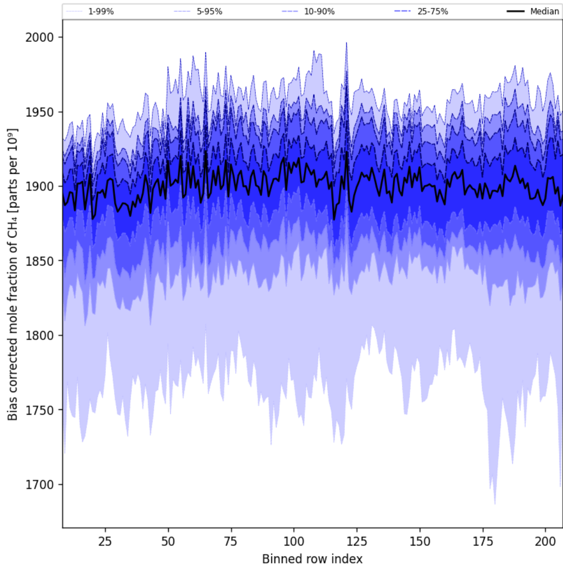
Figure 36: Along track statistics of “Bias corrected mole fraction of CH 4 ” for 2025-07-27 to 2025-07-29
