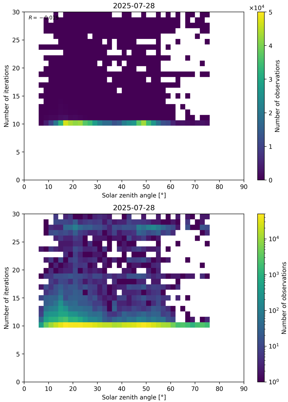
Figure 102: Scatter density plot of “Solar zenith angle” against “Number of iterations” for 2025-07-27 to 2025-07-29.
