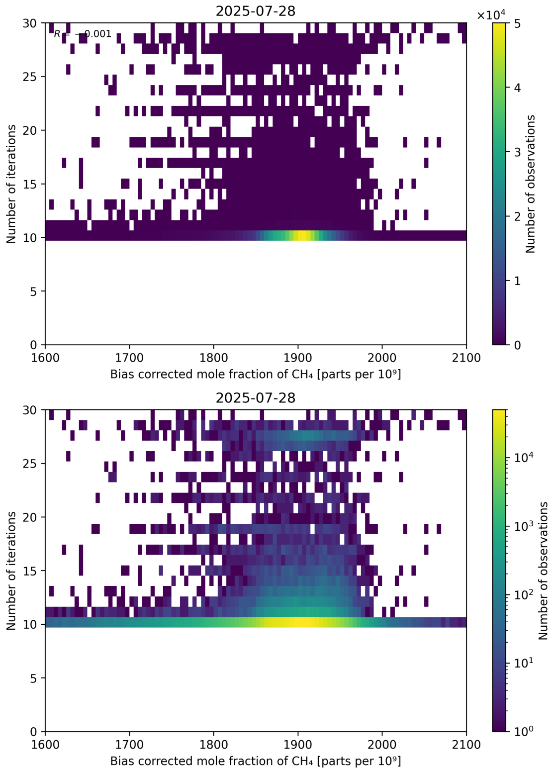
Figure 67: Scatter density plot of “Bias corrected mole fraction of CH 4 ” against “Number of iterations” for 2025-07-27 to 2025-07-29.
