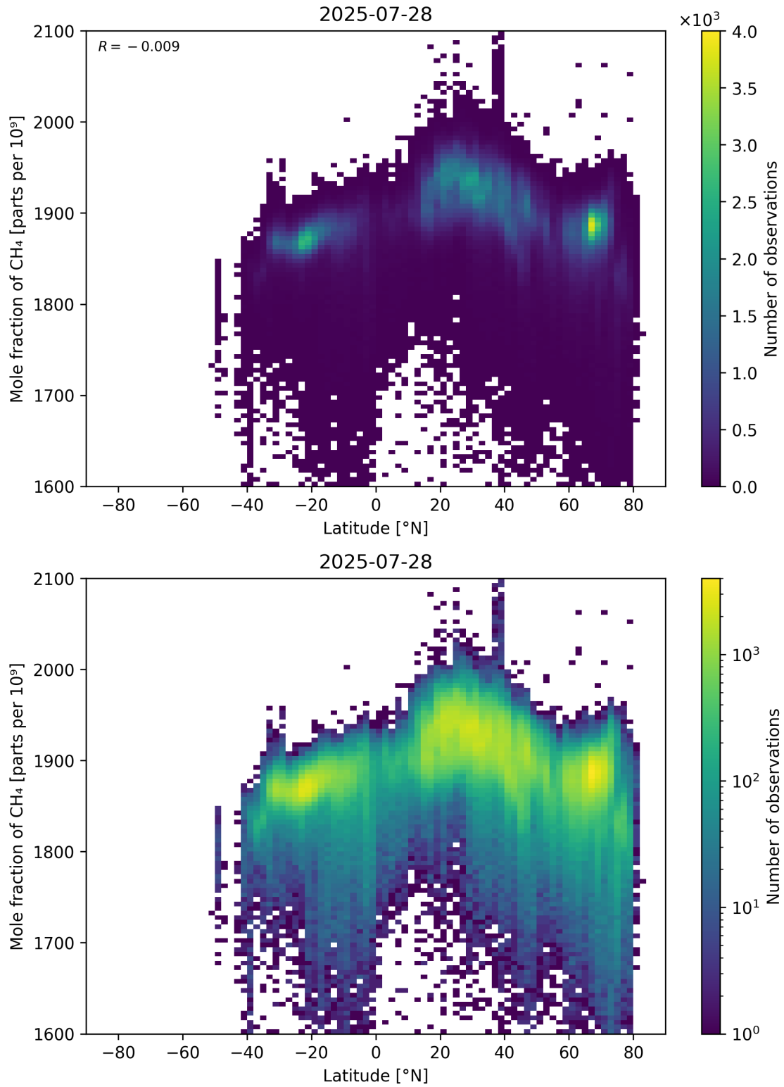
Figure 57: Scatter density plot of “Latitude” against “Mole fraction of \text{CH}_4 ” for 2025-07-27 to 2025-07-29.
