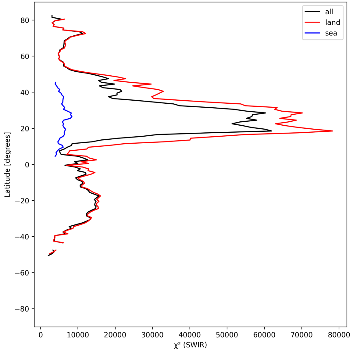
Figure 17: Zonal average of “ \chi^2 (SWIR)” for 2025-07-27 to 2025-07-29.
