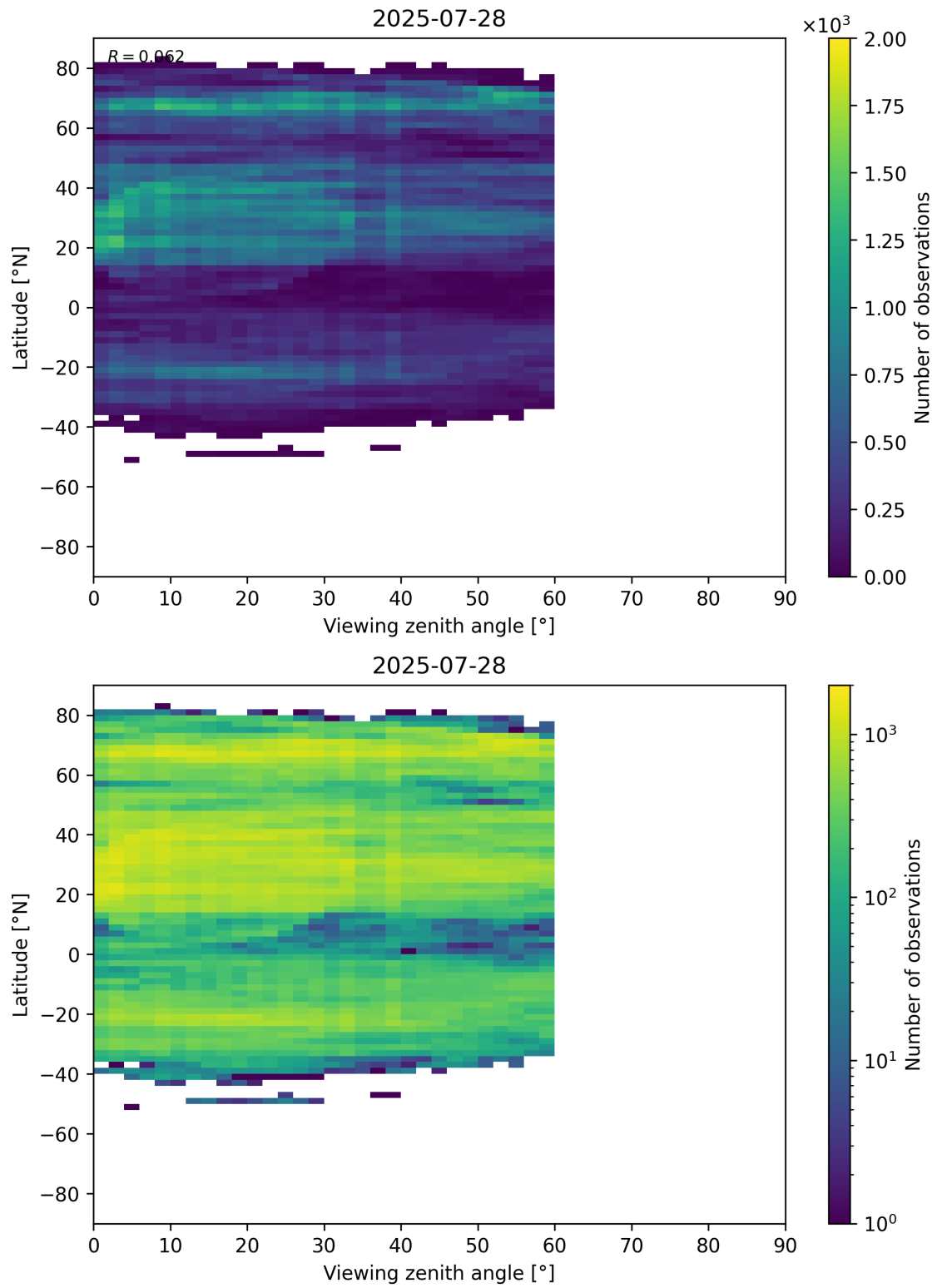
Figure 109: Scatter density plot of “Viewing zenith angle” against “Latitude” for 2025-07-27 to 2025-07-29.
