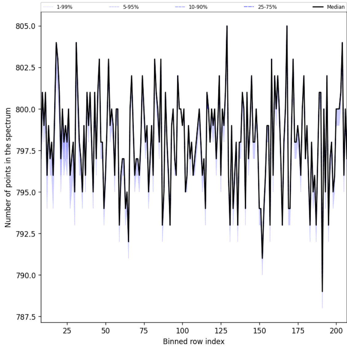
Figure 37: Along track statistics of “Number of points in the spectrum” for 2025-07-27 to 2025-07-29
