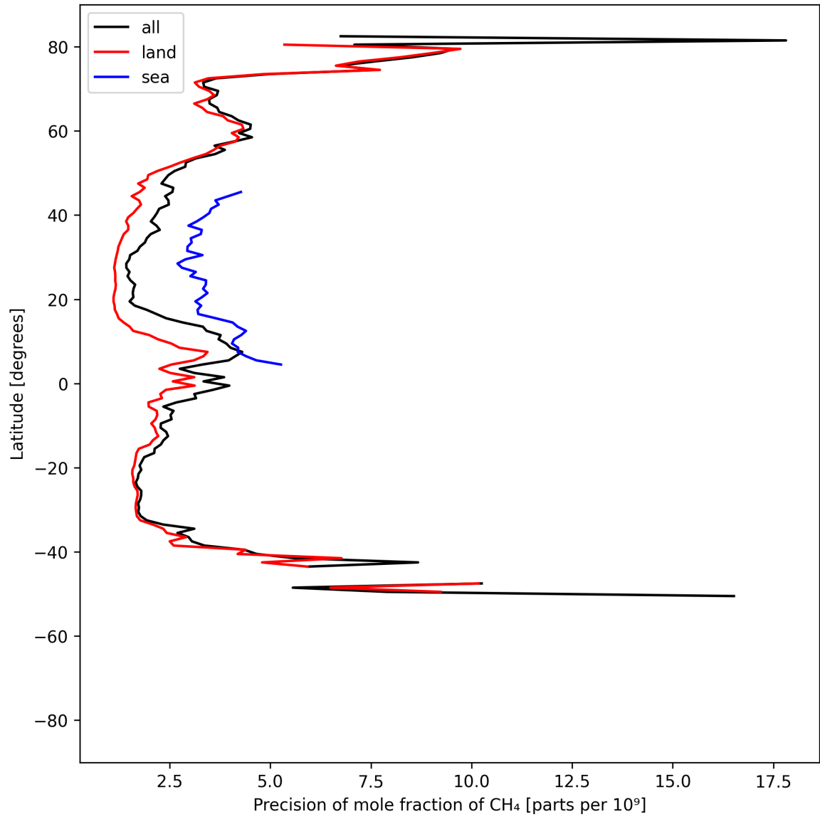
Figure 13: Zonal average of “Precision of mole fraction of CH 4 ” for 2025-07-27 to 2025-07-29.
