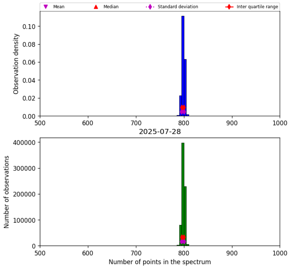
Figure 26: Histogram of “Number of points in the spectrum” for 2025-07-27 to 2025-07-29
