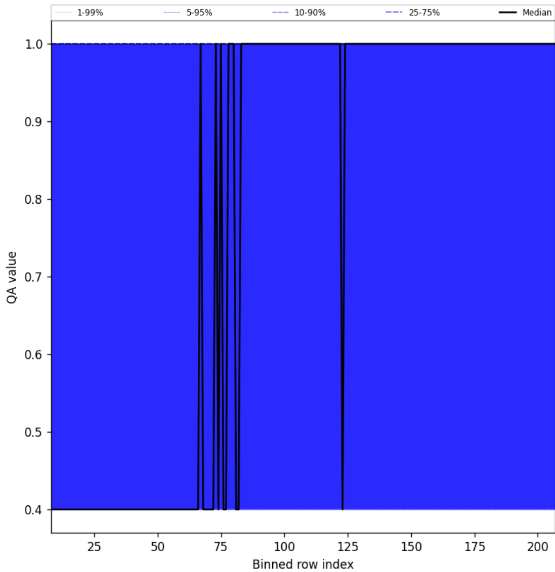
Figure 33: Along track statistics of “QA value” for 2025-07-27 to 2025-07-29
