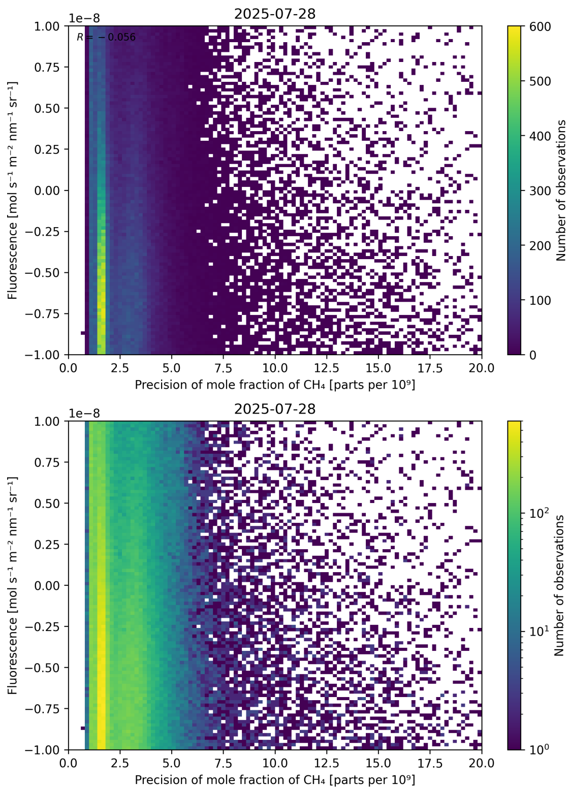
Figure 81: Scatter density plot of “Precision of mole fraction of CH 4 ” against “Fluorescence” for 2025-07-27 to 2025-07-29.
