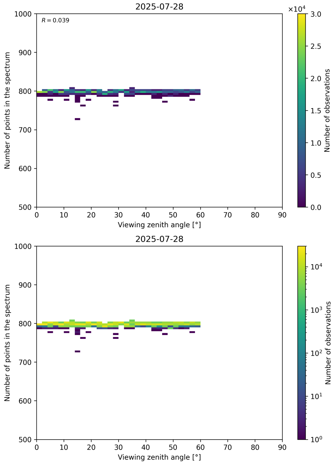
Figure 114: Scatter density plot of “Viewing zenith angle” against “Number of points in the spectrum” for 2025-07-27 to 2025-07-29.
