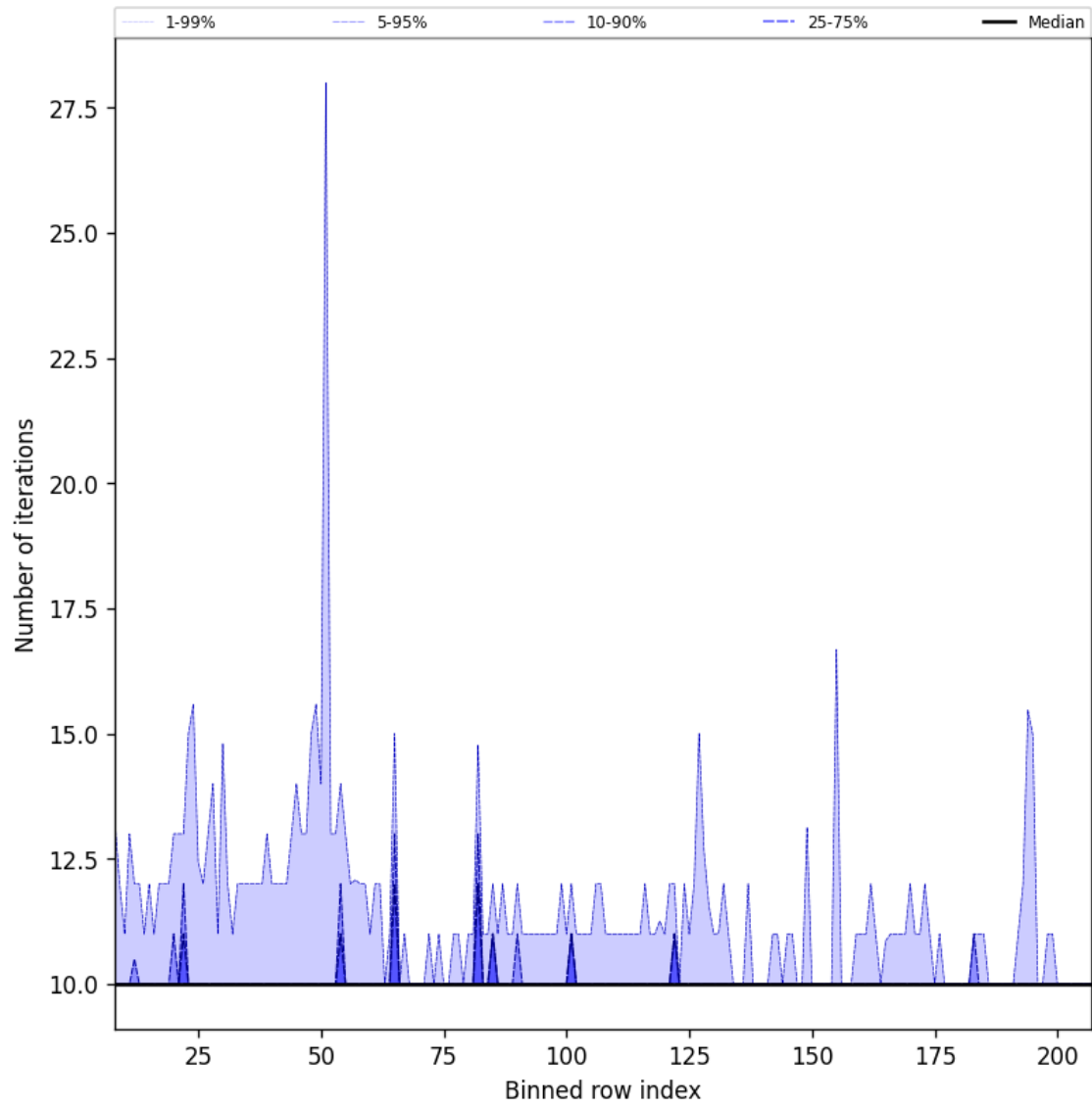
Figure 42: Along track statistics of “Number of iterations” for 2025-07-27 to 2025-07-29
