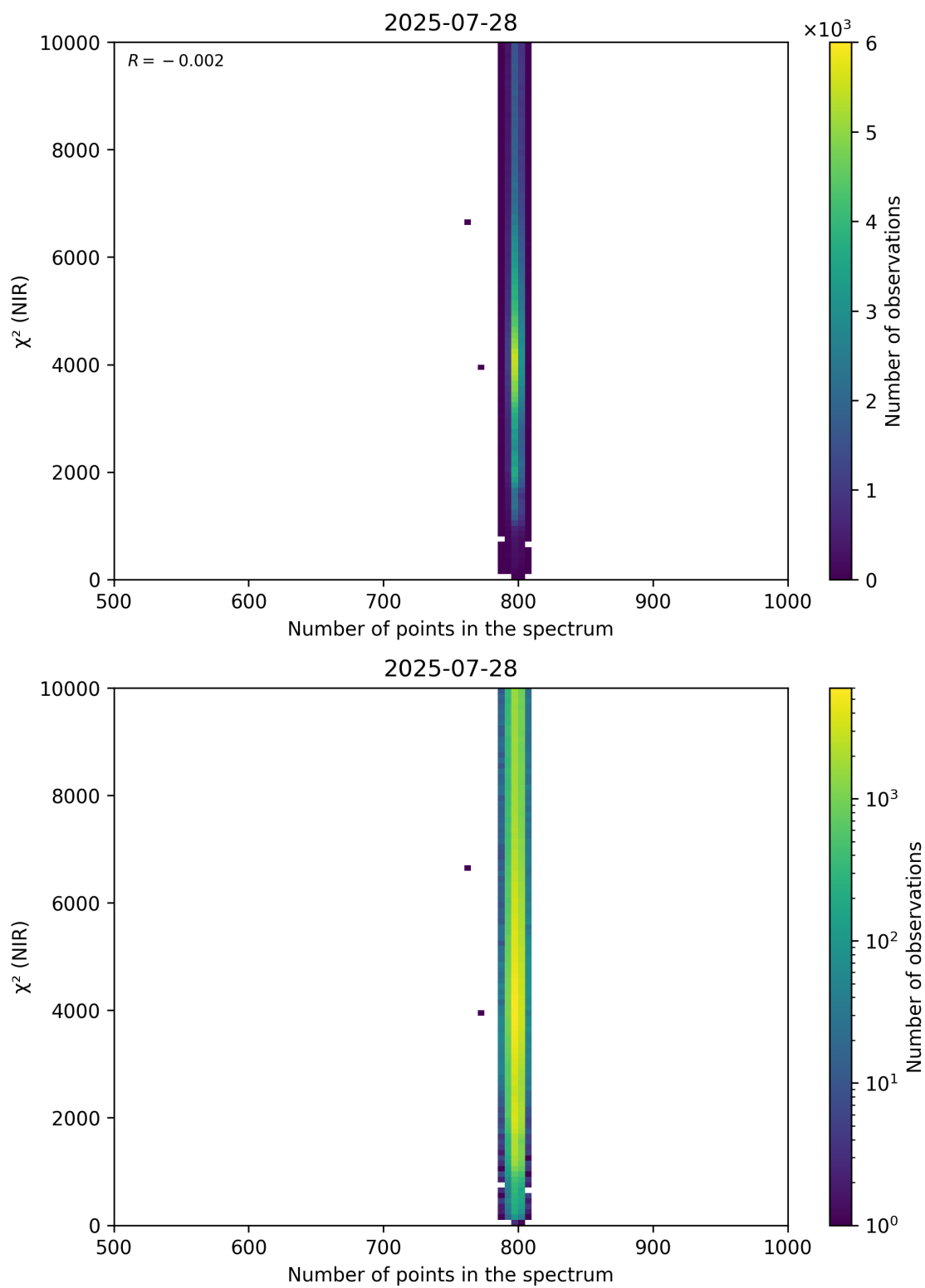
Figure 88: Scatter density plot of “Number of points in the spectrum” against “ \chi^2 (NIR)” for 2025-07-27 to 2025-07-29.
