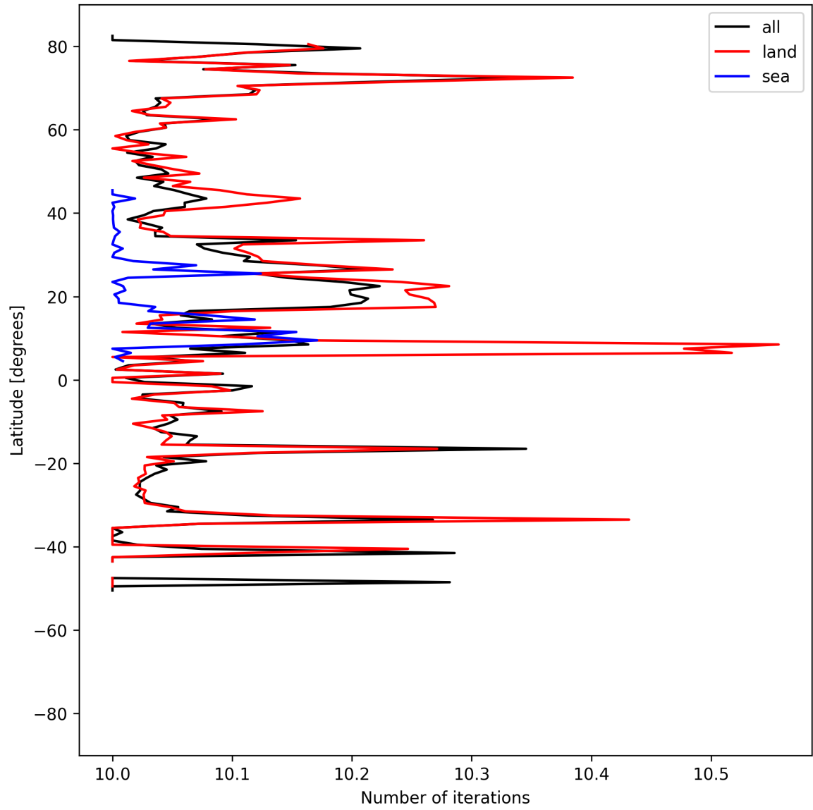
Figure 20: Zonal average of “Number of iterations” for 2025-07-27 to 2025-07-29.
