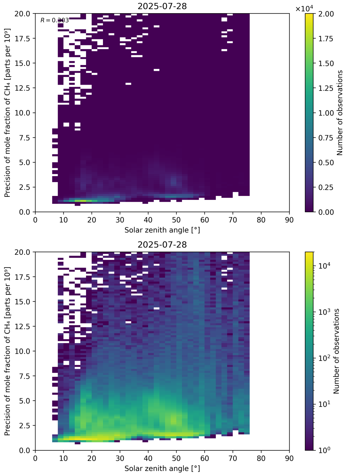
Figure 101: Scatter density plot of “Solar zenith angle” against “Precision of mole fraction of CH 4 ” for 2025-07-27 to 2025-07-29.
