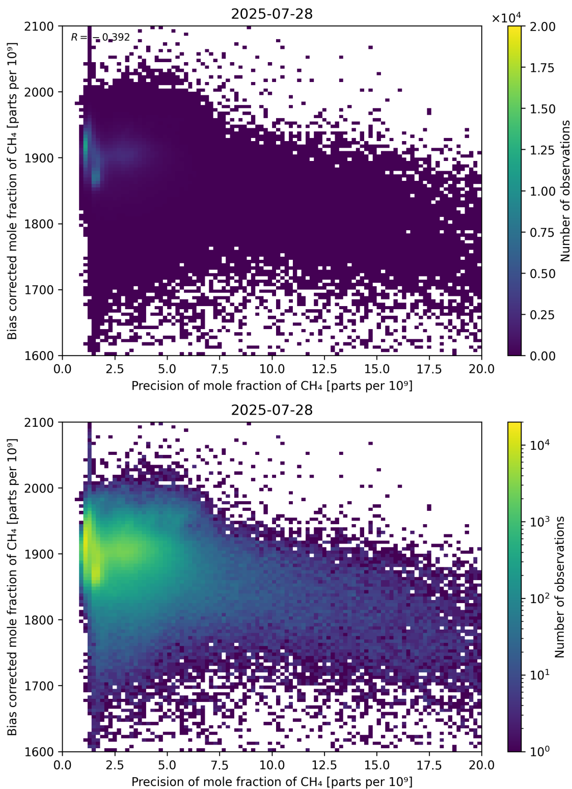
Figure 82: Scatter density plot of “Precision of mole fraction of CH 4 ” against “Bias corrected mole fraction of CH 4 ” for 2025-07-27 to 2025-07-29.
