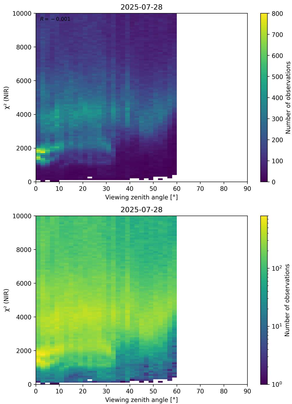
Figure 105: Scatter density plot of “Viewing zenith angle” against “ \chi^2 (NIR)” for 2025-07-27 to 2025-07-29.
