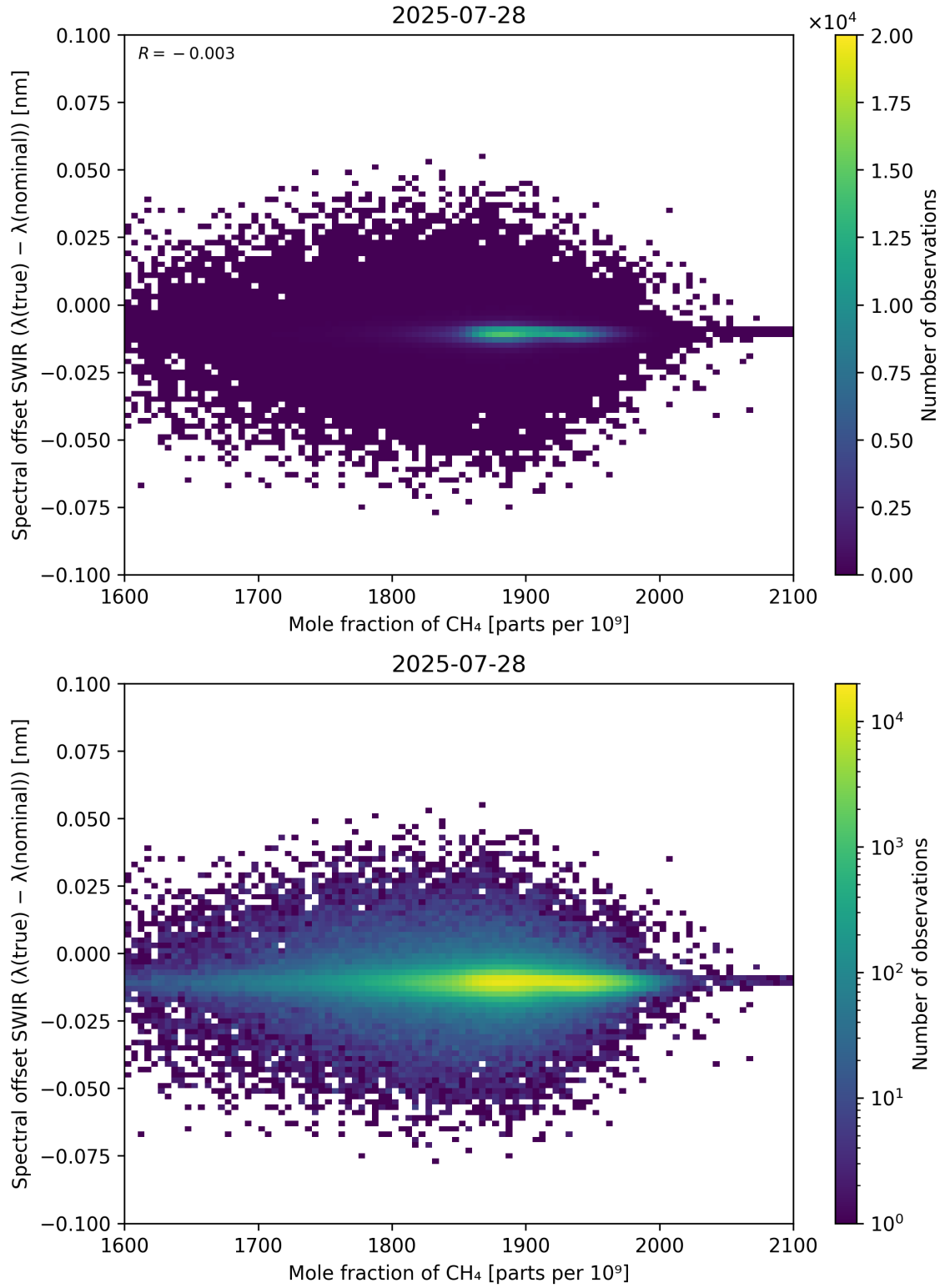
Figure 86: Scatter density plot of “Mole fraction of CH 4 ” against “Spectral offset SWIR ( \lambda_{\text{true}} - \lambda_{\text{nominal}} )” for 2025-07-27 to 2025-07-29.
