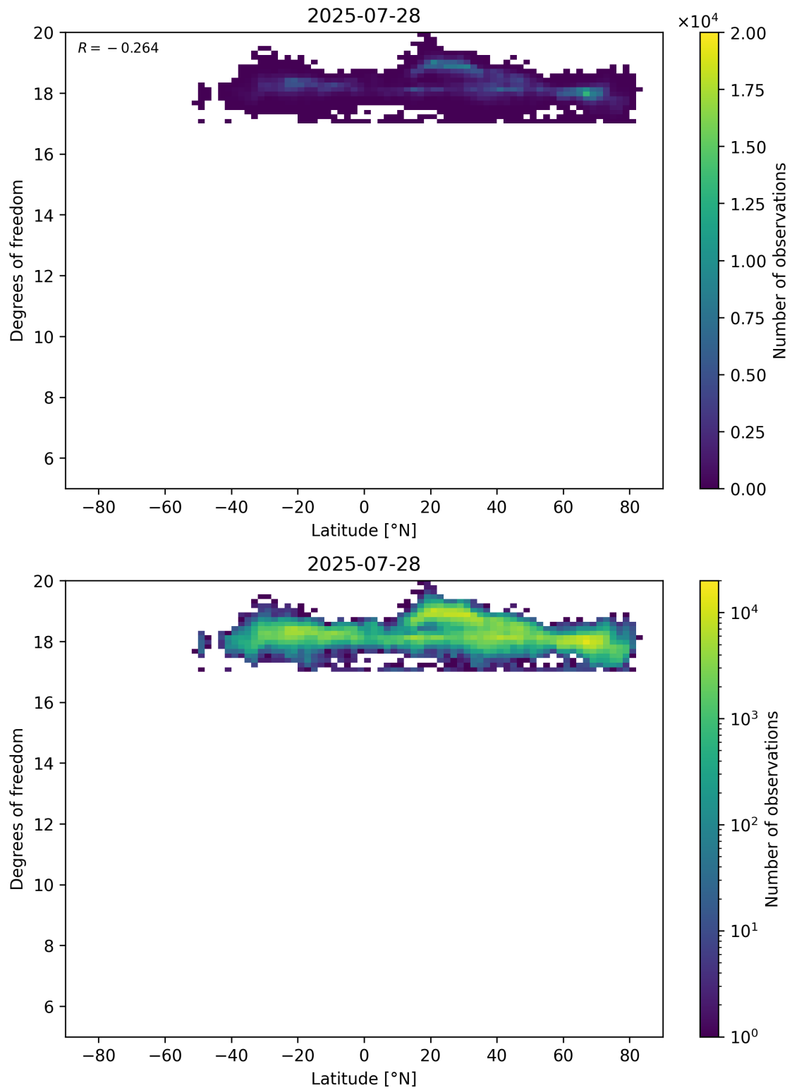
Figure 55: Scatter density plot of “Latitude” against “Degrees of freedom” for 2025-07-27 to 2025-07-29.
