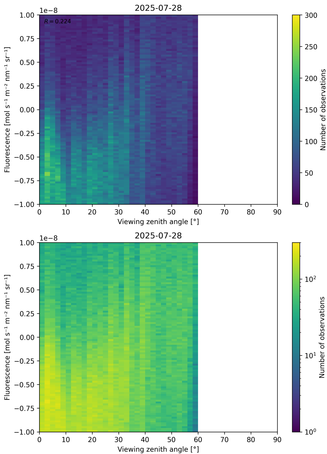
Figure 108: Scatter density plot of “Viewing zenith angle” against “Fluorescence” for 2025-07-27 to 2025-07-29.
