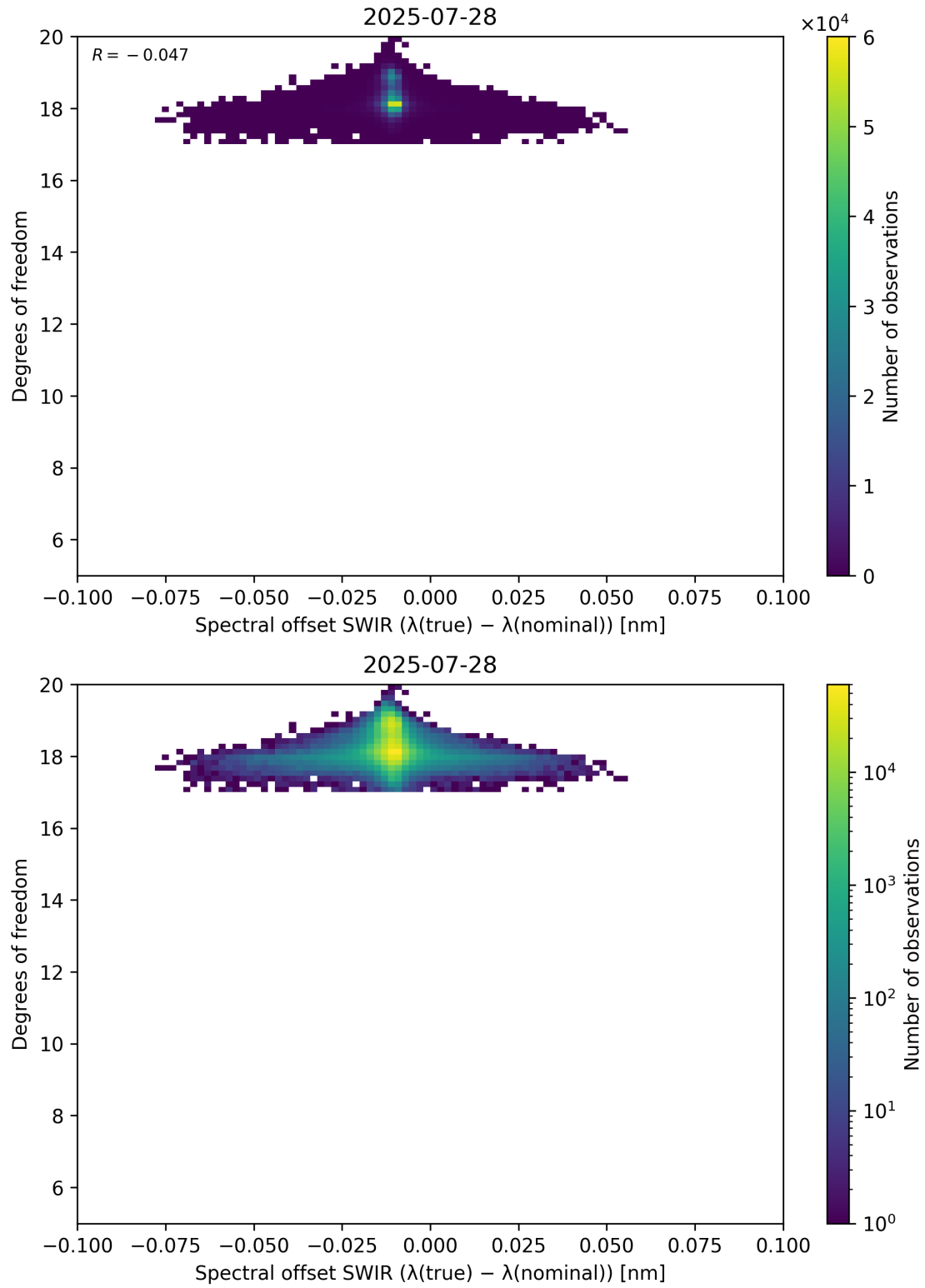
Figure 119: Scatter density plot of “Spectral offset SWIR ( \lambda_{\text{true}} - \lambda_{\text{nominal}} )” against “Degrees of freedom” for 2025-07-27 to 2025-07-29.
