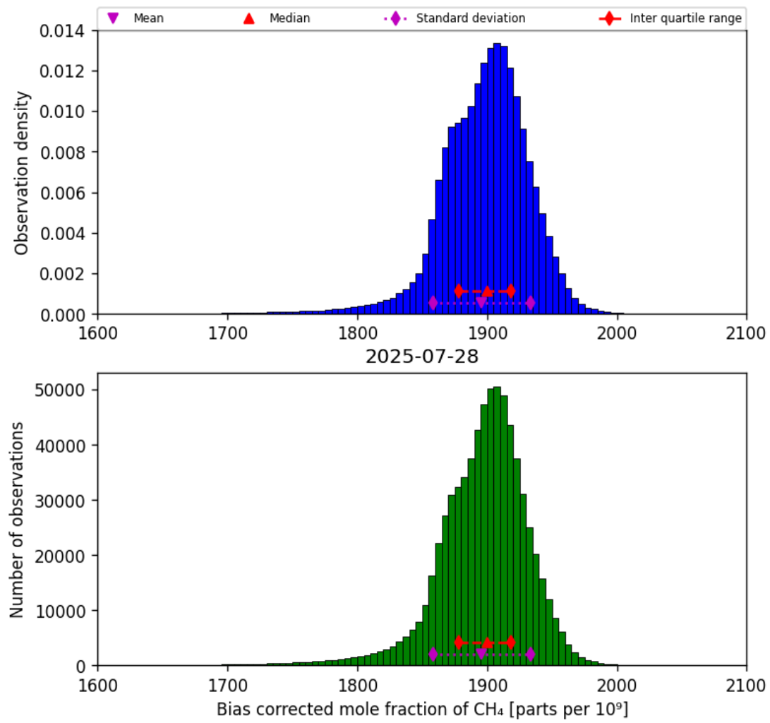
Figure 25: Histogram of “Bias corrected mole fraction of CH 4 ” for 2025-07-27 to 2025-07-29
