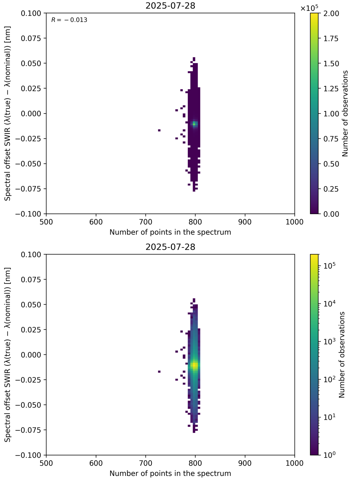
Figure 93: Scatter density plot of “Number of points in the spectrum” against “Spectral offset SWIR ( \lambda_{\text{true}} - \lambda_{\text{nominal}} )” for 2025-07-27 to 2025-07-29.
