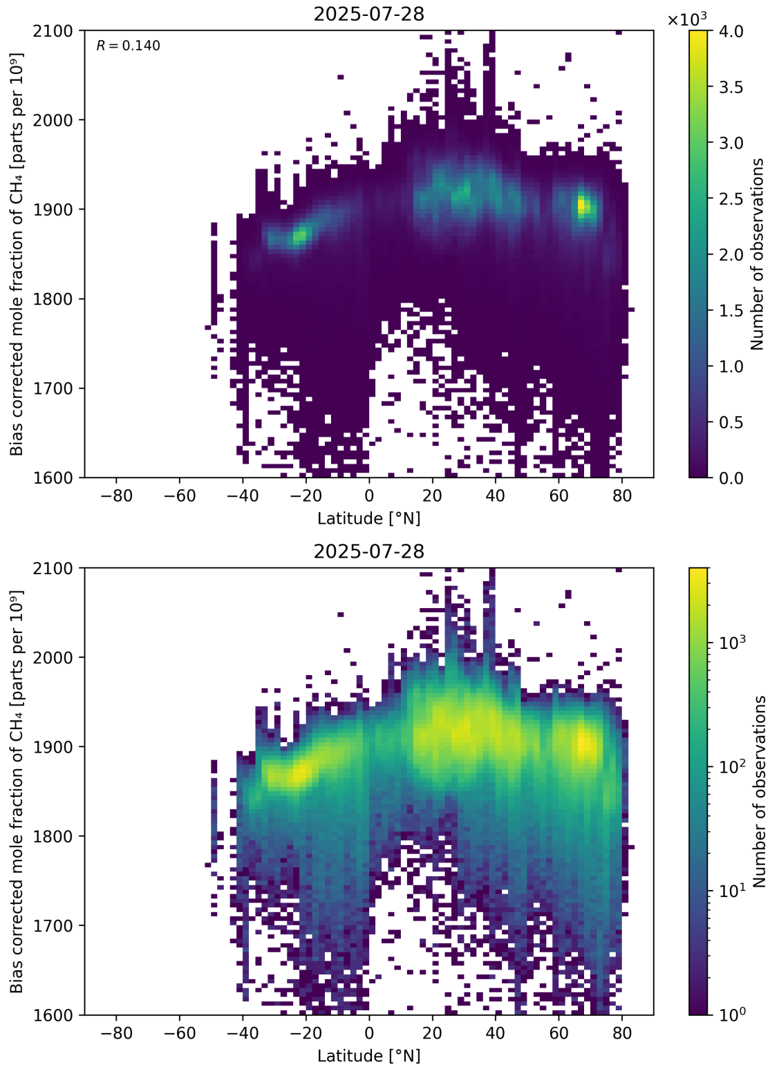
Figure 58: Scatter density plot of “Latitude” against “Bias corrected mole fraction of \text{CH}_4 ” for 2025-07-27 to 2025-07-29.
