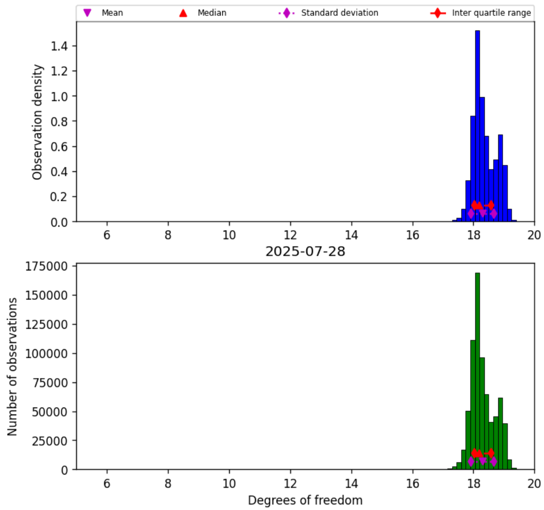
Figure 30: Histogram of “Degrees of freedom” for 2025-07-27 to 2025-07-29
