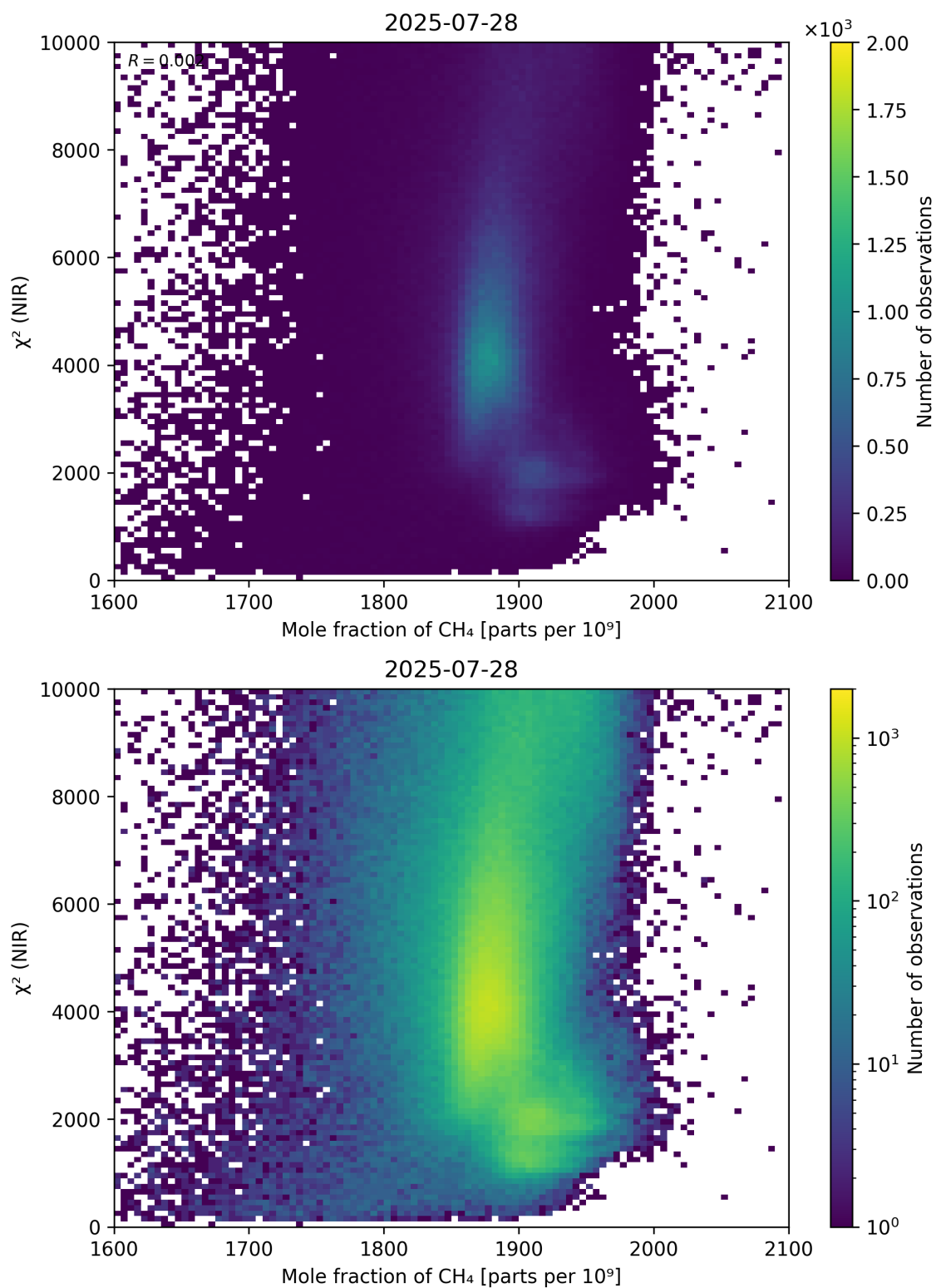
Figure 70: Scatter density plot of “Mole fraction of \text{CH}_4 ” against “ \chi^2 (NIR)” for 2025-07-27 to 2025-07-29.
