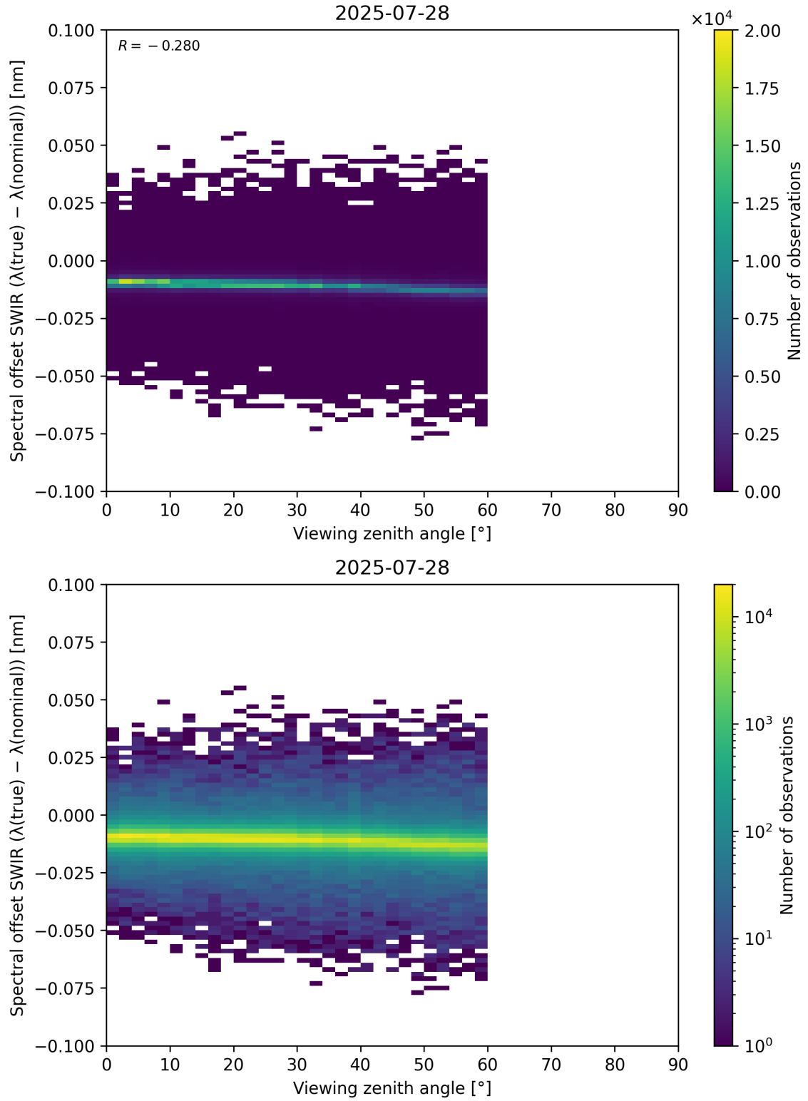
Figure 116: Scatter density plot of “Viewing zenith angle” against “Spectral offset SWIR ( \lambda_{\text{true}} - \lambda_{\text{nominal}} )” for 2025-07-27 to 2025-07-29.
