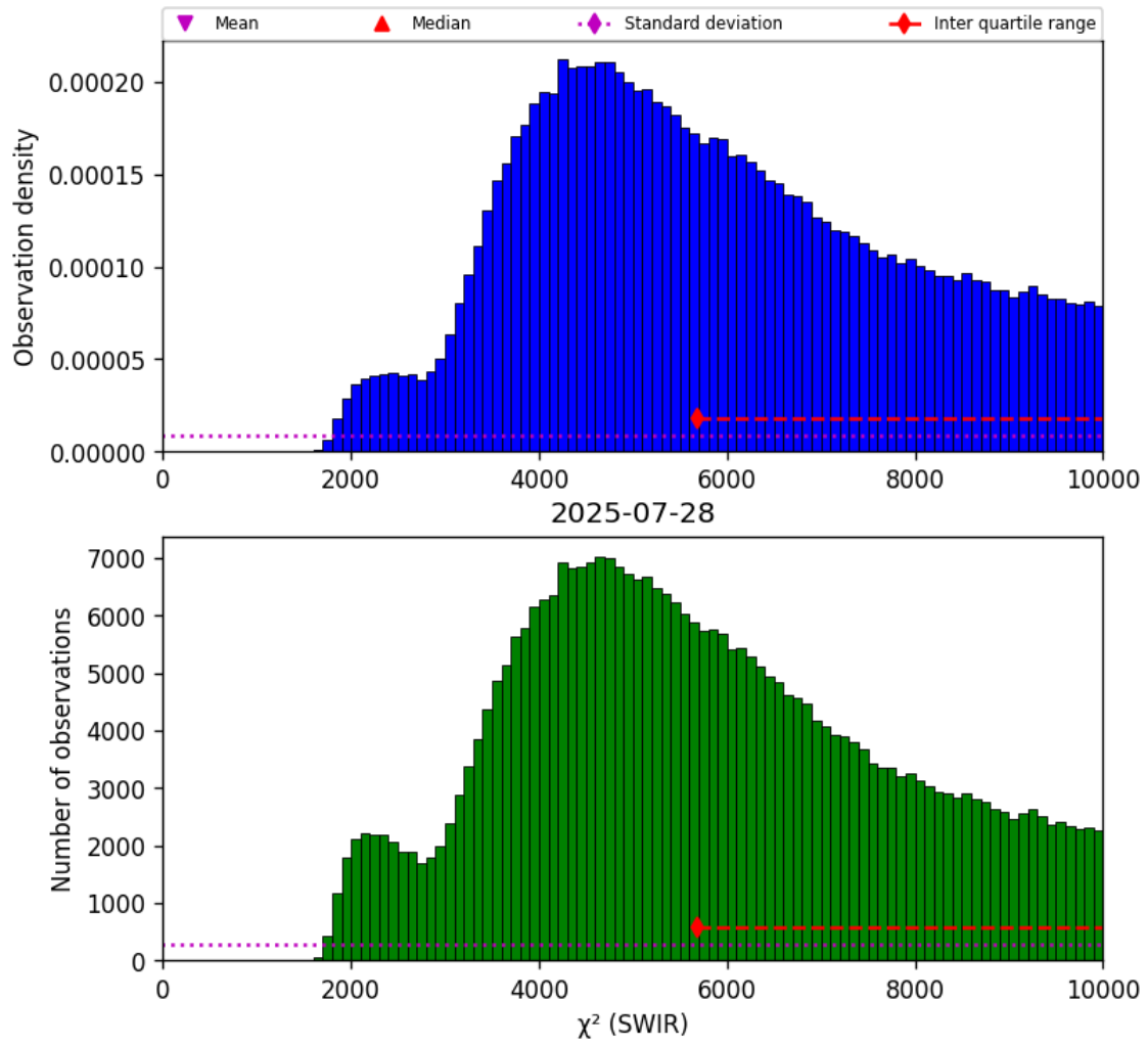
Figure 28: Histogram of “ \chi^2 (SWIR)” for 2025-07-27 to 2025-07-29
