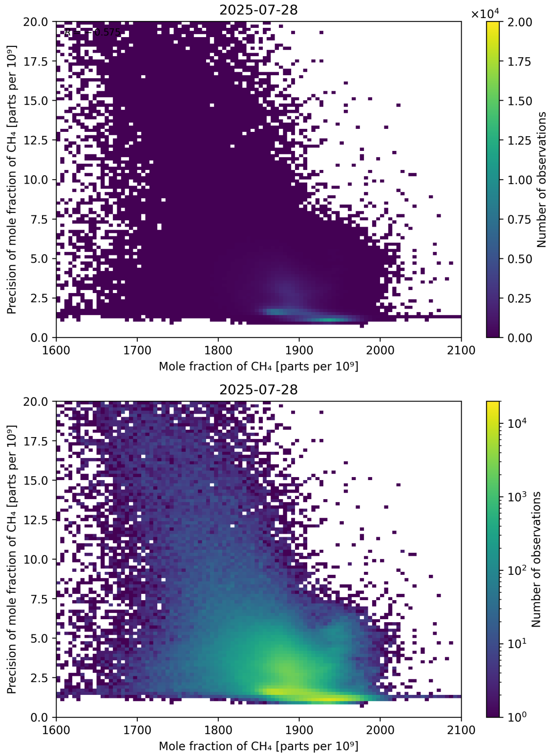
Figure 75: Scatter density plot of “Mole fraction of CH 4 ” against “Precision of mole fraction of CH 4 ” for 2025-07-27 to 2025-07-29.
