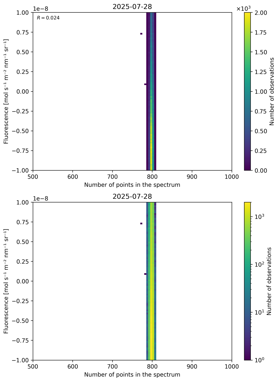
Figure 91: Scatter density plot of “Number of points in the spectrum” against “Fluorescence” for 2025-07-27 to 2025-07-29.
