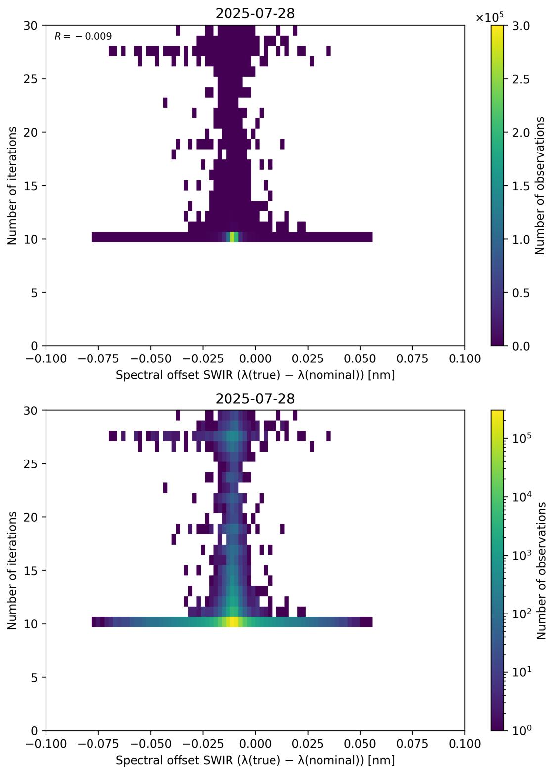
Figure 121: Scatter density plot of “Spectral offset SWIR ( \lambda_{\text{true}} - \lambda_{\text{nominal}} )” against “Number of iterations” for 2025-07-27 to 2025-07-29.
