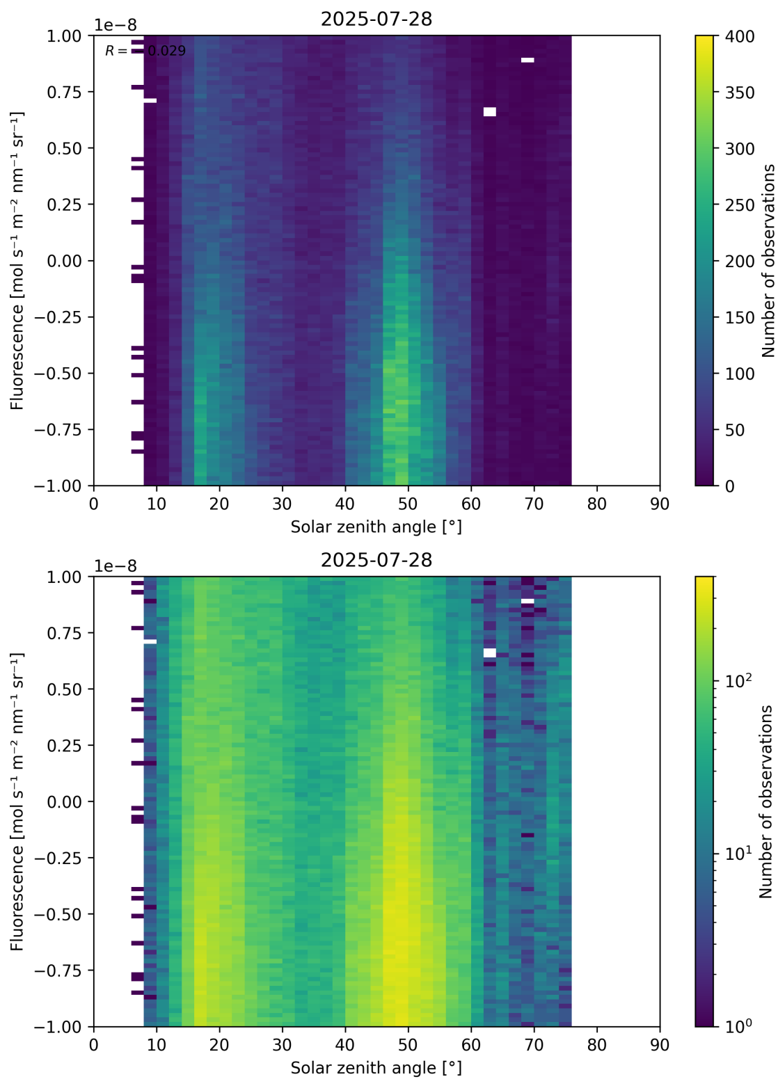
Figure 97: Scatter density plot of “Solar zenith angle” against “Fluorescence” for 2025-07-27 to 2025-07-29.
