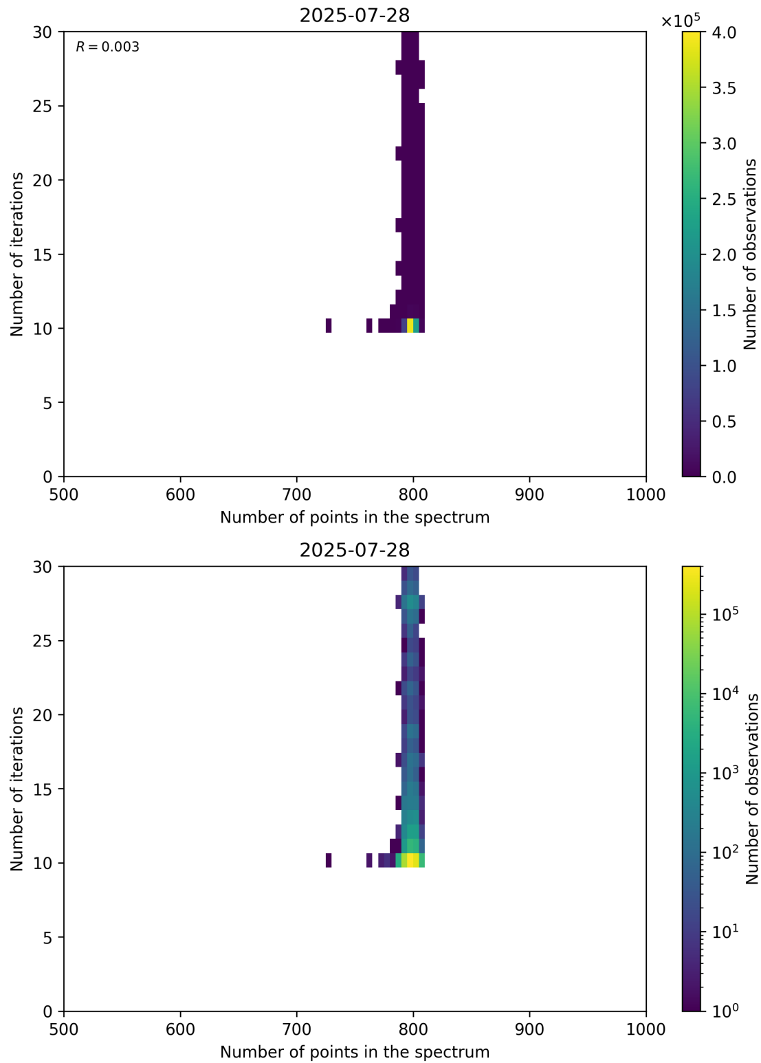
Figure 92: Scatter density plot of “Number of points in the spectrum” against “Number of iterations” for 2025-07-27 to 2025-07-29.
