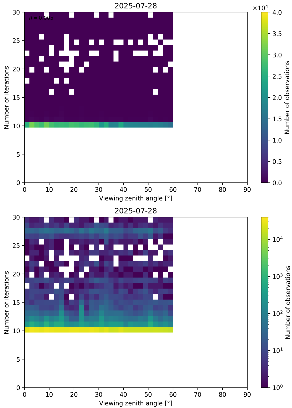
Figure 113: Scatter density plot of “Viewing zenith angle” against “Number of iterations” for 2025-07-27 to 2025-07-29.
