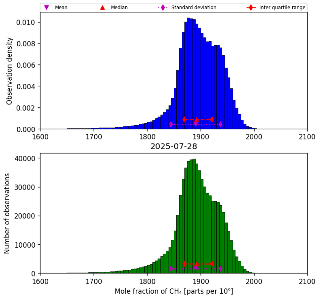
Figure 23: Histogram of “Mole fraction of CH 4 ” for 2025-07-27 to 2025-07-29
