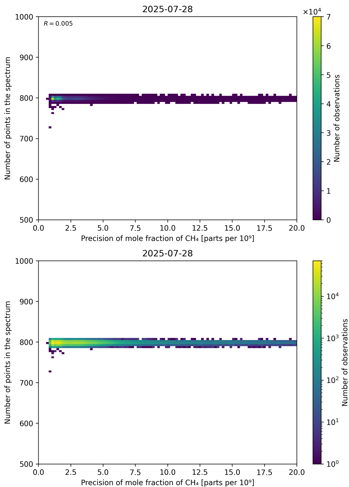
Figure 84: Scatter density plot of “Precision of mole fraction of CH 4 ” against “Number of points in the spectrum” for 2025-07-27 to 2025-07-29.
