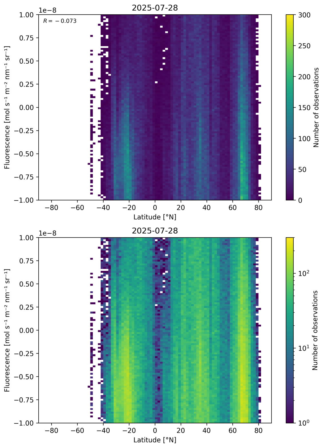
Figure 56: Scatter density plot of “Latitude” against “Fluorescence” for 2025-07-27 to 2025-07-29.
