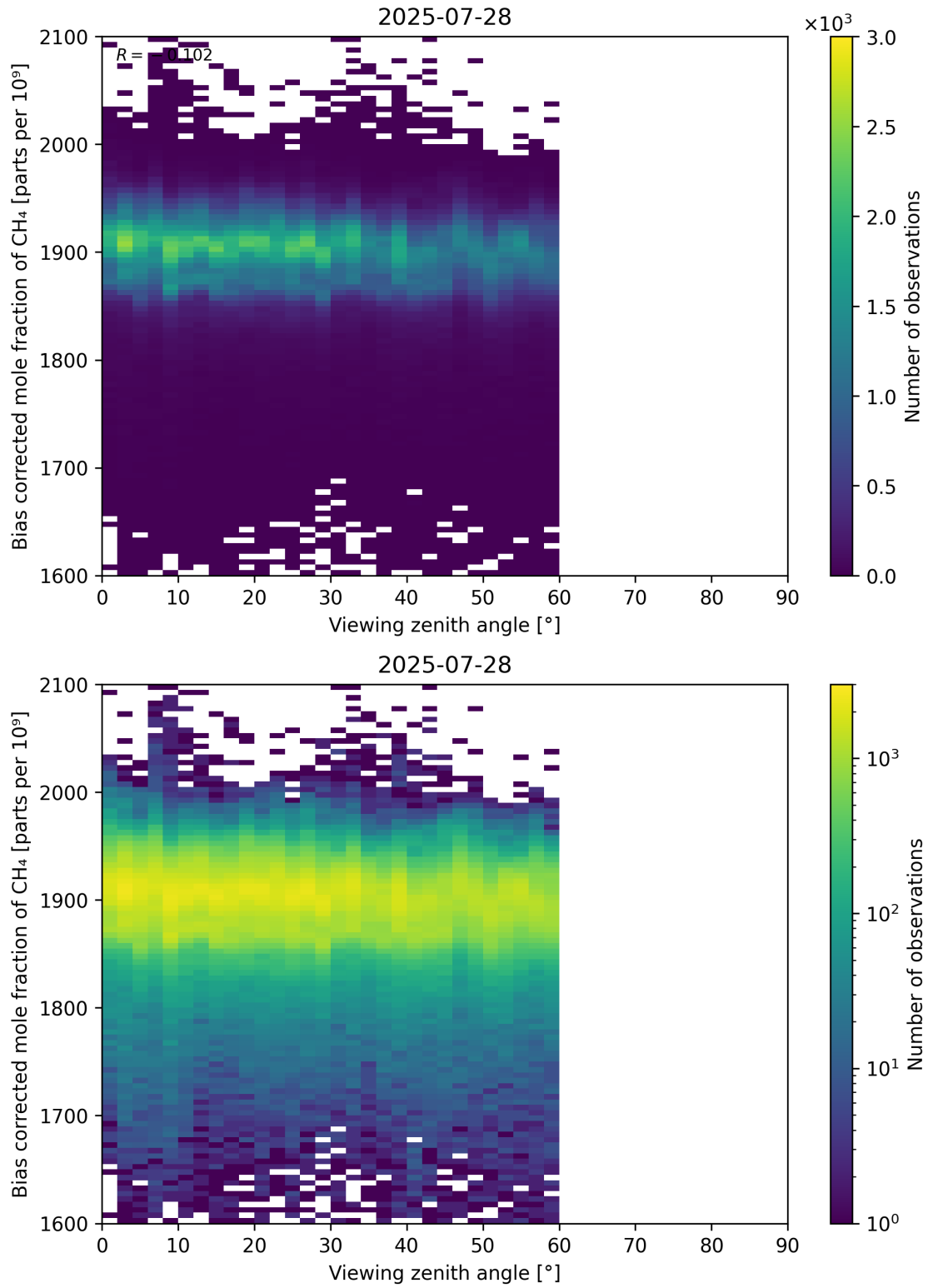
Figure 111: Scatter density plot of “Viewing zenith angle” against “Bias corrected mole fraction of CH 4 ” for 2025-07-27 to 2025-07-29.
