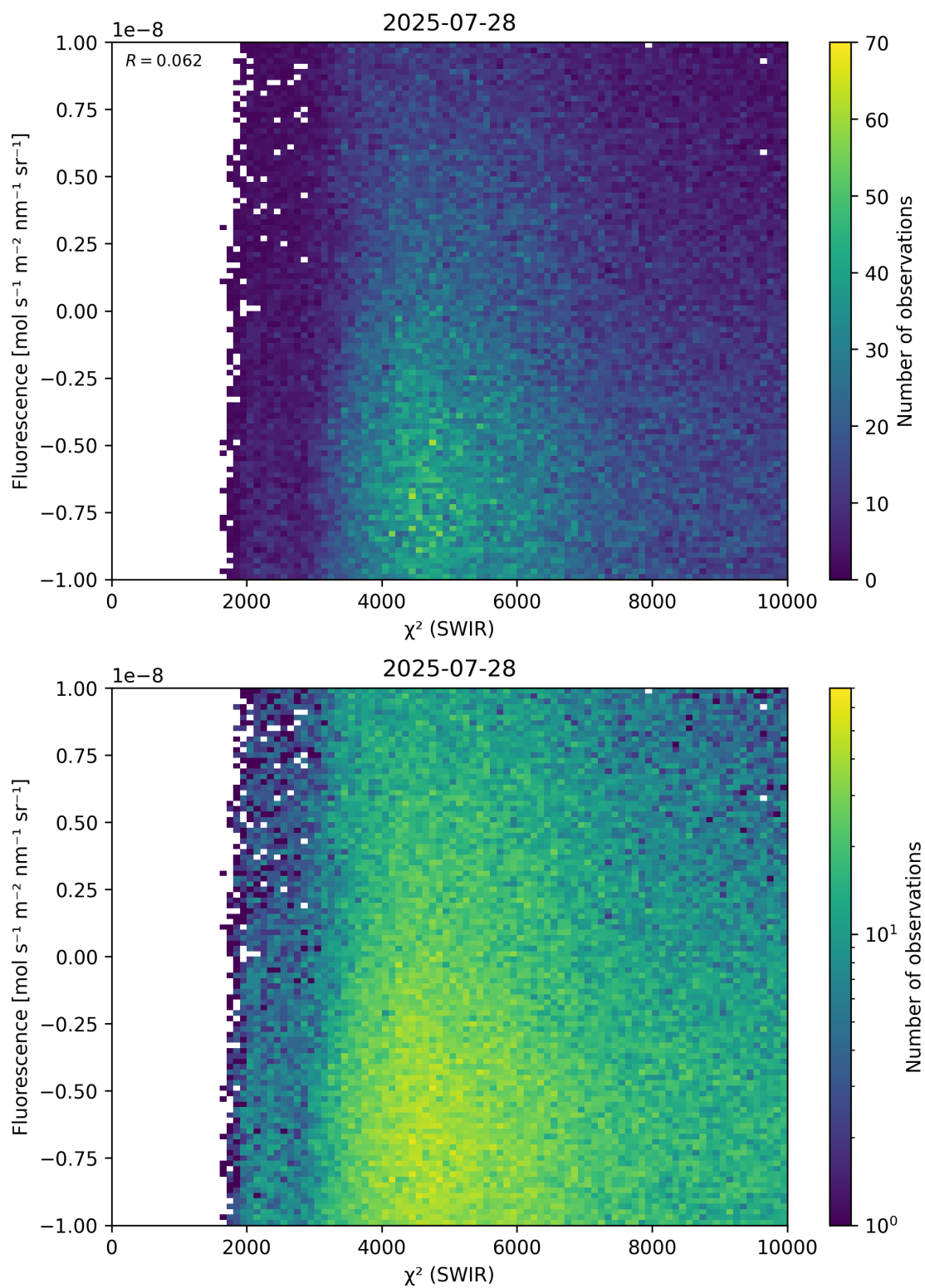
Figure 49: Scatter density plot of “ \chi^2 (SWIR)” against “Fluorescence” for 2025-07-27 to 2025-07-29.
