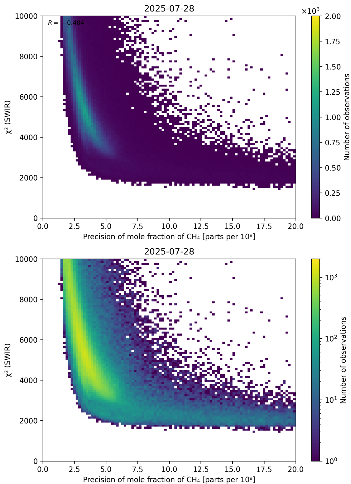
Figure 79: Scatter density plot of “Precision of mole fraction of CH 4 ” against “ \chi^2 (SWIR)” for 2025-07-27 to 2025-07-29.
