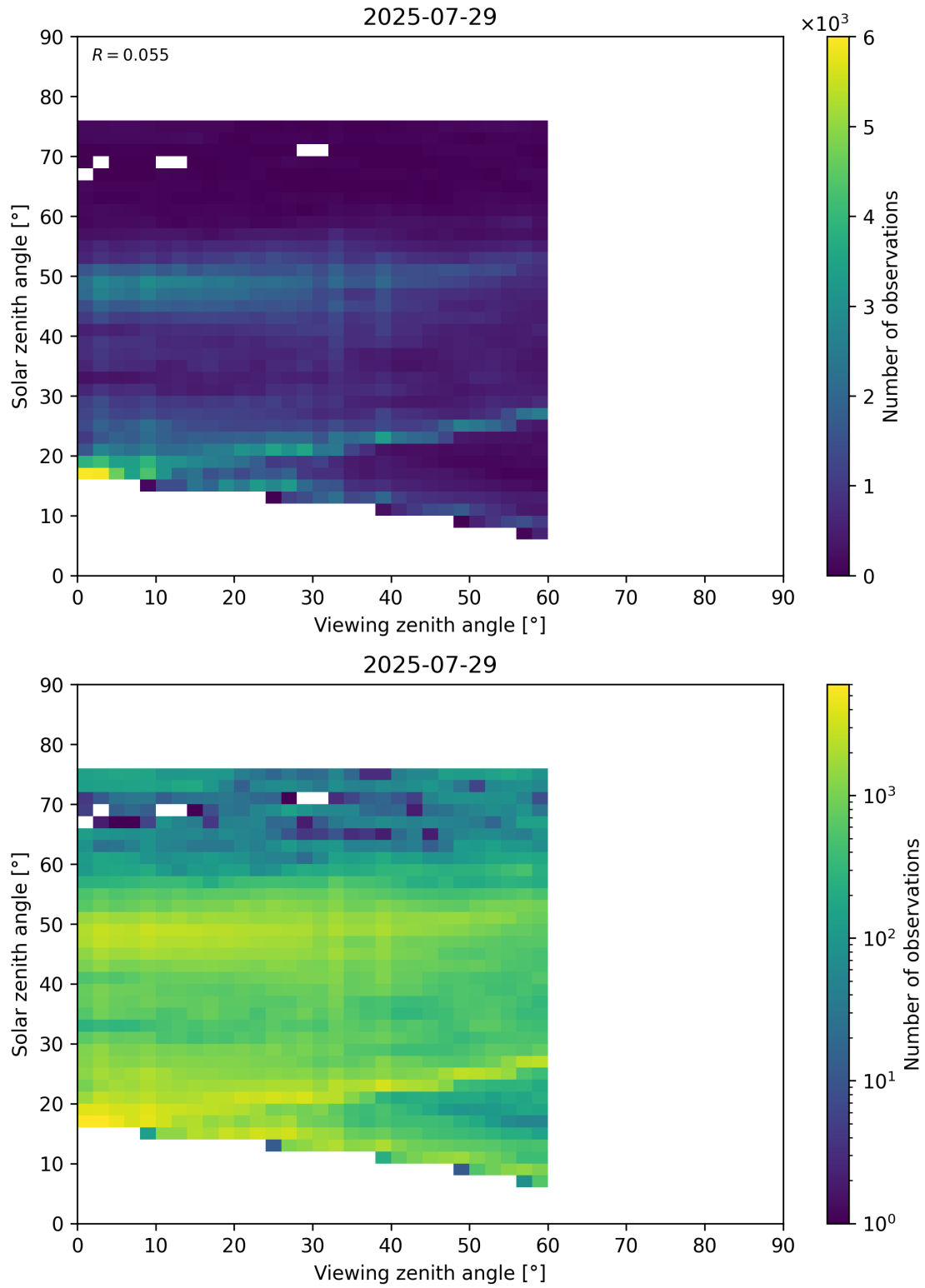
Figure 115: Scatter density plot of “Viewing zenith angle” against “Solar zenith angle” for 2025-07-29 to 2025-07-30.
