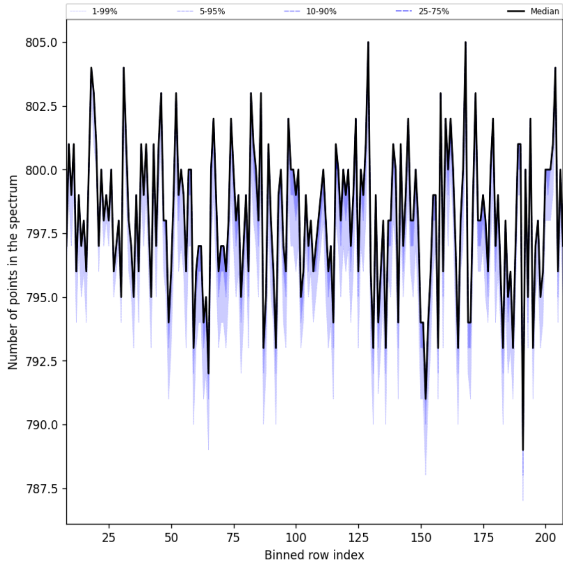
Figure 37: Along track statistics of “Number of points in the spectrum” for 2025-07-29 to 2025-07-30
