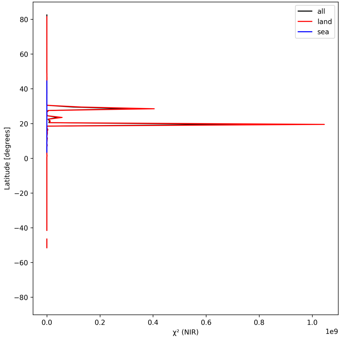
Figure 18: Zonal average of “ \chi^2 (NIR)” for 2025-07-29 to 2025-07-30.
