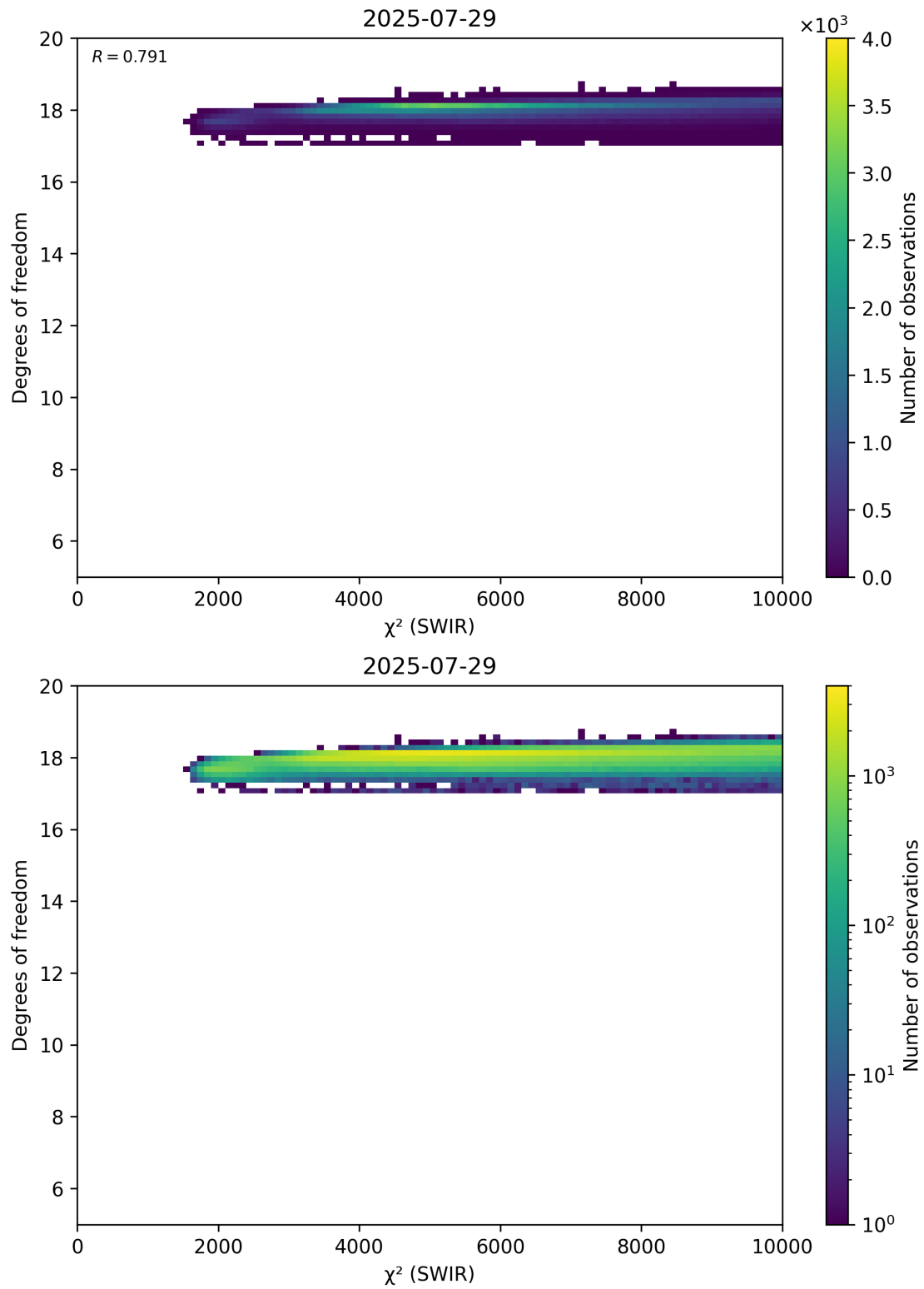
Figure 48: Scatter density plot of “ \chi^2 (SWIR)” against “Degrees of freedom” for 2025-07-29 to 2025-07-30.
