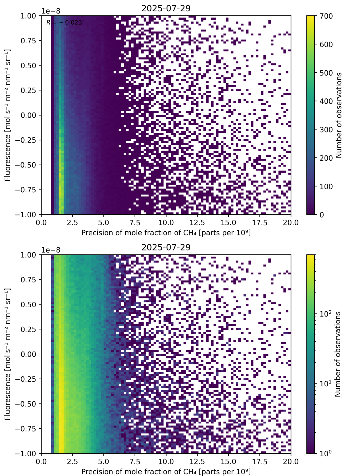
Figure 81: Scatter density plot of “Precision of mole fraction of \text{CH}_4 ” against “Fluorescence” for 2025-07-29 to 2025-07-30.
