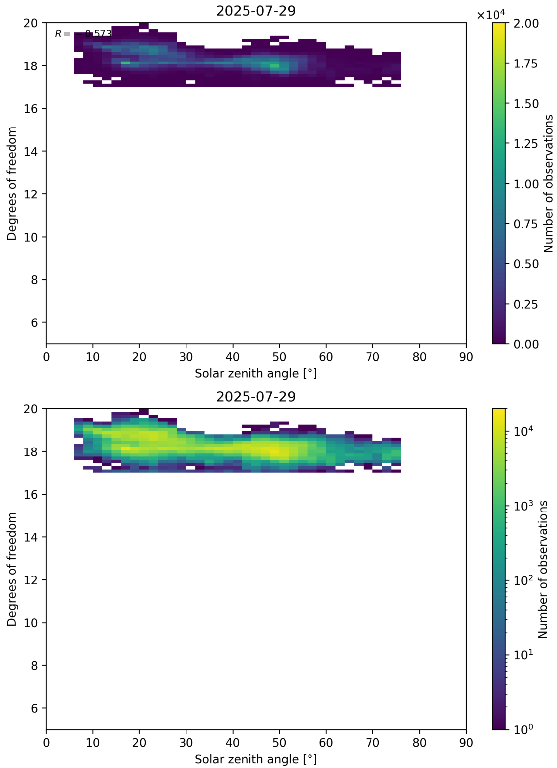
Figure 96: Scatter density plot of “Solar zenith angle” against “Degrees of freedom” for 2025-07-29 to 2025-07-30.
