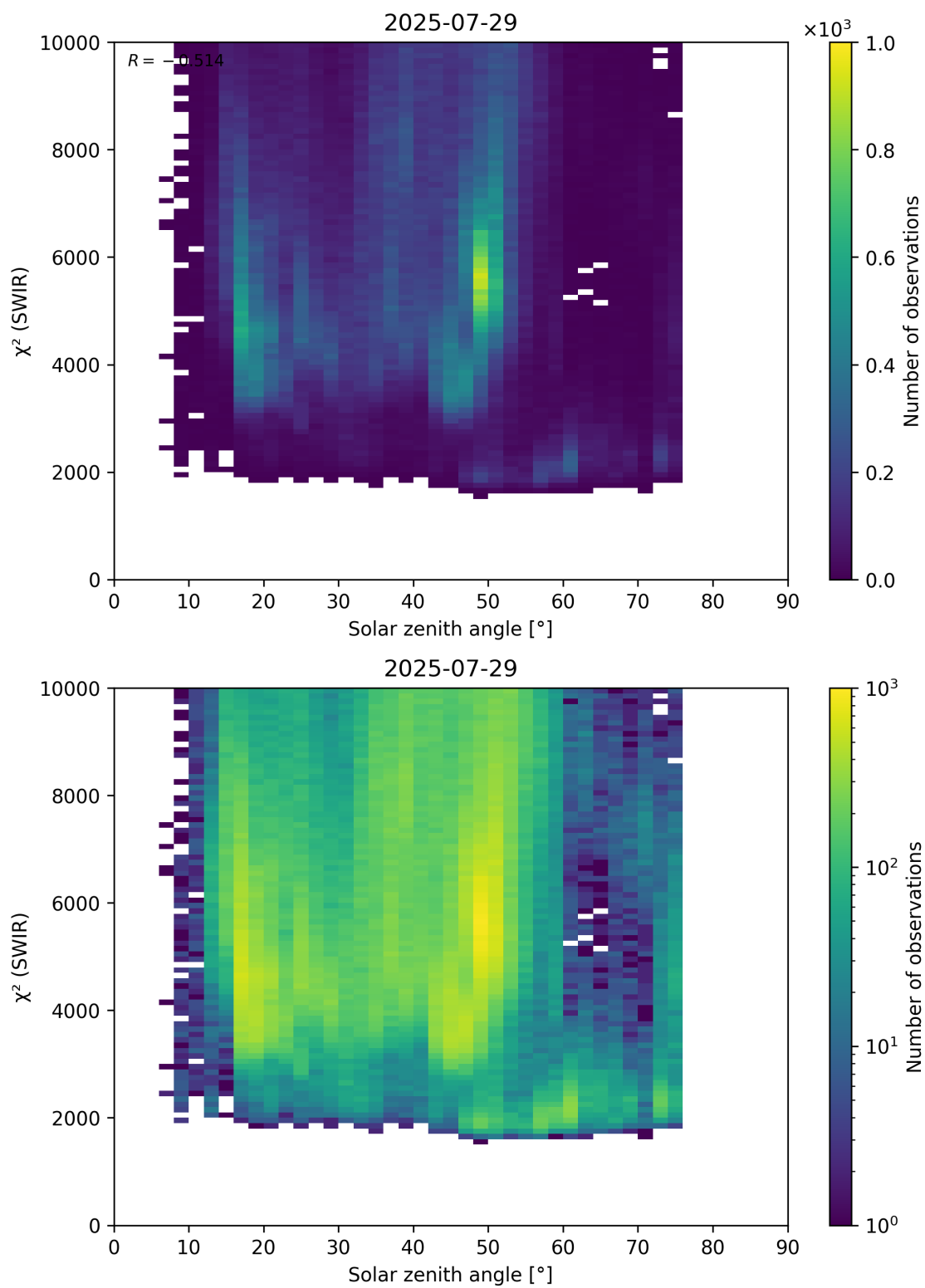
Figure 95: Scatter density plot of “Solar zenith angle” against “ \chi^2 (SWIR)” for 2025-07-29 to 2025-07-30.
