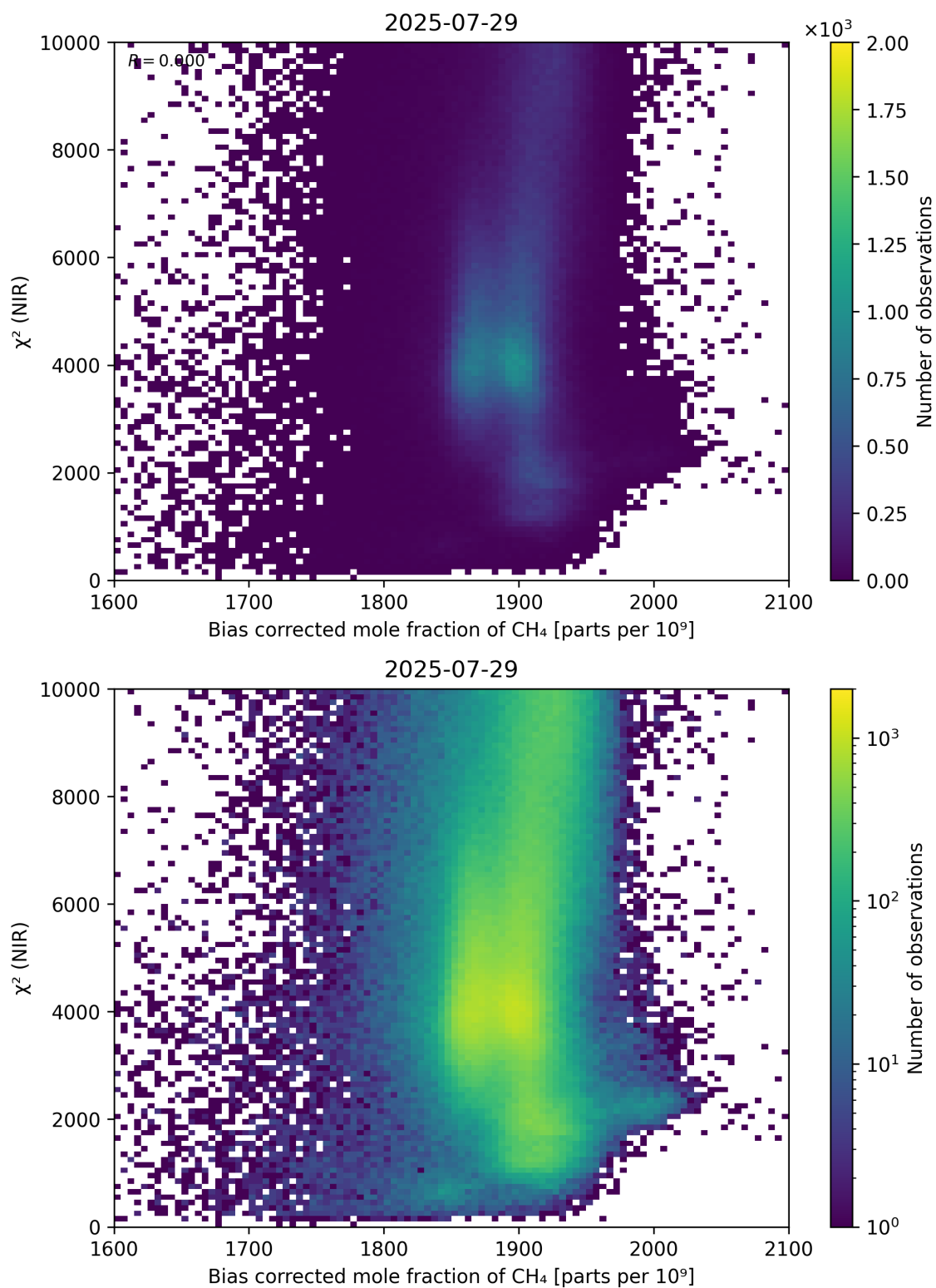
Figure 63: Scatter density plot of “Bias corrected mole fraction of \text{CH}_4 ” against “ \chi^2 (NIR)” for 2025-07-29 to 2025-07-30.
