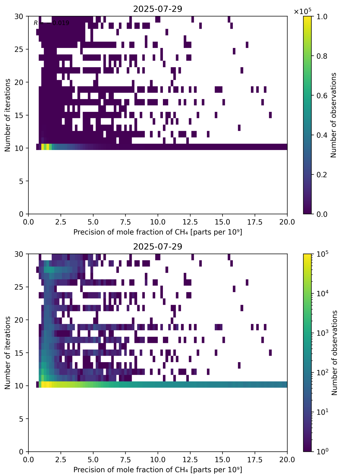
Figure 83: Scatter density plot of “Precision of mole fraction of CH 4 ” against “Number of iterations” for 2025-07-29 to 2025-07-30.
