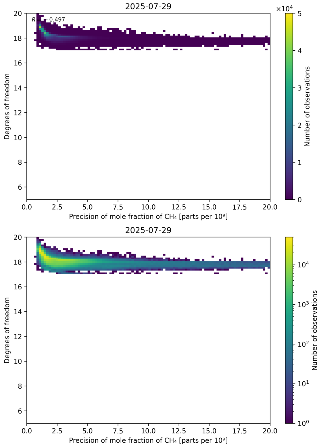
Figure 80: Scatter density plot of “Precision of mole fraction of CH 4 ” against “Degrees of freedom” for 2025-07-29 to 2025-07-30.
