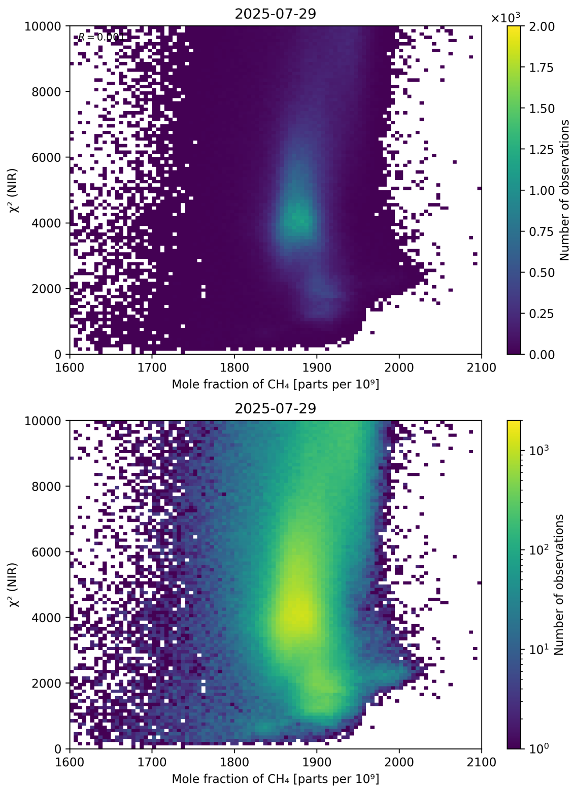
Figure 70: Scatter density plot of “Mole fraction of \text{CH}_4 ” against “ \chi^2 (NIR)” for 2025-07-29 to 2025-07-30.
