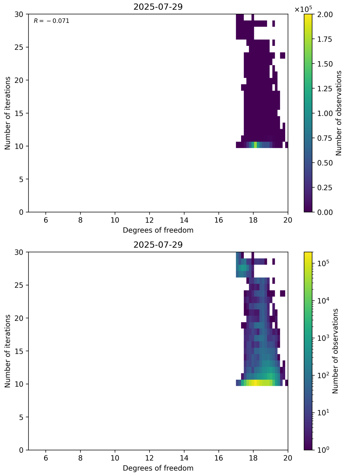
Figure 52: Scatter density plot of “Degrees of freedom” against “Number of iterations” for 2025-07-29 to 2025-07-30.
