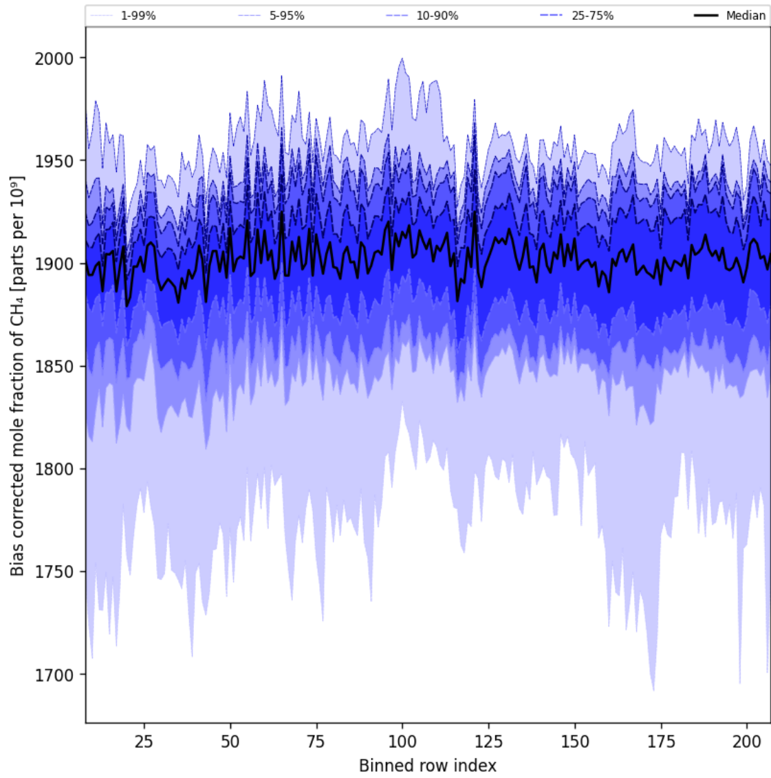
Figure 36: Along track statistics of “Bias corrected mole fraction of CH 4 ” for 2025-07-29 to 2025-07-30
