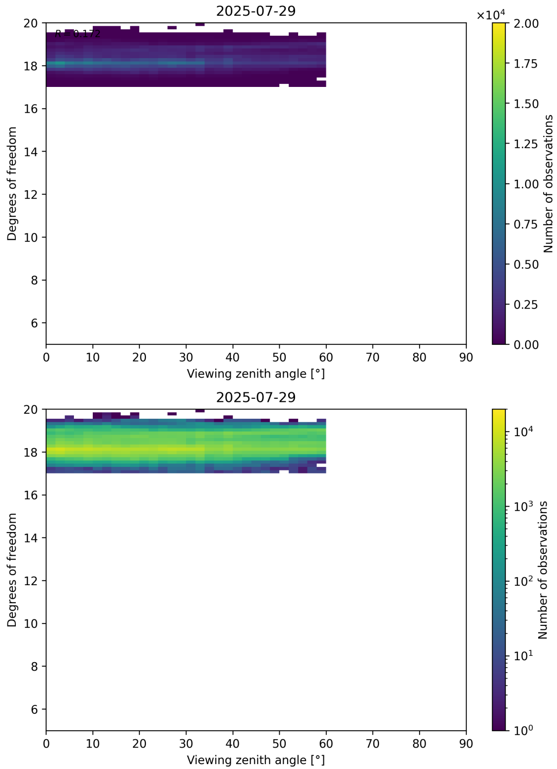
Figure 107: Scatter density plot of “Viewing zenith angle” against “Degrees of freedom” for 2025-07-29 to 2025-07-30.
