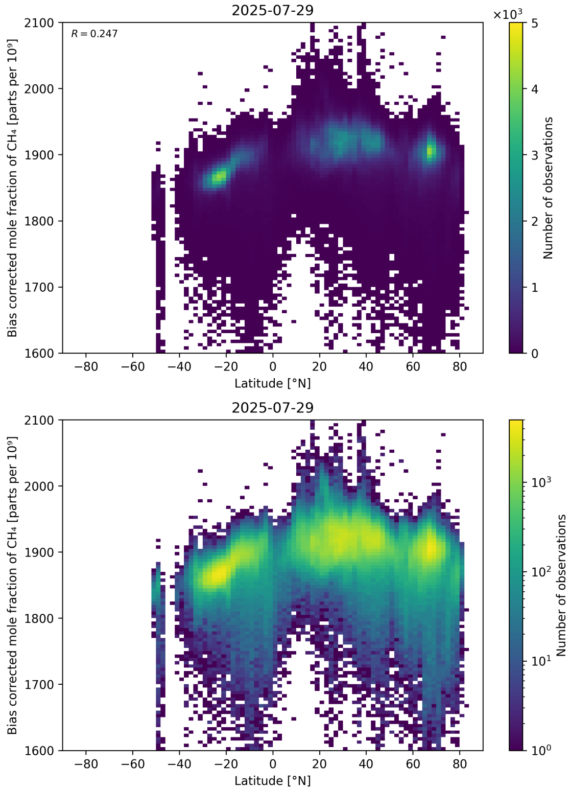
Figure 58: Scatter density plot of “Latitude” against “Bias corrected mole fraction of CH 4 ” for 2025-07-29 to 2025-07-30.
