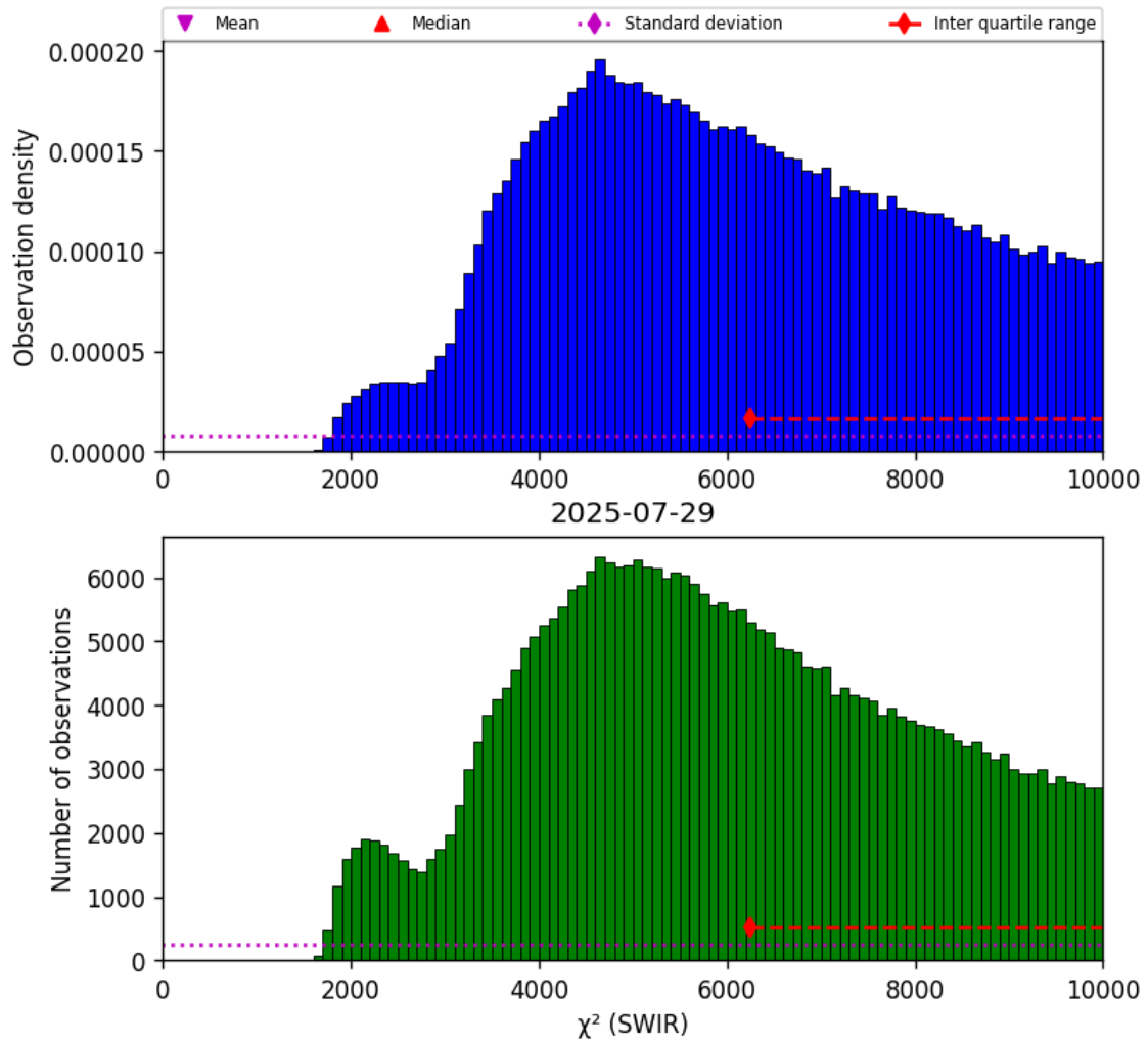
Figure 28: Histogram of “ \chi^2 (SWIR)” for 2025-07-29 to 2025-07-30
