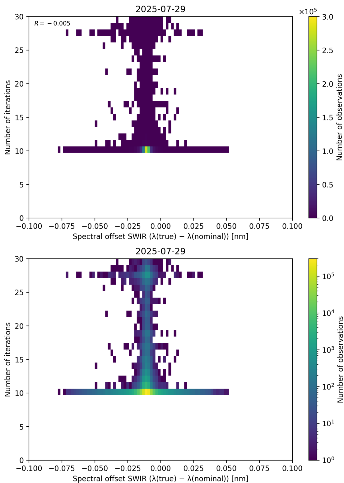
Figure 121: Scatter density plot of “Spectral offset SWIR ( \lambda_{\text{true}} - \lambda_{\text{nominal}} )” against “Number of iterations” for 2025-07-29 to 2025-07-30.
