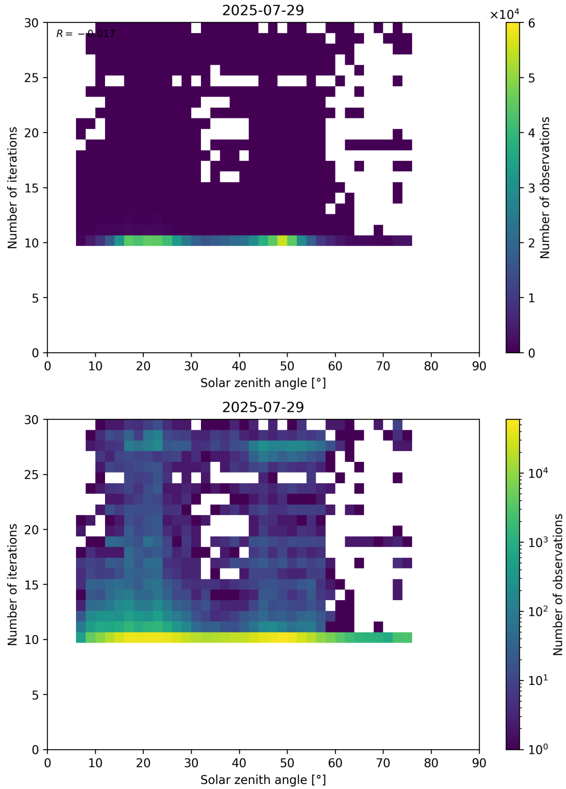
Figure 102: Scatter density plot of “Solar zenith angle” against “Number of iterations” for 2025-07-29 to 2025-07-30.
