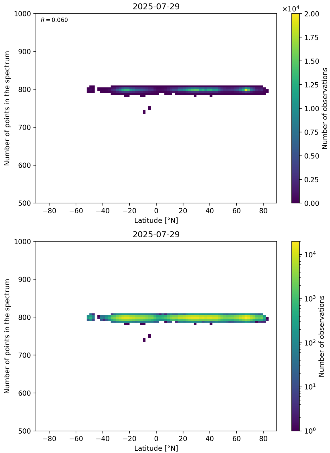
Figure 61: Scatter density plot of “Latitude” against “Number of points in the spectrum” for 2025-07-29 to 2025-07-30.
