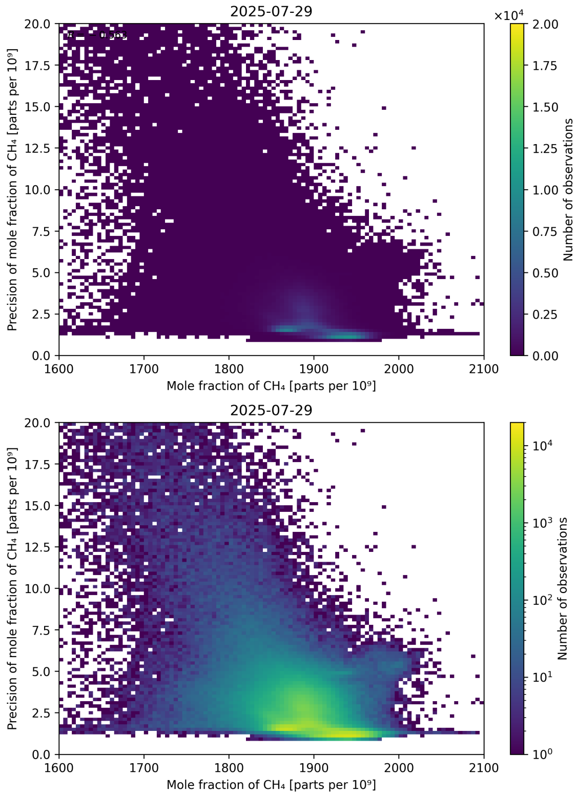
Figure 75: Scatter density plot of “Mole fraction of CH 4 ” against “Precision of mole fraction of CH 4 ” for 2025-07-29 to 2025-07-30.
