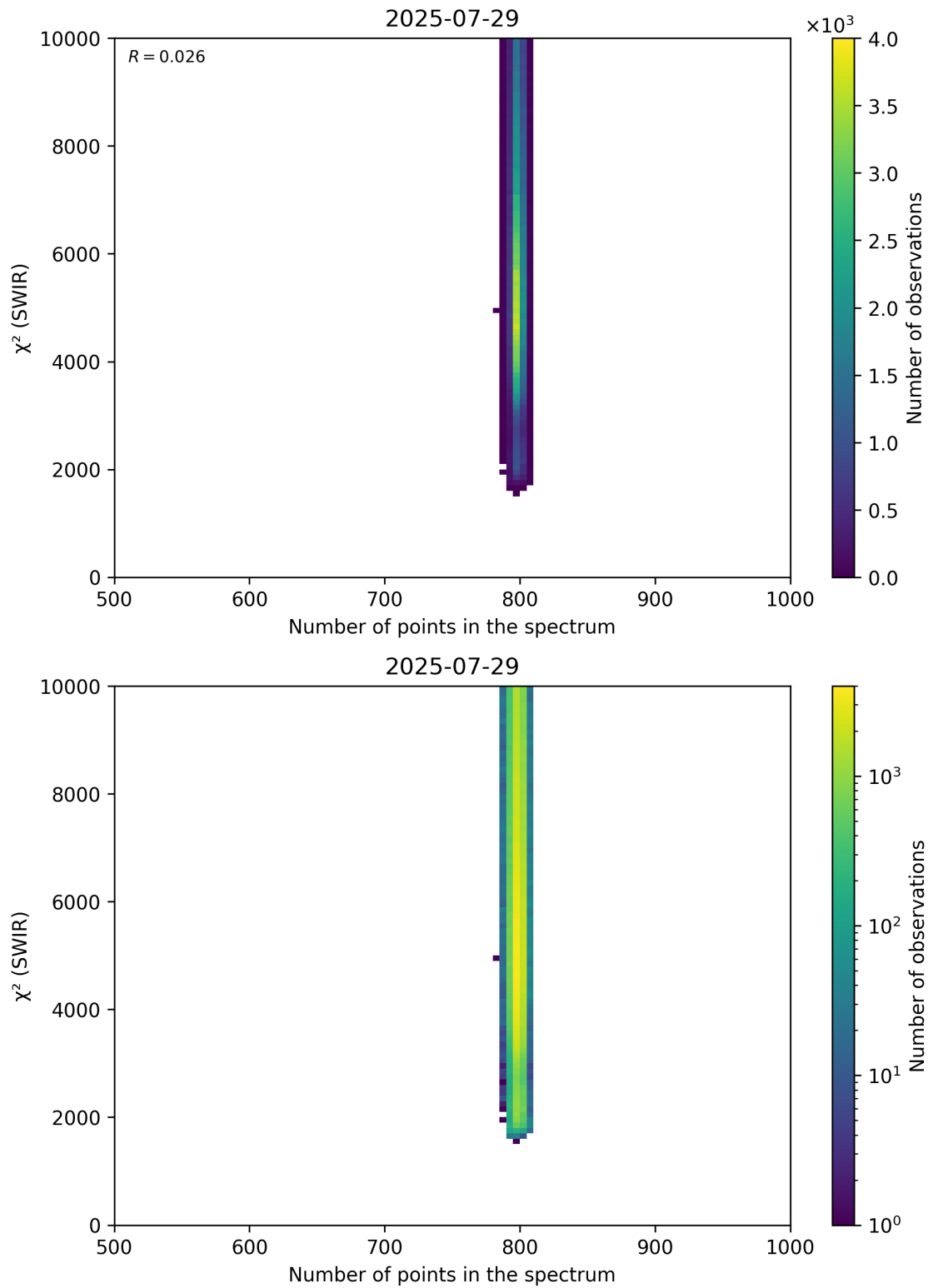
Figure 89: Scatter density plot of “Number of points in the spectrum” against “ \chi^2 (SWIR)” for 2025-07-29 to 2025-07-30.
