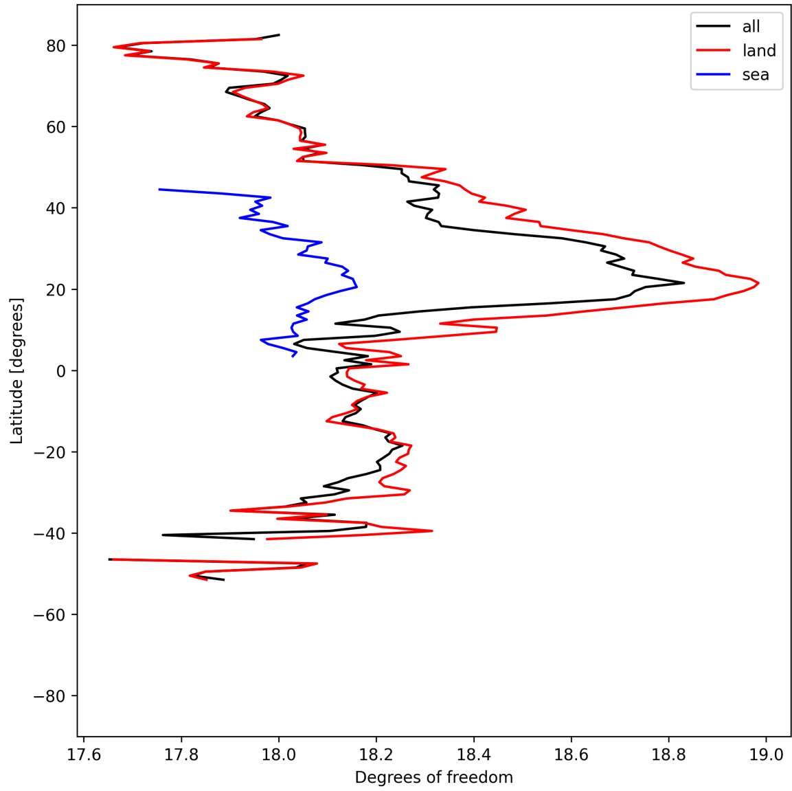
Figure 19: Zonal average of “Degrees of freedom” for 2025-07-29 to 2025-07-30.
