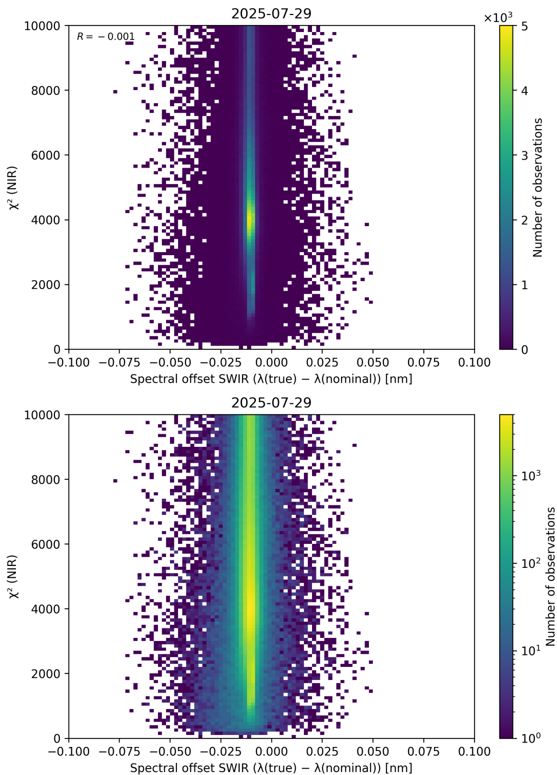
Figure 117: Scatter density plot of “Spectral offset SWIR ( \lambda_{\text{true}} - \lambda_{\text{nominal}} )” against “ \chi^2 (NIR)” for 2025-07-29 to 2025-07-30.
