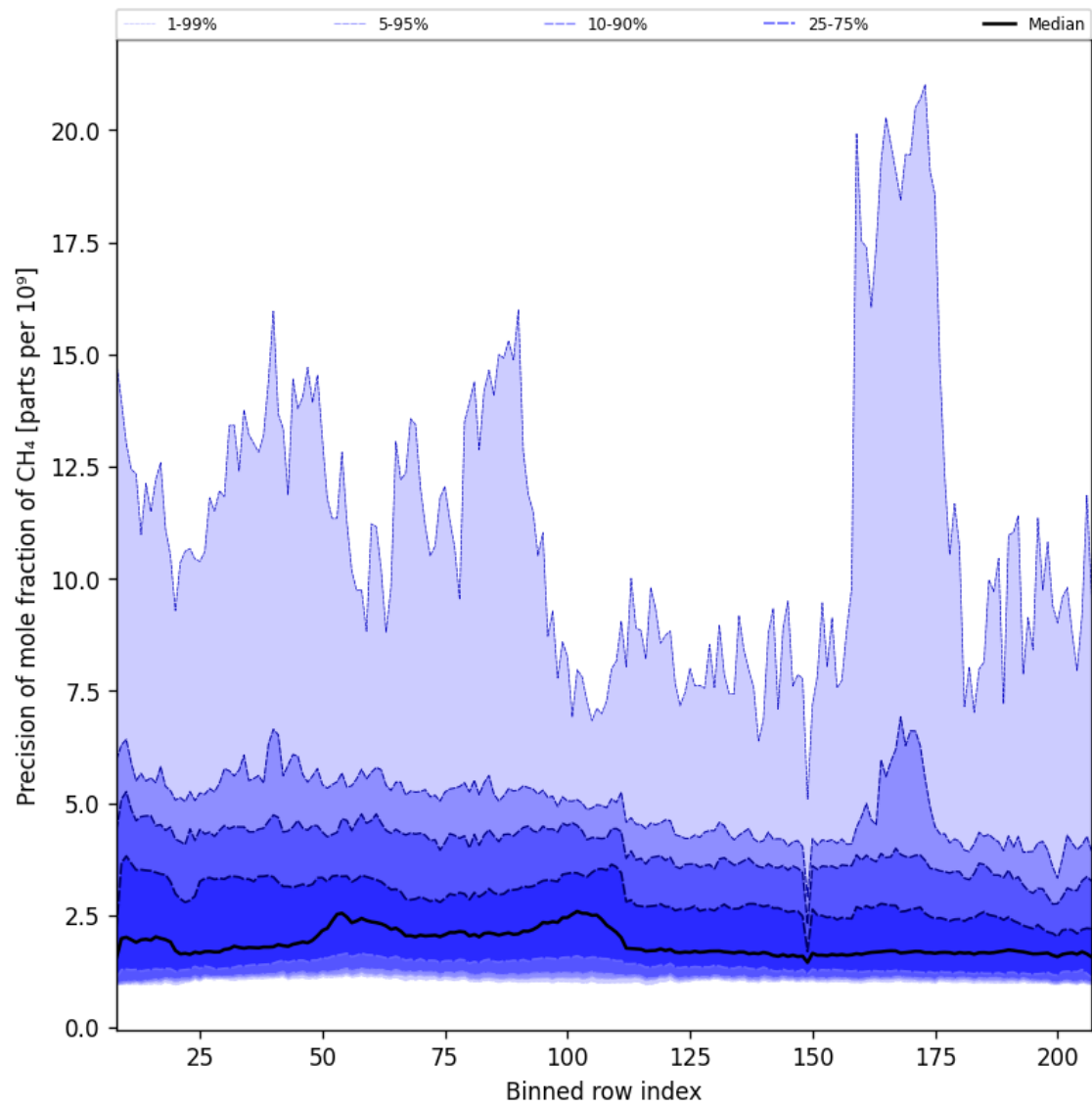
Figure 35: Along track statistics of “Precision of mole fraction of CH 4 ” for 2025-07-29 to 2025-07-30
