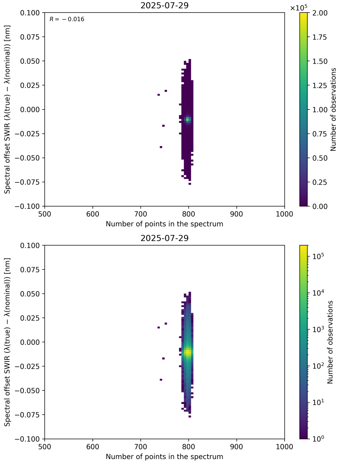
Figure 93: Scatter density plot of “Number of points in the spectrum” against “Spectral offset SWIR ( \lambda_{\text{true}} - \lambda_{\text{nominal}} )” for 2025-07-29 to 2025-07-30.
