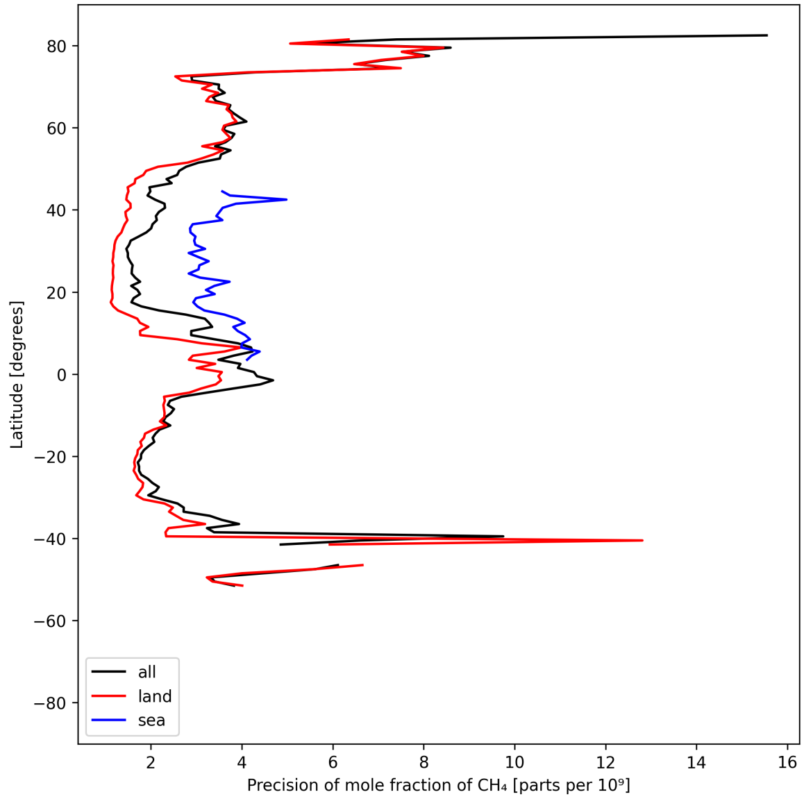
Figure 13: Zonal average of “Precision of mole fraction of \text{CH}_4 ” for 2025-07-29 to 2025-07-30.
