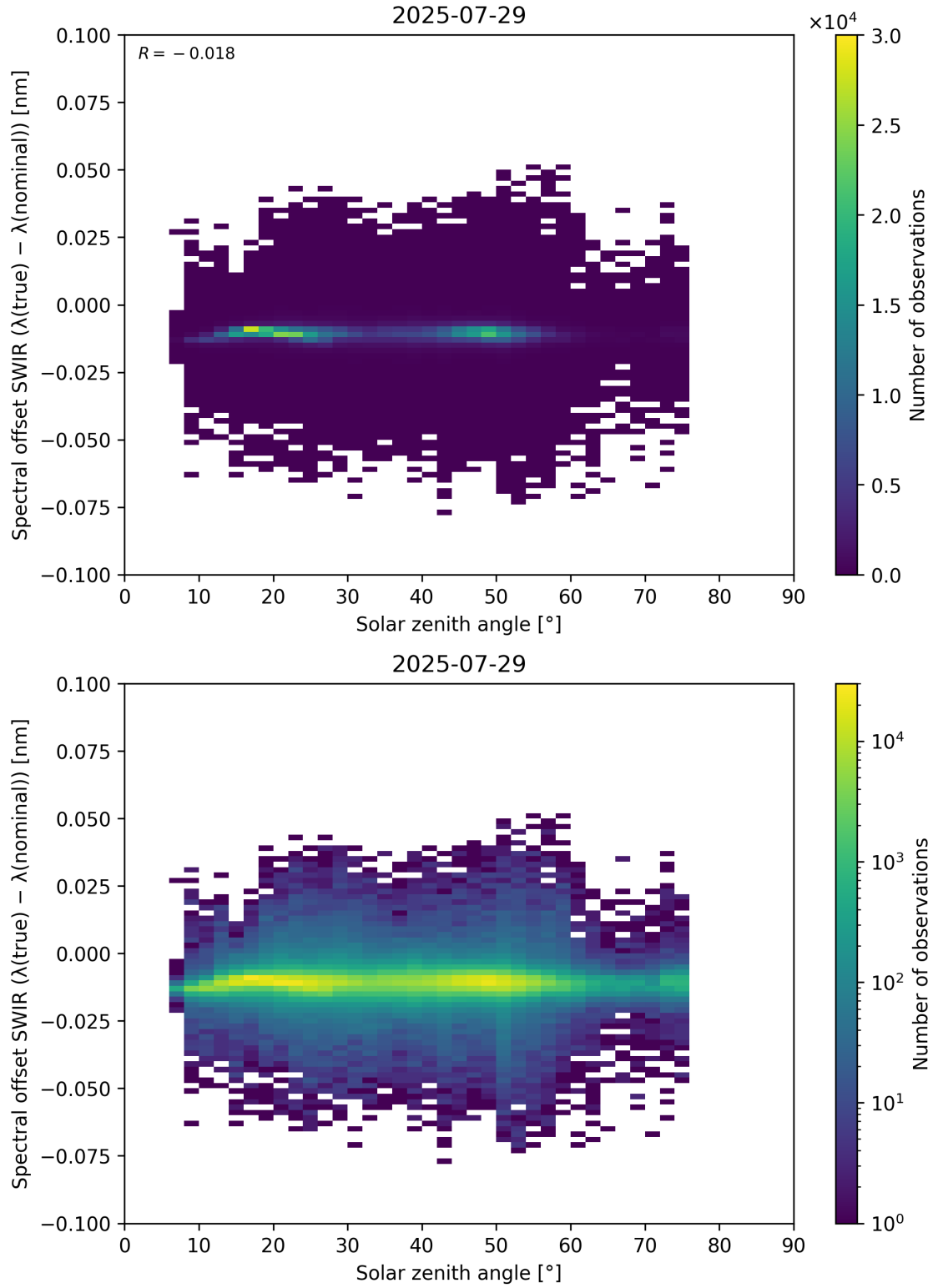
Figure 104: Scatter density plot of “Solar zenith angle” against “Spectral offset SWIR ( \lambda_{\text{true}} - \lambda_{\text{nominal}} )” for 2025-07-29 to 2025-07-30.
