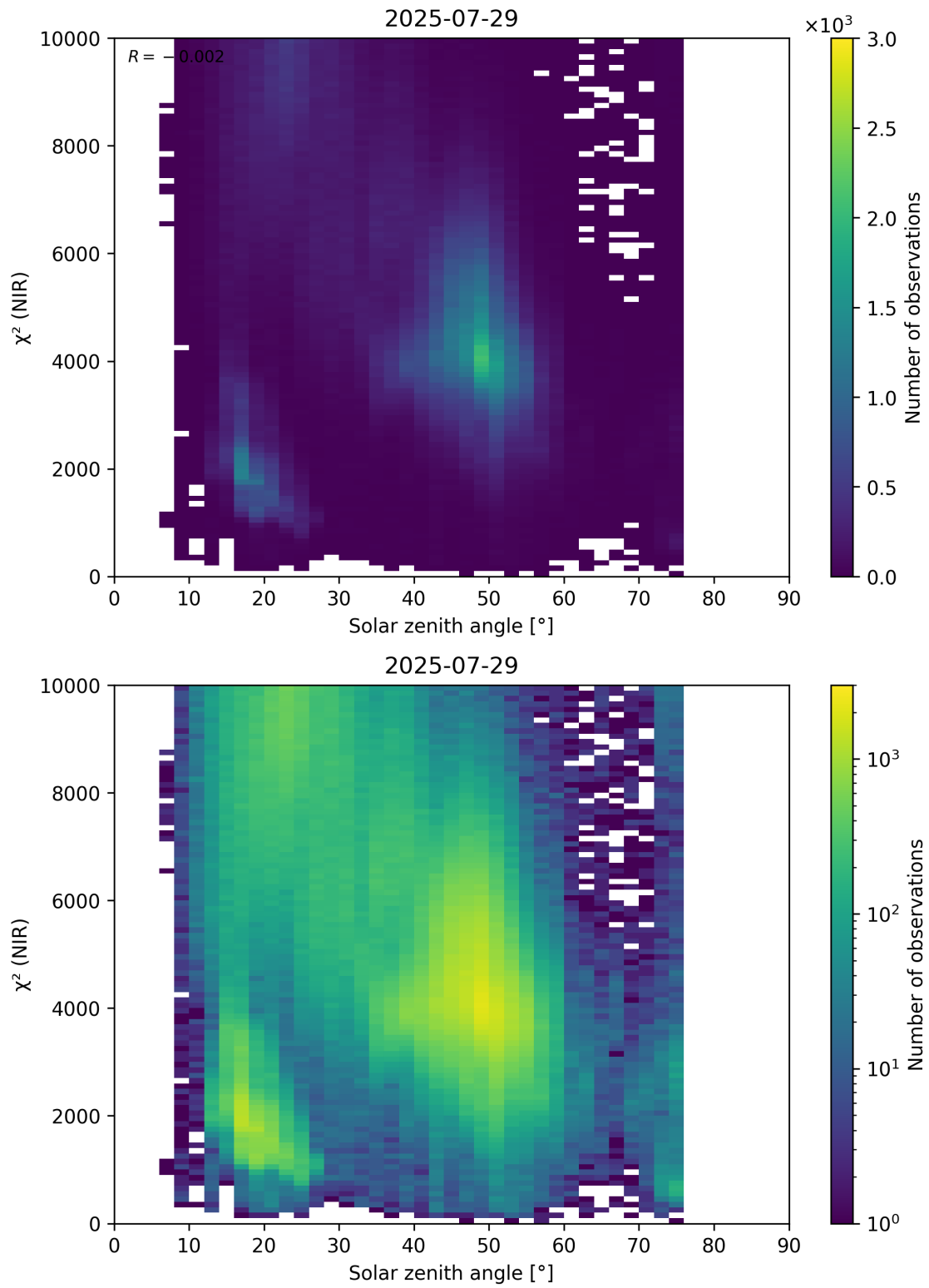
Figure 94: Scatter density plot of “Solar zenith angle” against “ \chi^2 (NIR)” for 2025-07-29 to 2025-07-30.
