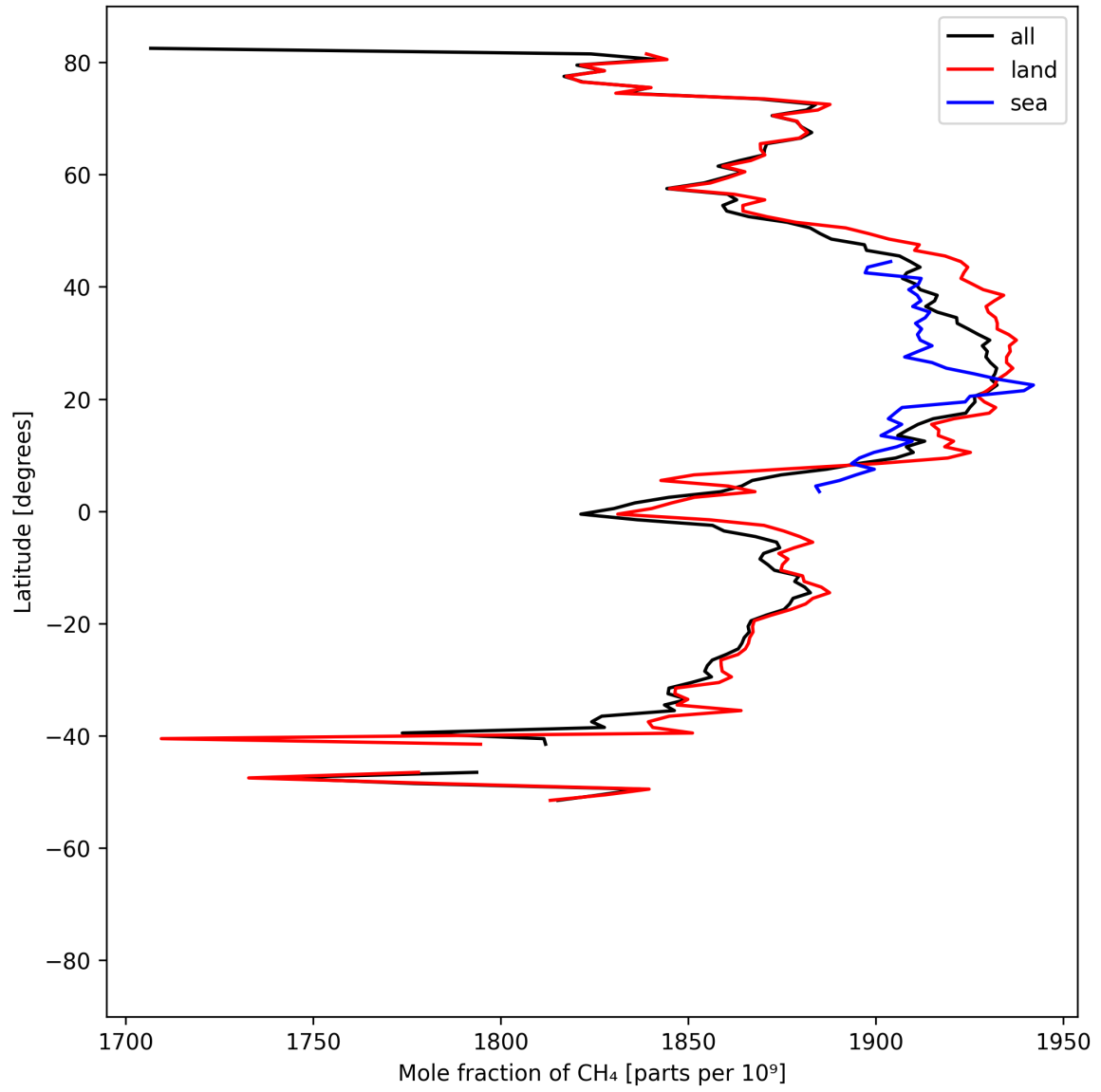
Figure 12: Zonal average of “Mole fraction of \text{CH}_4 ” for 2025-07-29 to 2025-07-30.
