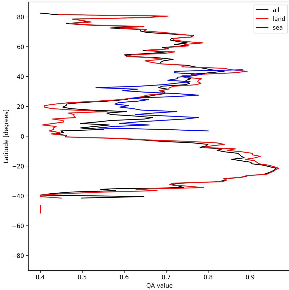
Figure 11: Zonal average of “QA value” for 2025-07-29 to 2025-07-30.
