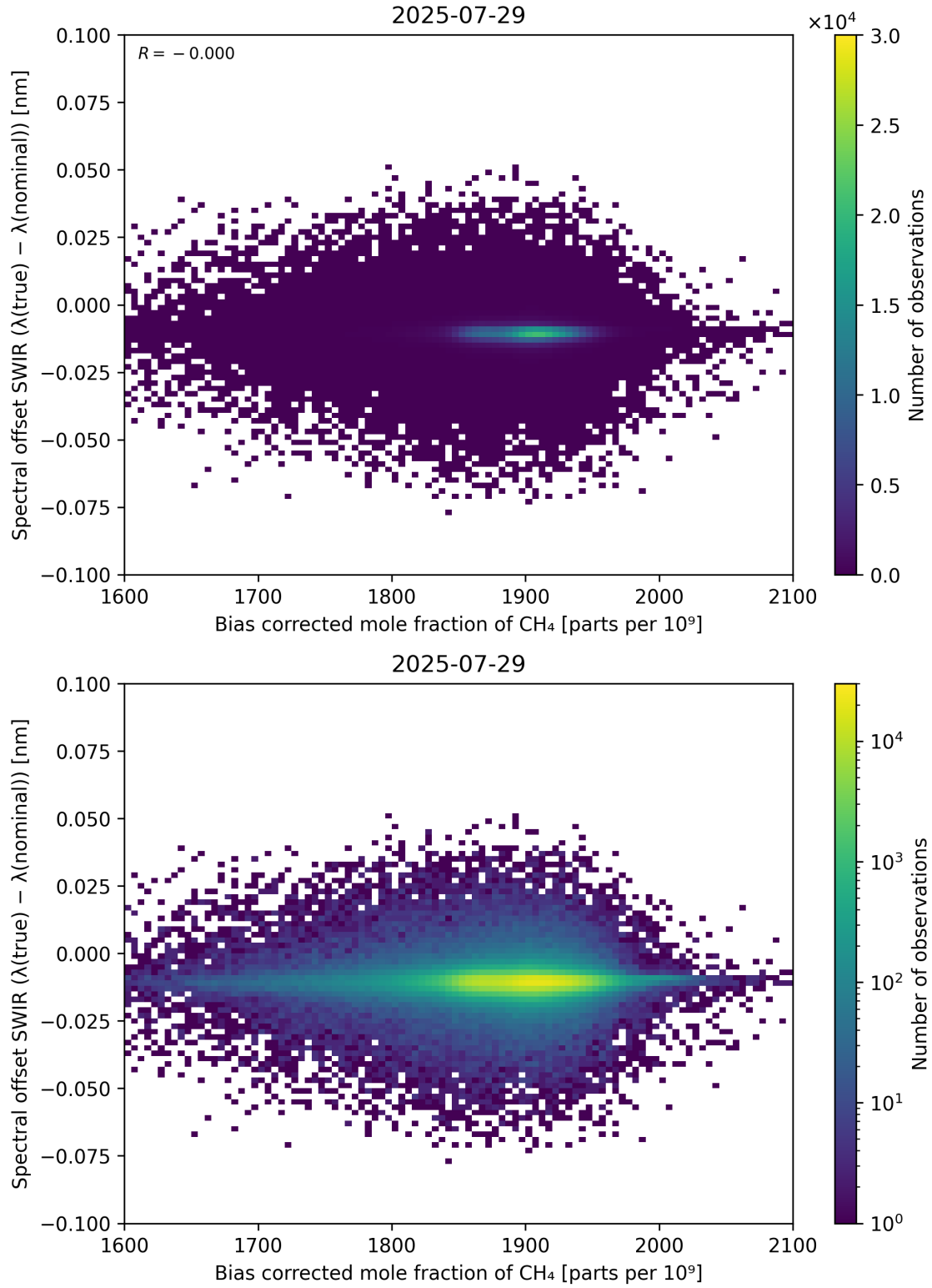
Figure 69: Scatter density plot of “Bias corrected mole fraction of \text{CH}_4 ” against “Spectral offset SWIR ( \lambda_{\text{true}} - \lambda_{\text{nominal}} )” for 2025-07-29 to 2025-07-30.
