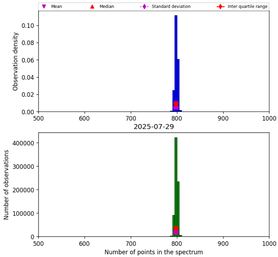
Figure 26: Histogram of “Number of points in the spectrum” for 2025-07-29 to 2025-07-30
