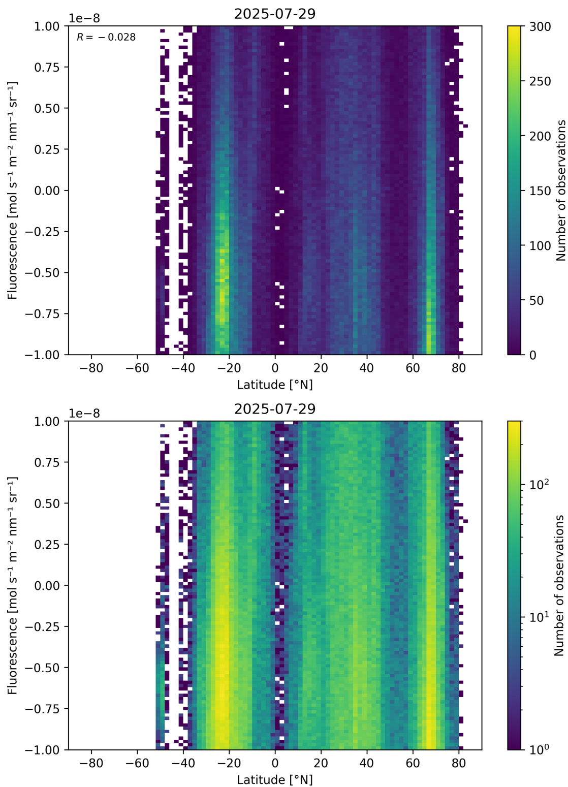
Figure 56: Scatter density plot of “Latitude” against “Fluorescence” for 2025-07-29 to 2025-07-30.
