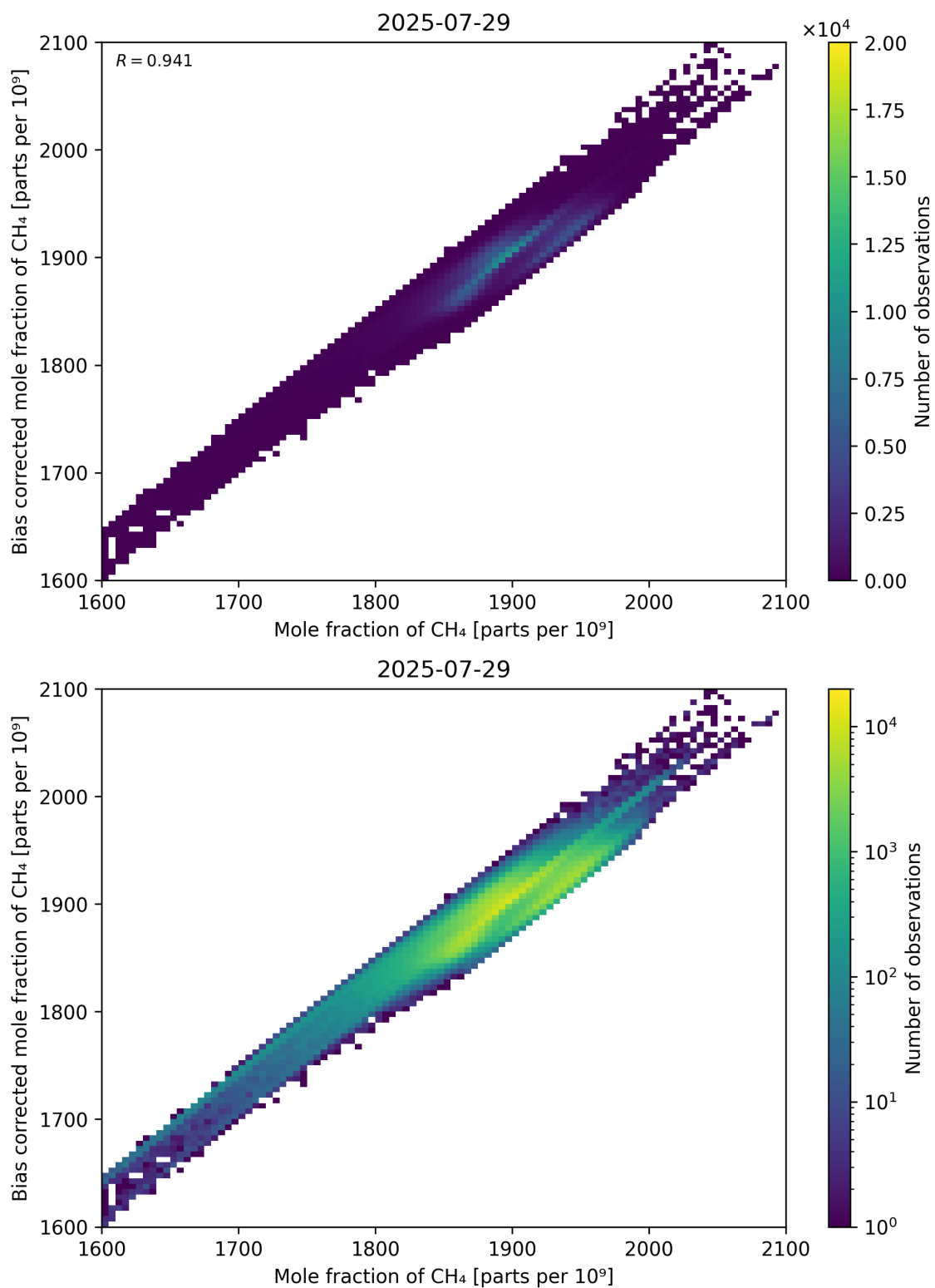
Figure 74: Scatter density plot of “Mole fraction of CH 4 ” against “Bias corrected mole fraction of CH 4 ” for 2025-07-29 to 2025-07-30.
