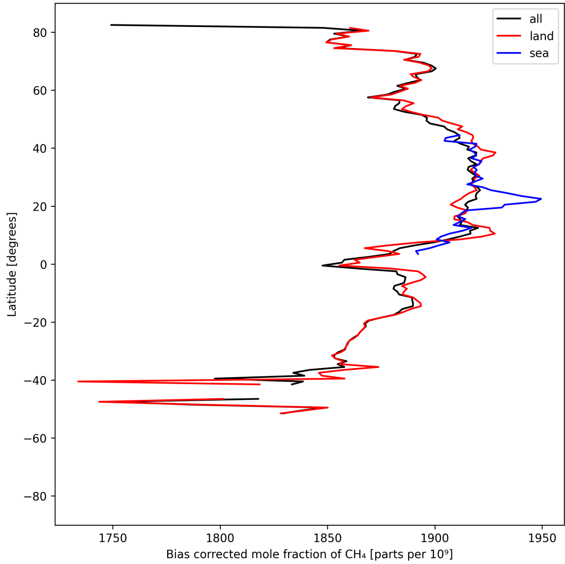
Figure 14: Zonal average of “Bias corrected mole fraction of CH 4 ” for 2025-07-29 to 2025-07-30.
