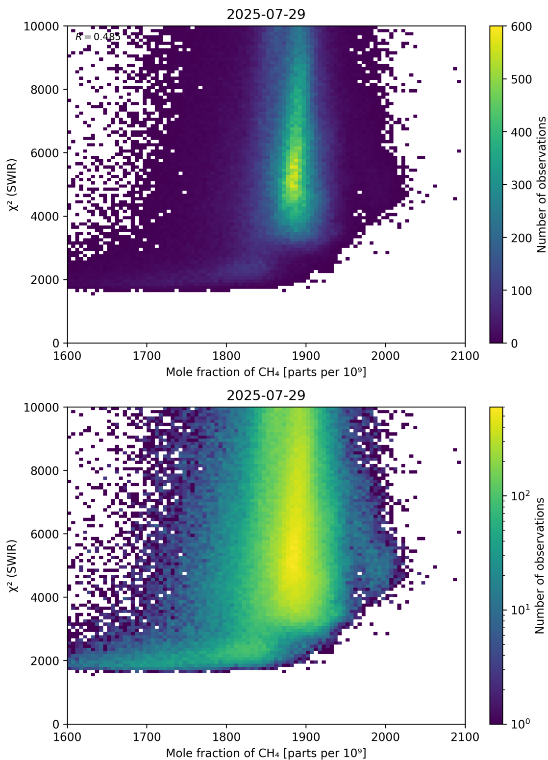
Figure 71: Scatter density plot of “Mole fraction of \text{CH}_4 ” against “ \chi^2 (SWIR)” for 2025-07-29 to 2025-07-30.
