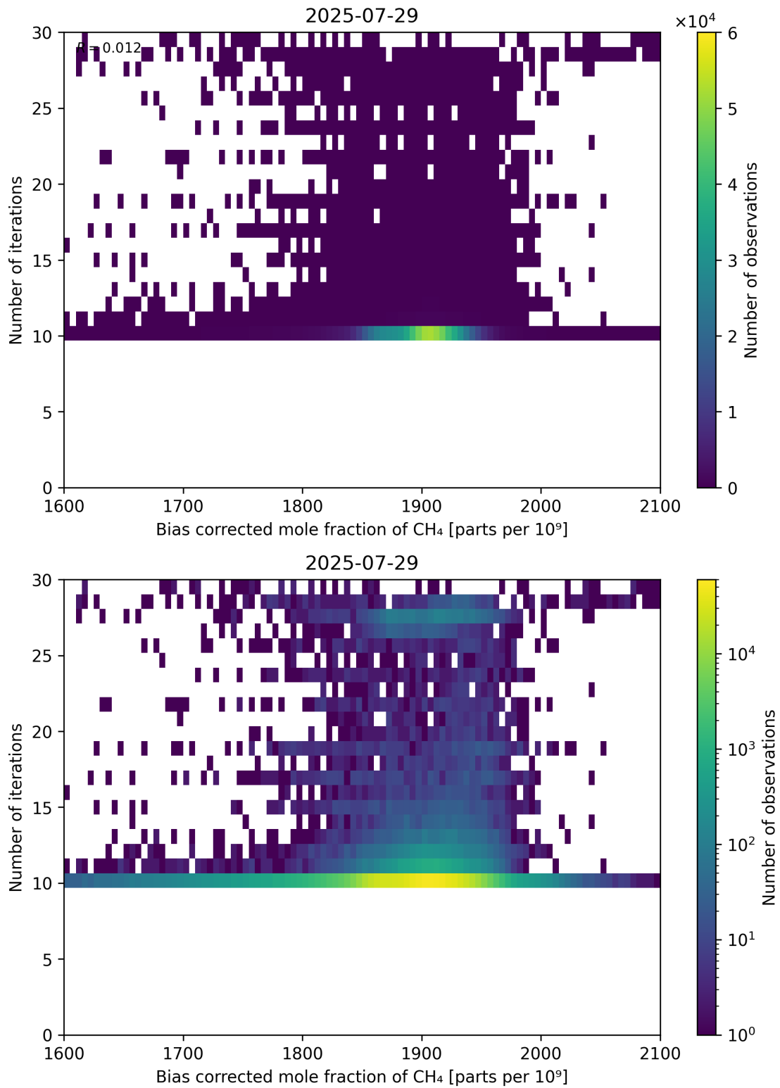
Figure 67: Scatter density plot of “Bias corrected mole fraction of CH 4 ” against “Number of iterations” for 2025-07-29 to 2025-07-30.
