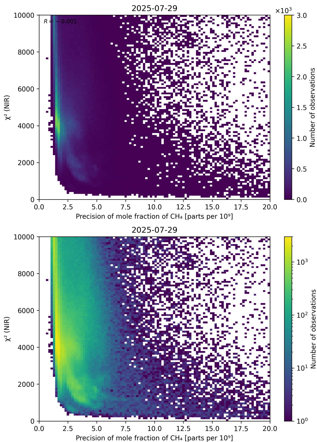
Figure 78: Scatter density plot of “Precision of mole fraction of CH 4 ” against “ \chi^2 (NIR)” for 2025-07-29 to 2025-07-30.
