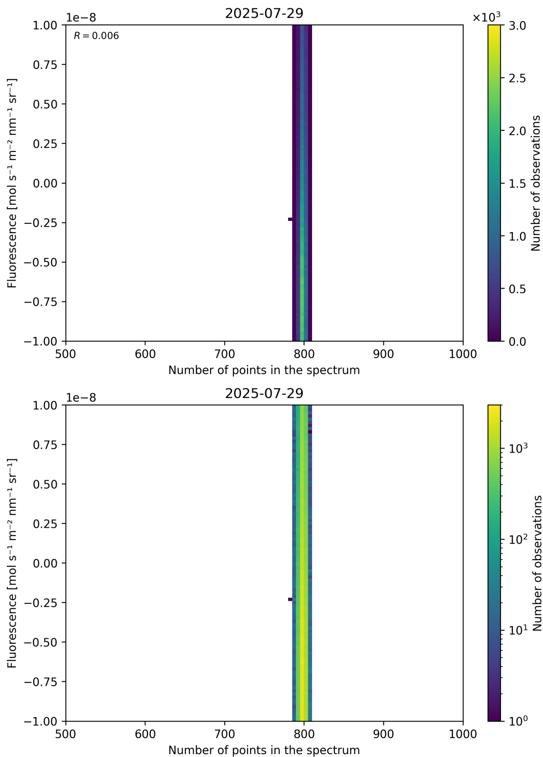
Figure 91: Scatter density plot of “Number of points in the spectrum” against “Fluorescence” for 2025-07-29 to 2025-07-30.
