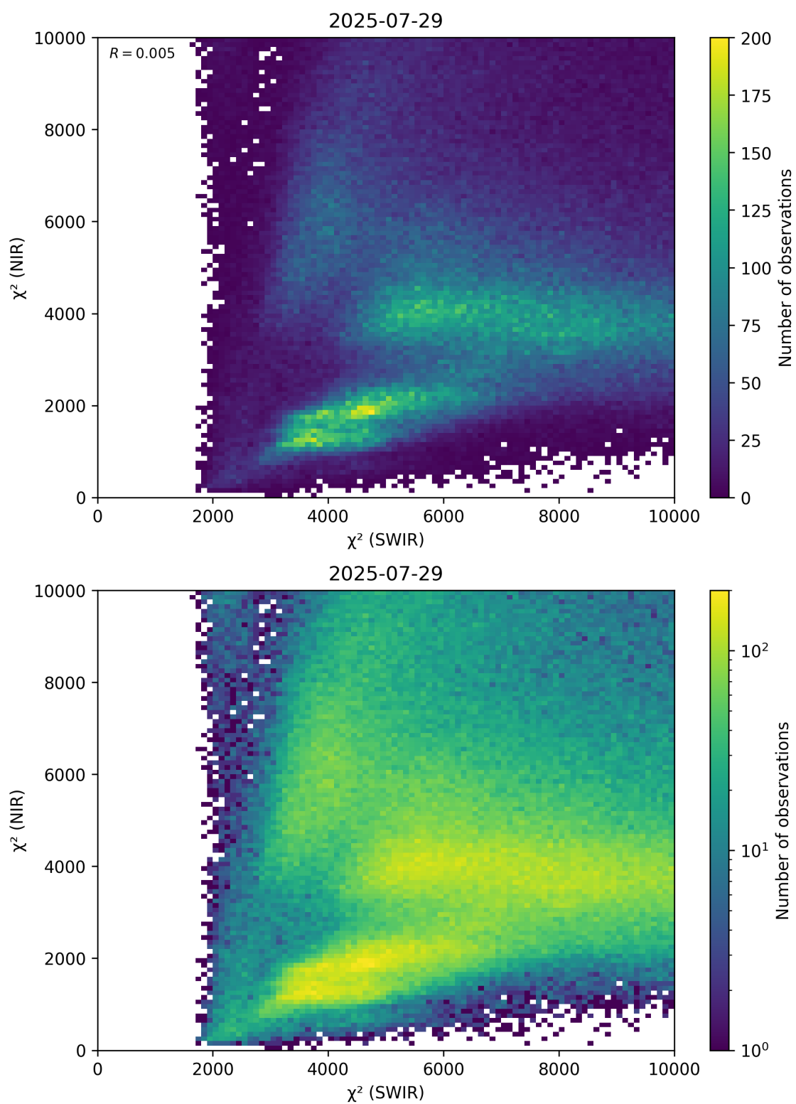
Figure 47: Scatter density plot of “ \chi^2 (SWIR)” against “ \chi^2 (NIR)” for 2025-07-29 to 2025-07-30.
