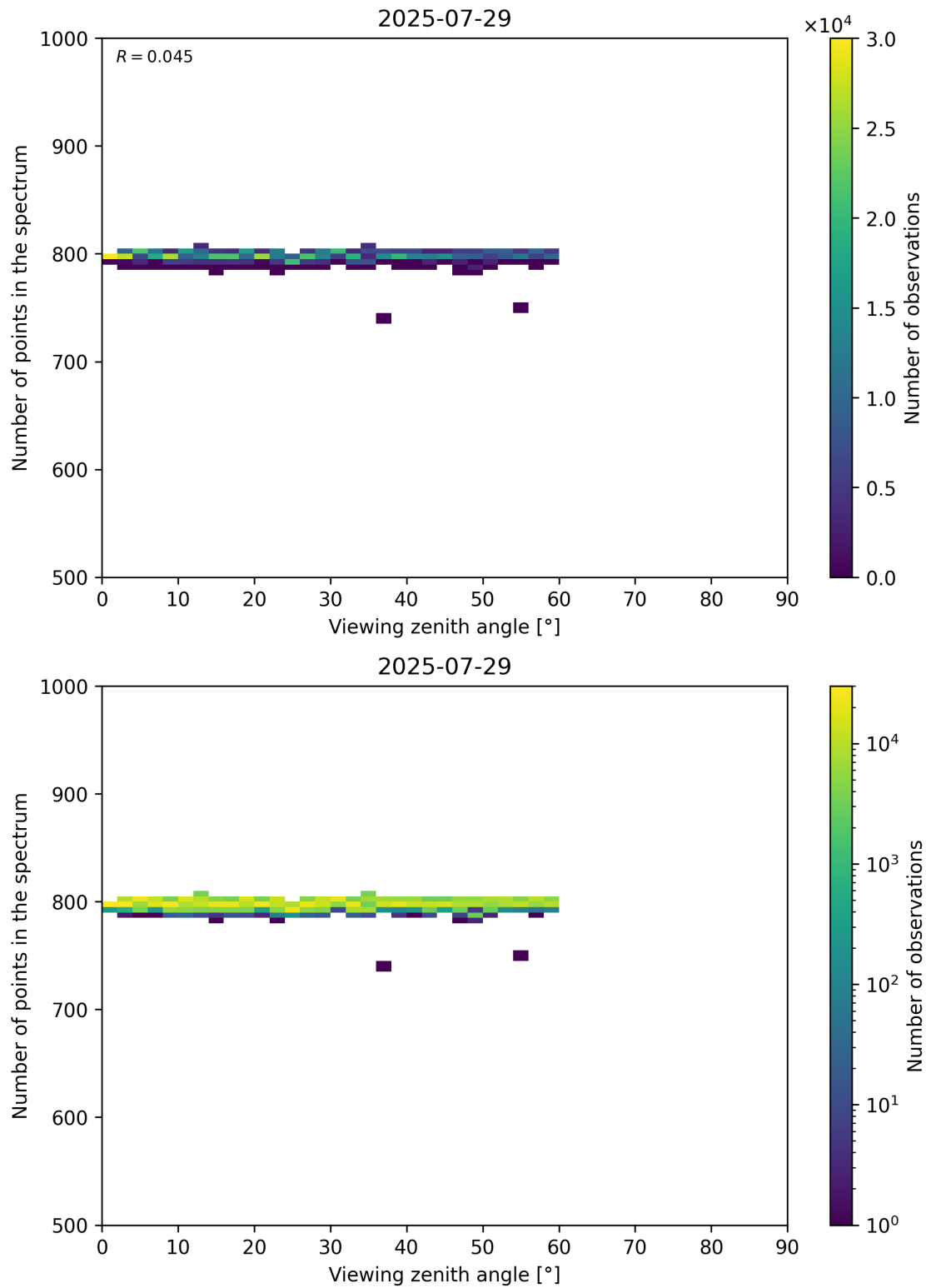
Figure 114: Scatter density plot of “Viewing zenith angle” against “Number of points in the spectrum” for 2025-07-29 to 2025-07-30.
