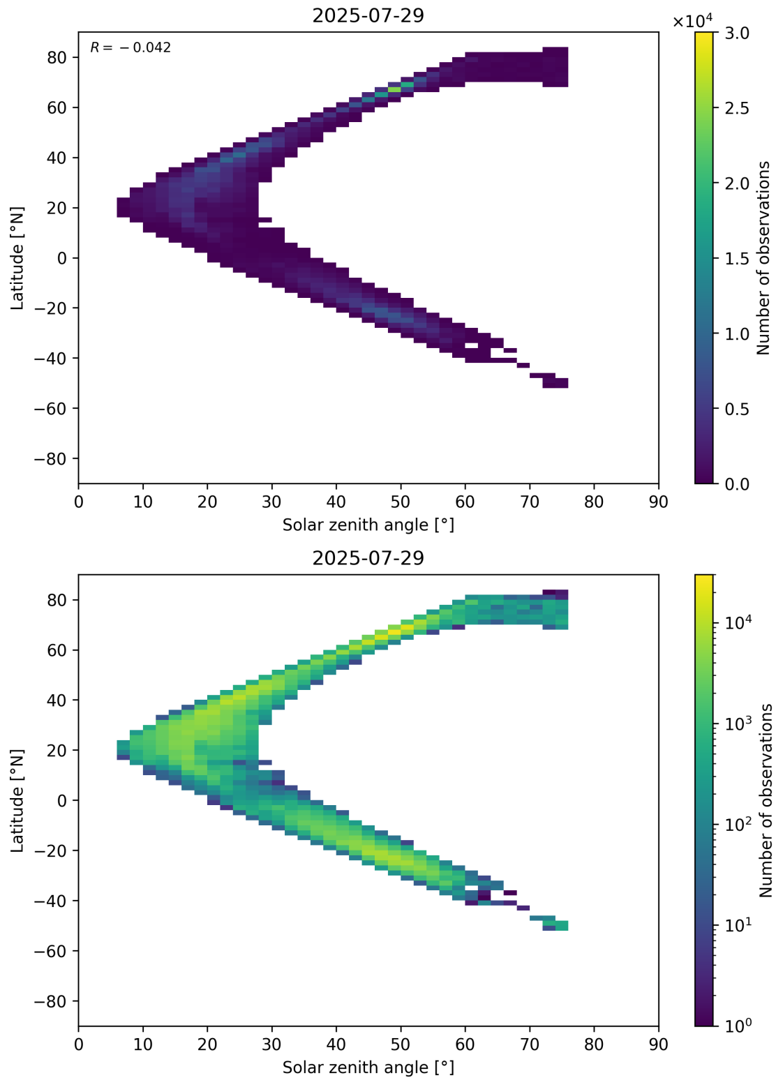
Figure 98: Scatter density plot of “Solar zenith angle” against “Latitude” for 2025-07-29 to 2025-07-30.
