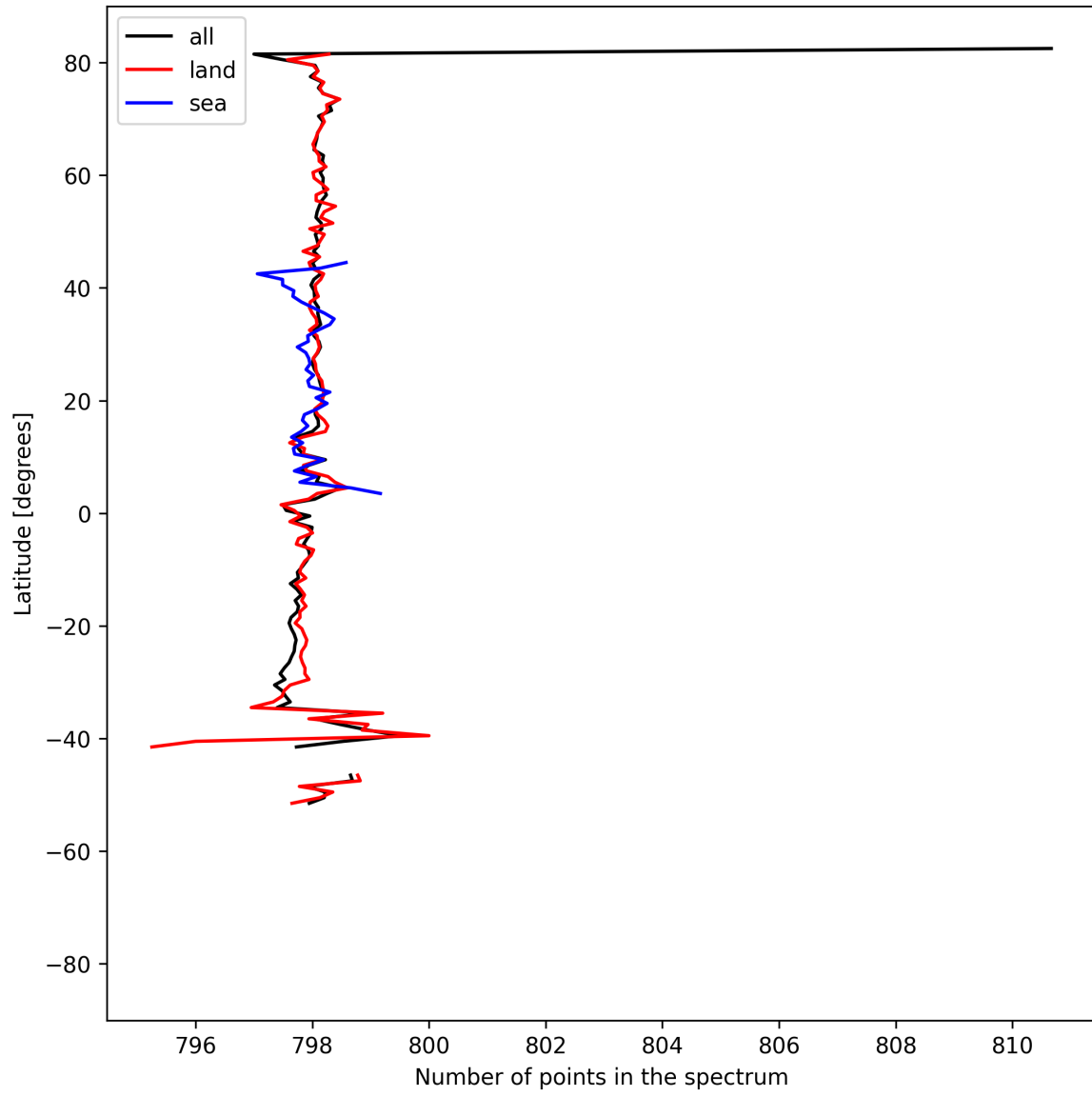
Figure 15: Zonal average of “Number of points in the spectrum” for 2025-07-29 to 2025-07-30.
