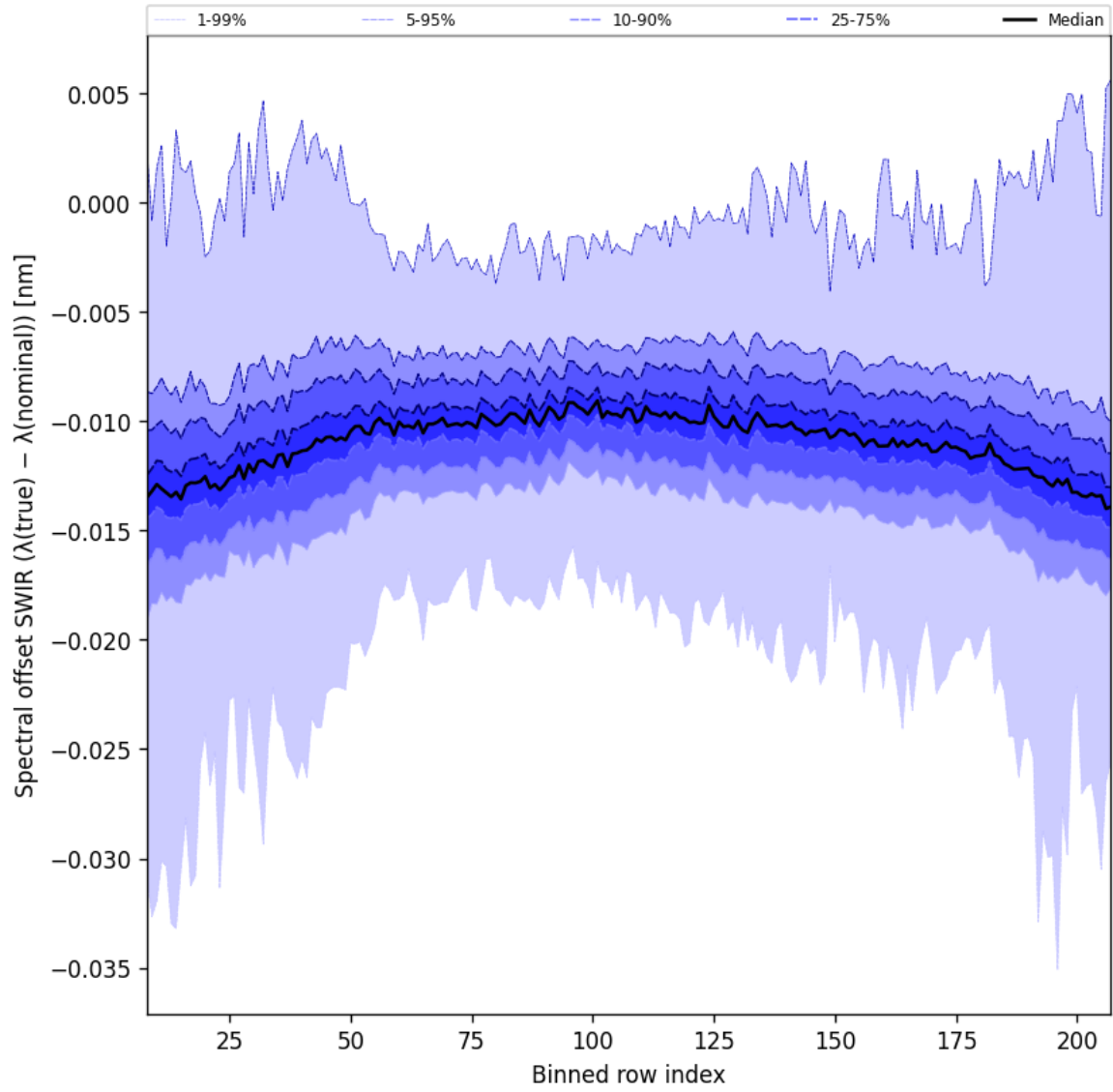
Figure 38: Along track statistics of “Spectral offset SWIR ( \lambda_{\text{true}} - \lambda_{\text{nominal}} )” for 2025-07-29 to 2025-07-30
