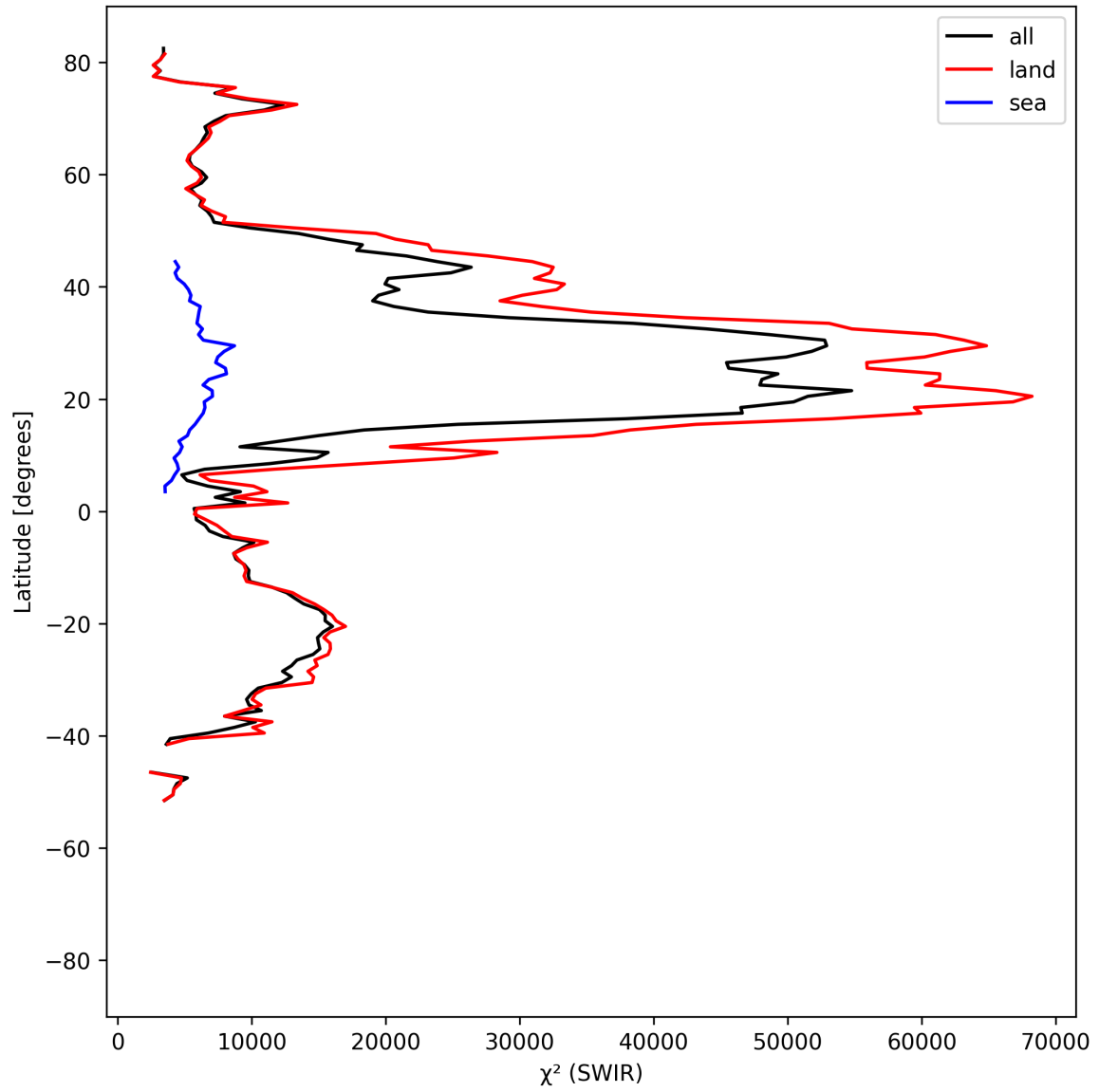
Figure 17: Zonal average of “ \chi^2 (SWIR)” for 2025-07-29 to 2025-07-30.
