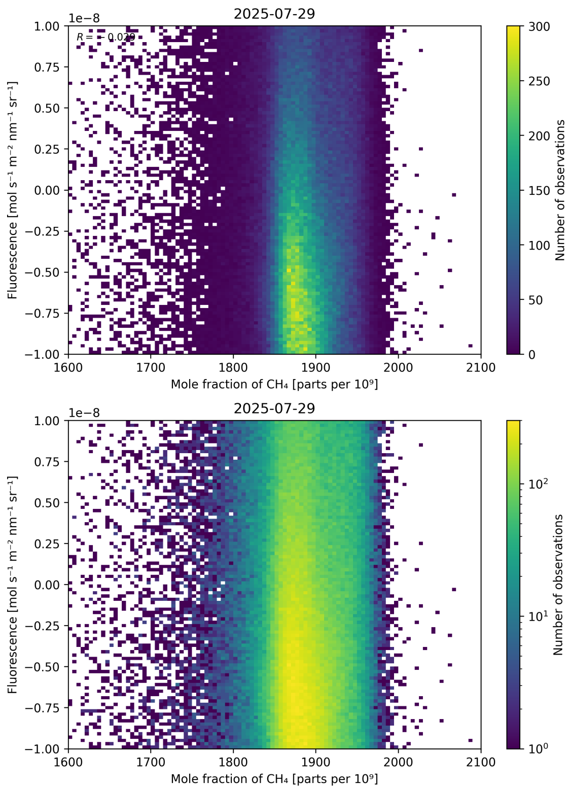
Figure 73: Scatter density plot of “Mole fraction of \text{CH}_4 ” against “Fluorescence” for 2025-07-29 to 2025-07-30.
