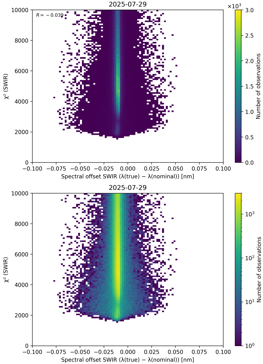
Figure 118: Scatter density plot of “Spectral offset SWIR ( \lambda_{\text{true}} - \lambda_{\text{nominal}} )” against “ \chi^2 (SWIR)” for 2025-07-29 to 2025-07-30.
