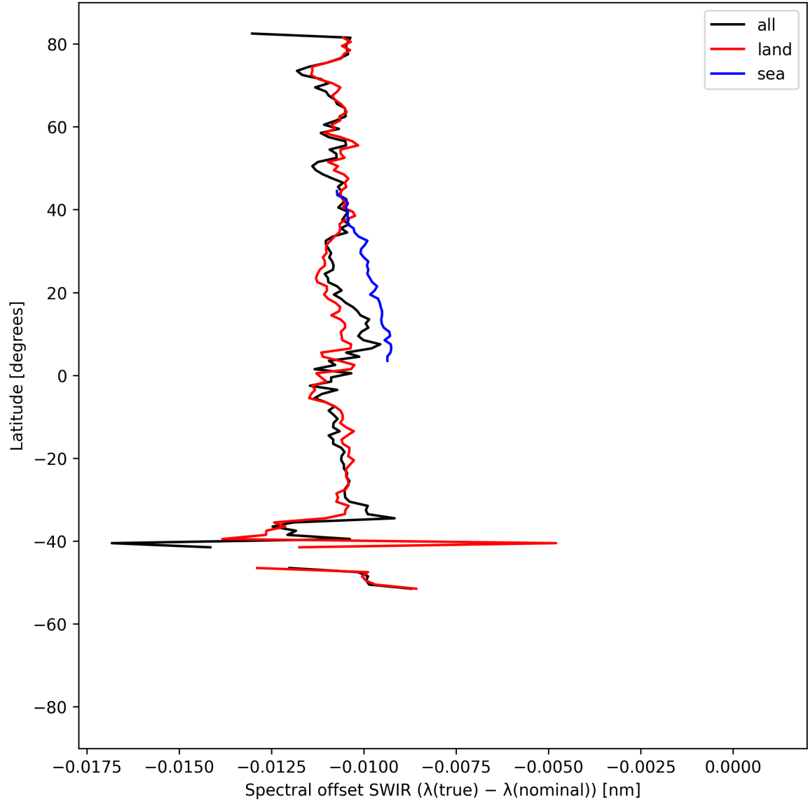
Figure 16: Zonal average of “Spectral offset SWIR ( \lambda_{\text{true}} - \lambda_{\text{nominal}} )” for 2025-07-29 to 2025-07-30.
