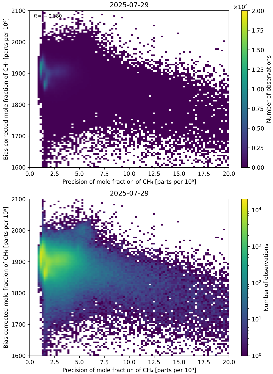
Figure 82: Scatter density plot of “Precision of mole fraction of CH 4 ” against “Bias corrected mole fraction of CH 4 ” for 2025-07-29 to 2025-07-30.
