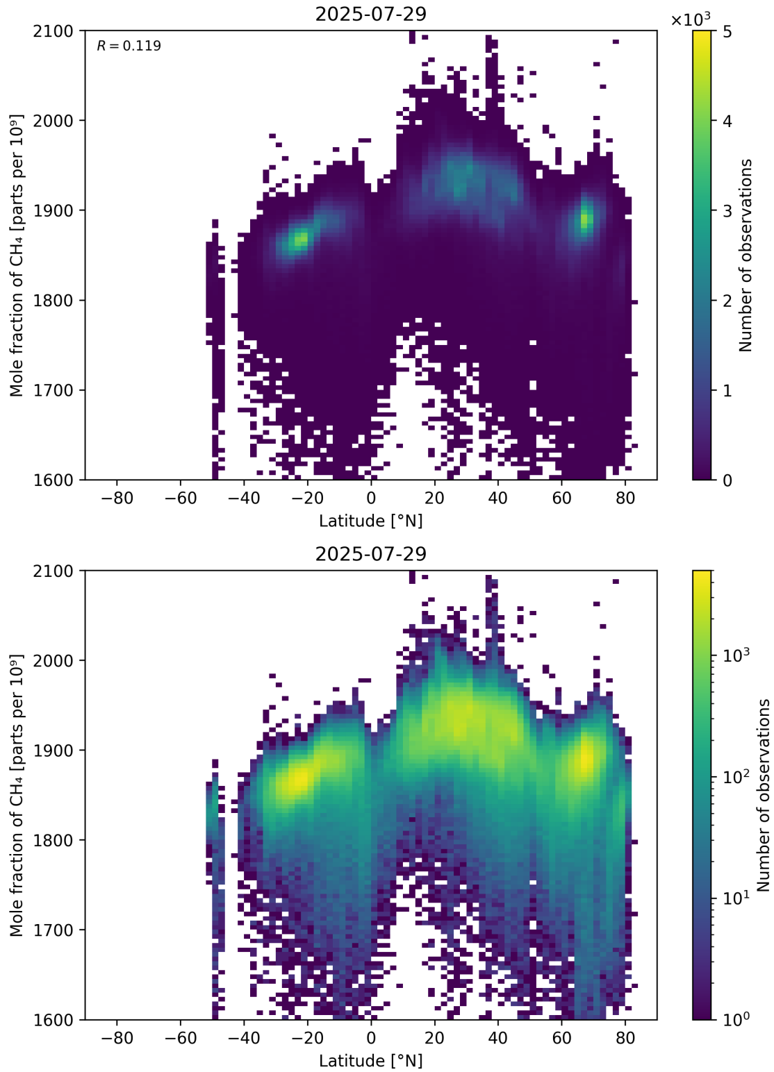
Figure 57: Scatter density plot of “Latitude” against “Mole fraction of CH 4 ” for 2025-07-29 to 2025-07-30.
