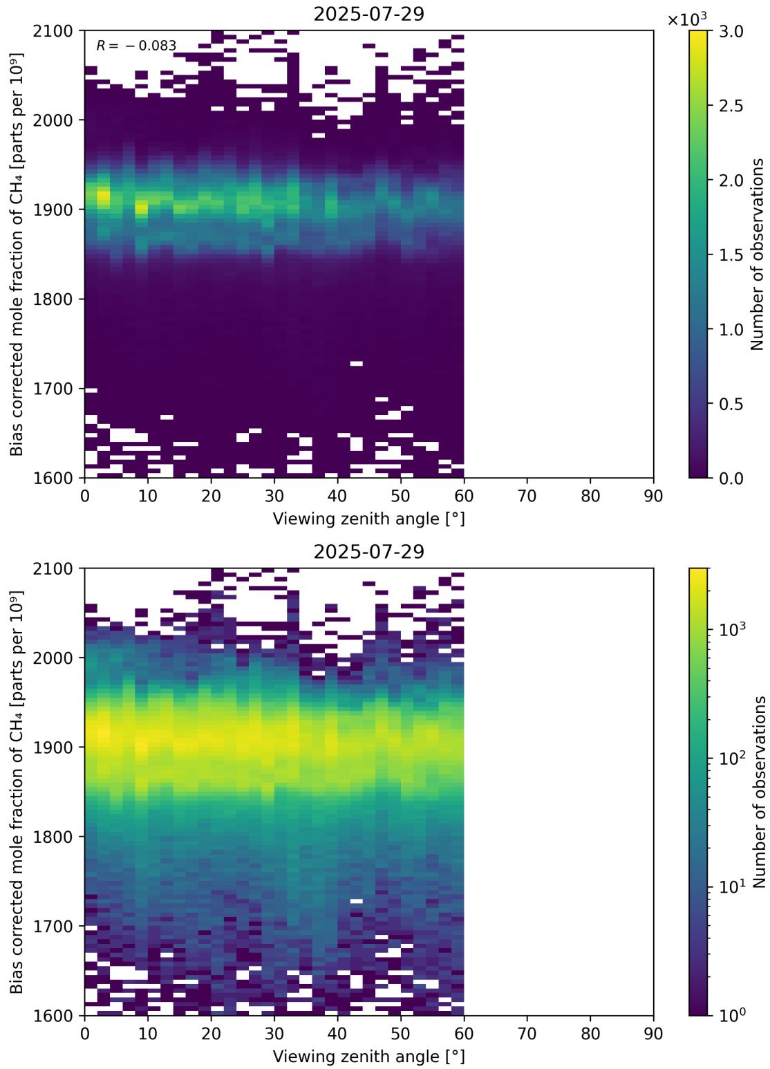
Figure 111: Scatter density plot of “Viewing zenith angle” against “Bias corrected mole fraction of CH 4 ” for 2025-07-29 to 2025-07-30.
