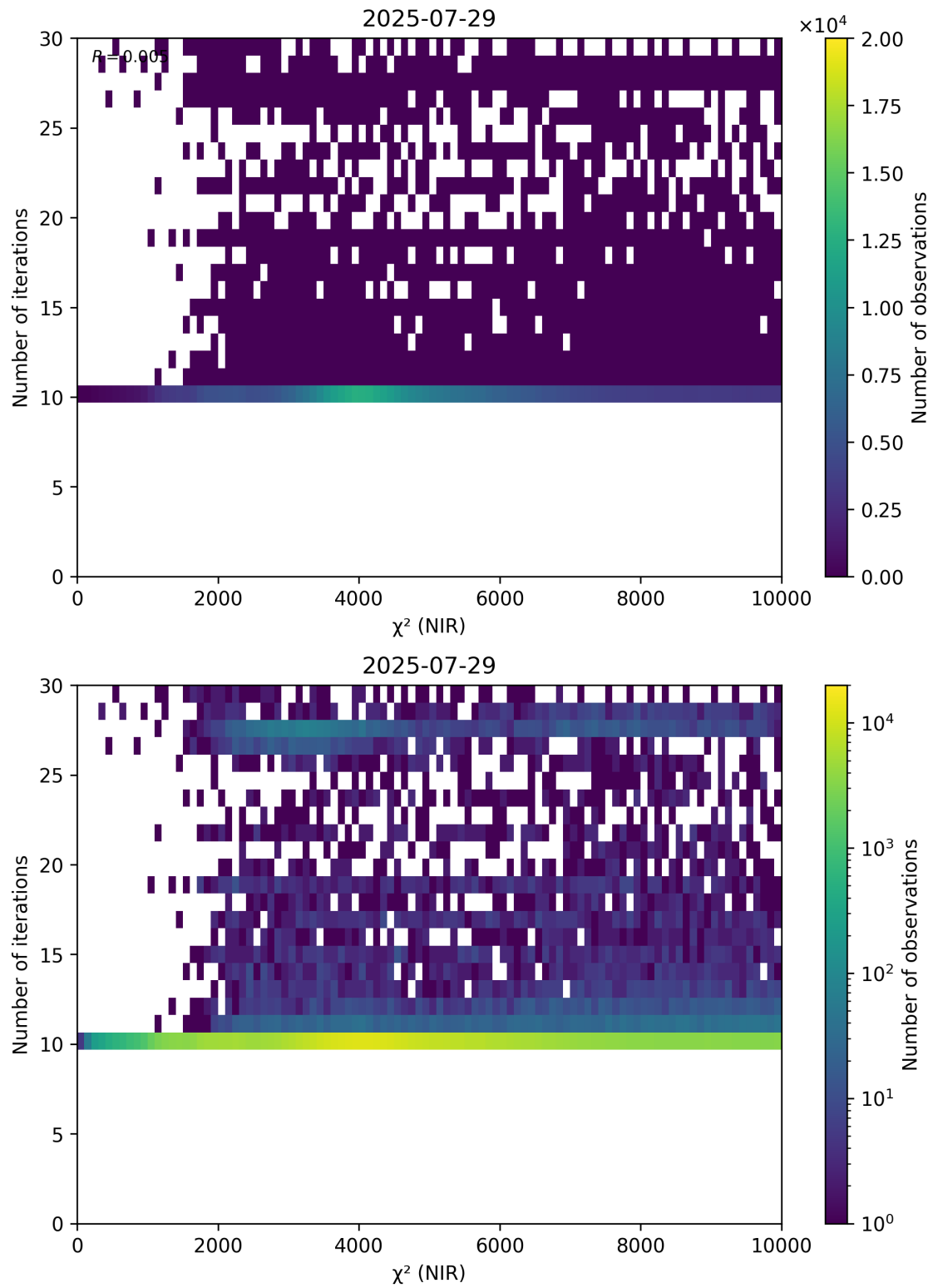
Figure 46: Scatter density plot of “ \chi^2 (NIR)” against “Number of iterations” for 2025-07-29 to 2025-07-30.
