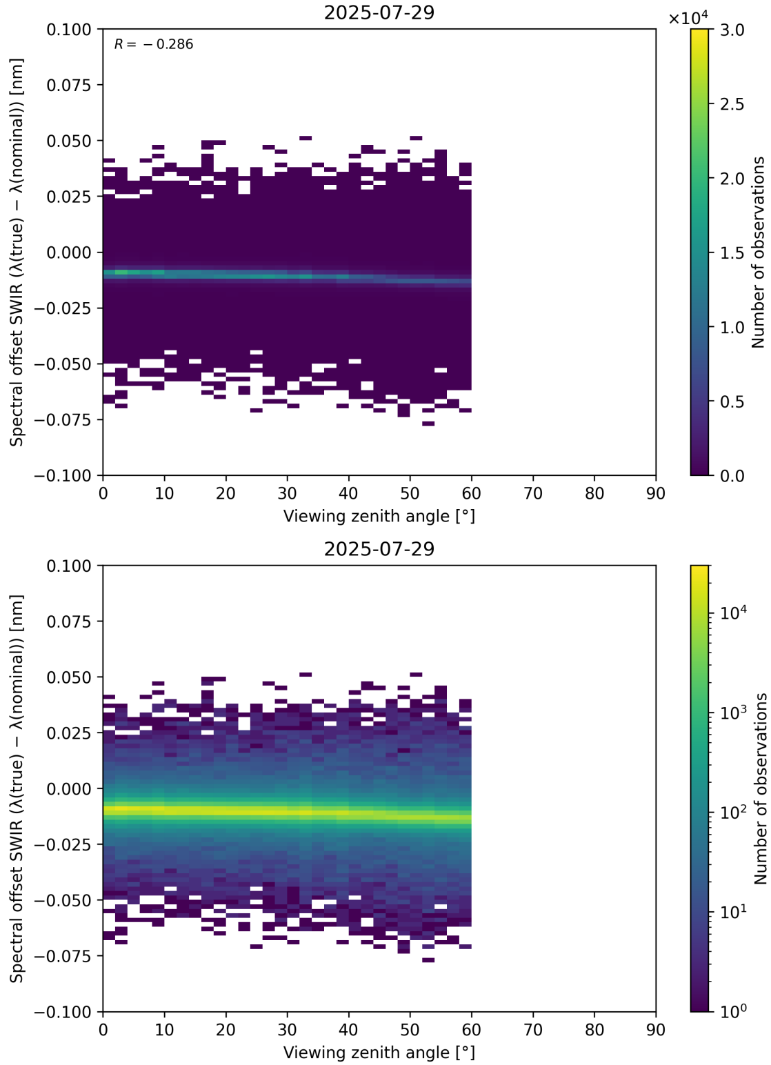
Figure 116: Scatter density plot of “Viewing zenith angle” against “Spectral offset SWIR ( \lambda_{\text{true}} - \lambda_{\text{nominal}} )” for 2025-07-29 to 2025-07-30.
