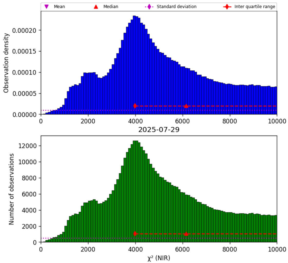
Figure 29: Histogram of “ \chi^2 (NIR)” for 2025-07-29 to 2025-07-30
