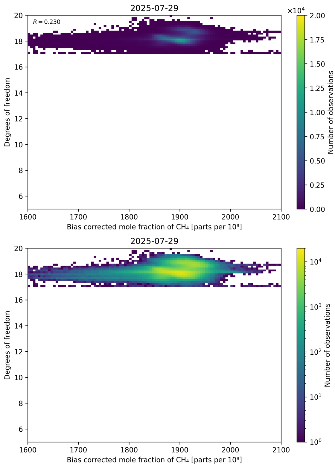
Figure 65: Scatter density plot of “Bias corrected mole fraction of CH 4 ” against “Degrees of freedom” for 2025-07-29 to 2025-07-30.
