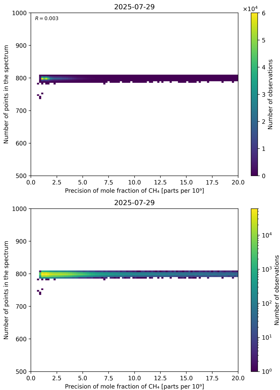
Figure 84: Scatter density plot of “Precision of mole fraction of CH 4 ” against “Number of points in the spectrum” for 2025-07-29 to 2025-07-30.
