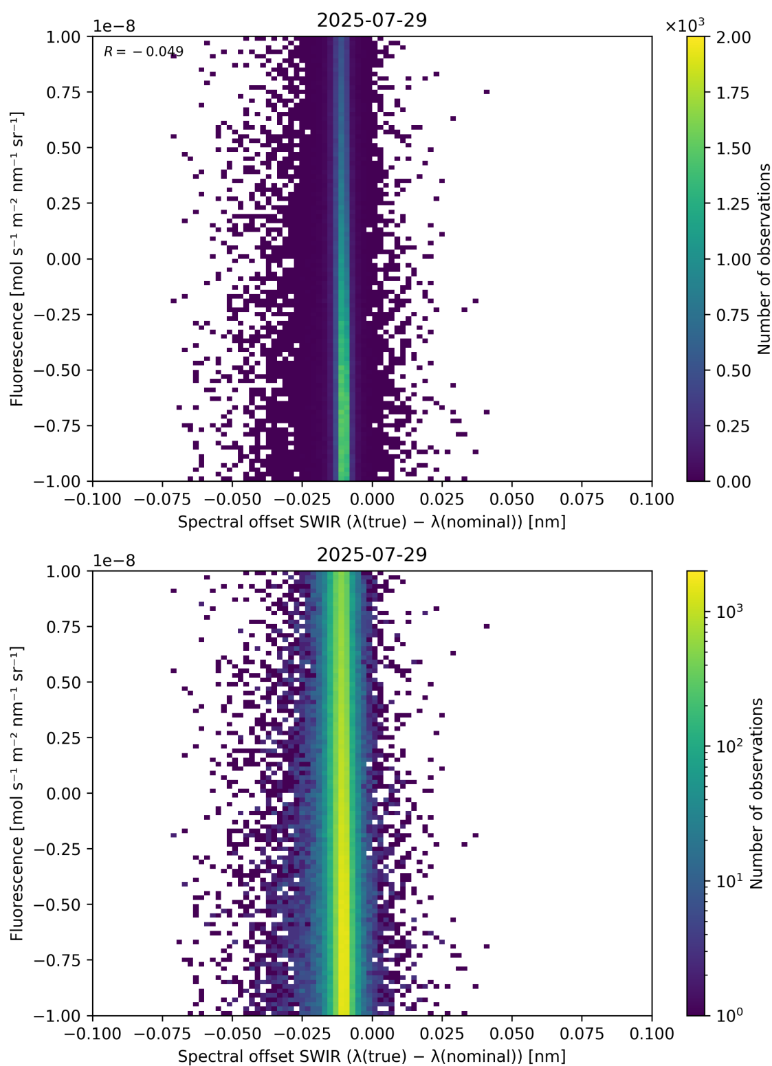
Figure 120: Scatter density plot of “Spectral offset SWIR ( \lambda_{\text{true}} - \lambda_{\text{nominal}} )” against “Fluorescence” for 2025-07-29 to 2025-07-30.
