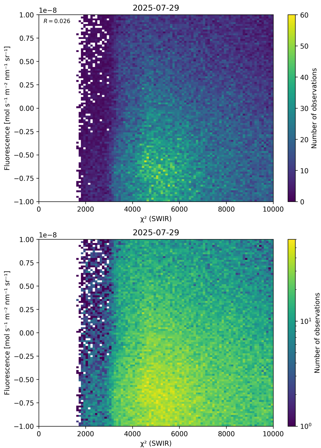
Figure 49: Scatter density plot of “ \chi^2 (SWIR)” against “Fluorescence” for 2025-07-29 to 2025-07-30.
