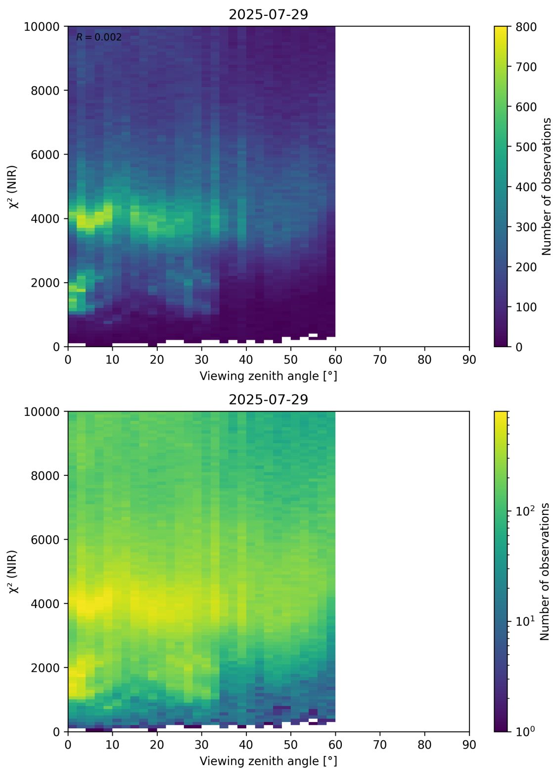
Figure 105: Scatter density plot of “Viewing zenith angle” against “ \chi^2 (NIR)” for 2025-07-29 to 2025-07-30.
