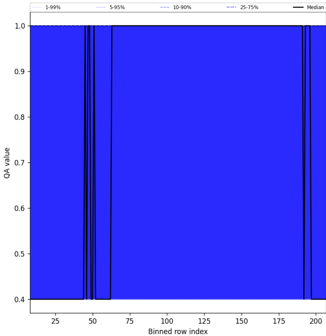
Figure 33: Along track statistics of “QA value” for 2025-07-29 to 2025-07-30
