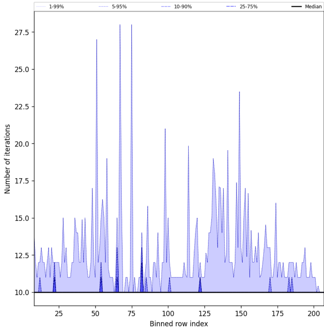
Figure 42: Along track statistics of “Number of iterations” for 2025-07-29 to 2025-07-30
