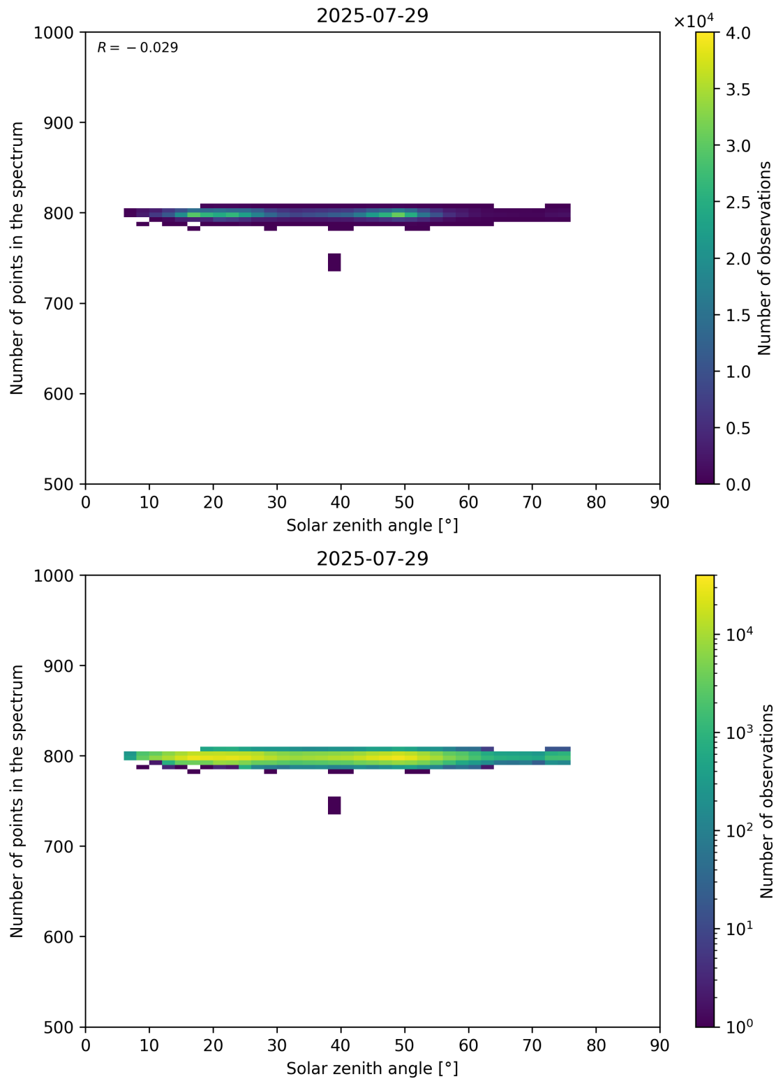
Figure 103: Scatter density plot of “Solar zenith angle” against “Number of points in the spectrum” for 2025-07-29 to 2025-07-30.
