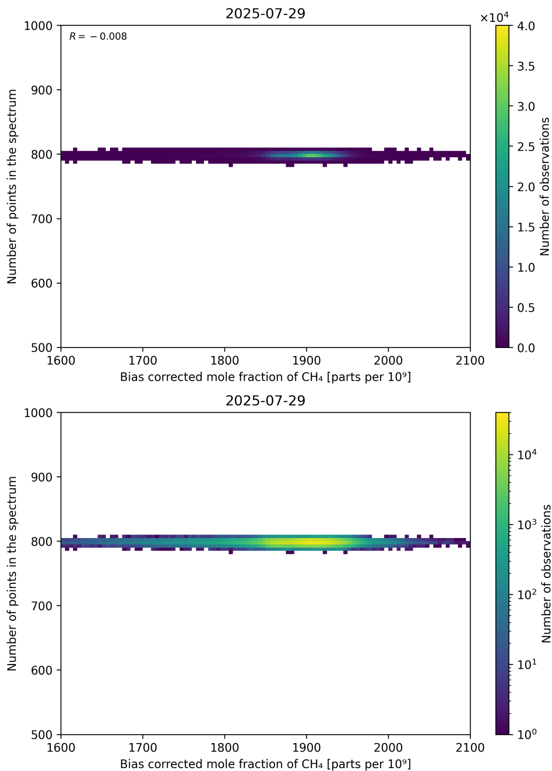
Figure 68: Scatter density plot of “Bias corrected mole fraction of CH 4 ” against “Number of points in the spectrum” for 2025-07-29 to 2025-07-30.
