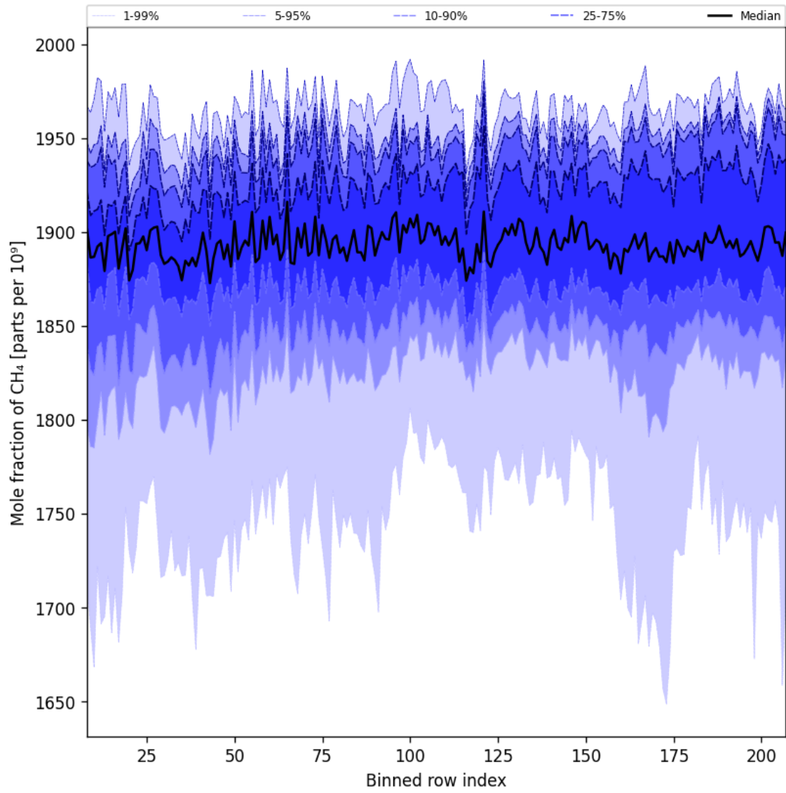
Figure 34: Along track statistics of “Mole fraction of CH 4 ” for 2025-07-29 to 2025-07-30
