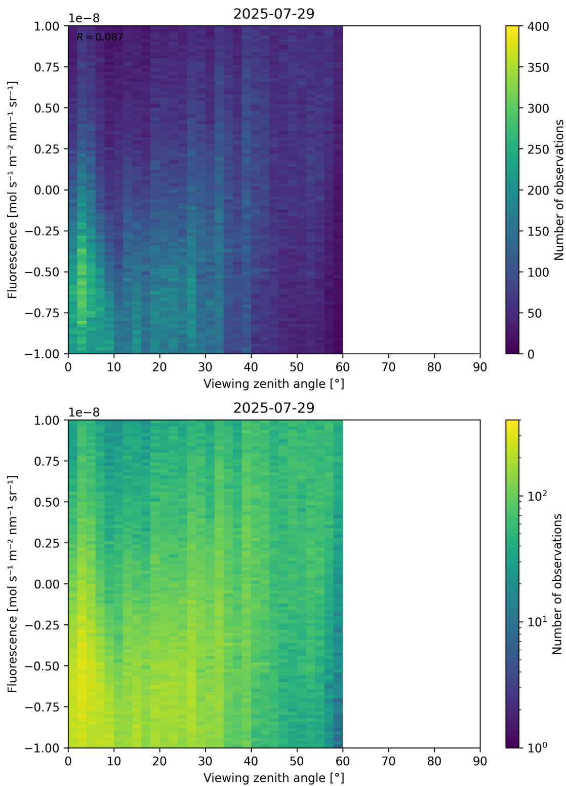
Figure 108: Scatter density plot of “Viewing zenith angle” against “Fluorescence” for 2025-07-29 to 2025-07-30.
