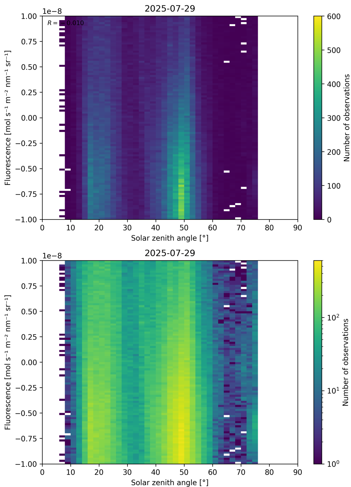
Figure 97: Scatter density plot of “Solar zenith angle” against “Fluorescence” for 2025-07-29 to 2025-07-30.
