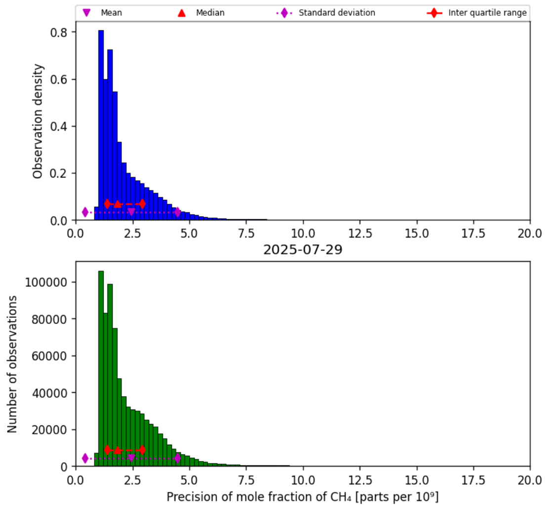
Figure 24: Histogram of “Precision of mole fraction of CH 4 ” for 2025-07-29 to 2025-07-30
