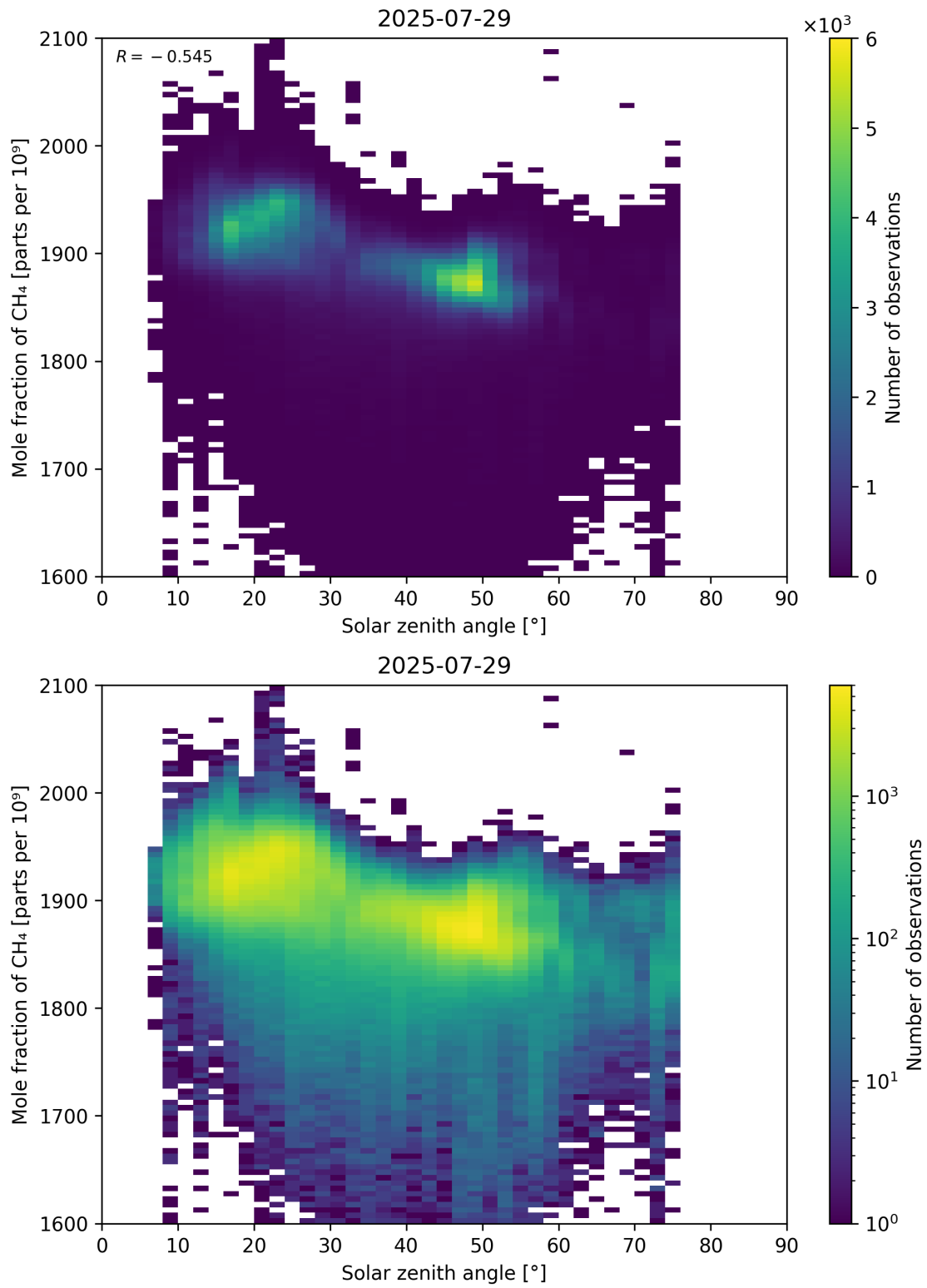
Figure 99: Scatter density plot of “Solar zenith angle” against “Mole fraction of CH 4 ” for 2025-07-29 to 2025-07-30.
