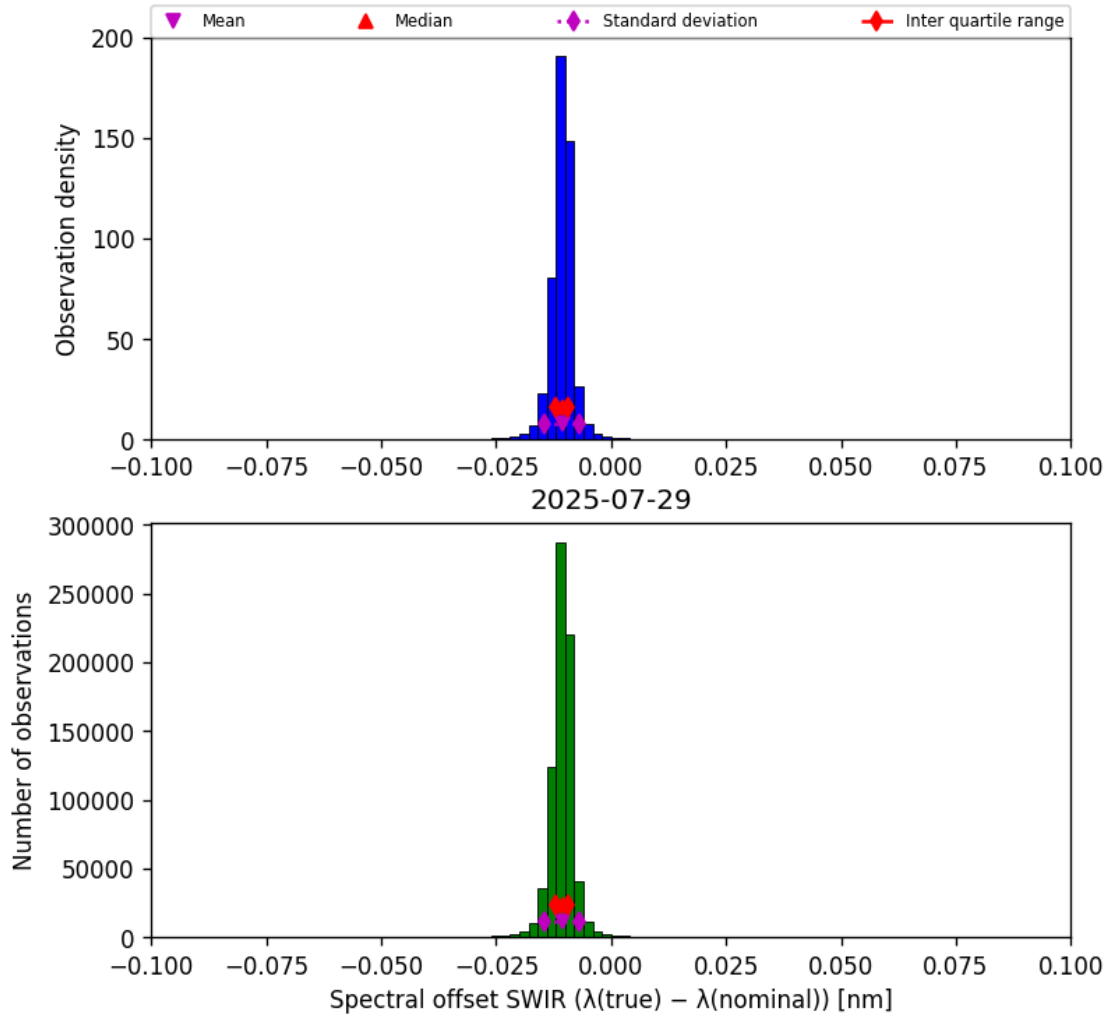
Figure 27: Histogram of “Spectral offset SWIR ( \lambda_{\text{true}} - \lambda_{\text{nominal}} )” for 2025-07-29 to 2025-07-30
