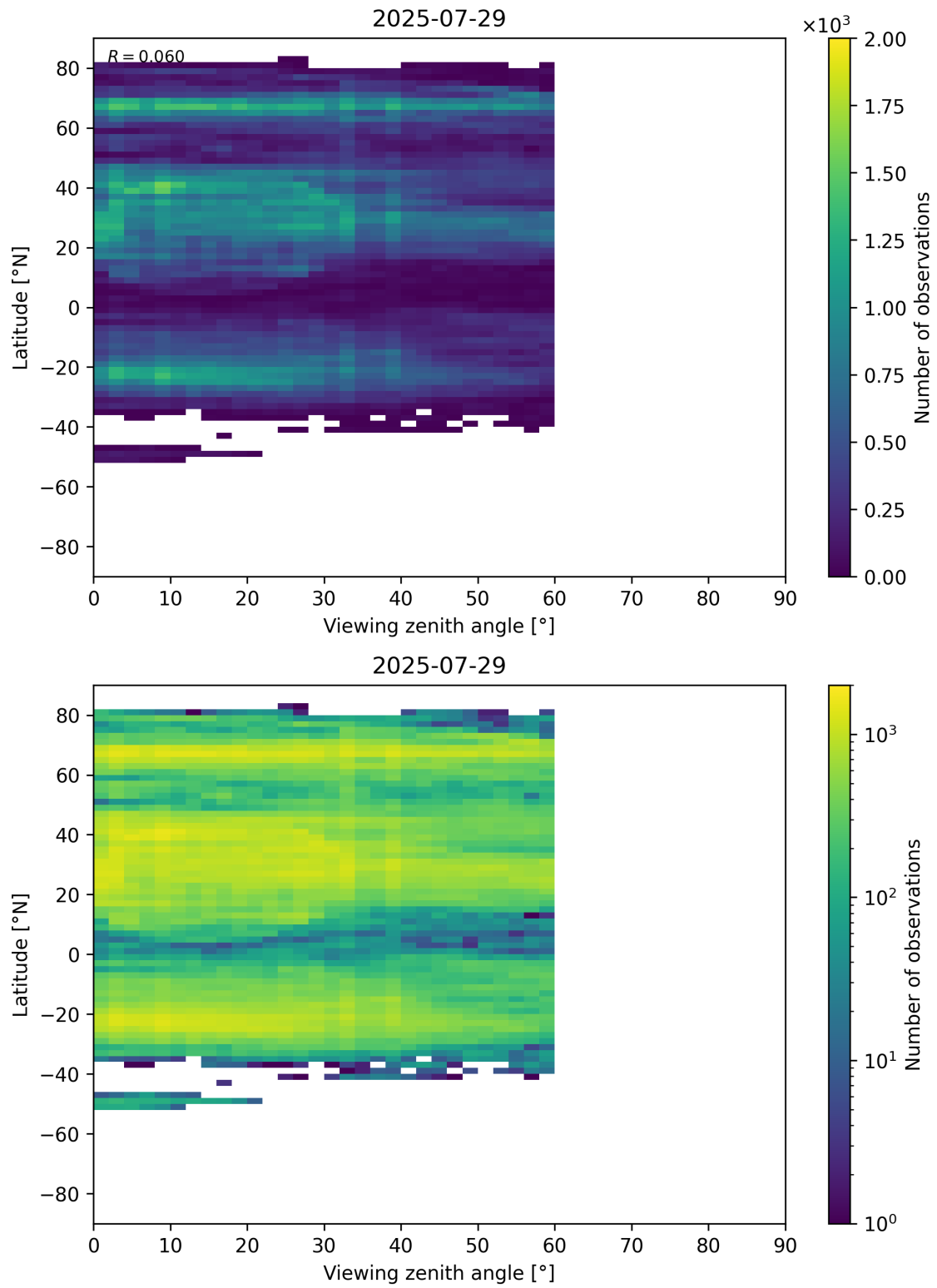
Figure 109: Scatter density plot of “Viewing zenith angle” against “Latitude” for 2025-07-29 to 2025-07-30.
