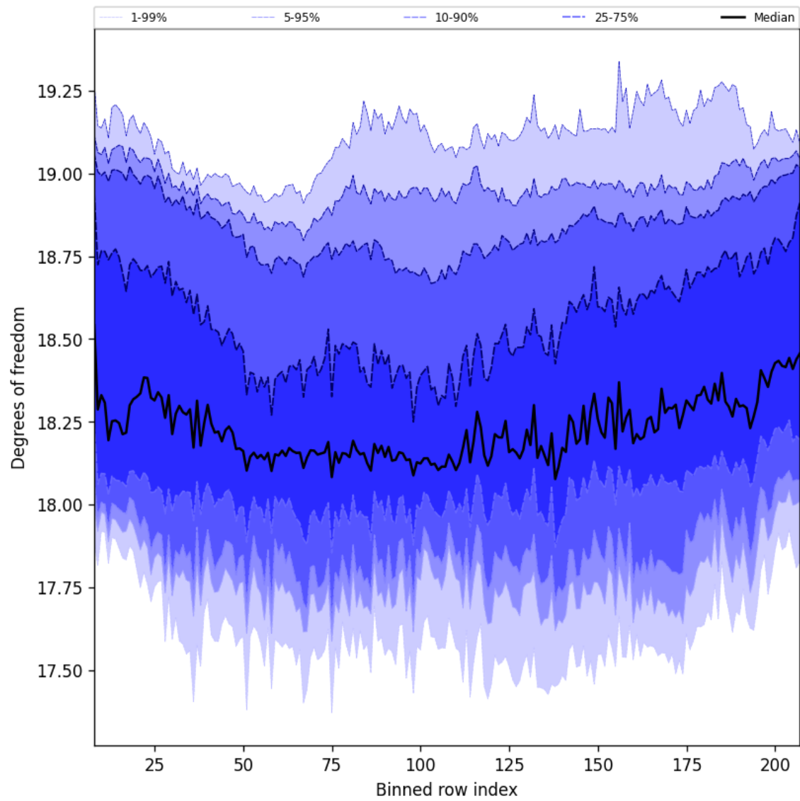
Figure 41: Along track statistics of “Degrees of freedom” for 2025-07-29 to 2025-07-30
