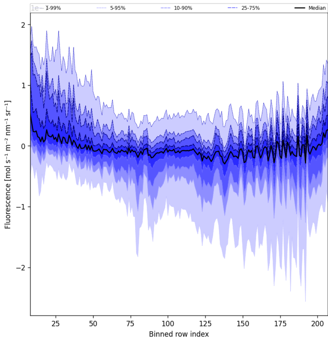
Figure 43: Along track statistics of “Fluorescence” for 2025-07-29 to 2025-07-30
