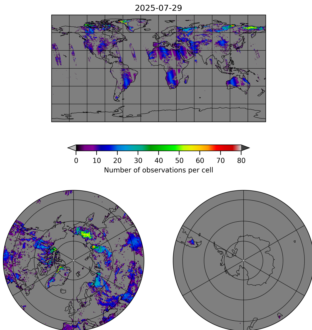
Figure 10: Map of the number of observations for 2025-07-29 to 2025-07-30
