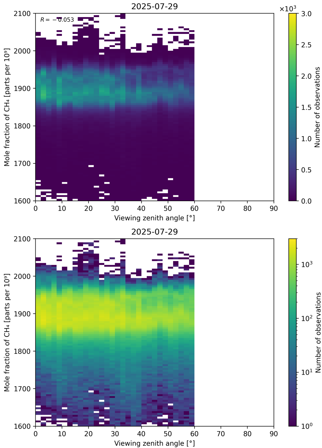
Figure 110: Scatter density plot of “Viewing zenith angle” against “Mole fraction of CH 4 ” for 2025-07-29 to 2025-07-30.
