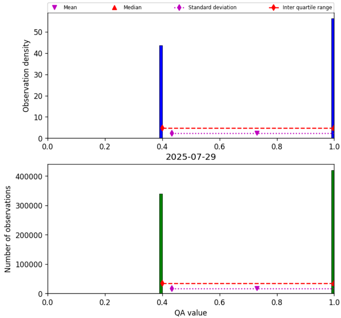
Figure 22: Histogram of “QA value” for 2025-07-29 to 2025-07-30
