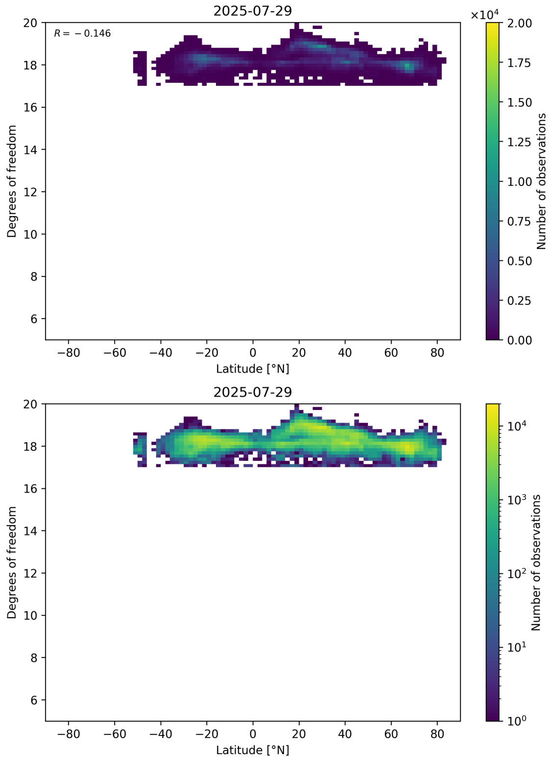
Figure 55: Scatter density plot of “Latitude” against “Degrees of freedom” for 2025-07-29 to 2025-07-30.
