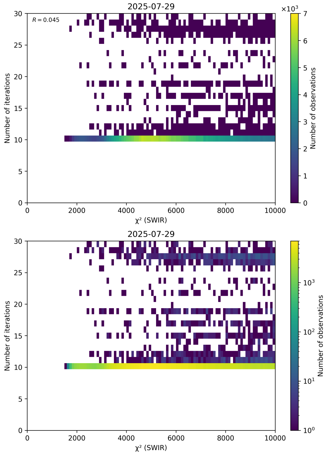
Figure 50: Scatter density plot of “ \chi^2 (SWIR)” against “Number of iterations” for 2025-07-29 to 2025-07-30.
