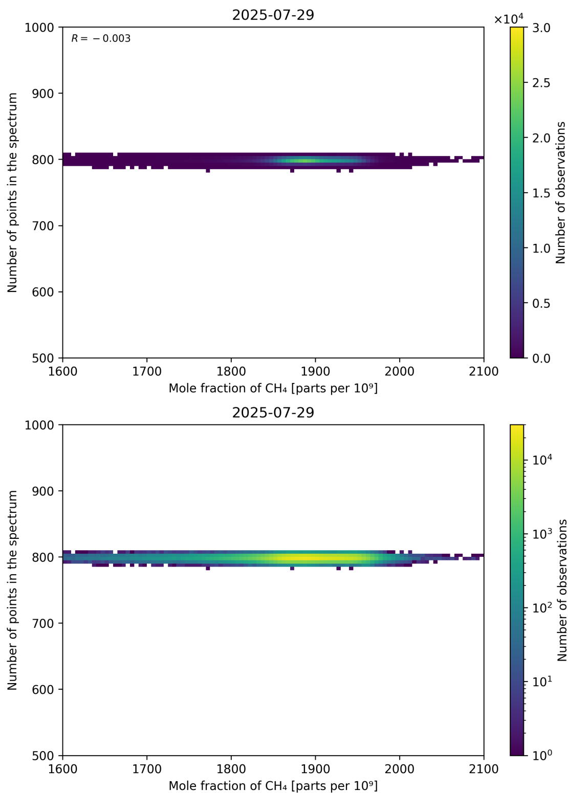
Figure 77: Scatter density plot of “Mole fraction of CH 4 ” against “Number of points in the spectrum” for 2025-07-29 to 2025-07-30.
