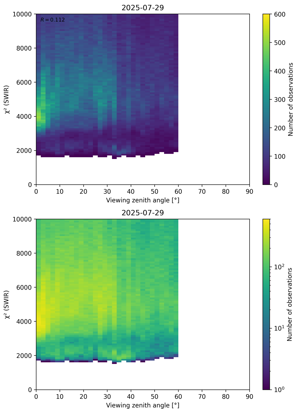
Figure 106: Scatter density plot of “Viewing zenith angle” against “ \chi^2 (SWIR)” for 2025-07-29 to 2025-07-30.
