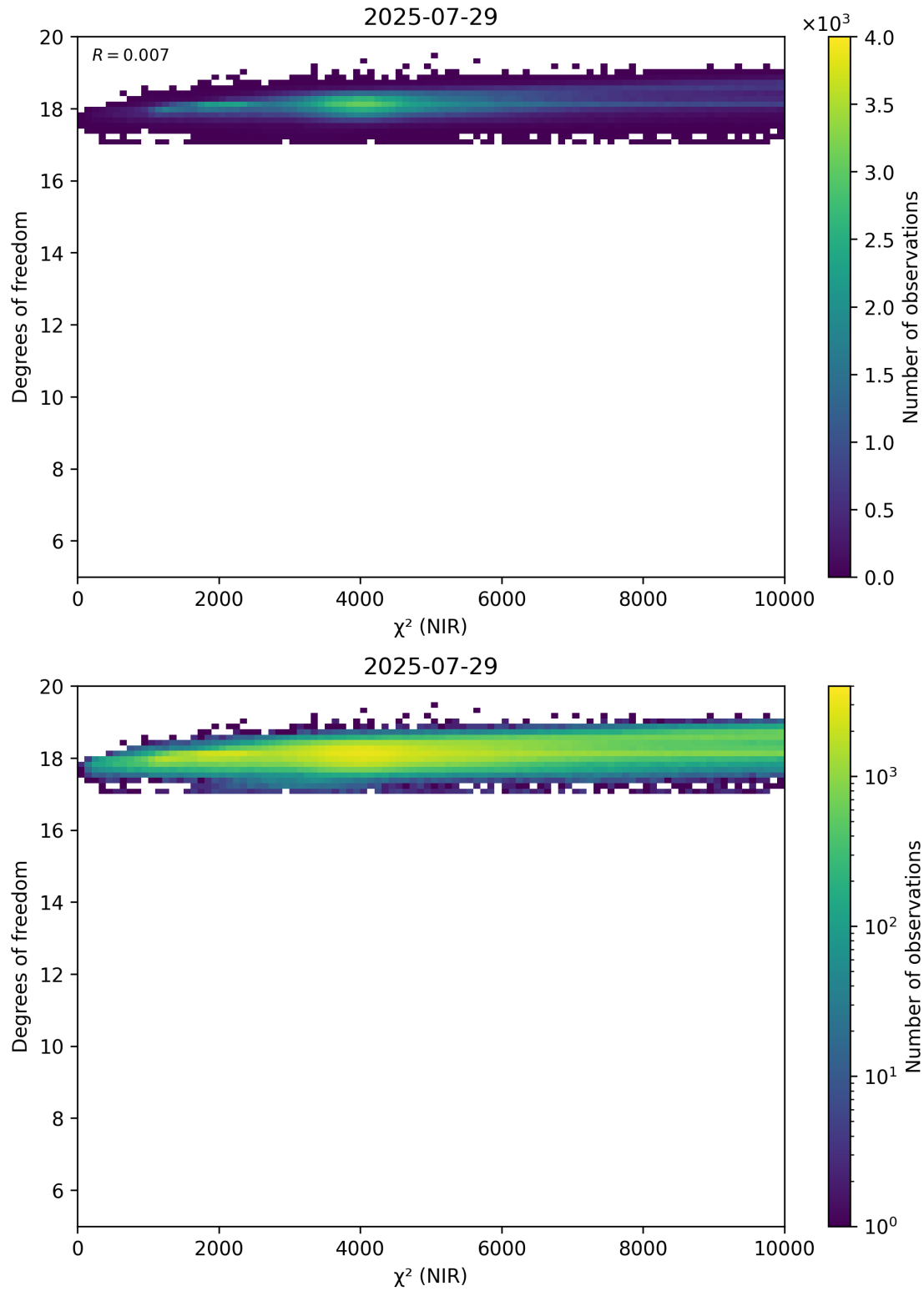
Figure 44: Scatter density plot of “ \chi^2 (NIR)” against “Degrees of freedom” for 2025-07-29 to 2025-07-30.
