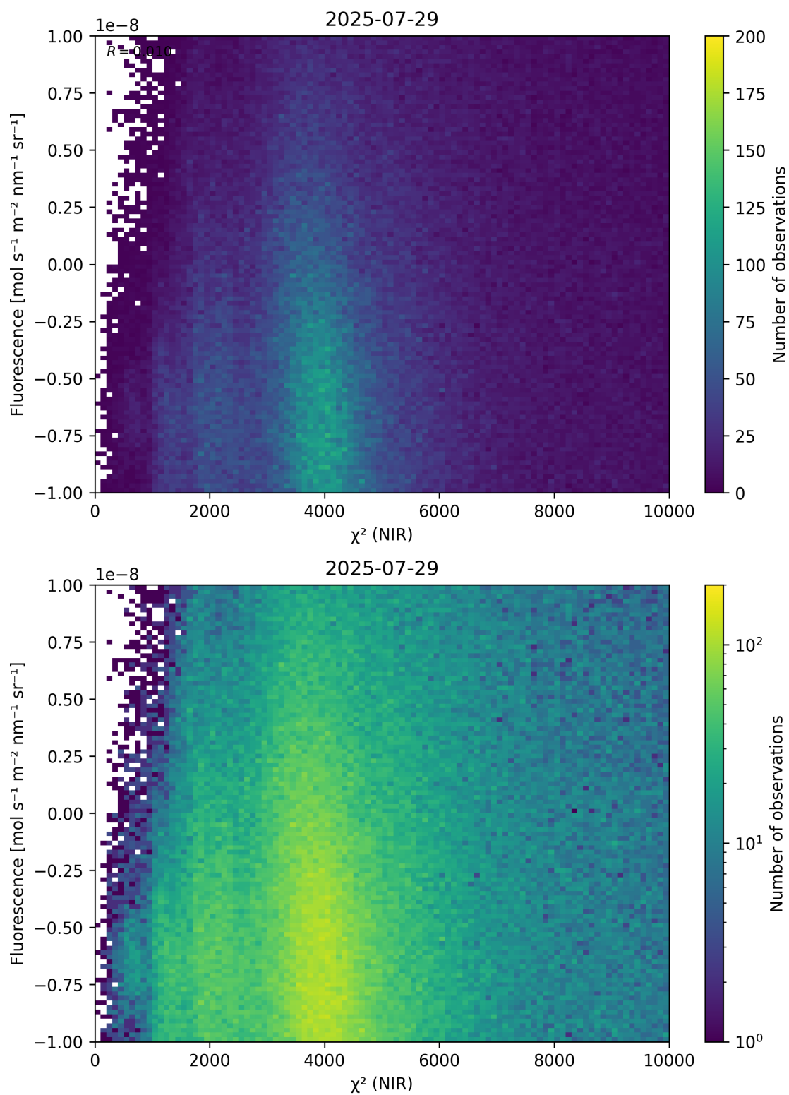
Figure 45: Scatter density plot of “ \chi^2 (NIR)” against “Fluorescence” for 2025-07-29 to 2025-07-30.
