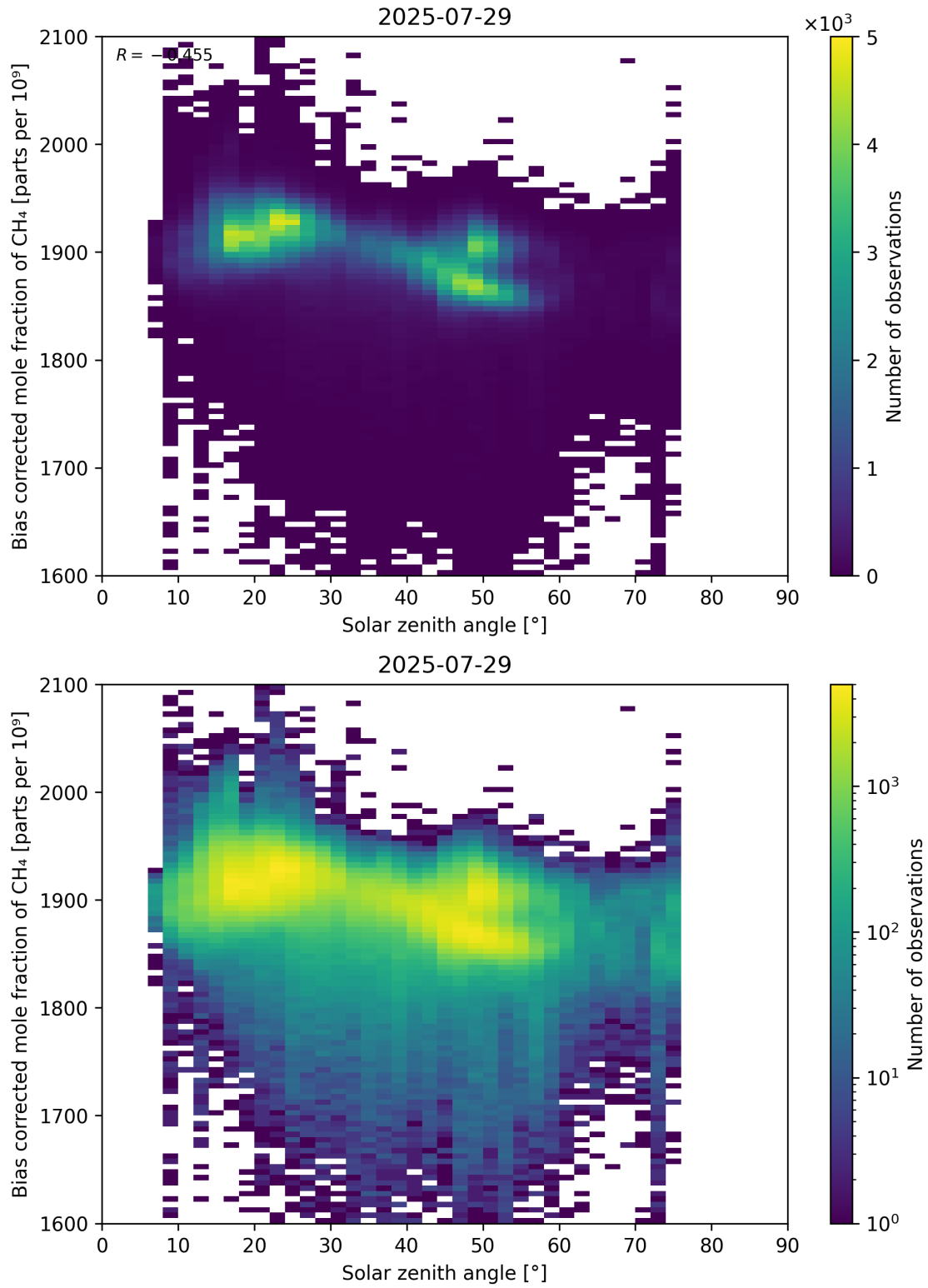
Figure 100: Scatter density plot of “Solar zenith angle” against “Bias corrected mole fraction of \text{CH}_4 ” for 2025-07-29 to 2025-07-30.
