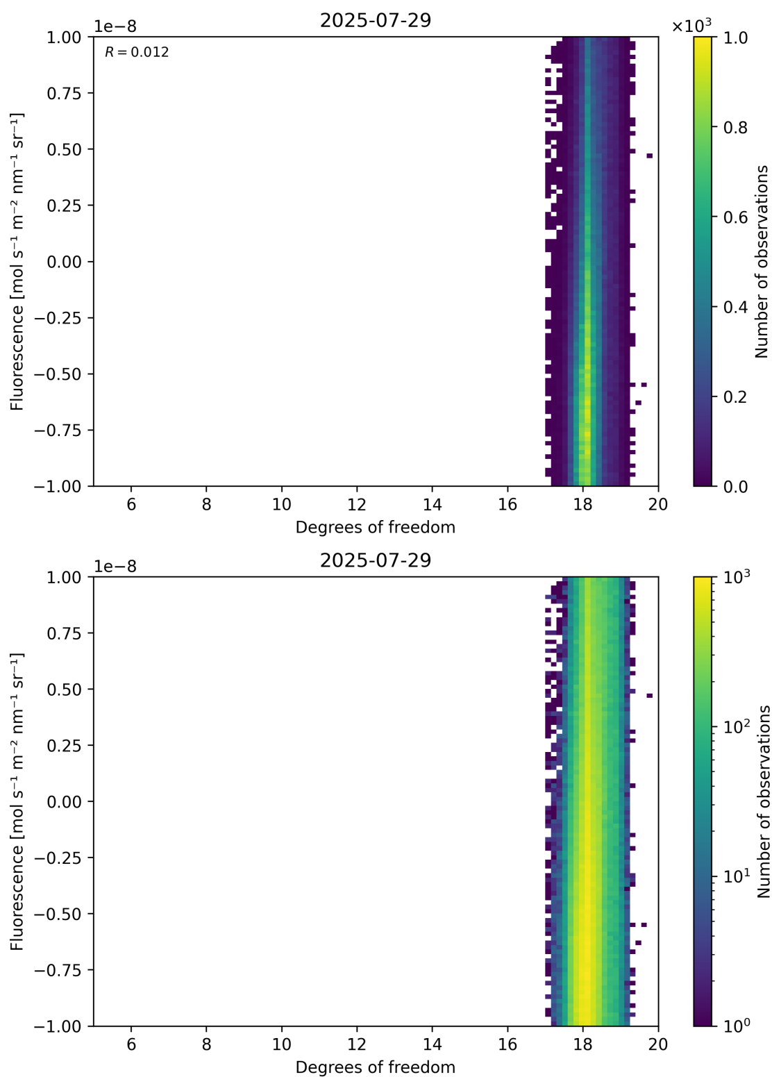
Figure 51: Scatter density plot of “Degrees of freedom” against “Fluorescence” for 2025-07-29 to 2025-07-30.
