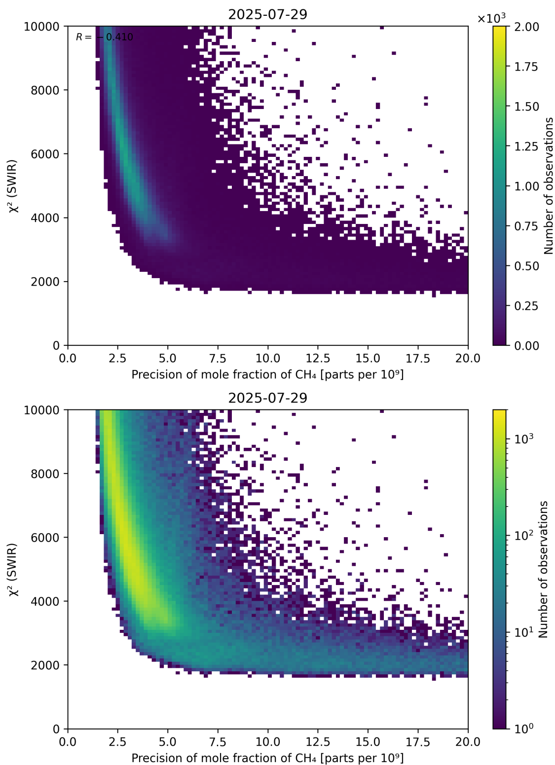
Figure 79: Scatter density plot of “Precision of mole fraction of \text{CH}_4 ” against “ \chi^2 (SWIR)” for 2025-07-29 to 2025-07-30.
