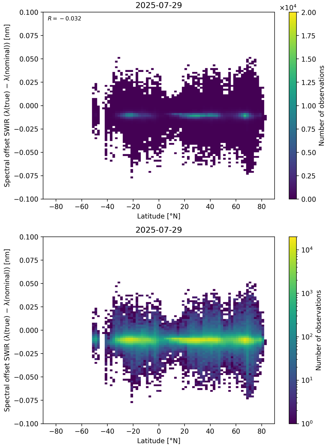
Figure 62: Scatter density plot of “Latitude” against “Spectral offset SWIR ( \lambda_{\text{true}} - \lambda_{\text{nominal}} )” for 2025-07-29 to 2025-07-30.
