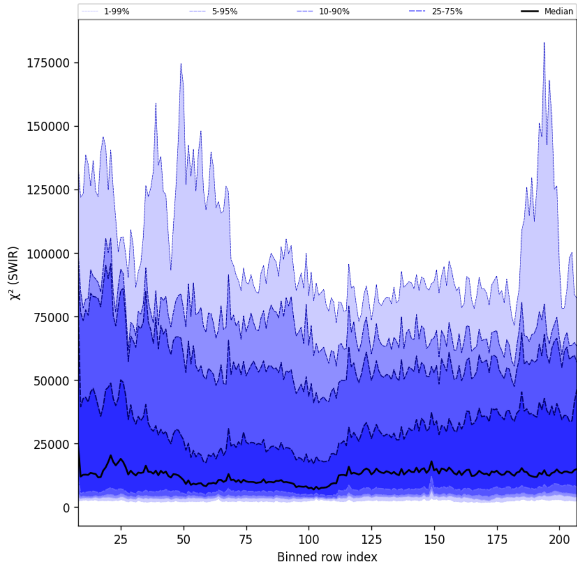
Figure 39: Along track statistics of " \chi^2 (SWIR)" for 2025-07-29 to 2025-07-30
