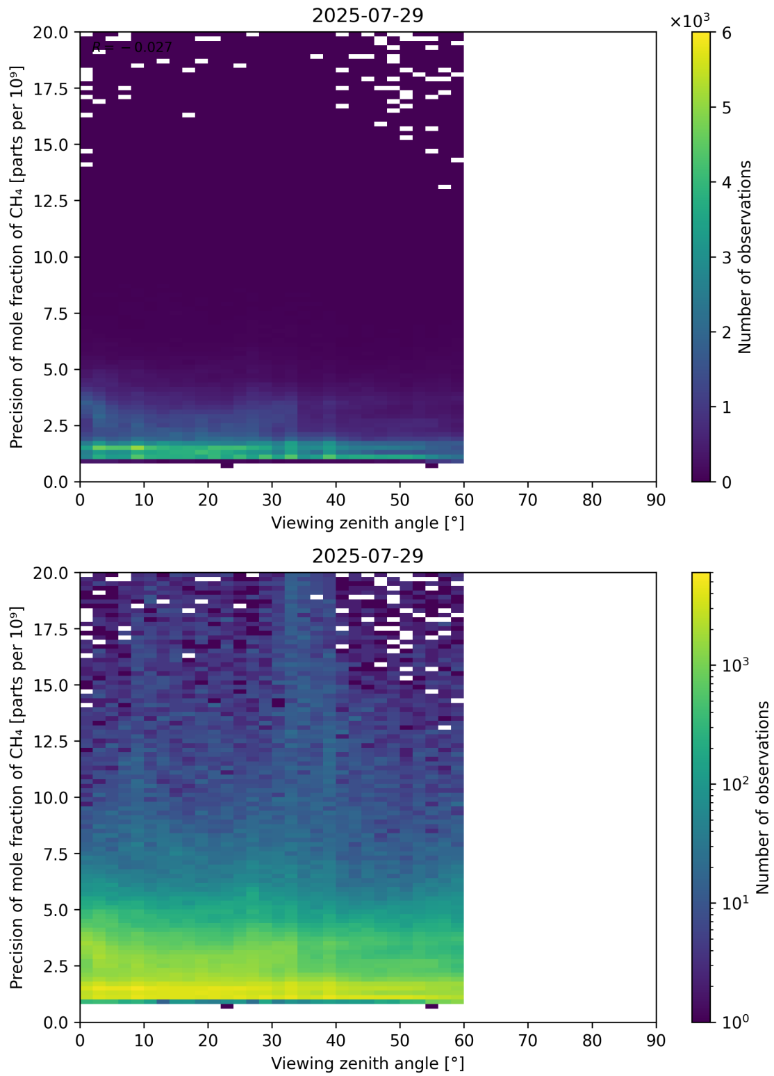
Figure 112: Scatter density plot of “Viewing zenith angle” against “Precision of mole fraction of CH 4 ” for 2025-07-29 to 2025-07-30.
