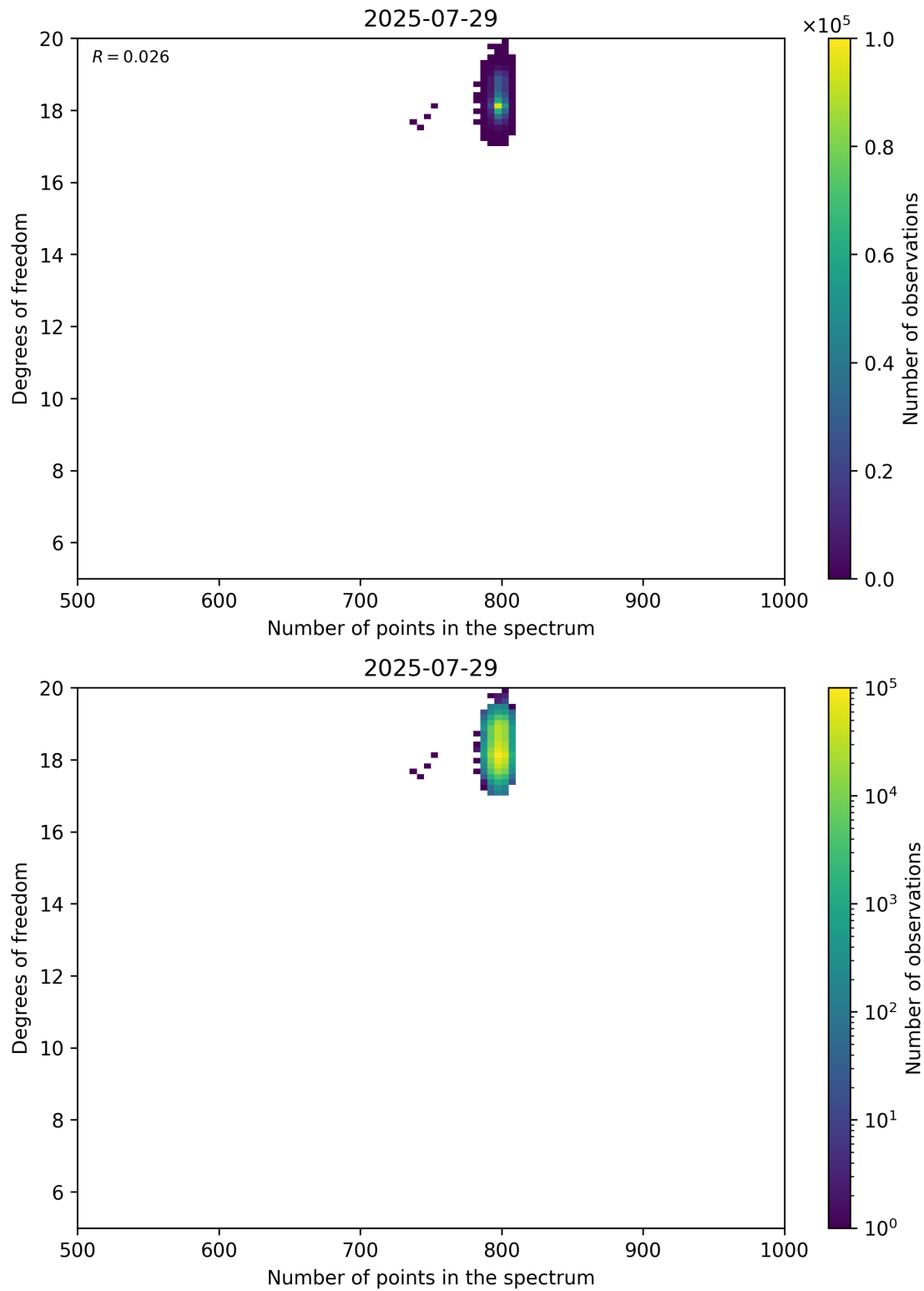
Figure 90: Scatter density plot of “Number of points in the spectrum” against “Degrees of freedom” for 2025-07-29 to 2025-07-30.
