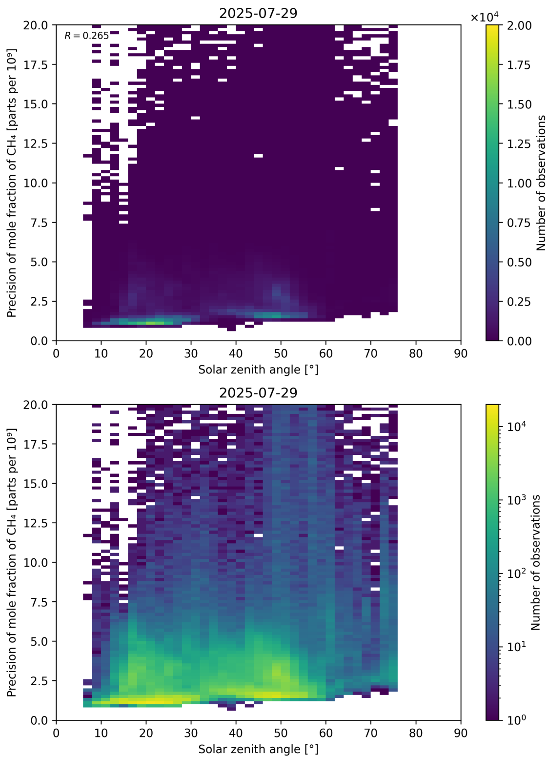
Figure 101: Scatter density plot of “Solar zenith angle” against “Precision of mole fraction of CH 4 ” for 2025-07-29 to 2025-07-30.
