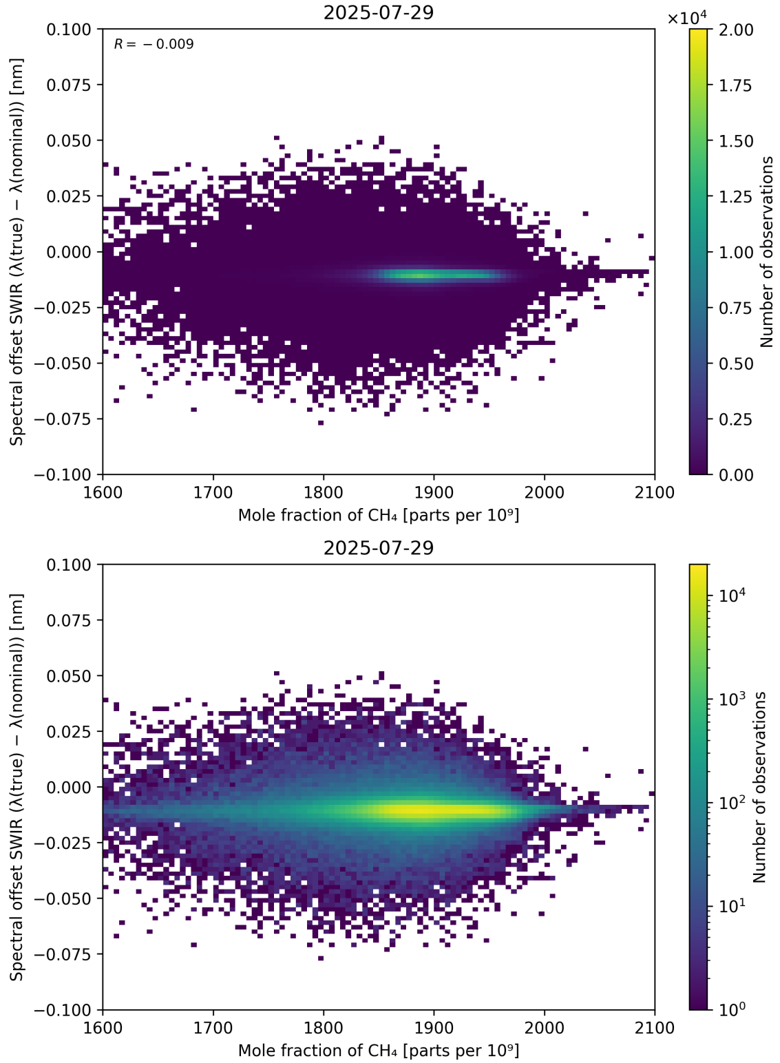
Figure 86: Scatter density plot of “Mole fraction of CH 4 ” against “Spectral offset SWIR ( \lambda_{\text{true}} - \lambda_{\text{nominal}} )” for 2025-07-29 to 2025-07-30.
