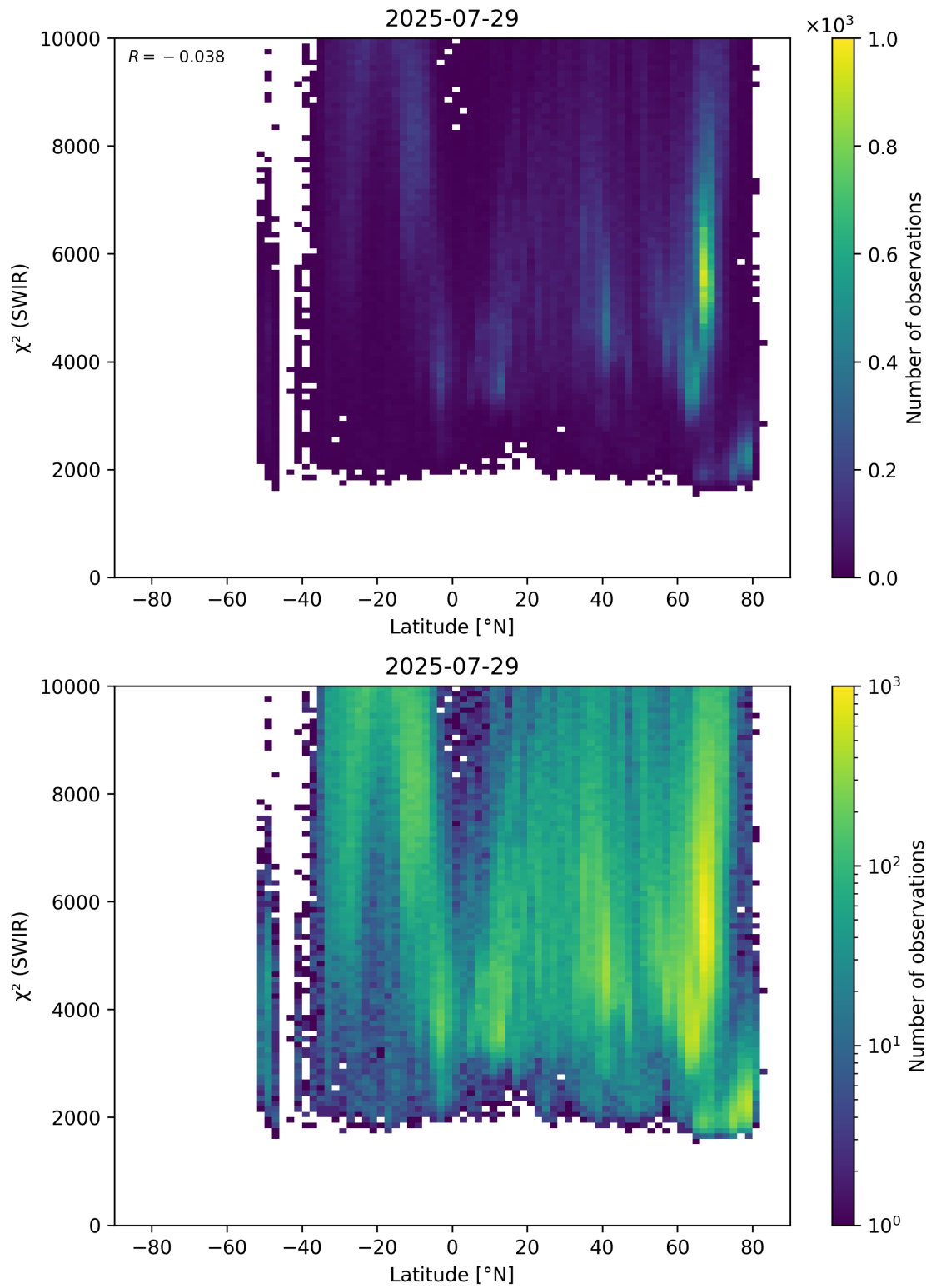
Figure 54: Scatter density plot of “Latitude” against “ \chi^2 (SWIR)” for 2025-07-29 to 2025-07-30.
