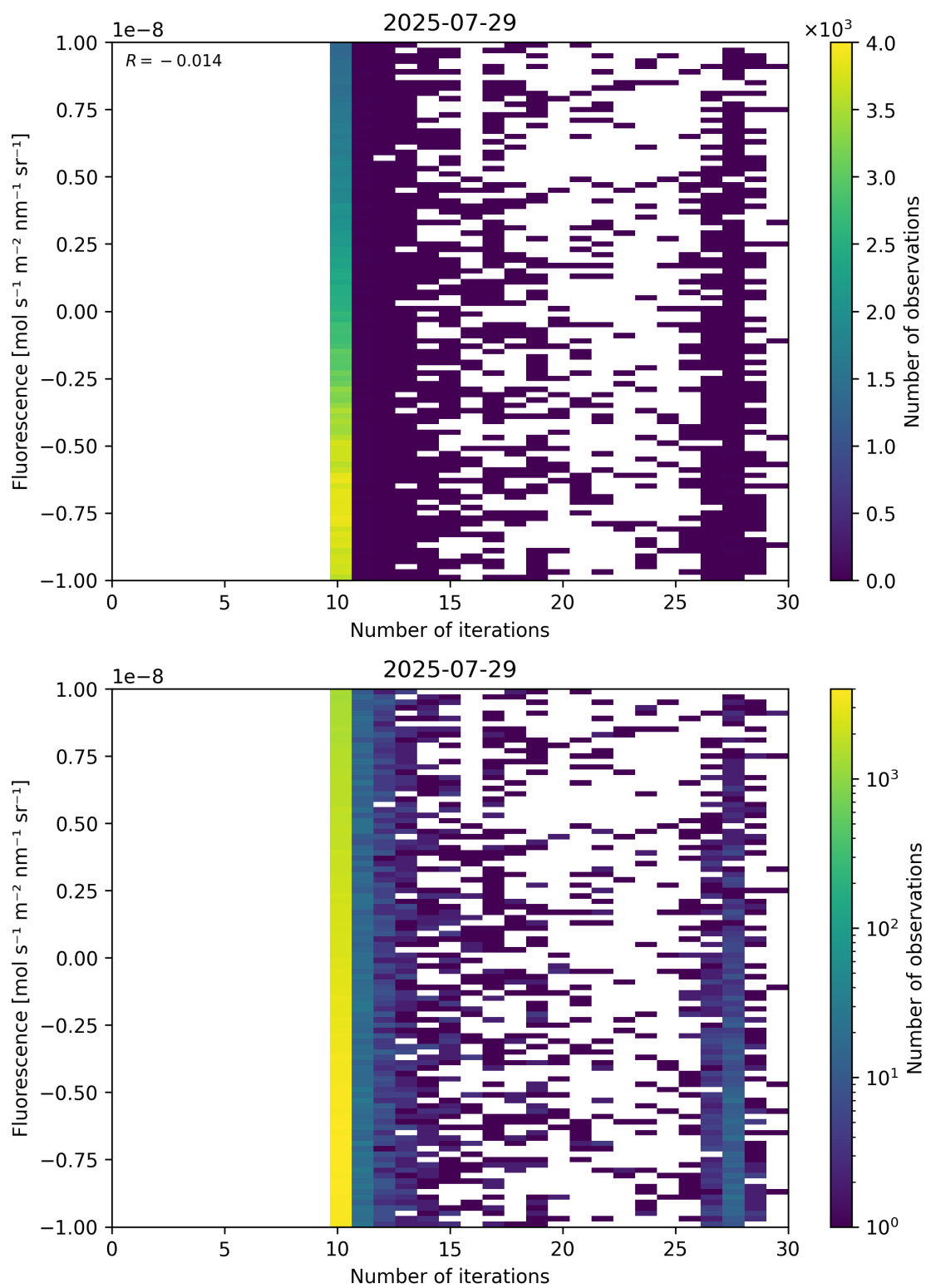
Figure 87: Scatter density plot of “Number of iterations” against “Fluorescence” for 2025-07-29 to 2025-07-30.
