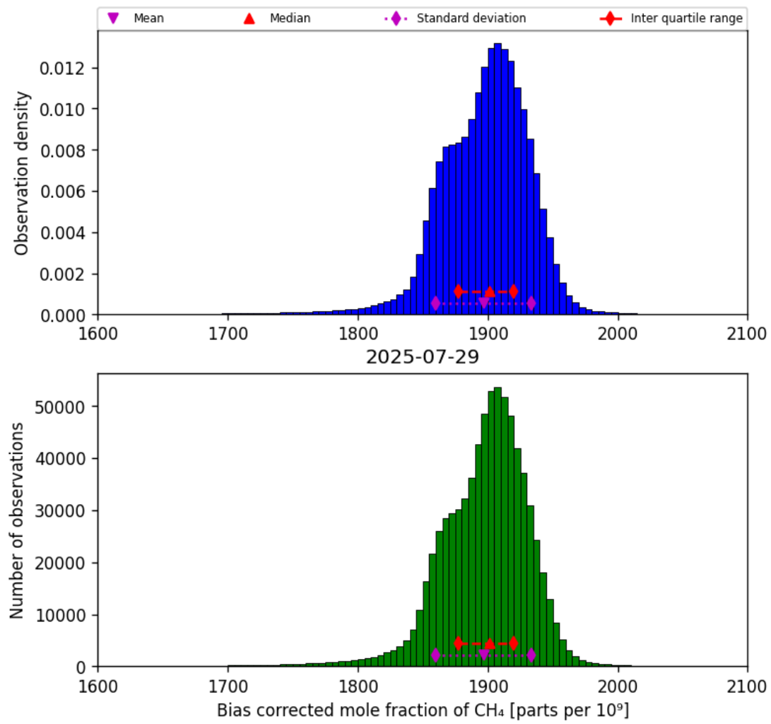
Figure 25: Histogram of “Bias corrected mole fraction of CH 4 ” for 2025-07-29 to 2025-07-30
