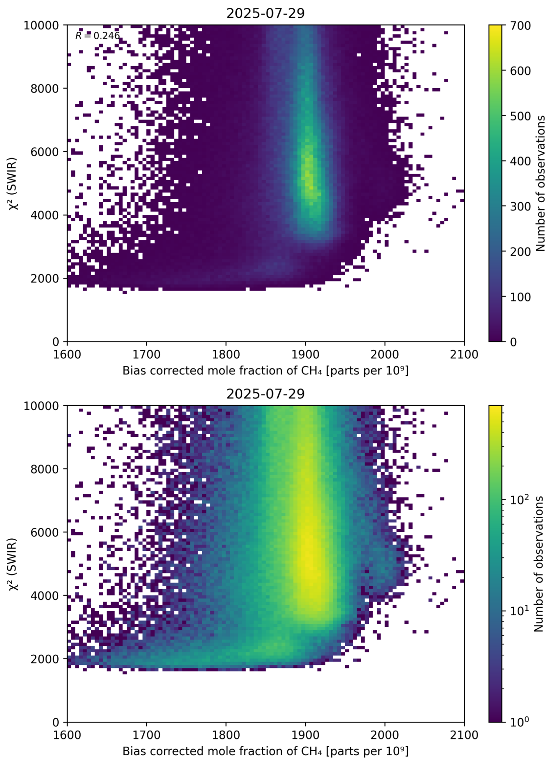
Figure 64: Scatter density plot of “Bias corrected mole fraction of \text{CH}_4 ” against “ \chi^2 (SWIR)” for 2025-07-29 to 2025-07-30.
