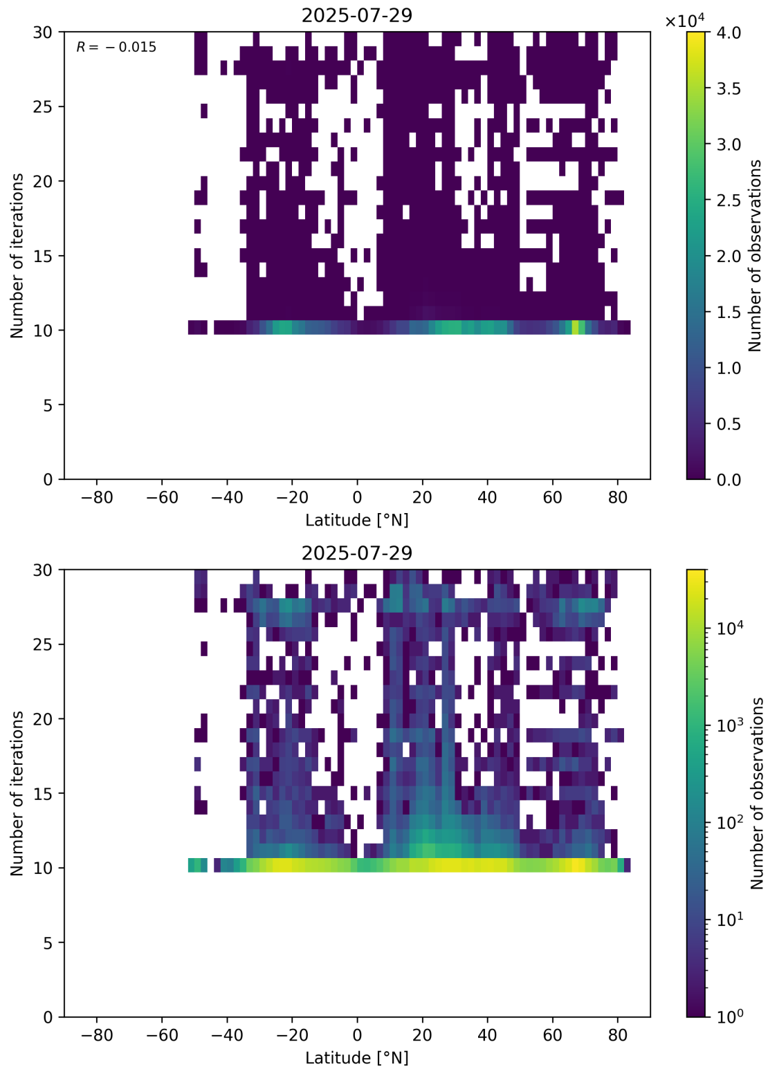
Figure 60: Scatter density plot of “Latitude” against “Number of iterations” for 2025-07-29 to 2025-07-30.
