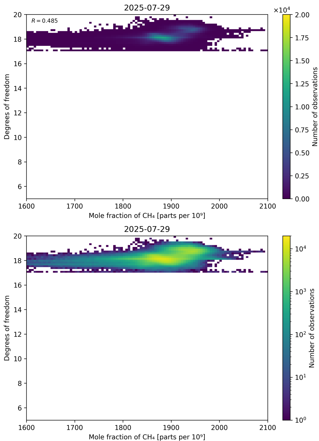
Figure 72: Scatter density plot of “Mole fraction of CH 4 ” against “Degrees of freedom” for 2025-07-29 to 2025-07-30.
