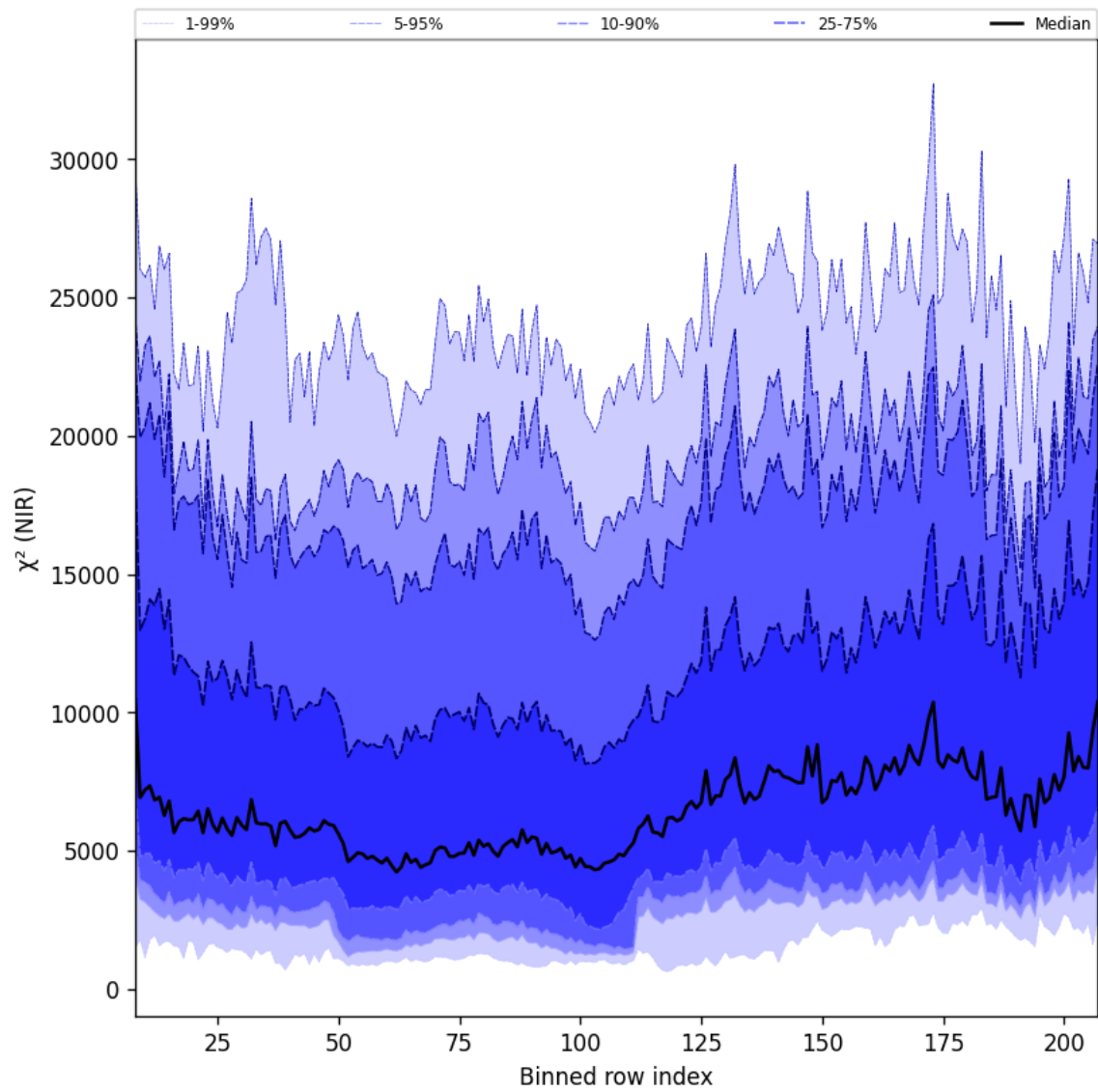
Figure 40: Along track statistics of “ \chi^2 (NIR)” for 2025-07-29 to 2025-07-30
