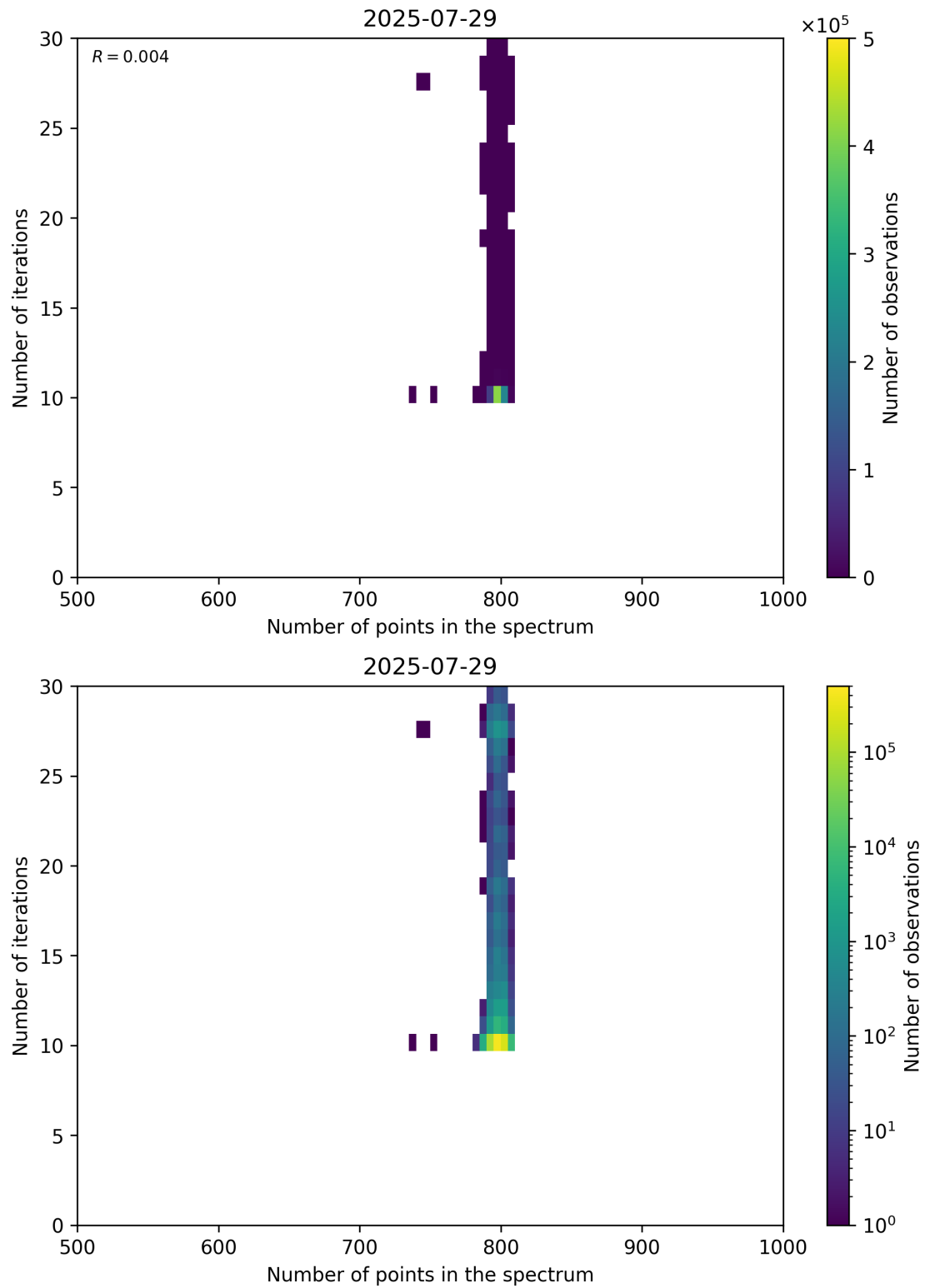
Figure 92: Scatter density plot of “Number of points in the spectrum” against “Number of iterations” for 2025-07-29 to 2025-07-30.
