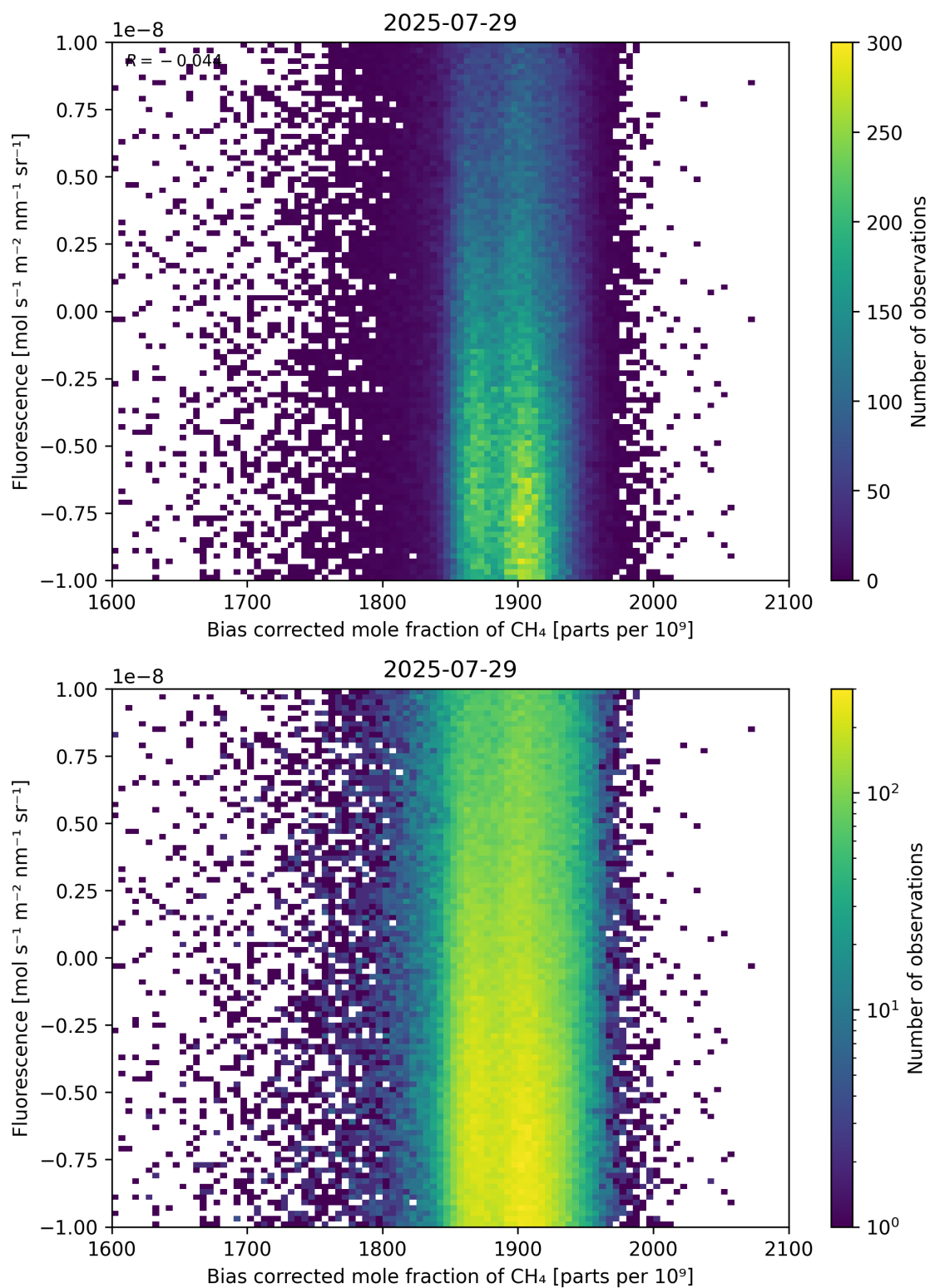
Figure 66: Scatter density plot of “Bias corrected mole fraction of \text{CH}_4 ” against “Fluorescence” for 2025-07-29 to 2025-07-30.
