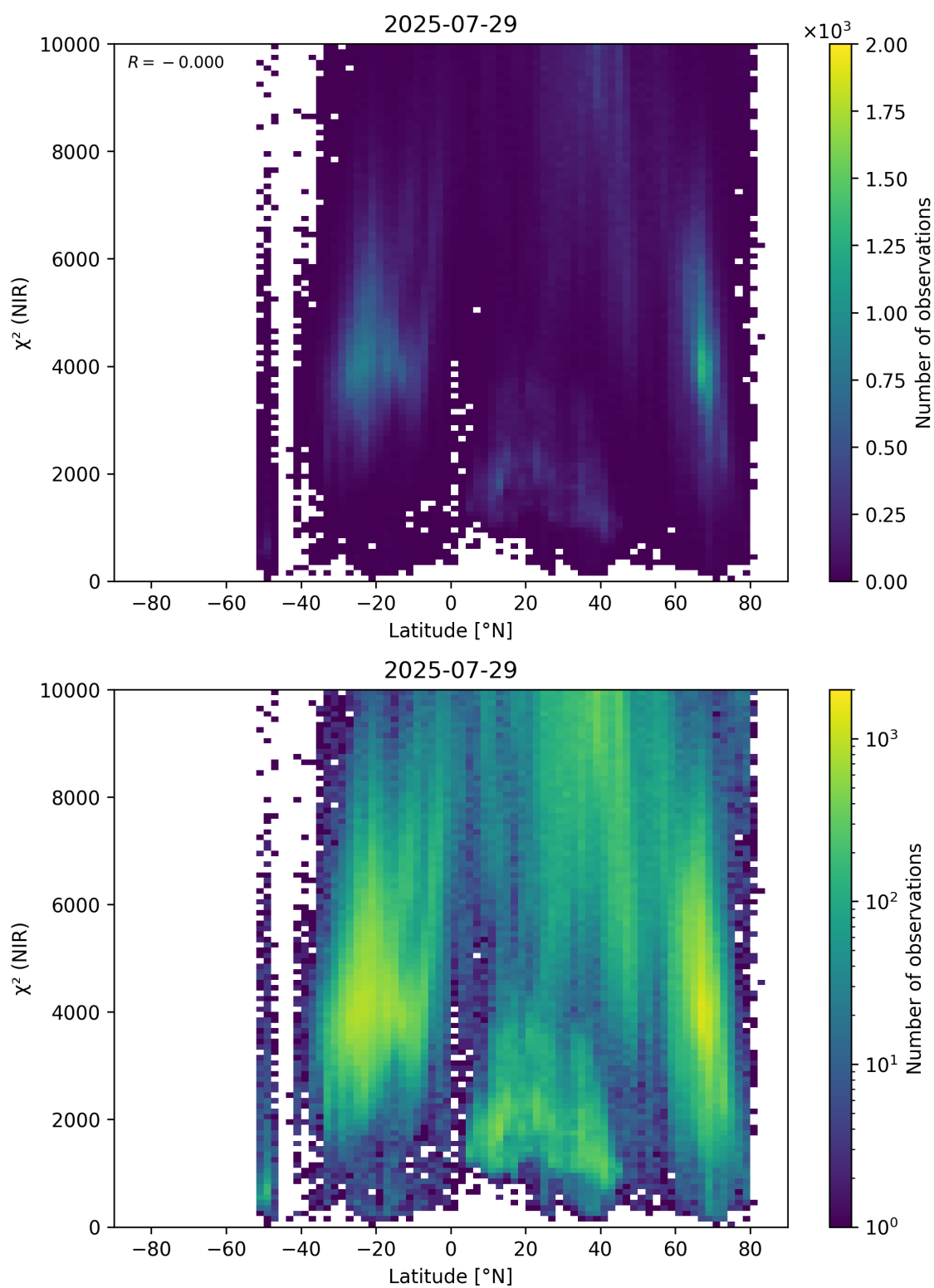
Figure 53: Scatter density plot of “Latitude” against “ \chi^2 (NIR)” for 2025-07-29 to 2025-07-30.
