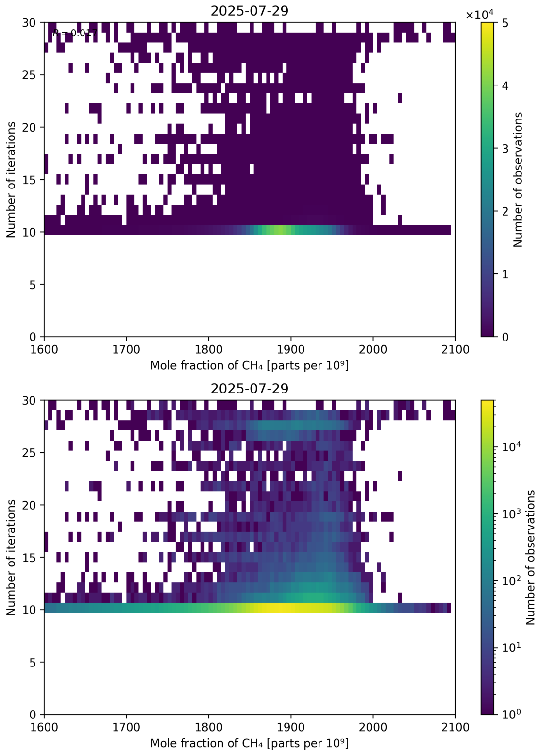
Figure 76: Scatter density plot of “Mole fraction of CH 4 ” against “Number of iterations” for 2025-07-29 to 2025-07-30.
