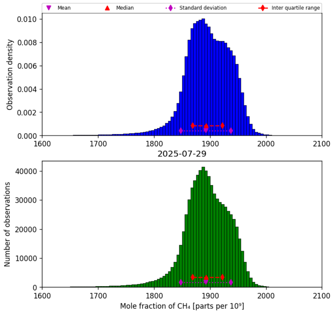
Figure 23: Histogram of “Mole fraction of CH 4 ” for 2025-07-29 to 2025-07-30
