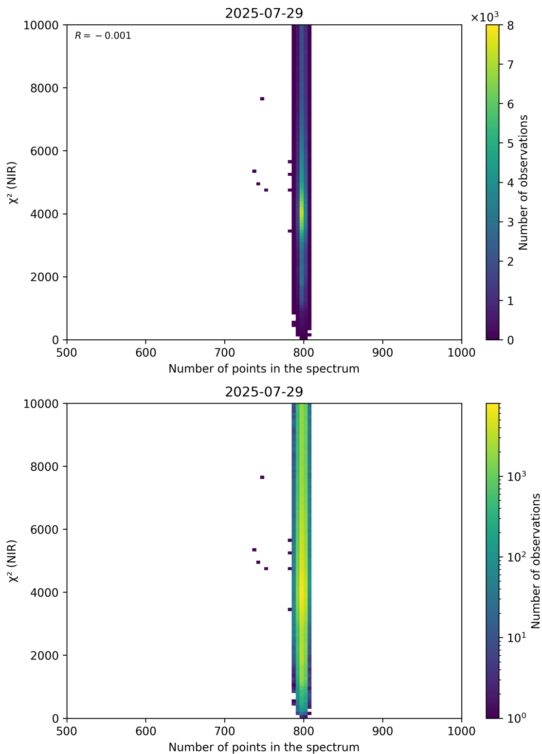
Figure 88: Scatter density plot of “Number of points in the spectrum” against “ \chi^2 (NIR)” for 2025-07-29 to 2025-07-30.
