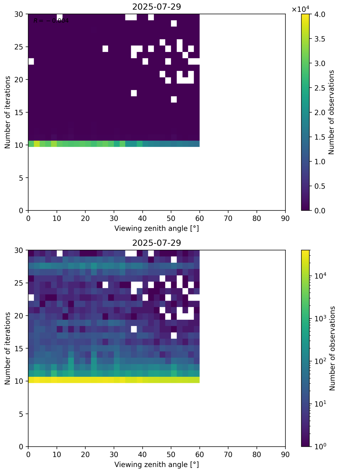
Figure 113: Scatter density plot of “Viewing zenith angle” against “Number of iterations” for 2025-07-29 to 2025-07-30.
