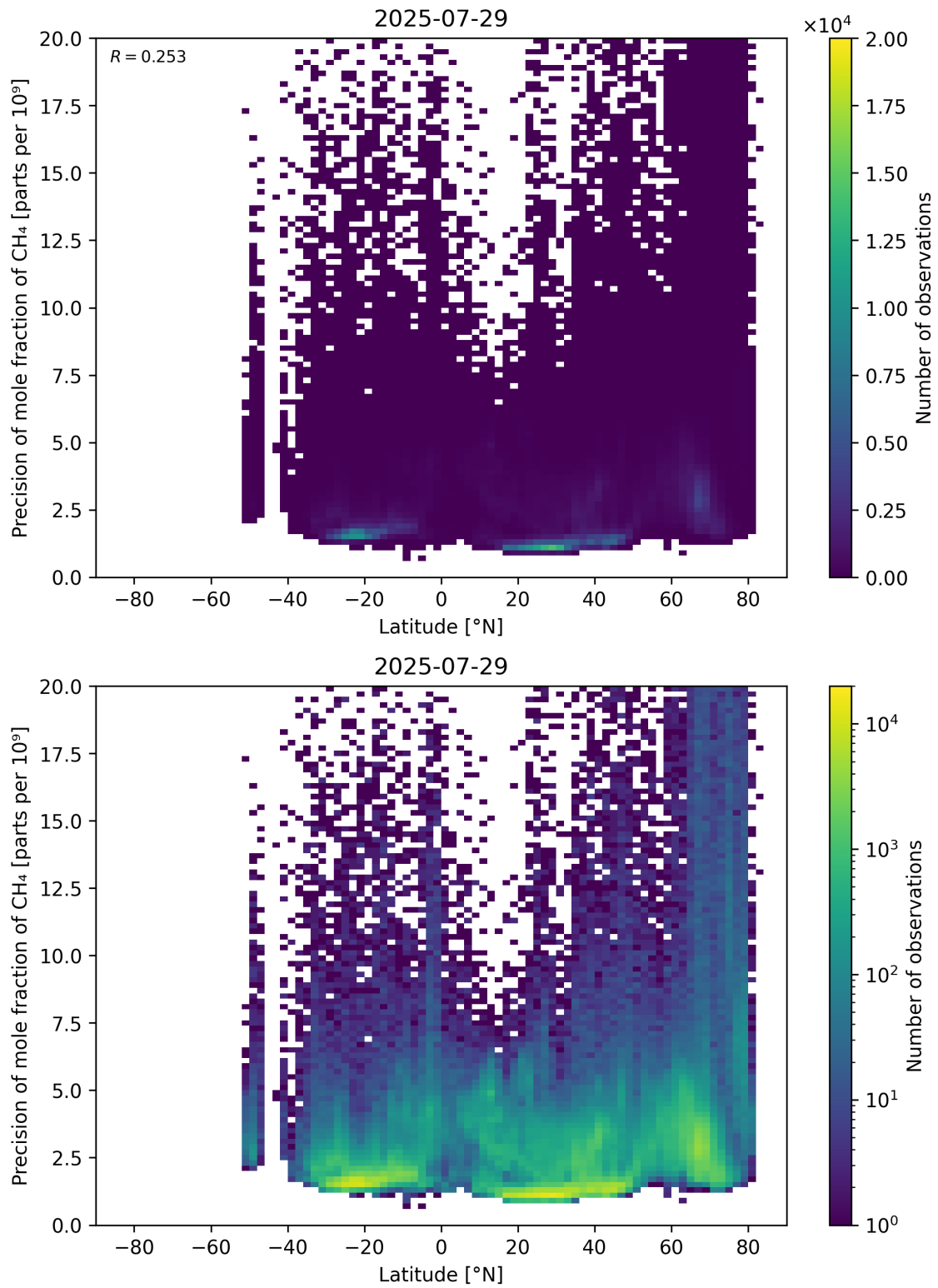
Figure 59: Scatter density plot of “Latitude” against “Precision of mole fraction of \text{CH}_4 ” for 2025-07-29 to 2025-07-30.
