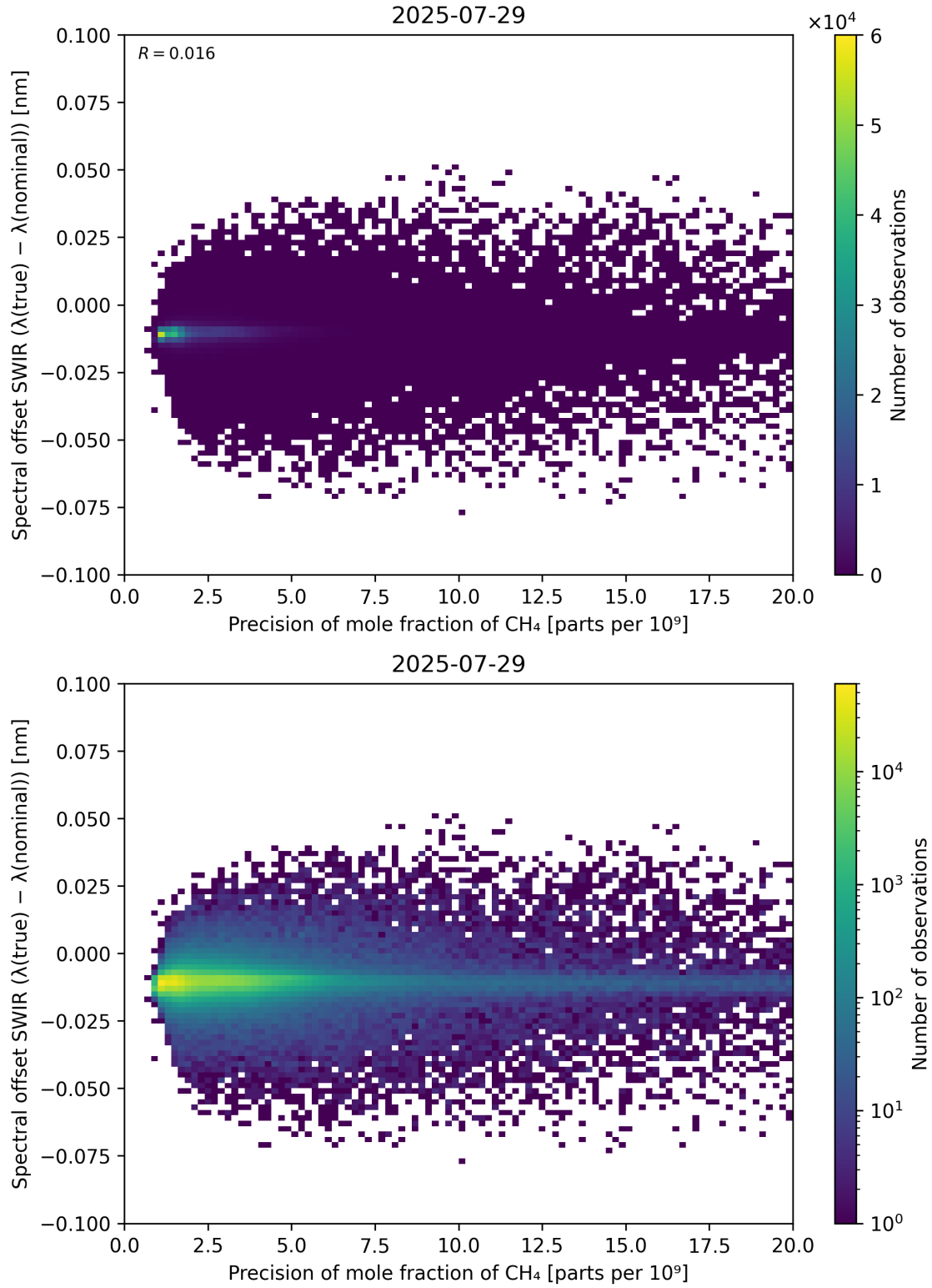
Figure 85: Scatter density plot of “Precision of mole fraction of CH 4 ” against “Spectral offset SWIR ( \lambda_{\text{true}} - \lambda_{\text{nominal}} )” for 2025-07-29 to 2025-07-30.
