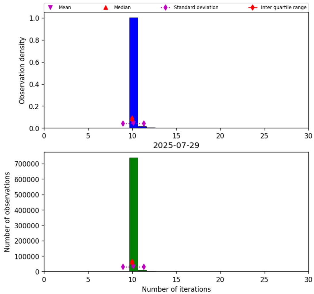
Figure 31: Histogram of “Number of iterations” for 2025-07-29 to 2025-07-30
