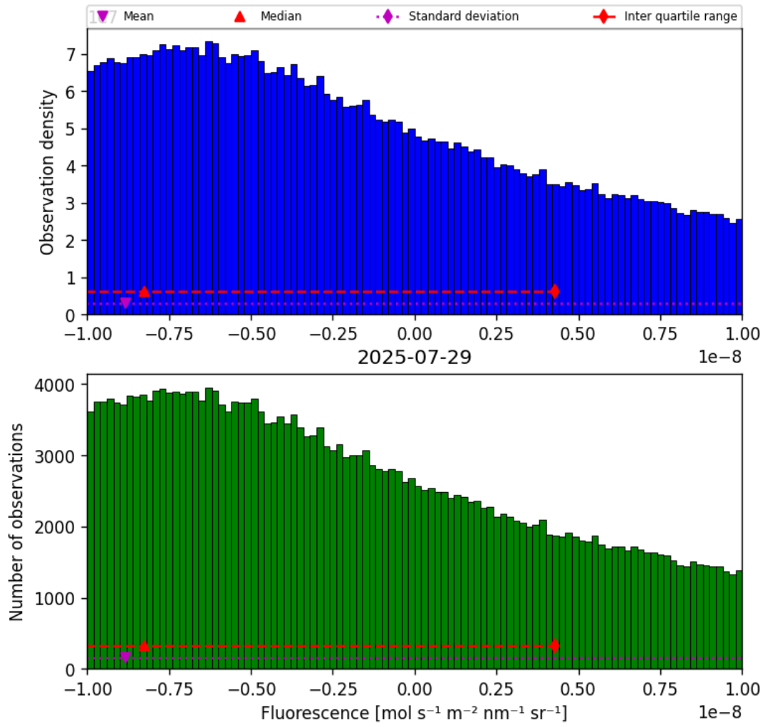
Figure 32: Histogram of “Fluorescence” for 2025-07-29 to 2025-07-30
