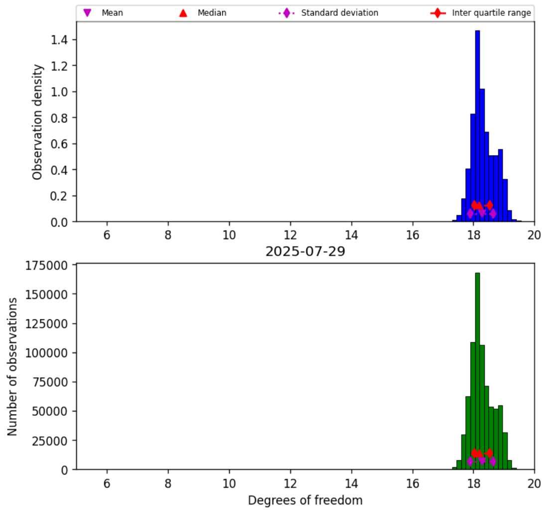
Figure 30: Histogram of “Degrees of freedom” for 2025-07-29 to 2025-07-30
