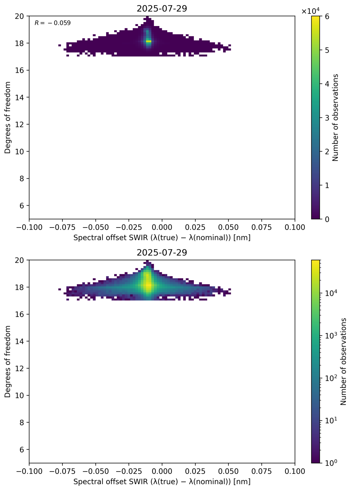
Figure 119: Scatter density plot of “Spectral offset SWIR ( \lambda_{\text{true}} - \lambda_{\text{nominal}} )” against “Degrees of freedom” for 2025-07-29 to 2025-07-30.
