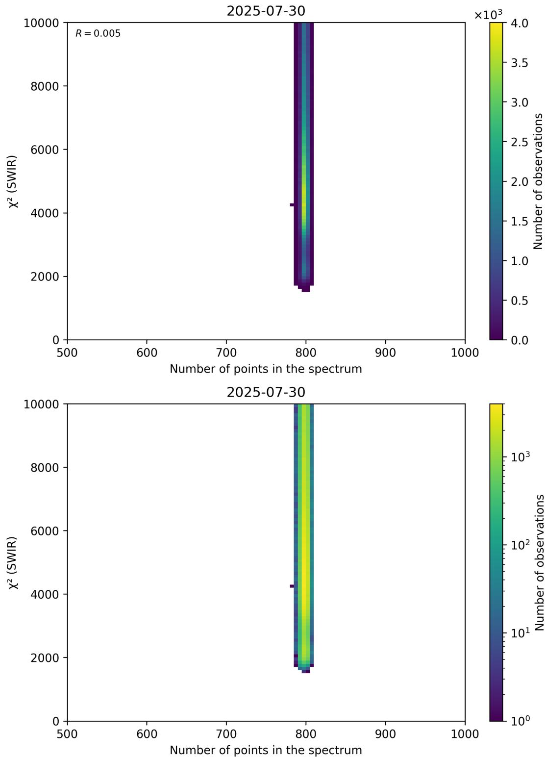
Figure 89: Scatter density plot of “Number of points in the spectrum” against “ \chi^2 (SWIR)” for 2025-07-29 to 2025-07-31.
