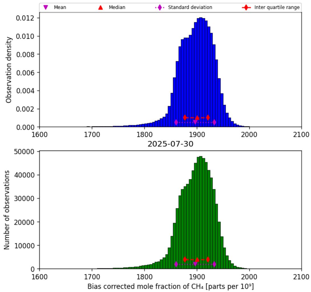
Figure 25: Histogram of “Bias corrected mole fraction of CH 4 ” for 2025-07-29 to 2025-07-31
