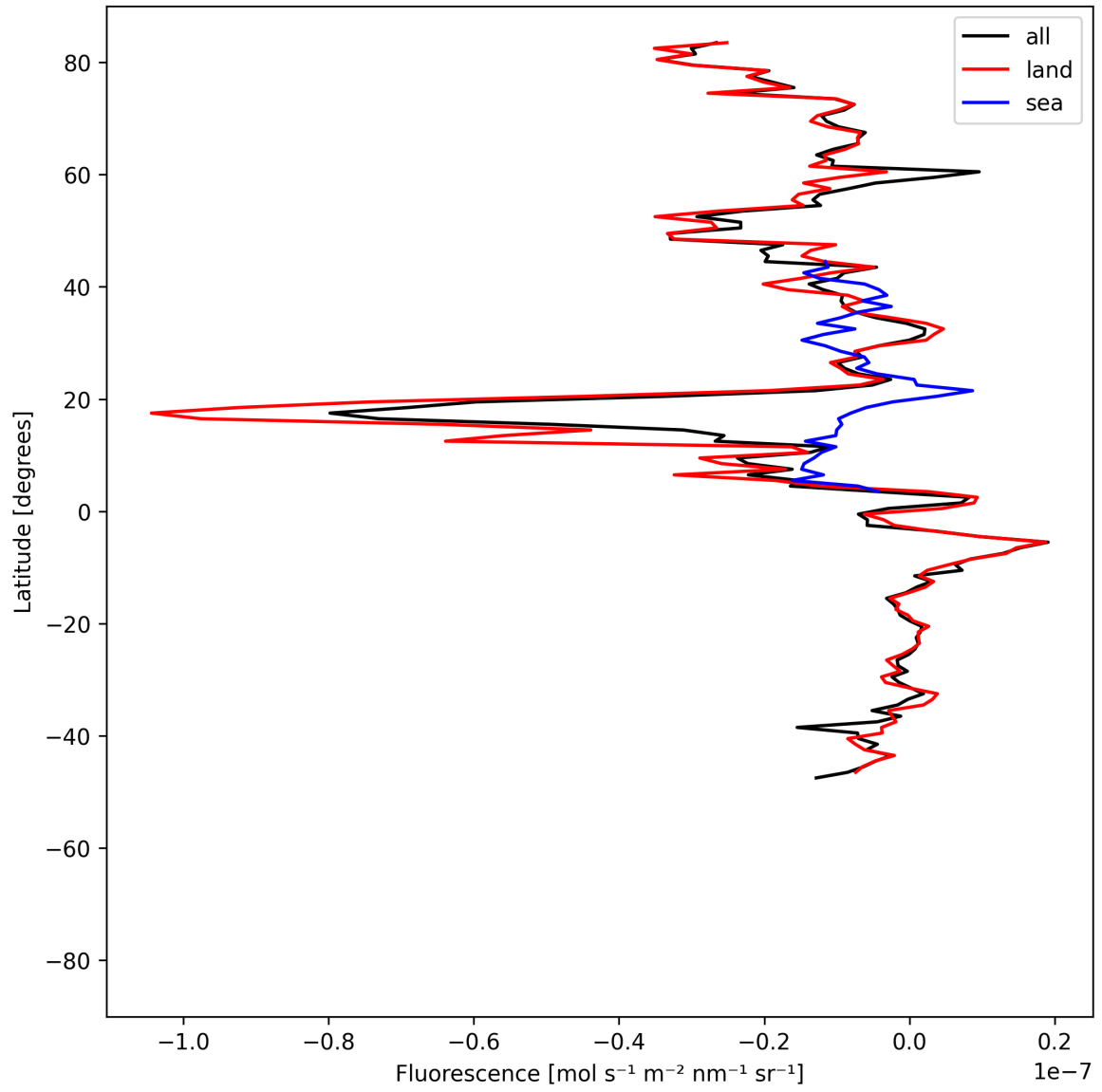
Figure 21: Zonal average of “Fluorescence” for 2025-07-29 to 2025-07-31.
