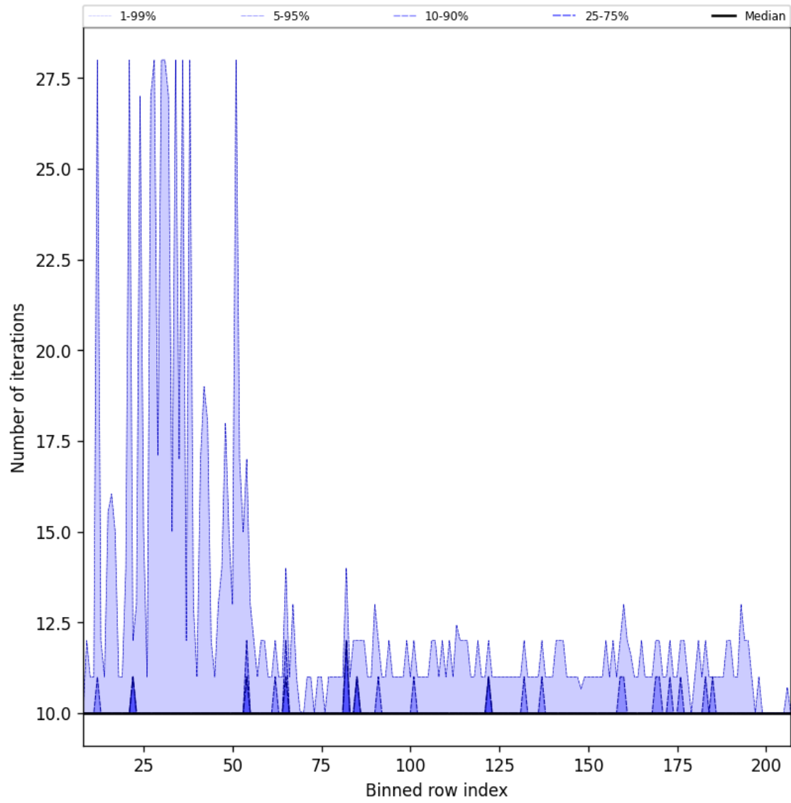
Figure 42: Along track statistics of “Number of iterations” for 2025-07-29 to 2025-07-31
