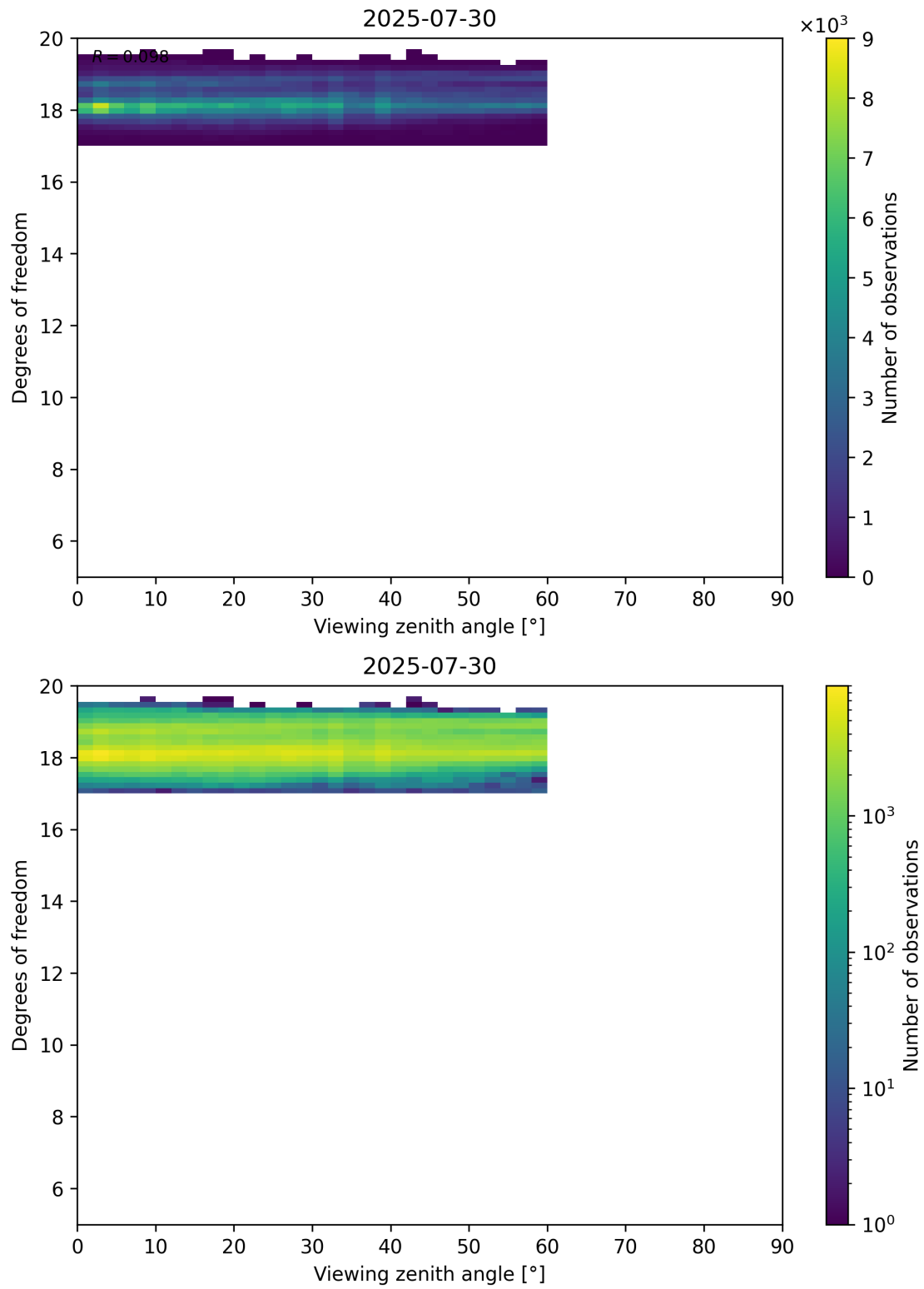
Figure 107: Scatter density plot of “Viewing zenith angle” against “Degrees of freedom” for 2025-07-29 to 2025-07-31.
