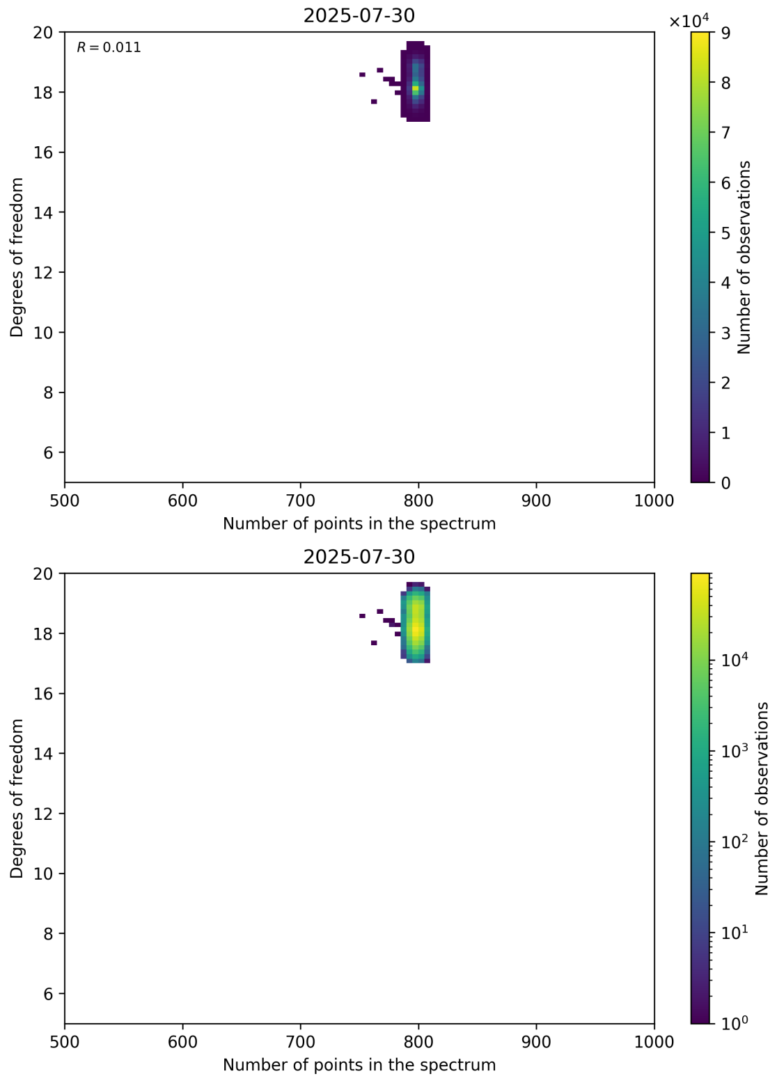
Figure 90: Scatter density plot of “Number of points in the spectrum” against “Degrees of freedom” for 2025-07-29 to 2025-07-31.
