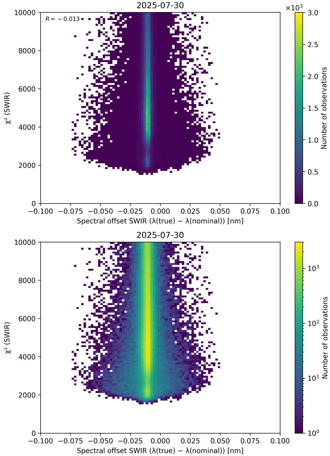
Figure 118: Scatter density plot of “Spectral offset SWIR ( \lambda_{\text{true}} - \lambda_{\text{nominal}} )” against “ \chi^2 (SWIR)” for 2025-07-29 to 2025-07-31.
