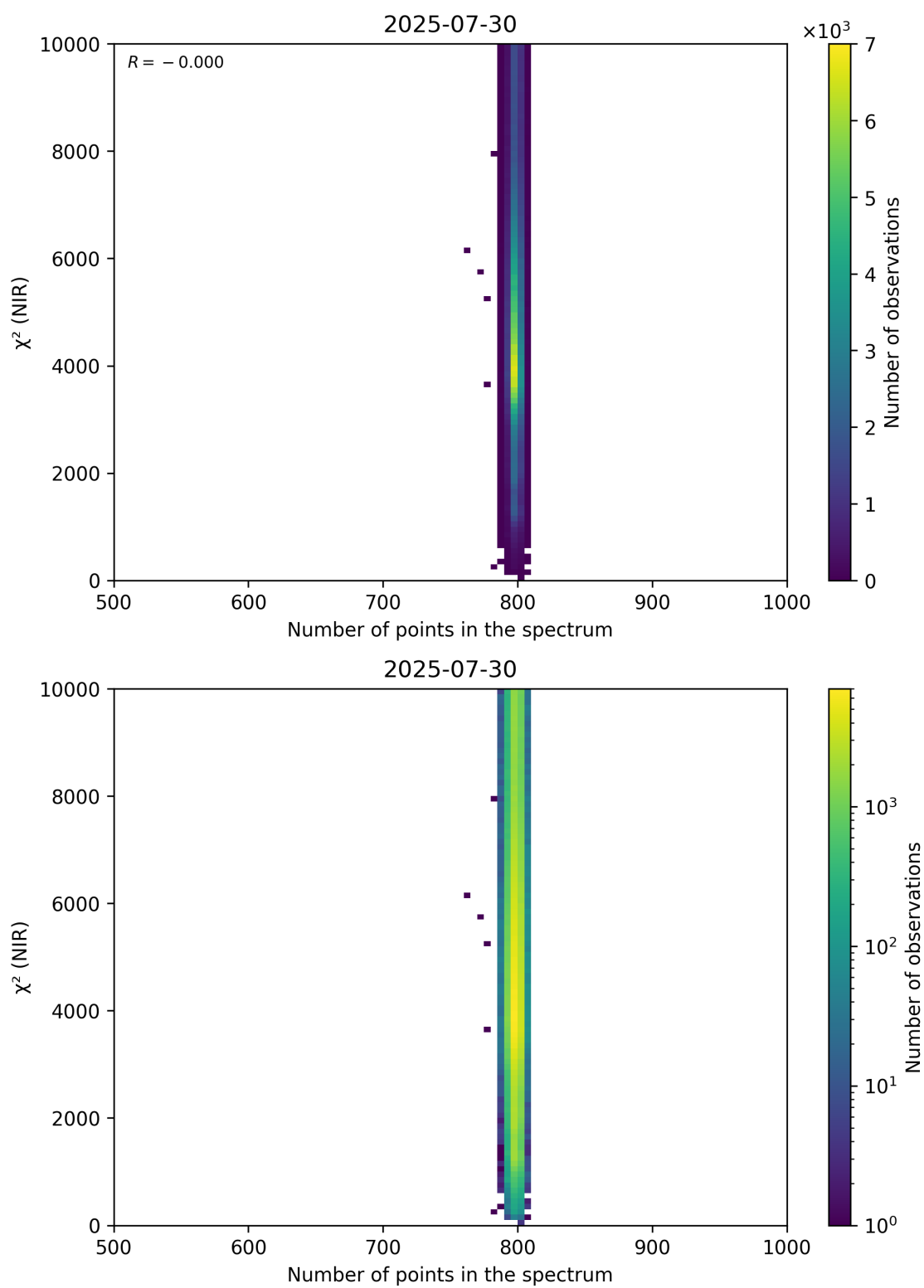
Figure 88: Scatter density plot of “Number of points in the spectrum” against “ \chi^2 (NIR)” for 2025-07-29 to 2025-07-31.
