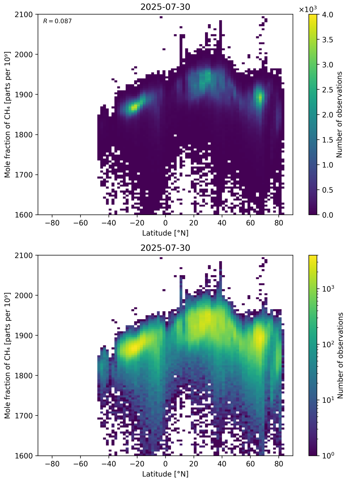
Figure 57: Scatter density plot of “Latitude” against “Mole fraction of CH 4 ” for 2025-07-29 to 2025-07-31.
