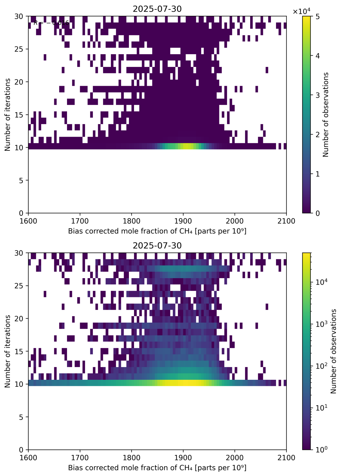
Figure 67: Scatter density plot of “Bias corrected mole fraction of CH 4 ” against “Number of iterations” for 2025-07-29 to 2025-07-31.
