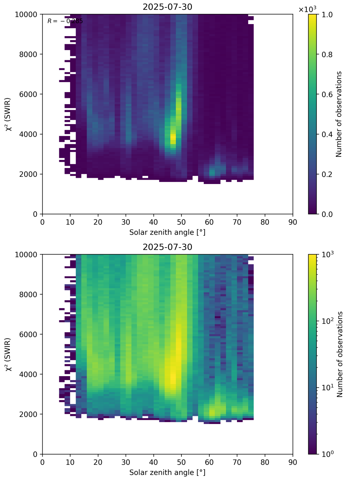
Figure 95: Scatter density plot of “Solar zenith angle” against “ \chi^2 (SWIR)” for 2025-07-29 to 2025-07-31.
