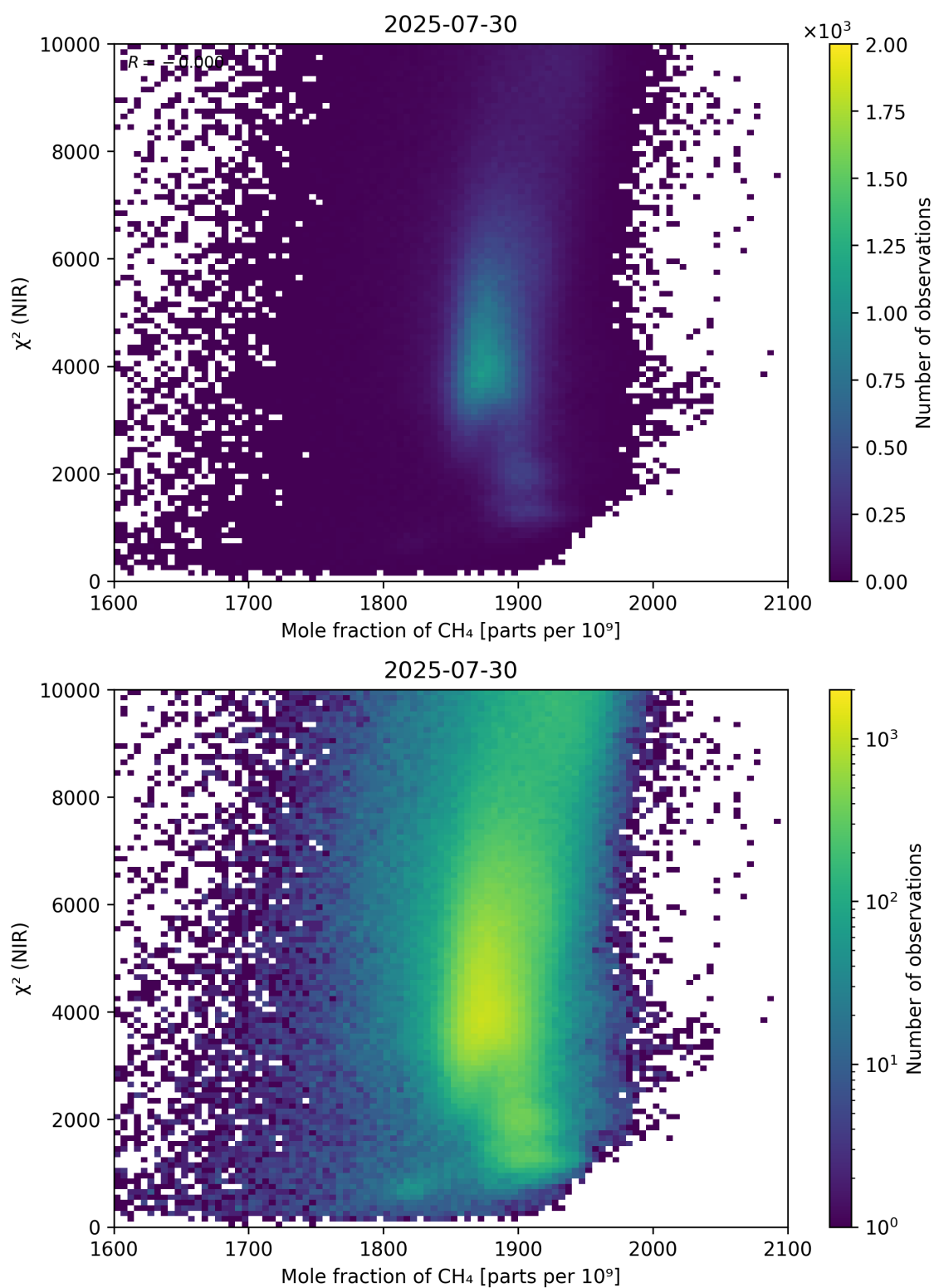
Figure 70: Scatter density plot of “Mole fraction of \text{CH}_4 ” against “ \chi^2 (NIR)” for 2025-07-29 to 2025-07-31.
