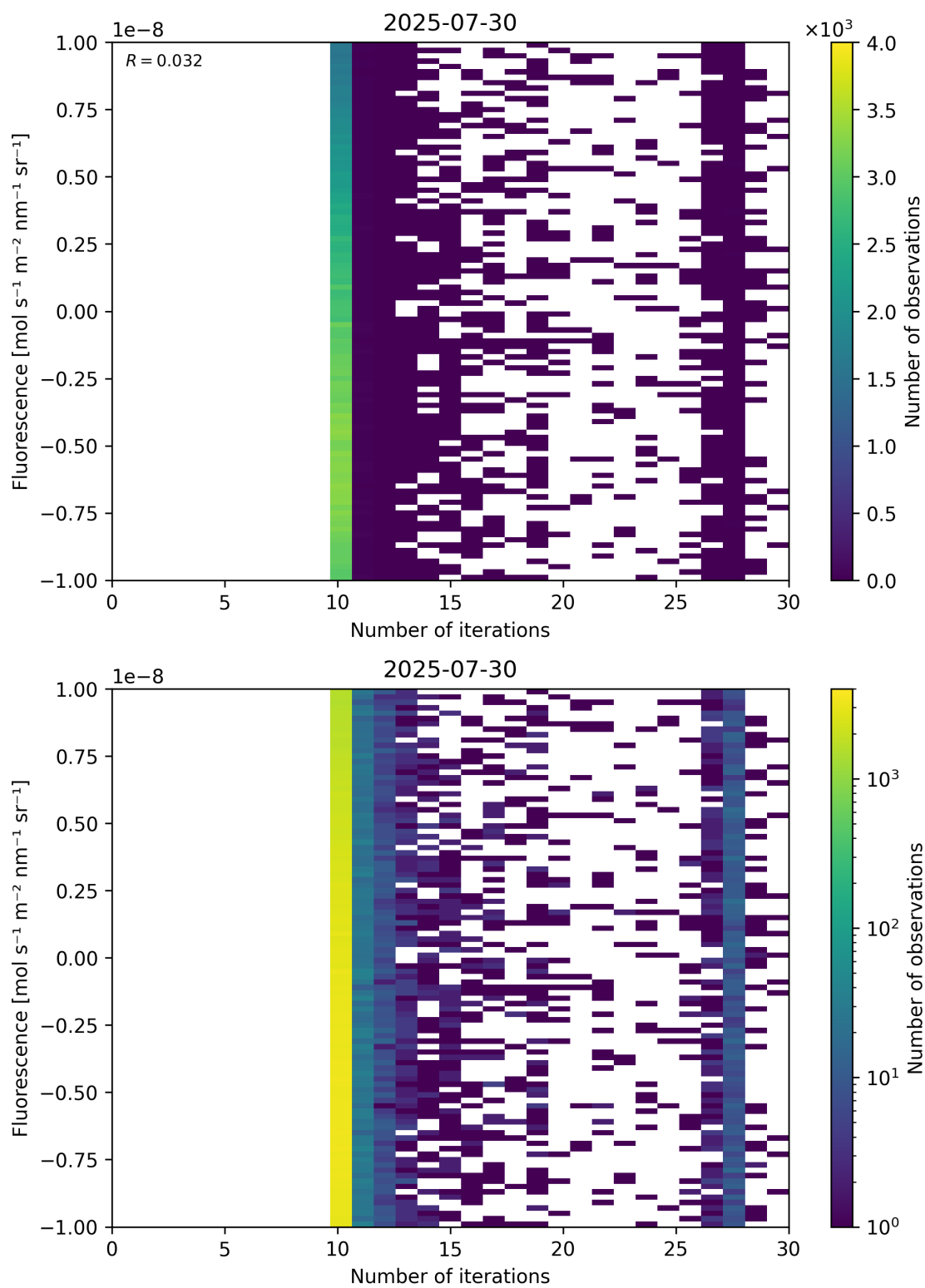
Figure 87: Scatter density plot of “Number of iterations” against “Fluorescence” for 2025-07-29 to 2025-07-31.
