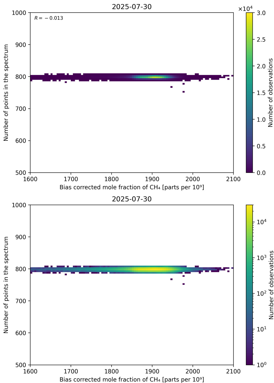
Figure 68: Scatter density plot of “Bias corrected mole fraction of CH 4 ” against “Number of points in the spectrum” for 2025-07-29 to 2025-07-31.
