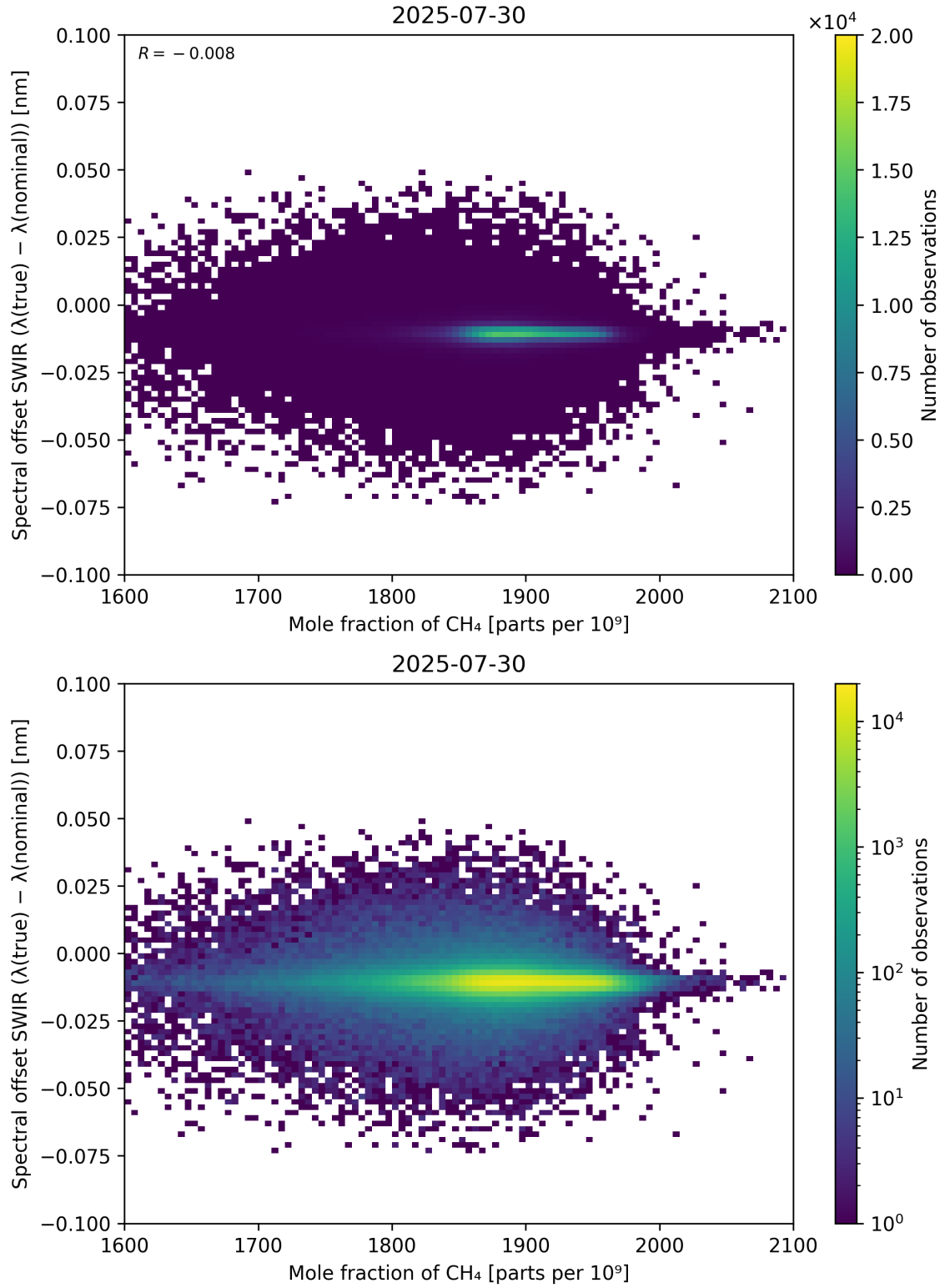
Figure 86: Scatter density plot of “Mole fraction of CH 4 ” against “Spectral offset SWIR ( \lambda_{\text{true}} - \lambda_{\text{nominal}} )” for 2025-07-29 to 2025-07-31.
