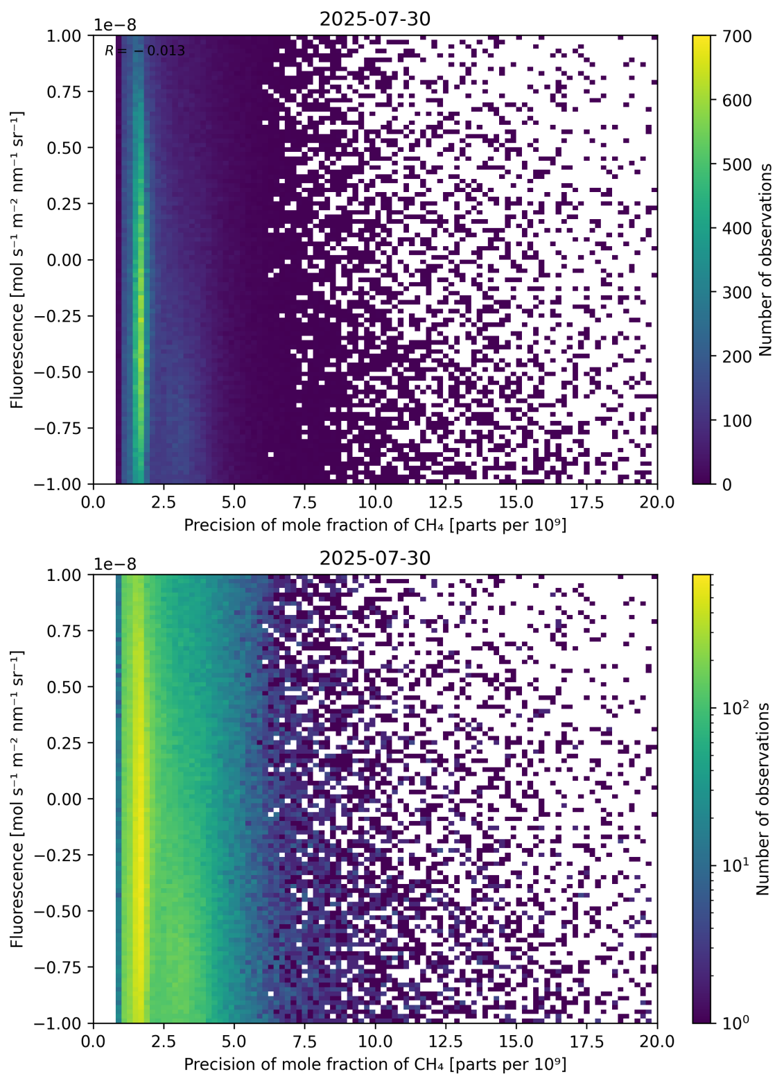
Figure 81: Scatter density plot of “Precision of mole fraction of \text{CH}_4 ” against “Fluorescence” for 2025-07-29 to 2025-07-31.
