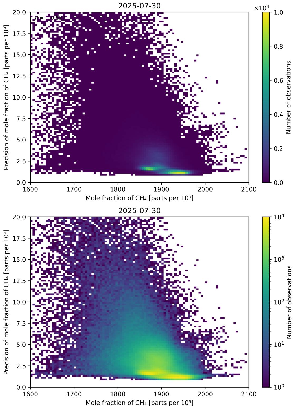
Figure 75: Scatter density plot of “Mole fraction of CH 4 ” against “Precision of mole fraction of CH 4 ” for 2025-07-29 to 2025-07-31.
