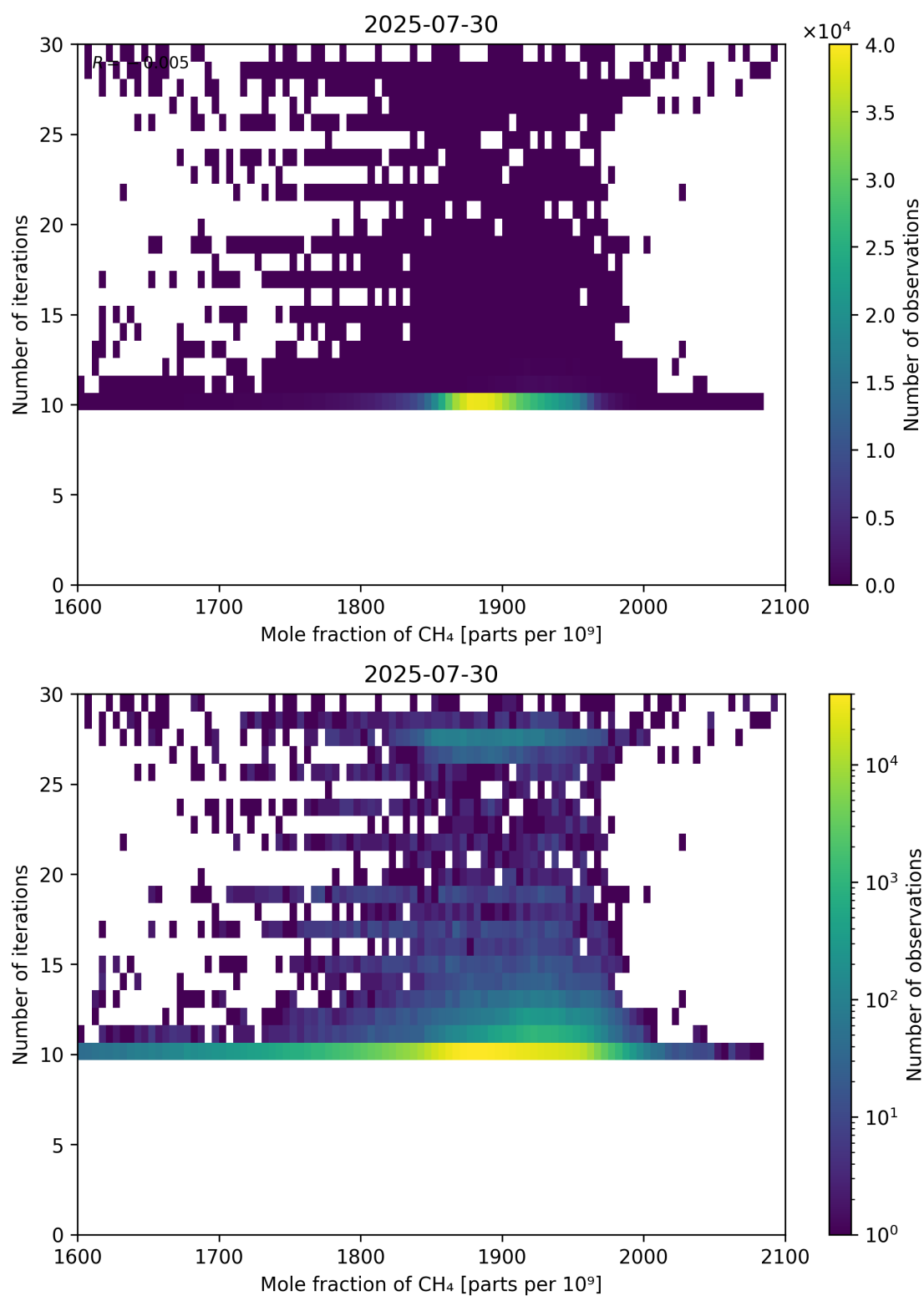
Figure 76: Scatter density plot of “Mole fraction of CH 4 ” against “Number of iterations” for 2025-07-29 to 2025-07-31.
