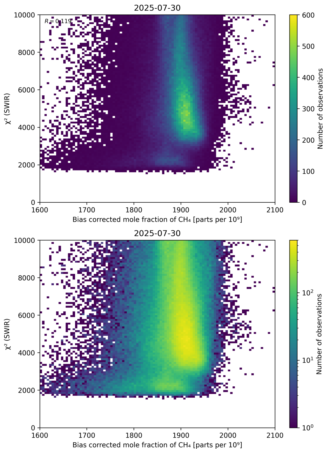
Figure 64: Scatter density plot of “Bias corrected mole fraction of \text{CH}_4 ” against “ \chi^2 (SWIR)” for 2025-07-29 to 2025-07-31.
