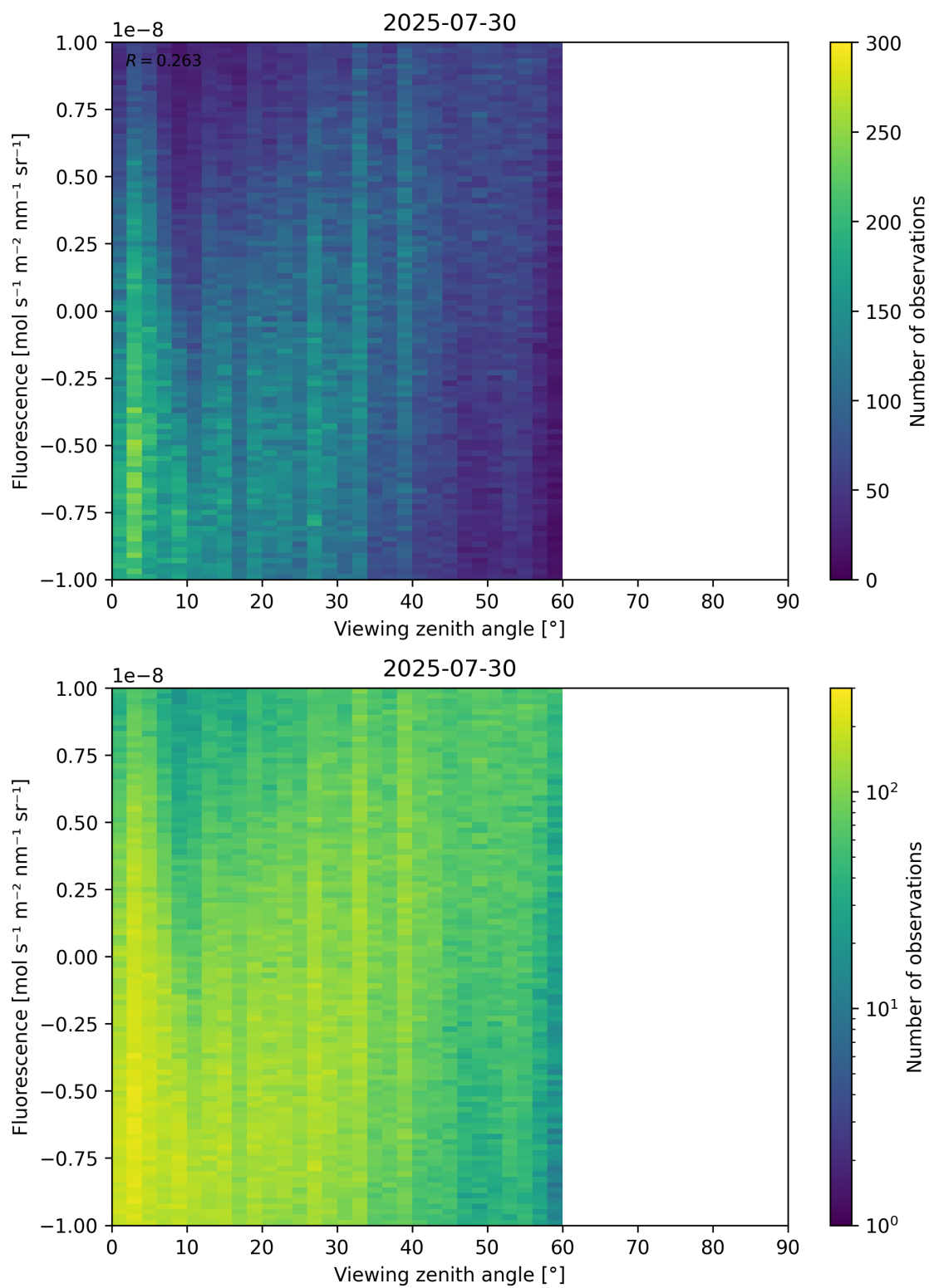
Figure 108: Scatter density plot of “Viewing zenith angle” against “Fluorescence” for 2025-07-29 to 2025-07-31.
