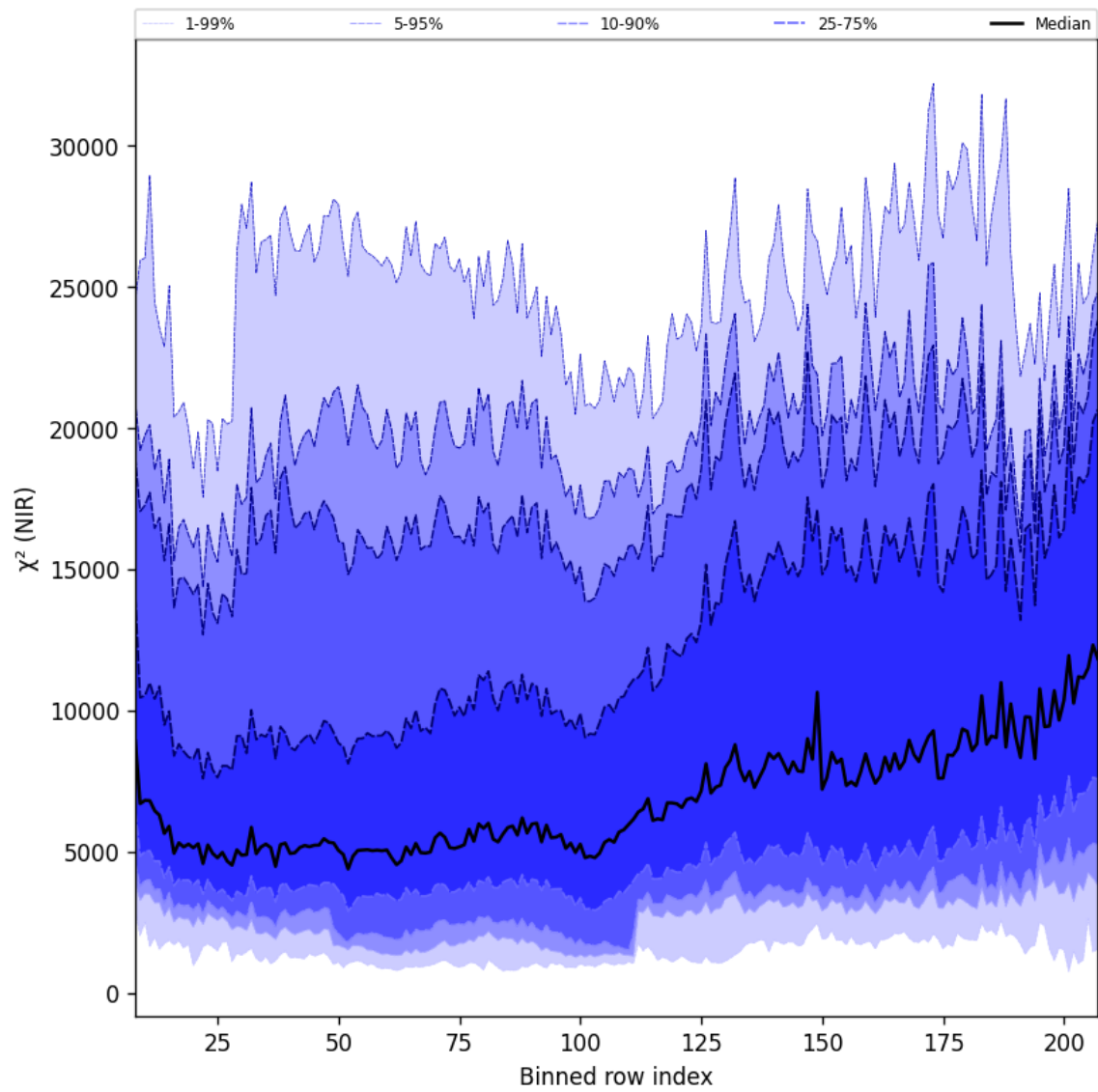
Figure 40: Along track statistics of “ \chi^2 (NIR)” for 2025-07-29 to 2025-07-31
