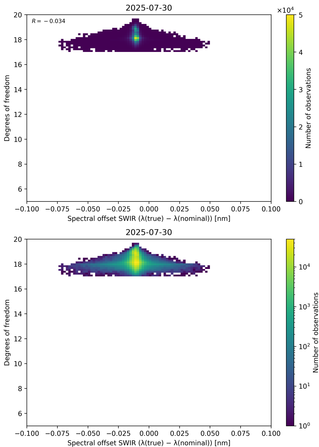
Figure 119: Scatter density plot of “Spectral offset SWIR ( \lambda_{\text{true}} - \lambda_{\text{nominal}} )” against “Degrees of freedom” for 2025-07-29 to 2025-07-31.
