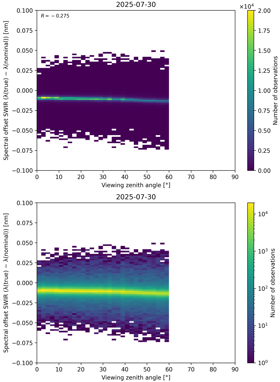
Figure 116: Scatter density plot of “Viewing zenith angle” against “Spectral offset SWIR ( \lambda_{\text{true}} - \lambda_{\text{nominal}} )” for 2025-07-29 to 2025-07-31.
