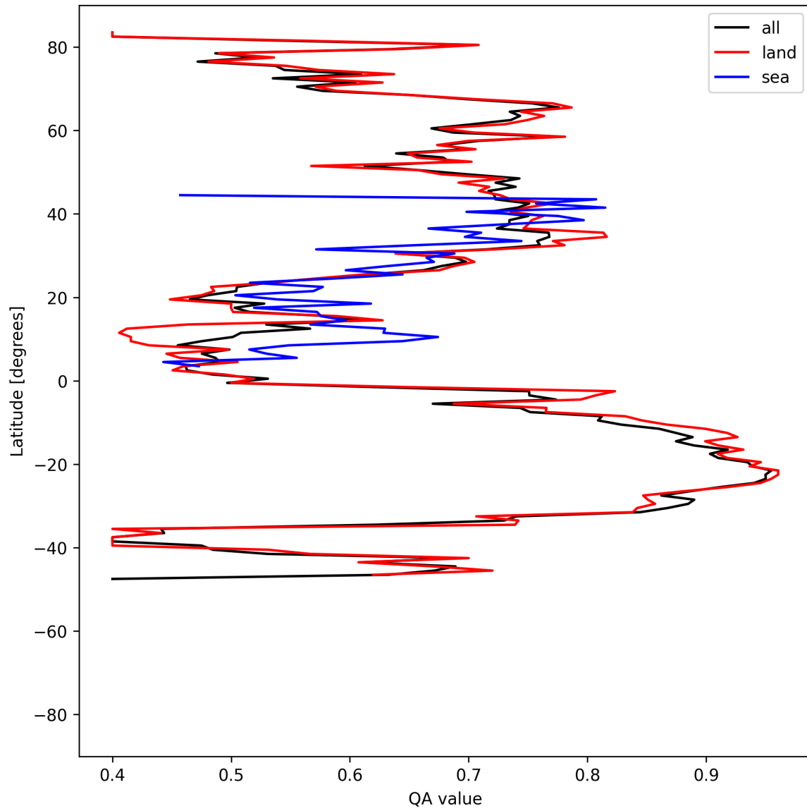
Figure 11: Zonal average of “QA value” for 2025-07-29 to 2025-07-31.
