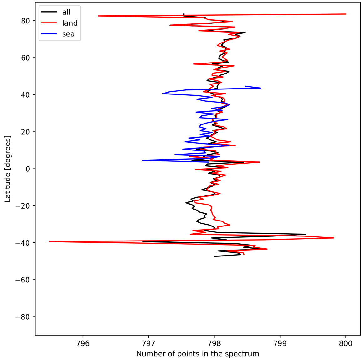
Figure 15: Zonal average of “Number of points in the spectrum” for 2025-07-29 to 2025-07-31.
