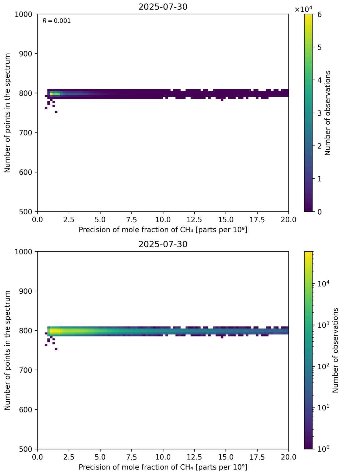
Figure 84: Scatter density plot of “Precision of mole fraction of CH 4 ” against “Number of points in the spectrum” for 2025-07-29 to 2025-07-31.
