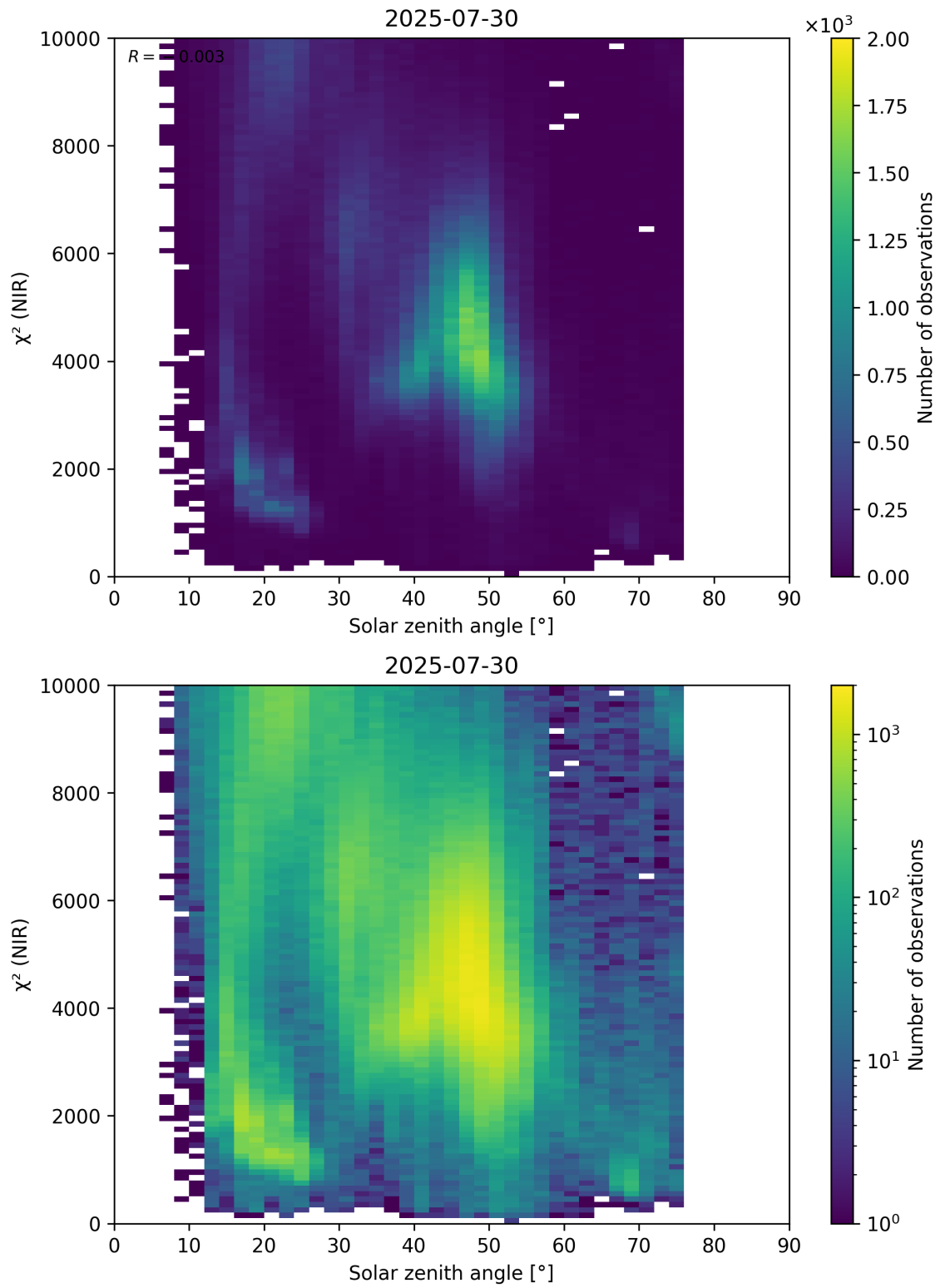
Figure 94: Scatter density plot of “Solar zenith angle” against “ \chi^2 (NIR)” for 2025-07-29 to 2025-07-31.
