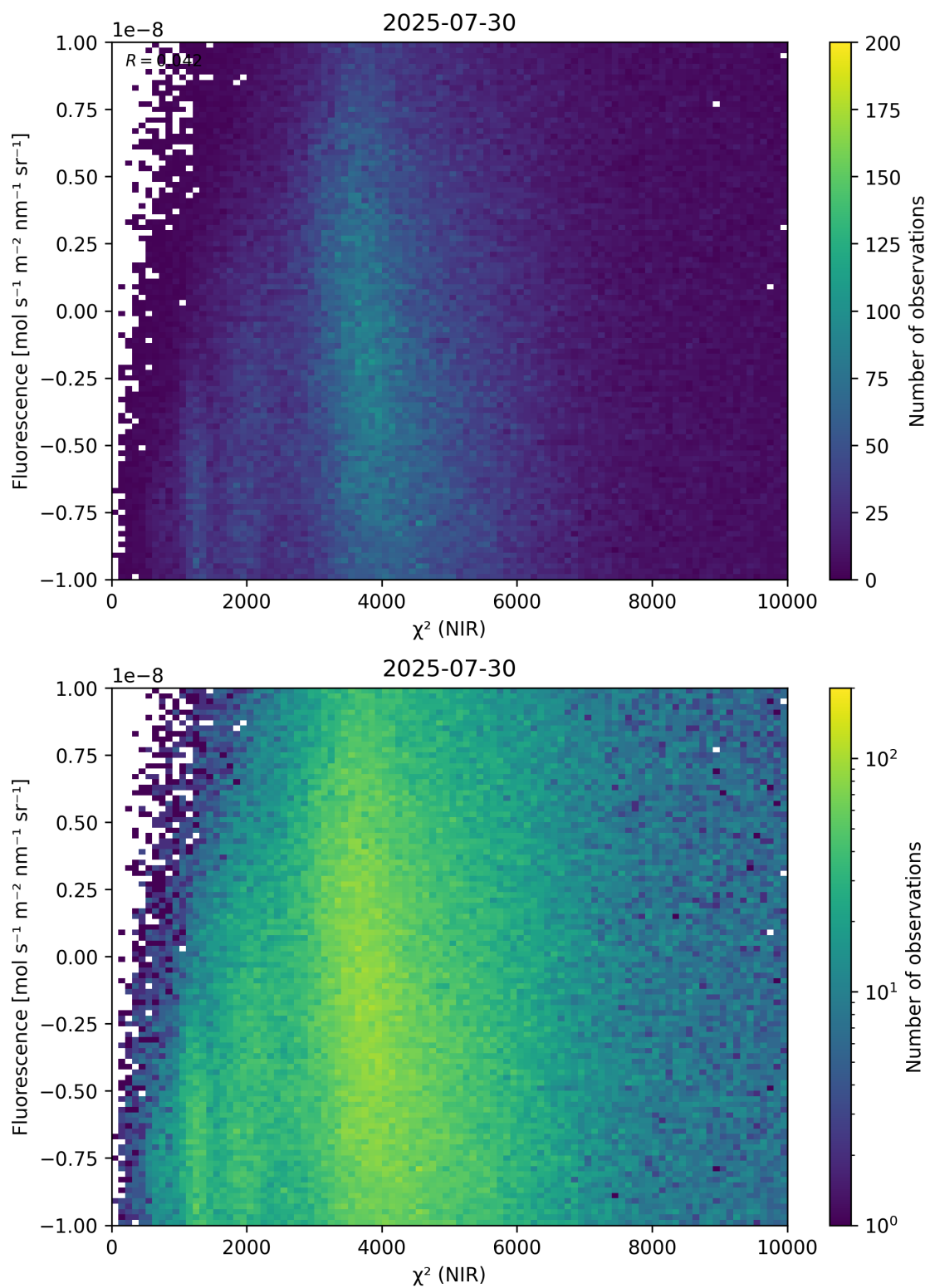
Figure 45: Scatter density plot of “ \chi^2 (NIR)” against “Fluorescence” for 2025-07-29 to 2025-07-31.
