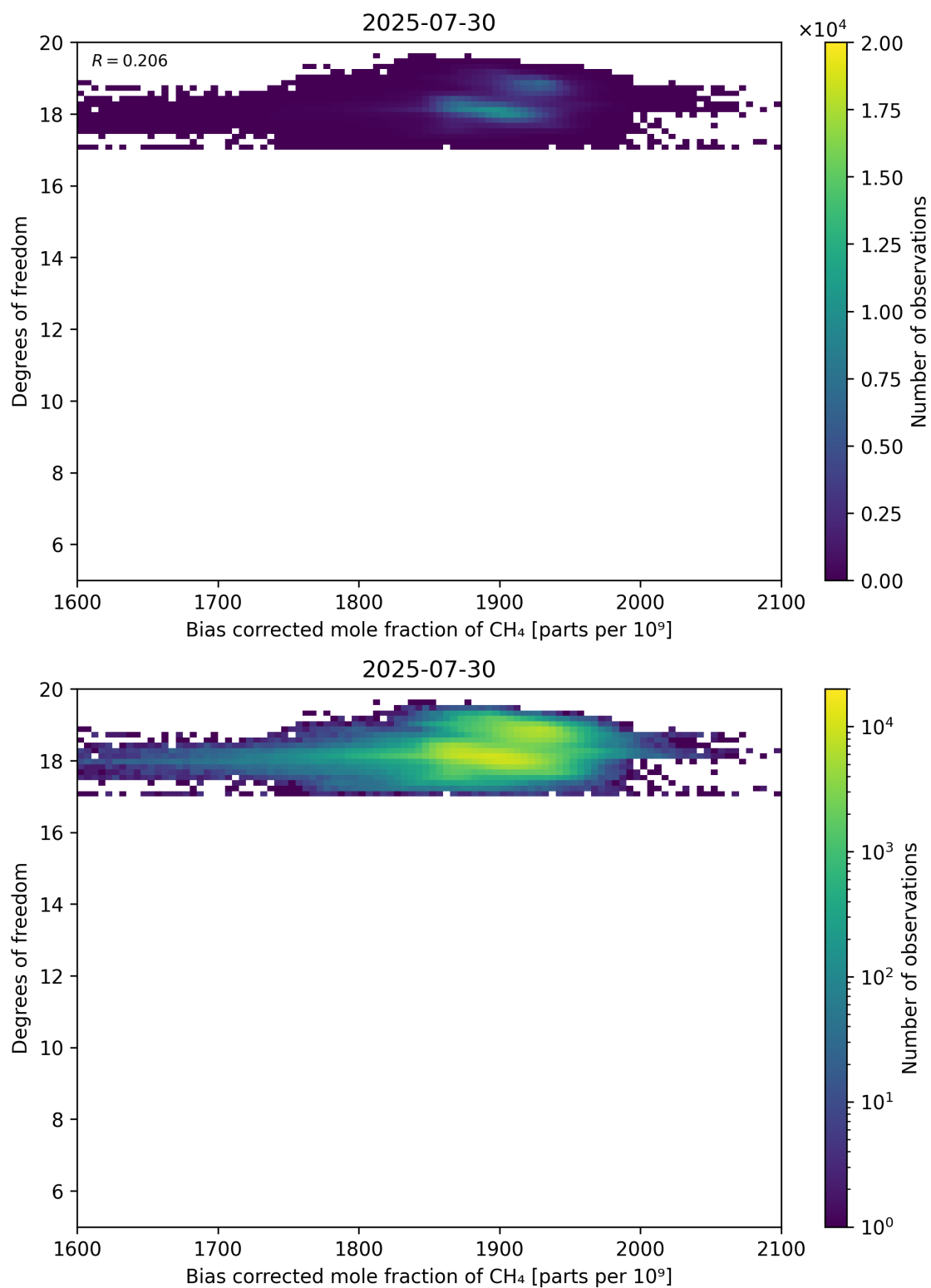
Figure 65: Scatter density plot of “Bias corrected mole fraction of CH 4 ” against “Degrees of freedom” for 2025-07-29 to 2025-07-31.
