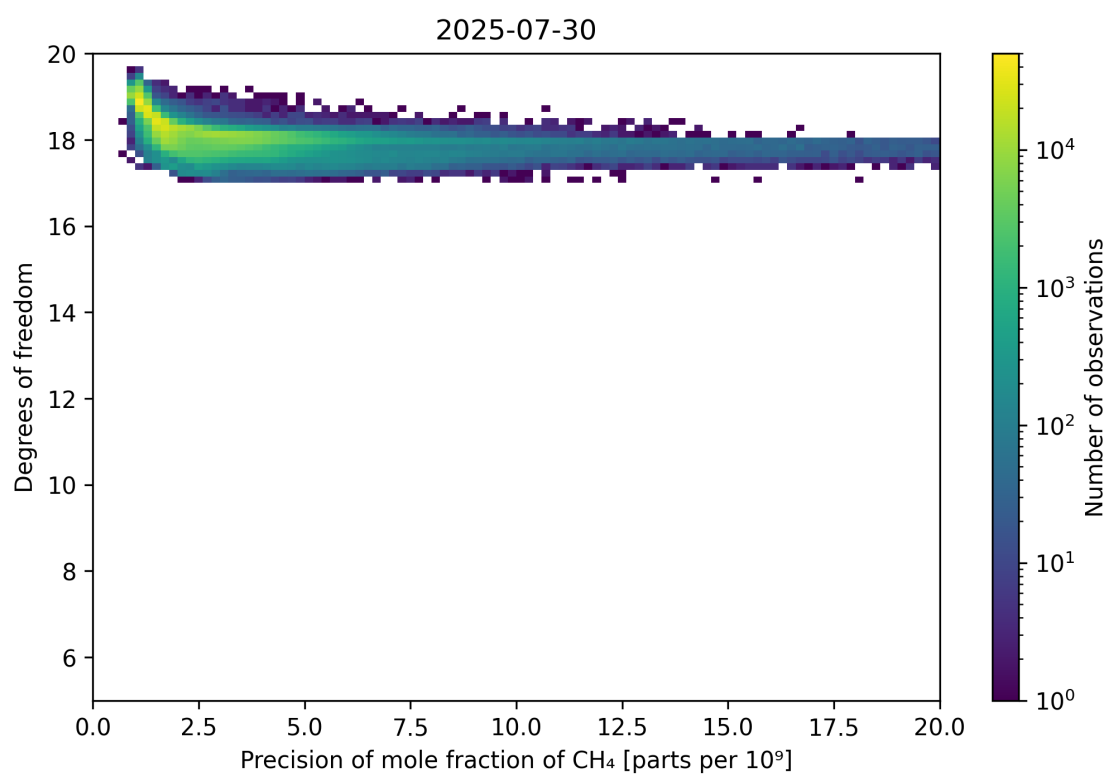
Figure 80: Scatter density plot of “Precision of mole fraction of CH 4 ” against “Degrees of freedom” for 2025-07-29 to 2025-07-31.
