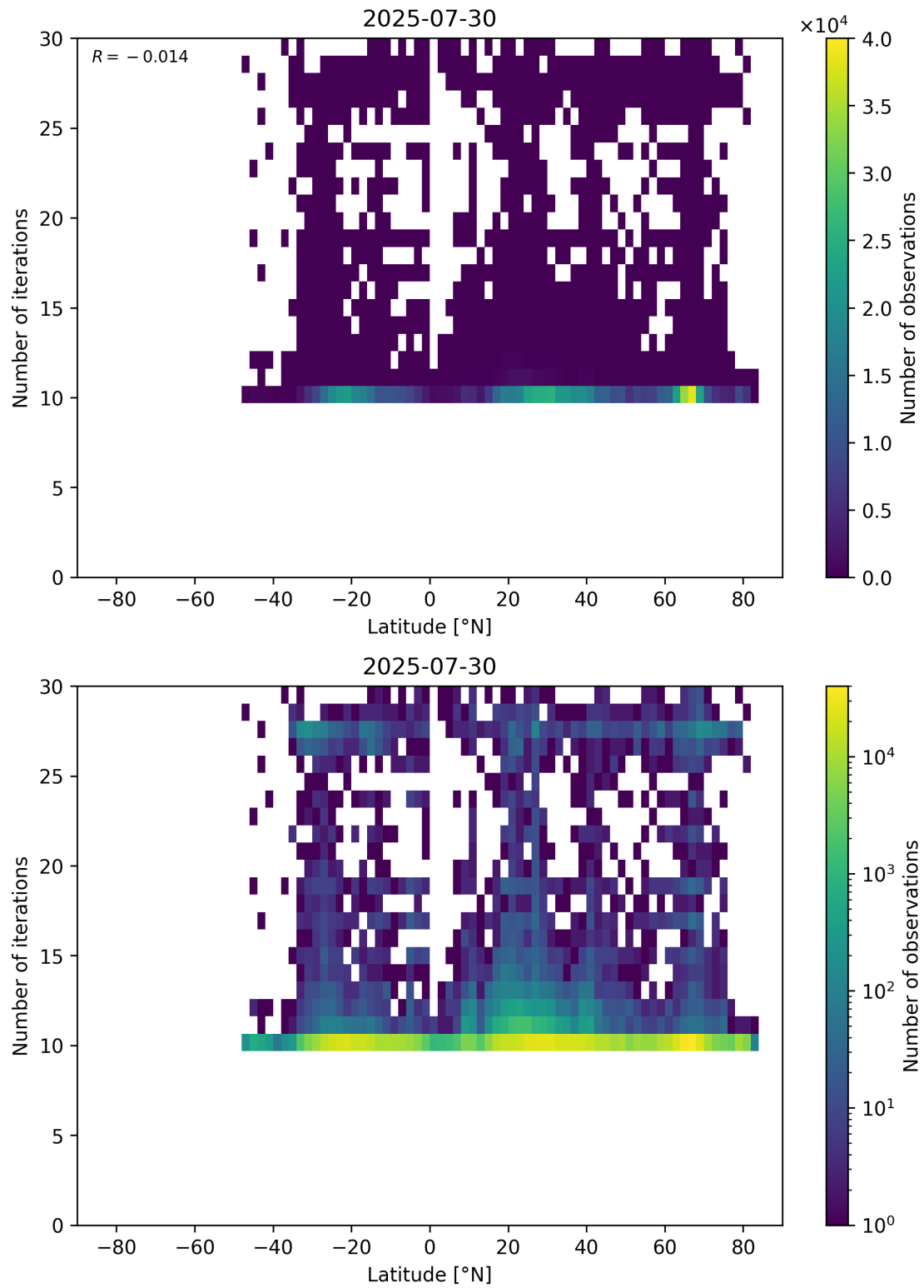
Figure 60: Scatter density plot of “Latitude” against “Number of iterations” for 2025-07-29 to 2025-07-31.
