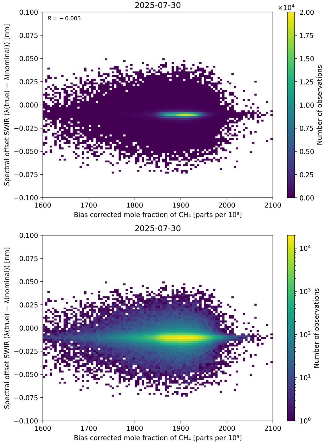
Figure 69: Scatter density plot of “Bias corrected mole fraction of CH 4 ” against “Spectral offset SWIR ( \lambda_{\text{true}} - \lambda_{\text{nominal}} )” for 2025-07-29 to 2025-07-31.
