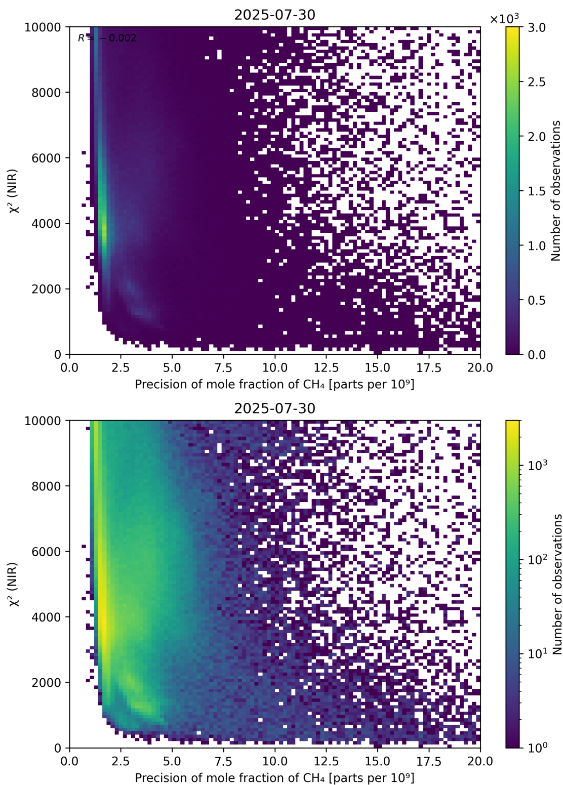
Figure 78: Scatter density plot of “Precision of mole fraction of \text{CH}_4 ” against “ \chi^2 (NIR)” for 2025-07-29 to 2025-07-31.
