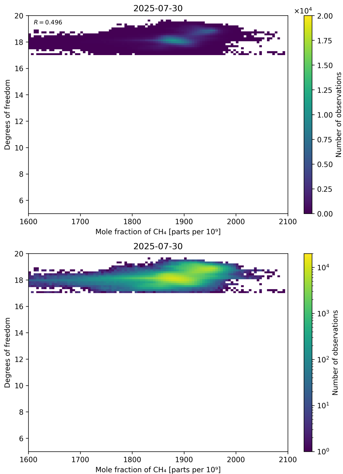
Figure 72: Scatter density plot of “Mole fraction of CH 4 ” against “Degrees of freedom” for 2025-07-29 to 2025-07-31.
