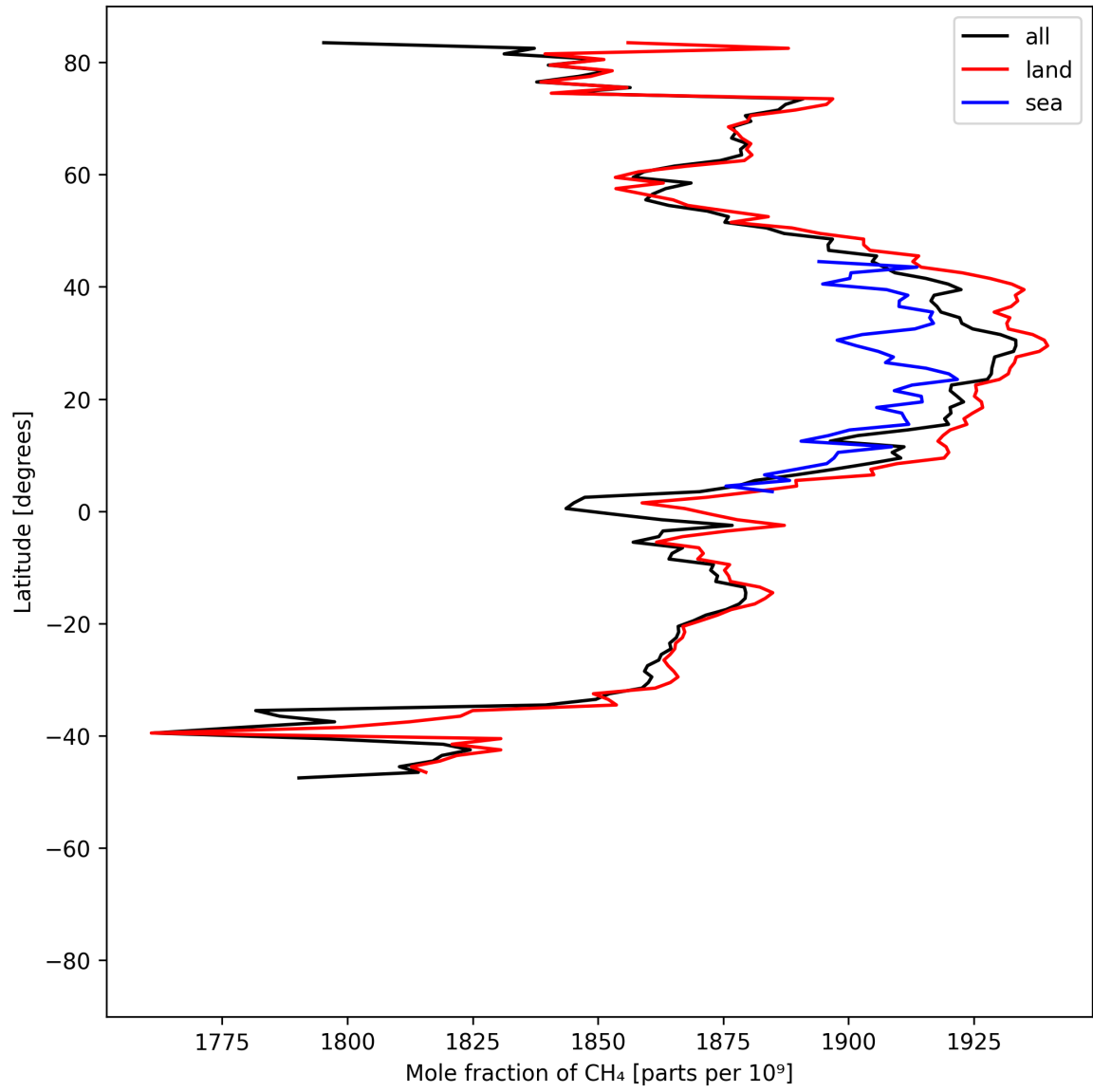
Figure 12: Zonal average of “Mole fraction of \text{CH}_4 ” for 2025-07-29 to 2025-07-31.
