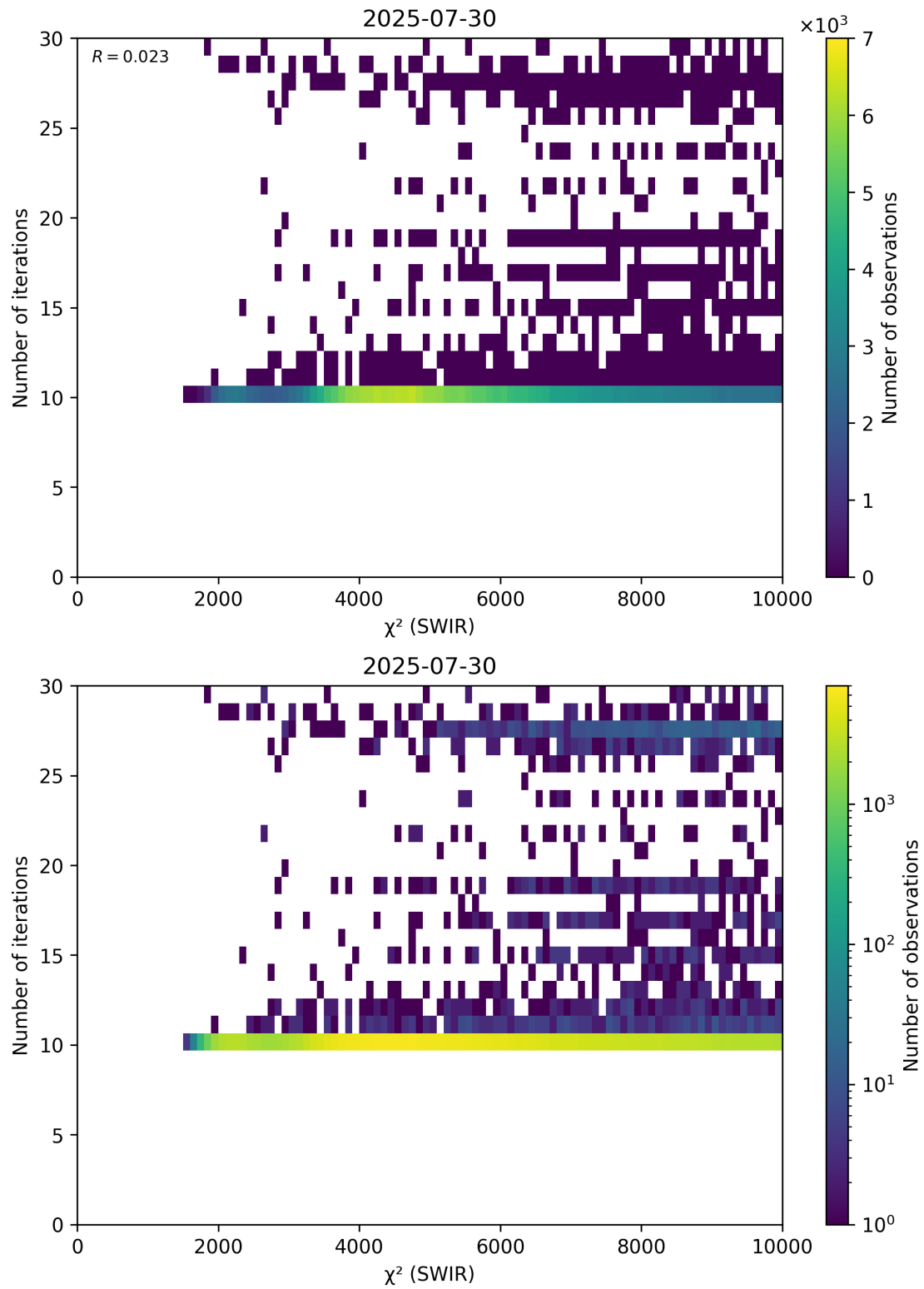
Figure 50: Scatter density plot of “ \chi^2 (SWIR)” against “Number of iterations” for 2025-07-29 to 2025-07-31.
