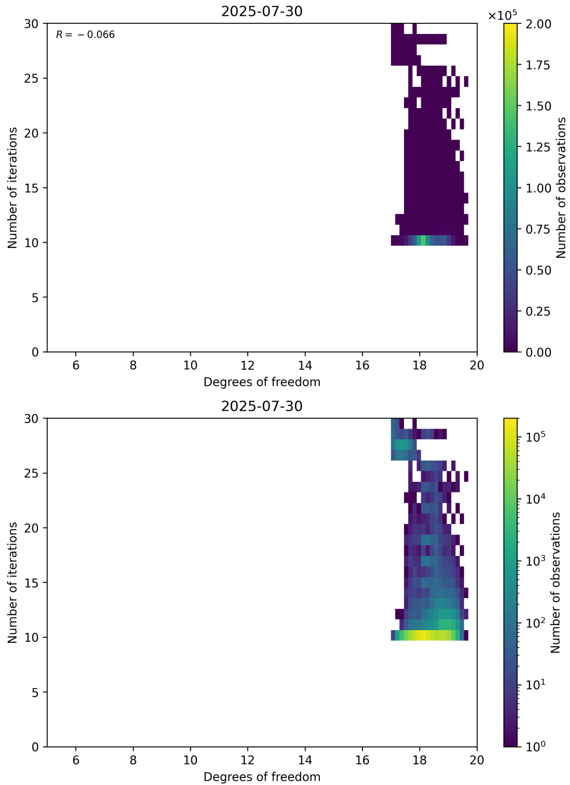
Figure 52: Scatter density plot of “Degrees of freedom” against “Number of iterations” for 2025-07-29 to 2025-07-31.
