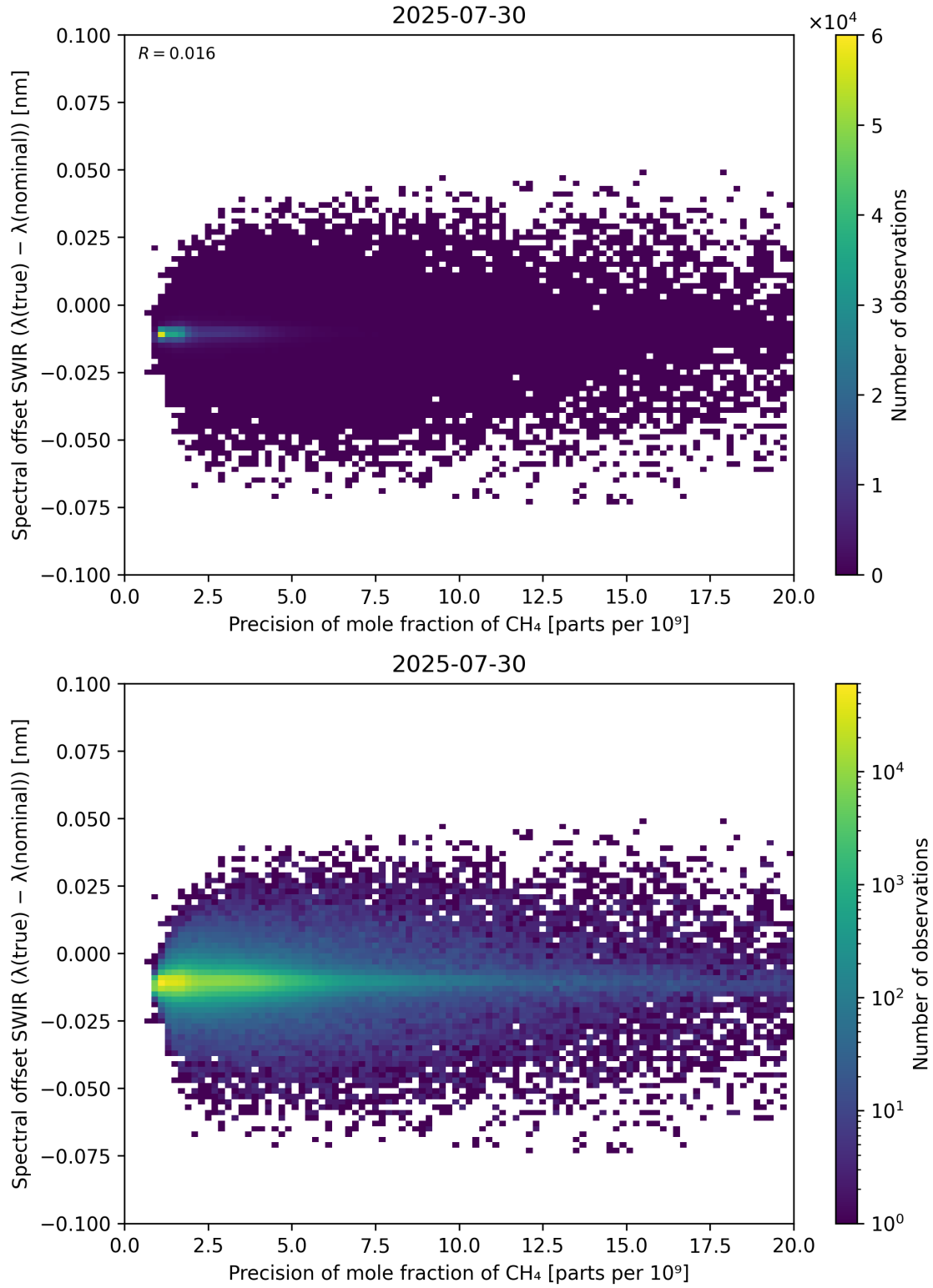
Figure 85: Scatter density plot of “Precision of mole fraction of \text{CH}_4 ” against “Spectral offset SWIR ( \lambda_{\text{true}} - \lambda_{\text{nominal}} )” for 2025-07-29 to 2025-07-31.
