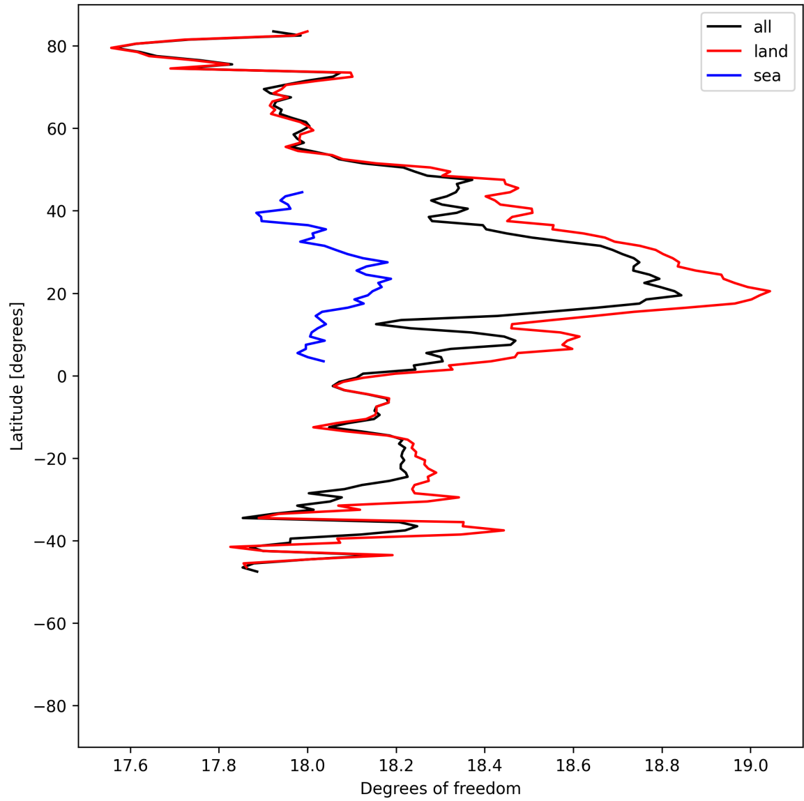
Figure 19: Zonal average of “Degrees of freedom” for 2025-07-29 to 2025-07-31.
