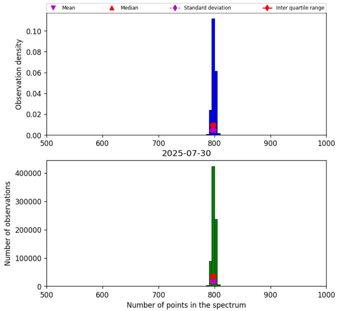
Figure 26: Histogram of “Number of points in the spectrum” for 2025-07-29 to 2025-07-31
