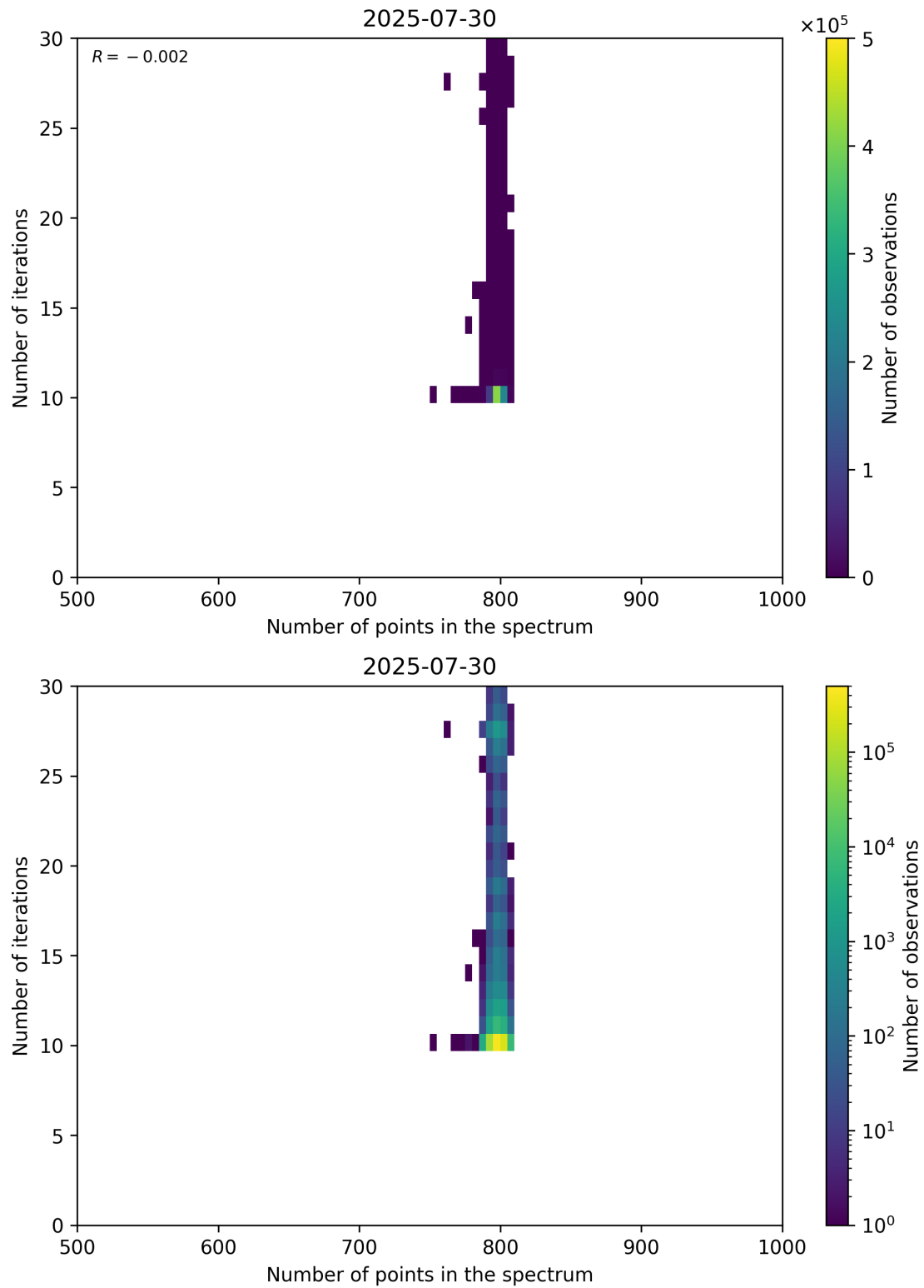
Figure 92: Scatter density plot of “Number of points in the spectrum” against “Number of iterations” for 2025-07-29 to 2025-07-31.
