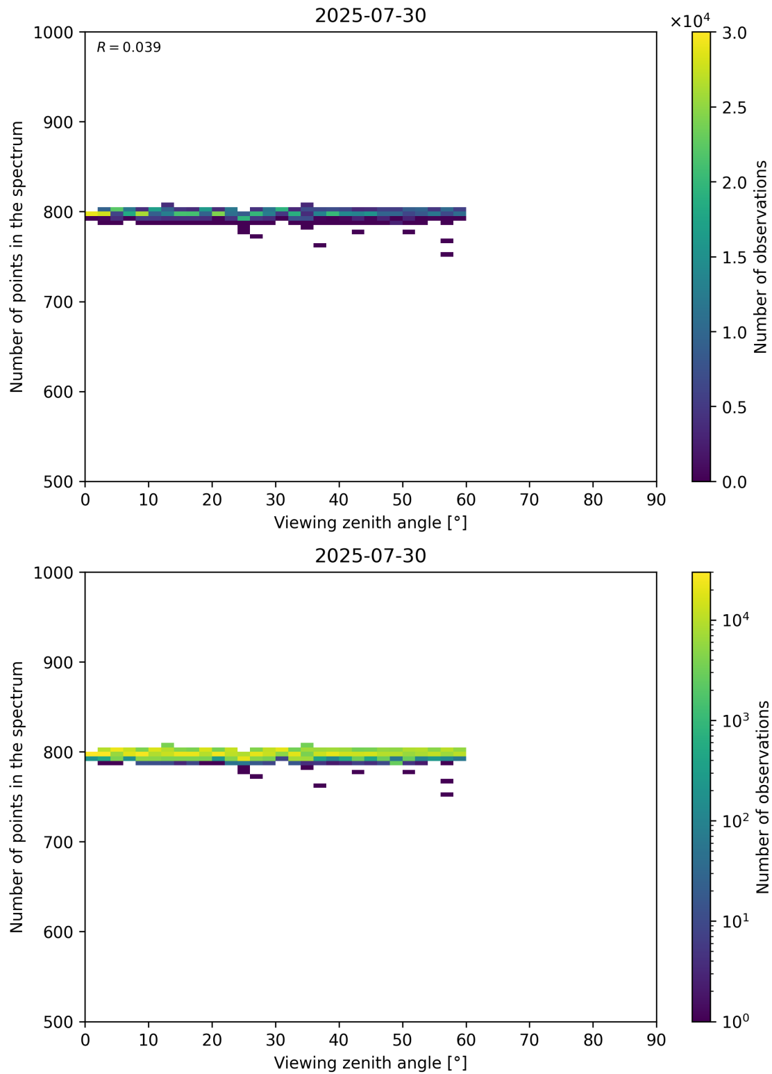
Figure 114: Scatter density plot of “Viewing zenith angle” against “Number of points in the spectrum” for 2025-07-29 to 2025-07-31.
