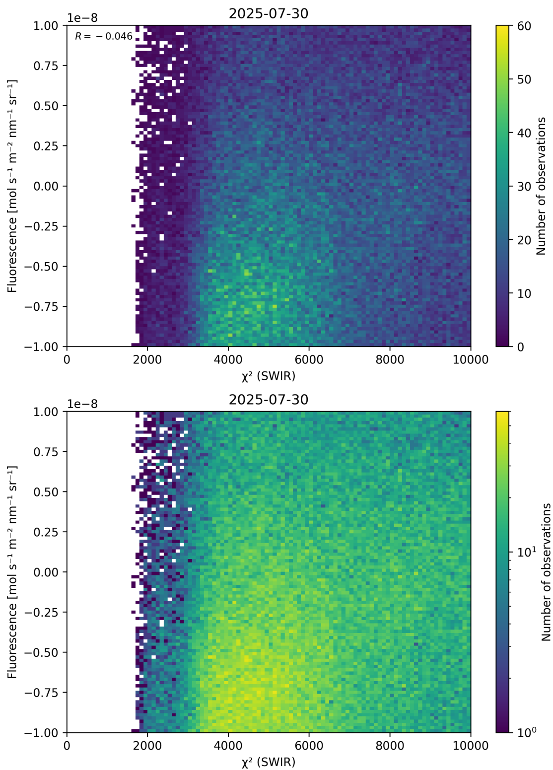
Figure 49: Scatter density plot of “ \chi^2 (SWIR)” against “Fluorescence” for 2025-07-29 to 2025-07-31.
