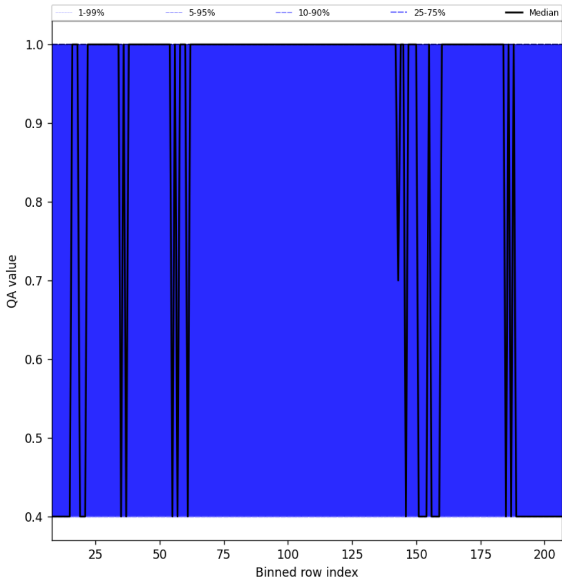
Figure 33: Along track statistics of “QA value” for 2025-07-29 to 2025-07-31
