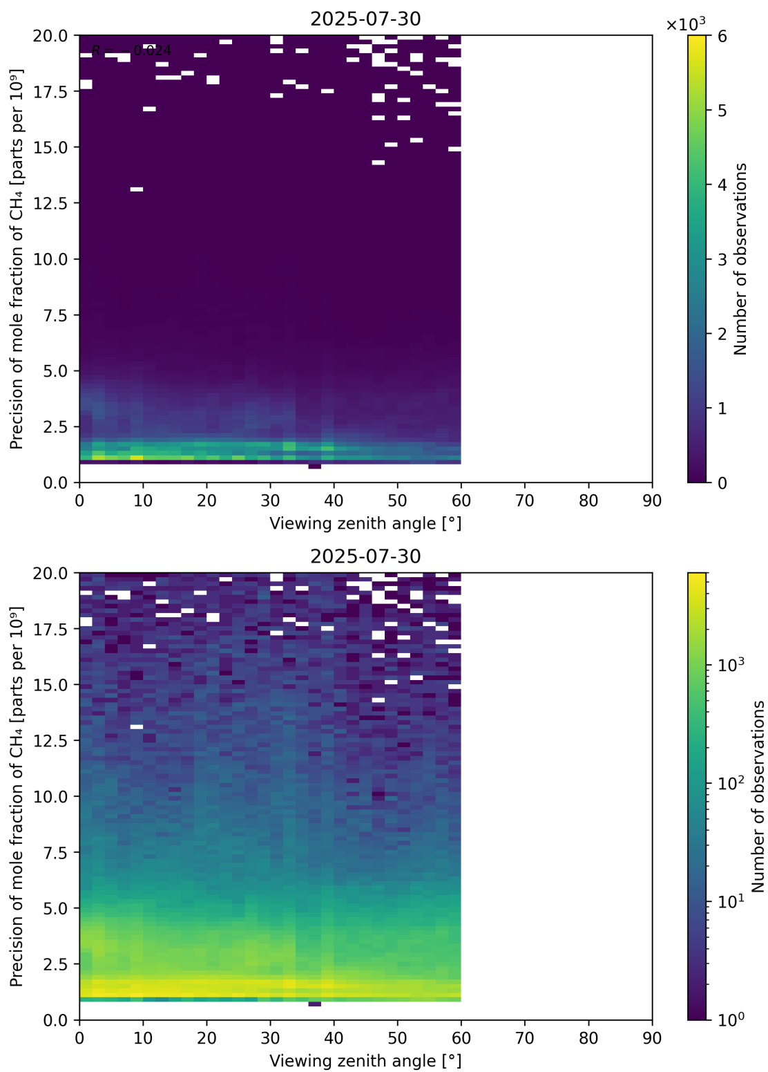
Figure 112: Scatter density plot of “Viewing zenith angle” against “Precision of mole fraction of CH 4 ” for 2025-07-29 to 2025-07-31.
