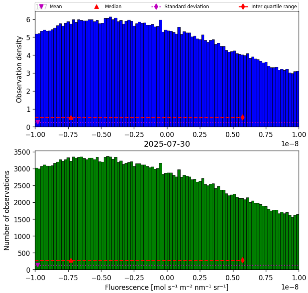
Figure 32: Histogram of “Fluorescence” for 2025-07-29 to 2025-07-31
