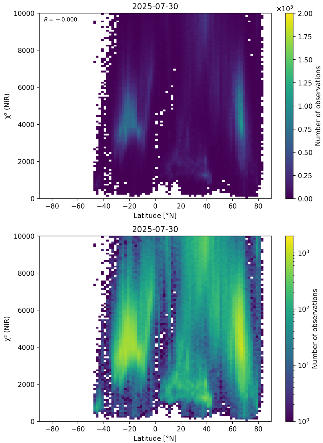
Figure 53: Scatter density plot of “Latitude” against “ \chi^2 (NIR)” for 2025-07-29 to 2025-07-31.
