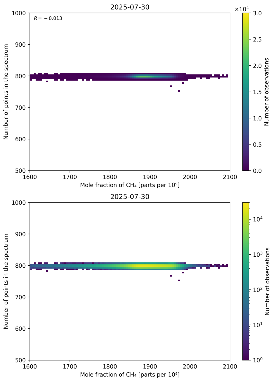
Figure 77: Scatter density plot of “Mole fraction of CH 4 ” against “Number of points in the spectrum” for 2025-07-29 to 2025-07-31.
