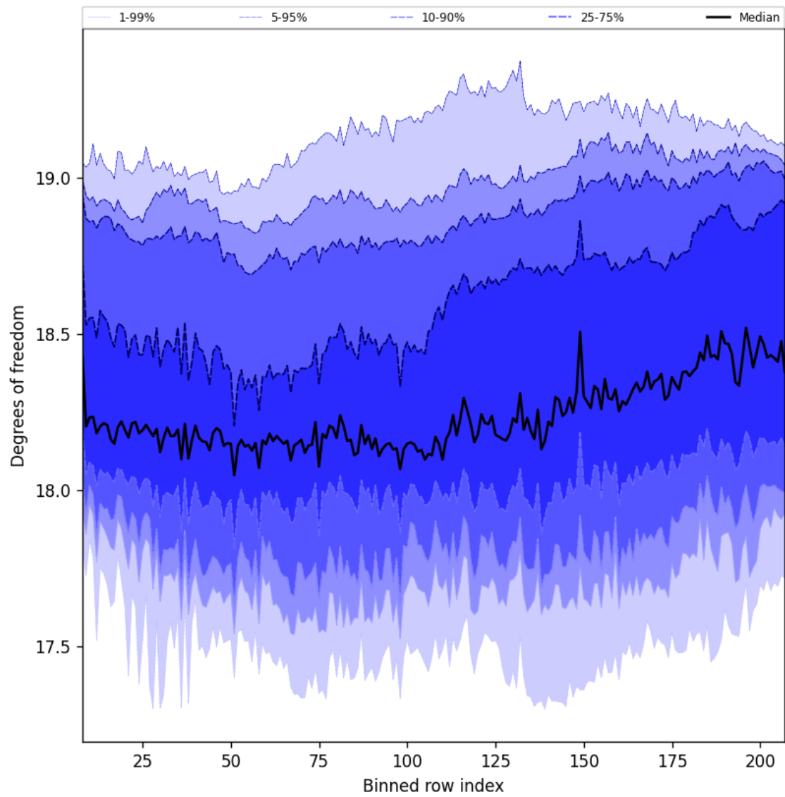
Figure 41: Along track statistics of “Degrees of freedom” for 2025-07-29 to 2025-07-31
