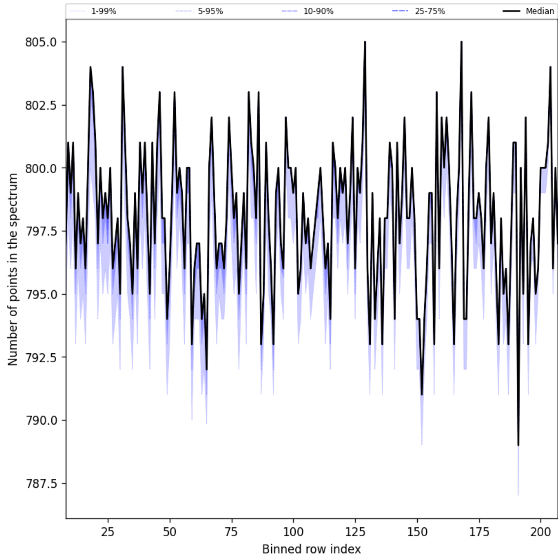
Figure 37: Along track statistics of “Number of points in the spectrum” for 2025-07-29 to 2025-07-31
