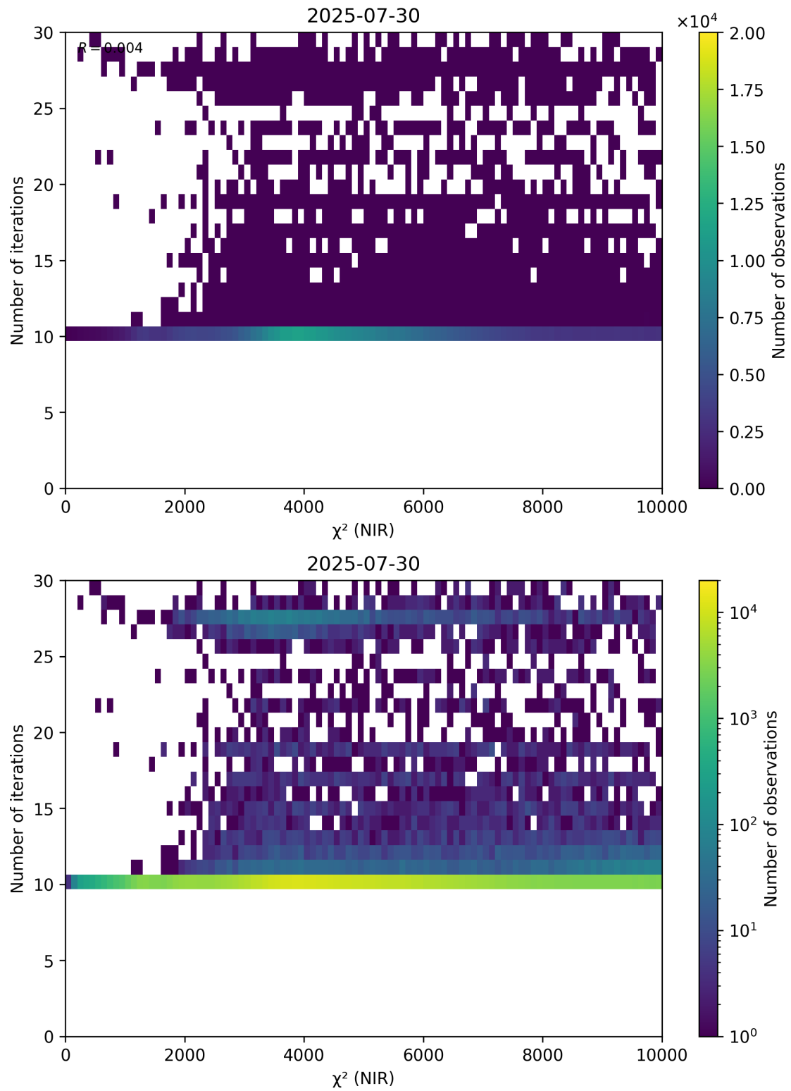
Figure 46: Scatter density plot of “ \chi^2 (NIR)” against “Number of iterations” for 2025-07-29 to 2025-07-31.
