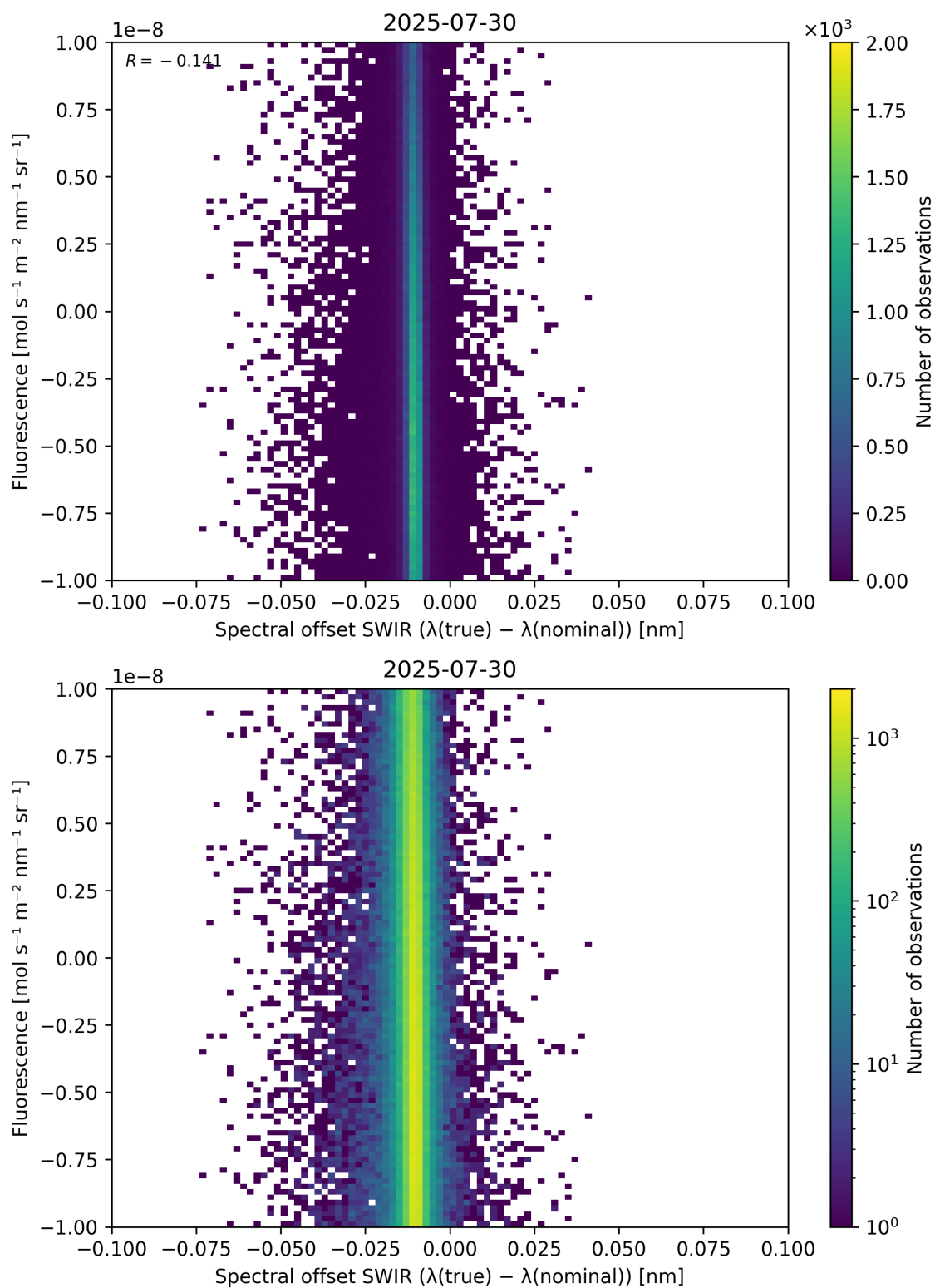
Figure 120: Scatter density plot of “Spectral offset SWIR ( \lambda_{\text{true}} - \lambda_{\text{nominal}} )” against “Fluorescence” for 2025-07-29 to 2025-07-31.
