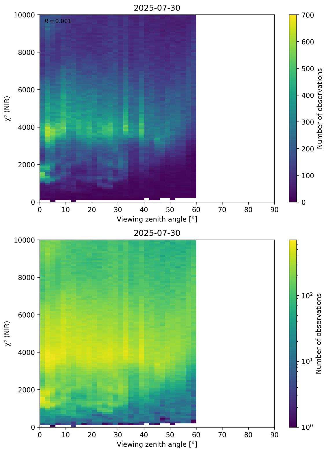
Figure 105: Scatter density plot of “Viewing zenith angle” against “ \chi^2 (NIR)” for 2025-07-29 to 2025-07-31.
