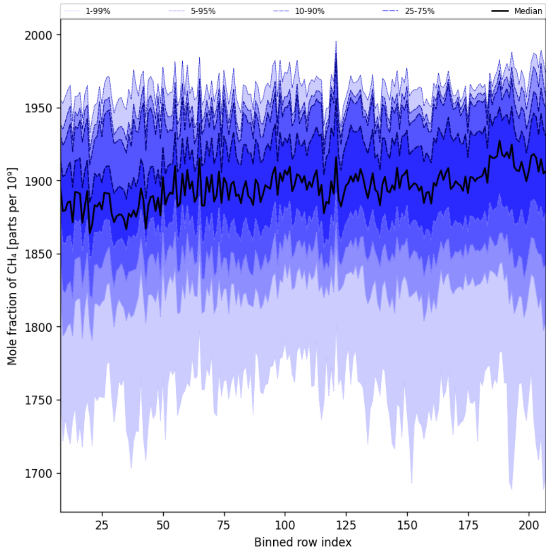
Figure 34: Along track statistics of “Mole fraction of CH 4 ” for 2025-07-29 to 2025-07-31
