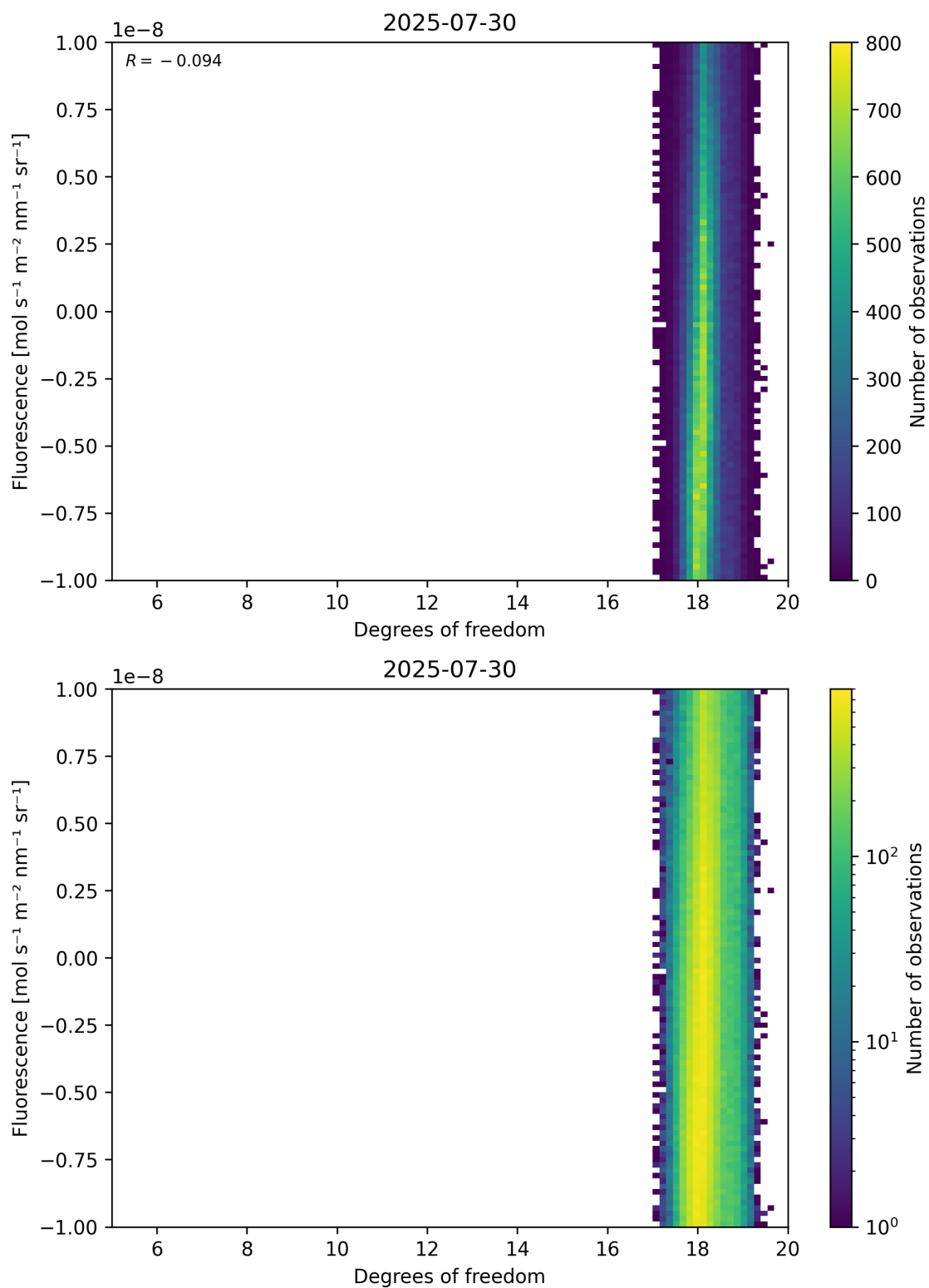
Figure 51: Scatter density plot of “Degrees of freedom” against “Fluorescence” for 2025-07-29 to 2025-07-31.
