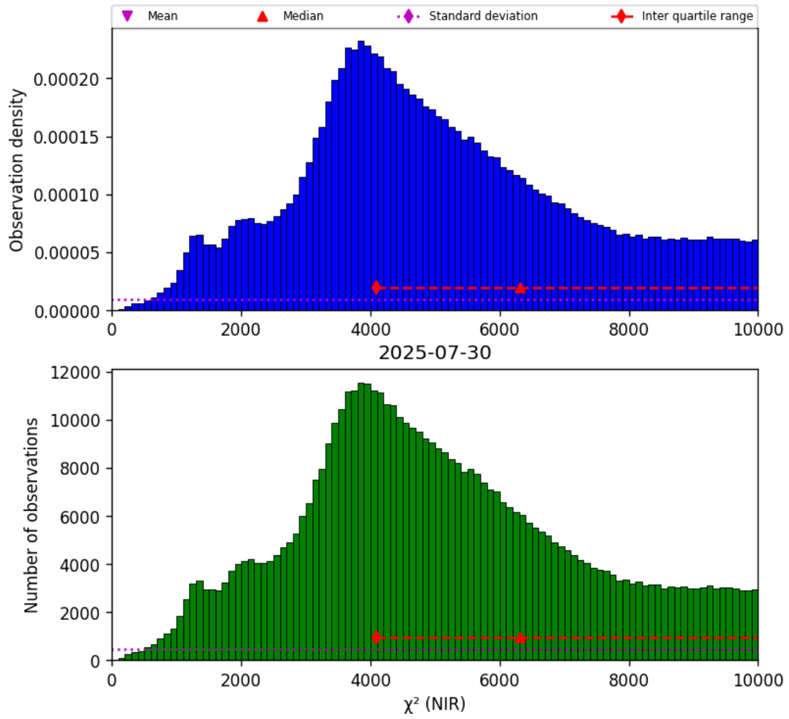
Figure 29: Histogram of “ \chi^2 (NIR)” for 2025-07-29 to 2025-07-31
