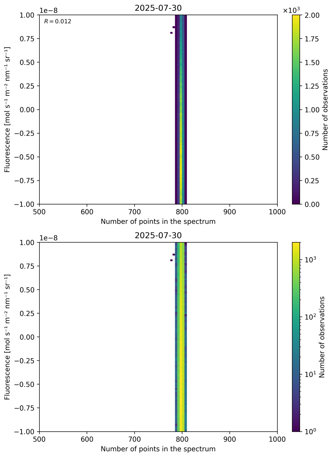
Figure 91: Scatter density plot of “Number of points in the spectrum” against “Fluorescence” for 2025-07-29 to 2025-07-31.
