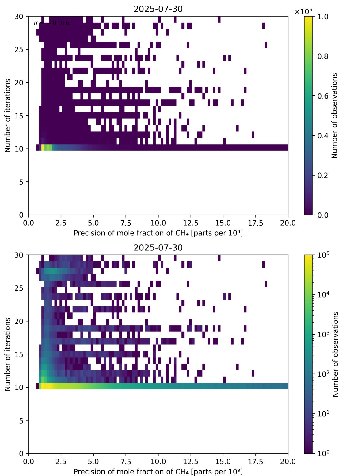
Figure 83: Scatter density plot of “Precision of mole fraction of CH 4 ” against “Number of iterations” for 2025-07-29 to 2025-07-31.
