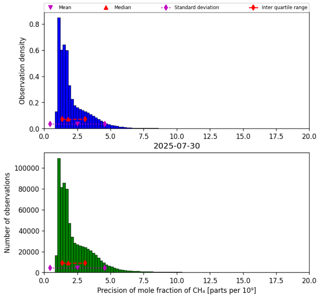
Figure 24: Histogram of “Precision of mole fraction of CH 4 ” for 2025-07-29 to 2025-07-31
