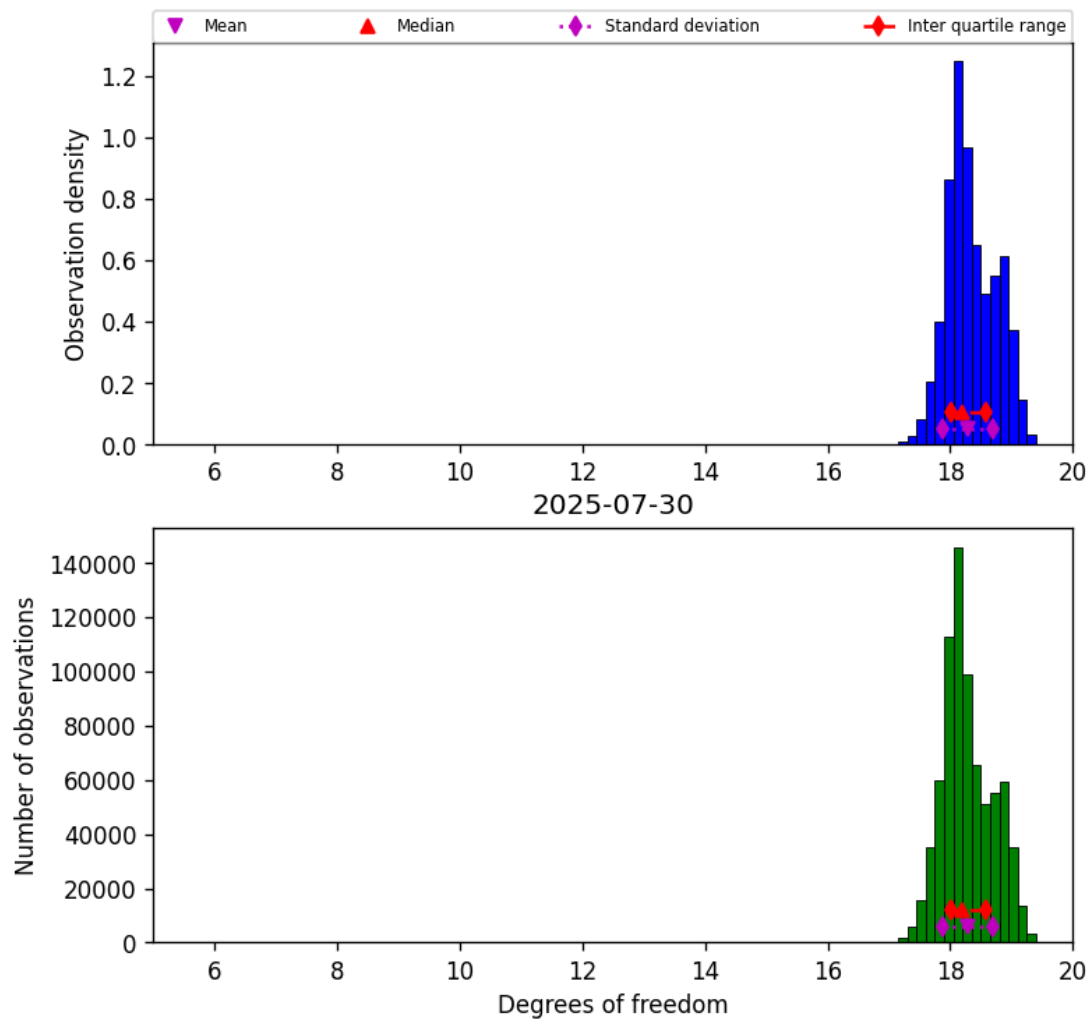
Figure 30: Histogram of “Degrees of freedom” for 2025-07-29 to 2025-07-31
