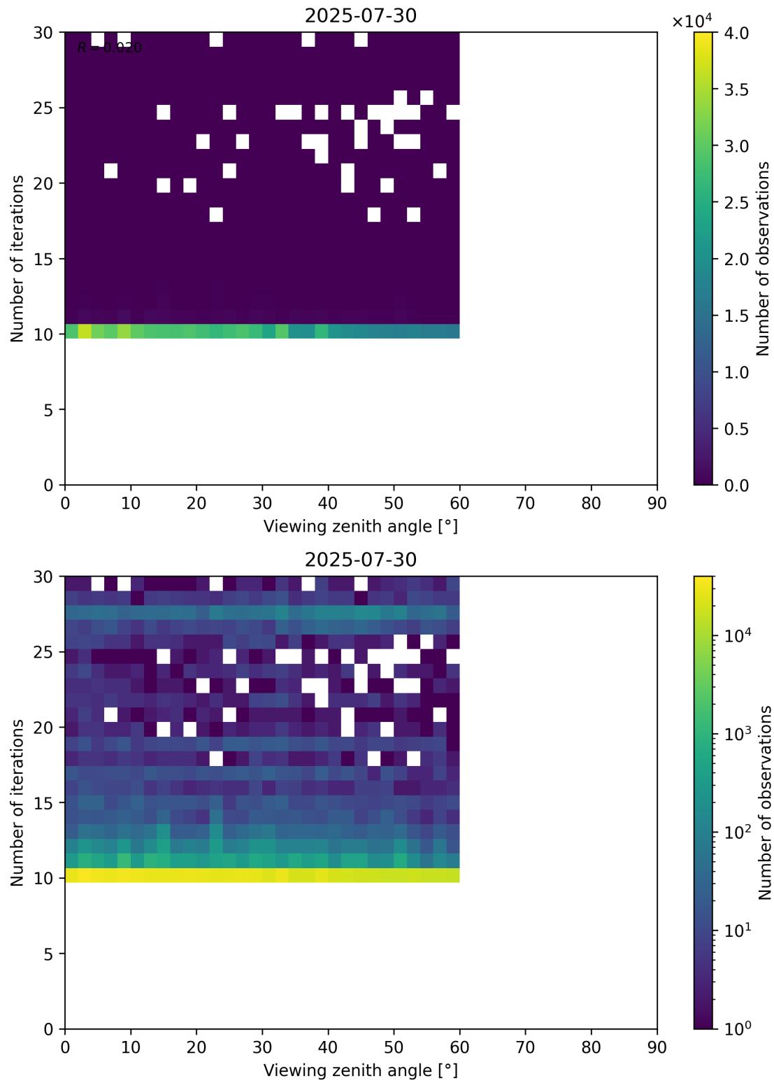
Figure 113: Scatter density plot of “Viewing zenith angle” against “Number of iterations” for 2025-07-29 to 2025-07-31.
