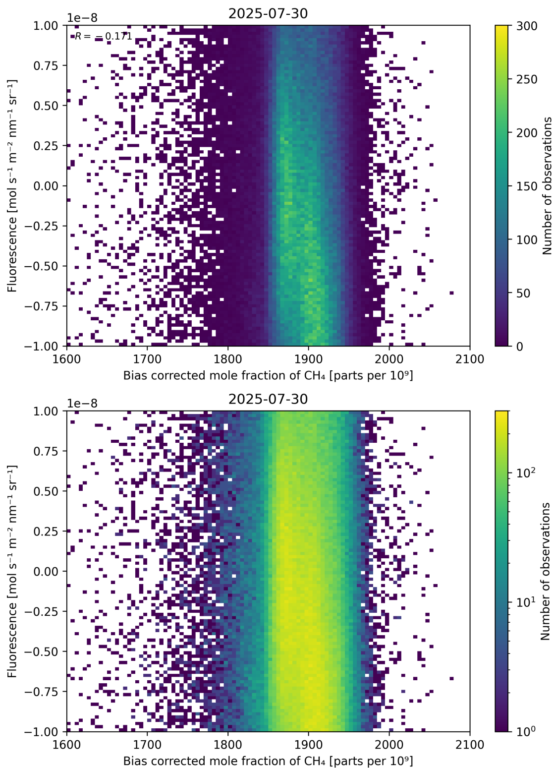
Figure 66: Scatter density plot of “Bias corrected mole fraction of \text{CH}_4 ” against “Fluorescence” for 2025-07-29 to 2025-07-31.
