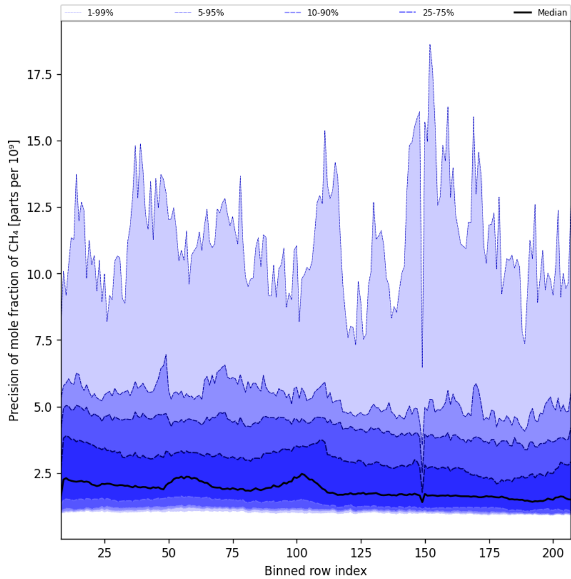
Figure 35: Along track statistics of “Precision of mole fraction of CH 4 ” for 2025-07-29 to 2025-07-31
