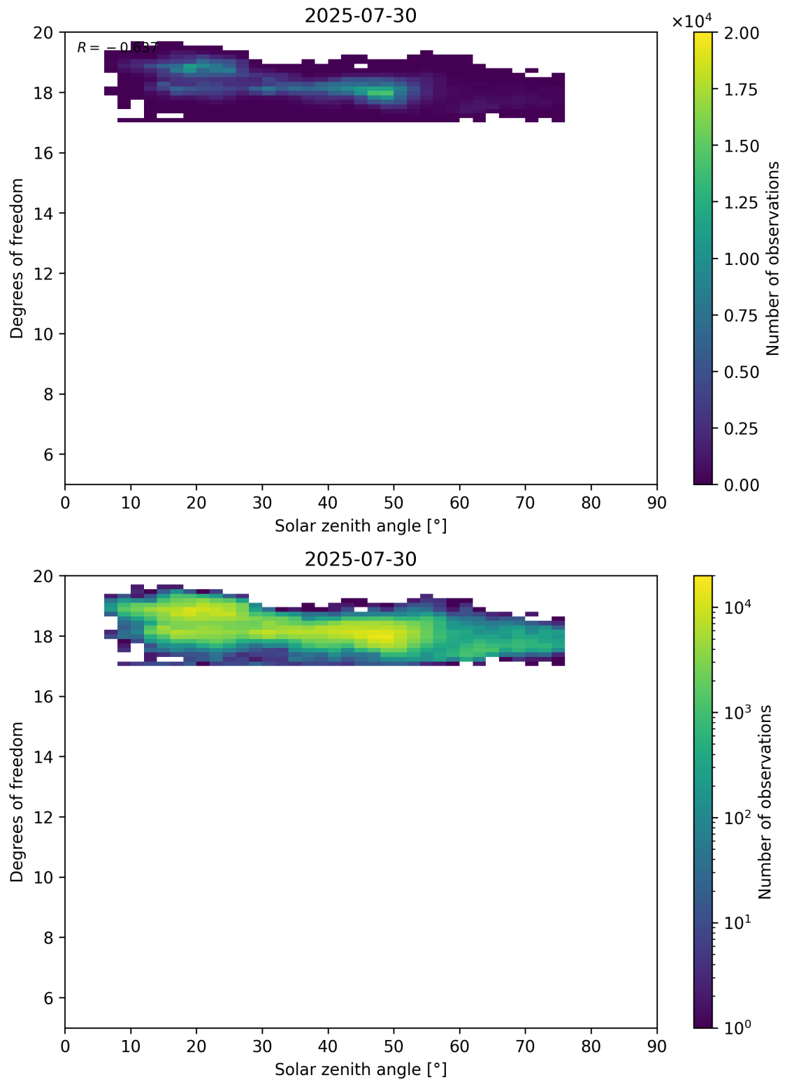
Figure 96: Scatter density plot of “Solar zenith angle” against “Degrees of freedom” for 2025-07-29 to 2025-07-31.
