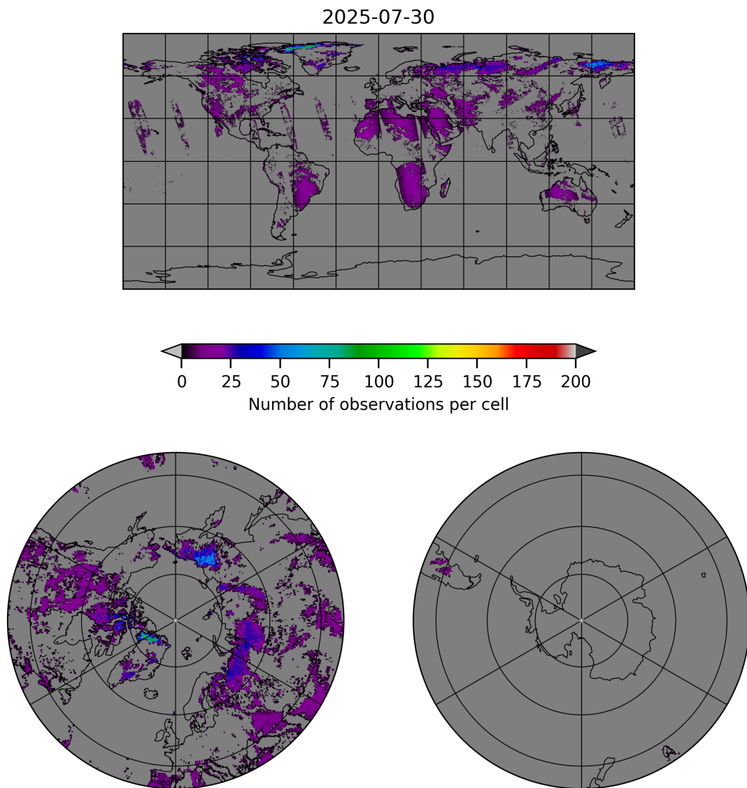
Figure 10: Map of the number of observations for 2025-07-29 to 2025-07-31
