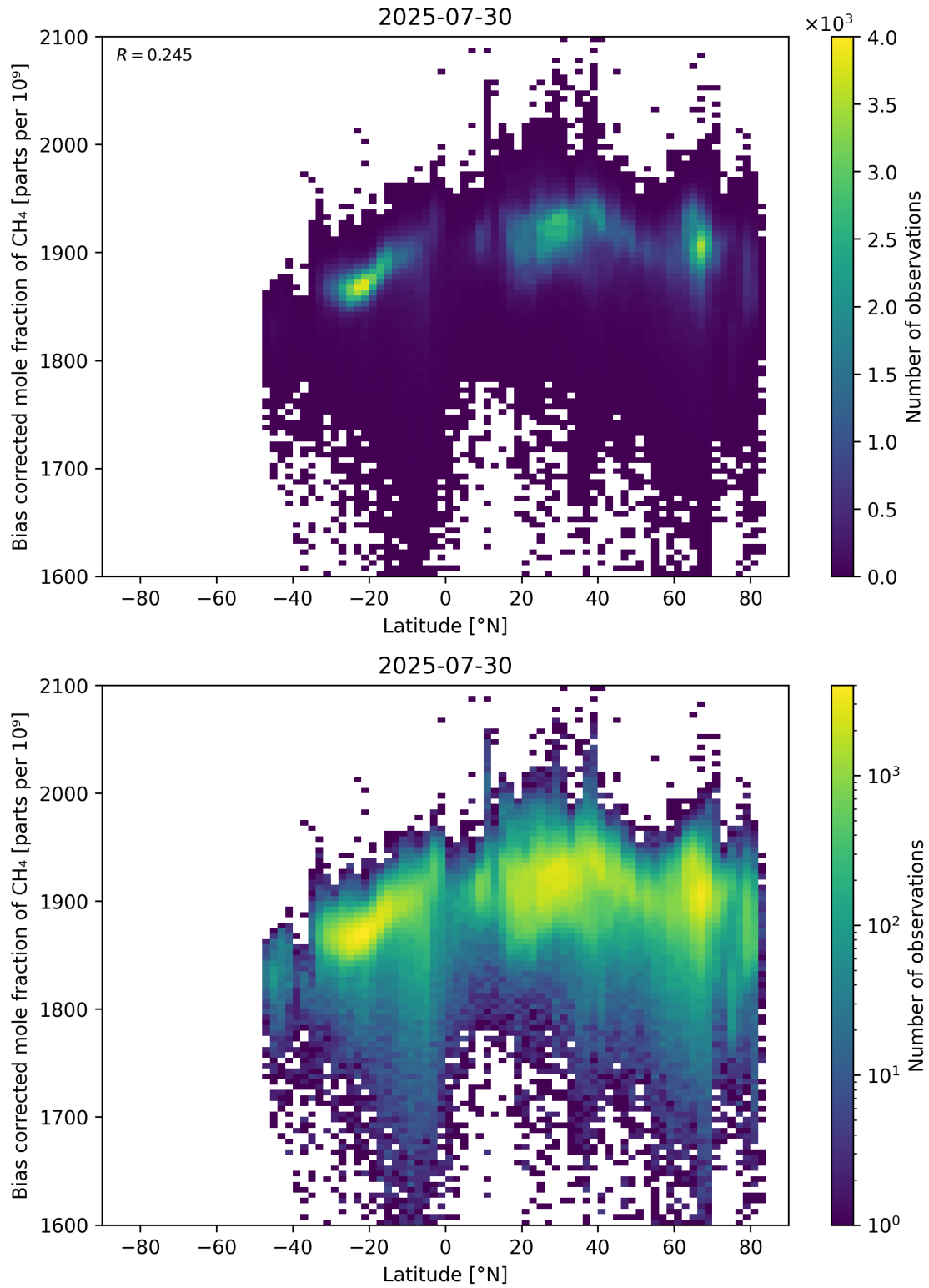
Figure 58: Scatter density plot of “Latitude” against “Bias corrected mole fraction of CH 4 ” for 2025-07-29 to 2025-07-31.
