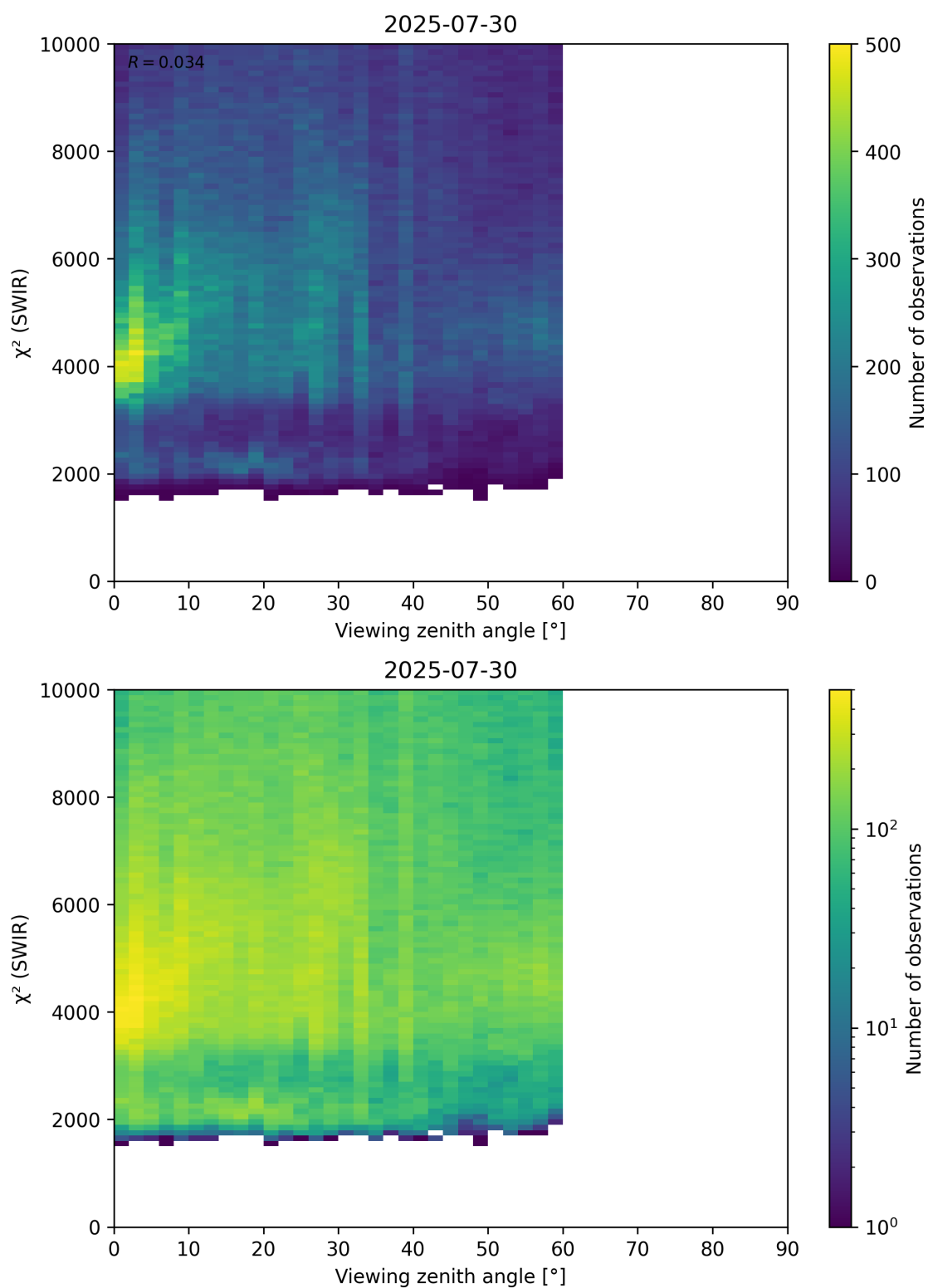
Figure 106: Scatter density plot of “Viewing zenith angle” against “ \chi^2 (SWIR)” for 2025-07-29 to 2025-07-31.
