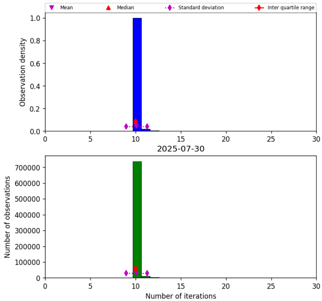
Figure 31: Histogram of “Number of iterations” for 2025-07-29 to 2025-07-31
