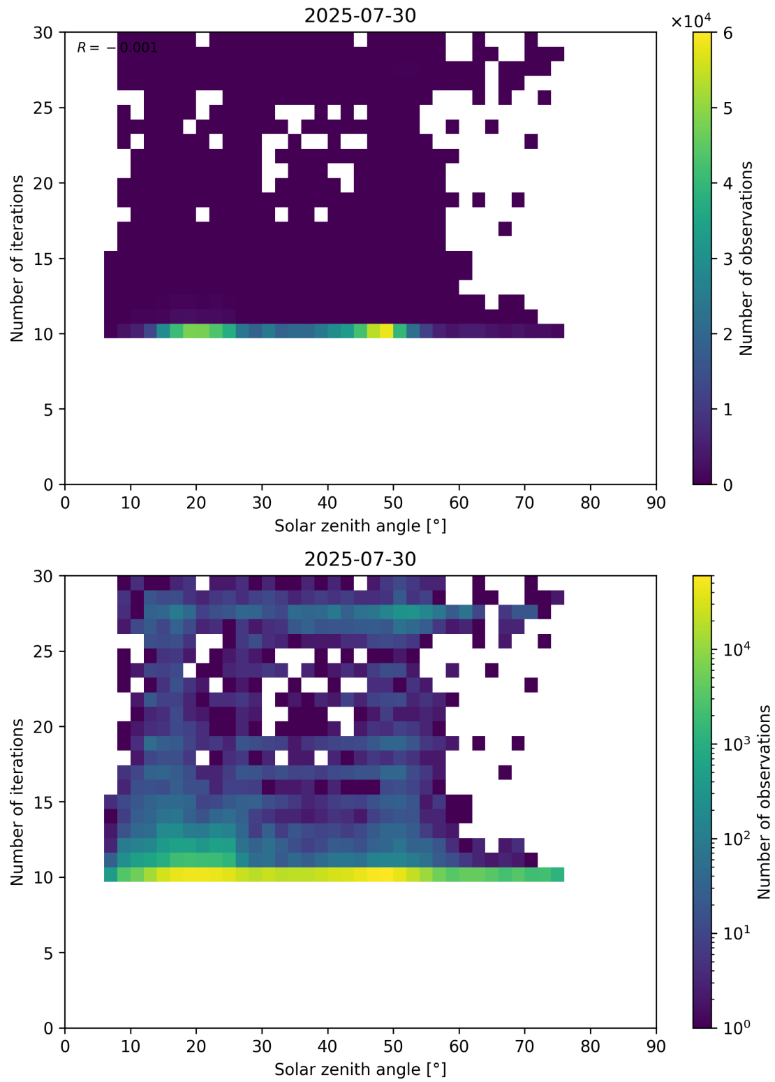
Figure 102: Scatter density plot of “Solar zenith angle” against “Number of iterations” for 2025-07-29 to 2025-07-31.
