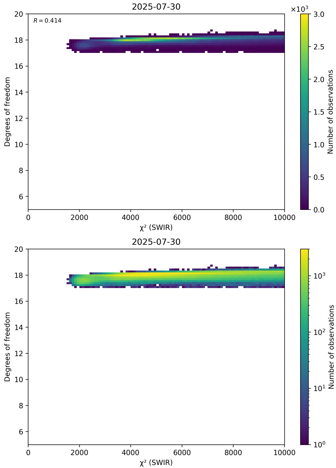
Figure 48: Scatter density plot of “ \chi^2 (SWIR)” against “Degrees of freedom” for 2025-07-29 to 2025-07-31.
