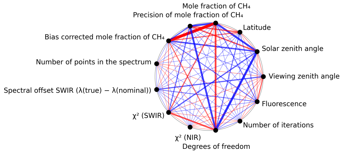
Figure 1: Map of correlation graph for 2025-07-29 to 2025-07-31.
