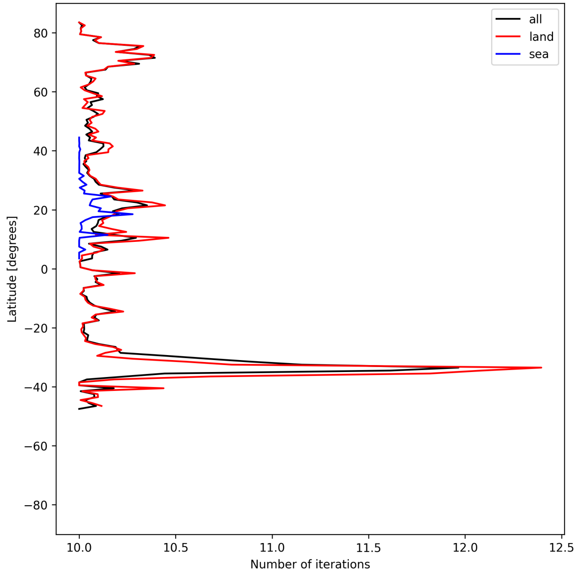
Figure 20: Zonal average of “Number of iterations” for 2025-07-29 to 2025-07-31.
