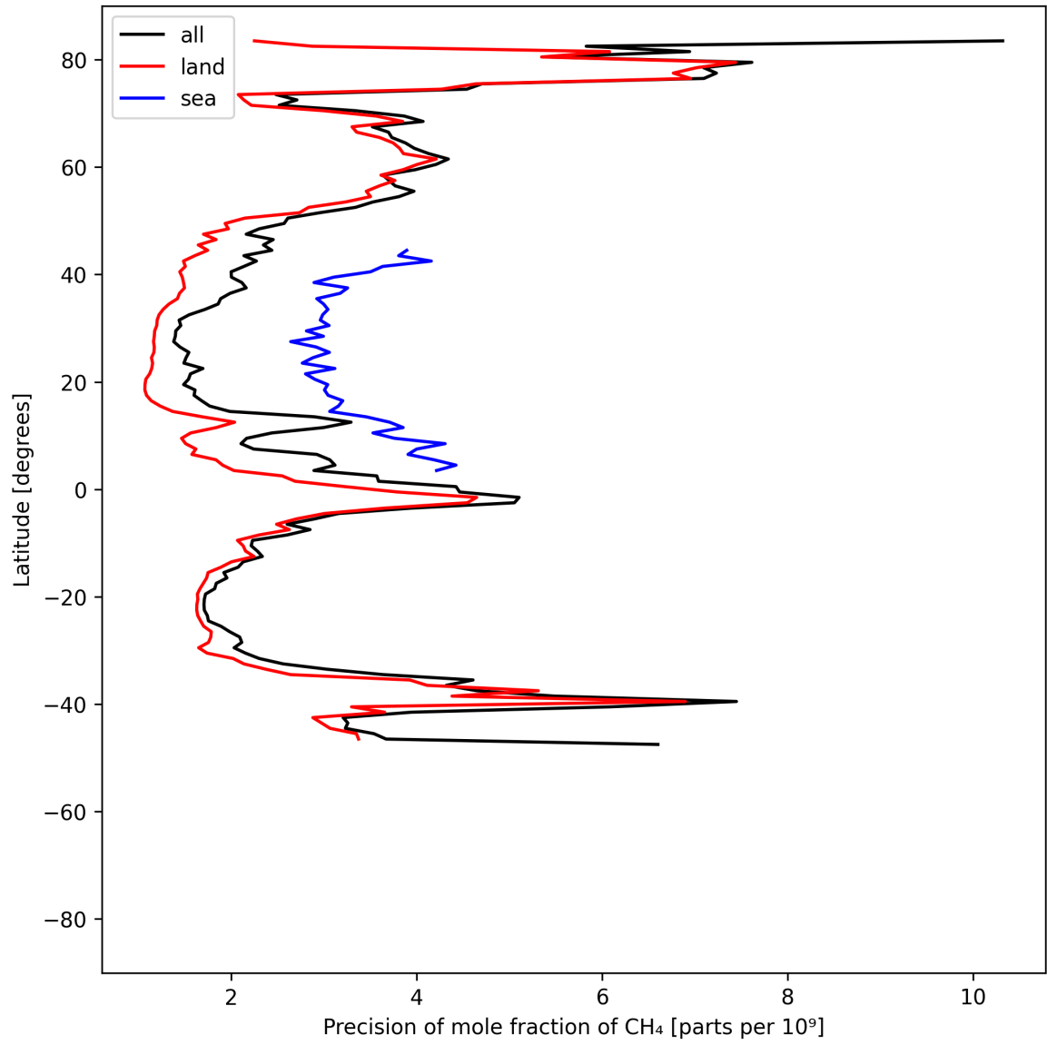
Figure 13: Zonal average of “Precision of mole fraction of CH 4 ” for 2025-07-29 to 2025-07-31.
