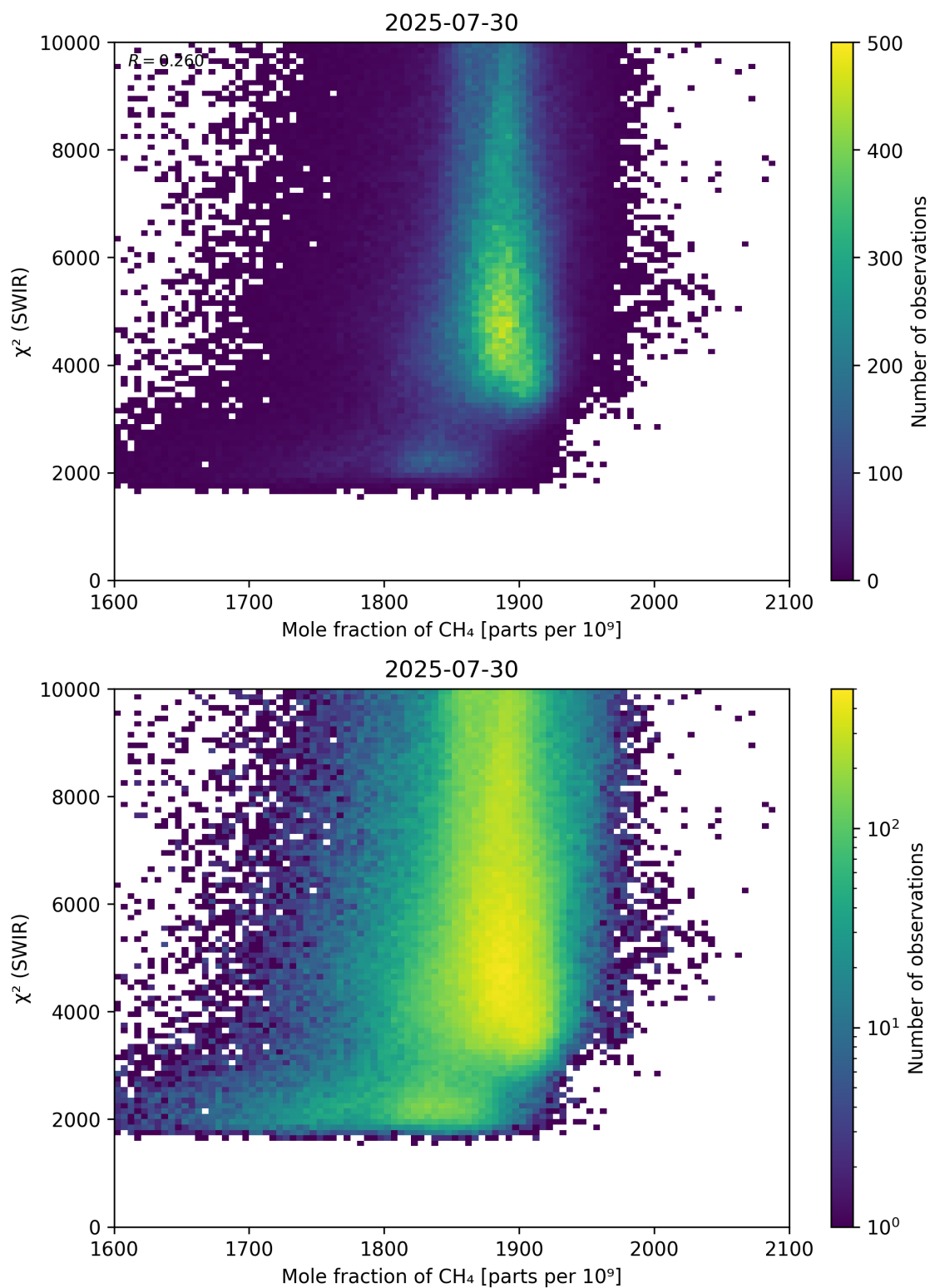
Figure 71: Scatter density plot of “Mole fraction of \text{CH}_4 ” against “ \chi^2 (SWIR)” for 2025-07-29 to 2025-07-31.
