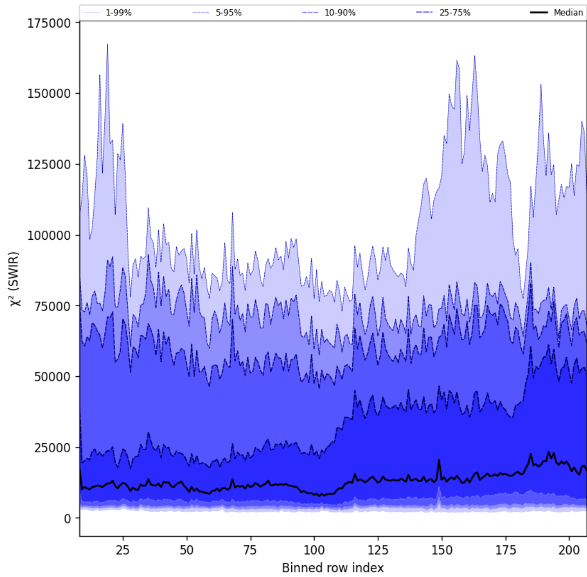
Figure 39: Along track statistics of “ \chi^2 (SWIR)” for 2025-07-29 to 2025-07-31
