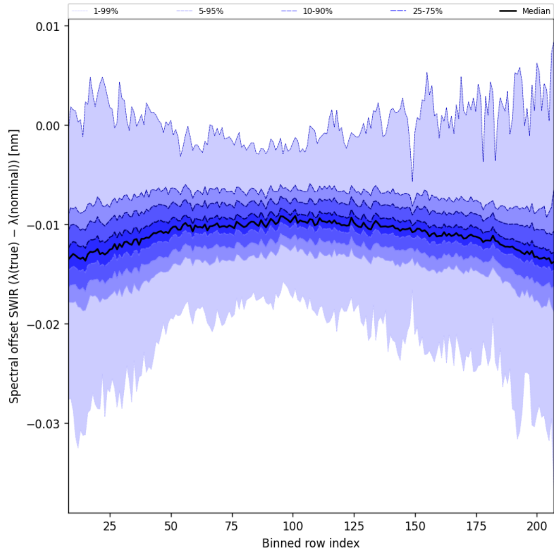
Figure 38: Along track statistics of “Spectral offset SWIR ( \lambda_{\text{true}} - \lambda_{\text{nominal}} )” for 2025-07-29 to 2025-07-31
