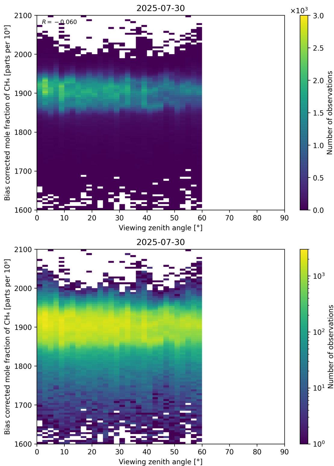
Figure 111: Scatter density plot of “Viewing zenith angle” against “Bias corrected mole fraction of CH 4 ” for 2025-07-29 to 2025-07-31.
