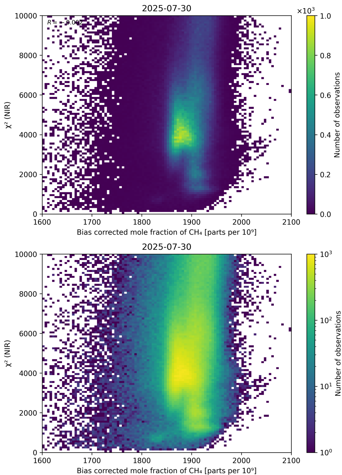
Figure 63: Scatter density plot of “Bias corrected mole fraction of \text{CH}_4 ” against “ \chi^2 (NIR)” for 2025-07-29 to 2025-07-31.
