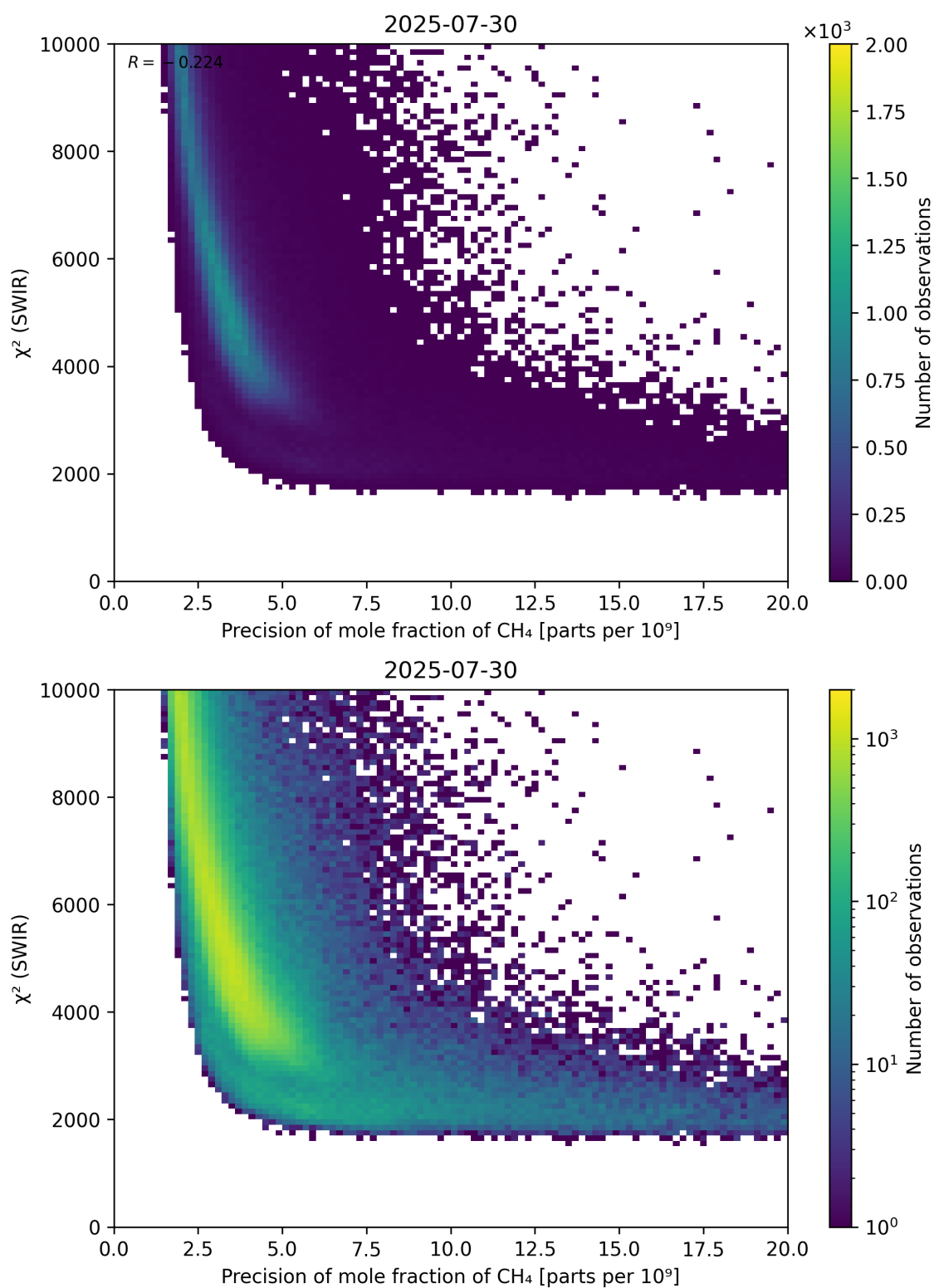
Figure 79: Scatter density plot of “Precision of mole fraction of \text{CH}_4 ” against “ \chi^2 (SWIR)” for 2025-07-29 to 2025-07-31.
