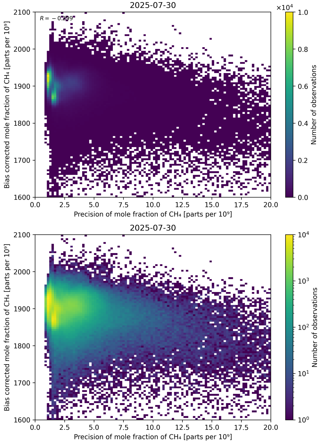
Figure 82: Scatter density plot of “Precision of mole fraction of \text{CH}_4 ” against “Bias corrected mole fraction of \text{CH}_4 ” for 2025-07-29 to 2025-07-31.
