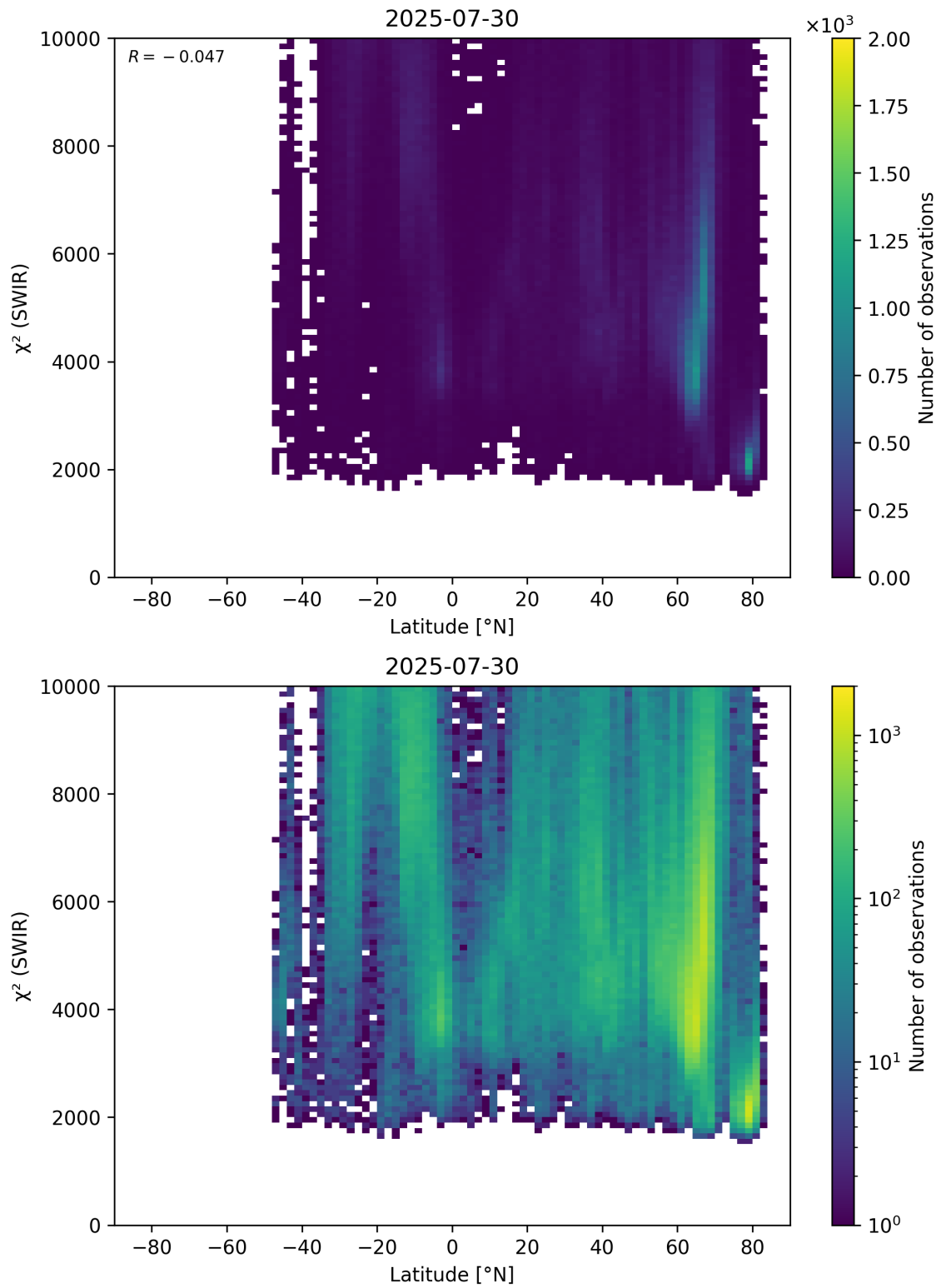
Figure 54: Scatter density plot of “Latitude” against “ \chi^2 (SWIR)” for 2025-07-29 to 2025-07-31.
