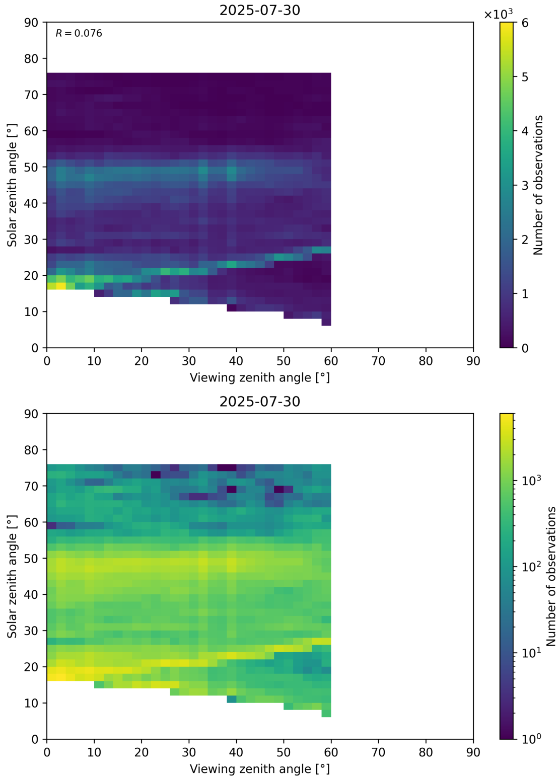
Figure 115: Scatter density plot of “Viewing zenith angle” against “Solar zenith angle” for 2025-07-29 to 2025-07-31.
