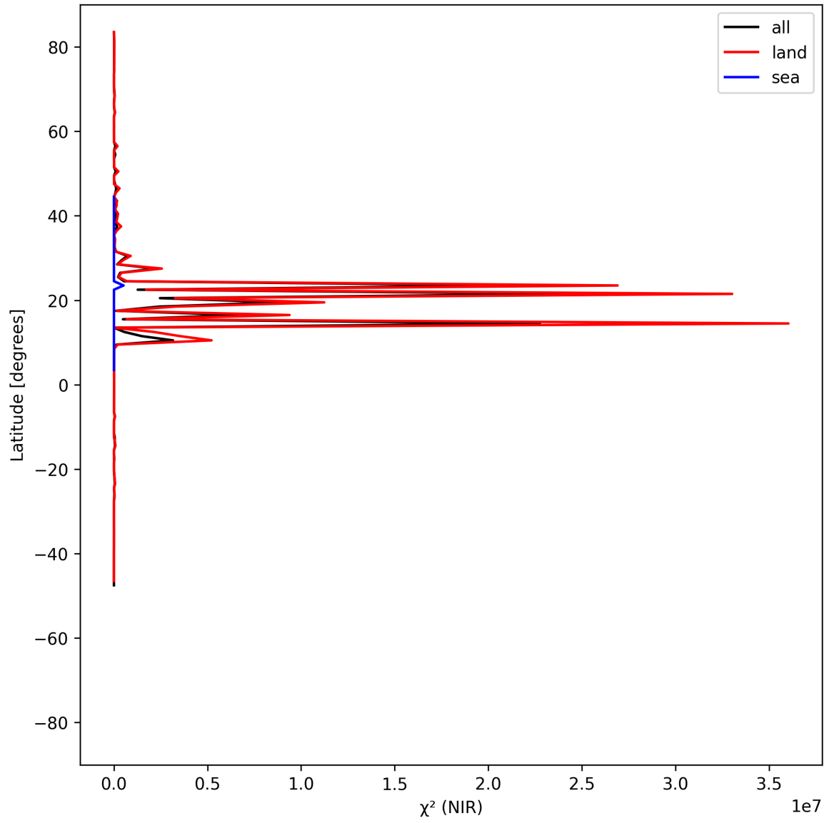
Figure 18: Zonal average of “ \chi^2 (NIR)” for 2025-07-29 to 2025-07-31.
