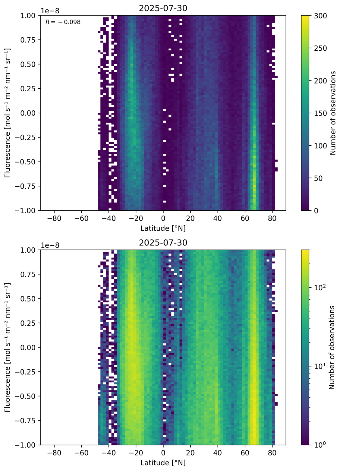
Figure 56: Scatter density plot of “Latitude” against “Fluorescence” for 2025-07-29 to 2025-07-31.
