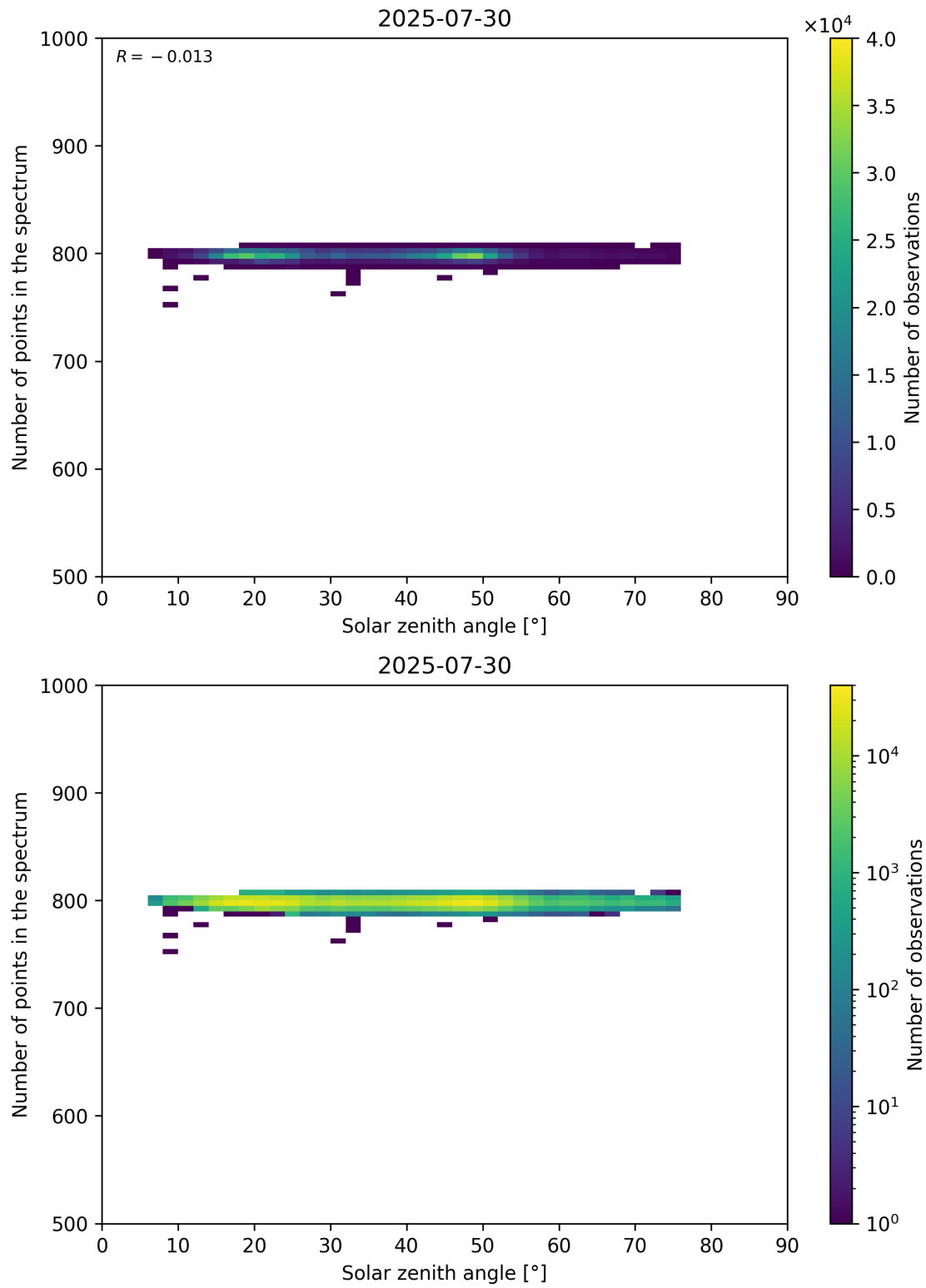
Figure 103: Scatter density plot of “Solar zenith angle” against “Number of points in the spectrum” for 2025-07-29 to 2025-07-31.
