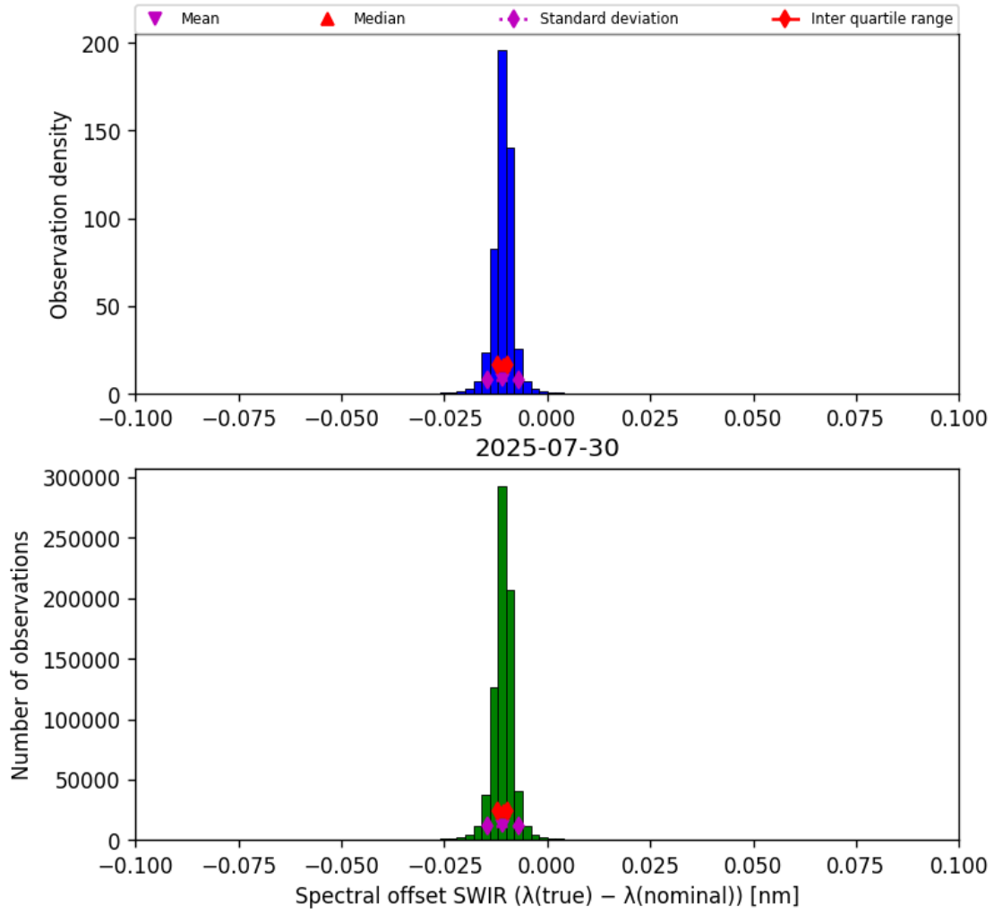
Figure 27: Histogram of “Spectral offset SWIR ( \lambda_{\text{true}} - \lambda_{\text{nominal}} )” for 2025-07-29 to 2025-07-31
