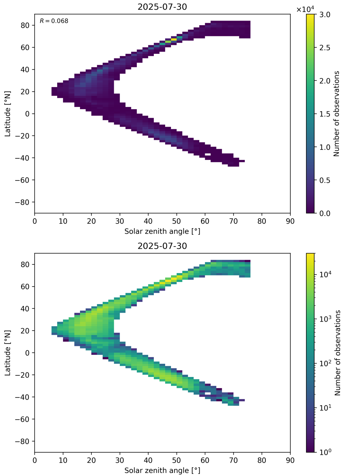
Figure 98: Scatter density plot of “Solar zenith angle” against “Latitude” for 2025-07-29 to 2025-07-31.
