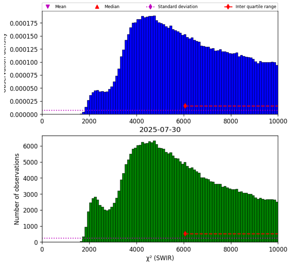
Figure 28: Histogram of “ \chi^2 (SWIR)” for 2025-07-29 to 2025-07-31
