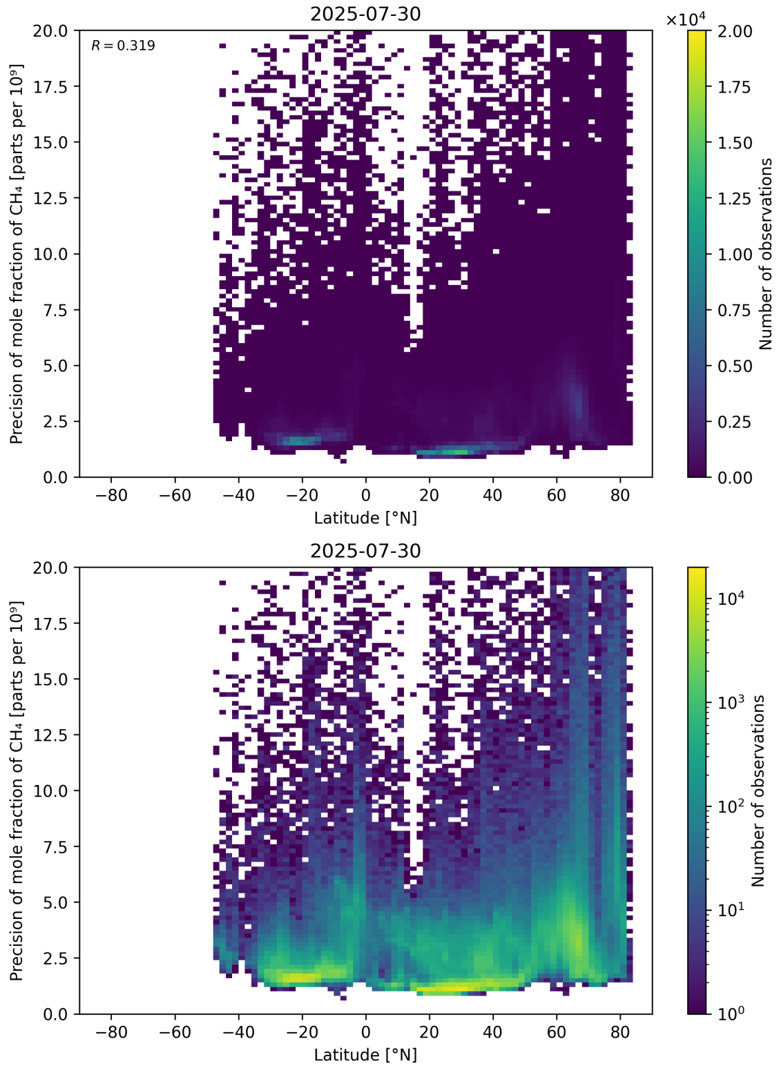
Figure 59: Scatter density plot of “Latitude” against “Precision of mole fraction of \text{CH}_4 ” for 2025-07-29 to 2025-07-31.
