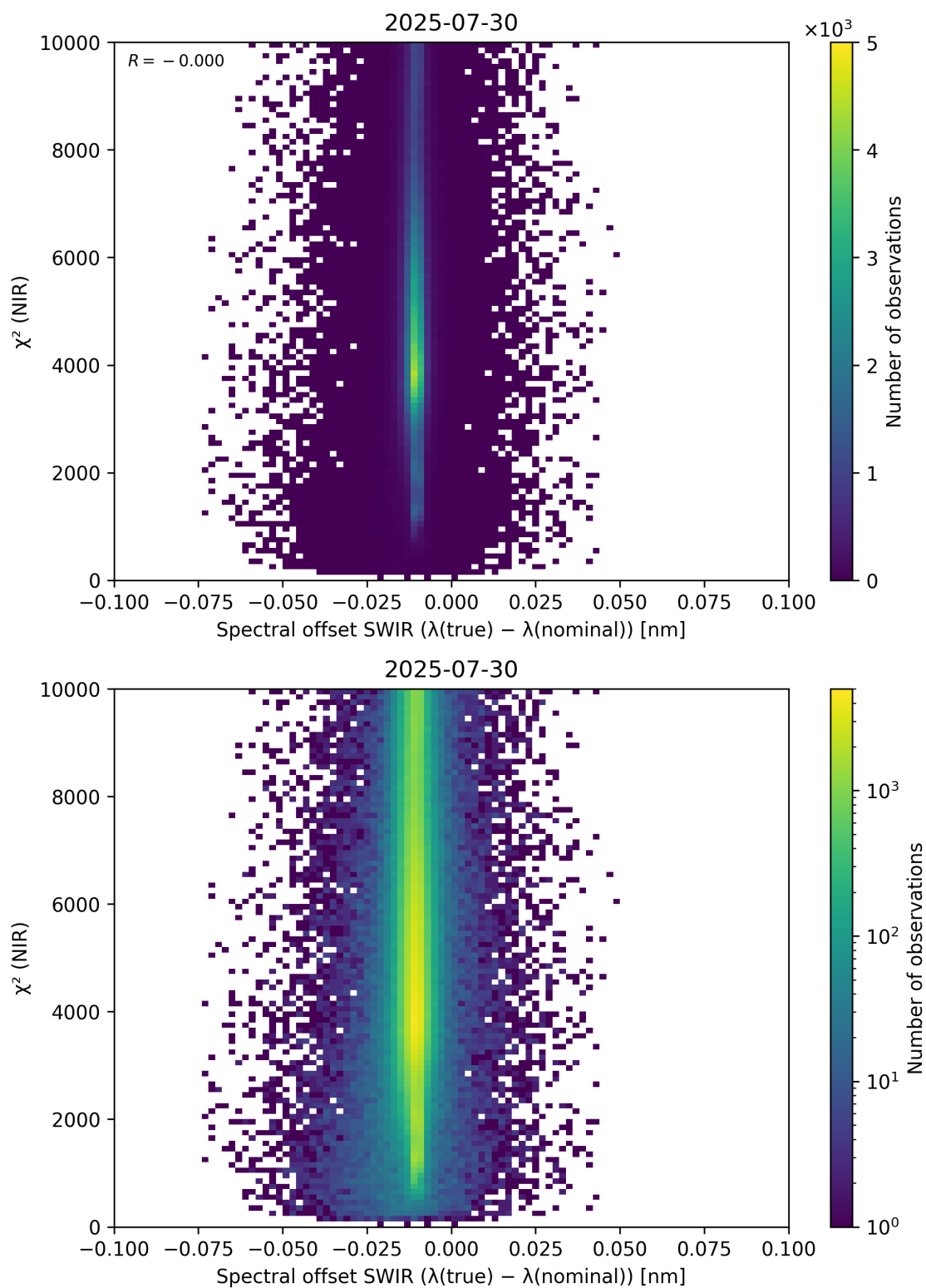
Figure 117: Scatter density plot of “Spectral offset SWIR ( \lambda_{\text{true}} - \lambda_{\text{nominal}} )” against “ \chi^2 (NIR)” for 2025-07-29 to 2025-07-31.
