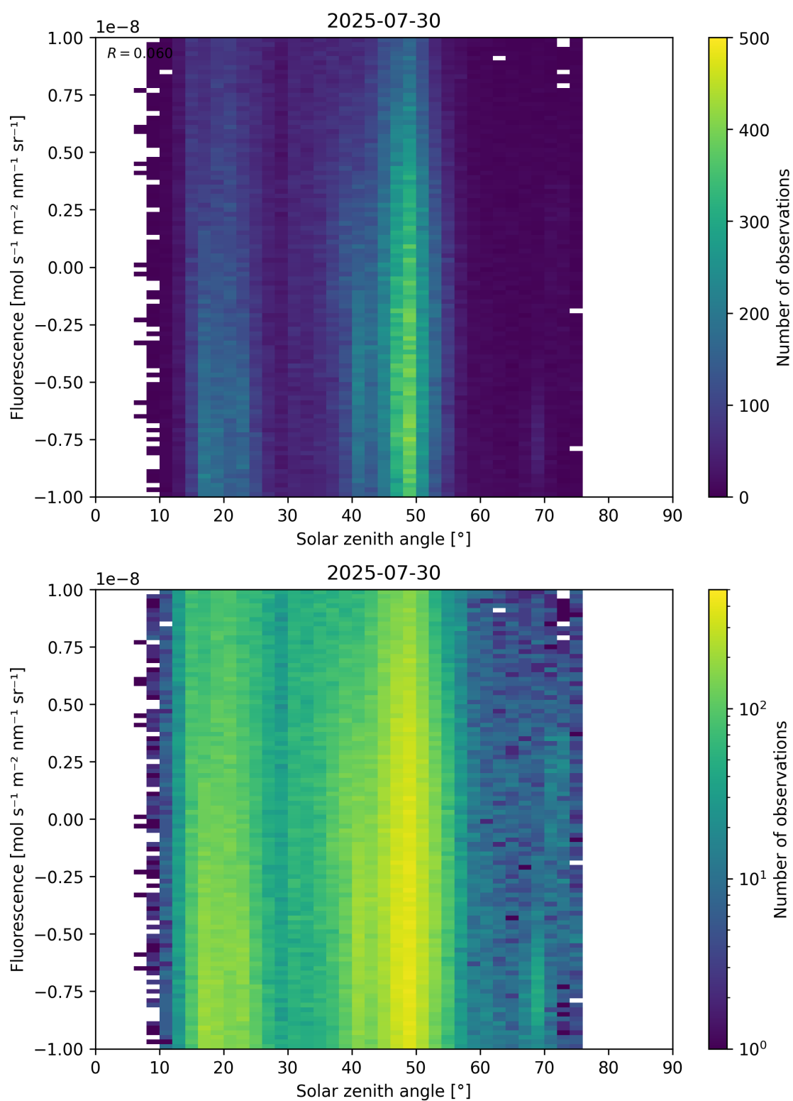
Figure 97: Scatter density plot of “Solar zenith angle” against “Fluorescence” for 2025-07-29 to 2025-07-31.
