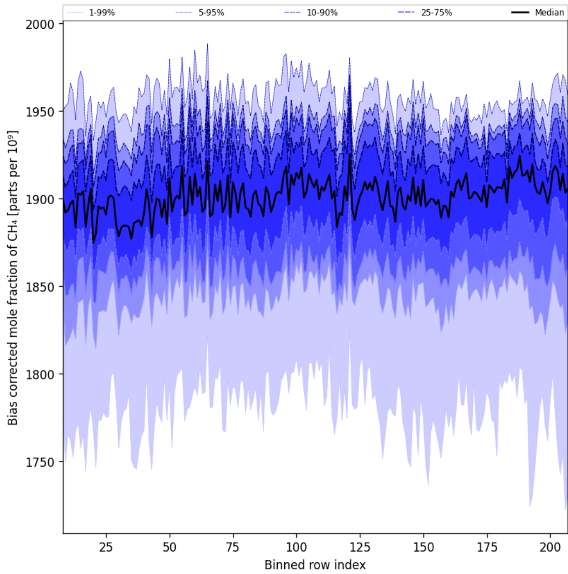
Figure 36: Along track statistics of “Bias corrected mole fraction of CH 4 ” for 2025-07-29 to 2025-07-31
