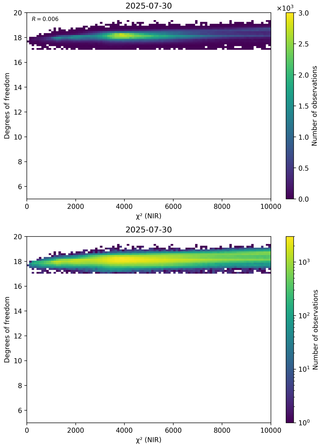
Figure 44: Scatter density plot of “ \chi^2 (NIR)” against “Degrees of freedom” for 2025-07-29 to 2025-07-31.
