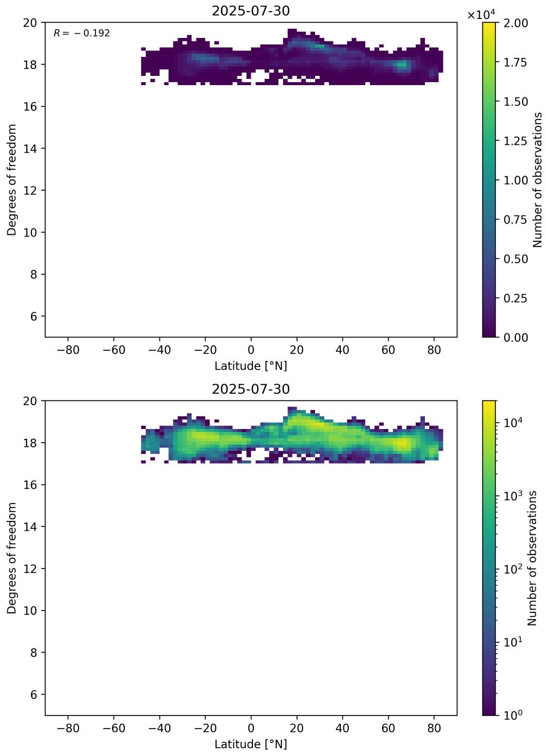
Figure 55: Scatter density plot of “Latitude” against “Degrees of freedom” for 2025-07-29 to 2025-07-31.
