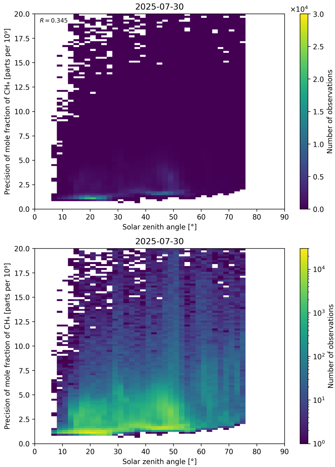
Figure 101: Scatter density plot of “Solar zenith angle” against “Precision of mole fraction of CH 4 ” for 2025-07-29 to 2025-07-31.
