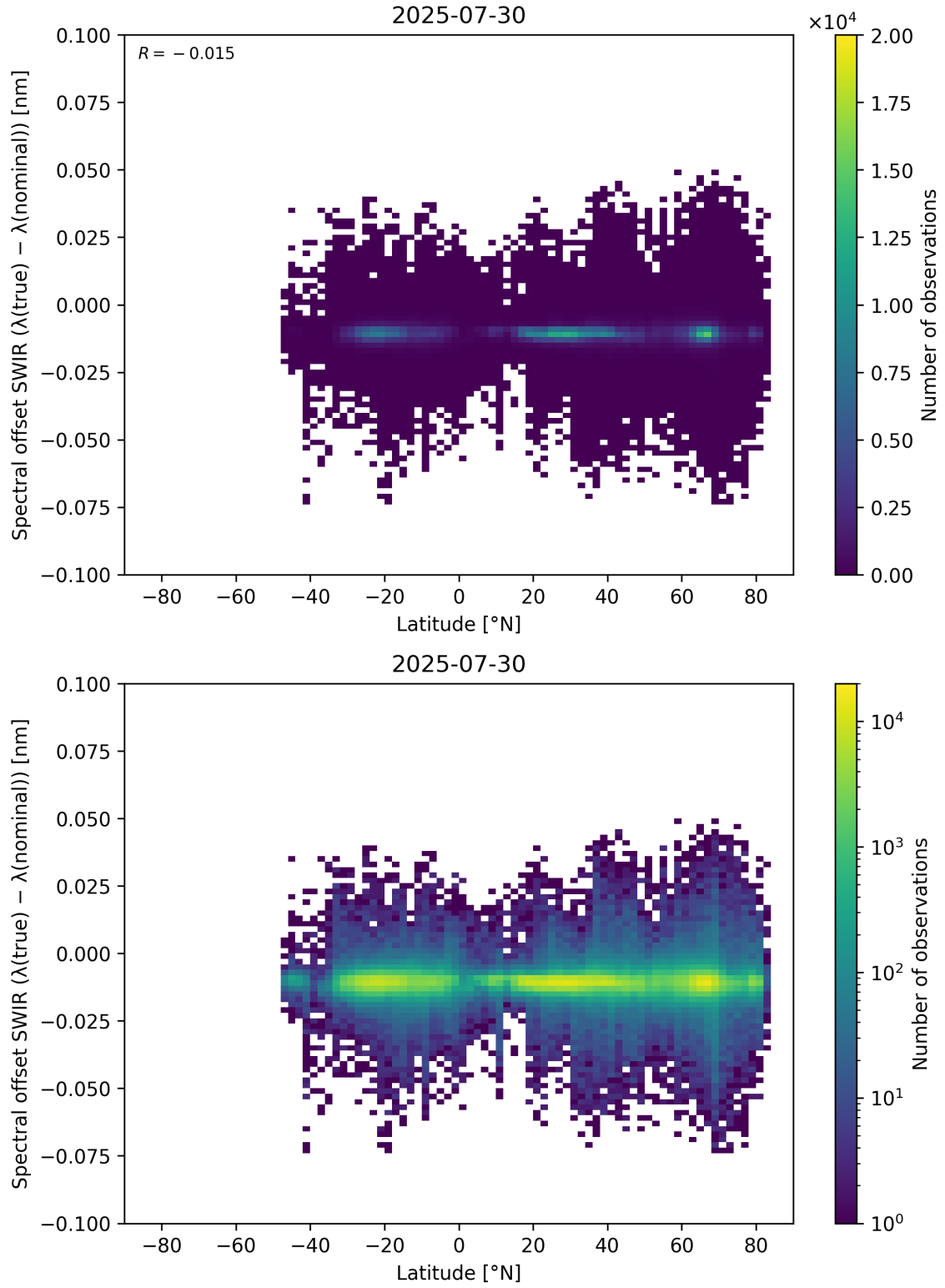
Figure 62: Scatter density plot of “Latitude” against “Spectral offset SWIR ( \lambda_{\text{true}} - \lambda_{\text{nominal}} )” for 2025-07-29 to 2025-07-31.
