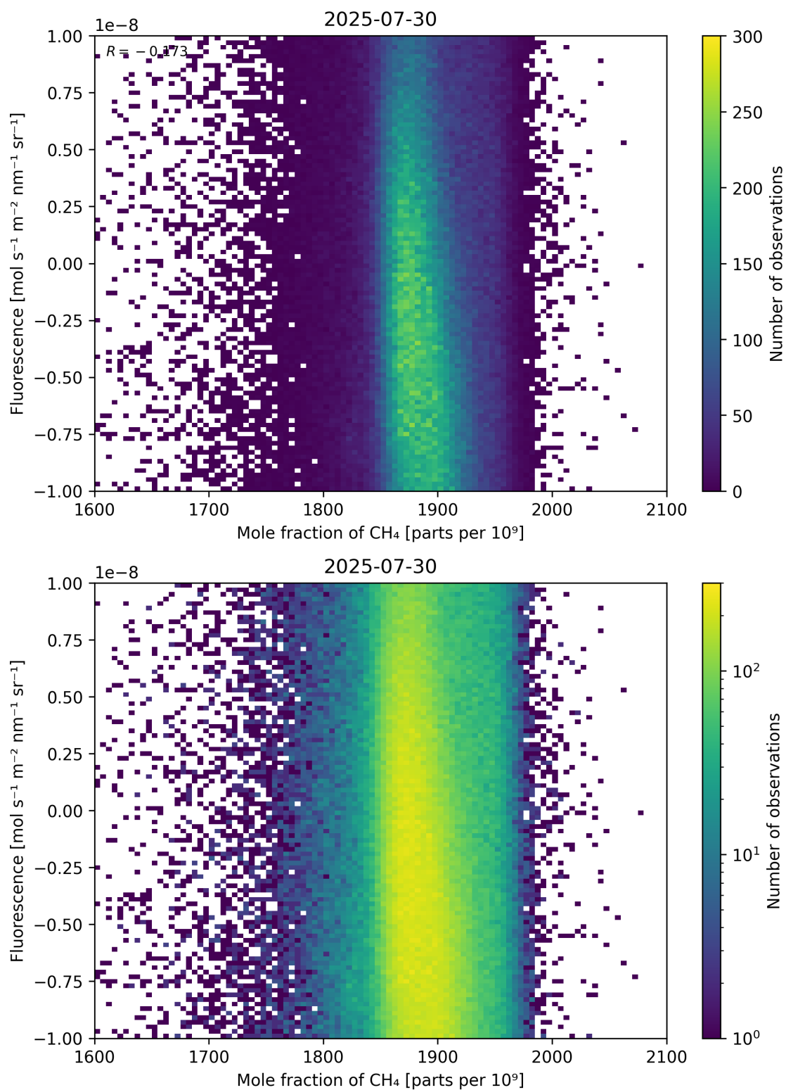
Figure 73: Scatter density plot of “Mole fraction of \text{CH}_4 ” against “Fluorescence” for 2025-07-29 to 2025-07-31.
