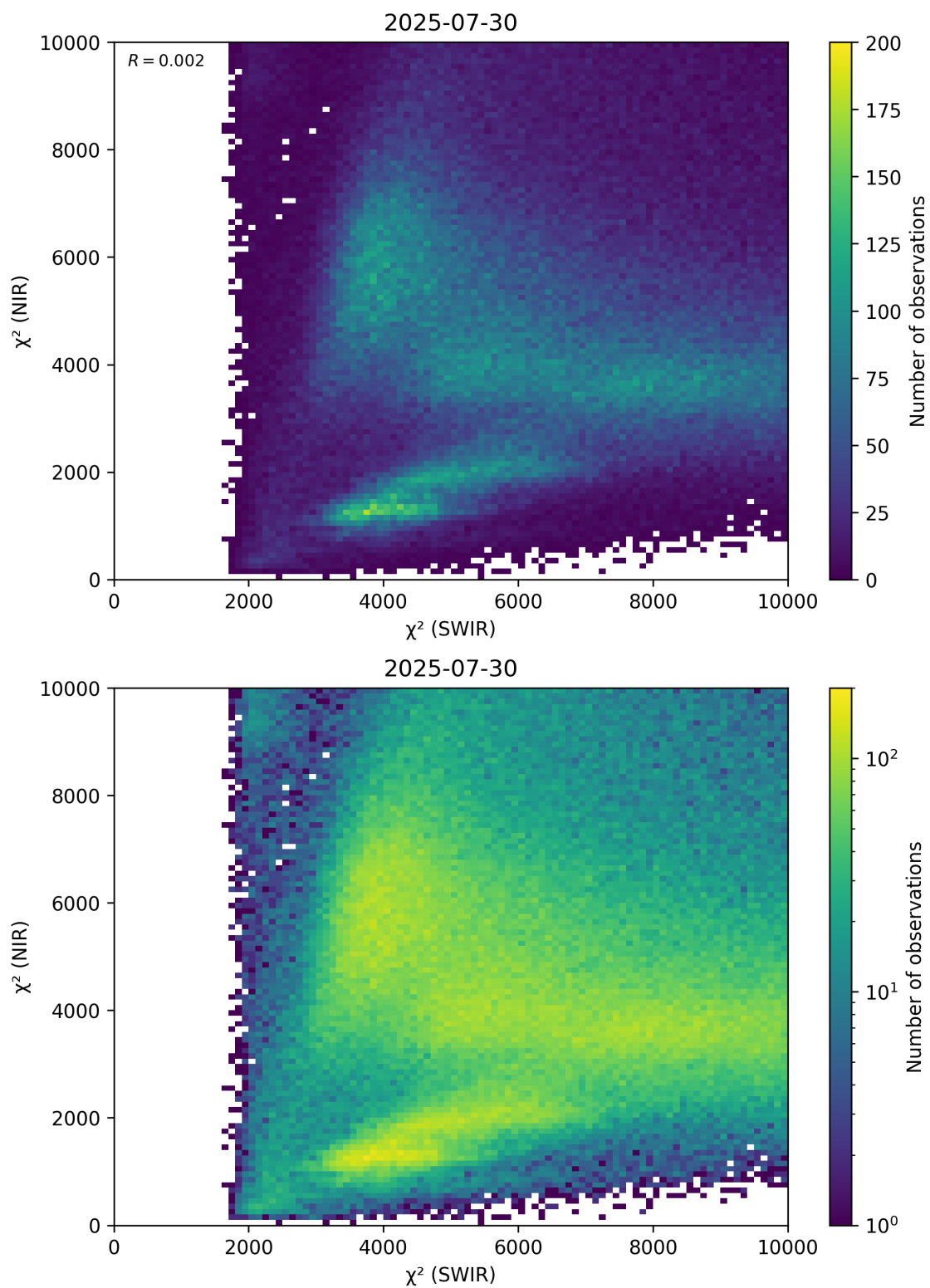
Figure 47: Scatter density plot of “ \chi^2 (SWIR)” against “ \chi^2 (NIR)” for 2025-07-29 to 2025-07-31.
