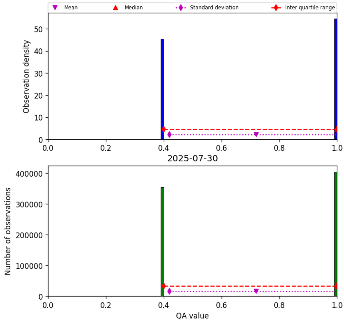
Figure 22: Histogram of “QA value” for 2025-07-29 to 2025-07-31
