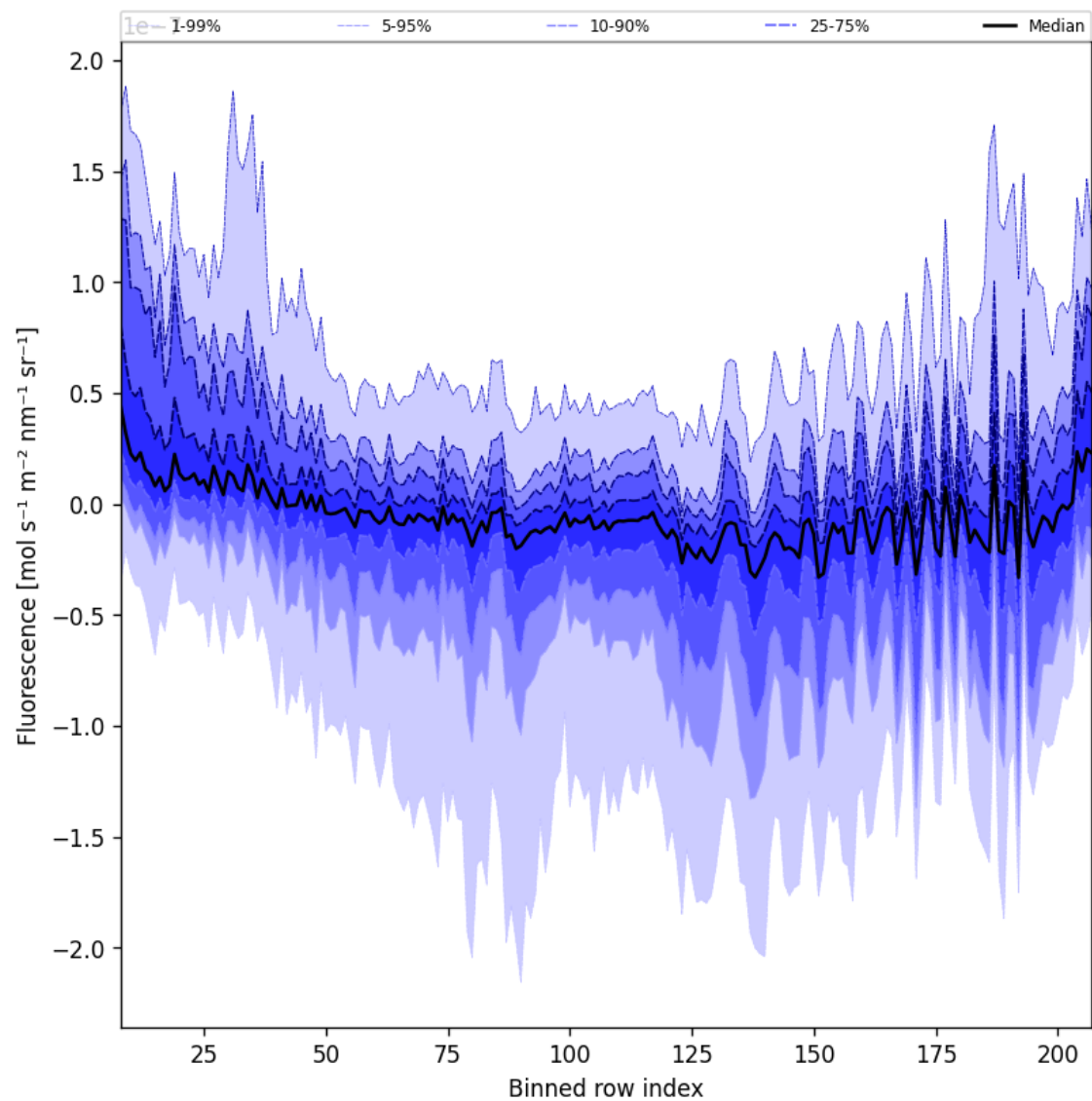
Figure 43: Along track statistics of “Fluorescence” for 2025-07-29 to 2025-07-31
