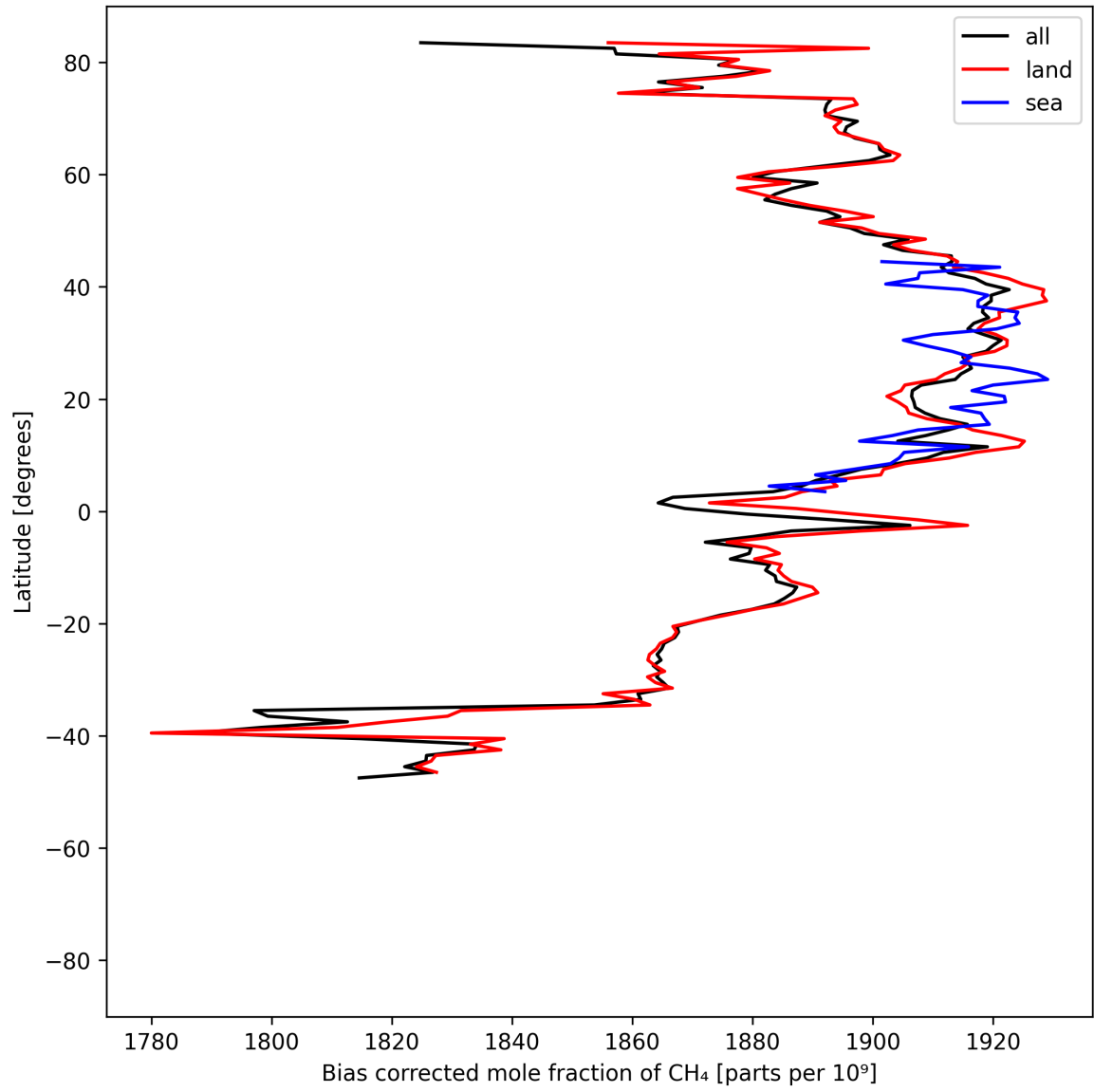
Figure 14: Zonal average of “Bias corrected mole fraction of \text{CH}_4 ” for 2025-07-29 to 2025-07-31.
