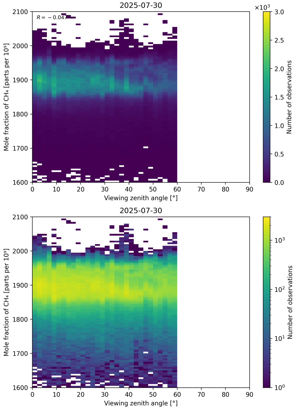
Figure 110: Scatter density plot of “Viewing zenith angle” against “Mole fraction of \text{CH}_4 ” for 2025-07-29 to 2025-07-31.
