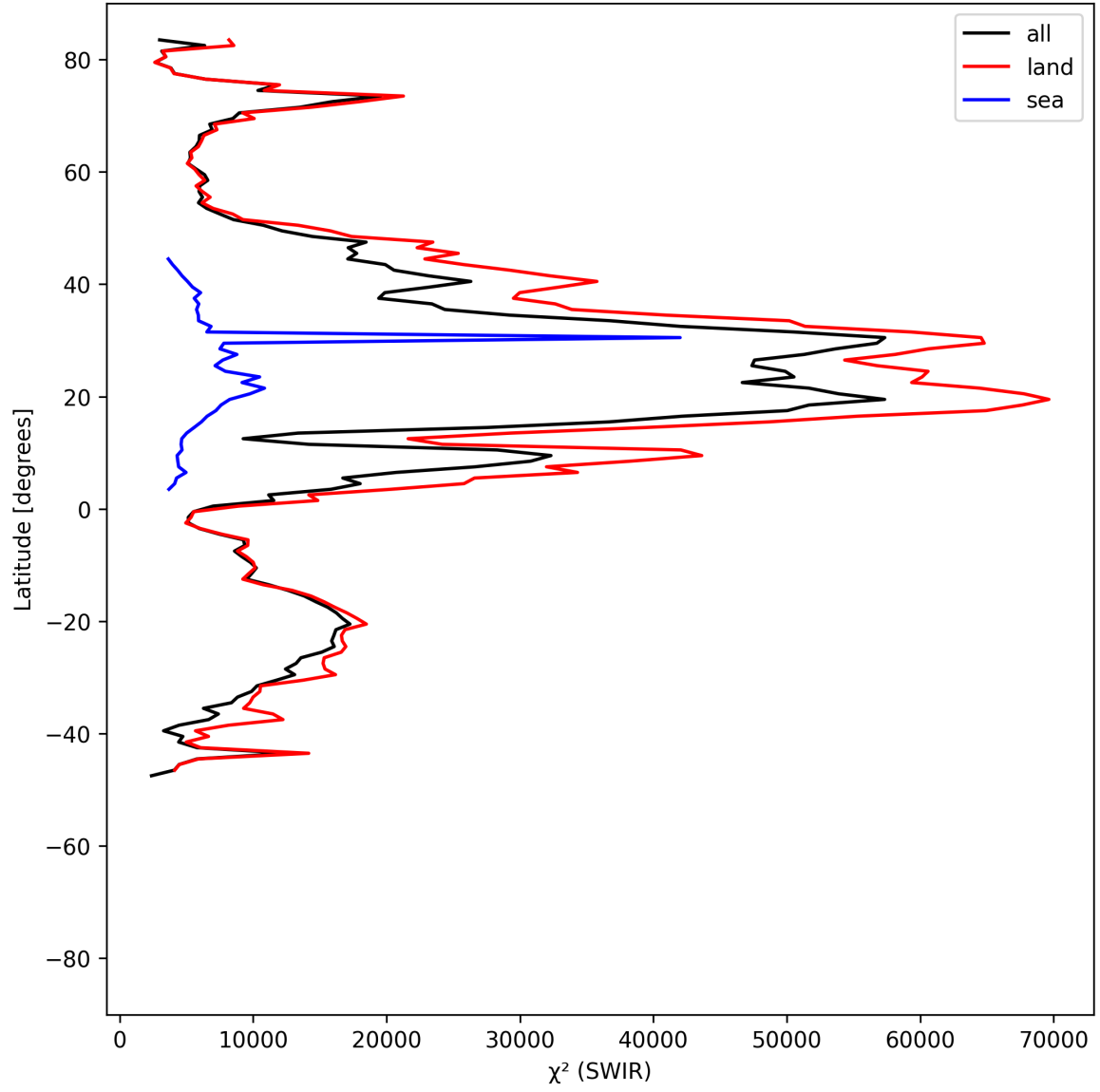
Figure 17: Zonal average of “ \chi^2 (SWIR)” for 2025-07-29 to 2025-07-31.
