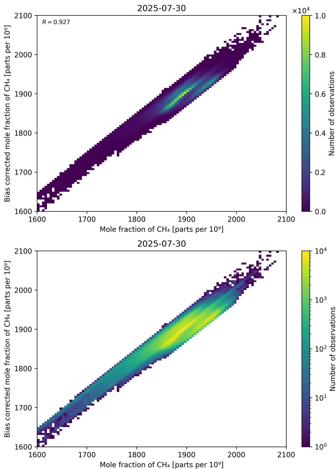
Figure 74: Scatter density plot of “Mole fraction of CH 4 ” against “Bias corrected mole fraction of CH 4 ” for 2025-07-29 to 2025-07-31.
