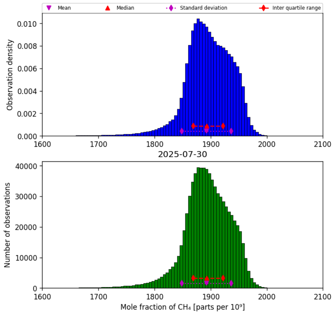
Figure 23: Histogram of “Mole fraction of CH 4 ” for 2025-07-29 to 2025-07-31
