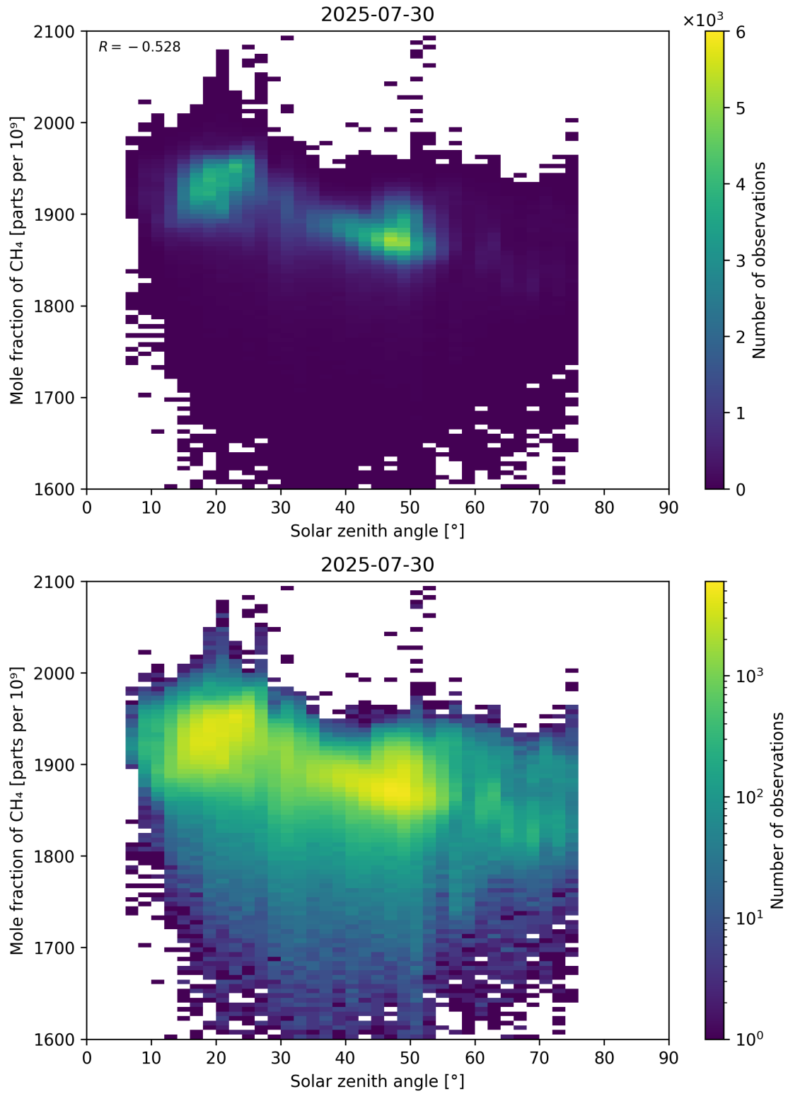
Figure 99: Scatter density plot of “Solar zenith angle” against “Mole fraction of CH 4 ” for 2025-07-29 to 2025-07-31.
