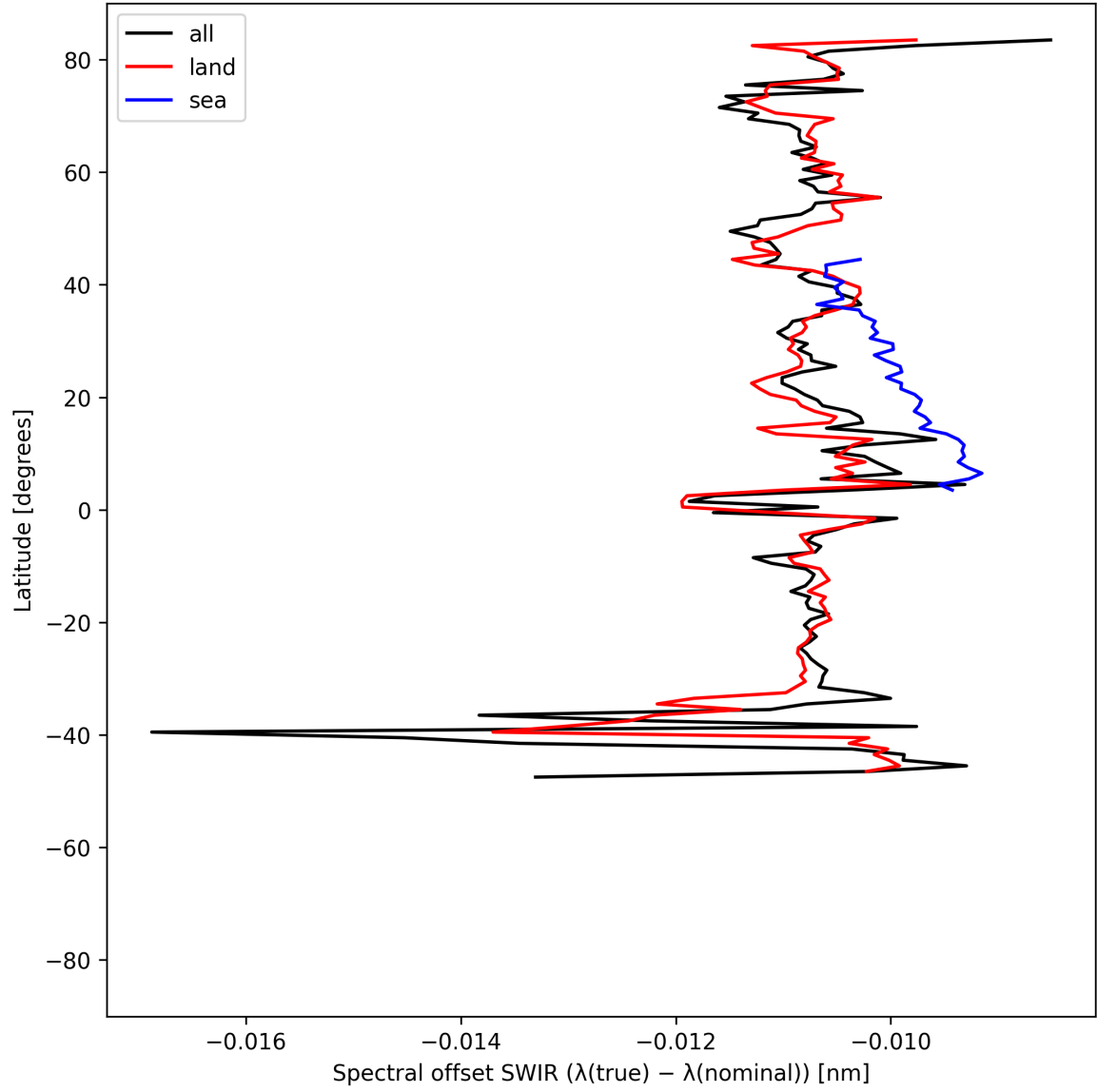
Figure 16: Zonal average of “Spectral offset SWIR ( \lambda_{\text{true}} - \lambda_{\text{nominal}} )” for 2025-07-29 to 2025-07-31.
