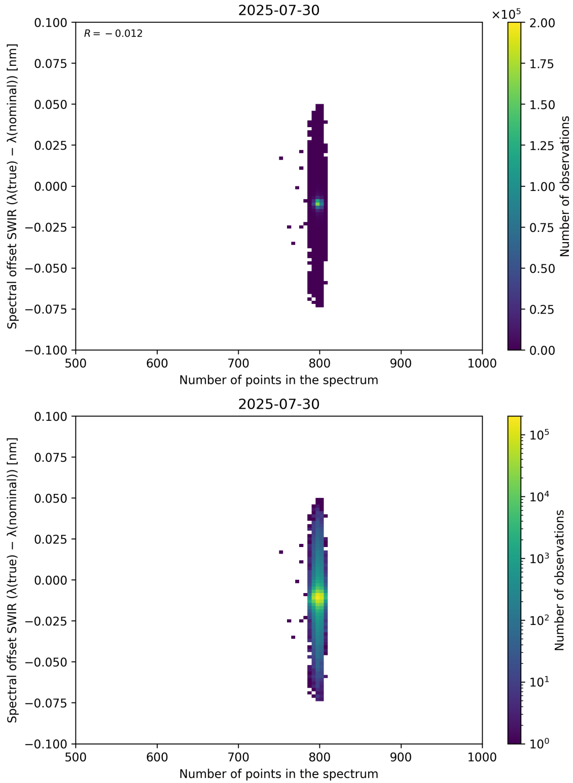
Figure 93: Scatter density plot of “Number of points in the spectrum” against “Spectral offset SWIR ( \lambda_{\text{true}} - \lambda_{\text{nominal}} )” for 2025-07-29 to 2025-07-31.
