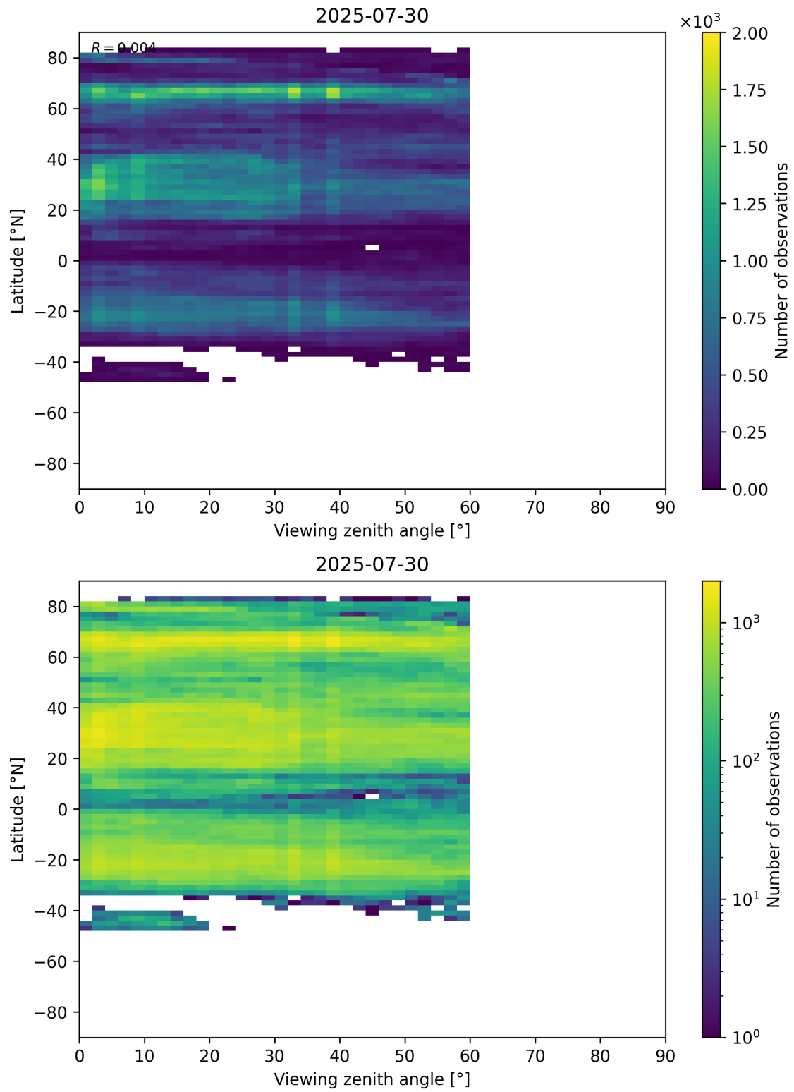
Figure 109: Scatter density plot of “Viewing zenith angle” against “Latitude” for 2025-07-29 to 2025-07-31.
