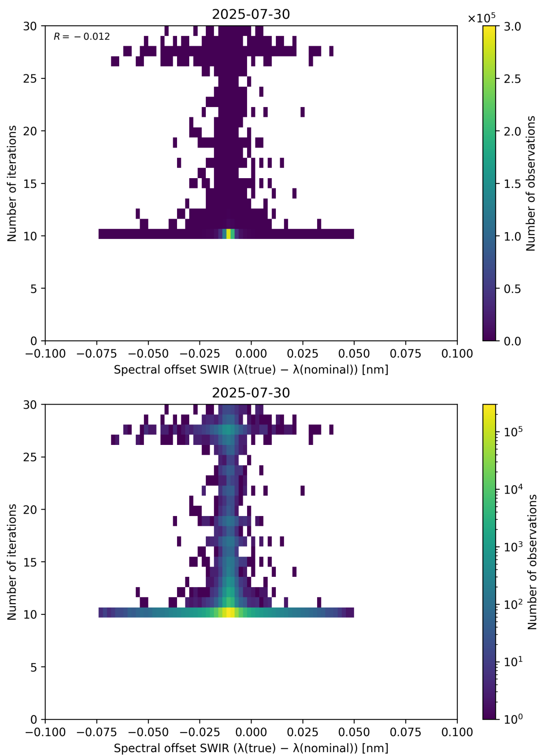
Figure 121: Scatter density plot of “Spectral offset SWIR ( \lambda_{\text{true}} - \lambda_{\text{nominal}} )” against “Number of iterations” for 2025-07-29 to 2025-07-31.
