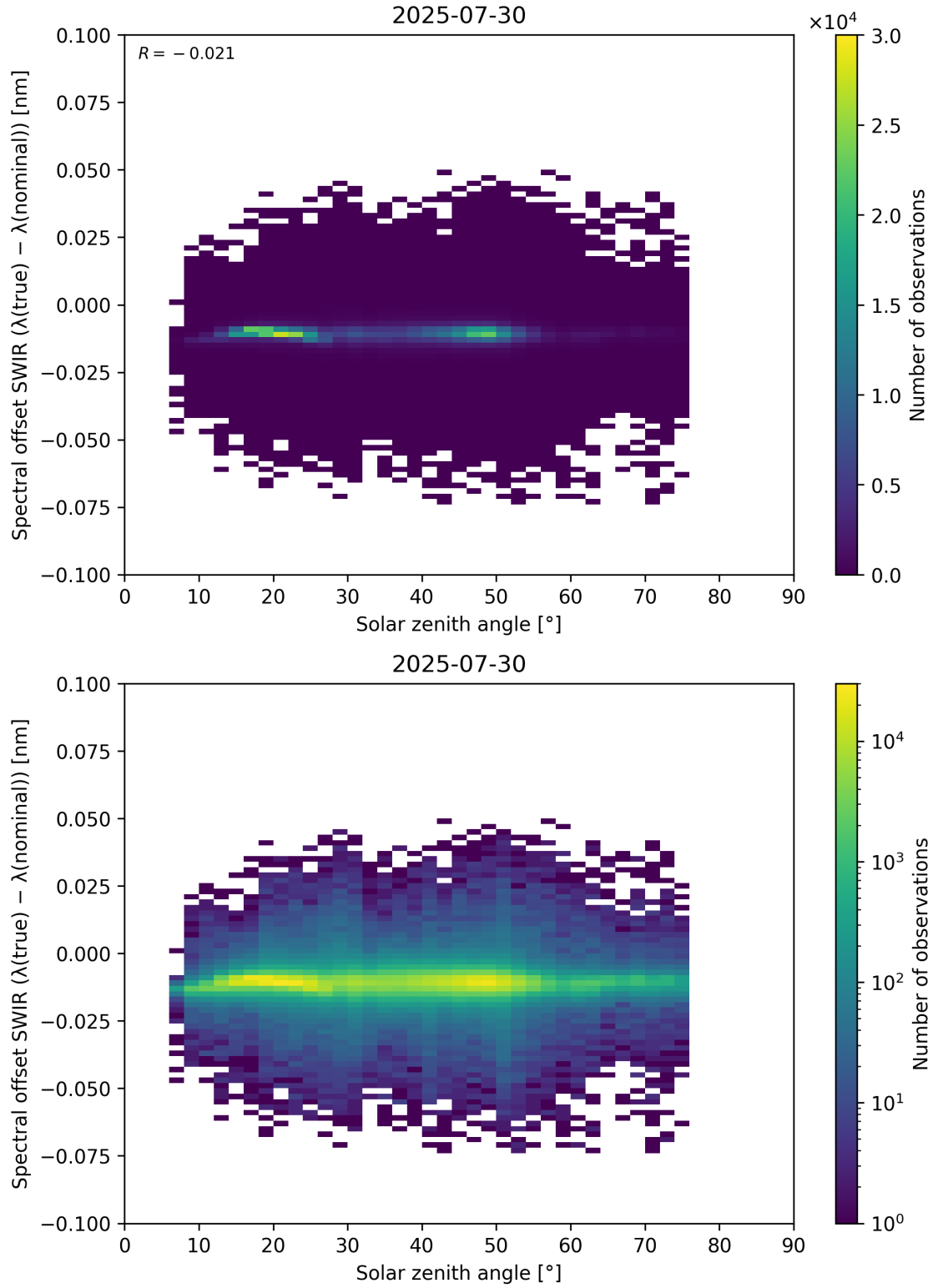
Figure 104: Scatter density plot of “Solar zenith angle” against “Spectral offset SWIR ( \lambda_{\text{true}} - \lambda_{\text{nominal}} )” for 2025-07-29 to 2025-07-31.
