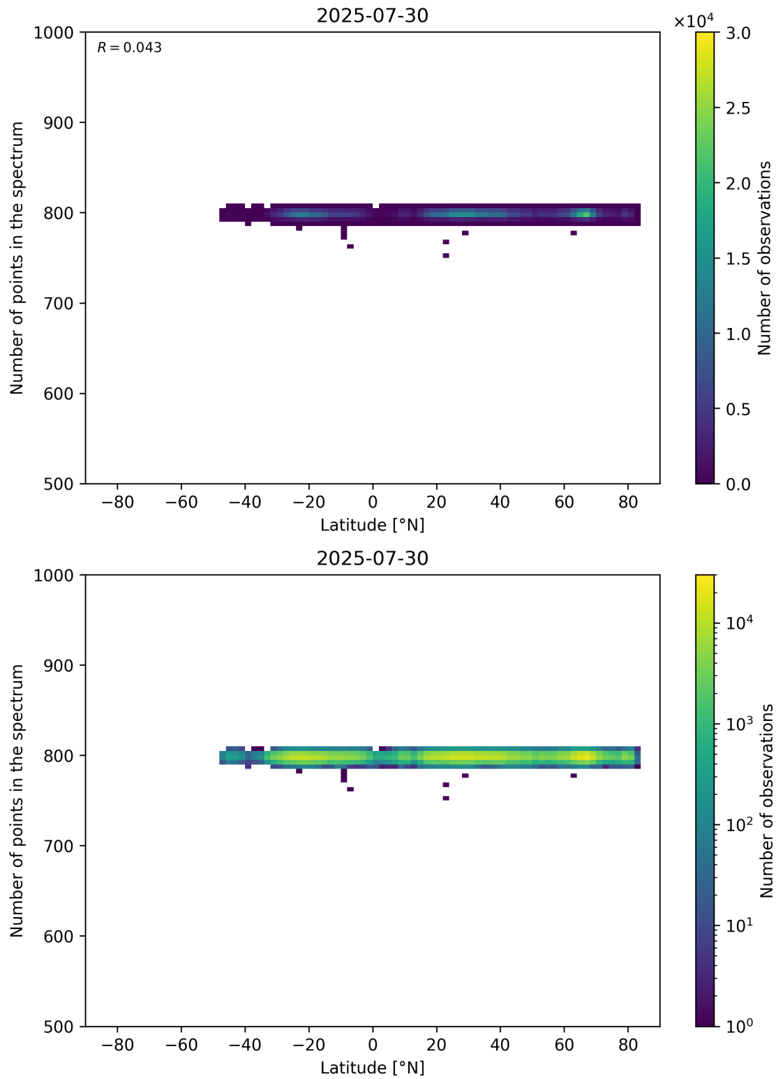
Figure 61: Scatter density plot of “Latitude” against “Number of points in the spectrum” for 2025-07-29 to 2025-07-31.
