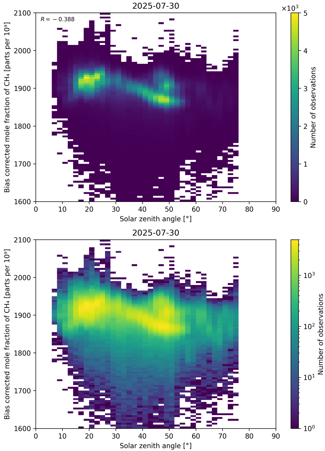
Figure 100: Scatter density plot of “Solar zenith angle” against “Bias corrected mole fraction of CH 4 ” for 2025-07-29 to 2025-07-31.
