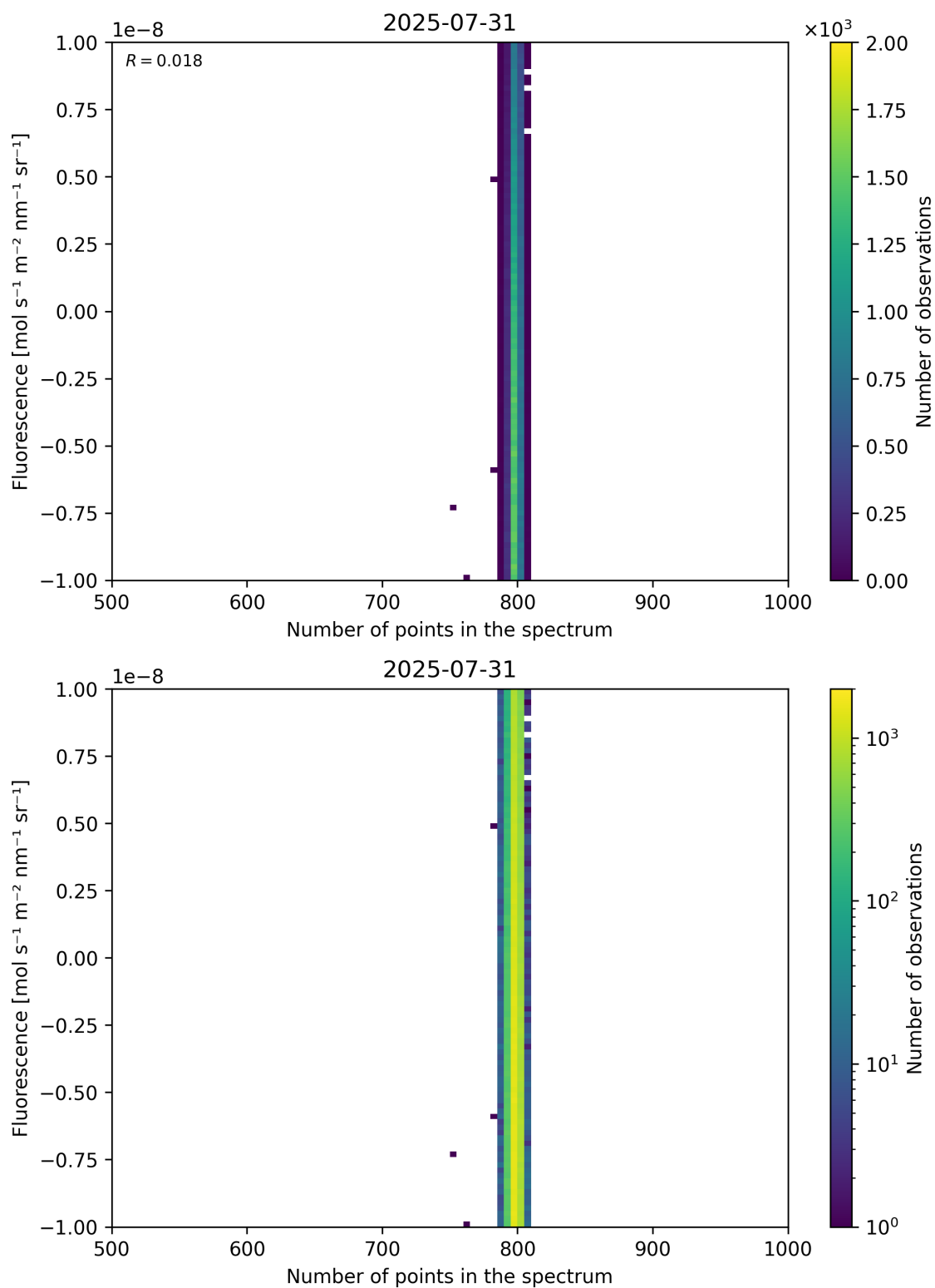
Figure 91: Scatter density plot of “Number of points in the spectrum” against “Fluorescence” for 2025-07-30 to 2025-08-01.
