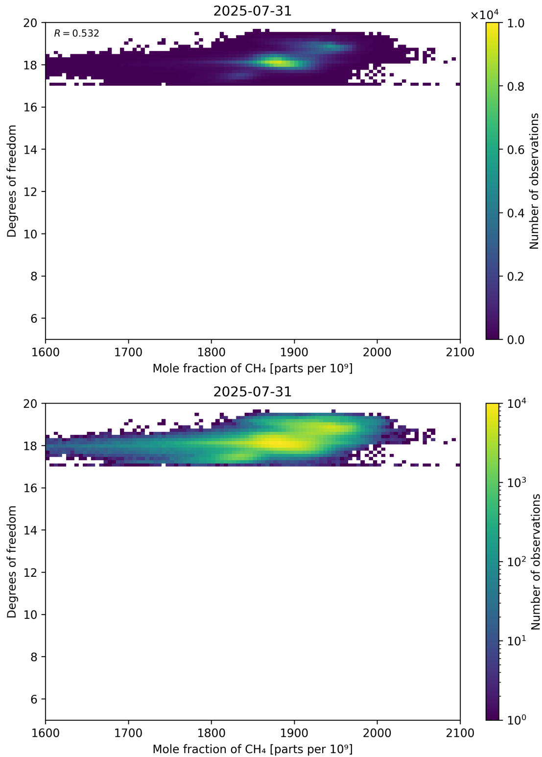
Figure 72: Scatter density plot of “Mole fraction of CH 4 ” against “Degrees of freedom” for 2025-07-30 to 2025-08-01.
