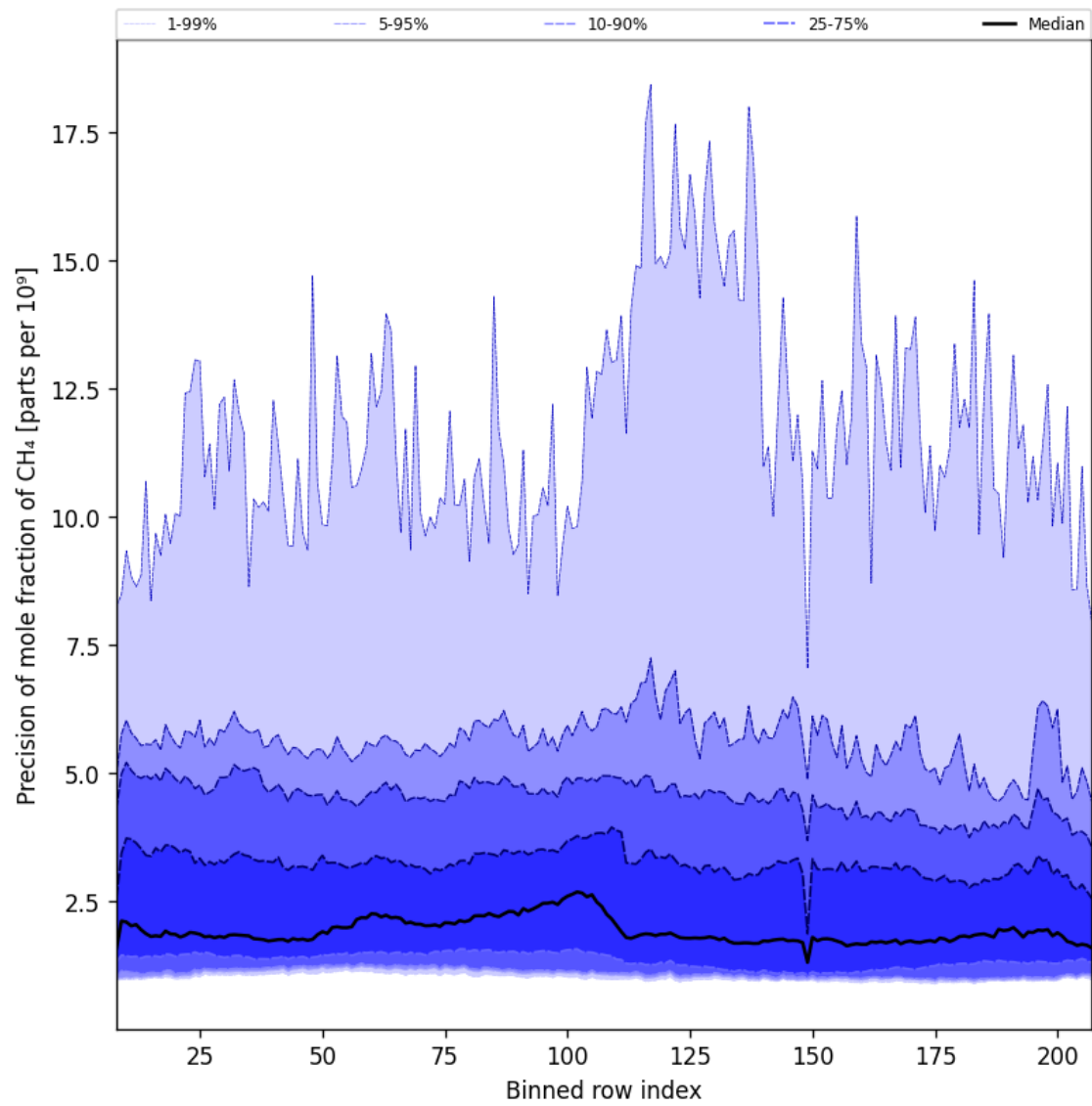
Figure 35: Along track statistics of “Precision of mole fraction of CH 4 ” for 2025-07-30 to 2025-08-01
