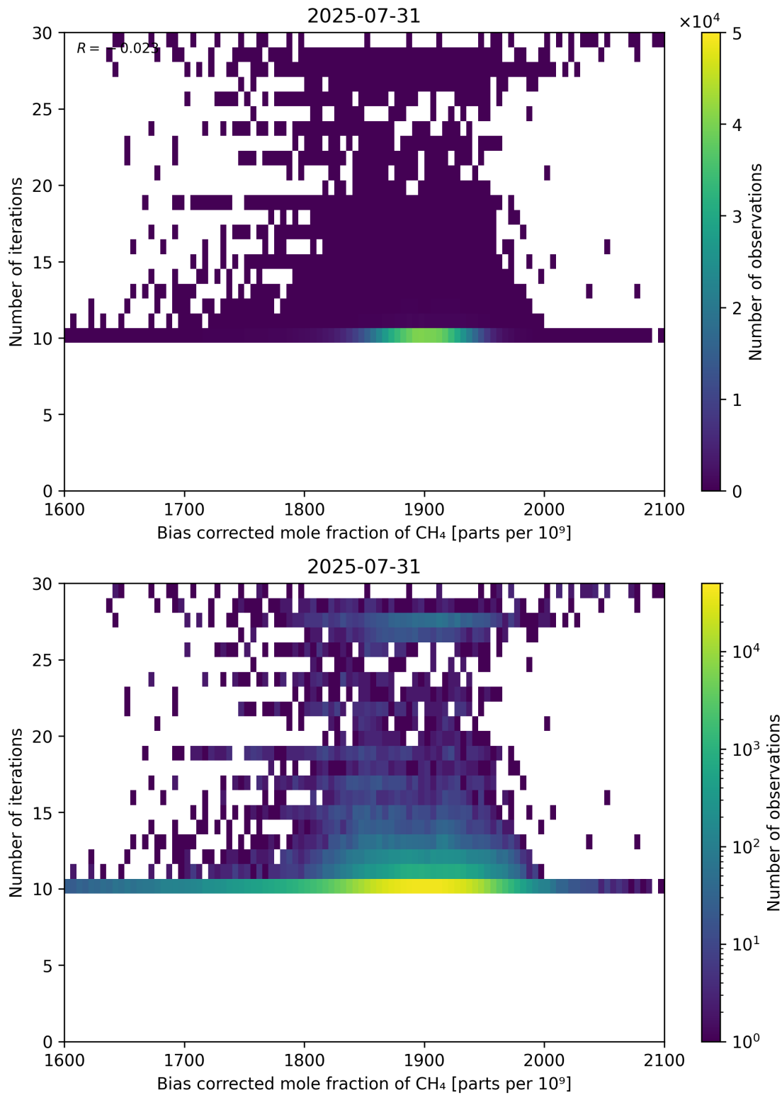
Figure 67: Scatter density plot of “Bias corrected mole fraction of CH 4 ” against “Number of iterations” for 2025-07-30 to 2025-08-01.
