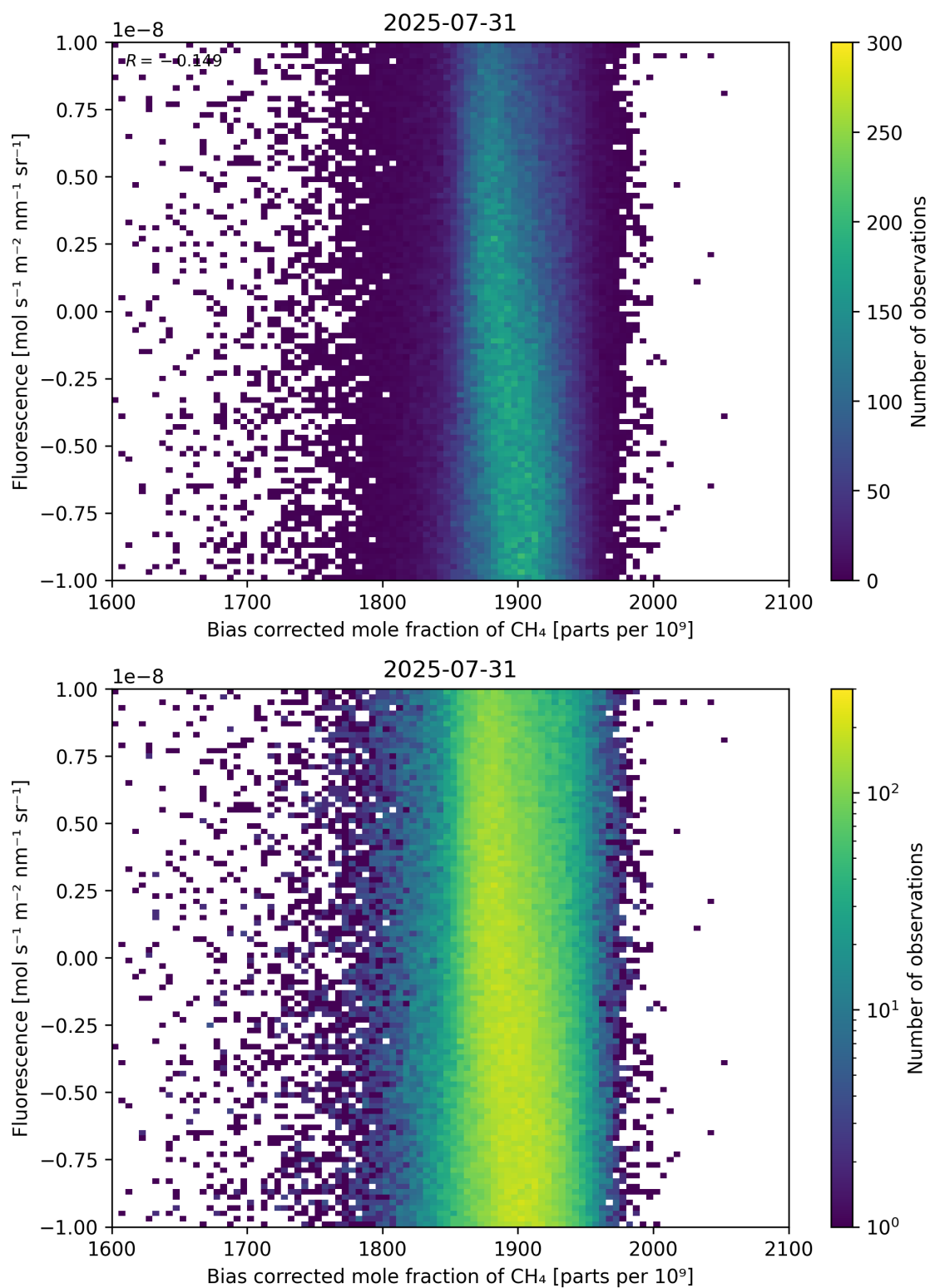
Figure 66: Scatter density plot of “Bias corrected mole fraction of \text{CH}_4 ” against “Fluorescence” for 2025-07-30 to 2025-08-01.
