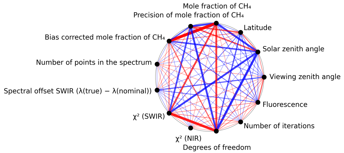
Figure 1: Map of correlation graph for 2025-07-30 to 2025-08-01.
