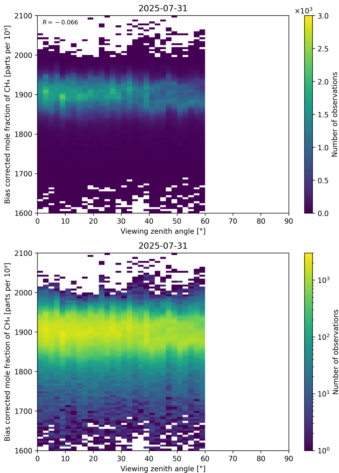
Figure 111: Scatter density plot of “Viewing zenith angle” against “Bias corrected mole fraction of CH 4 ” for 2025-07-30 to 2025-08-01.
