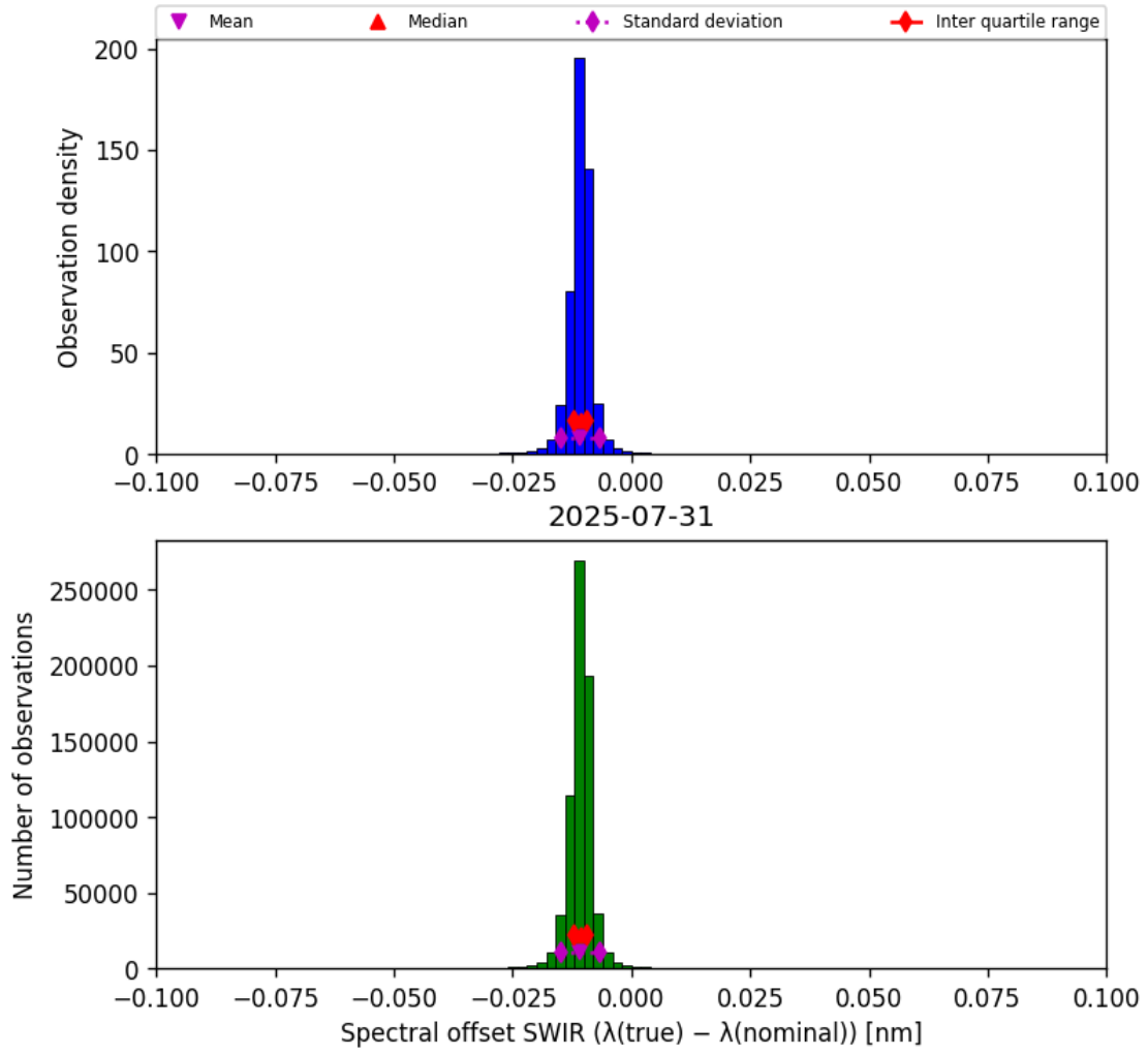
Figure 27: Histogram of “Spectral offset SWIR ( \lambda_{\text{true}} - \lambda_{\text{nominal}} )” for 2025-07-30 to 2025-08-01
