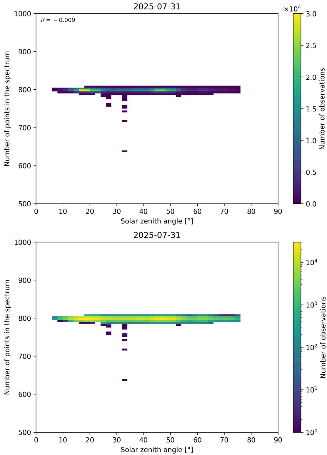
Figure 103: Scatter density plot of “Solar zenith angle” against “Number of points in the spectrum” for 2025-07-30 to 2025-08-01.
