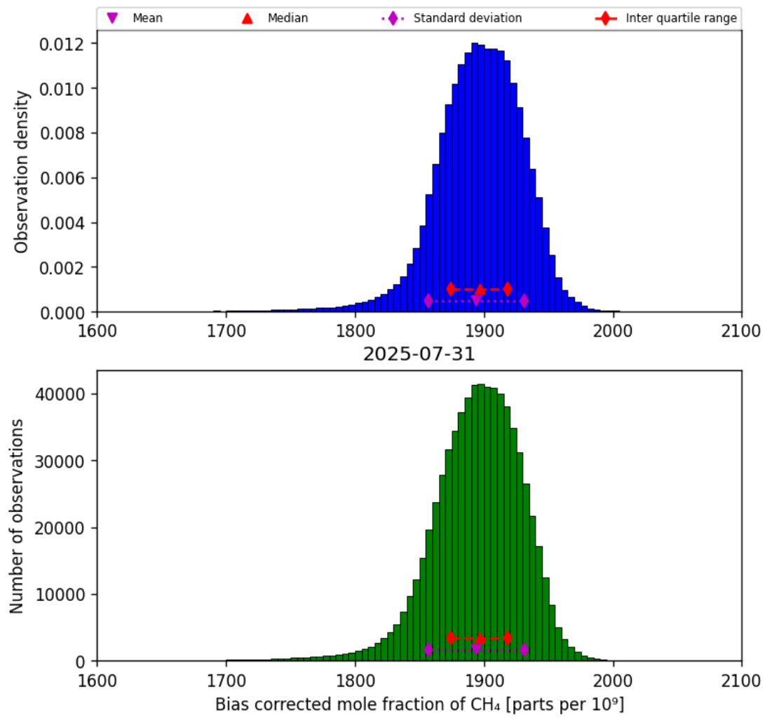
Figure 25: Histogram of “Bias corrected mole fraction of CH 4 ” for 2025-07-30 to 2025-08-01
