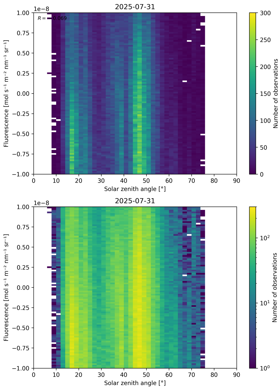
Figure 97: Scatter density plot of “Solar zenith angle” against “Fluorescence” for 2025-07-30 to 2025-08-01.
