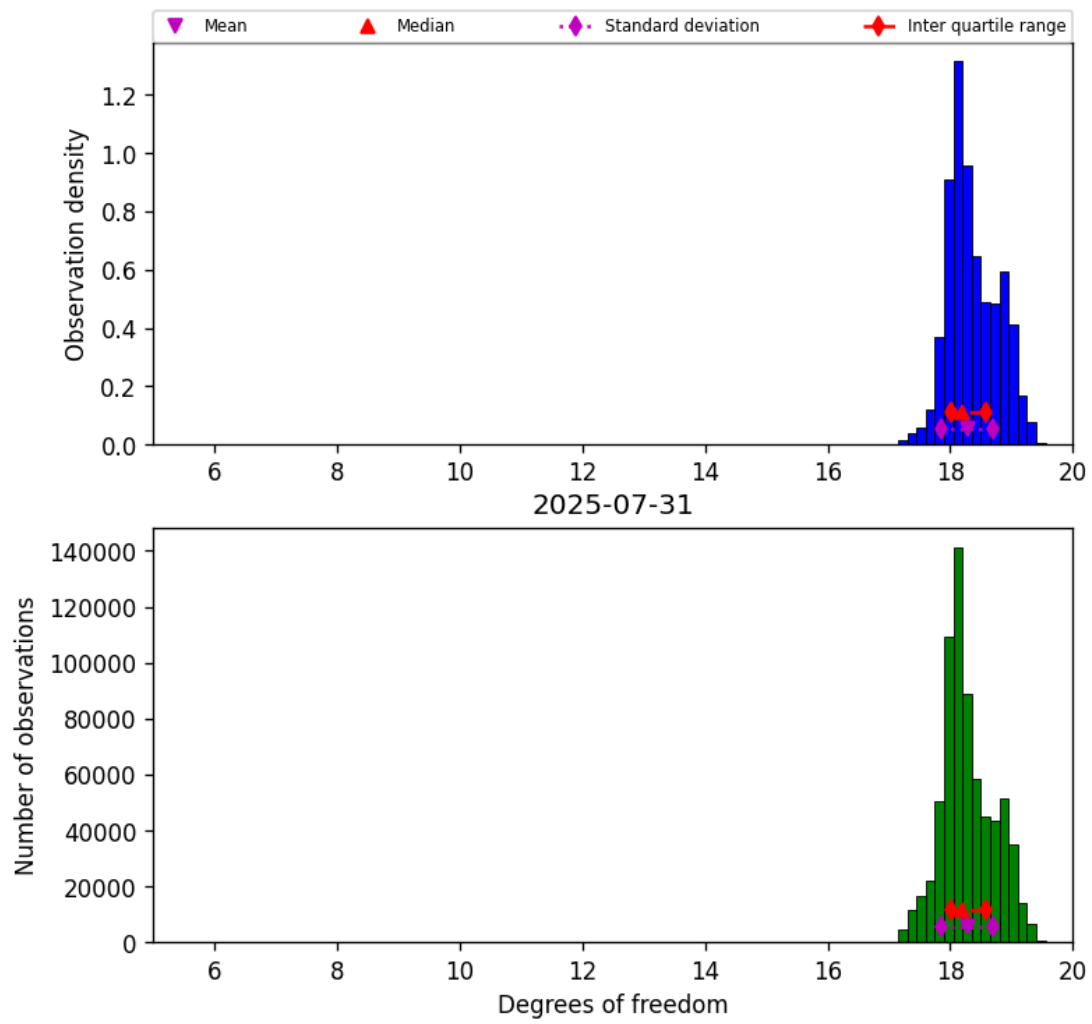
Figure 30: Histogram of “Degrees of freedom” for 2025-07-30 to 2025-08-01
