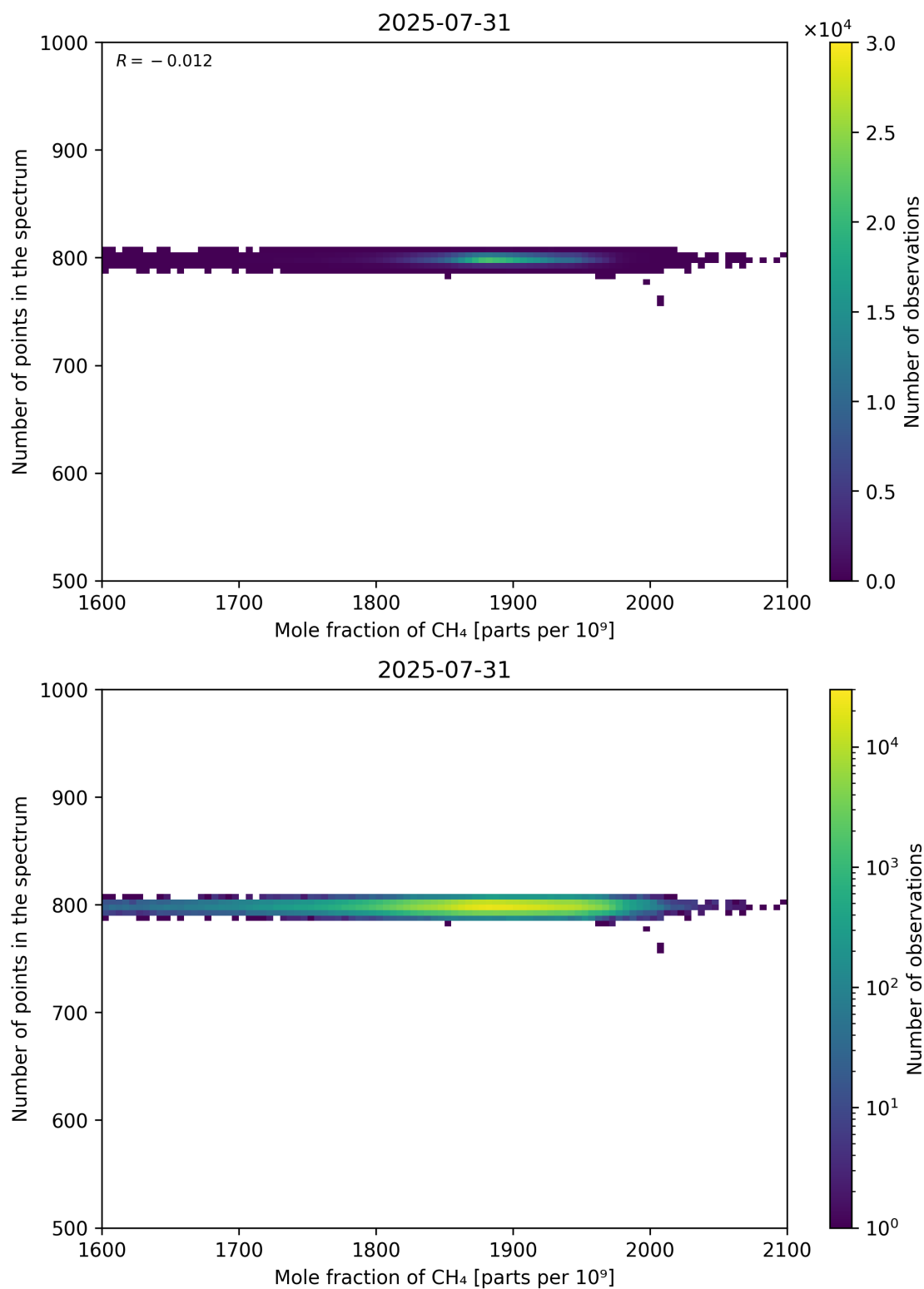
Figure 77: Scatter density plot of “Mole fraction of CH 4 ” against “Number of points in the spectrum” for 2025-07-30 to 2025-08-01.
