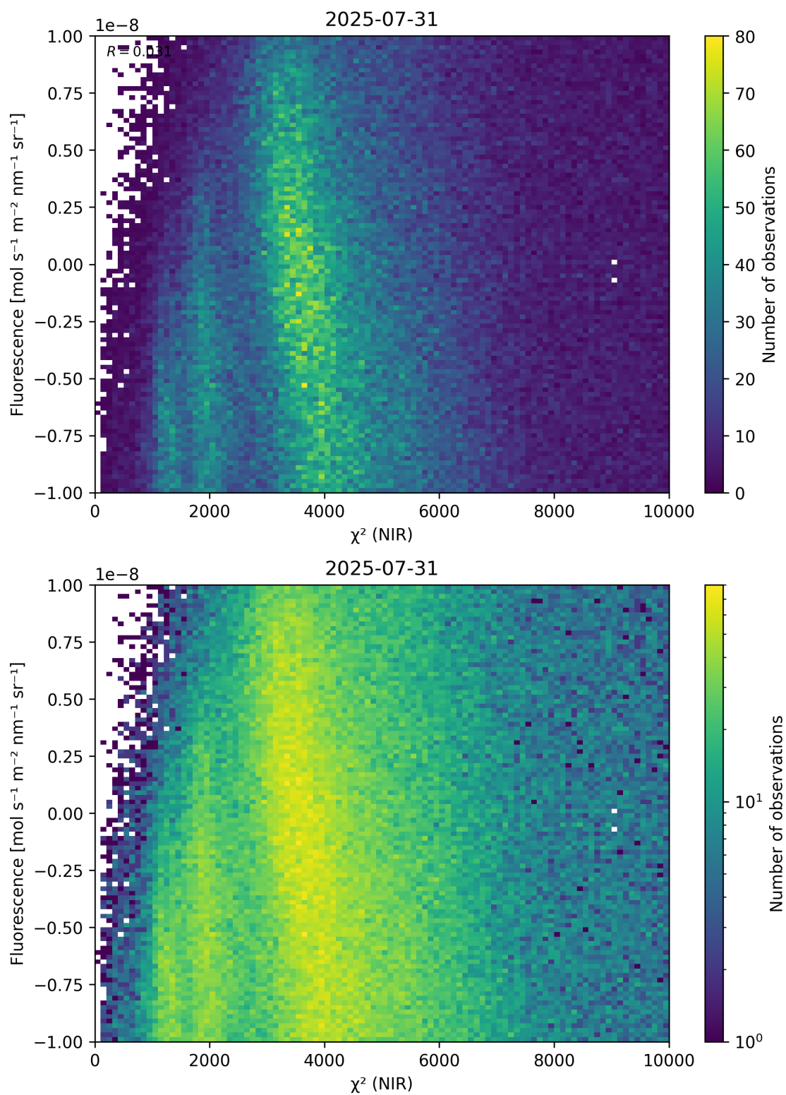
Figure 45: Scatter density plot of “ \chi^2 (NIR)” against “Fluorescence” for 2025-07-30 to 2025-08-01.
