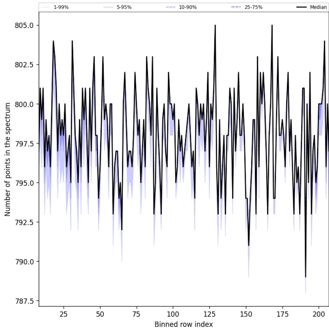
Figure 37: Along track statistics of “Number of points in the spectrum” for 2025-07-30 to 2025-08-01
