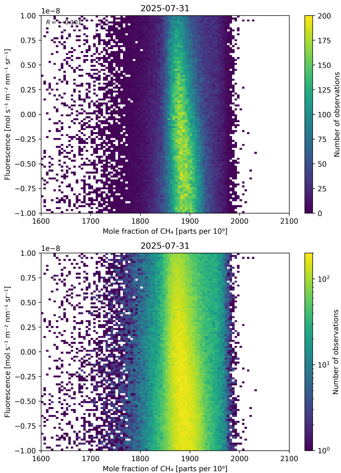
Figure 73: Scatter density plot of “Mole fraction of \text{CH}_4 ” against “Fluorescence” for 2025-07-30 to 2025-08-01.
