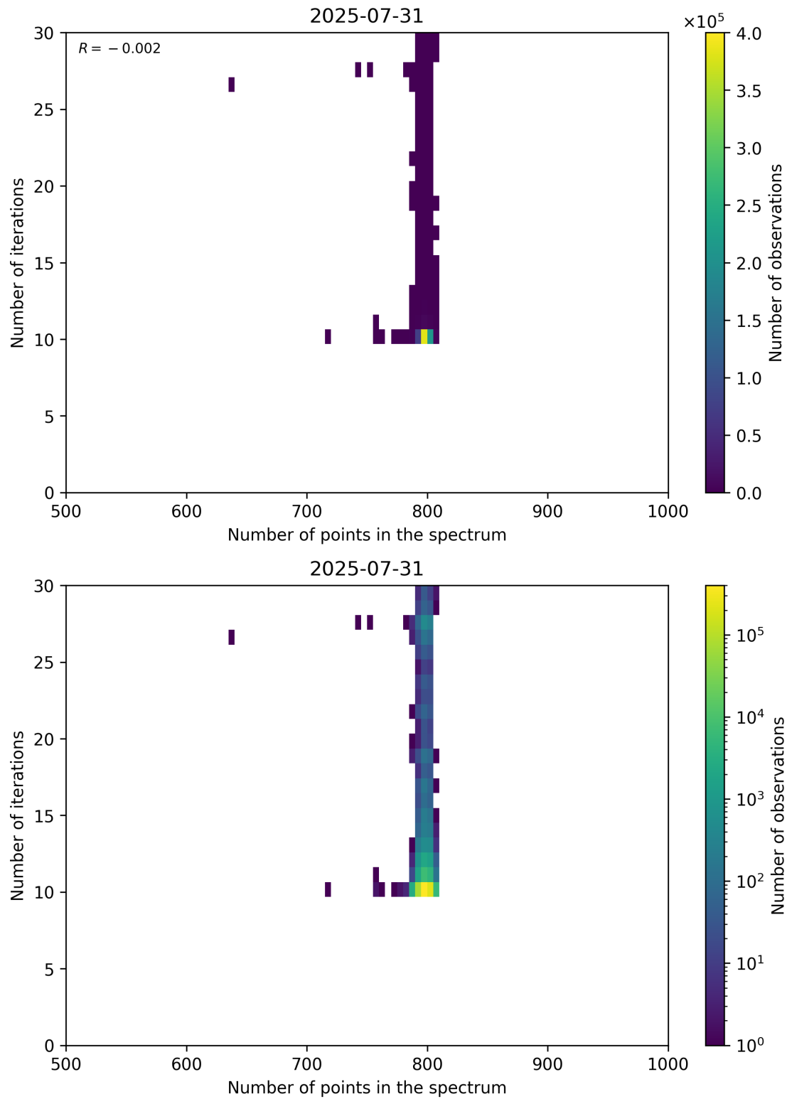
Figure 92: Scatter density plot of “Number of points in the spectrum” against “Number of iterations” for 2025-07-30 to 2025-08-01.
