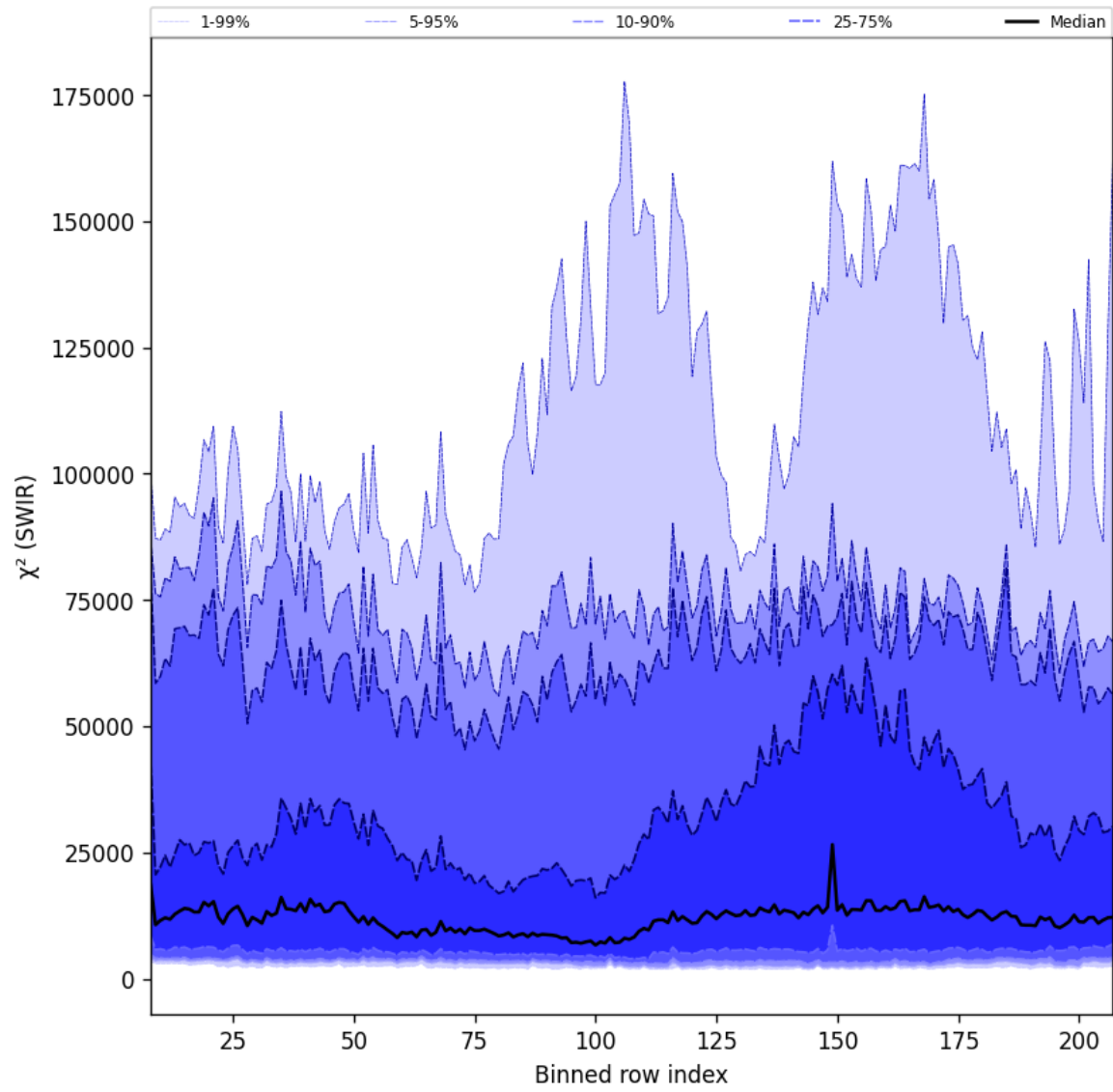
Figure 39: Along track statistics of “ \chi^2 (SWIR)” for 2025-07-30 to 2025-08-01
