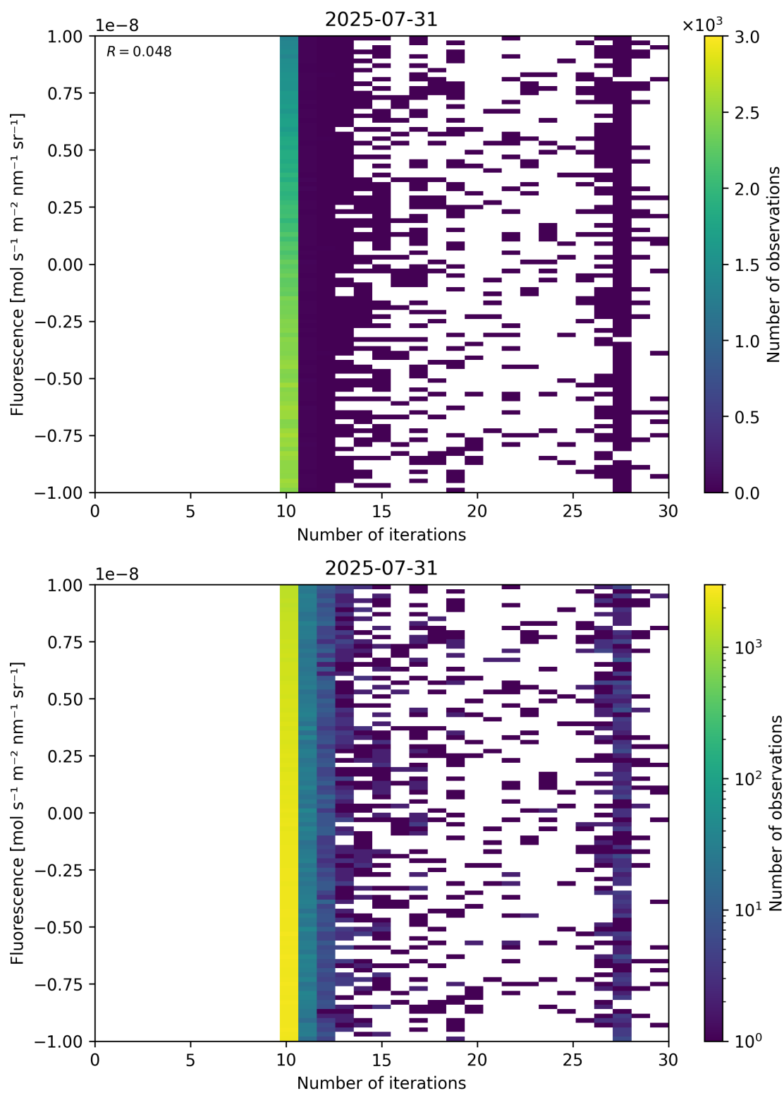
Figure 87: Scatter density plot of “Number of iterations” against “Fluorescence” for 2025-07-30 to 2025-08-01.
