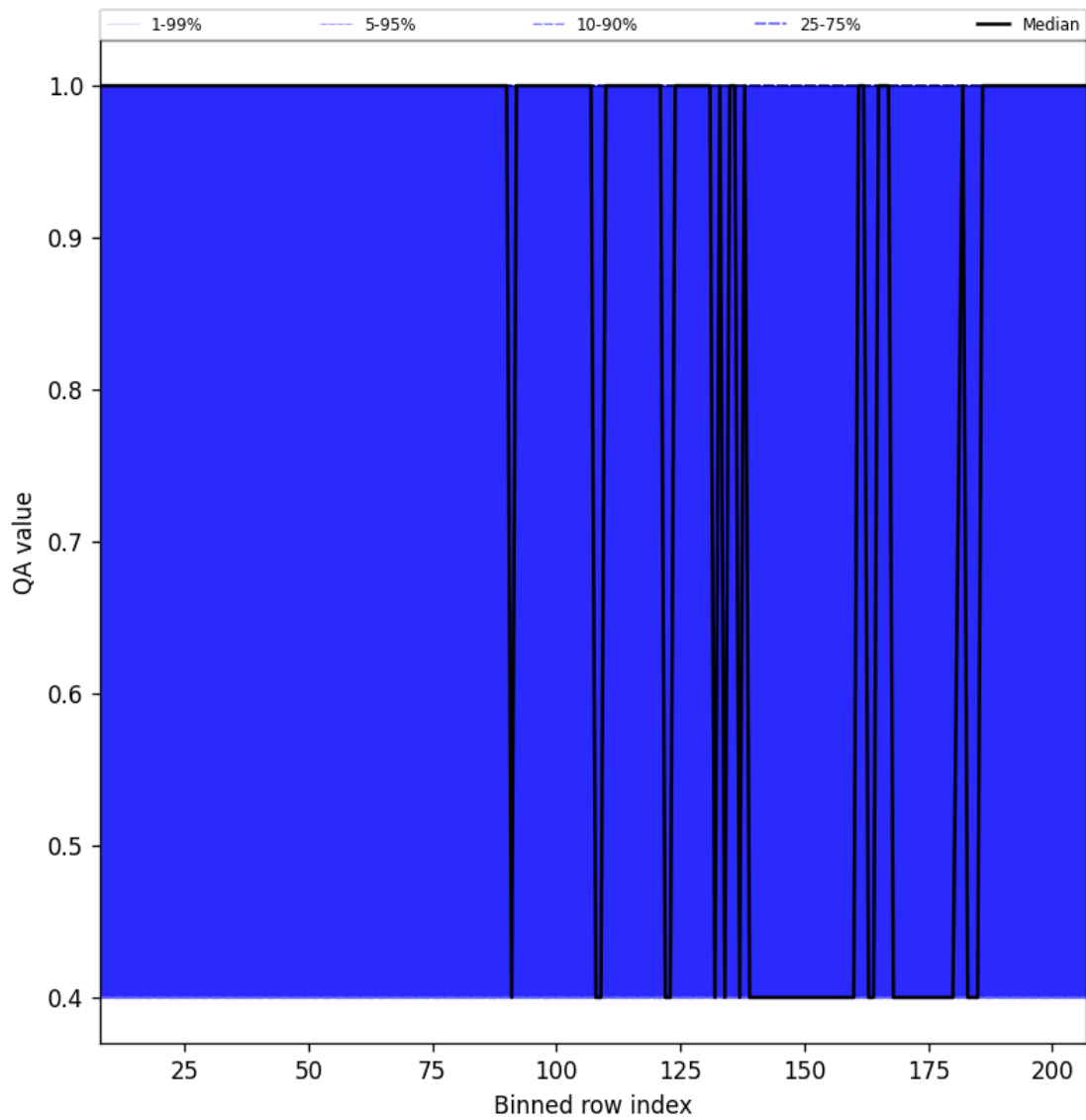
Figure 33: Along track statistics of “QA value” for 2025-07-30 to 2025-08-01
