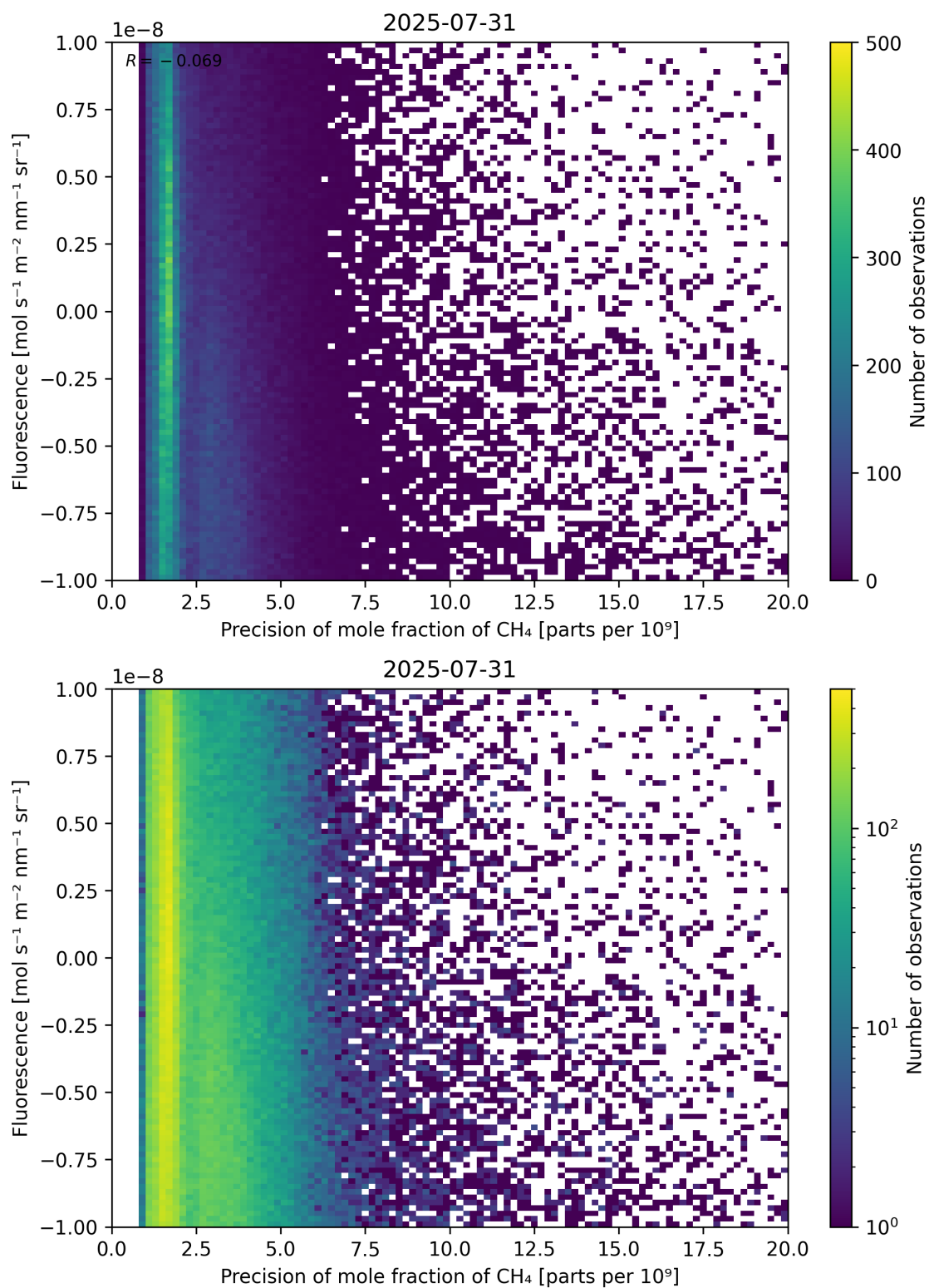
Figure 81: Scatter density plot of “Precision of mole fraction of CH 4 ” against “Fluorescence” for 2025-07-30 to 2025-08-01.
