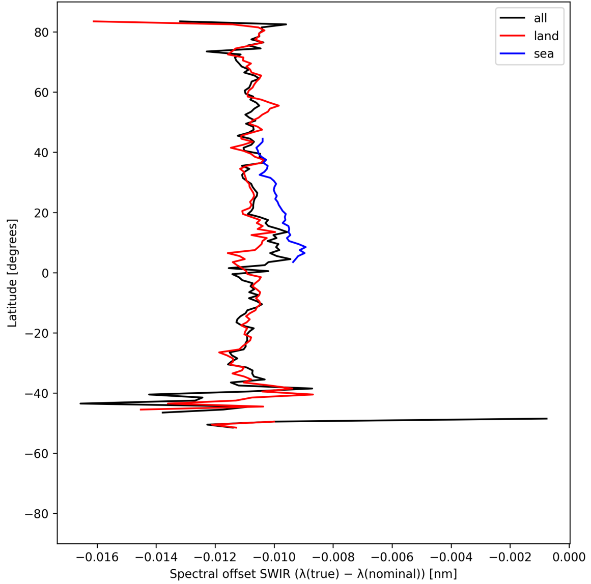
Figure 16: Zonal average of “Spectral offset SWIR ( \lambda_{\text{true}} - \lambda_{\text{nominal}} )” for 2025-07-30 to 2025-08-01.
