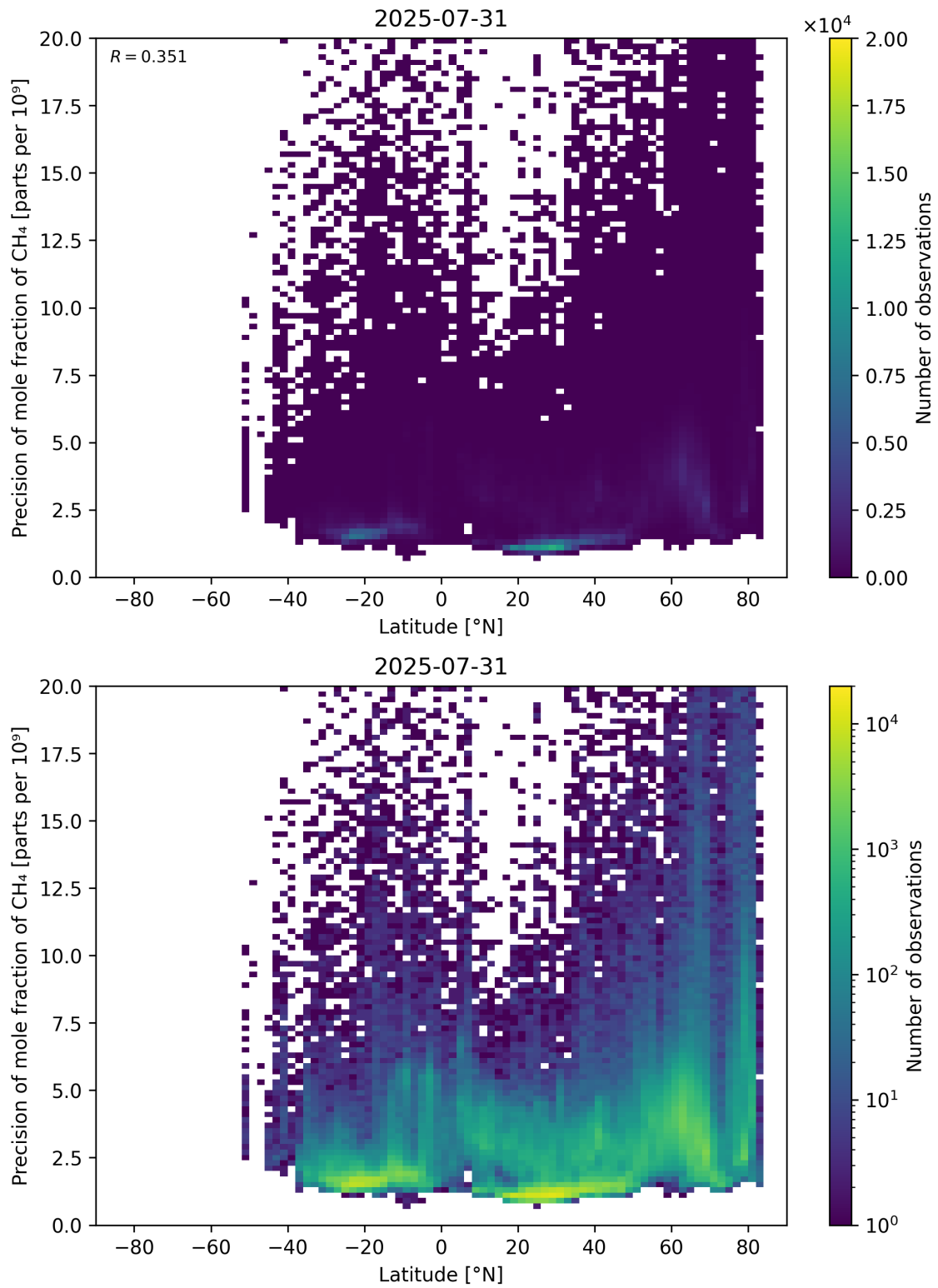
Figure 59: Scatter density plot of “Latitude” against “Precision of mole fraction of \text{CH}_4 ” for 2025-07-30 to 2025-08-01.
