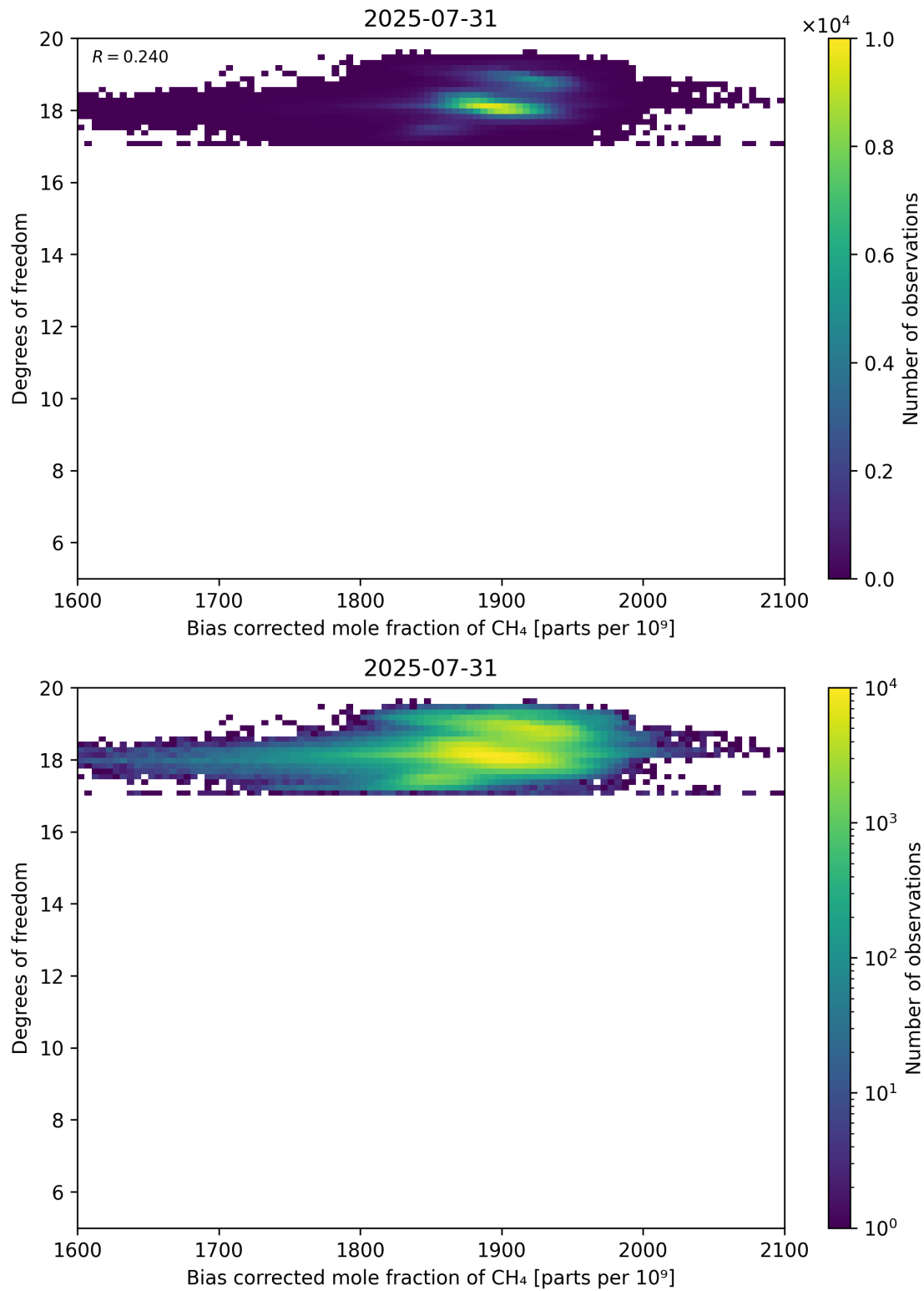
Figure 65: Scatter density plot of “Bias corrected mole fraction of CH 4 ” against “Degrees of freedom” for 2025-07-30 to 2025-08-01.
