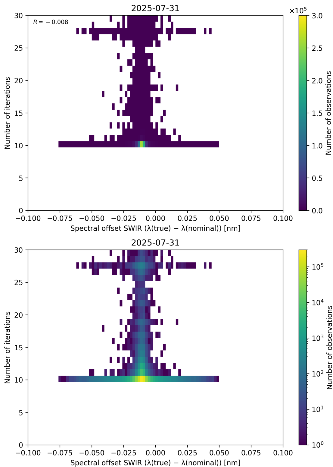
Figure 121: Scatter density plot of “Spectral offset SWIR ( \lambda_{\text{true}} - \lambda_{\text{nominal}} )” against “Number of iterations” for 2025-07-30 to 2025-08-01.
