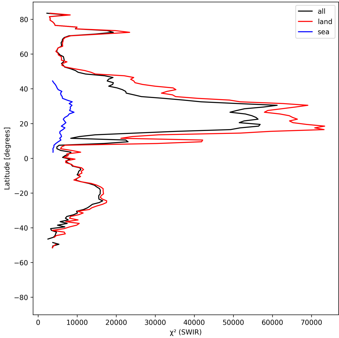
Figure 17: Zonal average of “ \chi^2 (SWIR)” for 2025-07-30 to 2025-08-01.
