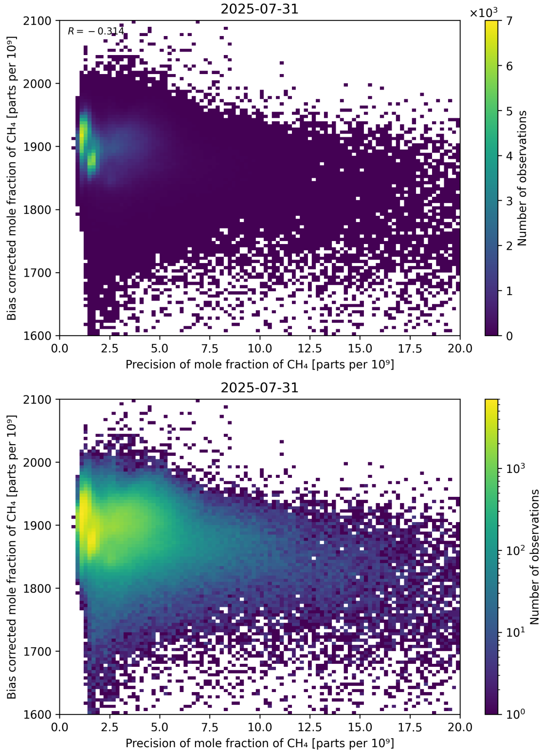
Figure 82: Scatter density plot of “Precision of mole fraction of CH 4 ” against “Bias corrected mole fraction of CH 4 ” for 2025-07-30 to 2025-08-01.
