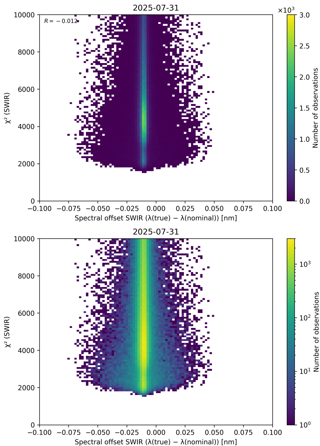
Figure 118: Scatter density plot of “Spectral offset SWIR ( \lambda_{\text{true}} - \lambda_{\text{nominal}} )” against “ \chi^2 (SWIR)” for 2025-07-30 to 2025-08-01.
