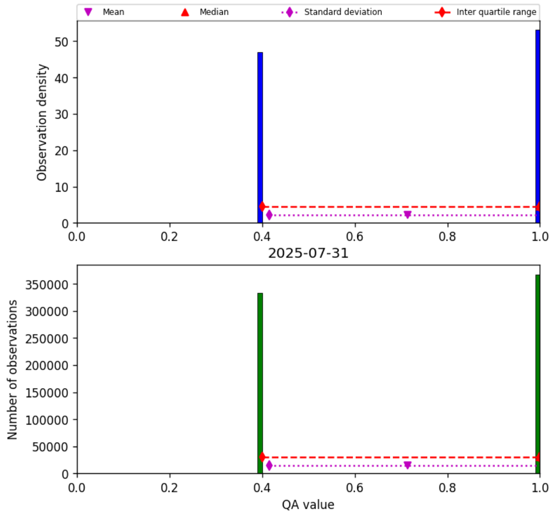
Figure 22: Histogram of “QA value” for 2025-07-30 to 2025-08-01
