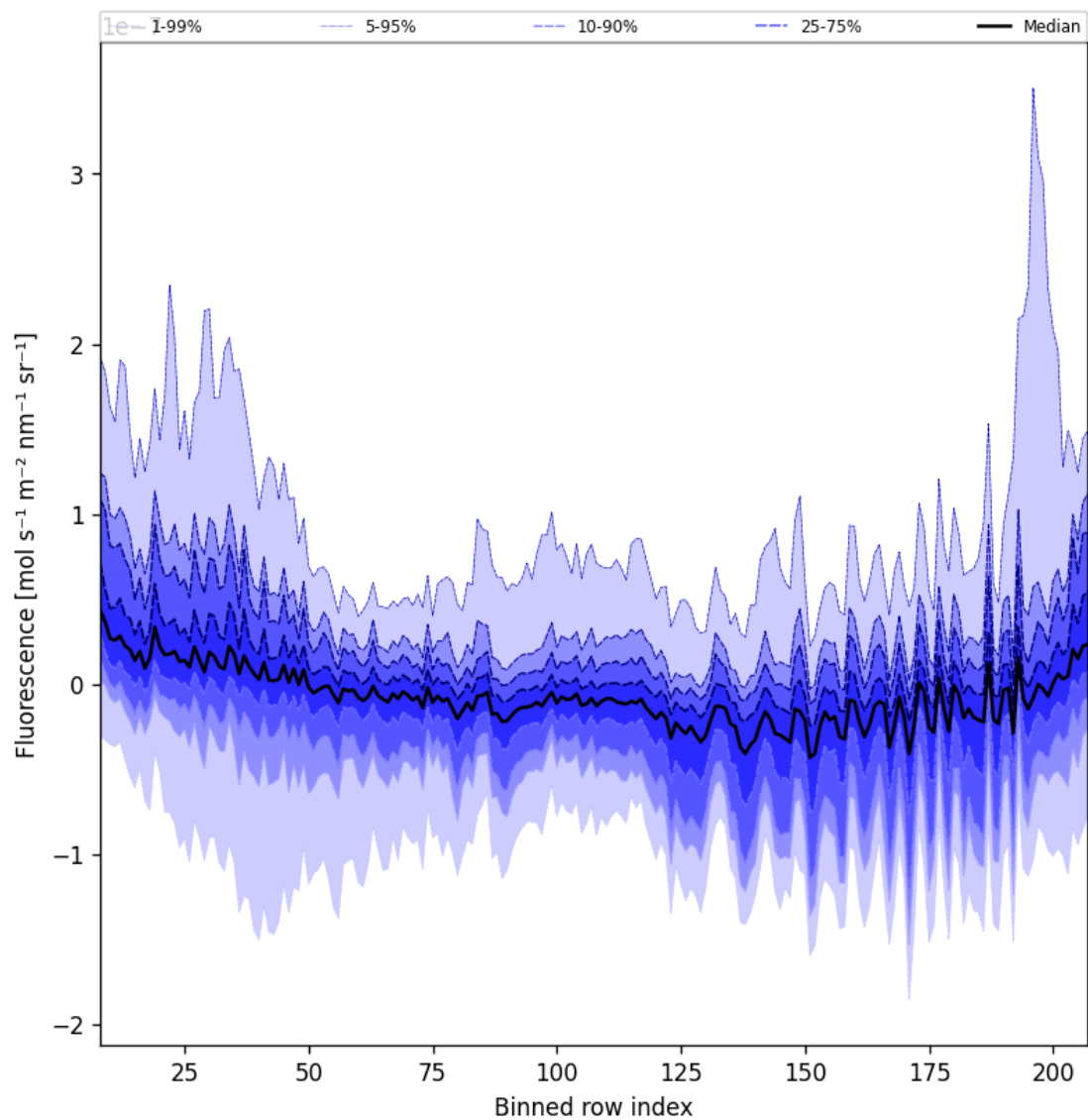
Figure 43: Along track statistics of “Fluorescence” for 2025-07-30 to 2025-08-01
