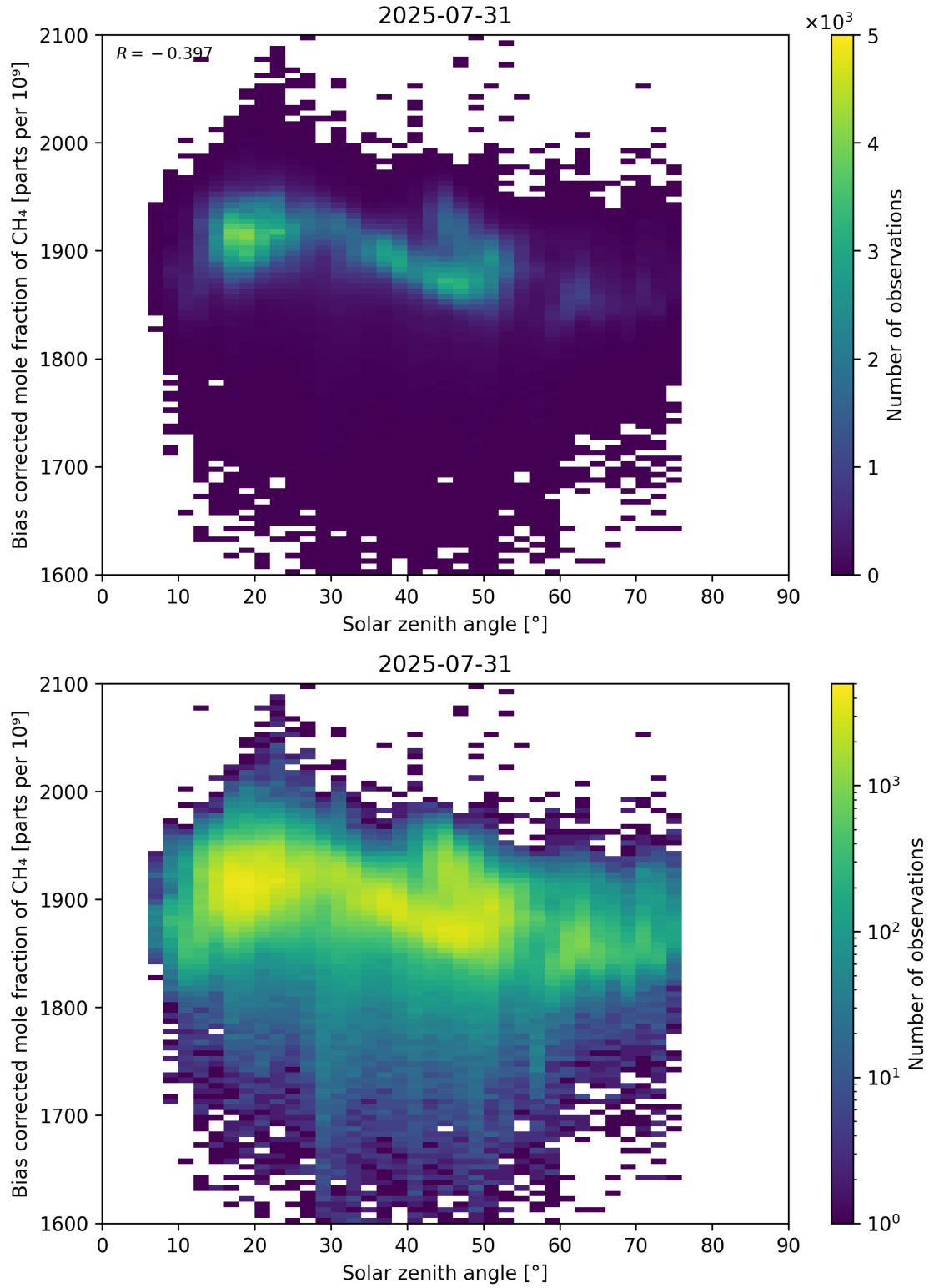
Figure 100: Scatter density plot of “Solar zenith angle” against “Bias corrected mole fraction of CH 4 ” for 2025-07-30 to 2025-08-01.
