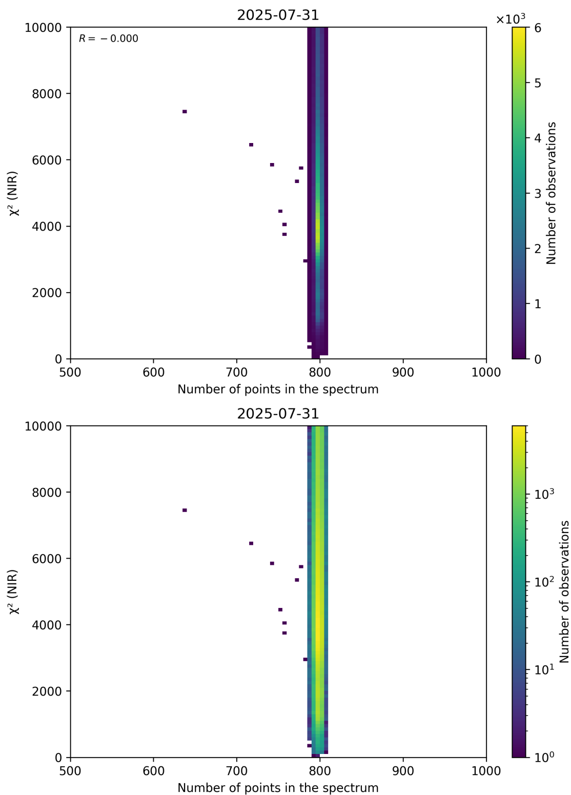
Figure 88: Scatter density plot of “Number of points in the spectrum” against “ \chi^2 (NIR)” for 2025-07-30 to 2025-08-01.
