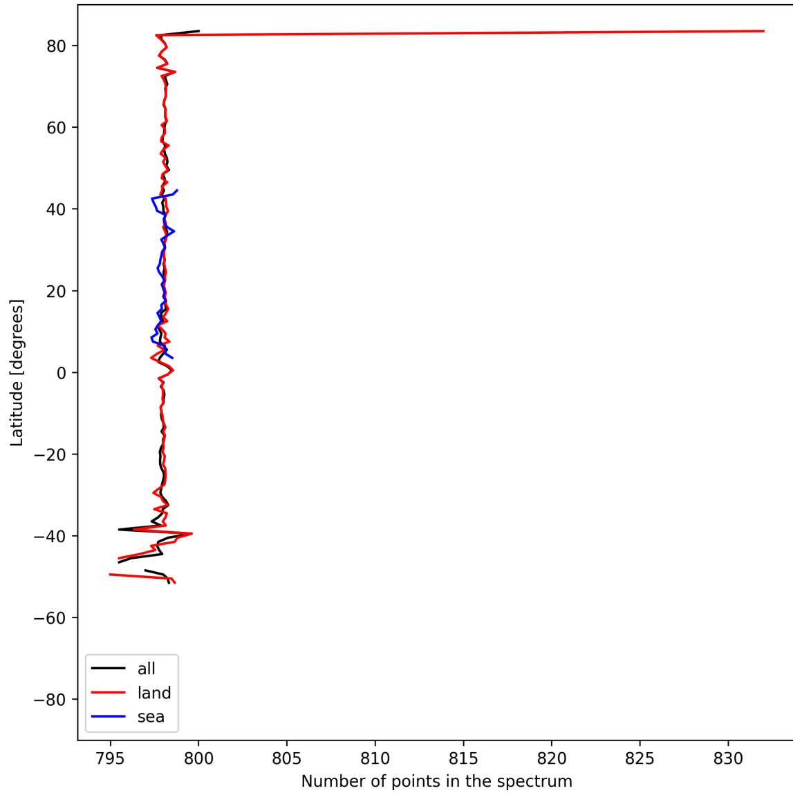
Figure 15: Zonal average of “Number of points in the spectrum” for 2025-07-30 to 2025-08-01.
