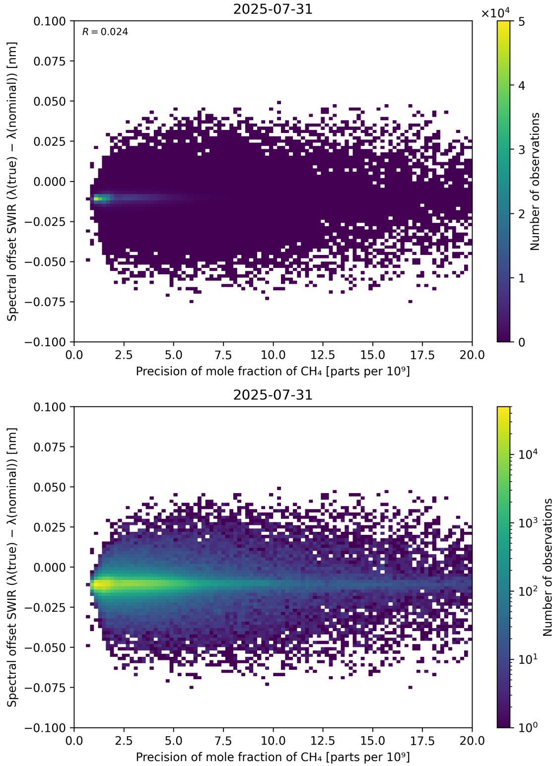
Figure 85: Scatter density plot of “Precision of mole fraction of CH 4 ” against “Spectral offset SWIR ( \lambda_{\text{true}} - \lambda_{\text{nominal}} )” for 2025-07-30 to 2025-08-01.
