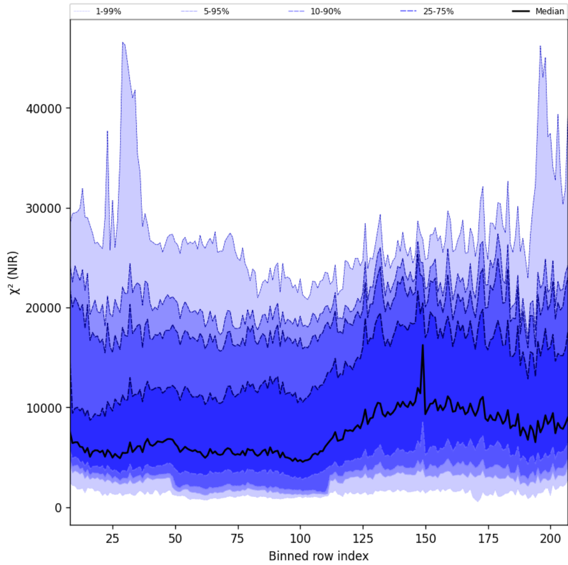
Figure 40: Along track statistics of “ \chi^2 (NIR)” for 2025-07-30 to 2025-08-01
