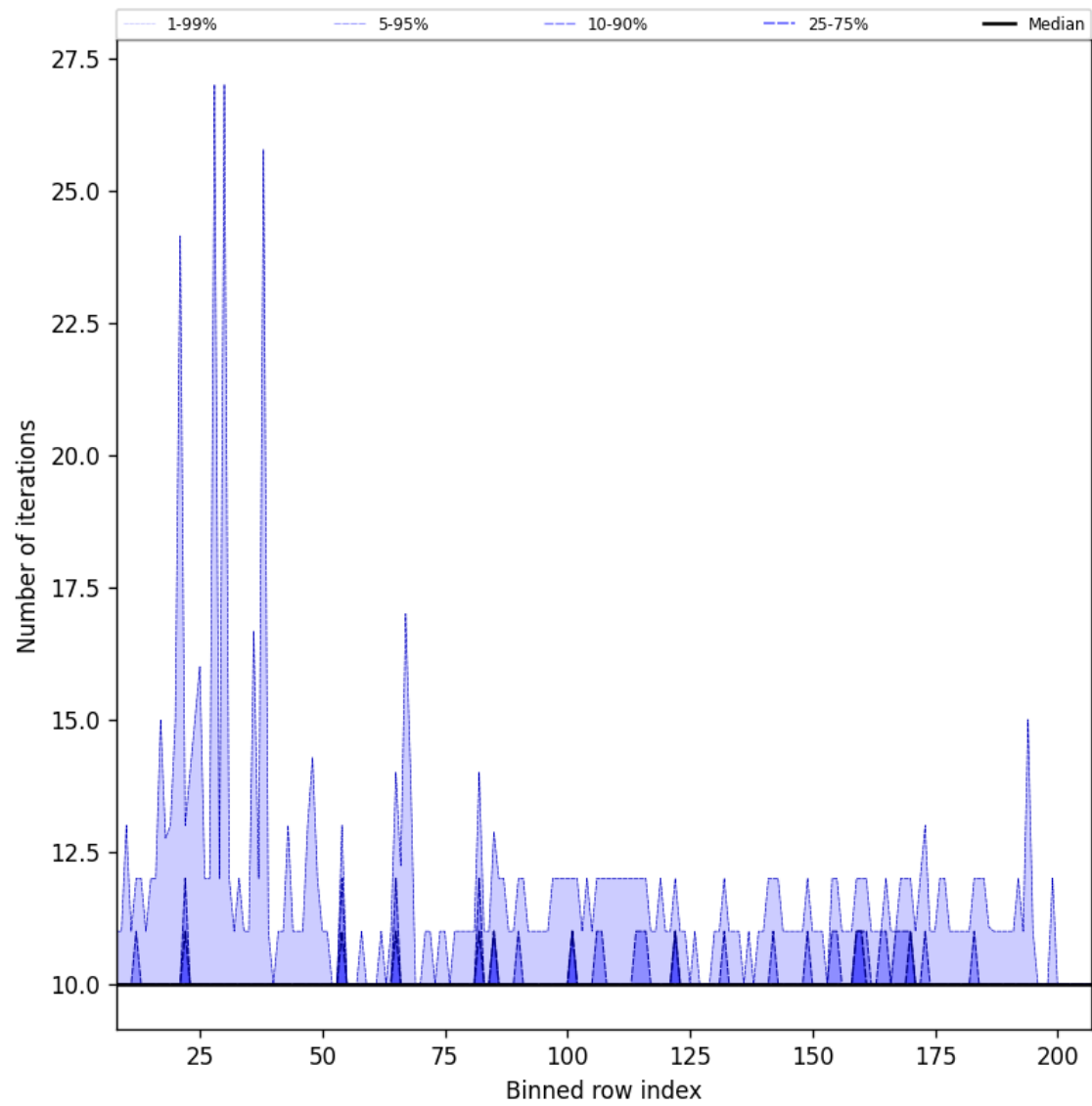
Figure 42: Along track statistics of “Number of iterations” for 2025-07-30 to 2025-08-01
