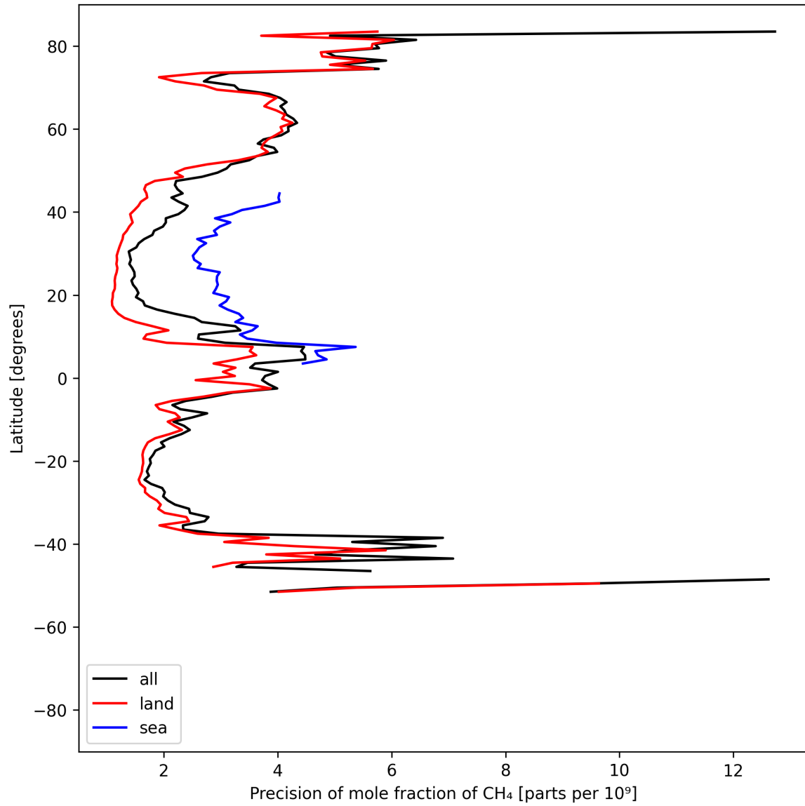
Figure 13: Zonal average of “Precision of mole fraction of CH 4 ” for 2025-07-30 to 2025-08-01.
