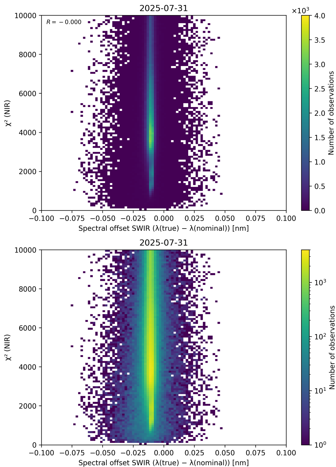
Figure 117: Scatter density plot of “Spectral offset SWIR ( \lambda_{\text{true}} - \lambda_{\text{nominal}} )” against “ \chi^2 (NIR)” for 2025-07-30 to 2025-08-01.
