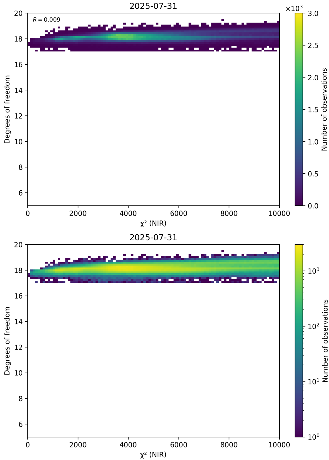
Figure 44: Scatter density plot of “ \chi^2 (NIR)” against “Degrees of freedom” for 2025-07-30 to 2025-08-01.
