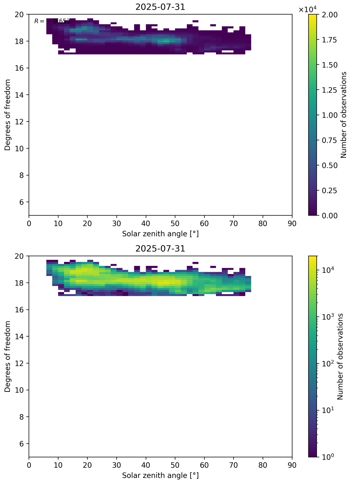
Figure 96: Scatter density plot of “Solar zenith angle” against “Degrees of freedom” for 2025-07-30 to 2025-08-01.
