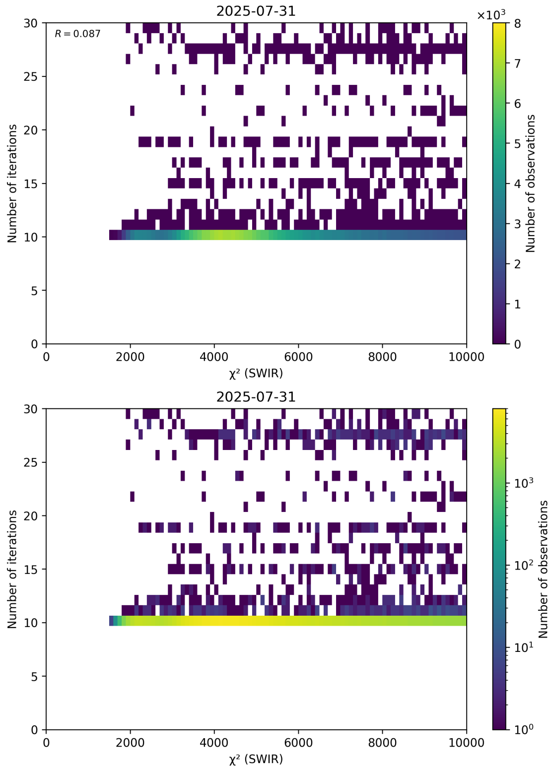
Figure 50: Scatter density plot of “ \chi^2 (SWIR)” against “Number of iterations” for 2025-07-30 to 2025-08-01.
