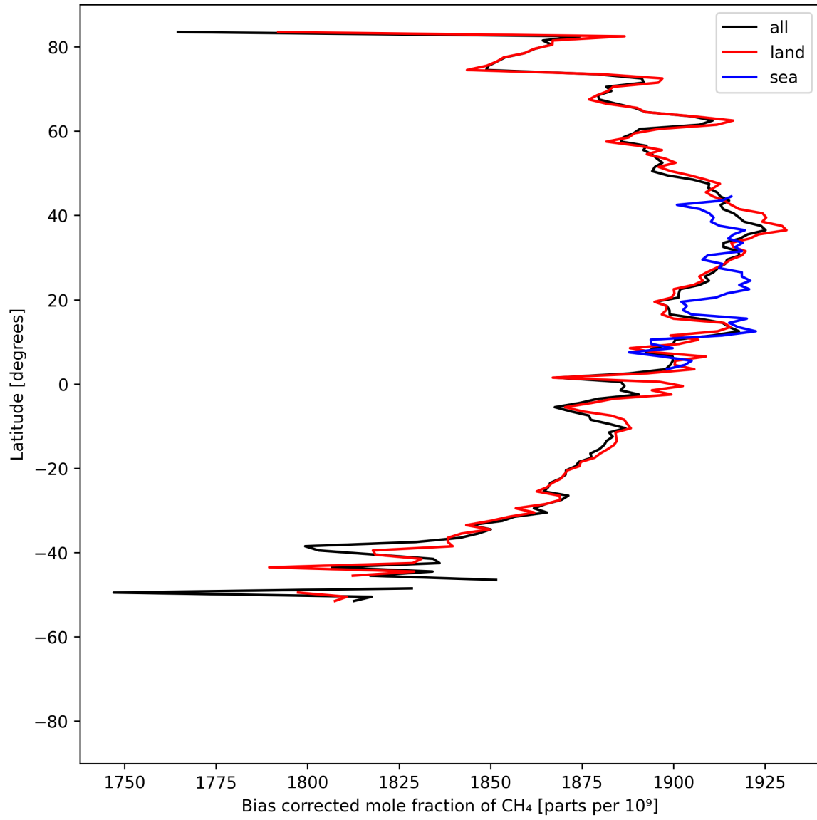
Figure 14: Zonal average of “Bias corrected mole fraction of \text{CH}_4 ” for 2025-07-30 to 2025-08-01.
