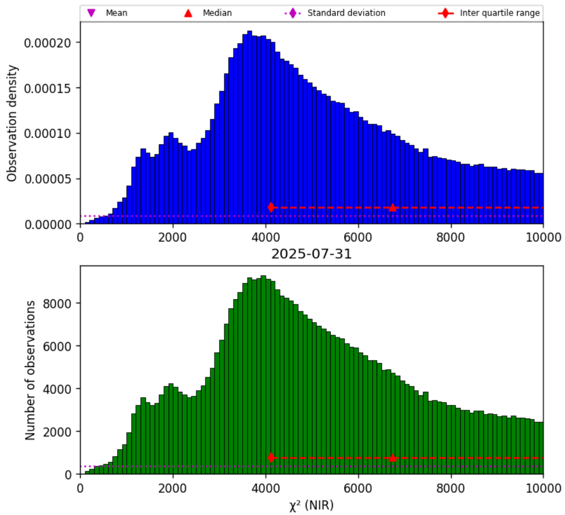
Figure 29: Histogram of " \chi^2 (NIR)" for 2025-07-30 to 2025-08-01
