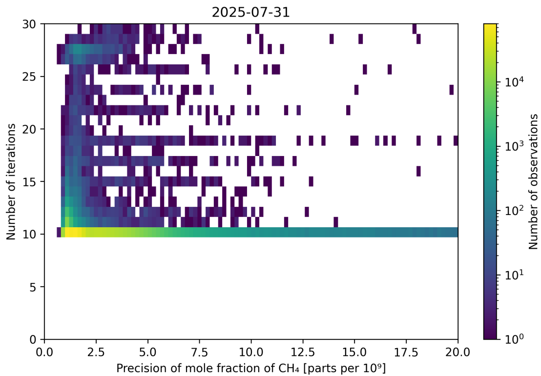
Figure 83: Scatter density plot of “Precision of mole fraction of CH 4 ” against “Number of iterations” for 2025-07-30 to 2025-08-01.
