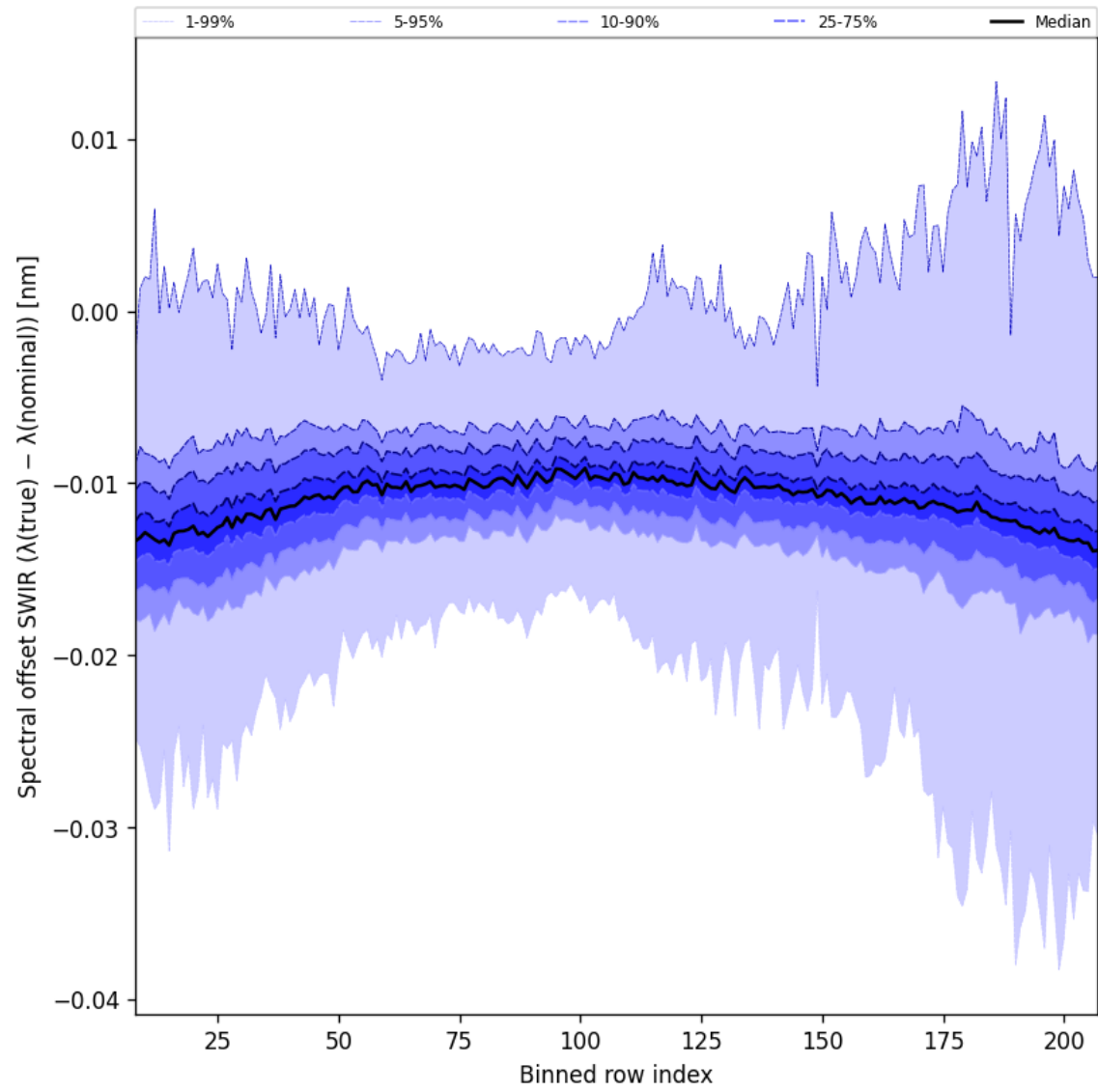
Figure 38: Along track statistics of “Spectral offset SWIR ( \lambda_{\text{true}} - \lambda_{\text{nominal}} )” for 2025-07-30 to 2025-08-01
