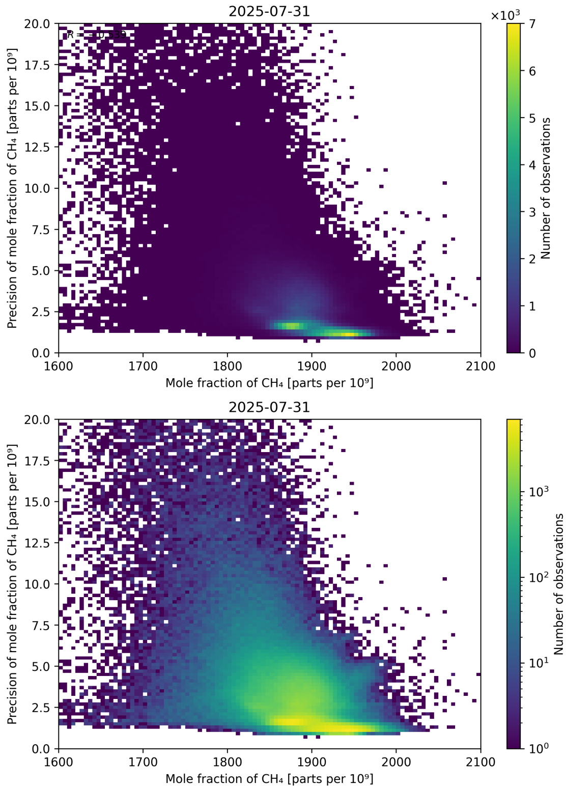
Figure 75: Scatter density plot of “Mole fraction of CH 4 ” against “Precision of mole fraction of CH 4 ” for 2025-07-30 to 2025-08-01.
