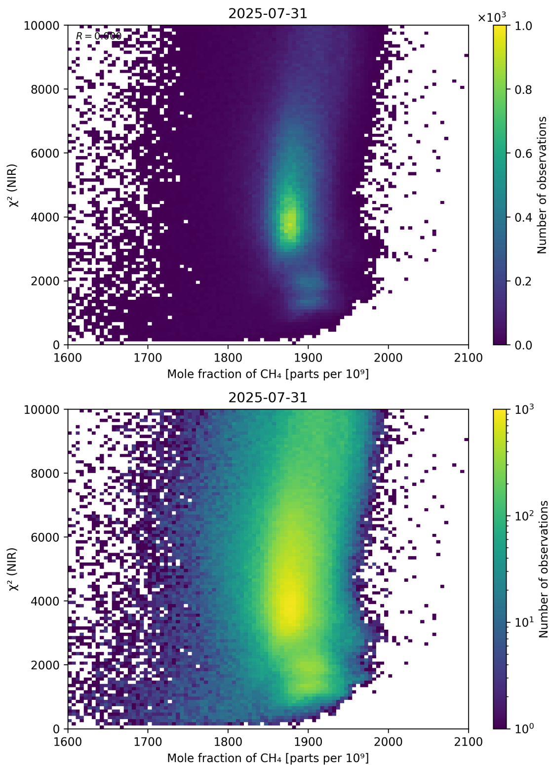
Figure 70: Scatter density plot of “Mole fraction of \text{CH}_4 ” against “ \chi^2 (NIR)” for 2025-07-30 to 2025-08-01.
