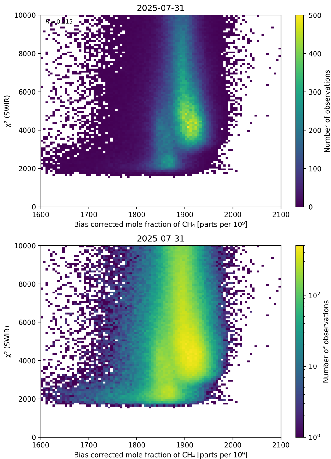
Figure 64: Scatter density plot of “Bias corrected mole fraction of \text{CH}_4 ” against “ \chi^2 (SWIR)” for 2025-07-30 to 2025-08-01.
