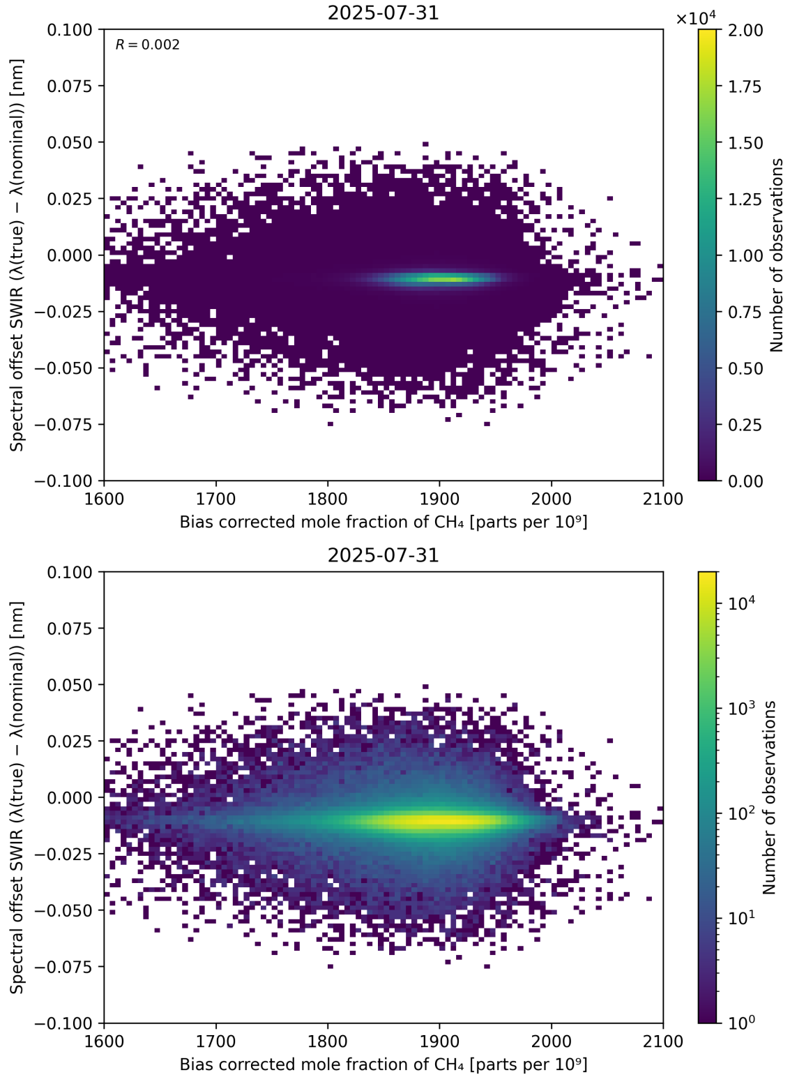
Figure 69: Scatter density plot of “Bias corrected mole fraction of \text{CH}_4 ” against “Spectral offset SWIR ( \lambda_{\text{true}} - \lambda_{\text{nominal}} )” for 2025-07-30 to 2025-08-01.
