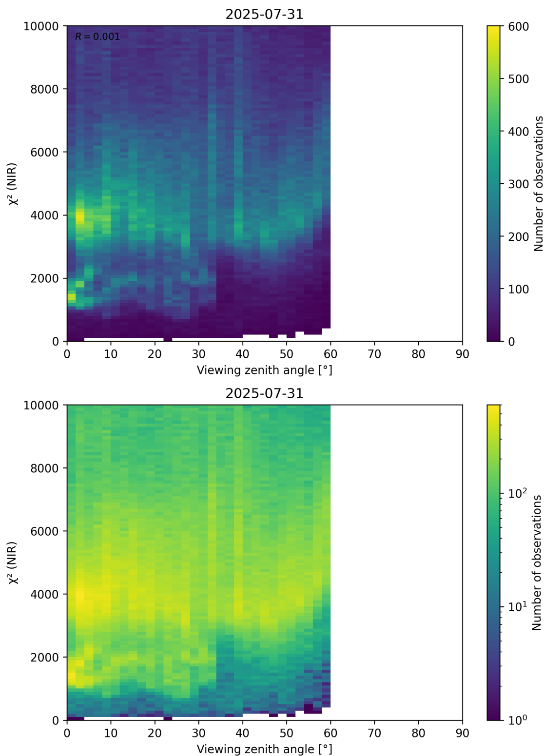
Figure 105: Scatter density plot of “Viewing zenith angle” against “ \chi^2 (NIR)” for 2025-07-30 to 2025-08-01.
