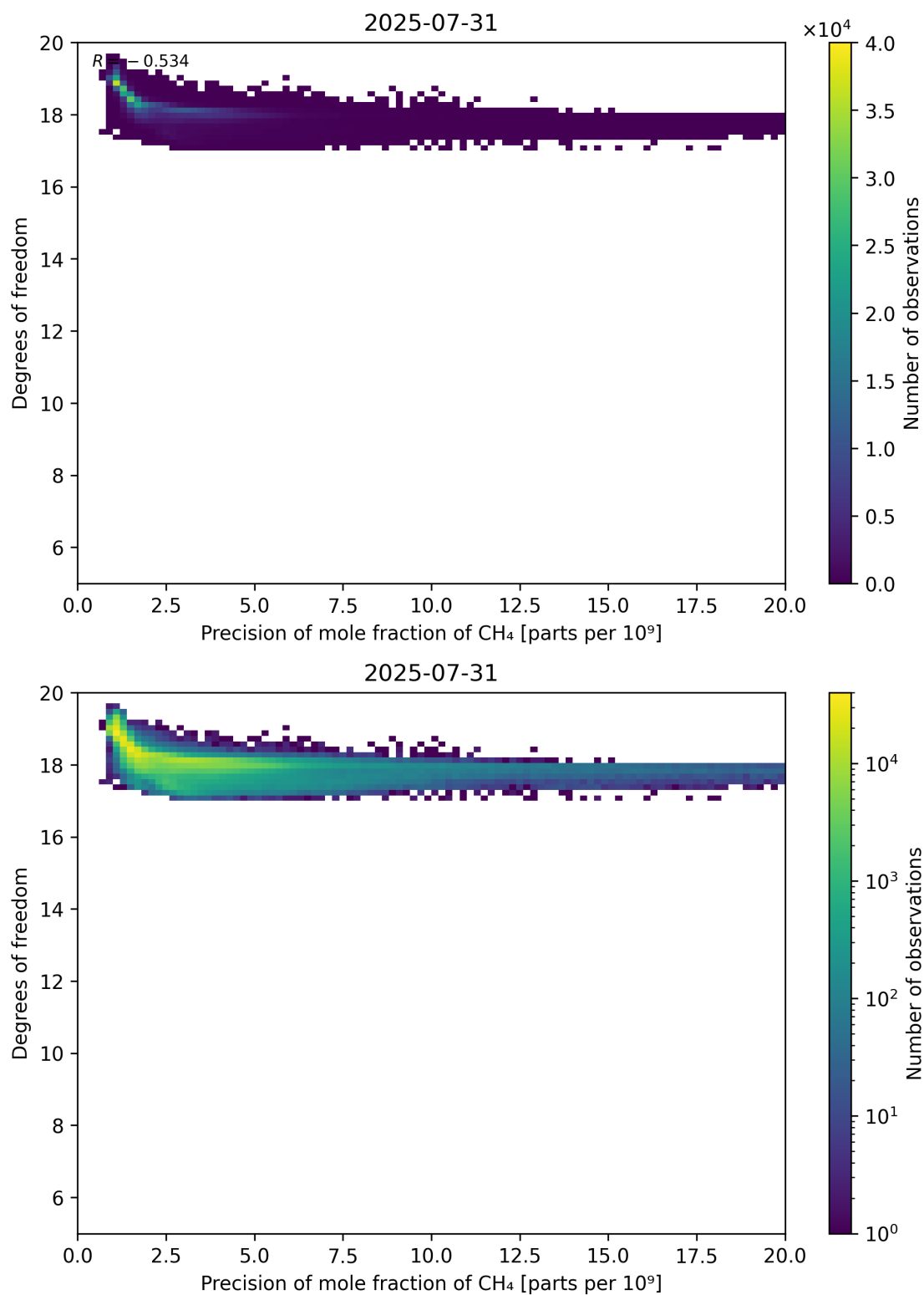
Figure 80: Scatter density plot of “Precision of mole fraction of CH 4 ” against “Degrees of freedom” for 2025-07-30 to 2025-08-01.
