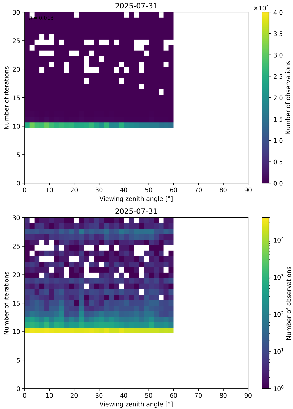
Figure 113: Scatter density plot of “Viewing zenith angle” against “Number of iterations” for 2025-07-30 to 2025-08-01.
