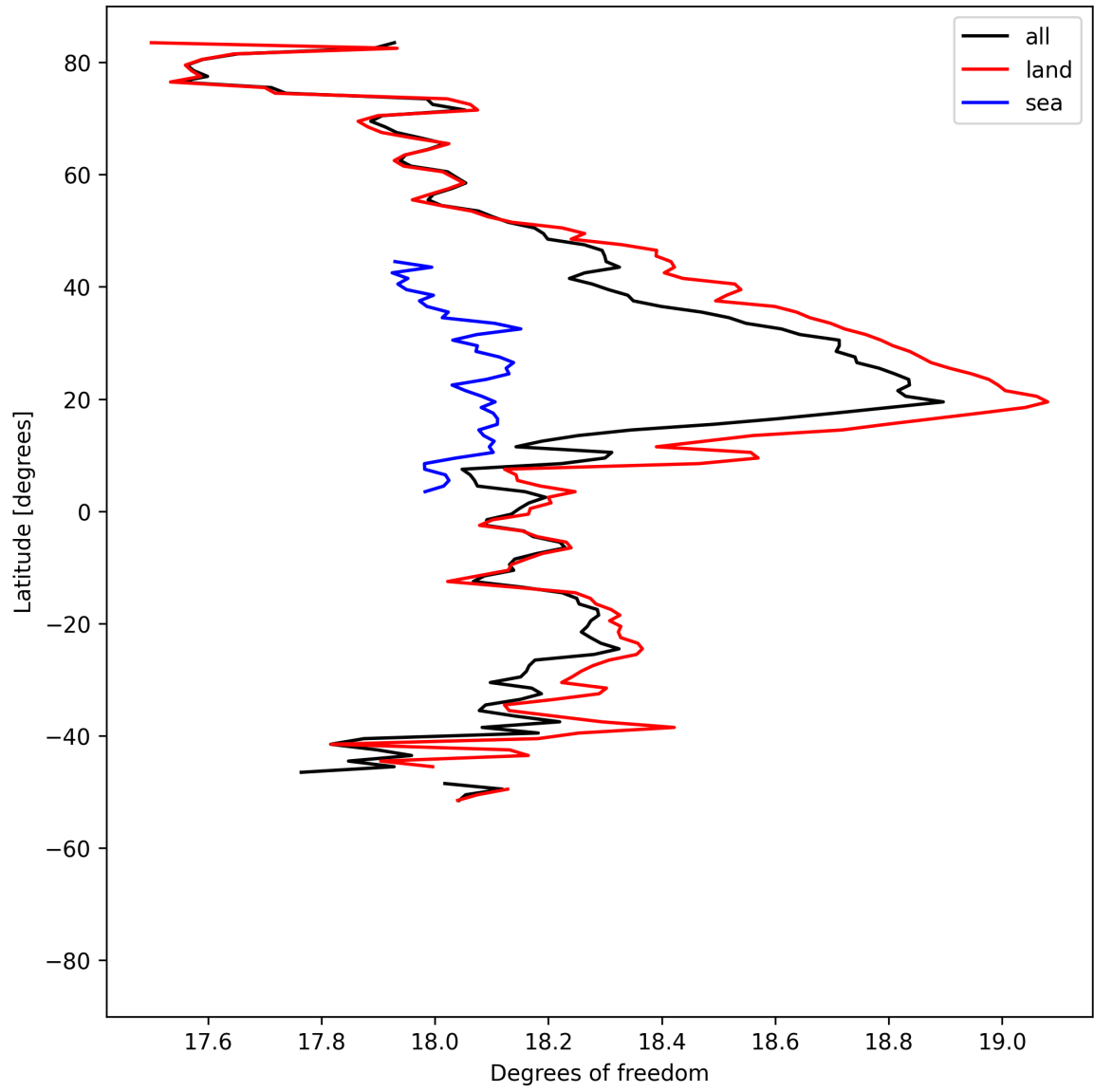
Figure 19: Zonal average of “Degrees of freedom” for 2025-07-30 to 2025-08-01.
