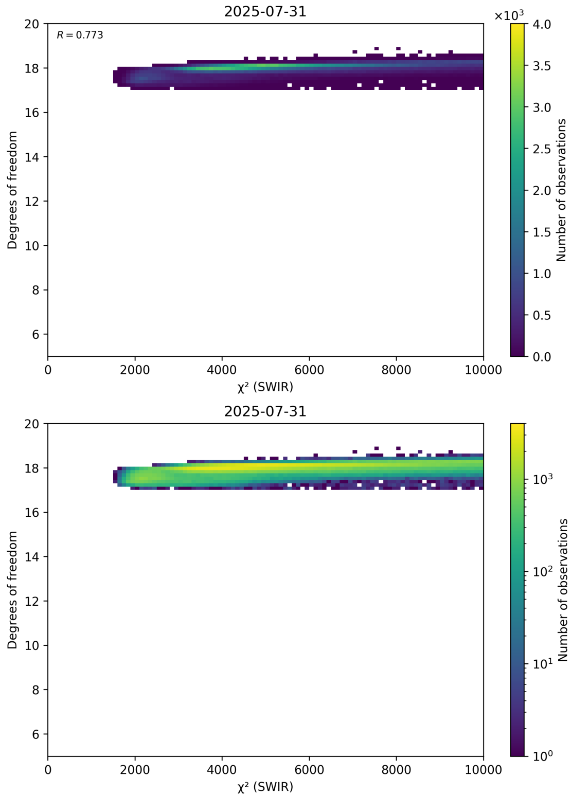
Figure 48: Scatter density plot of “ \chi^2 (SWIR)” against “Degrees of freedom” for 2025-07-30 to 2025-08-01.
