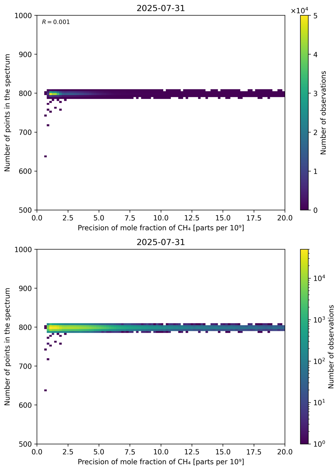
Figure 84: Scatter density plot of “Precision of mole fraction of CH 4 ” against “Number of points in the spectrum” for 2025-07-30 to 2025-08-01.
