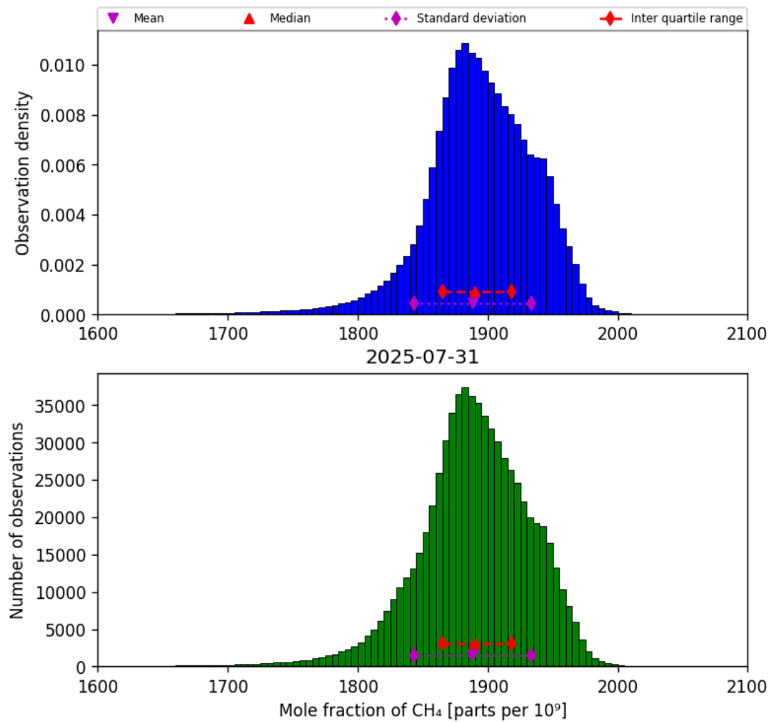
Figure 23: Histogram of "Mole fraction of CH 4 " for 2025-07-30 to 2025-08-01
