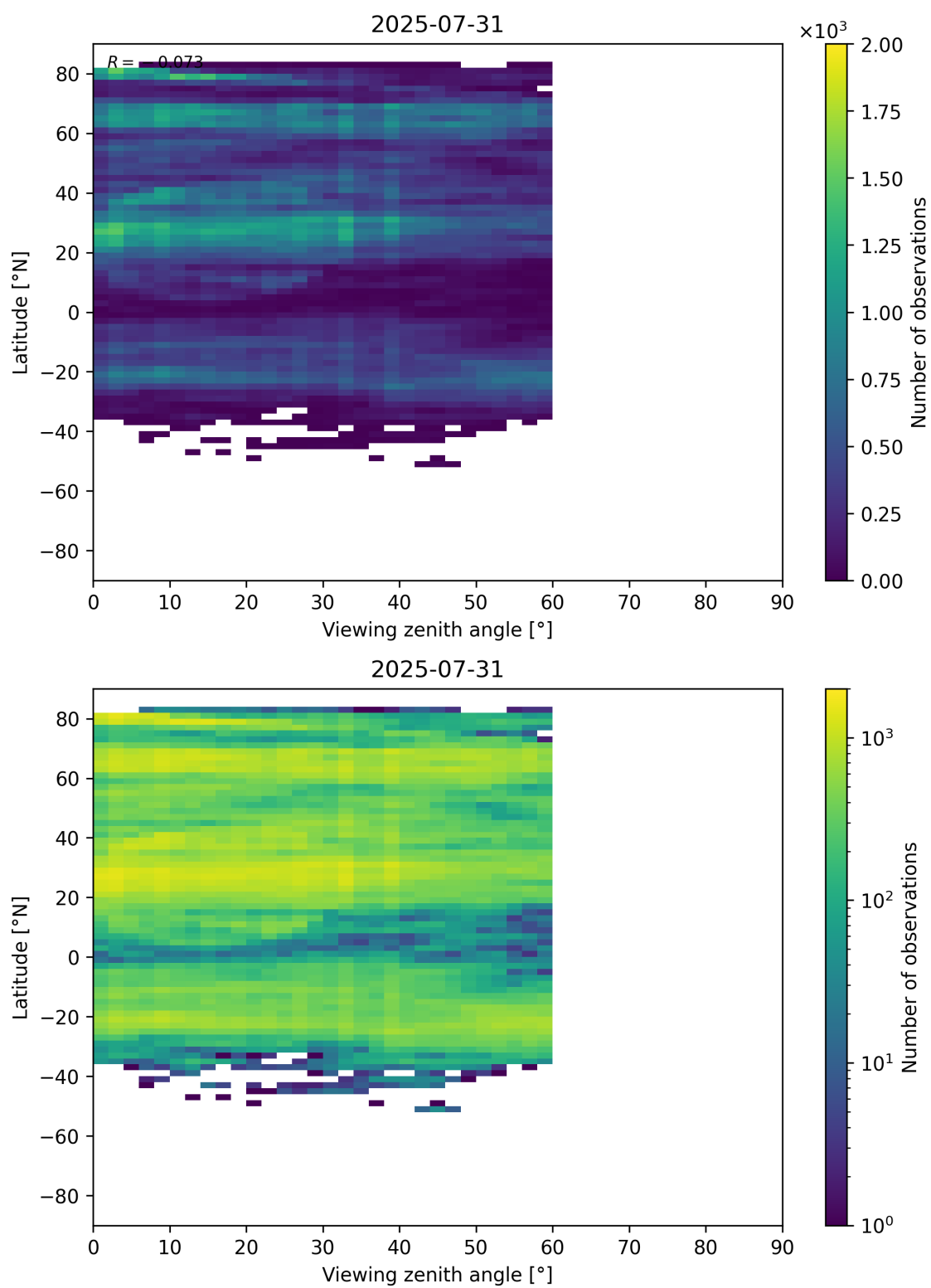
Figure 109: Scatter density plot of “Viewing zenith angle” against “Latitude” for 2025-07-30 to 2025-08-01.
