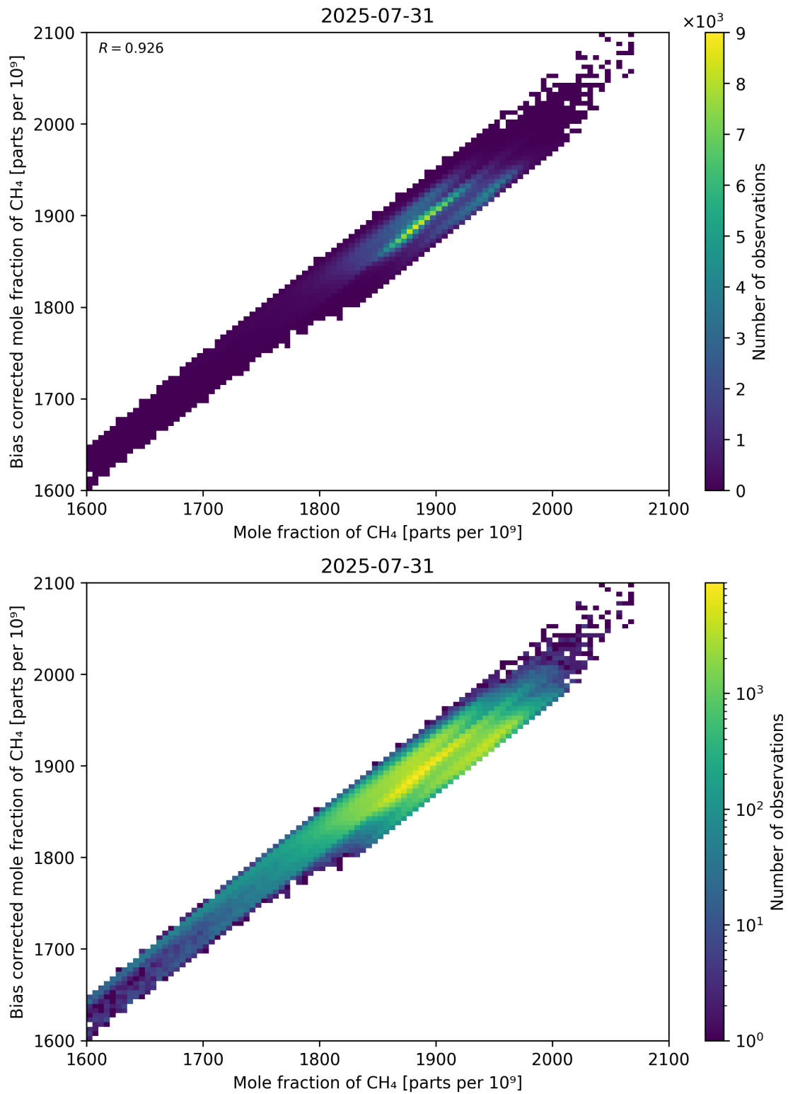
Figure 74: Scatter density plot of “Mole fraction of CH 4 ” against “Bias corrected mole fraction of CH 4 ” for 2025-07-30 to 2025-08-01.
