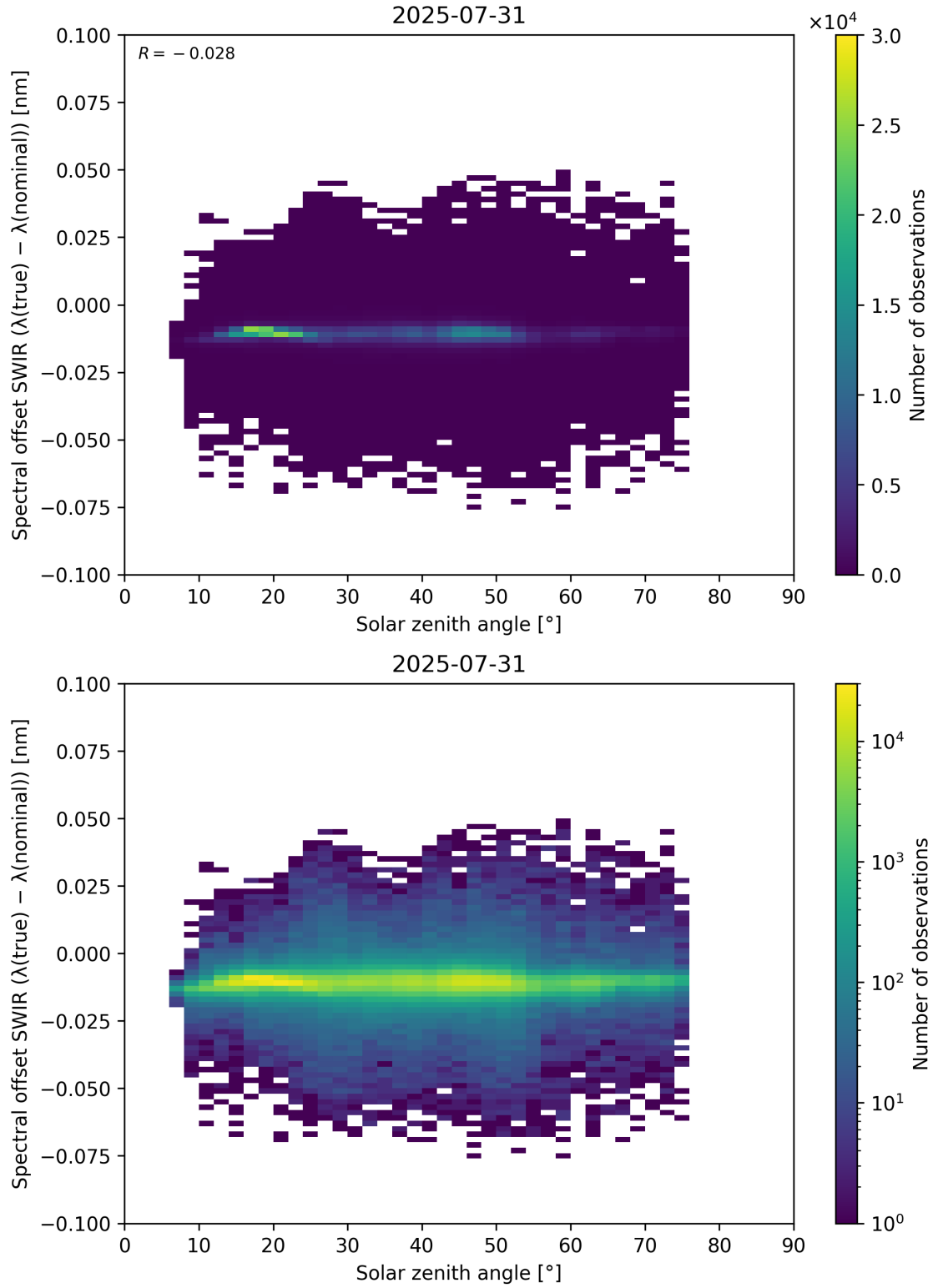
Figure 104: Scatter density plot of “Solar zenith angle” against “Spectral offset SWIR ( \lambda_{\text{true}} - \lambda_{\text{nominal}} )” for 2025-07-30 to 2025-08-01.
