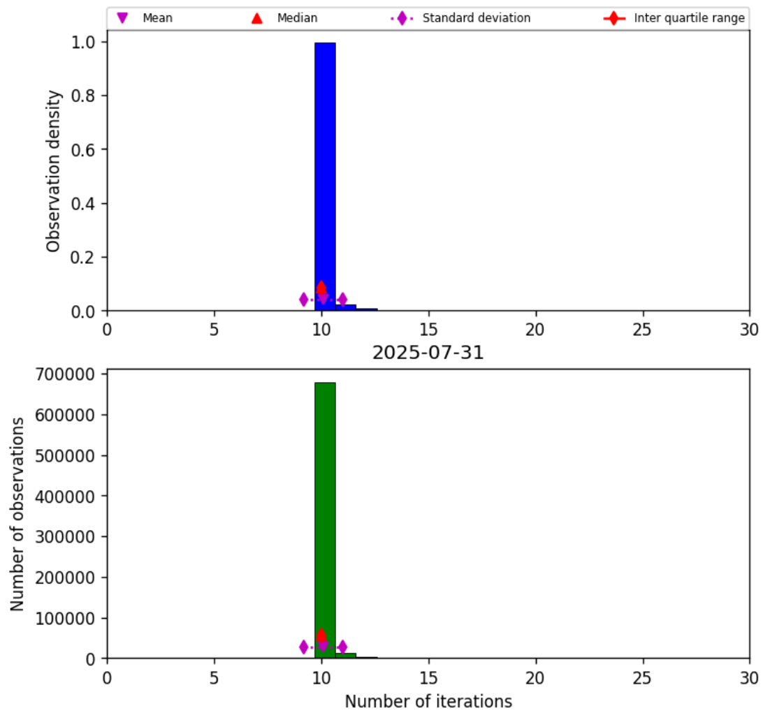
Figure 31: Histogram of “Number of iterations” for 2025-07-30 to 2025-08-01
