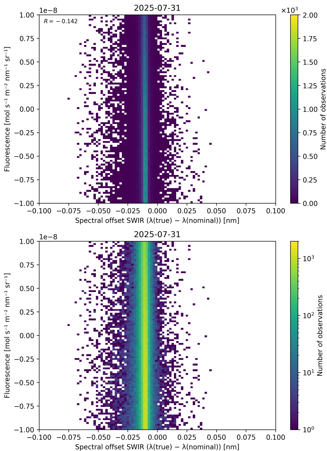
Figure 120: Scatter density plot of “Spectral offset SWIR ( \lambda_{\text{true}} - \lambda_{\text{nominal}} )” against “Fluorescence” for 2025-07-30 to 2025-08-01.
