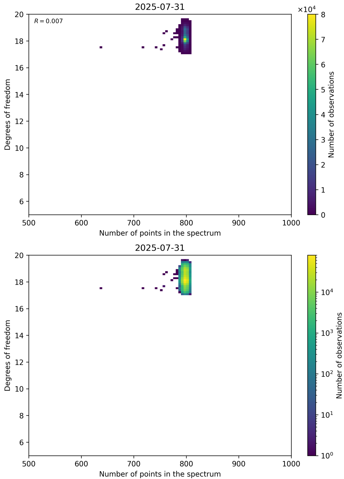
Figure 90: Scatter density plot of “Number of points in the spectrum” against “Degrees of freedom” for 2025-07-30 to 2025-08-01.
