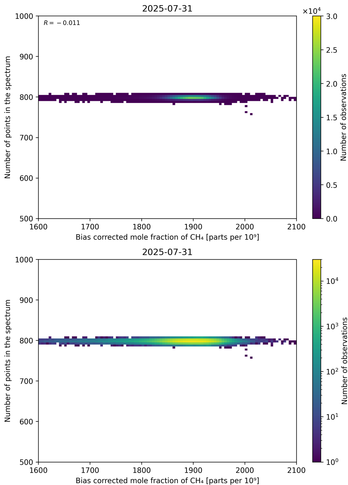
Figure 68: Scatter density plot of “Bias corrected mole fraction of CH 4 ” against “Number of points in the spectrum” for 2025-07-30 to 2025-08-01.
