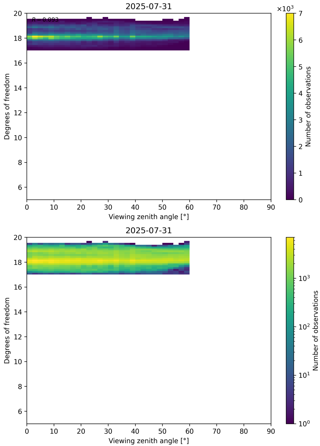
Figure 107: Scatter density plot of “Viewing zenith angle” against “Degrees of freedom” for 2025-07-30 to 2025-08-01.
