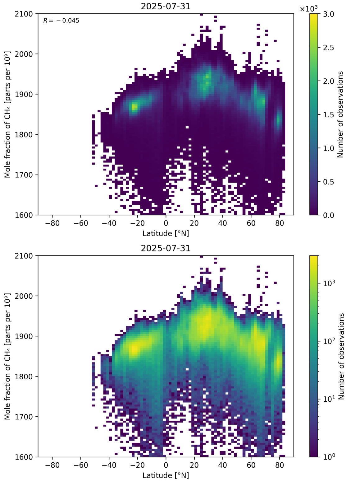
Figure 57: Scatter density plot of “Latitude” against “Mole fraction of \text{CH}_4 ” for 2025-07-30 to 2025-08-01.
