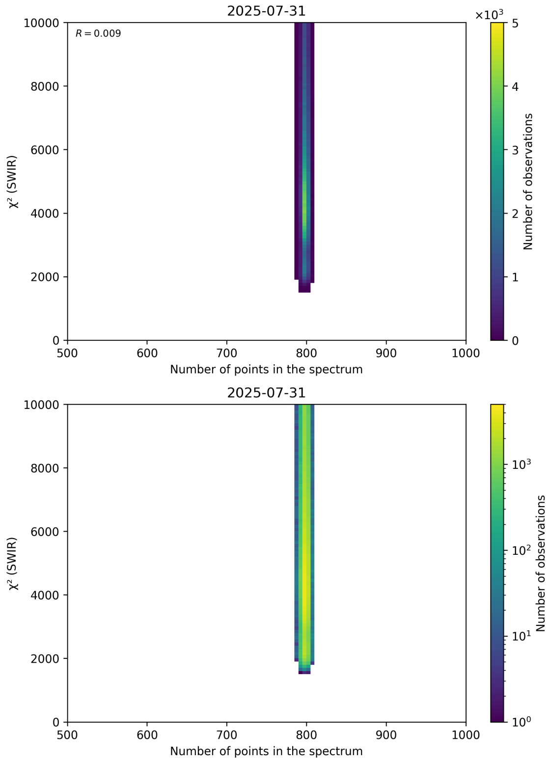
Figure 89: Scatter density plot of “Number of points in the spectrum” against “ \chi^2 (SWIR)” for 2025-07-30 to 2025-08-01.
