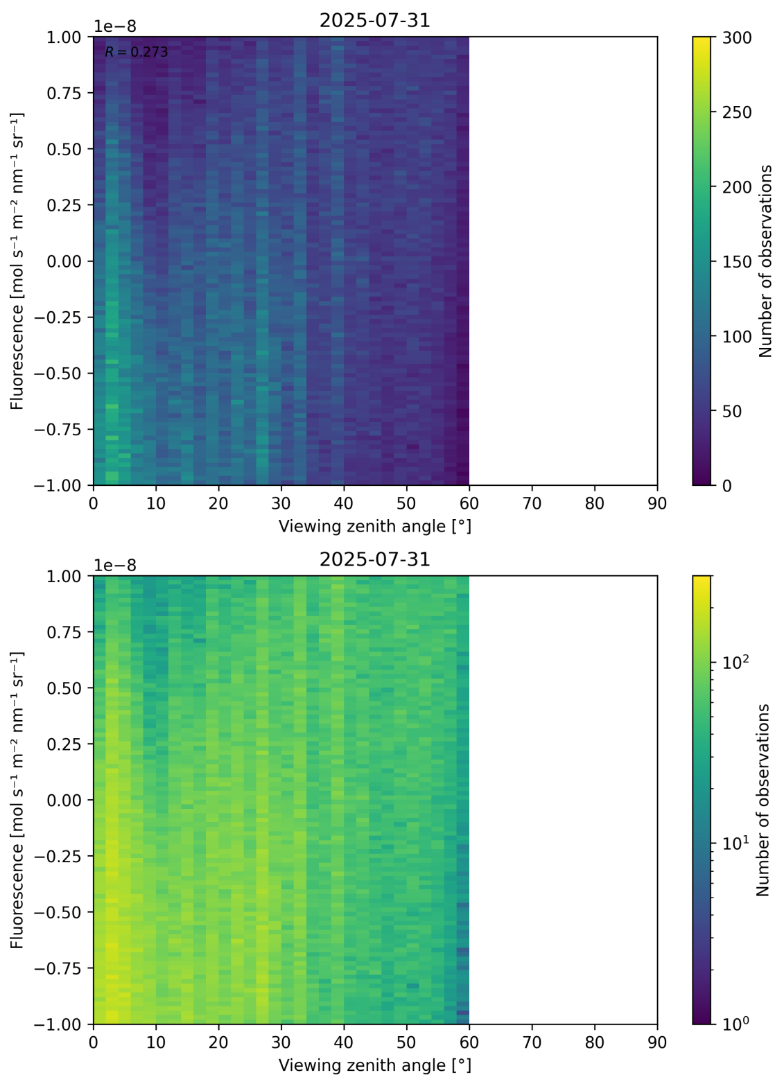
Figure 108: Scatter density plot of “Viewing zenith angle” against “Fluorescence” for 2025-07-30 to 2025-08-01.
