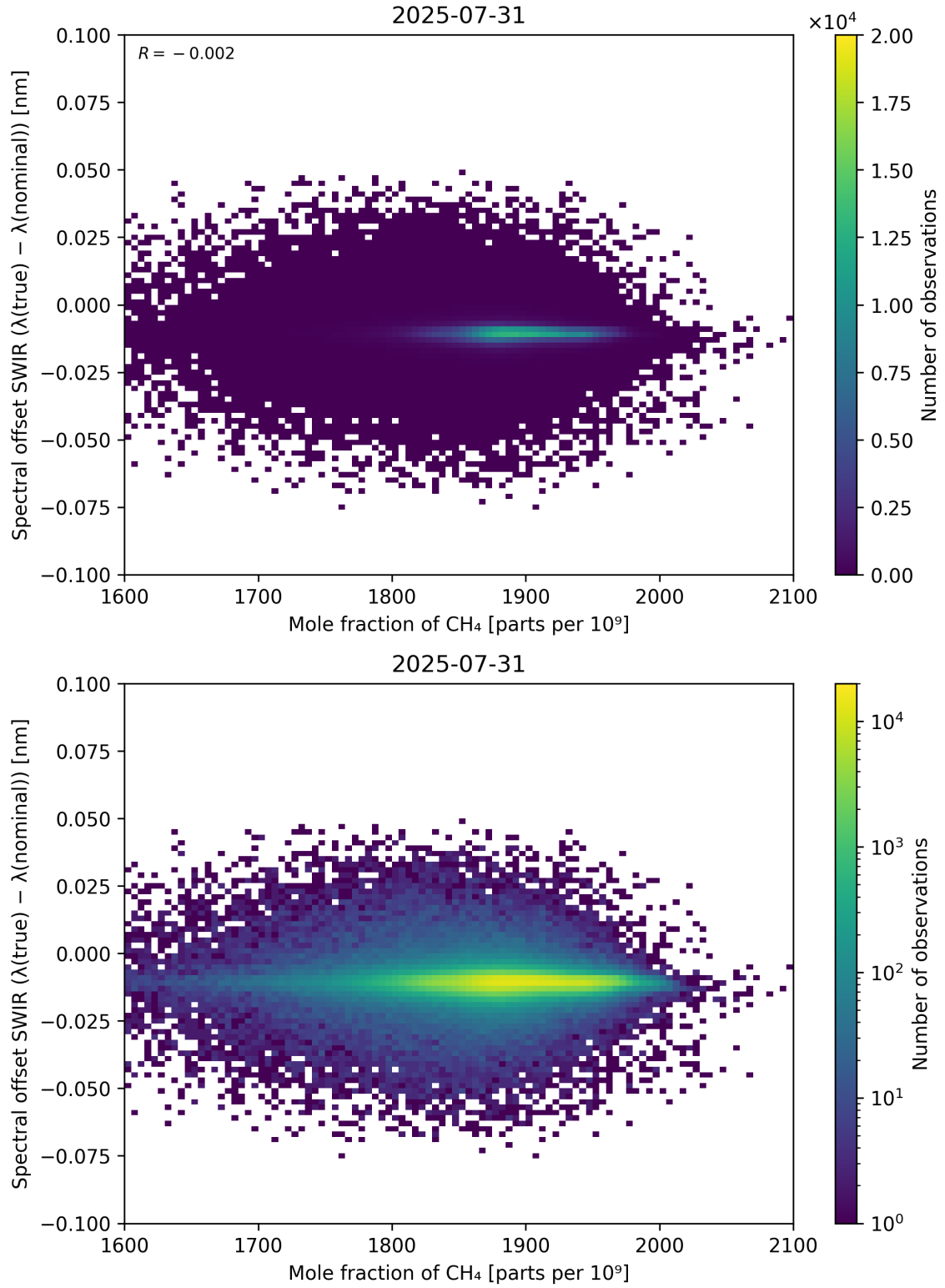
Figure 86: Scatter density plot of “Mole fraction of CH 4 ” against “Spectral offset SWIR ( \lambda_{\text{true}} - \lambda_{\text{nominal}} )” for 2025-07-30 to 2025-08-01.
