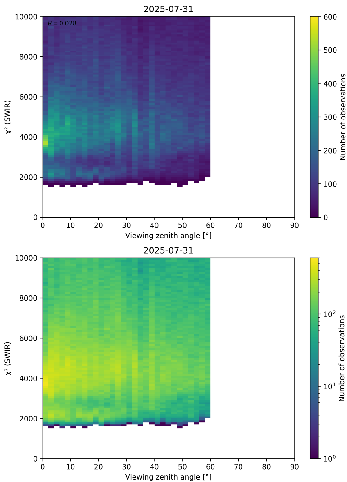
Figure 106: Scatter density plot of “Viewing zenith angle” against “ \chi^2 (SWIR)” for 2025-07-30 to 2025-08-01.
