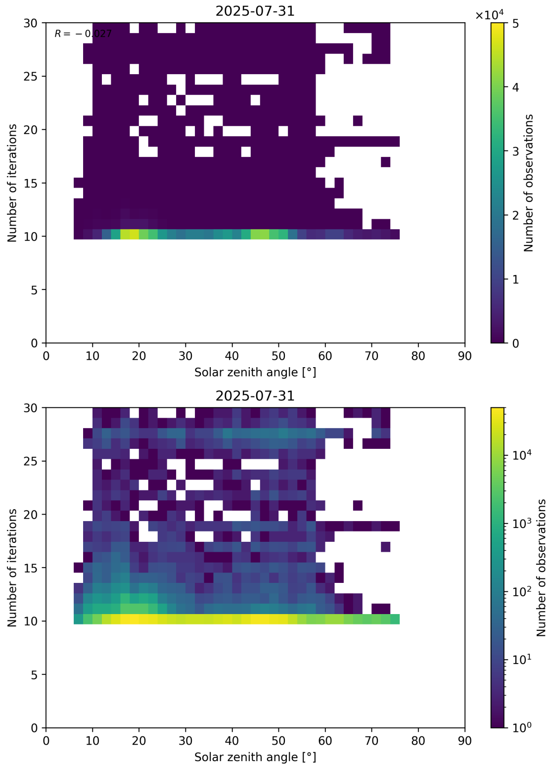
Figure 102: Scatter density plot of “Solar zenith angle” against “Number of iterations” for 2025-07-30 to 2025-08-01.
