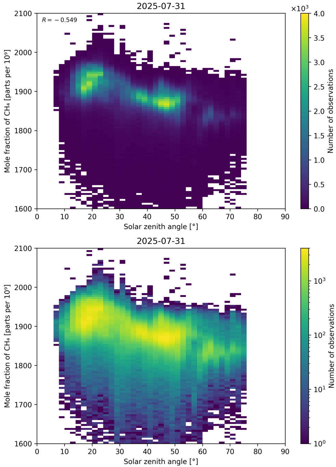
Figure 99: Scatter density plot of “Solar zenith angle” against “Mole fraction of CH 4 ” for 2025-07-30 to 2025-08-01.
