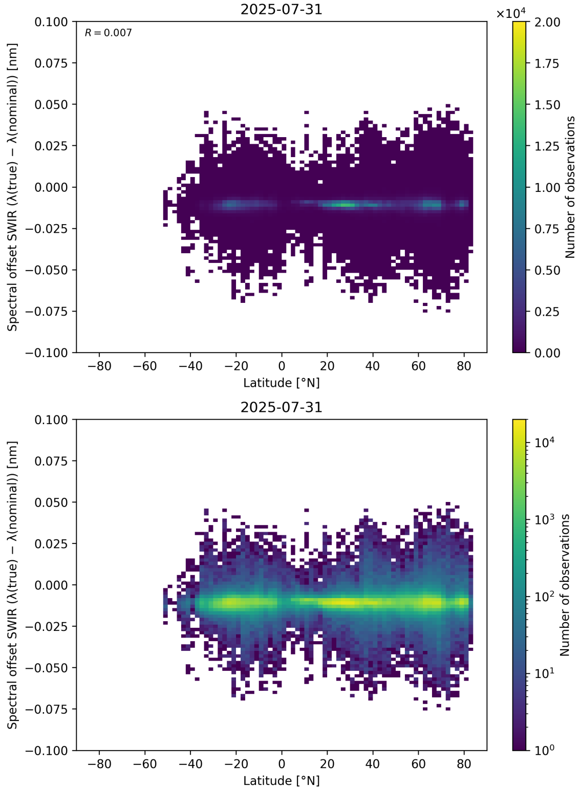
Figure 62: Scatter density plot of “Latitude” against “Spectral offset SWIR ( \lambda_{\text{true}} - \lambda_{\text{nominal}} )” for 2025-07-30 to 2025-08-01.
