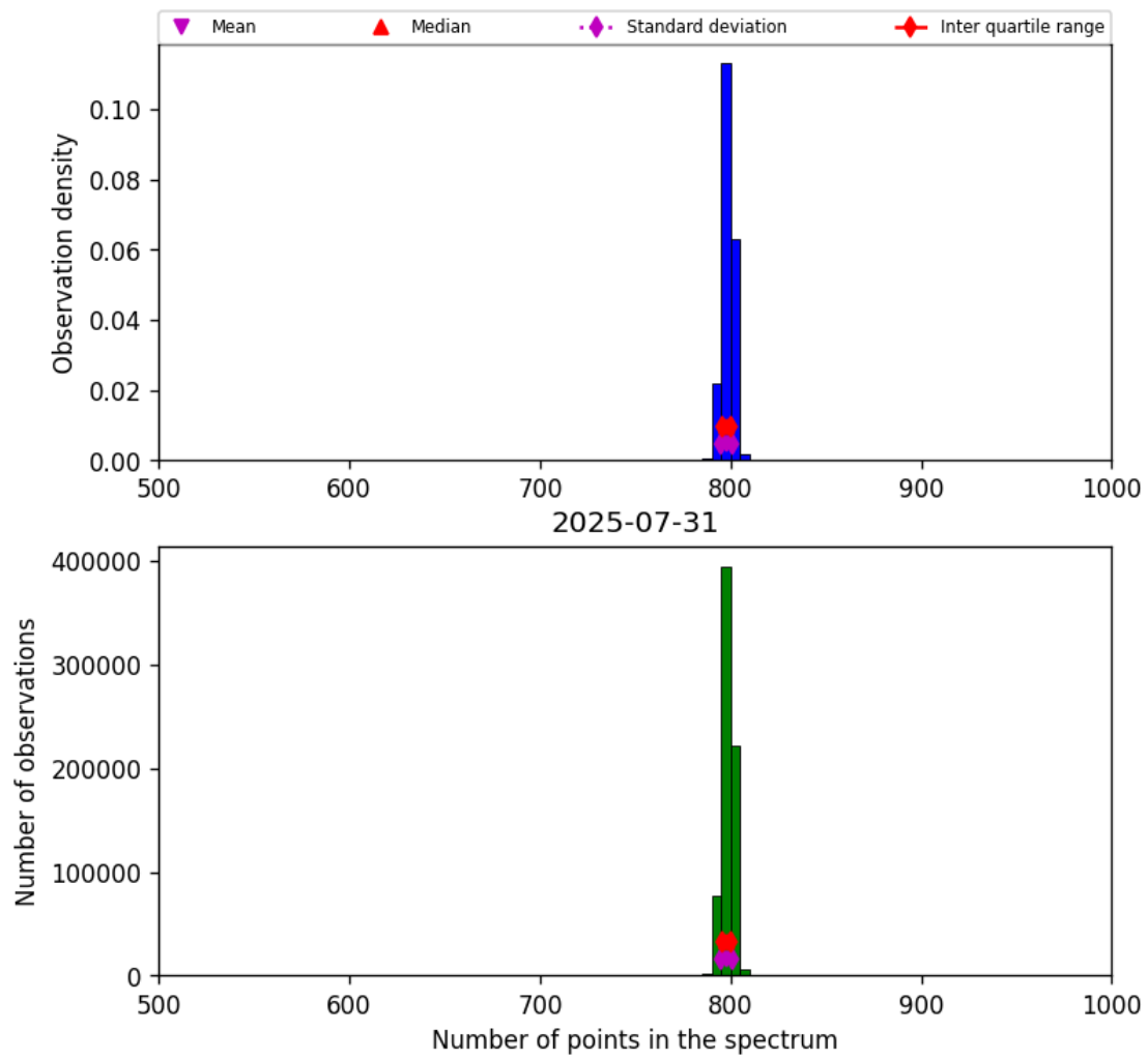
Figure 26: Histogram of “Number of points in the spectrum” for 2025-07-30 to 2025-08-01
