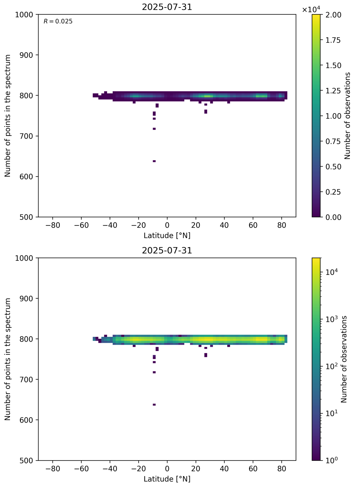
Figure 61: Scatter density plot of “Latitude” against “Number of points in the spectrum” for 2025-07-30 to 2025-08-01.
