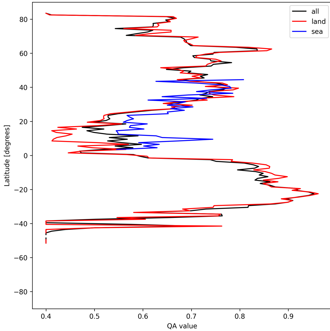
Figure 11: Zonal average of “QA value” for 2025-07-30 to 2025-08-01.
