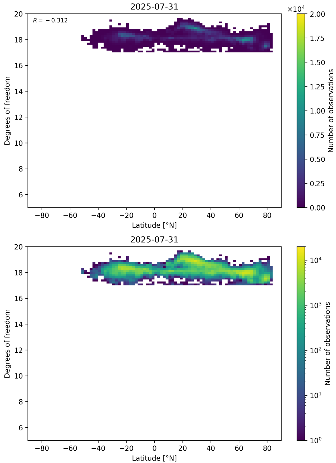
Figure 55: Scatter density plot of “Latitude” against “Degrees of freedom” for 2025-07-30 to 2025-08-01.
