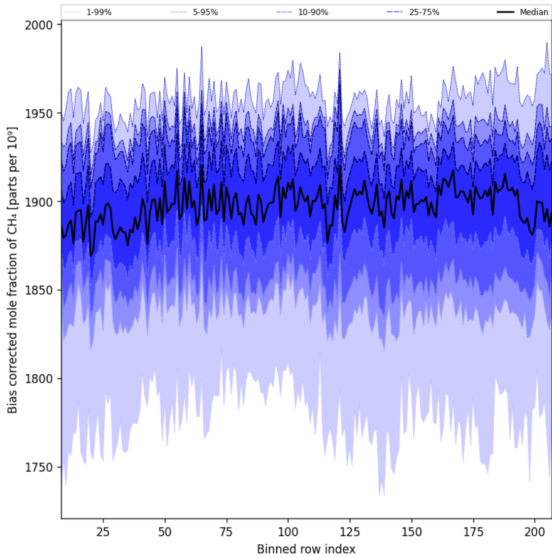
Figure 36: Along track statistics of “Bias corrected mole fraction of CH 4 ” for 2025-07-30 to 2025-08-01
