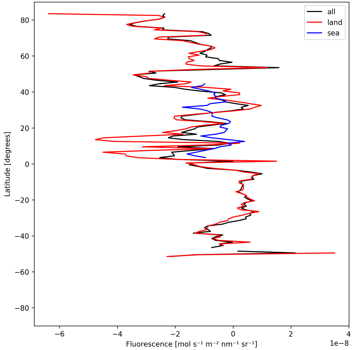
Figure 21: Zonal average of “Fluorescence” for 2025-07-30 to 2025-08-01.
