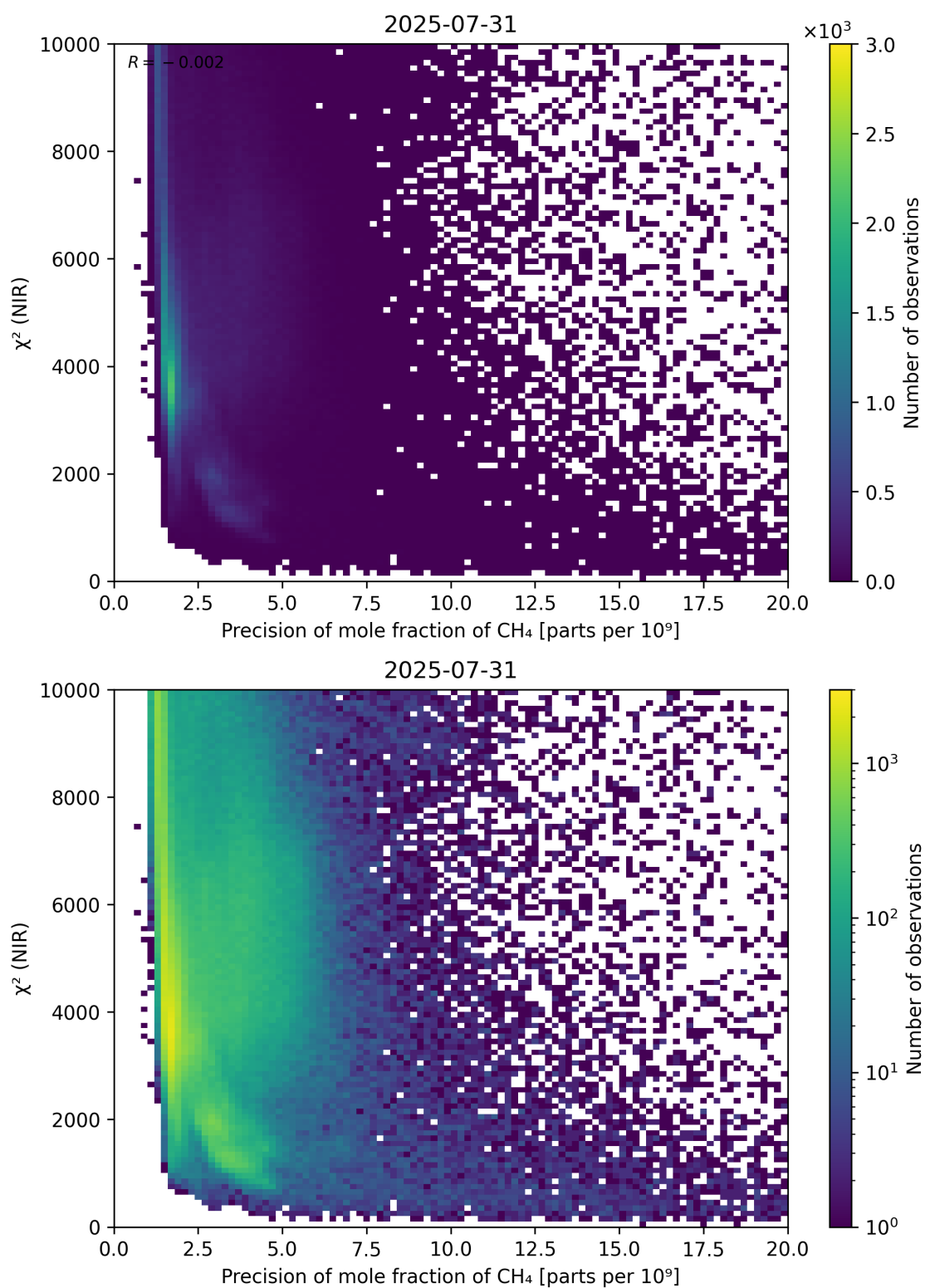
Figure 78: Scatter density plot of “Precision of mole fraction of CH 4 ” against “ \chi^2 (NIR)” for 2025-07-30 to 2025-08-01.
