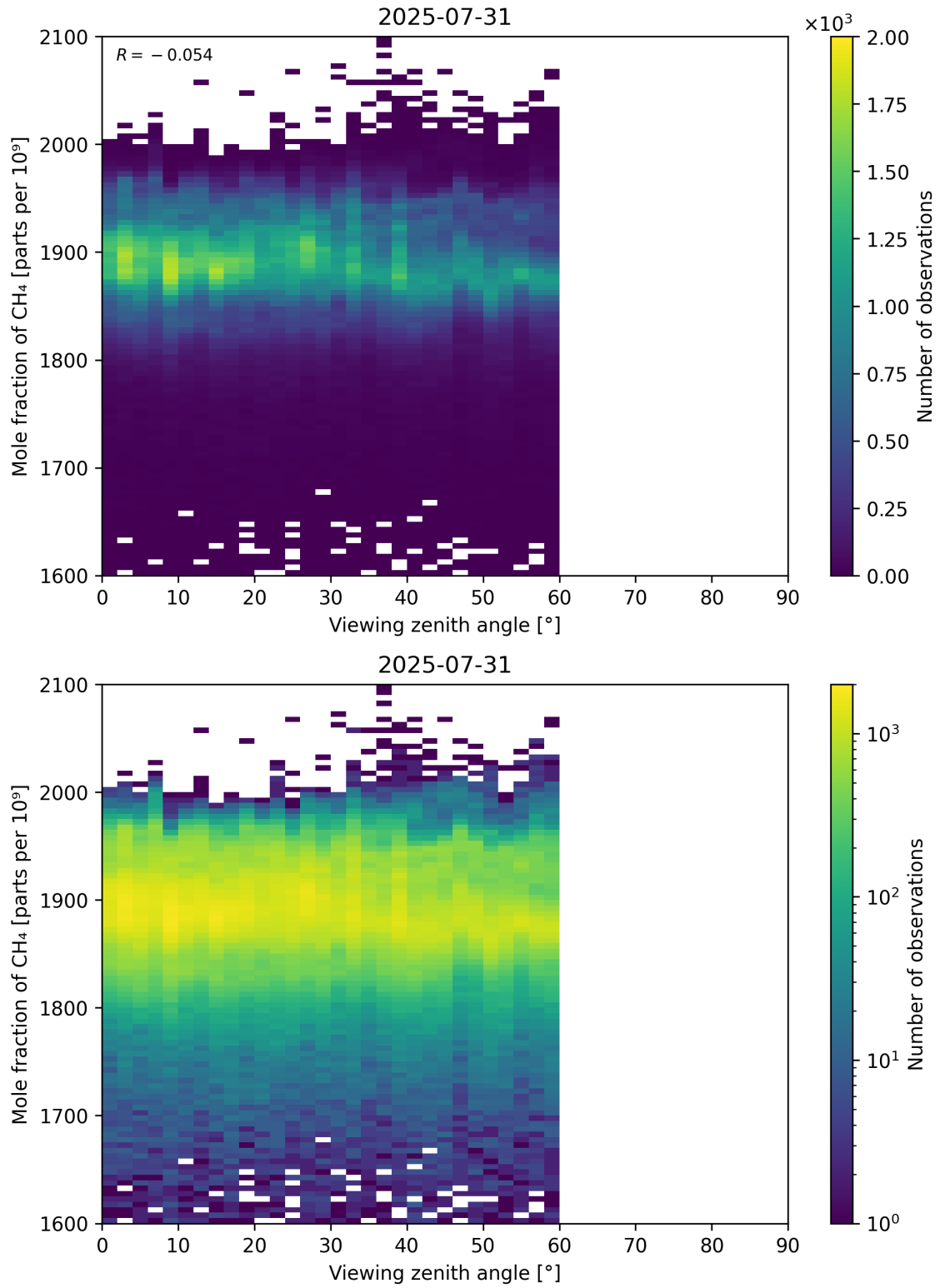
Figure 110: Scatter density plot of “Viewing zenith angle” against “Mole fraction of CH 4 ” for 2025-07-30 to 2025-08-01.
