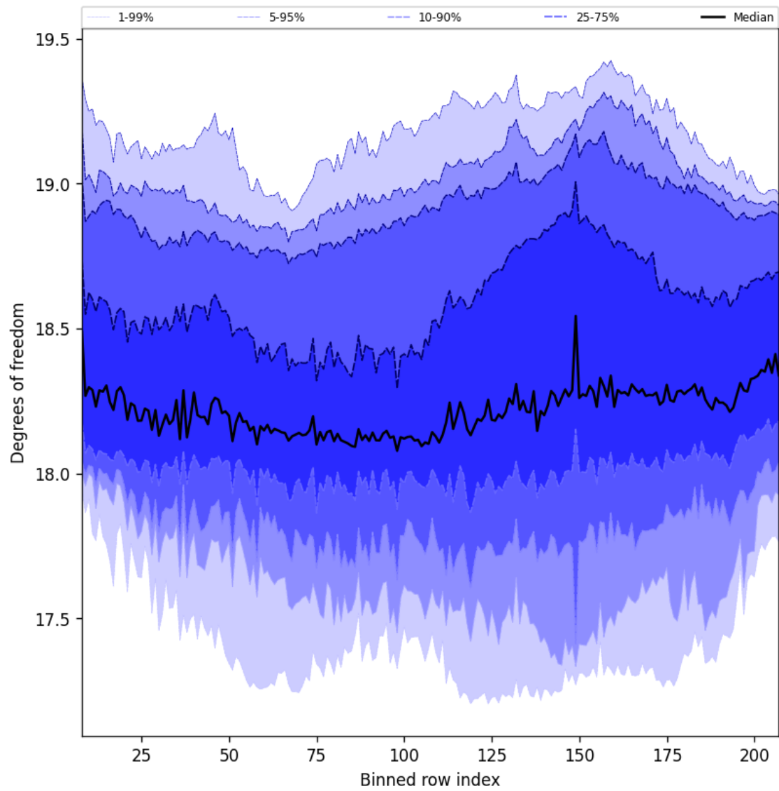
Figure 41: Along track statistics of “Degrees of freedom” for 2025-07-30 to 2025-08-01
