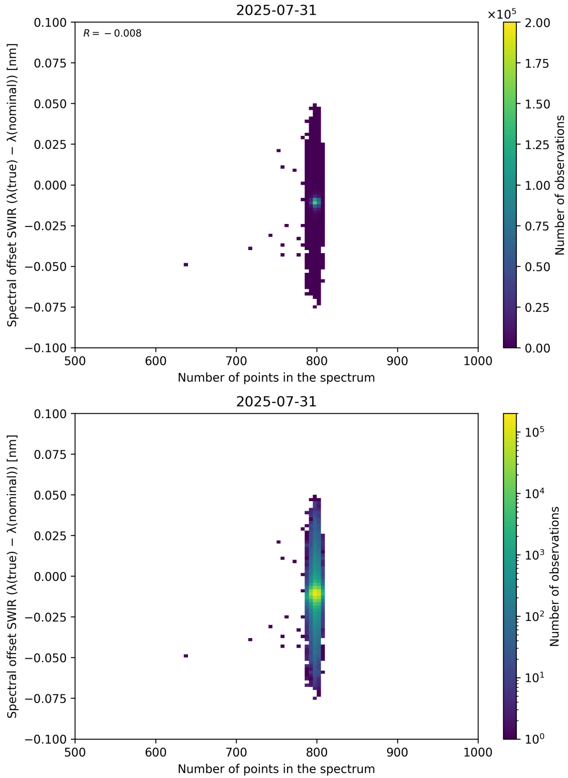
Figure 93: Scatter density plot of “Number of points in the spectrum” against “Spectral offset SWIR ( \lambda_{\text{true}} - \lambda_{\text{nominal}} )” for 2025-07-30 to 2025-08-01.
