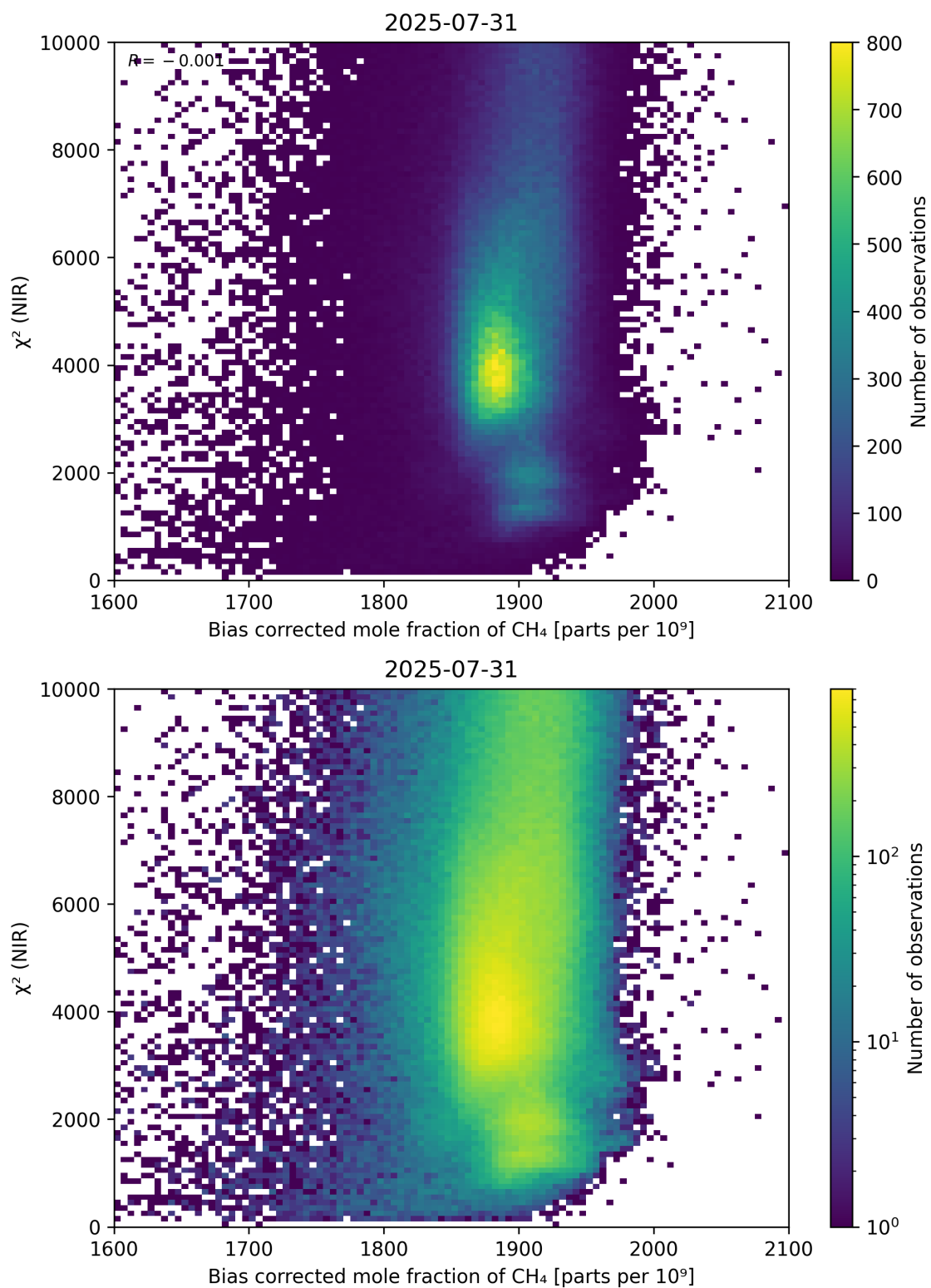
Figure 63: Scatter density plot of “Bias corrected mole fraction of CH 4 ” against “ \chi^2 (NIR)” for 2025-07-30 to 2025-08-01.
