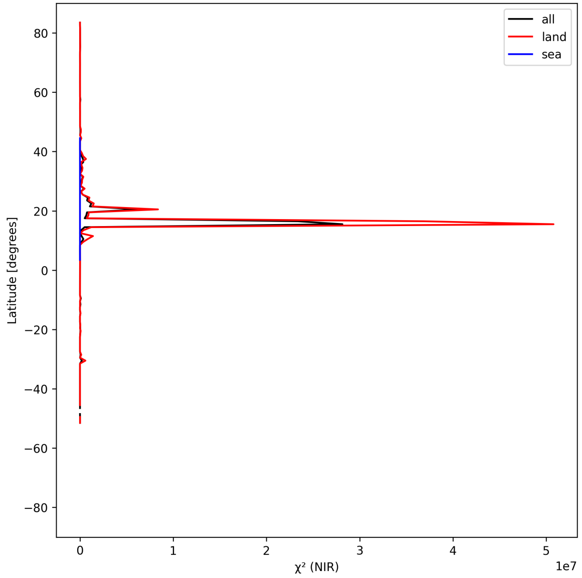
Figure 18: Zonal average of “ \chi^2 (NIR)” for 2025-07-30 to 2025-08-01.
