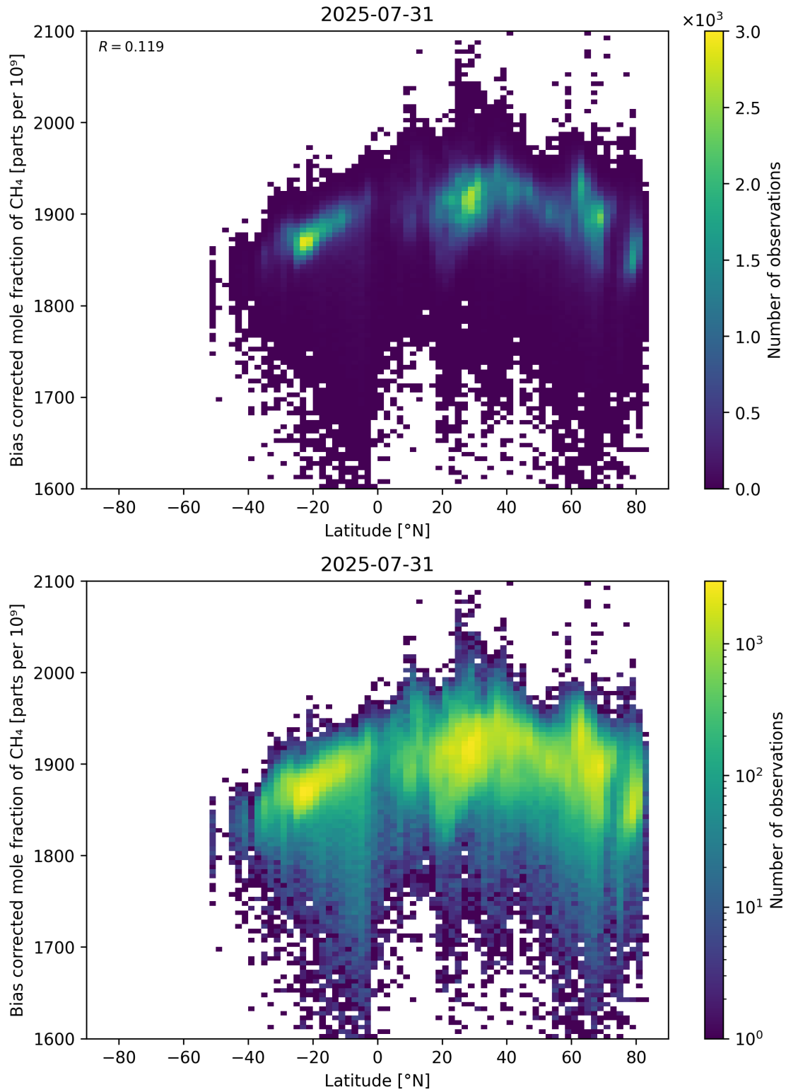
Figure 58: Scatter density plot of “Latitude” against “Bias corrected mole fraction of CH 4 ” for 2025-07-30 to 2025-08-01.
