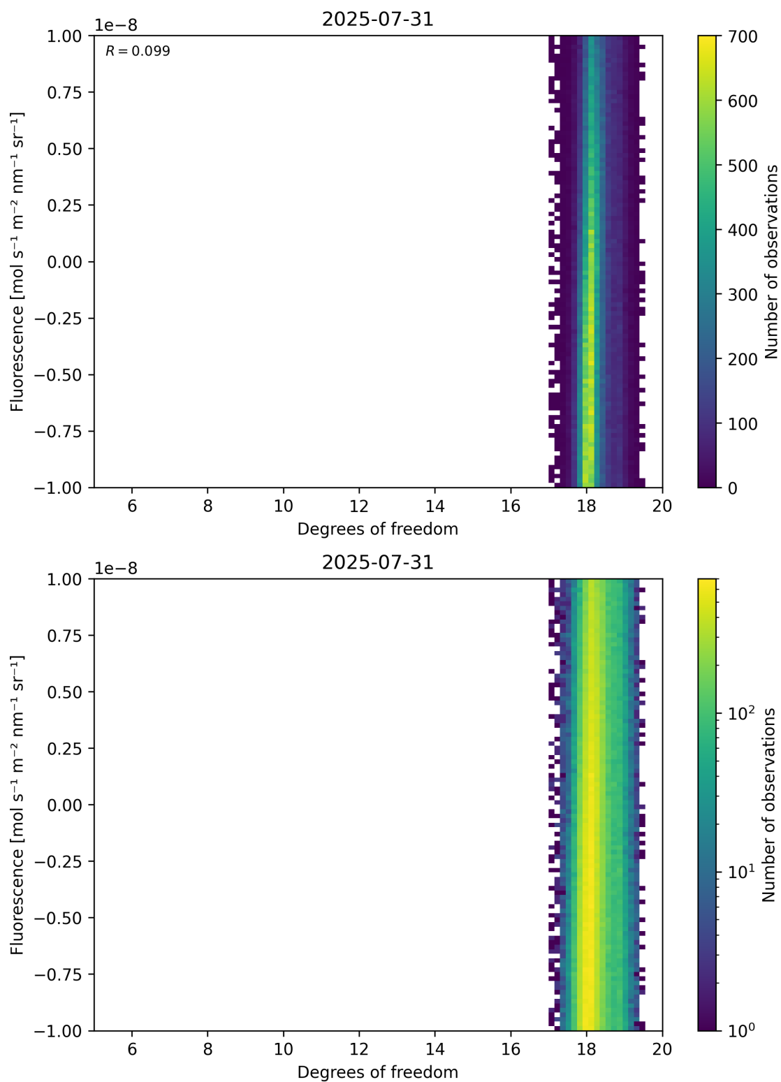
Figure 51: Scatter density plot of “Degrees of freedom” against “Fluorescence” for 2025-07-30 to 2025-08-01.
