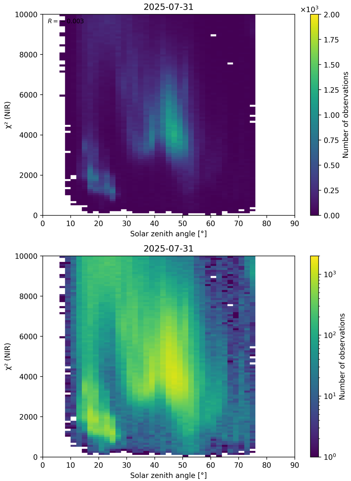
Figure 94: Scatter density plot of “Solar zenith angle” against “ \chi^2 (NIR)” for 2025-07-30 to 2025-08-01.
