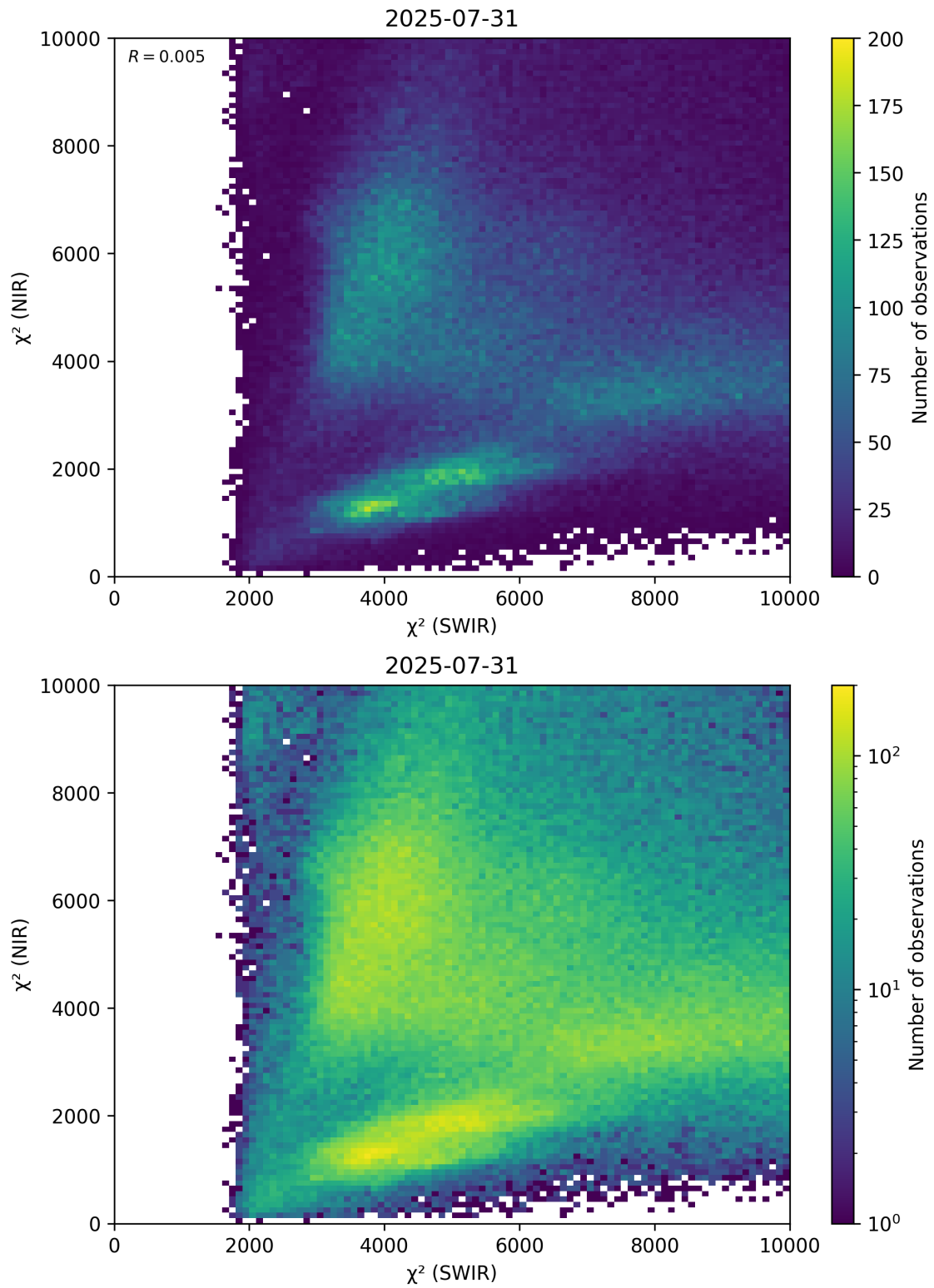
Figure 47: Scatter density plot of “ \chi^2 (SWIR)” against “ \chi^2 (NIR)” for 2025-07-30 to 2025-08-01.
