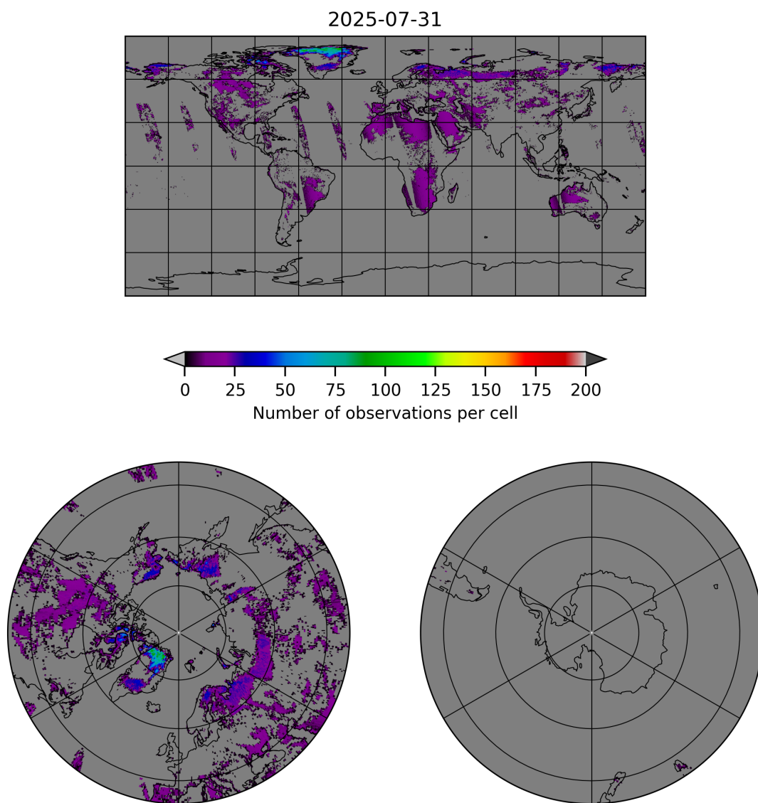
Figure 10: Map of the number of observations for 2025-07-30 to 2025-08-01
