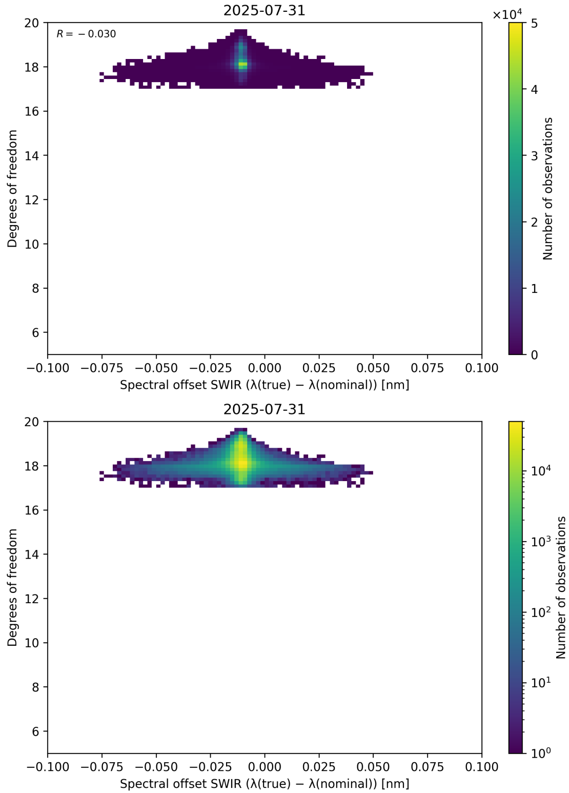
Figure 119: Scatter density plot of “Spectral offset SWIR ( \lambda_{\text{true}} - \lambda_{\text{nominal}} )” against “Degrees of freedom” for 2025-07-30 to 2025-08-01.
