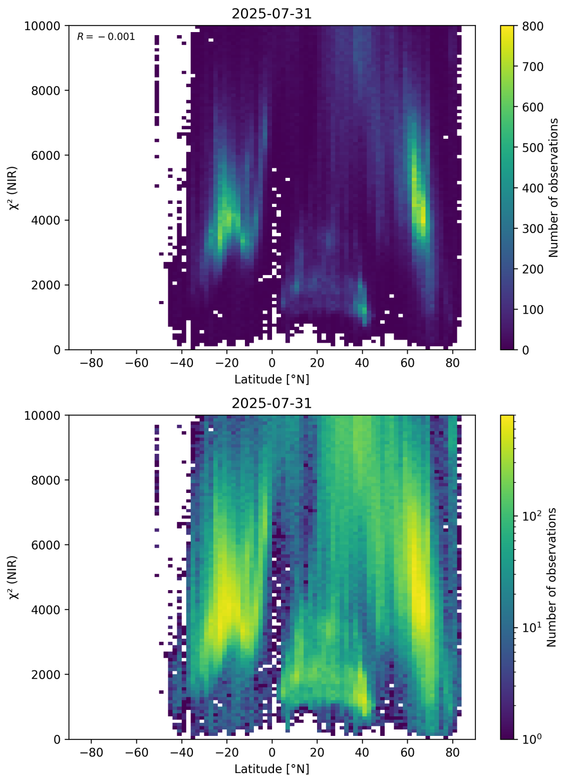
Figure 53: Scatter density plot of “Latitude” against “ \chi^2 (NIR)” for 2025-07-30 to 2025-08-01.
