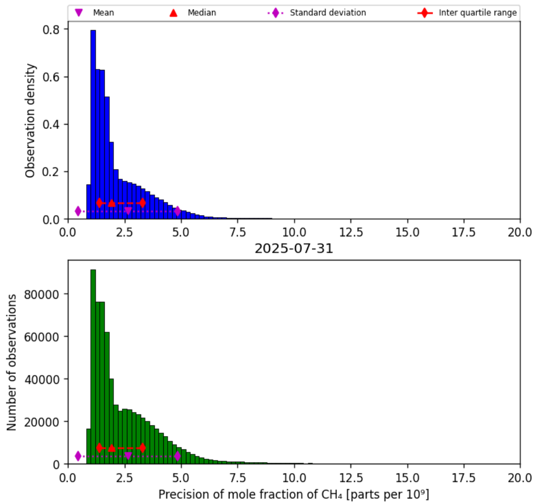
Figure 24: Histogram of “Precision of mole fraction of CH 4 ” for 2025-07-30 to 2025-08-01
