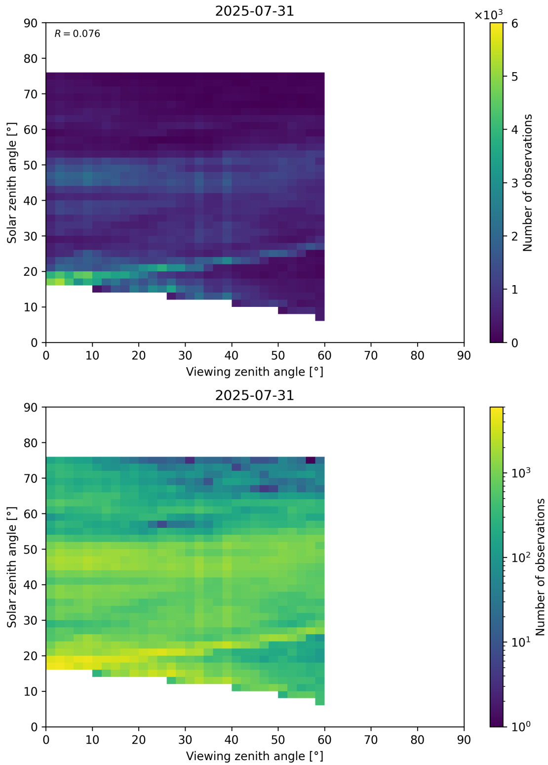
Figure 115: Scatter density plot of “Viewing zenith angle” against “Solar zenith angle” for 2025-07-30 to 2025-08-01.
