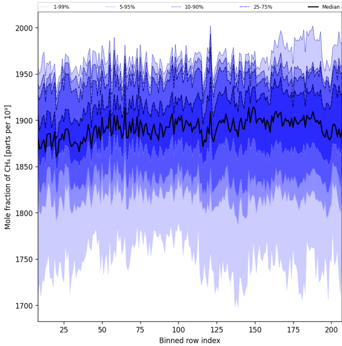
Figure 34: Along track statistics of “Mole fraction of CH 4 ” for 2025-07-30 to 2025-08-01
