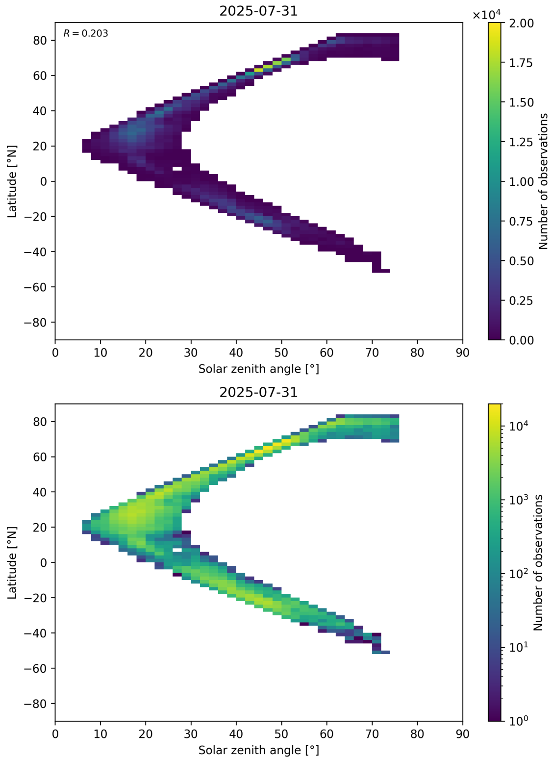
Figure 98: Scatter density plot of “Solar zenith angle” against “Latitude” for 2025-07-30 to 2025-08-01.
