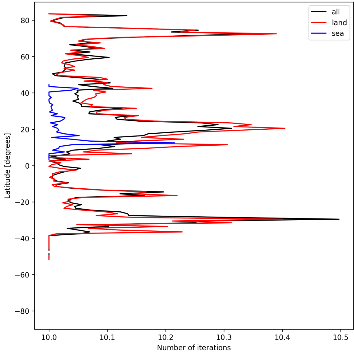
Figure 20: Zonal average of “Number of iterations” for 2025-07-30 to 2025-08-01.
