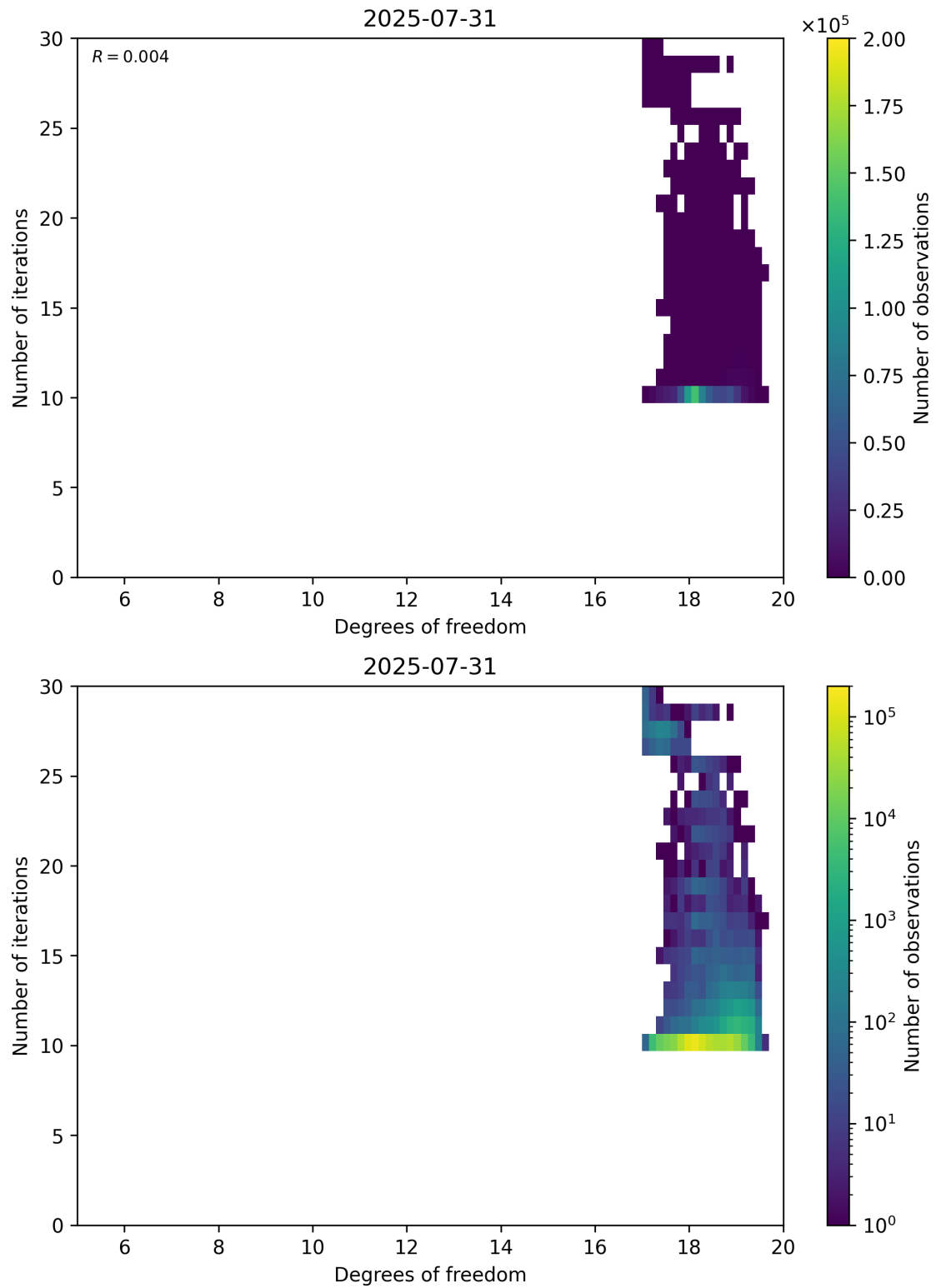
Figure 52: Scatter density plot of “Degrees of freedom” against “Number of iterations” for 2025-07-30 to 2025-08-01.
