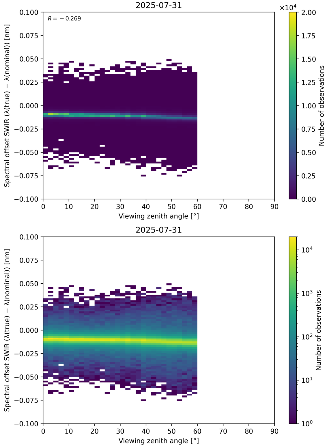
Figure 116: Scatter density plot of “Viewing zenith angle” against “Spectral offset SWIR ( \lambda_{\text{true}} - \lambda_{\text{nominal}} )” for 2025-07-30 to 2025-08-01.
