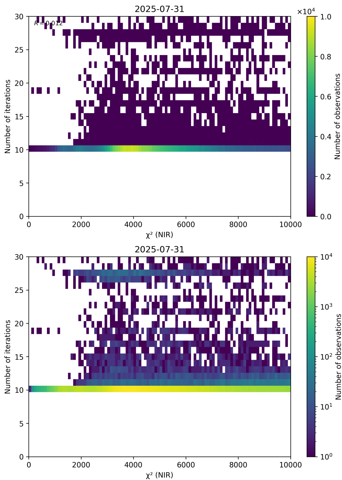
Figure 46: Scatter density plot of “ \chi^2 (NIR)” against “Number of iterations” for 2025-07-30 to 2025-08-01.
