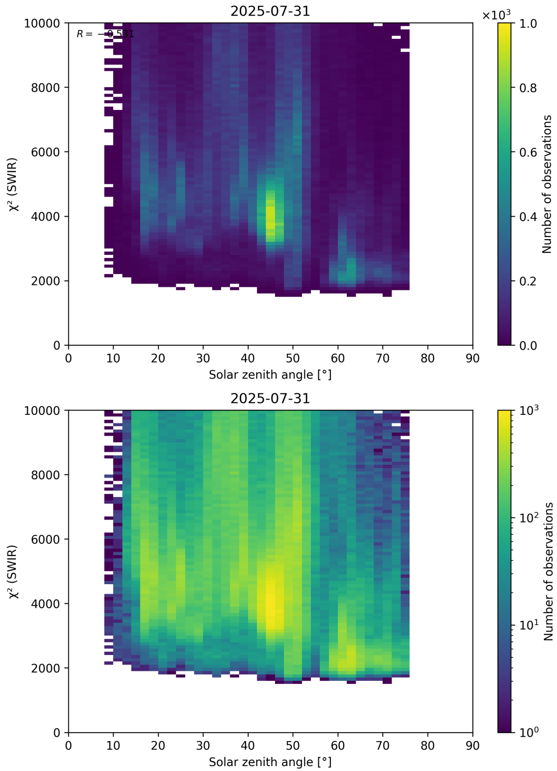
Figure 95: Scatter density plot of “Solar zenith angle” against “ \chi^2 (SWIR)” for 2025-07-30 to 2025-08-01.
