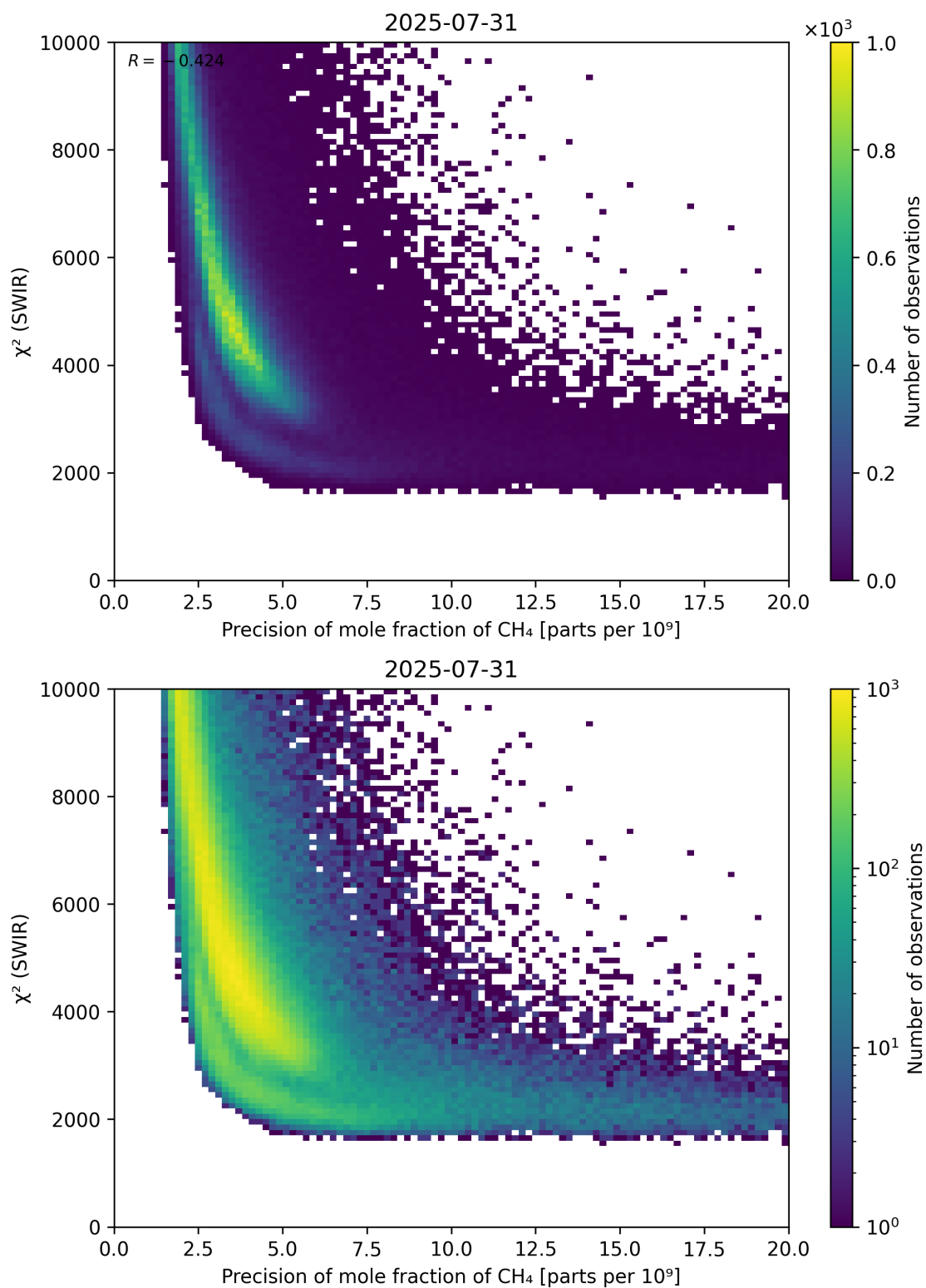
Figure 79: Scatter density plot of “Precision of mole fraction of \text{CH}_4 ” against “ \chi^2 (SWIR)” for 2025-07-30 to 2025-08-01.
