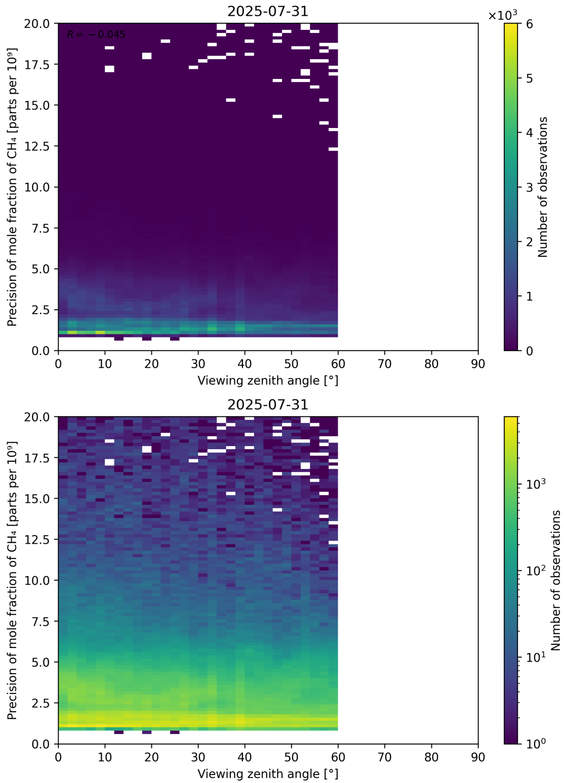
Figure 112: Scatter density plot of “Viewing zenith angle” against “Precision of mole fraction of CH 4 ” for 2025-07-30 to 2025-08-01.
