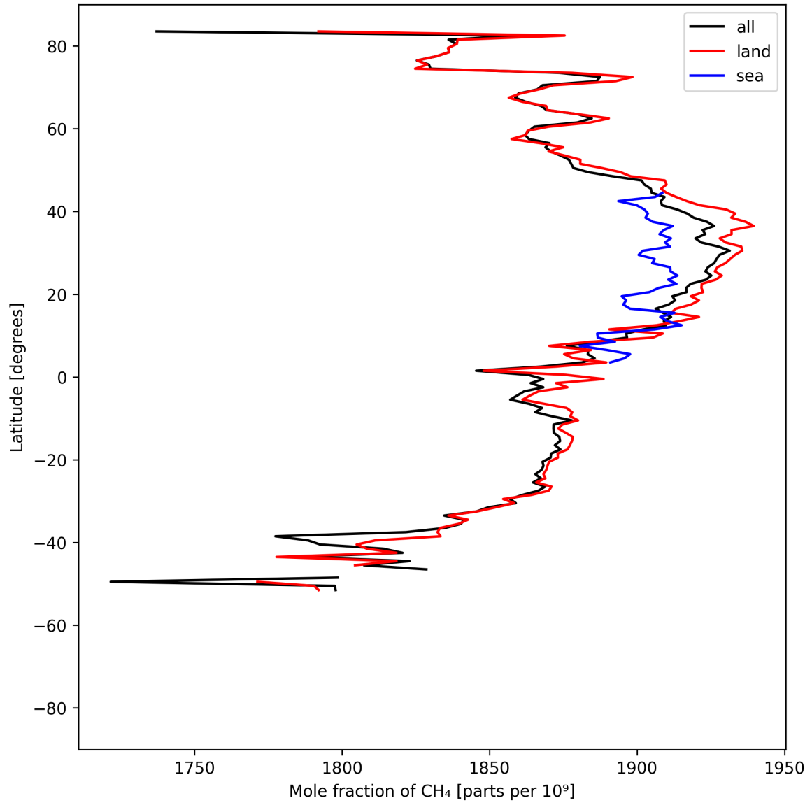
Figure 12: Zonal average of “Mole fraction of \text{CH}_4 ” for 2025-07-30 to 2025-08-01.
