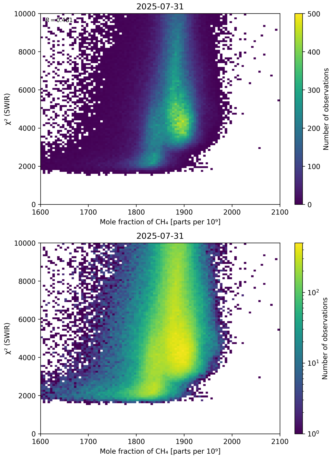
Figure 71: Scatter density plot of “Mole fraction of \text{CH}_4 ” against “ \chi^2 (SWIR)” for 2025-07-30 to 2025-08-01.
