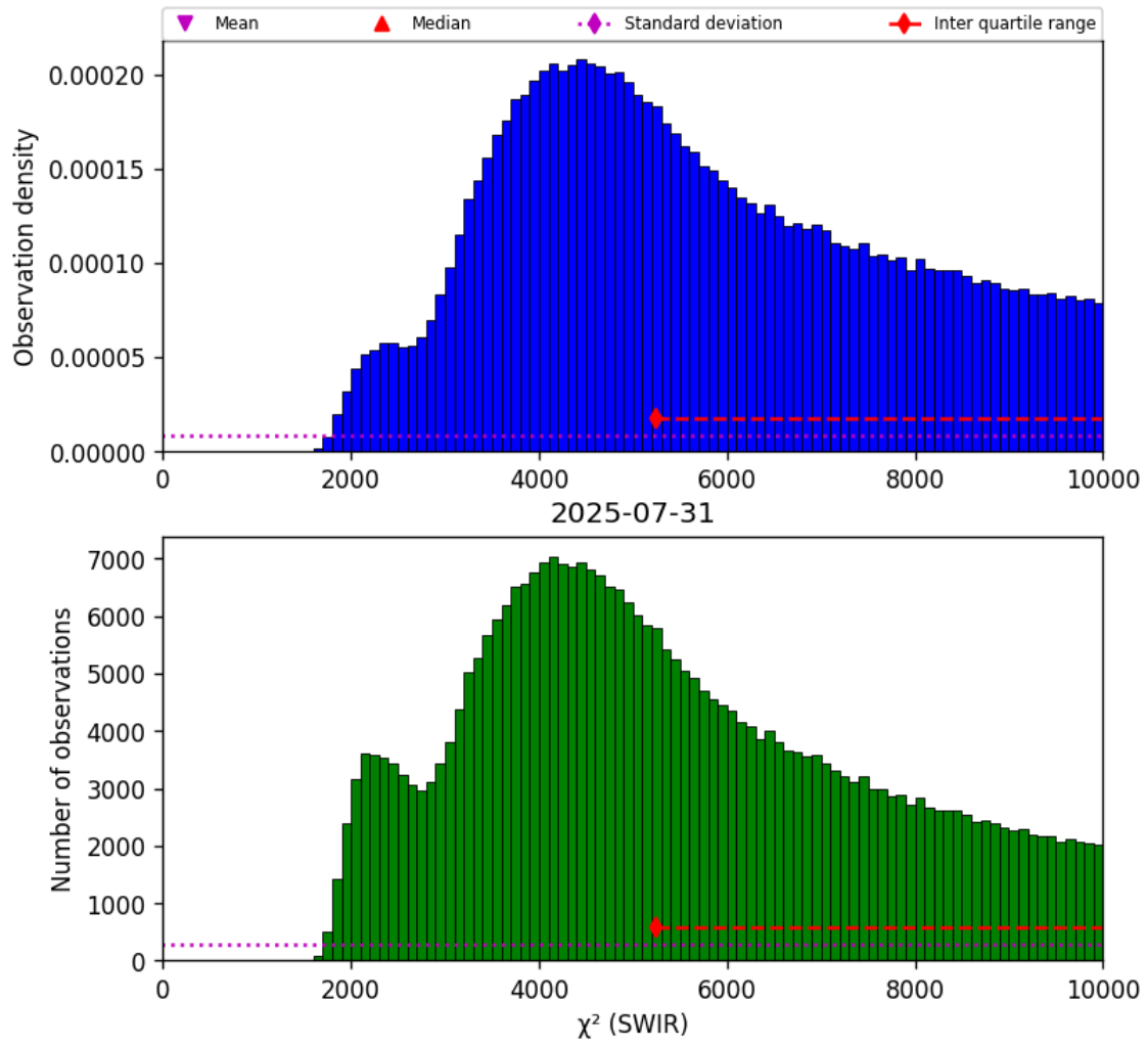
Figure 28: Histogram of “ \chi^2 (SWIR)” for 2025-07-30 to 2025-08-01
