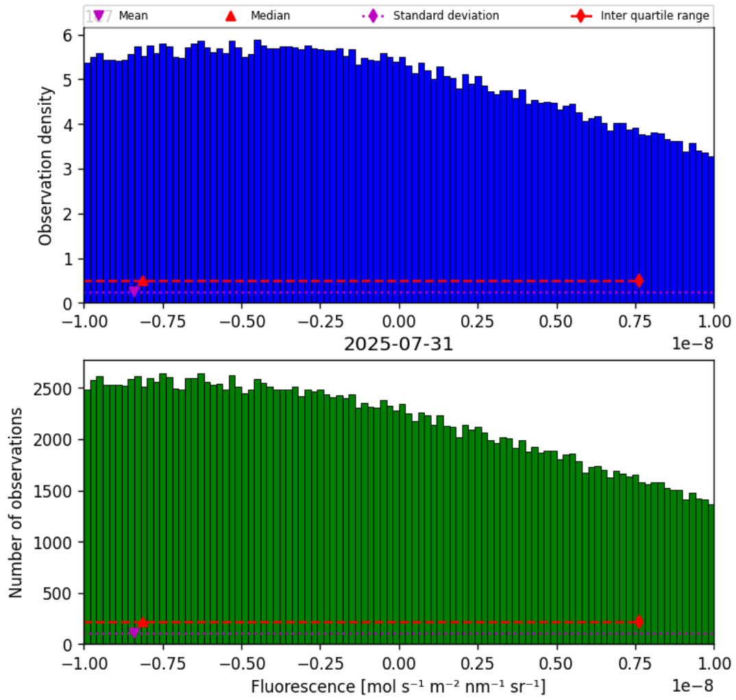
Figure 32: Histogram of “Fluorescence” for 2025-07-30 to 2025-08-01
