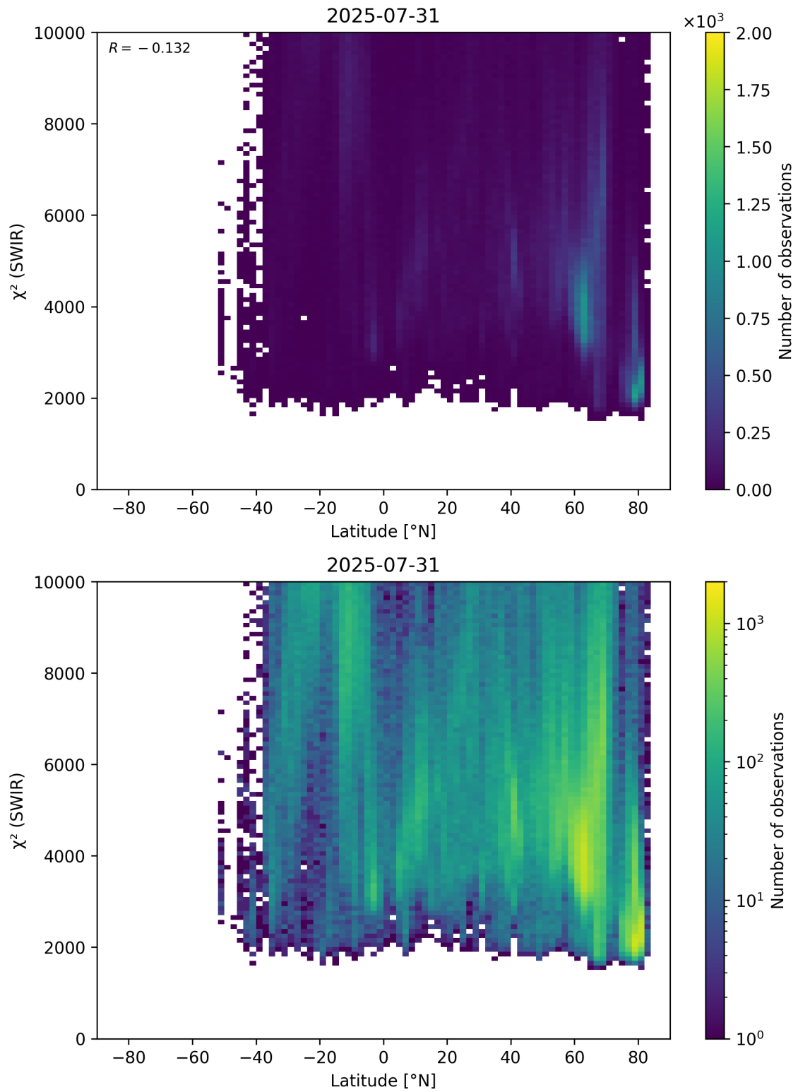
Figure 54: Scatter density plot of “Latitude” against “ \chi^2 (SWIR)” for 2025-07-30 to 2025-08-01.
