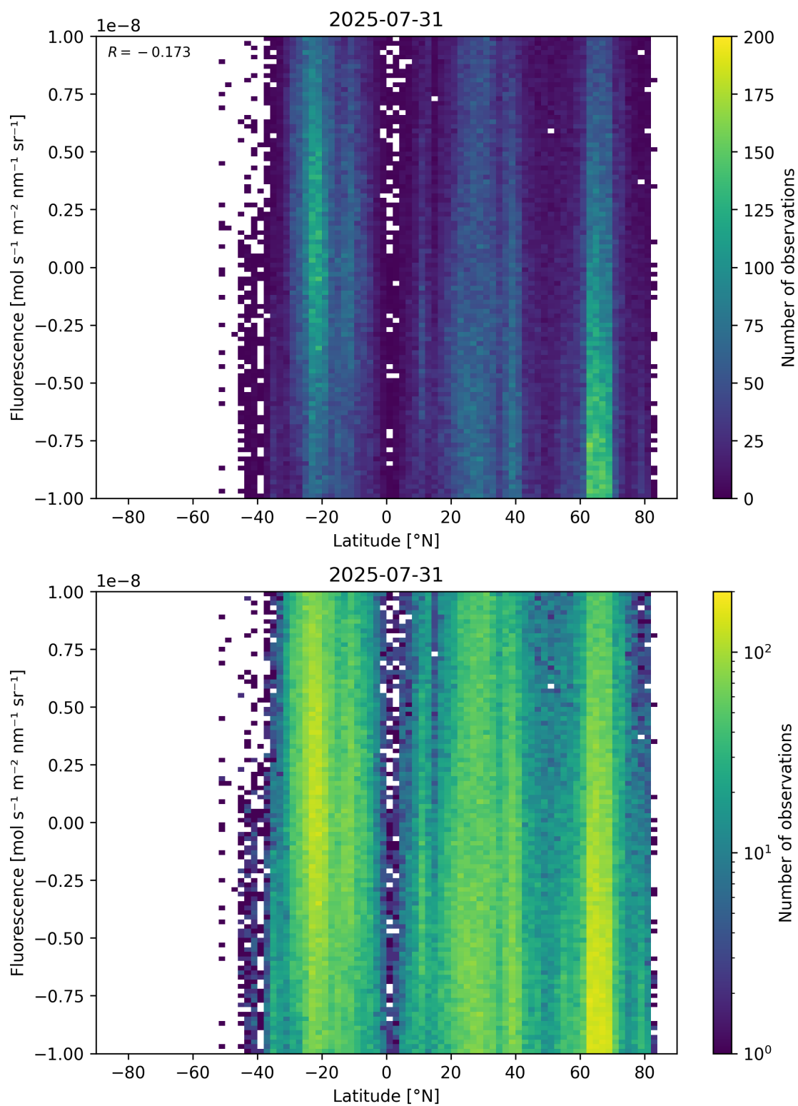
Figure 56: Scatter density plot of “Latitude” against “Fluorescence” for 2025-07-30 to 2025-08-01.
