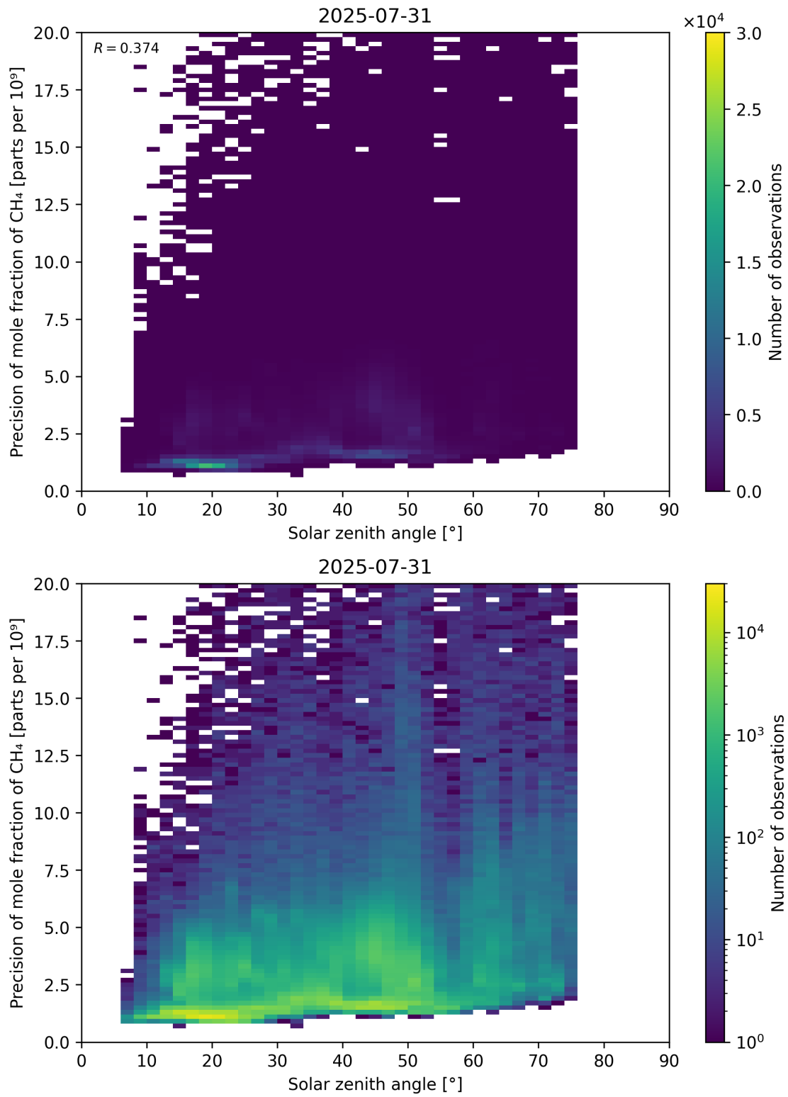
Figure 101: Scatter density plot of “Solar zenith angle” against “Precision of mole fraction of CH 4 ” for 2025-07-30 to 2025-08-01.
