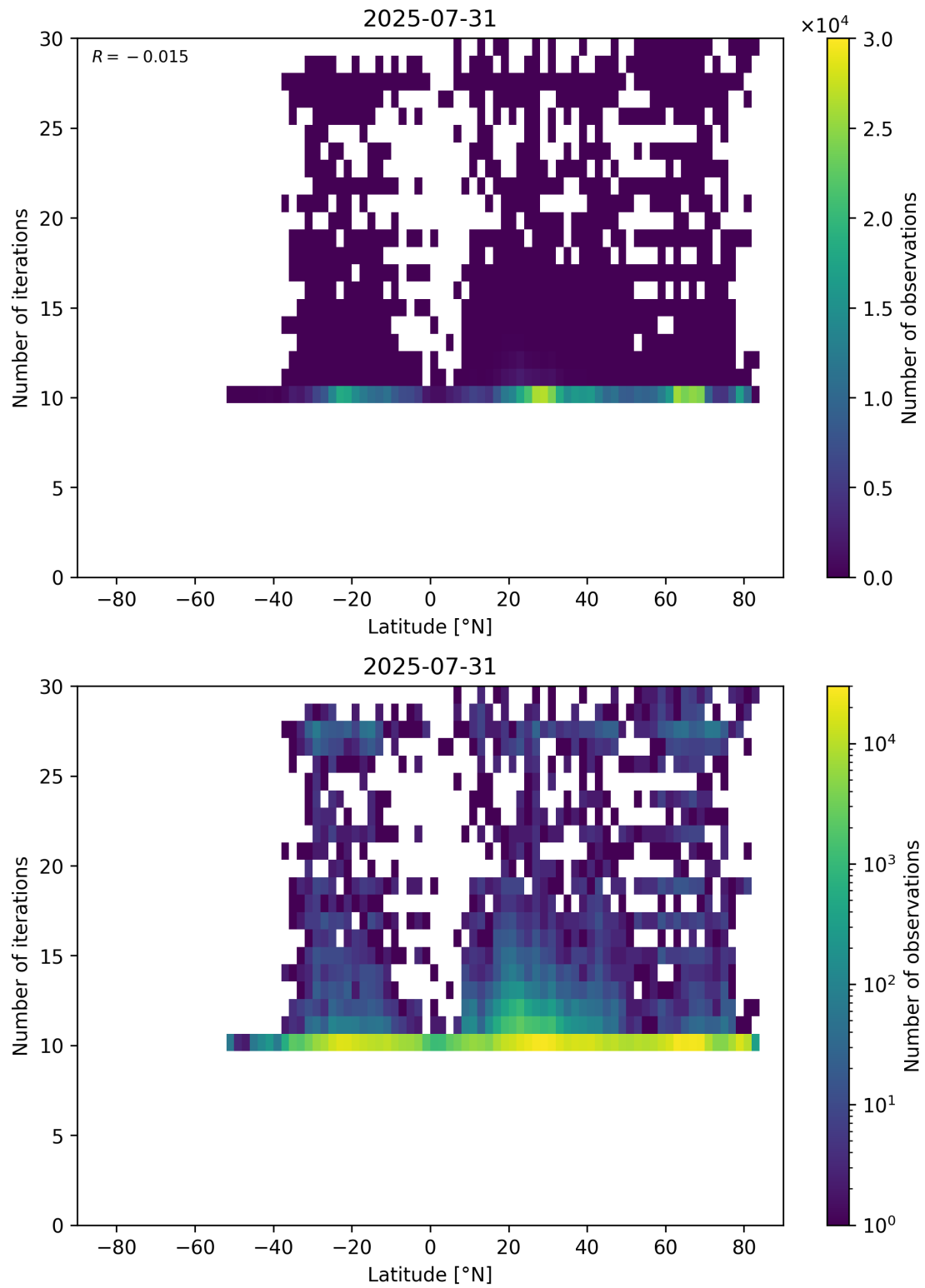
Figure 60: Scatter density plot of “Latitude” against “Number of iterations” for 2025-07-30 to 2025-08-01.
