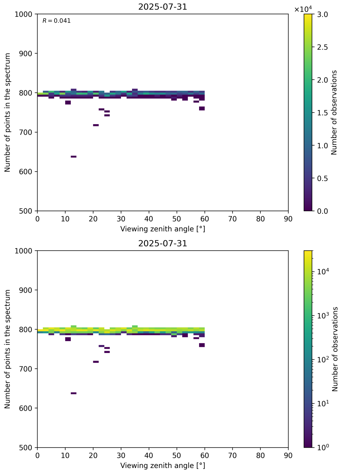
Figure 114: Scatter density plot of “Viewing zenith angle” against “Number of points in the spectrum” for 2025-07-30 to 2025-08-01.
