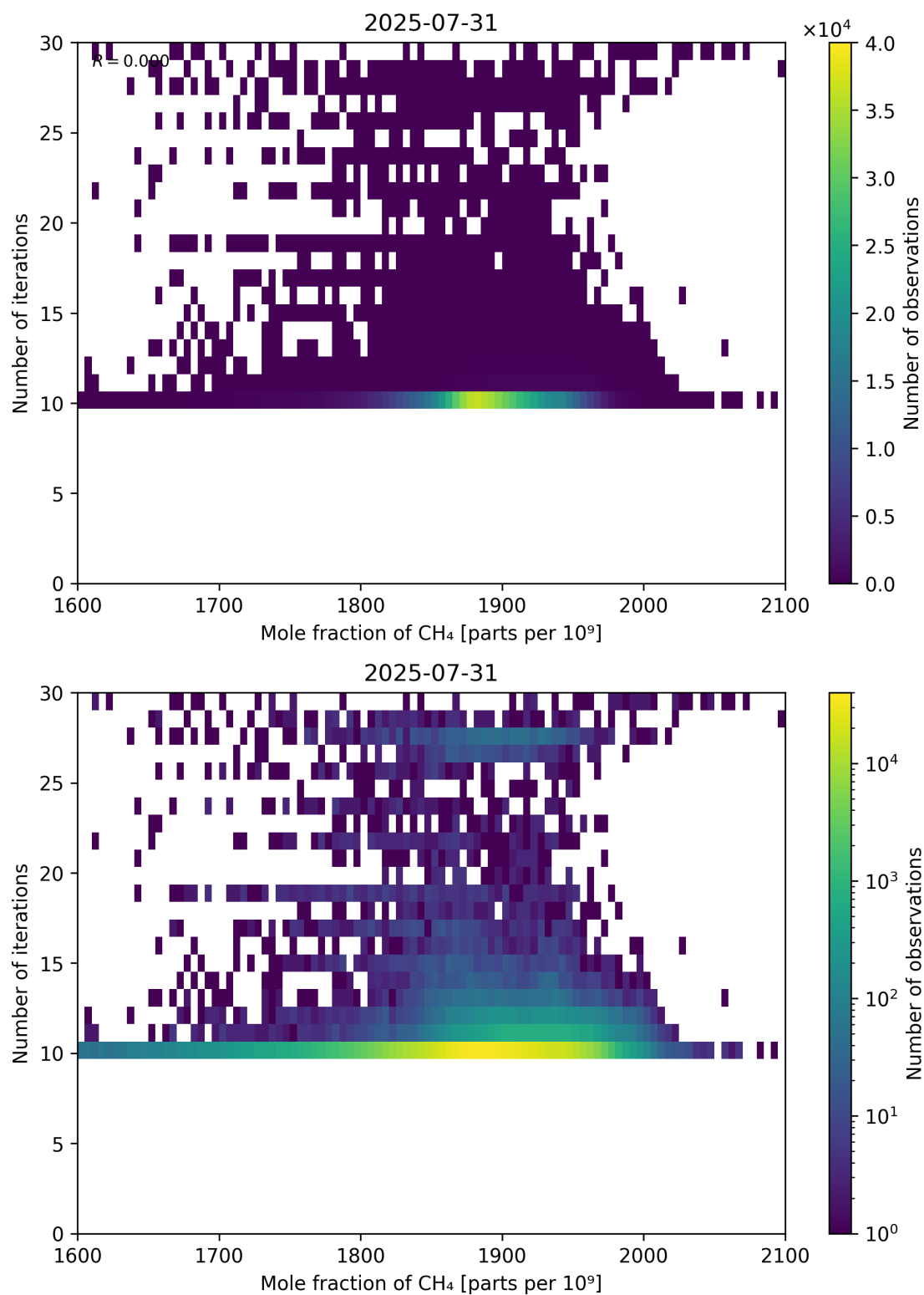
Figure 76: Scatter density plot of “Mole fraction of CH 4 ” against “Number of iterations” for 2025-07-30 to 2025-08-01.
