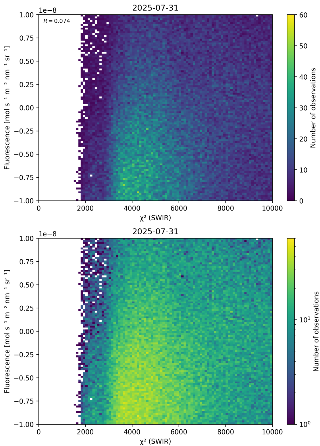
Figure 49: Scatter density plot of “ \chi^2 (SWIR)” against “Fluorescence” for 2025-07-30 to 2025-08-01.
