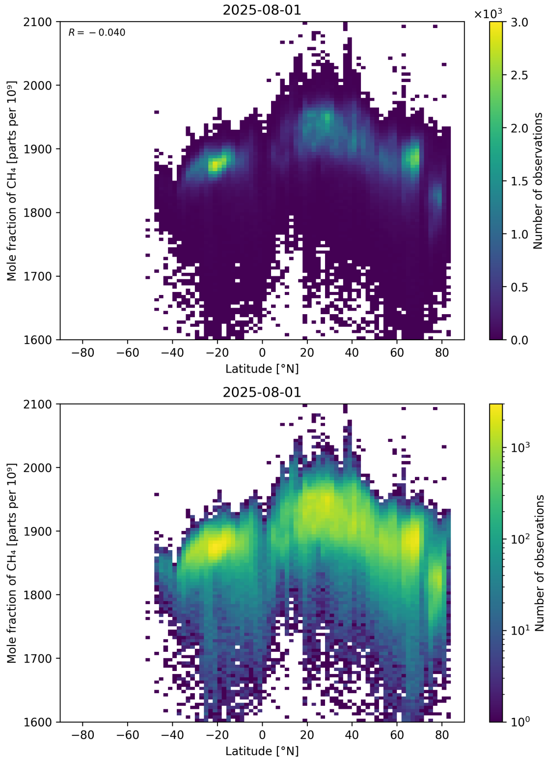
Figure 57: Scatter density plot of “Latitude” against “Mole fraction of CH 4 ” for 2025-07-31 to 2025-08-02.
