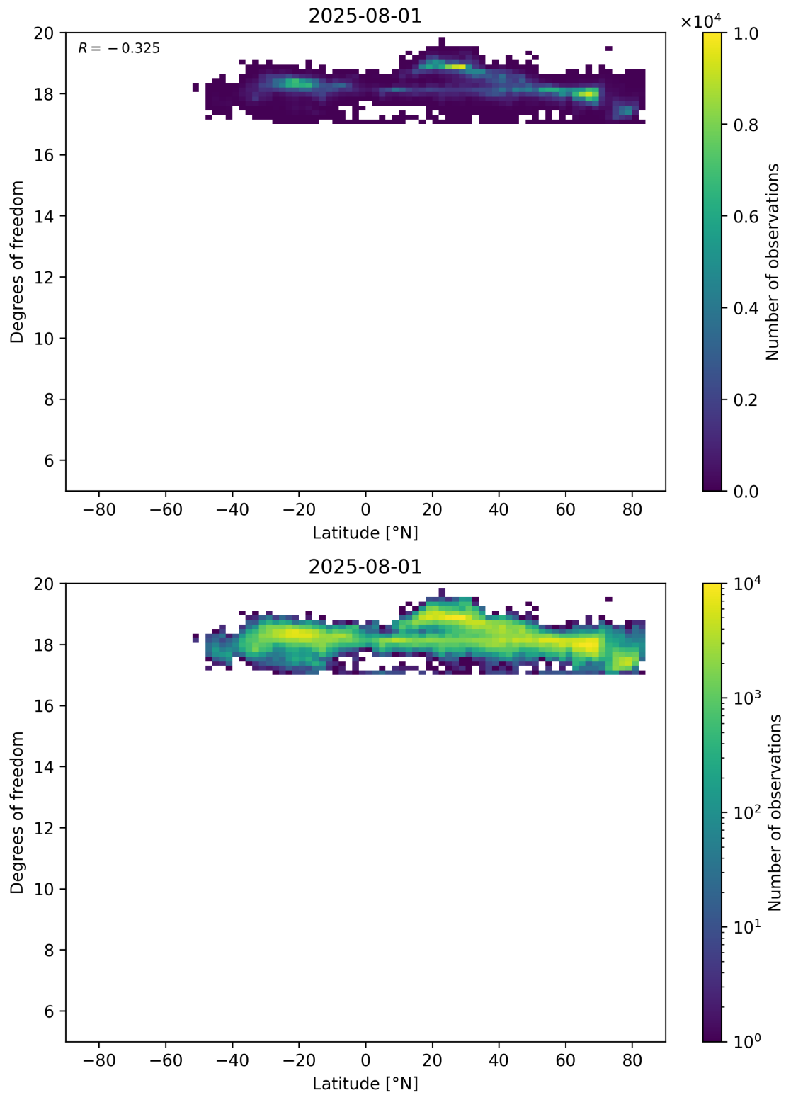
Figure 55: Scatter density plot of “Latitude” against “Degrees of freedom” for 2025-07-31 to 2025-08-02.
