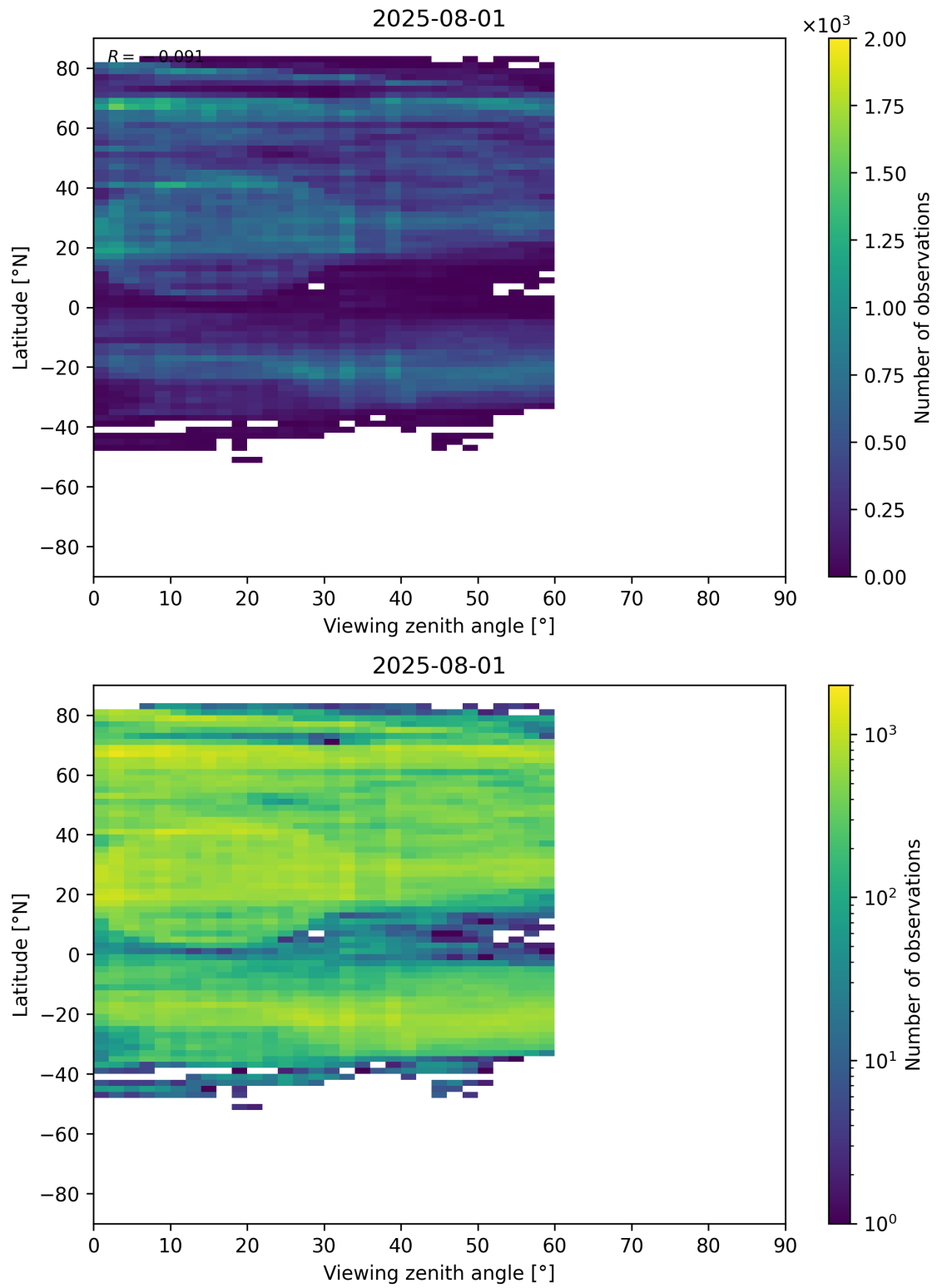
Figure 109: Scatter density plot of “Viewing zenith angle” against “Latitude” for 2025-07-31 to 2025-08-02.
