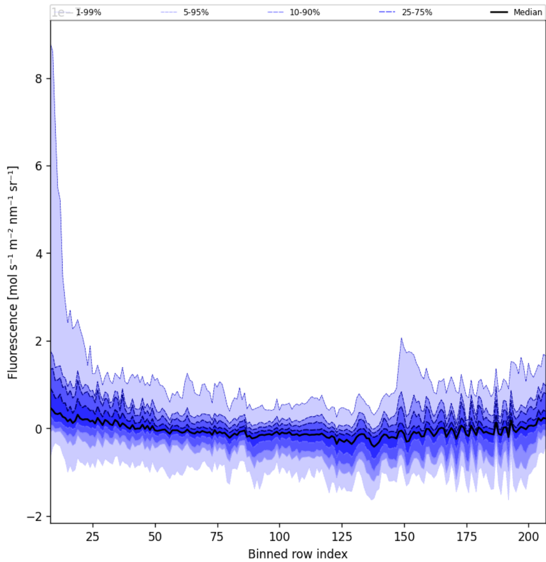
Figure 43: Along track statistics of “Fluorescence” for 2025-07-31 to 2025-08-02
