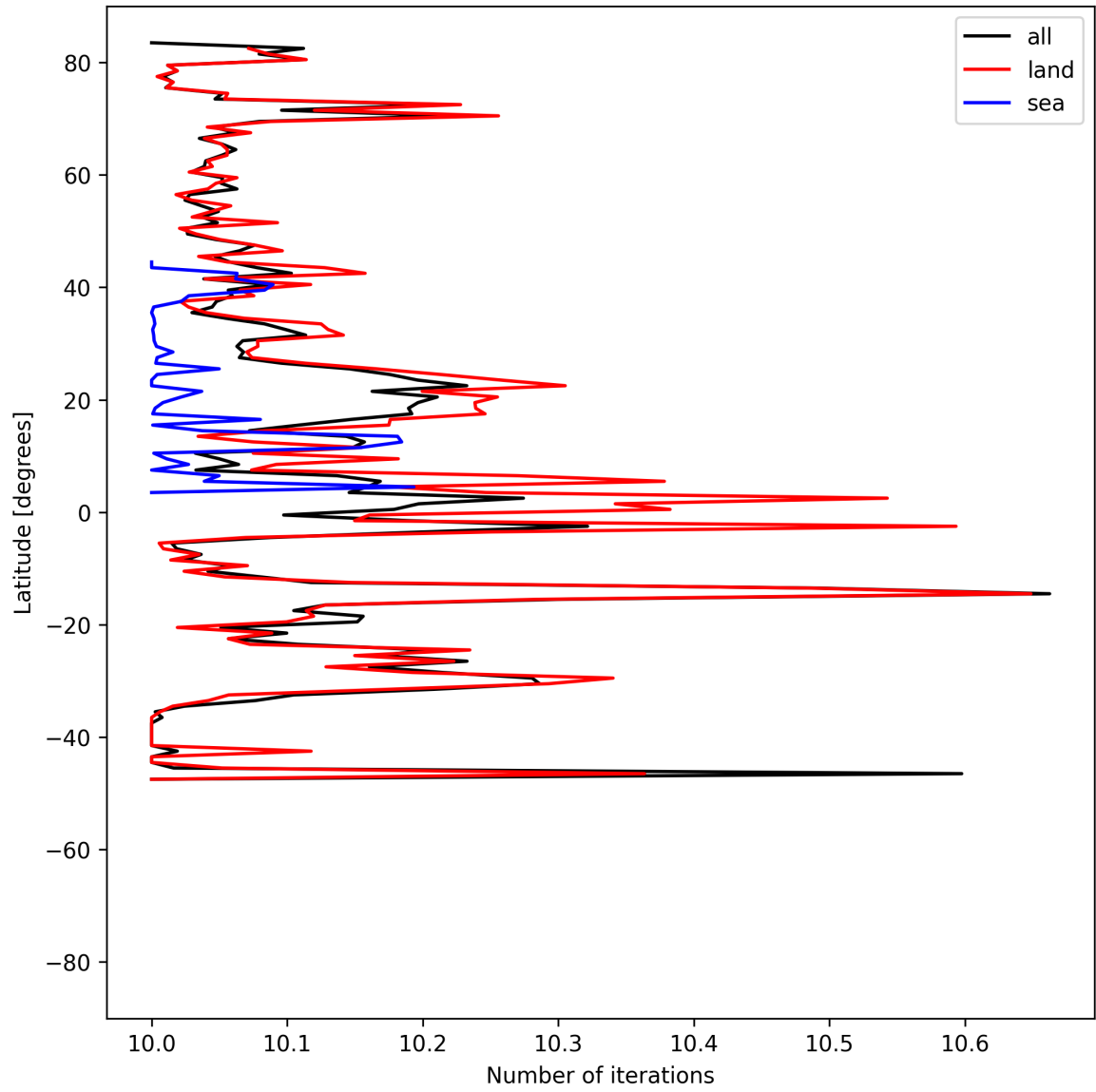
Figure 20: Zonal average of “Number of iterations” for 2025-07-31 to 2025-08-02.
