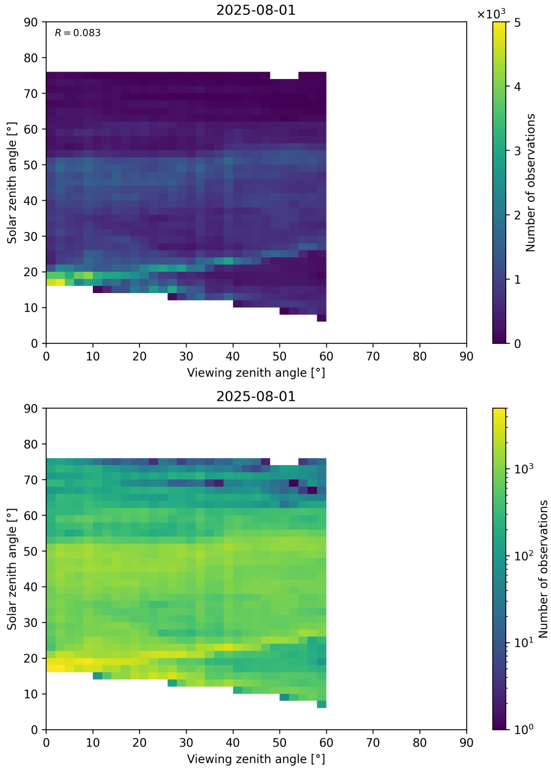
Figure 115: Scatter density plot of “Viewing zenith angle” against “Solar zenith angle” for 2025-07-31 to 2025-08-02.
