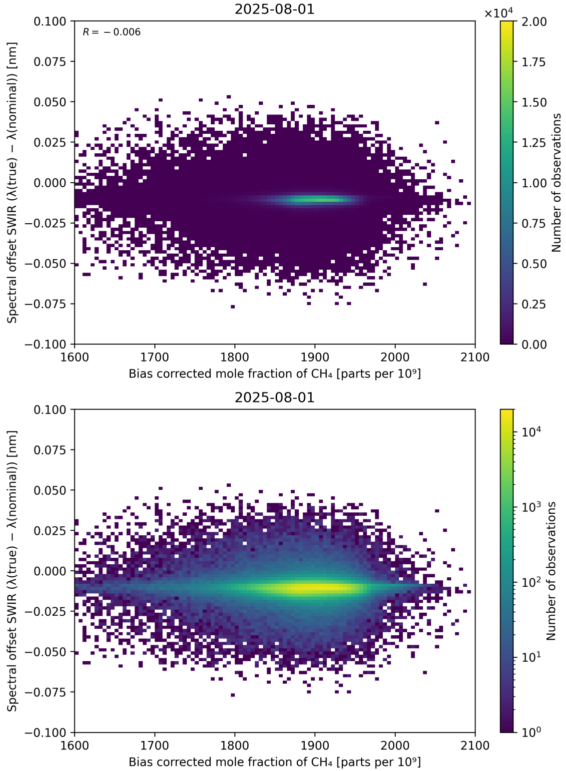
Figure 69: Scatter density plot of “Bias corrected mole fraction of \text{CH}_4 ” against “Spectral offset SWIR ( \lambda_{\text{true}} - \lambda_{\text{nominal}} )” for 2025-07-31 to 2025-08-02.
