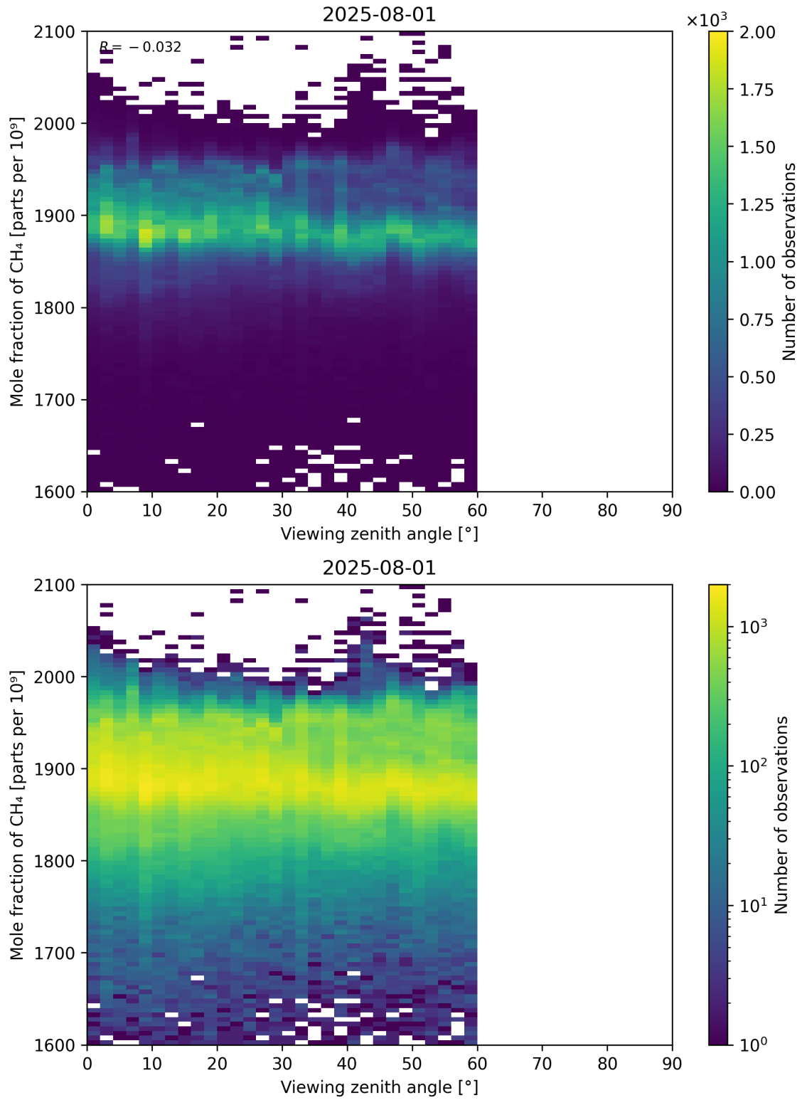
Figure 110: Scatter density plot of “Viewing zenith angle” against “Mole fraction of CH 4 ” for 2025-07-31 to 2025-08-02.
