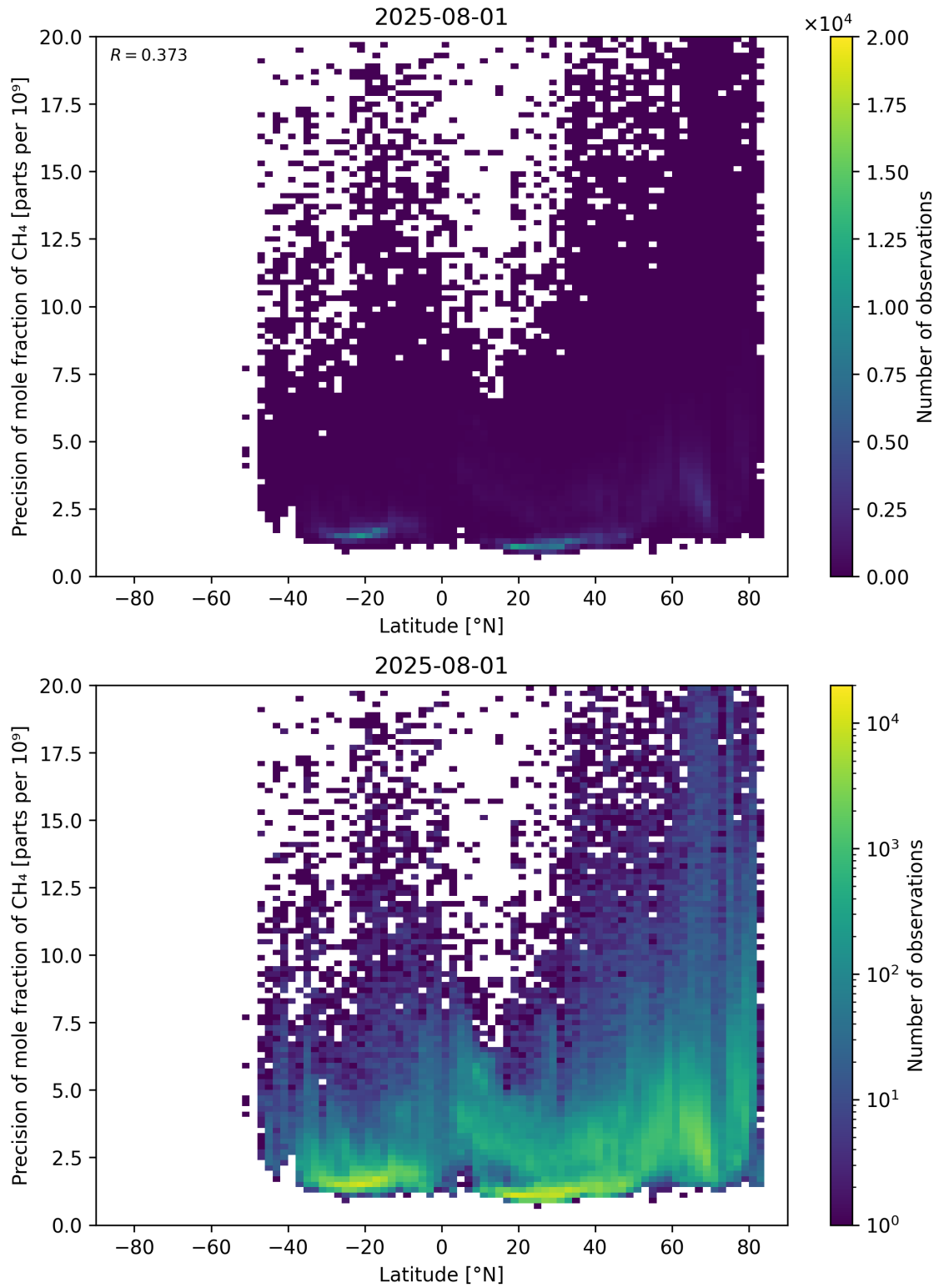
Figure 59: Scatter density plot of “Latitude” against “Precision of mole fraction of \text{CH}_4 ” for 2025-07-31 to 2025-08-02.
