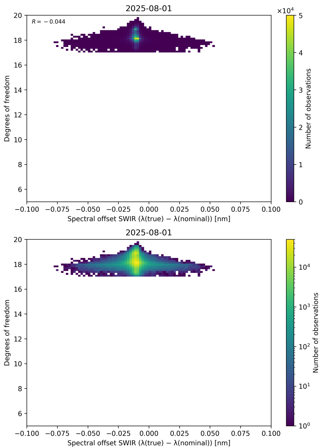
Figure 119: Scatter density plot of “Spectral offset SWIR ( \lambda_{\text{true}} - \lambda_{\text{nominal}} )” against “Degrees of freedom” for 2025-07-31 to 2025-08-02.
