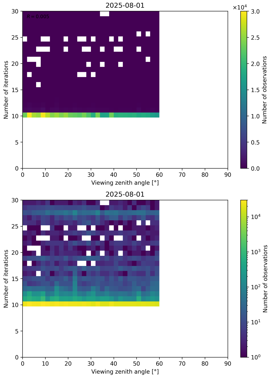
Figure 113: Scatter density plot of “Viewing zenith angle” against “Number of iterations” for 2025-07-31 to 2025-08-02.
