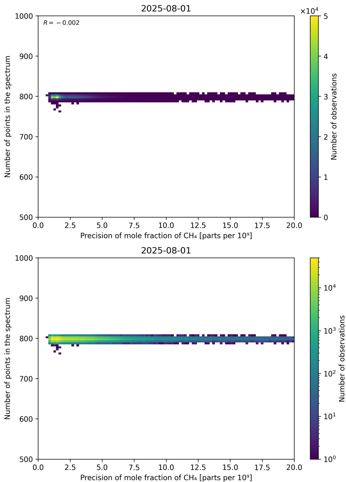
Figure 84: Scatter density plot of “Precision of mole fraction of CH 4 ” against “Number of points in the spectrum” for 2025-07-31 to 2025-08-02.
