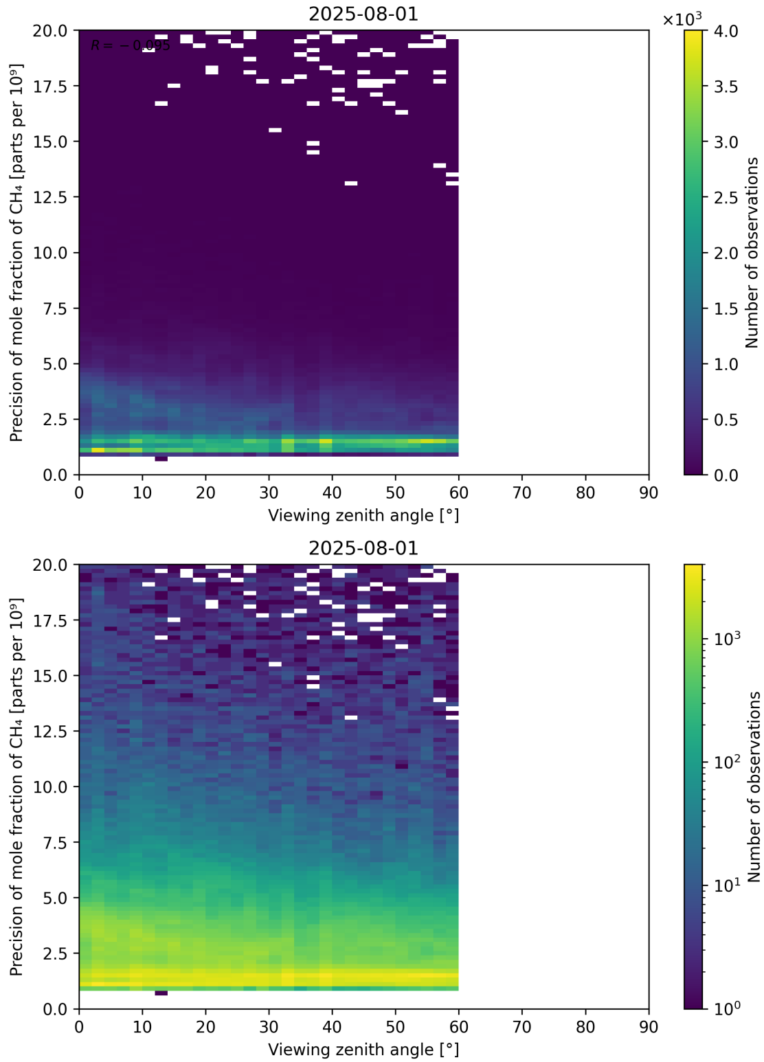
Figure 112: Scatter density plot of “Viewing zenith angle” against “Precision of mole fraction of CH 4 ” for 2025-07-31 to 2025-08-02.
