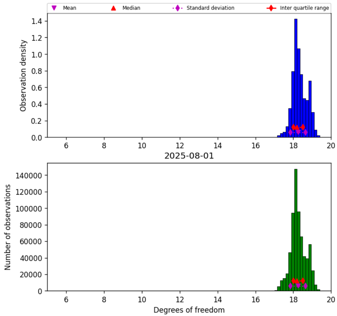
Figure 30: Histogram of “Degrees of freedom” for 2025-07-31 to 2025-08-02
