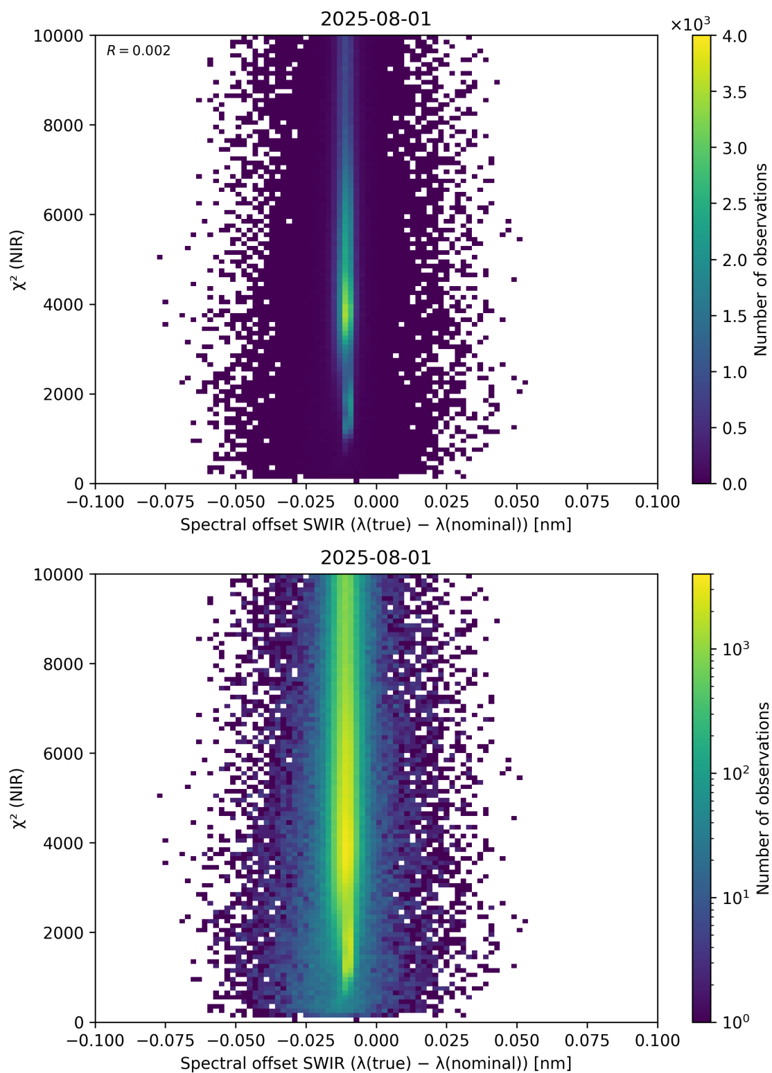
Figure 117: Scatter density plot of “Spectral offset SWIR ( \lambda_{\text{true}} - \lambda_{\text{nominal}} )” against “ \chi^2 (NIR)” for 2025-07-31 to 2025-08-02.
