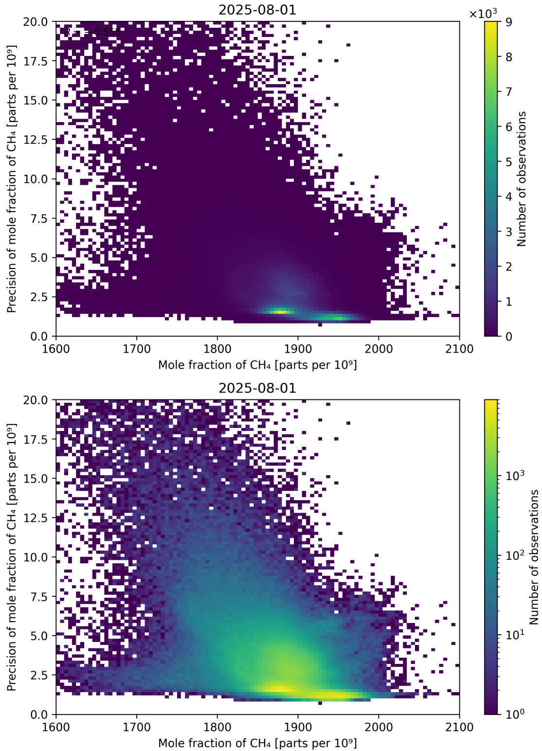
Figure 75: Scatter density plot of “Mole fraction of CH 4 ” against “Precision of mole fraction of CH 4 ” for 2025-07-31 to 2025-08-02.
