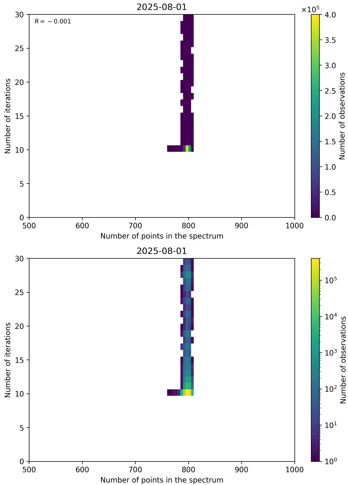
Figure 92: Scatter density plot of “Number of points in the spectrum” against “Number of iterations” for 2025-07-31 to 2025-08-02.
