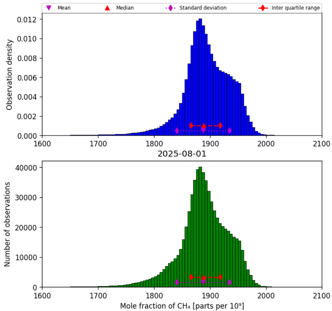
Figure 23: Histogram of “Mole fraction of CH 4 ” for 2025-07-31 to 2025-08-02
