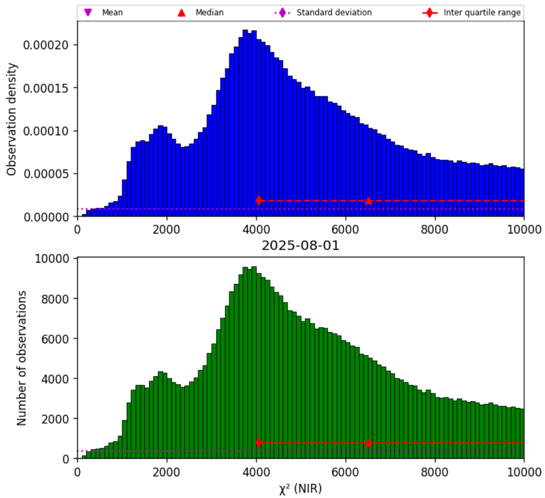
Figure 29: Histogram of " \chi^2 (NIR)" for 2025-07-31 to 2025-08-02
