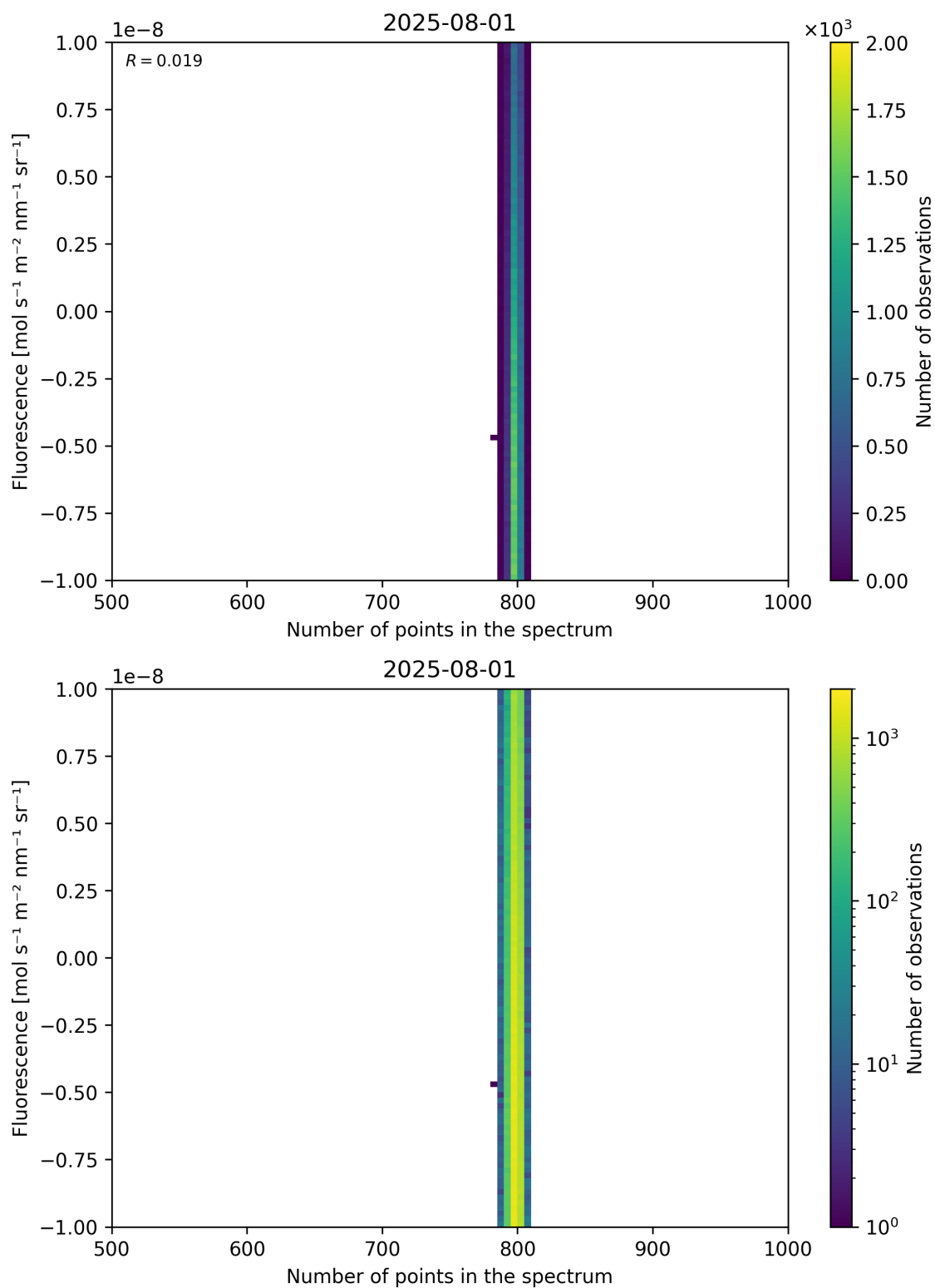
Figure 91: Scatter density plot of “Number of points in the spectrum” against “Fluorescence” for 2025-07-31 to 2025-08-02.
