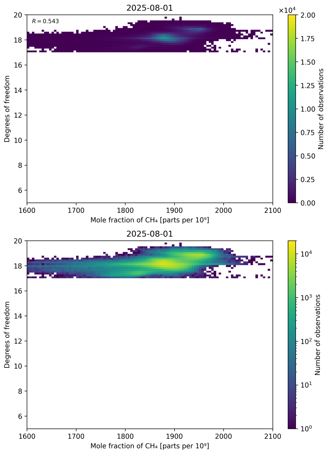
Figure 72: Scatter density plot of “Mole fraction of CH 4 ” against “Degrees of freedom” for 2025-07-31 to 2025-08-02.
