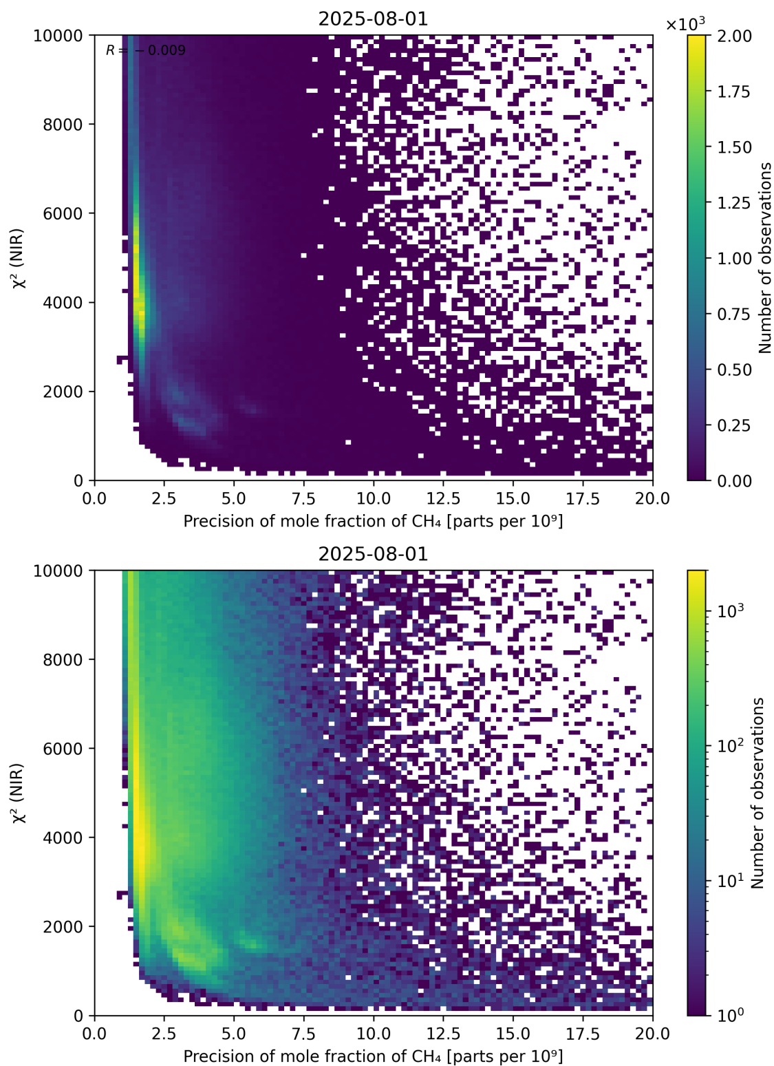
Figure 78: Scatter density plot of “Precision of mole fraction of CH 4 ” against “ \chi^2 (NIR)” for 2025-07-31 to 2025-08-02.
