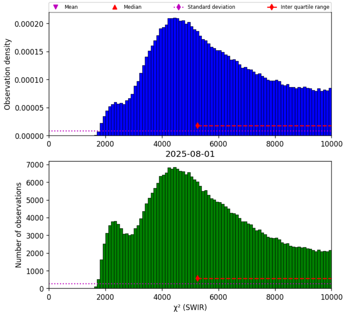
Figure 28: Histogram of " \chi^2 (SWIR)" for 2025-07-31 to 2025-08-02
