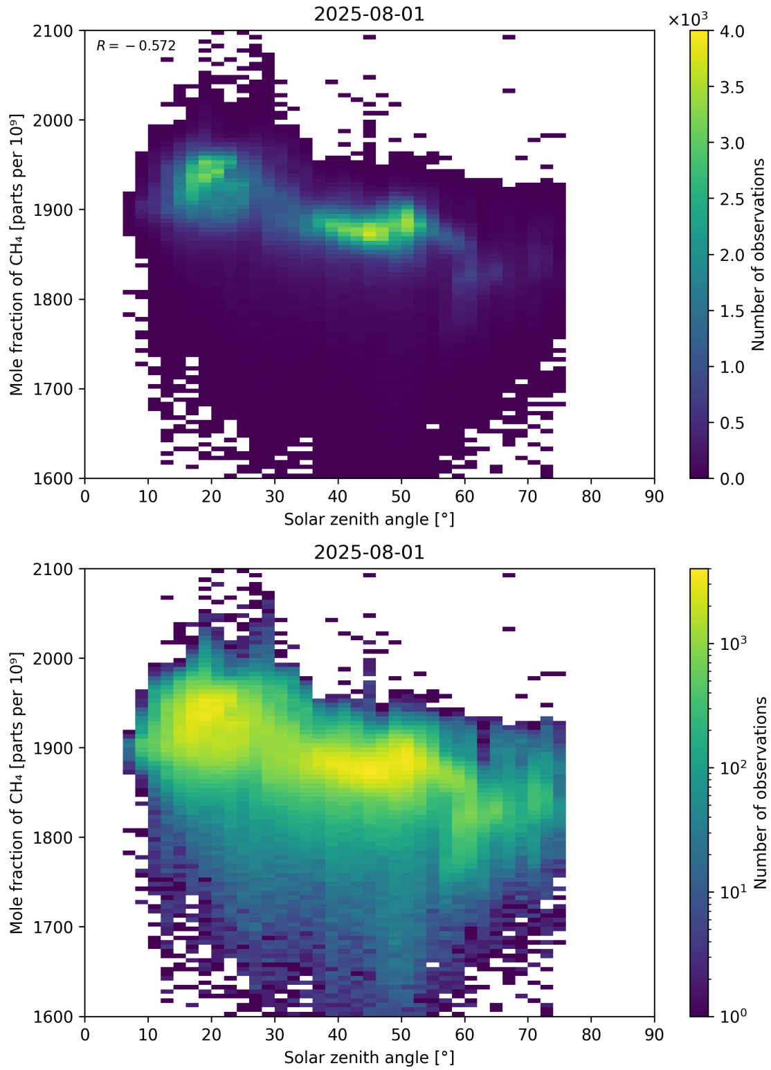
Figure 99: Scatter density plot of “Solar zenith angle” against “Mole fraction of CH 4 ” for 2025-07-31 to 2025-08-02.
