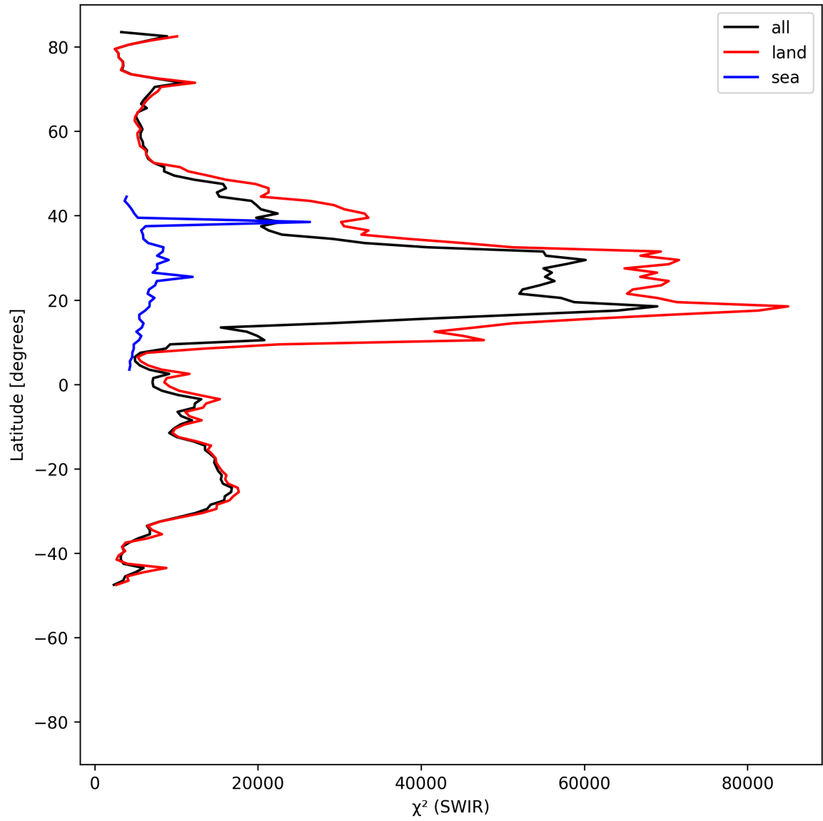
Figure 17: Zonal average of “ \chi^2 (SWIR)” for 2025-07-31 to 2025-08-02.
