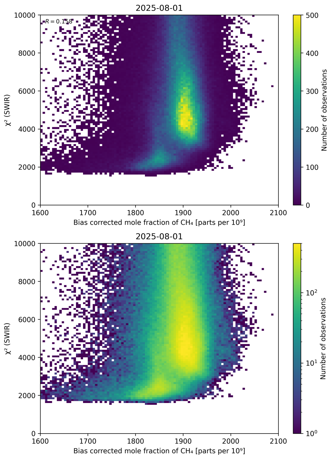
Figure 64: Scatter density plot of “Bias corrected mole fraction of \text{CH}_4 ” against “ \chi^2 (SWIR)” for 2025-07-31 to 2025-08-02.
