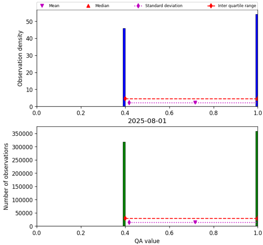
Figure 22: Histogram of “QA value” for 2025-07-31 to 2025-08-02
