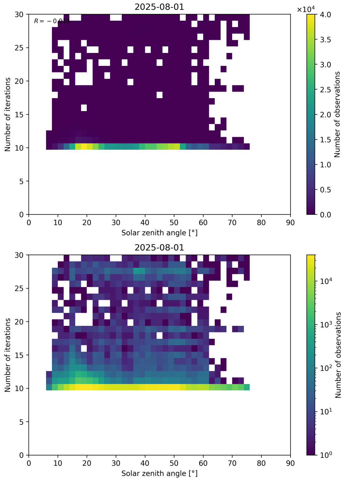
Figure 102: Scatter density plot of “Solar zenith angle” against “Number of iterations” for 2025-07-31 to 2025-08-02.
