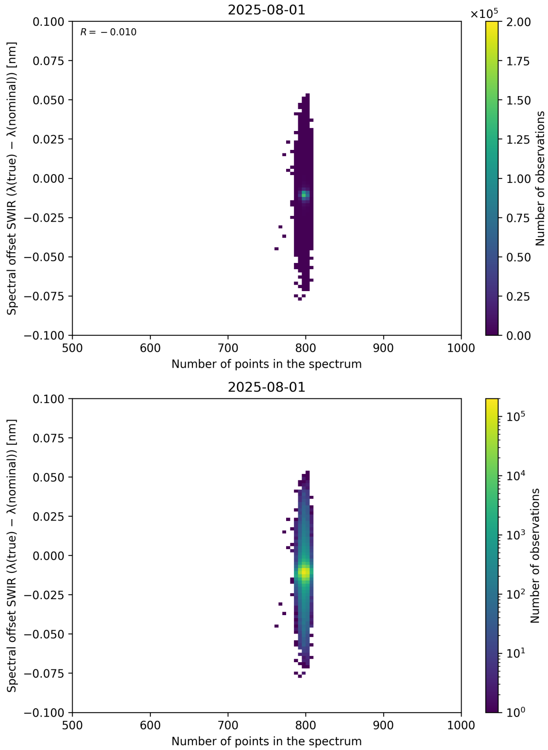
Figure 93: Scatter density plot of “Number of points in the spectrum” against “Spectral offset SWIR ( \lambda_{\text{true}} - \lambda_{\text{nominal}} )” for 2025-07-31 to 2025-08-02.
