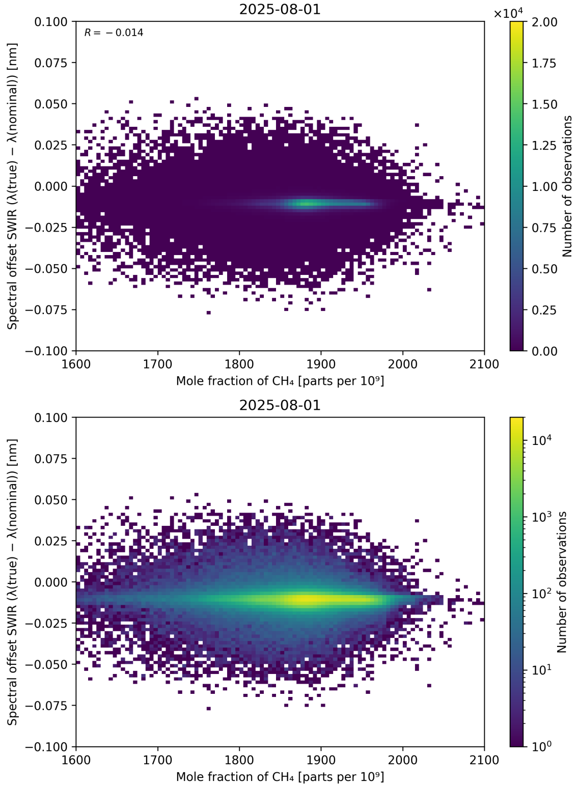
Figure 86: Scatter density plot of “Mole fraction of CH 4 ” against “Spectral offset SWIR ( \lambda_{\text{true}} - \lambda_{\text{nominal}} )” for 2025-07-31 to 2025-08-02.
