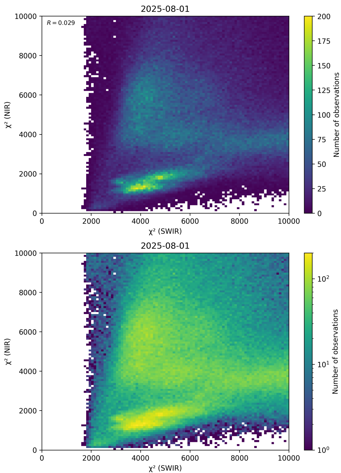
Figure 47: Scatter density plot of “ \chi^2 (SWIR)” against “ \chi^2 (NIR)” for 2025-07-31 to 2025-08-02.
