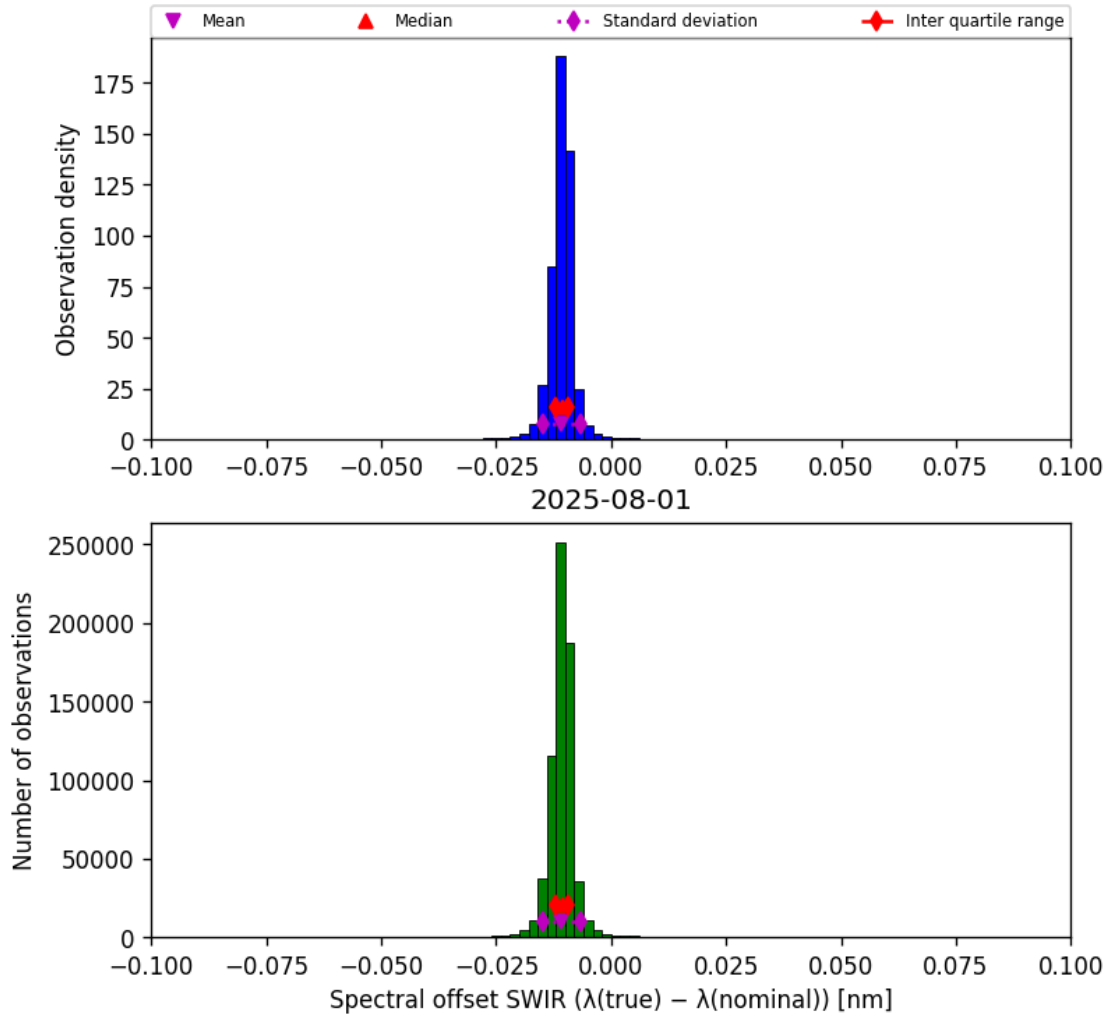
Figure 27: Histogram of “Spectral offset SWIR ( \lambda_{\text{true}} - \lambda_{\text{nominal}} )” for 2025-07-31 to 2025-08-02
