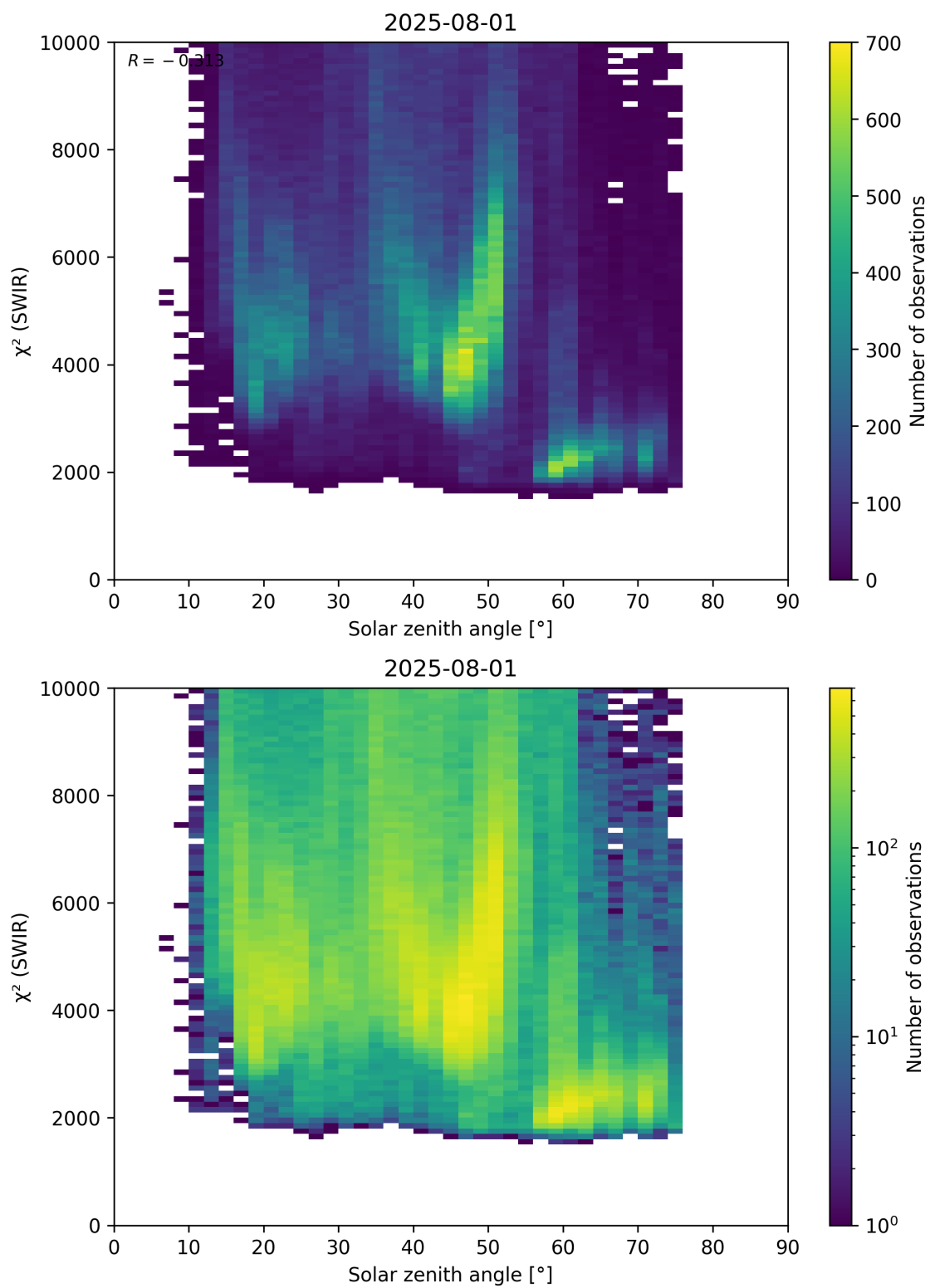
Figure 95: Scatter density plot of “Solar zenith angle” against “ \chi^2 (SWIR)” for 2025-07-31 to 2025-08-02.
