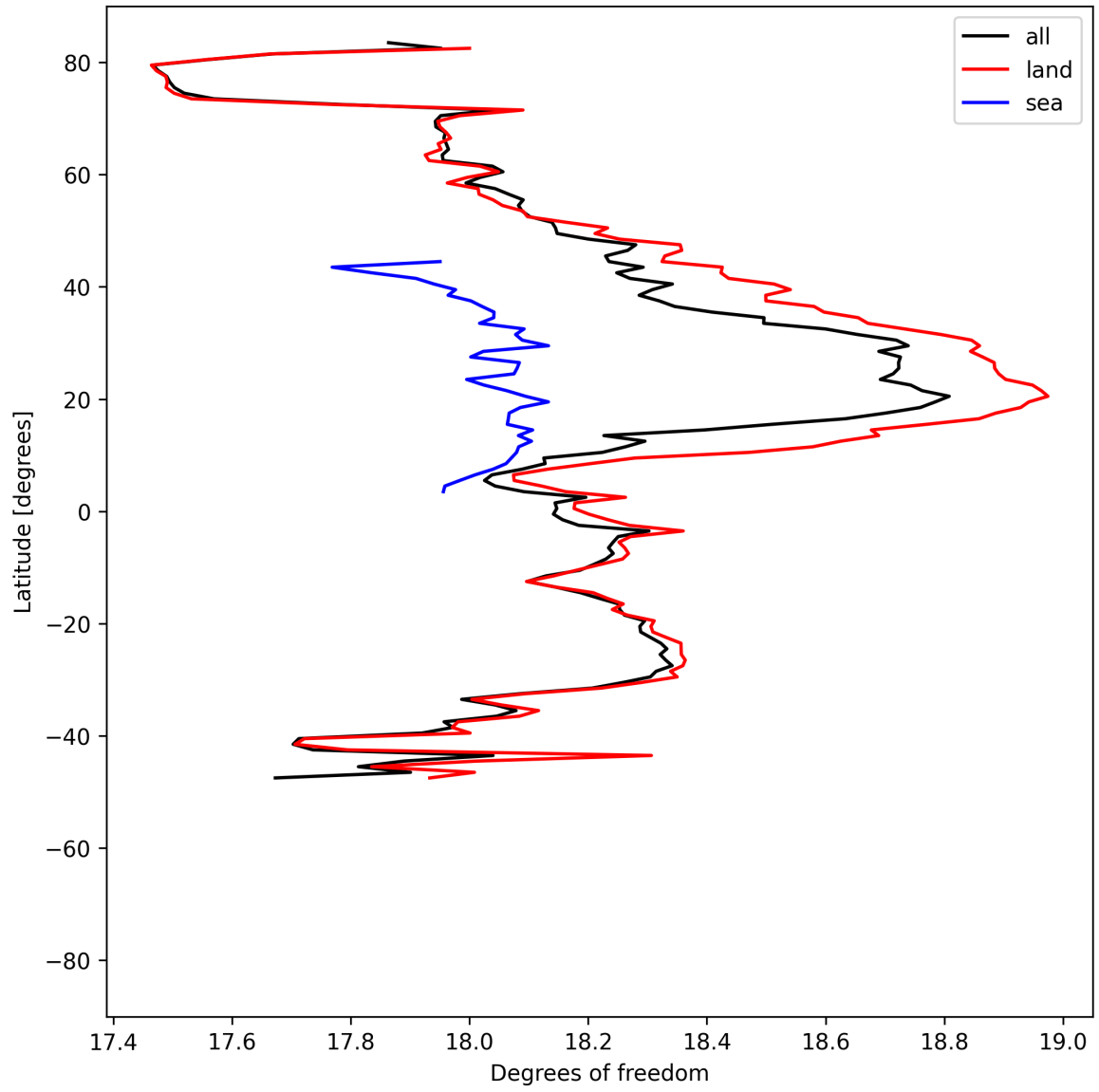
Figure 19: Zonal average of “Degrees of freedom” for 2025-07-31 to 2025-08-02.
