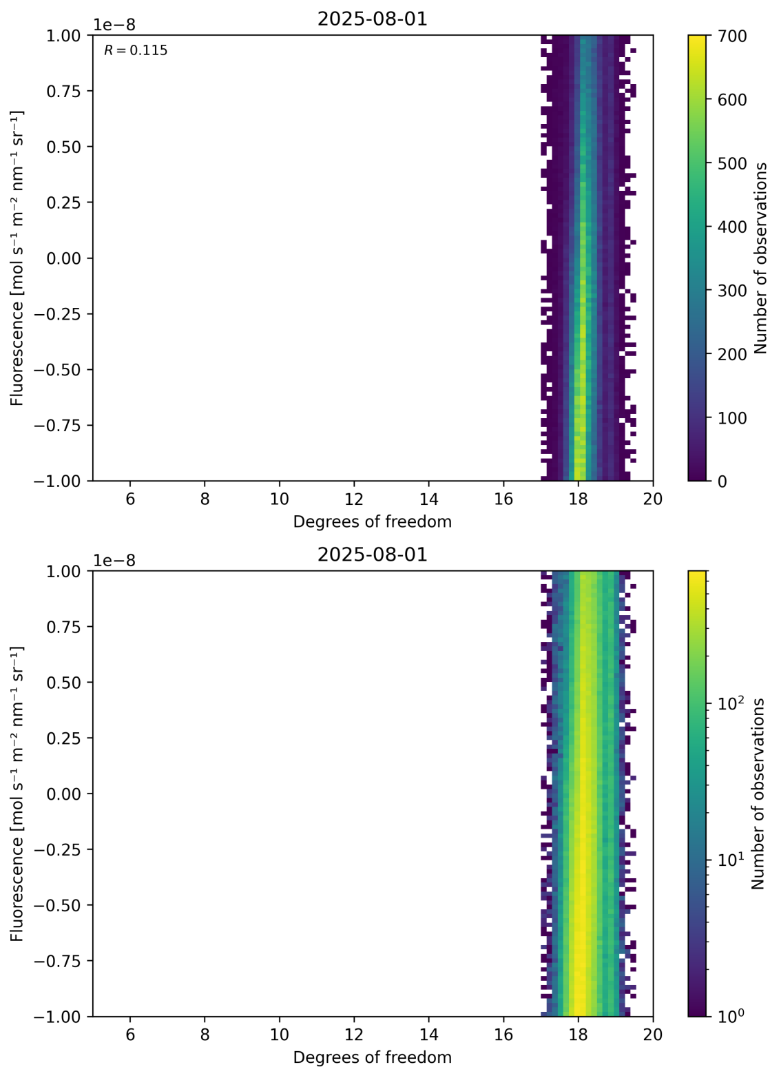
Figure 51: Scatter density plot of “Degrees of freedom” against “Fluorescence” for 2025-07-31 to 2025-08-02.
