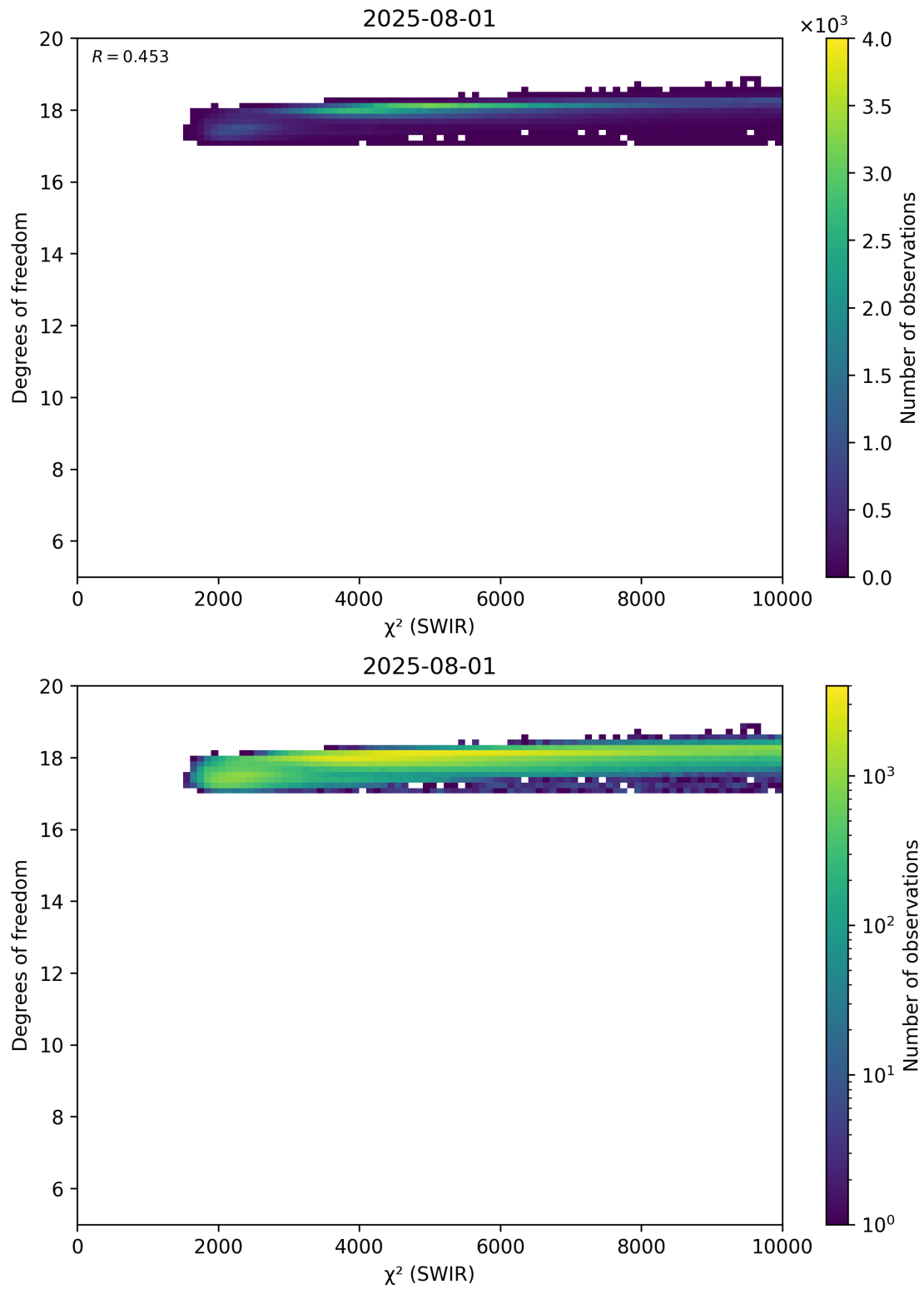
Figure 48: Scatter density plot of “ \chi^2 (SWIR)” against “Degrees of freedom” for 2025-07-31 to 2025-08-02.
