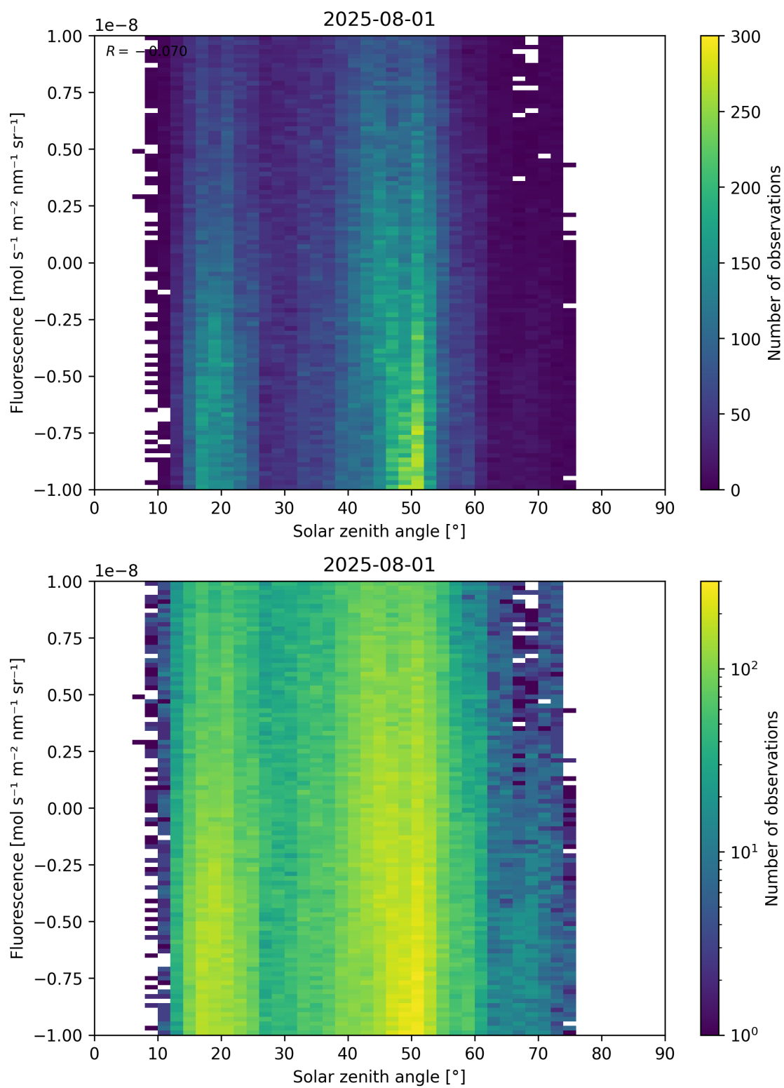
Figure 97: Scatter density plot of “Solar zenith angle” against “Fluorescence” for 2025-07-31 to 2025-08-02.
