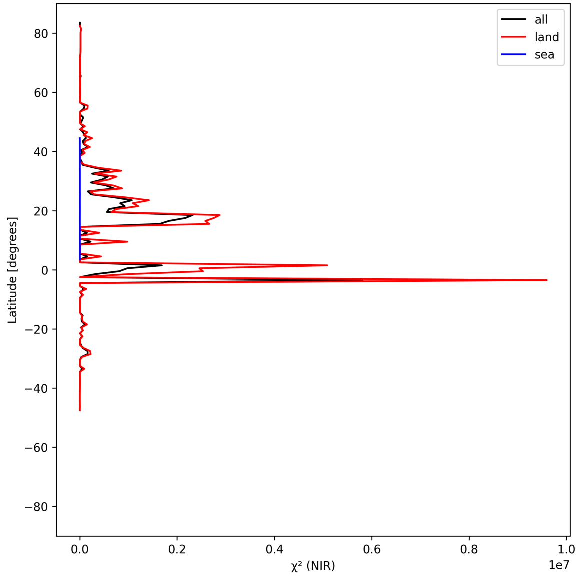
Figure 18: Zonal average of “ \chi^2 (NIR)” for 2025-07-31 to 2025-08-02.
