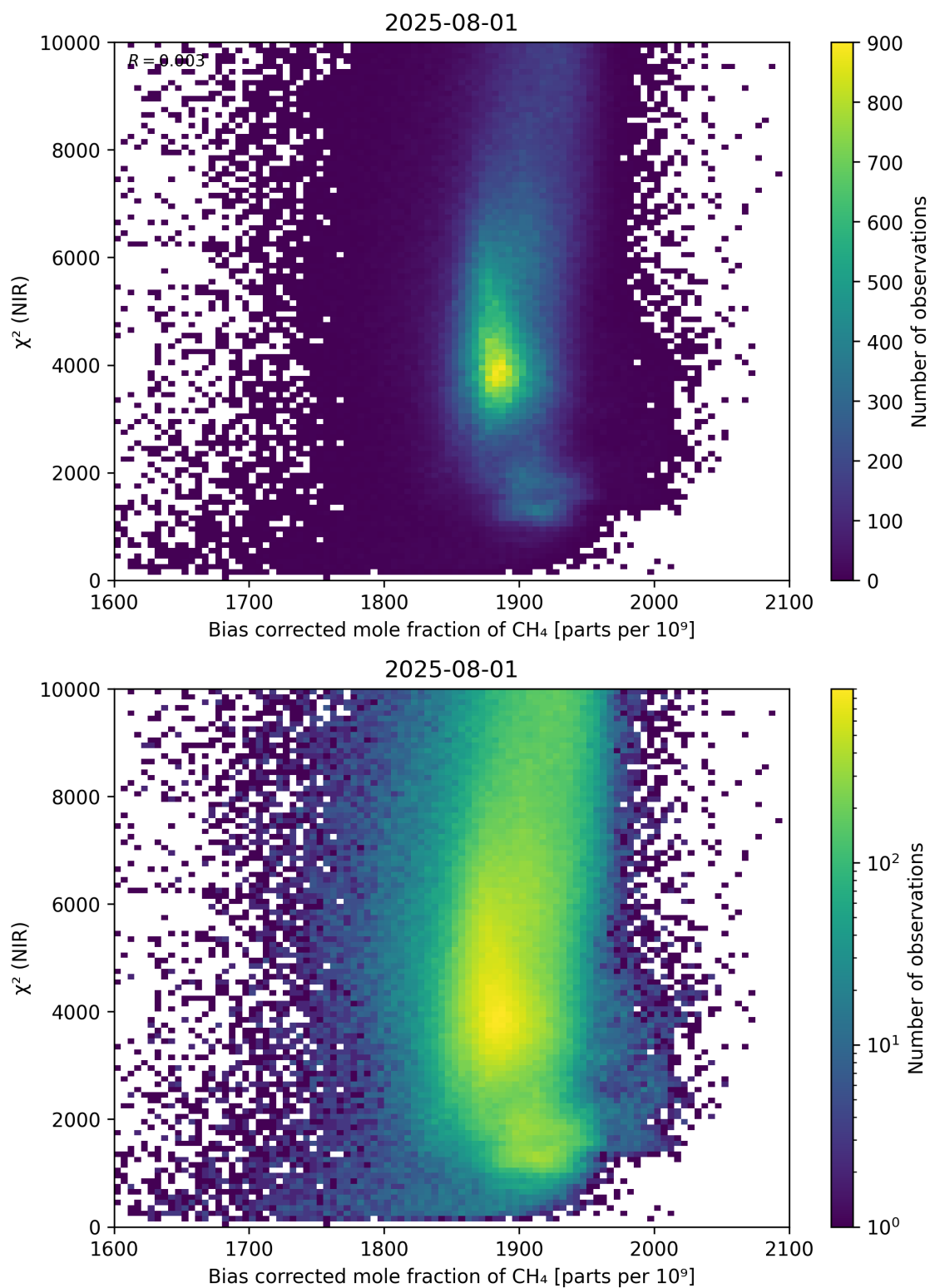
Figure 63: Scatter density plot of “Bias corrected mole fraction of \text{CH}_4 ” against “ \chi^2 (NIR)” for 2025-07-31 to 2025-08-02.
