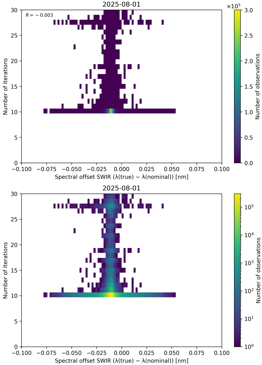
Figure 121: Scatter density plot of “Spectral offset SWIR ( \lambda_{\text{true}} - \lambda_{\text{nominal}} )” against “Number of iterations” for 2025-07-31 to 2025-08-02.
