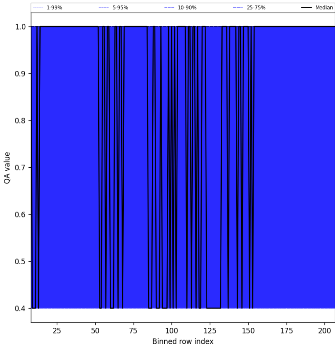
Figure 33: Along track statistics of “QA value” for 2025-07-31 to 2025-08-02
