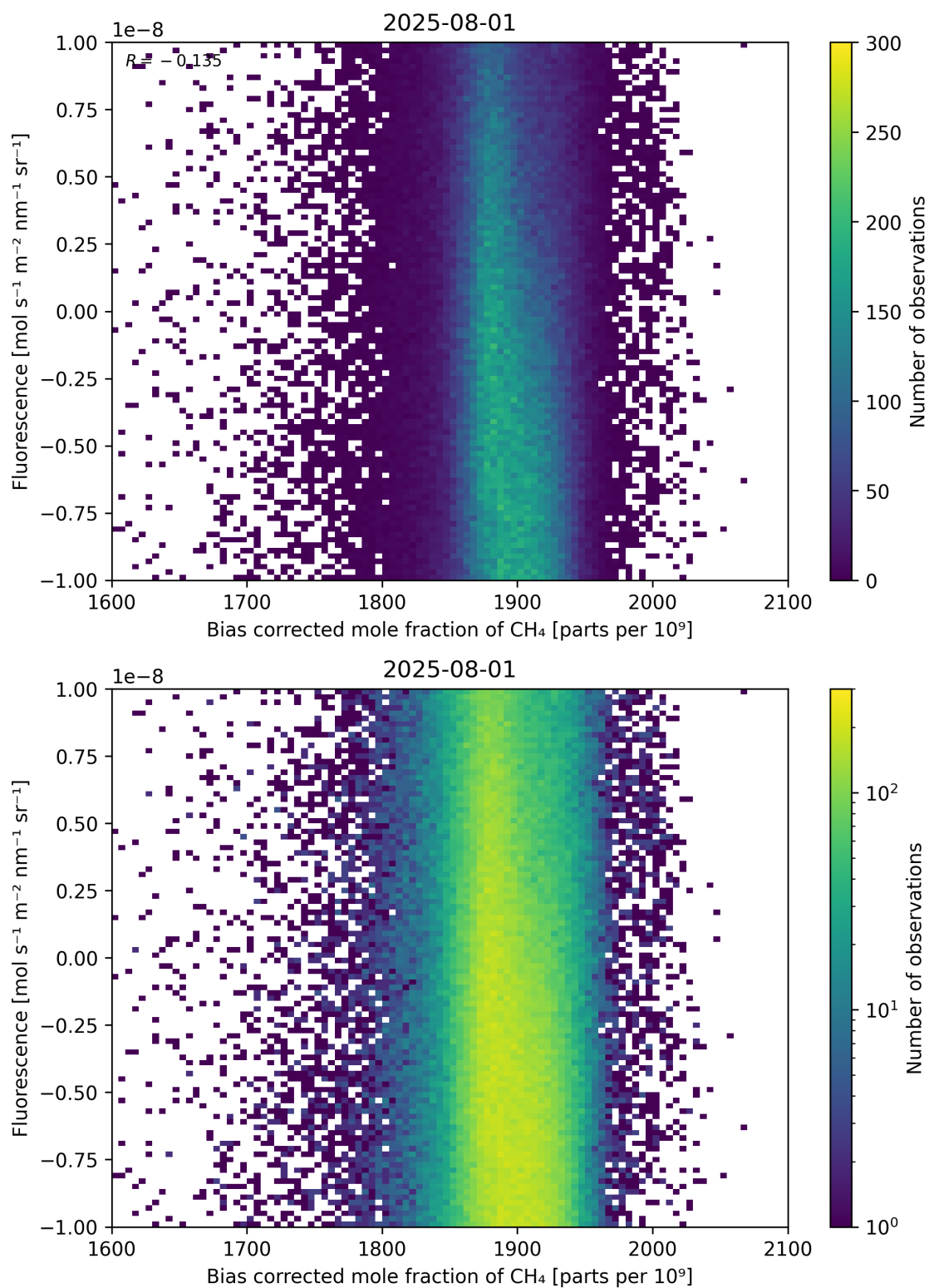
Figure 66: Scatter density plot of “Bias corrected mole fraction of CH 4 ” against “Fluorescence” for 2025-07-31 to 2025-08-02.
