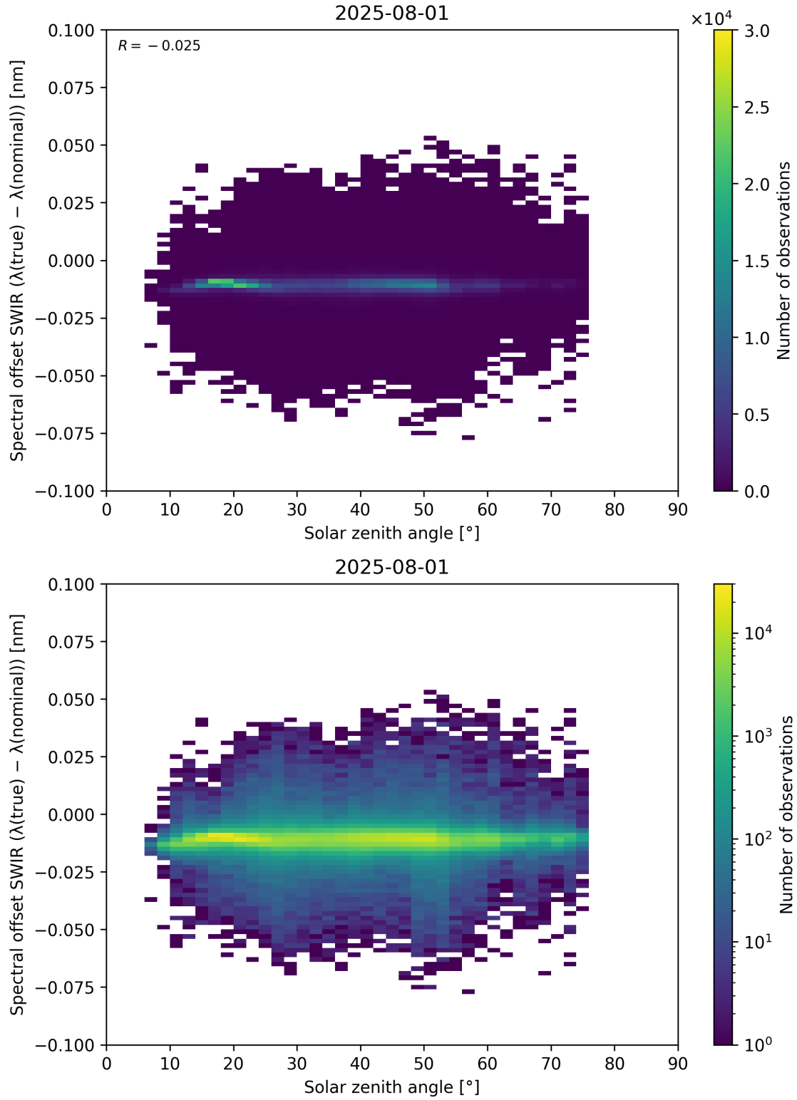
Figure 104: Scatter density plot of “Solar zenith angle” against “Spectral offset SWIR ( \lambda_{\text{true}} - \lambda_{\text{nominal}} )” for 2025-07-31 to 2025-08-02.
