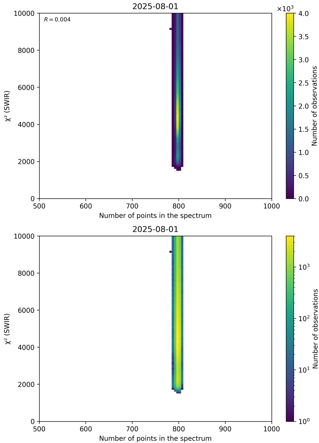
Figure 89: Scatter density plot of “Number of points in the spectrum” against “ \chi^2 (SWIR)” for 2025-07-31 to 2025-08-02.
