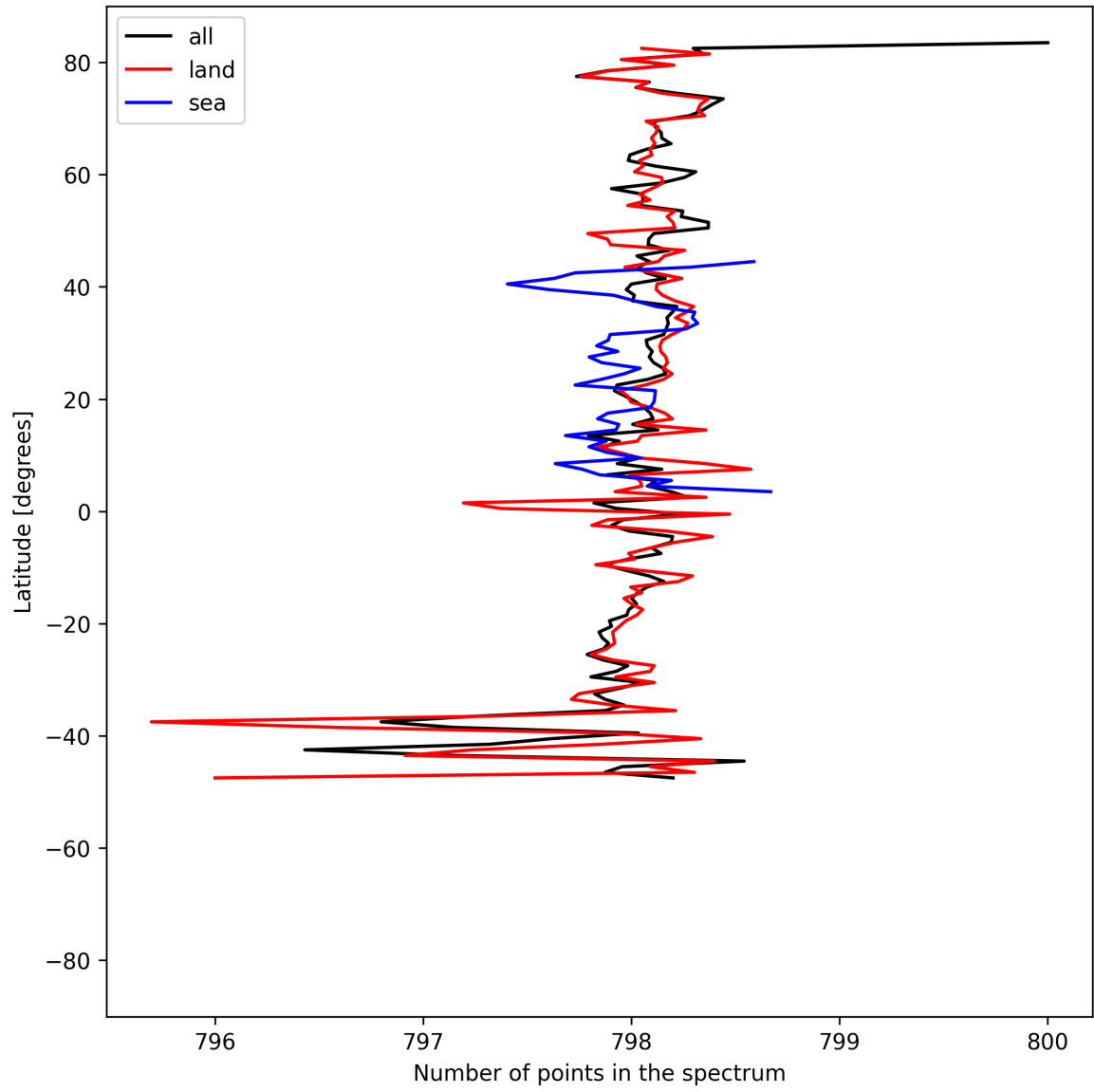
Figure 15: Zonal average of “Number of points in the spectrum” for 2025-07-31 to 2025-08-02.
