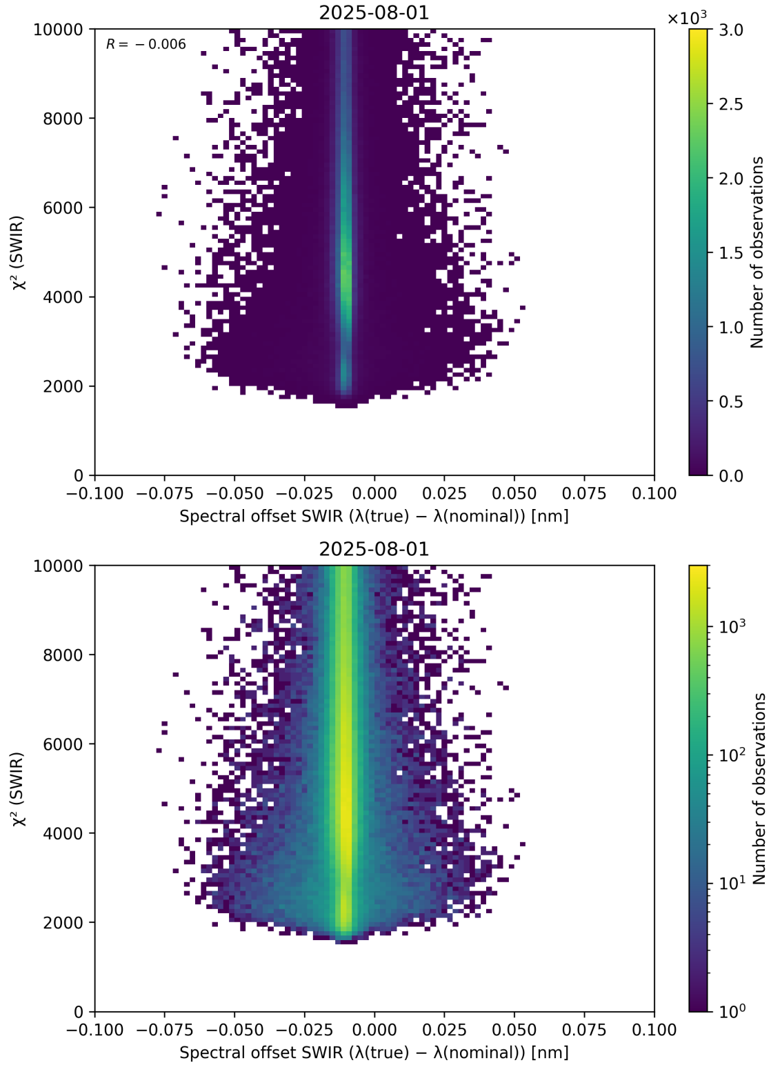
Figure 118: Scatter density plot of “Spectral offset SWIR ( \lambda_{\text{true}} - \lambda_{\text{nominal}} )” against “ \chi^2 (SWIR)” for 2025-07-31 to 2025-08-02.
