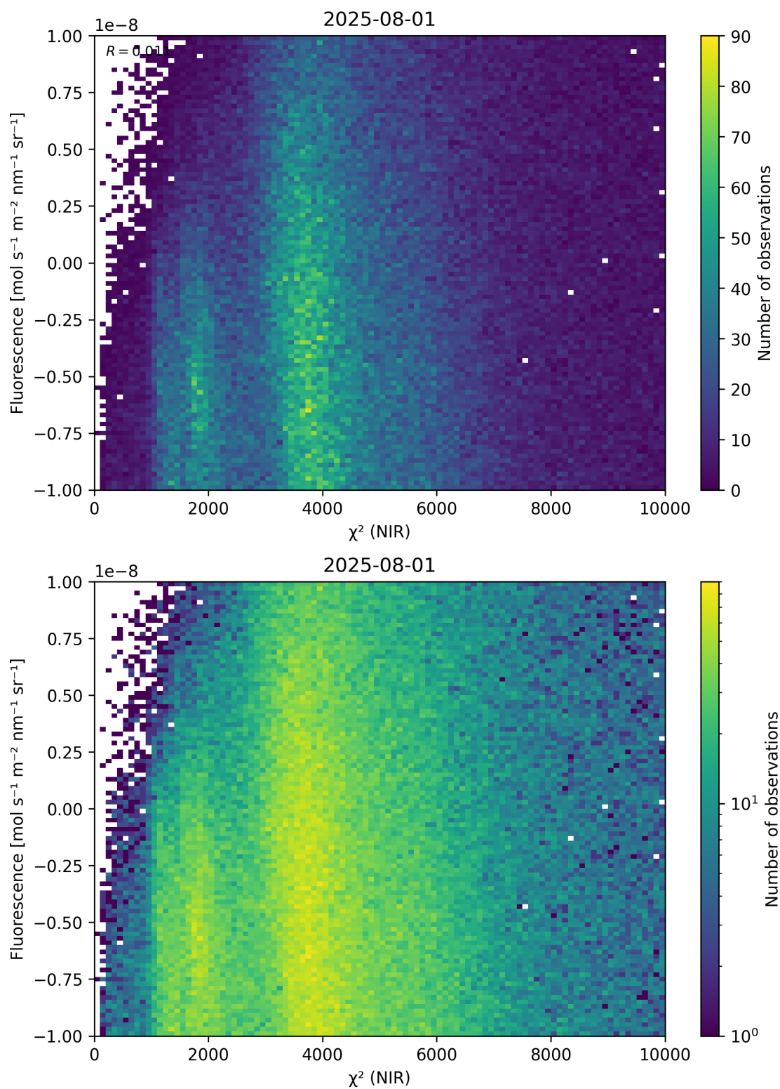
Figure 45: Scatter density plot of “ \chi^2 (NIR)” against “Fluorescence” for 2025-07-31 to 2025-08-02.
