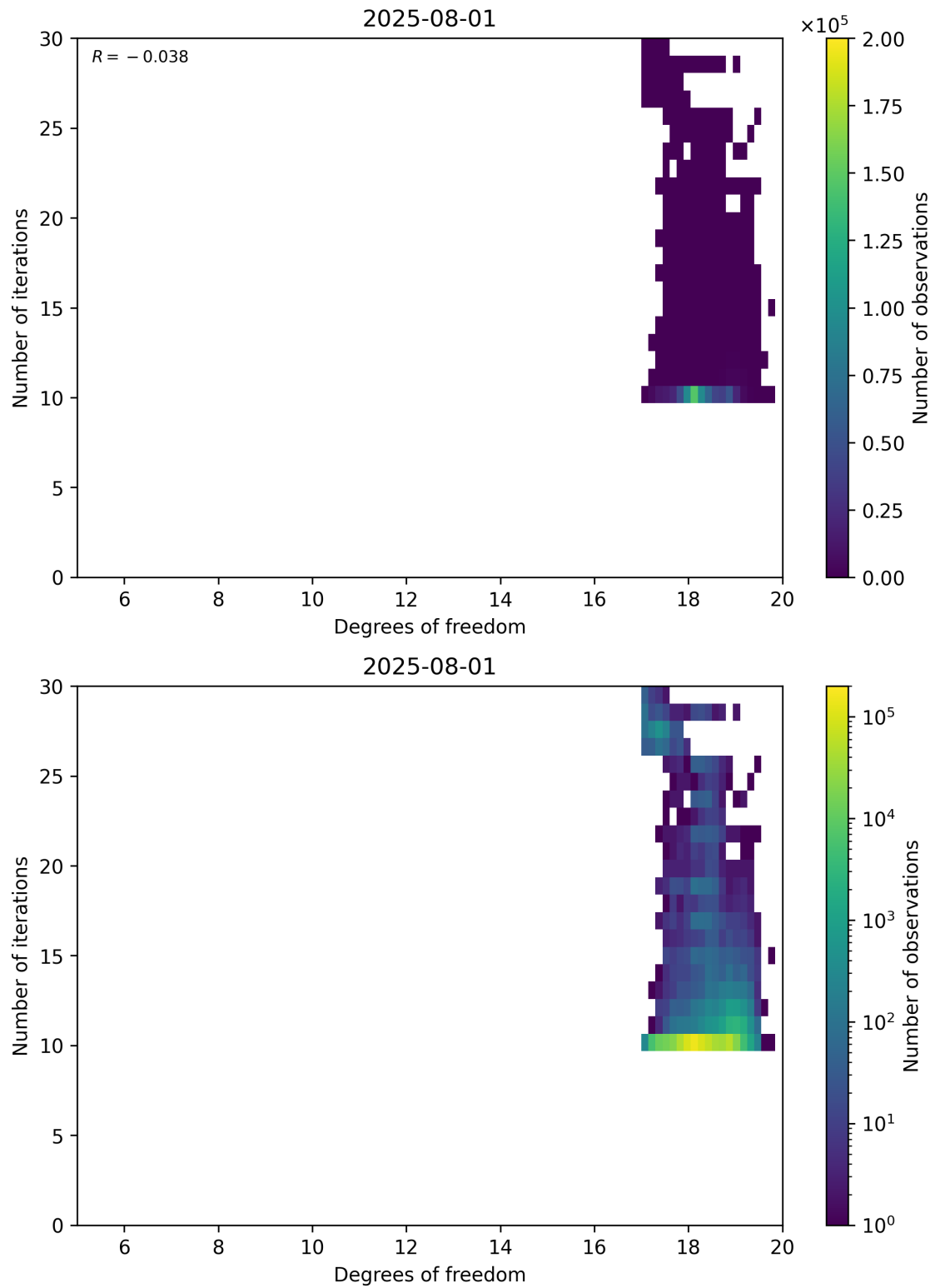
Figure 52: Scatter density plot of “Degrees of freedom” against “Number of iterations” for 2025-07-31 to 2025-08-02.
