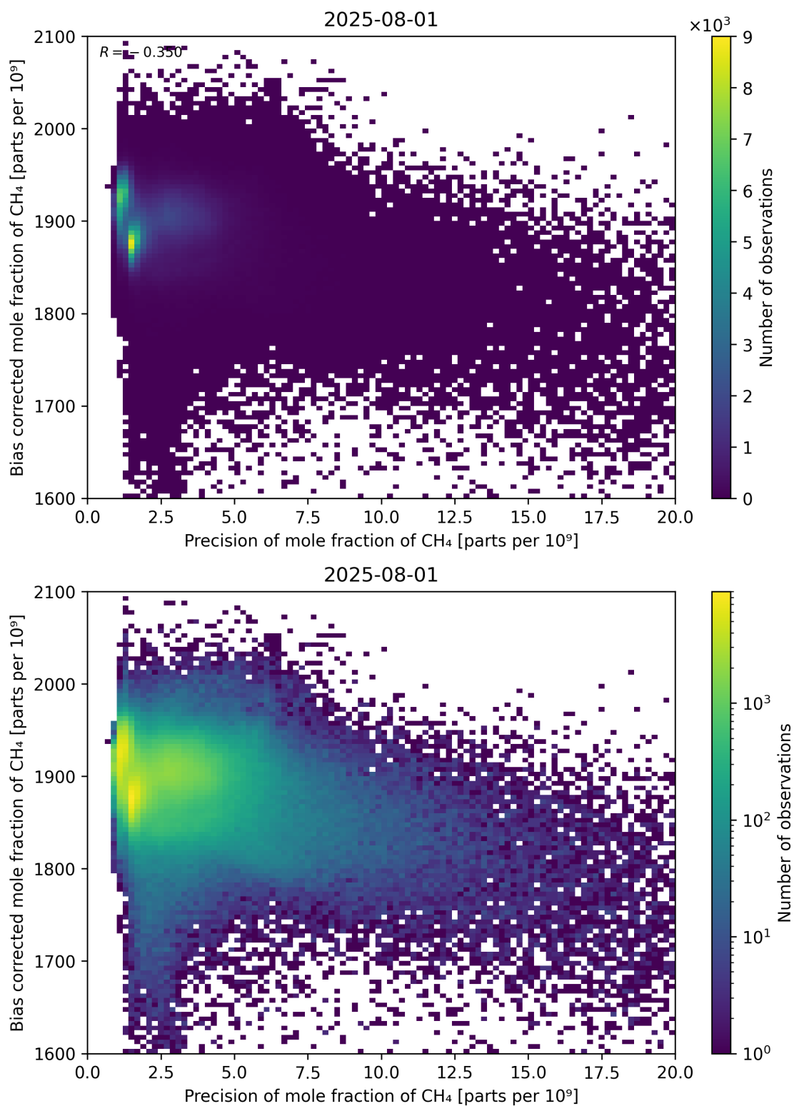
Figure 82: Scatter density plot of “Precision of mole fraction of CH 4 ” against “Bias corrected mole fraction of CH 4 ” for 2025-07-31 to 2025-08-02.
