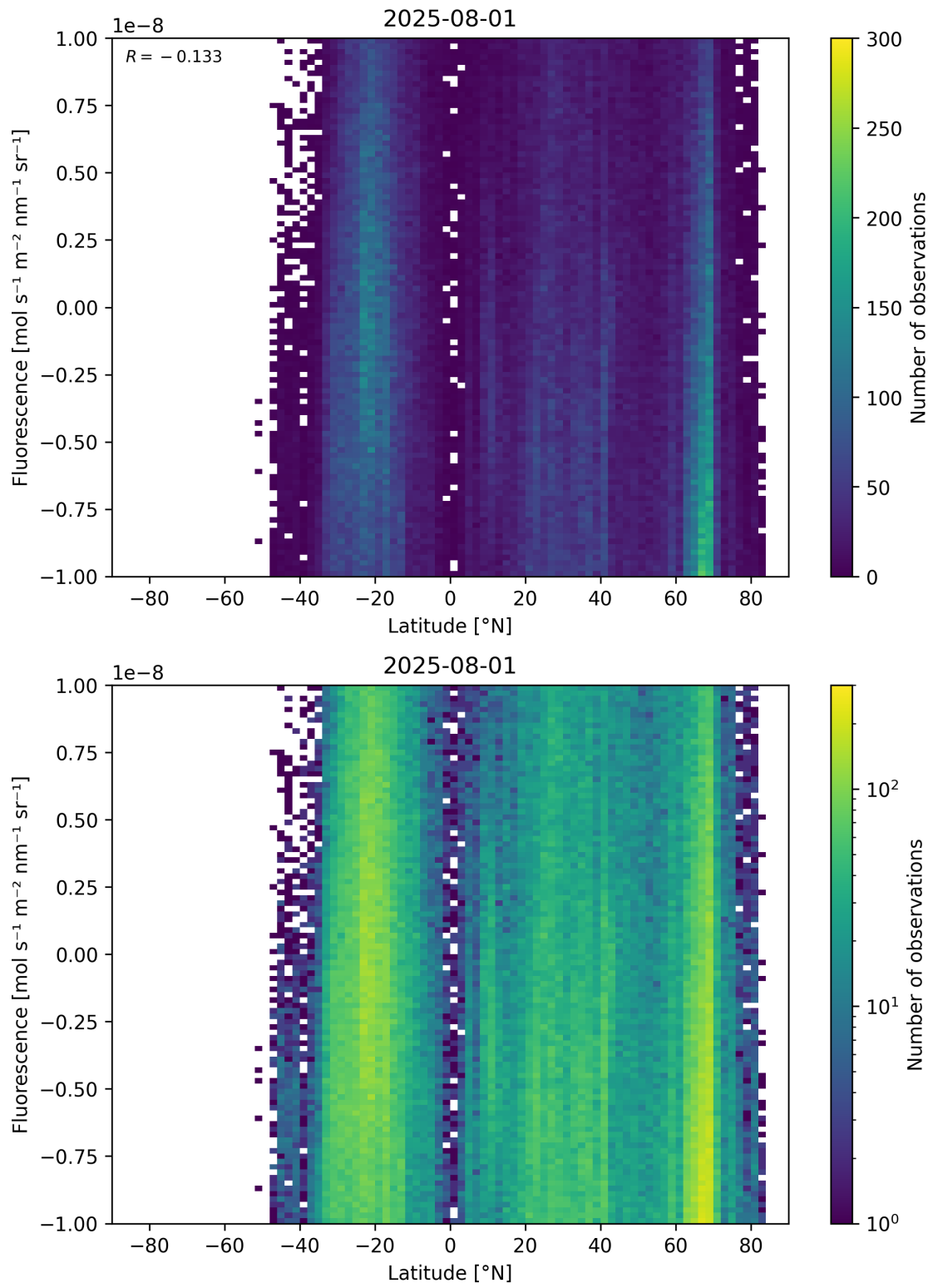
Figure 56: Scatter density plot of “Latitude” against “Fluorescence” for 2025-07-31 to 2025-08-02.
