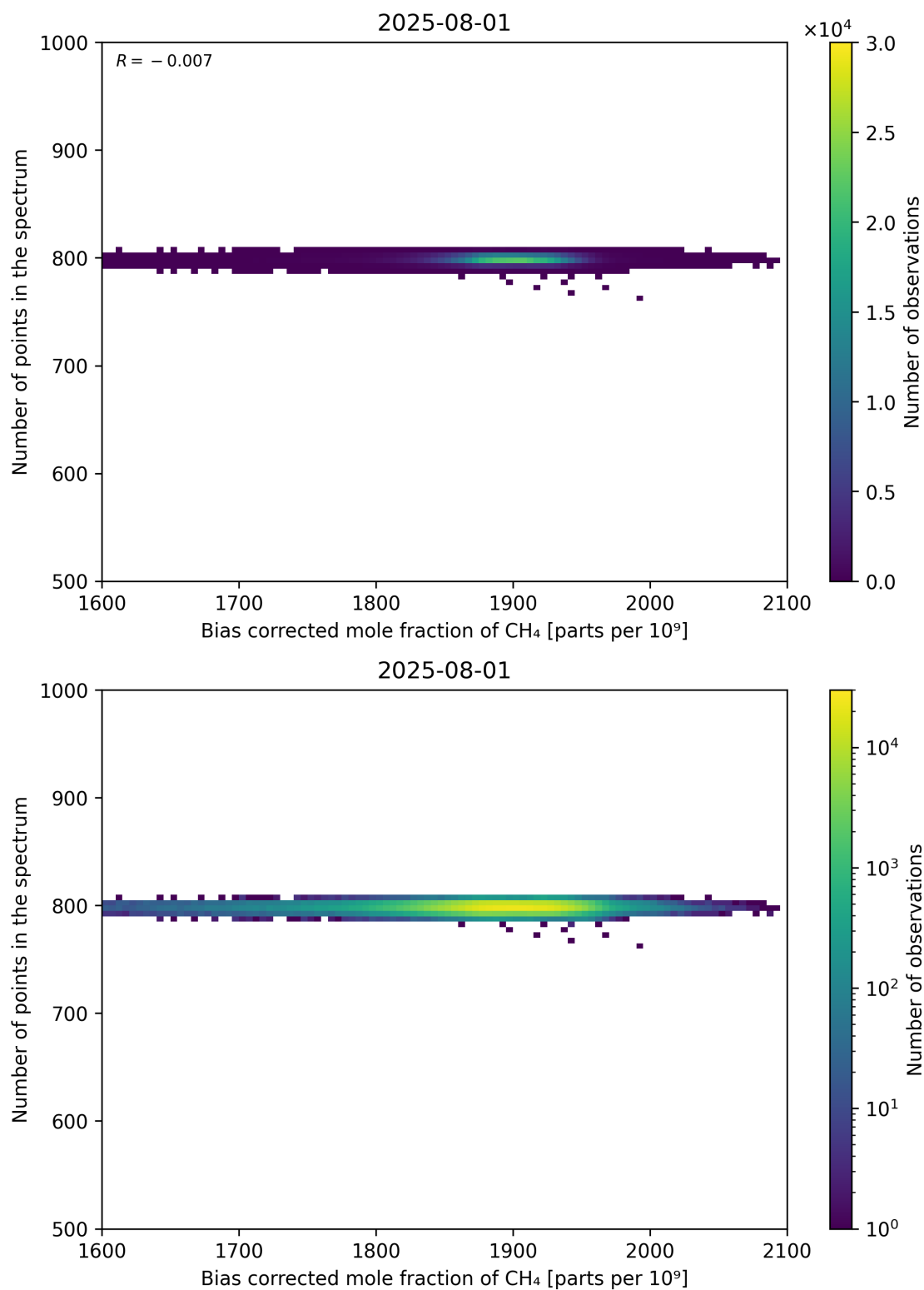
Figure 68: Scatter density plot of “Bias corrected mole fraction of CH 4 ” against “Number of points in the spectrum” for 2025-07-31 to 2025-08-02.
