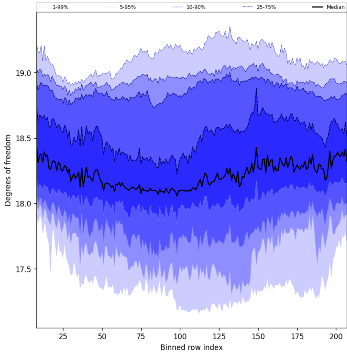
Figure 41: Along track statistics of “Degrees of freedom” for 2025-07-31 to 2025-08-02
