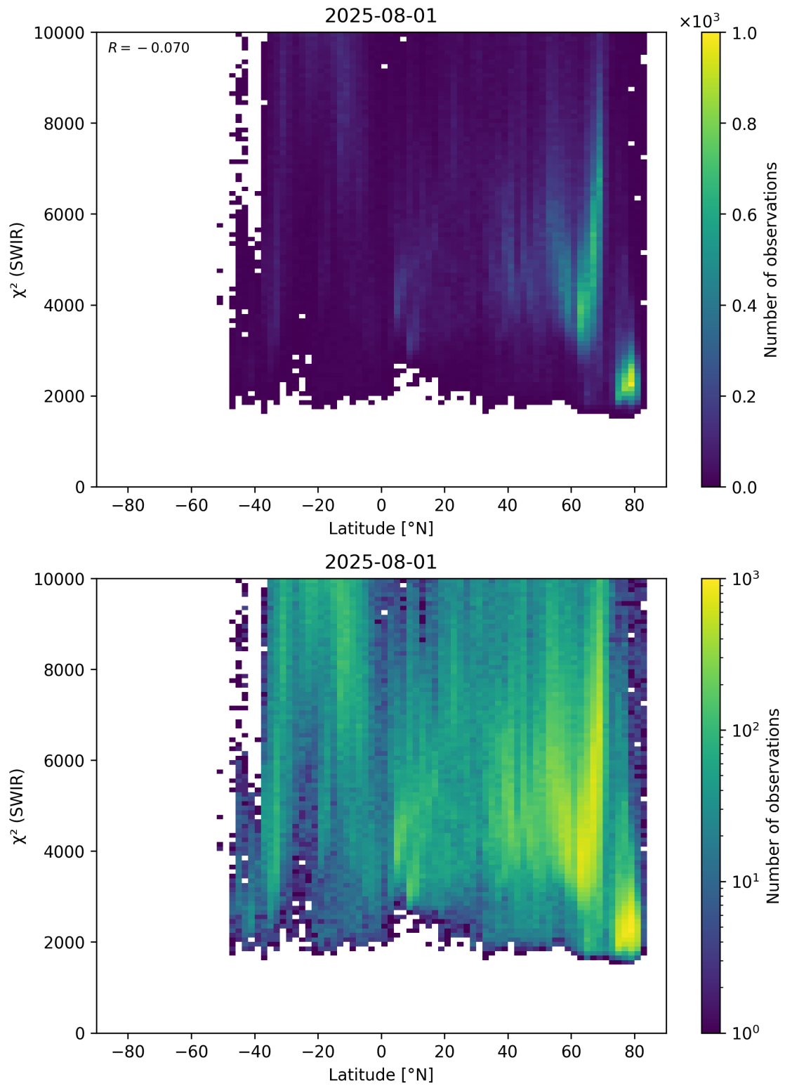
Figure 54: Scatter density plot of “Latitude” against “ \chi^2 (SWIR)” for 2025-07-31 to 2025-08-02.
