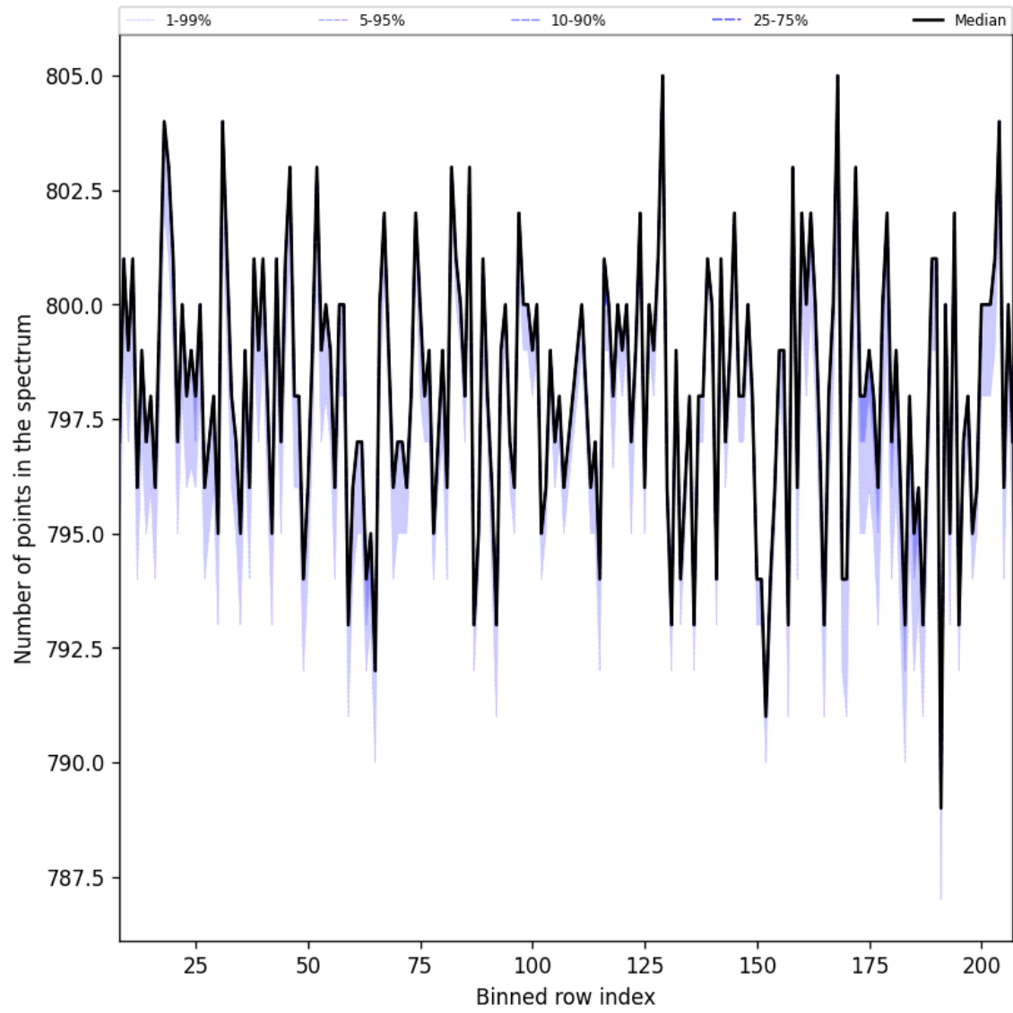
Figure 37: Along track statistics of “Number of points in the spectrum” for 2025-07-31 to 2025-08-02
