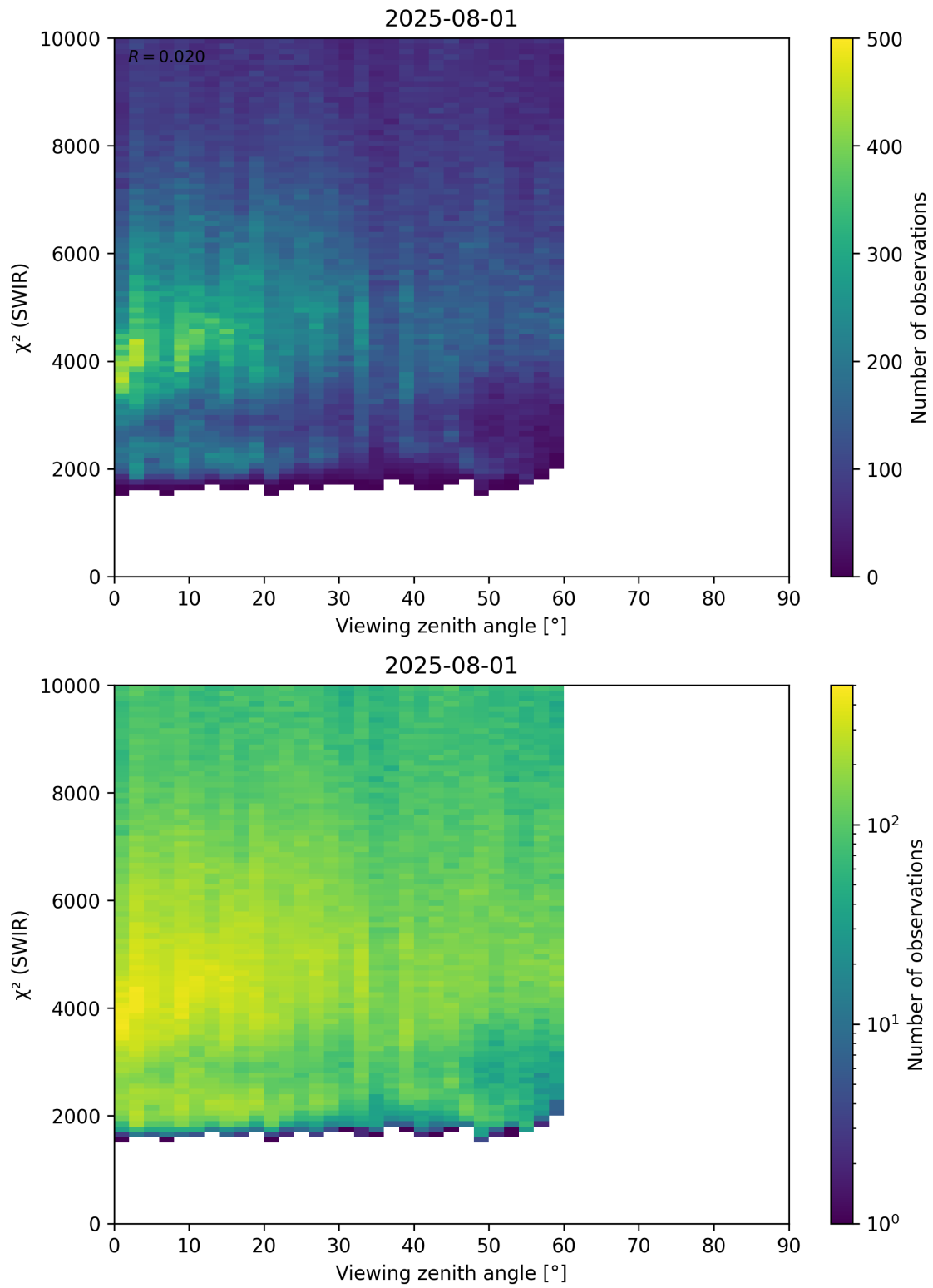
Figure 106: Scatter density plot of “Viewing zenith angle” against “ \chi^2 (SWIR)” for 2025-07-31 to 2025-08-02.
