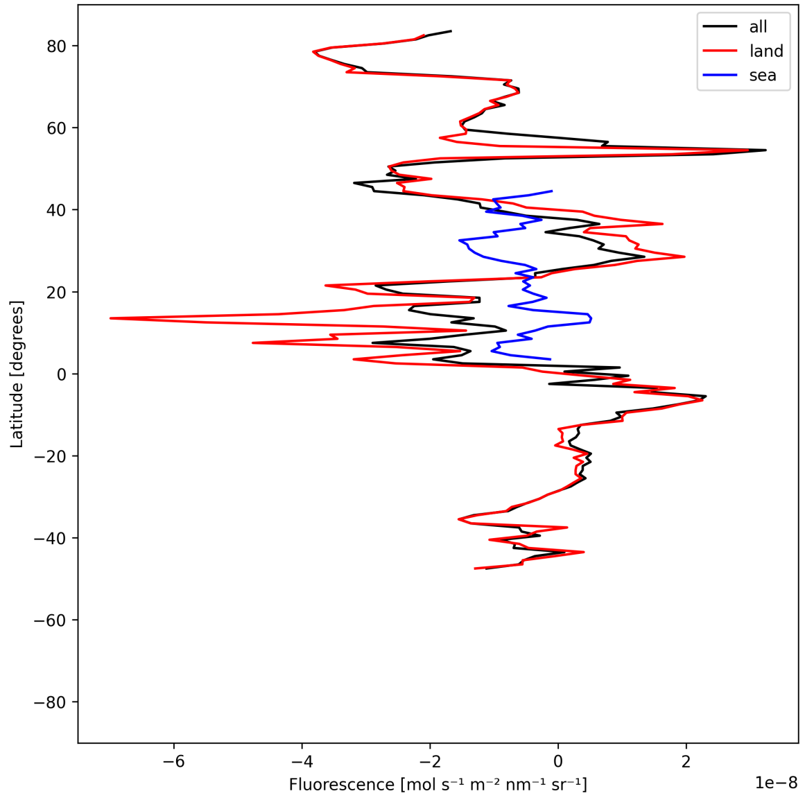
Figure 21: Zonal average of “Fluorescence” for 2025-07-31 to 2025-08-02.
