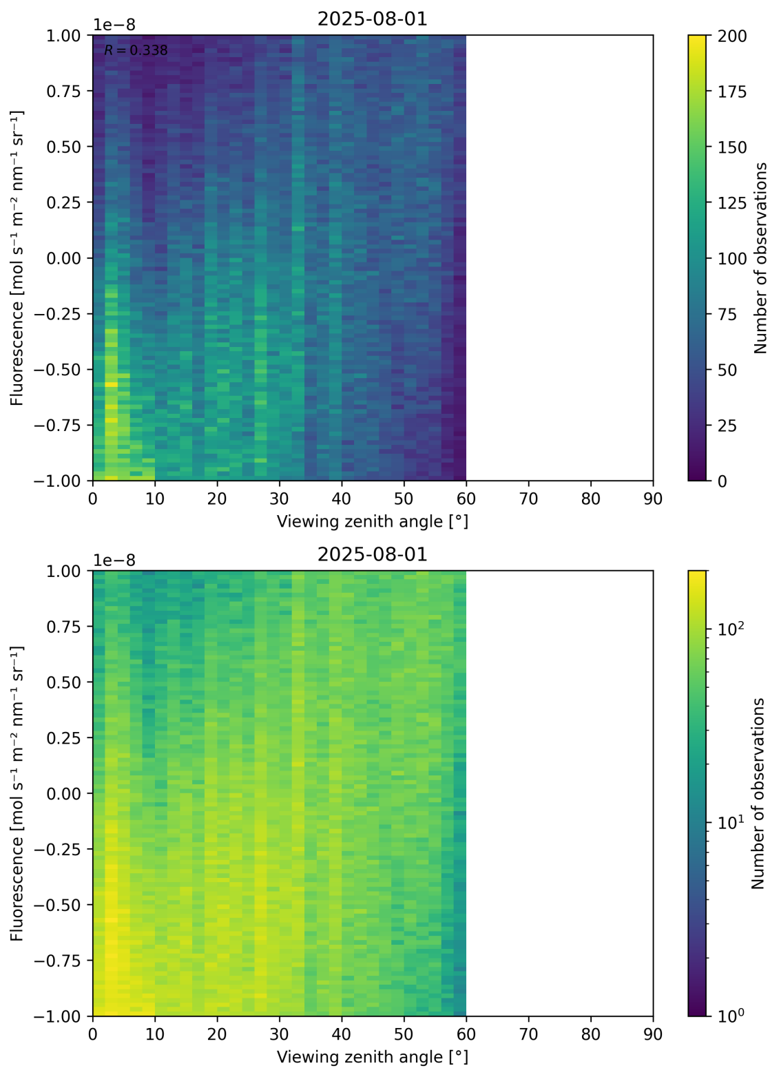
Figure 108: Scatter density plot of “Viewing zenith angle” against “Fluorescence” for 2025-07-31 to 2025-08-02.
