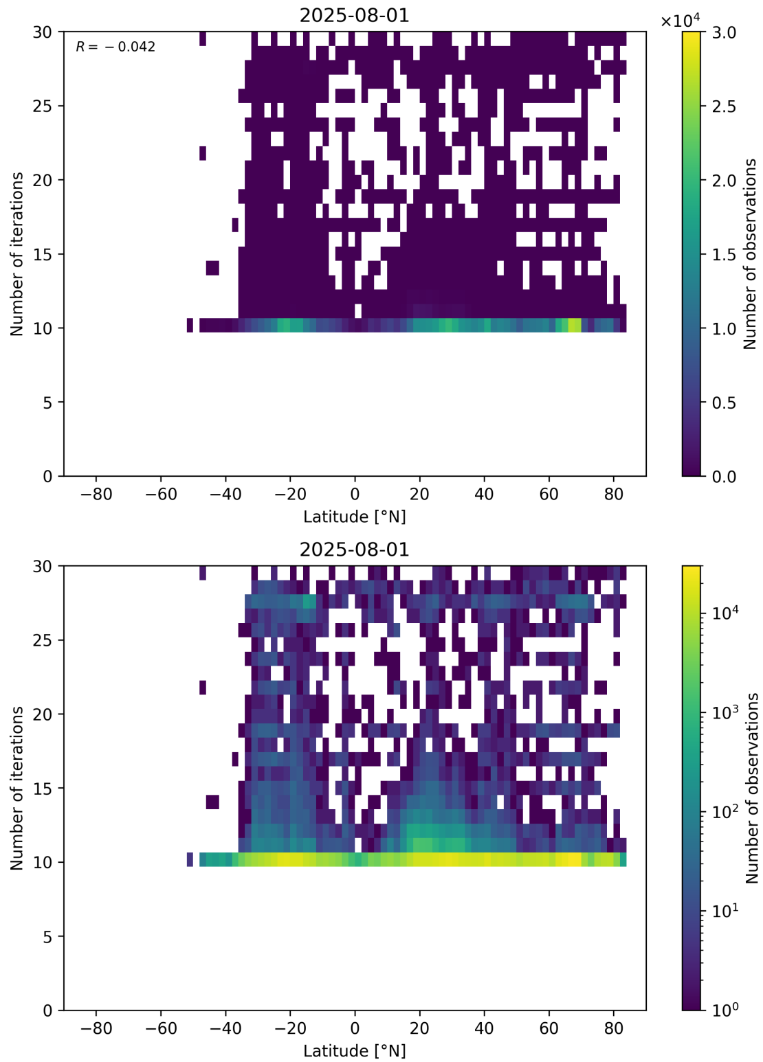
Figure 60: Scatter density plot of “Latitude” against “Number of iterations” for 2025-07-31 to 2025-08-02.
