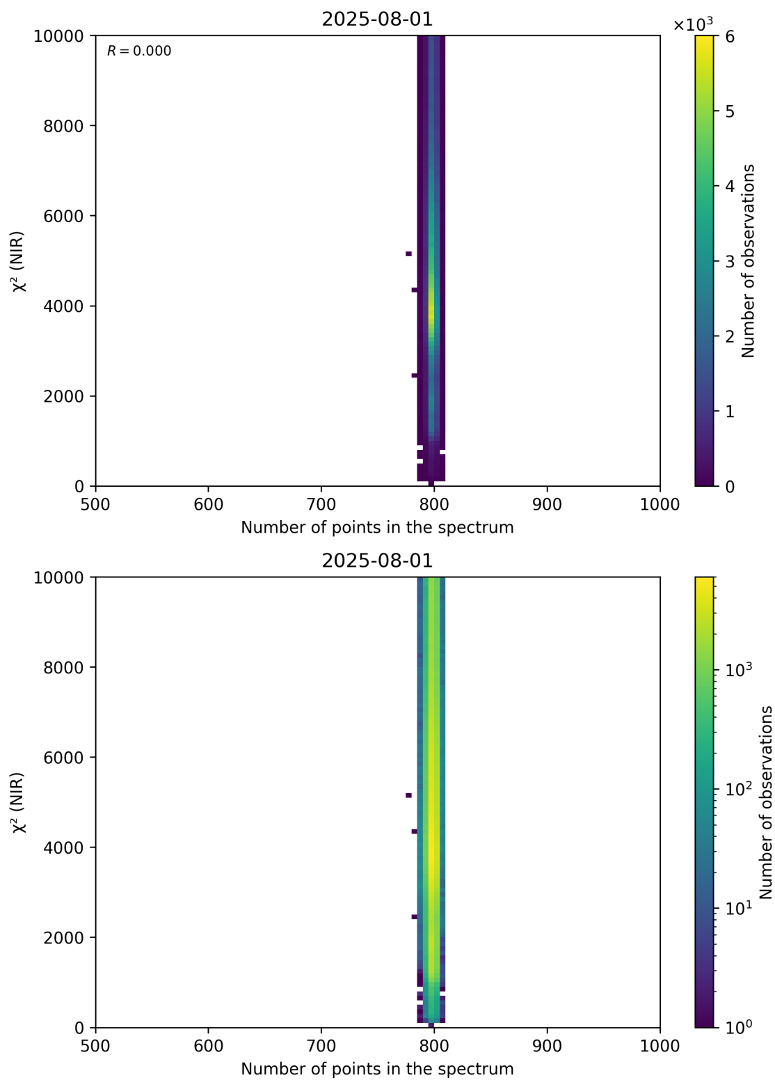
Figure 88: Scatter density plot of “Number of points in the spectrum” against “ \chi^2 (NIR)” for 2025-07-31 to 2025-08-02.
