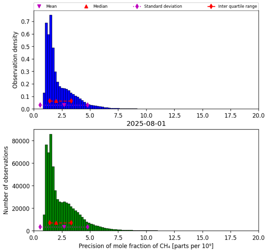
Figure 24: Histogram of “Precision of mole fraction of CH 4 ” for 2025-07-31 to 2025-08-02
