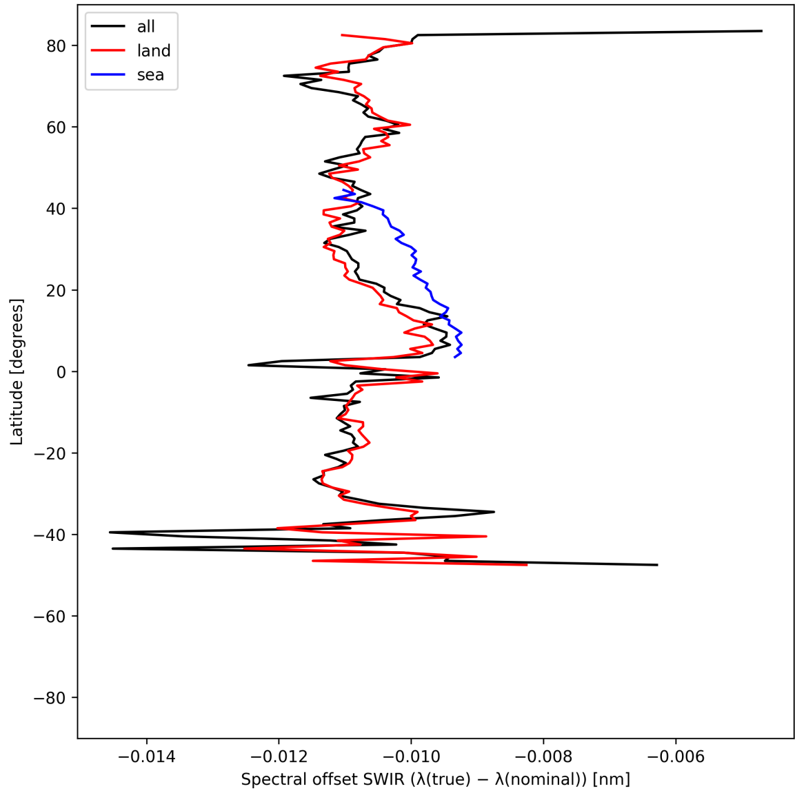
Figure 16: Zonal average of “Spectral offset SWIR ( \lambda_{\text{true}} - \lambda_{\text{nominal}} )” for 2025-07-31 to 2025-08-02.
