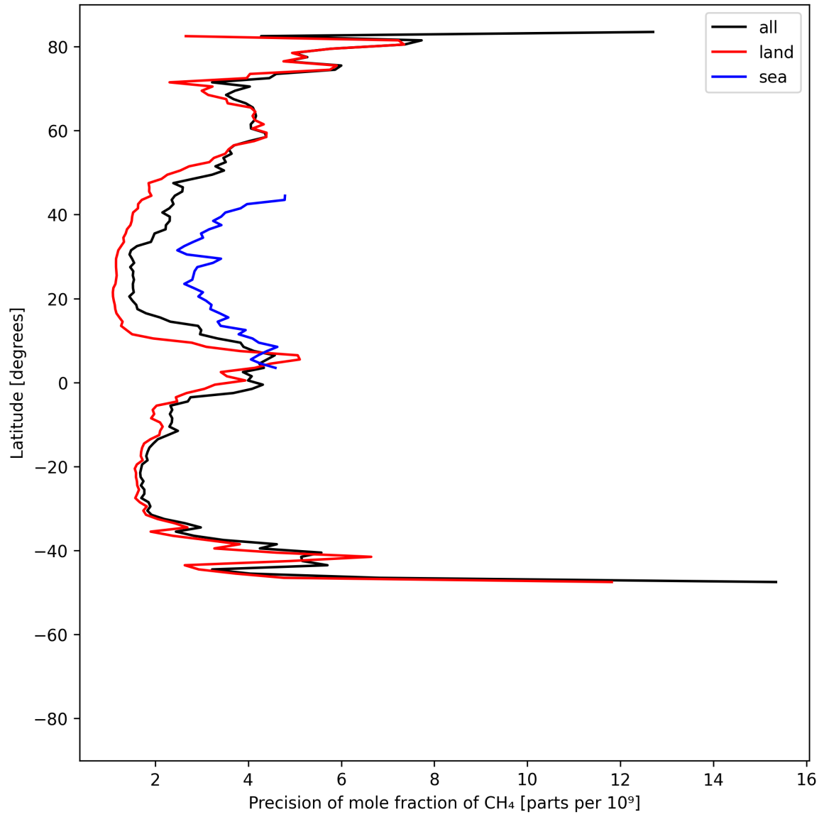
Figure 13: Zonal average of “Precision of mole fraction of CH 4 ” for 2025-07-31 to 2025-08-02.
