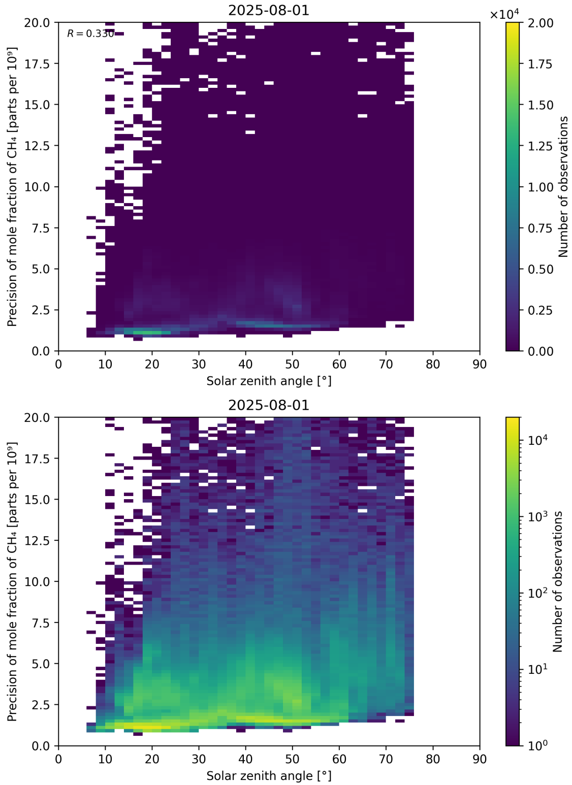
Figure 101: Scatter density plot of “Solar zenith angle” against “Precision of mole fraction of \text{CH}_4 ” for 2025-07-31 to 2025-08-02.
