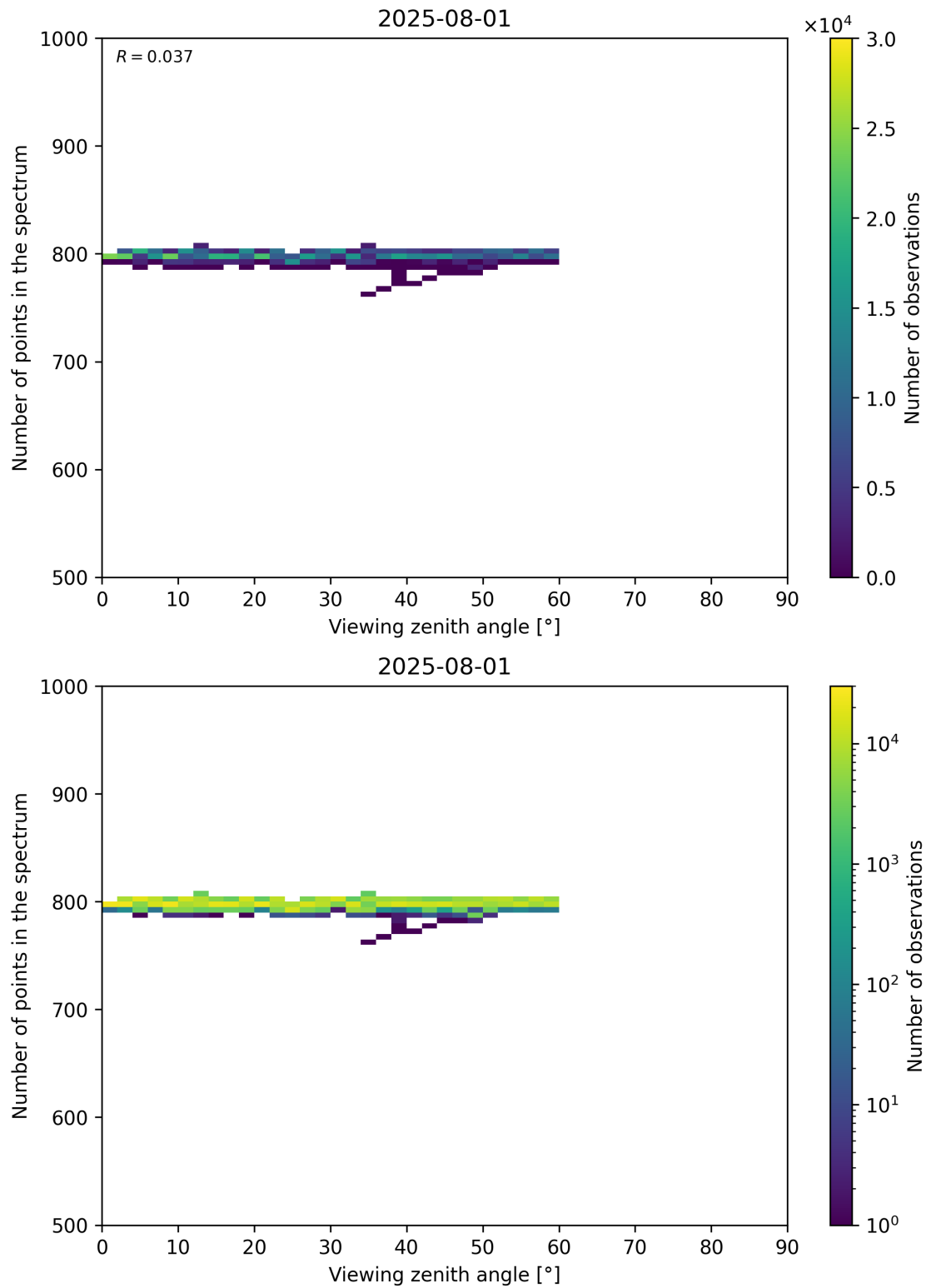
Figure 114: Scatter density plot of “Viewing zenith angle” against “Number of points in the spectrum” for 2025-07-31 to 2025-08-02.
