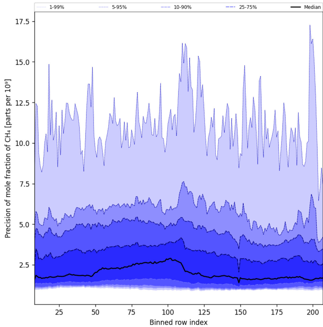
Figure 35: Along track statistics of “Precision of mole fraction of CH 4 ” for 2025-07-31 to 2025-08-02
