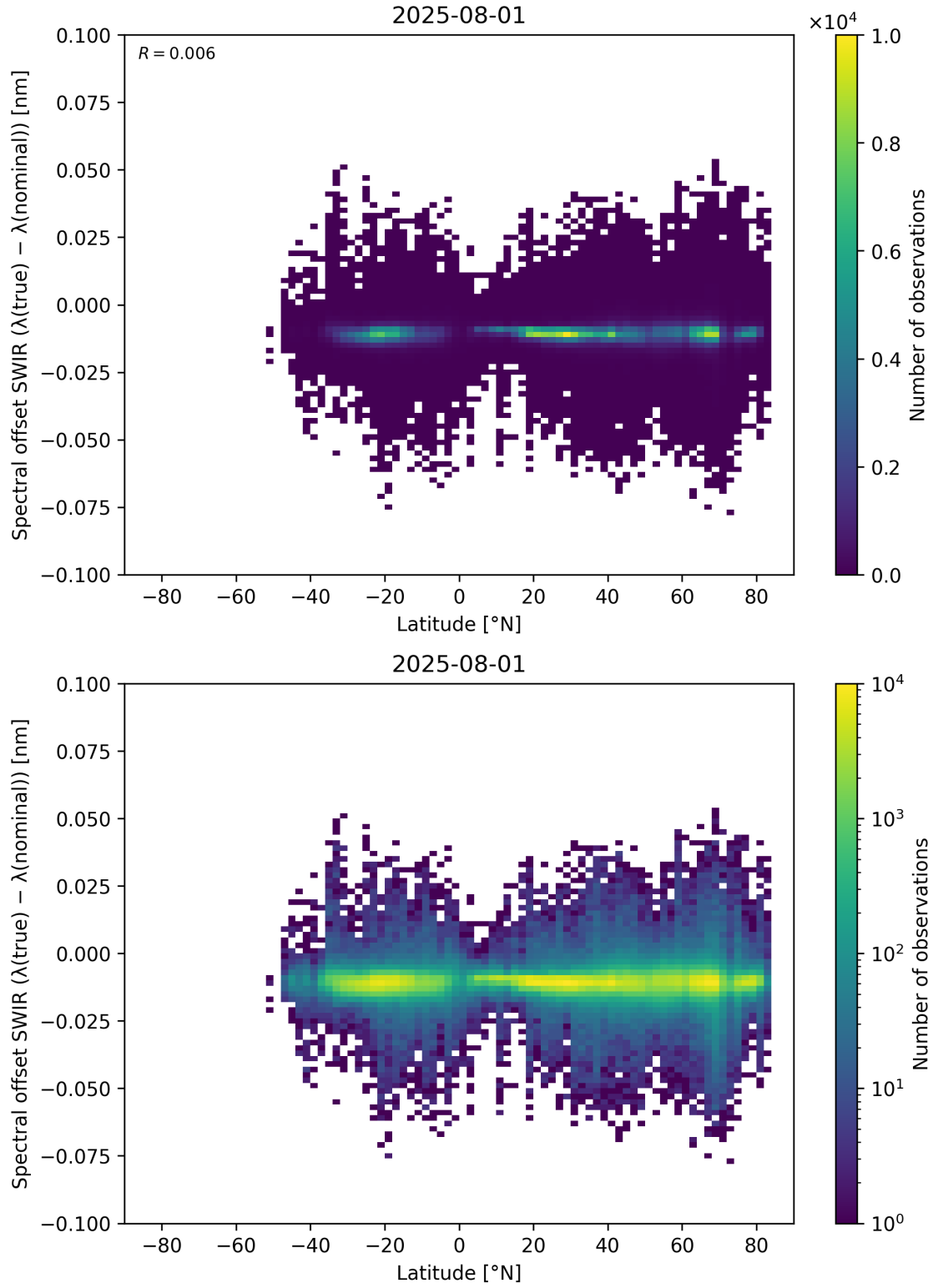
Figure 62: Scatter density plot of “Latitude” against “Spectral offset SWIR ( \lambda_{\text{true}} - \lambda_{\text{nominal}} )” for 2025-07-31 to 2025-08-02.
