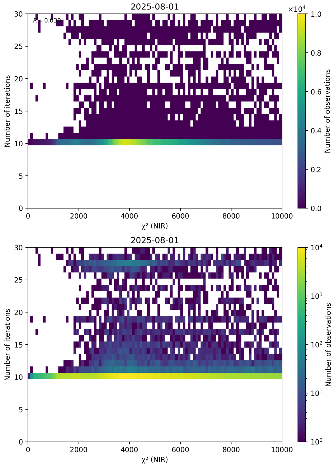
Figure 46: Scatter density plot of “ \chi^2 (NIR)” against “Number of iterations” for 2025-07-31 to 2025-08-02.
