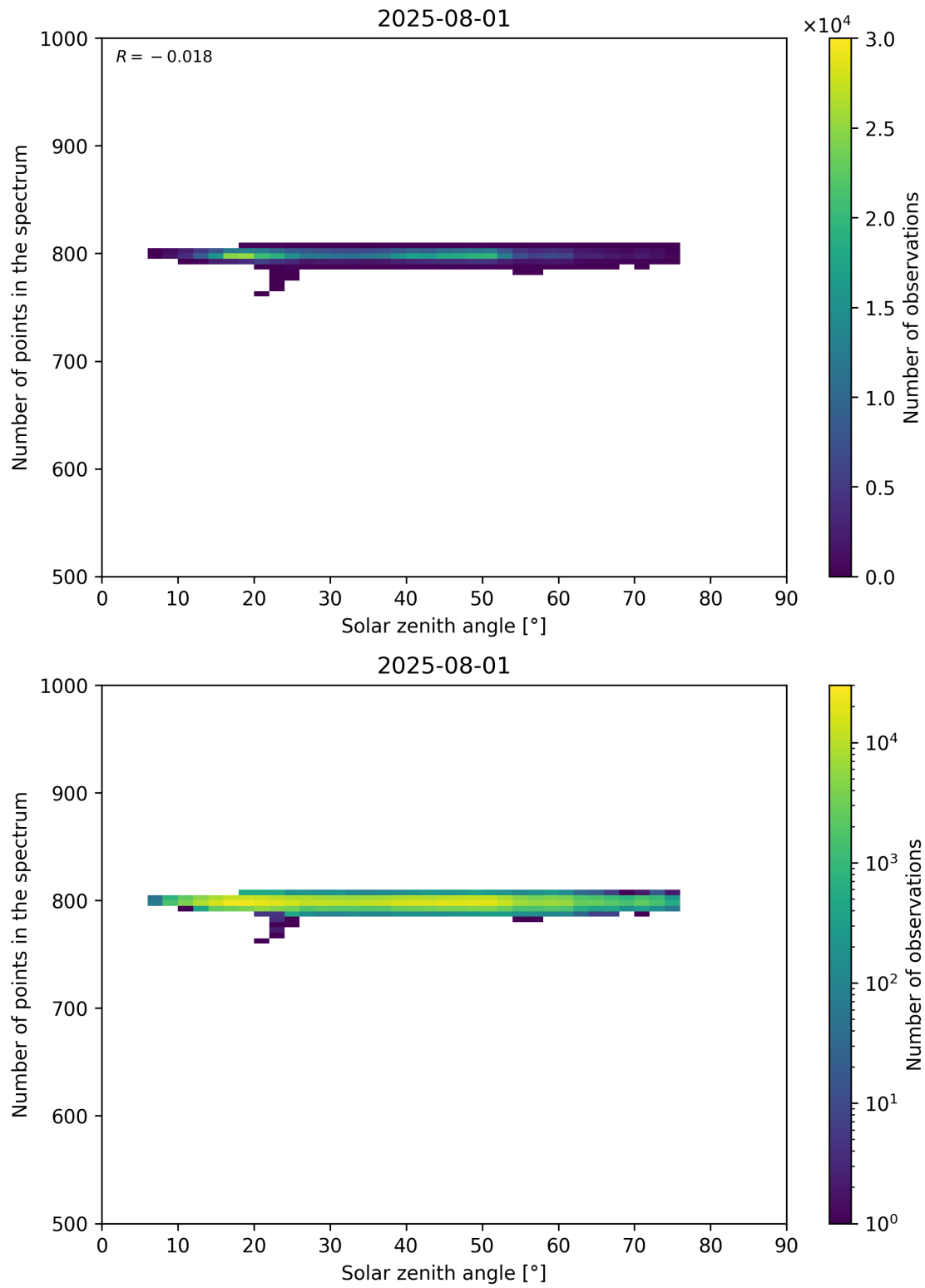
Figure 103: Scatter density plot of “Solar zenith angle” against “Number of points in the spectrum” for 2025-07-31 to 2025-08-02.
