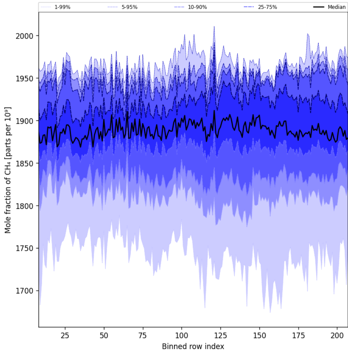
Figure 34: Along track statistics of “Mole fraction of CH 4 ” for 2025-07-31 to 2025-08-02
