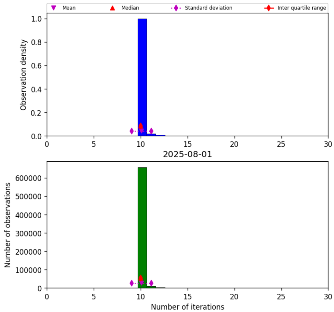
Figure 31: Histogram of “Number of iterations” for 2025-07-31 to 2025-08-02
