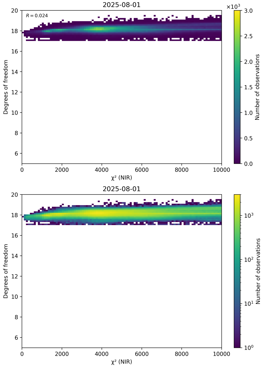
Figure 44: Scatter density plot of “ \chi^2 (NIR)” against “Degrees of freedom” for 2025-07-31 to 2025-08-02.
