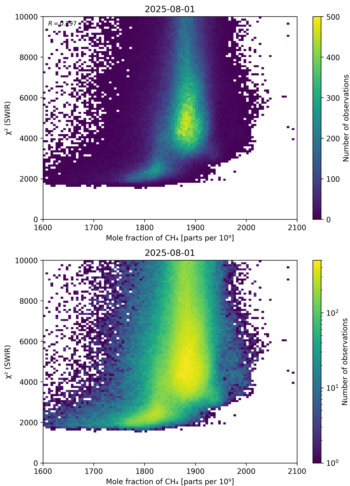
Figure 71: Scatter density plot of “Mole fraction of \text{CH}_4 ” against “ \chi^2 (SWIR)” for 2025-07-31 to 2025-08-02.
