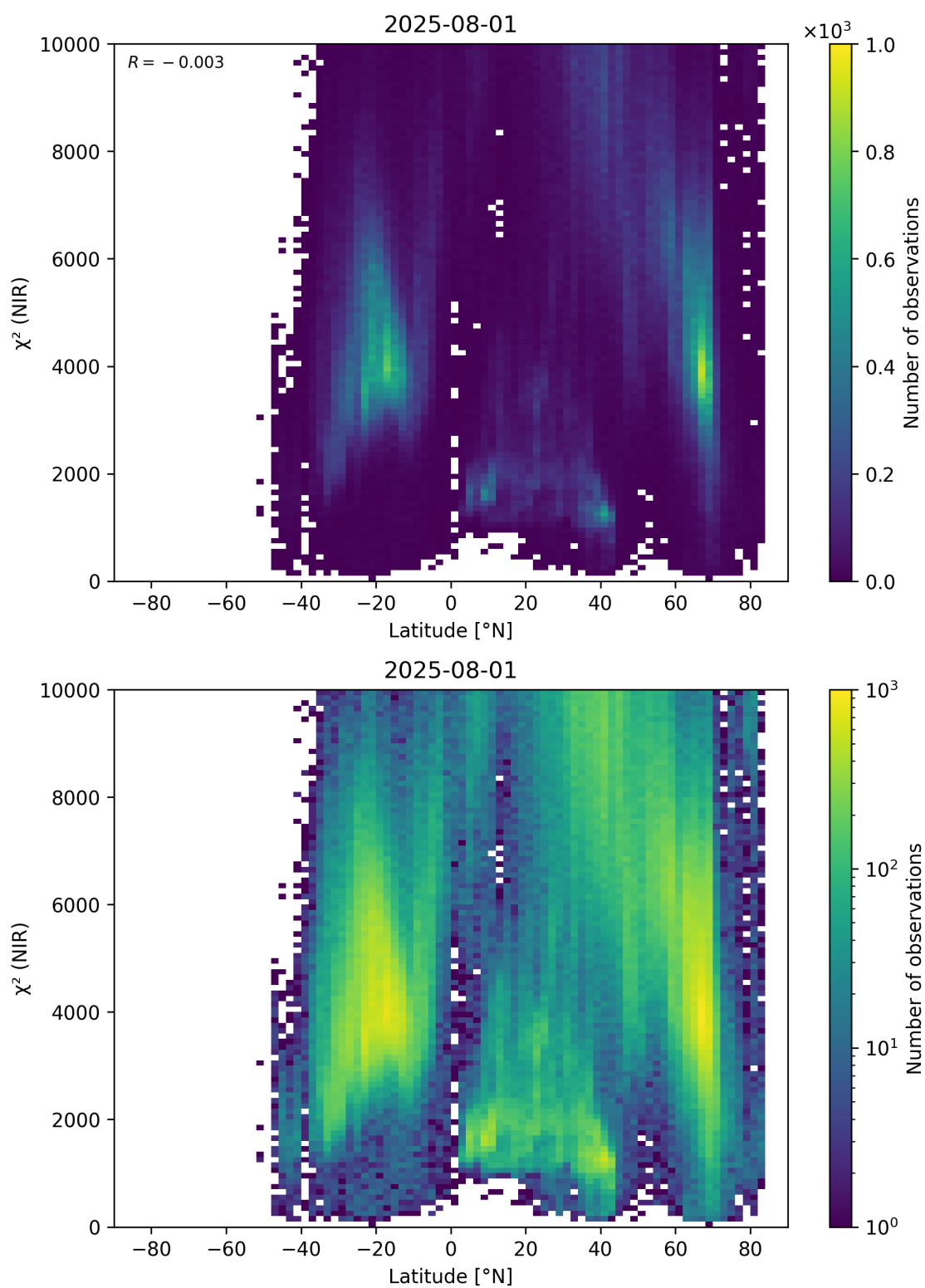
Figure 53: Scatter density plot of “Latitude” against “ \chi^2 (NIR)” for 2025-07-31 to 2025-08-02.
