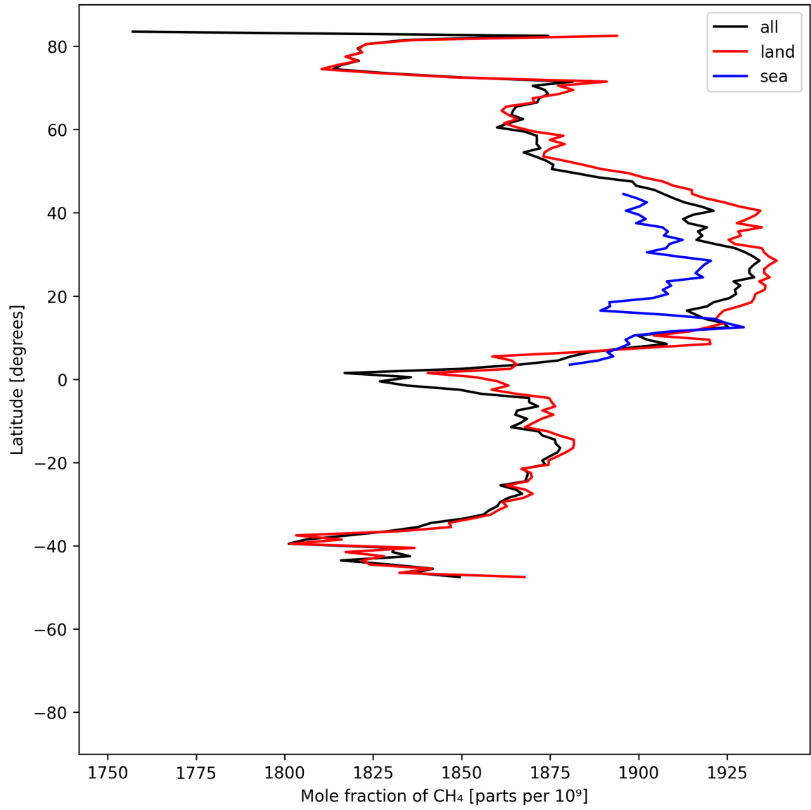
Figure 12: Zonal average of “Mole fraction of \text{CH}_4 ” for 2025-07-31 to 2025-08-02.
