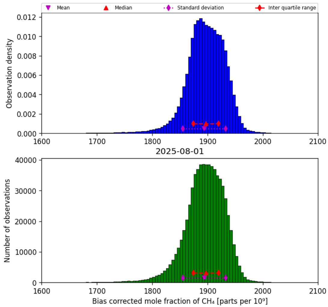
Figure 25: Histogram of “Bias corrected mole fraction of CH 4 ” for 2025-07-31 to 2025-08-02
