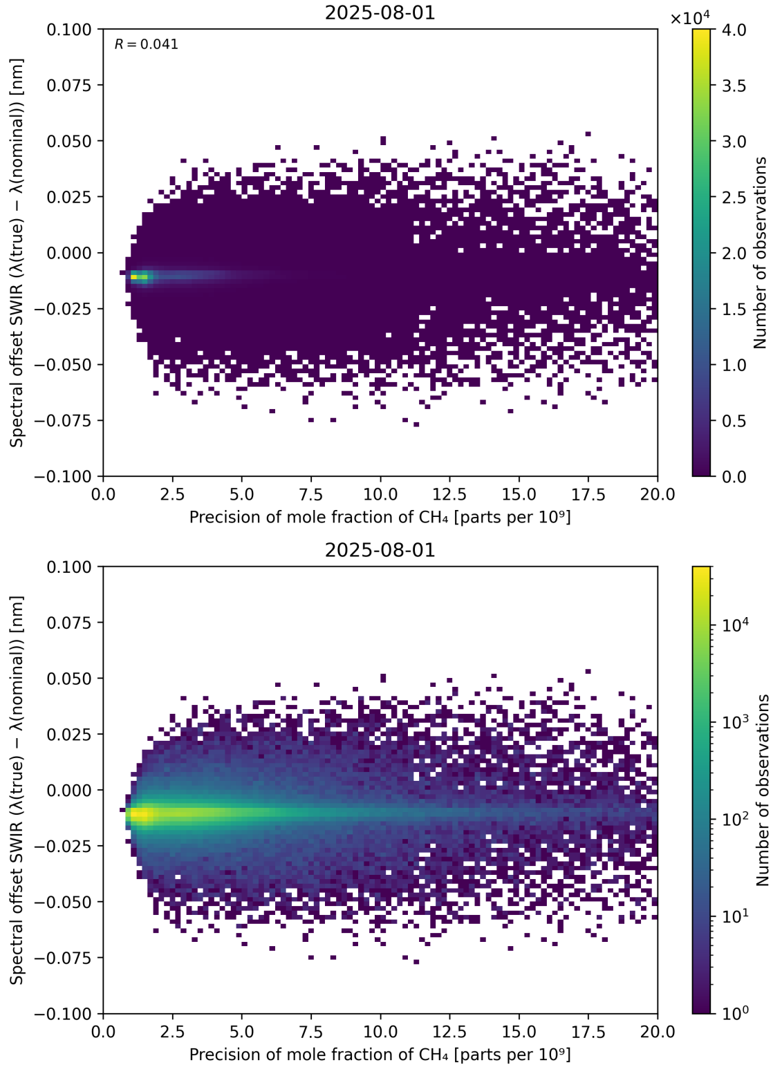
Figure 85: Scatter density plot of “Precision of mole fraction of \text{CH}_4 ” against “Spectral offset SWIR ( \lambda_{\text{true}} - \lambda_{\text{nominal}} )” for 2025-07-31 to 2025-08-02.
