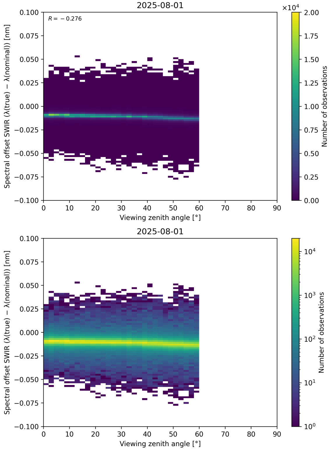
Figure 116: Scatter density plot of “Viewing zenith angle” against “Spectral offset SWIR ( \lambda_{\text{true}} - \lambda_{\text{nominal}} )” for 2025-07-31 to 2025-08-02.
