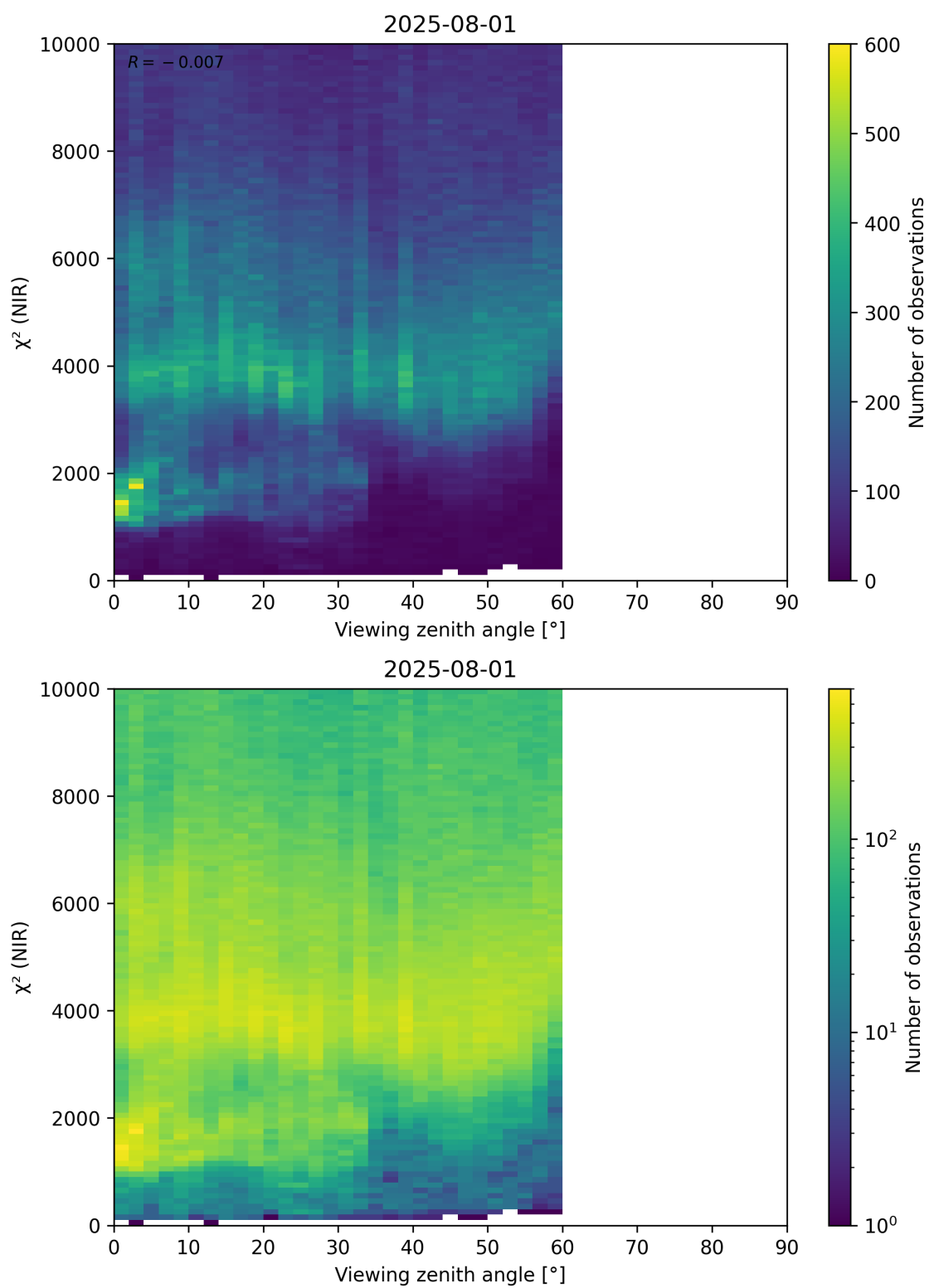
Figure 105: Scatter density plot of “Viewing zenith angle” against “ \chi^2 (NIR)” for 2025-07-31 to 2025-08-02.
