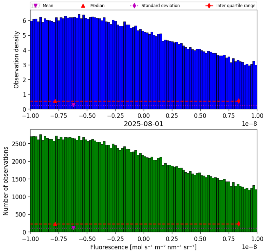
Figure 32: Histogram of “Fluorescence” for 2025-07-31 to 2025-08-02
