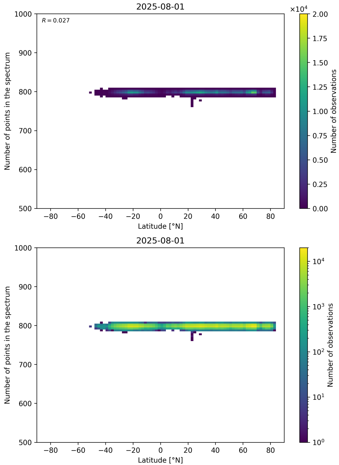
Figure 61: Scatter density plot of “Latitude” against “Number of points in the spectrum” for 2025-07-31 to 2025-08-02.
