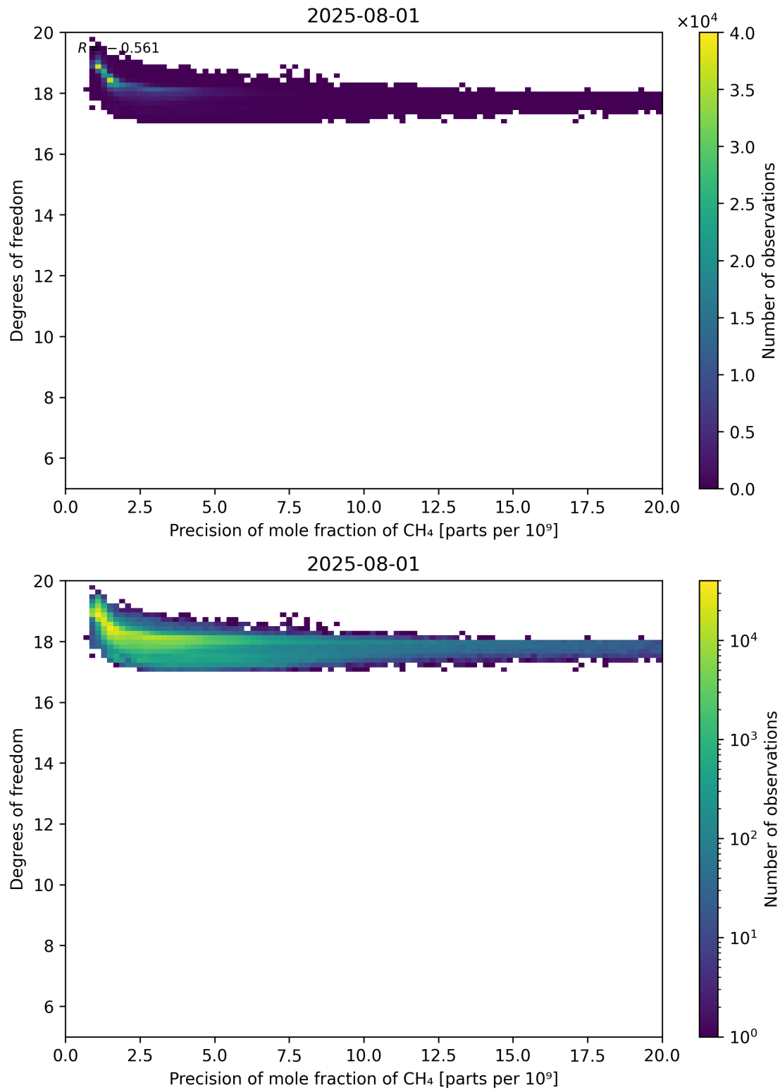
Figure 80: Scatter density plot of “Precision of mole fraction of CH 4 ” against “Degrees of freedom” for 2025-07-31 to 2025-08-02.
