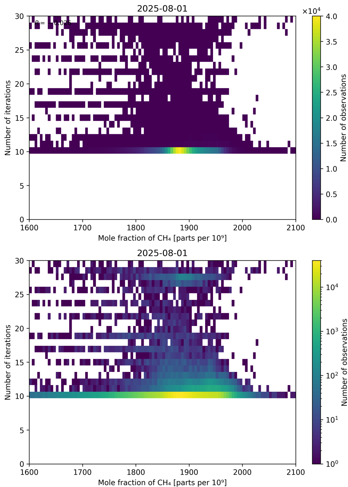
Figure 76: Scatter density plot of “Mole fraction of CH 4 ” against “Number of iterations” for 2025-07-31 to 2025-08-02.
