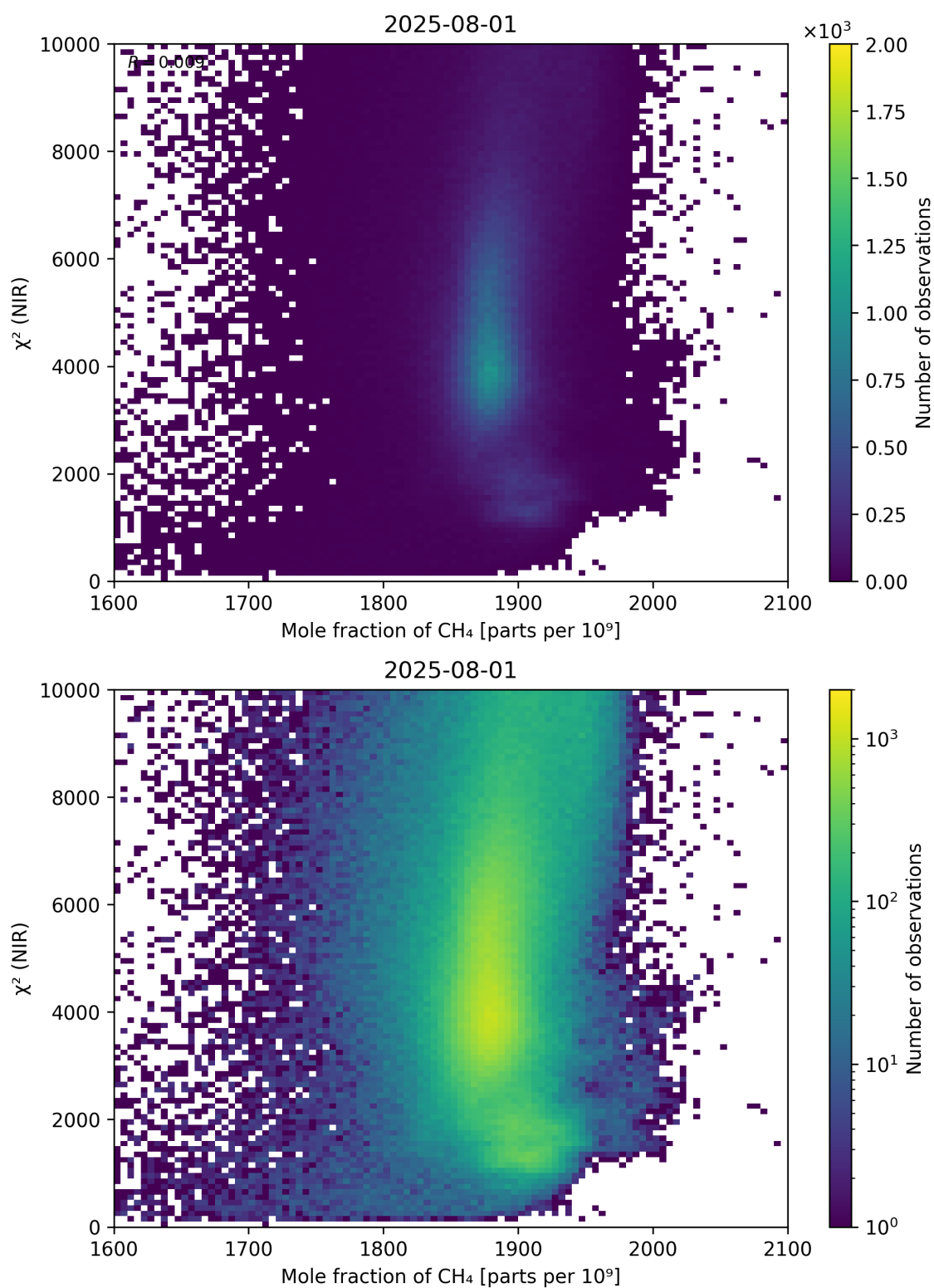
Figure 70: Scatter density plot of “Mole fraction of \text{CH}_4 ” against “ \chi^2 (NIR)” for 2025-07-31 to 2025-08-02.
