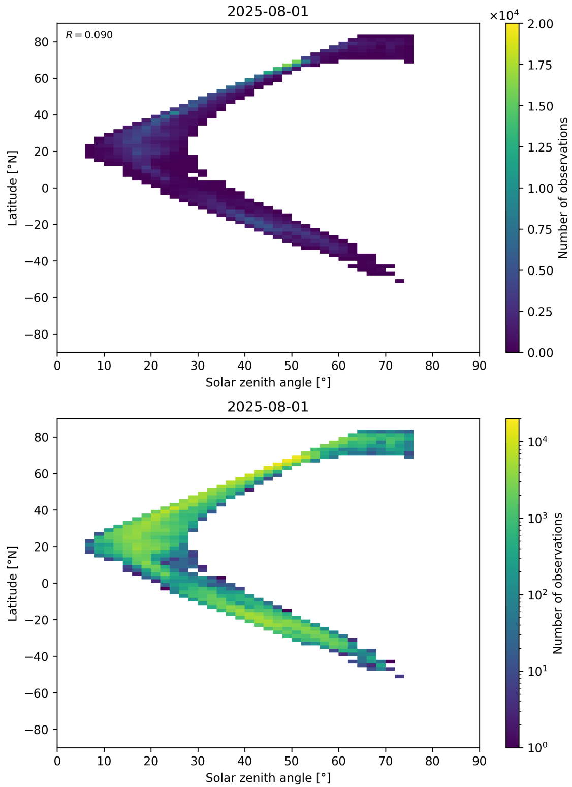
Figure 98: Scatter density plot of “Solar zenith angle” against “Latitude” for 2025-07-31 to 2025-08-02.
