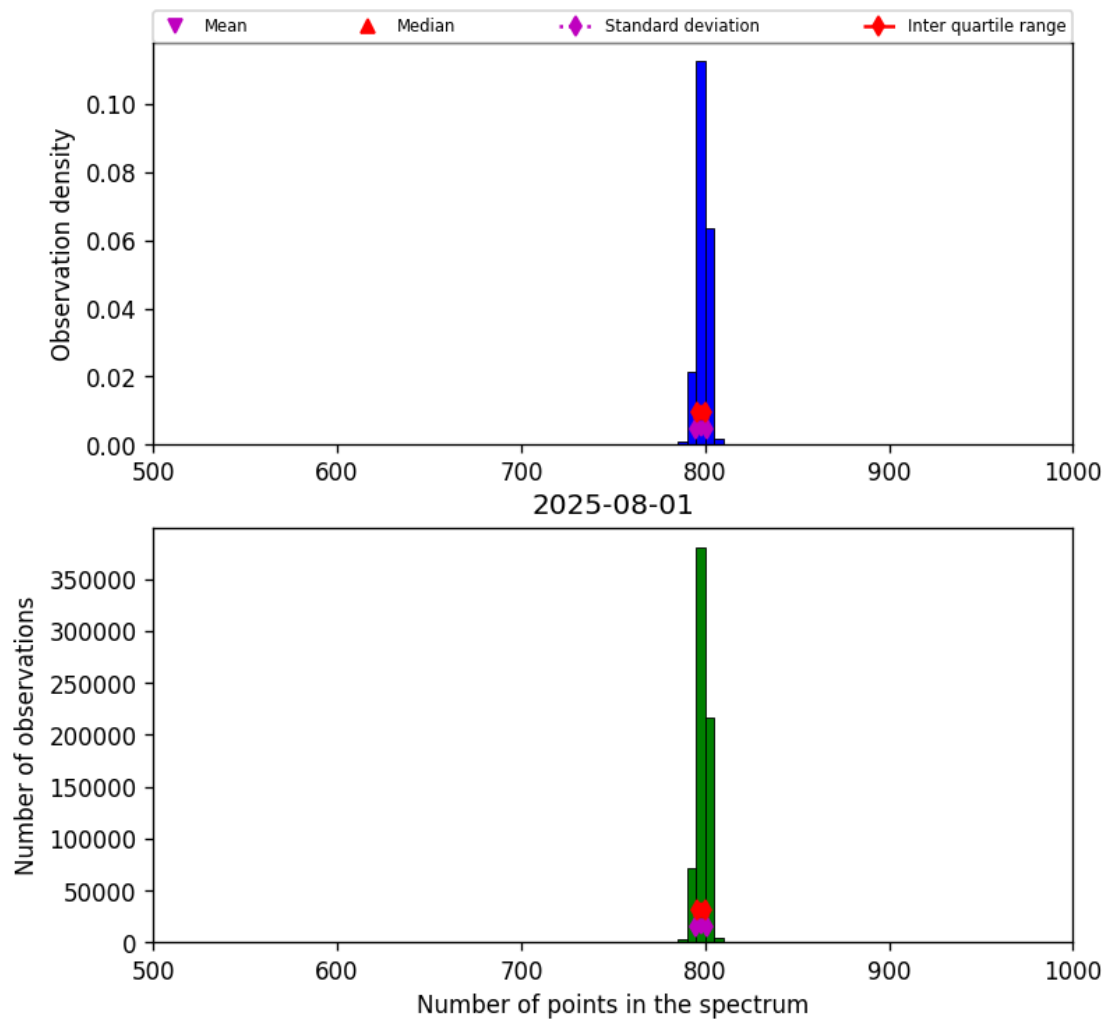
Figure 26: Histogram of “Number of points in the spectrum” for 2025-07-31 to 2025-08-02
