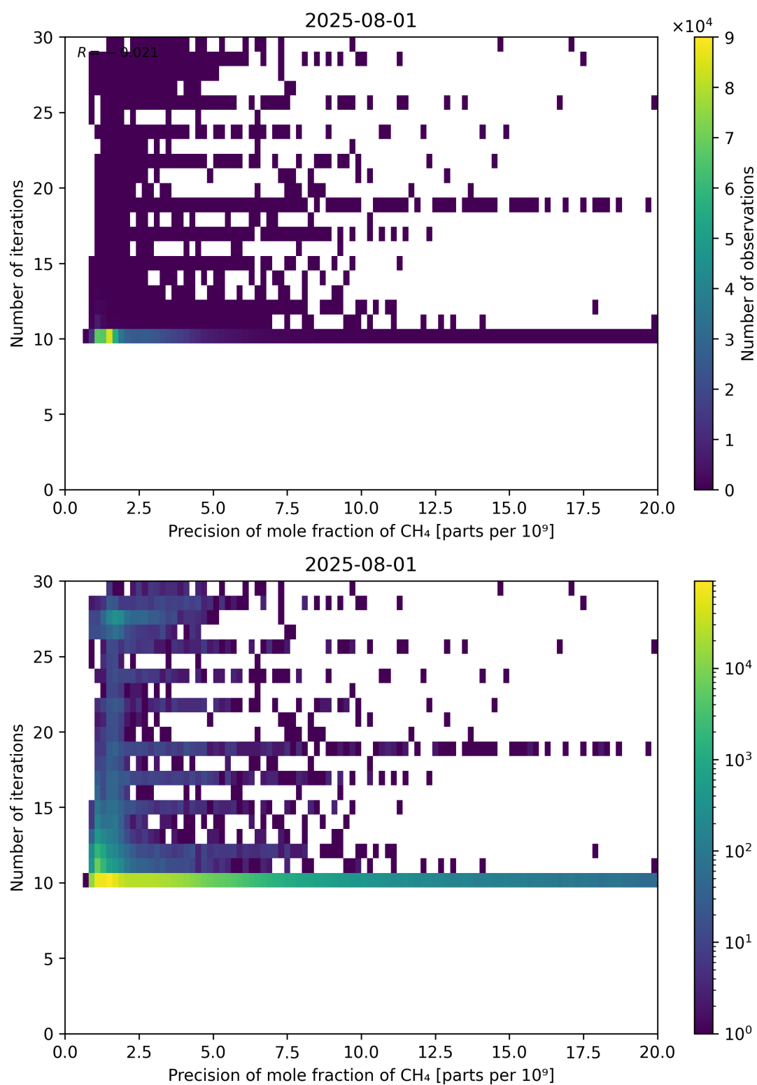
Figure 83: Scatter density plot of “Precision of mole fraction of CH 4 ” against “Number of iterations” for 2025-07-31 to 2025-08-02.
