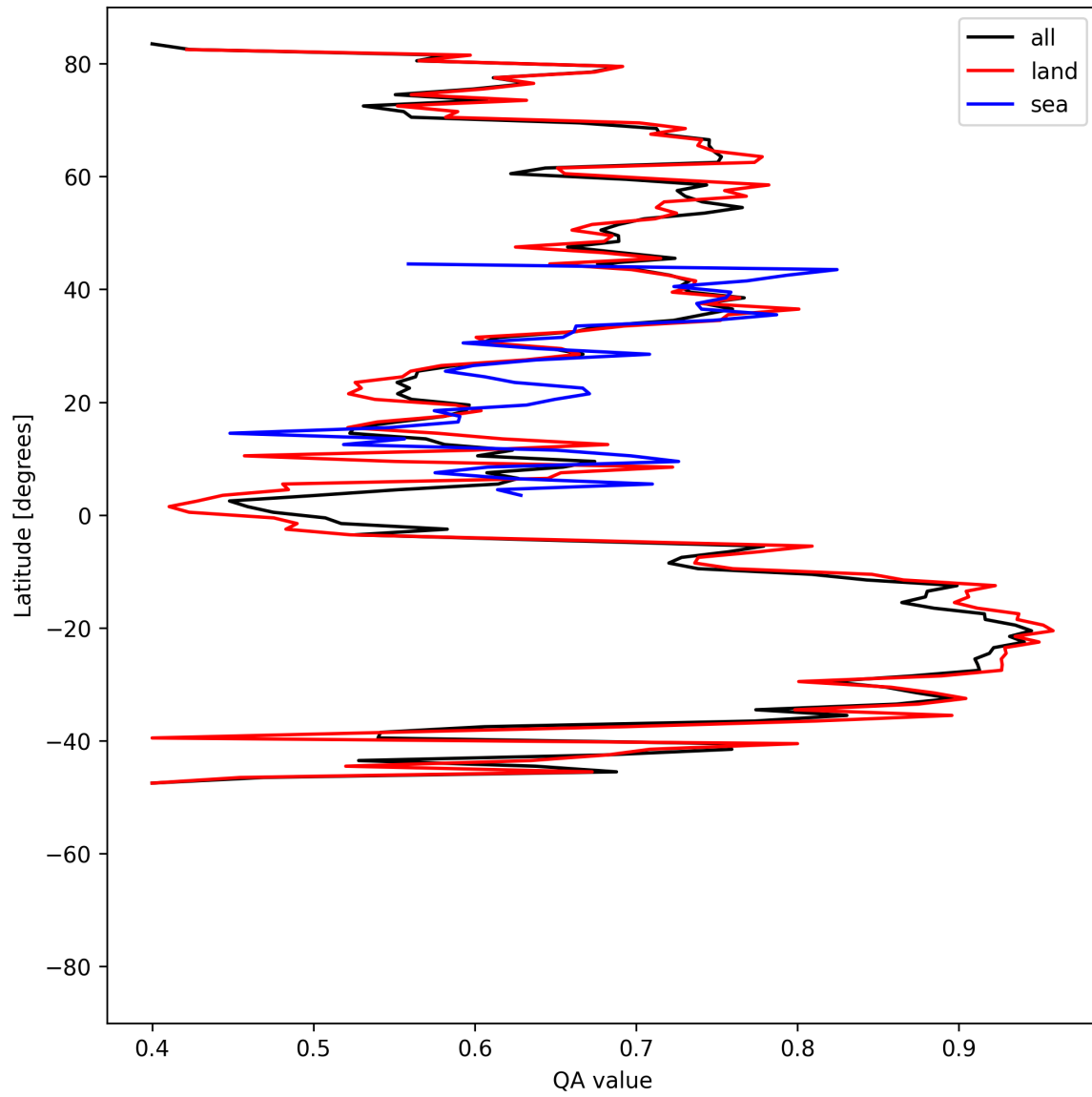
Figure 11: Zonal average of “QA value” for 2025-07-31 to 2025-08-02.
