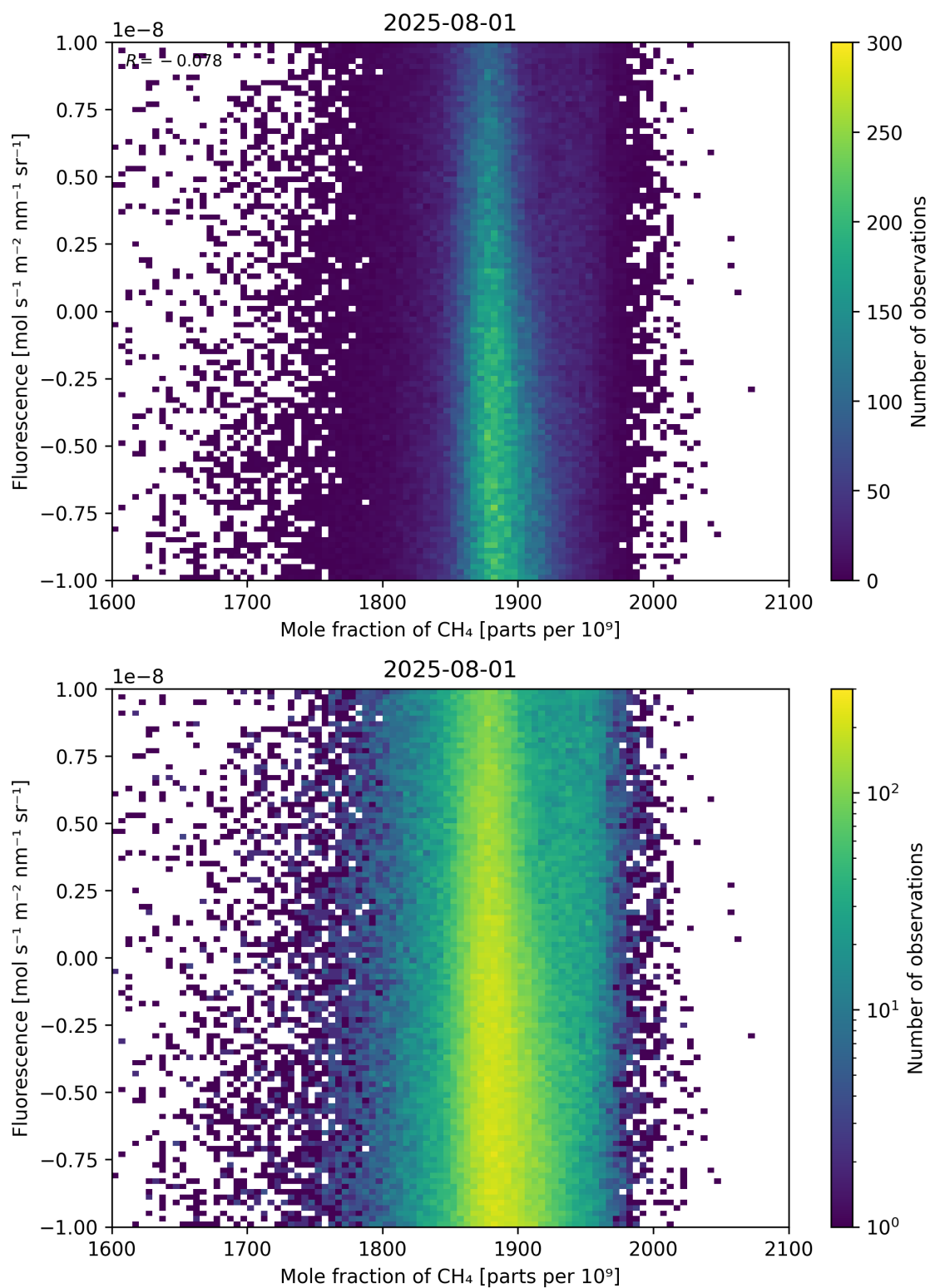
Figure 73: Scatter density plot of “Mole fraction of \text{CH}_4 ” against “Fluorescence” for 2025-07-31 to 2025-08-02.
