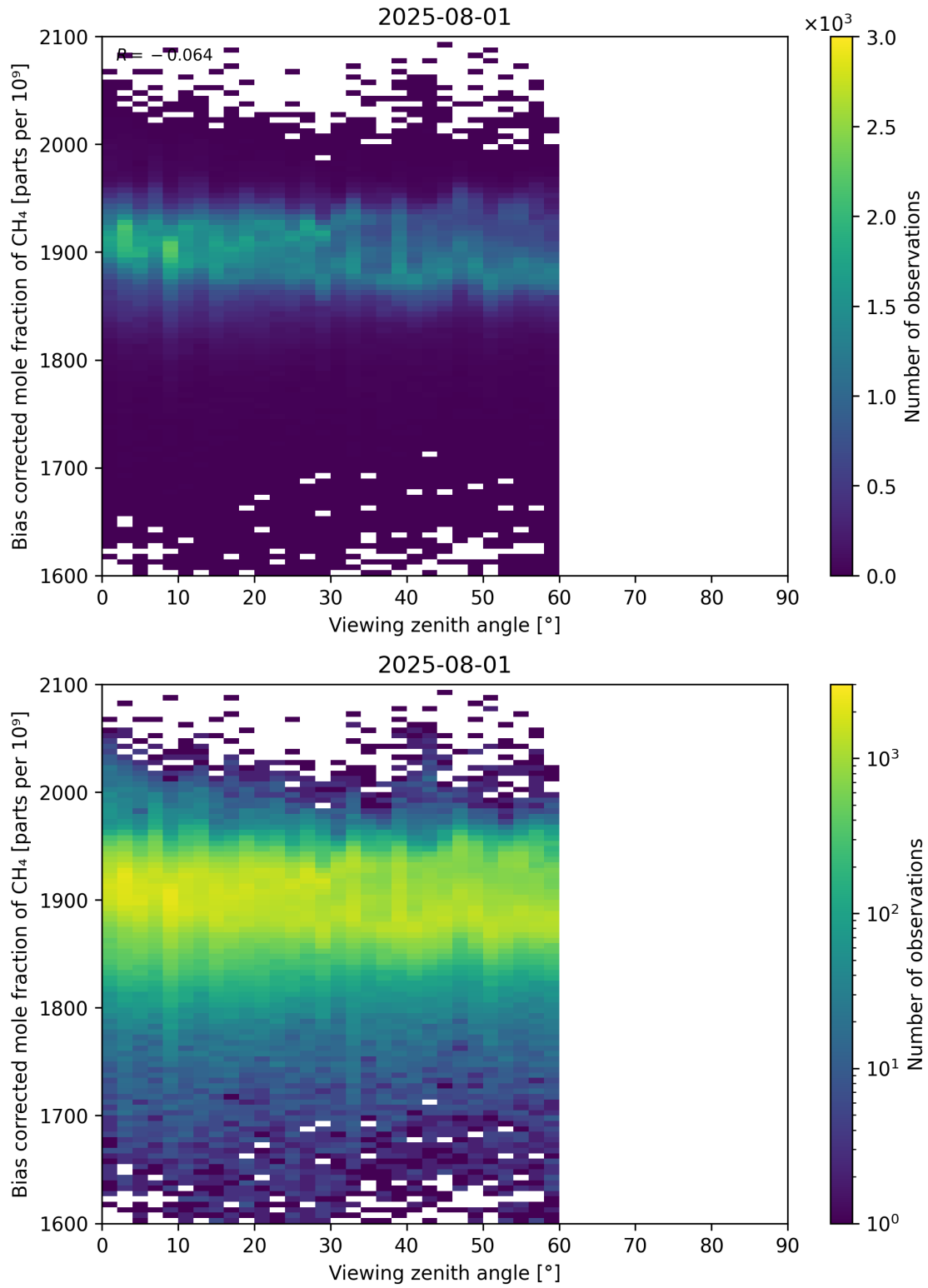
Figure 111: Scatter density plot of “Viewing zenith angle” against “Bias corrected mole fraction of CH 4 ” for 2025-07-31 to 2025-08-02.
