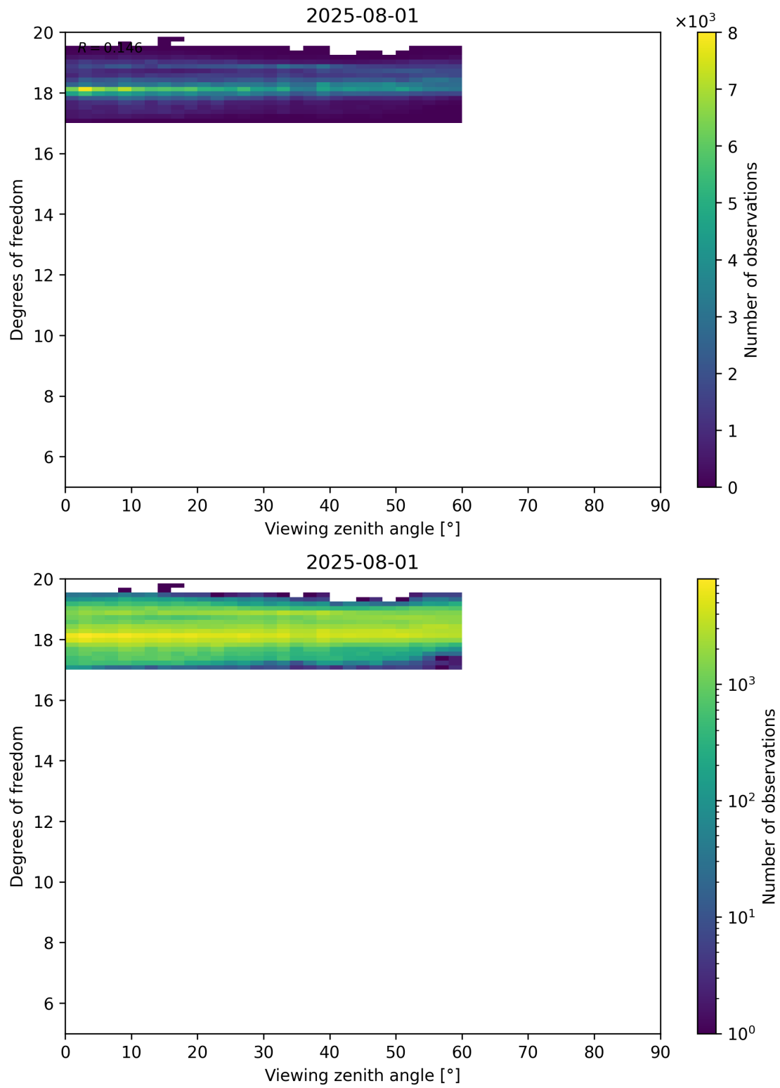
Figure 107: Scatter density plot of “Viewing zenith angle” against “Degrees of freedom” for 2025-07-31 to 2025-08-02.
