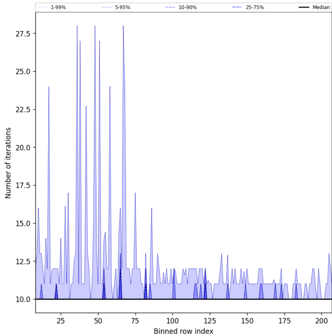
Figure 42: Along track statistics of “Number of iterations” for 2025-07-31 to 2025-08-02
