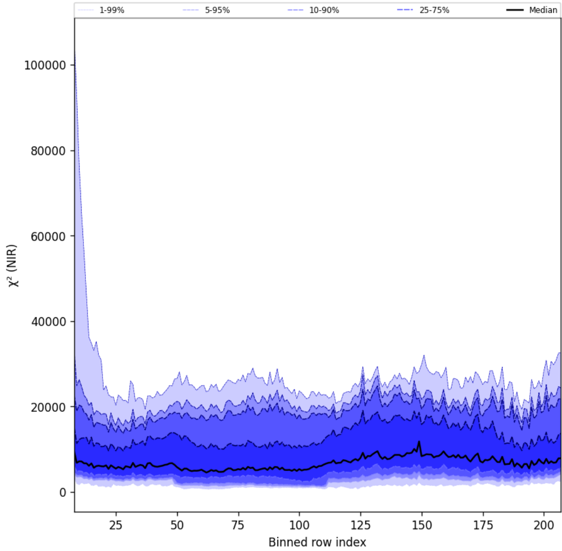
Figure 40: Along track statistics of “ \chi^2 (NIR)” for 2025-07-31 to 2025-08-02
