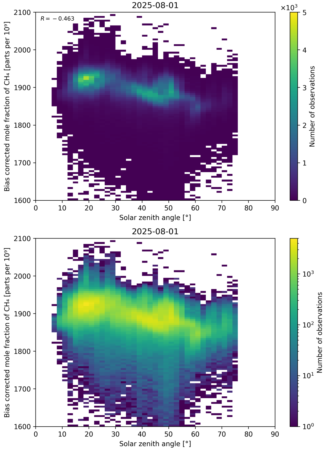
Figure 100: Scatter density plot of “Solar zenith angle” against “Bias corrected mole fraction of \text{CH}_4 ” for 2025-07-31 to 2025-08-02.
