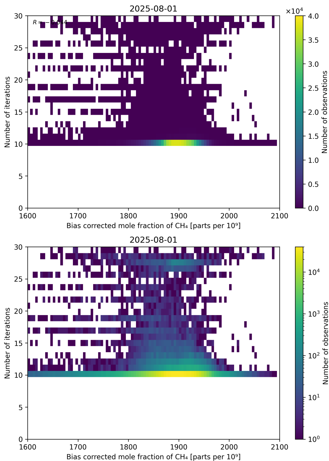
Figure 67: Scatter density plot of “Bias corrected mole fraction of CH 4 ” against “Number of iterations” for 2025-07-31 to 2025-08-02.
