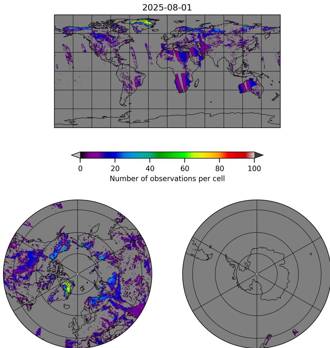
Figure 10: Map of the number of observations for 2025-07-31 to 2025-08-02
