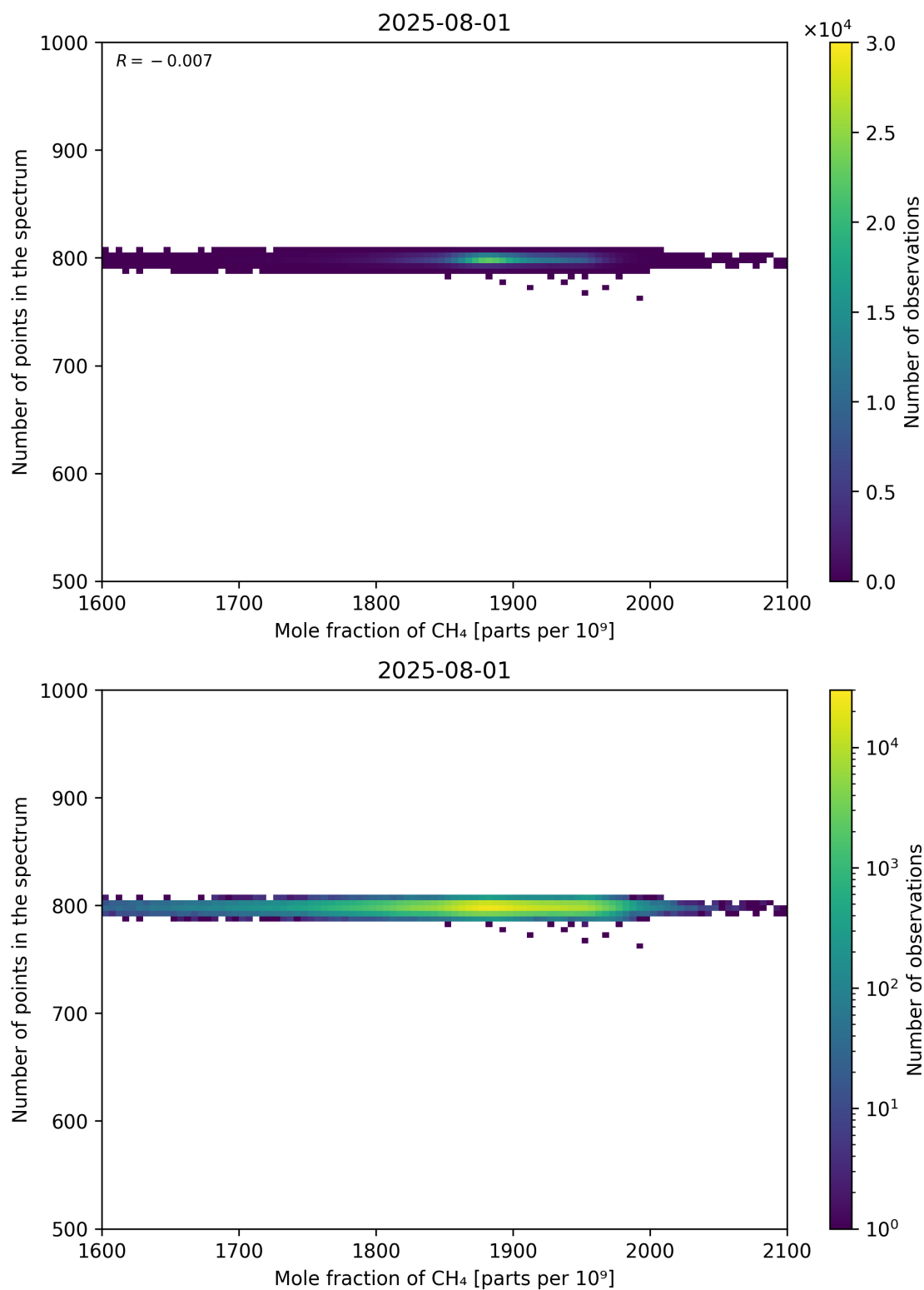
Figure 77: Scatter density plot of “Mole fraction of CH 4 ” against “Number of points in the spectrum” for 2025-07-31 to 2025-08-02.
