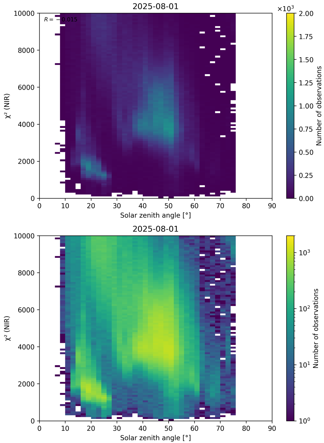
Figure 94: Scatter density plot of “Solar zenith angle” against “ \chi^2 (NIR)” for 2025-07-31 to 2025-08-02.
