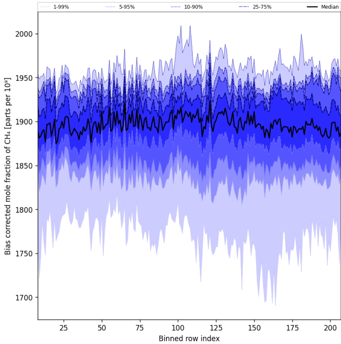
Figure 36: Along track statistics of “Bias corrected mole fraction of CH 4 ” for 2025-07-31 to 2025-08-02
