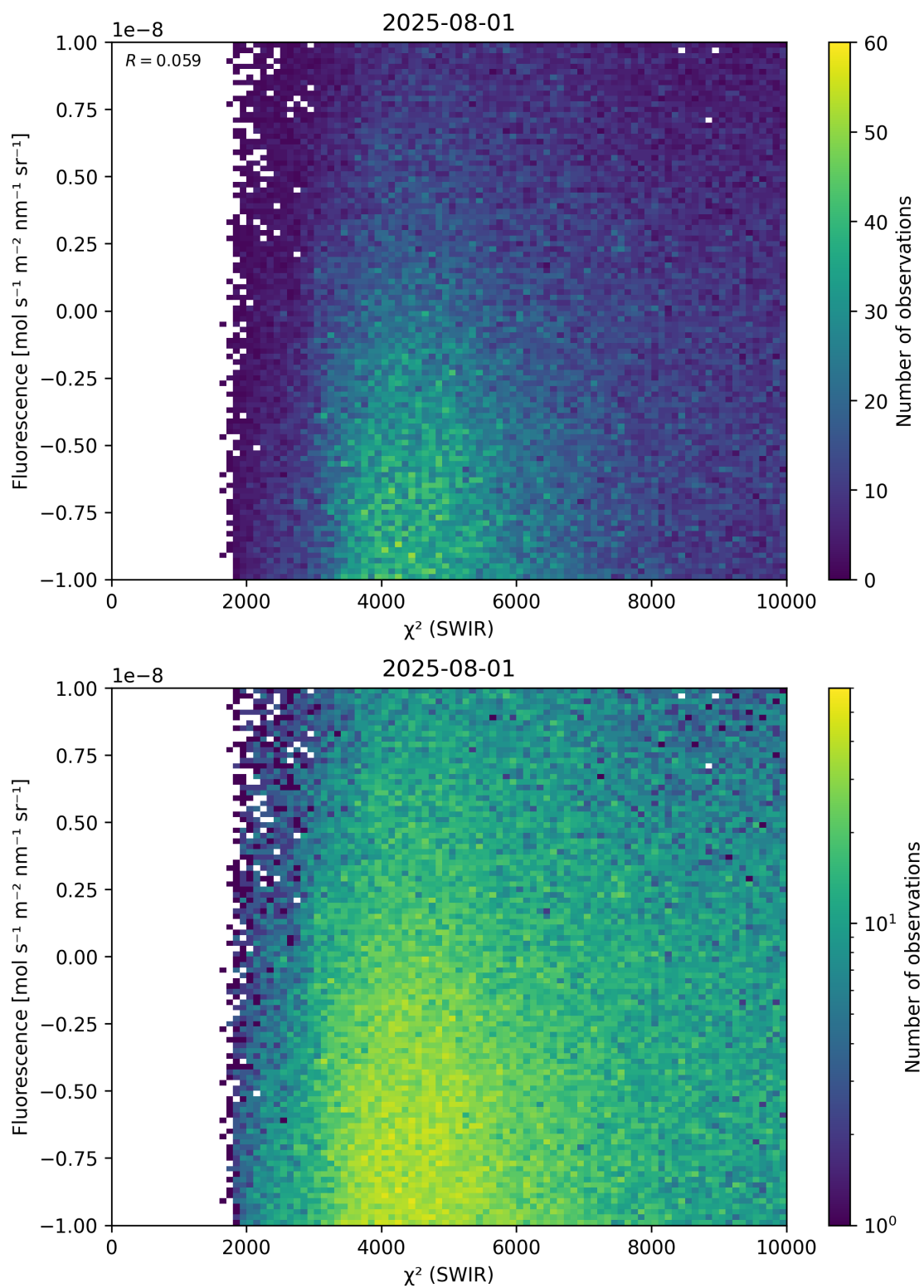
Figure 49: Scatter density plot of “ \chi^2 (SWIR)” against “Fluorescence” for 2025-07-31 to 2025-08-02.
