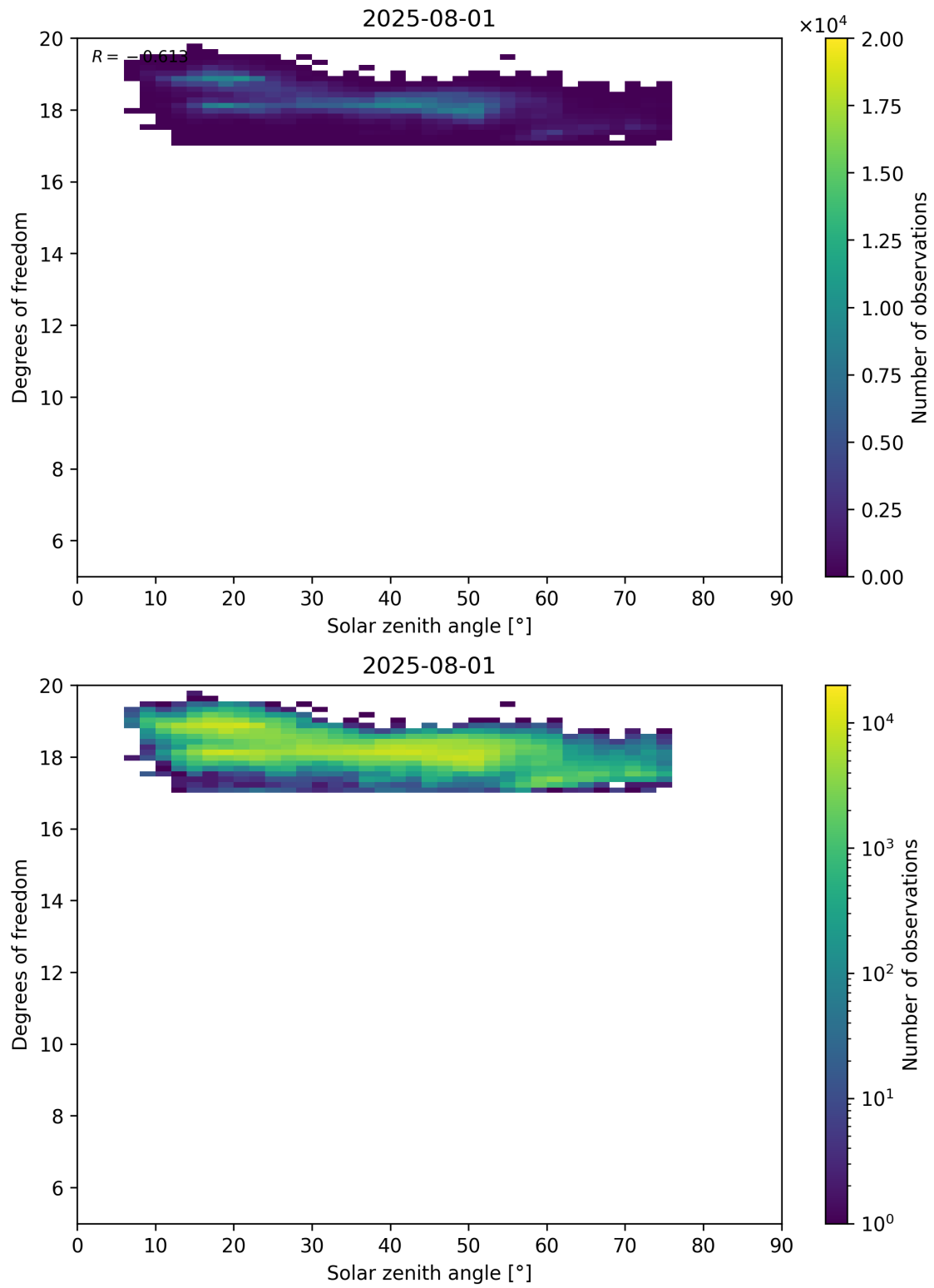
Figure 96: Scatter density plot of “Solar zenith angle” against “Degrees of freedom” for 2025-07-31 to 2025-08-02.
