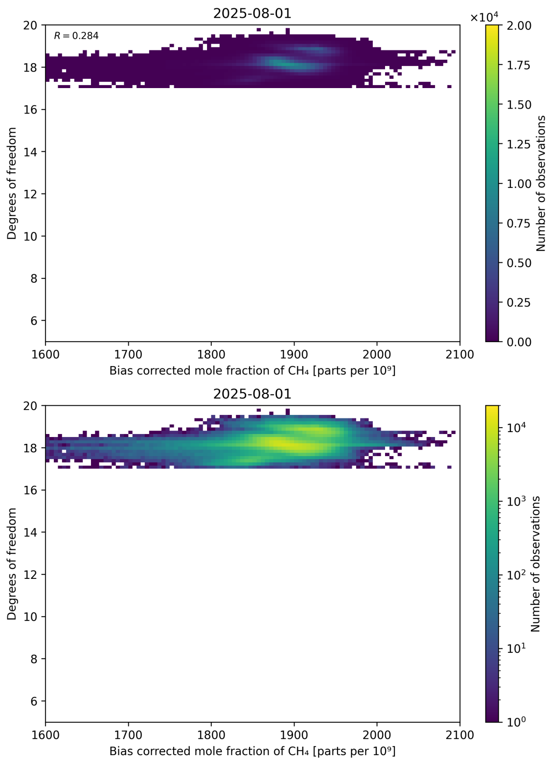
Figure 65: Scatter density plot of “Bias corrected mole fraction of CH 4 ” against “Degrees of freedom” for 2025-07-31 to 2025-08-02.
