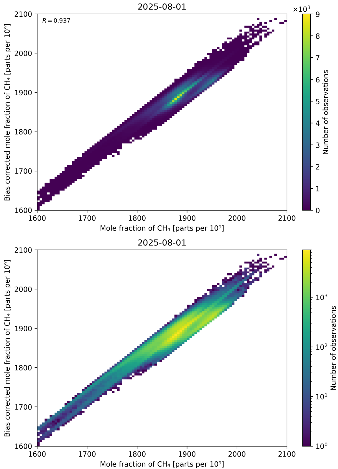
Figure 74: Scatter density plot of “Mole fraction of CH 4 ” against “Bias corrected mole fraction of CH 4 ” for 2025-07-31 to 2025-08-02.
