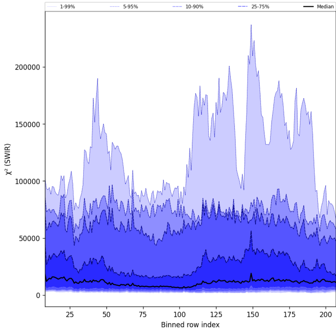
Figure 39: Along track statistics of “ \chi^2 (SWIR)” for 2025-07-31 to 2025-08-02
