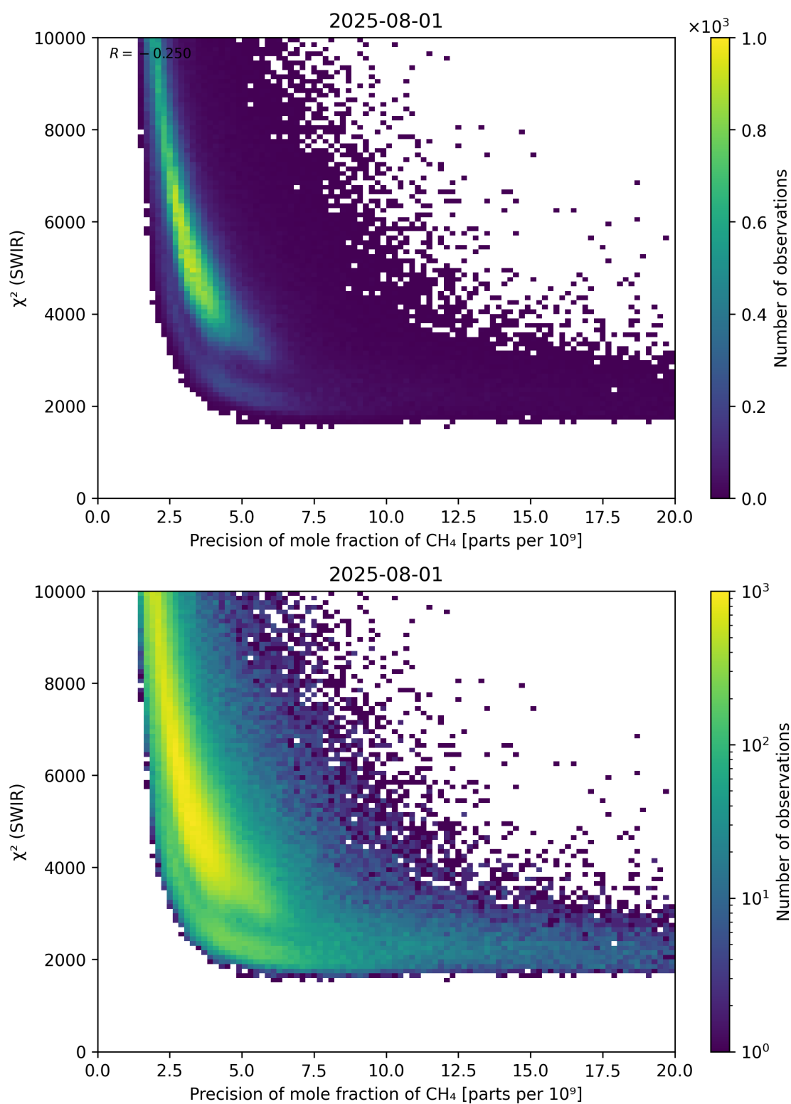
Figure 79: Scatter density plot of “Precision of mole fraction of \text{CH}_4 ” against “ \chi^2 (SWIR)” for 2025-07-31 to 2025-08-02.
