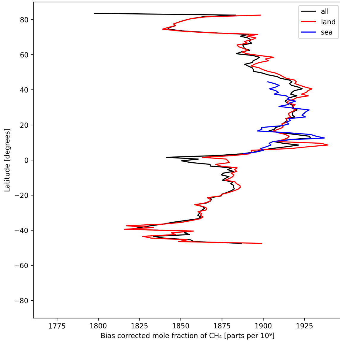
Figure 14: Zonal average of “Bias corrected mole fraction of \text{CH}_4 ” for 2025-07-31 to 2025-08-02.
