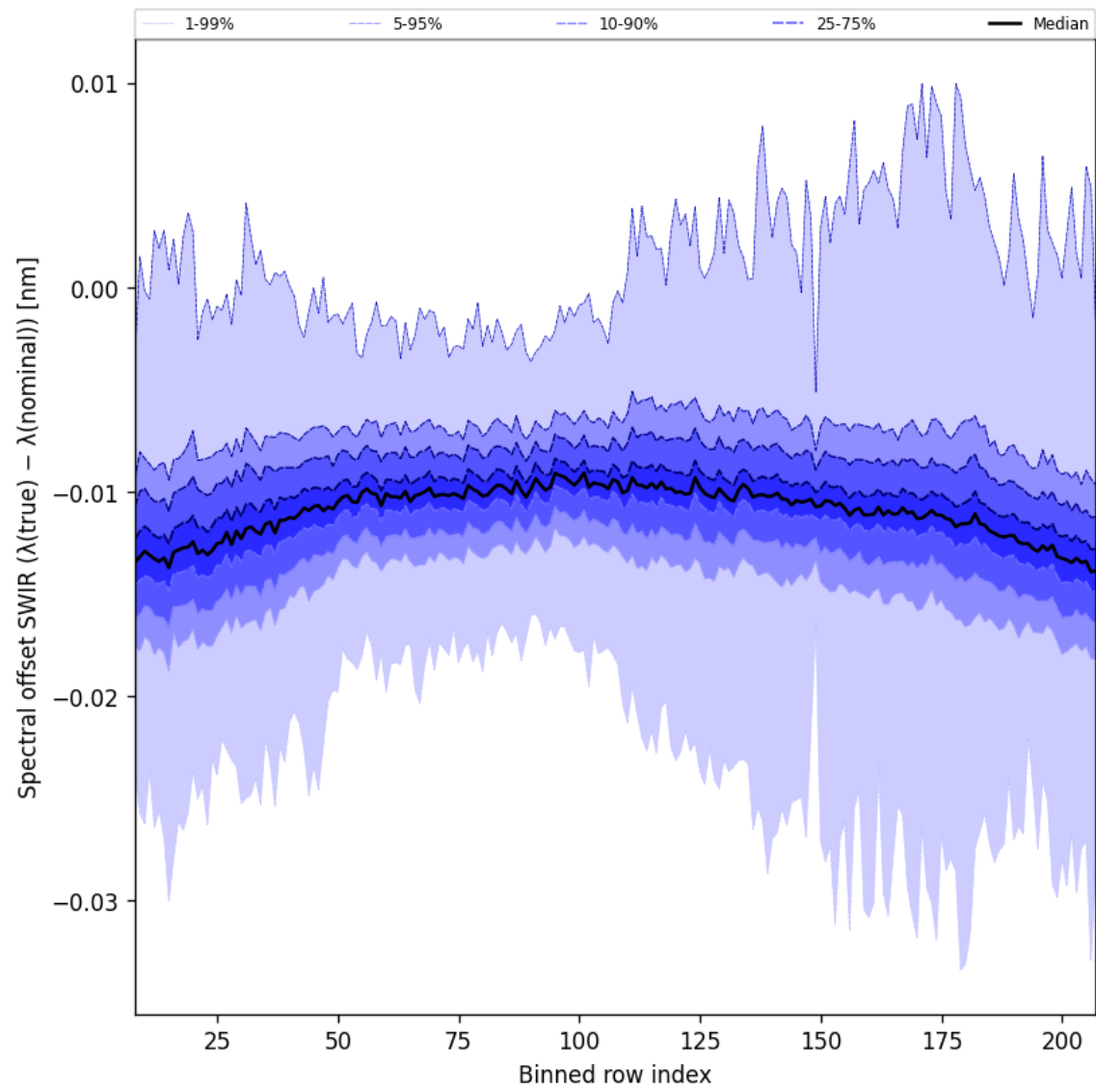
Figure 38: Along track statistics of “Spectral offset SWIR ( \lambda_{\text{true}} - \lambda_{\text{nominal}} )” for 2025-07-31 to 2025-08-02
