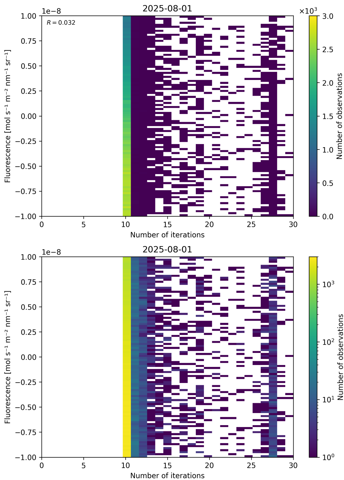
Figure 87: Scatter density plot of "Number of iterations" against "Fluorescence" for 2025-07-31 to 2025-08-02.
