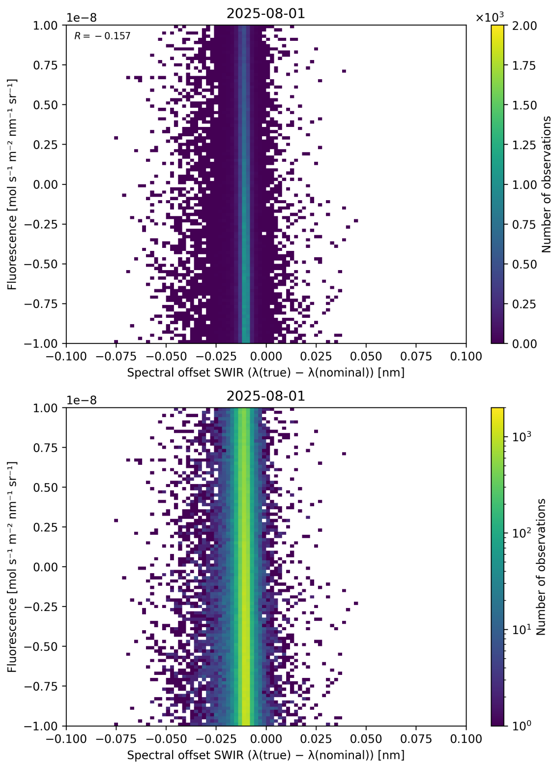
Figure 120: Scatter density plot of “Spectral offset SWIR ( \lambda_{\text{true}} - \lambda_{\text{nominal}} )” against “Fluorescence” for 2025-07-31 to 2025-08-02.
