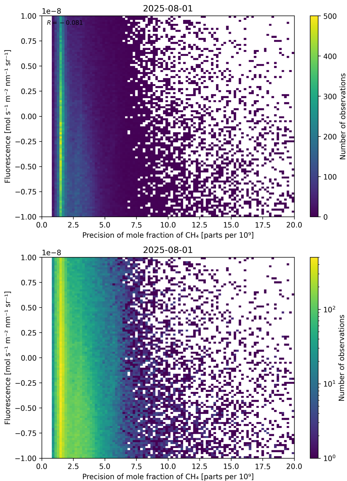
Figure 81: Scatter density plot of “Precision of mole fraction of \text{CH}_4 ” against “Fluorescence” for 2025-07-31 to 2025-08-02.
