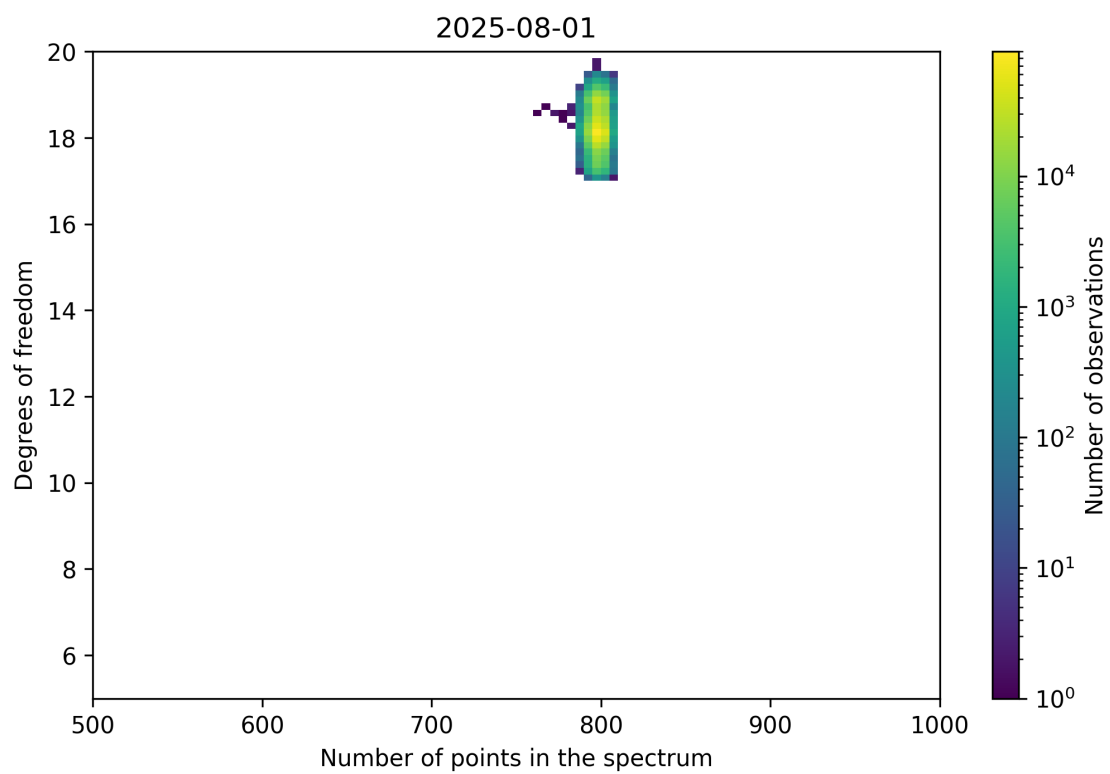
Figure 90: Scatter density plot of “Number of points in the spectrum” against “Degrees of freedom” for 2025-07-31 to 2025-08-02.
