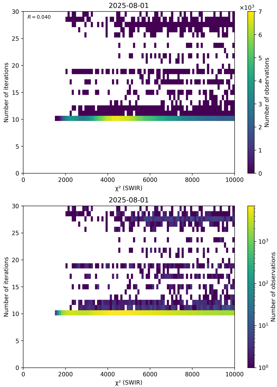
Figure 50: Scatter density plot of “ \chi^2 (SWIR)” against “Number of iterations” for 2025-07-31 to 2025-08-02.
