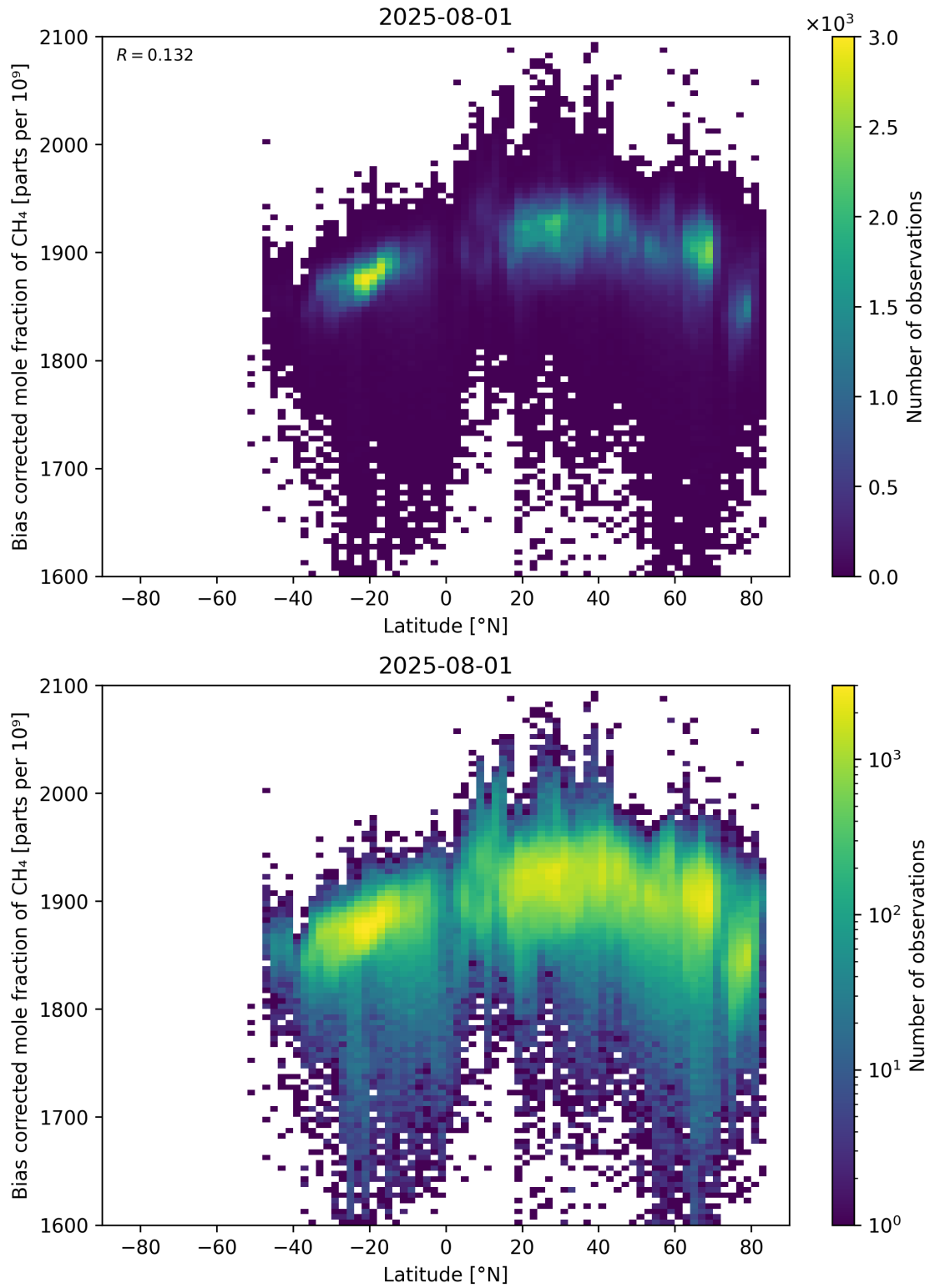
Figure 58: Scatter density plot of “Latitude” against “Bias corrected mole fraction of \text{CH}_4 ” for 2025-07-31 to 2025-08-02.
