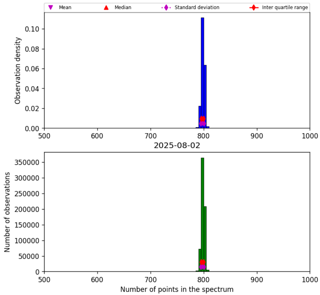
Figure 26: Histogram of “Number of points in the spectrum” for 2025-08-01 to 2025-08-03
