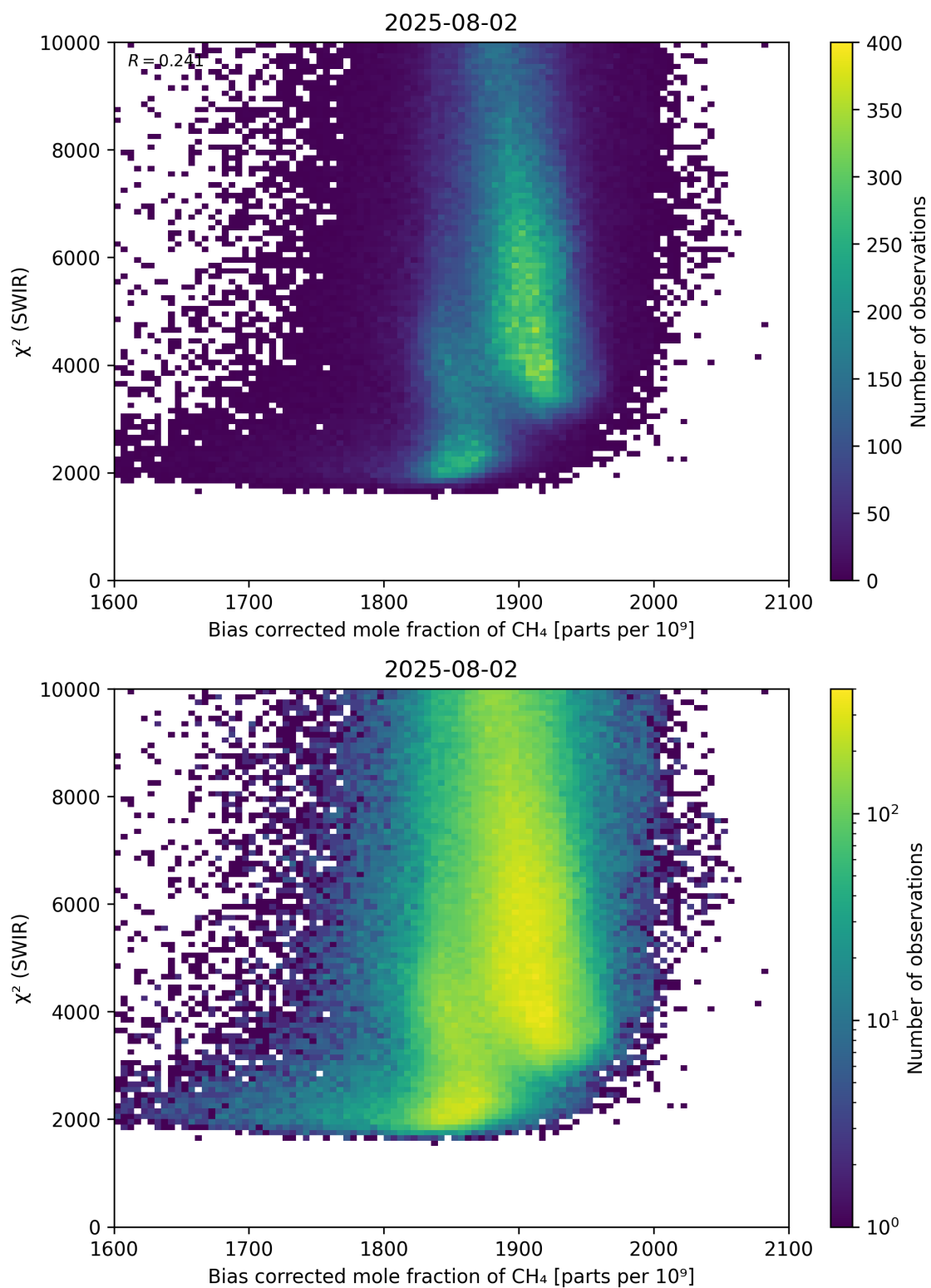
Figure 64: Scatter density plot of “Bias corrected mole fraction of \text{CH}_4 ” against “ \chi^2 (SWIR)” for 2025-08-01 to 2025-08-03.
