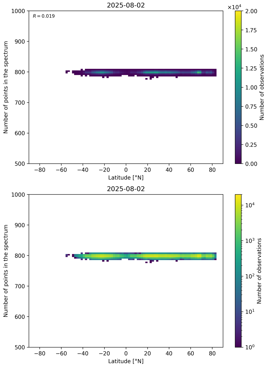
Figure 61: Scatter density plot of “Latitude” against “Number of points in the spectrum” for 2025-08-01 to 2025-08-03.
