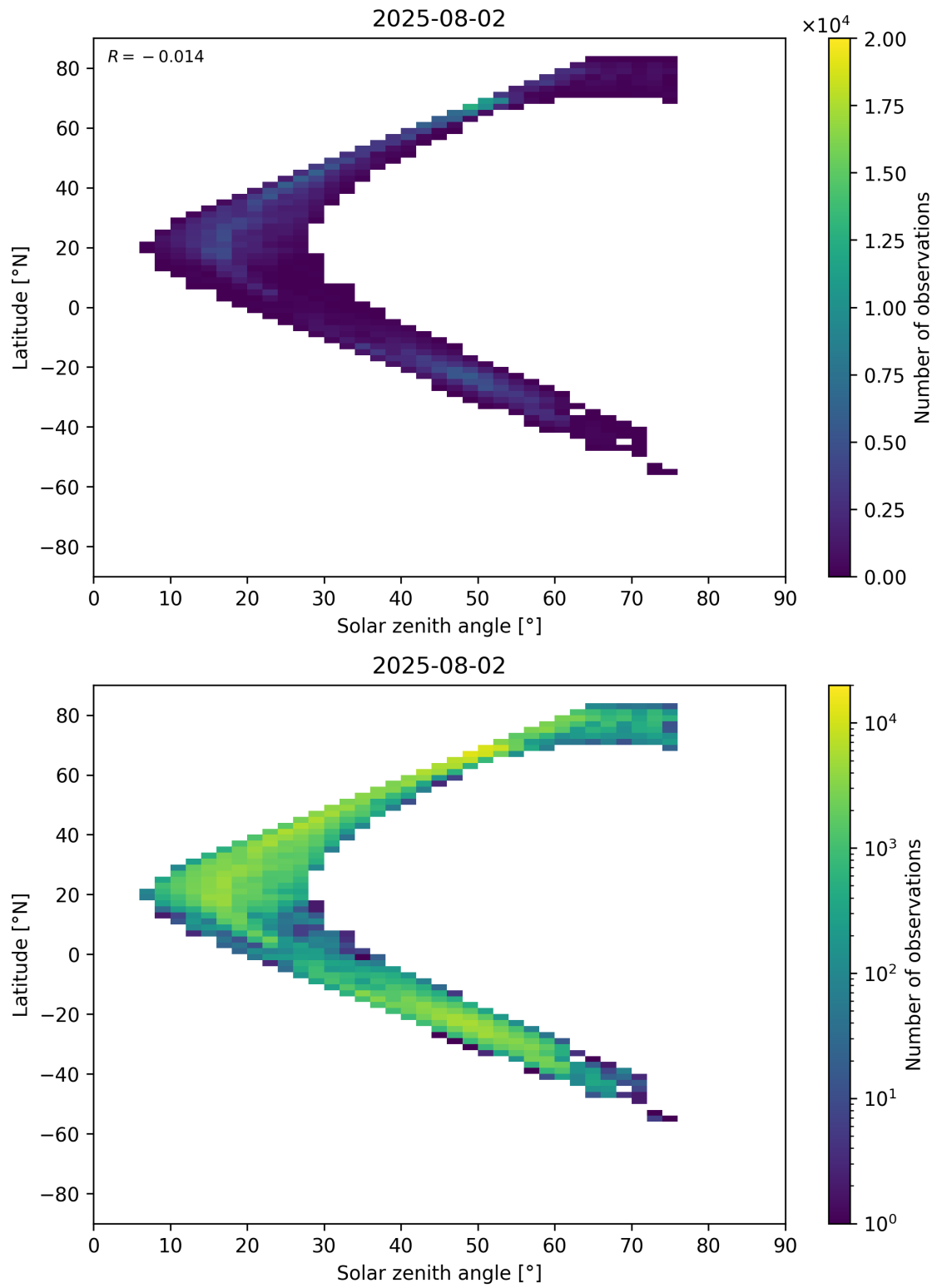
Figure 98: Scatter density plot of “Solar zenith angle” against “Latitude” for 2025-08-01 to 2025-08-03.
