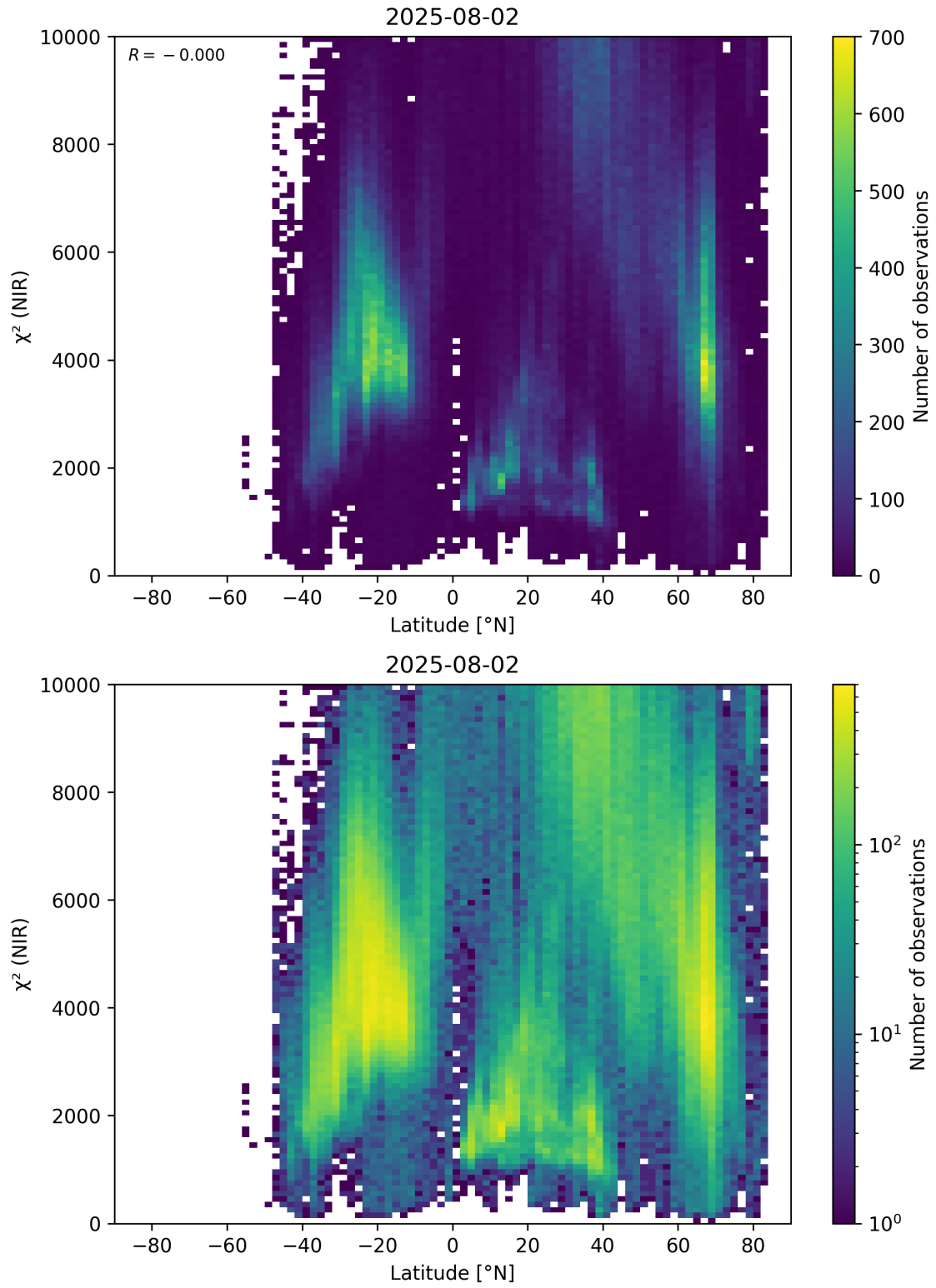
Figure 53: Scatter density plot of “Latitude” against “ \chi^2 (NIR)” for 2025-08-01 to 2025-08-03.
