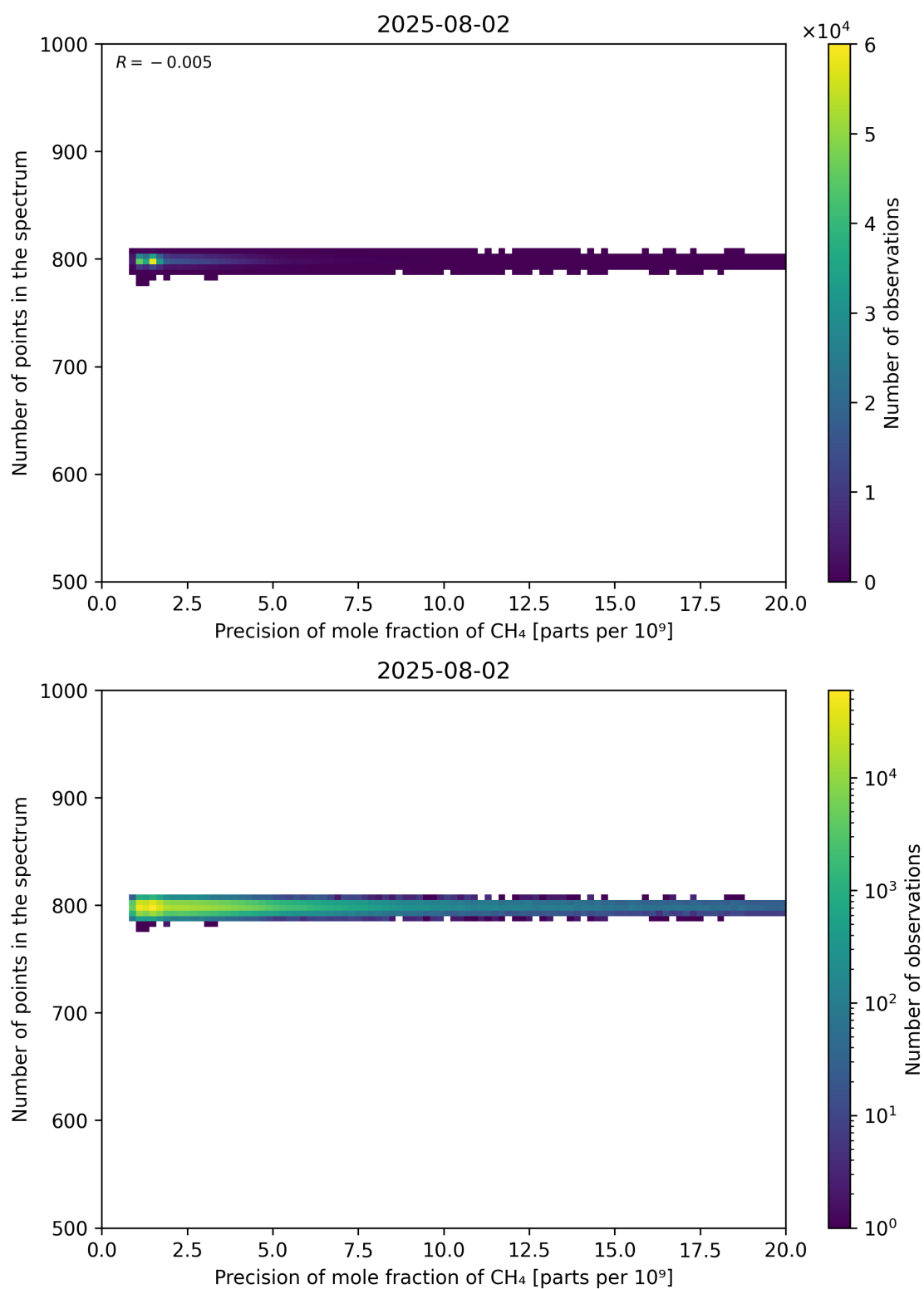
Figure 84: Scatter density plot of “Precision of mole fraction of CH 4 ” against “Number of points in the spectrum” for 2025-08-01 to 2025-08-03.
