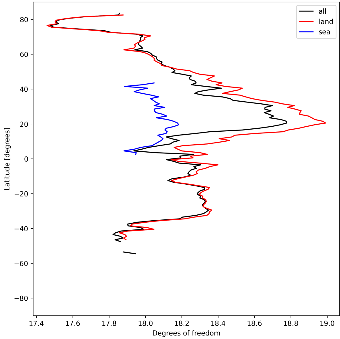
Figure 19: Zonal average of “Degrees of freedom” for 2025-08-01 to 2025-08-03.
