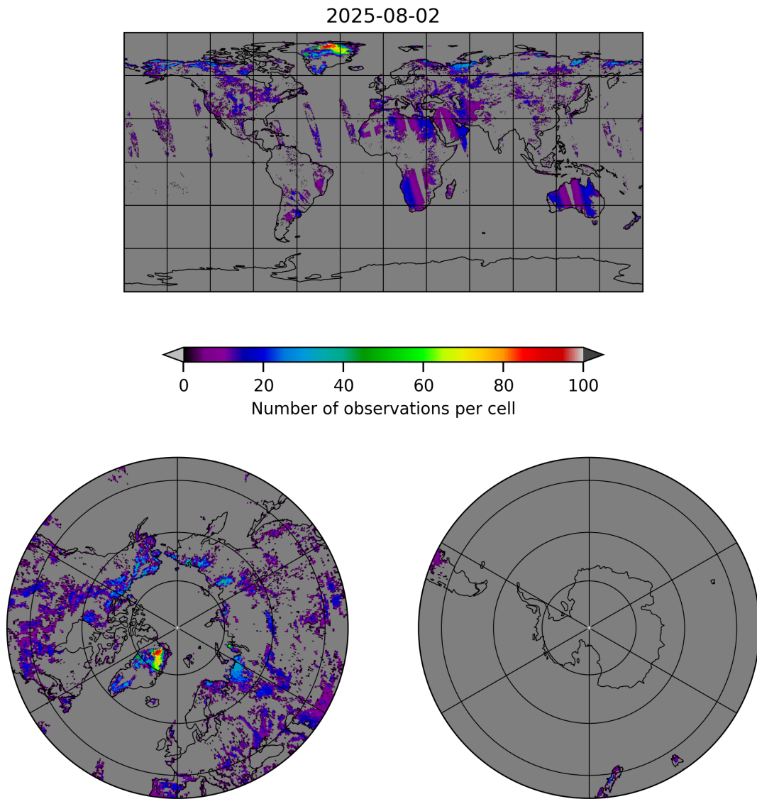
Figure 10: Map of the number of observations for 2025-08-01 to 2025-08-03
