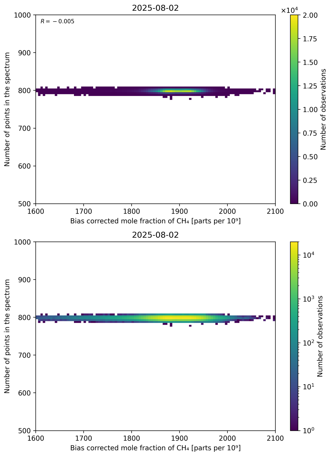
Figure 68: Scatter density plot of “Bias corrected mole fraction of CH 4 ” against “Number of points in the spectrum” for 2025-08-01 to 2025-08-03.
