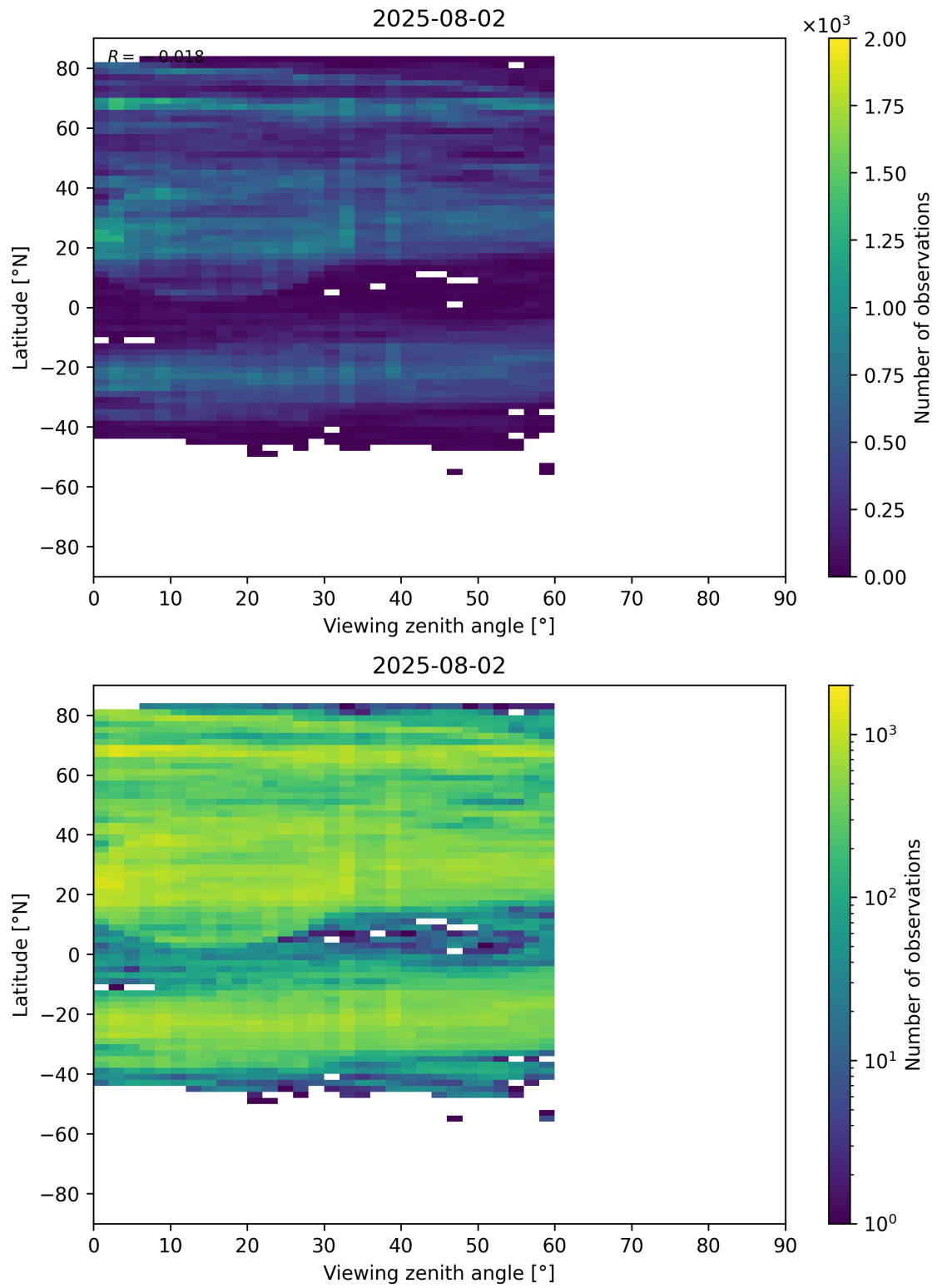
Figure 109: Scatter density plot of “Viewing zenith angle” against “Latitude” for 2025-08-01 to 2025-08-03.
