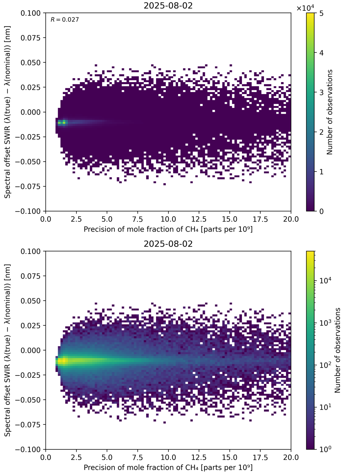
Figure 85: Scatter density plot of “Precision of mole fraction of CH 4 ” against “Spectral offset SWIR ( \lambda_{\text{true}} - \lambda_{\text{nominal}} )” for 2025-08-01 to 2025-08-03.
