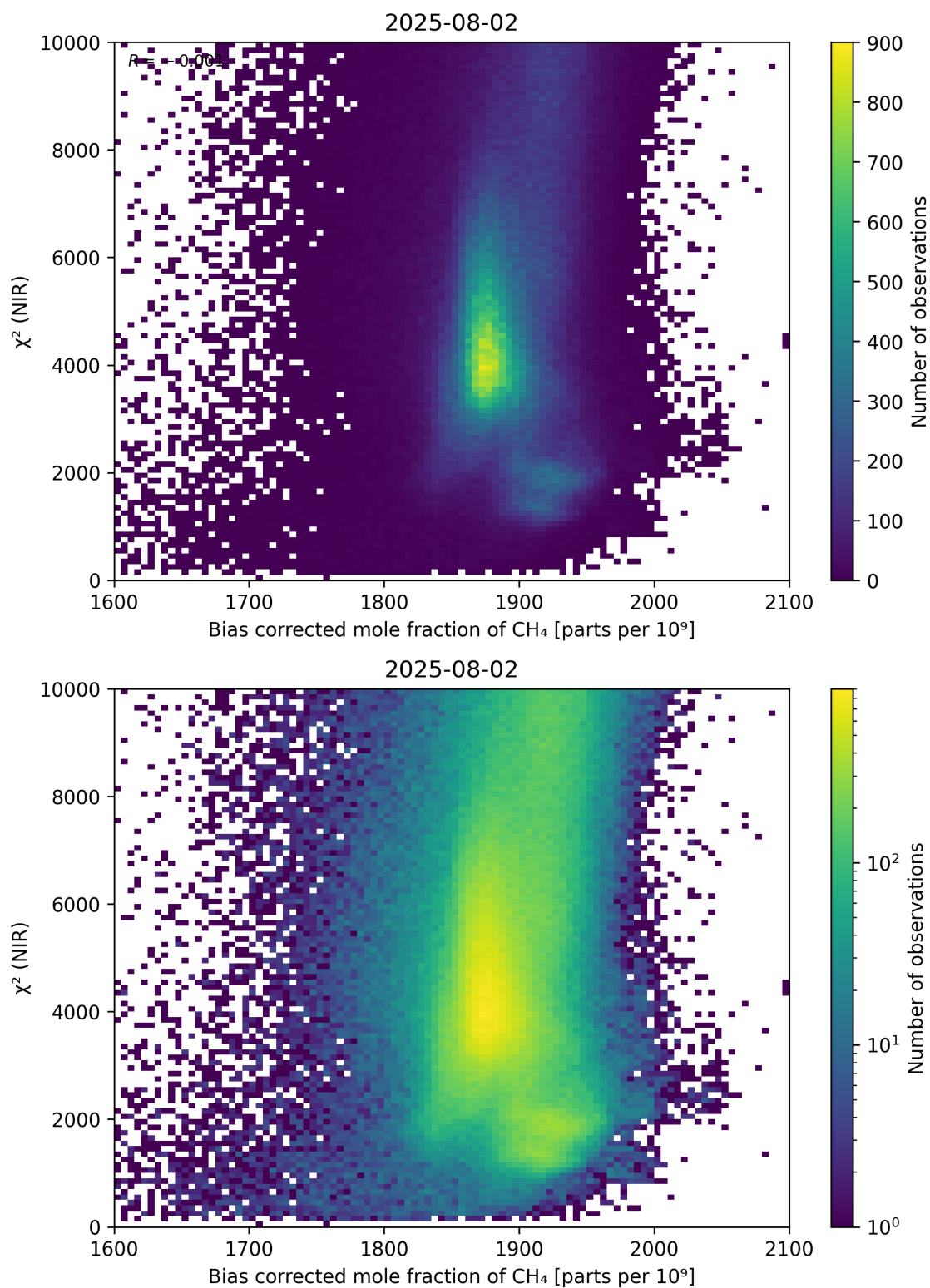
Figure 63: Scatter density plot of “Bias corrected mole fraction of CH 4 ” against “ \chi^2 (NIR)” for 2025-08-01 to 2025-08-03.
