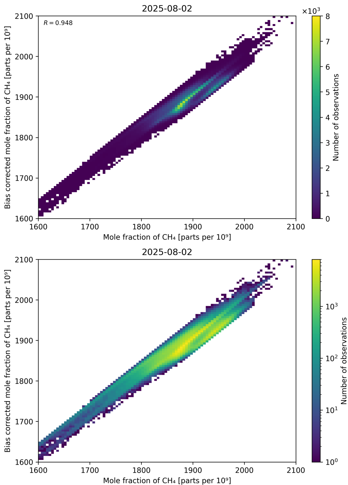
Figure 74: Scatter density plot of “Mole fraction of CH 4 ” against “Bias corrected mole fraction of CH 4 ” for 2025-08-01 to 2025-08-03.
