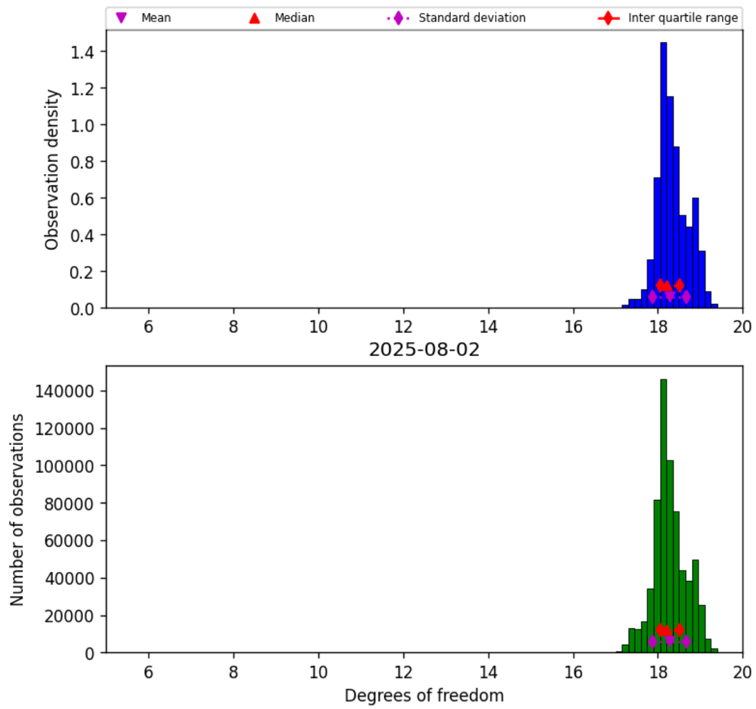
Figure 30: Histogram of “Degrees of freedom” for 2025-08-01 to 2025-08-03
