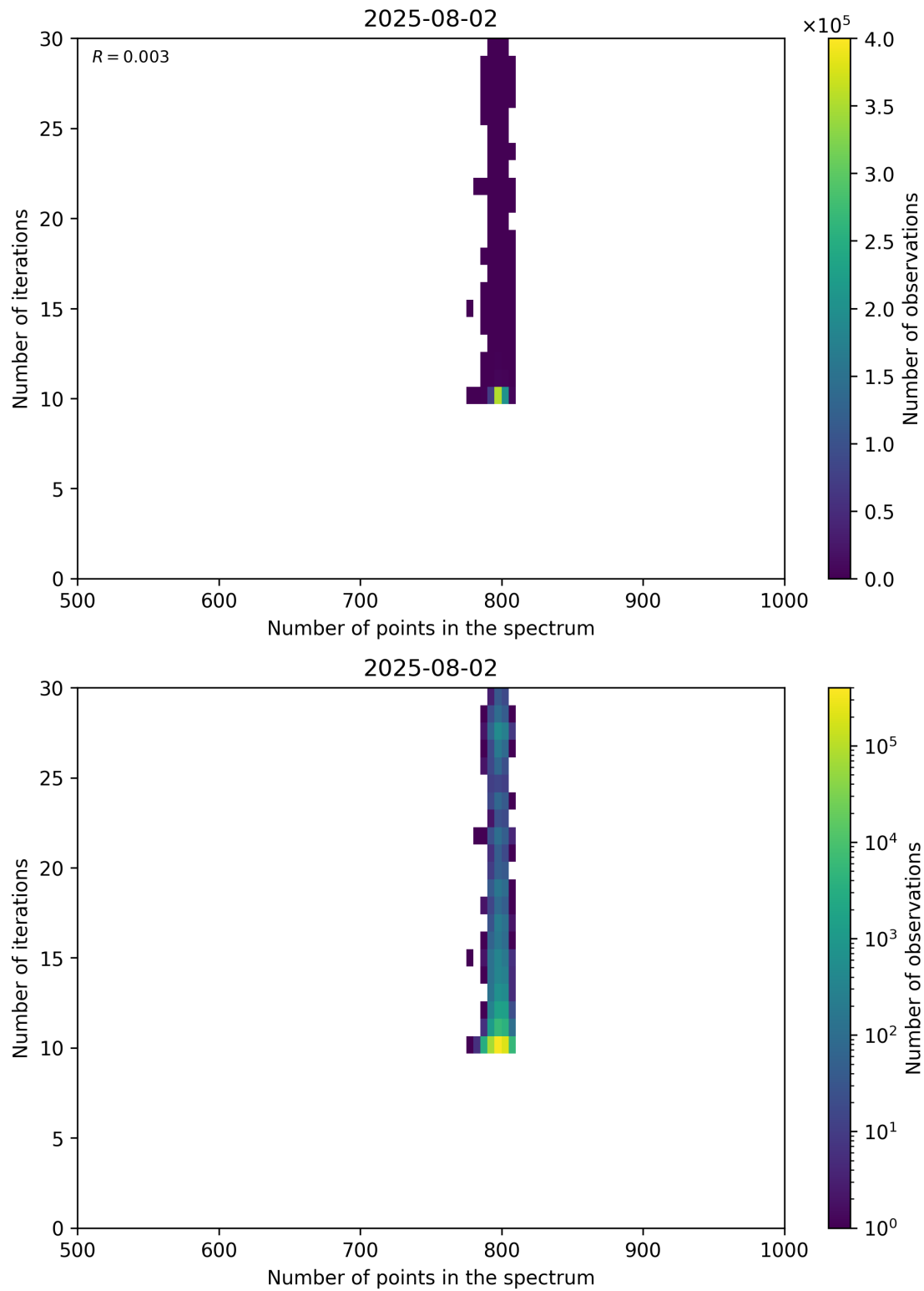
Figure 92: Scatter density plot of “Number of points in the spectrum” against “Number of iterations” for 2025-08-01 to 2025-08-03.
