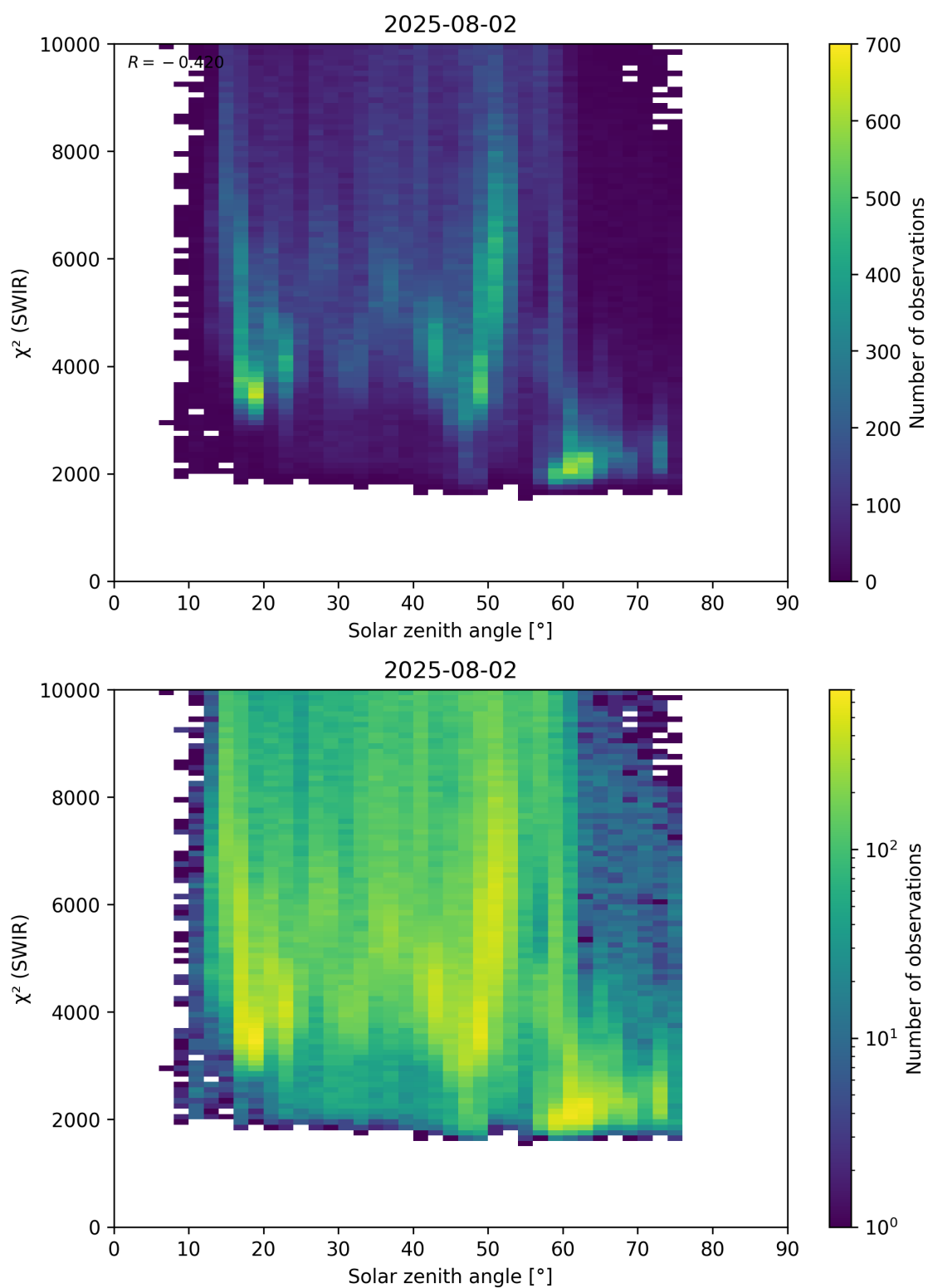
Figure 95: Scatter density plot of “Solar zenith angle” against “ \chi^2 (SWIR)” for 2025-08-01 to 2025-08-03.
