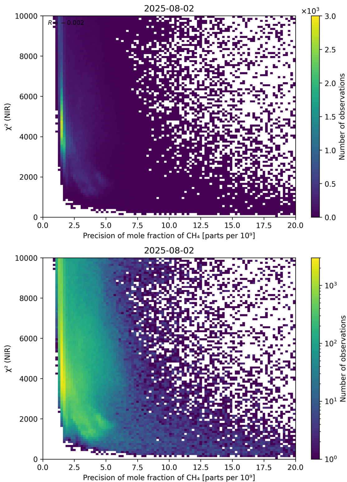
Figure 78: Scatter density plot of “Precision of mole fraction of \text{CH}_4 ” against “ \chi^2 (NIR)” for 2025-08-01 to 2025-08-03.
