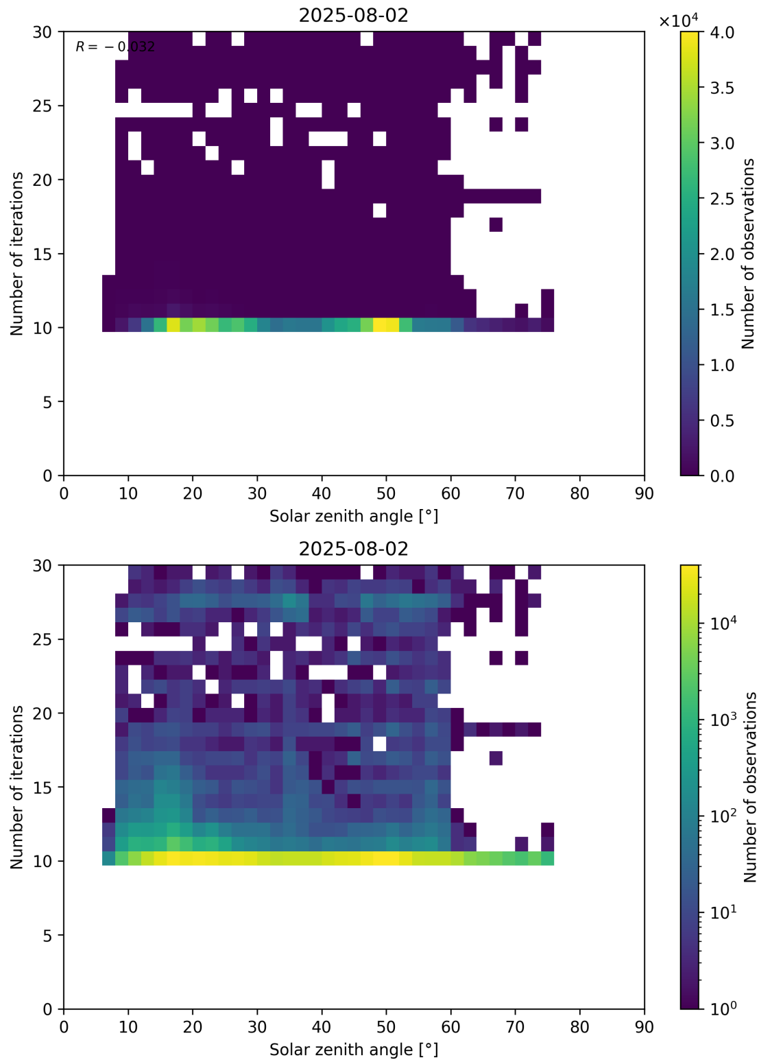
Figure 102: Scatter density plot of “Solar zenith angle” against “Number of iterations” for 2025-08-01 to 2025-08-03.
