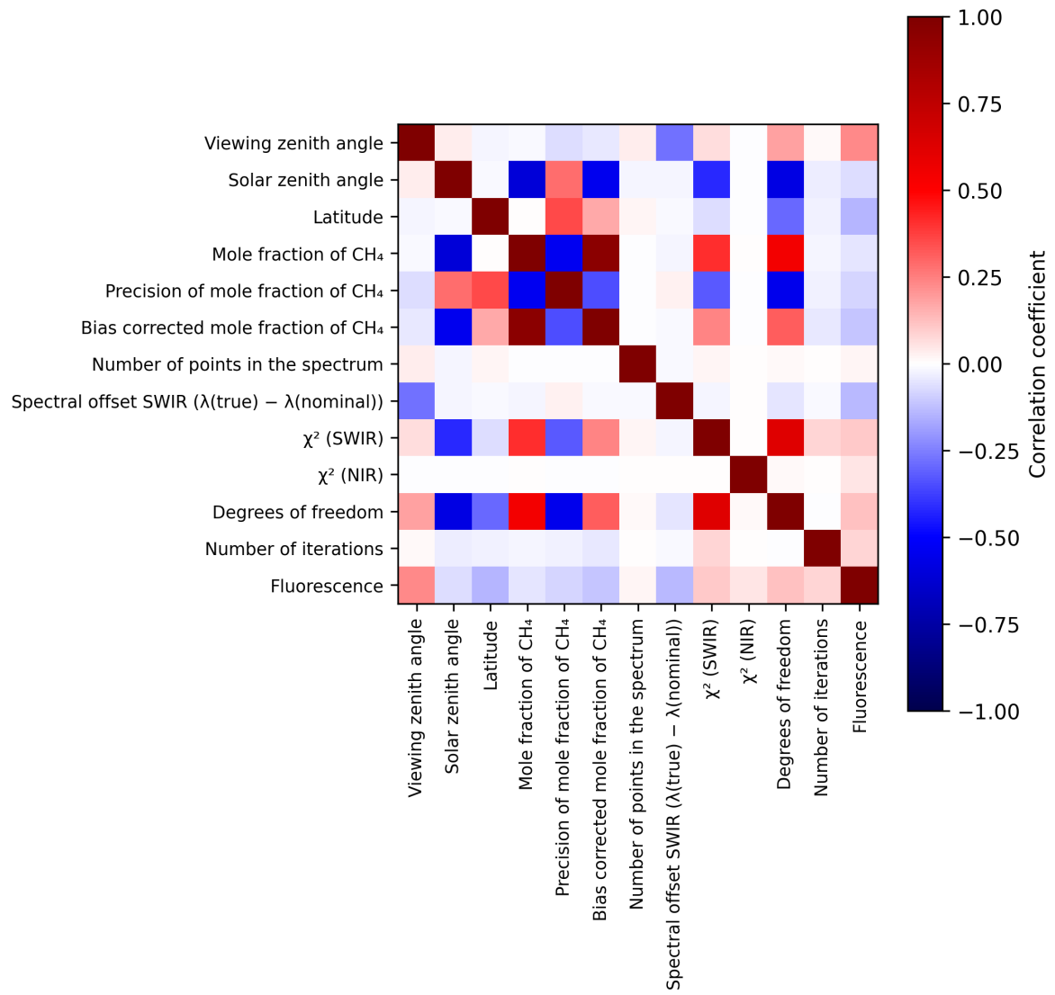
Figure 2: Map of correlation matrix for 2025-08-01 to 2025-08-03.
