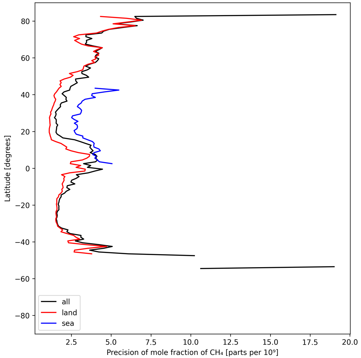
Figure 13: Zonal average of “Precision of mole fraction of CH 4 ” for 2025-08-01 to 2025-08-03.
