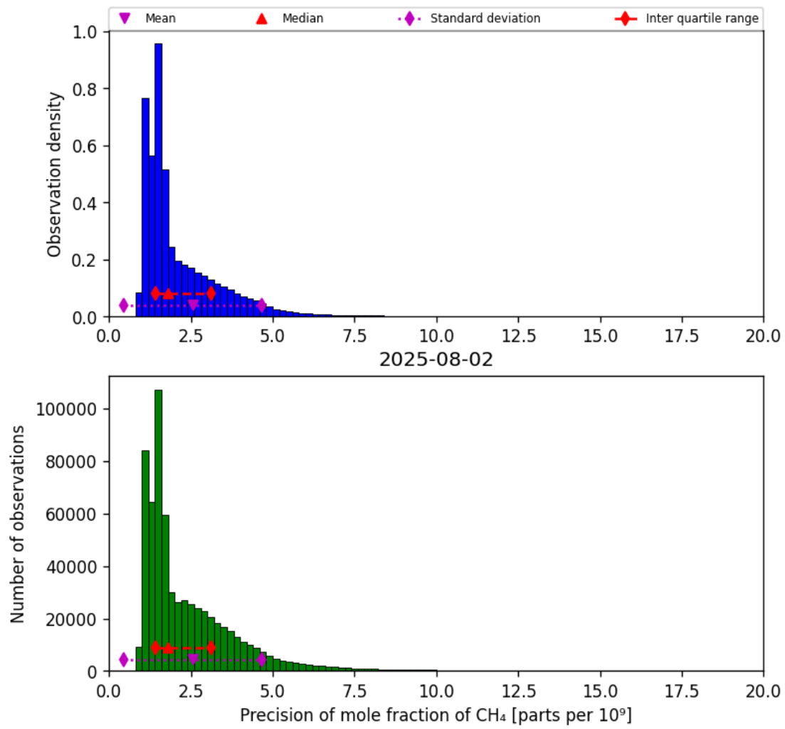
Figure 24: Histogram of “Precision of mole fraction of CH 4 ” for 2025-08-01 to 2025-08-03
