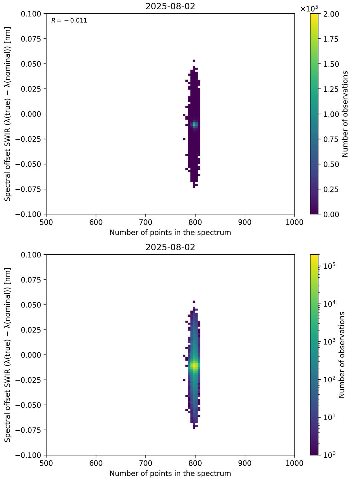
Figure 93: Scatter density plot of “Number of points in the spectrum” against “Spectral offset SWIR ( \lambda_{\text{true}} - \lambda_{\text{nominal}} )” for 2025-08-01 to 2025-08-03.
