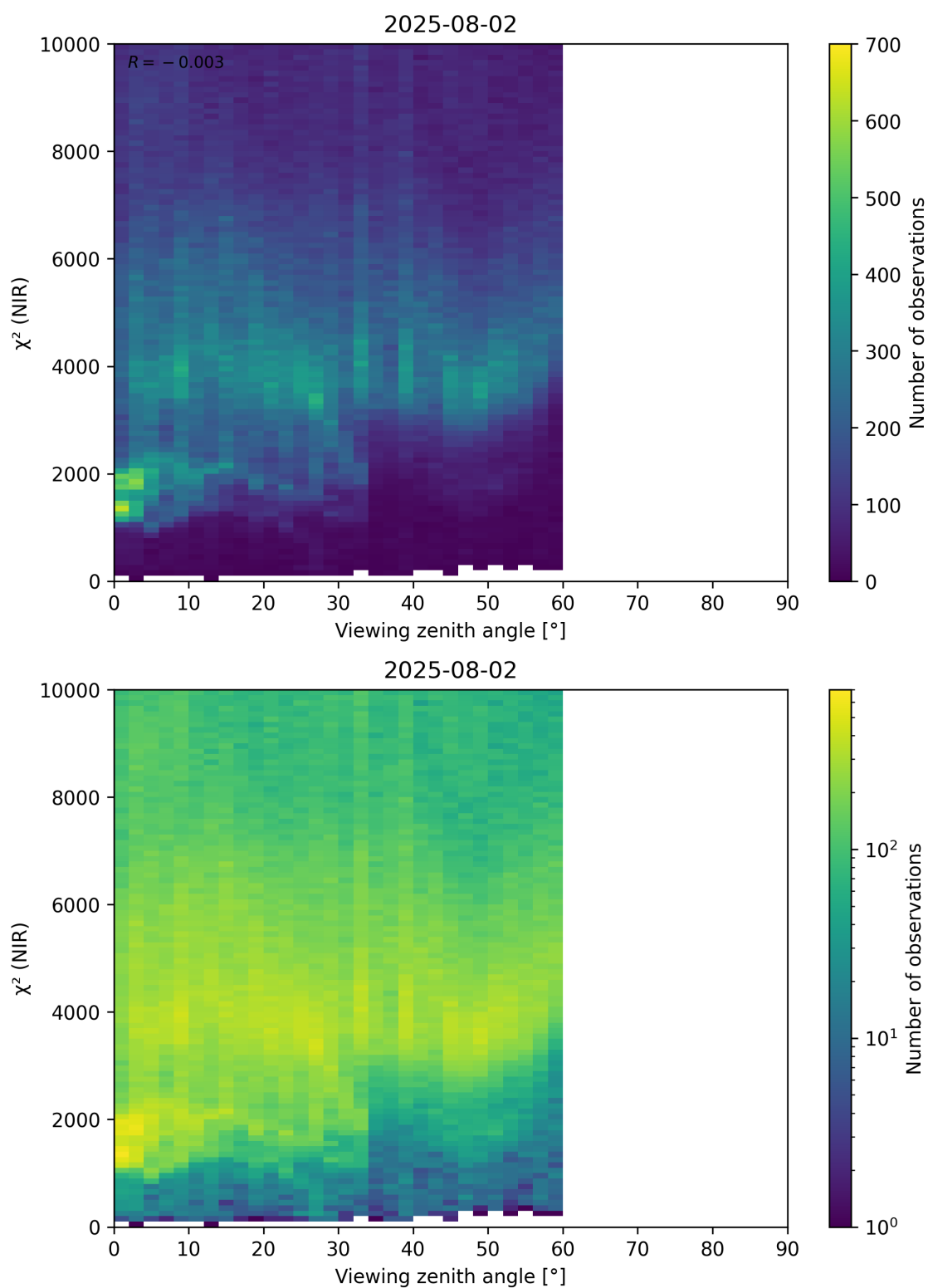
Figure 105: Scatter density plot of “Viewing zenith angle” against “ \chi^2 (NIR)” for 2025-08-01 to 2025-08-03.
