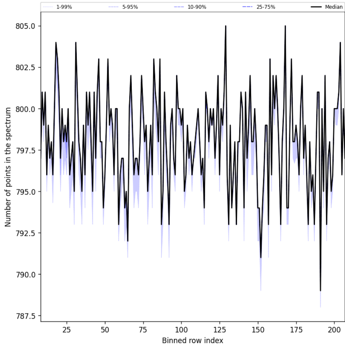
Figure 37: Along track statistics of “Number of points in the spectrum” for 2025-08-01 to 2025-08-03
