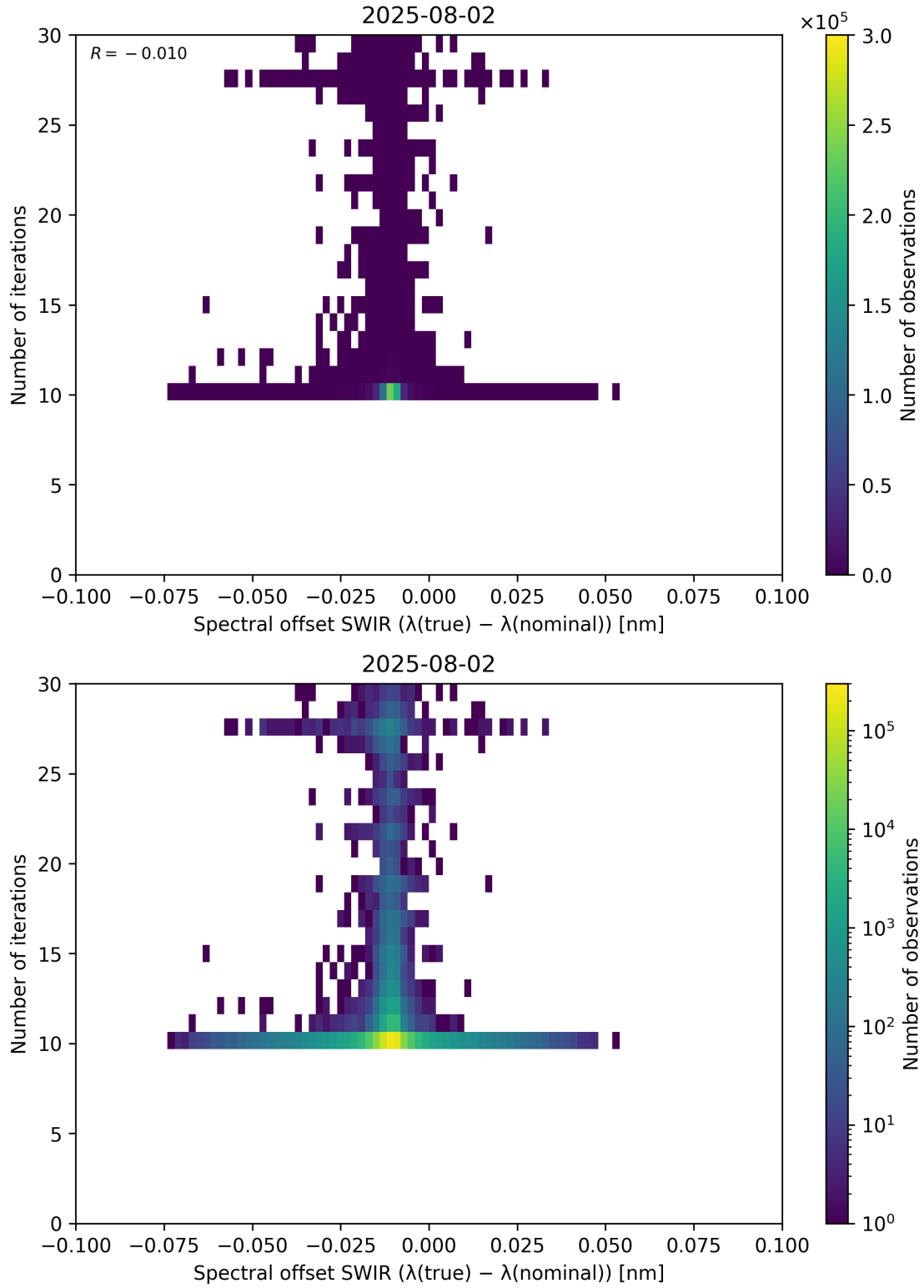
Figure 121: Scatter density plot of “Spectral offset SWIR ( \lambda_{\text{true}} - \lambda_{\text{nominal}} )” against “Number of iterations” for 2025-08-01 to 2025-08-03.
