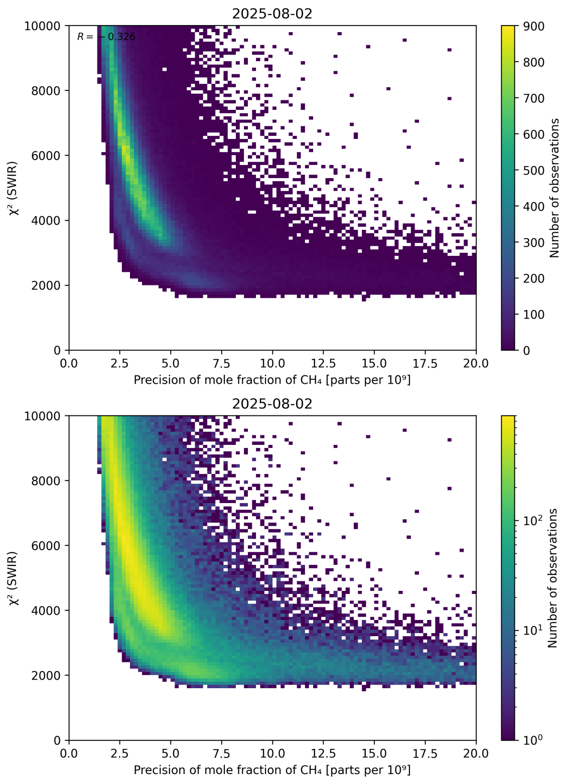
Figure 79: Scatter density plot of “Precision of mole fraction of \text{CH}_4 ” against “ \chi^2 (SWIR)” for 2025-08-01 to 2025-08-03.
