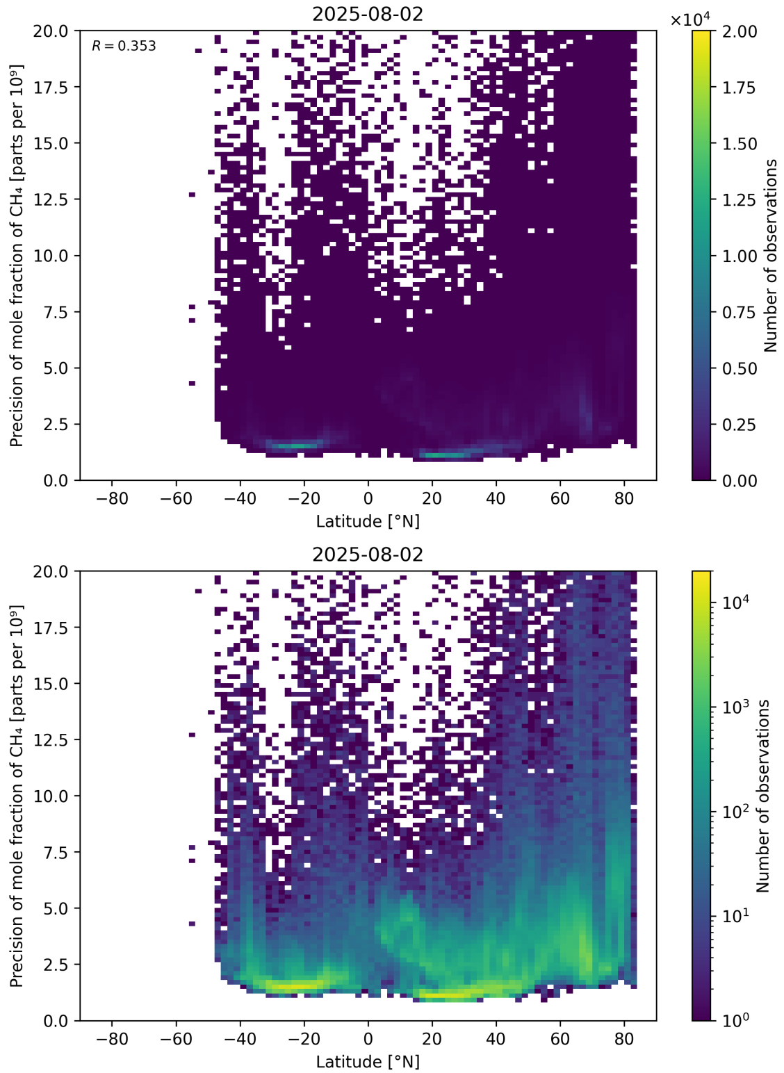
Figure 59: Scatter density plot of “Latitude” against “Precision of mole fraction of CH 4 ” for 2025-08-01 to 2025-08-03.
