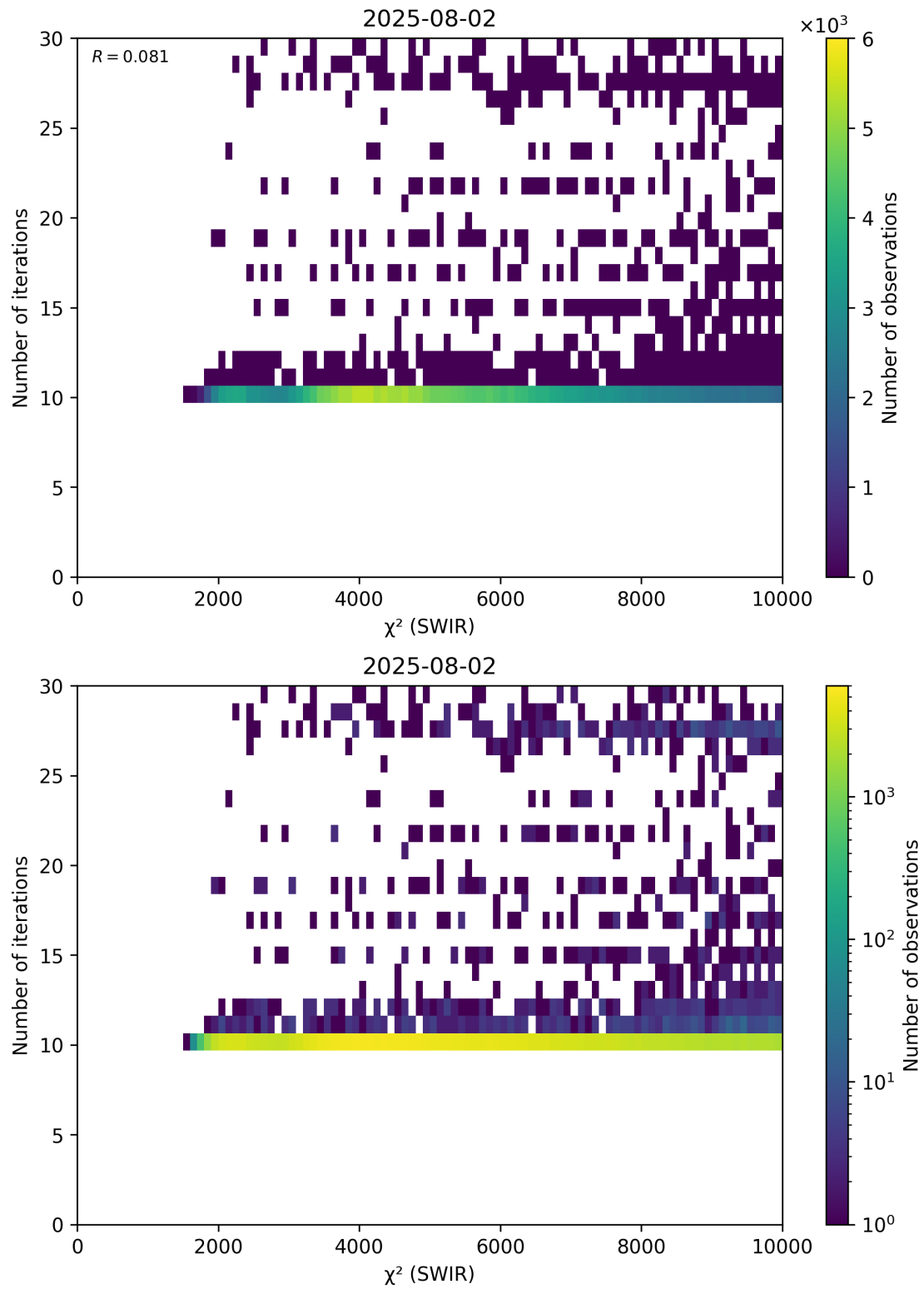
Figure 50: Scatter density plot of “ \chi^2 (SWIR)” against “Number of iterations” for 2025-08-01 to 2025-08-03.
