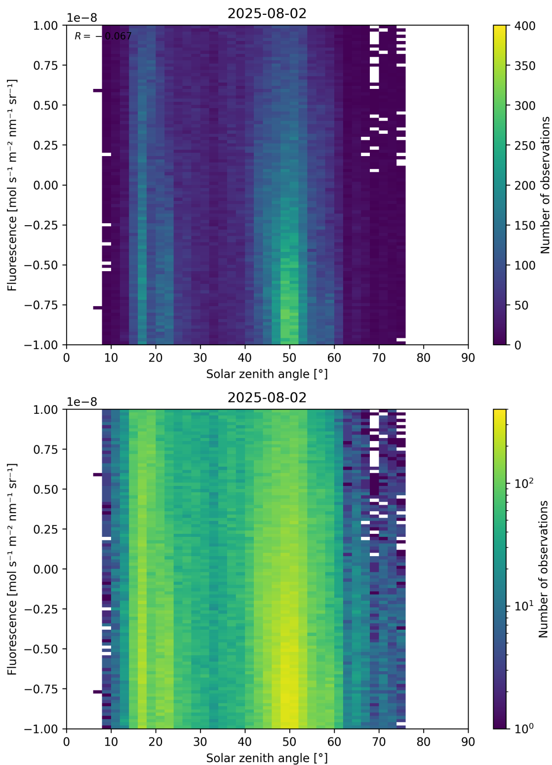
Figure 97: Scatter density plot of “Solar zenith angle” against “Fluorescence” for 2025-08-01 to 2025-08-03.
