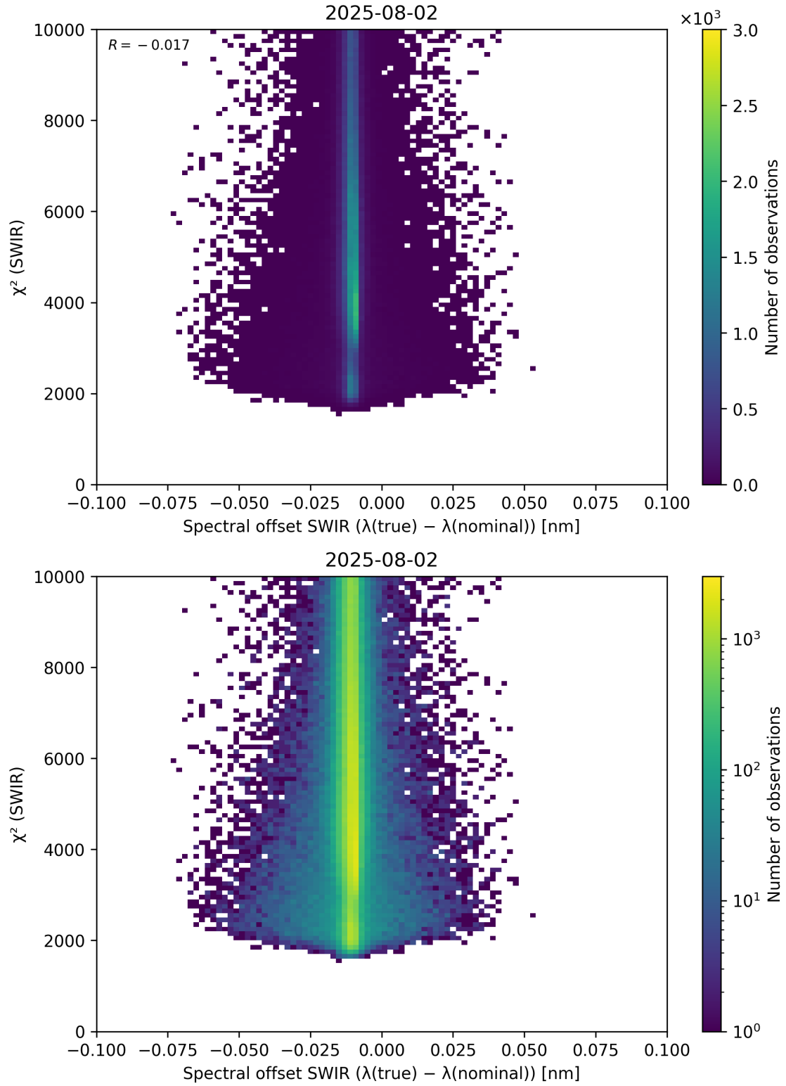
Figure 118: Scatter density plot of “Spectral offset SWIR ( \lambda_{\text{true}} - \lambda_{\text{nominal}} )” against “ \chi^2 (SWIR)” for 2025-08-01 to 2025-08-03.
