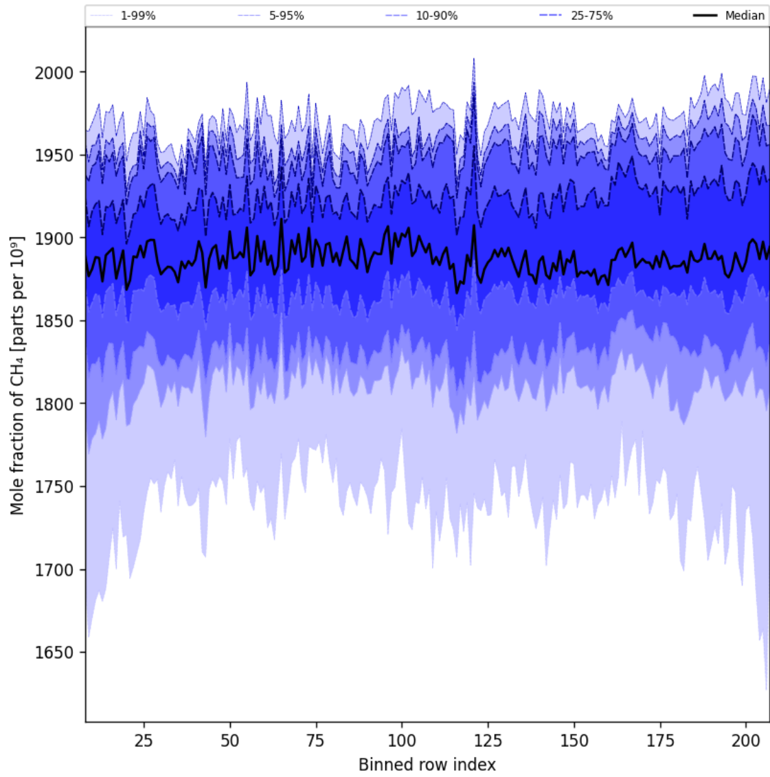
Figure 34: Along track statistics of “Mole fraction of CH 4 ” for 2025-08-01 to 2025-08-03
