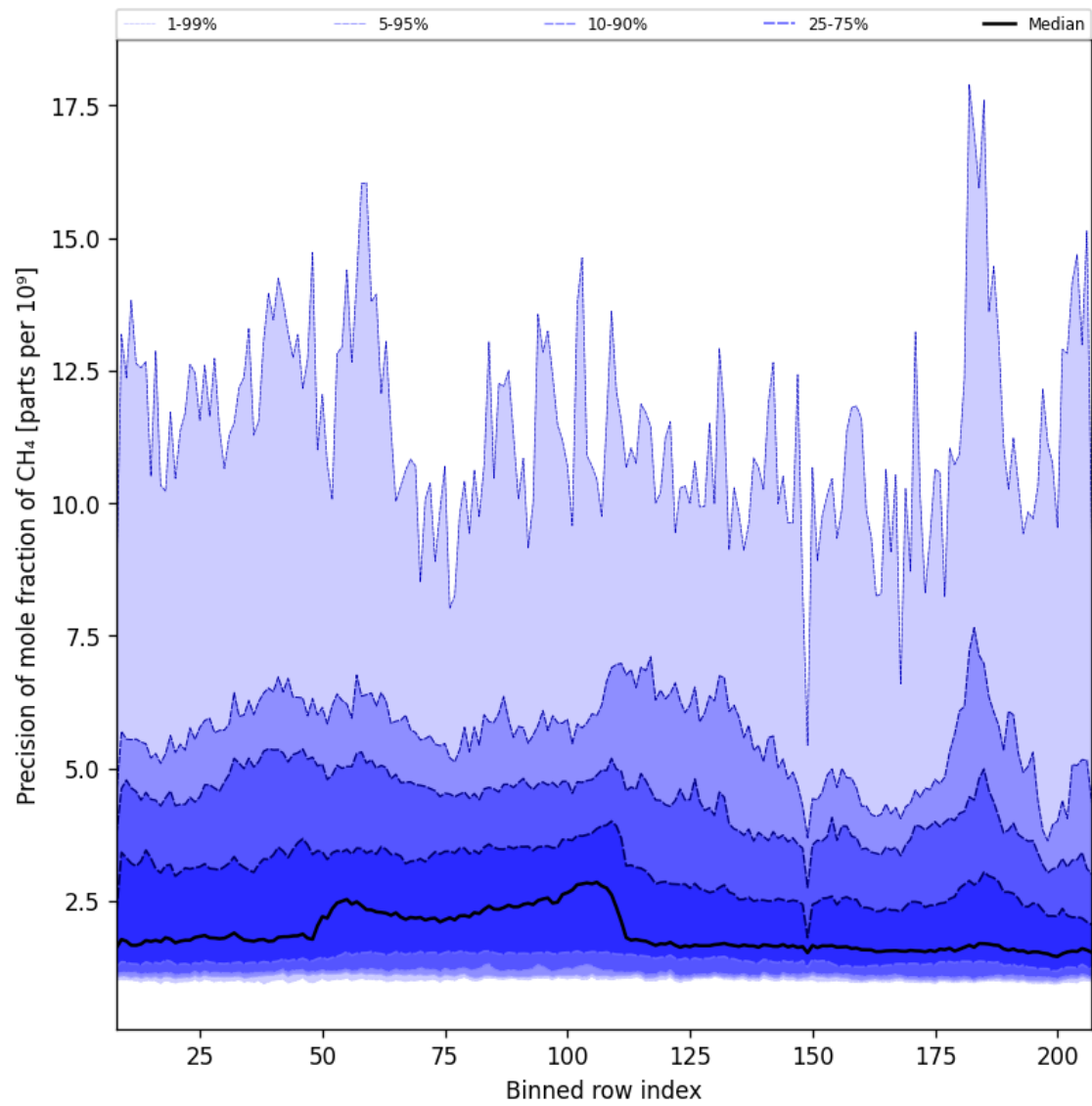
Figure 35: Along track statistics of “Precision of mole fraction of CH 4 ” for 2025-08-01 to 2025-08-03
