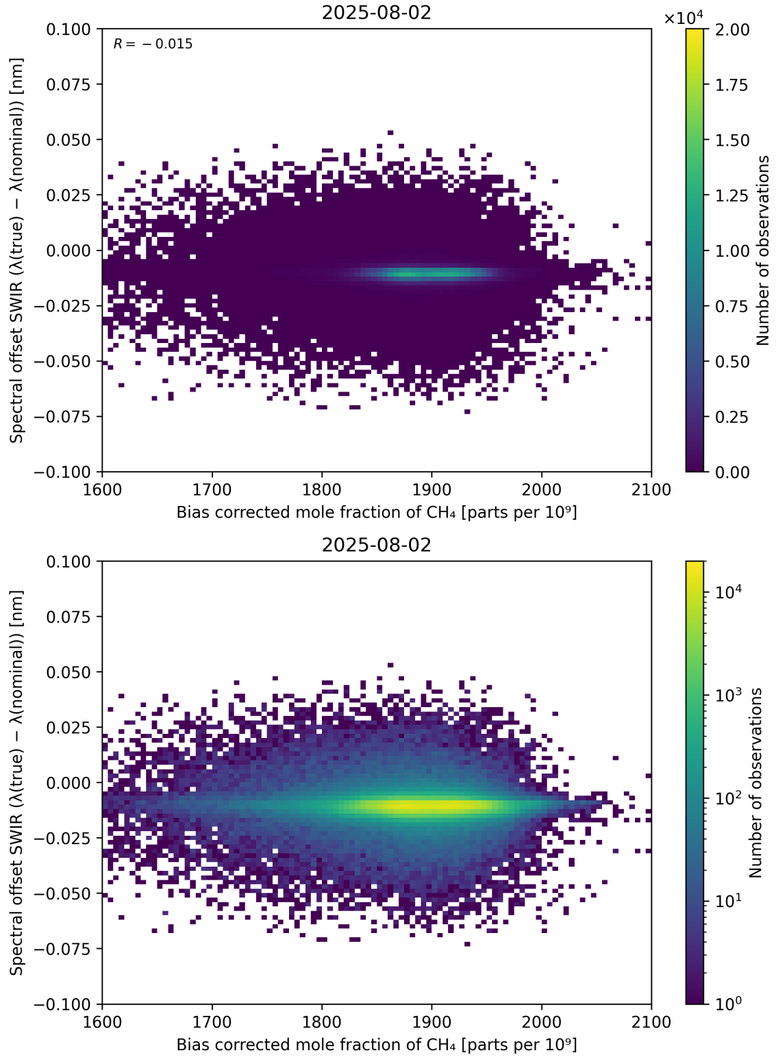
Figure 69: Scatter density plot of “Bias corrected mole fraction of \text{CH}_4 ” against “Spectral offset SWIR ( \lambda_{\text{true}} - \lambda_{\text{nominal}} )” for 2025-08-01 to 2025-08-03.
