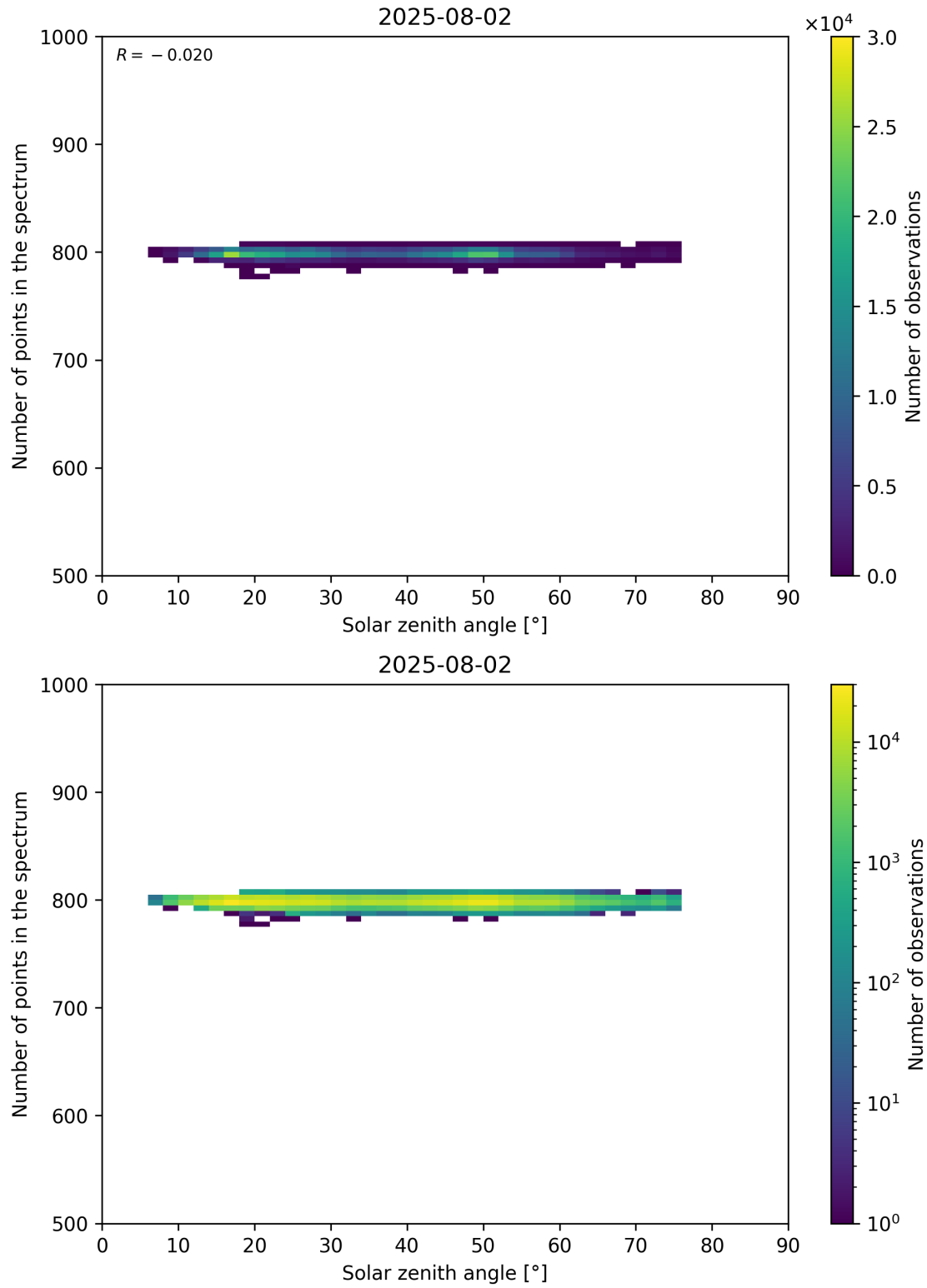
Figure 103: Scatter density plot of “Solar zenith angle” against “Number of points in the spectrum” for 2025-08-01 to 2025-08-03.
