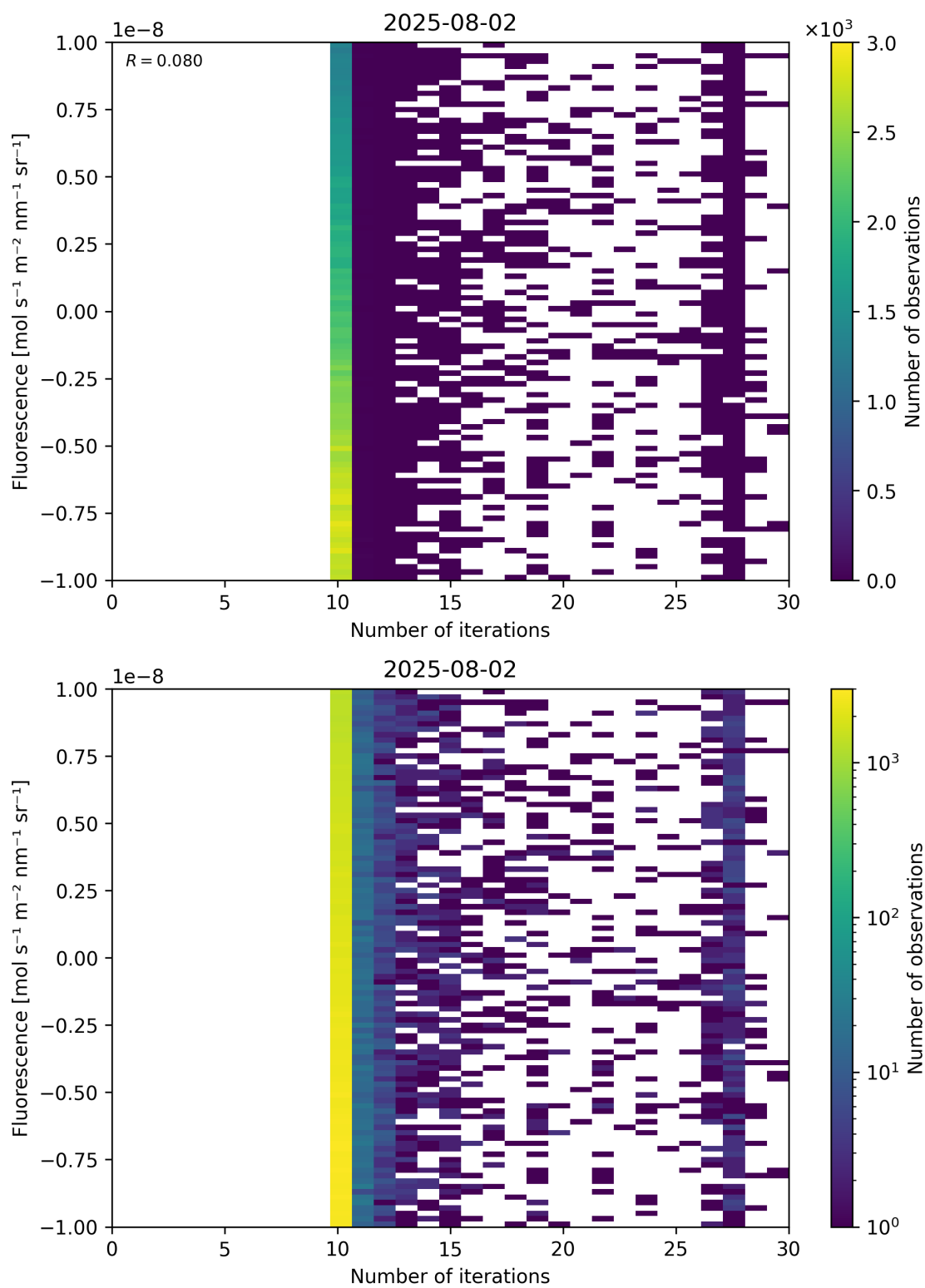
Figure 87: Scatter density plot of “Number of iterations” against “Fluorescence” for 2025-08-01 to 2025-08-03.
