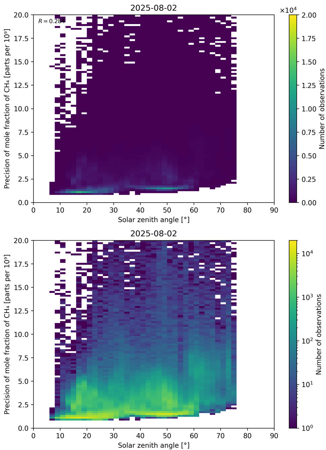
Figure 101: Scatter density plot of “Solar zenith angle” against “Precision of mole fraction of CH 4 ” for 2025-08-01 to 2025-08-03.
