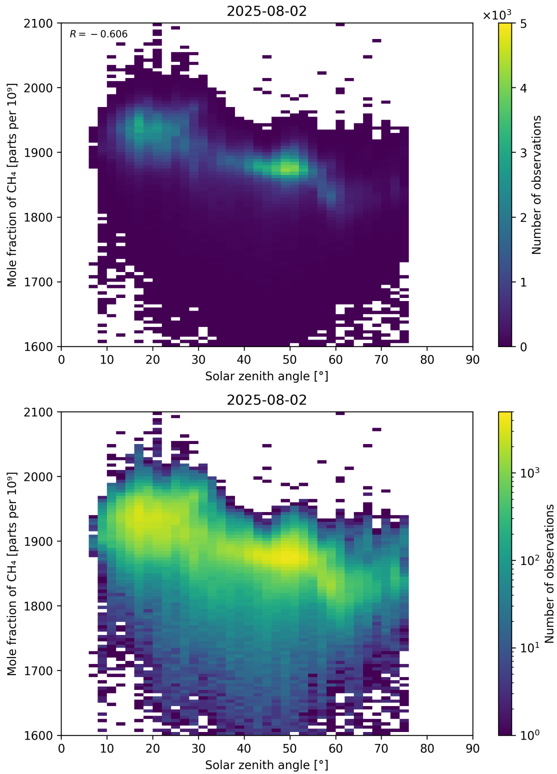
Figure 99: Scatter density plot of “Solar zenith angle” against “Mole fraction of CH 4 ” for 2025-08-01 to 2025-08-03.
