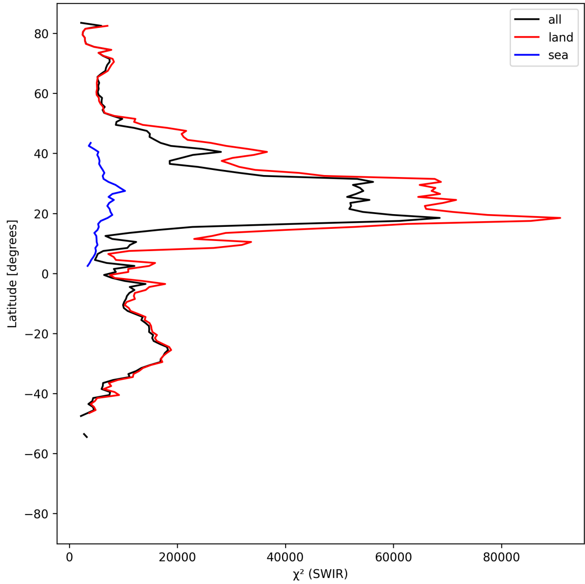
Figure 17: Zonal average of “ \chi^2 (SWIR)” for 2025-08-01 to 2025-08-03.
