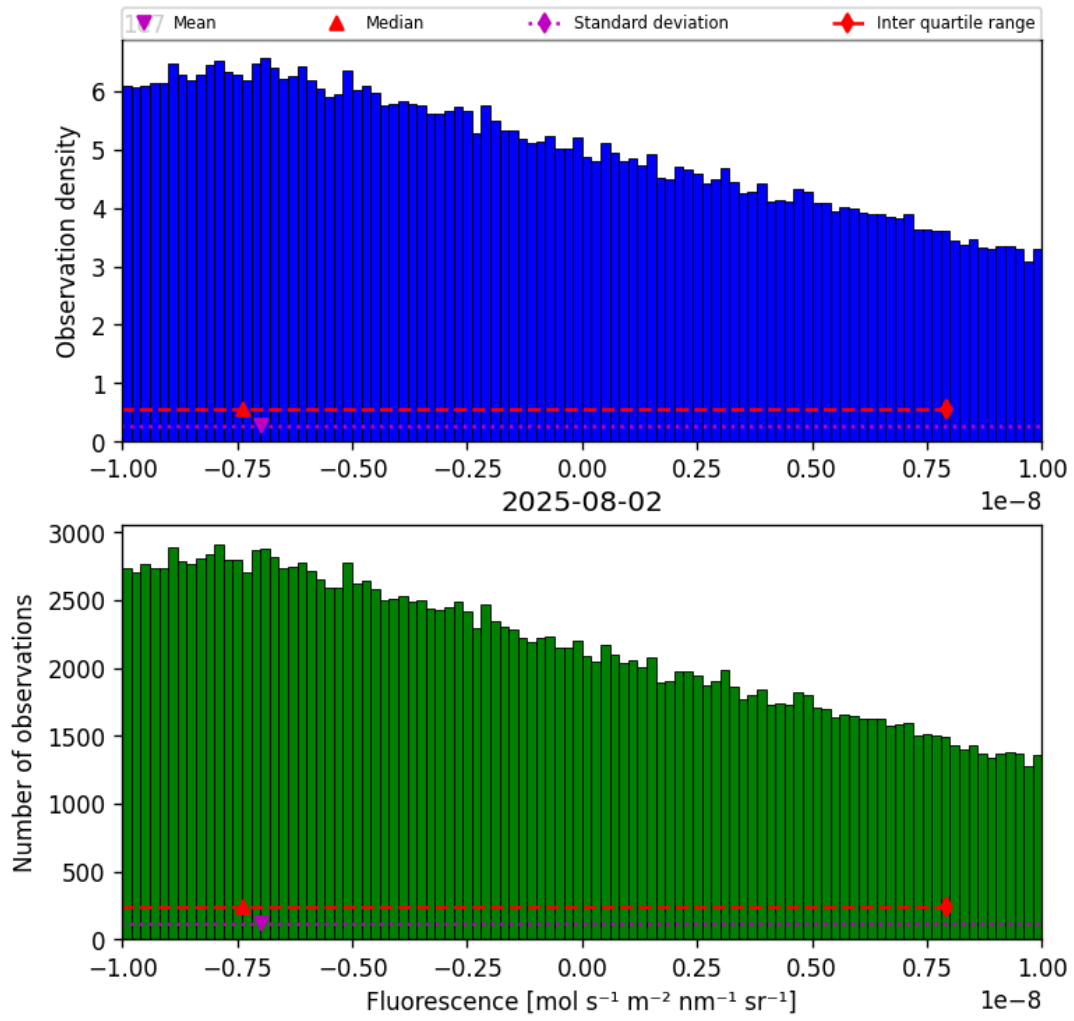
Figure 32: Histogram of “Fluorescence” for 2025-08-01 to 2025-08-03
