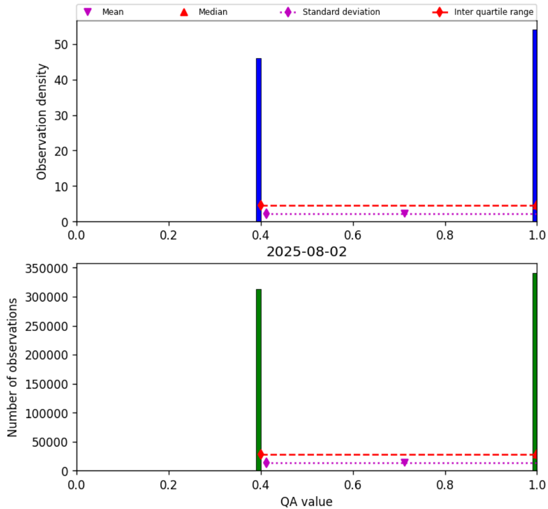
Figure 22: Histogram of “QA value” for 2025-08-01 to 2025-08-03
