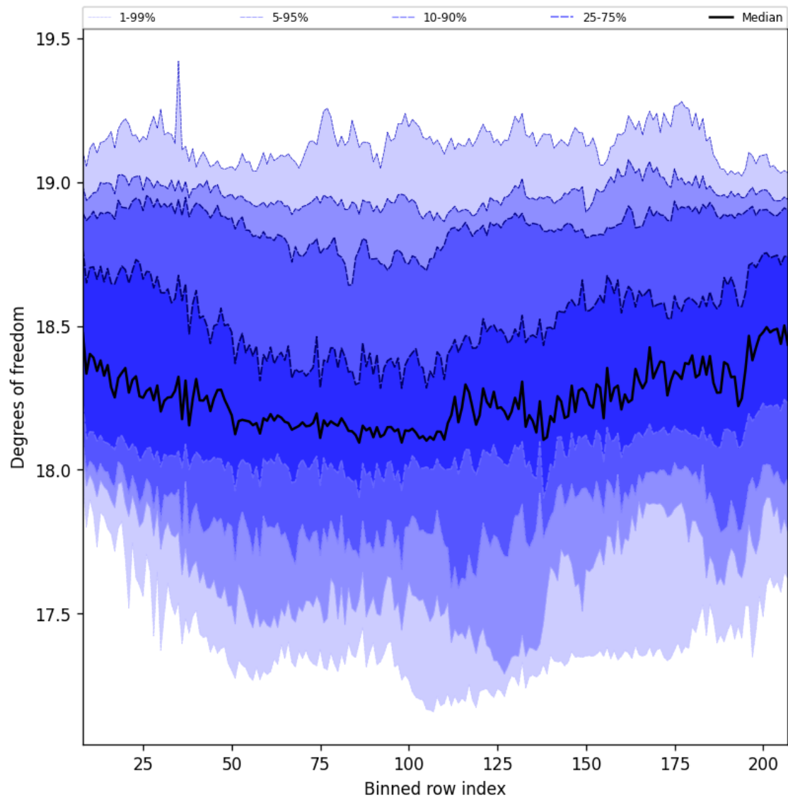
Figure 41: Along track statistics of “Degrees of freedom” for 2025-08-01 to 2025-08-03
