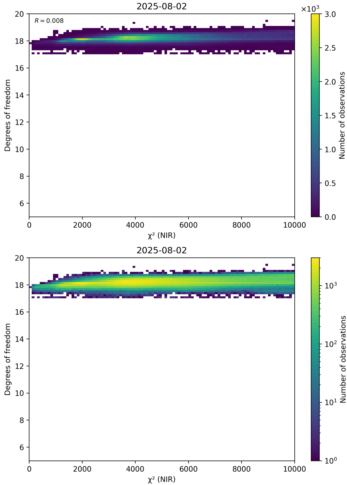
Figure 44: Scatter density plot of “ \chi^2 (NIR)” against “Degrees of freedom” for 2025-08-01 to 2025-08-03.
