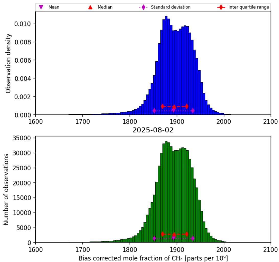
Figure 25: Histogram of “Bias corrected mole fraction of CH 4 ” for 2025-08-01 to 2025-08-03
