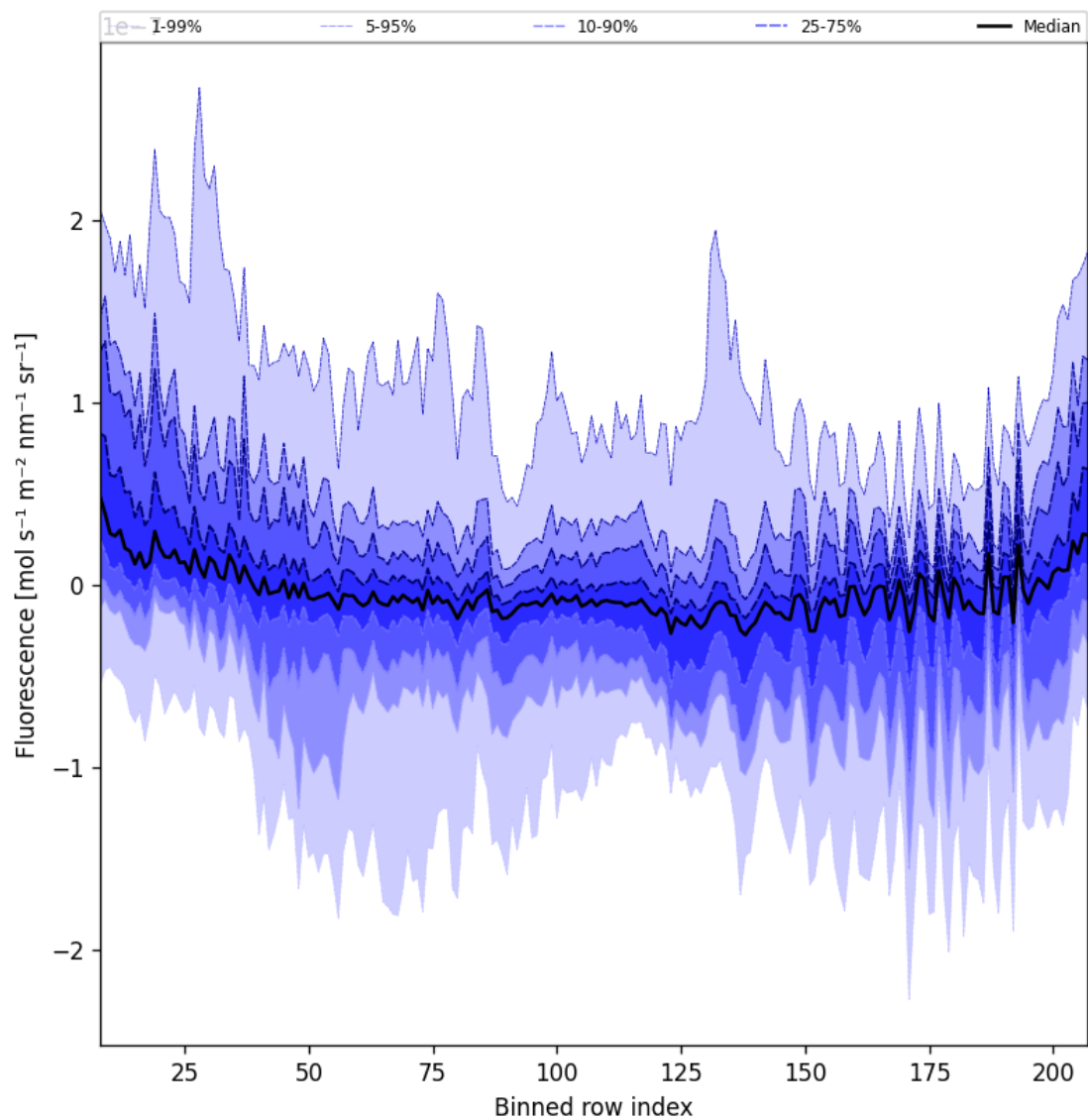
Figure 43: Along track statistics of “Fluorescence” for 2025-08-01 to 2025-08-03
