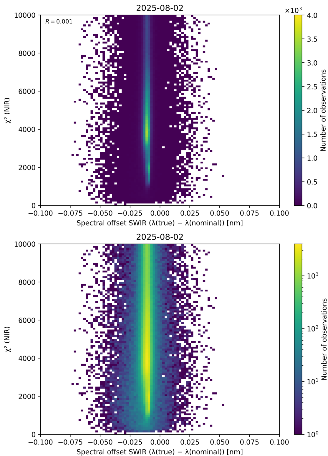
Figure 117: Scatter density plot of “Spectral offset SWIR ( \lambda_{\text{true}} - \lambda_{\text{nominal}} )” against “ \chi^2 (NIR)” for 2025-08-01 to 2025-08-03.
