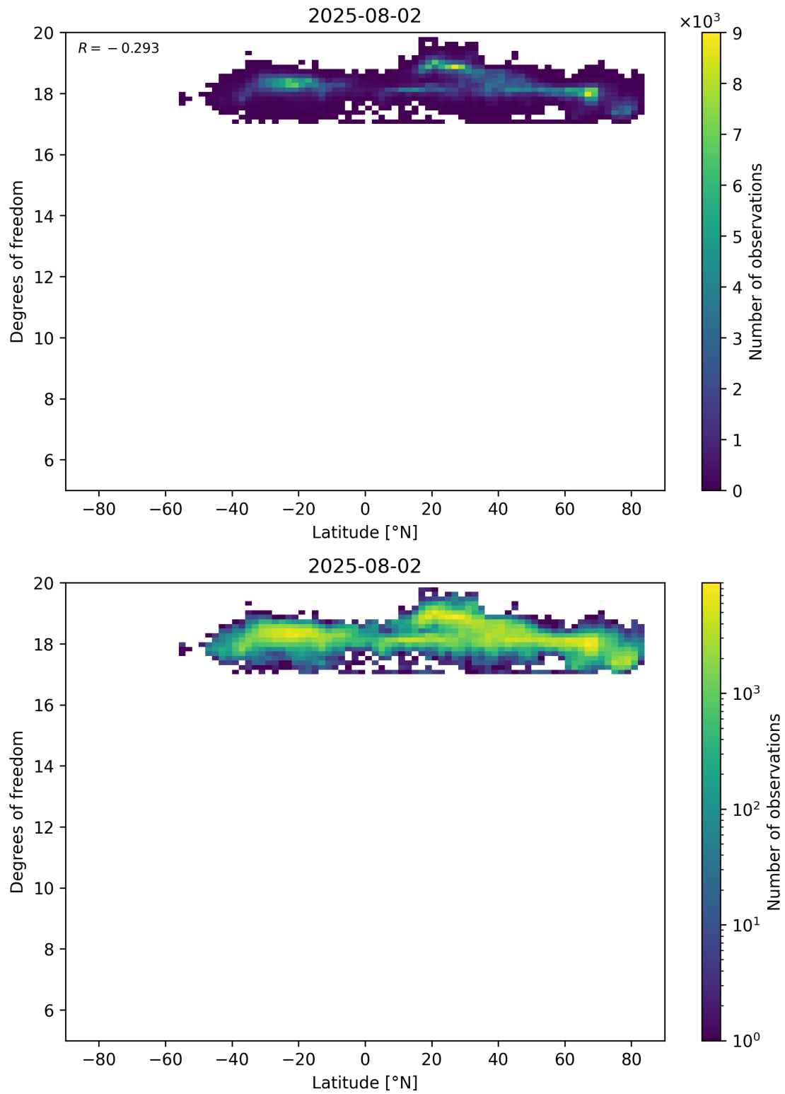
Figure 55: Scatter density plot of “Latitude” against “Degrees of freedom” for 2025-08-01 to 2025-08-03.
