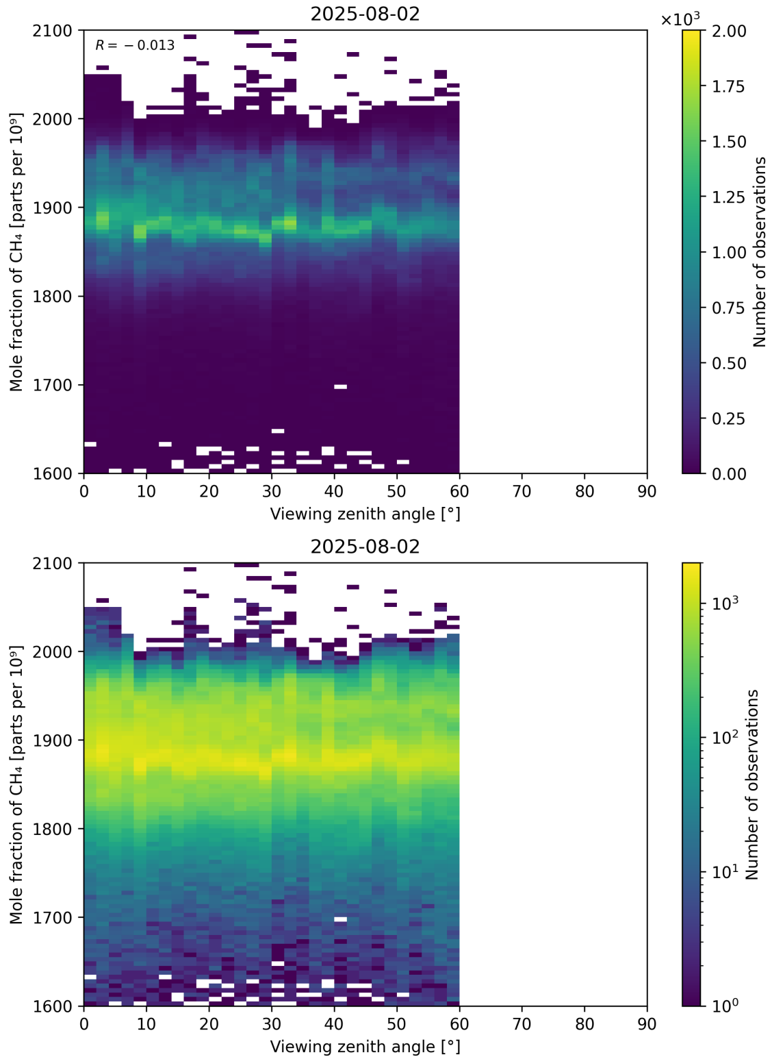
Figure 110: Scatter density plot of “Viewing zenith angle” against “Mole fraction of CH 4 ” for 2025-08-01 to 2025-08-03.
