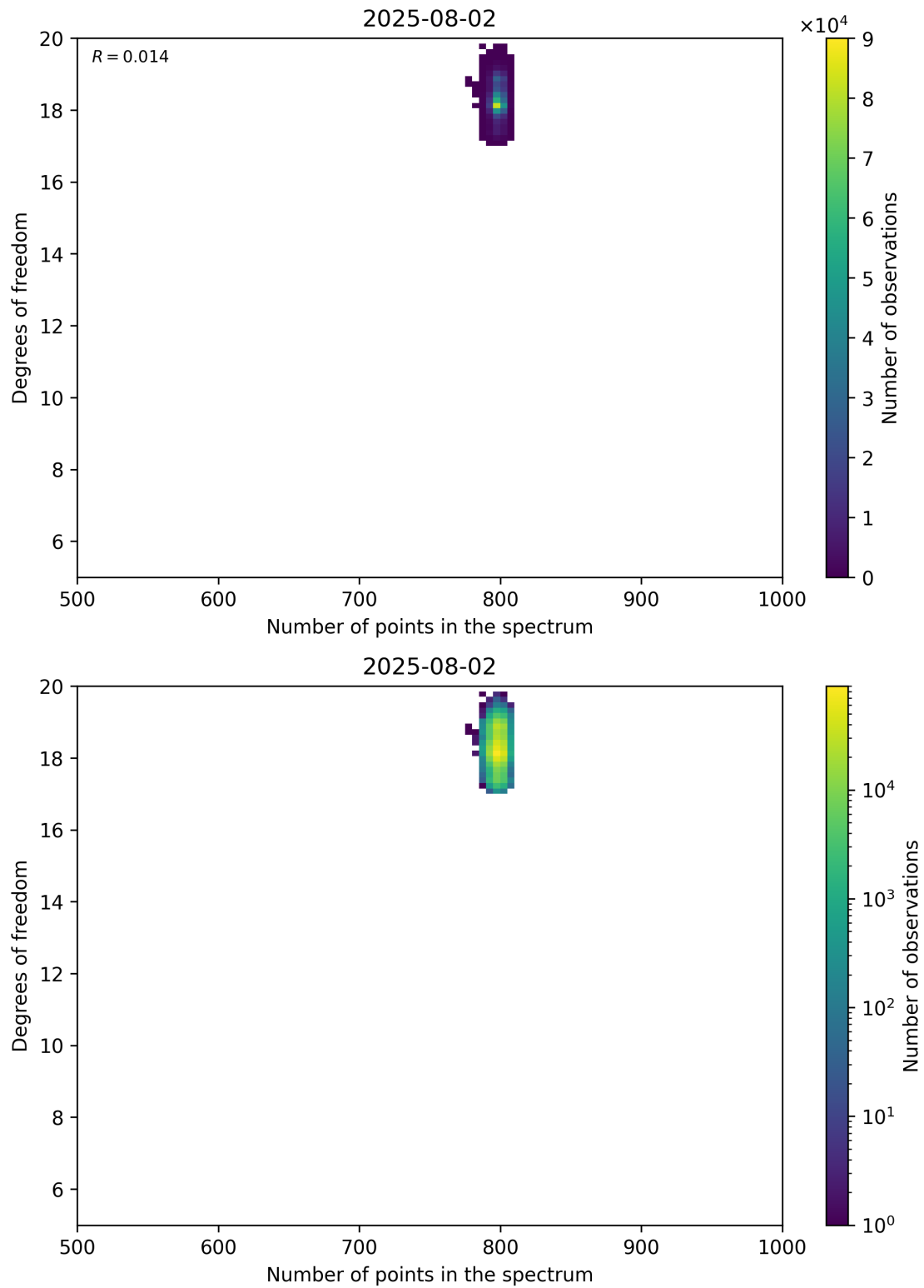
Figure 90: Scatter density plot of “Number of points in the spectrum” against “Degrees of freedom” for 2025-08-01 to 2025-08-03.
