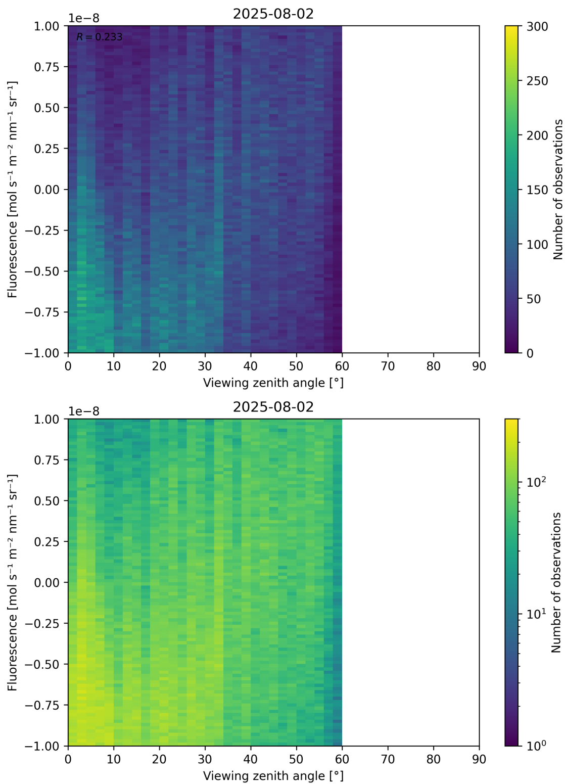
Figure 108: Scatter density plot of “Viewing zenith angle” against “Fluorescence” for 2025-08-01 to 2025-08-03.
