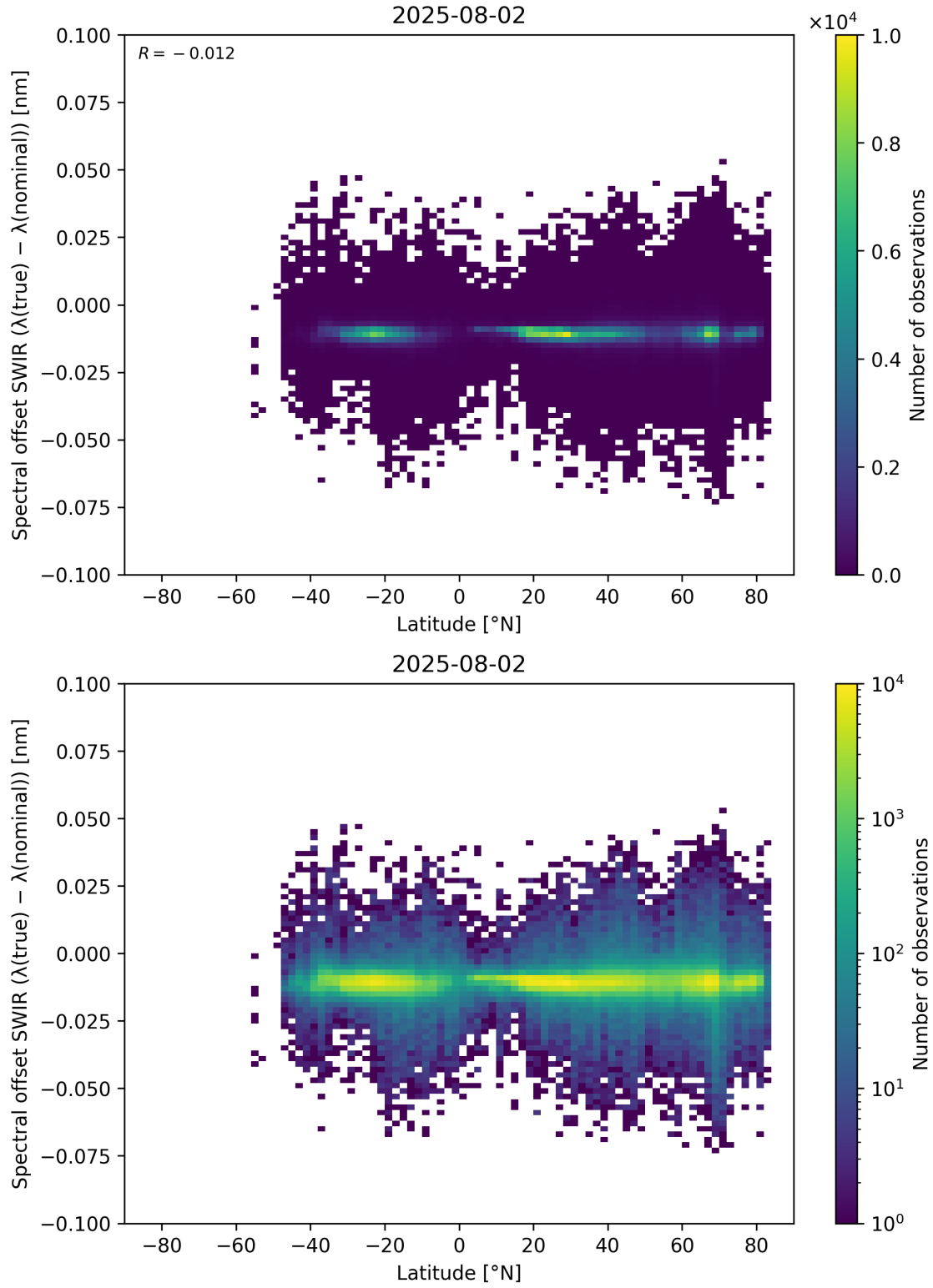
Figure 62: Scatter density plot of “Latitude” against “Spectral offset SWIR ( \lambda_{\text{true}} - \lambda_{\text{nominal}} )” for 2025-08-01 to 2025-08-03.
