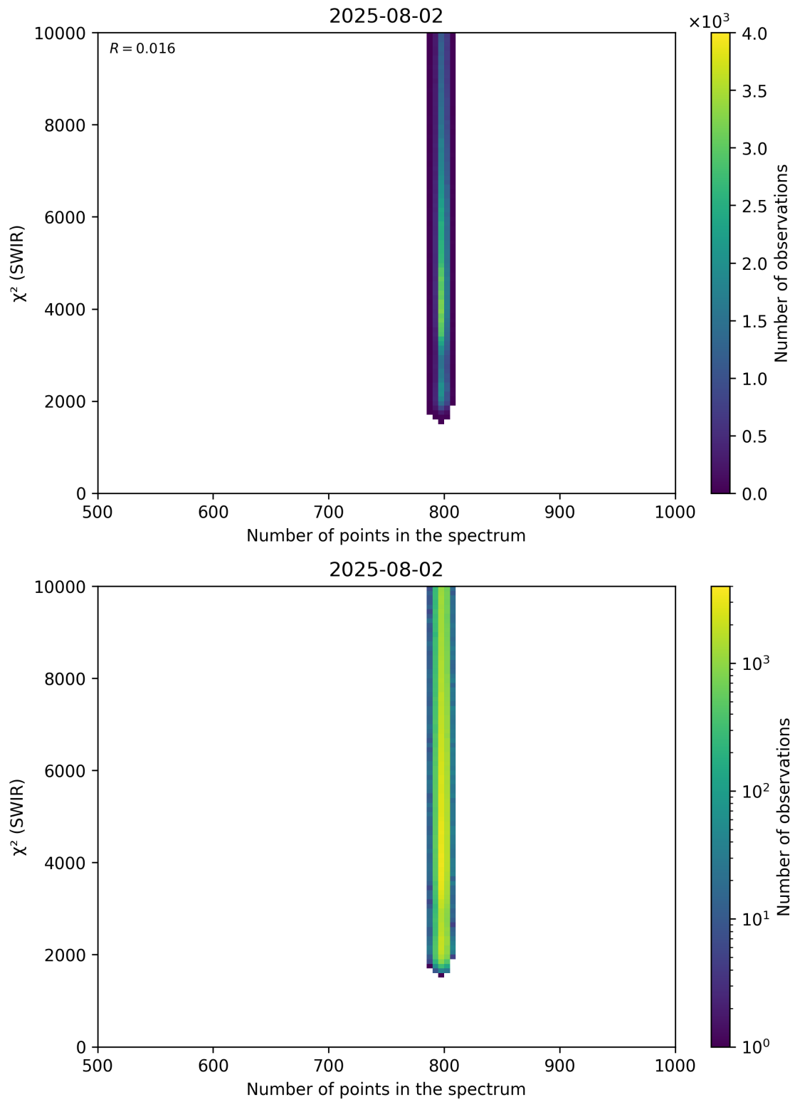
Figure 89: Scatter density plot of “Number of points in the spectrum” against “ \chi^2 (SWIR)” for 2025-08-01 to 2025-08-03.
