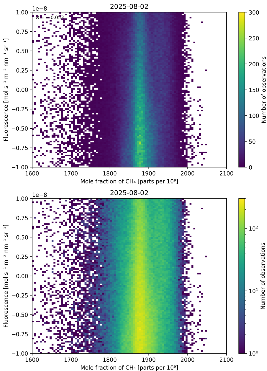
Figure 73: Scatter density plot of “Mole fraction of \text{CH}_4 ” against “Fluorescence” for 2025-08-01 to 2025-08-03.
