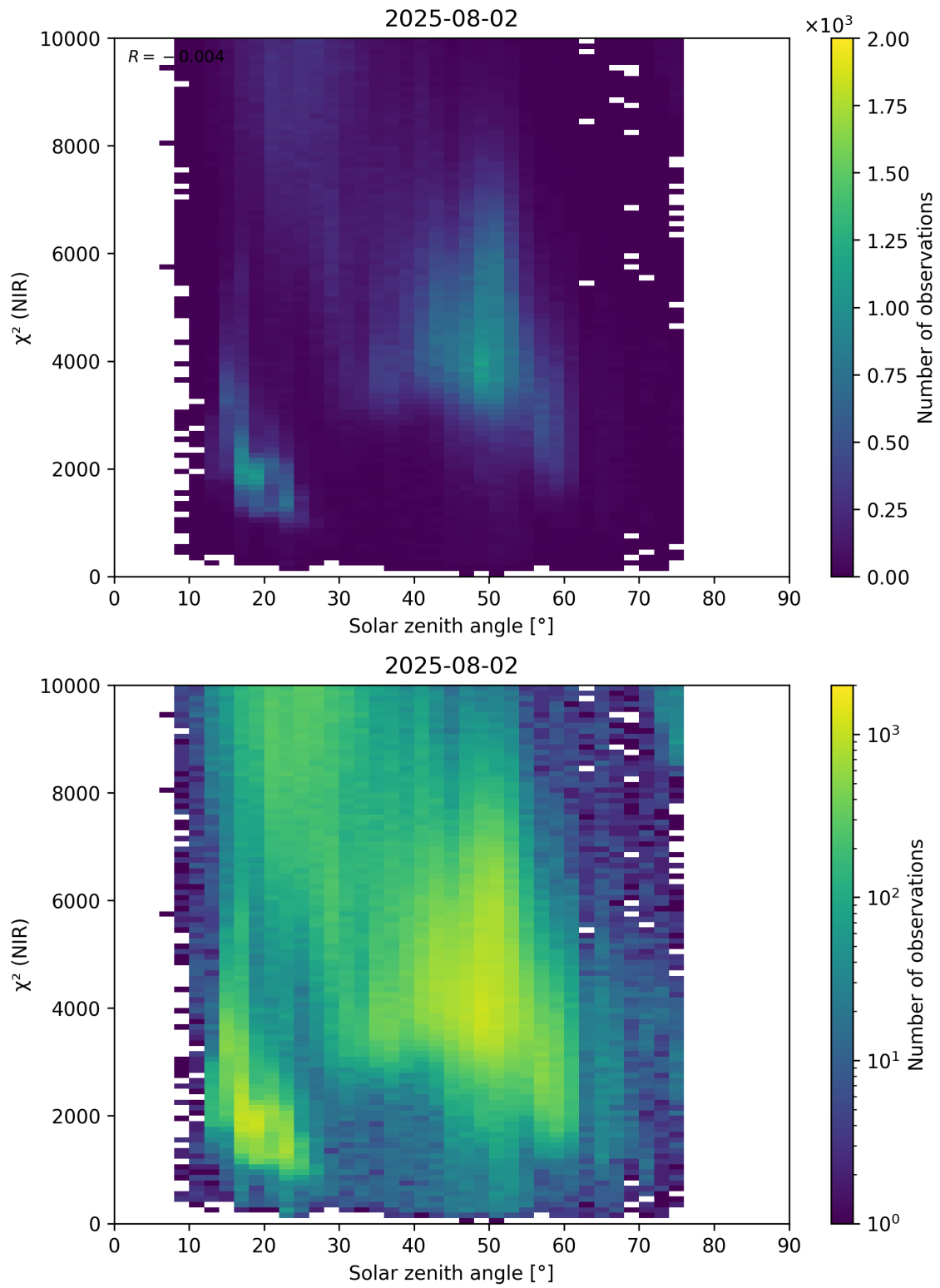
Figure 94: Scatter density plot of “Solar zenith angle” against “ \chi^2 (NIR)” for 2025-08-01 to 2025-08-03.
