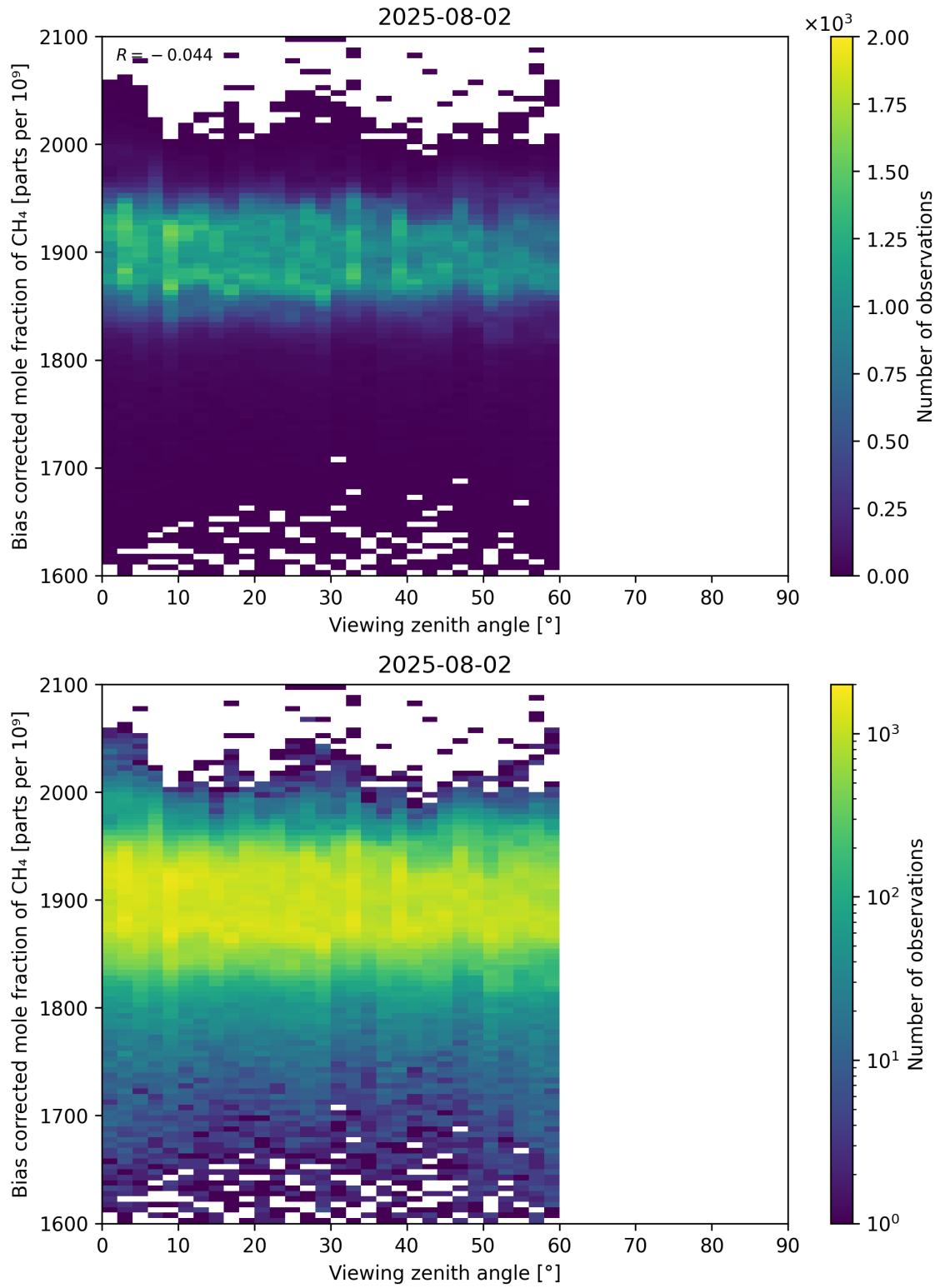
Figure 111: Scatter density plot of “Viewing zenith angle” against “Bias corrected mole fraction of CH 4 ” for 2025-08-01 to 2025-08-03.
