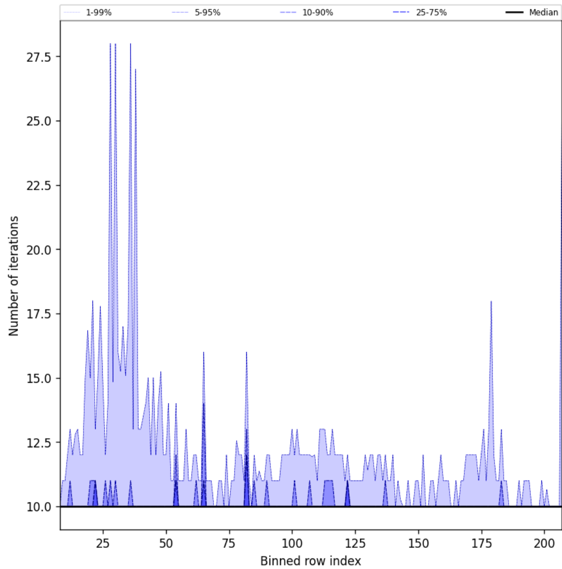
Figure 42: Along track statistics of “Number of iterations” for 2025-08-01 to 2025-08-03
