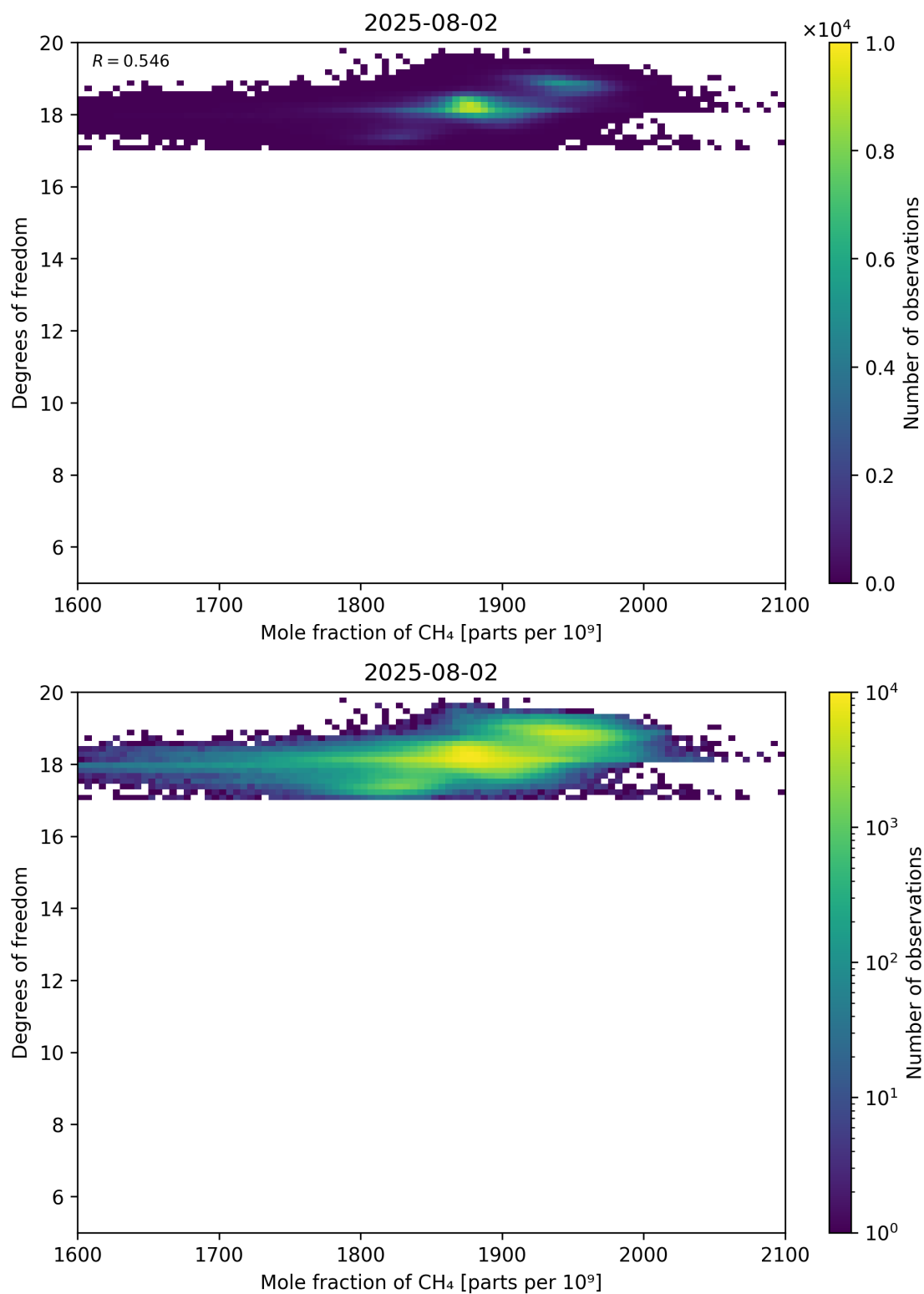
Figure 72: Scatter density plot of “Mole fraction of CH 4 ” against “Degrees of freedom” for 2025-08-01 to 2025-08-03.
