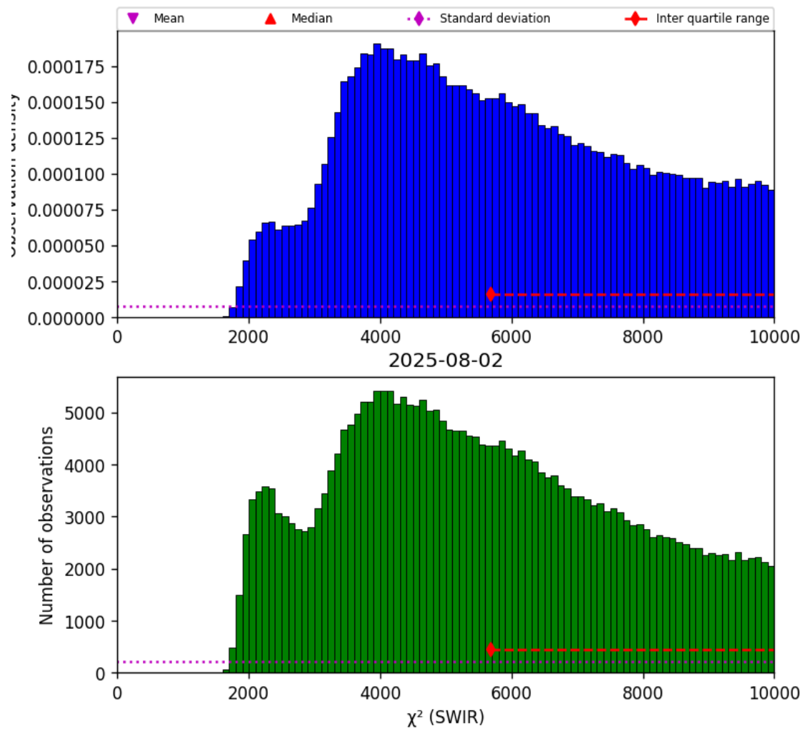
Figure 28: Histogram of “ \chi^2 (SWIR)” for 2025-08-01 to 2025-08-03
