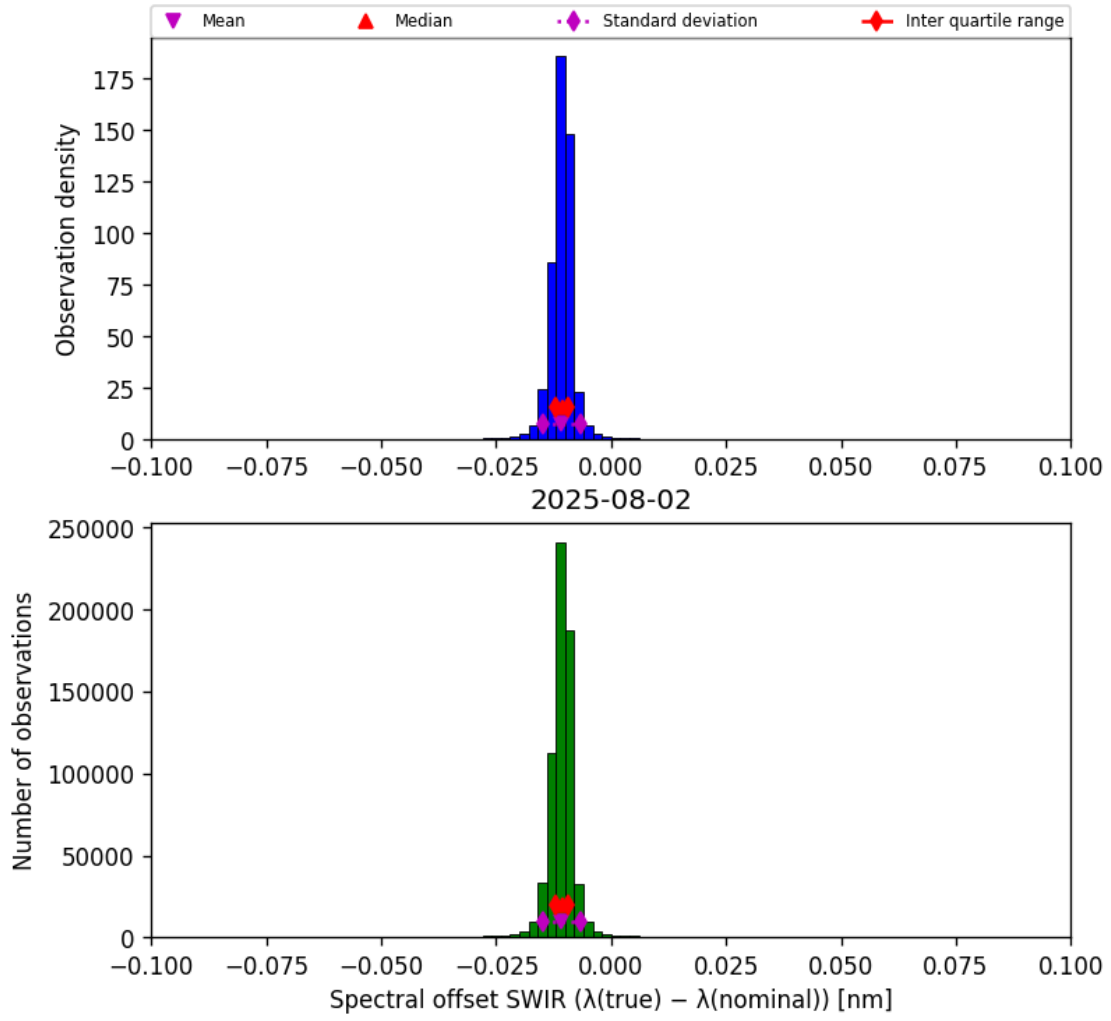
Figure 27: Histogram of “Spectral offset SWIR ( \lambda_{\text{true}} - \lambda_{\text{nominal}} )” for 2025-08-01 to 2025-08-03
