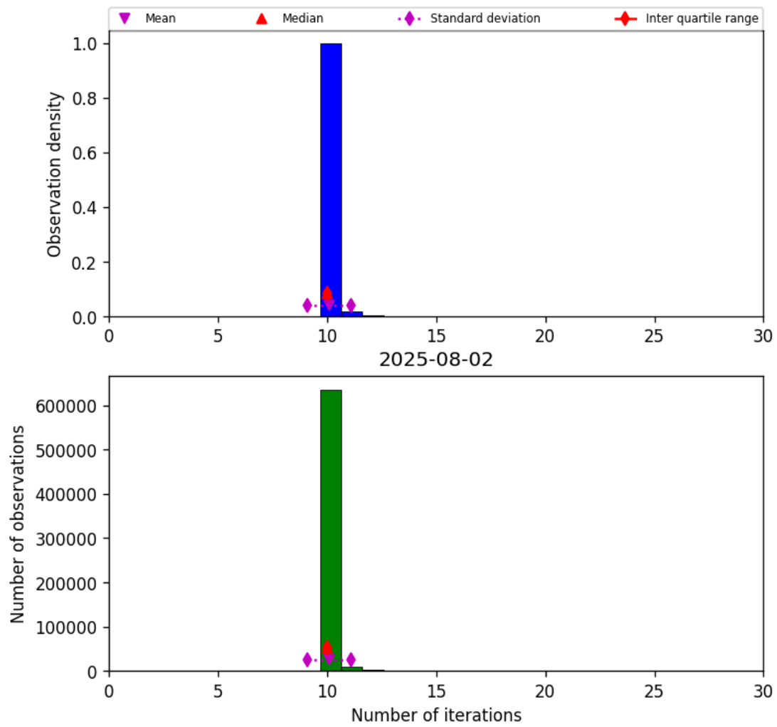
Figure 31: Histogram of “Number of iterations” for 2025-08-01 to 2025-08-03
