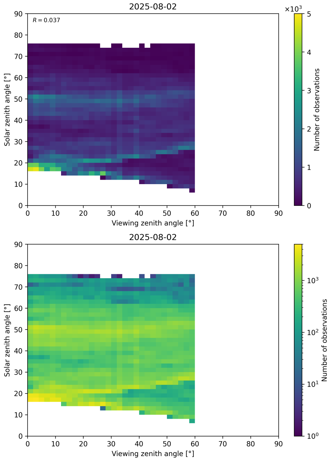
Figure 115: Scatter density plot of “Viewing zenith angle” against “Solar zenith angle” for 2025-08-01 to 2025-08-03.
