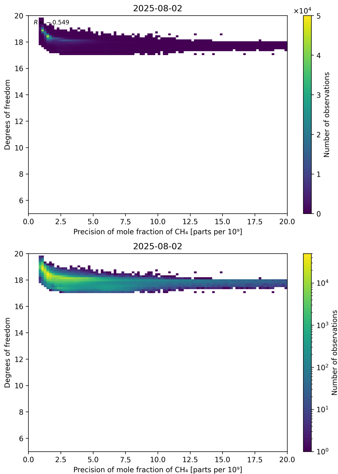
Figure 80: Scatter density plot of “Precision of mole fraction of CH 4 ” against “Degrees of freedom” for 2025-08-01 to 2025-08-03.
