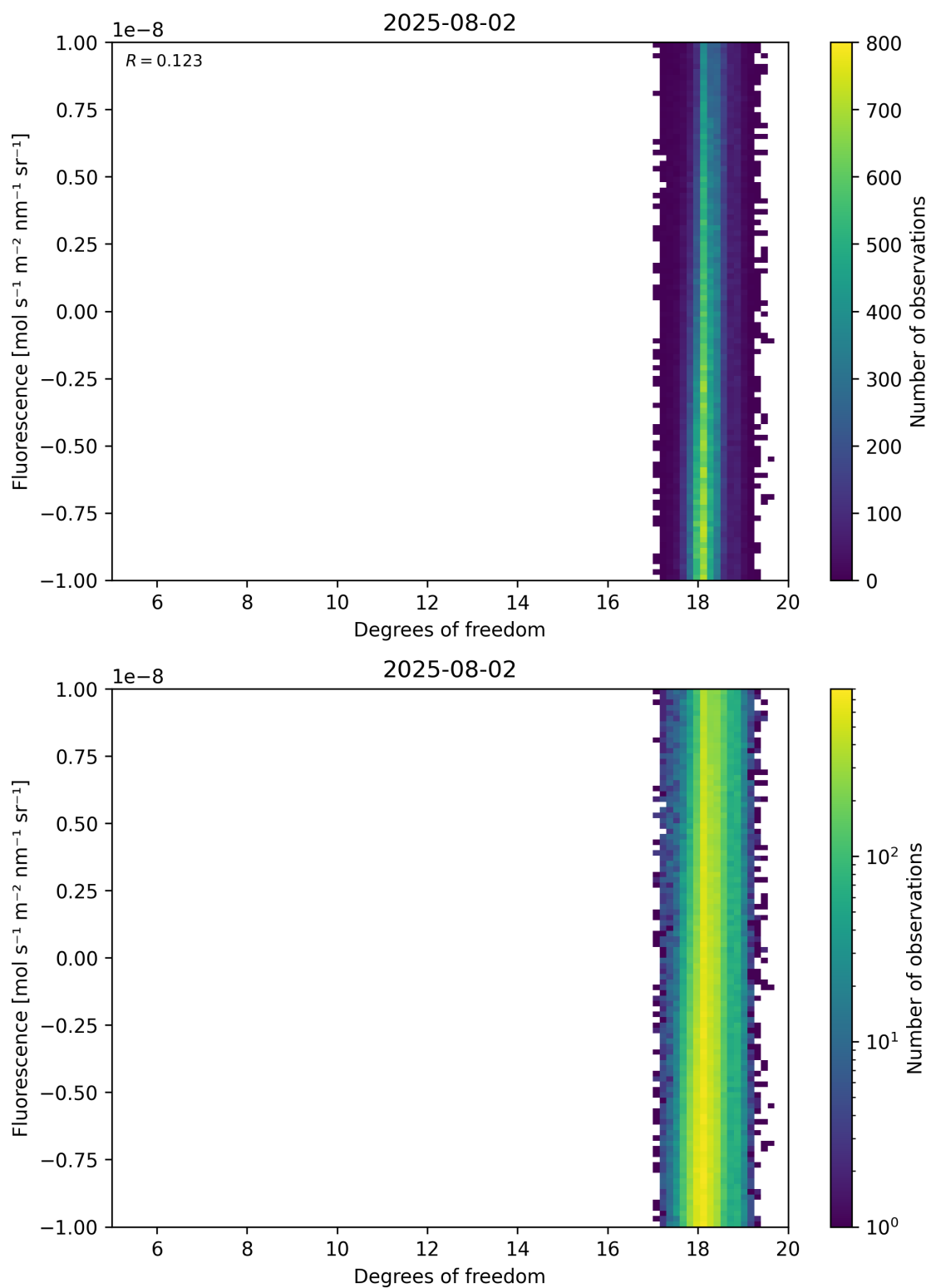
Figure 51: Scatter density plot of “Degrees of freedom” against “Fluorescence” for 2025-08-01 to 2025-08-03.
