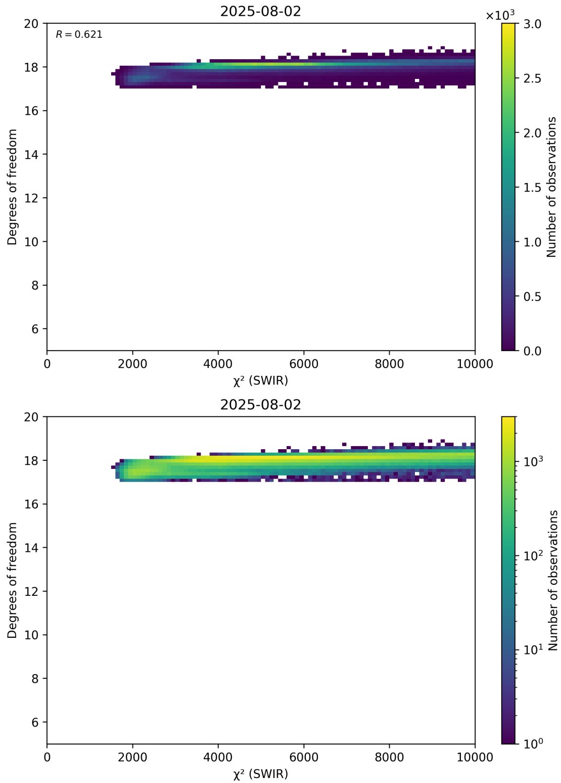
Figure 48: Scatter density plot of “ \chi^2 (SWIR)” against “Degrees of freedom” for 2025-08-01 to 2025-08-03.
