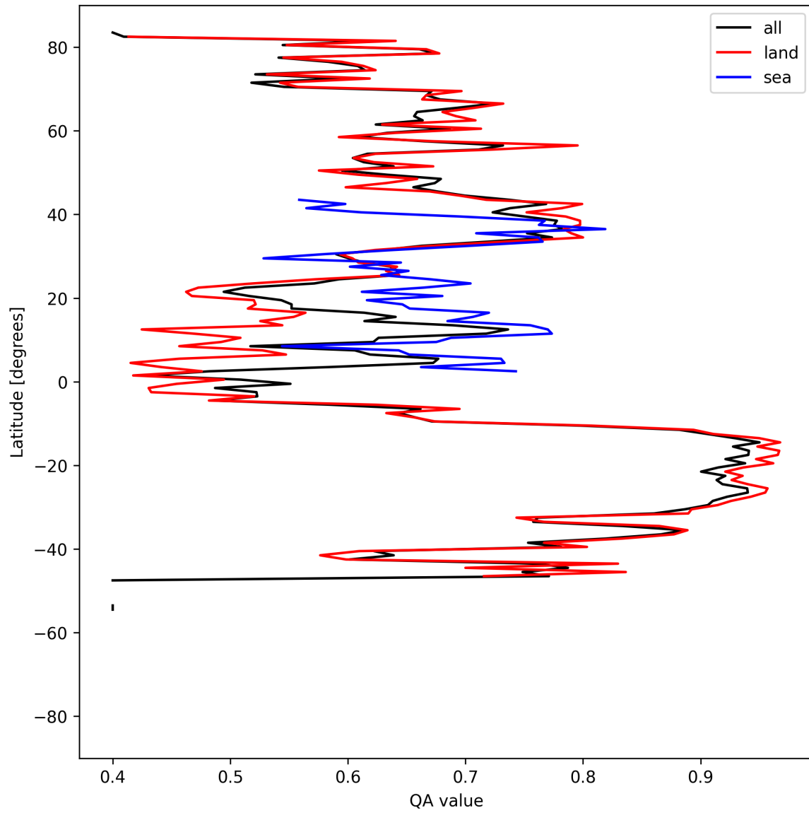
Figure 11: Zonal average of “QA value” for 2025-08-01 to 2025-08-03.
