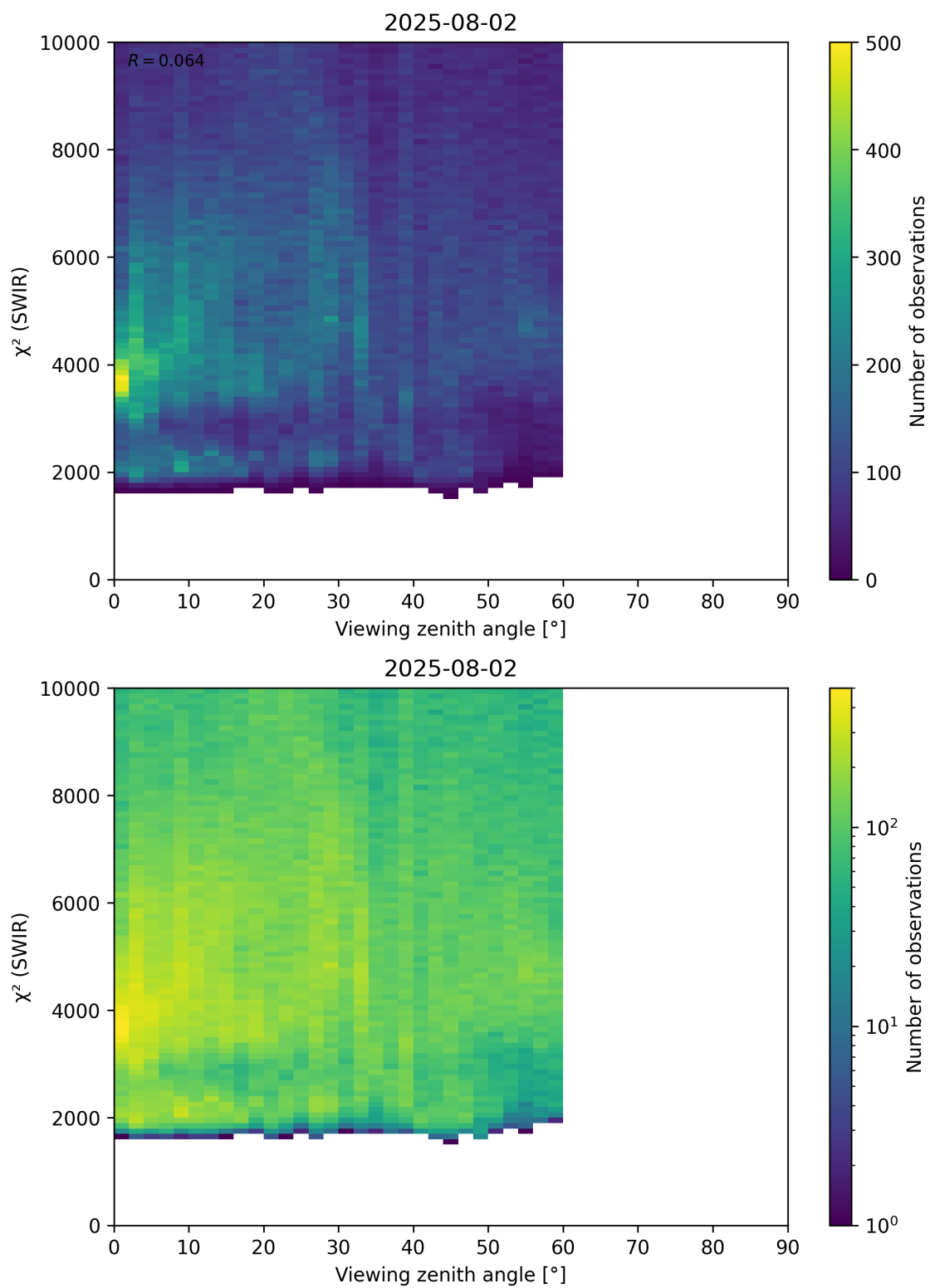
Figure 106: Scatter density plot of “Viewing zenith angle” against “ \chi^2 (SWIR)” for 2025-08-01 to 2025-08-03.
