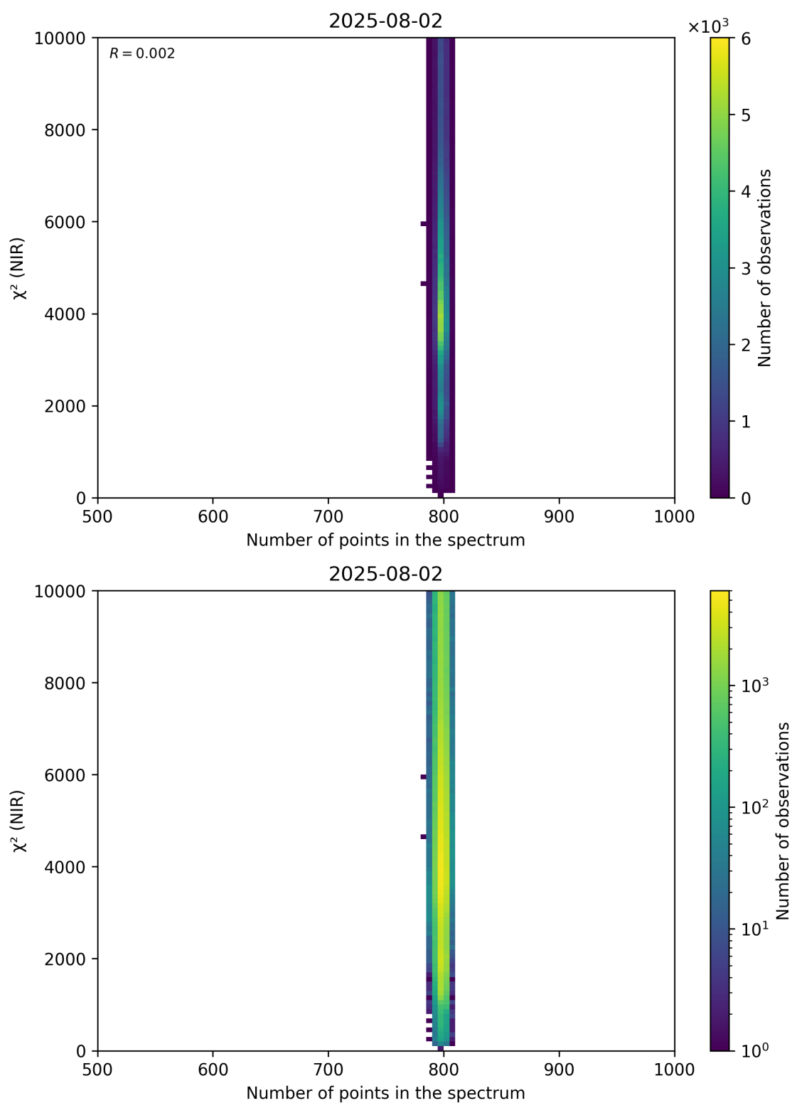
Figure 88: Scatter density plot of “Number of points in the spectrum” against “ \chi^2 (NIR)” for 2025-08-01 to 2025-08-03.
