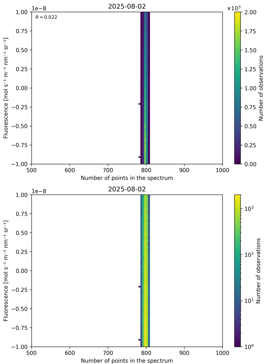
Figure 91: Scatter density plot of “Number of points in the spectrum” against “Fluorescence” for 2025-08-01 to 2025-08-03.
