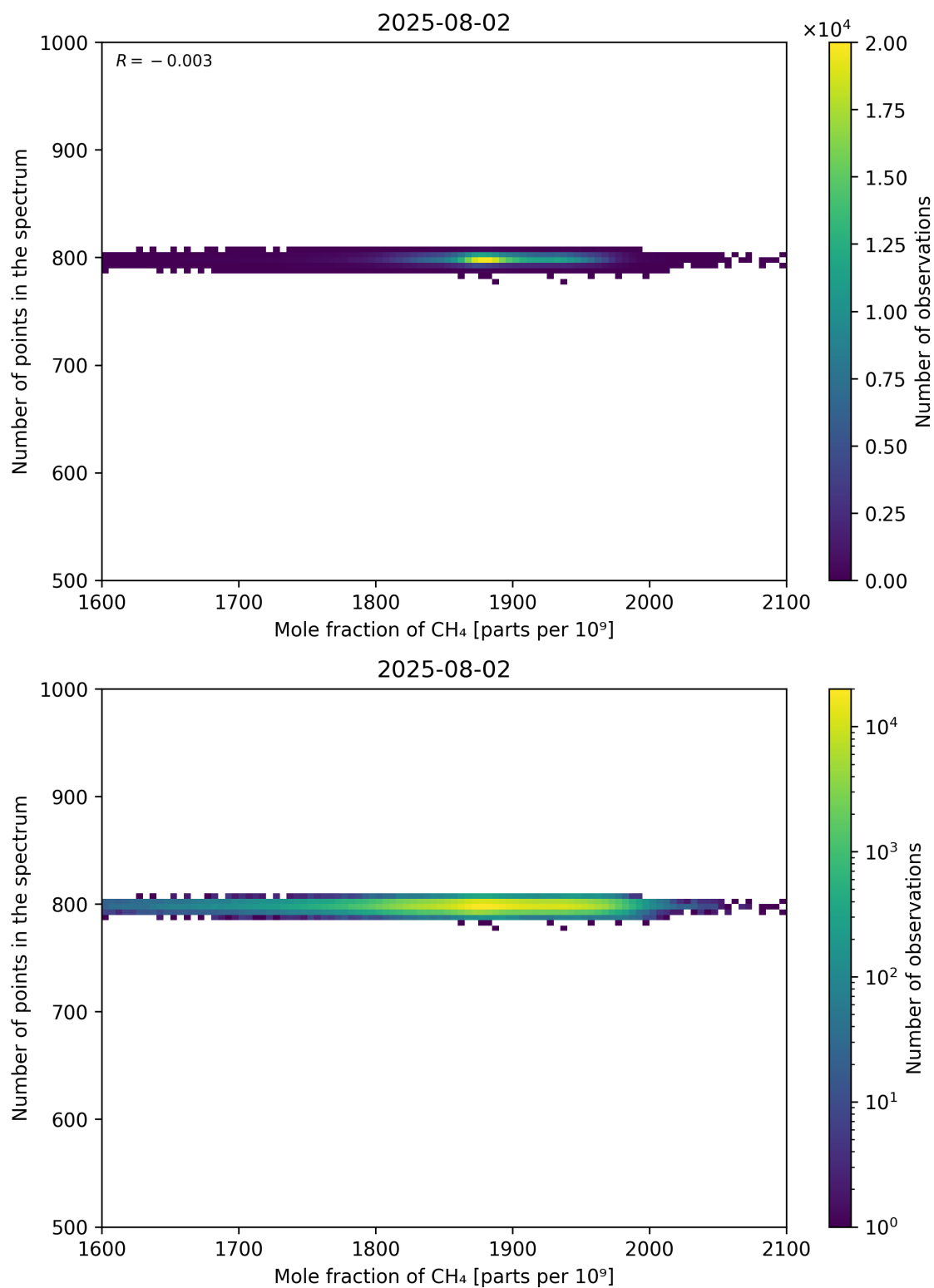
Figure 77: Scatter density plot of “Mole fraction of CH 4 ” against “Number of points in the spectrum” for 2025-08-01 to 2025-08-03.
