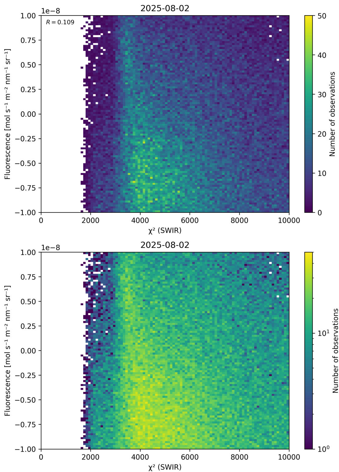
Figure 49: Scatter density plot of “ \chi^2 (SWIR)” against “Fluorescence” for 2025-08-01 to 2025-08-03.
