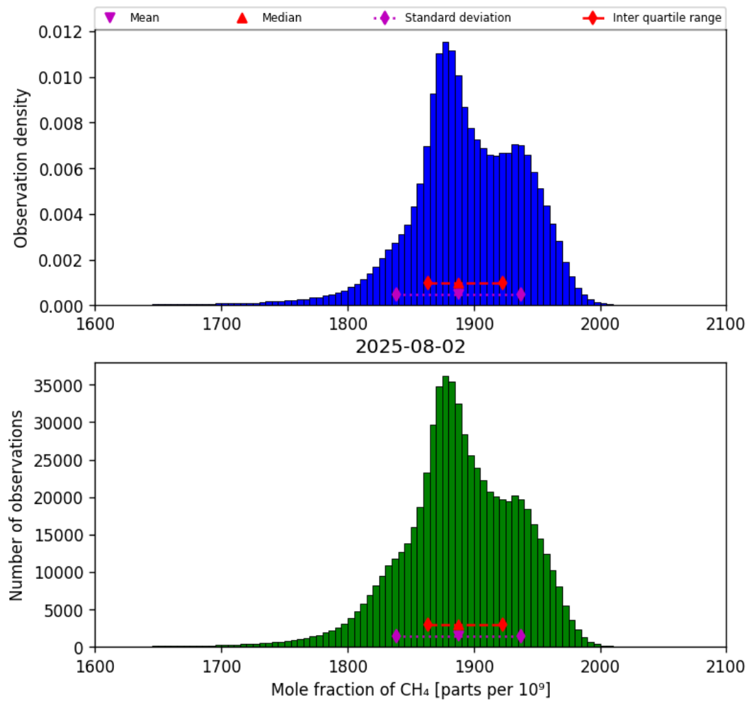
Figure 23: Histogram of “Mole fraction of CH 4 ” for 2025-08-01 to 2025-08-03
