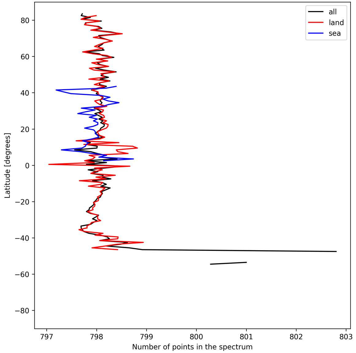
Figure 15: Zonal average of “Number of points in the spectrum” for 2025-08-01 to 2025-08-03.
