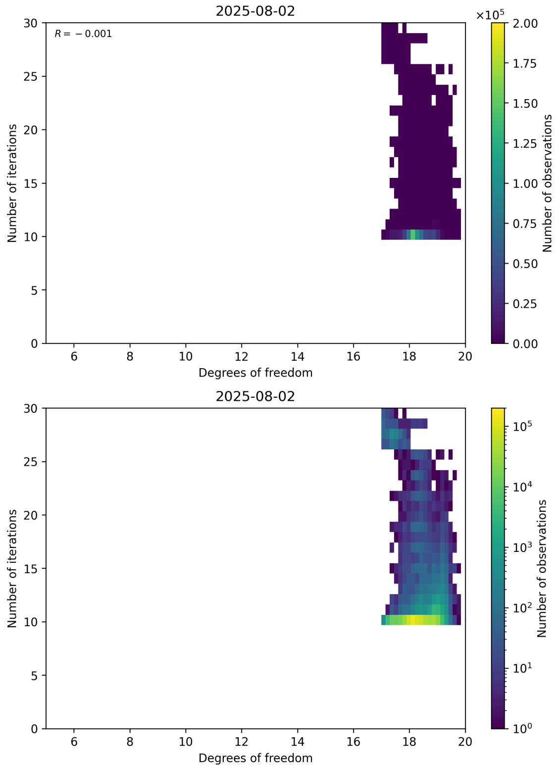
Figure 52: Scatter density plot of “Degrees of freedom” against “Number of iterations” for 2025-08-01 to 2025-08-03.
