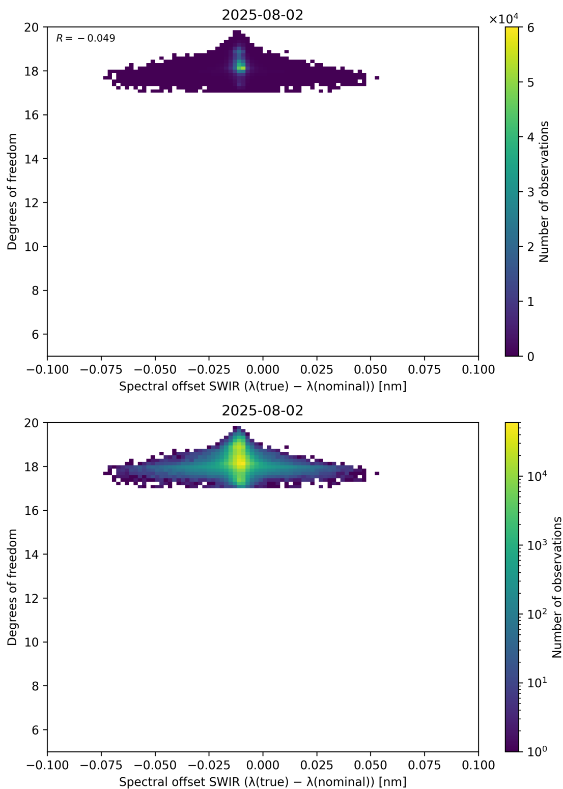
Figure 119: Scatter density plot of “Spectral offset SWIR ( \lambda_{\text{true}} - \lambda_{\text{nominal}} )” against “Degrees of freedom” for 2025-08-01 to 2025-08-03.
