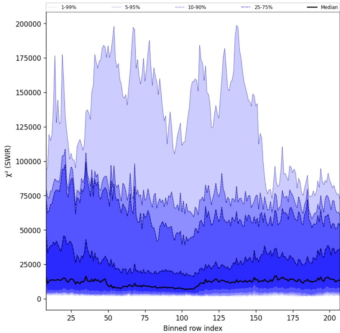
Figure 39: Along track statistics of “ \chi^2 (SWIR)” for 2025-08-01 to 2025-08-03
