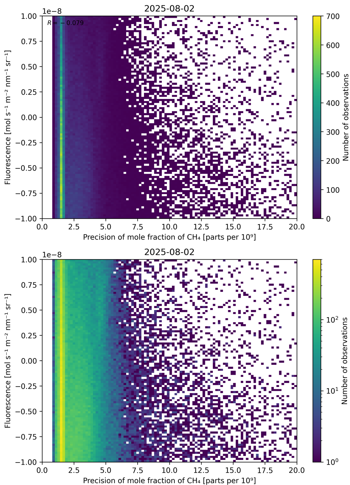
Figure 81: Scatter density plot of “Precision of mole fraction of \text{CH}_4 ” against “Fluorescence” for 2025-08-01 to 2025-08-03.
