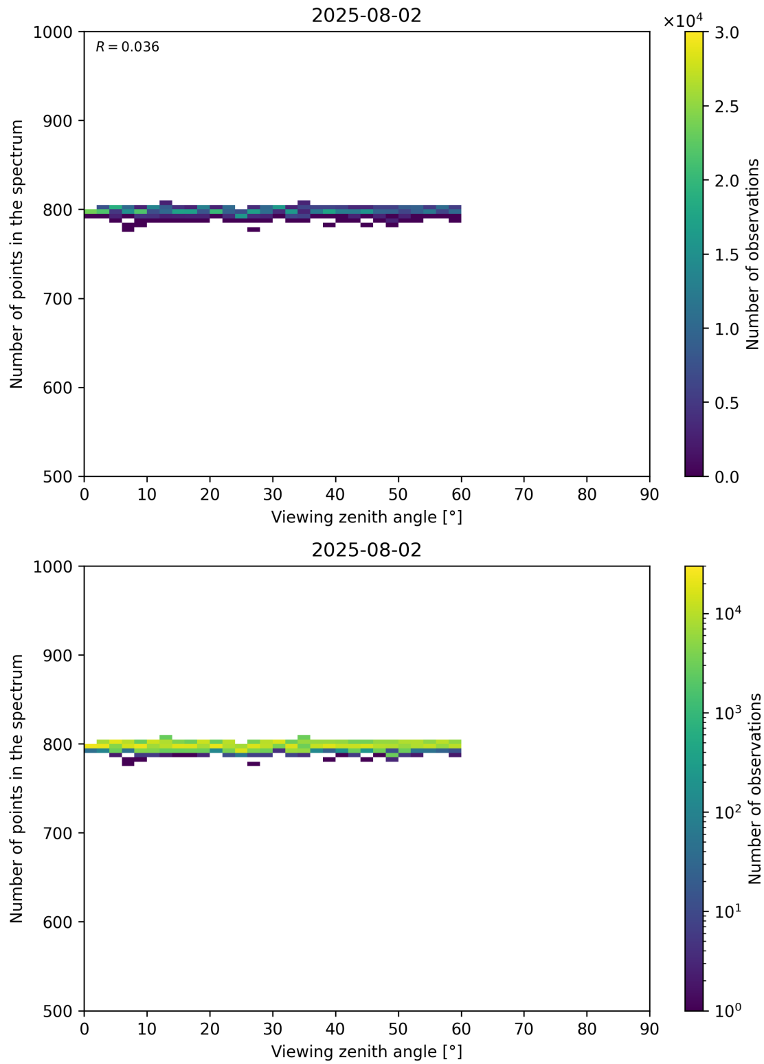
Figure 114: Scatter density plot of “Viewing zenith angle” against “Number of points in the spectrum” for 2025-08-01 to 2025-08-03.
