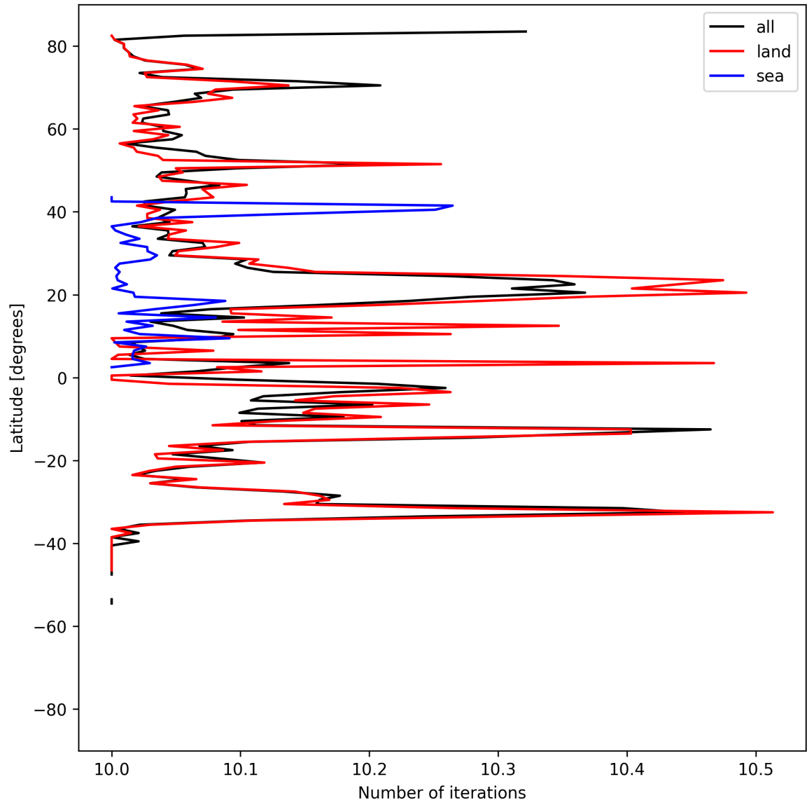
Figure 20: Zonal average of “Number of iterations” for 2025-08-01 to 2025-08-03.
