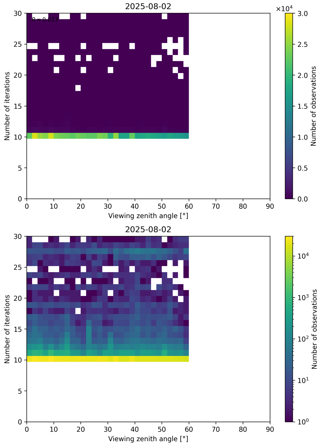
Figure 113: Scatter density plot of “Viewing zenith angle” against “Number of iterations” for 2025-08-01 to 2025-08-03.
