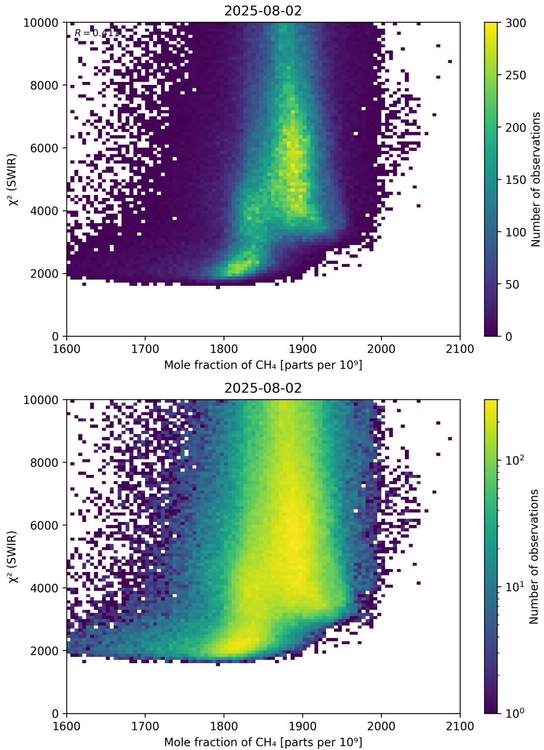
Figure 71: Scatter density plot of “Mole fraction of \text{CH}_4 ” against “ \chi^2 (SWIR)” for 2025-08-01 to 2025-08-03.
