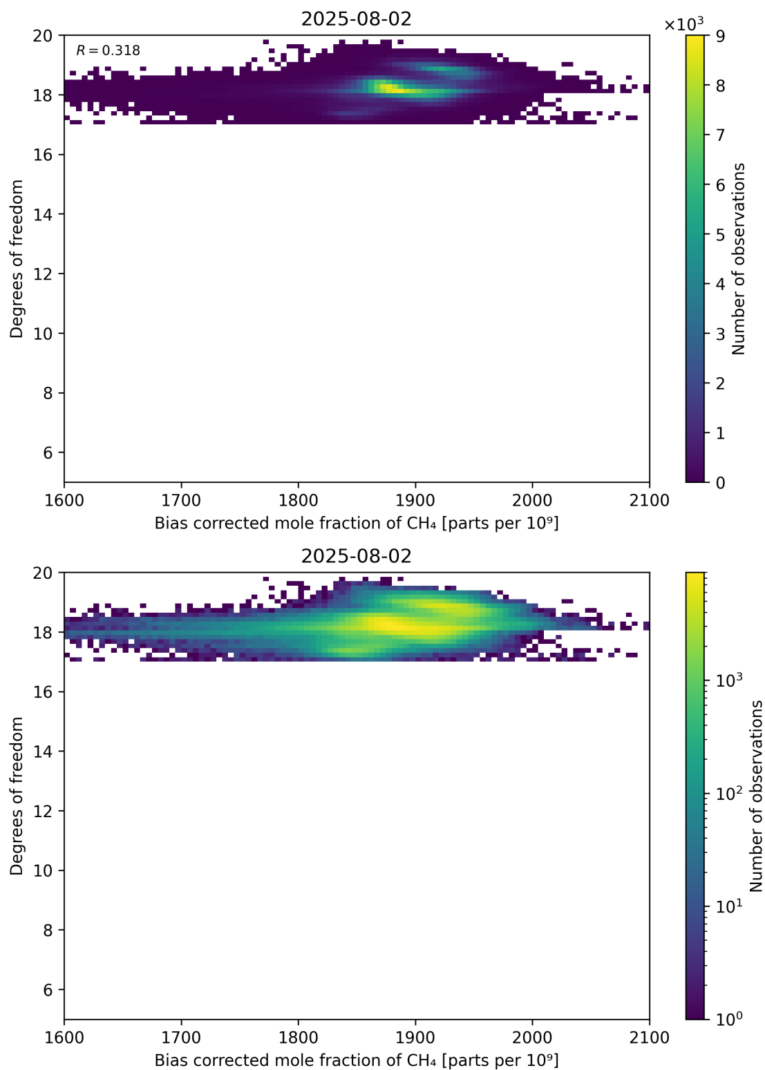
Figure 65: Scatter density plot of “Bias corrected mole fraction of CH 4 ” against “Degrees of freedom” for 2025-08-01 to 2025-08-03.
