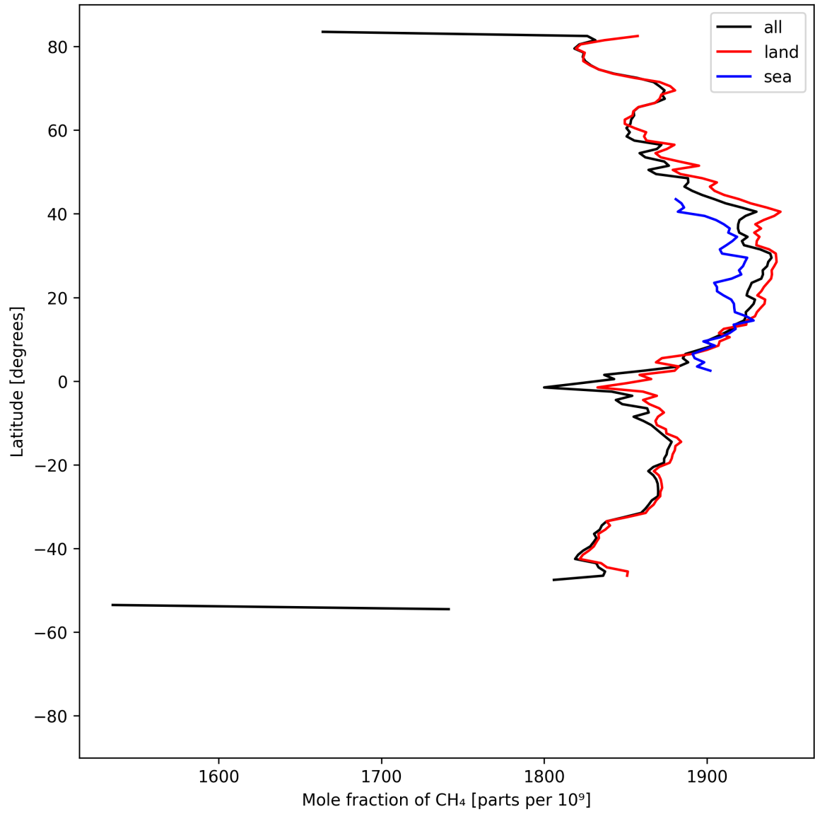
Figure 12: Zonal average of “Mole fraction of CH 4 ” for 2025-08-01 to 2025-08-03.
