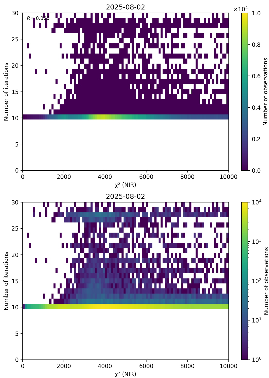
Figure 46: Scatter density plot of “ \chi^2 (NIR)” against “Number of iterations” for 2025-08-01 to 2025-08-03.
