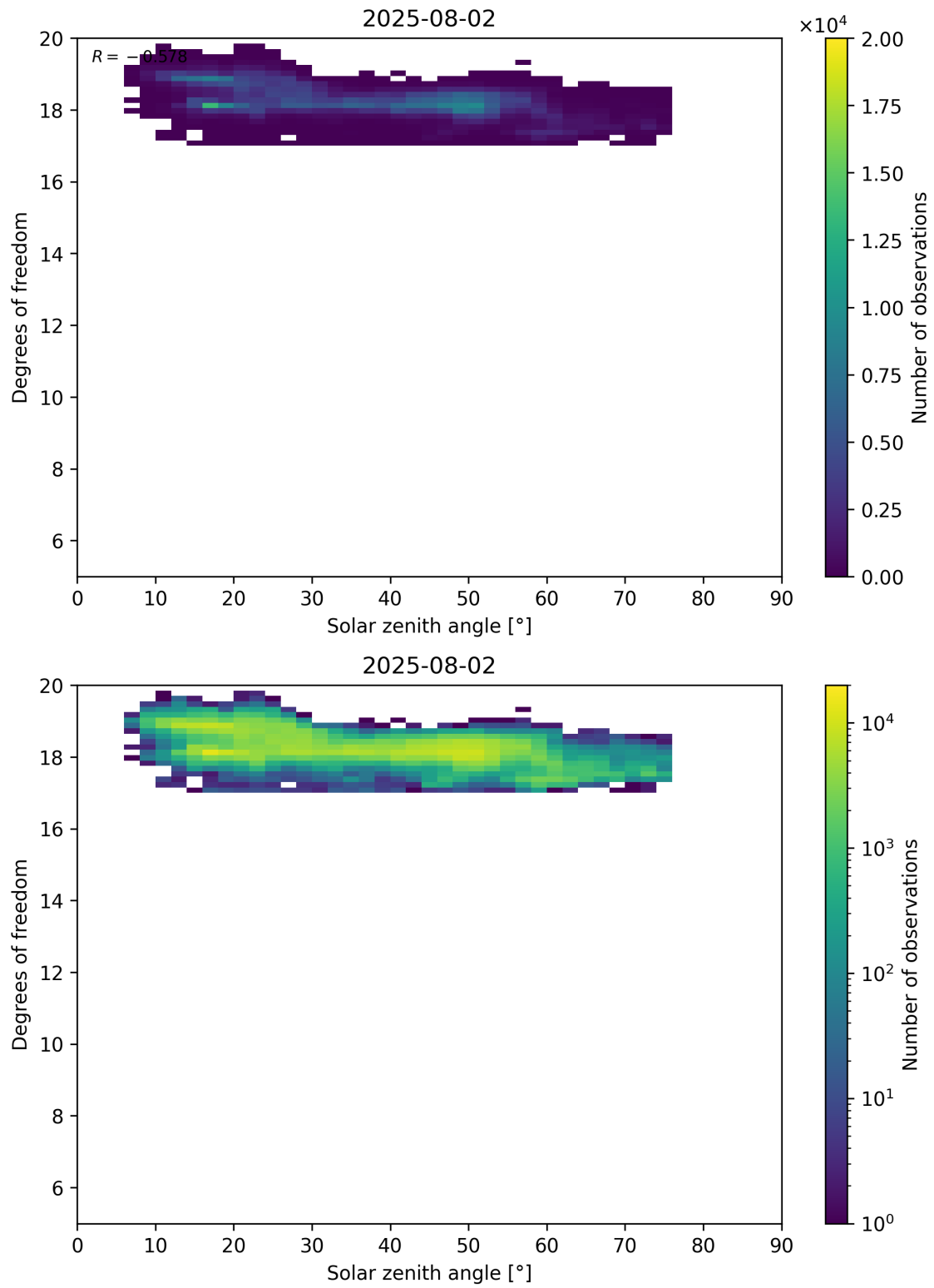
Figure 96: Scatter density plot of “Solar zenith angle” against “Degrees of freedom” for 2025-08-01 to 2025-08-03.
