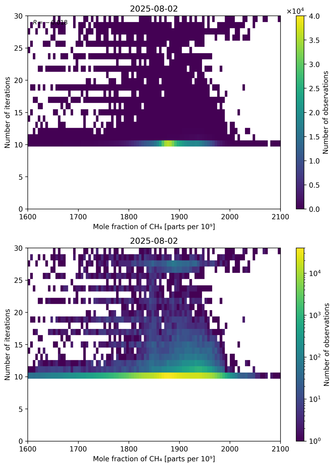
Figure 76: Scatter density plot of “Mole fraction of CH 4 ” against “Number of iterations” for 2025-08-01 to 2025-08-03.
