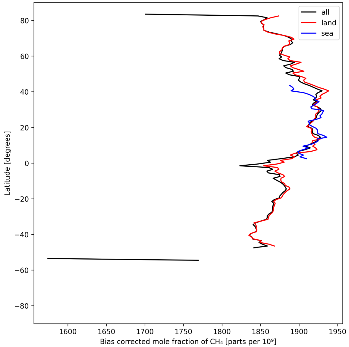
Figure 14: Zonal average of “Bias corrected mole fraction of CH 4 ” for 2025-08-01 to 2025-08-03.
