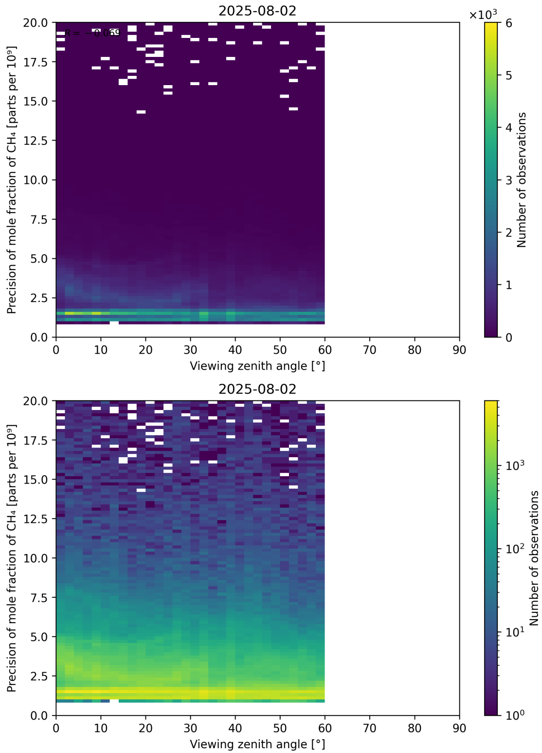
Figure 112: Scatter density plot of “Viewing zenith angle” against “Precision of mole fraction of CH 4 ” for 2025-08-01 to 2025-08-03.
