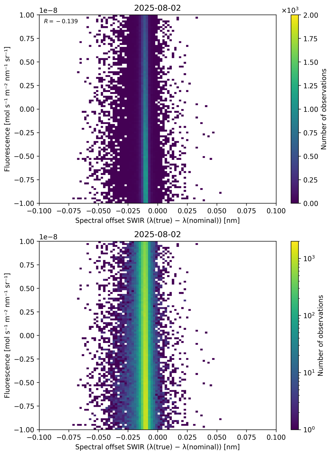
Figure 120: Scatter density plot of “Spectral offset SWIR ( \lambda_{\text{true}} - \lambda_{\text{nominal}} )” against “Fluorescence” for 2025-08-01 to 2025-08-03.
