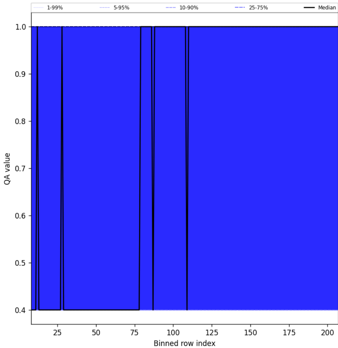
Figure 33: Along track statistics of “QA value” for 2025-08-01 to 2025-08-03
