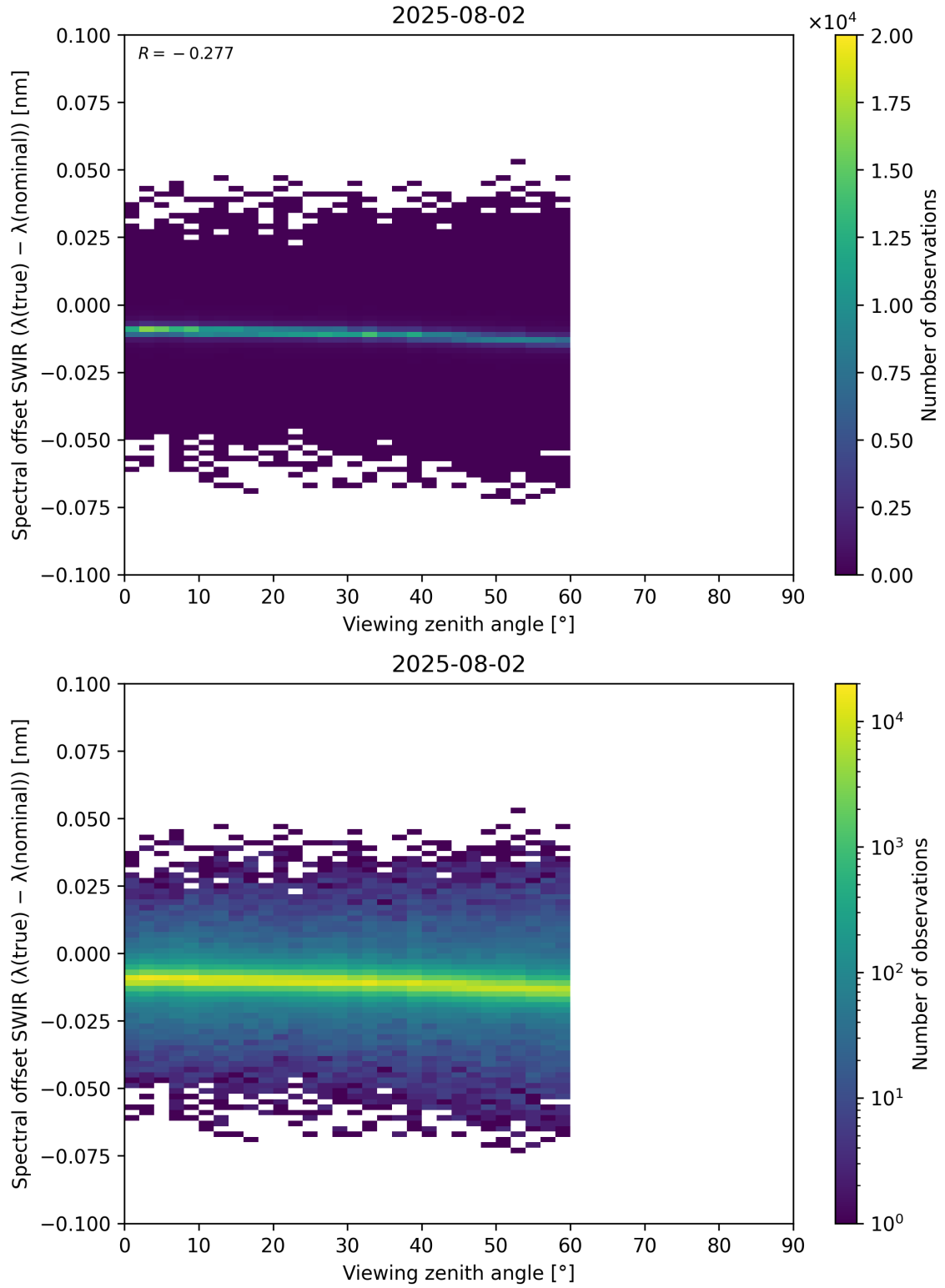
Figure 116: Scatter density plot of “Viewing zenith angle” against “Spectral offset SWIR ( \lambda_{\text{true}} - \lambda_{\text{nominal}} )” for 2025-08-01 to 2025-08-03.
