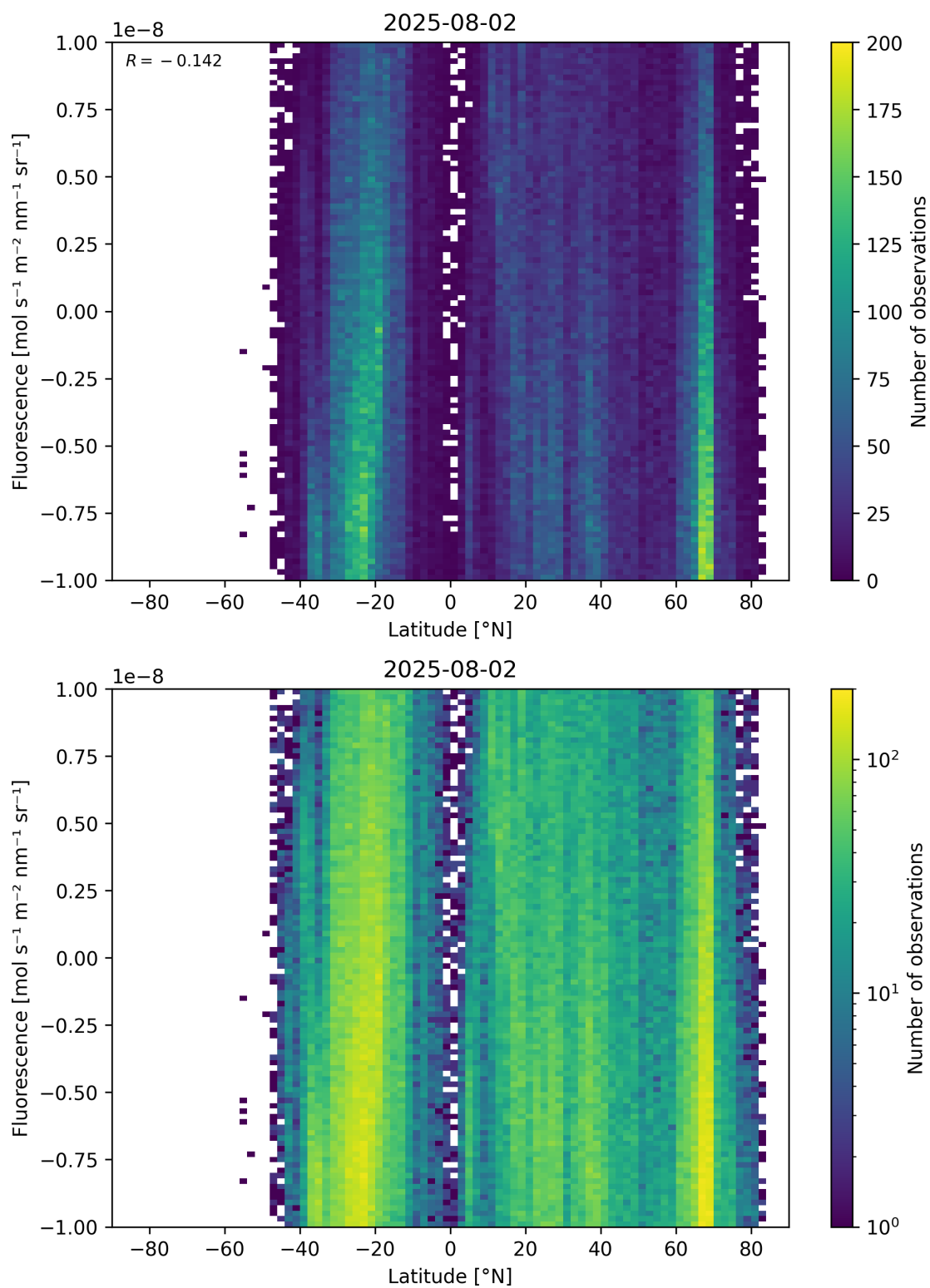
Figure 56: Scatter density plot of “Latitude” against “Fluorescence” for 2025-08-01 to 2025-08-03.
