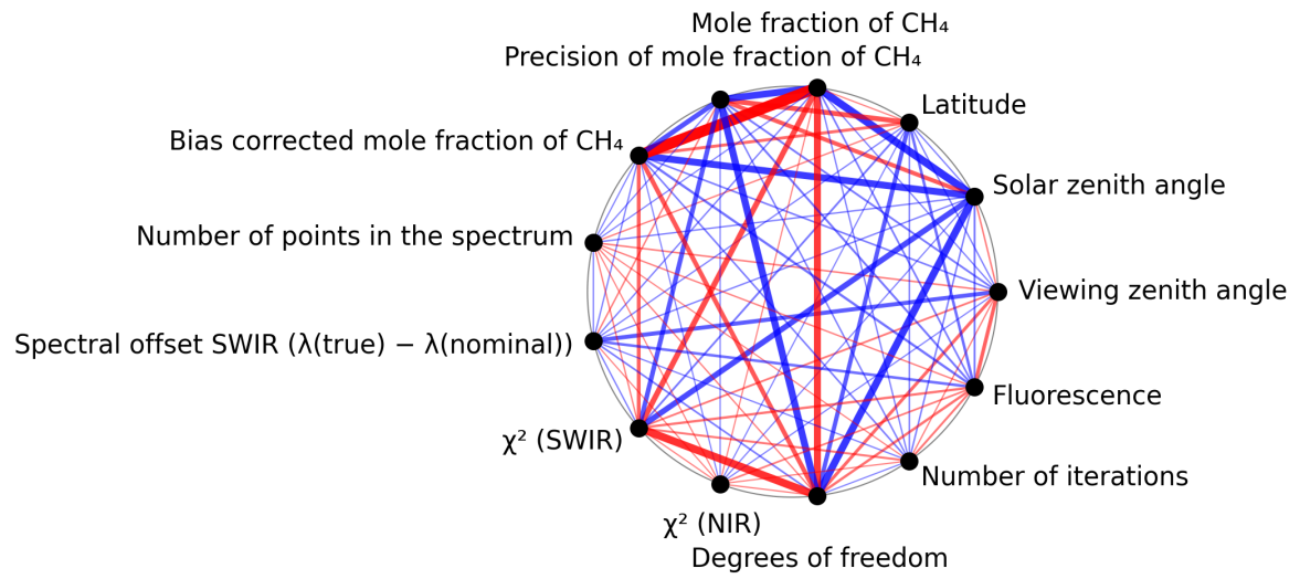
Figure 1: Map of correlation graph for 2025-08-01 to 2025-08-03.
