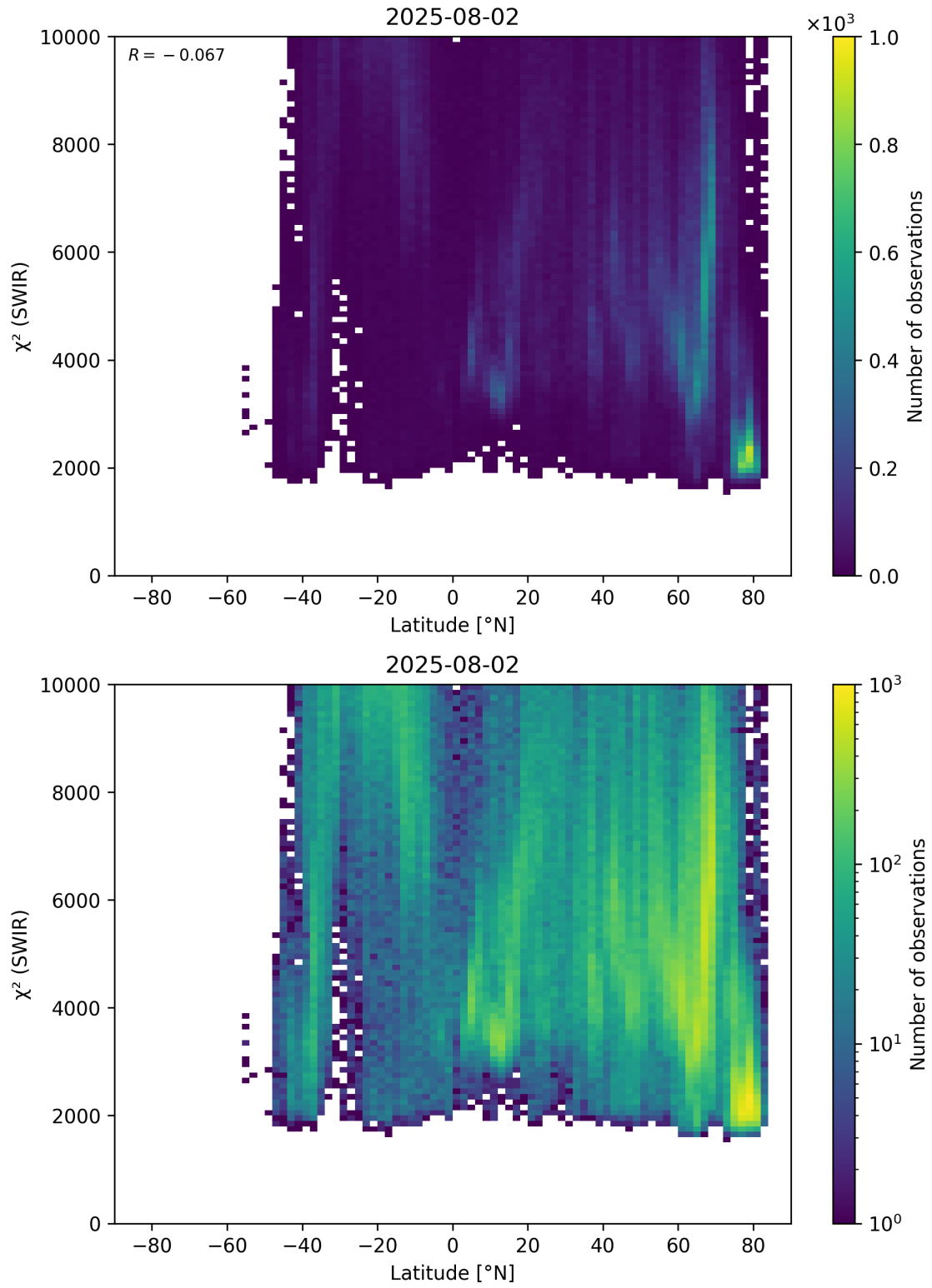
Figure 54: Scatter density plot of “Latitude” against “ \chi^2 (SWIR)” for 2025-08-01 to 2025-08-03.
