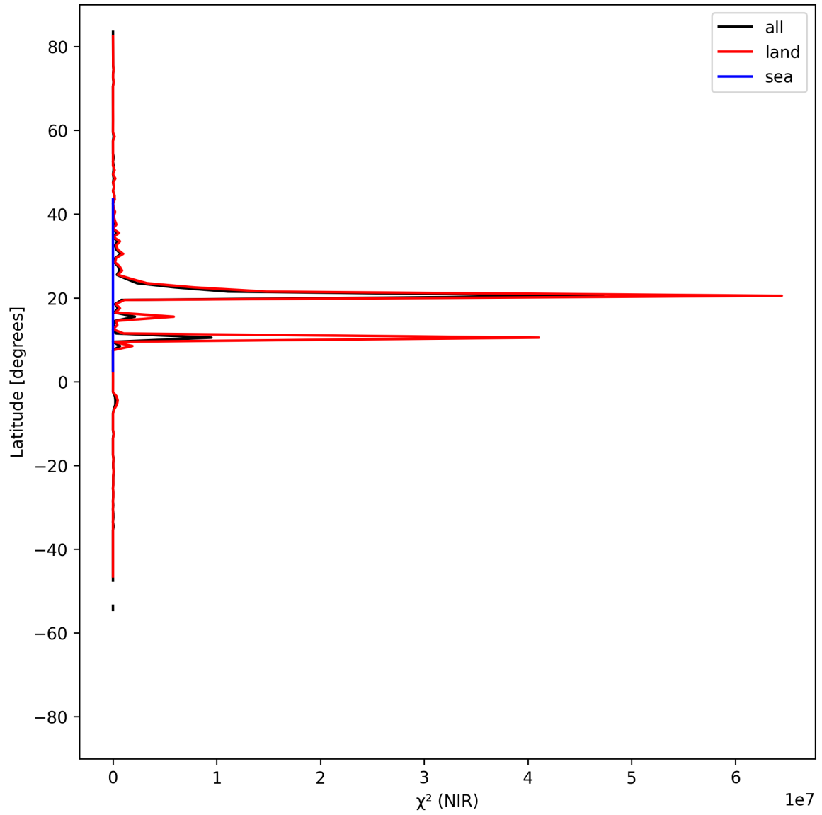
Figure 18: Zonal average of “ \chi^2 (NIR)” for 2025-08-01 to 2025-08-03.
