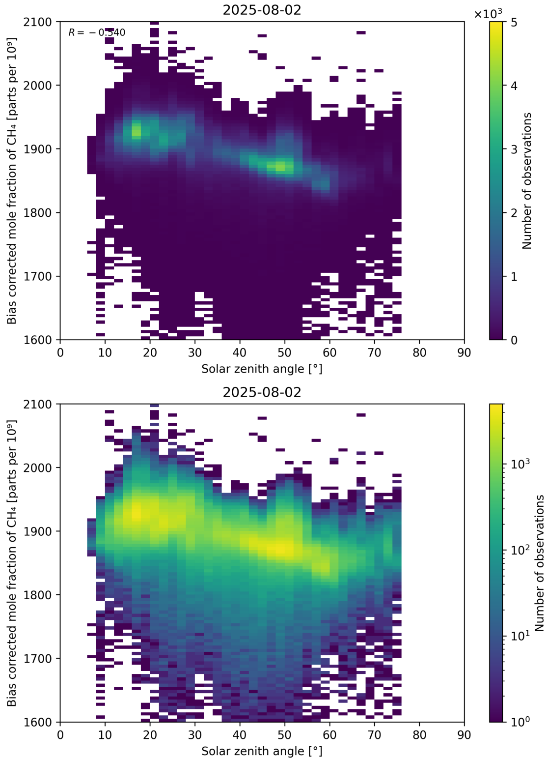
Figure 100: Scatter density plot of “Solar zenith angle” against “Bias corrected mole fraction of CH 4 ” for 2025-08-01 to 2025-08-03.
