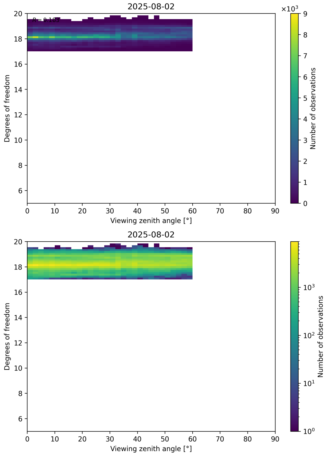
Figure 107: Scatter density plot of “Viewing zenith angle” against “Degrees of freedom” for 2025-08-01 to 2025-08-03.
