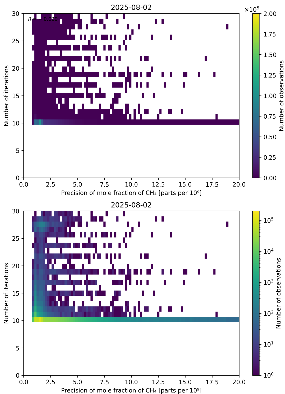
Figure 83: Scatter density plot of “Precision of mole fraction of CH 4 ” against “Number of iterations” for 2025-08-01 to 2025-08-03.
