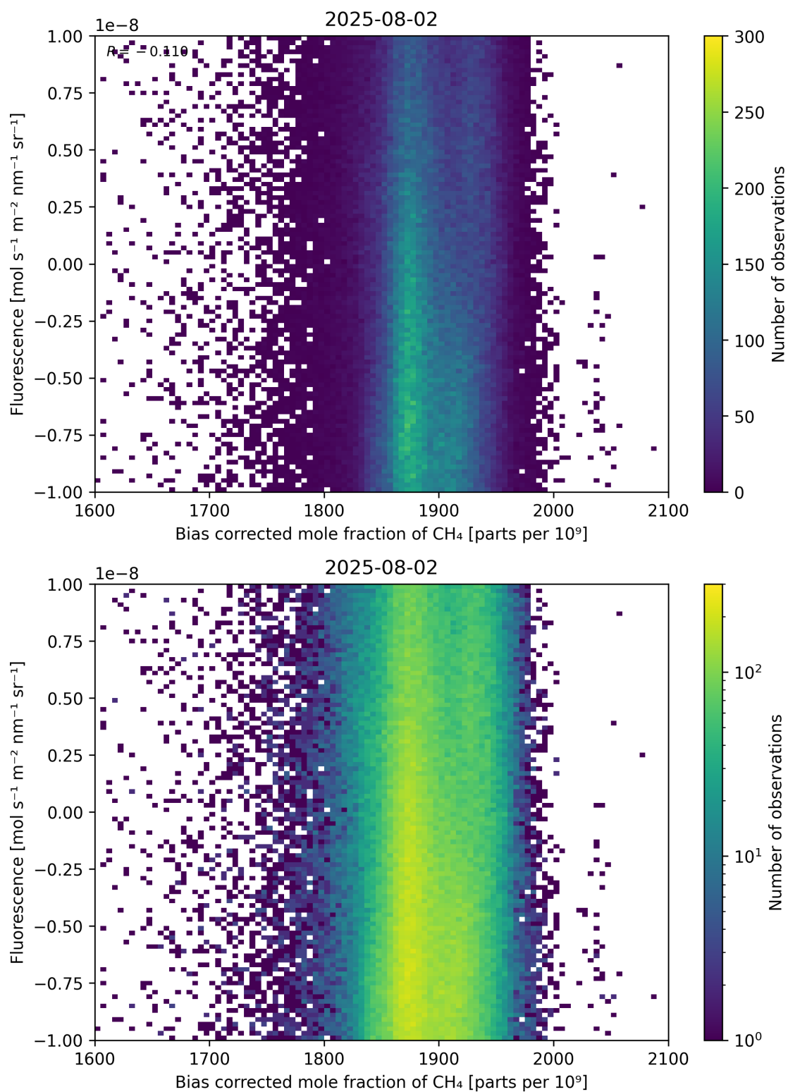
Figure 66: Scatter density plot of “Bias corrected mole fraction of \text{CH}_4 ” against “Fluorescence” for 2025-08-01 to 2025-08-03.
