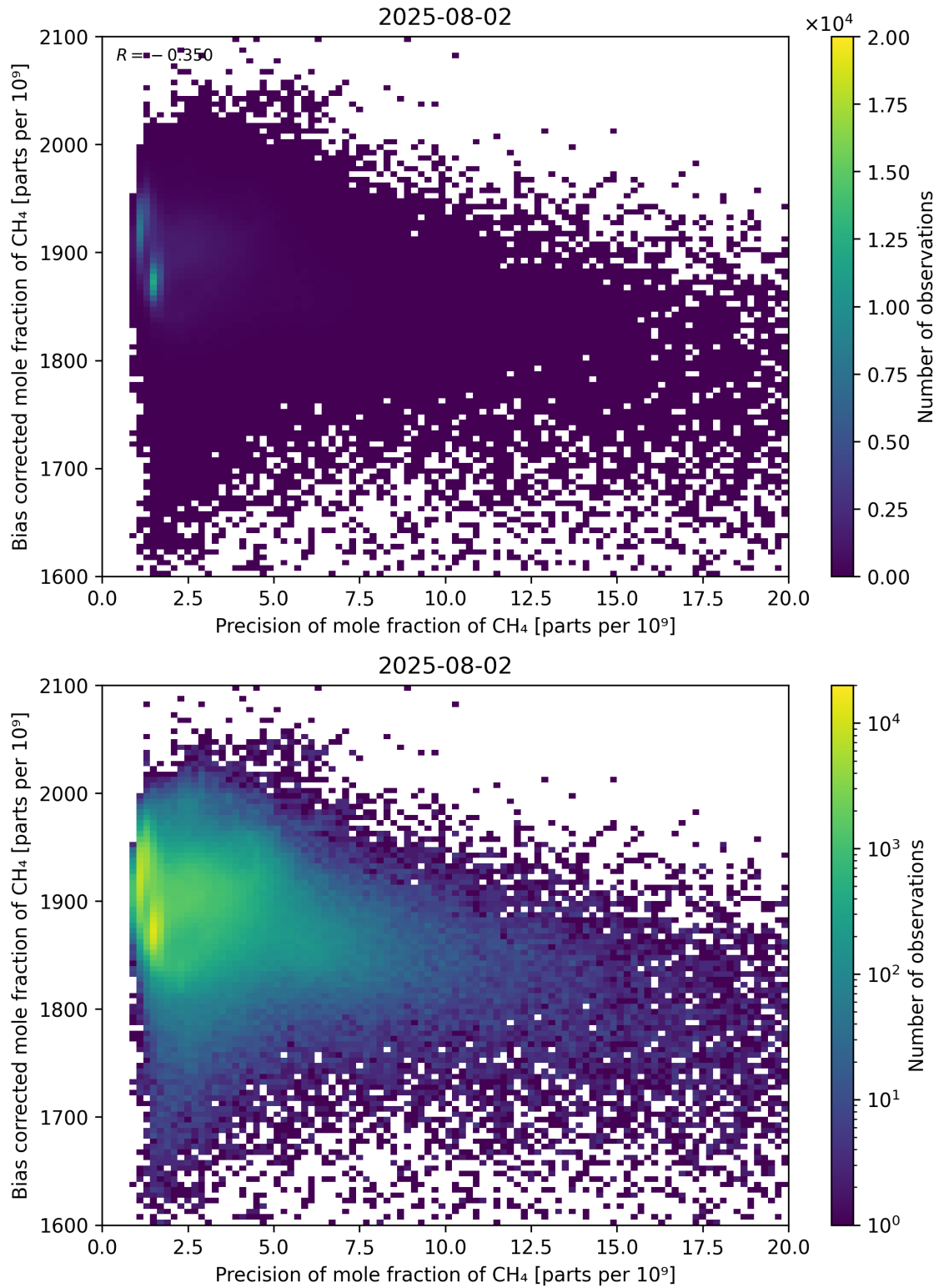
Figure 82: Scatter density plot of “Precision of mole fraction of CH 4 ” against “Bias corrected mole fraction of CH 4 ” for 2025-08-01 to 2025-08-03.
