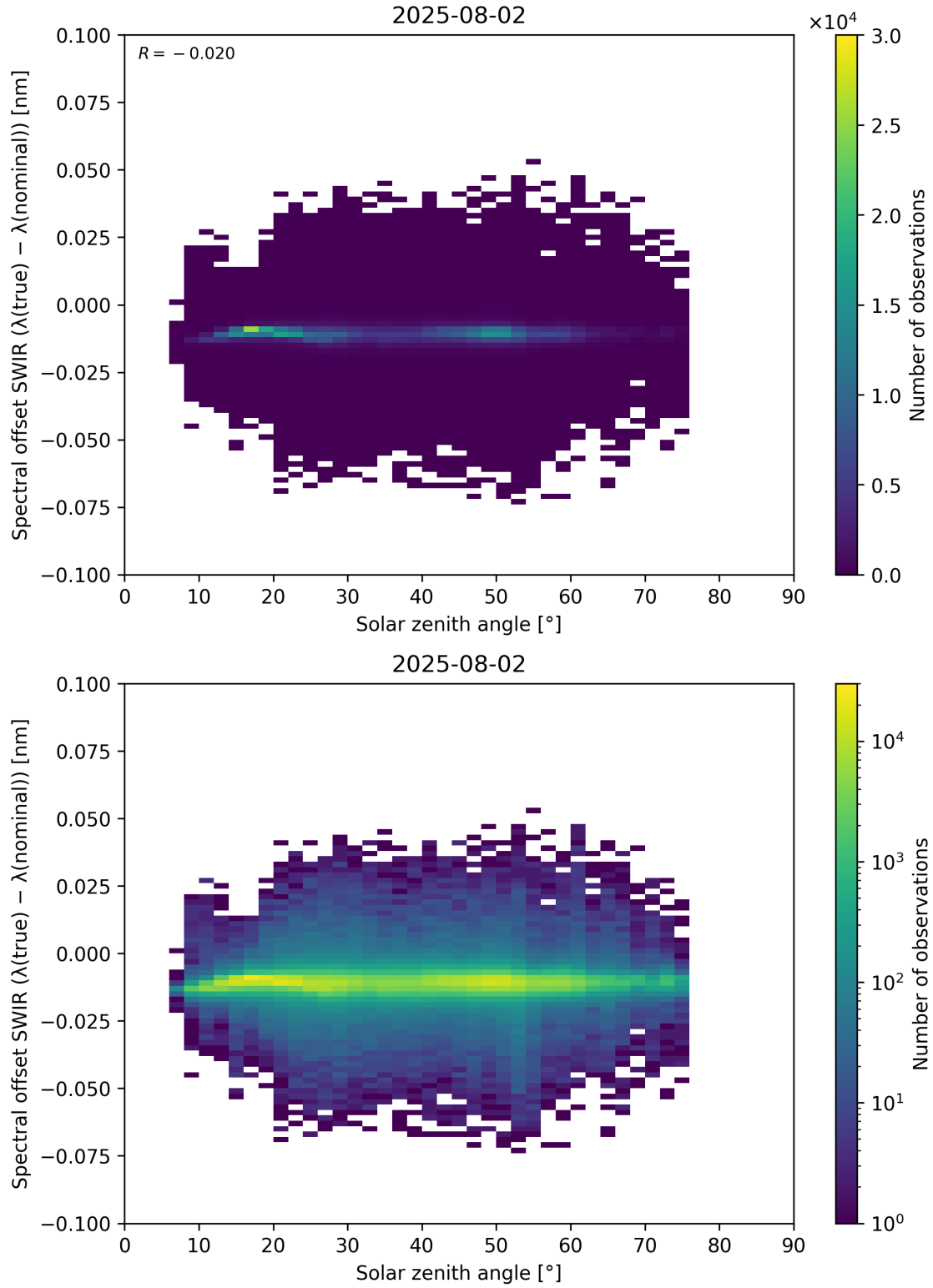
Figure 104: Scatter density plot of “Solar zenith angle” against “Spectral offset SWIR ( \lambda_{\text{true}} - \lambda_{\text{nominal}} )” for 2025-08-01 to 2025-08-03.
