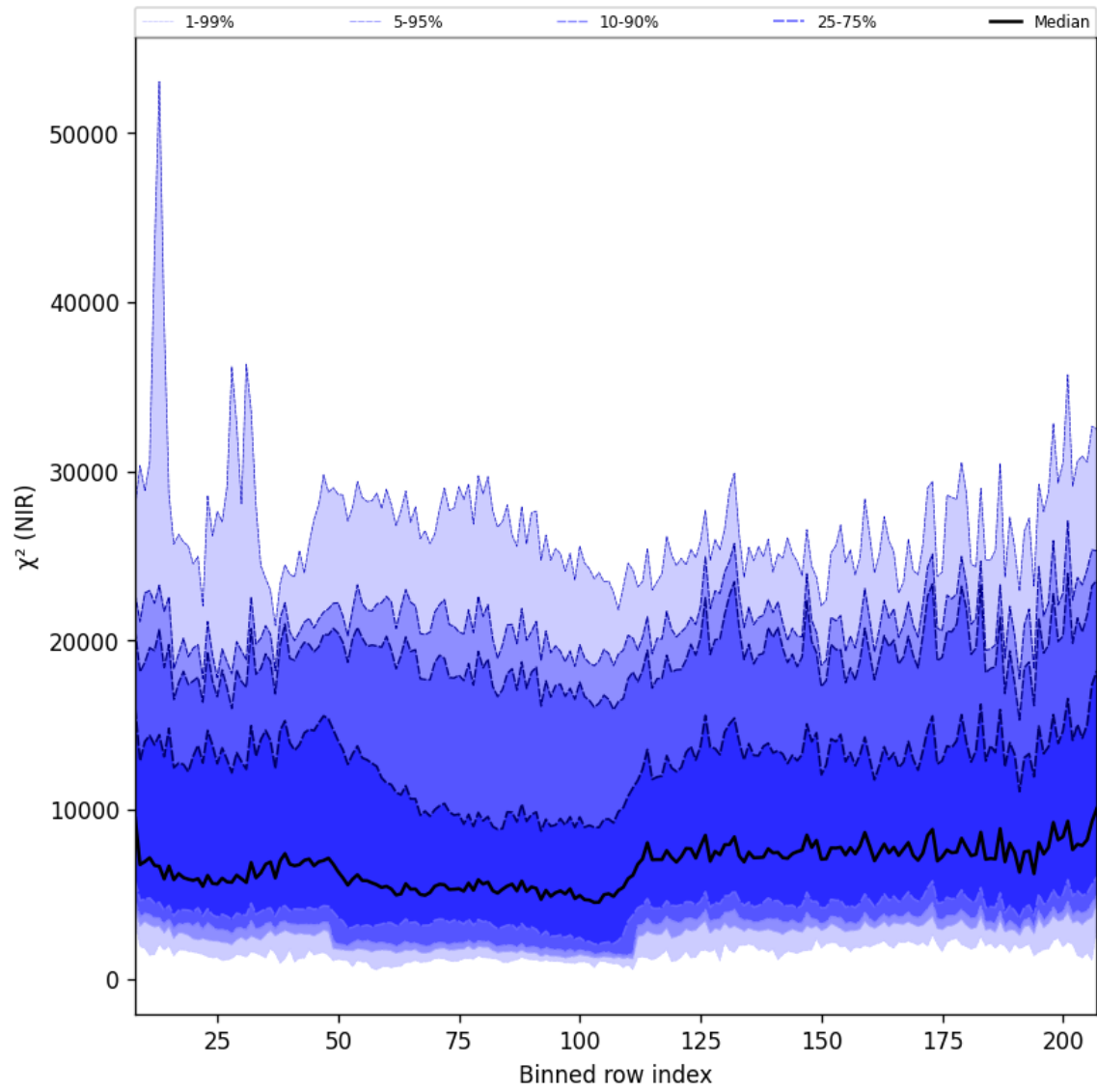
Figure 40: Along track statistics of “ \chi^2 (NIR)” for 2025-08-01 to 2025-08-03
