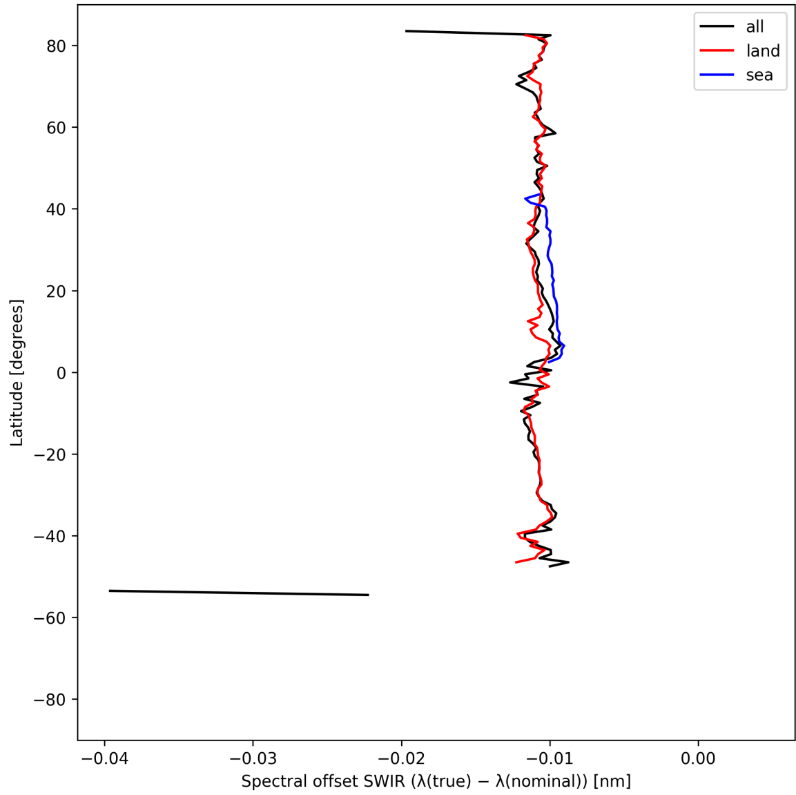
Figure 16: Zonal average of “Spectral offset SWIR ( \lambda_{\text{true}} - \lambda_{\text{nominal}} )” for 2025-08-01 to 2025-08-03.
