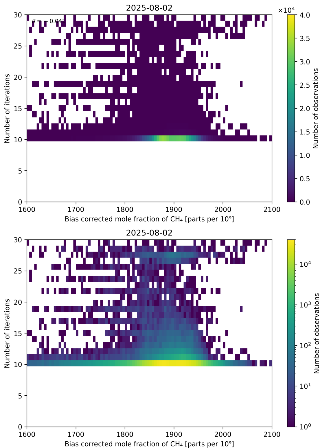
Figure 67: Scatter density plot of “Bias corrected mole fraction of CH 4 ” against “Number of iterations” for 2025-08-01 to 2025-08-03.
