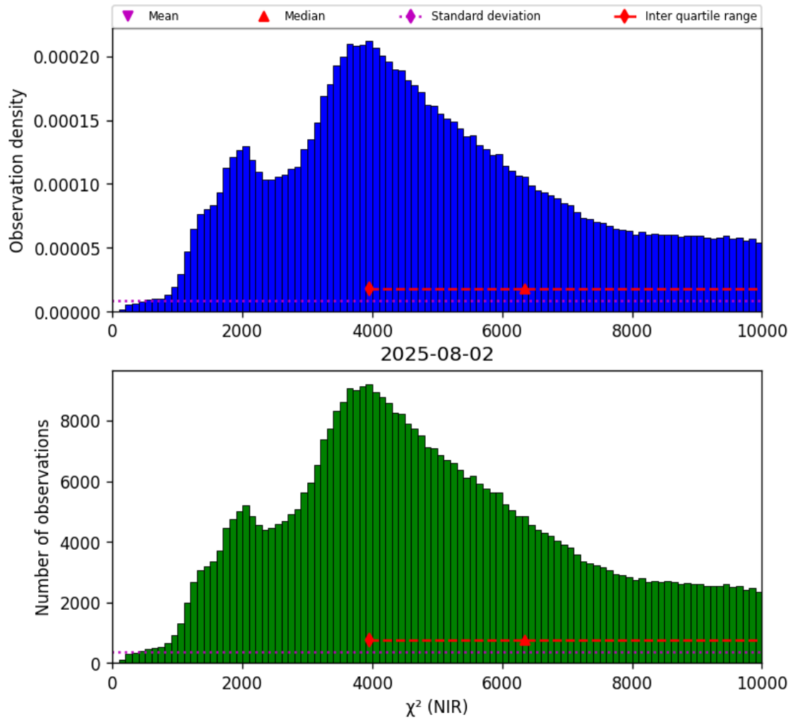
Figure 29: Histogram of " \chi^2 (NIR)" for 2025-08-01 to 2025-08-03
