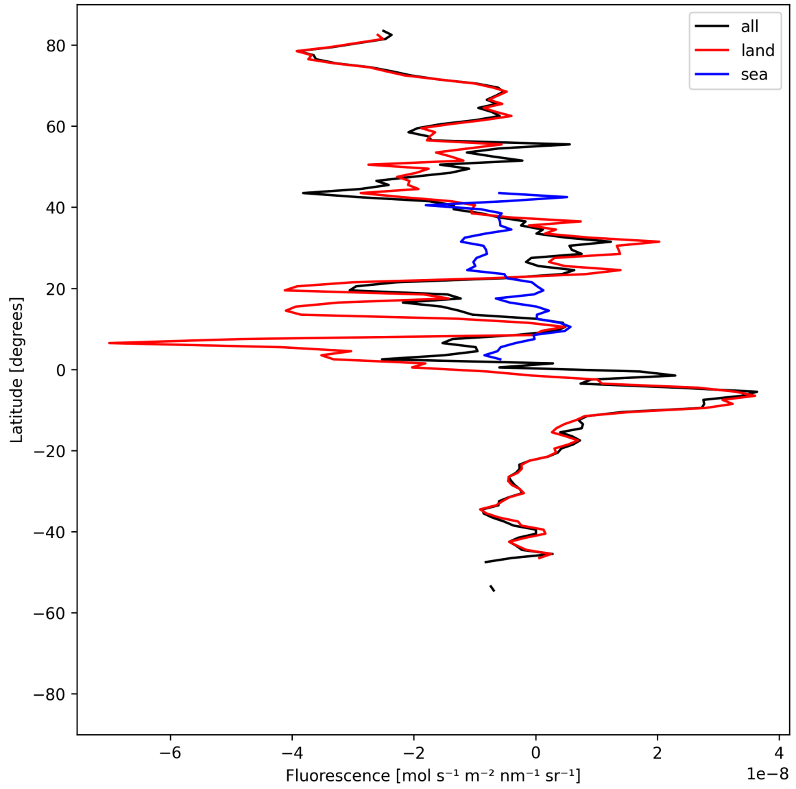
Figure 21: Zonal average of “Fluorescence” for 2025-08-01 to 2025-08-03.
