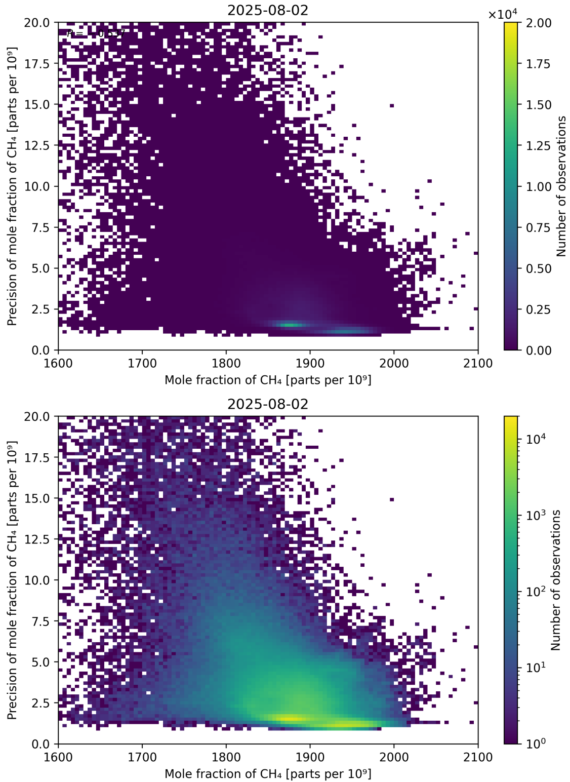
Figure 75: Scatter density plot of “Mole fraction of CH 4 ” against “Precision of mole fraction of CH 4 ” for 2025-08-01 to 2025-08-03.
