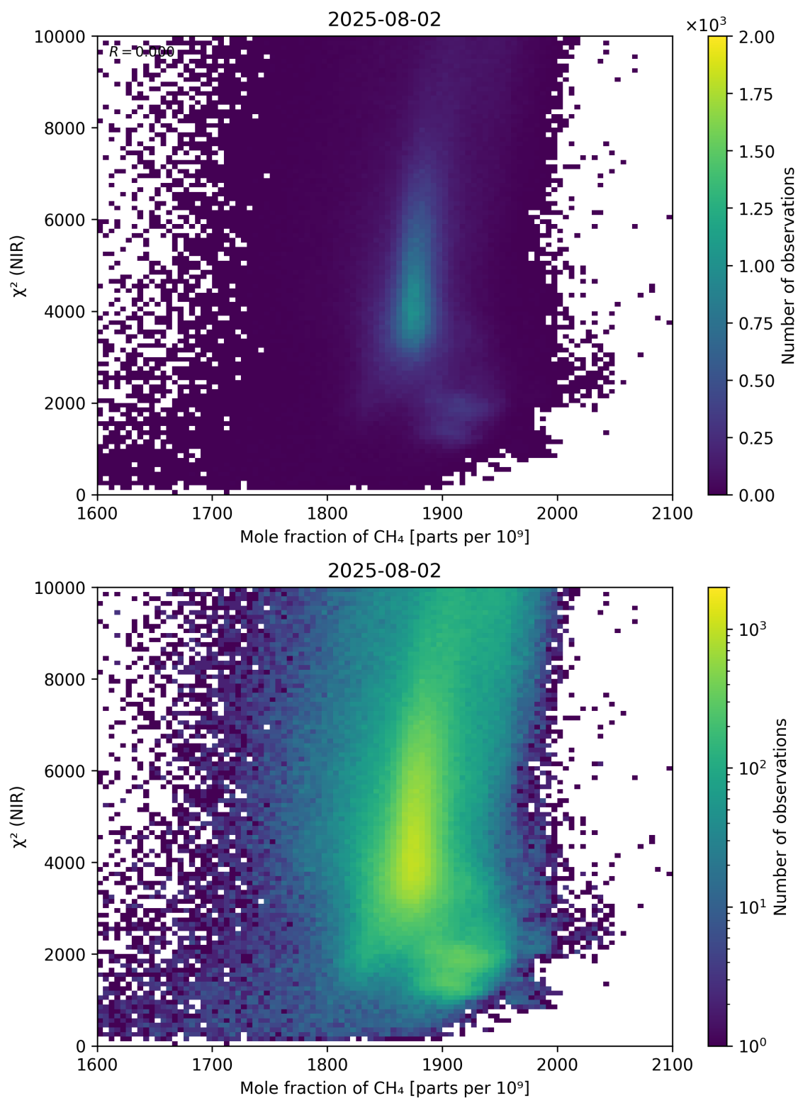
Figure 70: Scatter density plot of “Mole fraction of \text{CH}_4 ” against “ \chi^2 (NIR)” for 2025-08-01 to 2025-08-03.
