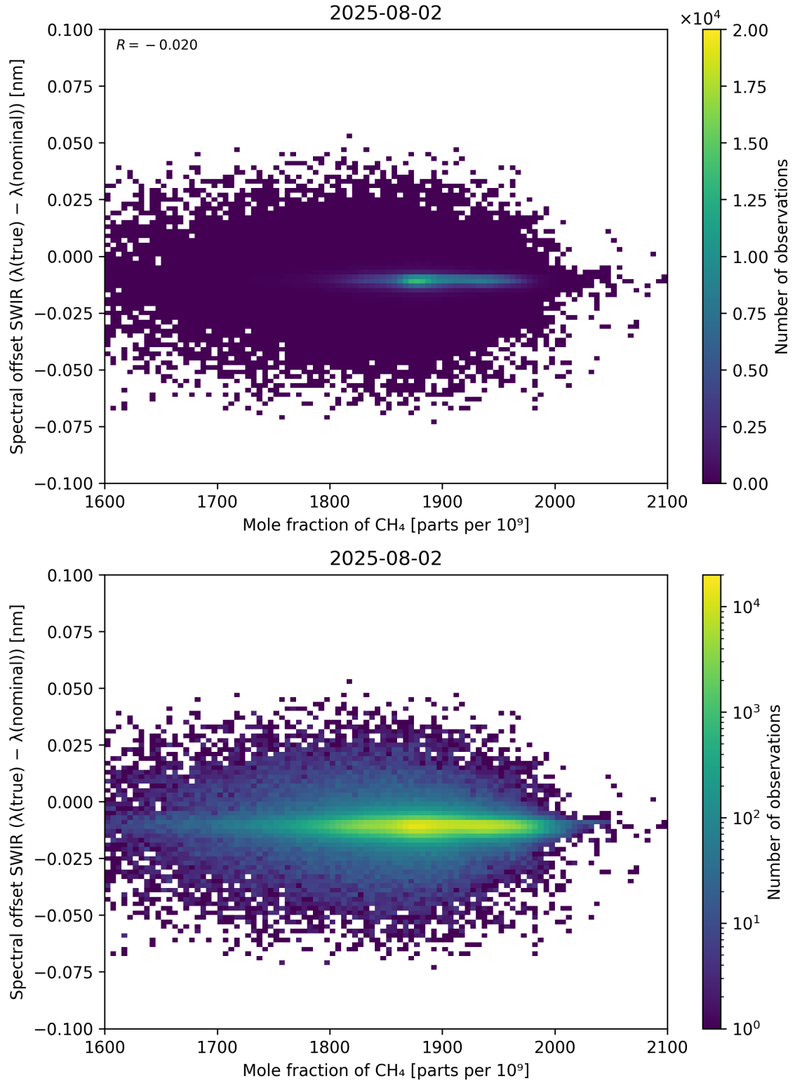
Figure 86: Scatter density plot of “Mole fraction of CH 4 ” against “Spectral offset SWIR ( \lambda_{\text{true}} - \lambda_{\text{nominal}} )” for 2025-08-01 to 2025-08-03.
