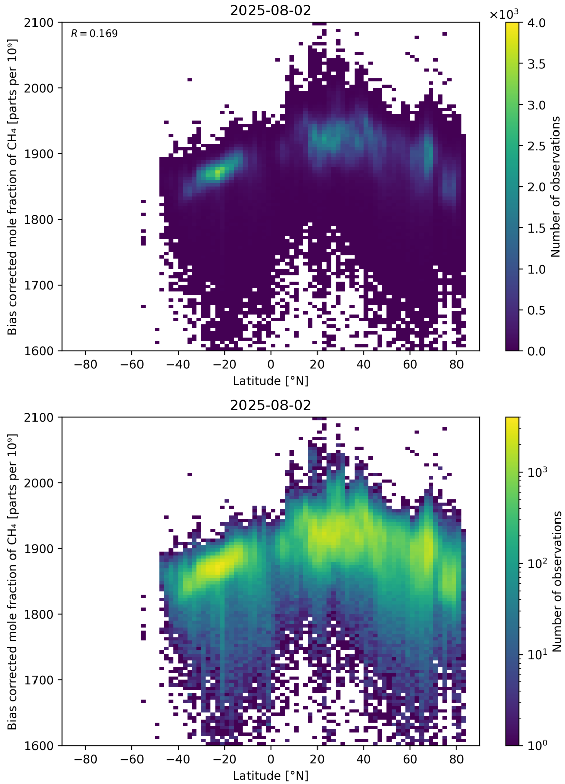
Figure 58: Scatter density plot of “Latitude” against “Bias corrected mole fraction of CH 4 ” for 2025-08-01 to 2025-08-03.
