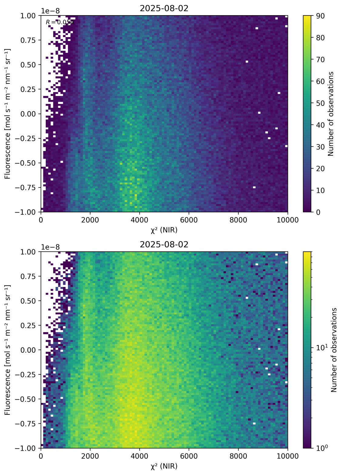
Figure 45: Scatter density plot of “ \chi^2 (NIR)” against “Fluorescence” for 2025-08-01 to 2025-08-03.
