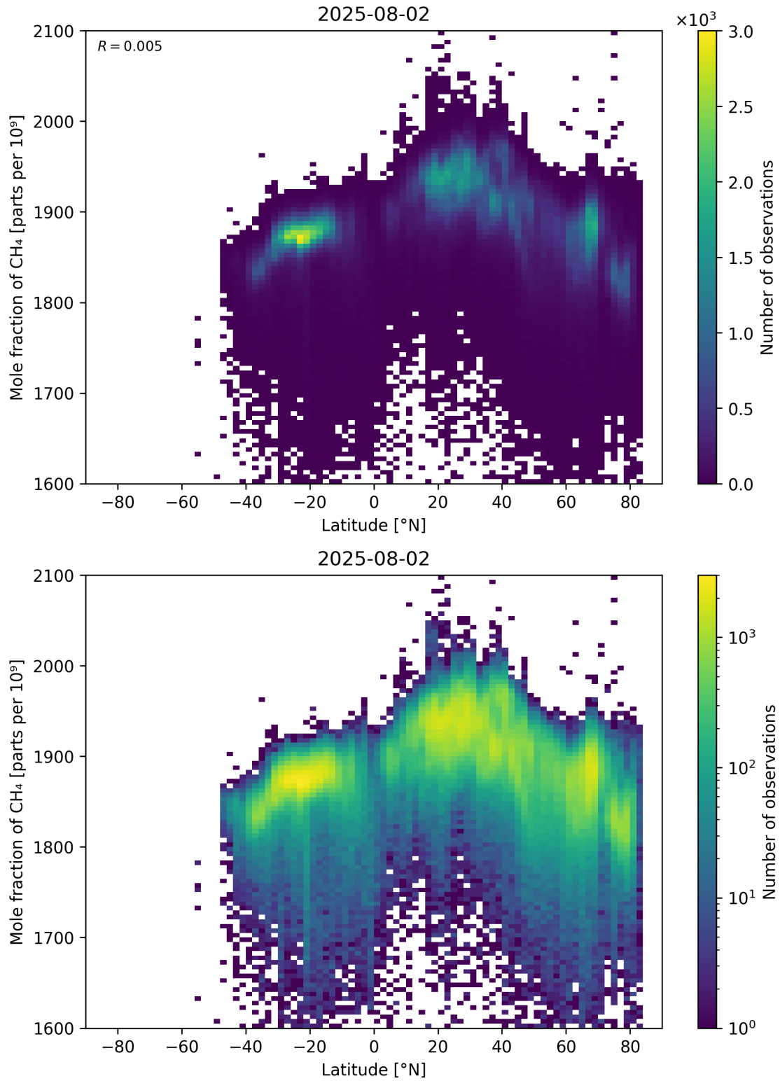
Figure 57: Scatter density plot of “Latitude” against “Mole fraction of \text{CH}_4 ” for 2025-08-01 to 2025-08-03.
