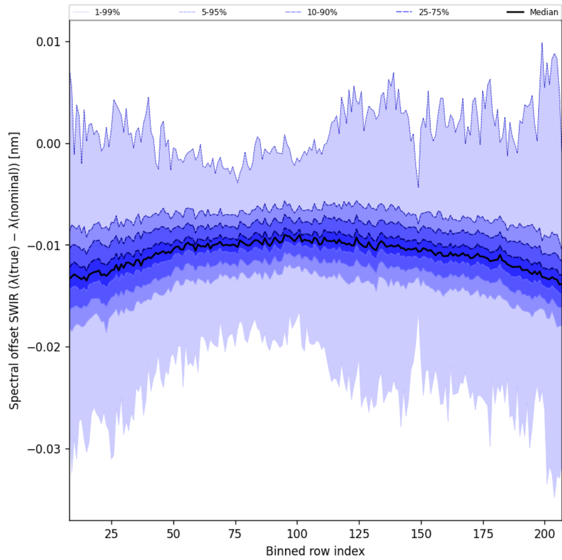
Figure 38: Along track statistics of “Spectral offset SWIR ( \lambda_{\text{true}} - \lambda_{\text{nominal}} )” for 2025-08-01 to 2025-08-03
