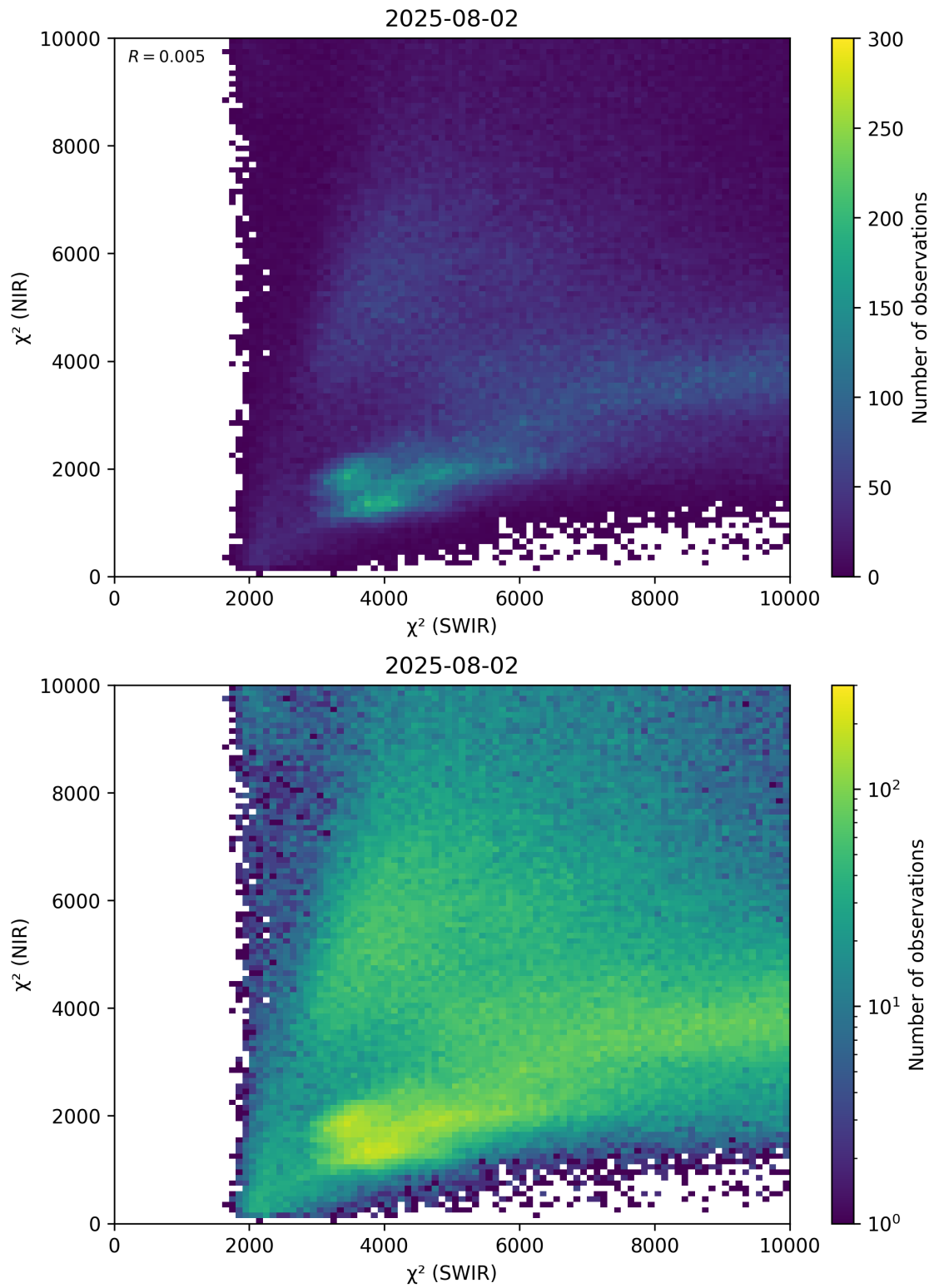
Figure 47: Scatter density plot of “ \chi^2 (SWIR)” against “ \chi^2 (NIR)” for 2025-08-01 to 2025-08-03.
