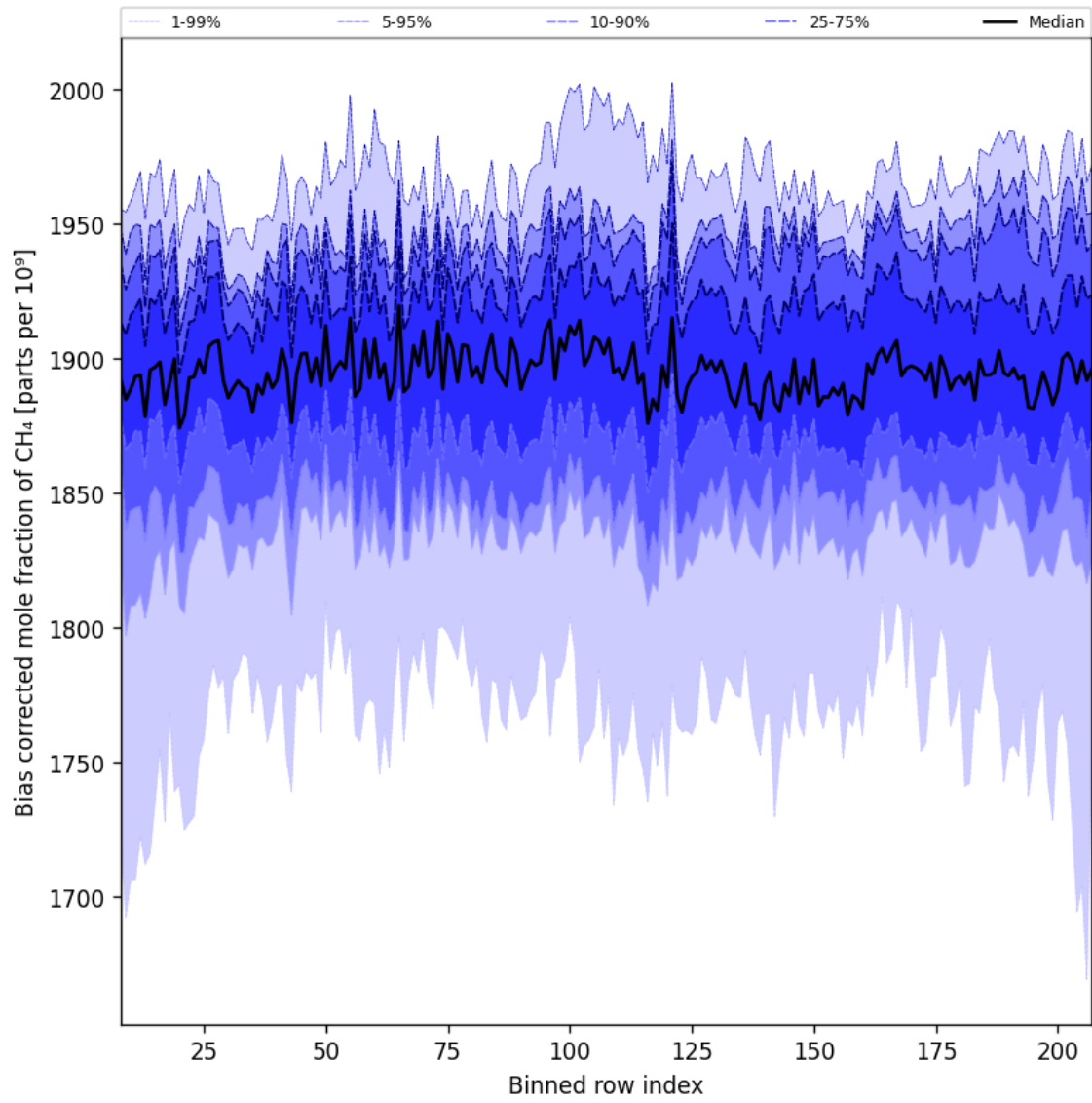
Figure 36: Along track statistics of “Bias corrected mole fraction of CH 4 ” for 2025-08-01 to 2025-08-03
