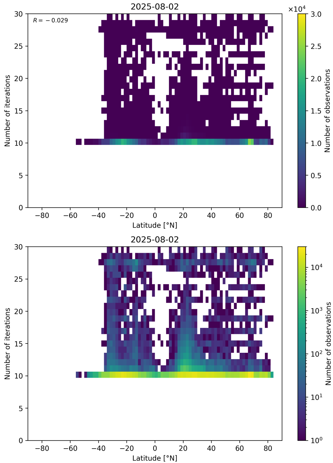
Figure 60: Scatter density plot of “Latitude” against “Number of iterations” for 2025-08-01 to 2025-08-03.
