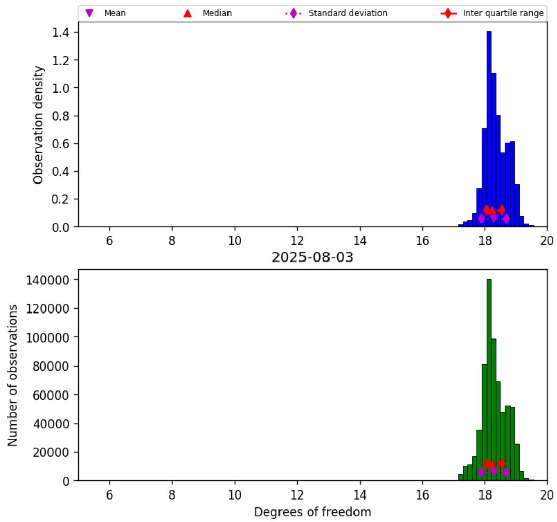
Figure 30: Histogram of “Degrees of freedom” for 2025-08-03 to 2025-08-04
