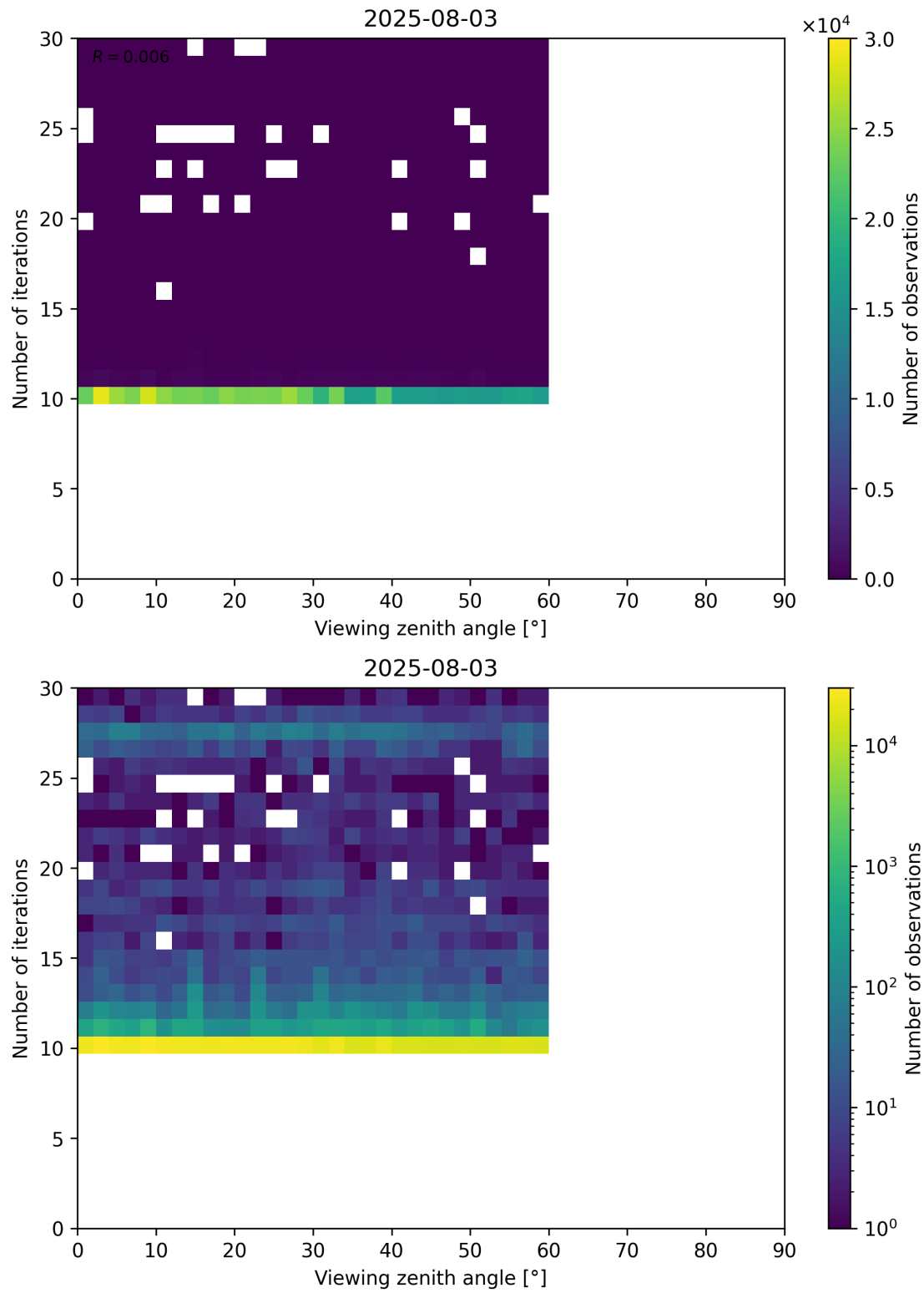
Figure 113: Scatter density plot of “Viewing zenith angle” against “Number of iterations” for 2025-08-03 to 2025-08-04.
