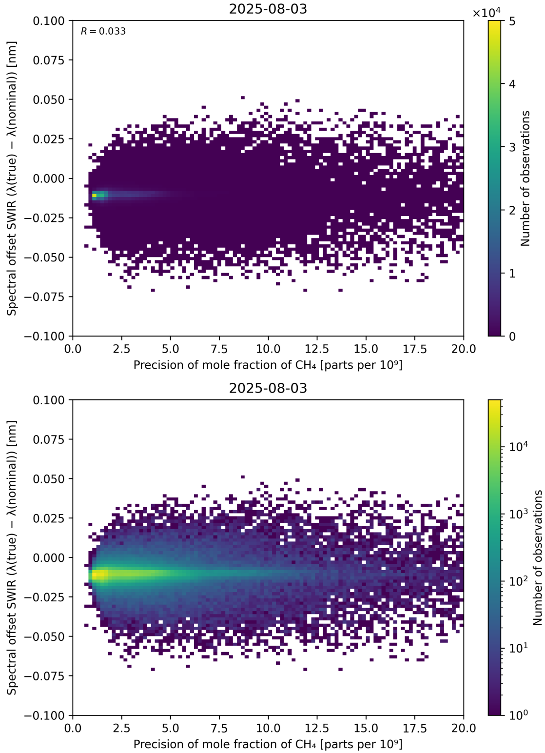
Figure 85: Scatter density plot of “Precision of mole fraction of CH 4 ” against “Spectral offset SWIR ( \lambda_{\text{true}} - \lambda_{\text{nominal}} )” for 2025-08-03 to 2025-08-04.
