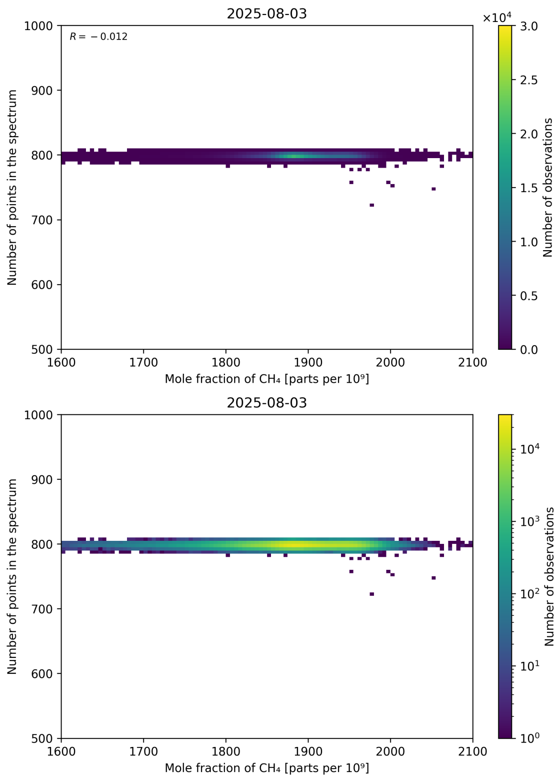
Figure 77: Scatter density plot of “Mole fraction of CH 4 ” against “Number of points in the spectrum” for 2025-08-03 to 2025-08-04.
