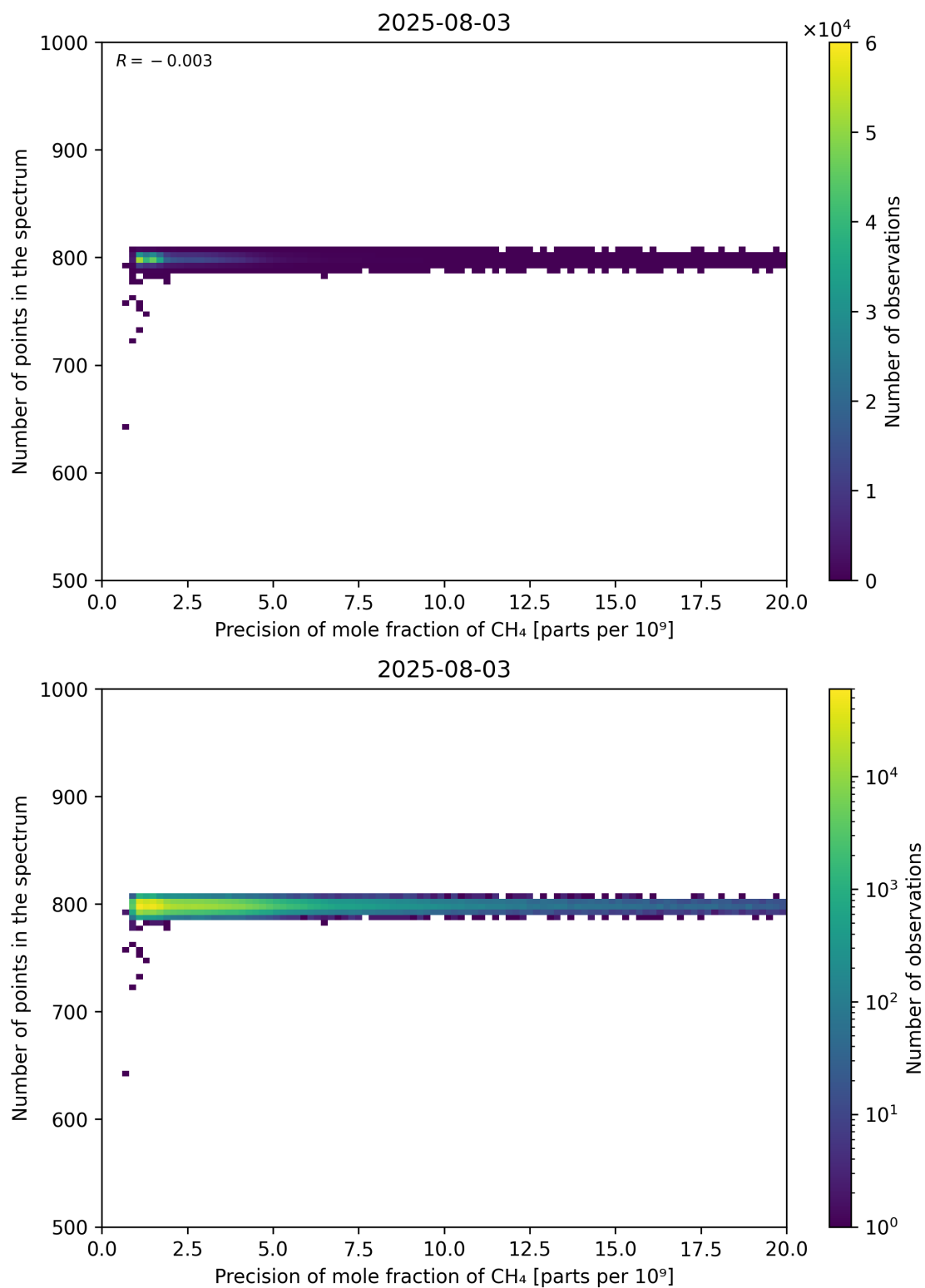
Figure 84: Scatter density plot of “Precision of mole fraction of CH 4 ” against “Number of points in the spectrum” for 2025-08-03 to 2025-08-04.
