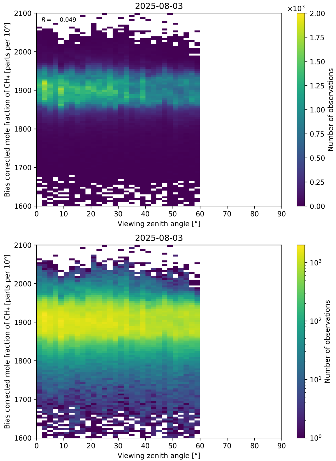
Figure 111: Scatter density plot of “Viewing zenith angle” against “Bias corrected mole fraction of CH 4 ” for 2025-08-03 to 2025-08-04.
