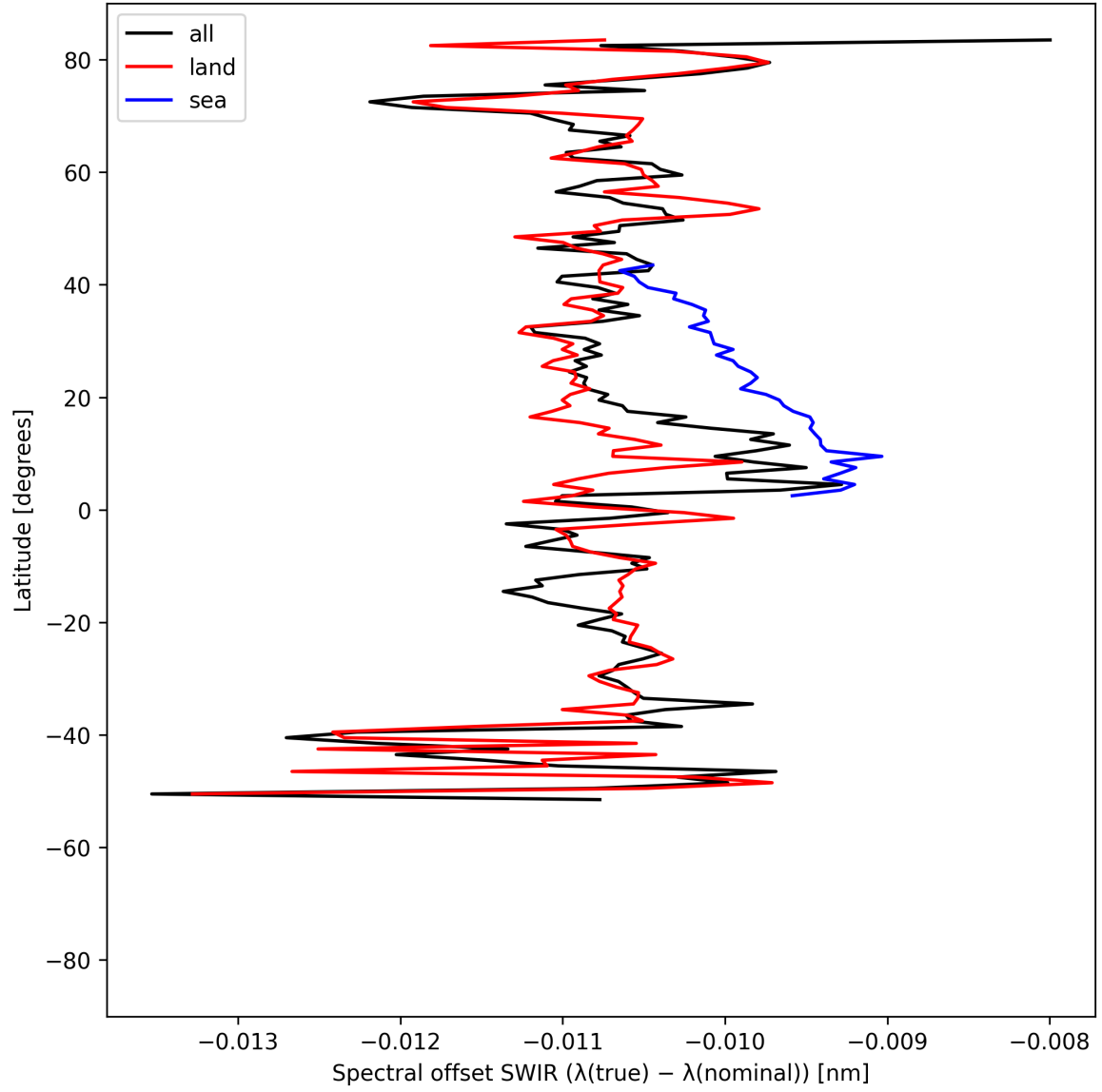
Figure 16: Zonal average of “Spectral offset SWIR ( \lambda_{\text{true}} - \lambda_{\text{nominal}} )” for 2025-08-03 to 2025-08-04.
