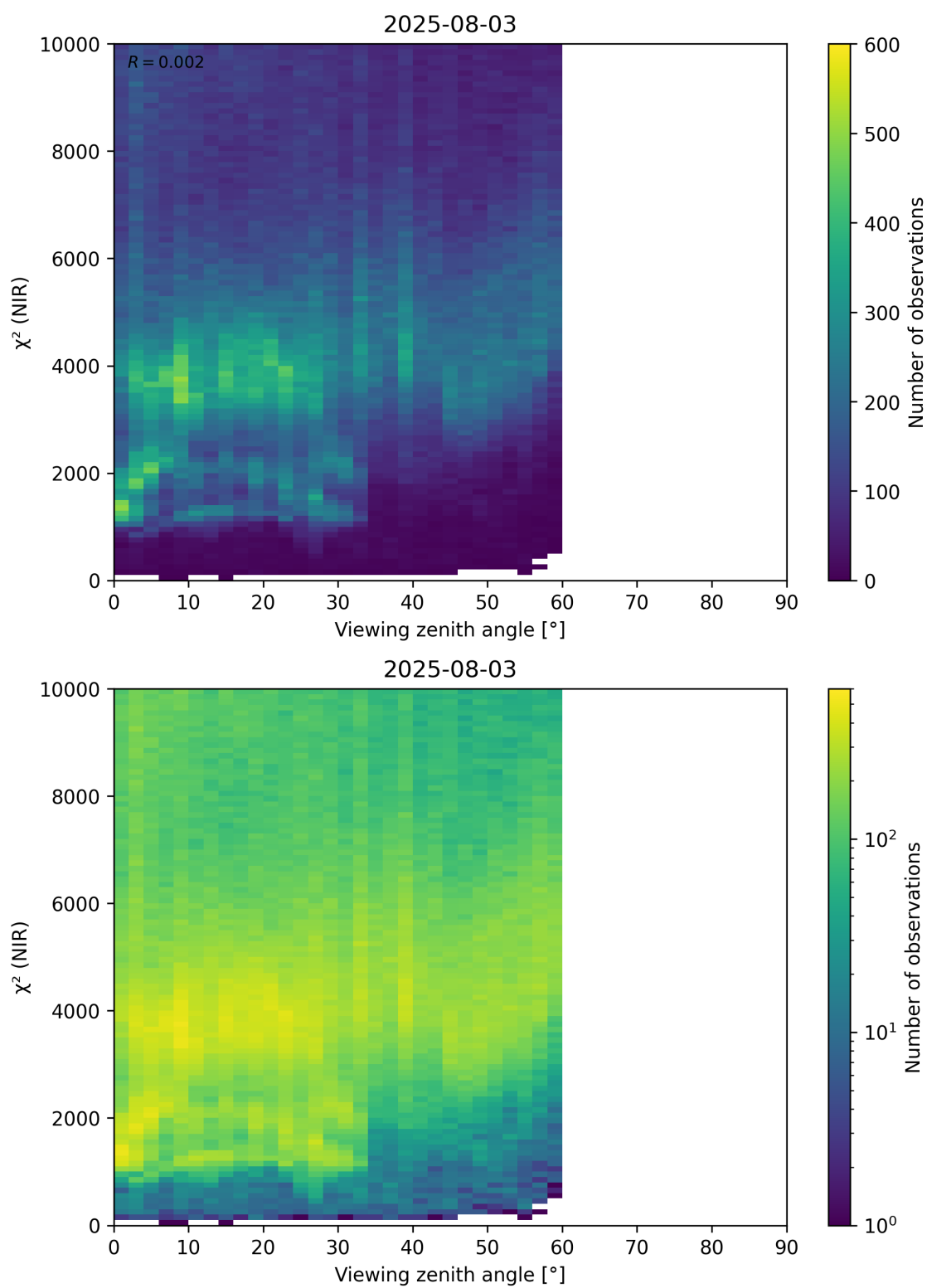
Figure 105: Scatter density plot of “Viewing zenith angle” against “ \chi^2 (NIR)” for 2025-08-03 to 2025-08-04.
