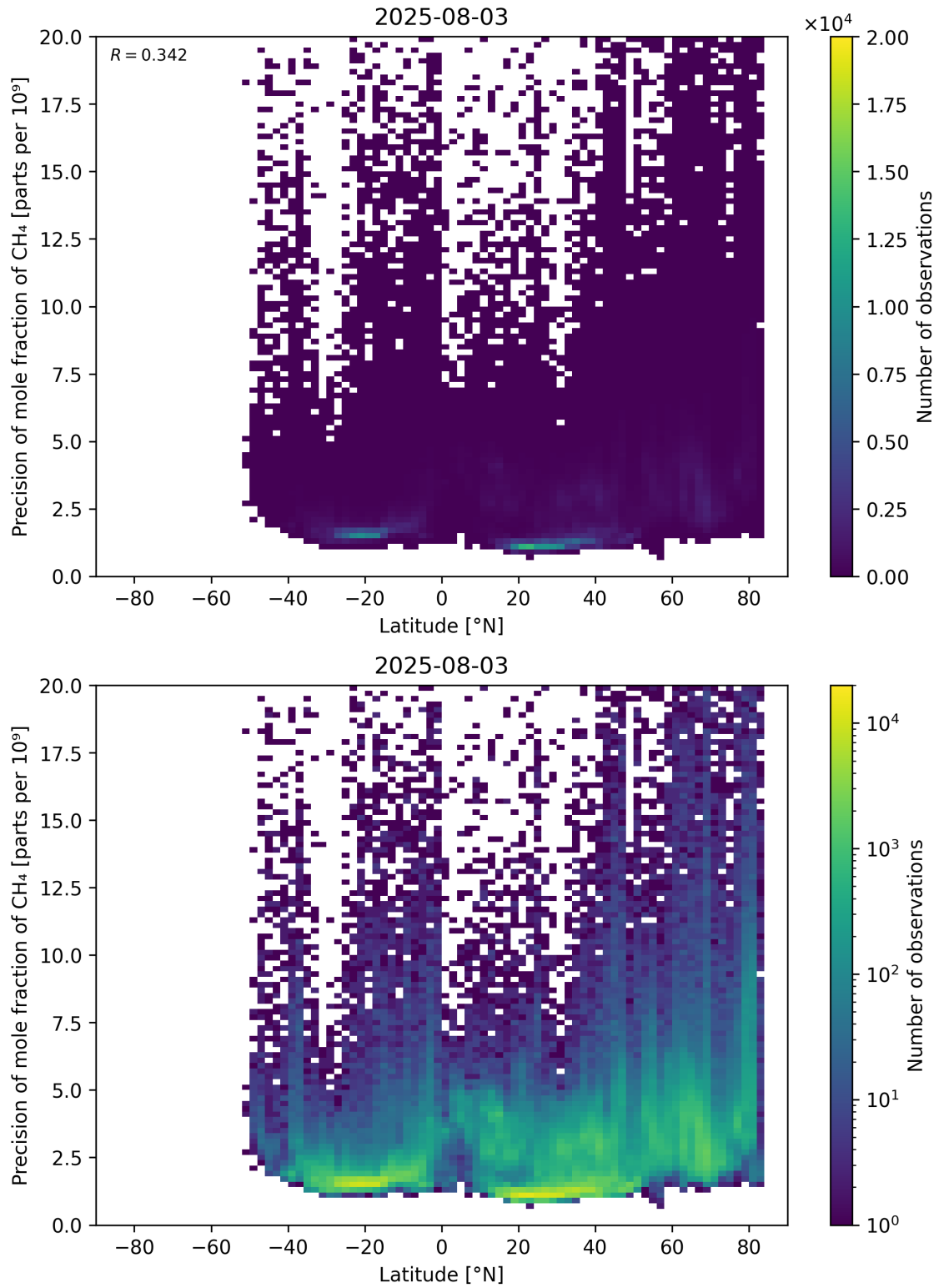
Figure 59: Scatter density plot of “Latitude” against “Precision of mole fraction of \text{CH}_4 ” for 2025-08-03 to 2025-08-04.
