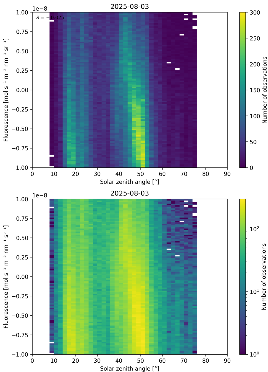
Figure 97: Scatter density plot of “Solar zenith angle” against “Fluorescence” for 2025-08-03 to 2025-08-04.
