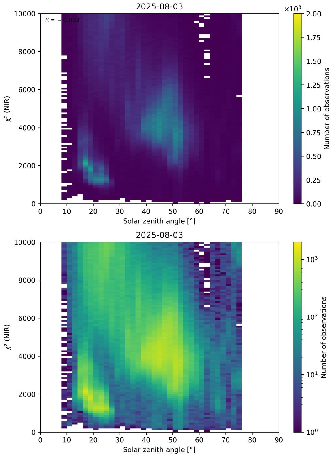
Figure 94: Scatter density plot of “Solar zenith angle” against “ \chi^2 (NIR)” for 2025-08-03 to 2025-08-04.
