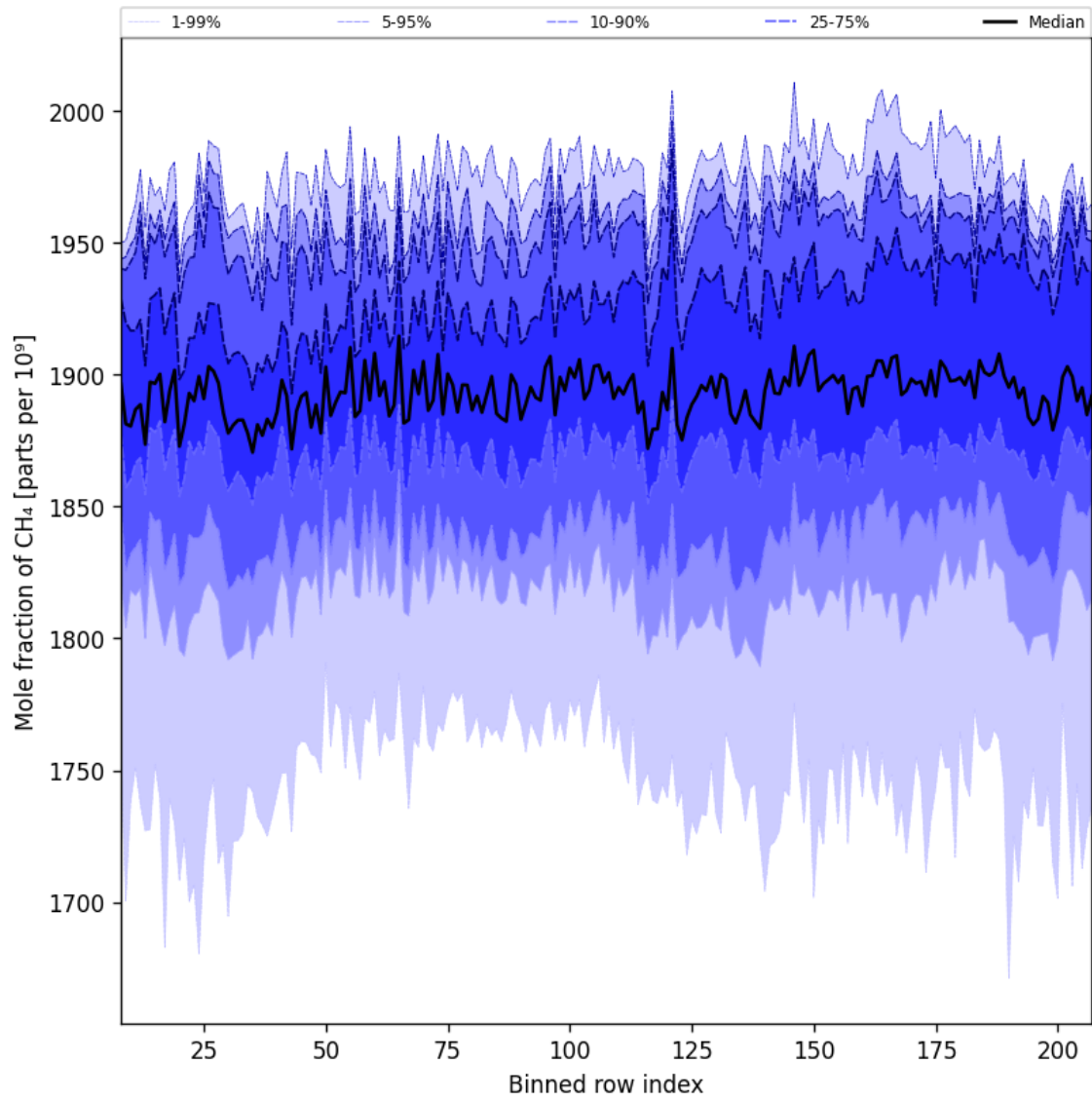
Figure 34: Along track statistics of “Mole fraction of CH 4 ” for 2025-08-03 to 2025-08-04
