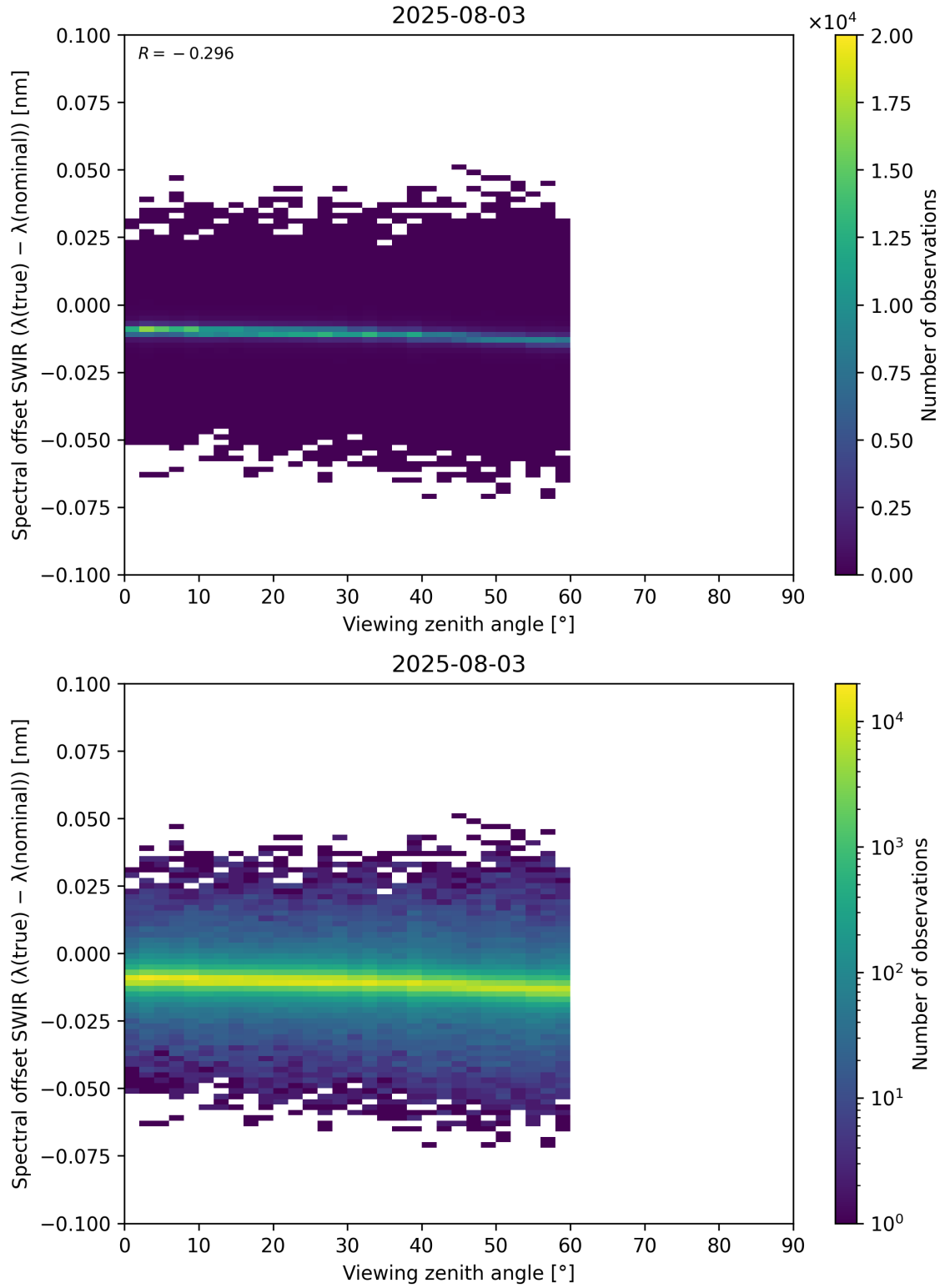
Figure 116: Scatter density plot of “Viewing zenith angle” against “Spectral offset SWIR ( \lambda_{\text{true}} - \lambda_{\text{nominal}} )” for 2025-08-03 to 2025-08-04.
