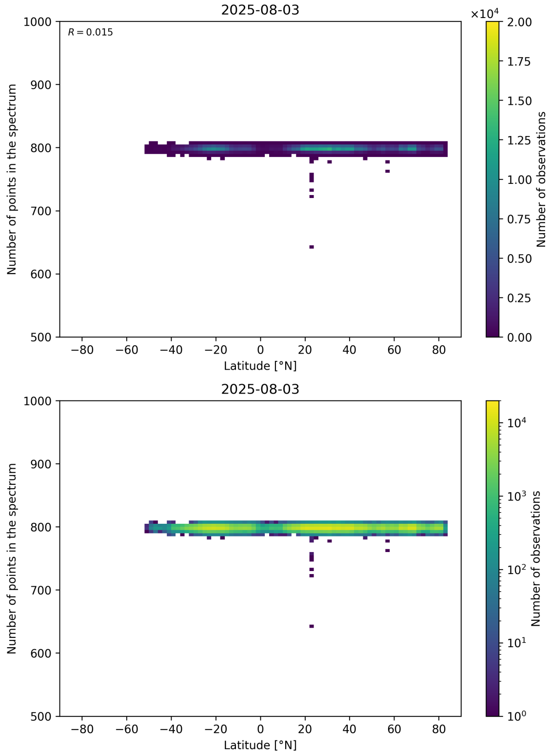
Figure 61: Scatter density plot of “Latitude” against “Number of points in the spectrum” for 2025-08-03 to 2025-08-04.
