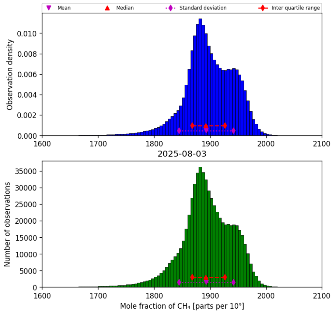
Figure 23: Histogram of “Mole fraction of CH 4 ” for 2025-08-03 to 2025-08-04
