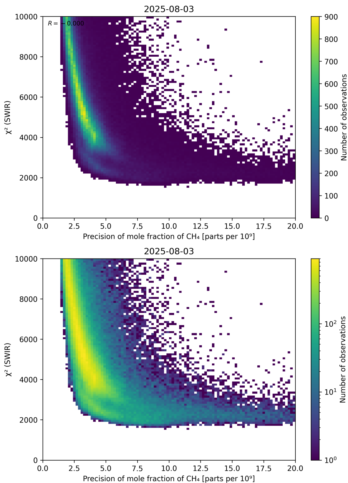
Figure 79: Scatter density plot of “Precision of mole fraction of CH 4 ” against “ \chi^2 (SWIR)” for 2025-08-03 to 2025-08-04.
