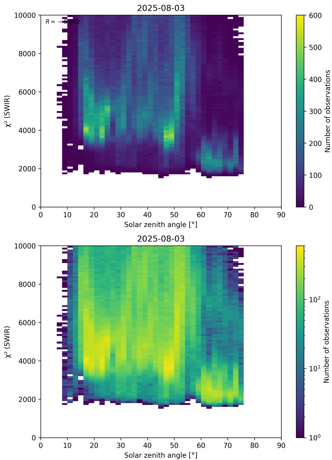
Figure 95: Scatter density plot of “Solar zenith angle” against “ \chi^2 (SWIR)” for 2025-08-03 to 2025-08-04.
