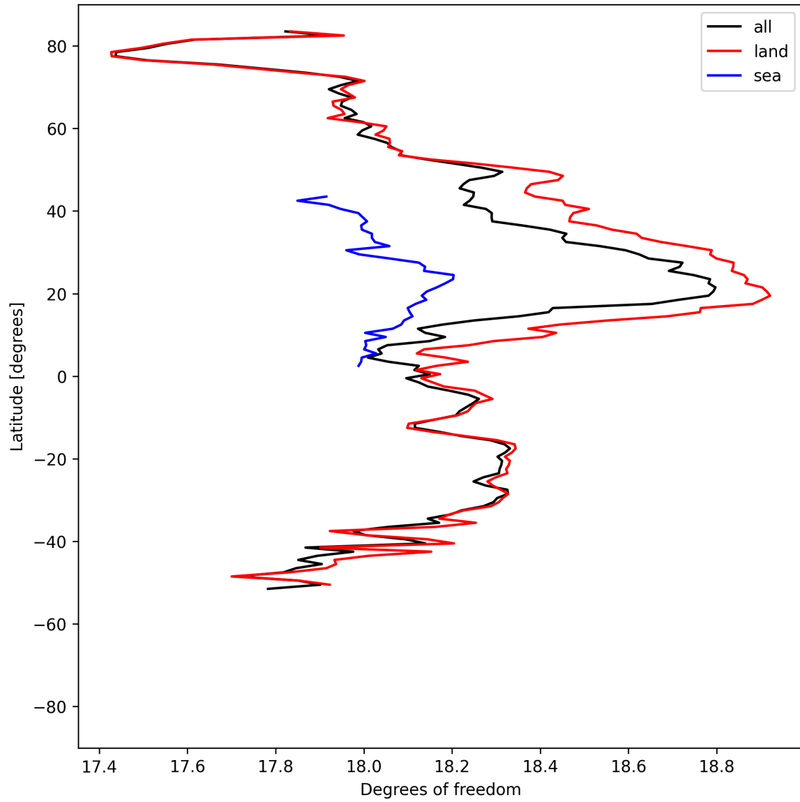
Figure 19: Zonal average of “Degrees of freedom” for 2025-08-03 to 2025-08-04.
