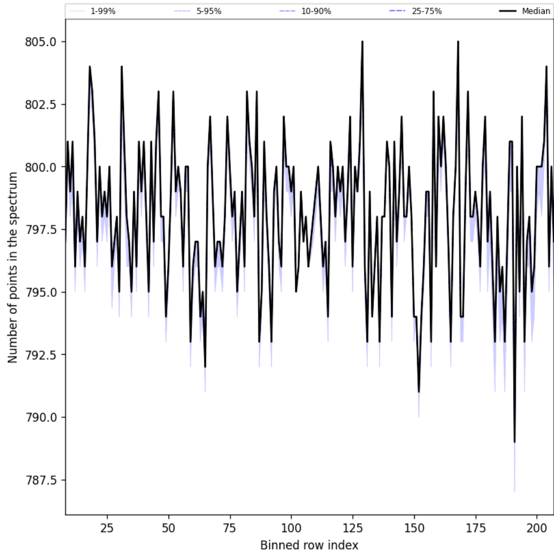
Figure 37: Along track statistics of “Number of points in the spectrum” for 2025-08-03 to 2025-08-04
