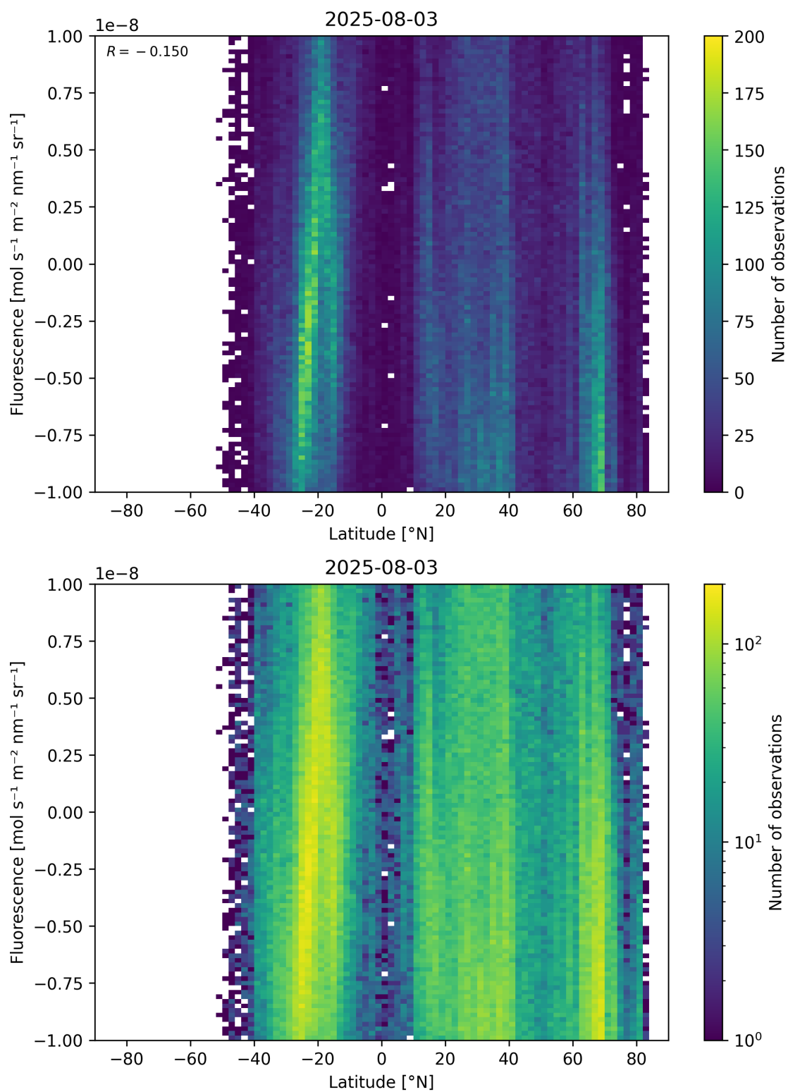
Figure 56: Scatter density plot of “Latitude” against “Fluorescence” for 2025-08-03 to 2025-08-04.
