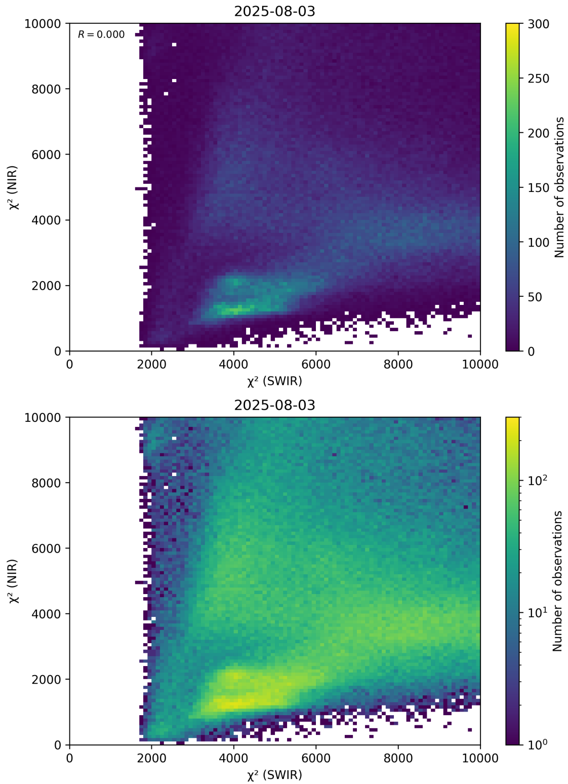
Figure 47: Scatter density plot of “ \chi^2 (SWIR)” against “ \chi^2 (NIR)” for 2025-08-03 to 2025-08-04.
