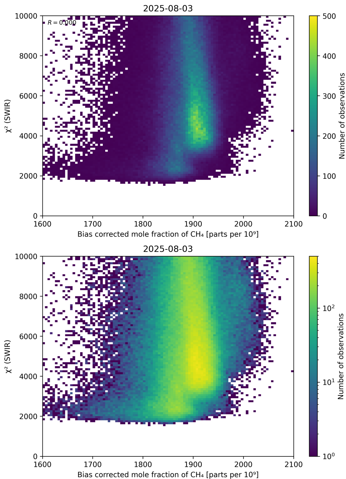
Figure 64: Scatter density plot of “Bias corrected mole fraction of \text{CH}_4 ” against “ \chi^2 (SWIR)” for 2025-08-03 to 2025-08-04.
