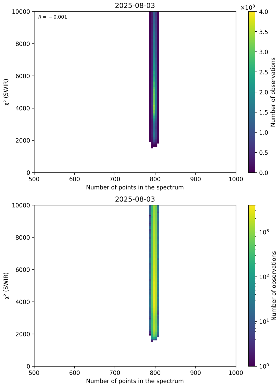
Figure 89: Scatter density plot of “Number of points in the spectrum” against “ \chi^2 (SWIR)” for 2025-08-03 to 2025-08-04.
