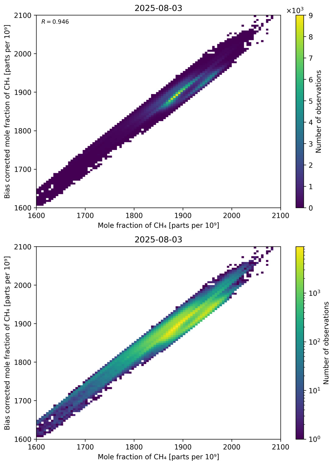
Figure 74: Scatter density plot of “Mole fraction of CH 4 ” against “Bias corrected mole fraction of CH 4 ” for 2025-08-03 to 2025-08-04.
