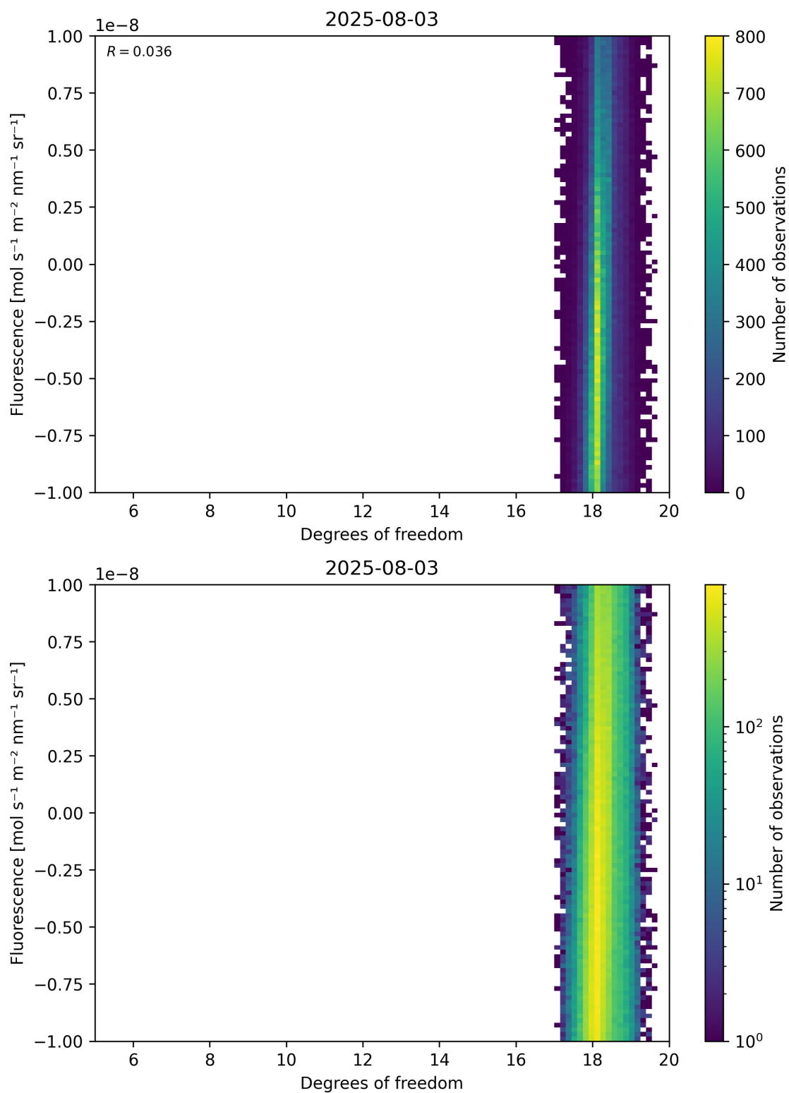
Figure 51: Scatter density plot of “Degrees of freedom” against “Fluorescence” for 2025-08-03 to 2025-08-04.
