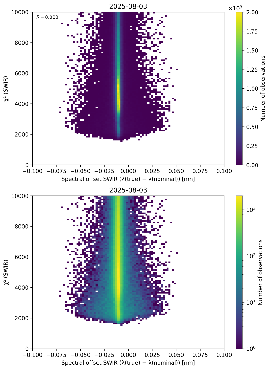
Figure 118: Scatter density plot of “Spectral offset SWIR ( \lambda_{\text{true}} - \lambda_{\text{nominal}} )” against “ \chi^2 (SWIR)” for 2025-08-03 to 2025-08-04.
