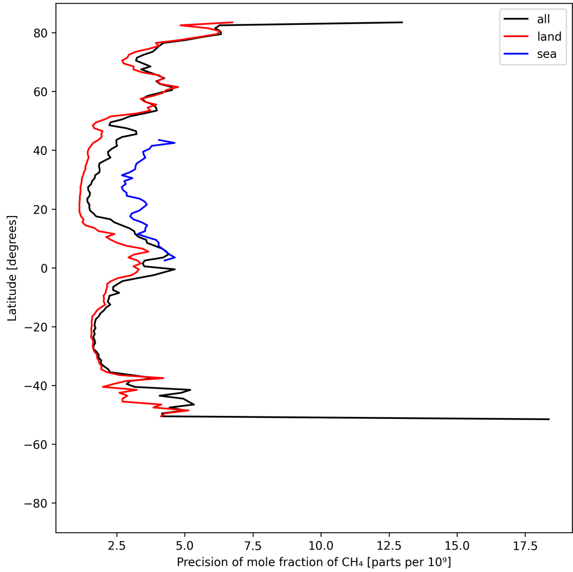
Figure 13: Zonal average of “Precision of mole fraction of CH 4 ” for 2025-08-03 to 2025-08-04.
