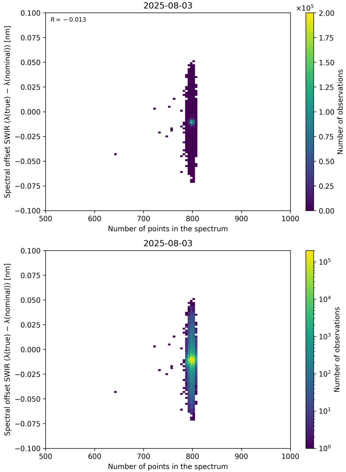
Figure 93: Scatter density plot of “Number of points in the spectrum” against “Spectral offset SWIR ( \lambda_{\text{true}} - \lambda_{\text{nominal}} )” for 2025-08-03 to 2025-08-04.
