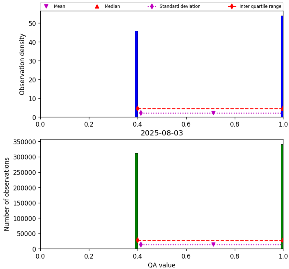
Figure 22: Histogram of “QA value” for 2025-08-03 to 2025-08-04
