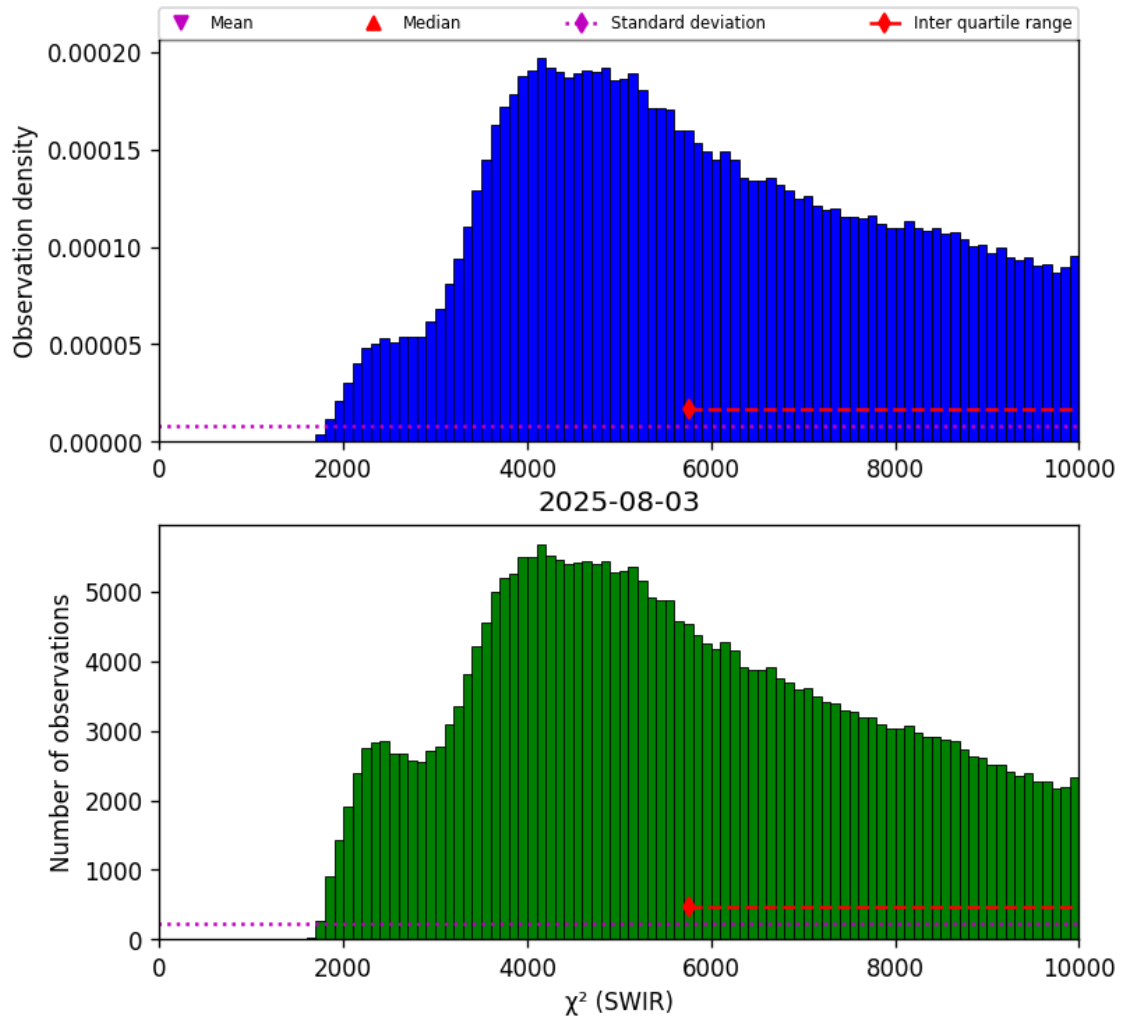
Figure 28: Histogram of " \chi^2 (SWIR)" for 2025-08-03 to 2025-08-04
