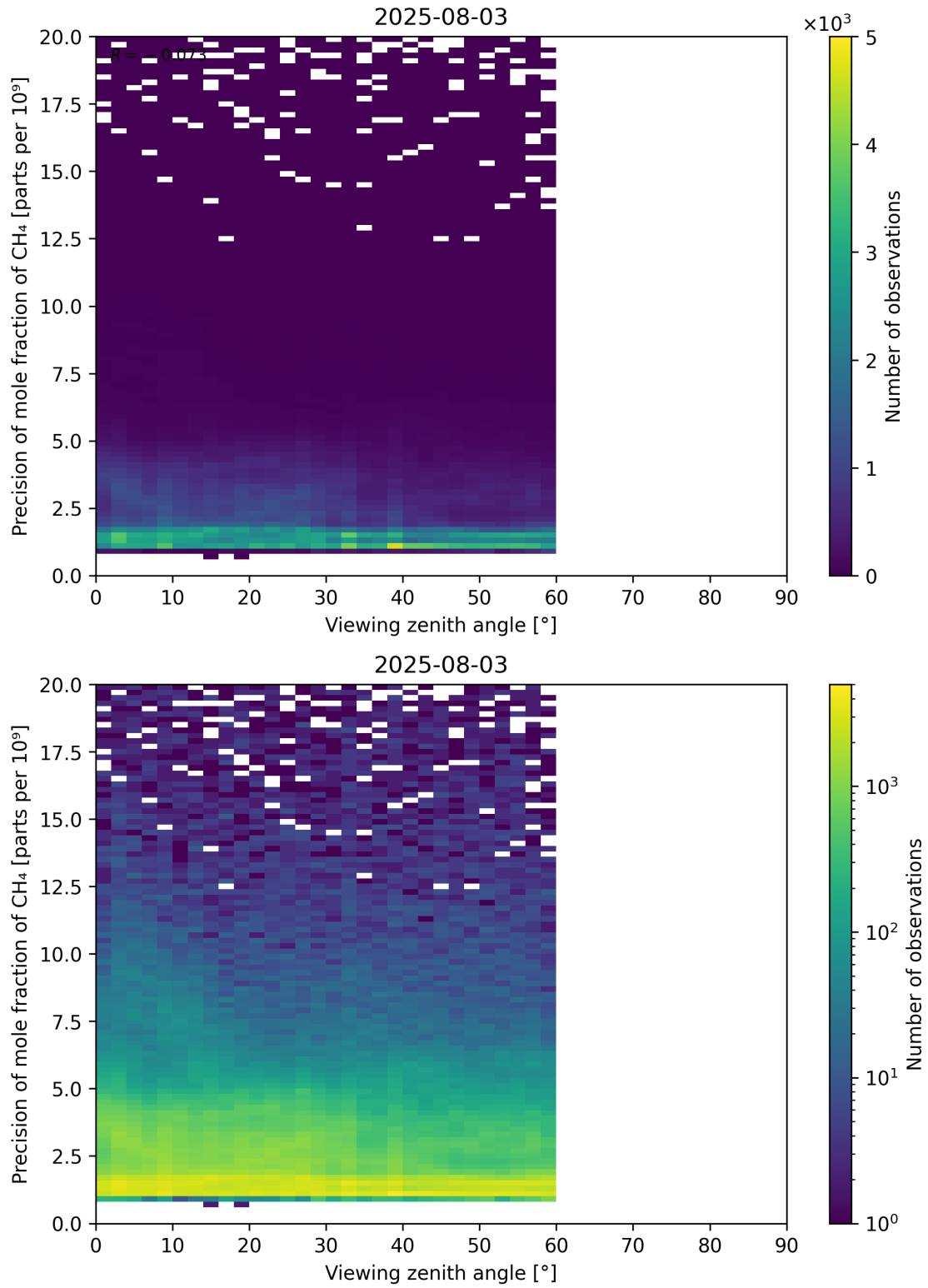
Figure 112: Scatter density plot of “Viewing zenith angle” against “Precision of mole fraction of CH 4 ” for 2025-08-03 to 2025-08-04.
