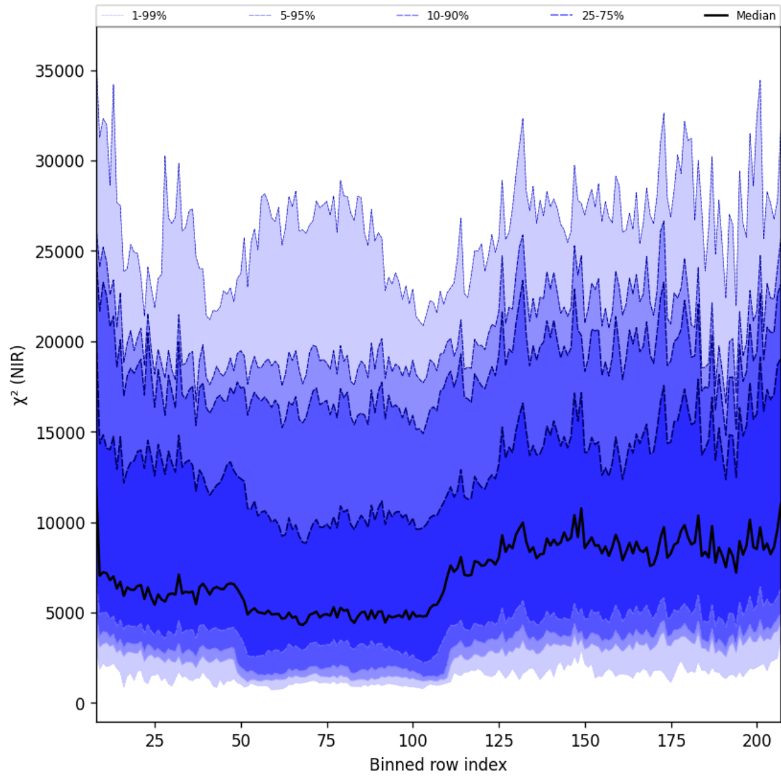
Figure 40: Along track statistics of “ \chi^2 (NIR)” for 2025-08-03 to 2025-08-04
