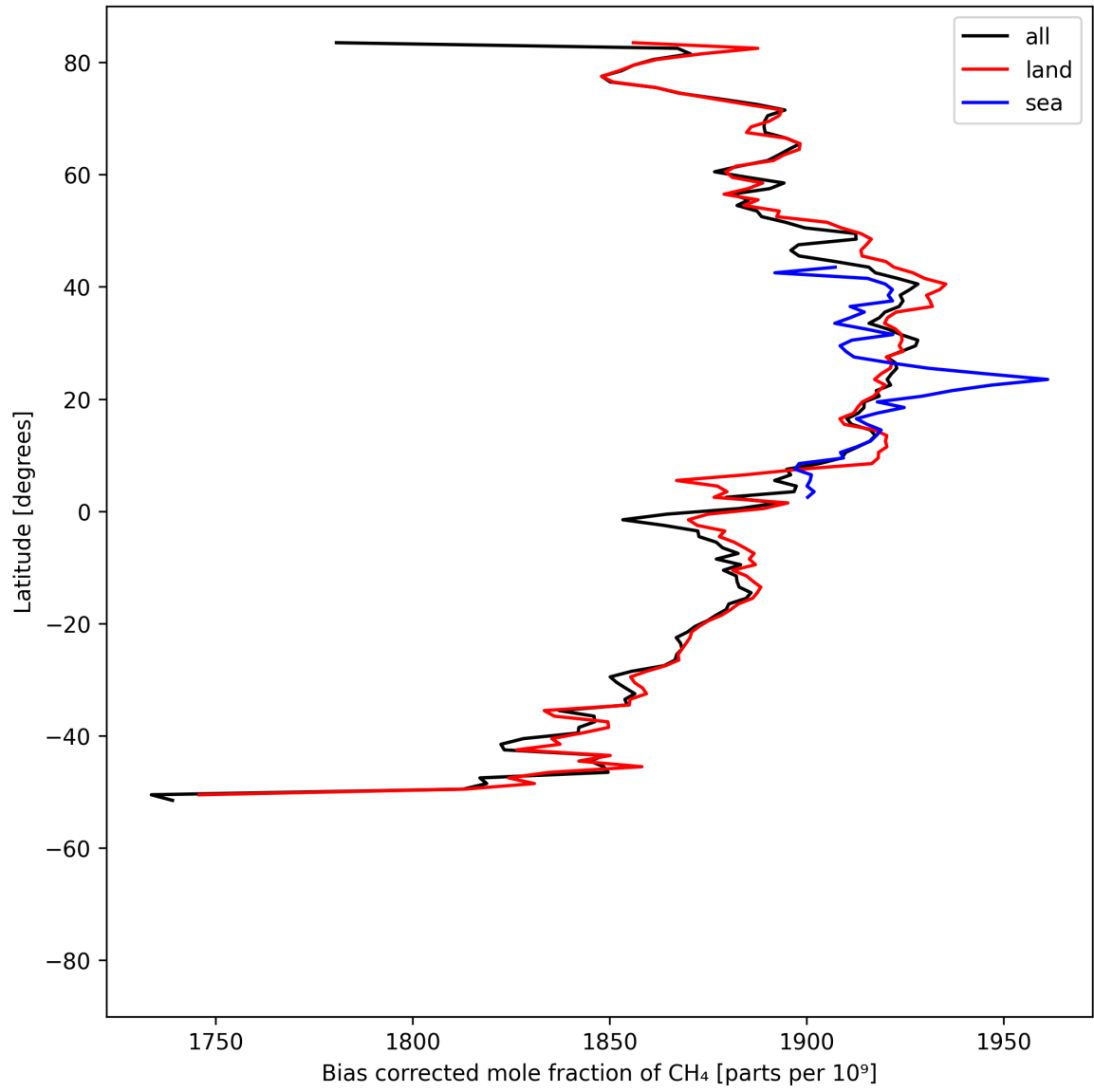
Figure 14: Zonal average of “Bias corrected mole fraction of CH 4 ” for 2025-08-03 to 2025-08-04.
