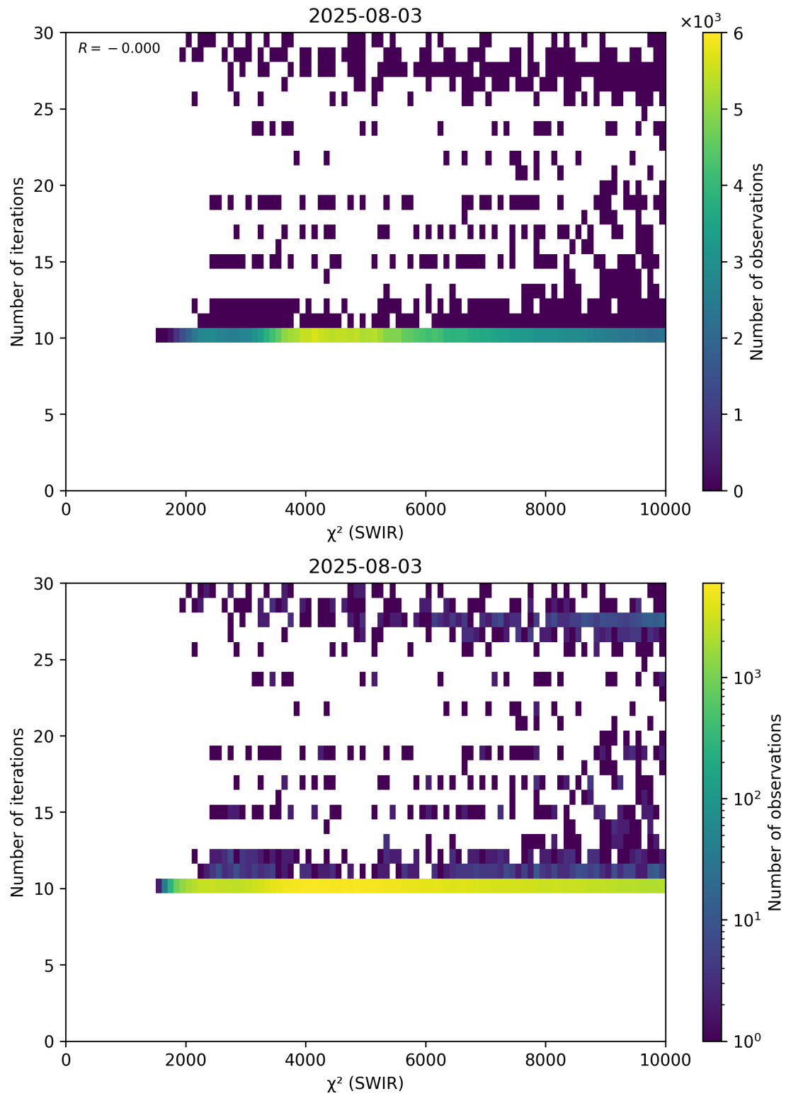
Figure 50: Scatter density plot of " \chi^2 (SWIR)" against "Number of iterations" for 2025-08-03 to 2025-08-04.
