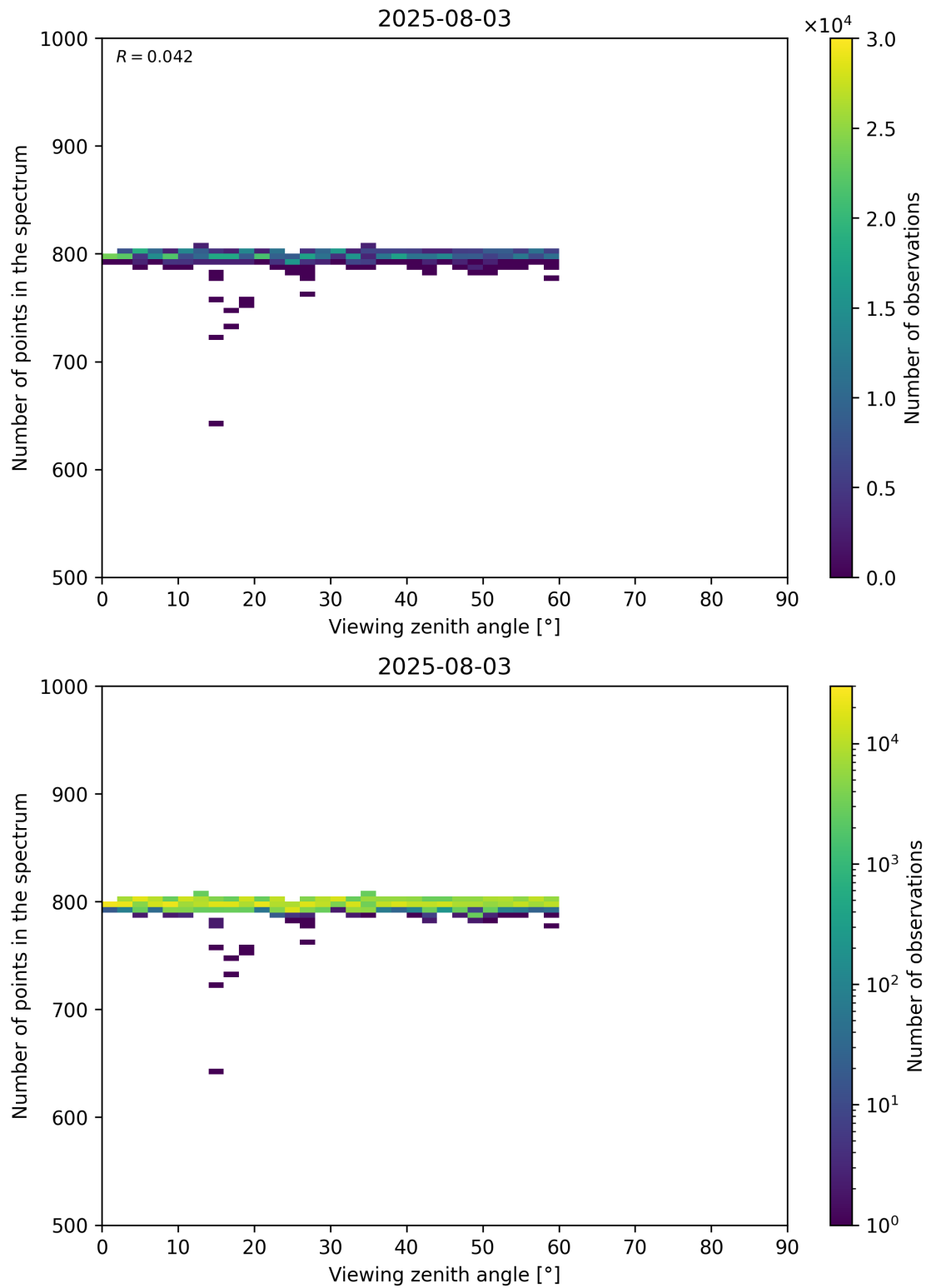
Figure 114: Scatter density plot of “Viewing zenith angle” against “Number of points in the spectrum” for 2025-08-03 to 2025-08-04.
