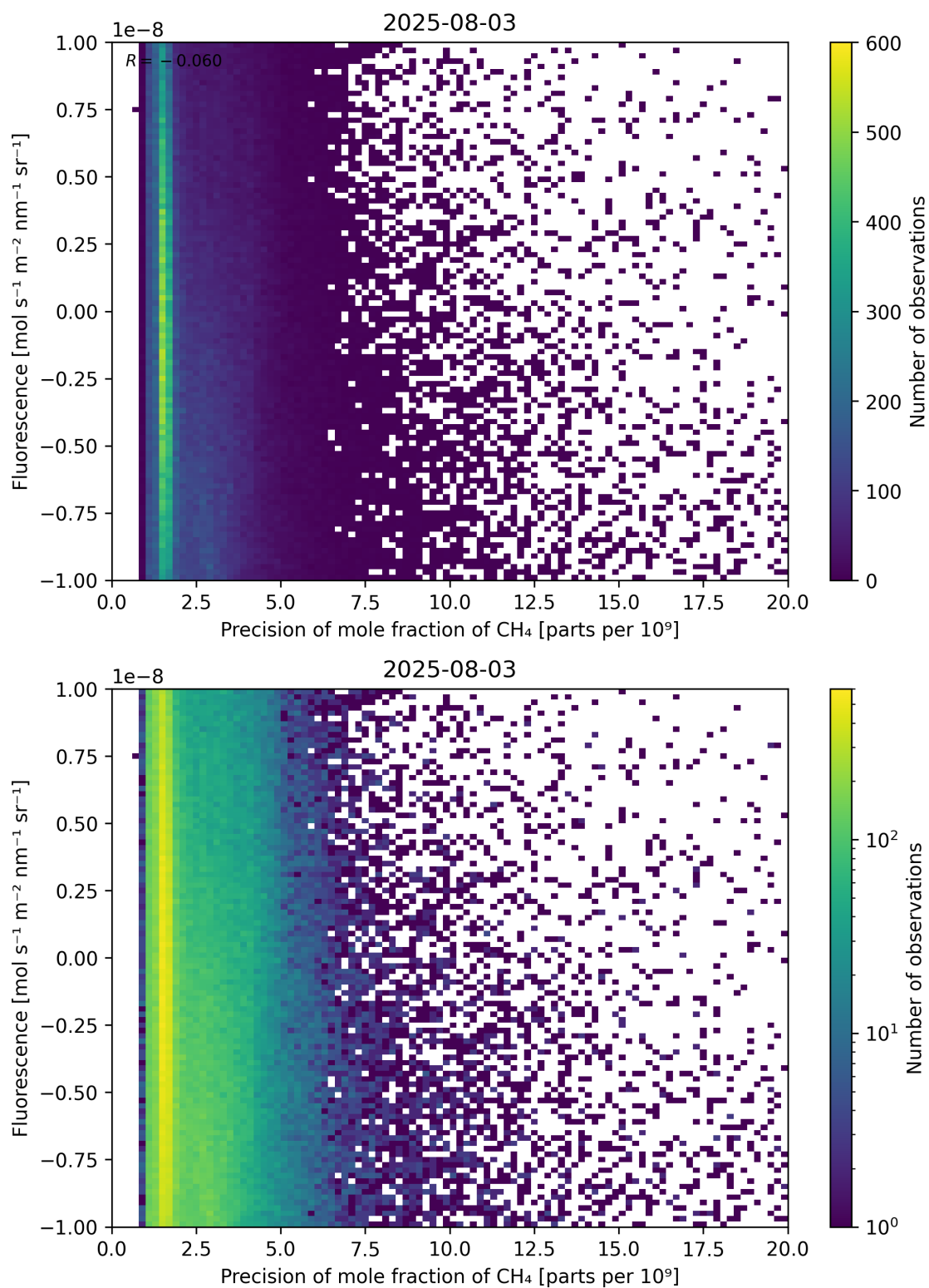
Figure 81: Scatter density plot of “Precision of mole fraction of CH 4 ” against “Fluorescence” for 2025-08-03 to 2025-08-04.
