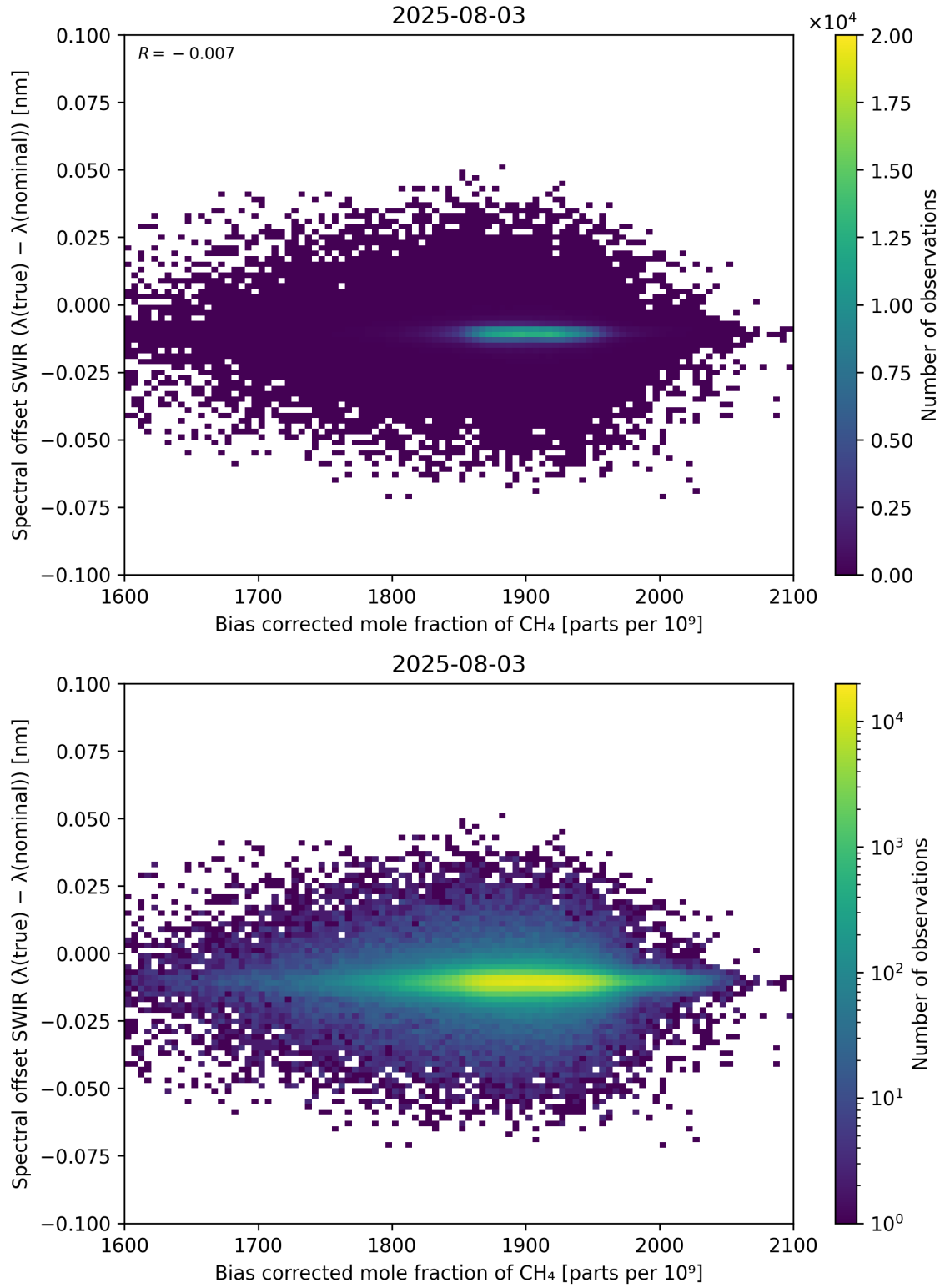
Figure 69: Scatter density plot of “Bias corrected mole fraction of \text{CH}_4 ” against “Spectral offset SWIR ( \lambda_{\text{true}} - \lambda_{\text{nominal}} )” for 2025-08-03 to 2025-08-04.
