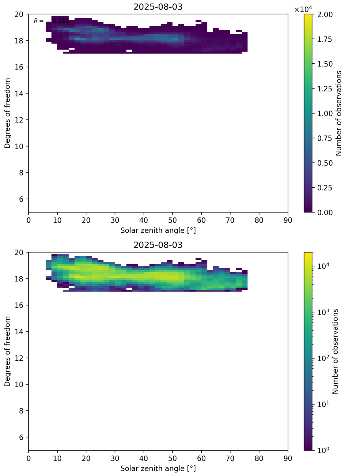
Figure 96: Scatter density plot of “Solar zenith angle” against “Degrees of freedom” for 2025-08-03 to 2025-08-04.
