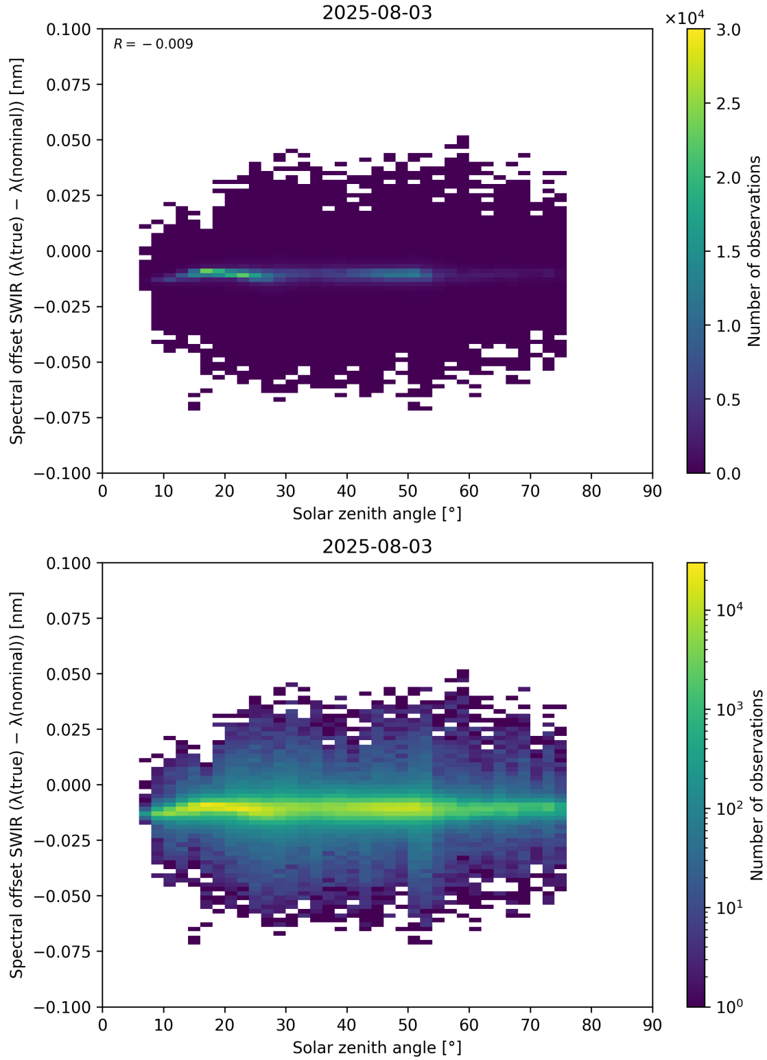
Figure 104: Scatter density plot of “Solar zenith angle” against “Spectral offset SWIR ( \lambda_{\text{true}} - \lambda_{\text{nominal}} )” for 2025-08-03 to 2025-08-04.
