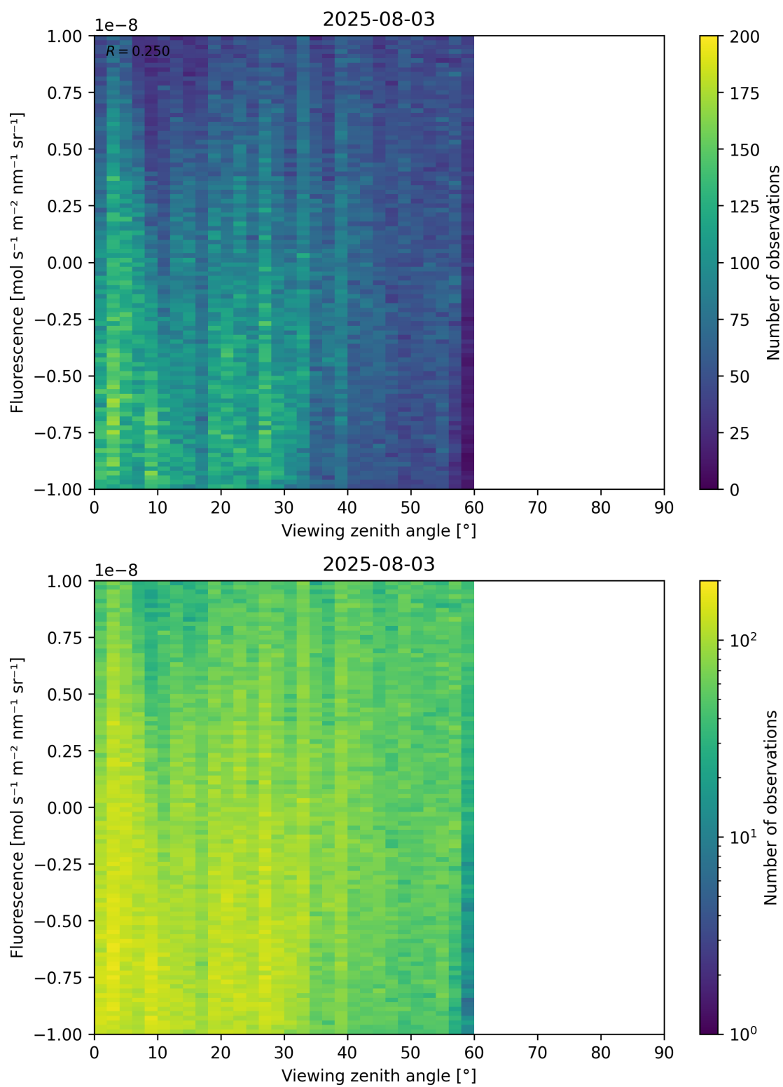
Figure 108: Scatter density plot of “Viewing zenith angle” against “Fluorescence” for 2025-08-03 to 2025-08-04.
