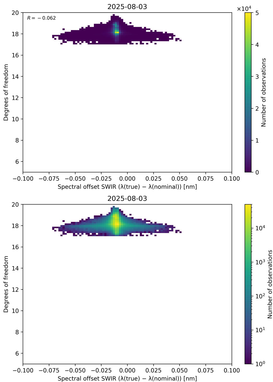
Figure 119: Scatter density plot of “Spectral offset SWIR ( \lambda_{\text{true}} - \lambda_{\text{nominal}} )” against “Degrees of freedom” for 2025-08-03 to 2025-08-04.
