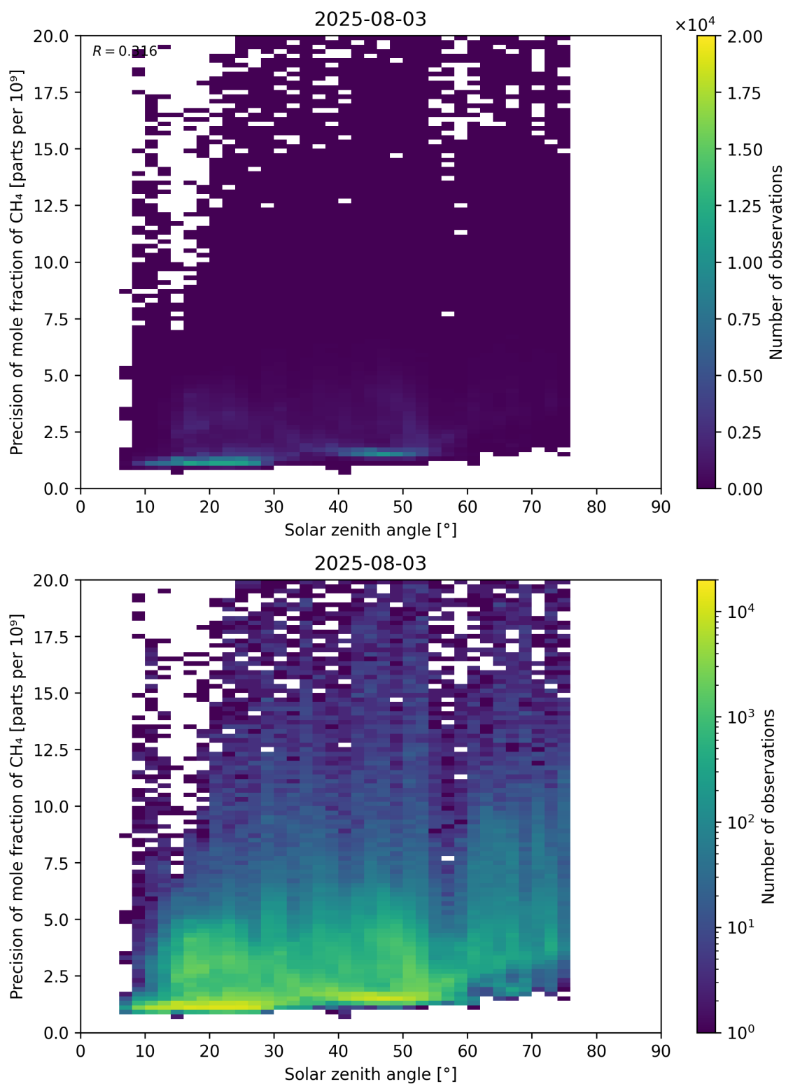
Figure 101: Scatter density plot of “Solar zenith angle” against “Precision of mole fraction of CH 4 ” for 2025-08-03 to 2025-08-04.
