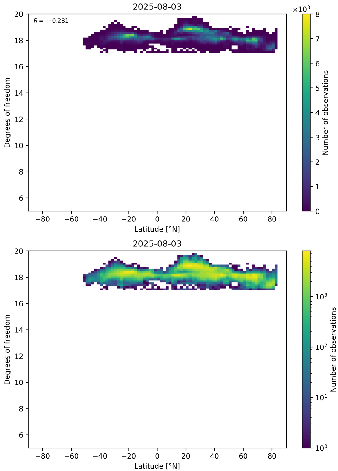
Figure 55: Scatter density plot of “Latitude” against “Degrees of freedom” for 2025-08-03 to 2025-08-04.
