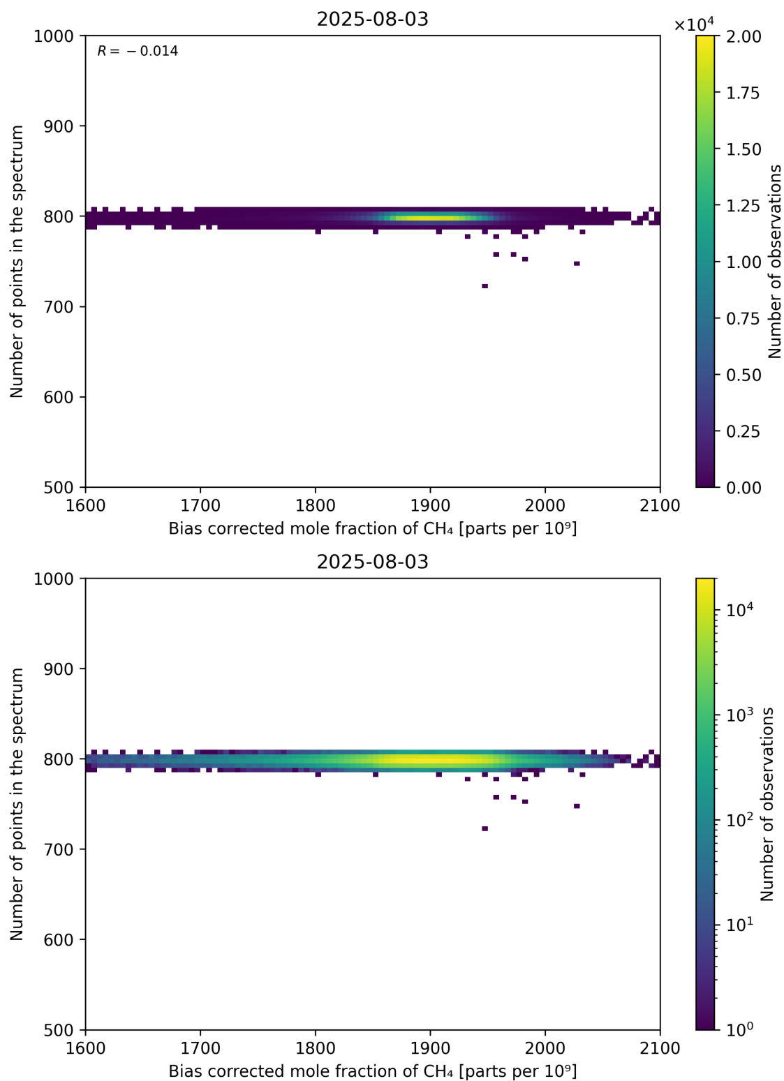
Figure 68: Scatter density plot of “Bias corrected mole fraction of CH 4 ” against “Number of points in the spectrum” for 2025-08-03 to 2025-08-04.
