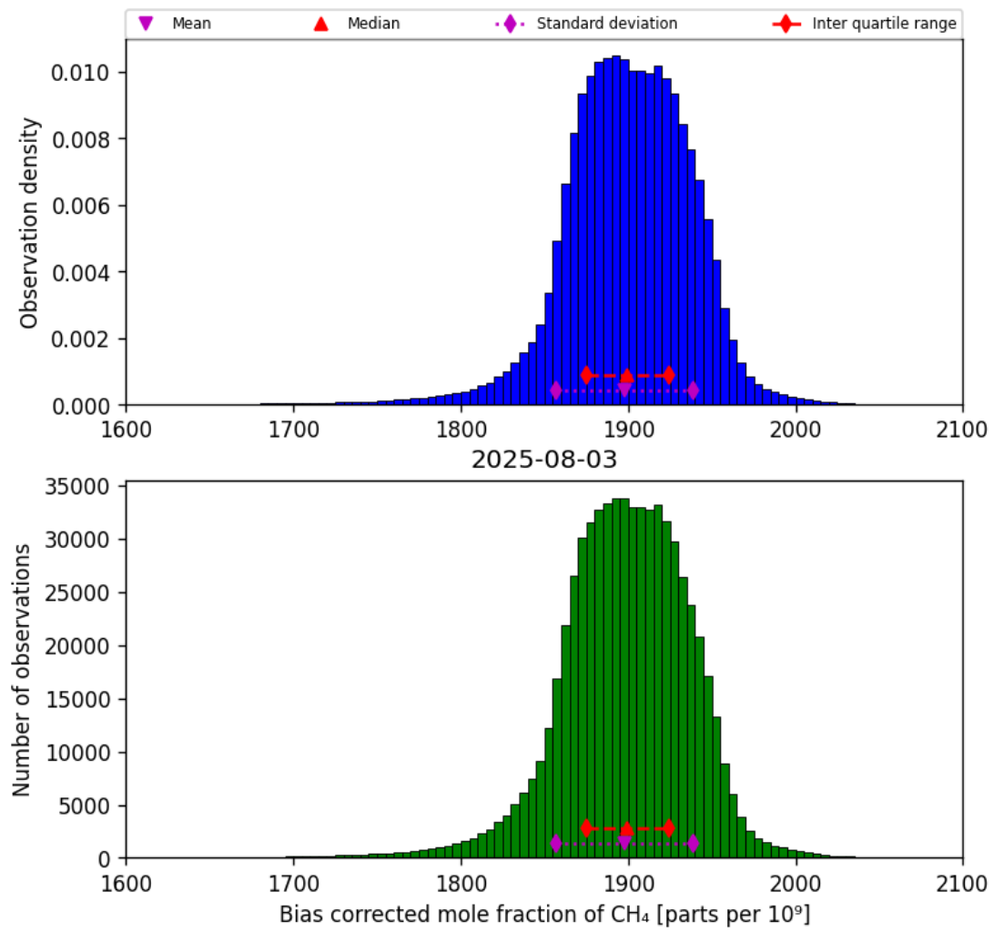
Figure 25: Histogram of “Bias corrected mole fraction of CH 4 ” for 2025-08-03 to 2025-08-04
