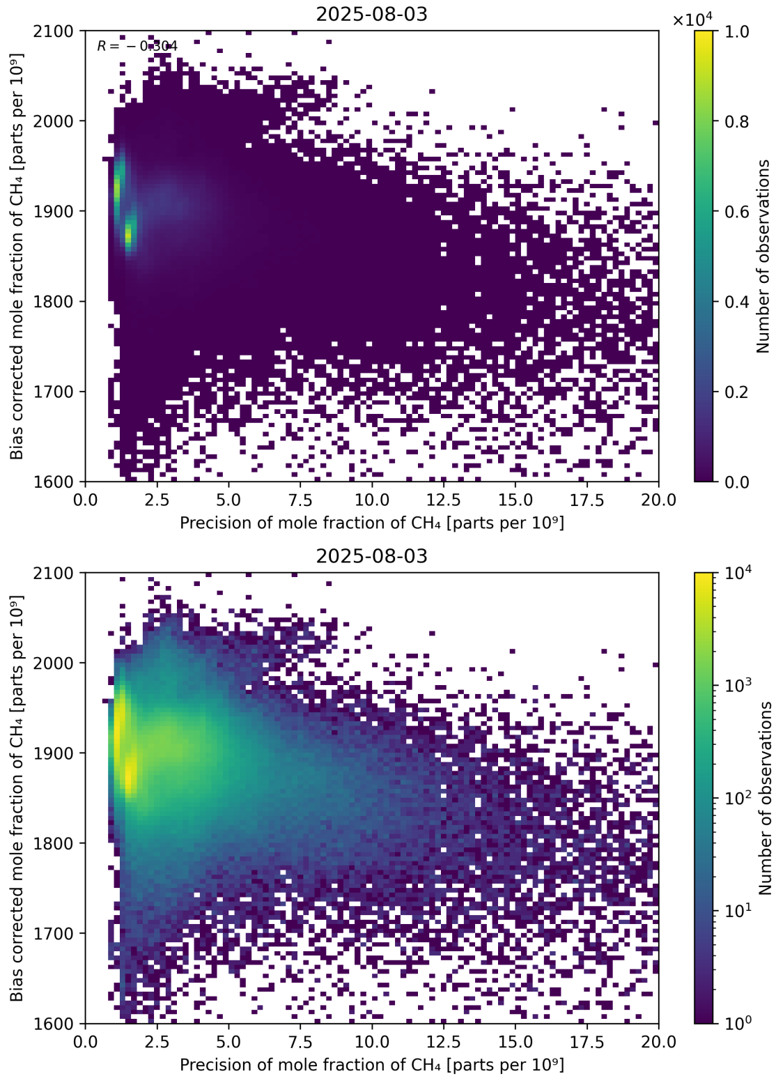
Figure 82: Scatter density plot of “Precision of mole fraction of CH 4 ” against “Bias corrected mole fraction of CH 4 ” for 2025-08-03 to 2025-08-04.
