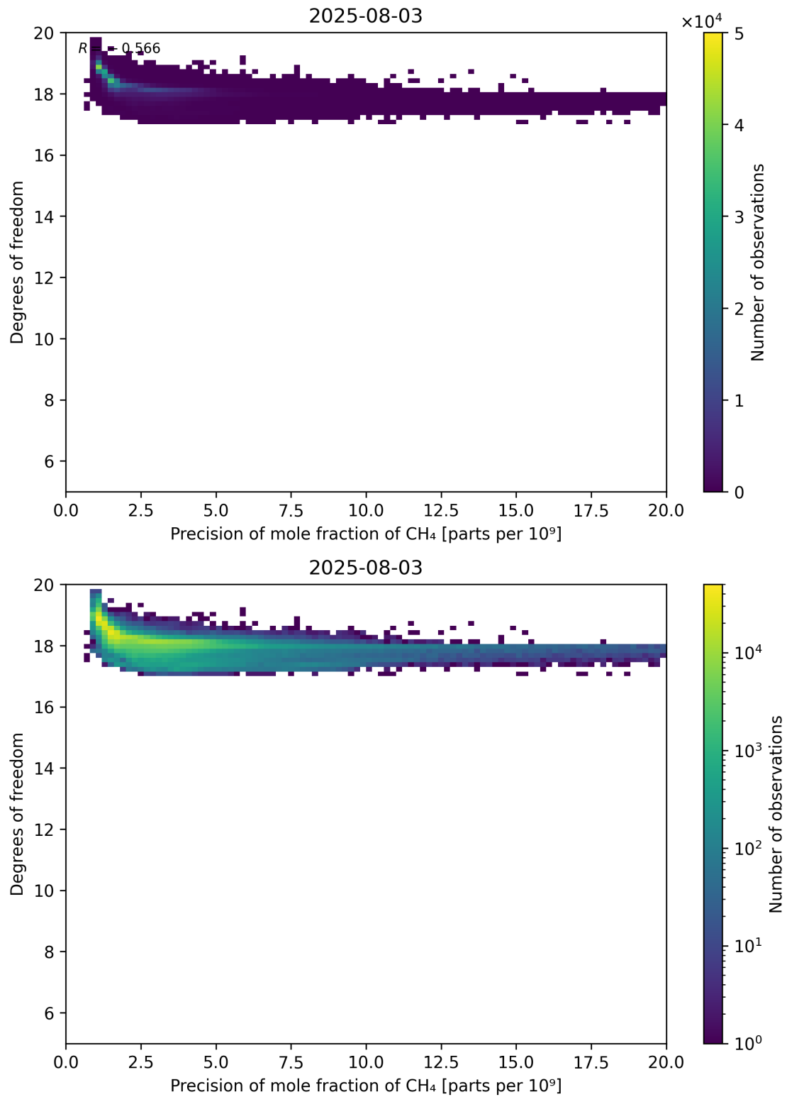
Figure 80: Scatter density plot of “Precision of mole fraction of CH 4 ” against “Degrees of freedom” for 2025-08-03 to 2025-08-04.
