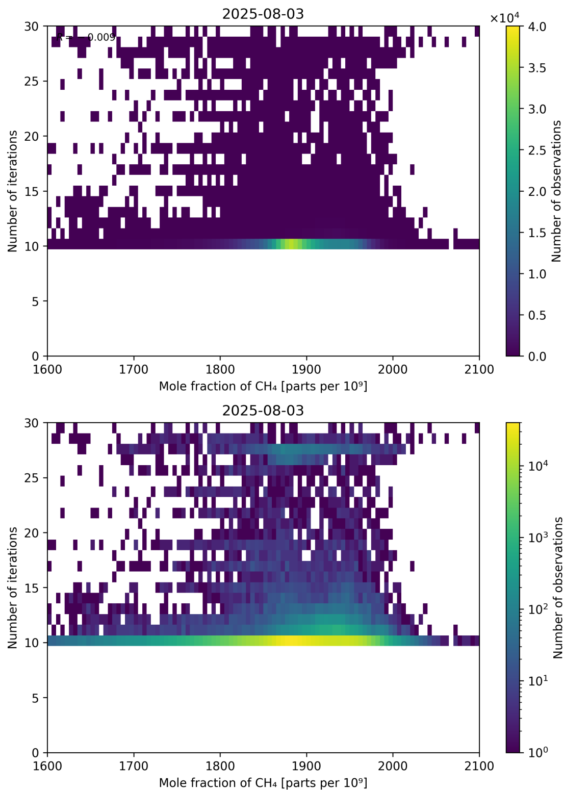
Figure 76: Scatter density plot of “Mole fraction of CH 4 ” against “Number of iterations” for 2025-08-03 to 2025-08-04.
