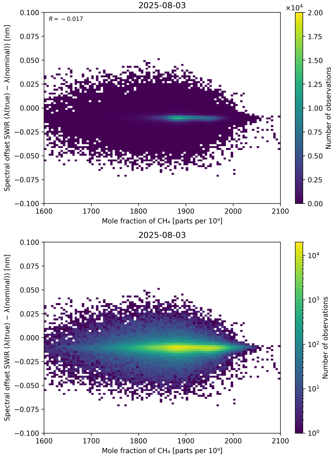
Figure 86: Scatter density plot of “Mole fraction of \text{CH}_4 ” against “Spectral offset SWIR ( \lambda_{\text{true}} - \lambda_{\text{nominal}} )” for 2025-08-03 to 2025-08-04.
