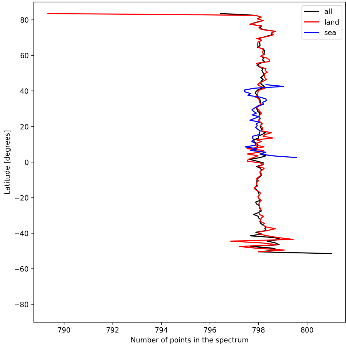
Figure 15: Zonal average of “Number of points in the spectrum” for 2025-08-03 to 2025-08-04.
