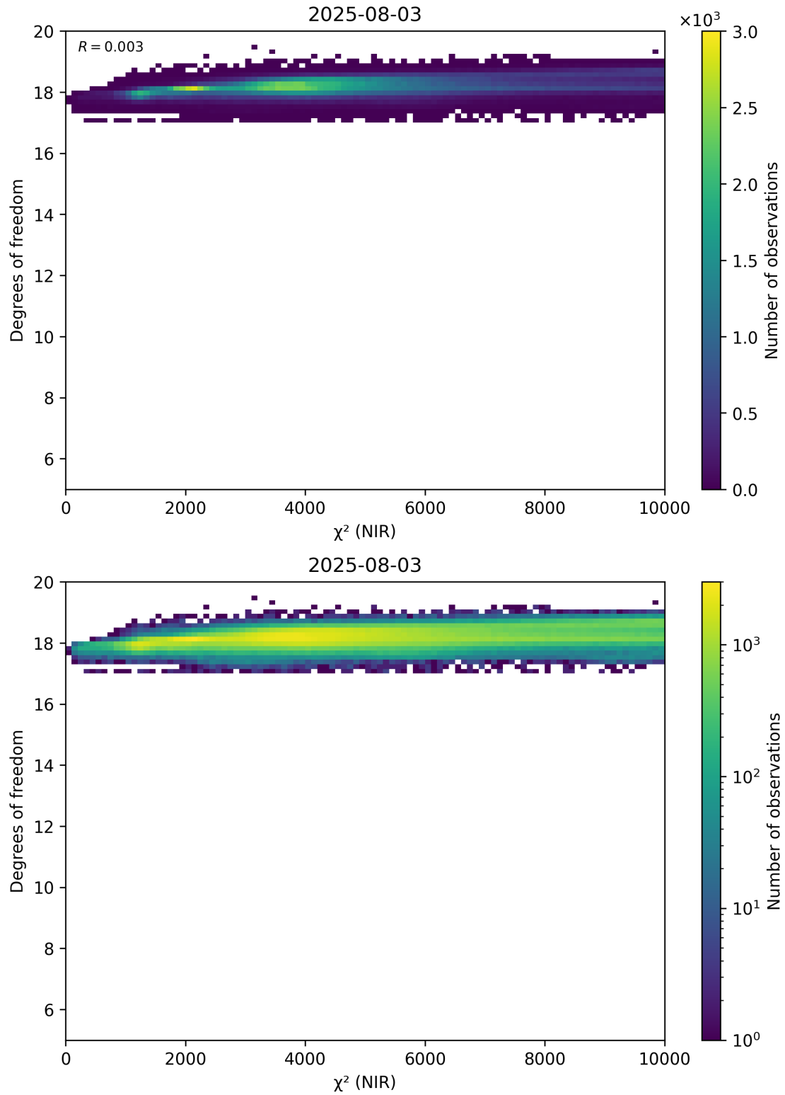
Figure 44: Scatter density plot of “ \chi^2 (NIR)” against “Degrees of freedom” for 2025-08-03 to 2025-08-04.
