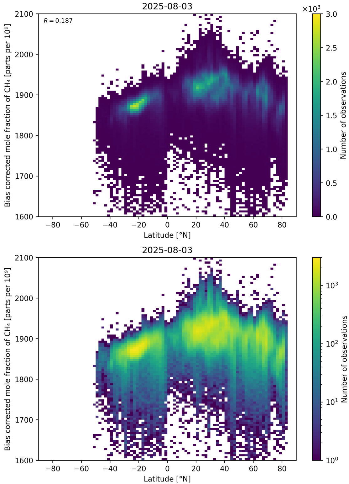
Figure 58: Scatter density plot of “Latitude” against “Bias corrected mole fraction of \text{CH}_4 ” for 2025-08-03 to 2025-08-04.
