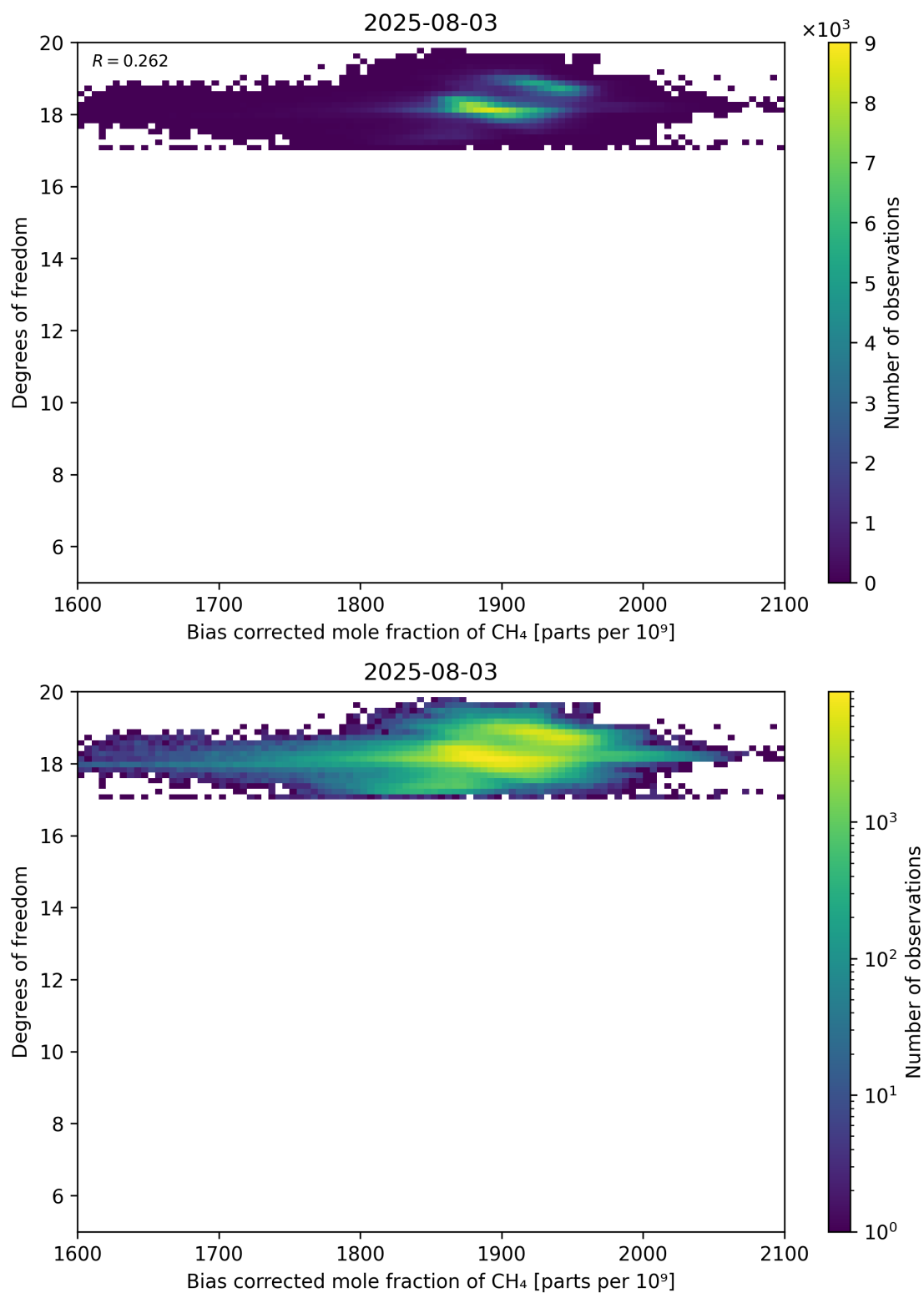
Figure 65: Scatter density plot of “Bias corrected mole fraction of CH 4 ” against “Degrees of freedom” for 2025-08-03 to 2025-08-04.
