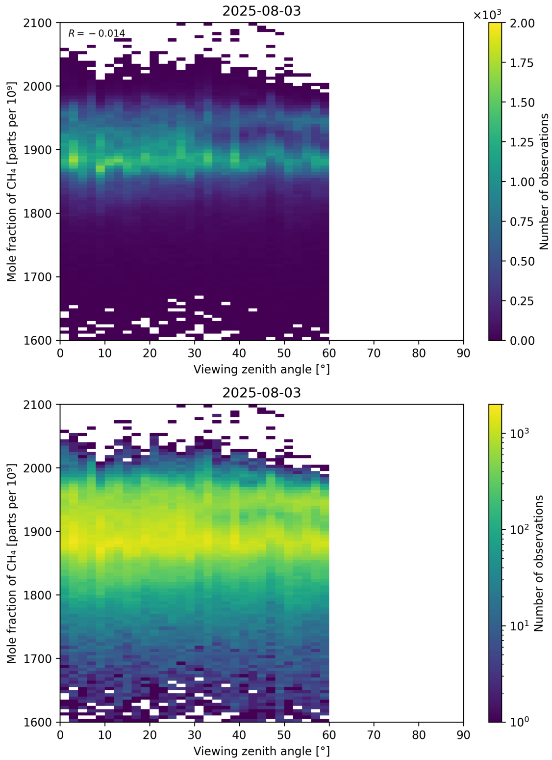
Figure 110: Scatter density plot of “Viewing zenith angle” against “Mole fraction of CH 4 ” for 2025-08-03 to 2025-08-04.
