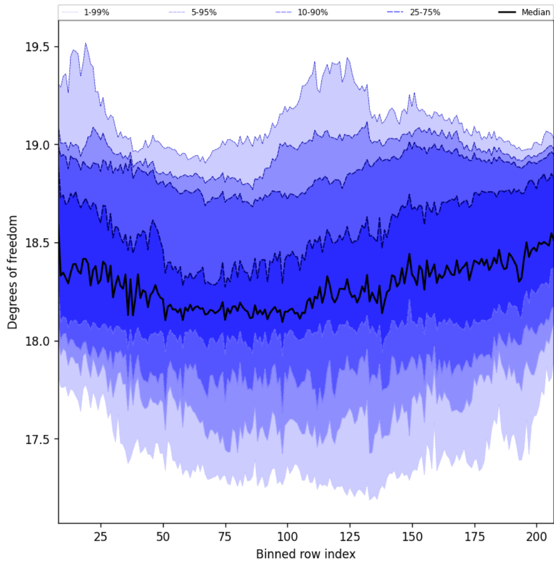
Figure 41: Along track statistics of “Degrees of freedom” for 2025-08-03 to 2025-08-04
