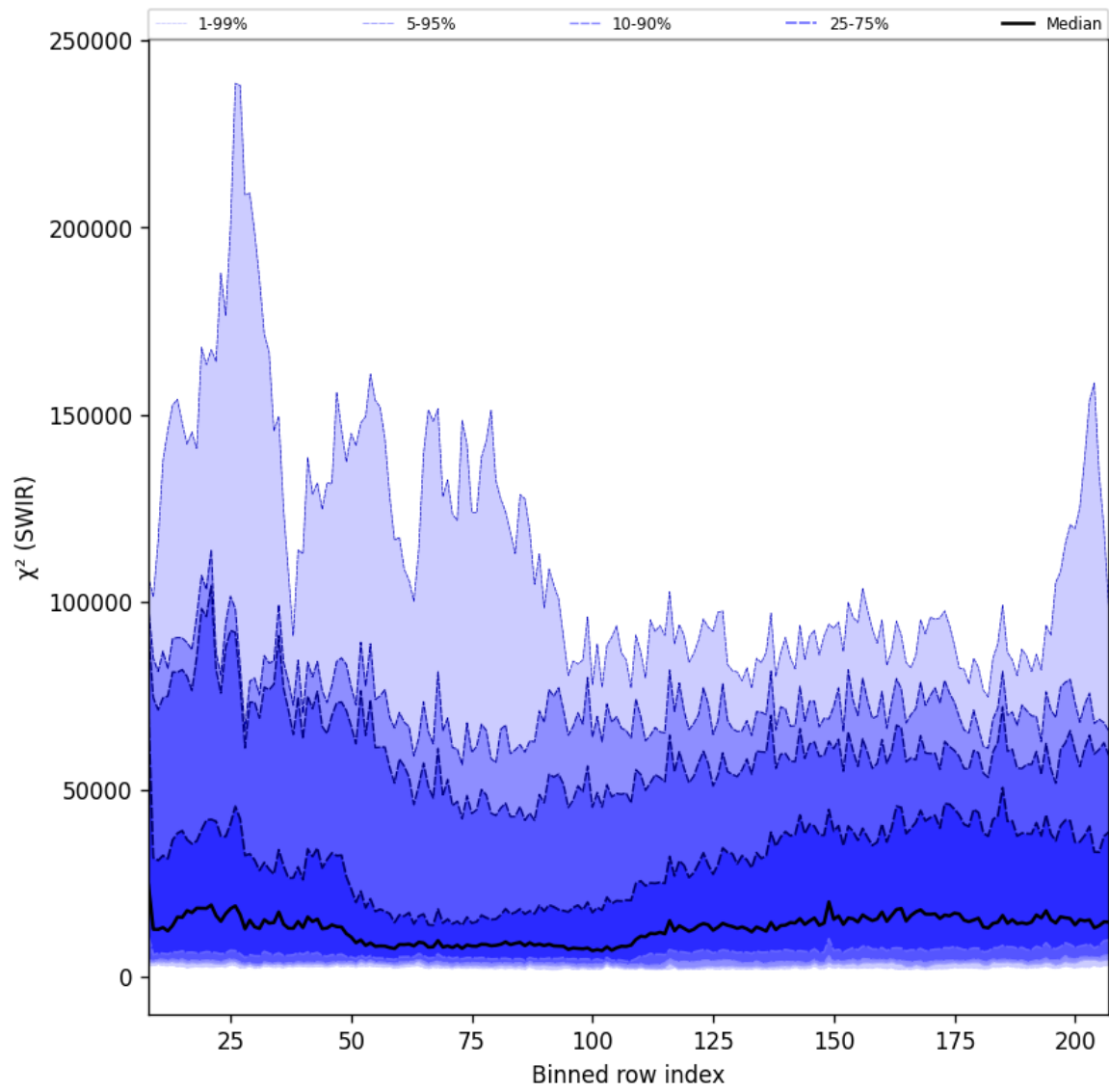
Figure 39: Along track statistics of “ \chi^2 (SWIR)” for 2025-08-03 to 2025-08-04
