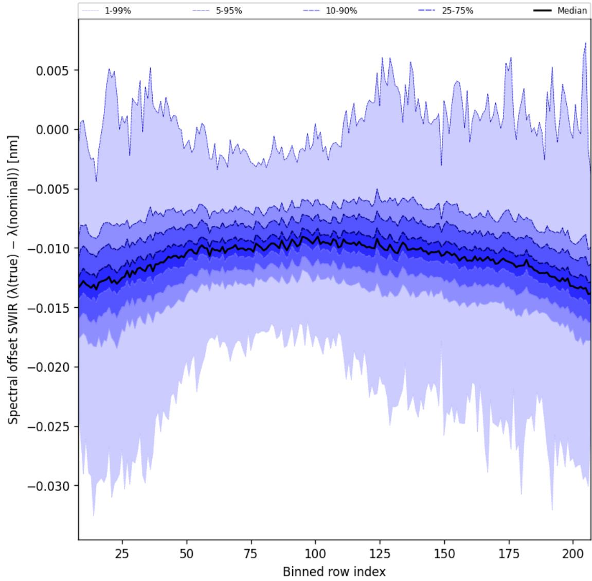
Figure 38: Along track statistics of “Spectral offset SWIR ( \lambda_{\text{true}} - \lambda_{\text{nominal}} )” for 2025-08-03 to 2025-08-04
