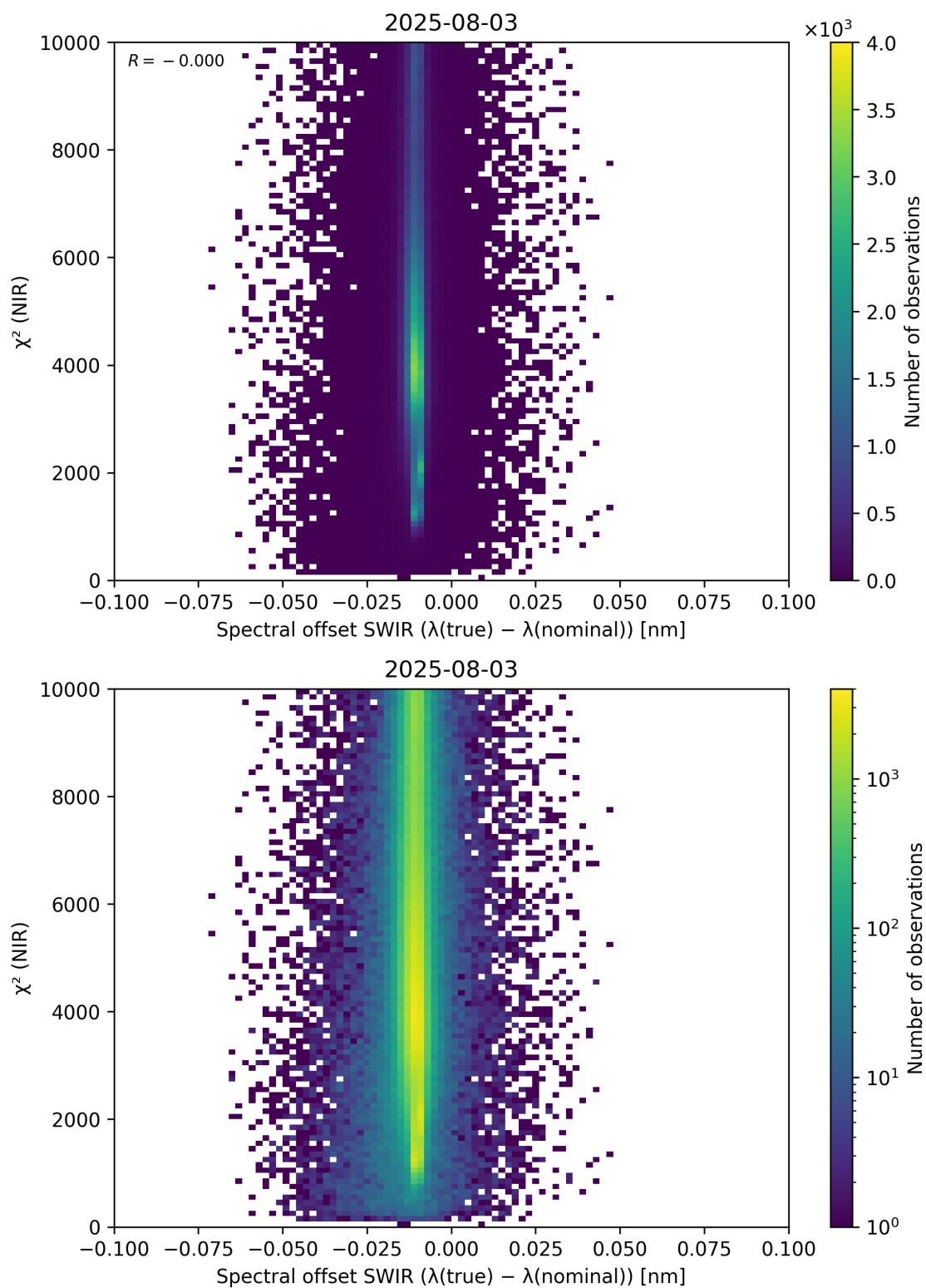
Figure 117: Scatter density plot of “Spectral offset SWIR ( \lambda_{\text{true}} - \lambda_{\text{nominal}} )” against “ \chi^2 (NIR)” for 2025-08-03 to 2025-08-04.
