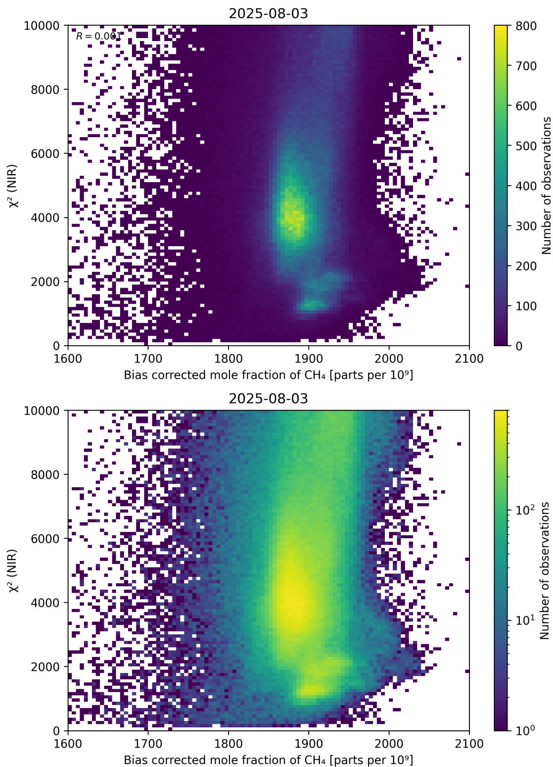
Figure 63: Scatter density plot of “Bias corrected mole fraction of CH 4 ” against “ \chi^2 (NIR)” for 2025-08-03 to 2025-08-04.
