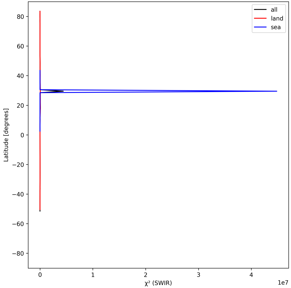
Figure 17: Zonal average of “ \chi^2 (SWIR)” for 2025-08-03 to 2025-08-04.
