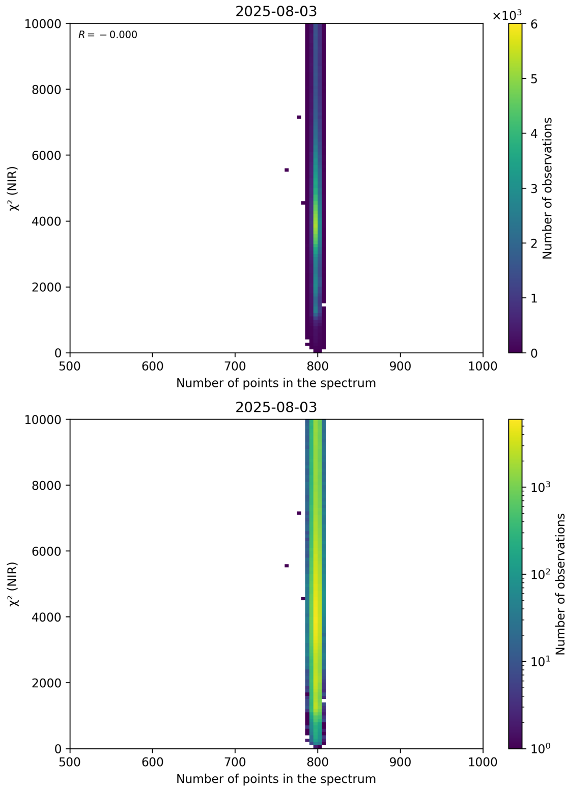
Figure 88: Scatter density plot of “Number of points in the spectrum” against “ \chi^2 (NIR)” for 2025-08-03 to 2025-08-04.
