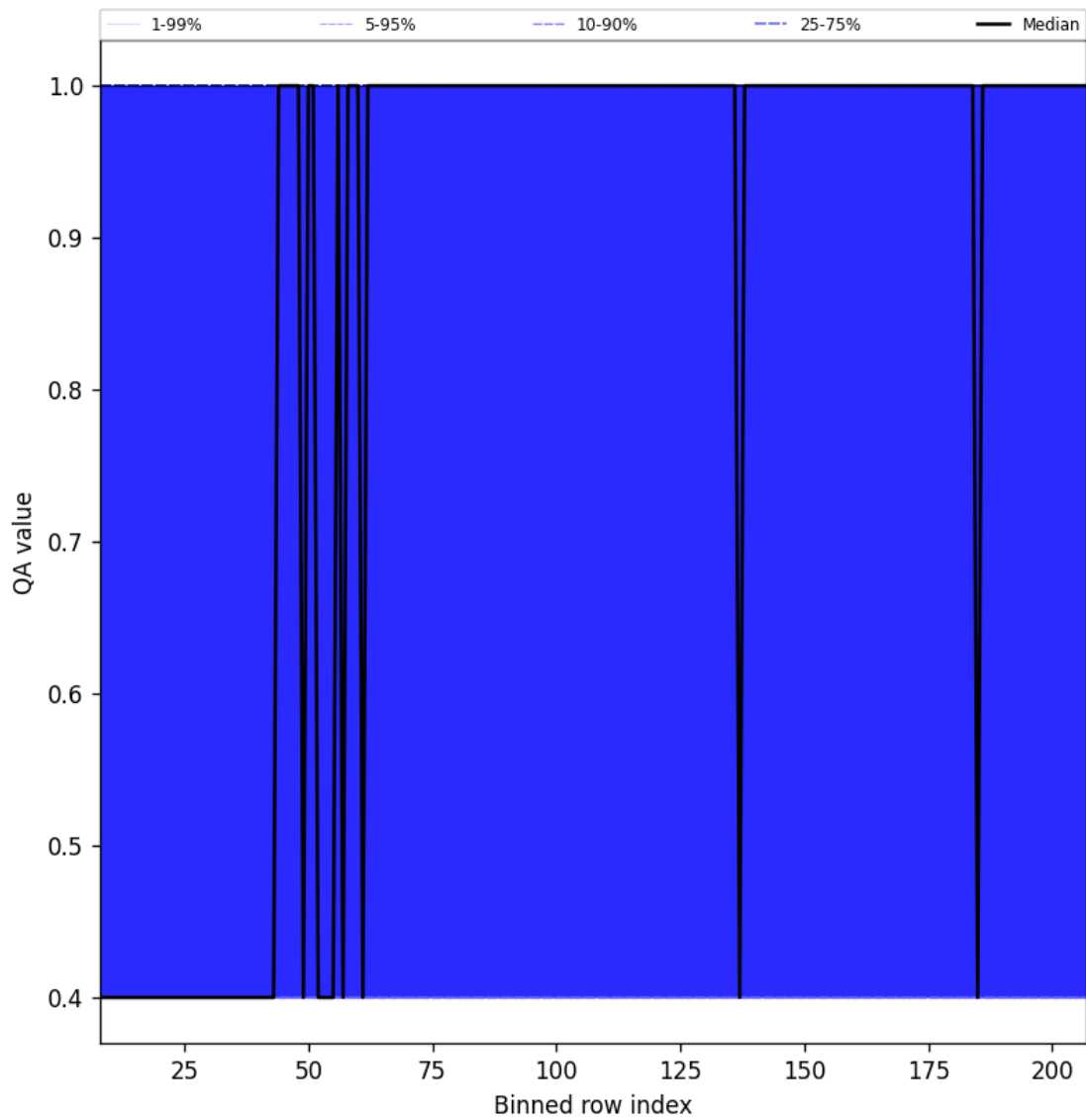
Figure 33: Along track statistics of “QA value” for 2025-08-03 to 2025-08-04
