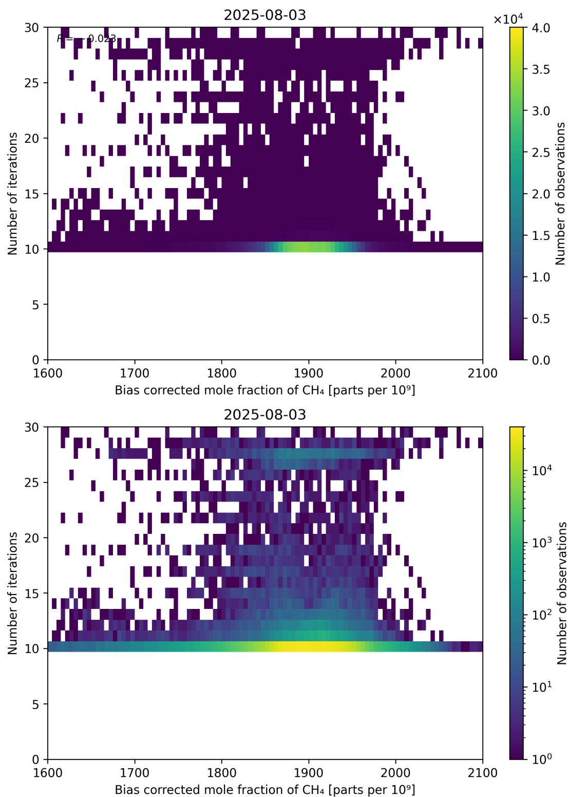
Figure 67: Scatter density plot of “Bias corrected mole fraction of CH 4 ” against “Number of iterations” for 2025-08-03 to 2025-08-04.
