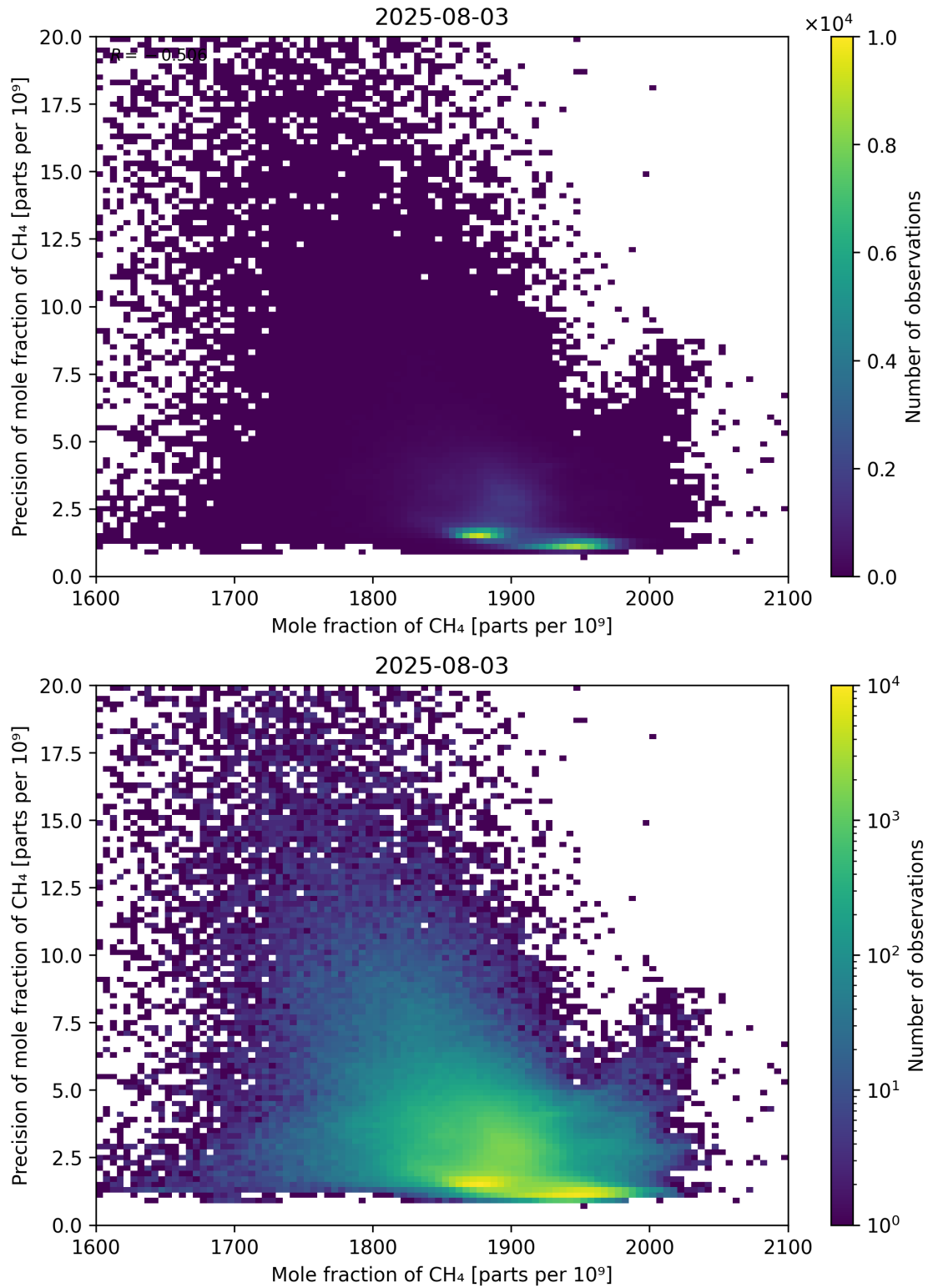
Figure 75: Scatter density plot of “Mole fraction of CH 4 ” against “Precision of mole fraction of CH 4 ” for 2025-08-03 to 2025-08-04.
