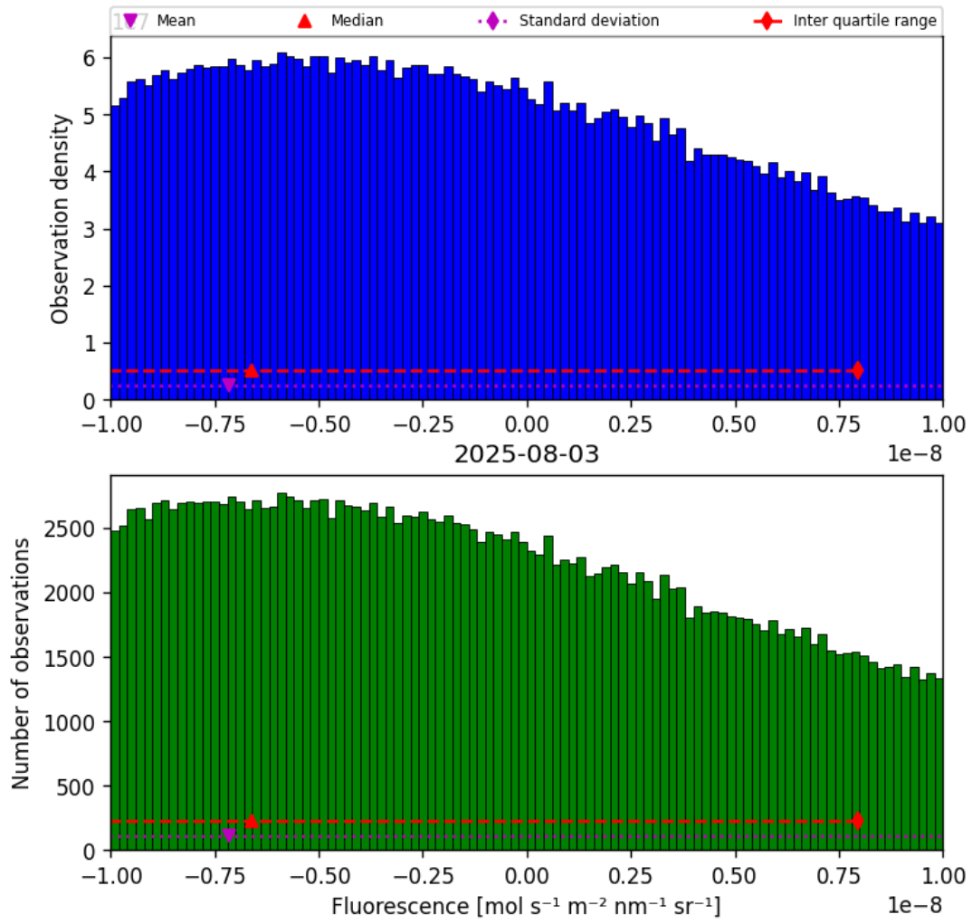
Figure 32: Histogram of “Fluorescence” for 2025-08-03 to 2025-08-04
