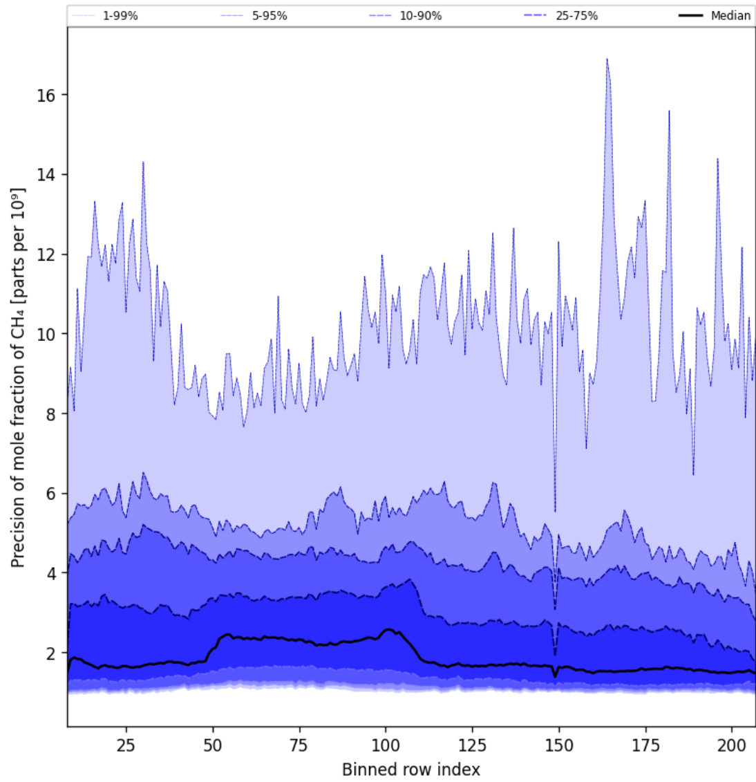
Figure 35: Along track statistics of “Precision of mole fraction of CH 4 ” for 2025-08-03 to 2025-08-04
