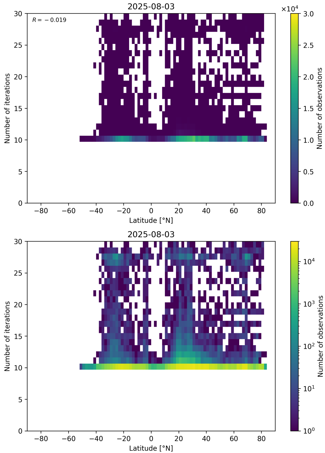
Figure 60: Scatter density plot of “Latitude” against “Number of iterations” for 2025-08-03 to 2025-08-04.
