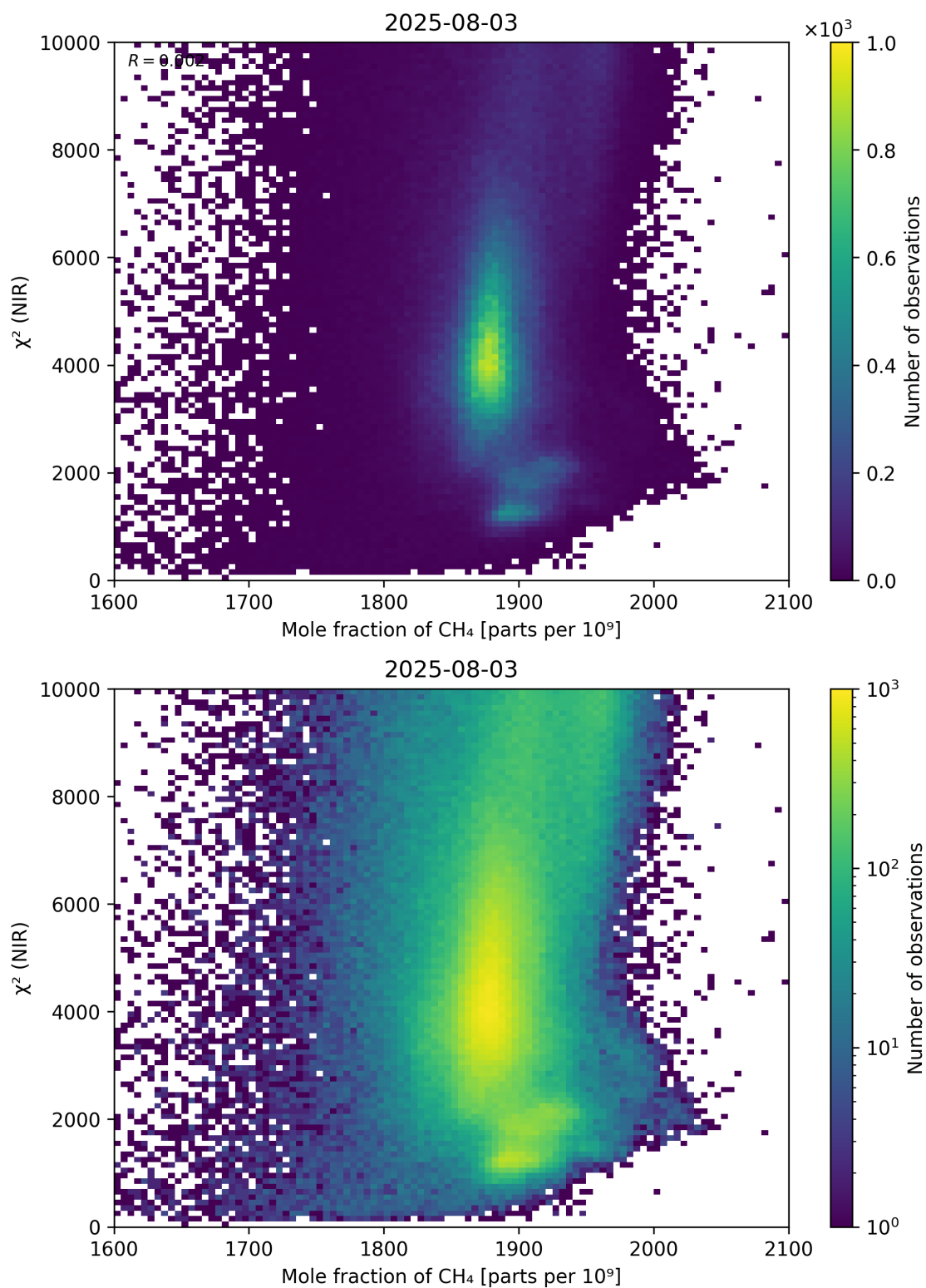
Figure 70: Scatter density plot of “Mole fraction of \text{CH}_4 ” against “ \chi^2 (NIR)” for 2025-08-03 to 2025-08-04.
