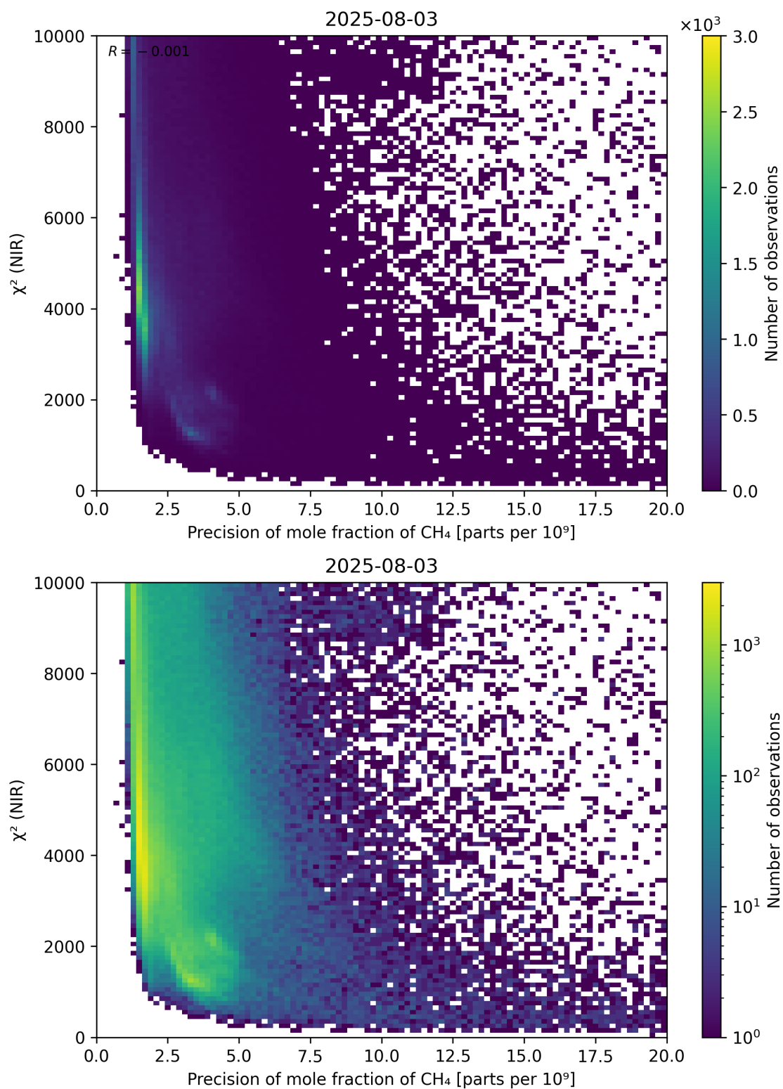
Figure 78: Scatter density plot of “Precision of mole fraction of CH 4 ” against “ \chi^2 (NIR)” for 2025-08-03 to 2025-08-04.
