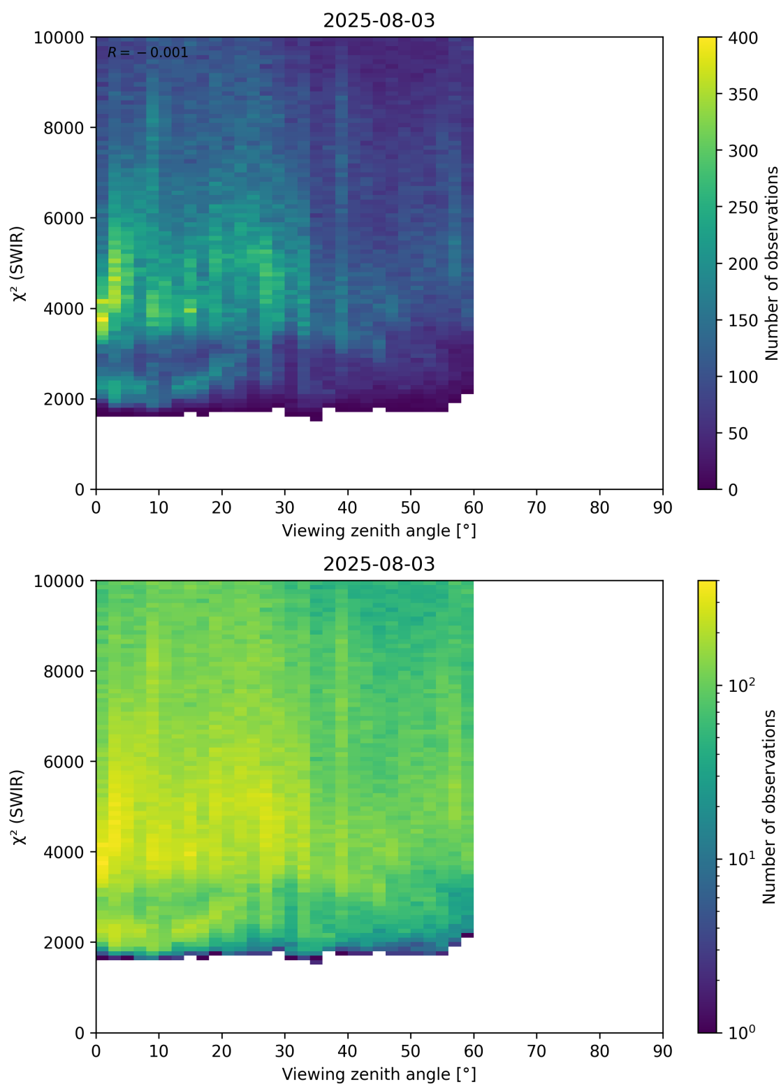
Figure 106: Scatter density plot of “Viewing zenith angle” against “ \chi^2 (SWIR)” for 2025-08-03 to 2025-08-04.
