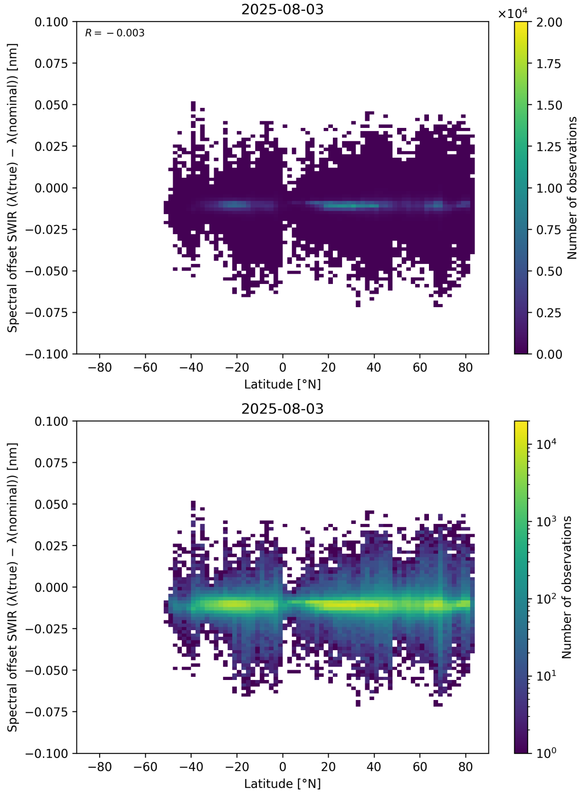
Figure 62: Scatter density plot of “Latitude” against “Spectral offset SWIR ( \lambda_{\text{true}} - \lambda_{\text{nominal}} )” for 2025-08-03 to 2025-08-04.
