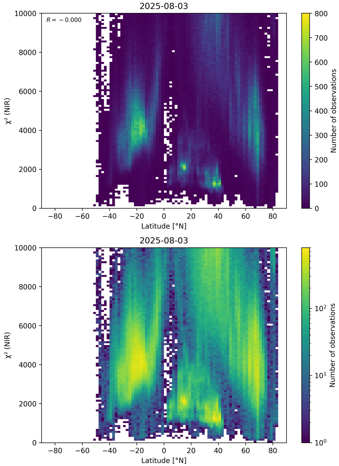
Figure 53: Scatter density plot of “Latitude” against “ \chi^2 (NIR)” for 2025-08-03 to 2025-08-04.
