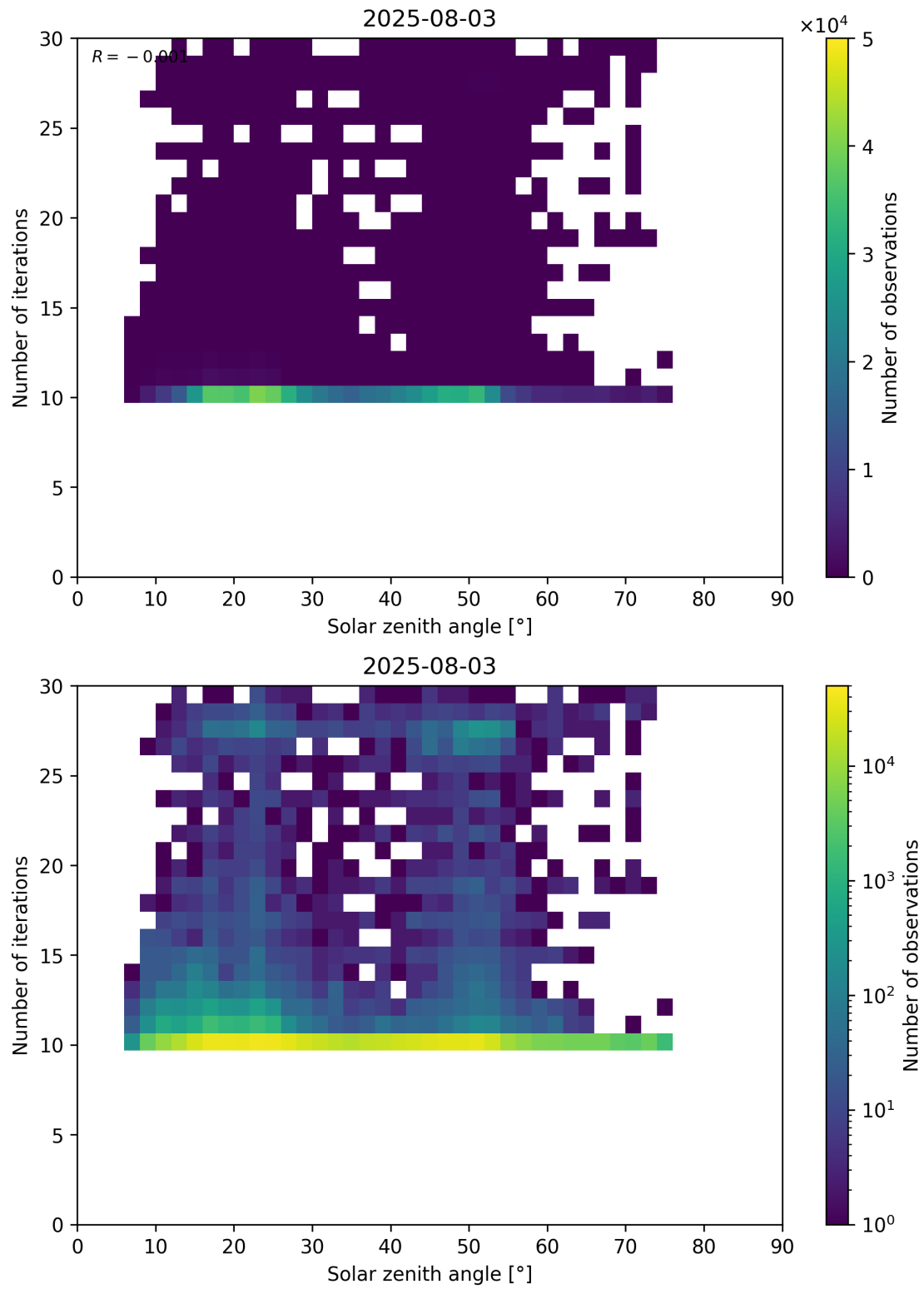
Figure 102: Scatter density plot of “Solar zenith angle” against “Number of iterations” for 2025-08-03 to 2025-08-04.
