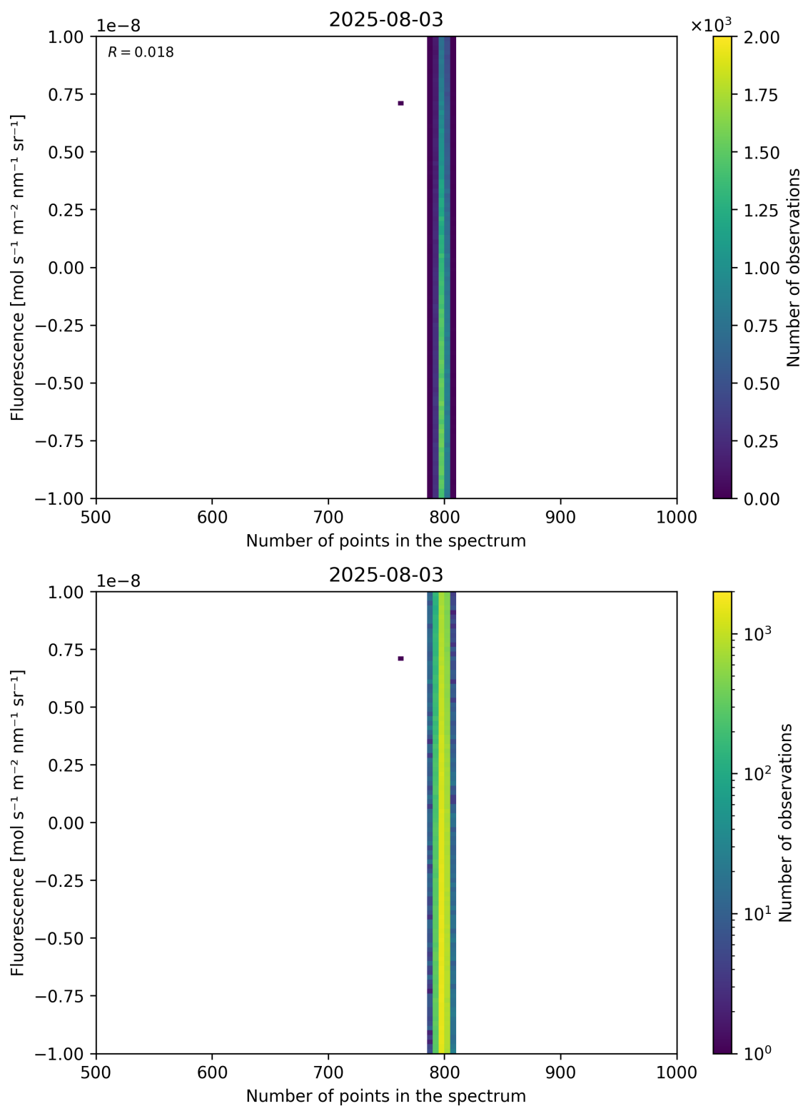
Figure 91: Scatter density plot of “Number of points in the spectrum” against “Fluorescence” for 2025-08-03 to 2025-08-04.
