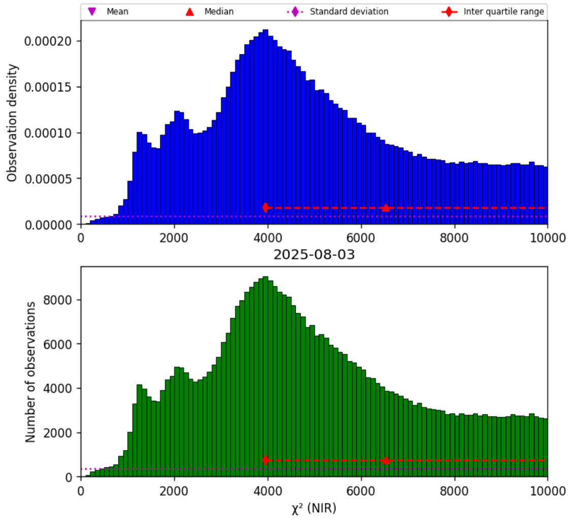
Figure 29: Histogram of " \chi^2 (NIR)" for 2025-08-03 to 2025-08-04
