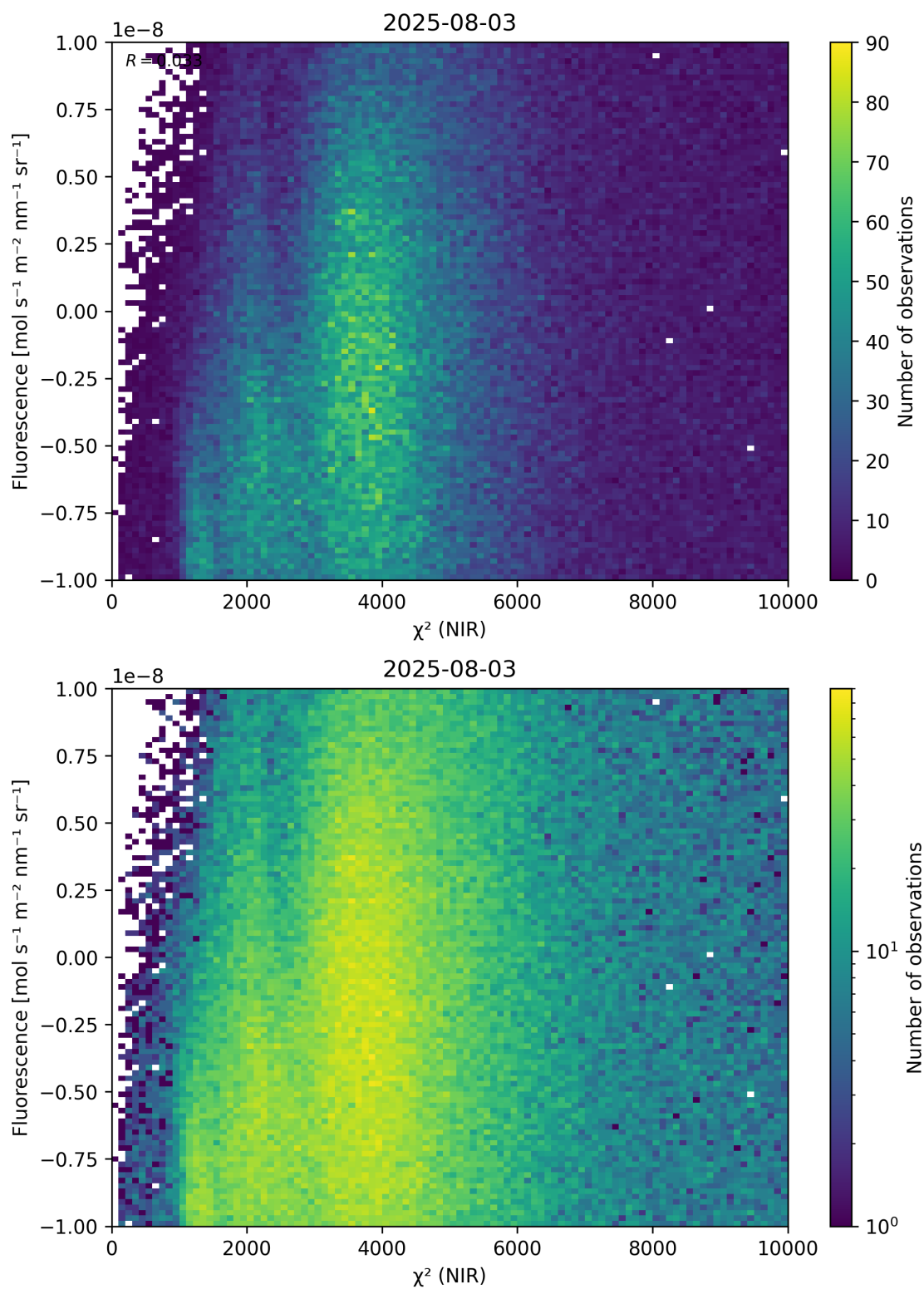
Figure 45: Scatter density plot of “ \chi^2 (NIR)” against “Fluorescence” for 2025-08-03 to 2025-08-04.
