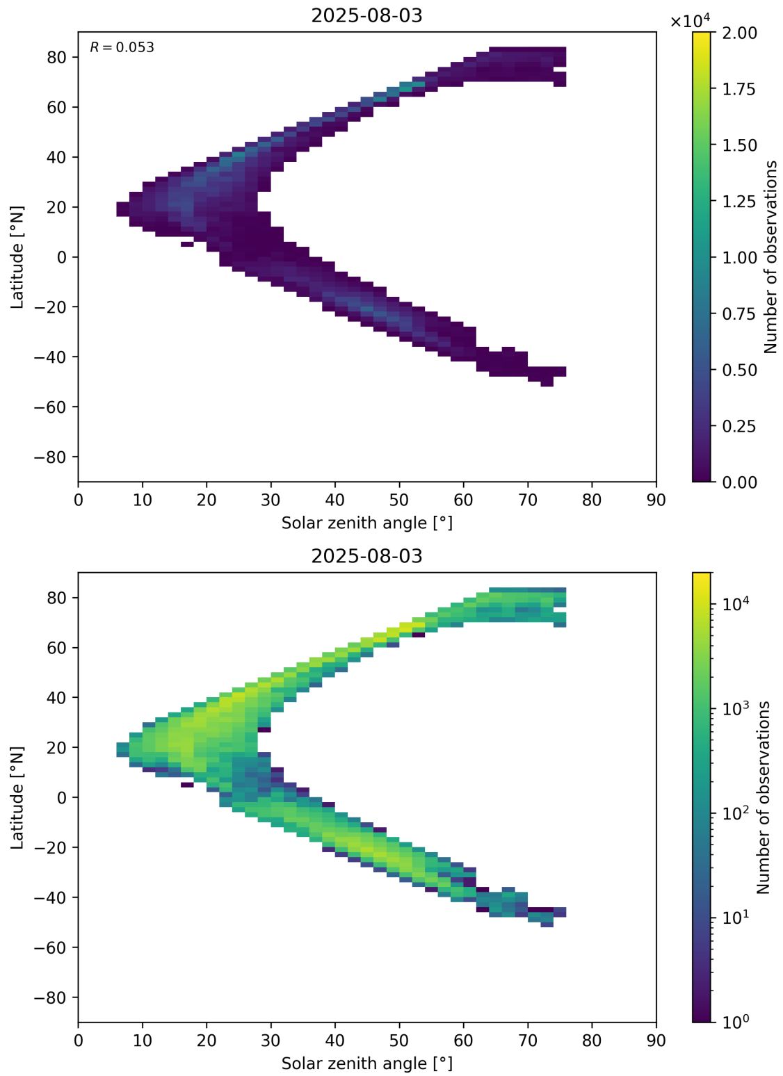
Figure 98: Scatter density plot of “Solar zenith angle” against “Latitude” for 2025-08-03 to 2025-08-04.
