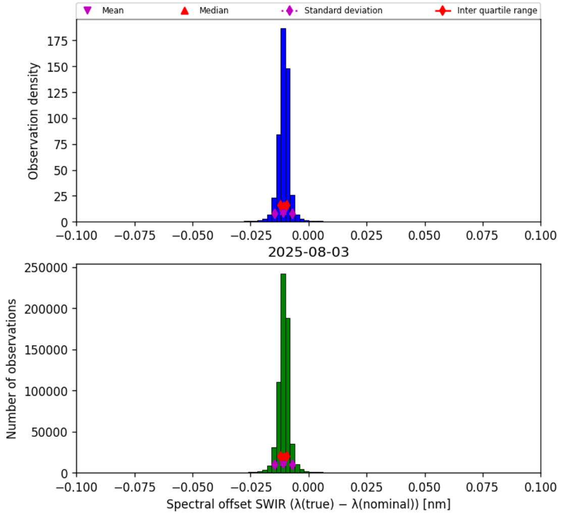
Figure 27: Histogram of “Spectral offset SWIR ( \lambda_{\text{true}} - \lambda_{\text{nominal}} )” for 2025-08-03 to 2025-08-04
