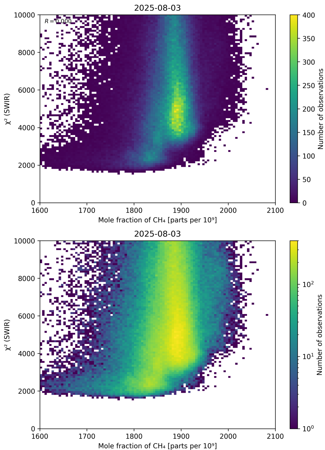
Figure 71: Scatter density plot of “Mole fraction of \text{CH}_4 ” against “ \chi^2 (SWIR)” for 2025-08-03 to 2025-08-04.
