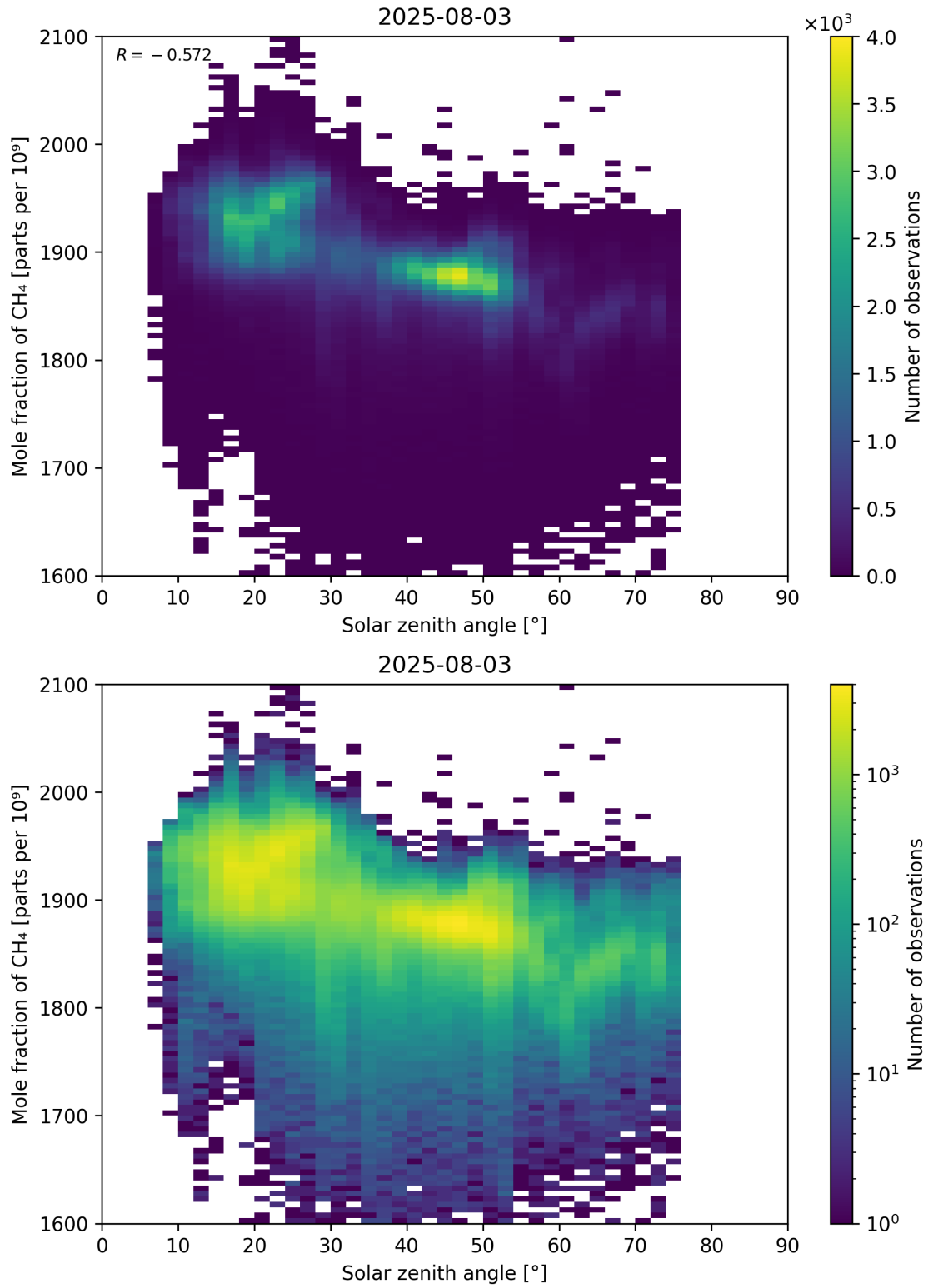
Figure 99: Scatter density plot of “Solar zenith angle” against “Mole fraction of \text{CH}_4 ” for 2025-08-03 to 2025-08-04.
