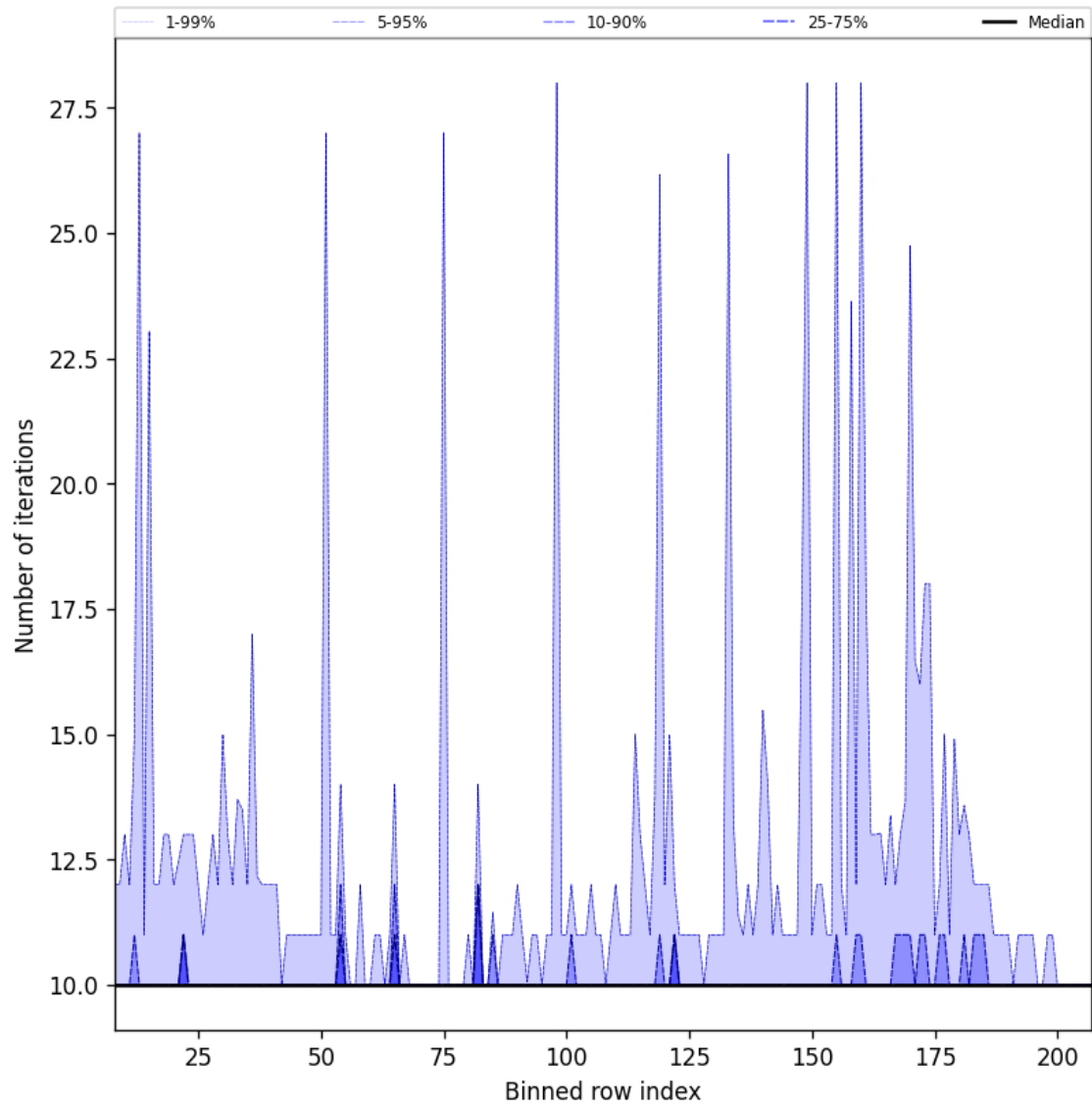
Figure 42: Along track statistics of “Number of iterations” for 2025-08-03 to 2025-08-04
