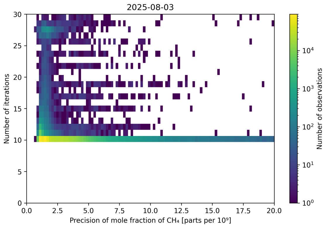
Figure 83: Scatter density plot of “Precision of mole fraction of CH 4 ” against “Number of iterations” for 2025-08-03 to 2025-08-04.
