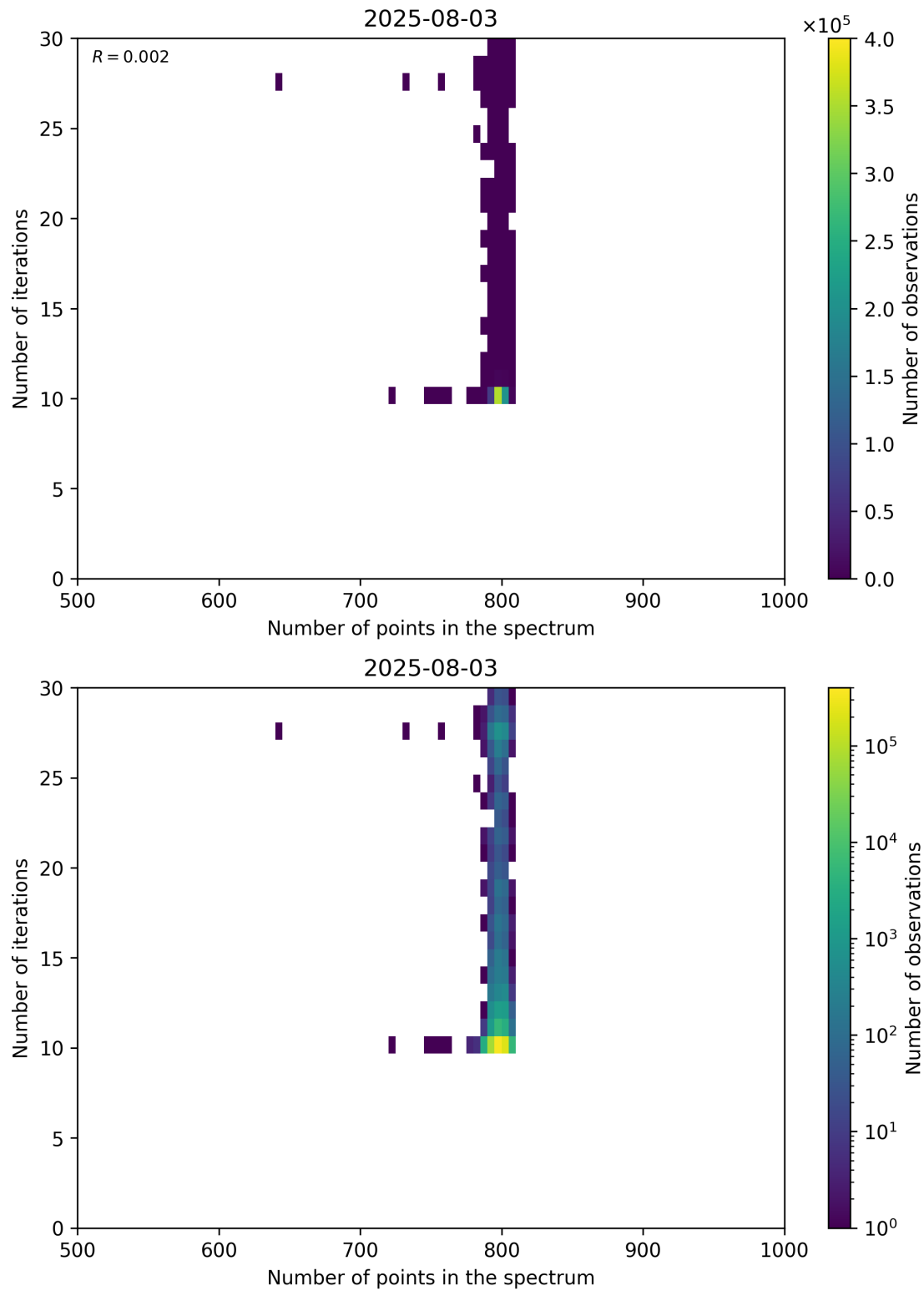
Figure 92: Scatter density plot of “Number of points in the spectrum” against “Number of iterations” for 2025-08-03 to 2025-08-04.
