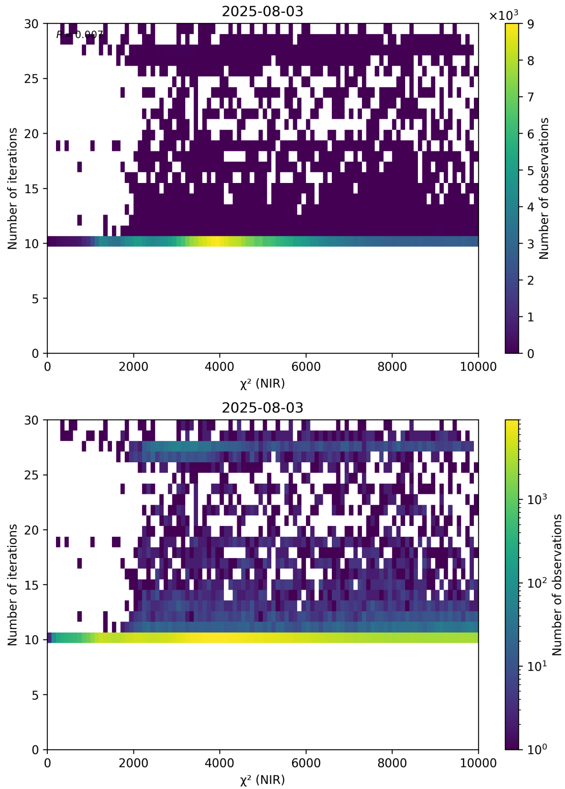
Figure 46: Scatter density plot of “ \chi^2 (NIR)” against “Number of iterations” for 2025-08-03 to 2025-08-04.
