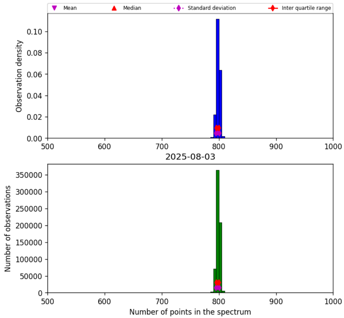
Figure 26: Histogram of “Number of points in the spectrum” for 2025-08-03 to 2025-08-04
