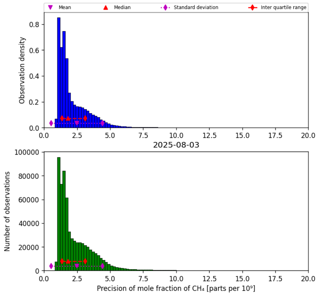
Figure 24: Histogram of “Precision of mole fraction of CH 4 ” for 2025-08-03 to 2025-08-04
