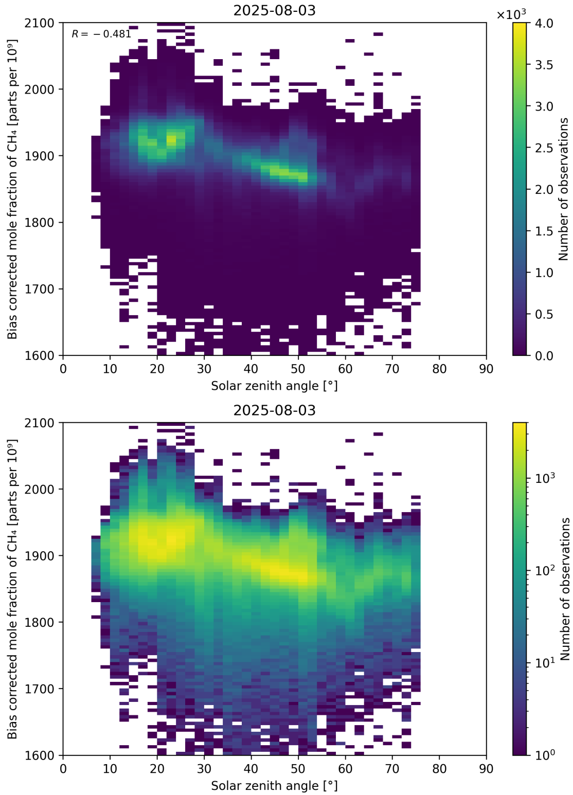
Figure 100: Scatter density plot of “Solar zenith angle” against “Bias corrected mole fraction of CH 4 ” for 2025-08-03 to 2025-08-04.
