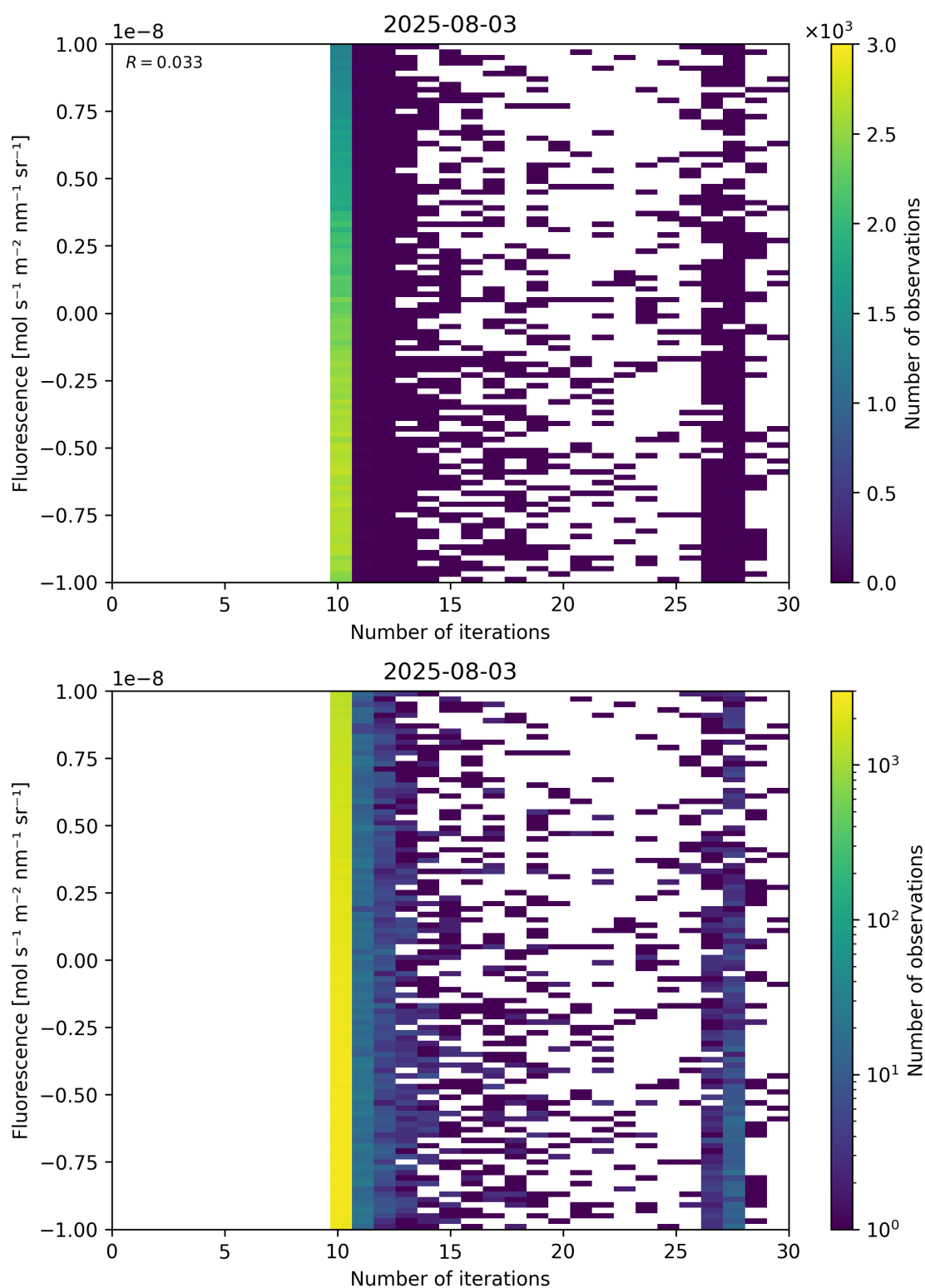
Figure 87: Scatter density plot of “Number of iterations” against “Fluorescence” for 2025-08-03 to 2025-08-04.
