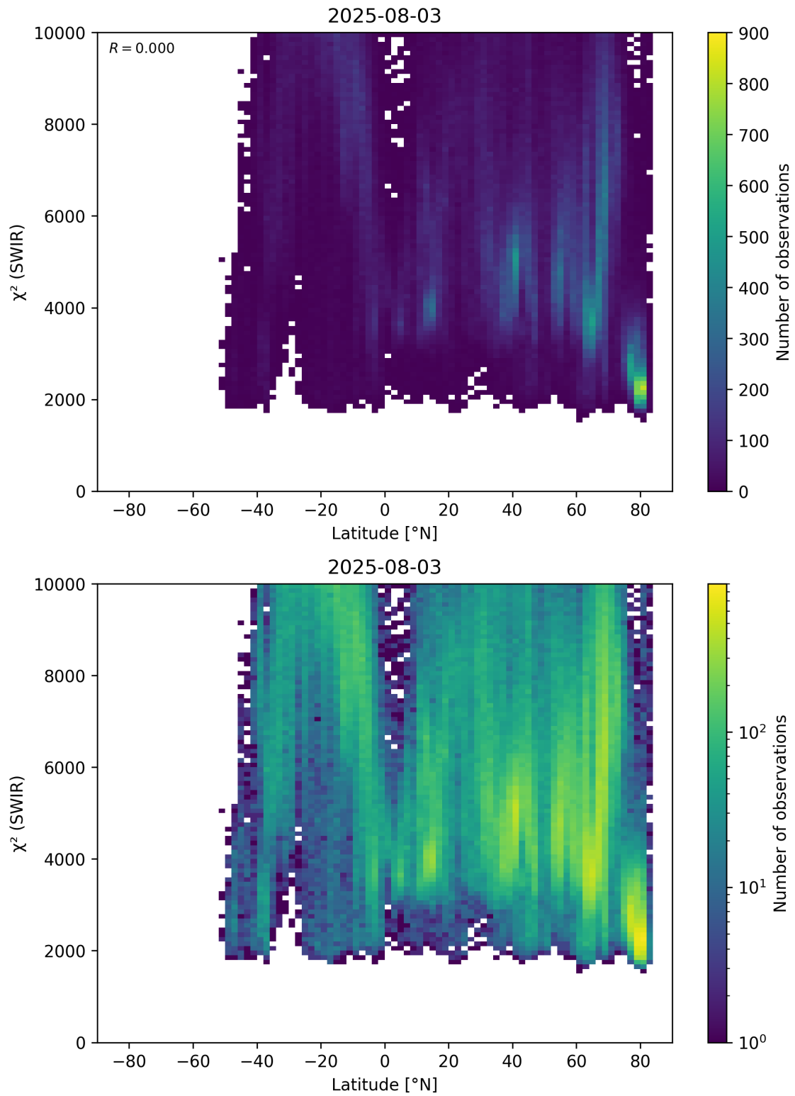
Figure 54: Scatter density plot of “Latitude” against “ \chi^2 (SWIR)” for 2025-08-03 to 2025-08-04.
