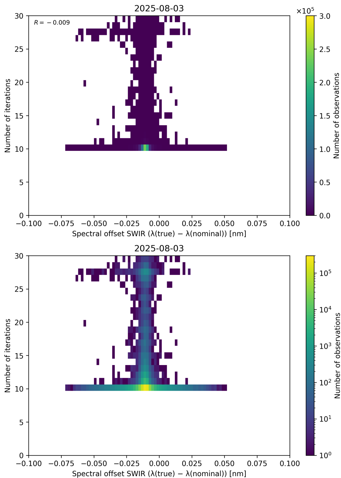
Figure 121: Scatter density plot of “Spectral offset SWIR ( \lambda_{\text{true}} - \lambda_{\text{nominal}} )” against “Number of iterations” for 2025-08-03 to 2025-08-04.
