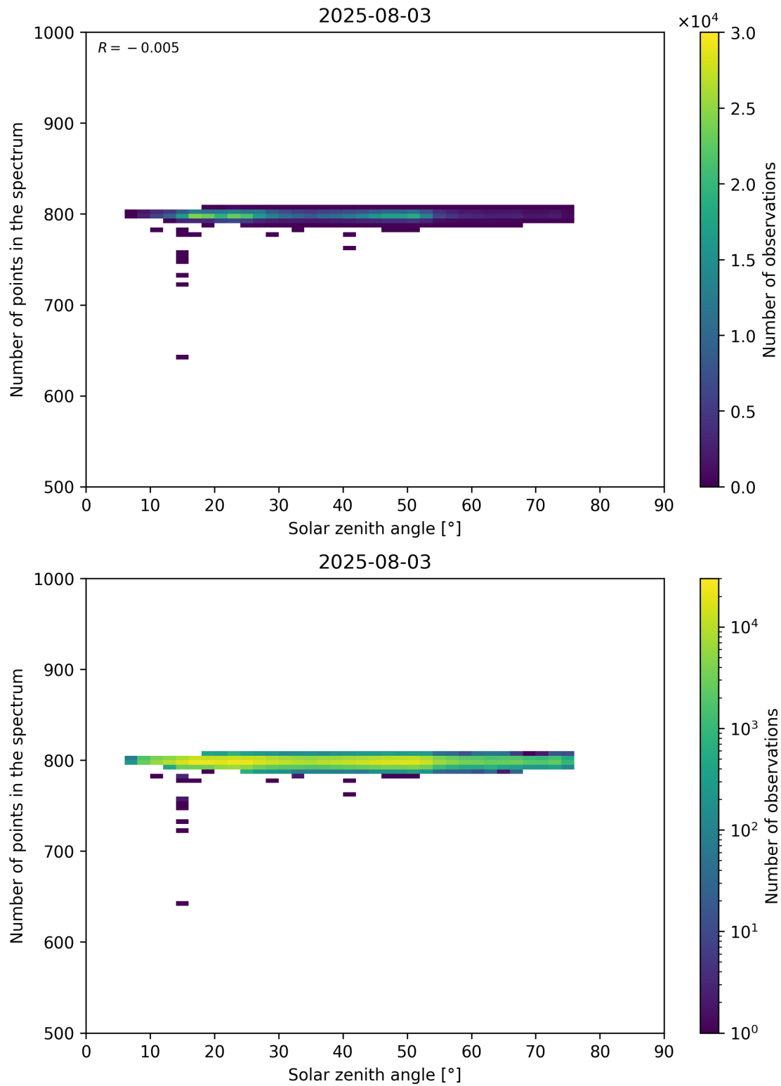
Figure 103: Scatter density plot of “Solar zenith angle” against “Number of points in the spectrum” for 2025-08-03 to 2025-08-04.
