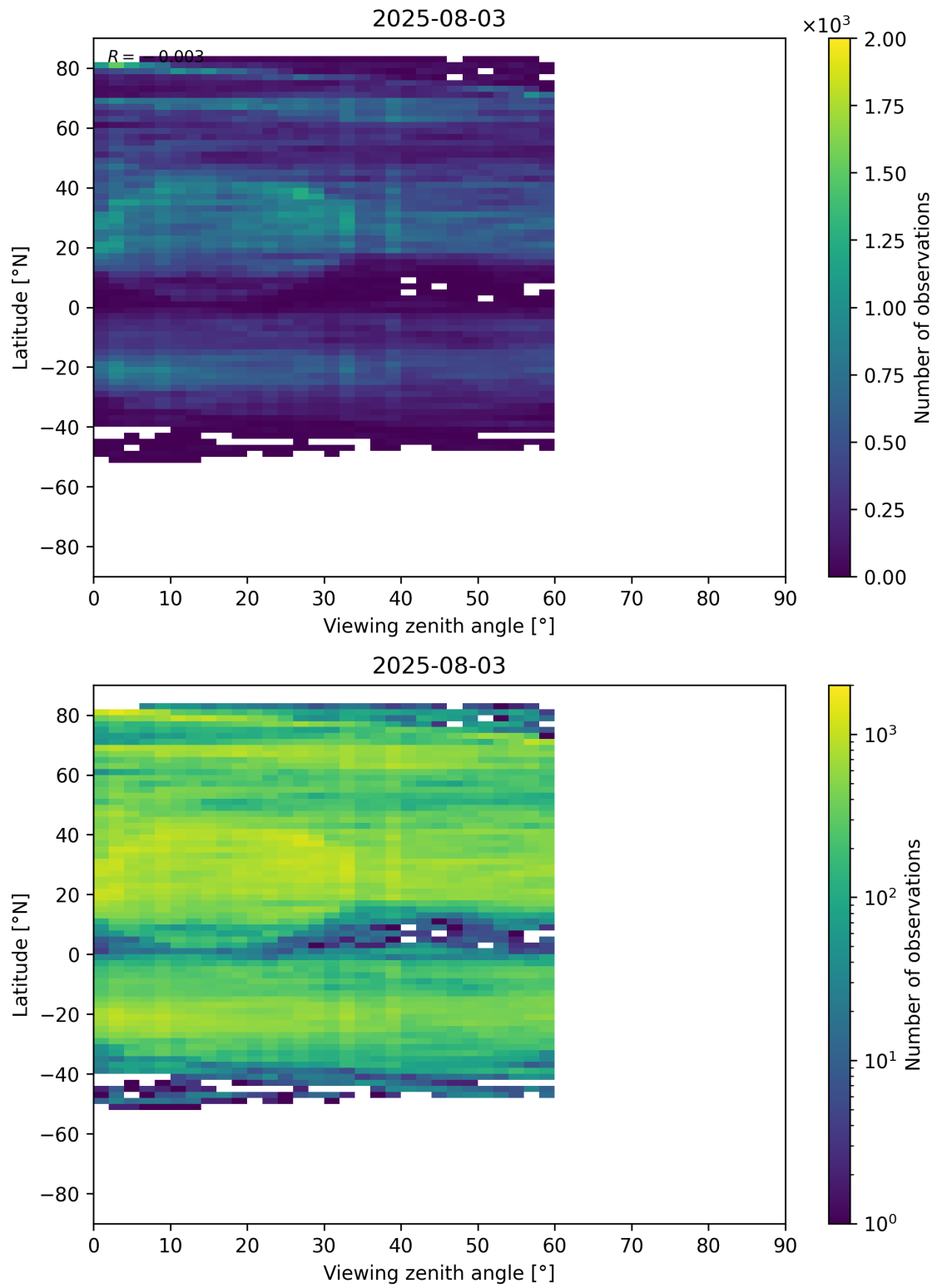
Figure 109: Scatter density plot of “Viewing zenith angle” against “Latitude” for 2025-08-03 to 2025-08-04.
