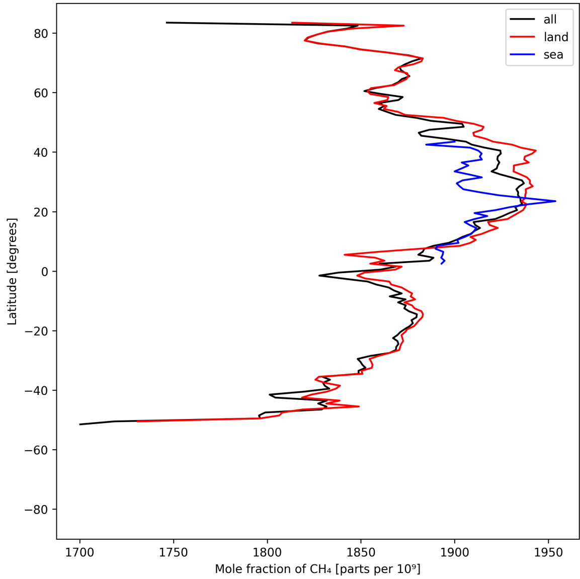
Figure 12: Zonal average of “Mole fraction of \text{CH}_4 ” for 2025-08-03 to 2025-08-04.
