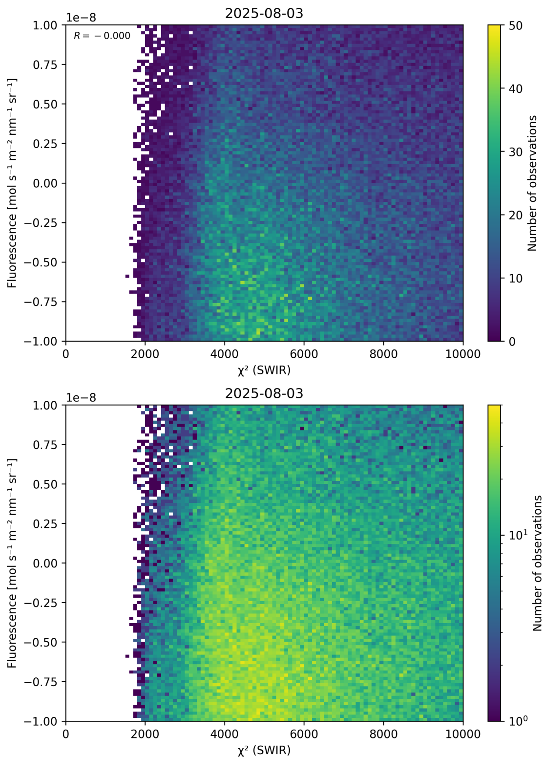
Figure 49: Scatter density plot of “ \chi^2 (SWIR)” against “Fluorescence” for 2025-08-03 to 2025-08-04.
