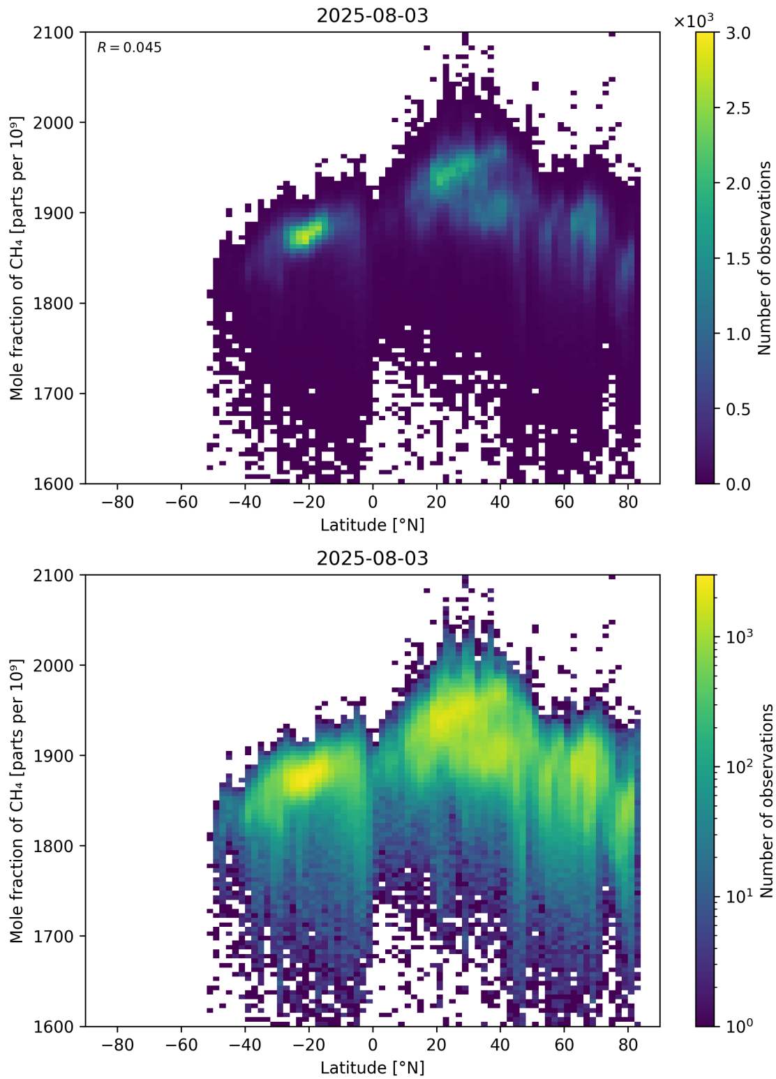
Figure 57: Scatter density plot of “Latitude” against “Mole fraction of CH 4 ” for 2025-08-03 to 2025-08-04.
