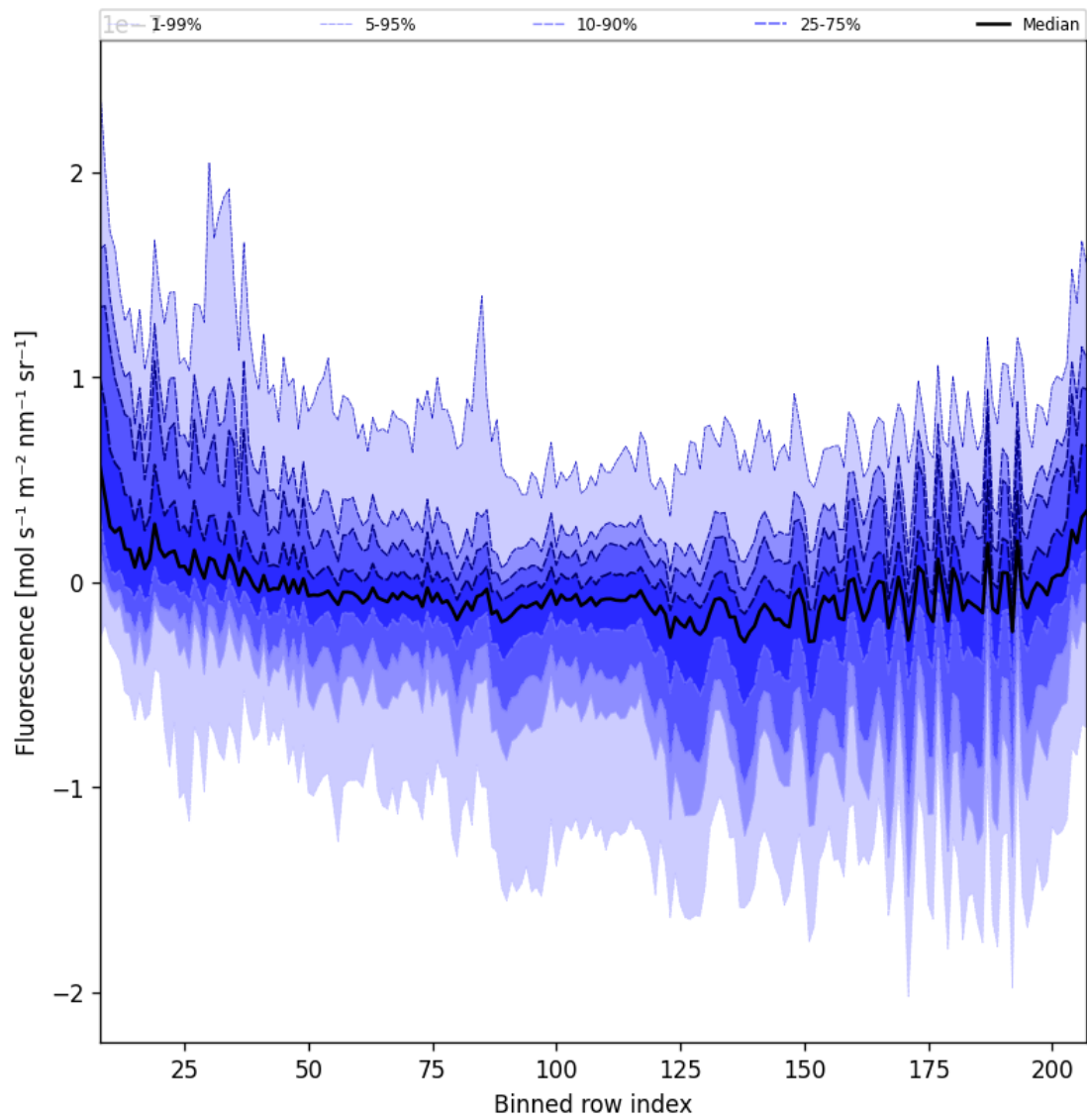
Figure 43: Along track statistics of “Fluorescence” for 2025-08-03 to 2025-08-04
