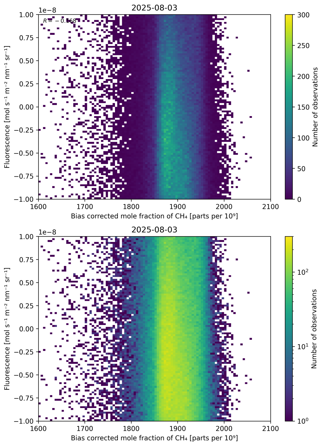
Figure 66: Scatter density plot of “Bias corrected mole fraction of \text{CH}_4 ” against “Fluorescence” for 2025-08-03 to 2025-08-04.
