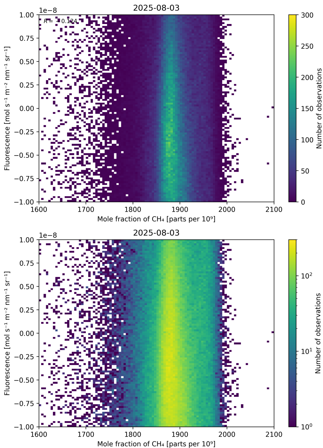
Figure 73: Scatter density plot of “Mole fraction of \text{CH}_4 ” against “Fluorescence” for 2025-08-03 to 2025-08-04.
