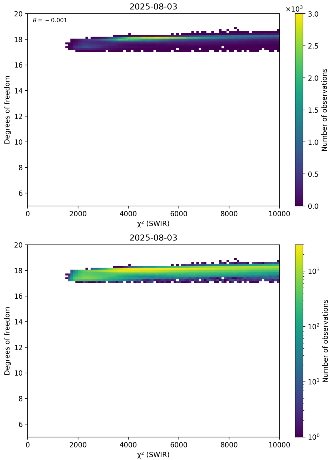
Figure 48: Scatter density plot of “ \chi^2 (SWIR)” against “Degrees of freedom” for 2025-08-03 to 2025-08-04.
