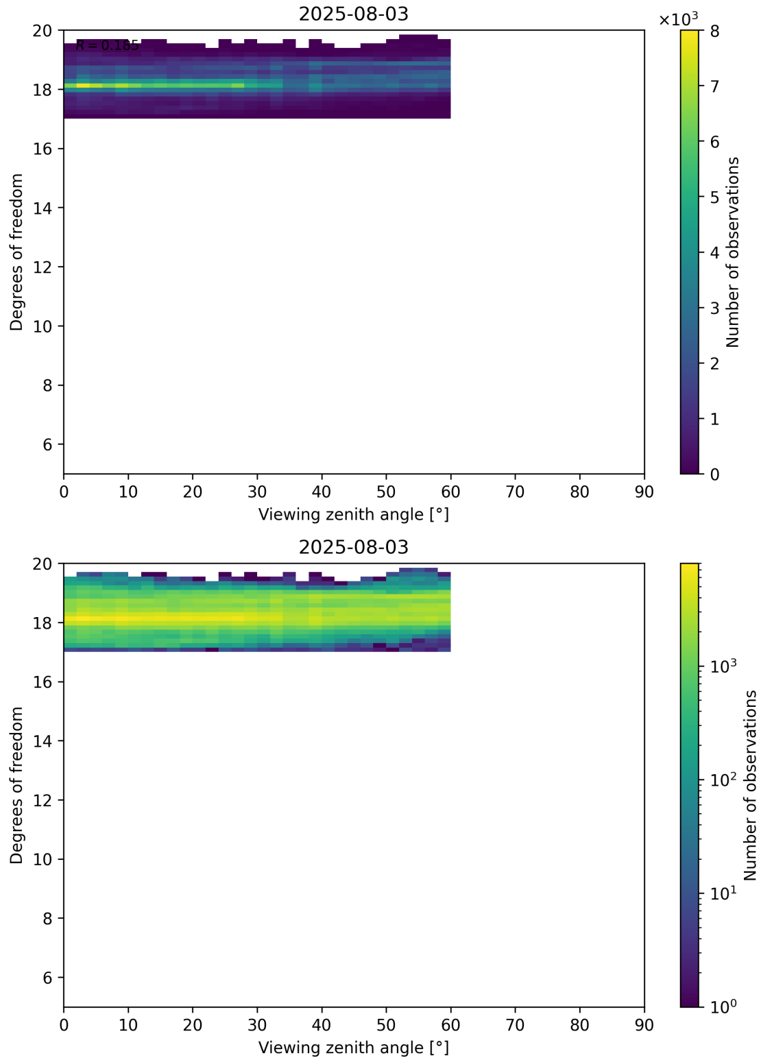
Figure 107: Scatter density plot of “Viewing zenith angle” against “Degrees of freedom” for 2025-08-03 to 2025-08-04.
