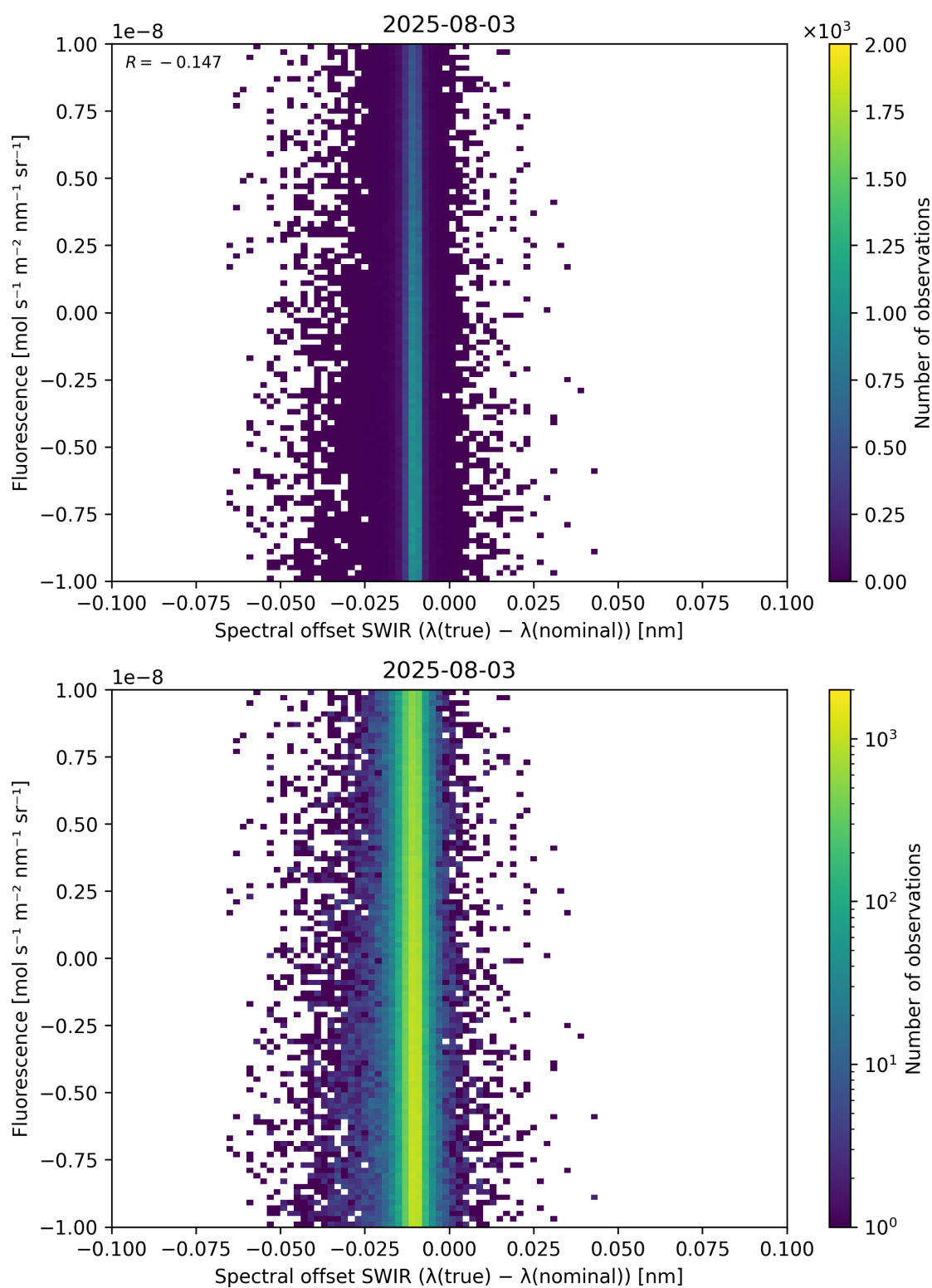
Figure 120: Scatter density plot of “Spectral offset SWIR ( \lambda_{\text{true}} - \lambda_{\text{nominal}} )” against “Fluorescence” for 2025-08-03 to 2025-08-04.
