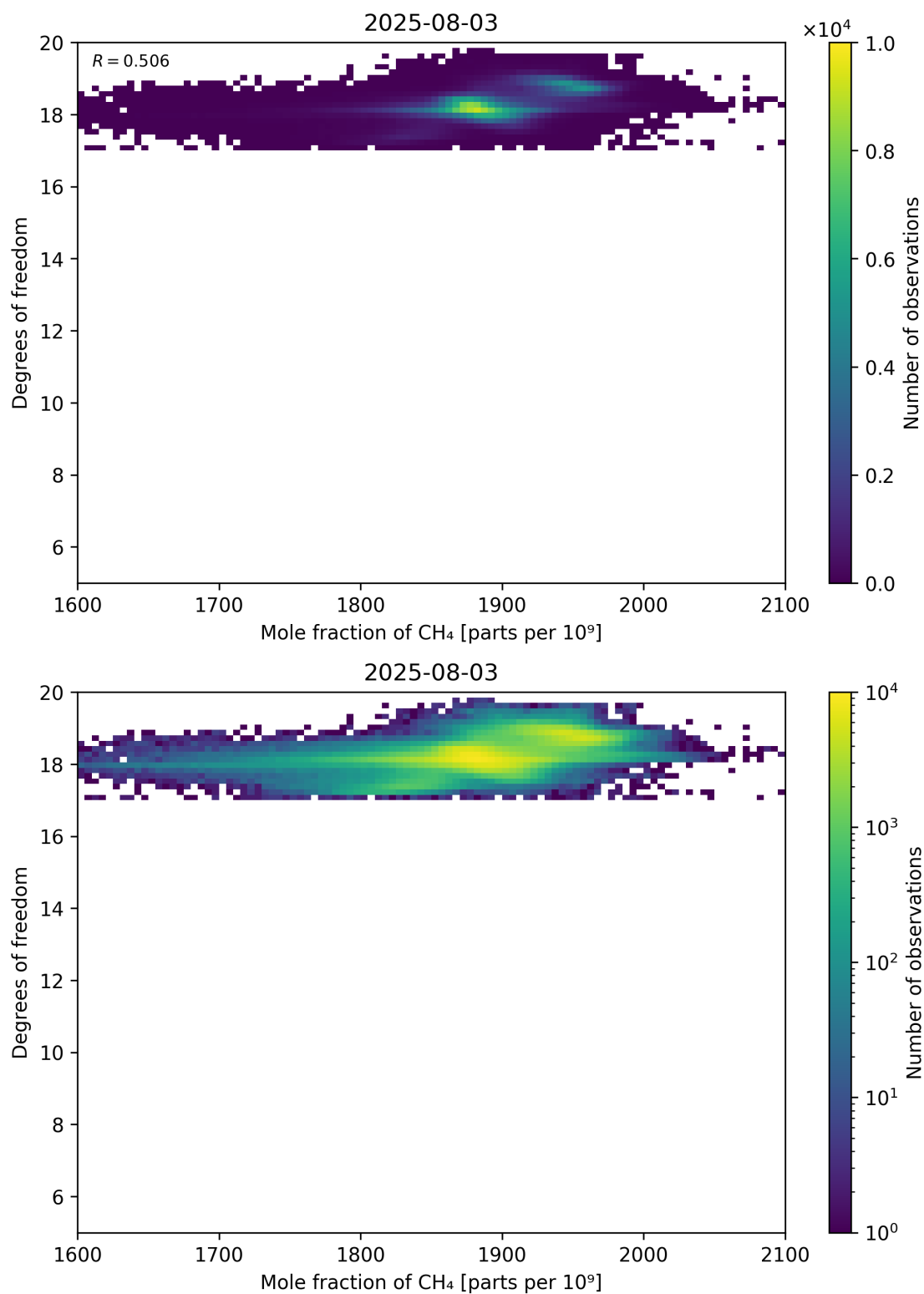
Figure 72: Scatter density plot of “Mole fraction of CH 4 ” against “Degrees of freedom” for 2025-08-03 to 2025-08-04.
