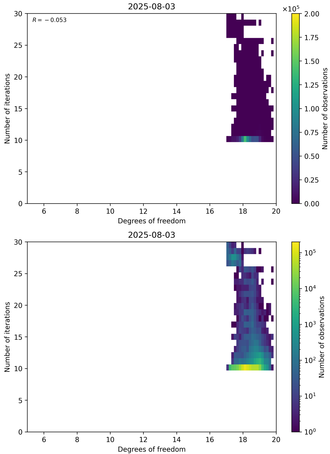
Figure 52: Scatter density plot of “Degrees of freedom” against “Number of iterations” for 2025-08-03 to 2025-08-04.
