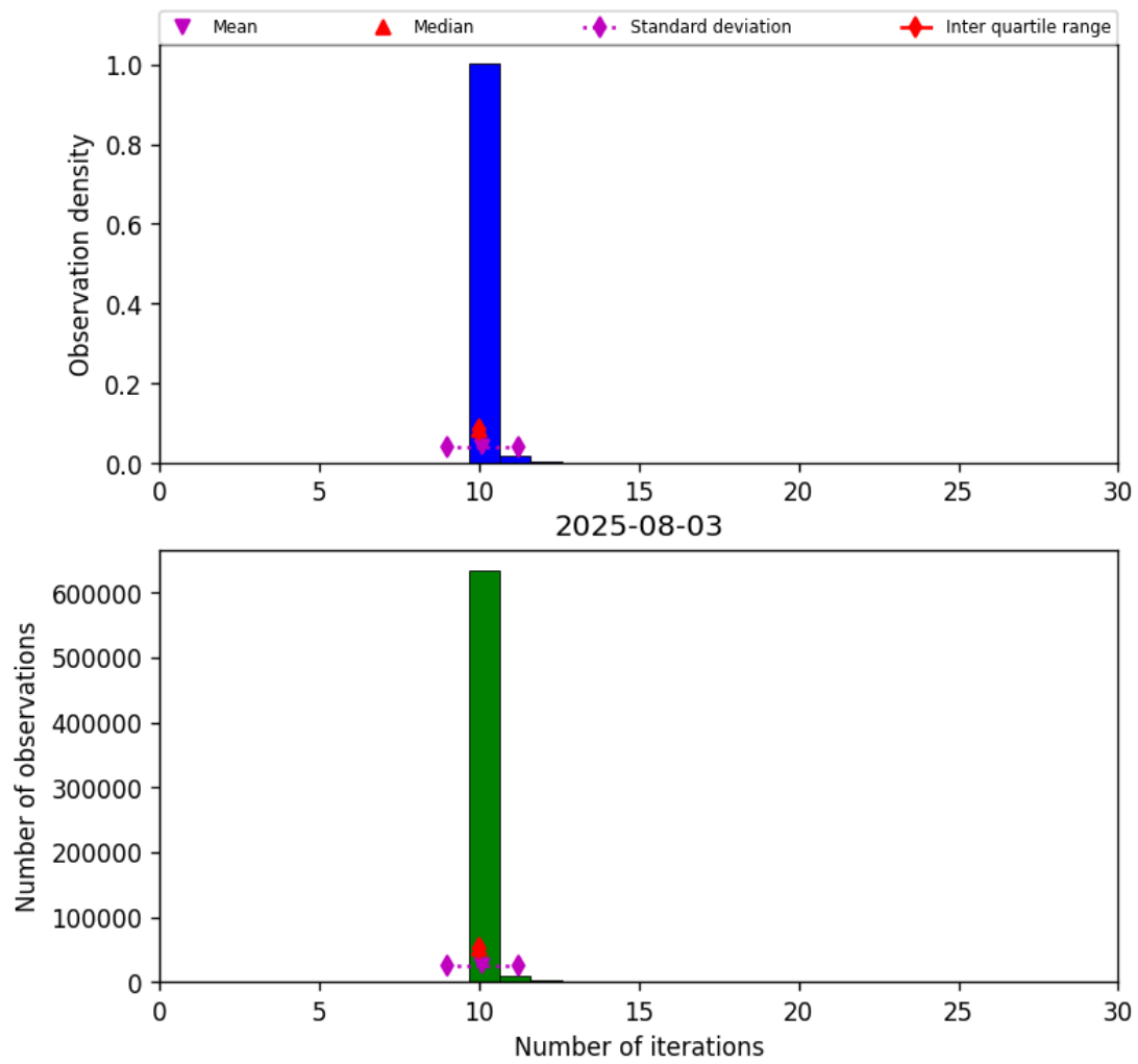
Figure 31: Histogram of “Number of iterations” for 2025-08-03 to 2025-08-04
