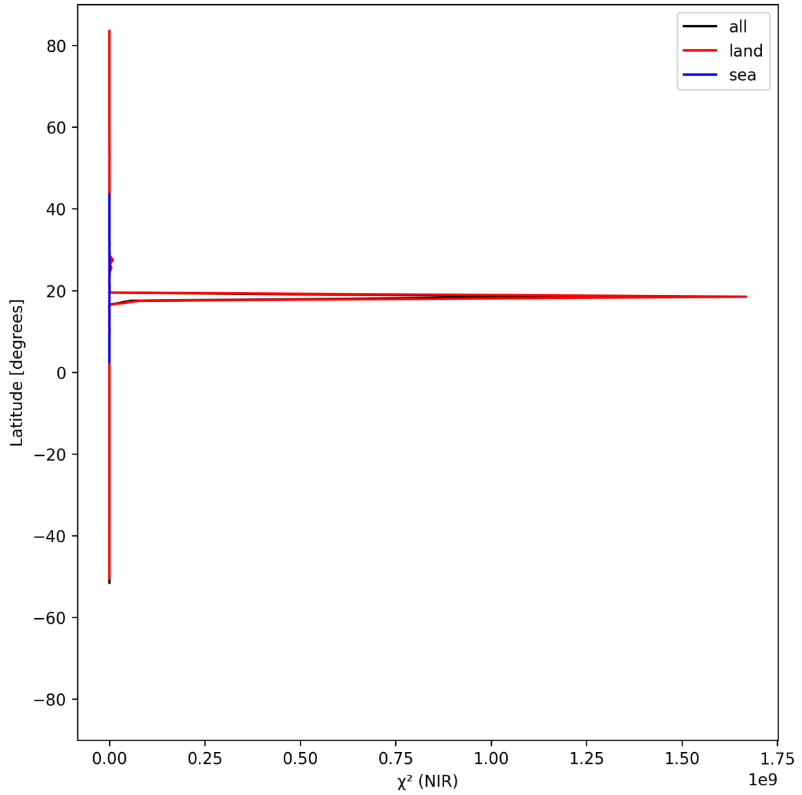
Figure 18: Zonal average of “ \chi^2 (NIR)” for 2025-08-03 to 2025-08-04.
