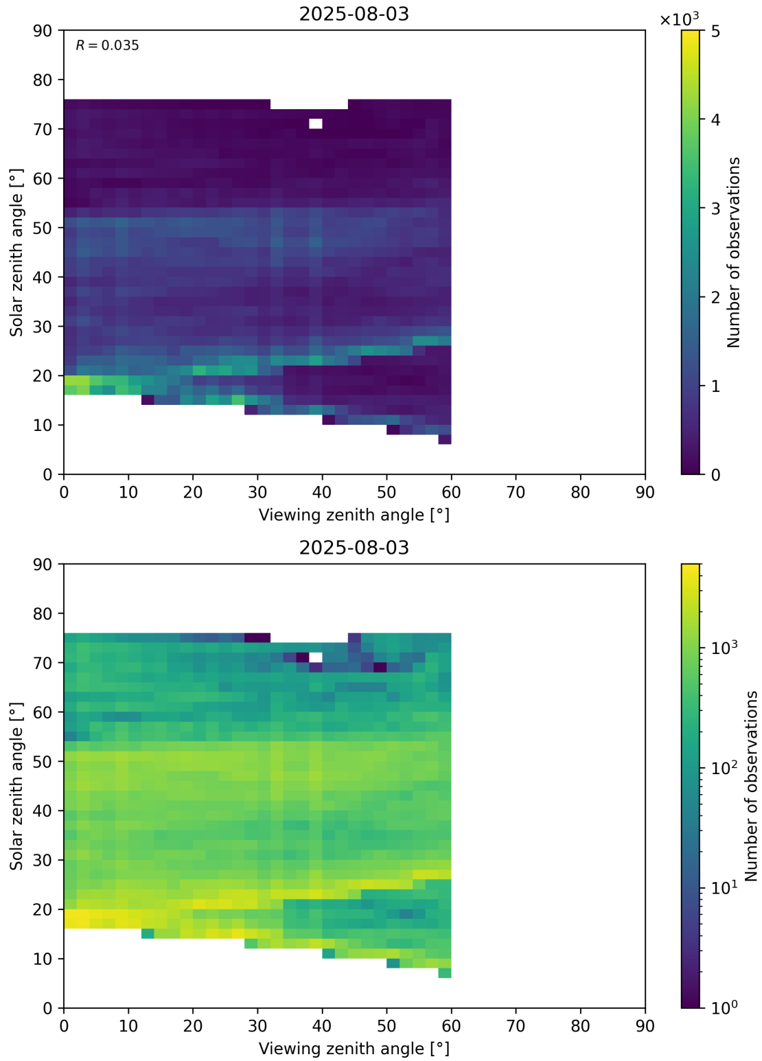
Figure 115: Scatter density plot of “Viewing zenith angle” against “Solar zenith angle” for 2025-08-03 to 2025-08-04.
