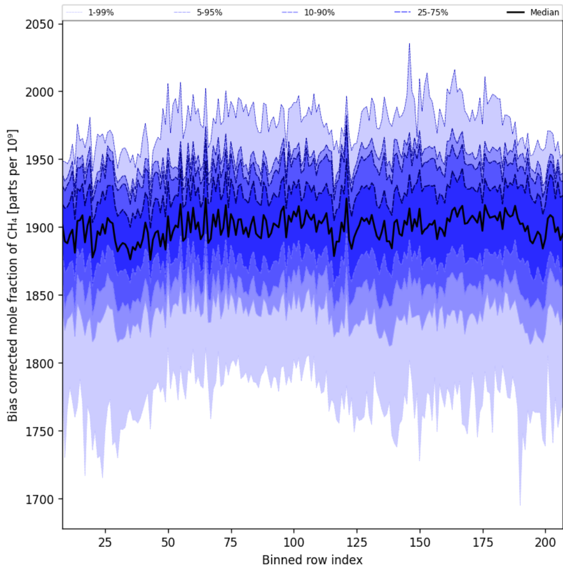
Figure 36: Along track statistics of “Bias corrected mole fraction of CH 4 ” for 2025-08-03 to 2025-08-04
