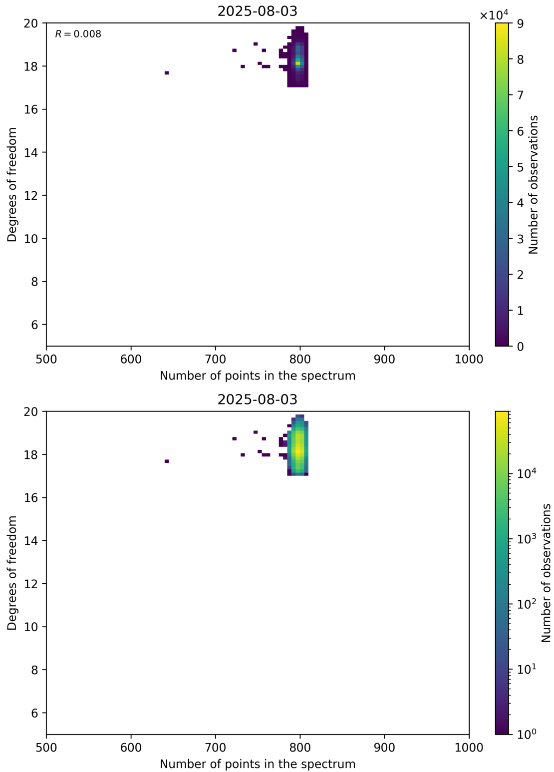
Figure 90: Scatter density plot of “Number of points in the spectrum” against “Degrees of freedom” for 2025-08-03 to 2025-08-04.
