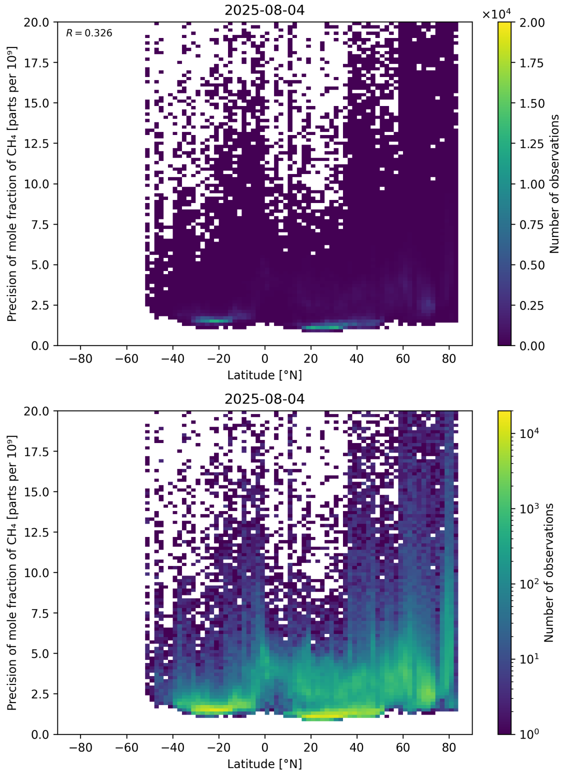
Figure 59: Scatter density plot of “Latitude” against “Precision of mole fraction of \text{CH}_4 ” for 2025-08-04 to 2025-08-05.
