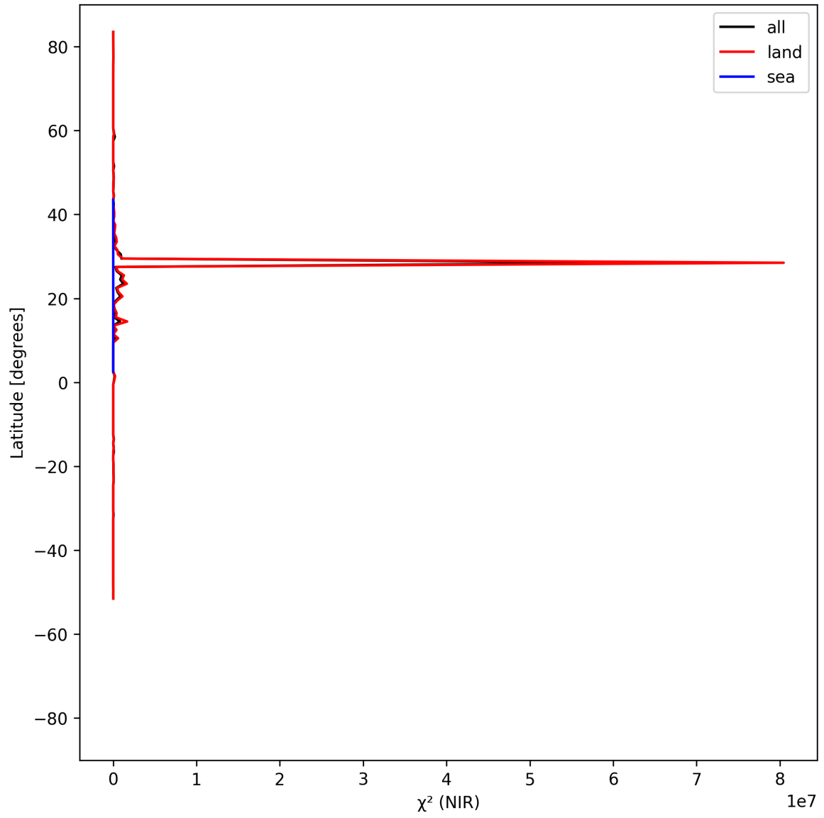
Figure 18: Zonal average of “ \chi^2 (NIR)” for 2025-08-04 to 2025-08-05.
