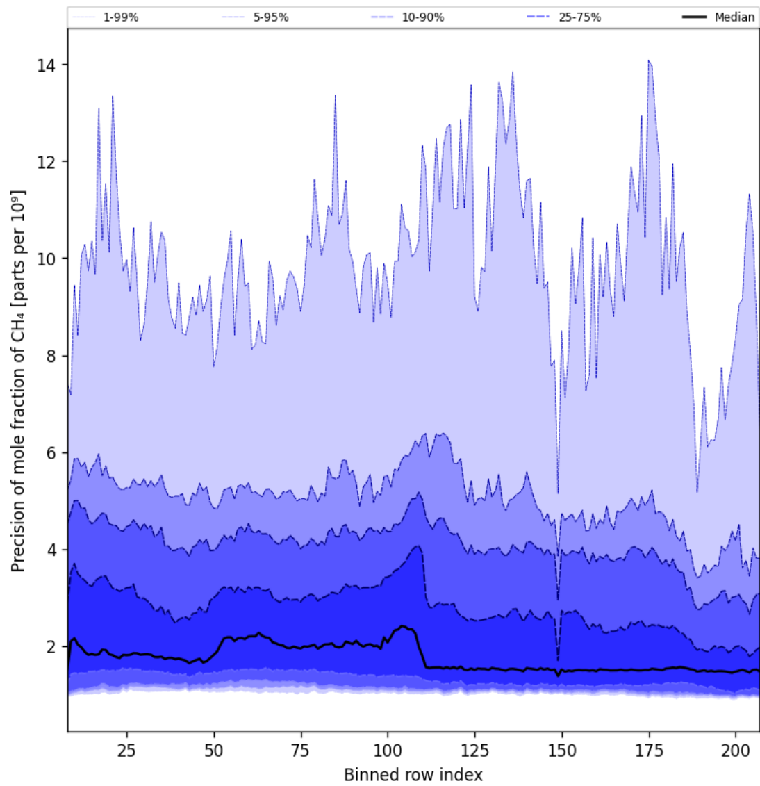
Figure 35: Along track statistics of “Precision of mole fraction of CH 4 ” for 2025-08-04 to 2025-08-05
