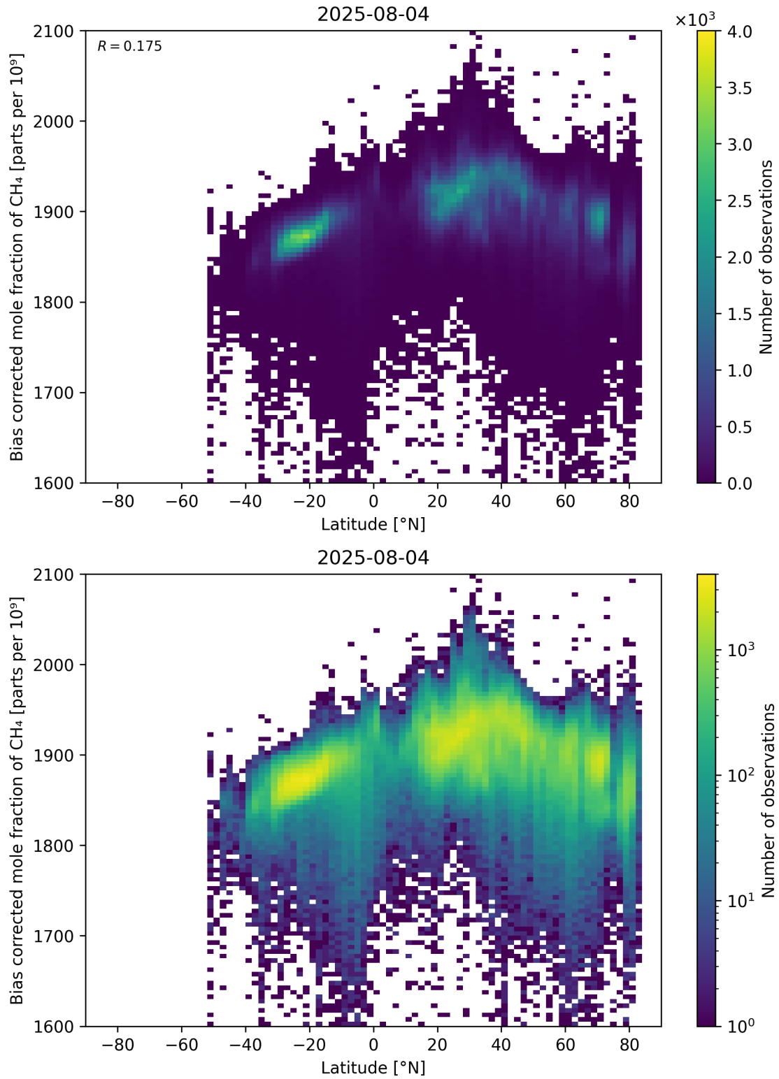
Figure 58: Scatter density plot of “Latitude” against “Bias corrected mole fraction of CH 4 ” for 2025-08-04 to 2025-08-05.
