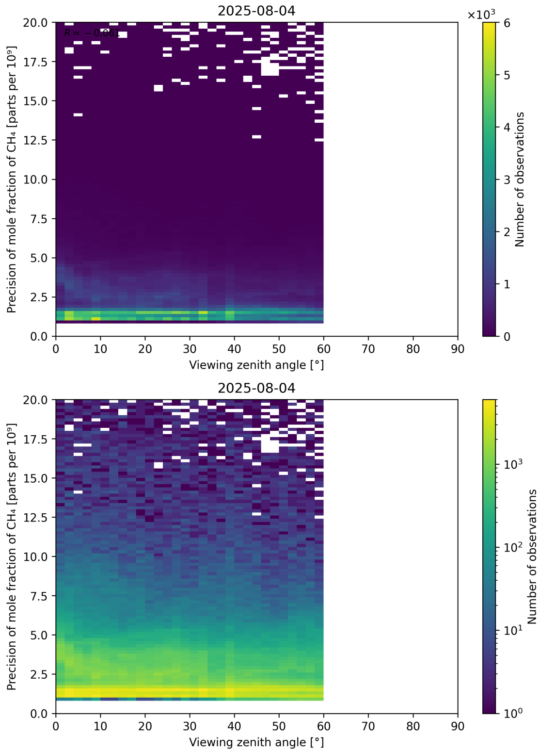
Figure 112: Scatter density plot of “Viewing zenith angle” against “Precision of mole fraction of CH 4 ” for 2025-08-04 to 2025-08-05.
