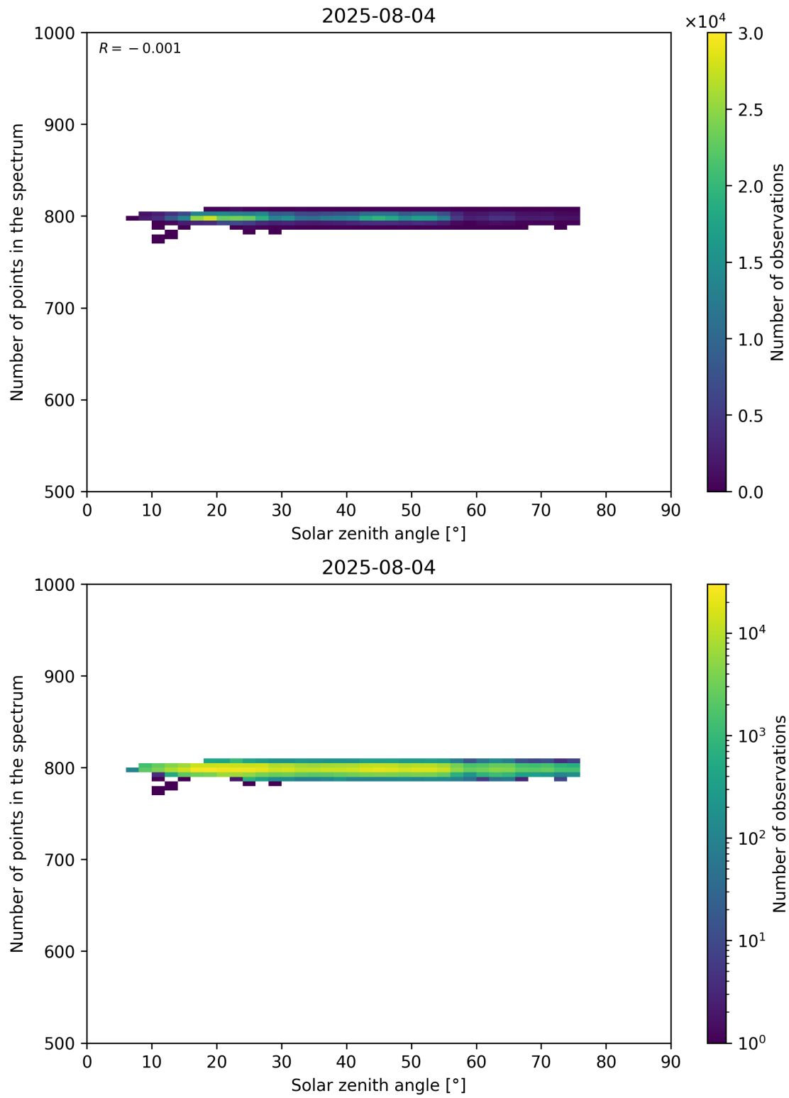
Figure 103: Scatter density plot of “Solar zenith angle” against “Number of points in the spectrum” for 2025-08-04 to 2025-08-05.
