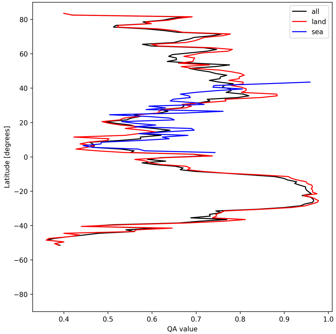
Figure 11: Zonal average of “QA value” for 2025-08-04 to 2025-08-05.
