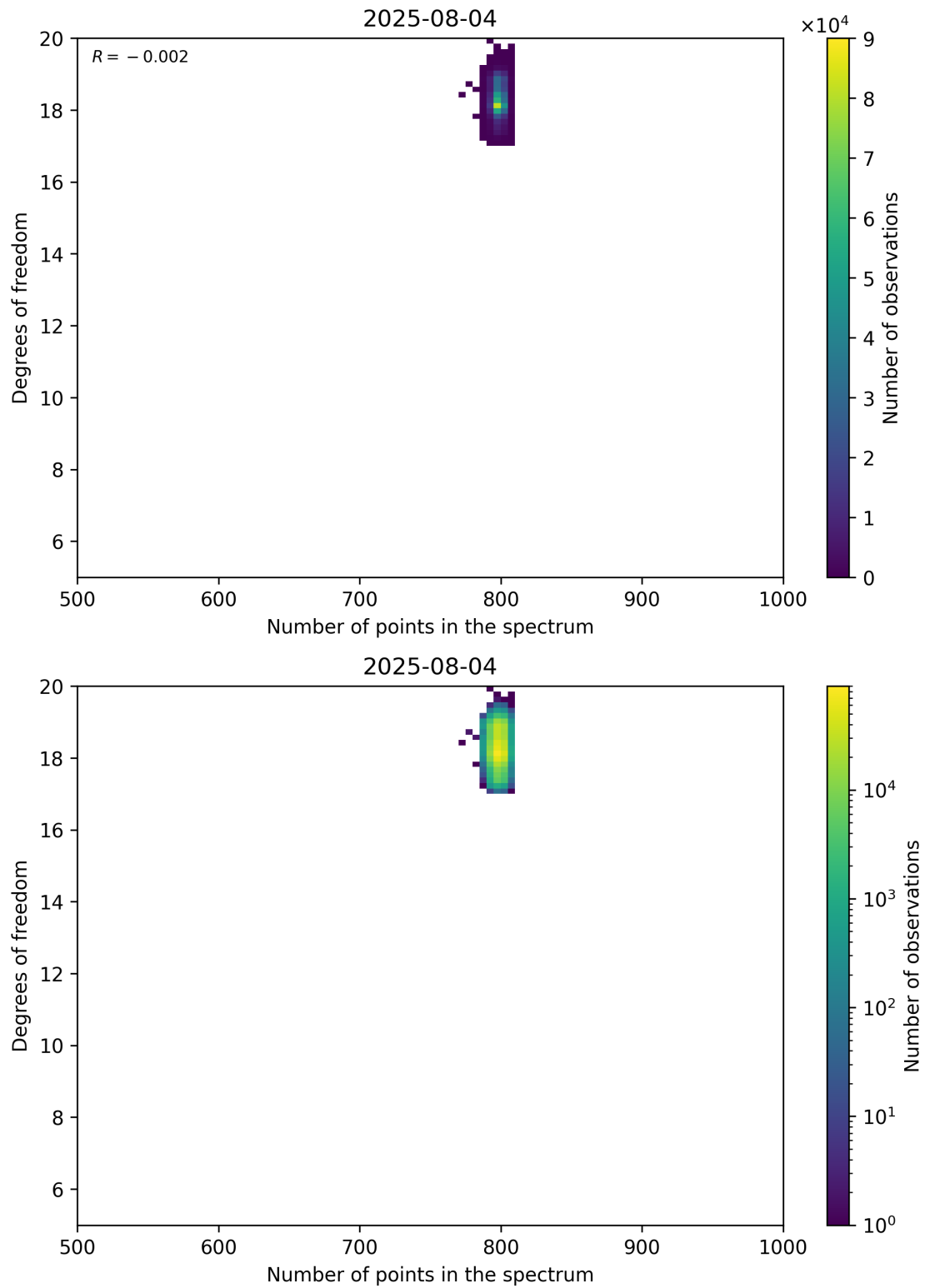
Figure 90: Scatter density plot of “Number of points in the spectrum” against “Degrees of freedom” for 2025-08-04 to 2025-08-05.
