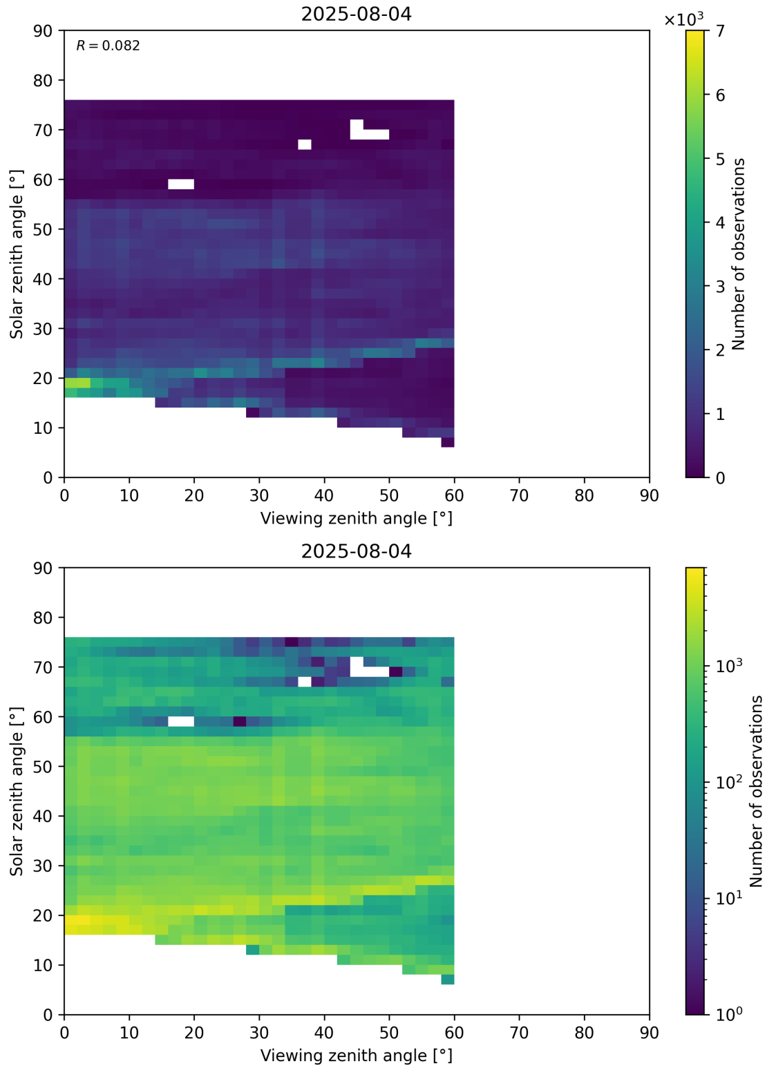
Figure 115: Scatter density plot of “Viewing zenith angle” against “Solar zenith angle” for 2025-08-04 to 2025-08-05.
