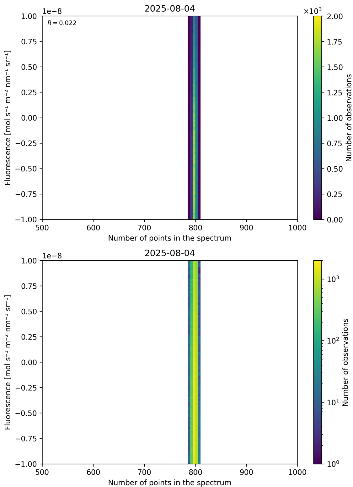
Figure 91: Scatter density plot of “Number of points in the spectrum” against “Fluorescence” for 2025-08-04 to 2025-08-05.
