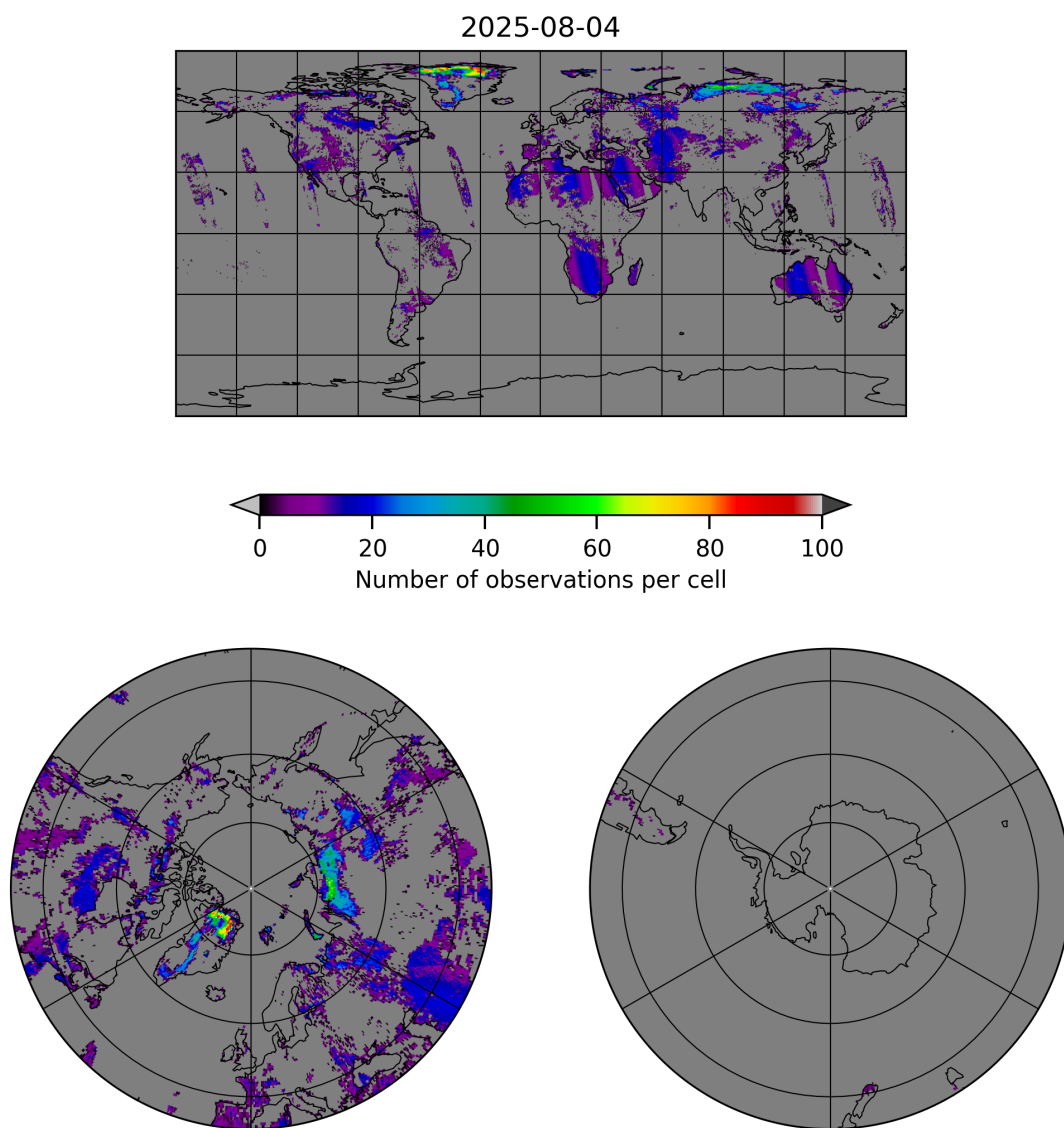
Figure 10: Map of the number of observations for 2025-08-04 to 2025-08-05
