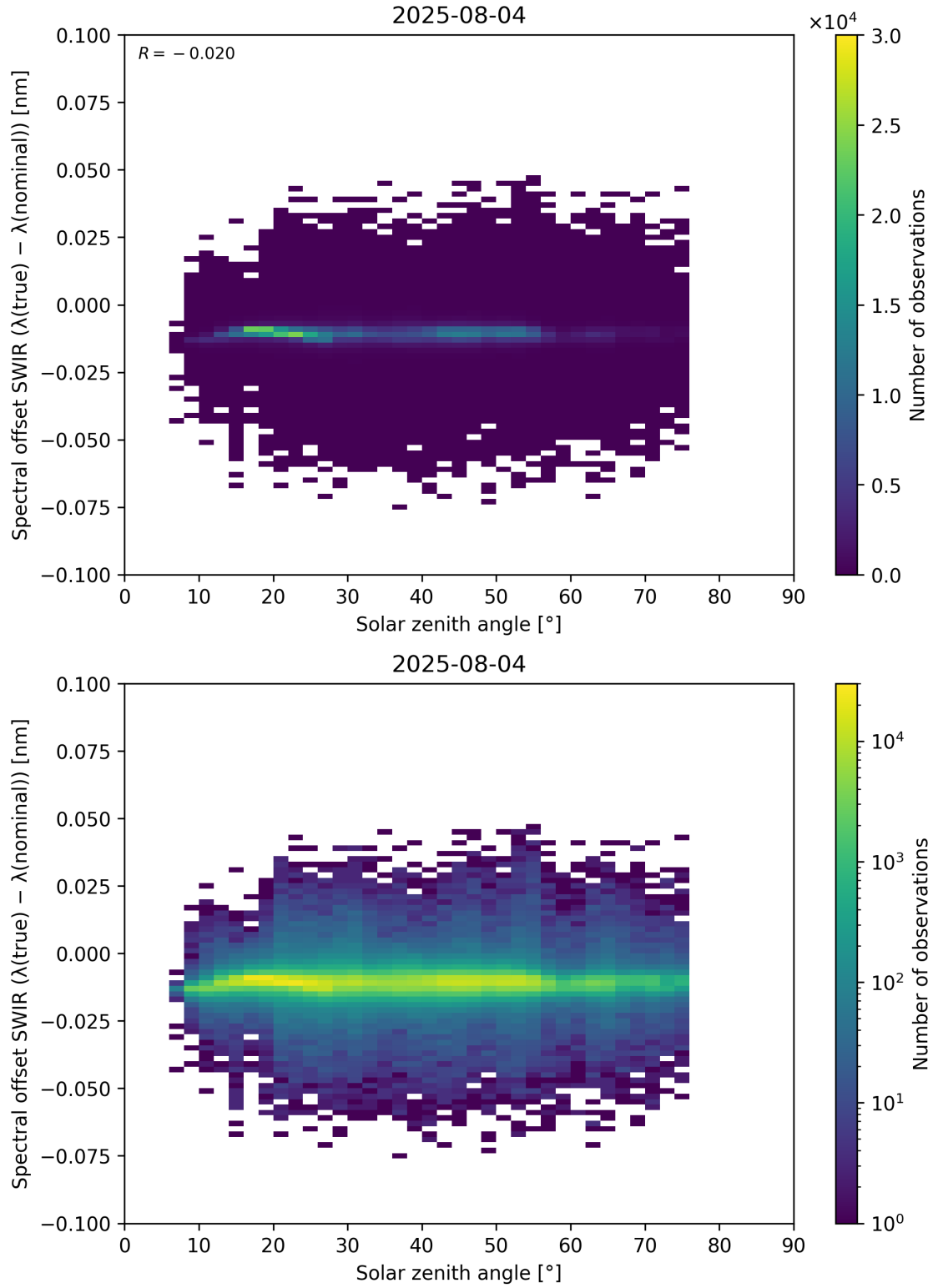
Figure 104: Scatter density plot of “Solar zenith angle” against “Spectral offset SWIR ( \lambda_{\text{true}} - \lambda_{\text{nominal}} )” for 2025-08-04 to 2025-08-05.
