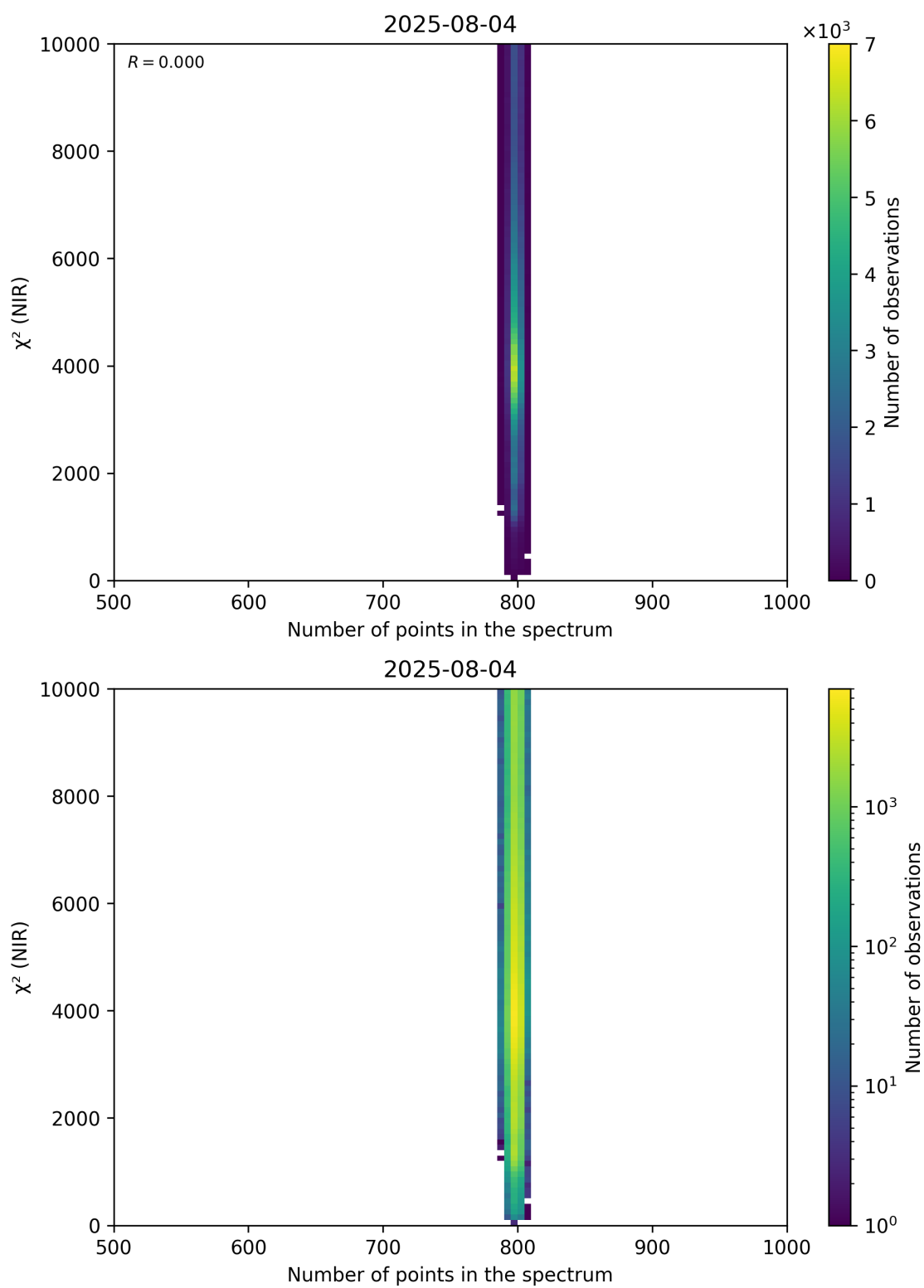
Figure 88: Scatter density plot of “Number of points in the spectrum” against “ \chi^2 (NIR)” for 2025-08-04 to 2025-08-05.
