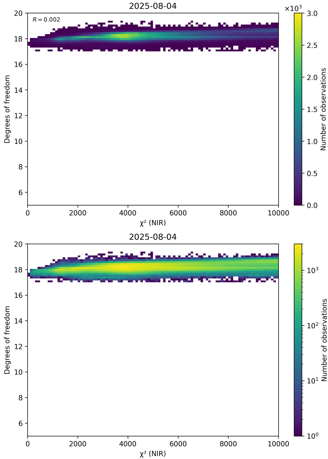
Figure 44: Scatter density plot of “ \chi^2 (NIR)” against “Degrees of freedom” for 2025-08-04 to 2025-08-05.
