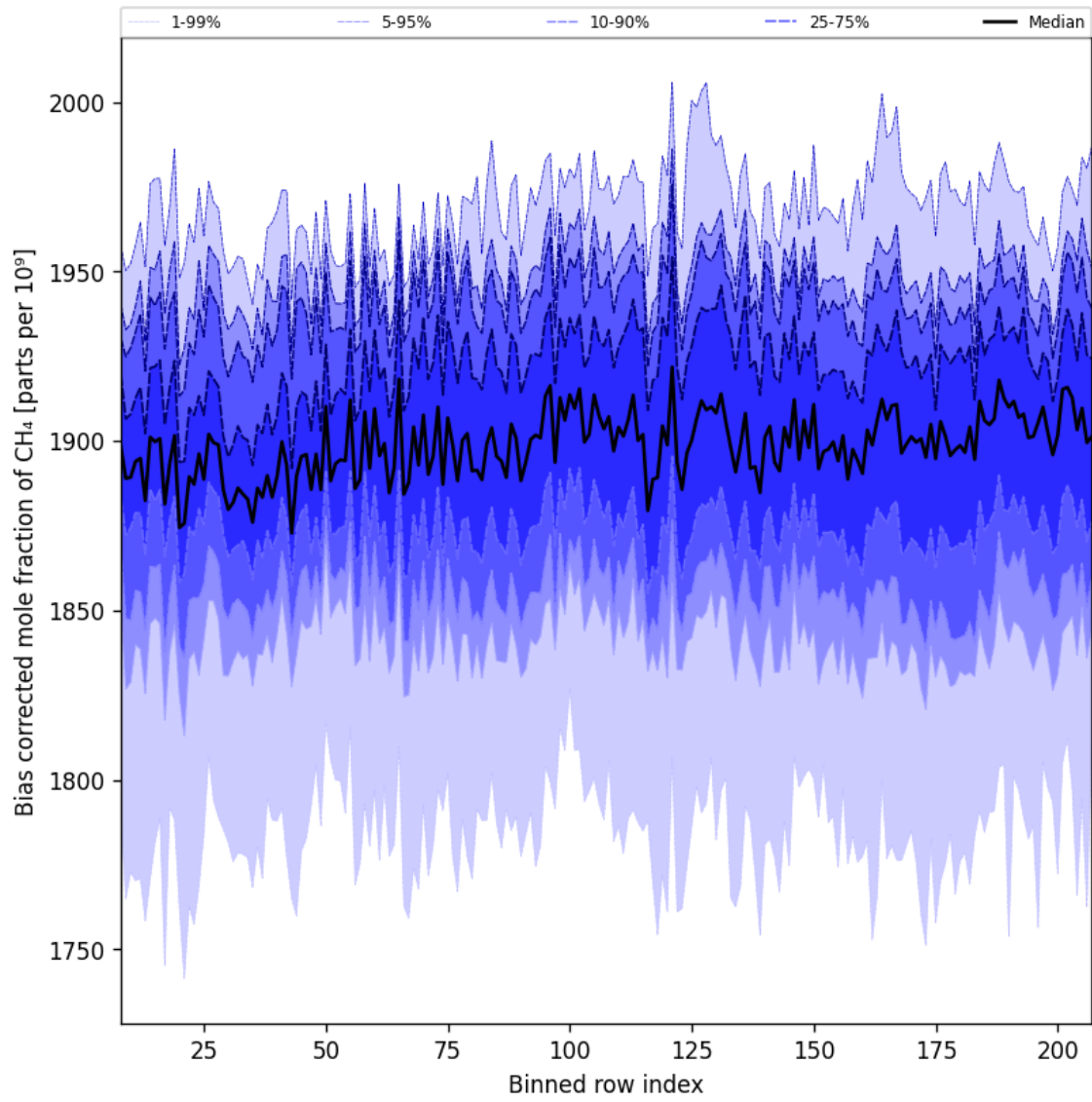
Figure 36: Along track statistics of “Bias corrected mole fraction of \text{CH}_4 ” for 2025-08-04 to 2025-08-05
