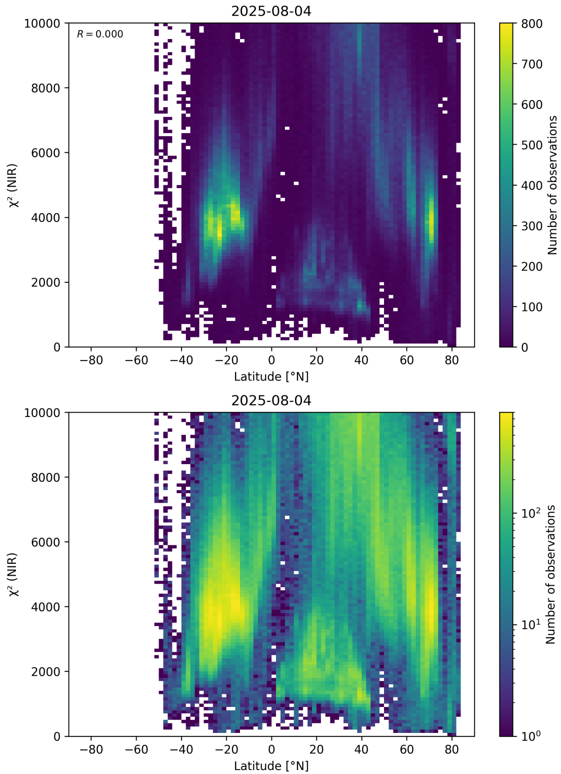
Figure 53: Scatter density plot of “Latitude” against “ \chi^2 (NIR)” for 2025-08-04 to 2025-08-05.
