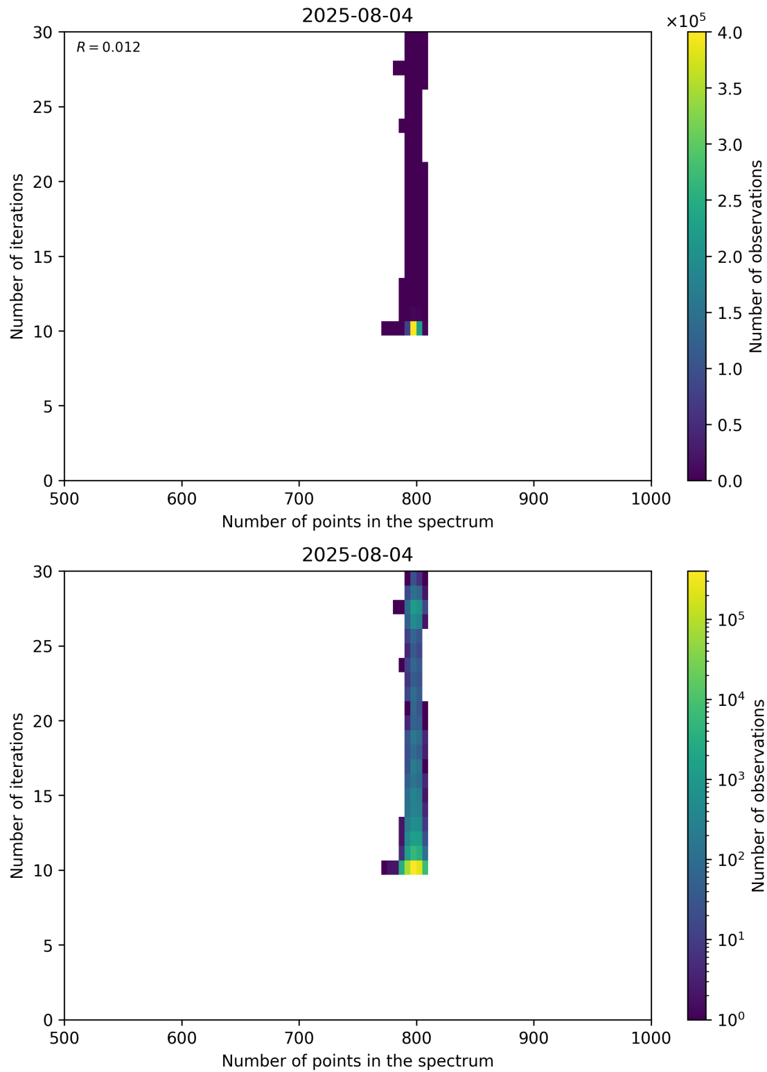
Figure 92: Scatter density plot of “Number of points in the spectrum” against “Number of iterations” for 2025-08-04 to 2025-08-05.
