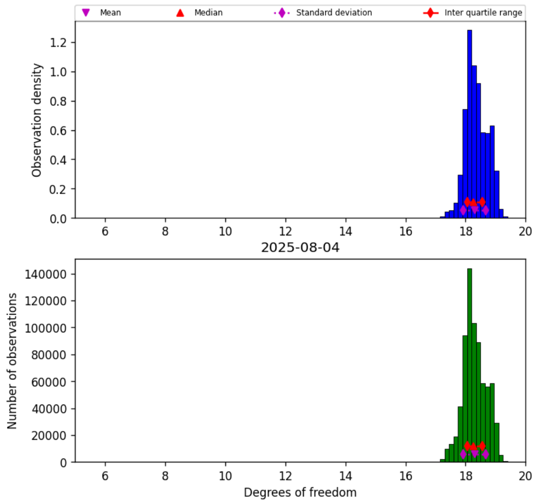
Figure 30: Histogram of “Degrees of freedom” for 2025-08-04 to 2025-08-05
