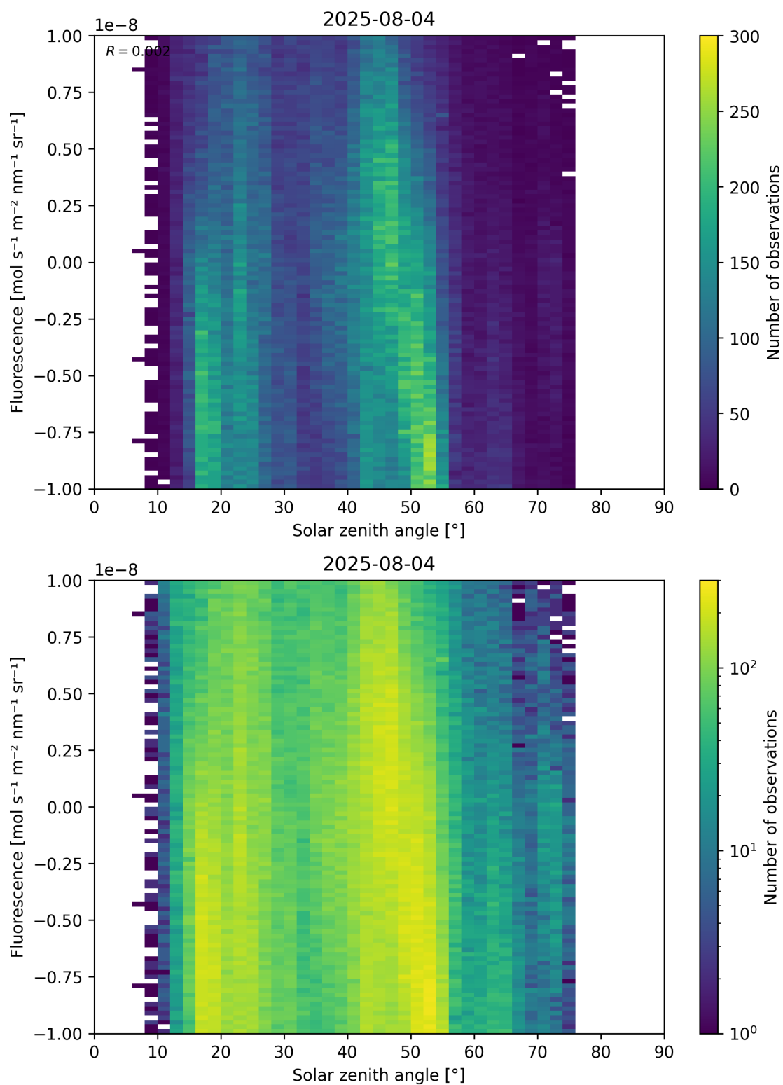
Figure 97: Scatter density plot of “Solar zenith angle” against “Fluorescence” for 2025-08-04 to 2025-08-05.
