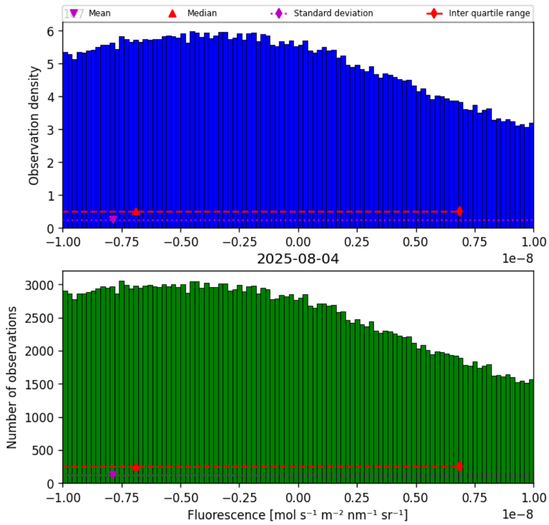
Figure 32: Histogram of “Fluorescence” for 2025-08-04 to 2025-08-05
