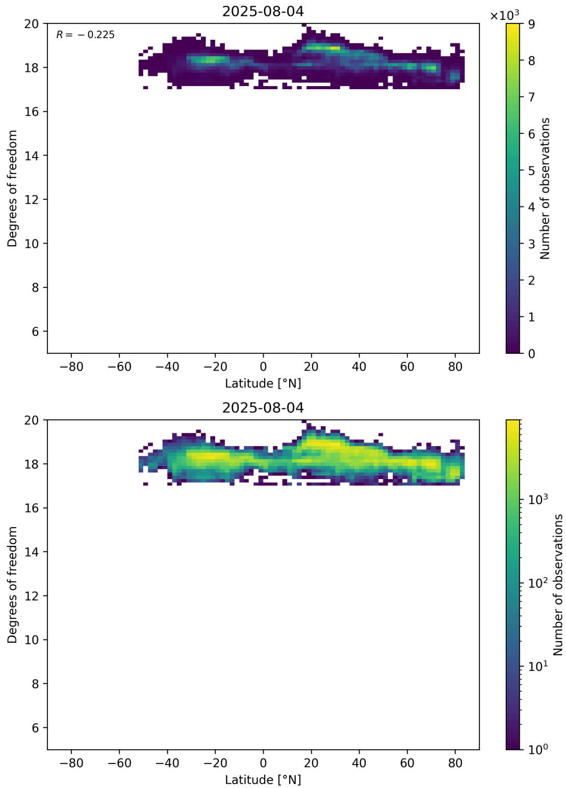
Figure 55: Scatter density plot of “Latitude” against “Degrees of freedom” for 2025-08-04 to 2025-08-05.
