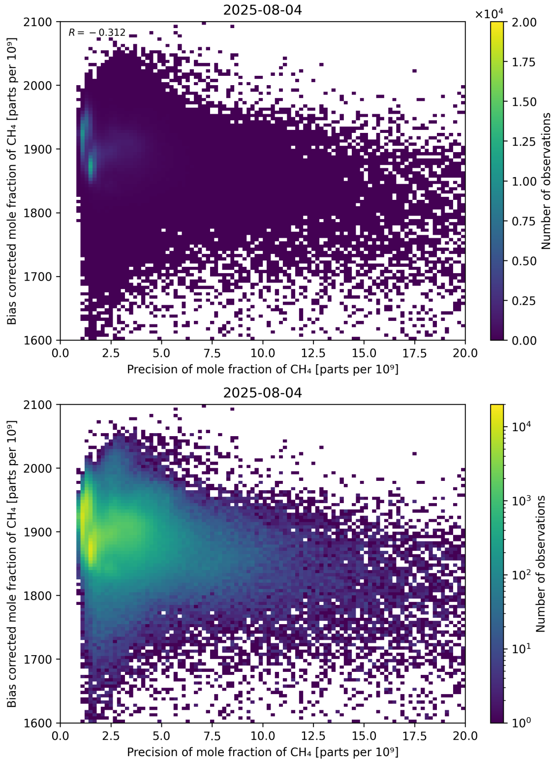
Figure 82: Scatter density plot of “Precision of mole fraction of CH 4 ” against “Bias corrected mole fraction of CH 4 ” for 2025-08-04 to 2025-08-05.
