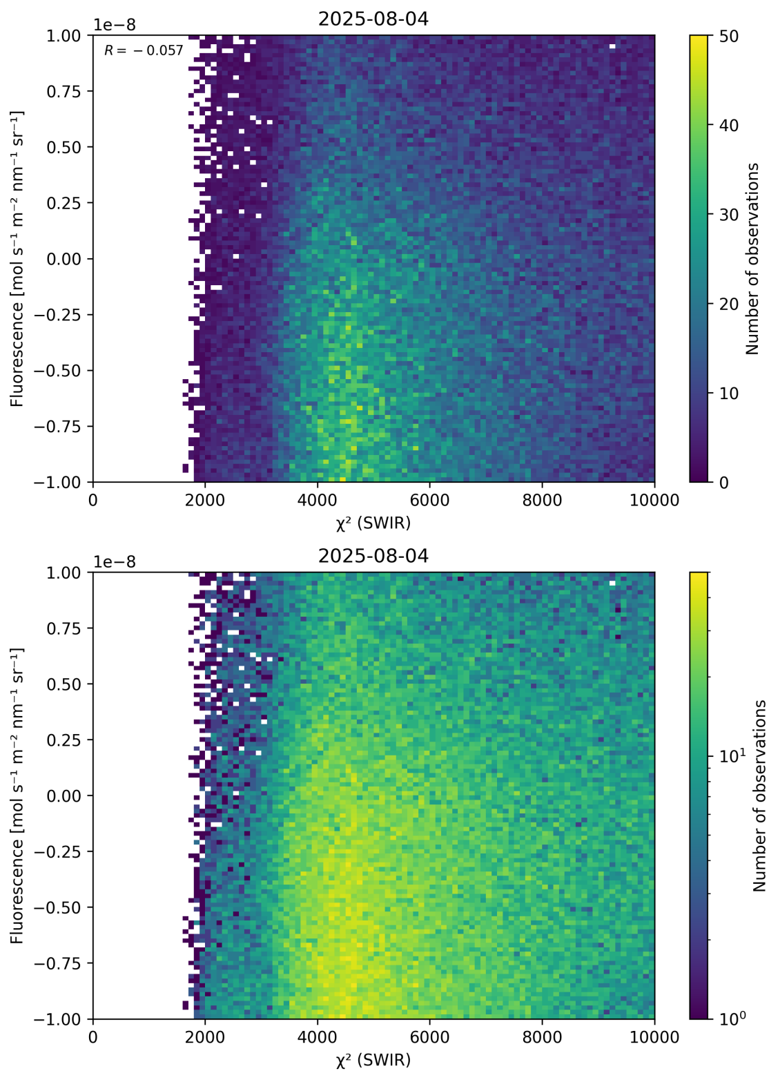
Figure 49: Scatter density plot of “ \chi^2 (SWIR)” against “Fluorescence” for 2025-08-04 to 2025-08-05.
