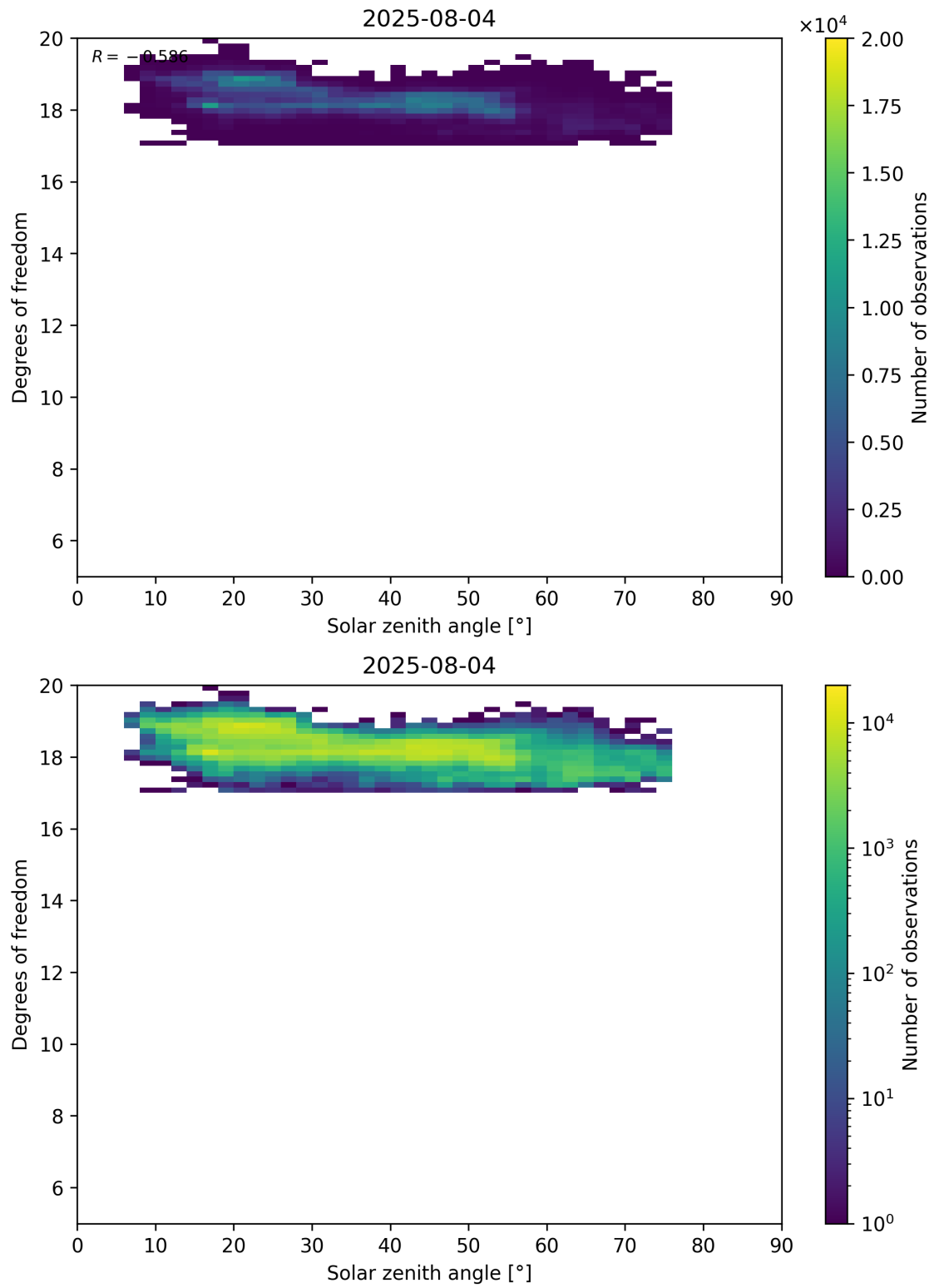
Figure 96: Scatter density plot of “Solar zenith angle” against “Degrees of freedom” for 2025-08-04 to 2025-08-05.
