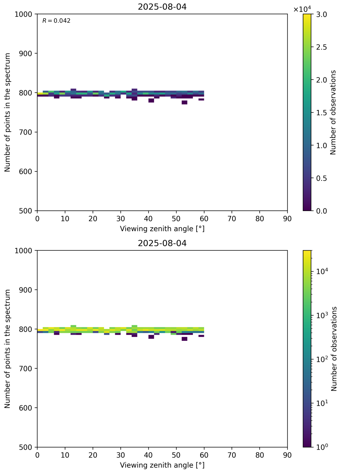
Figure 114: Scatter density plot of “Viewing zenith angle” against “Number of points in the spectrum” for 2025-08-04 to 2025-08-05.
