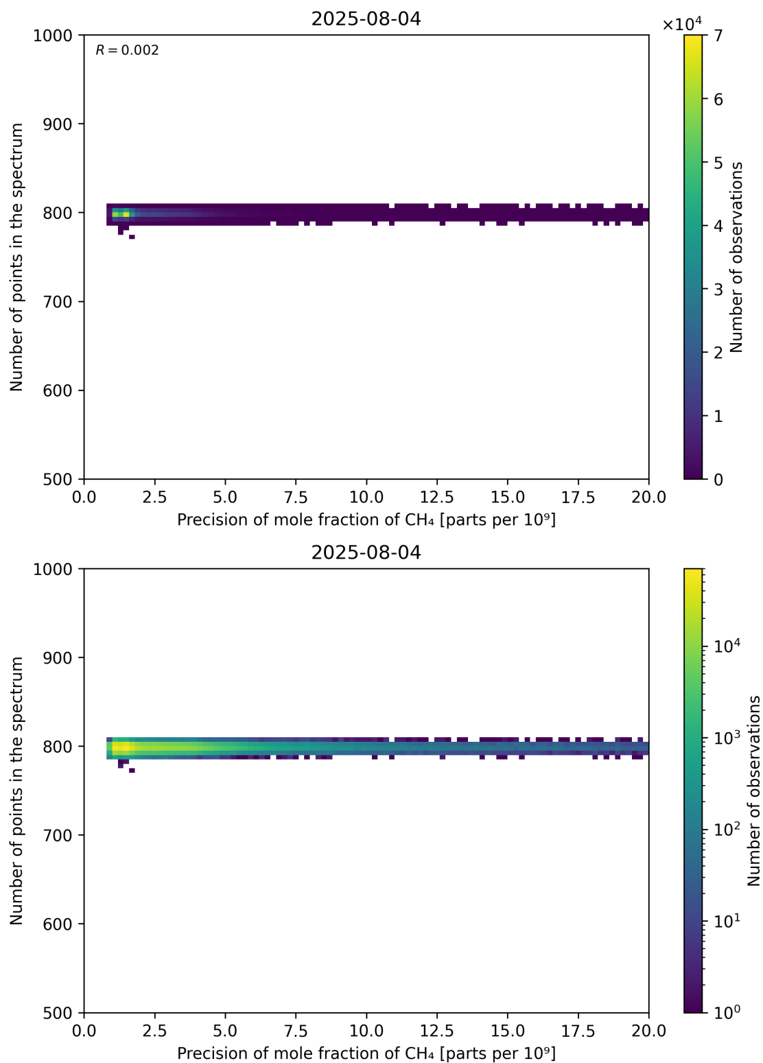
Figure 84: Scatter density plot of “Precision of mole fraction of CH 4 ” against “Number of points in the spectrum” for 2025-08-04 to 2025-08-05.
