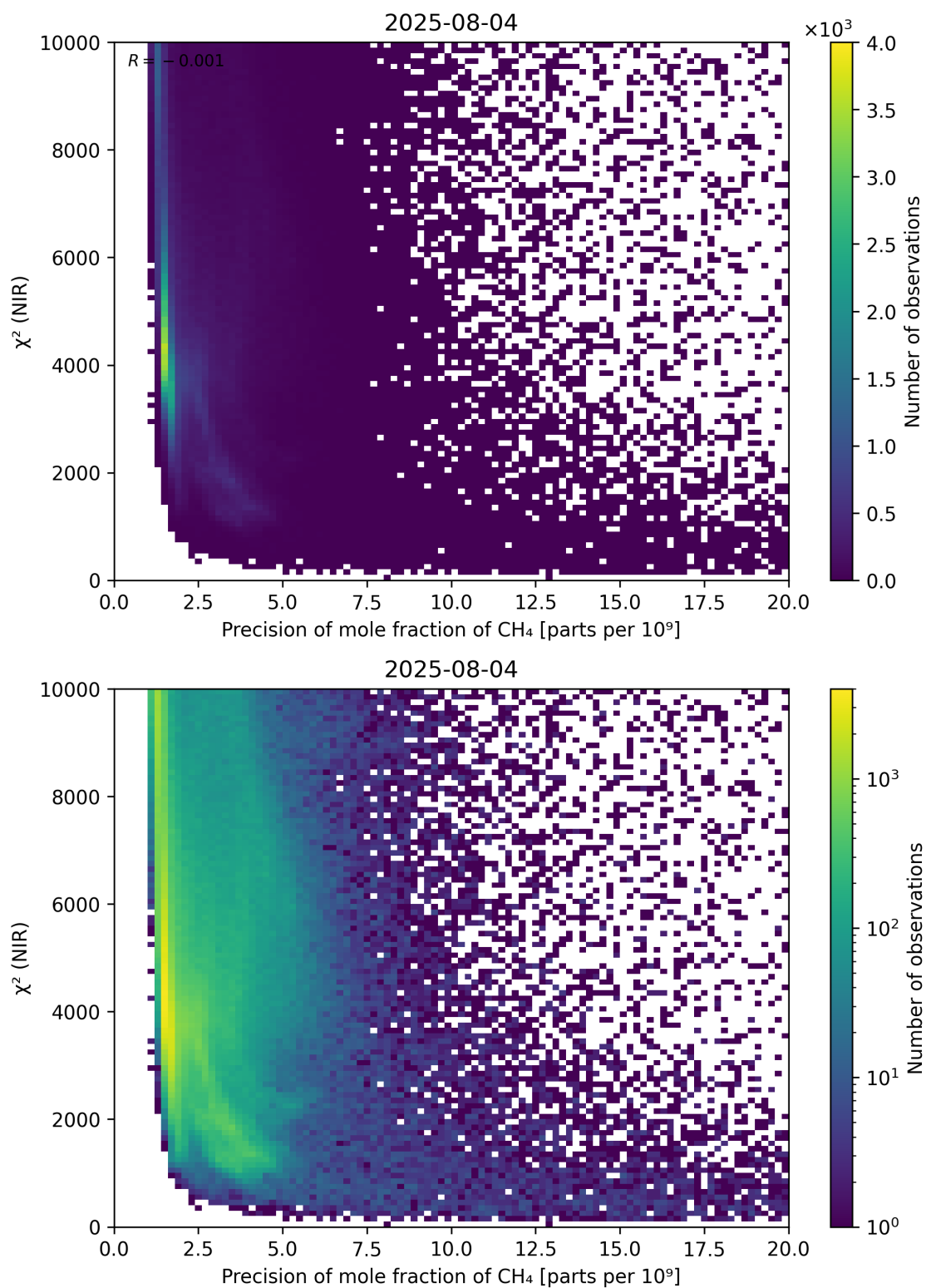
Figure 78: Scatter density plot of “Precision of mole fraction of CH 4 ” against “ \chi^2 (NIR)” for 2025-08-04 to 2025-08-05.
