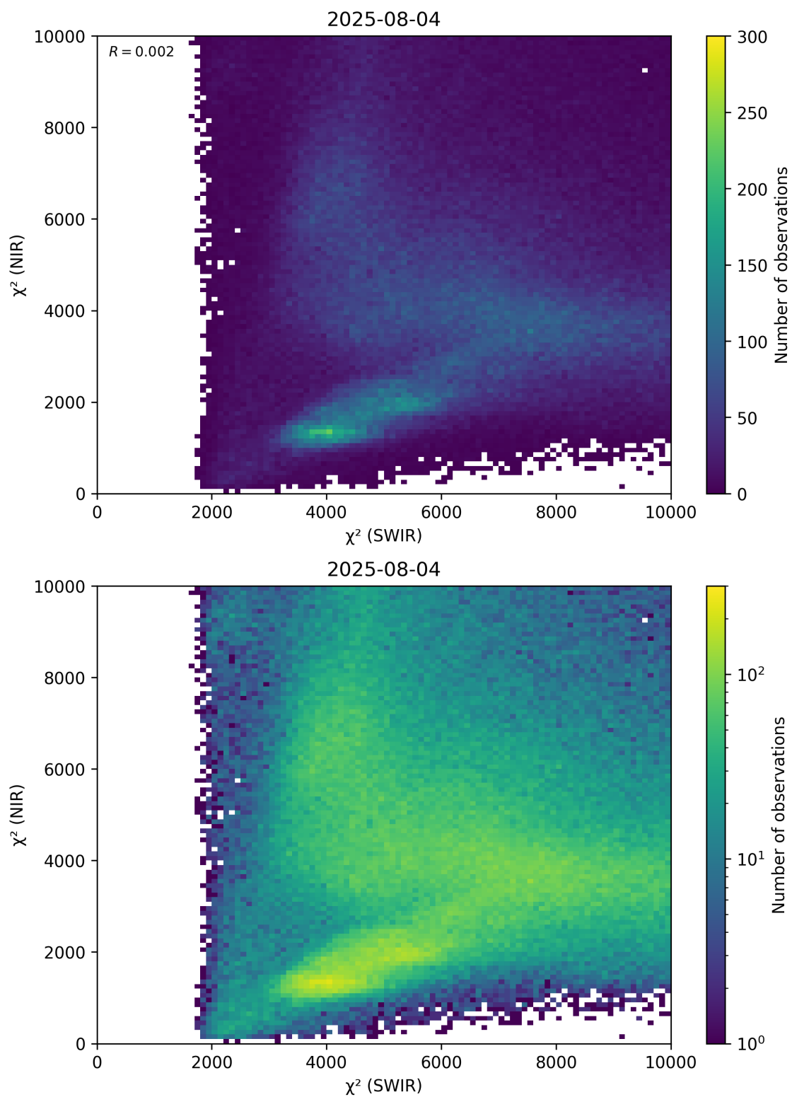
Figure 47: Scatter density plot of “ \chi^2 (SWIR)” against “ \chi^2 (NIR)” for 2025-08-04 to 2025-08-05.
