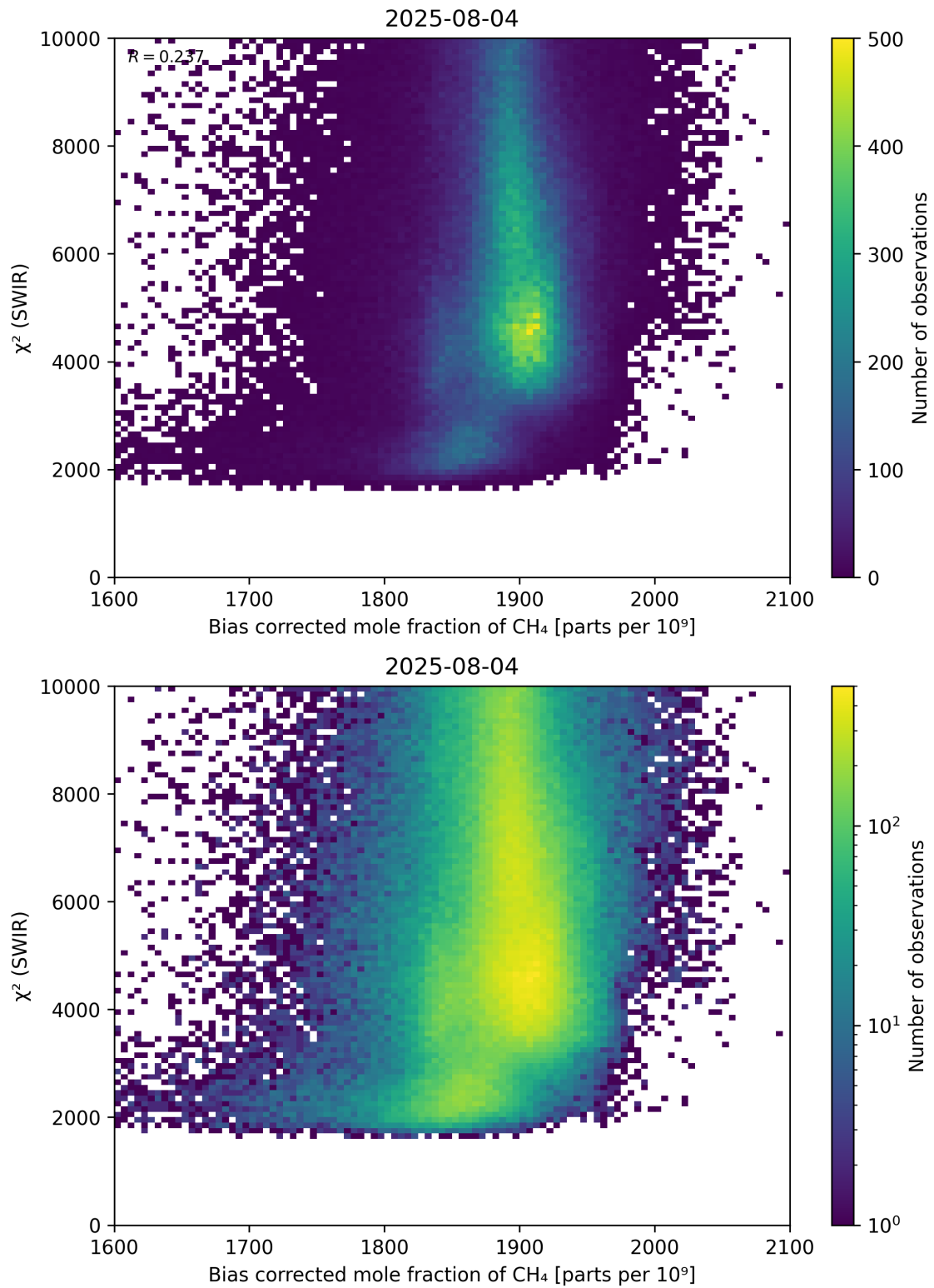
Figure 64: Scatter density plot of “Bias corrected mole fraction of \text{CH}_4 ” against “ \chi^2 (SWIR)” for 2025-08-04 to 2025-08-05.
