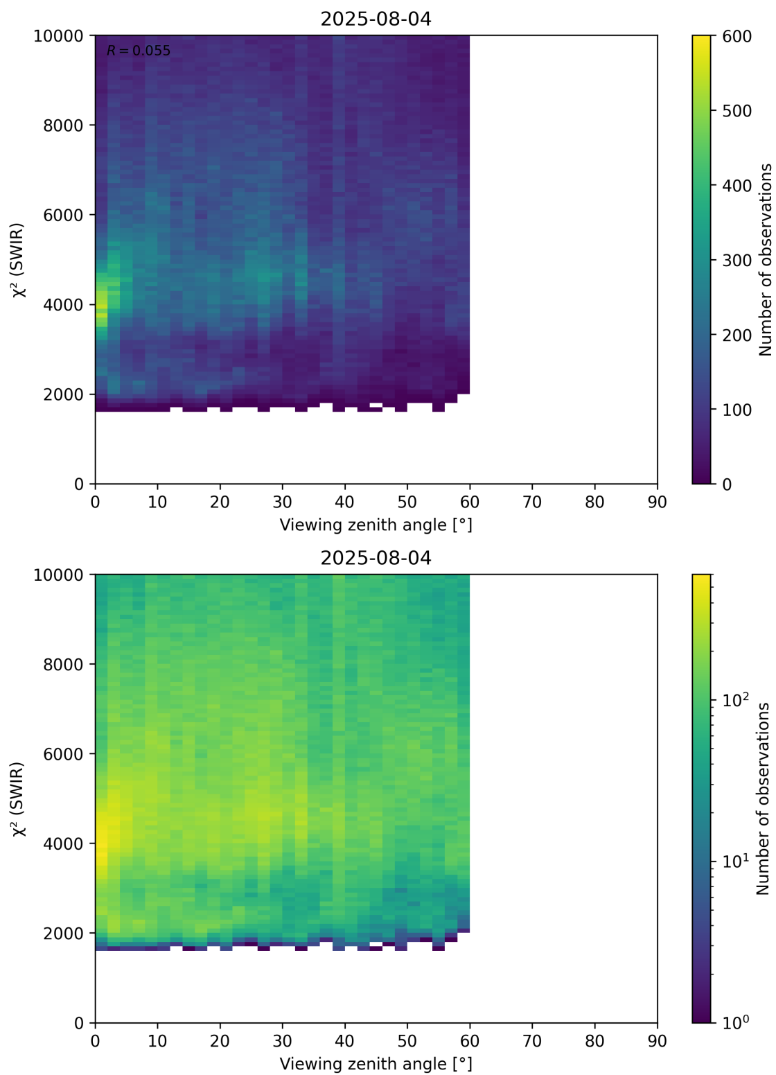
Figure 106: Scatter density plot of “Viewing zenith angle” against “ \chi^2 (SWIR)” for 2025-08-04 to 2025-08-05.
