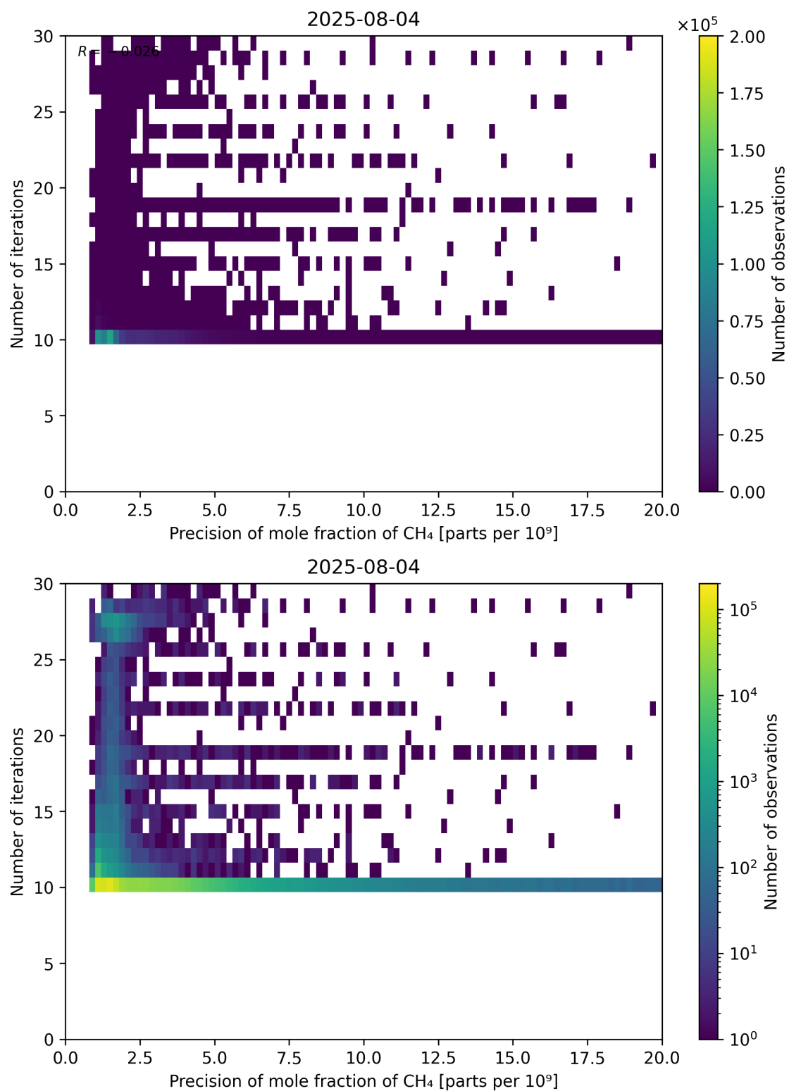
Figure 83: Scatter density plot of “Precision of mole fraction of CH 4 ” against “Number of iterations” for 2025-08-04 to 2025-08-05.
