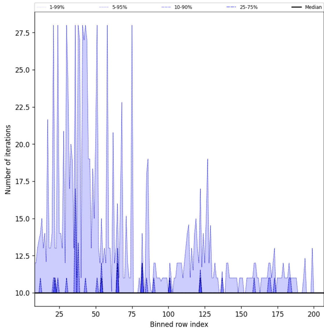
Figure 42: Along track statistics of “Number of iterations” for 2025-08-04 to 2025-08-05
