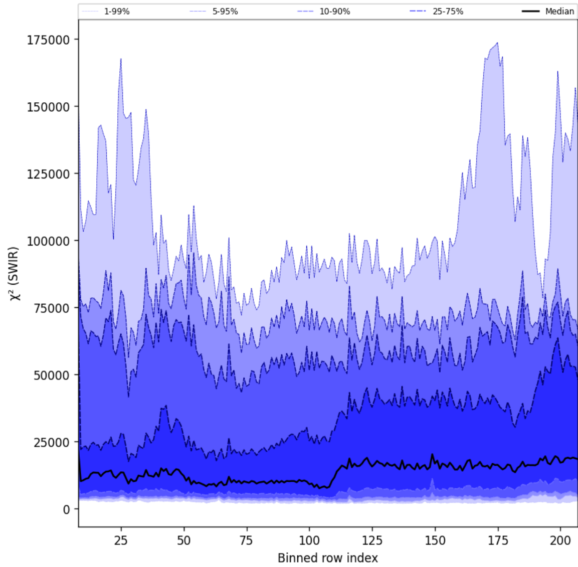
Figure 39: Along track statistics of " \chi^2 (SWIR)" for 2025-08-04 to 2025-08-05
