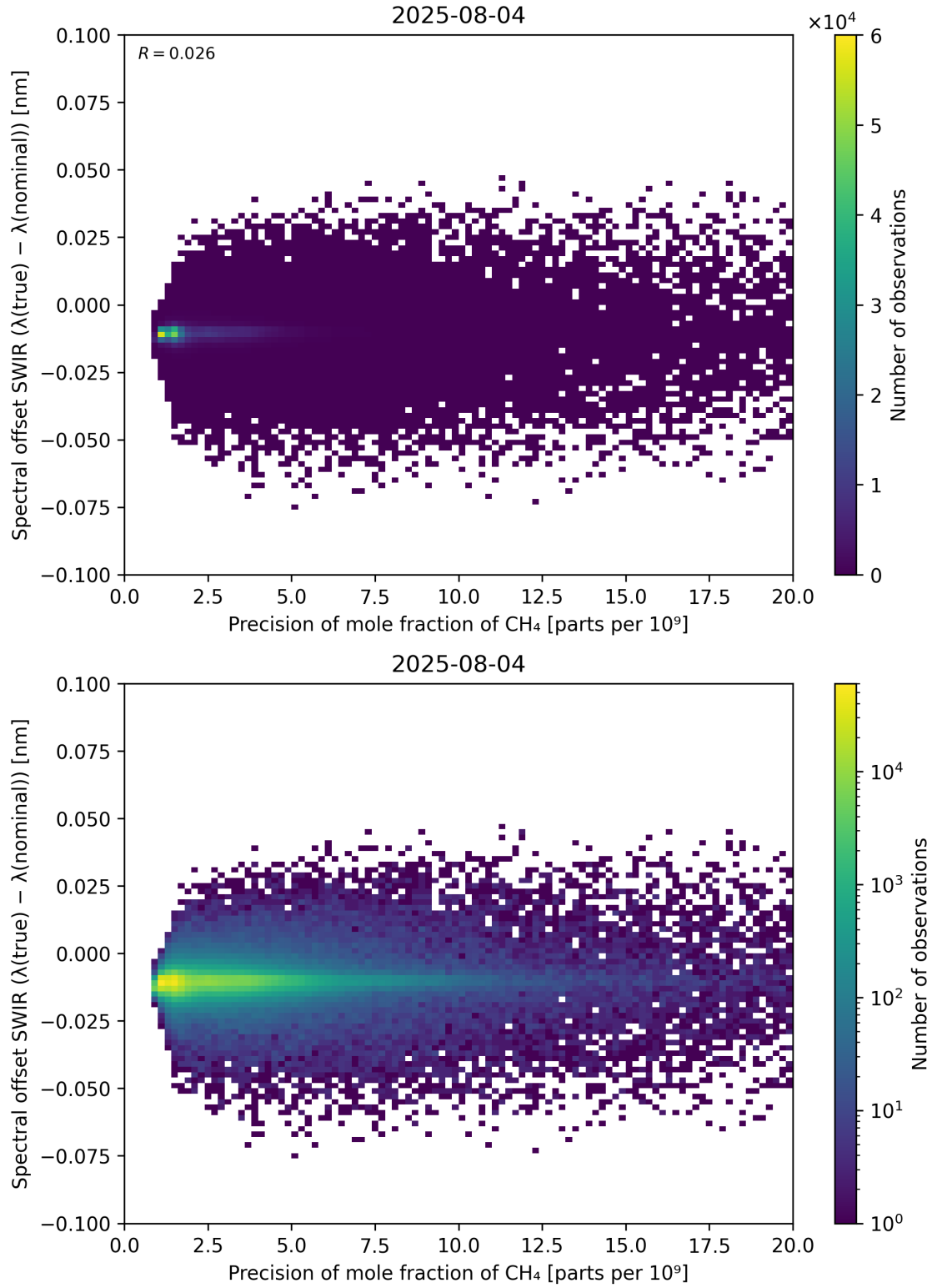
Figure 85: Scatter density plot of “Precision of mole fraction of CH 4 ” against “Spectral offset SWIR ( \lambda_{\text{true}} - \lambda_{\text{nominal}} )” for 2025-08-04 to 2025-08-05.
