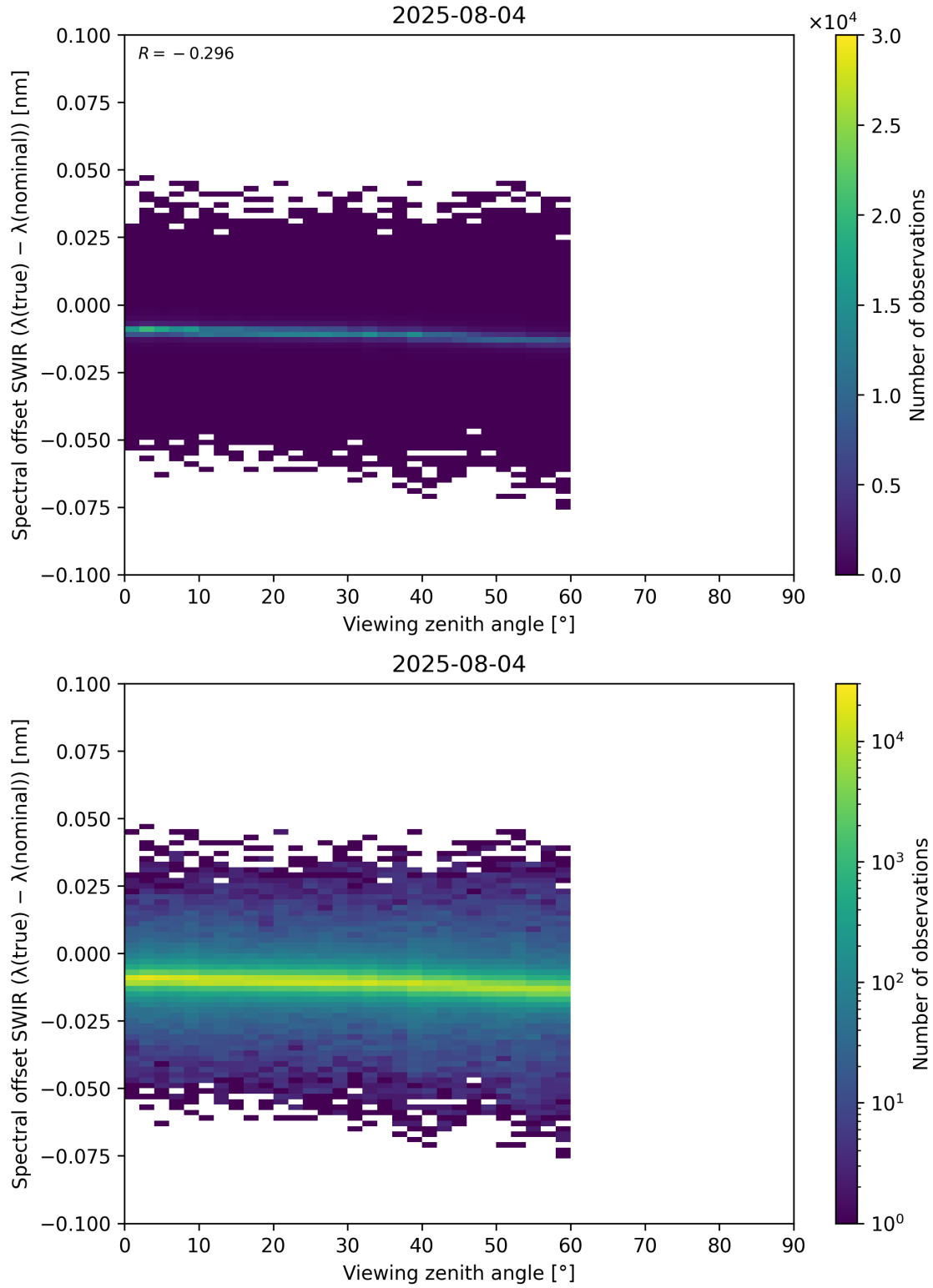
Figure 116: Scatter density plot of “Viewing zenith angle” against “Spectral offset SWIR ( \lambda_{\text{true}} - \lambda_{\text{nominal}} )” for 2025-08-04 to 2025-08-05.
