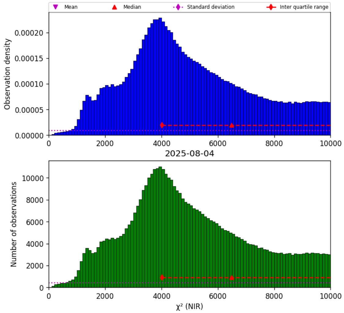
Figure 29: Histogram of “ \chi^2 (NIR)” for 2025-08-04 to 2025-08-05
