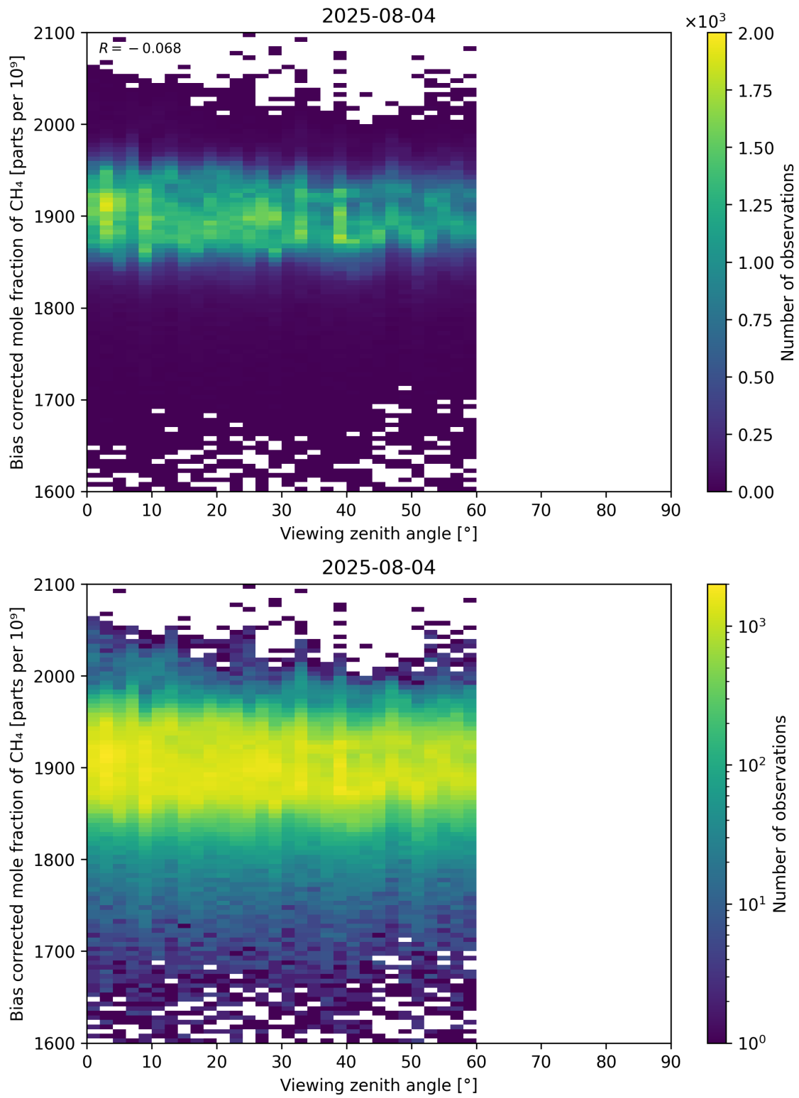
Figure 111: Scatter density plot of “Viewing zenith angle” against “Bias corrected mole fraction of CH 4 ” for 2025-08-04 to 2025-08-05.
