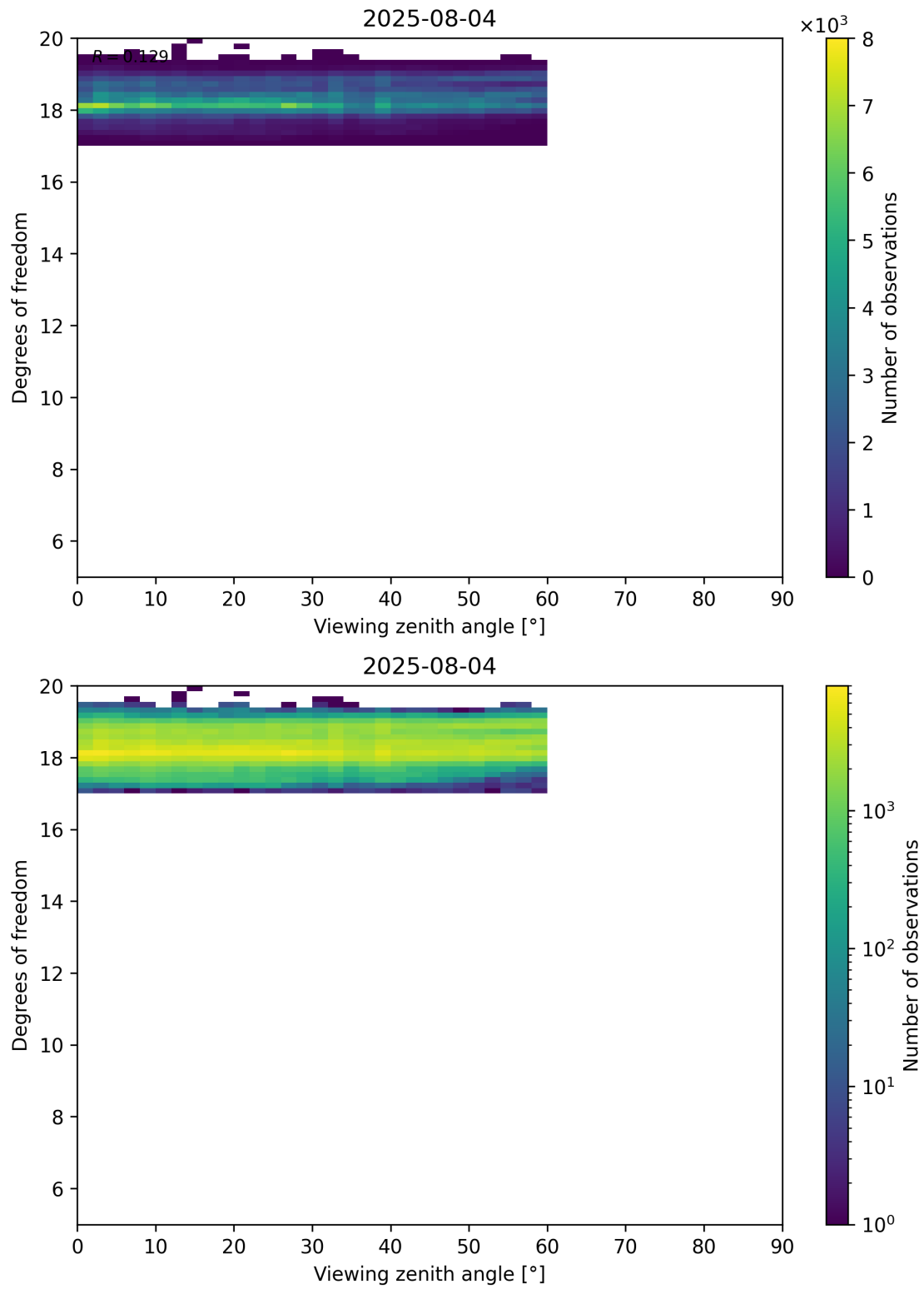
Figure 107: Scatter density plot of “Viewing zenith angle” against “Degrees of freedom” for 2025-08-04 to 2025-08-05.
