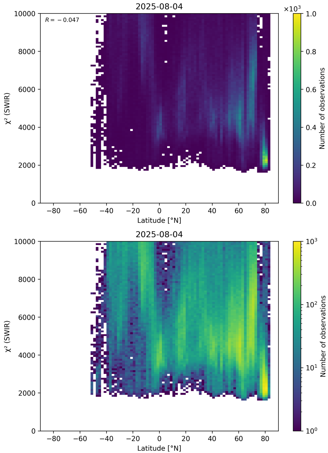
Figure 54: Scatter density plot of “Latitude” against “ \chi^2 (SWIR)” for 2025-08-04 to 2025-08-05.
