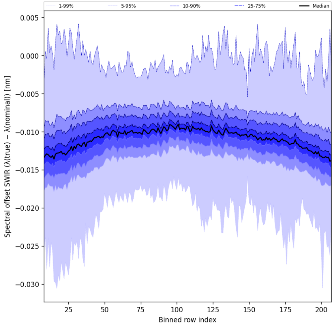
Figure 38: Along track statistics of “Spectral offset SWIR ( \lambda_{\text{true}} - \lambda_{\text{nominal}} )” for 2025-08-04 to 2025-08-05
