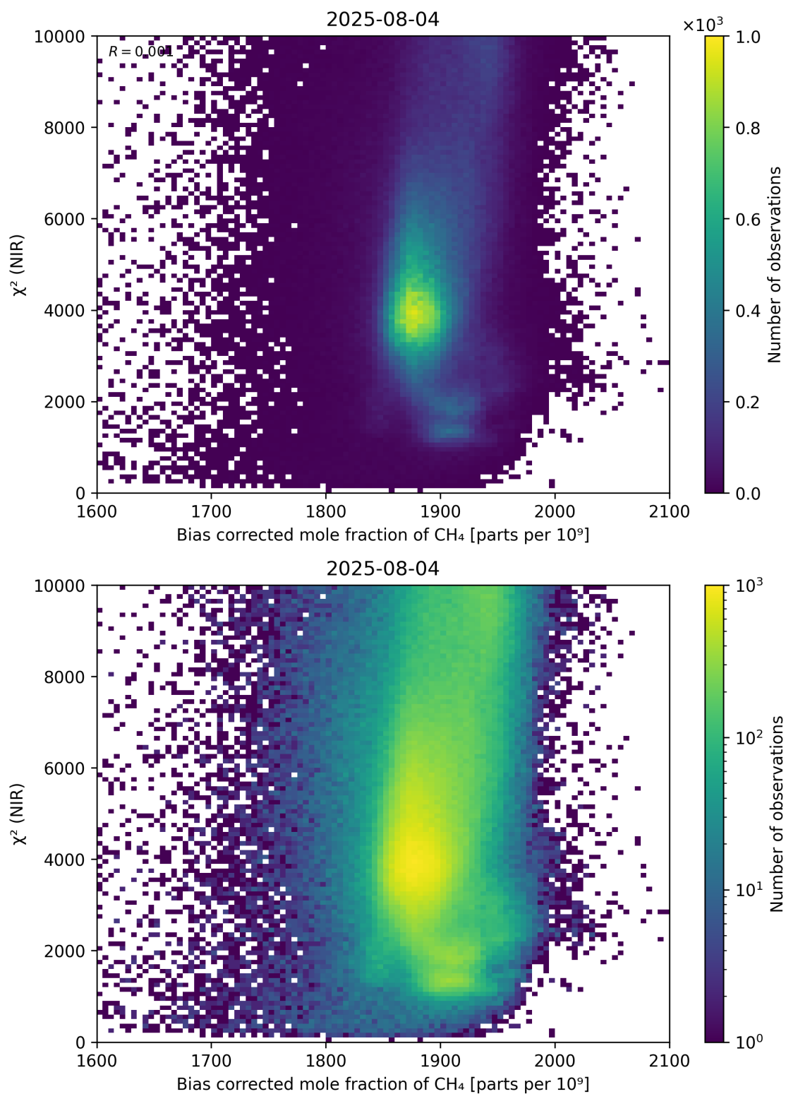
Figure 63: Scatter density plot of “Bias corrected mole fraction of \text{CH}_4 ” against “ \chi^2 (NIR)” for 2025-08-04 to 2025-08-05.
