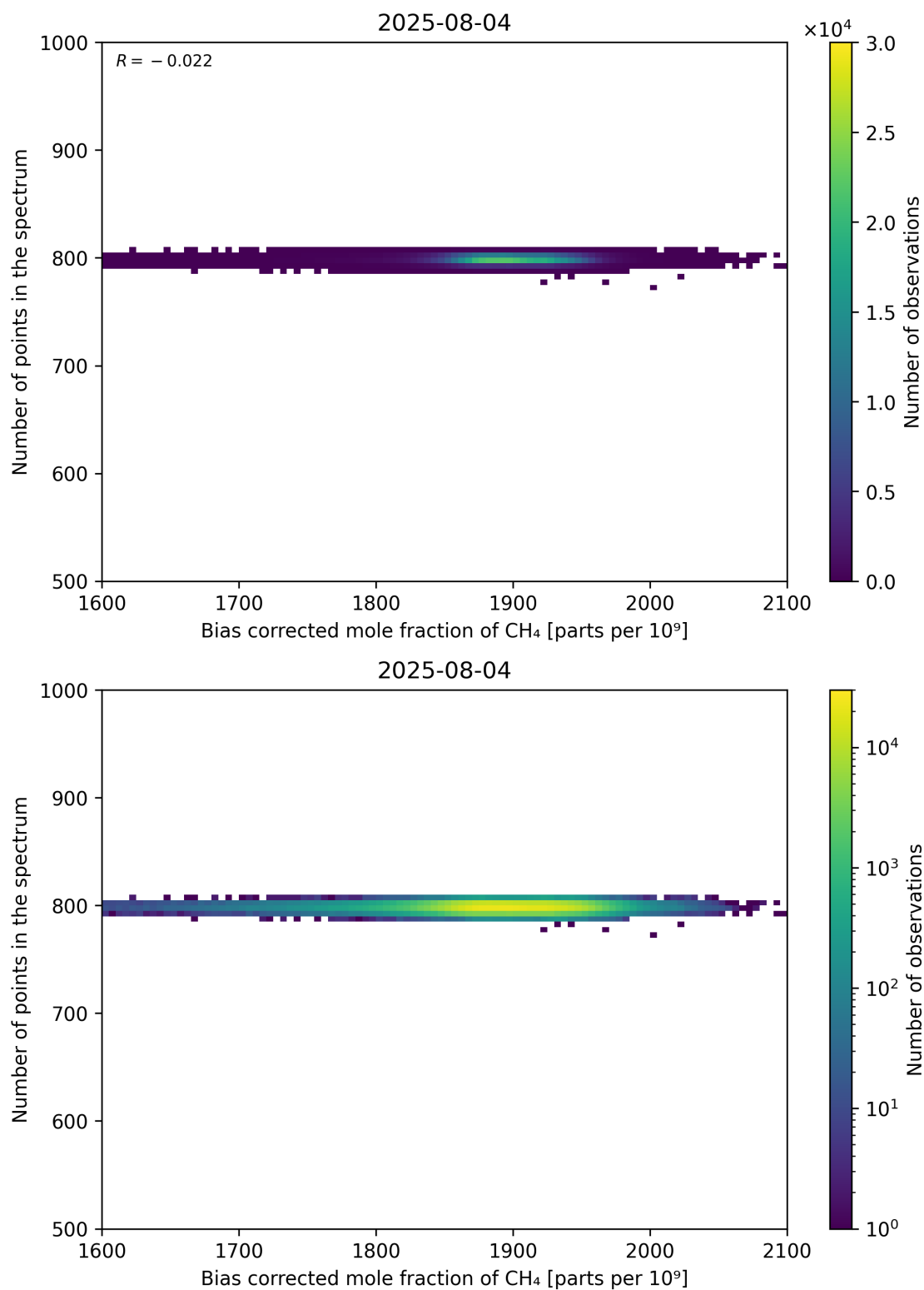
Figure 68: Scatter density plot of “Bias corrected mole fraction of CH 4 ” against “Number of points in the spectrum” for 2025-08-04 to 2025-08-05.
