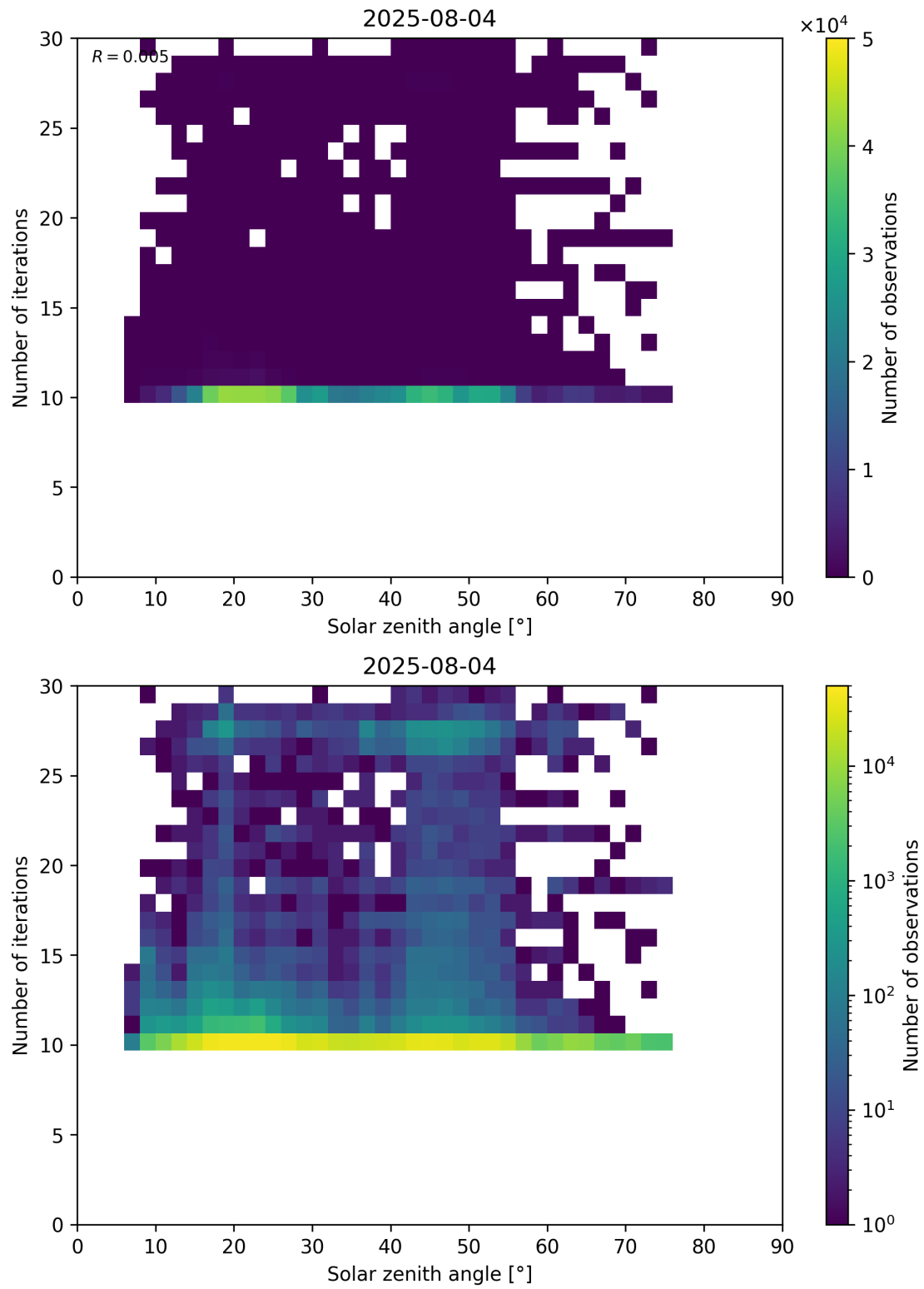
Figure 102: Scatter density plot of “Solar zenith angle” against “Number of iterations” for 2025-08-04 to 2025-08-05.
