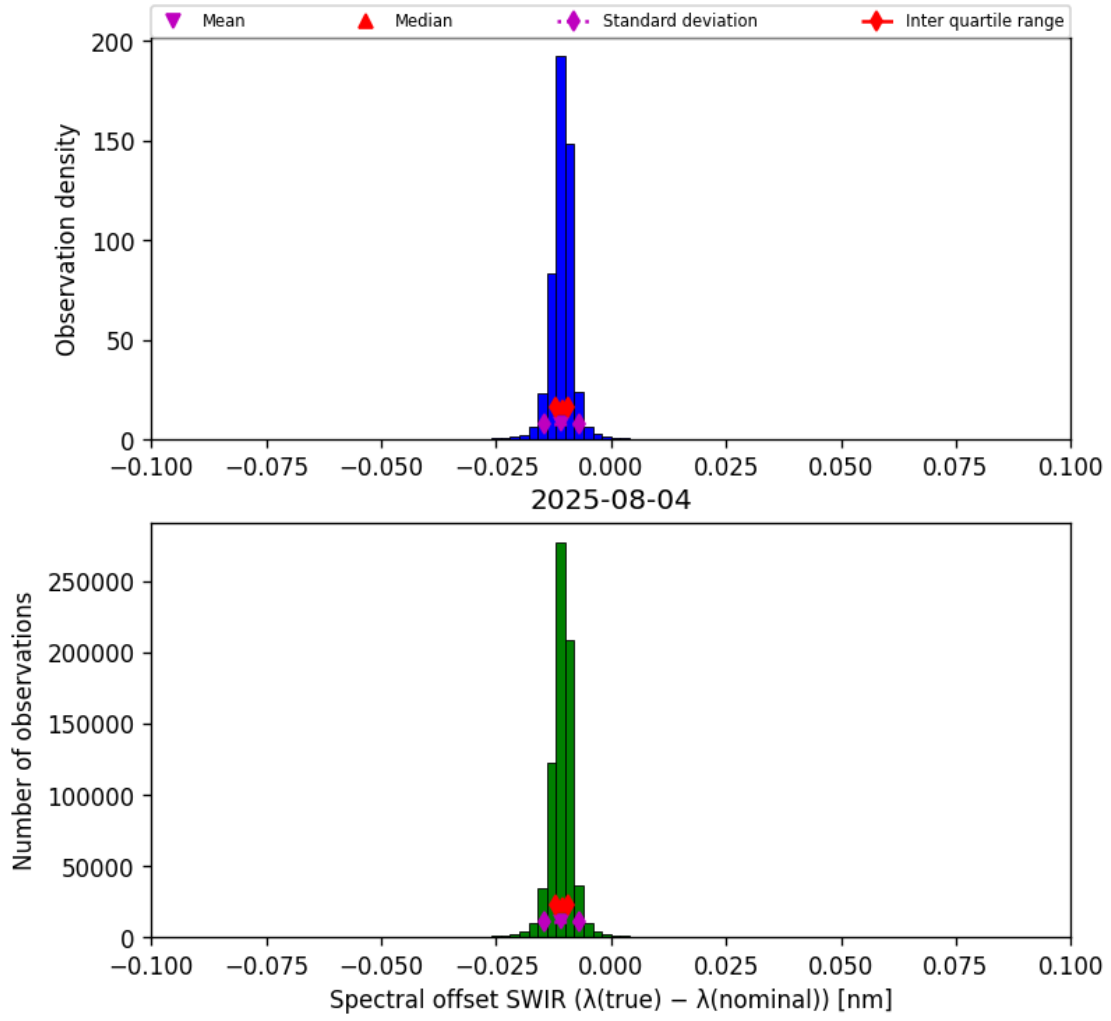
Figure 27: Histogram of “Spectral offset SWIR ( \lambda_{\text{true}} - \lambda_{\text{nominal}} )” for 2025-08-04 to 2025-08-05
