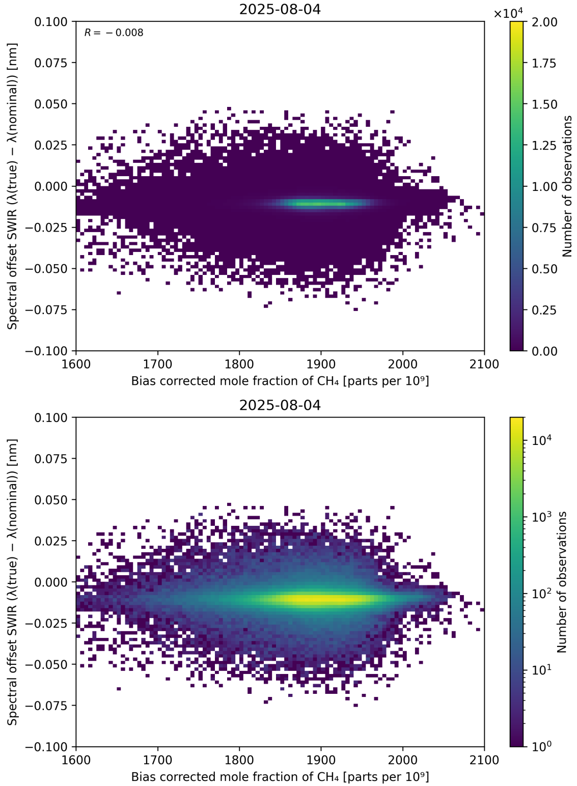
Figure 69: Scatter density plot of “Bias corrected mole fraction of \text{CH}_4 ” against “Spectral offset SWIR ( \lambda_{\text{true}} - \lambda_{\text{nominal}} )” for 2025-08-04 to 2025-08-05.
