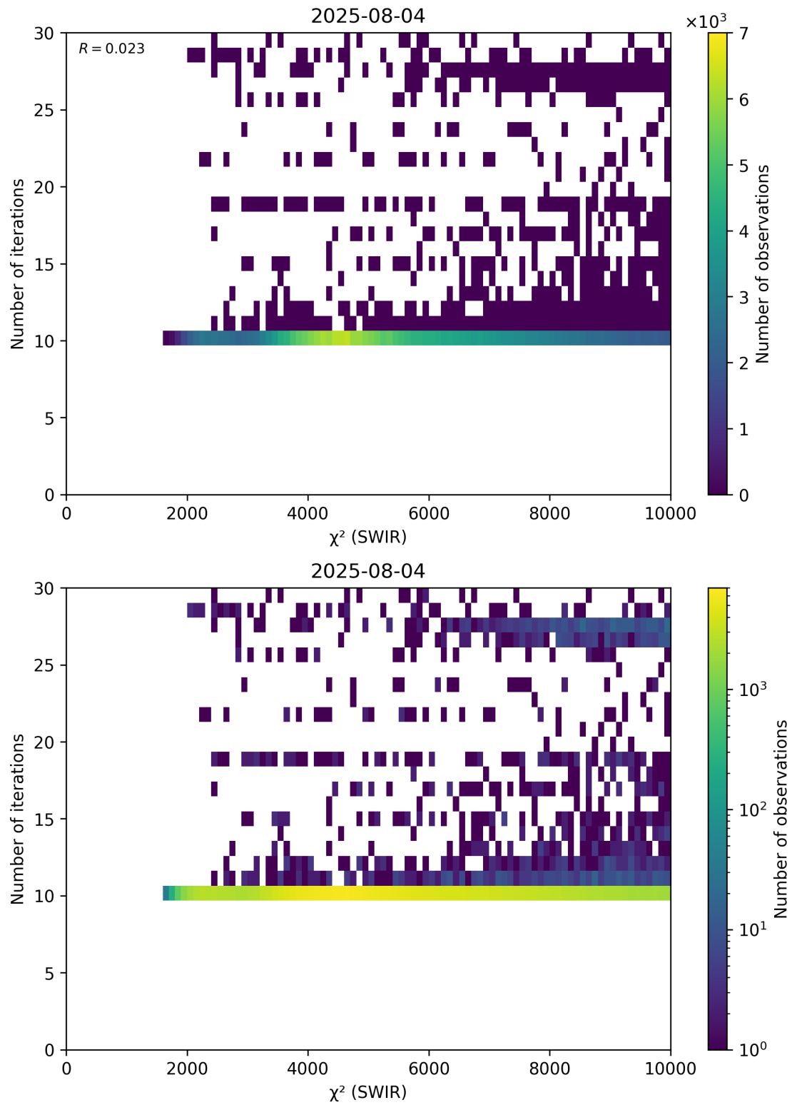
Figure 50: Scatter density plot of “ \chi^2 (SWIR)” against “Number of iterations” for 2025-08-04 to 2025-08-05.
