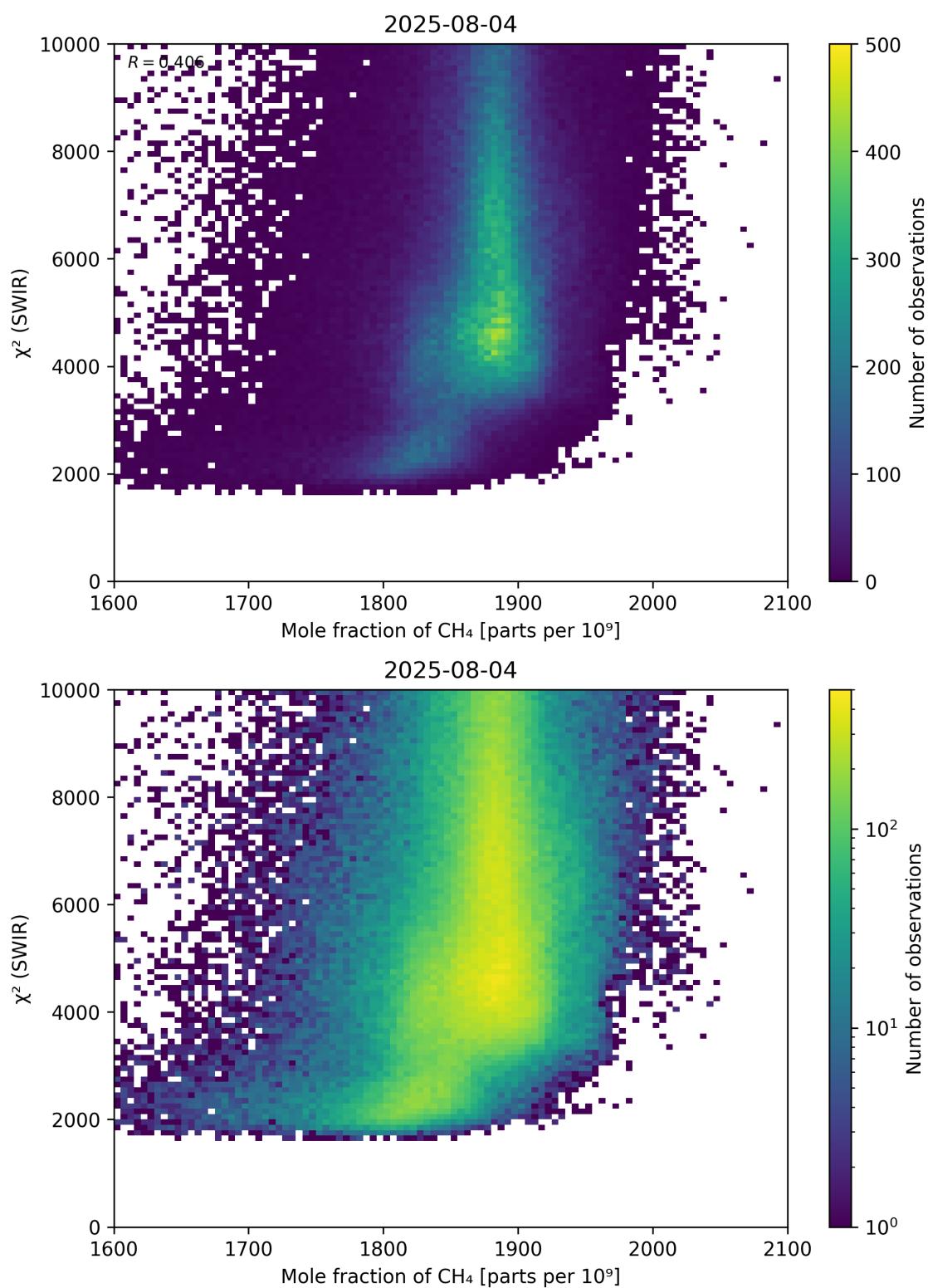
Figure 71: Scatter density plot of “Mole fraction of CH 4 ” against “ \chi^2 (SWIR)” for 2025-08-04 to 2025-08-05.
