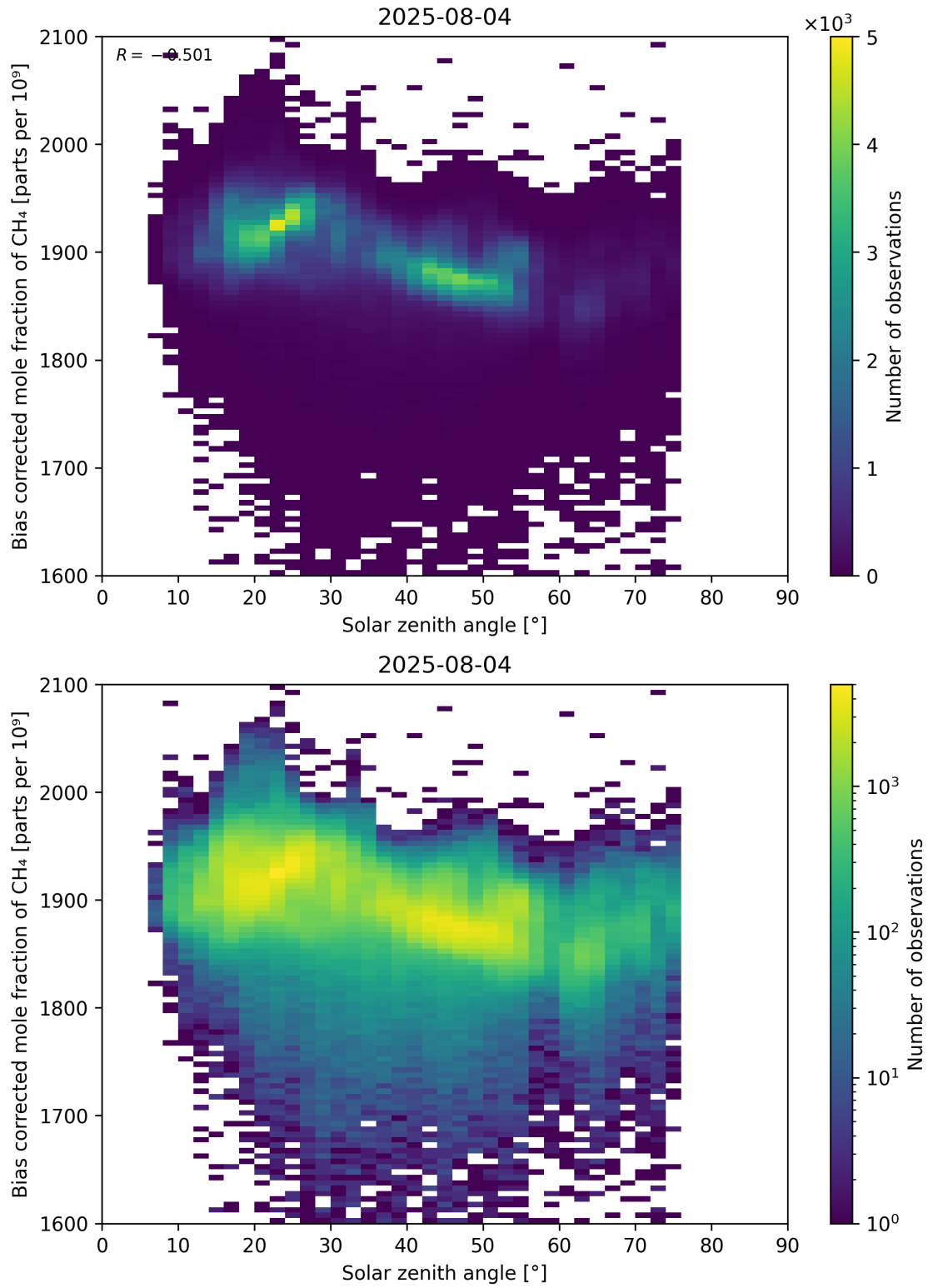
Figure 100: Scatter density plot of “Solar zenith angle” against “Bias corrected mole fraction of CH 4 ” for 2025-08-04 to 2025-08-05.
