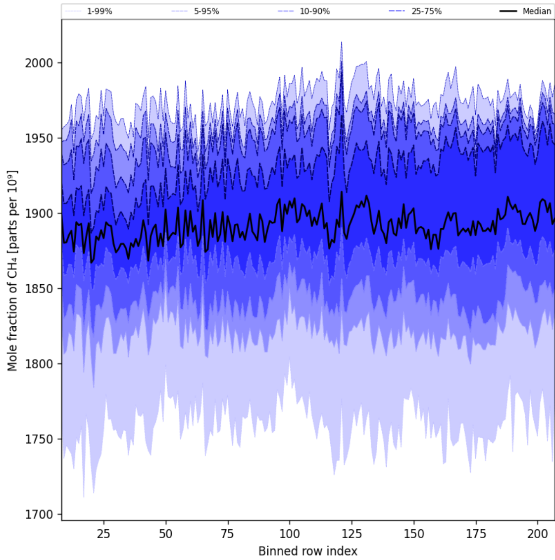
Figure 34: Along track statistics of “Mole fraction of CH 4 ” for 2025-08-04 to 2025-08-05
