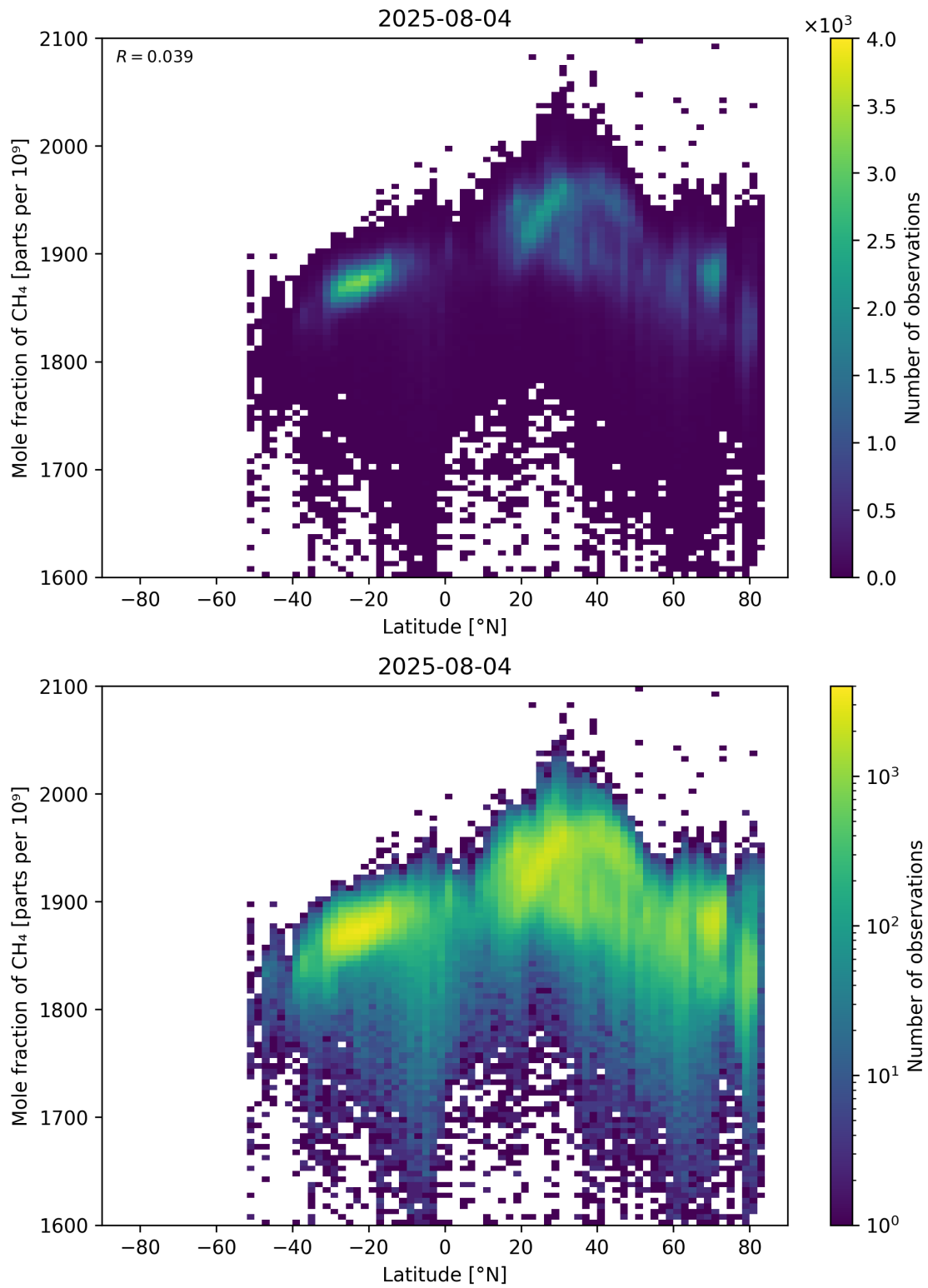
Figure 57: Scatter density plot of “Latitude” against “Mole fraction of \text{CH}_4 ” for 2025-08-04 to 2025-08-05.
