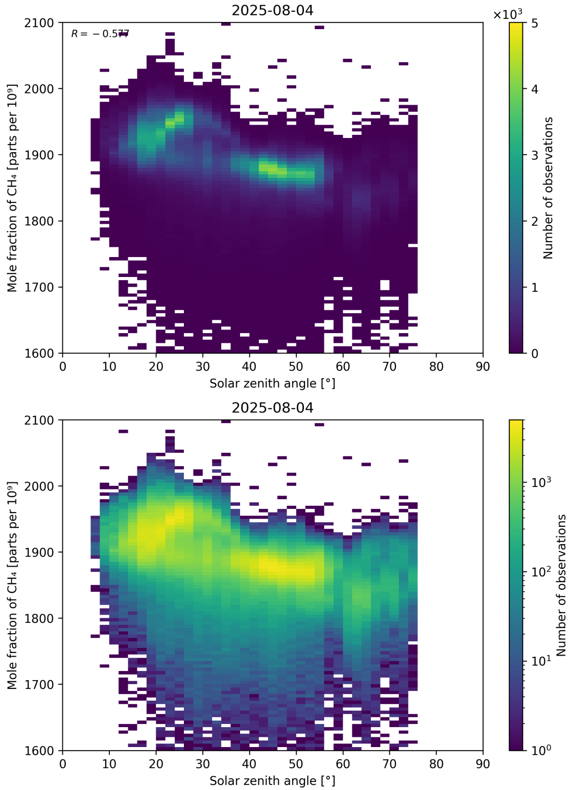
Figure 99: Scatter density plot of “Solar zenith angle” against “Mole fraction of CH 4 ” for 2025-08-04 to 2025-08-05.
