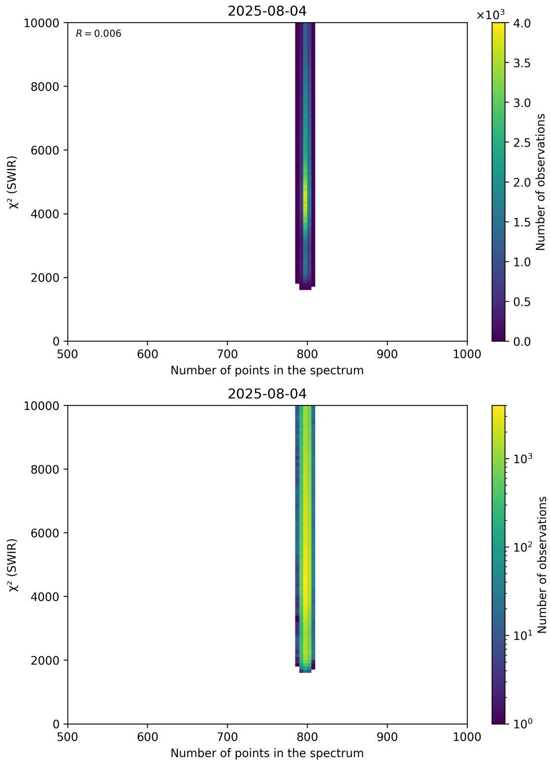
Figure 89: Scatter density plot of “Number of points in the spectrum” against “ \chi^2 (SWIR)” for 2025-08-04 to 2025-08-05.
