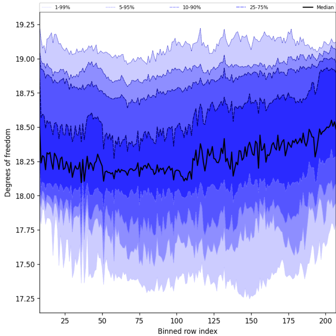
Figure 41: Along track statistics of “Degrees of freedom” for 2025-08-04 to 2025-08-05
