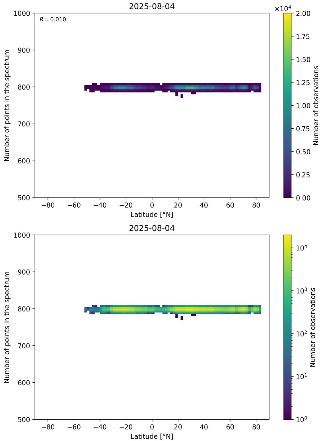
Figure 61: Scatter density plot of “Latitude” against “Number of points in the spectrum” for 2025-08-04 to 2025-08-05.
