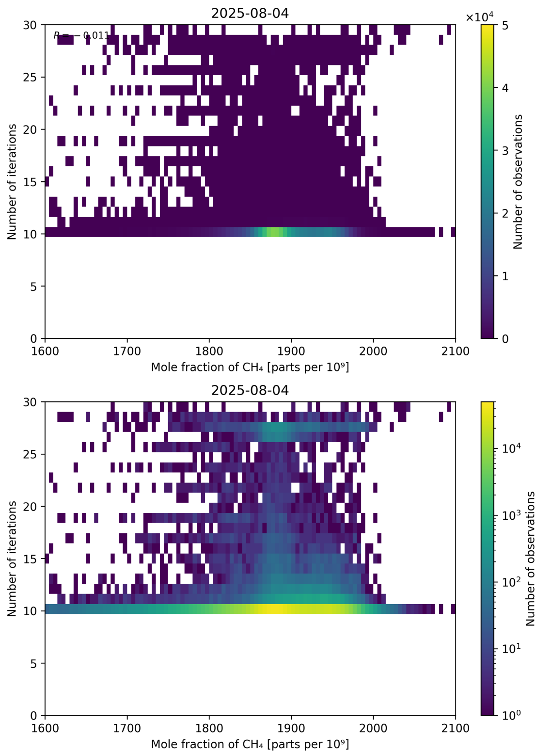
Figure 76: Scatter density plot of “Mole fraction of CH 4 ” against “Number of iterations” for 2025-08-04 to 2025-08-05.
