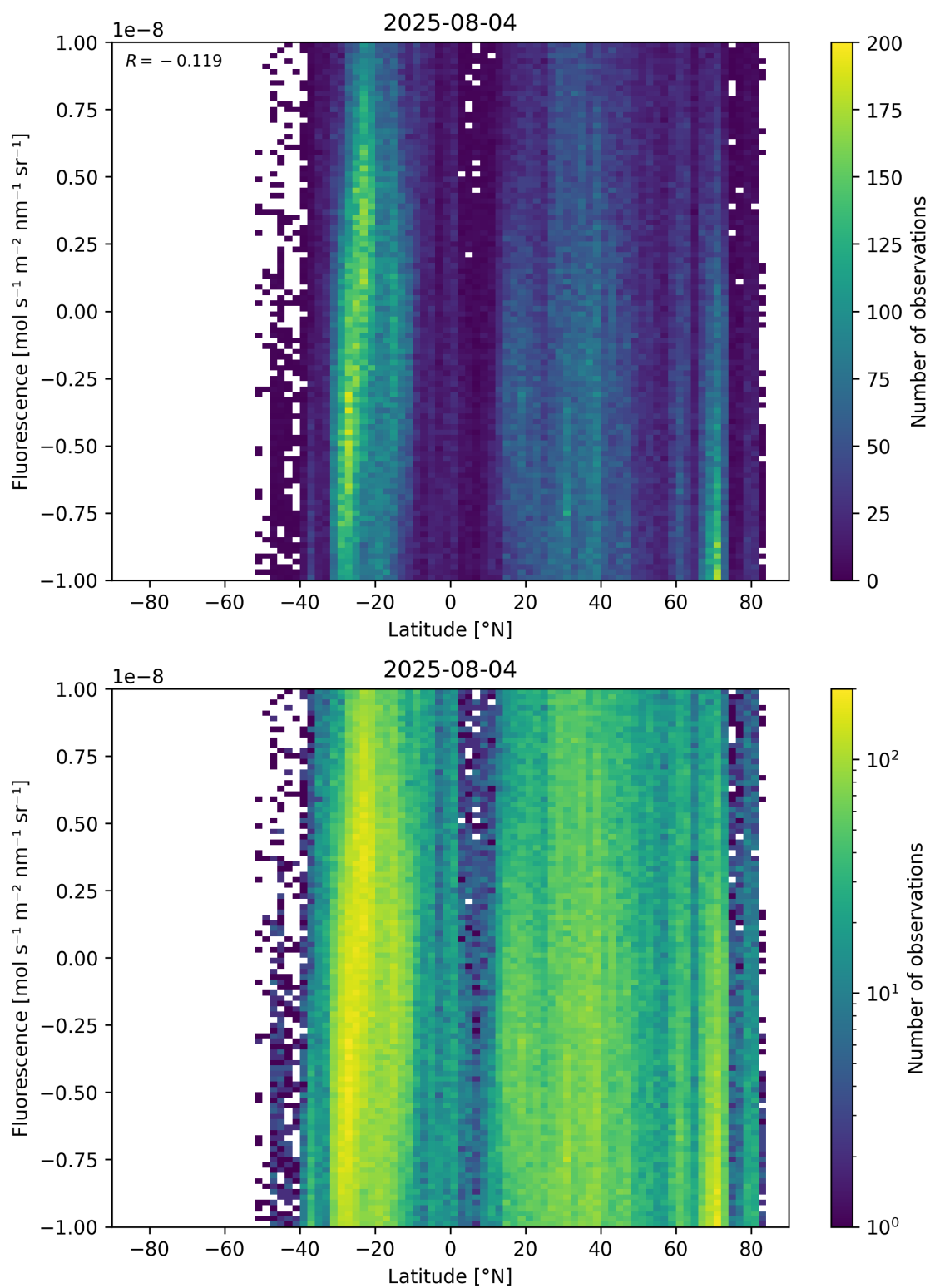
Figure 56: Scatter density plot of “Latitude” against “Fluorescence” for 2025-08-04 to 2025-08-05.
