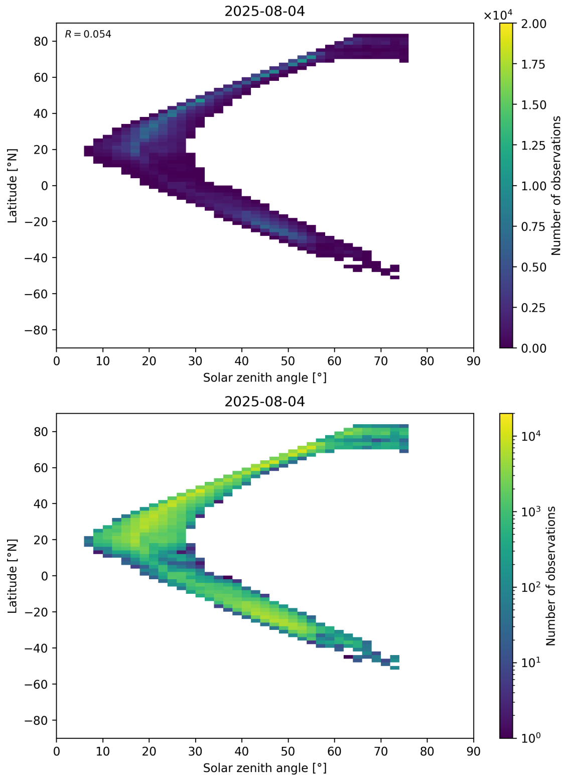
Figure 98: Scatter density plot of “Solar zenith angle” against “Latitude” for 2025-08-04 to 2025-08-05.
