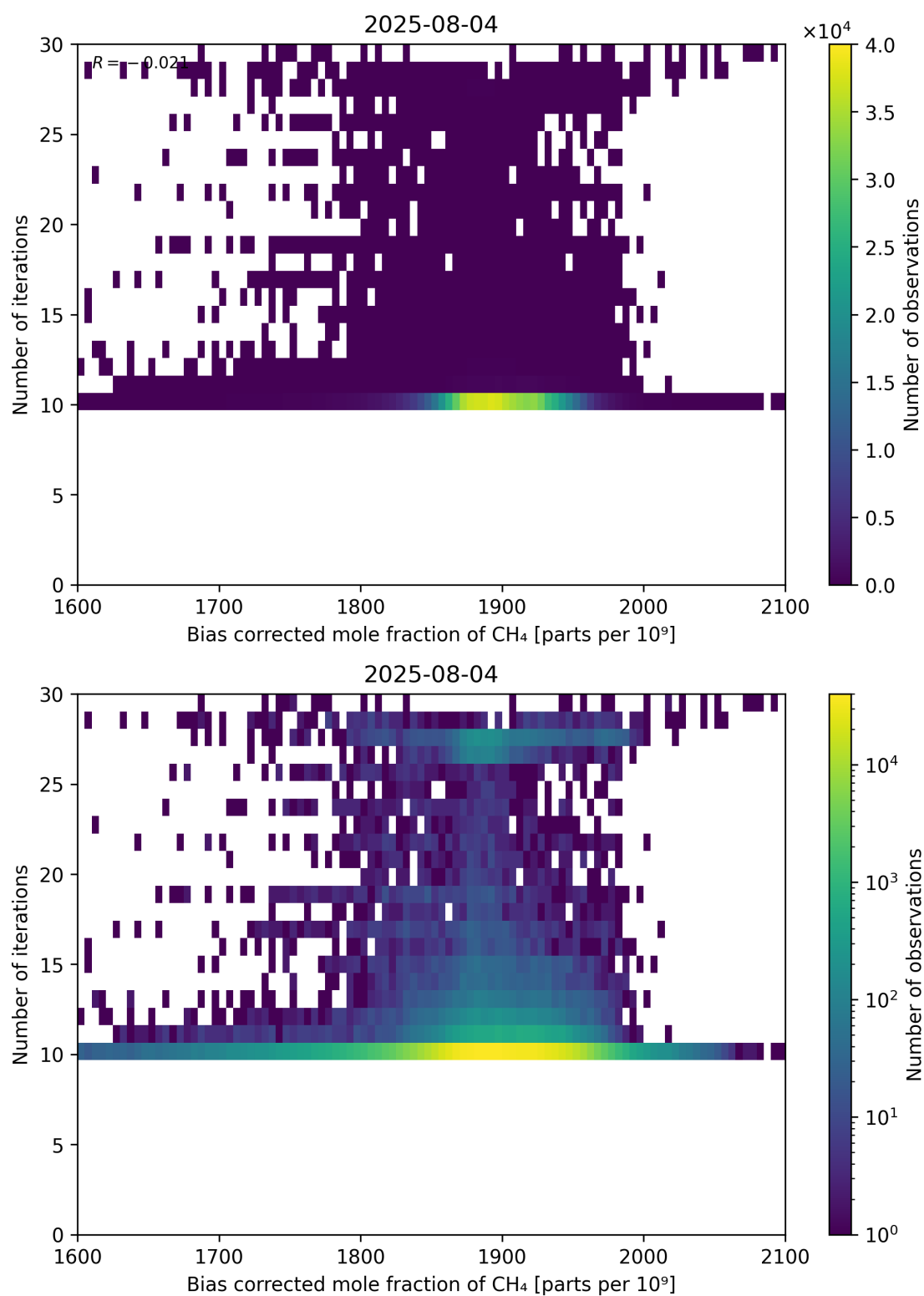
Figure 67: Scatter density plot of “Bias corrected mole fraction of CH 4 ” against “Number of iterations” for 2025-08-04 to 2025-08-05.
