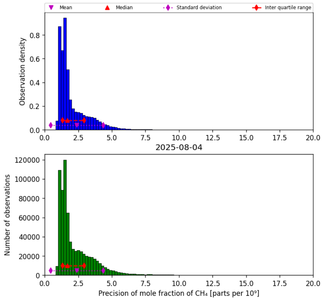
Figure 24: Histogram of “Precision of mole fraction of CH 4 ” for 2025-08-04 to 2025-08-05
