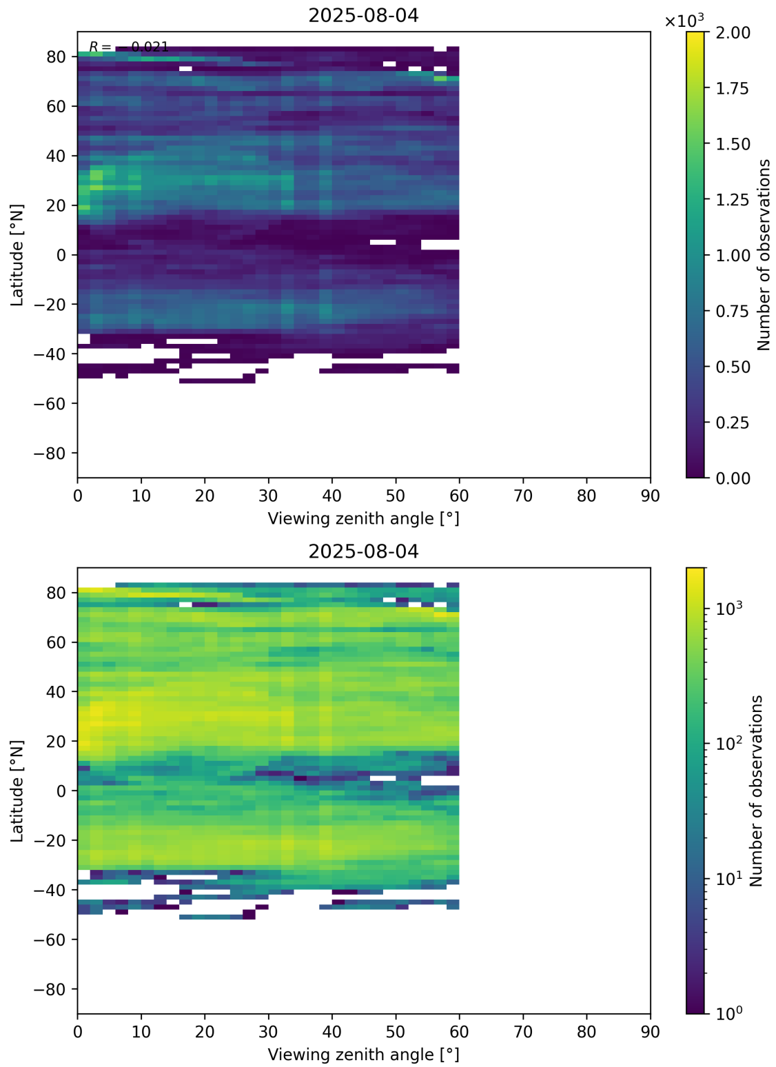
Figure 109: Scatter density plot of “Viewing zenith angle” against “Latitude” for 2025-08-04 to 2025-08-05.
