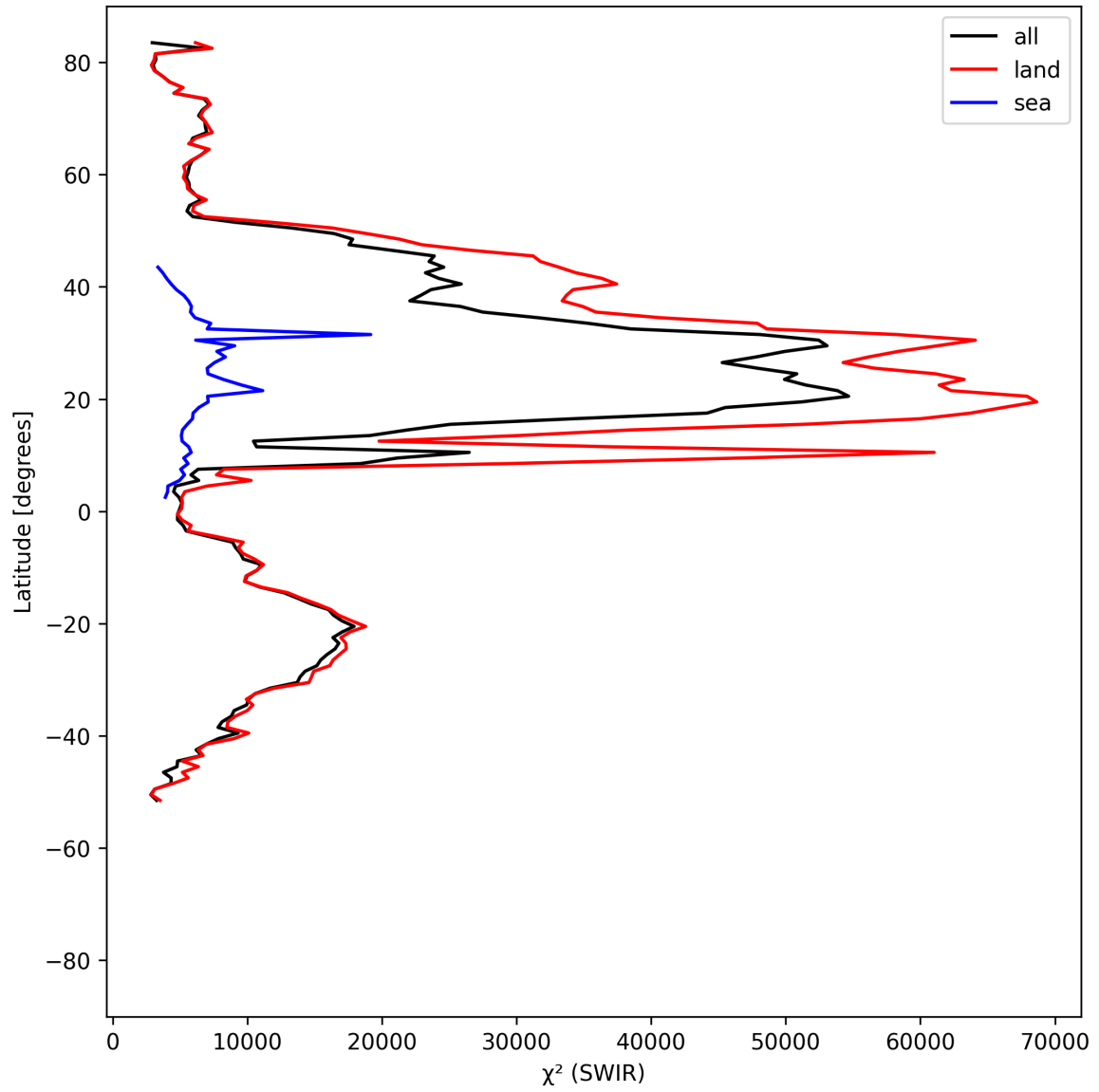
Figure 17: Zonal average of “ \chi^2 (SWIR)” for 2025-08-04 to 2025-08-05.
