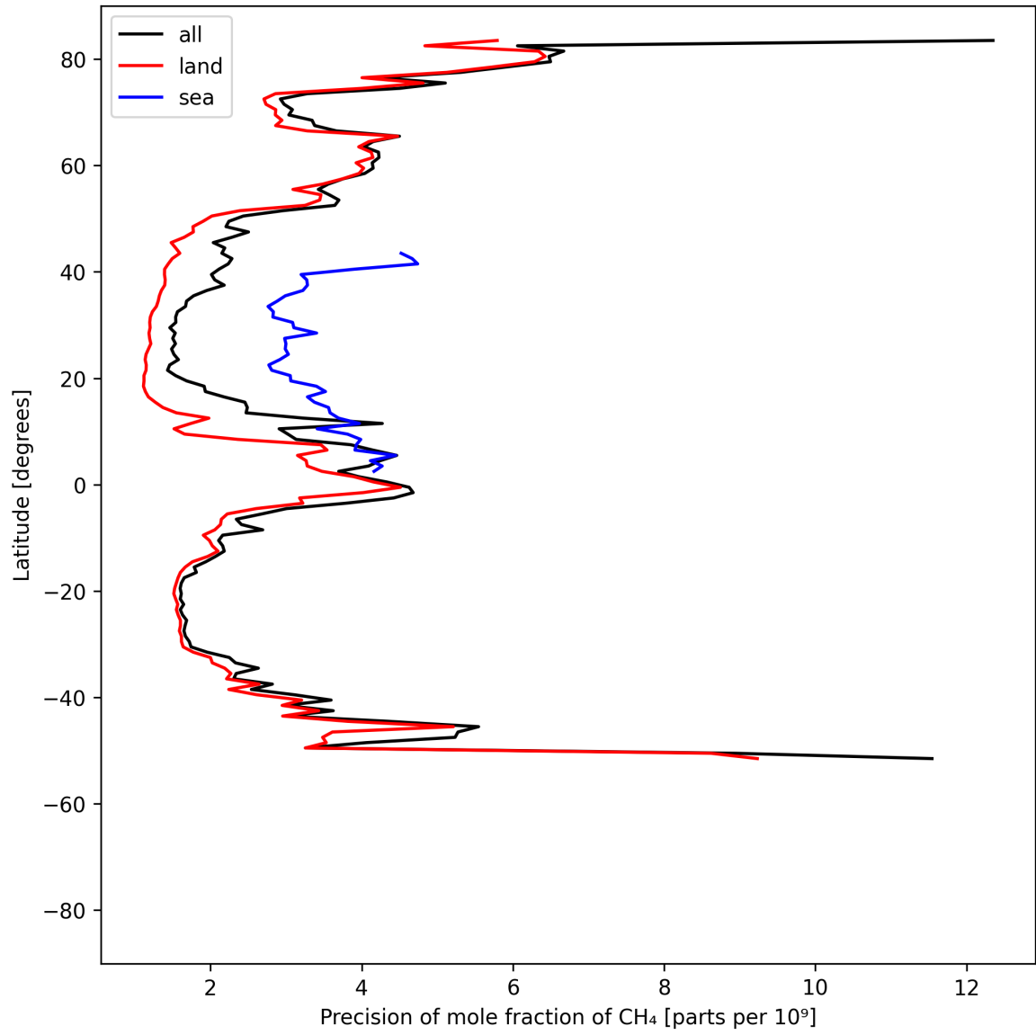
Figure 13: Zonal average of “Precision of mole fraction of CH 4 ” for 2025-08-04 to 2025-08-05.
