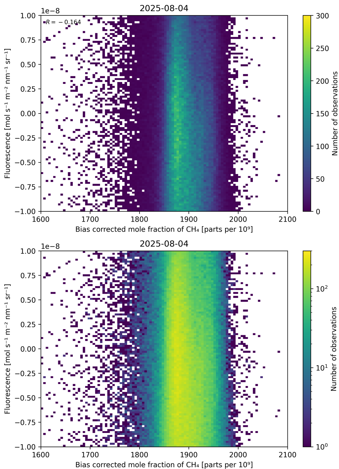
Figure 66: Scatter density plot of “Bias corrected mole fraction of \text{CH}_4 ” against “Fluorescence” for 2025-08-04 to 2025-08-05.
