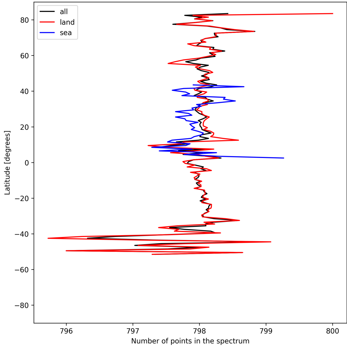
Figure 15: Zonal average of “Number of points in the spectrum” for 2025-08-04 to 2025-08-05.
