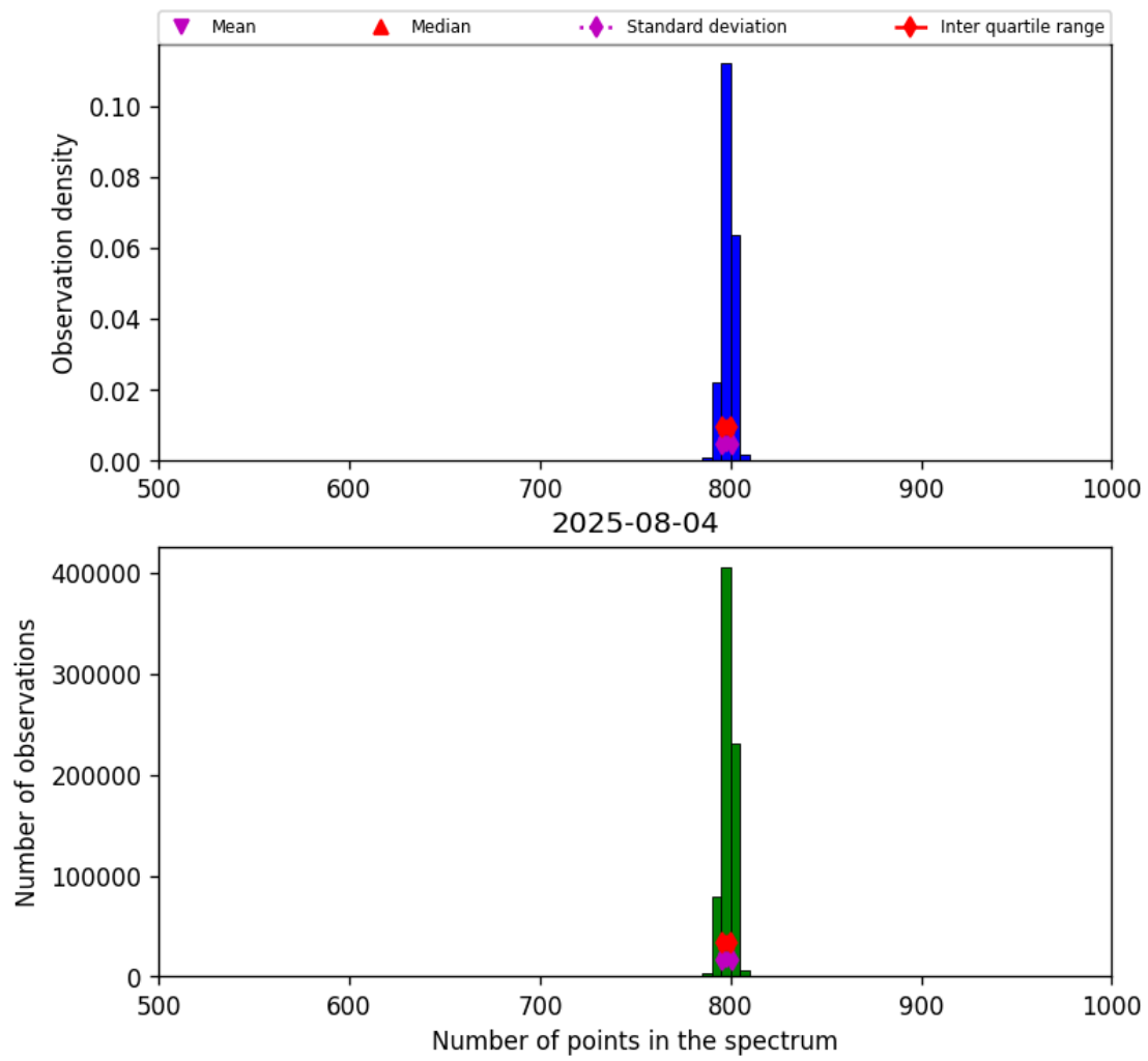
Figure 26: Histogram of “Number of points in the spectrum” for 2025-08-04 to 2025-08-05
