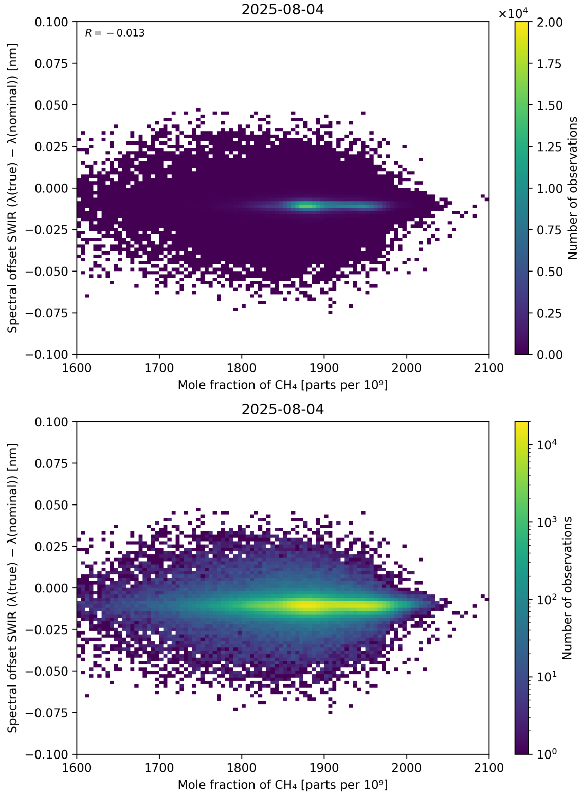
Figure 86: Scatter density plot of “Mole fraction of \text{CH}_4 ” against “Spectral offset SWIR ( \lambda_{\text{true}} - \lambda_{\text{nominal}} )” for 2025-08-04 to 2025-08-05.
