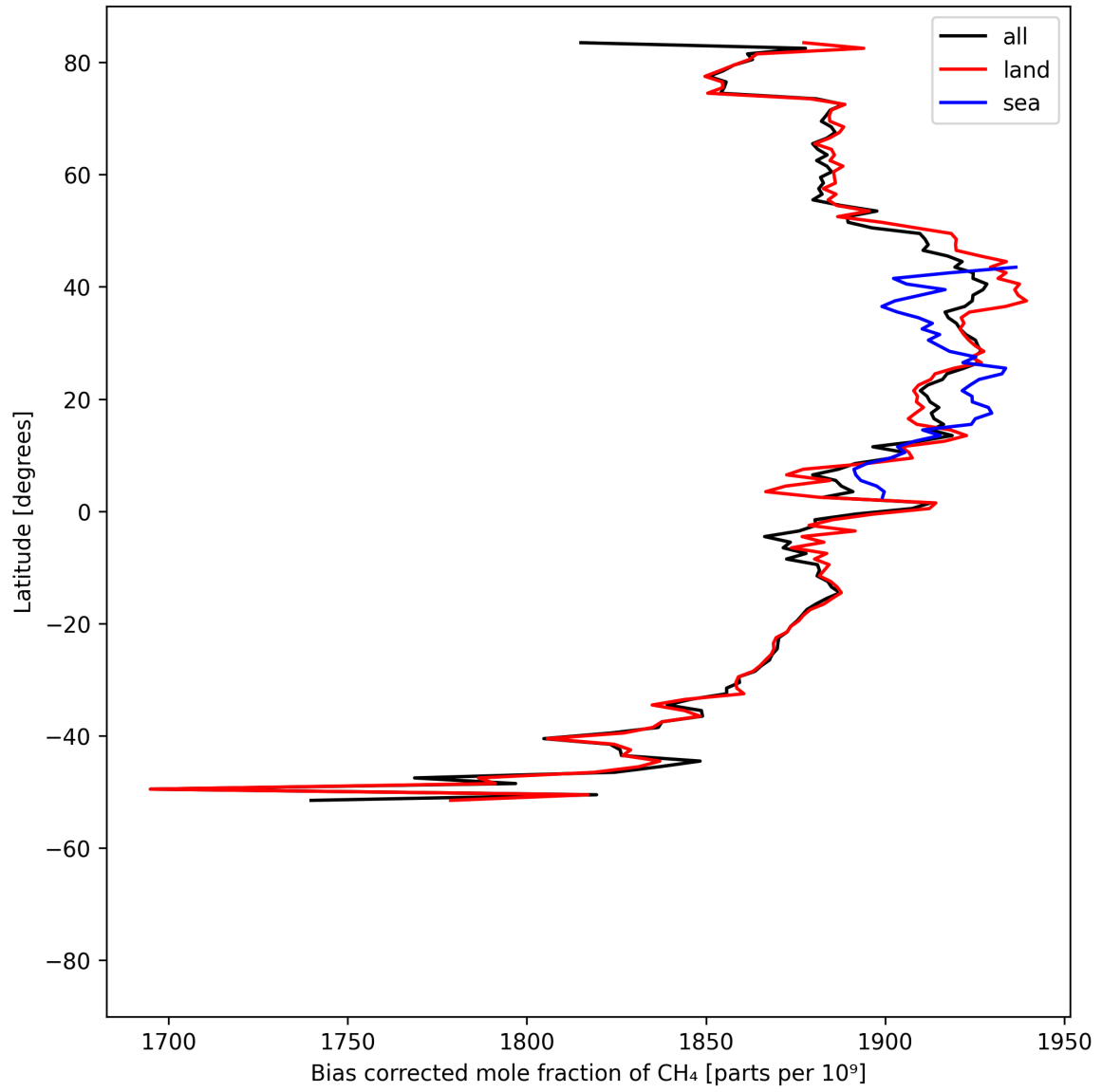
Figure 14: Zonal average of “Bias corrected mole fraction of CH 4 ” for 2025-08-04 to 2025-08-05.
