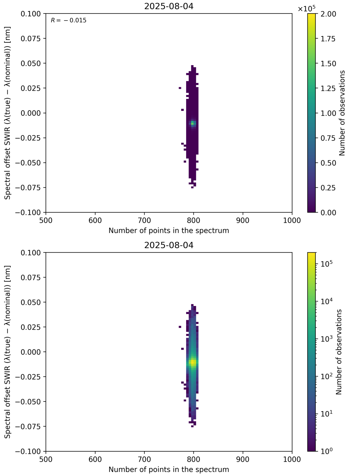
Figure 93: Scatter density plot of “Number of points in the spectrum” against “Spectral offset SWIR ( \lambda_{\text{true}} - \lambda_{\text{nominal}} )” for 2025-08-04 to 2025-08-05.
