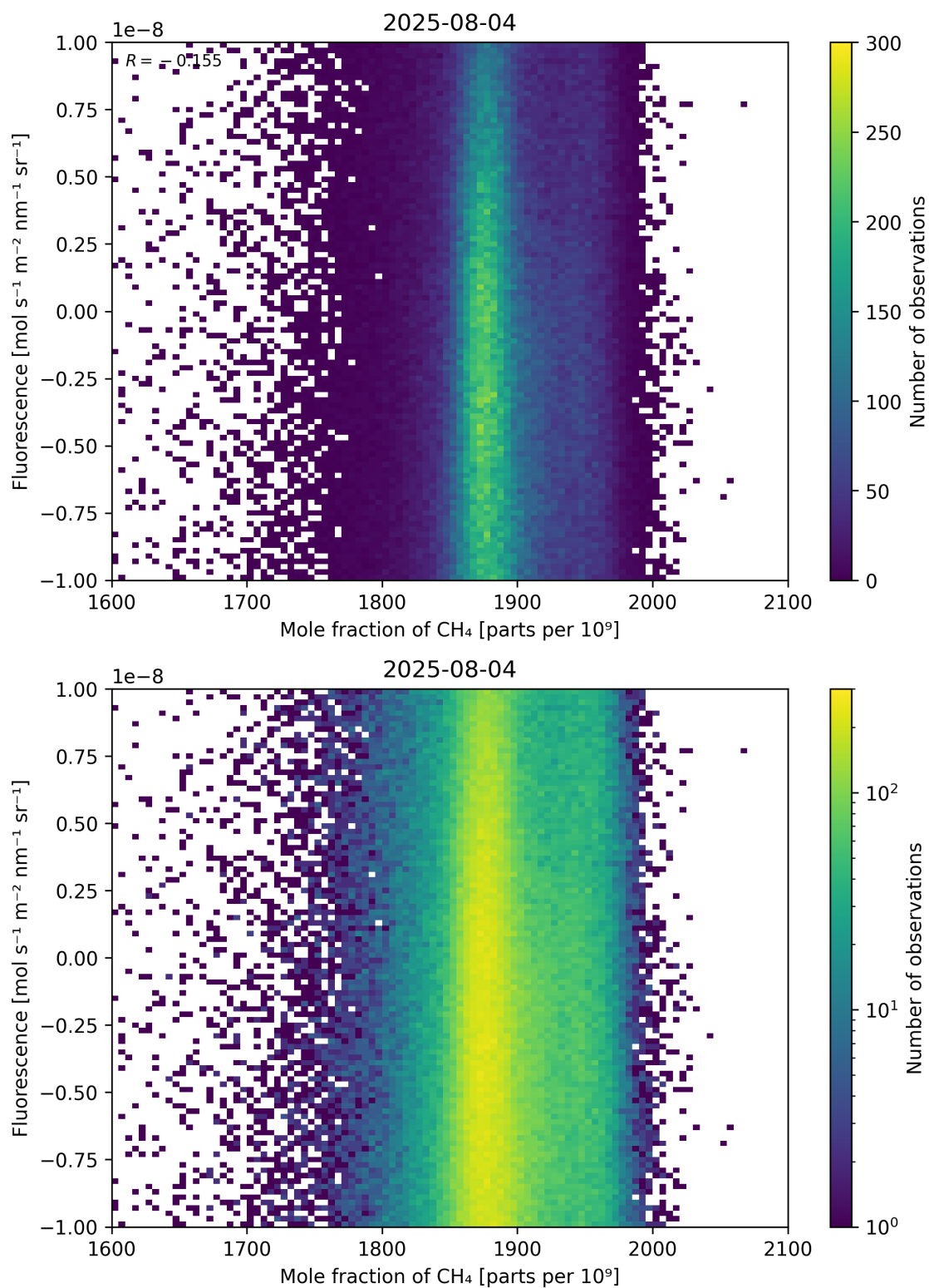
Figure 73: Scatter density plot of “Mole fraction of \text{CH}_4 ” against “Fluorescence” for 2025-08-04 to 2025-08-05.
