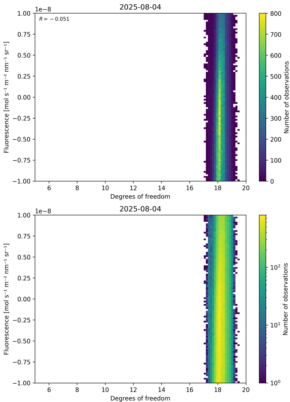
Figure 51: Scatter density plot of “Degrees of freedom” against “Fluorescence” for 2025-08-04 to 2025-08-05.
