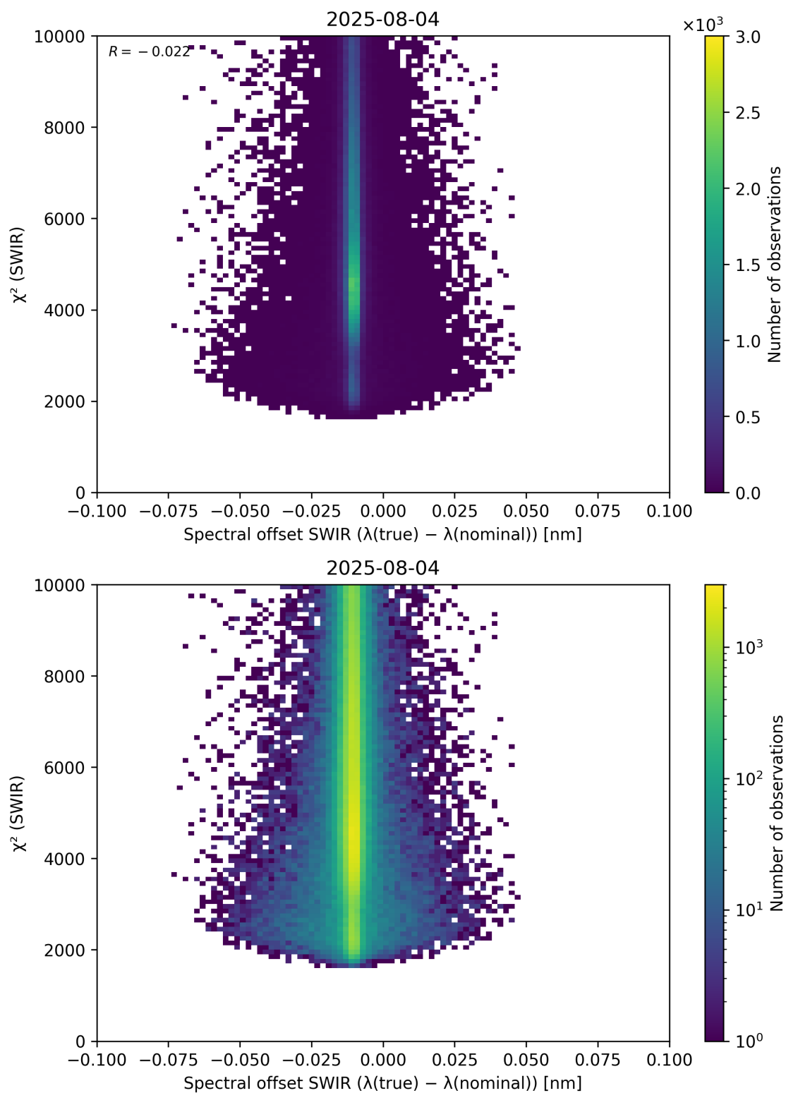
Figure 118: Scatter density plot of “Spectral offset SWIR ( \lambda_{\text{true}} - \lambda_{\text{nominal}} )” against “ \chi^2 (SWIR)” for 2025-08-04 to 2025-08-05.
