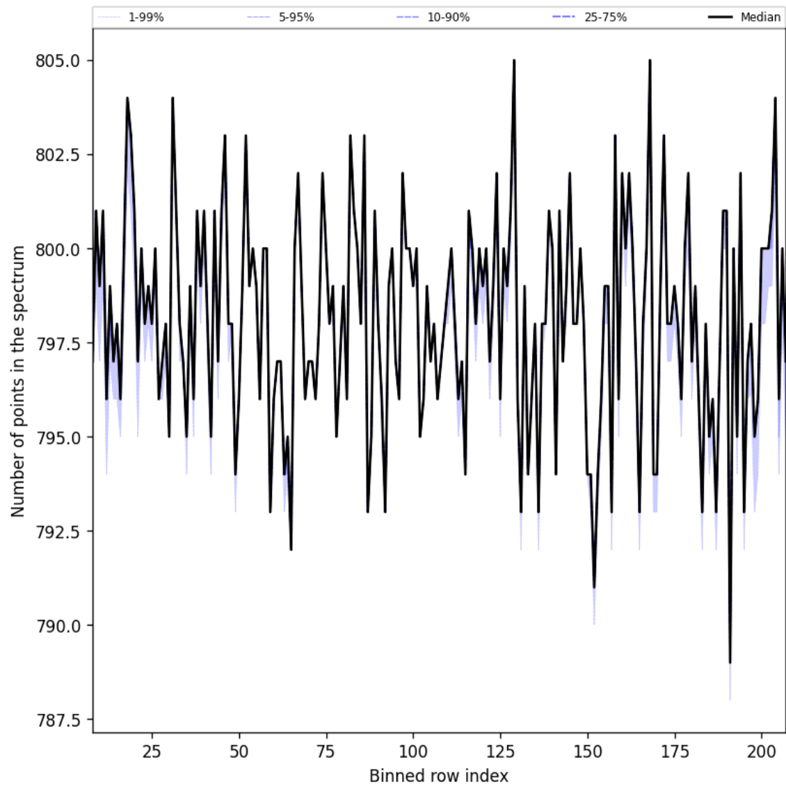
Figure 37: Along track statistics of “Number of points in the spectrum” for 2025-08-04 to 2025-08-05
