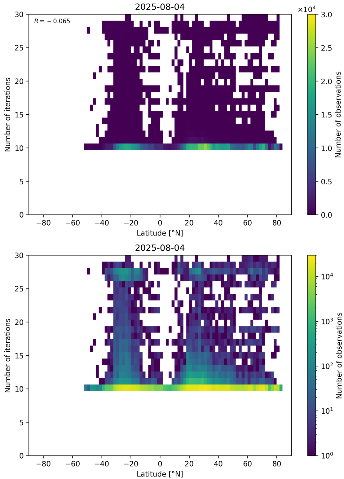
Figure 60: Scatter density plot of “Latitude” against “Number of iterations” for 2025-08-04 to 2025-08-05.
