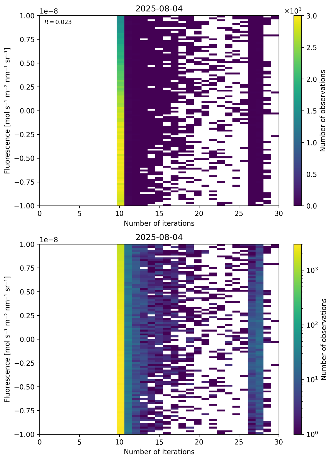
Figure 87: Scatter density plot of “Number of iterations” against “Fluorescence” for 2025-08-04 to 2025-08-05.
