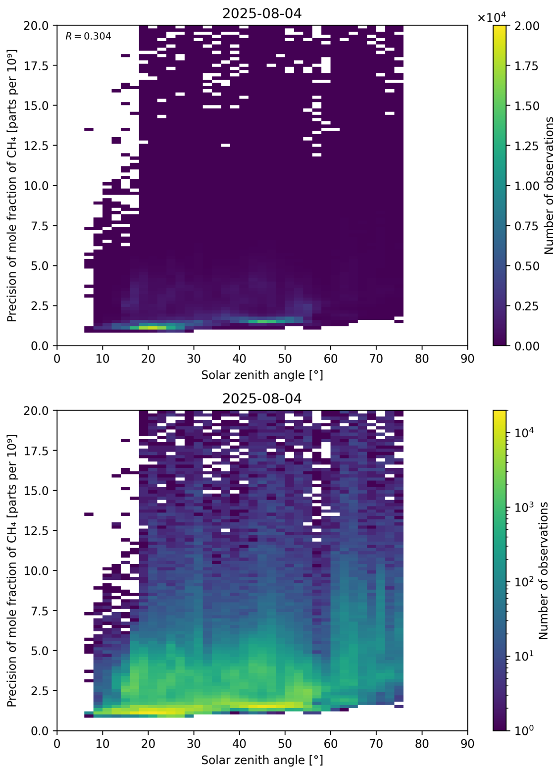
Figure 101: Scatter density plot of “Solar zenith angle” against “Precision of mole fraction of CH 4 ” for 2025-08-04 to 2025-08-05.
