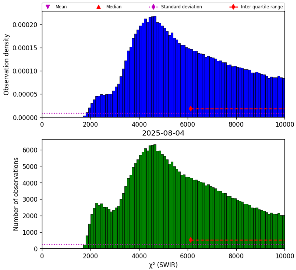
Figure 28: Histogram of “ \chi^2 (SWIR)” for 2025-08-04 to 2025-08-05
