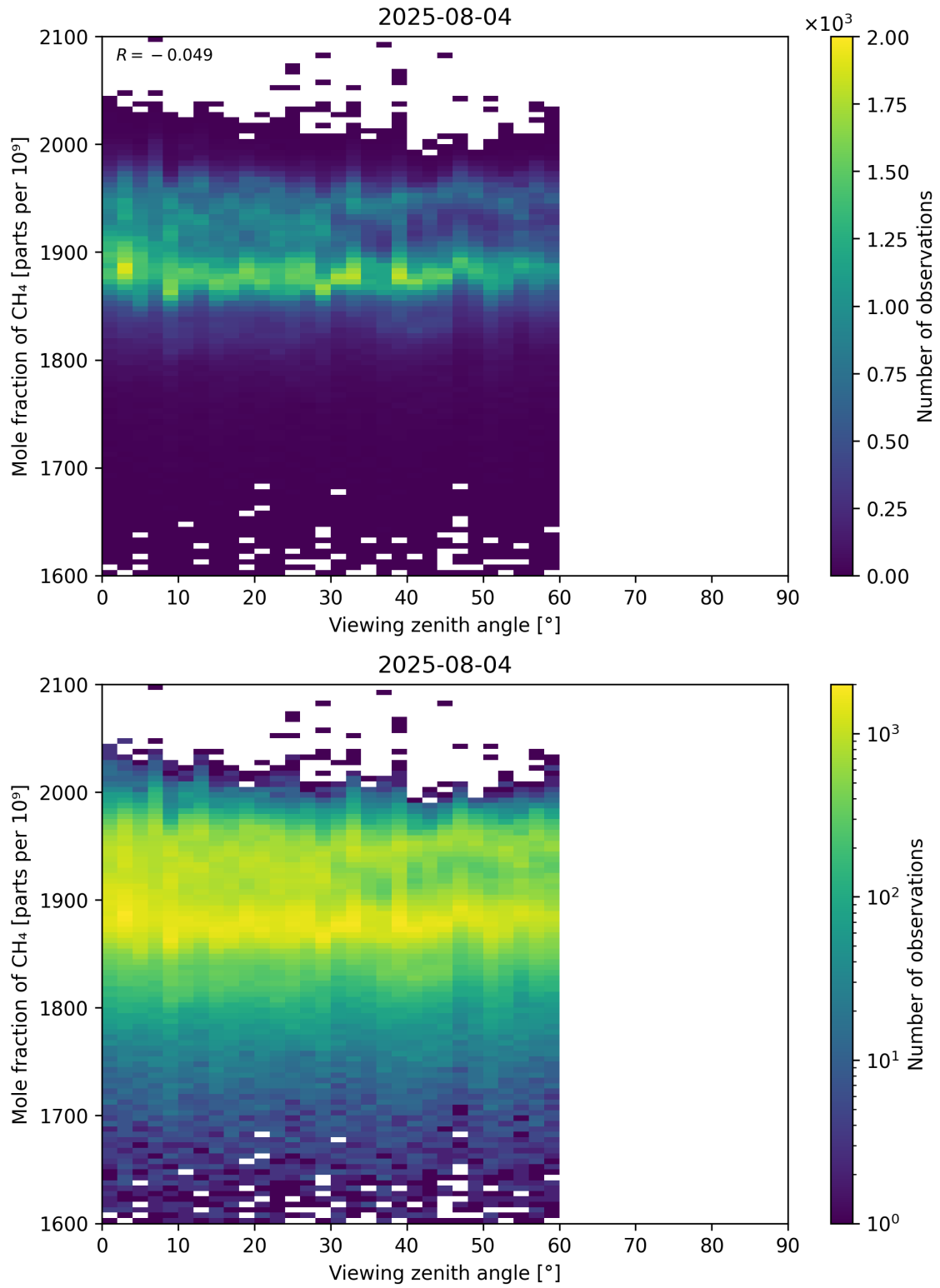
Figure 110: Scatter density plot of “Viewing zenith angle” against “Mole fraction of CH 4 ” for 2025-08-04 to 2025-08-05.
