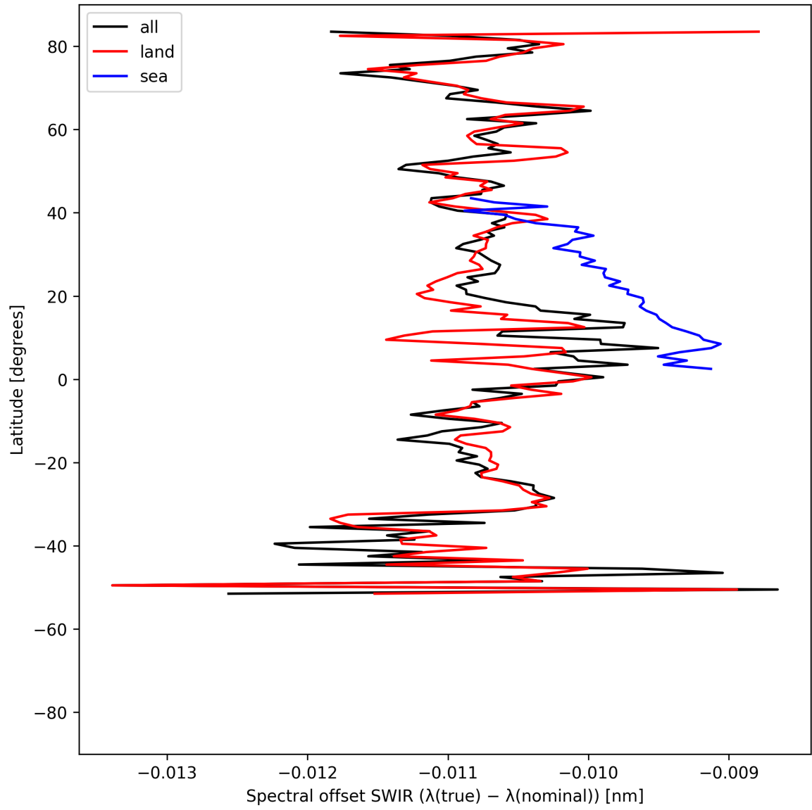
Figure 16: Zonal average of “Spectral offset SWIR ( \lambda_{\text{true}} - \lambda_{\text{nominal}} )” for 2025-08-04 to 2025-08-05.
