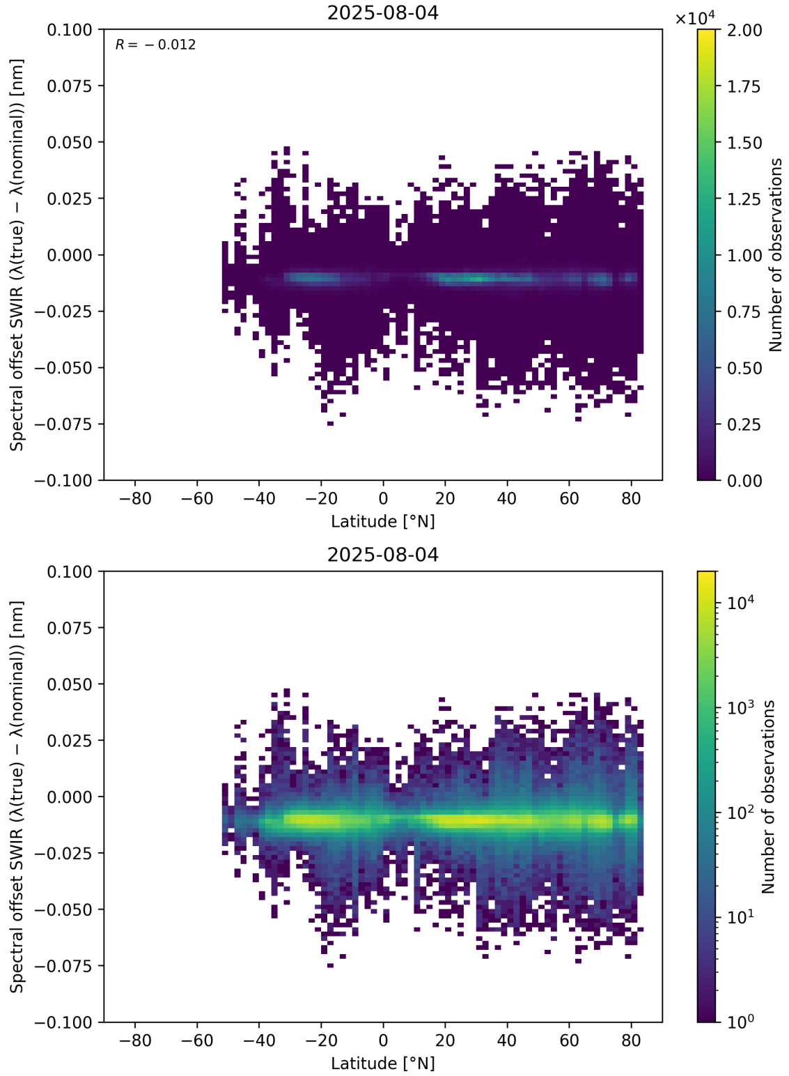
Figure 62: Scatter density plot of “Latitude” against “Spectral offset SWIR ( \lambda_{\text{true}} - \lambda_{\text{nominal}} )” for 2025-08-04 to 2025-08-05.
