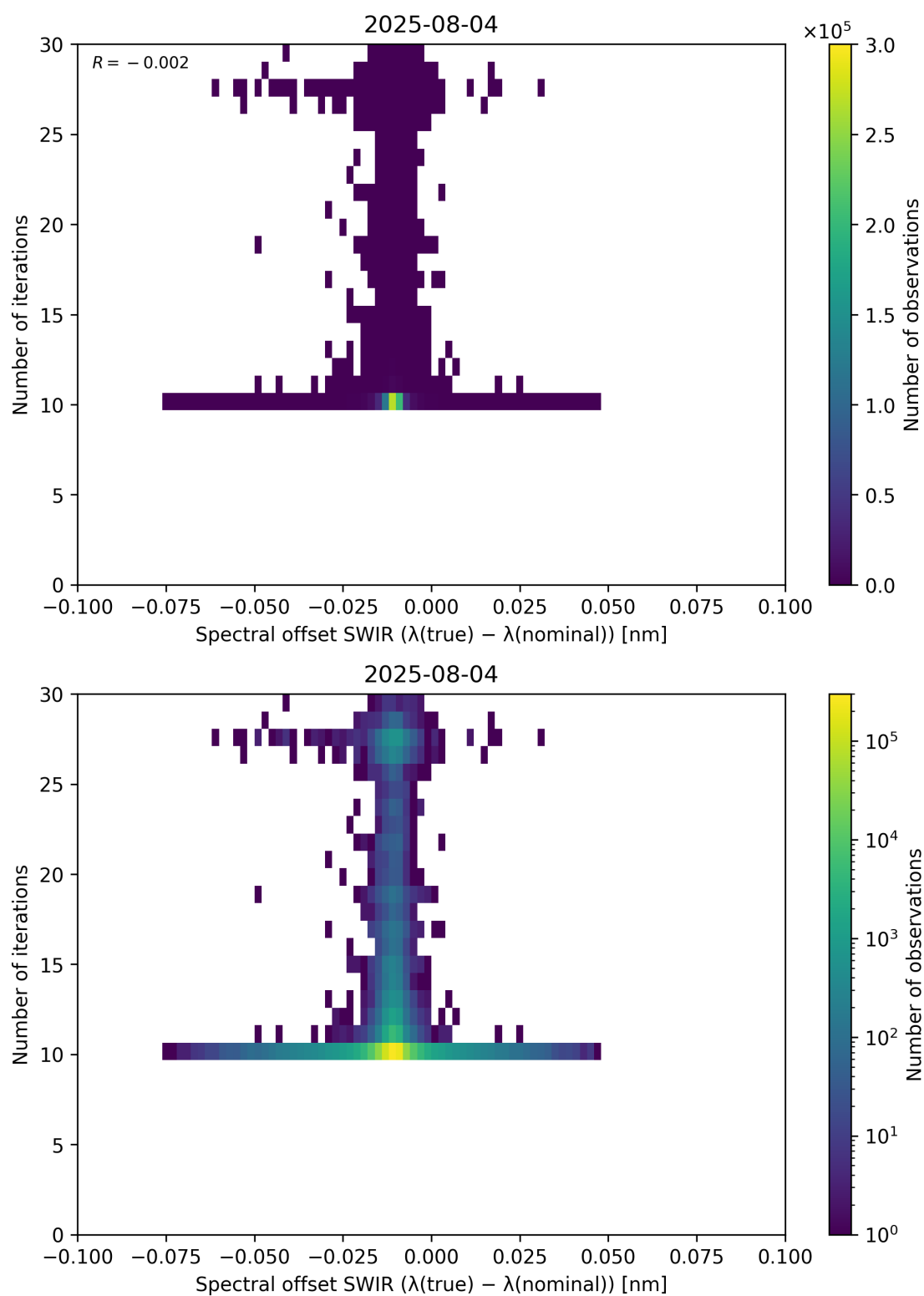
Figure 121: Scatter density plot of “Spectral offset SWIR ( \lambda_{\text{true}} - \lambda_{\text{nominal}} )” against “Number of iterations” for 2025-08-04 to 2025-08-05.
