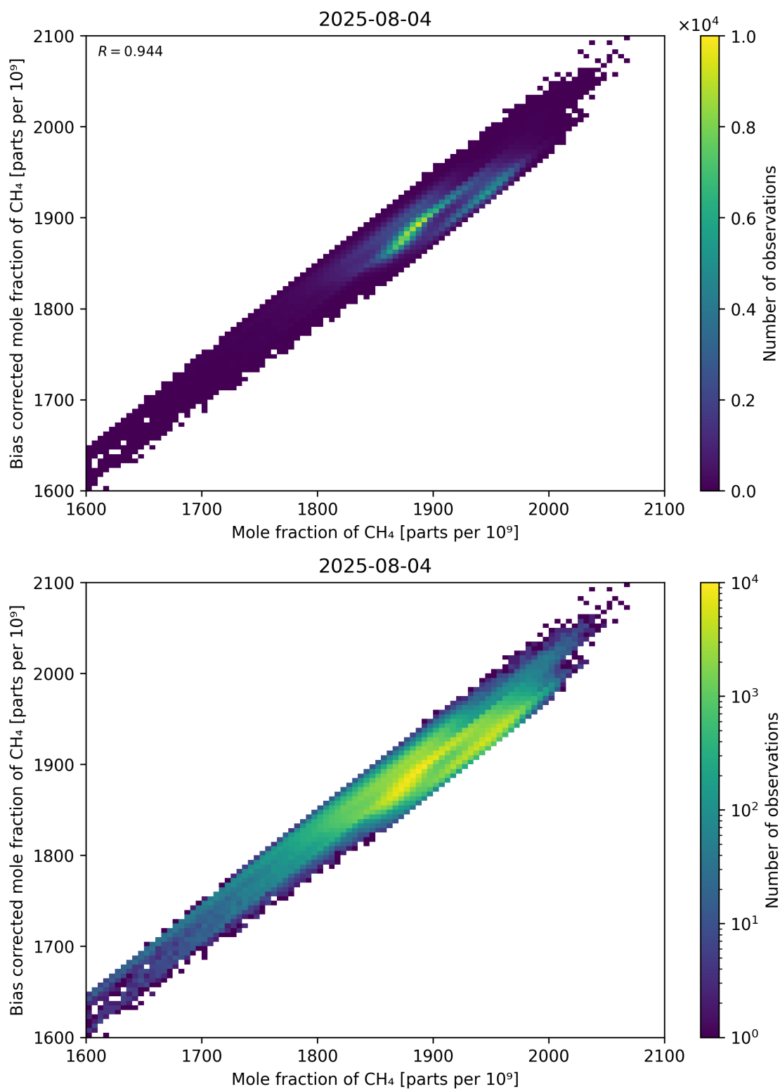
Figure 74: Scatter density plot of “Mole fraction of CH 4 ” against “Bias corrected mole fraction of CH 4 ” for 2025-08-04 to 2025-08-05.
