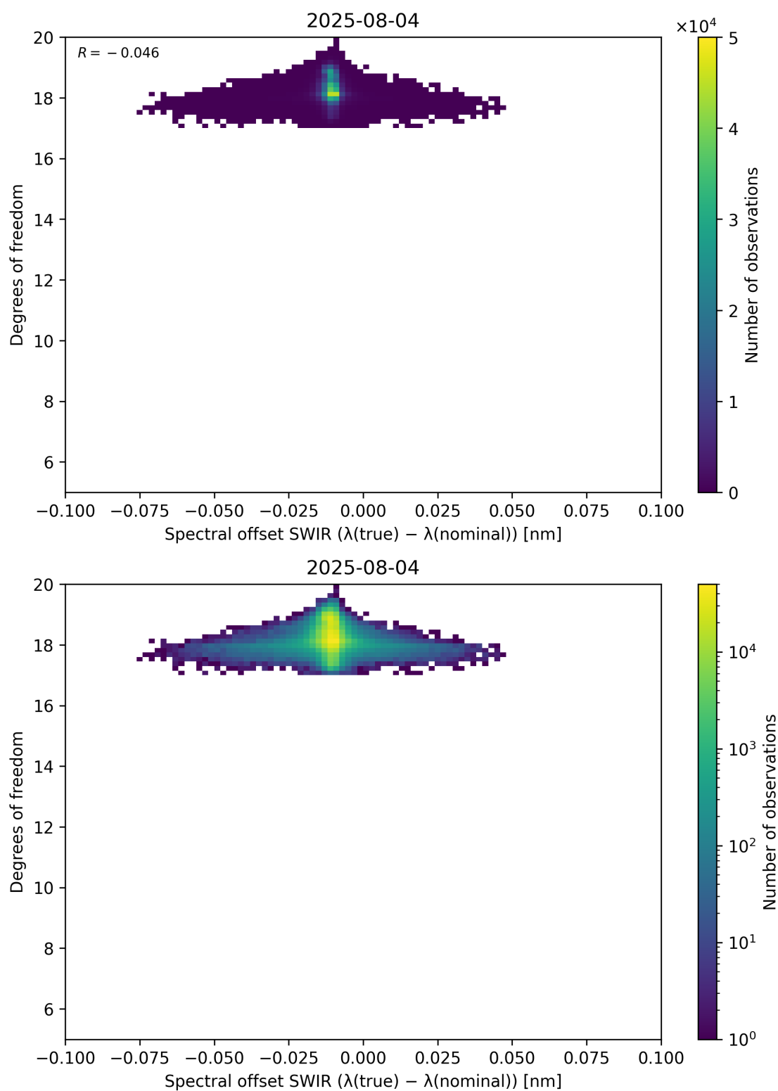
Figure 119: Scatter density plot of “Spectral offset SWIR ( \lambda_{\text{true}} - \lambda_{\text{nominal}} )” against “Degrees of freedom” for 2025-08-04 to 2025-08-05.
