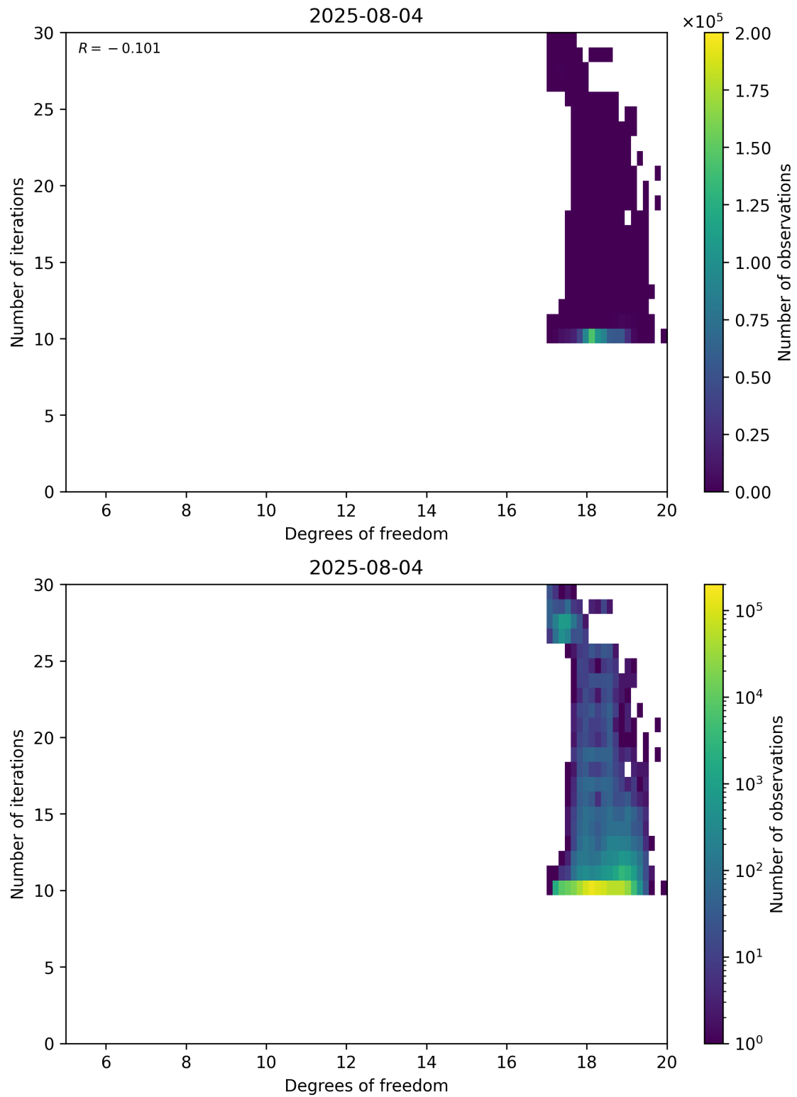
Figure 52: Scatter density plot of “Degrees of freedom” against “Number of iterations” for 2025-08-04 to 2025-08-05.
