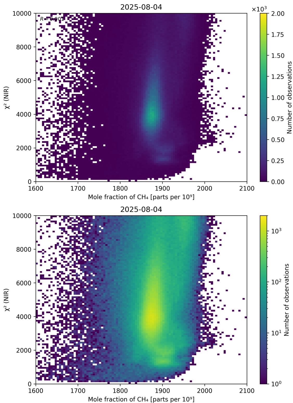
Figure 70: Scatter density plot of “Mole fraction of \text{CH}_4 ” against “ \chi^2 (NIR)” for 2025-08-04 to 2025-08-05.
