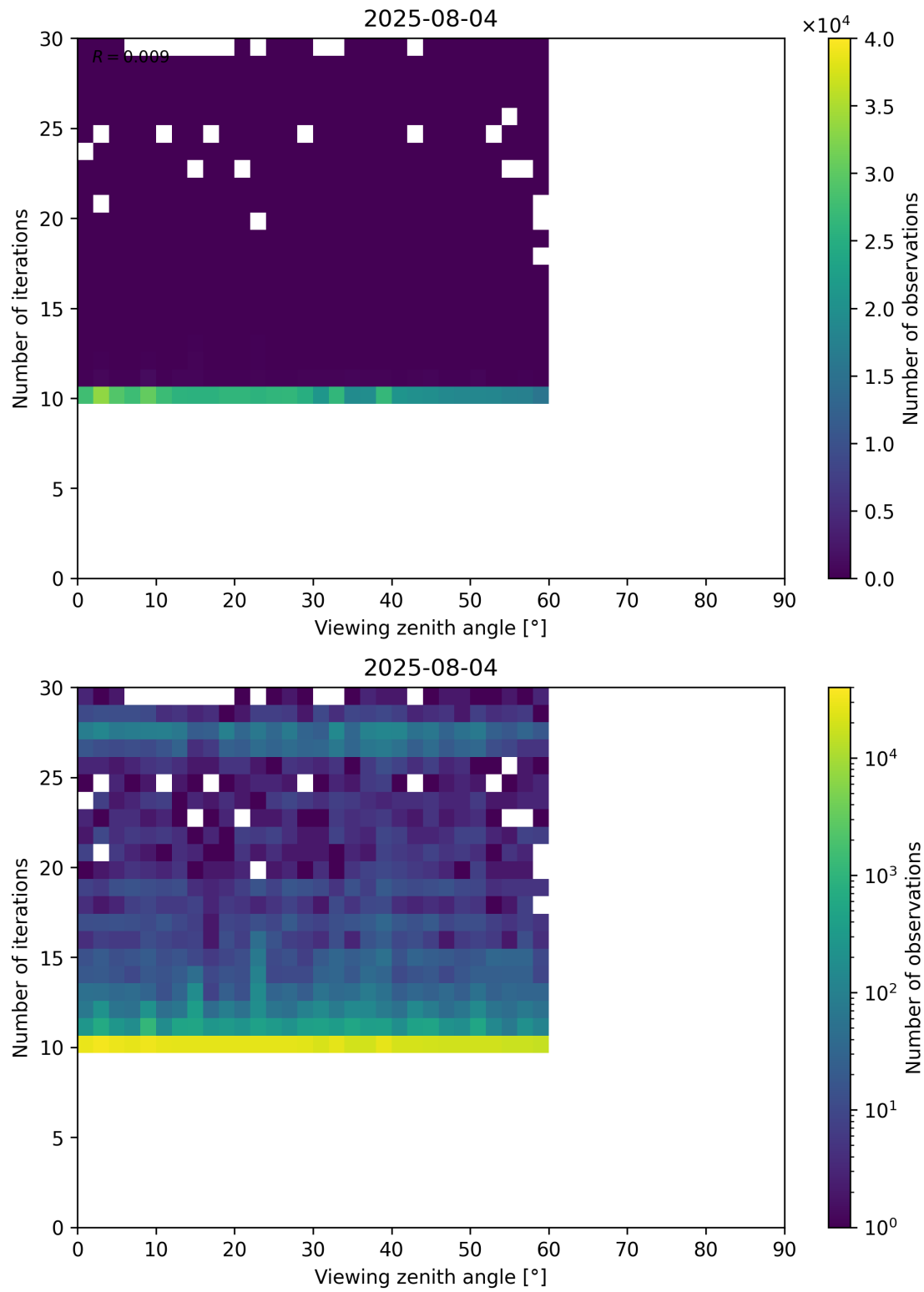
Figure 113: Scatter density plot of “Viewing zenith angle” against “Number of iterations” for 2025-08-04 to 2025-08-05.
