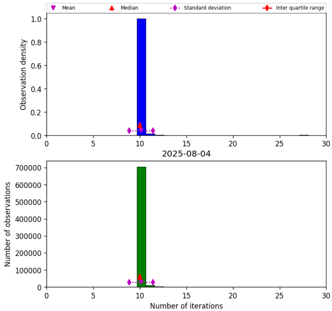
Figure 31: Histogram of “Number of iterations” for 2025-08-04 to 2025-08-05
