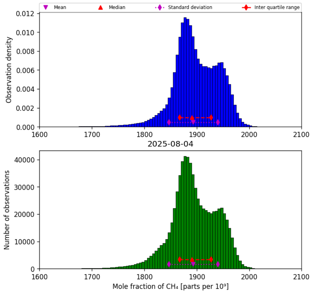
Figure 23: Histogram of “Mole fraction of CH 4 ” for 2025-08-04 to 2025-08-05
