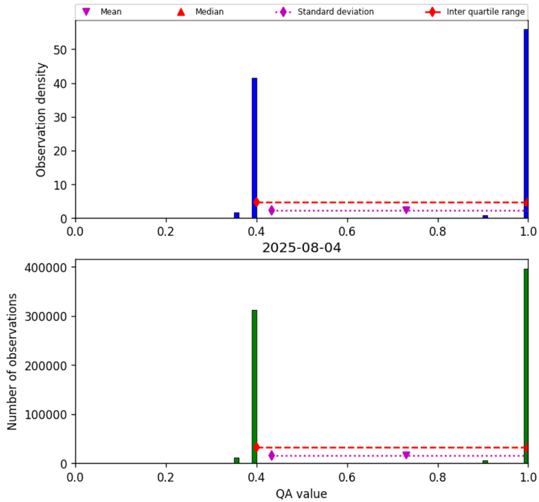
Figure 22: Histogram of “QA value” for 2025-08-04 to 2025-08-05
