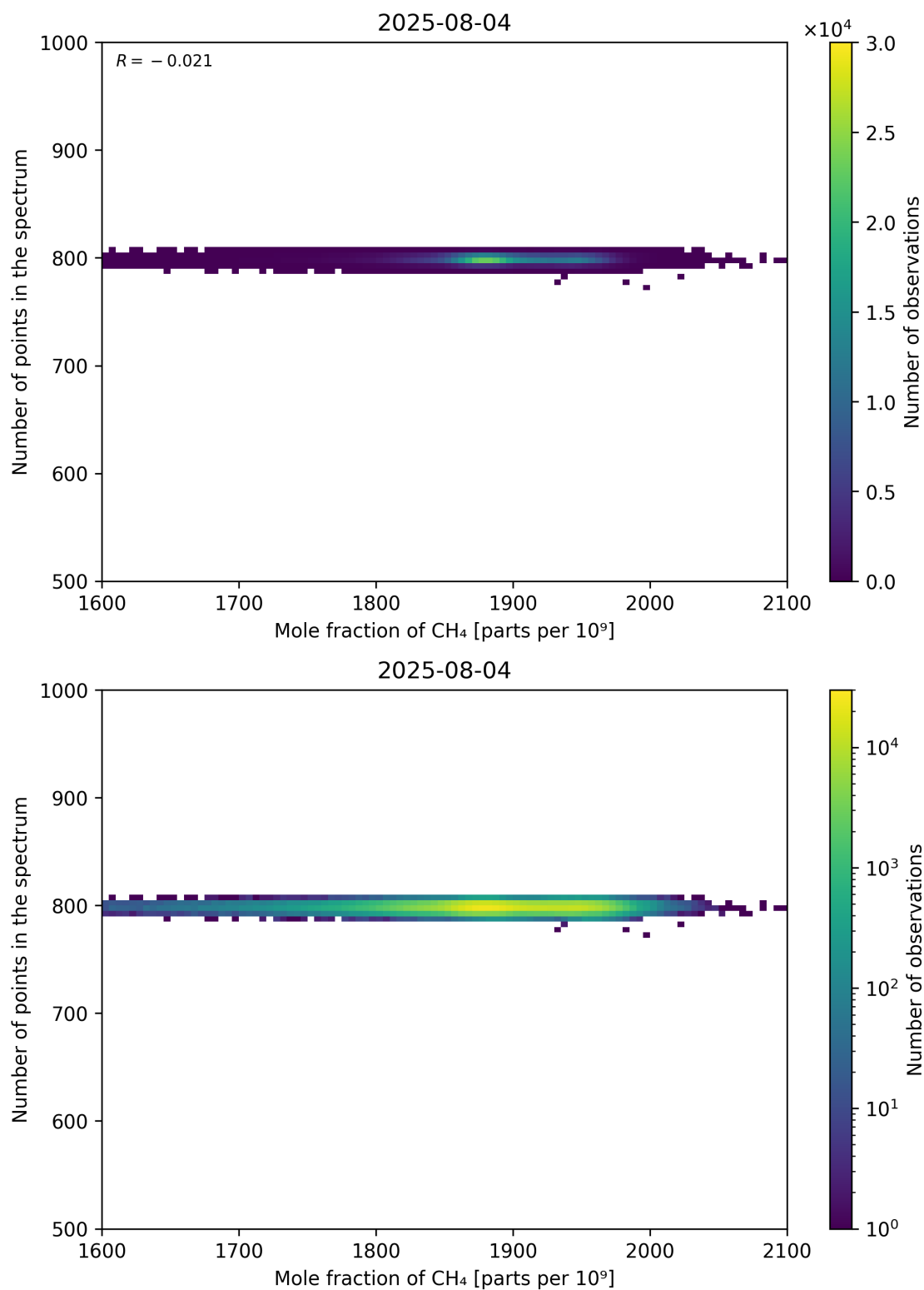
Figure 77: Scatter density plot of “Mole fraction of CH 4 ” against “Number of points in the spectrum” for 2025-08-04 to 2025-08-05.
