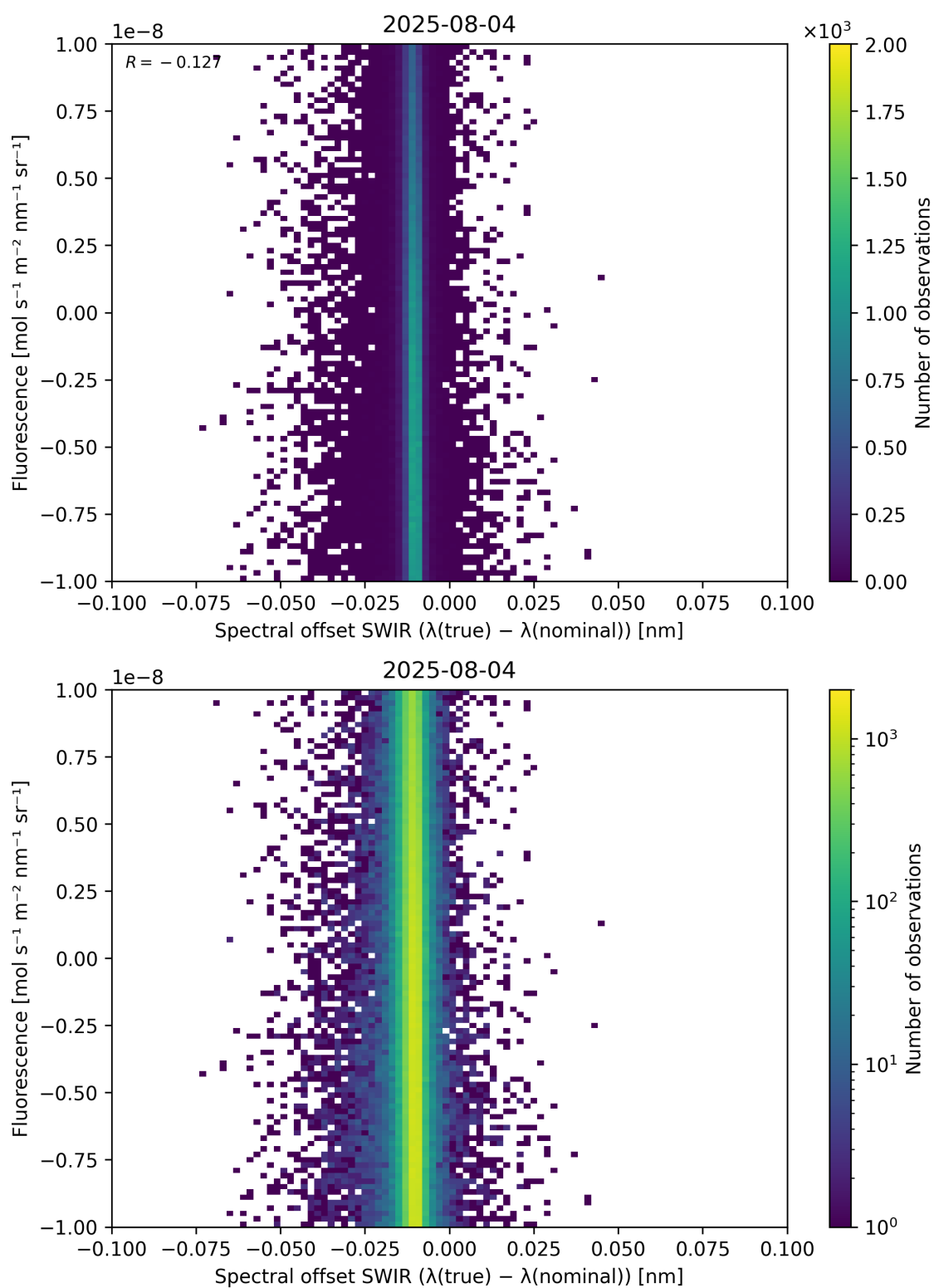
Figure 120: Scatter density plot of “Spectral offset SWIR ( \lambda_{\text{true}} - \lambda_{\text{nominal}} )” against “Fluorescence” for 2025-08-04 to 2025-08-05.
