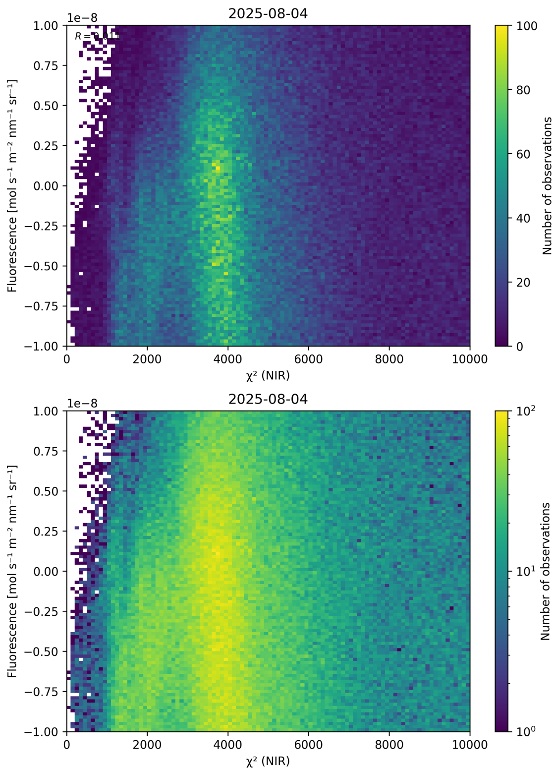
Figure 45: Scatter density plot of “ \chi^2 (NIR)” against “Fluorescence” for 2025-08-04 to 2025-08-05.
