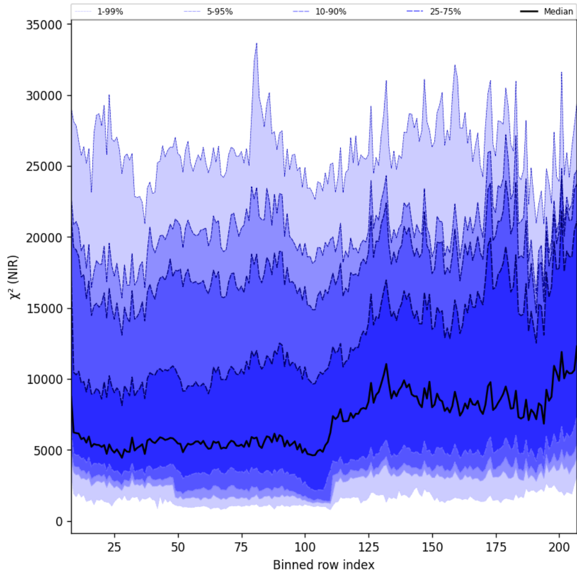
Figure 40: Along track statistics of “ \chi^2 (NIR)” for 2025-08-04 to 2025-08-05
