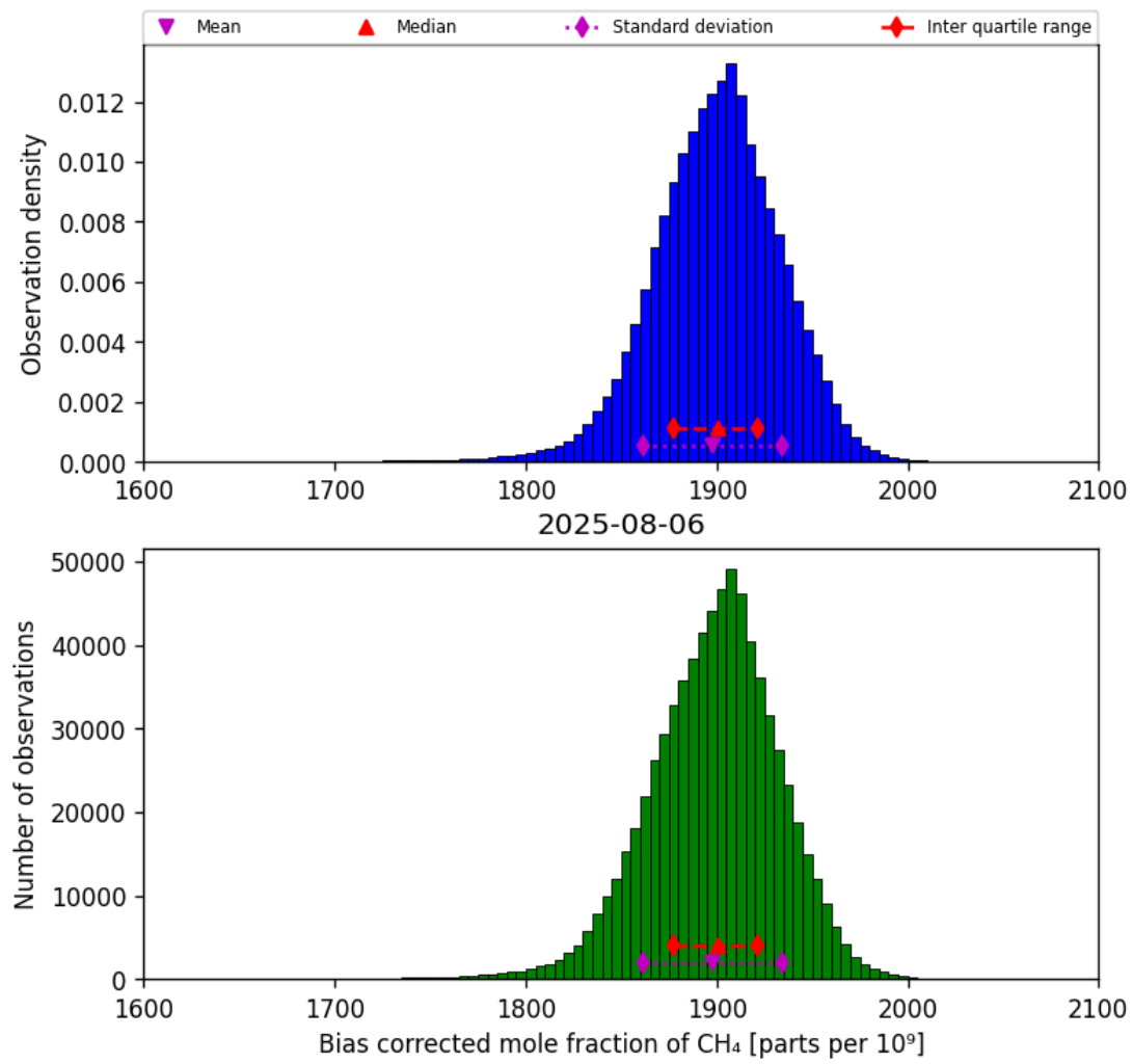
Figure 25: Histogram of “Bias corrected mole fraction of CH 4 ” for 2025-08-05 to 2025-08-07
