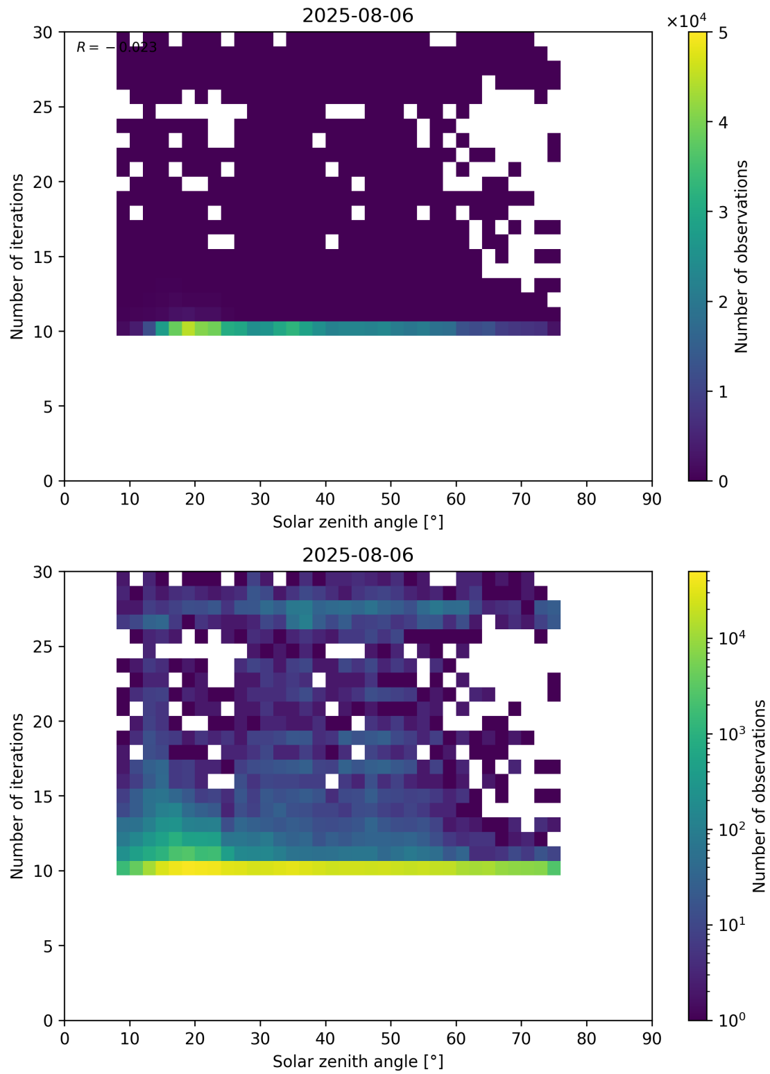
Figure 102: Scatter density plot of “Solar zenith angle” against “Number of iterations” for 2025-08-05 to 2025-08-07.
