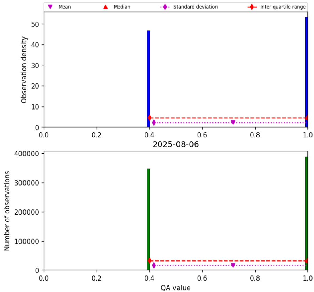
Figure 22: Histogram of “QA value” for 2025-08-05 to 2025-08-07
