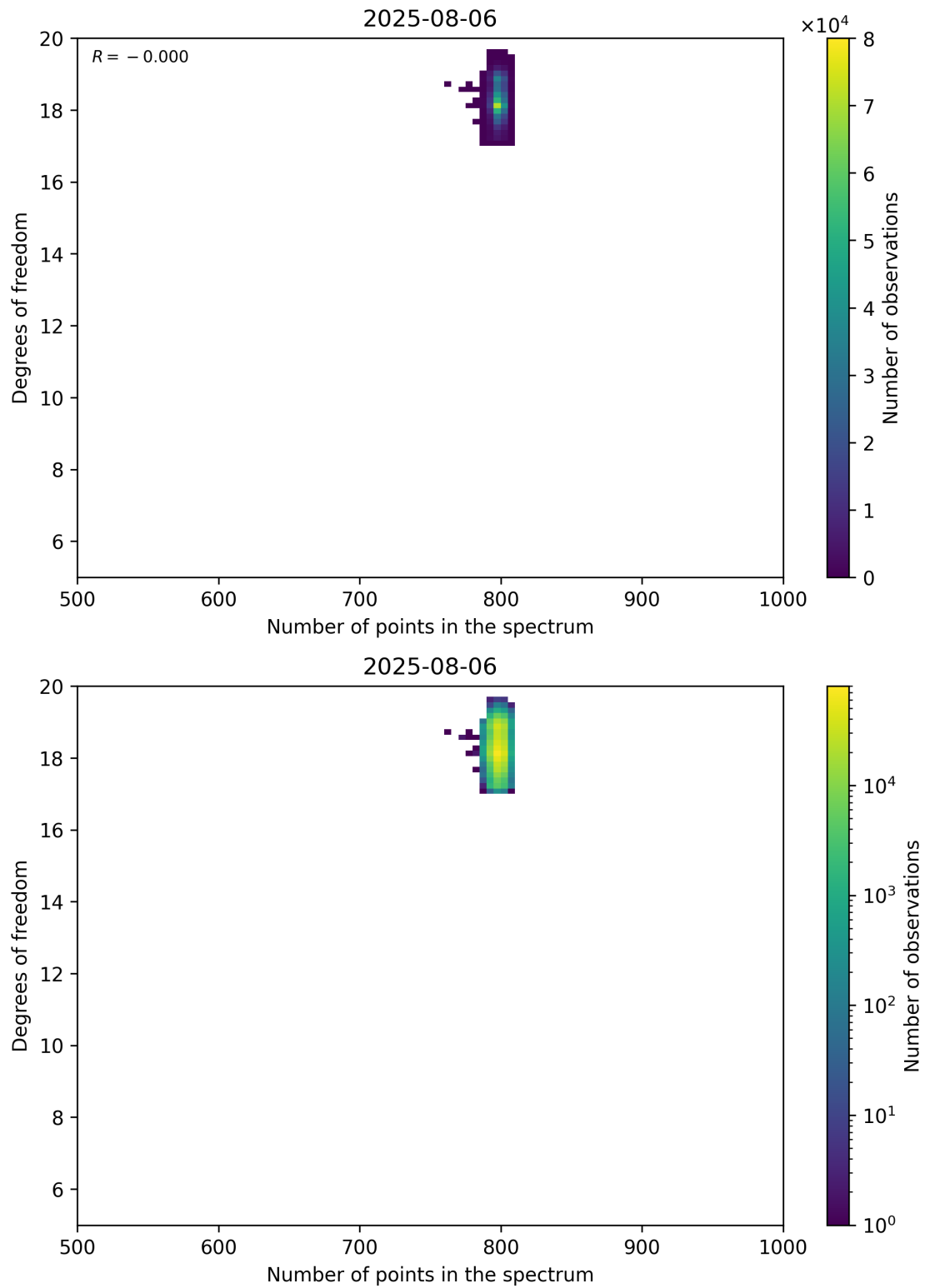
Figure 90: Scatter density plot of “Number of points in the spectrum” against “Degrees of freedom” for 2025-08-05 to 2025-08-07.
