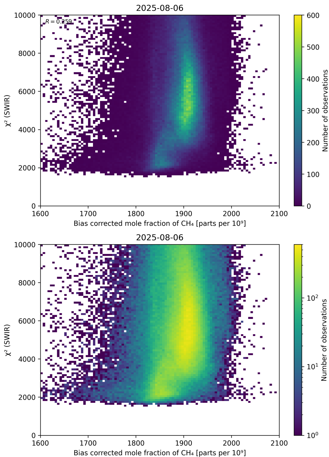
Figure 64: Scatter density plot of “Bias corrected mole fraction of \text{CH}_4 ” against “ \chi^2 (SWIR)” for 2025-08-05 to 2025-08-07.
