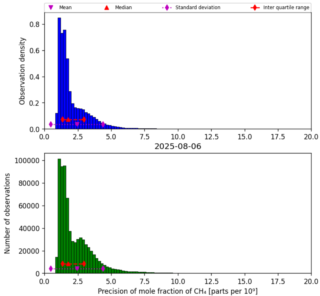
Figure 24: Histogram of “Precision of mole fraction of CH 4 ” for 2025-08-05 to 2025-08-07
