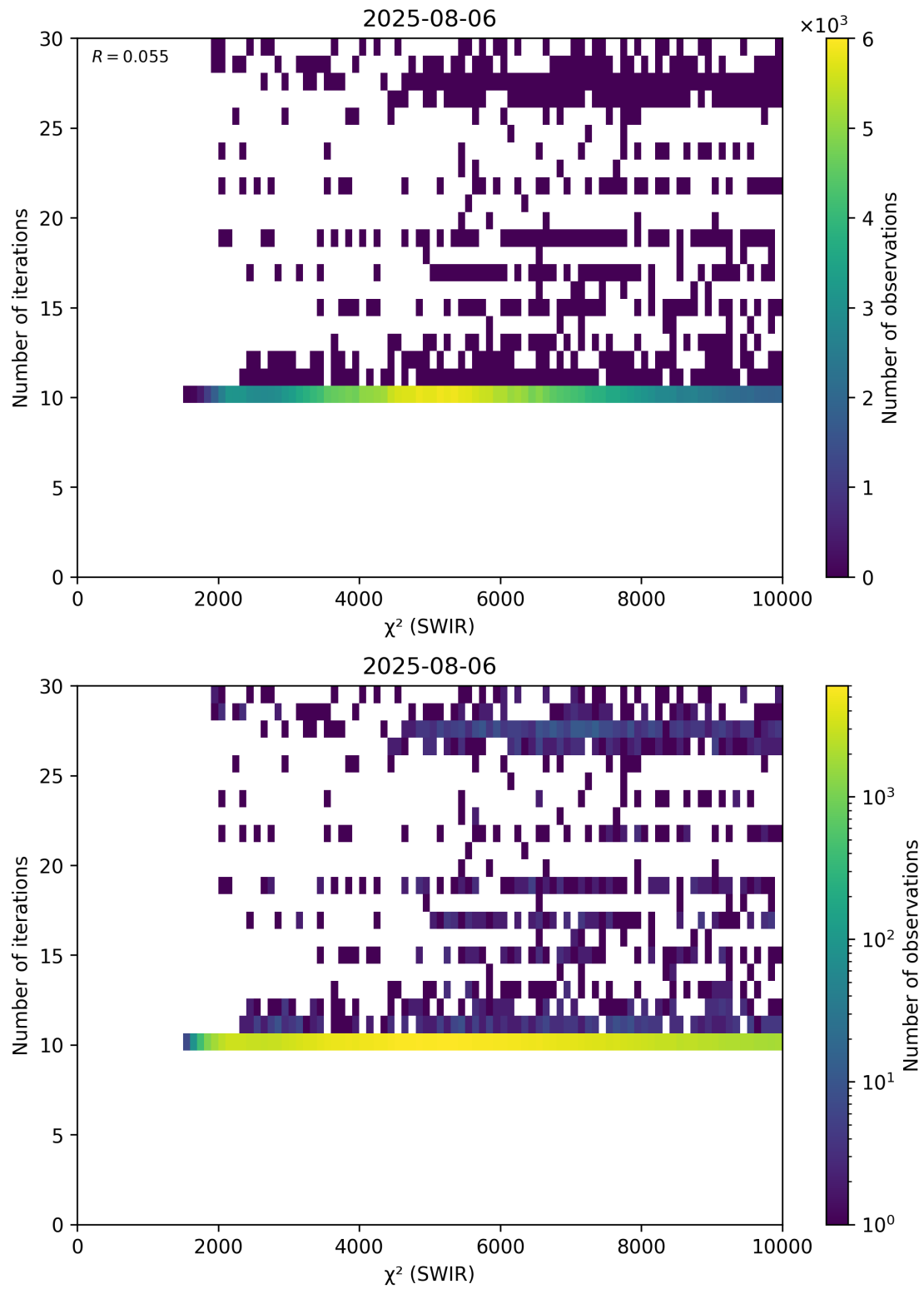
Figure 50: Scatter density plot of “ \chi^2 (SWIR)” against “Number of iterations” for 2025-08-05 to 2025-08-07.
