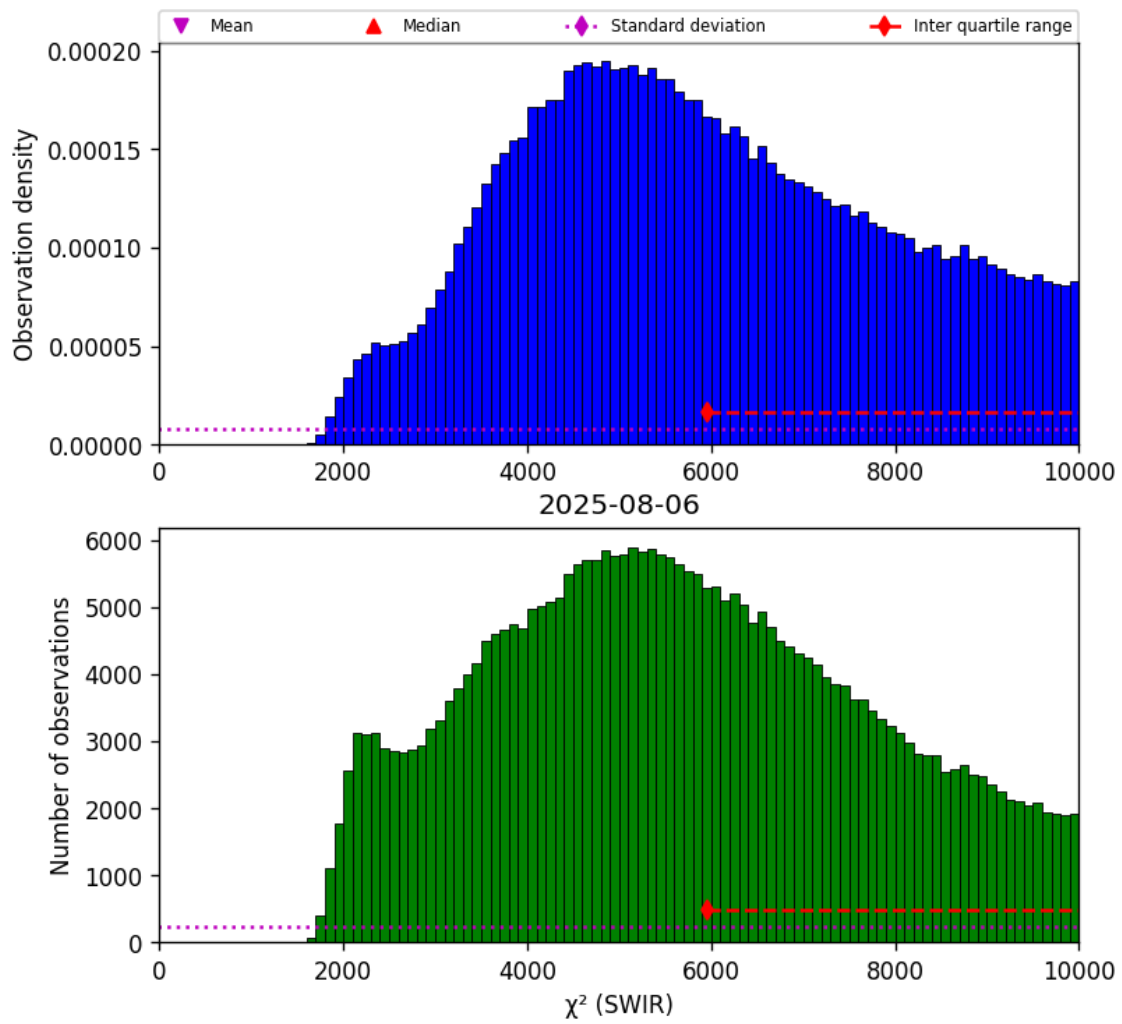
Figure 28: Histogram of " \chi^2 (SWIR)" for 2025-08-05 to 2025-08-07
