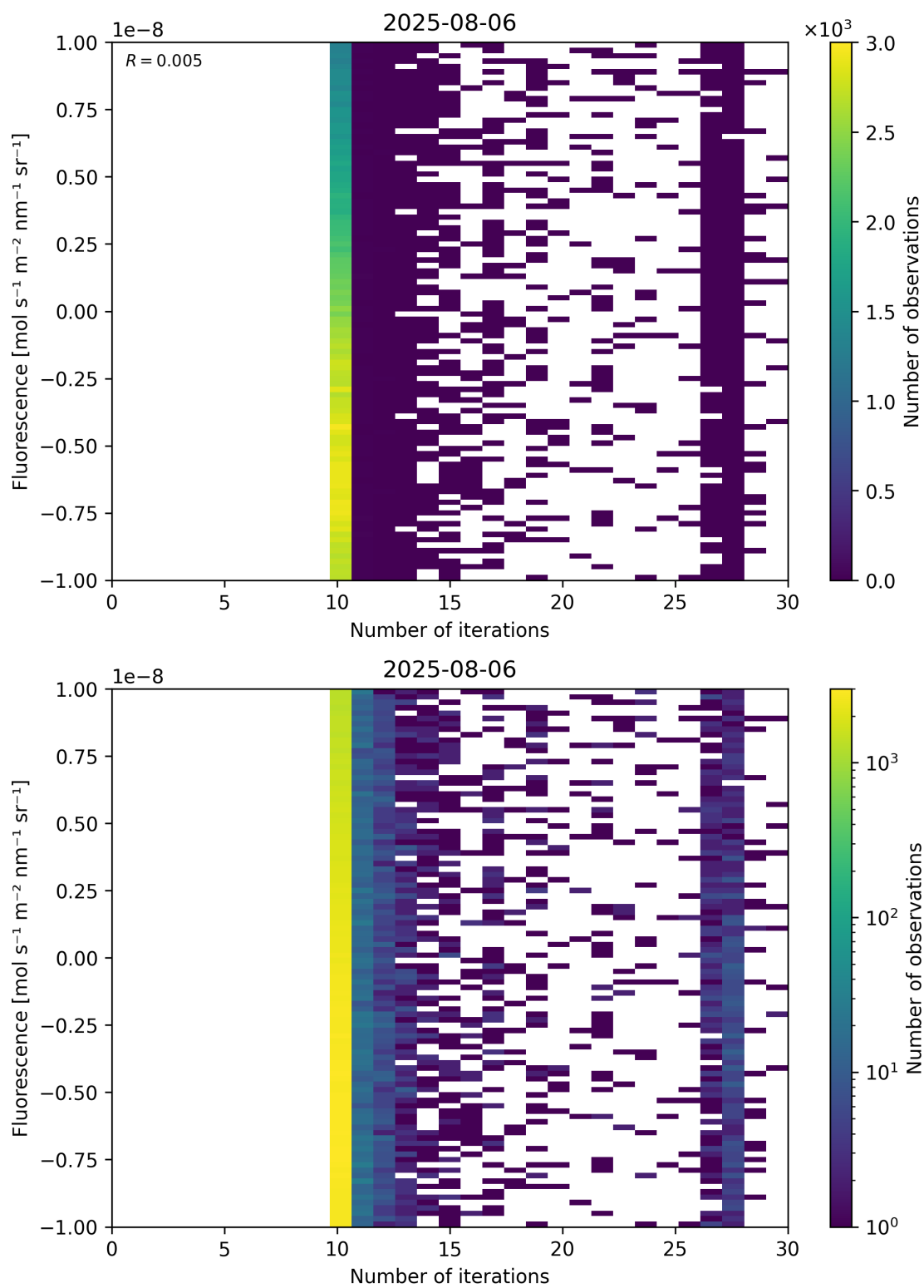
Figure 87: Scatter density plot of "Number of iterations" against "Fluorescence" for 2025-08-05 to 2025-08-07.
