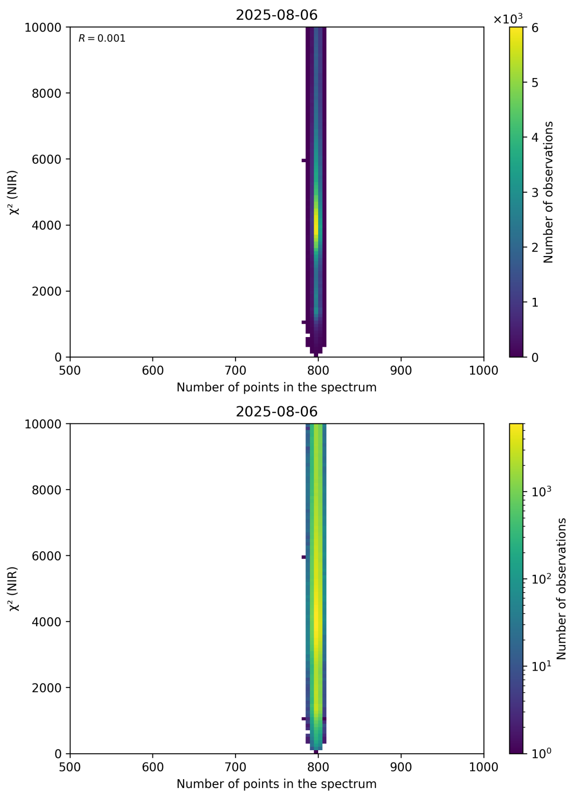
Figure 88: Scatter density plot of “Number of points in the spectrum” against “ \chi^2 (NIR)” for 2025-08-05 to 2025-08-07.
