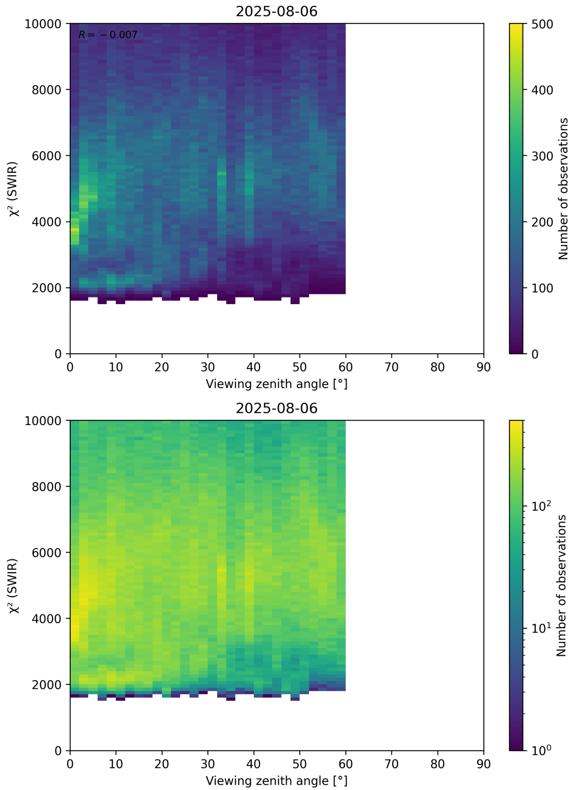
Figure 106: Scatter density plot of “Viewing zenith angle” against “ \chi^2 (SWIR)” for 2025-08-05 to 2025-08-07.
