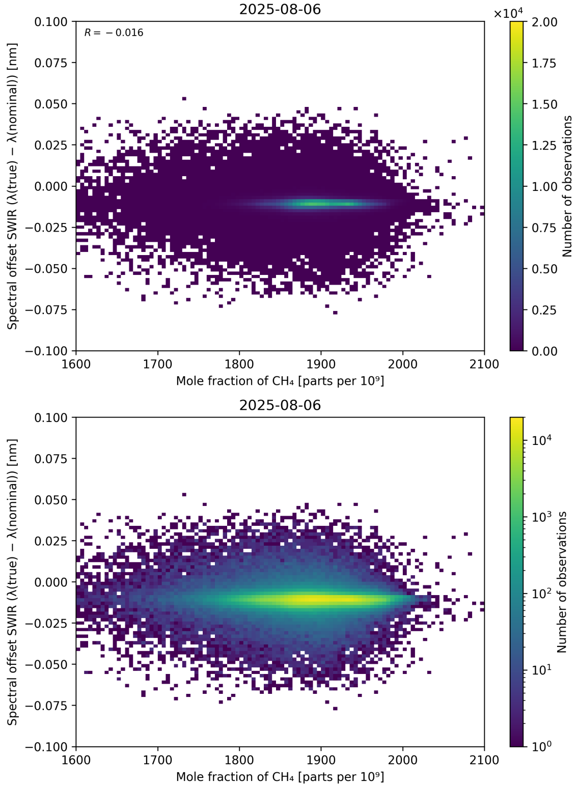
Figure 86: Scatter density plot of “Mole fraction of CH 4 ” against “Spectral offset SWIR ( \lambda_{\text{true}} - \lambda_{\text{nominal}} )” for 2025-08-05 to 2025-08-07.
