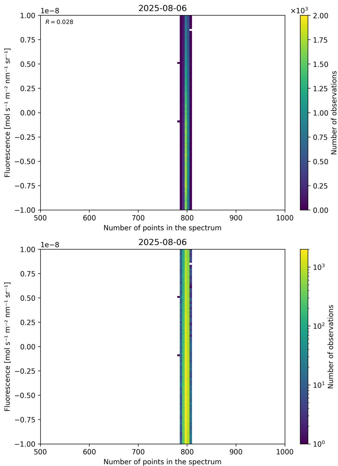
Figure 91: Scatter density plot of “Number of points in the spectrum” against “Fluorescence” for 2025-08-05 to 2025-08-07.
