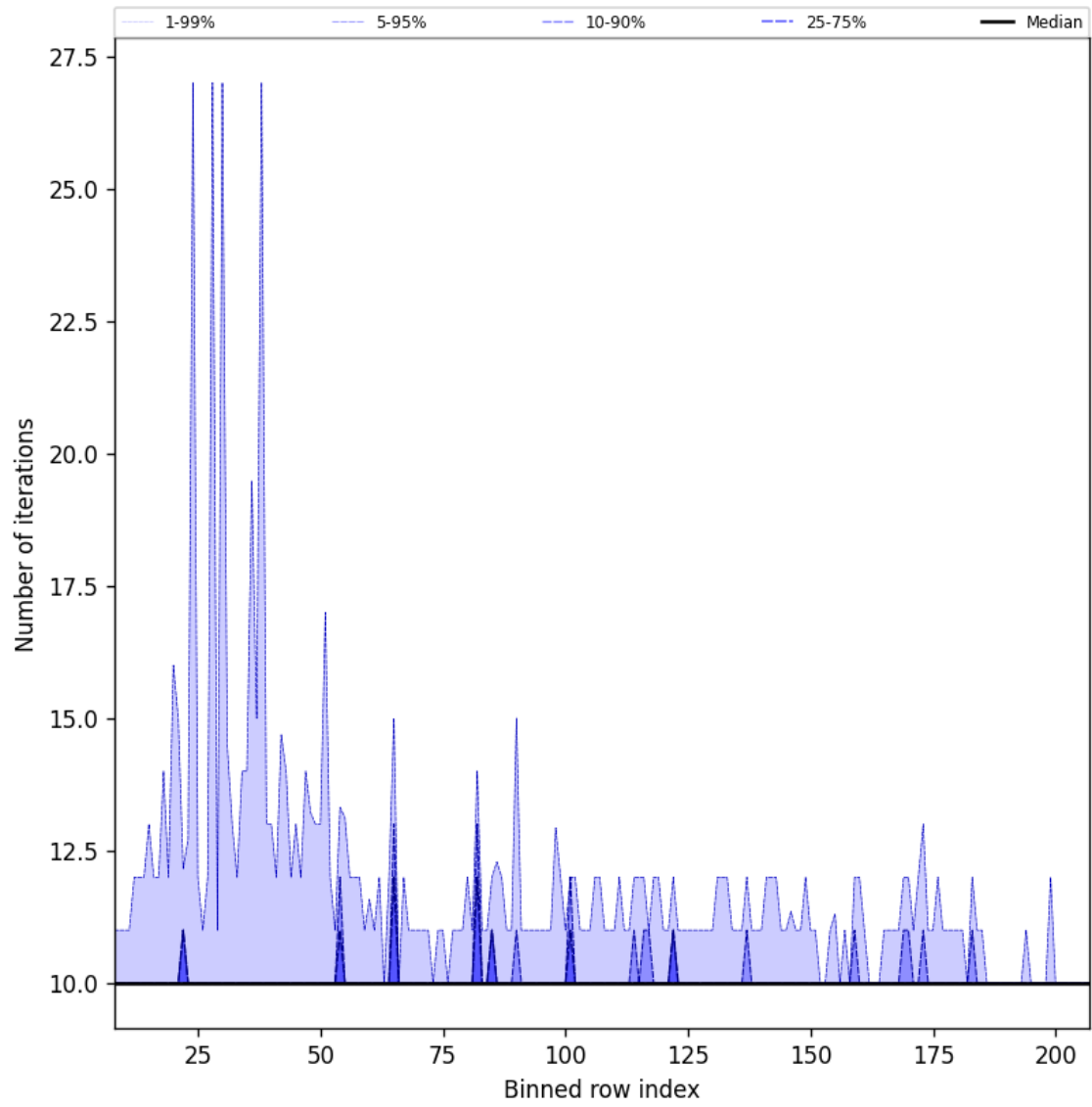
Figure 42: Along track statistics of “Number of iterations” for 2025-08-05 to 2025-08-07
