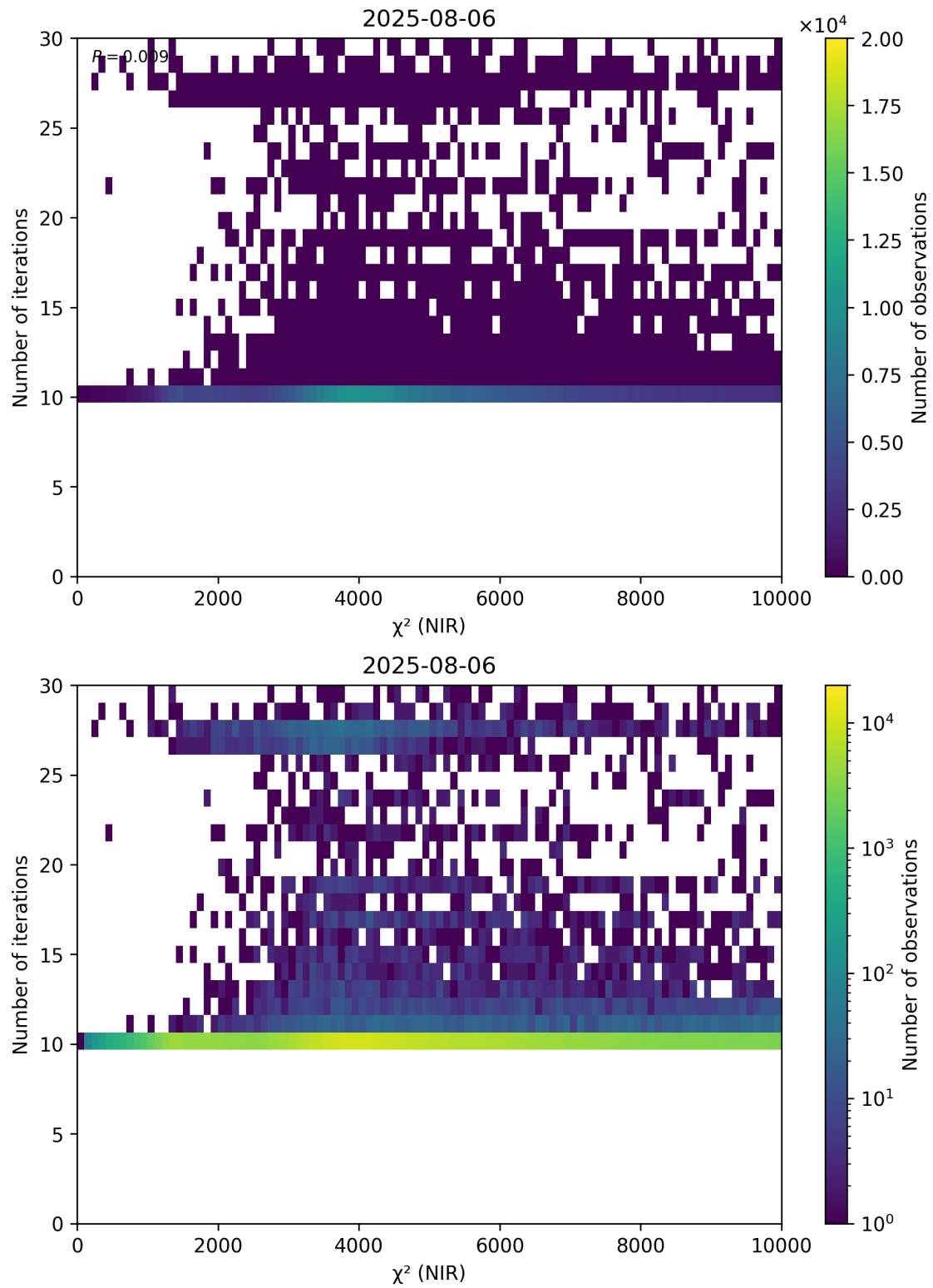
Figure 46: Scatter density plot of “ \chi^2 (NIR)” against “Number of iterations” for 2025-08-05 to 2025-08-07.
