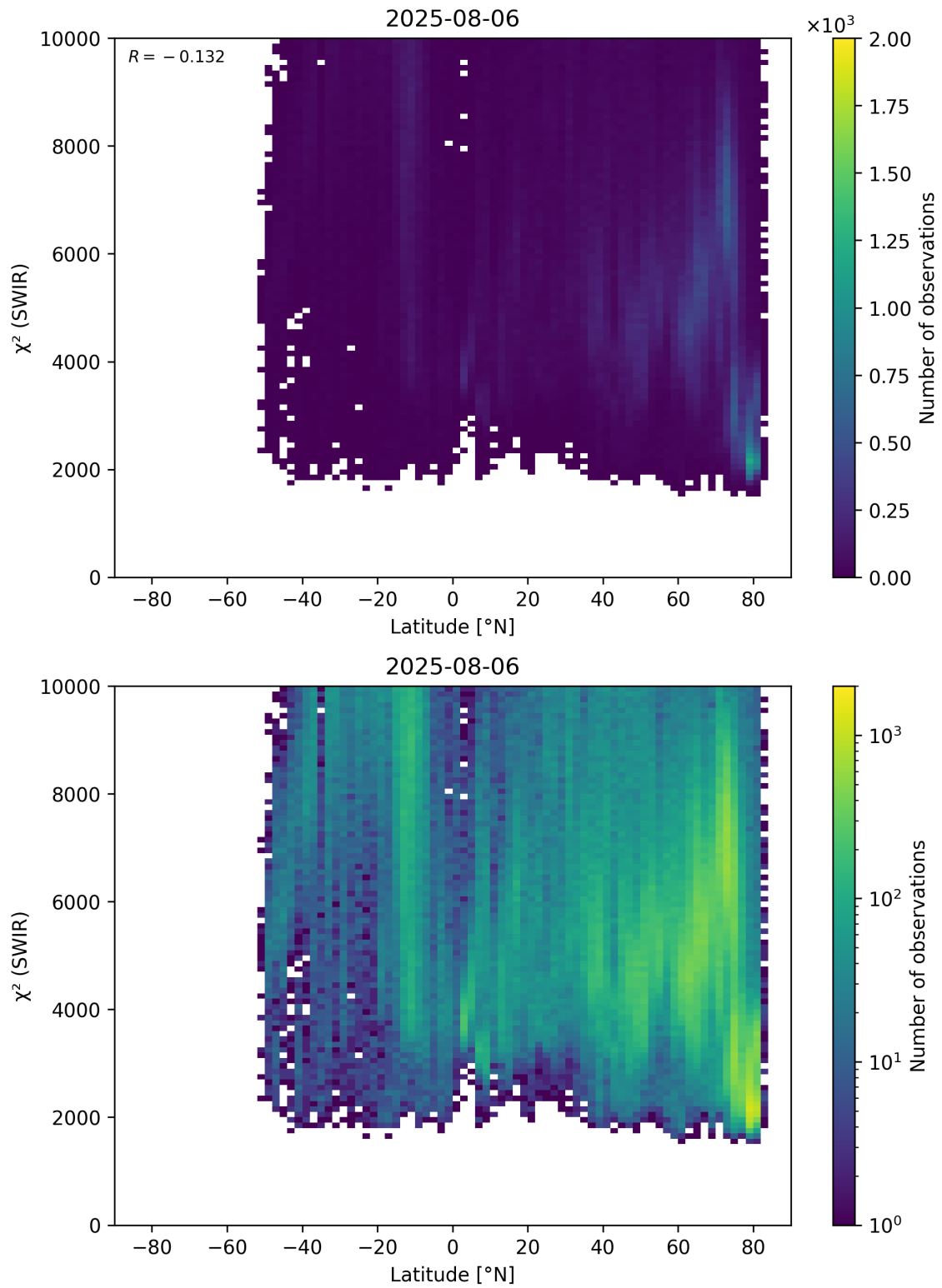
Figure 54: Scatter density plot of “Latitude” against “ \chi^2 (SWIR)” for 2025-08-05 to 2025-08-07.
