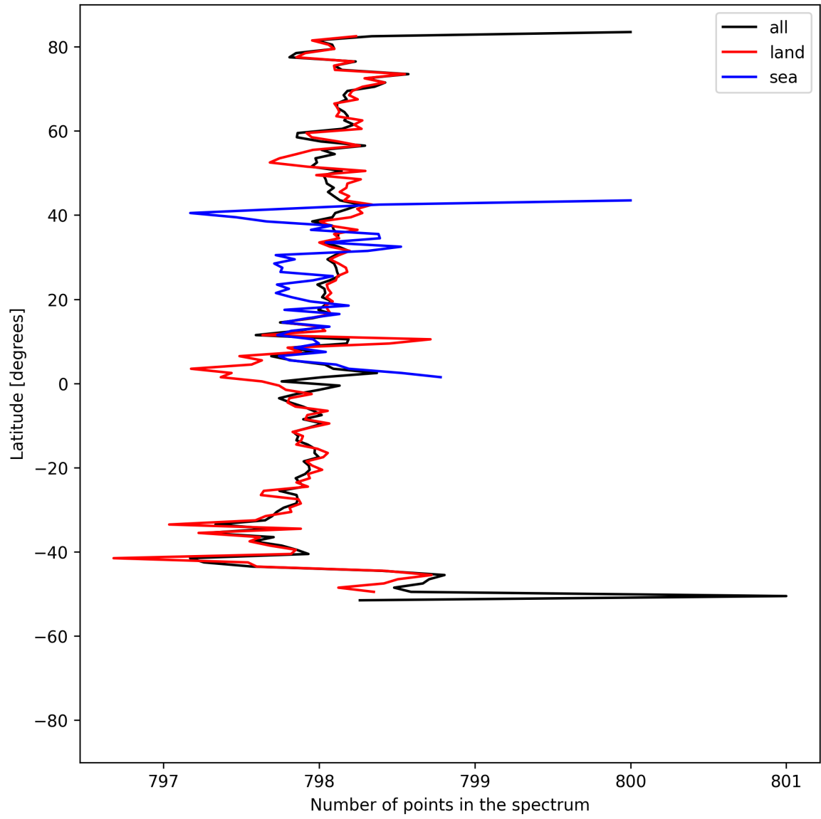
Figure 15: Zonal average of “Number of points in the spectrum” for 2025-08-05 to 2025-08-07.
