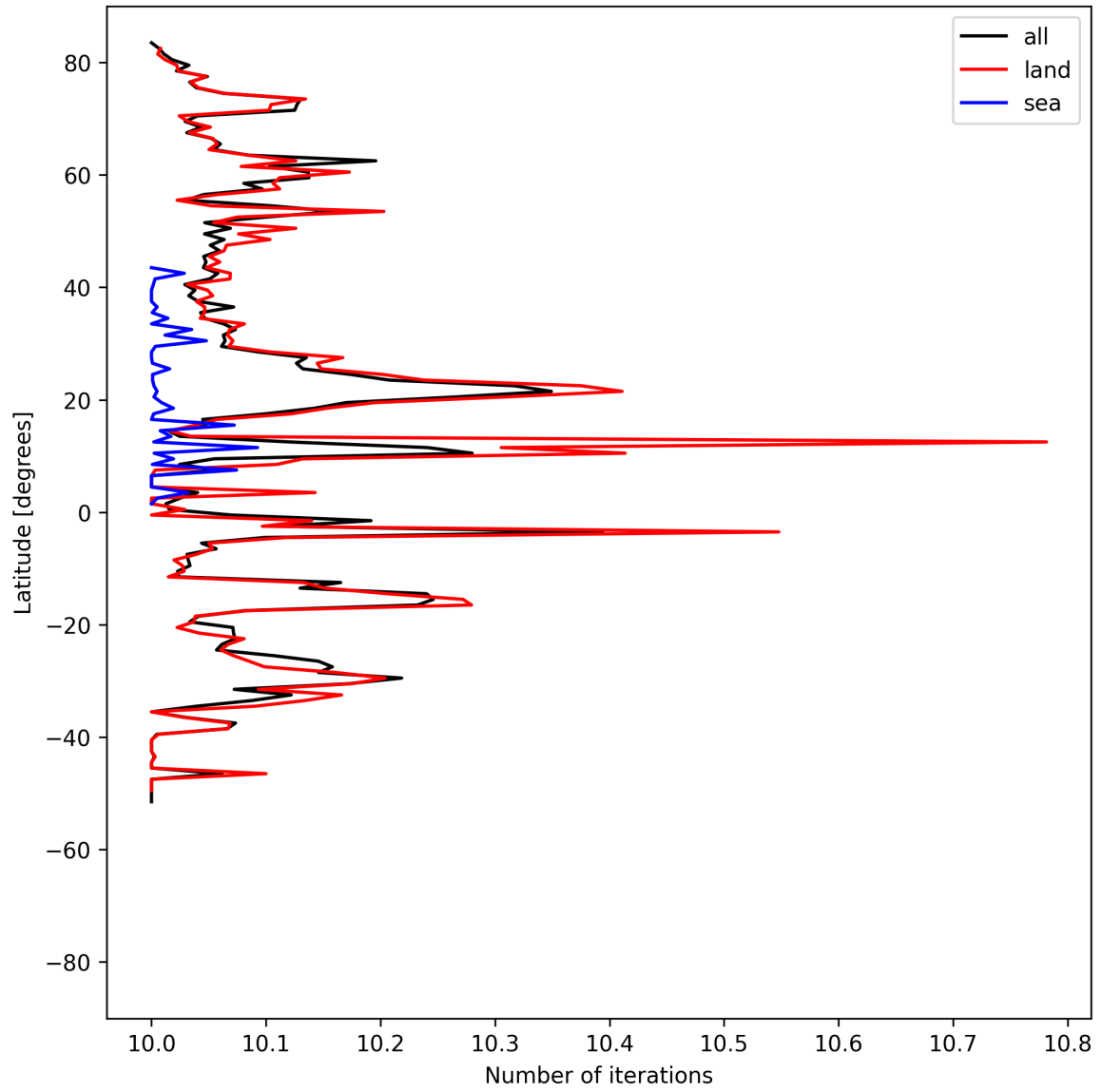
Figure 20: Zonal average of “Number of iterations” for 2025-08-05 to 2025-08-07.
