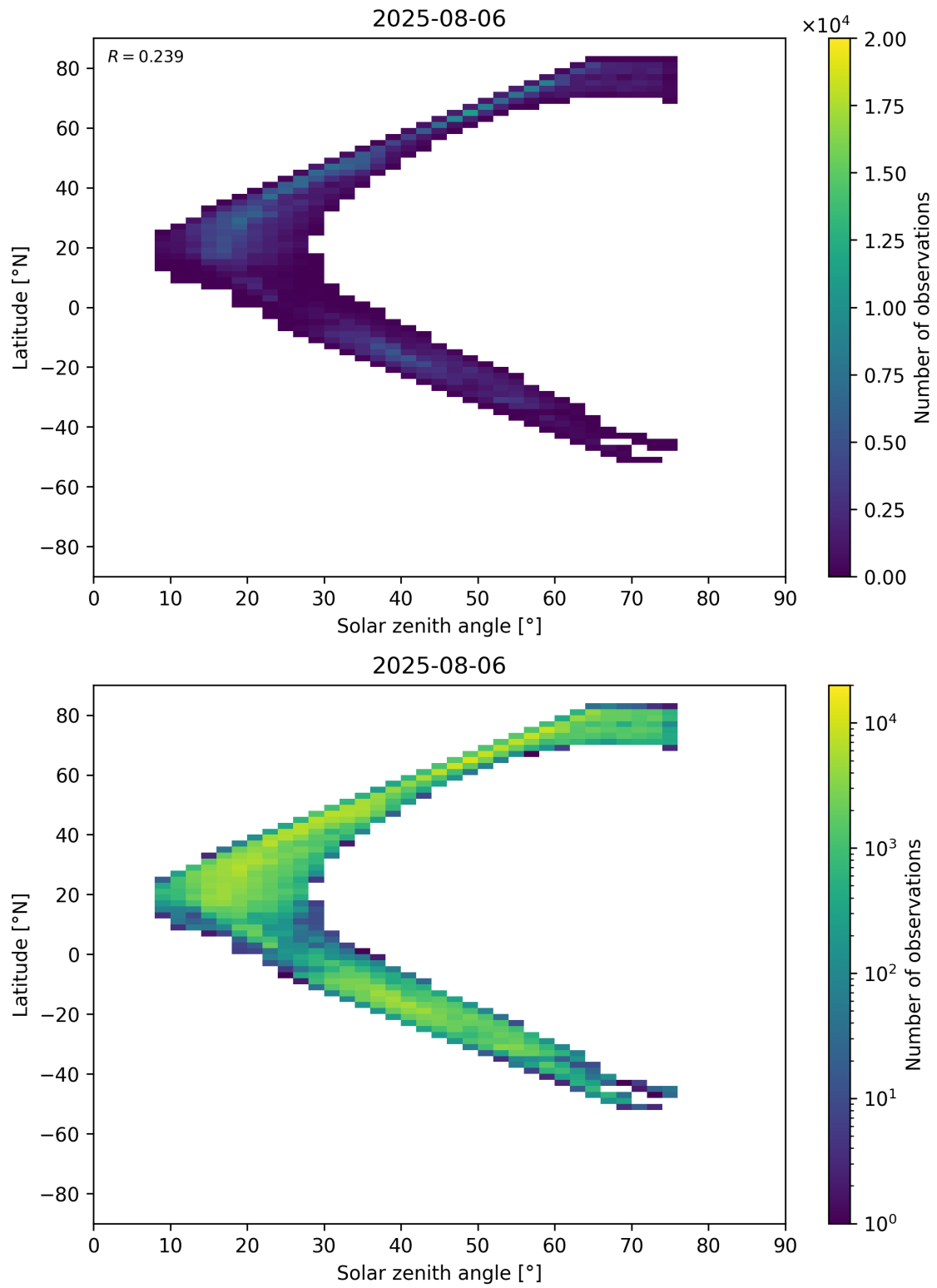
Figure 98: Scatter density plot of “Solar zenith angle” against “Latitude” for 2025-08-05 to 2025-08-07.
