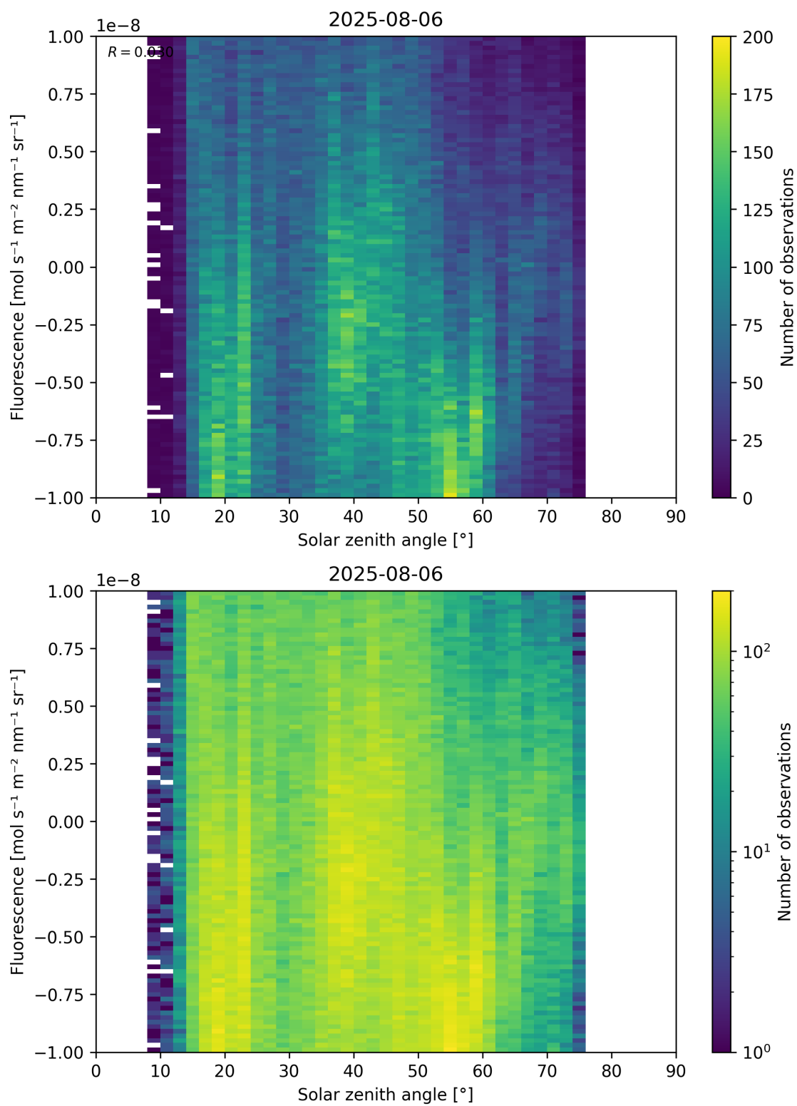
Figure 97: Scatter density plot of “Solar zenith angle” against “Fluorescence” for 2025-08-05 to 2025-08-07.
