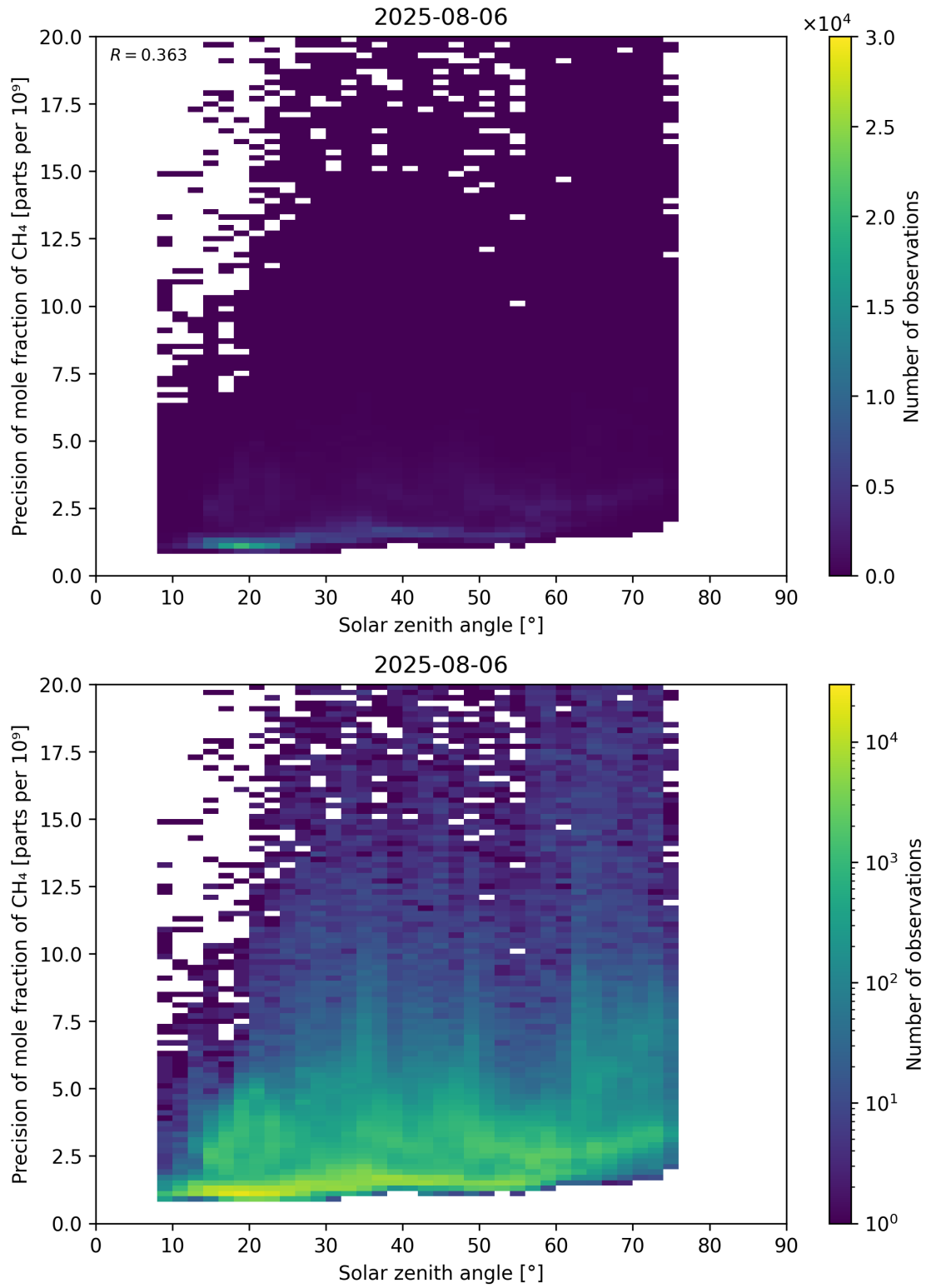
Figure 101: Scatter density plot of “Solar zenith angle” against “Precision of mole fraction of CH 4 ” for 2025-08-05 to 2025-08-07.
