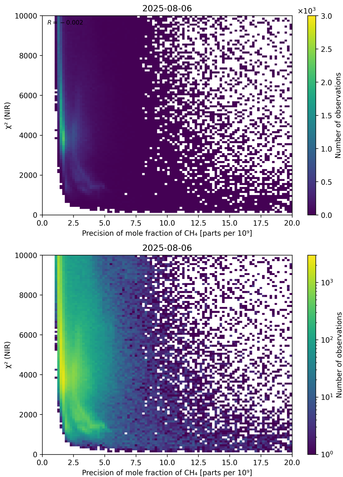
Figure 78: Scatter density plot of “Precision of mole fraction of CH 4 ” against “ \chi^2 (NIR)” for 2025-08-05 to 2025-08-07.
