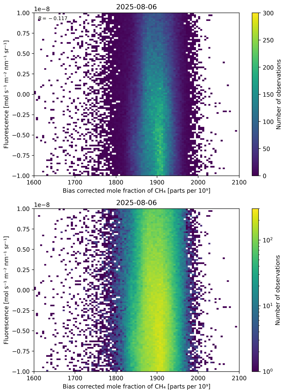
Figure 66: Scatter density plot of “Bias corrected mole fraction of \text{CH}_4 ” against “Fluorescence” for 2025-08-05 to 2025-08-07.
