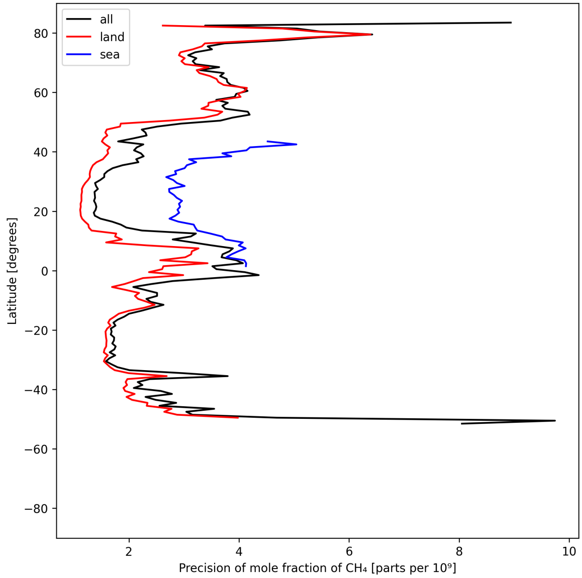
Figure 13: Zonal average of “Precision of mole fraction of CH 4 ” for 2025-08-05 to 2025-08-07.
