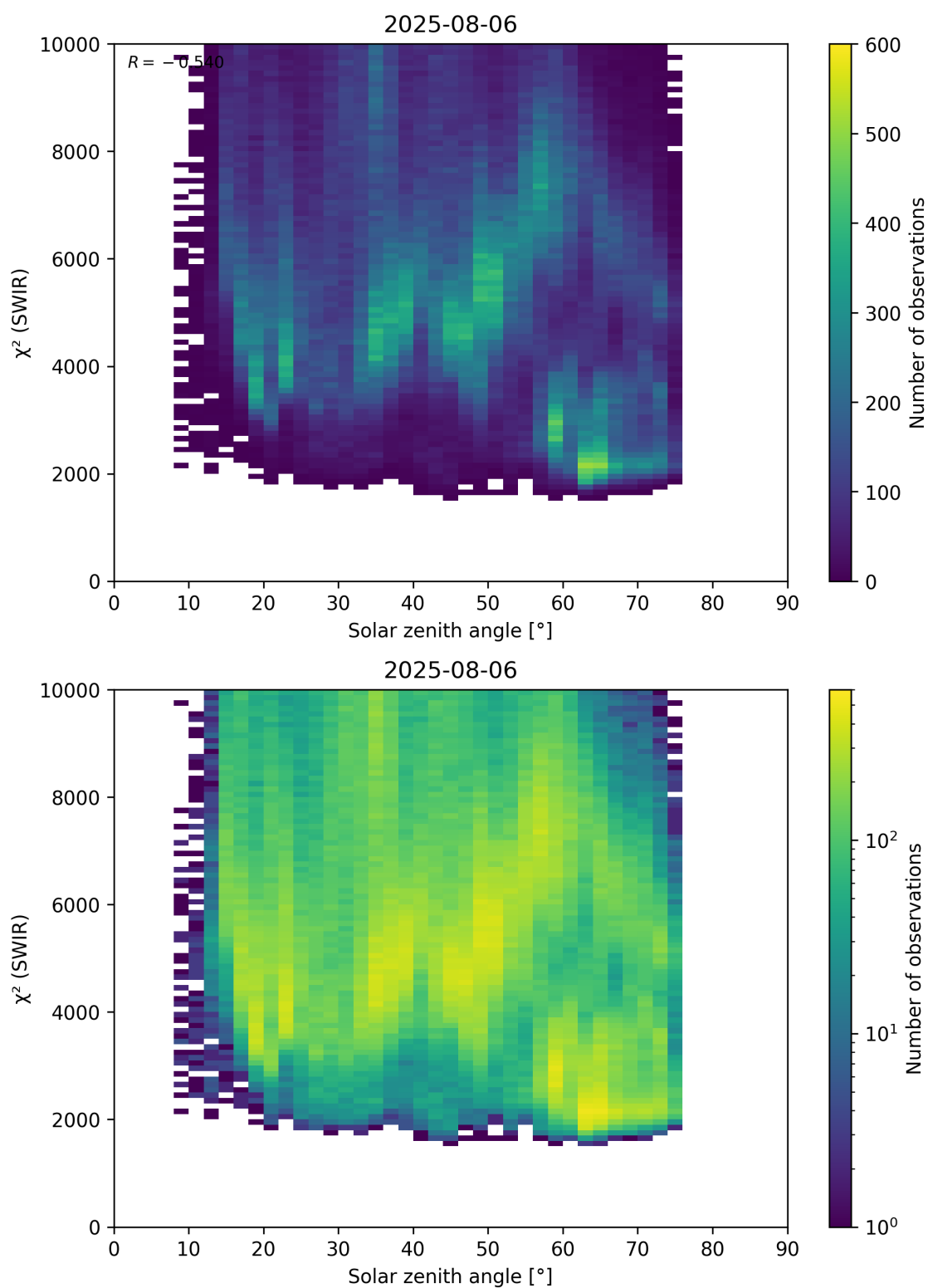
Figure 95: Scatter density plot of “Solar zenith angle” against “ \chi^2 (SWIR)” for 2025-08-05 to 2025-08-07.
