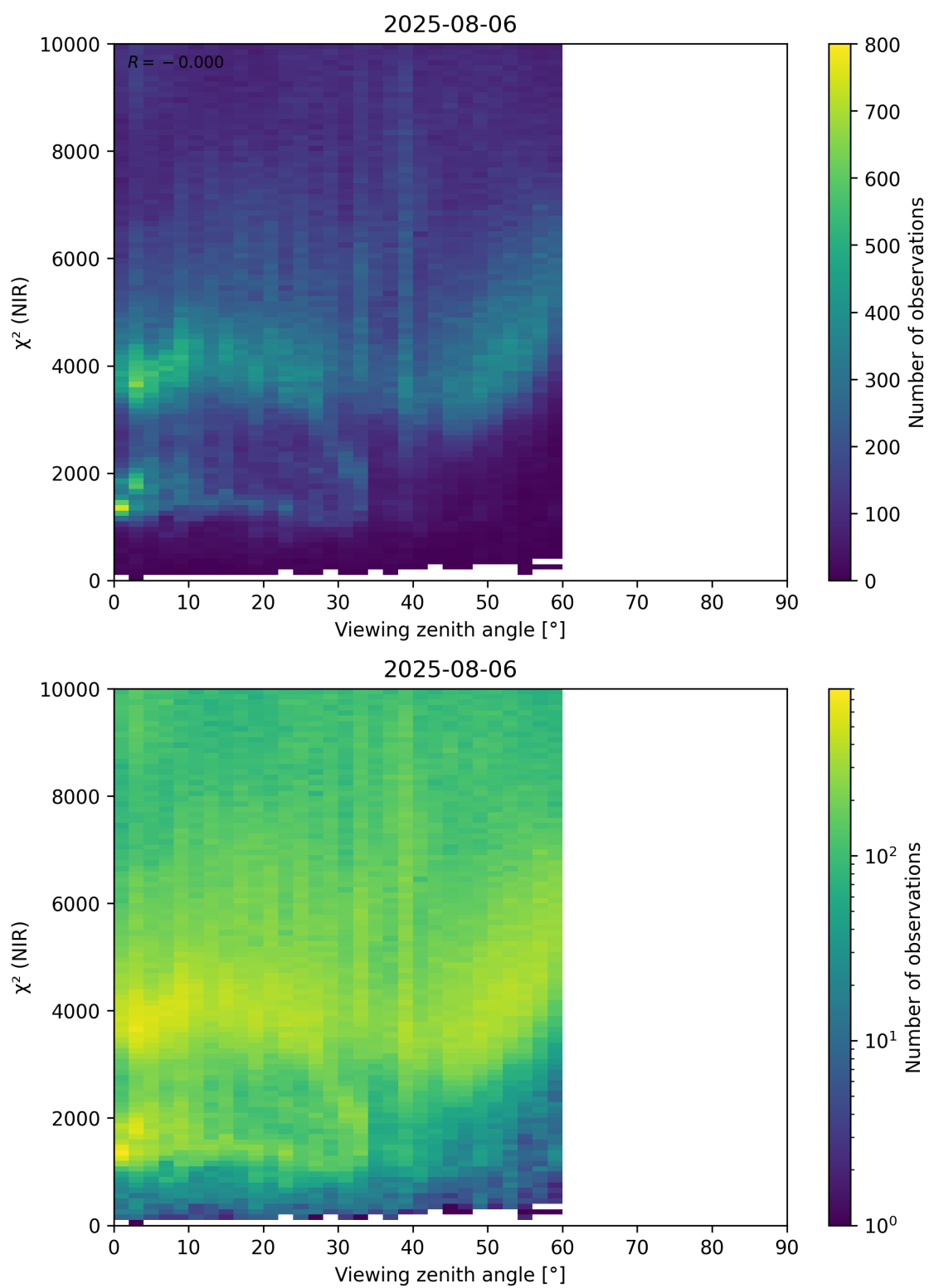
Figure 105: Scatter density plot of “Viewing zenith angle” against “ \chi^2 (NIR)” for 2025-08-05 to 2025-08-07.
