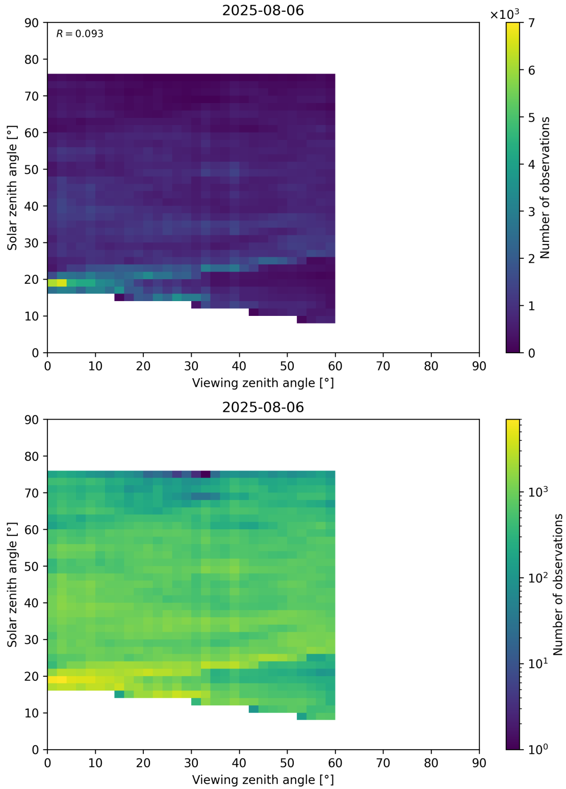
Figure 115: Scatter density plot of “Viewing zenith angle” against “Solar zenith angle” for 2025-08-05 to 2025-08-07.
