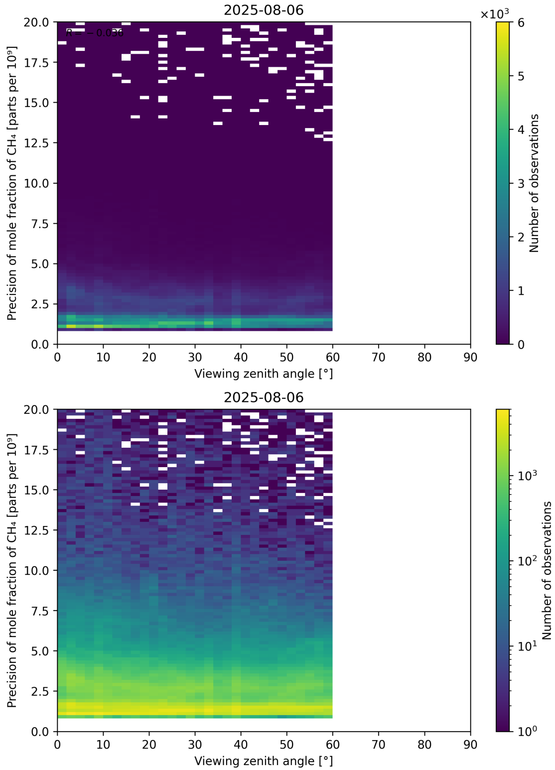
Figure 112: Scatter density plot of “Viewing zenith angle” against “Precision of mole fraction of CH 4 ” for 2025-08-05 to 2025-08-07.
