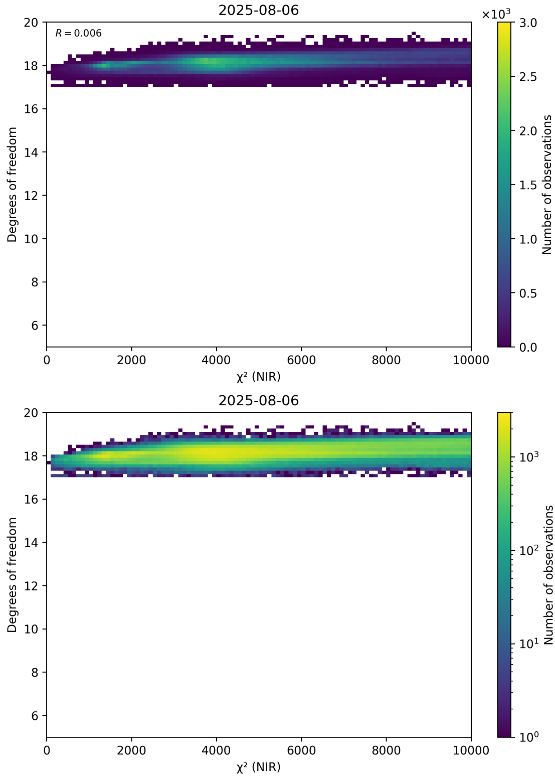
Figure 44: Scatter density plot of “ \chi^2 (NIR)” against “Degrees of freedom” for 2025-08-05 to 2025-08-07.
