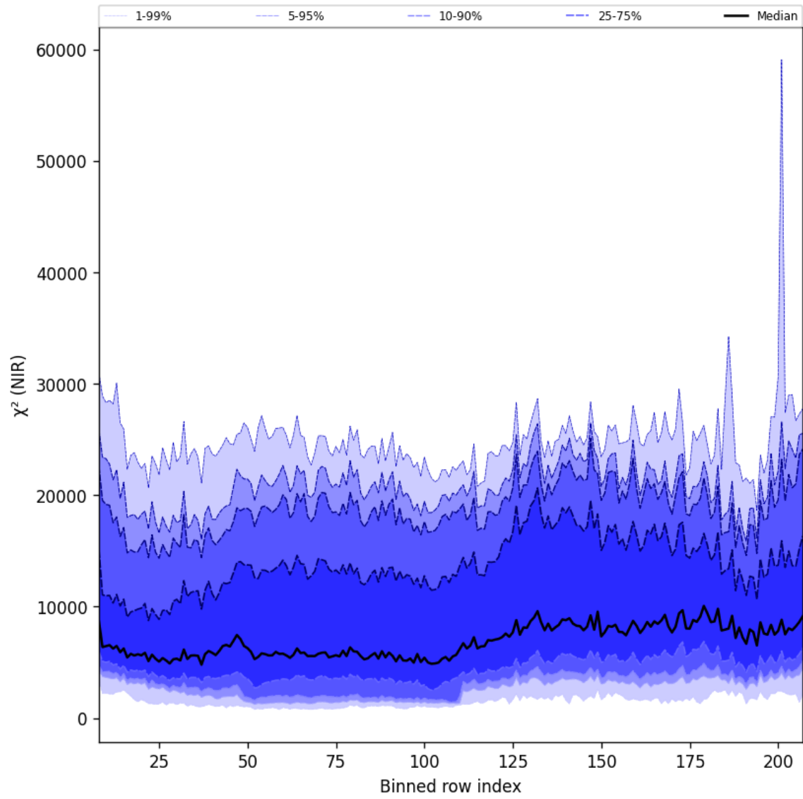
Figure 40: Along track statistics of “ \chi^2 (NIR)” for 2025-08-05 to 2025-08-07
