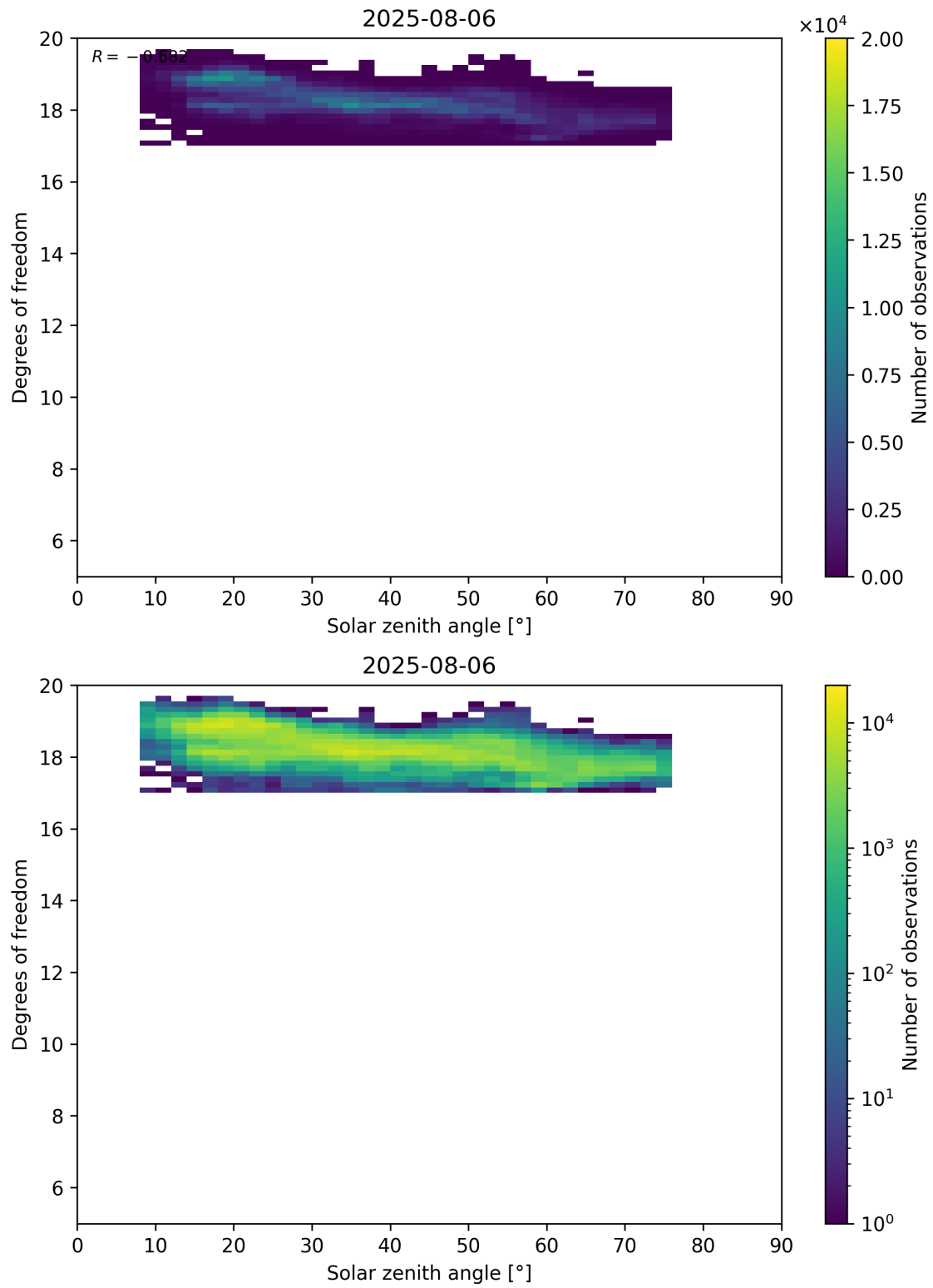
Figure 96: Scatter density plot of “Solar zenith angle” against “Degrees of freedom” for 2025-08-05 to 2025-08-07.
