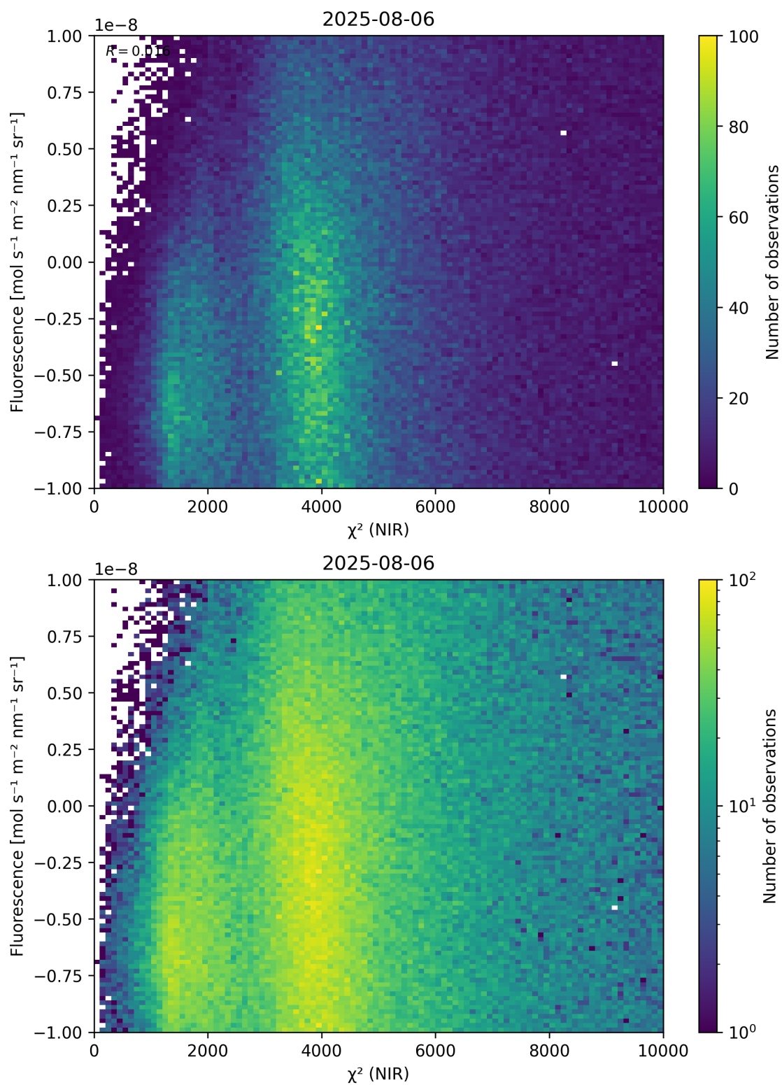
Figure 45: Scatter density plot of “ \chi^2 (NIR)” against “Fluorescence” for 2025-08-05 to 2025-08-07.
