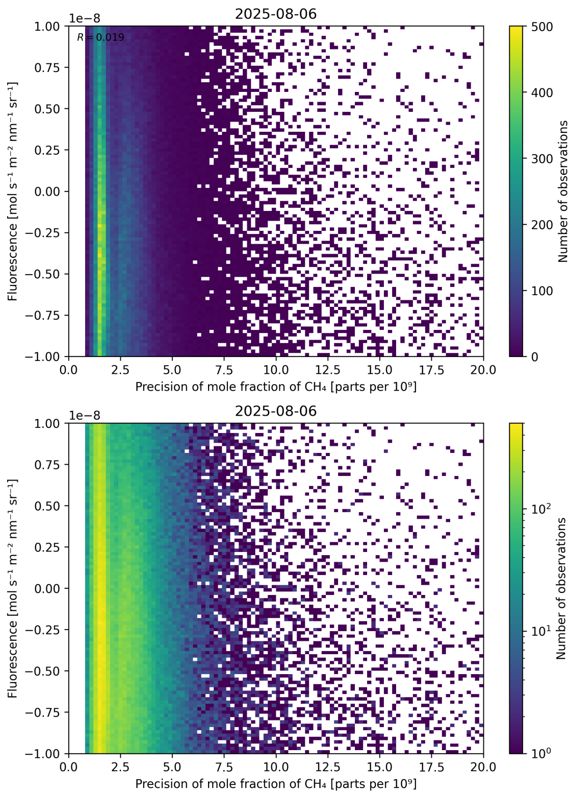
Figure 81: Scatter density plot of “Precision of mole fraction of \text{CH}_4 ” against “Fluorescence” for 2025-08-05 to 2025-08-07.
