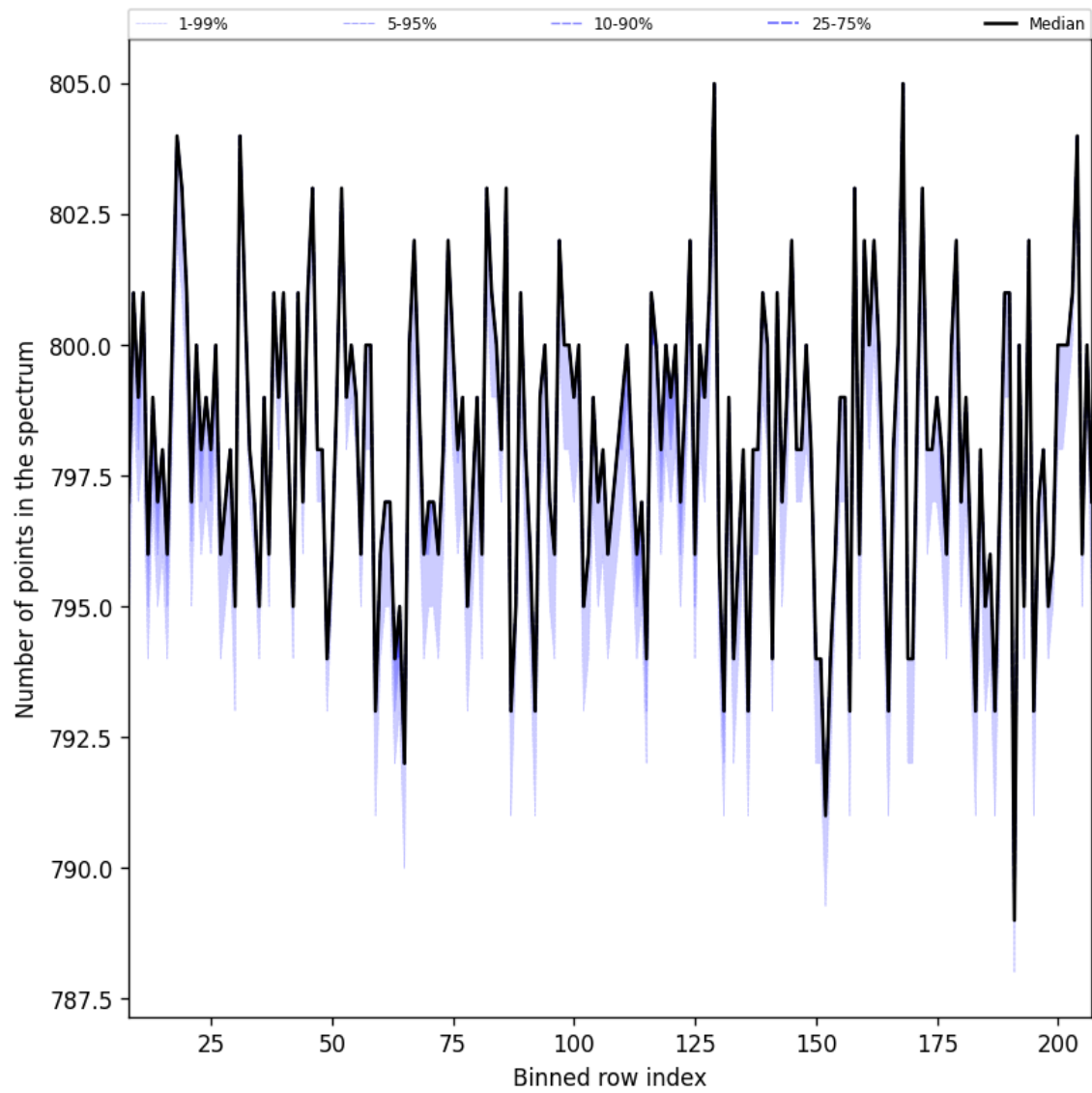
Figure 37: Along track statistics of “Number of points in the spectrum” for 2025-08-05 to 2025-08-07
