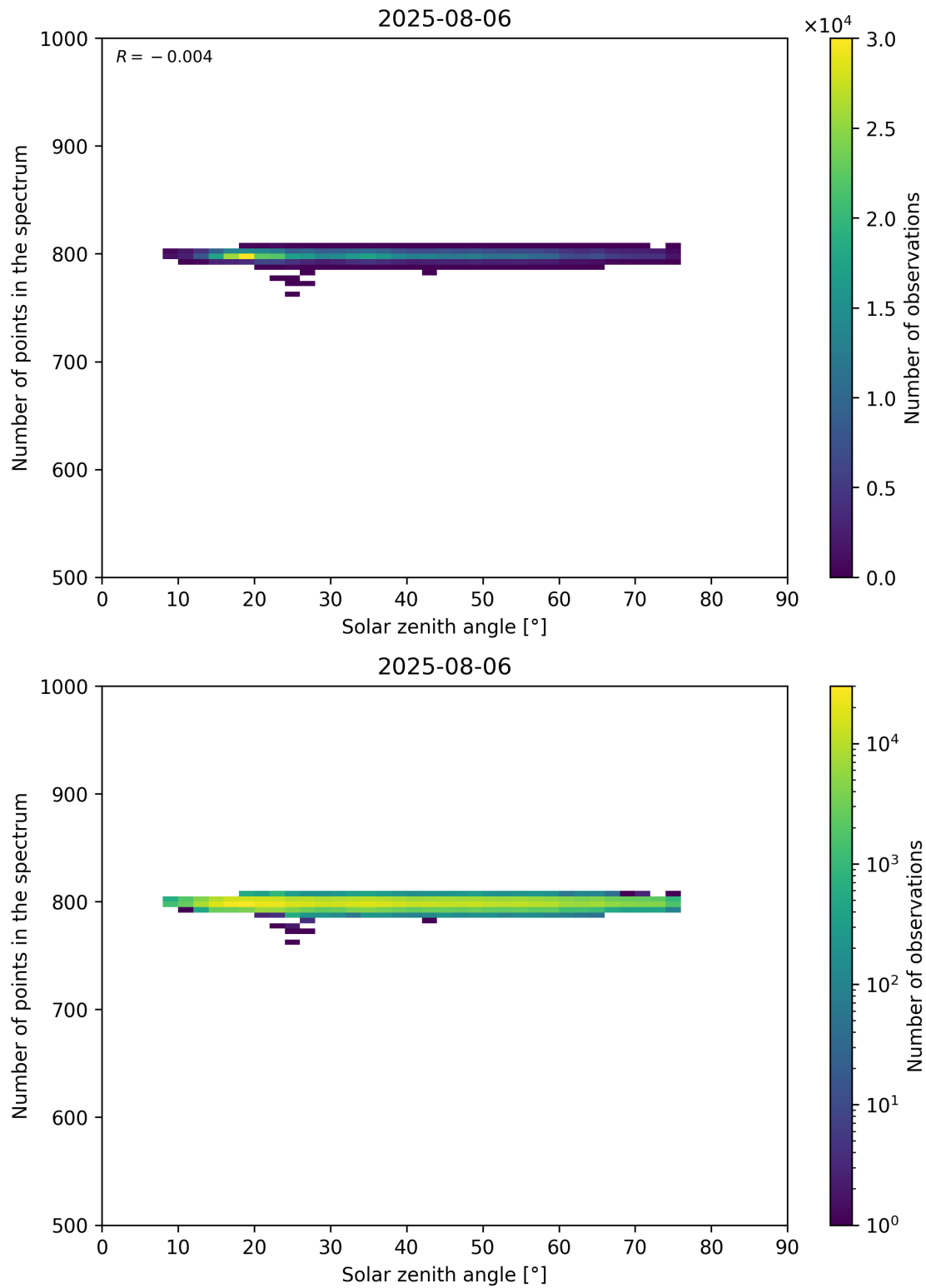
Figure 103: Scatter density plot of “Solar zenith angle” against “Number of points in the spectrum” for 2025-08-05 to 2025-08-07.
