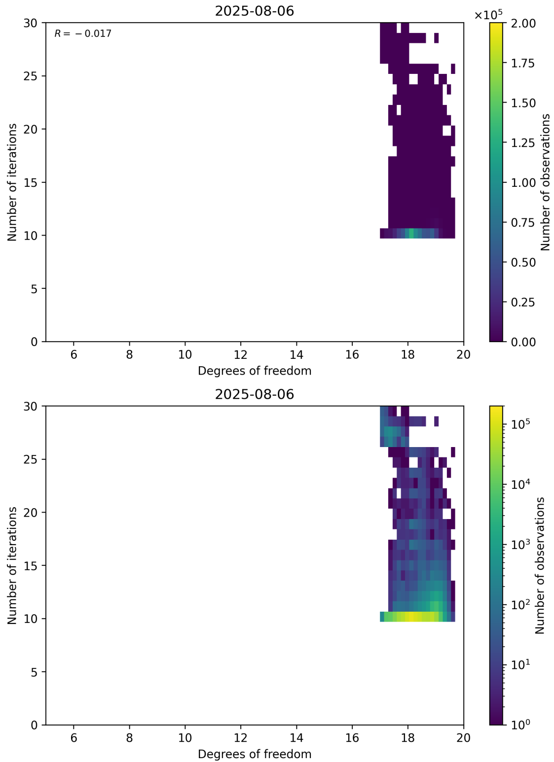
Figure 52: Scatter density plot of “Degrees of freedom” against “Number of iterations” for 2025-08-05 to 2025-08-07.
