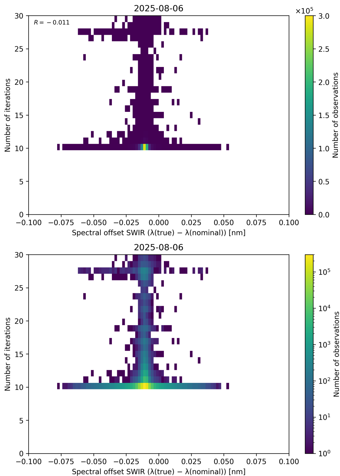
Figure 121: Scatter density plot of “Spectral offset SWIR ( \lambda_{\text{true}} - \lambda_{\text{nominal}} )” against “Number of iterations” for 2025-08-05 to 2025-08-07.
