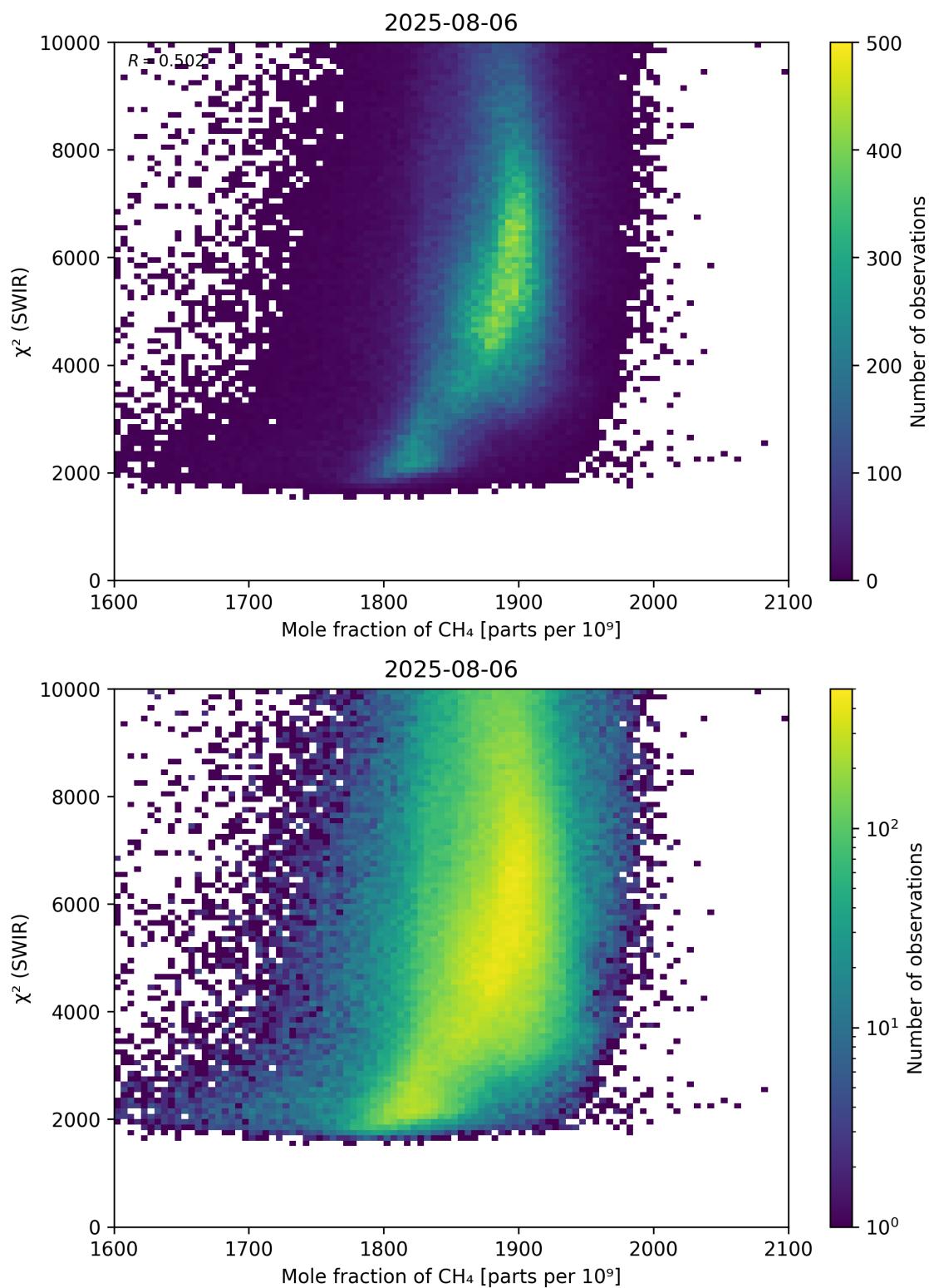
Figure 71: Scatter density plot of “Mole fraction of \text{CH}_4 ” against “ \chi^2 (SWIR)” for 2025-08-05 to 2025-08-07.
