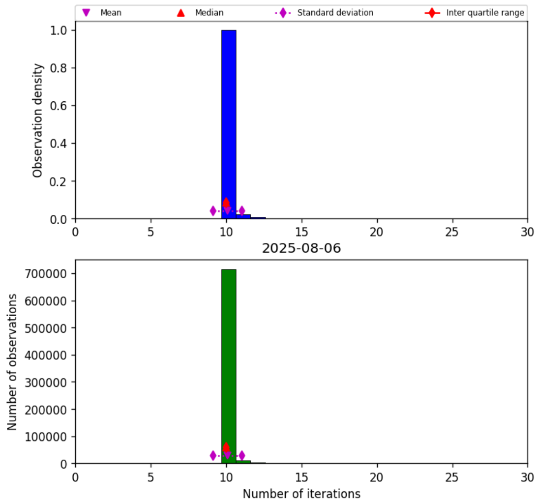
Figure 31: Histogram of “Number of iterations” for 2025-08-05 to 2025-08-07
