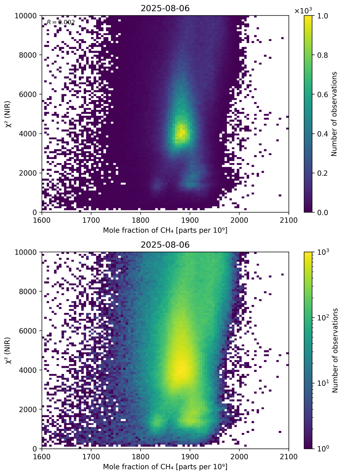
Figure 70: Scatter density plot of “Mole fraction of \text{CH}_4 ” against “ \chi^2 (NIR)” for 2025-08-05 to 2025-08-07.
