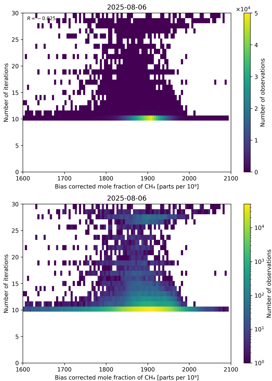
Figure 67: Scatter density plot of “Bias corrected mole fraction of CH 4 ” against “Number of iterations” for 2025-08-05 to 2025-08-07.
