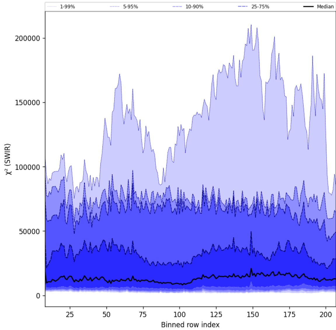
Figure 39: Along track statistics of " \chi^2 (SWIR)" for 2025-08-05 to 2025-08-07
