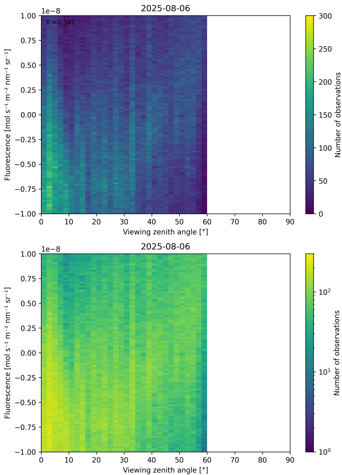
Figure 108: Scatter density plot of “Viewing zenith angle” against “Fluorescence” for 2025-08-05 to 2025-08-07.
