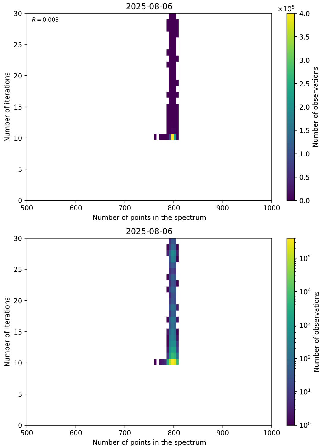
Figure 92: Scatter density plot of “Number of points in the spectrum” against “Number of iterations” for 2025-08-05 to 2025-08-07.
