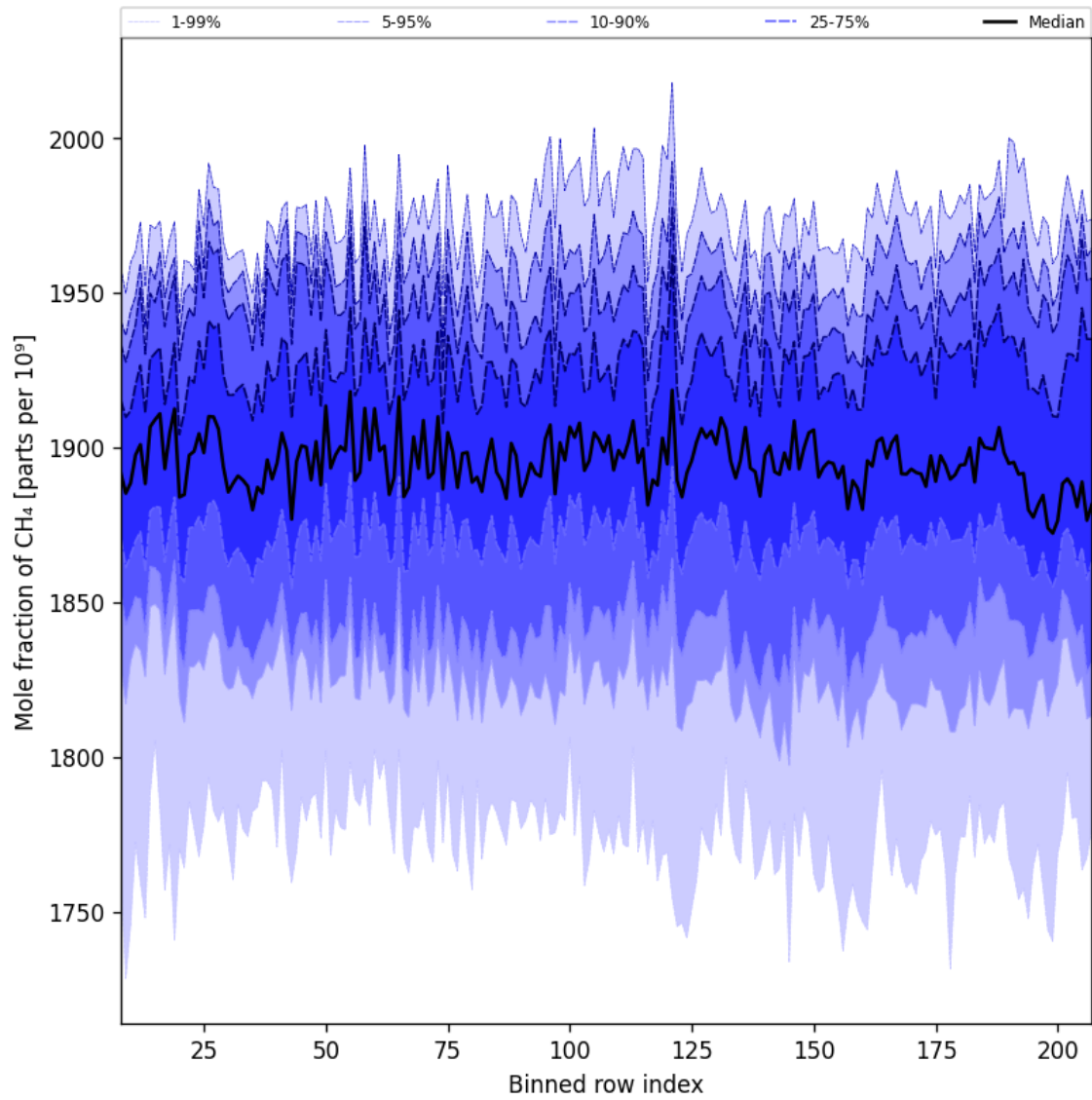
Figure 34: Along track statistics of “Mole fraction of CH 4 ” for 2025-08-05 to 2025-08-07
