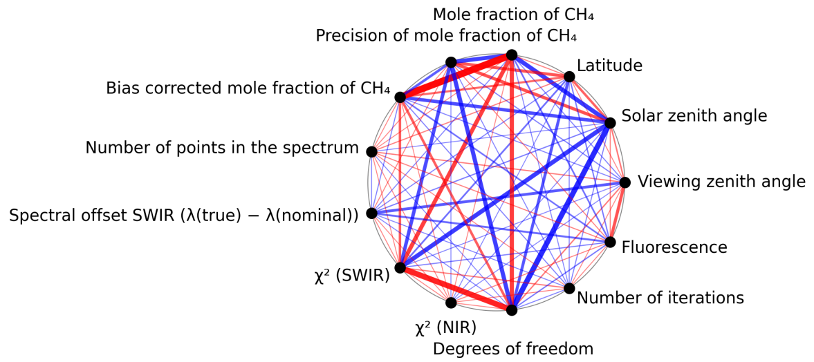
Figure 1: Map of correlation graph for 2025-08-05 to 2025-08-07.
