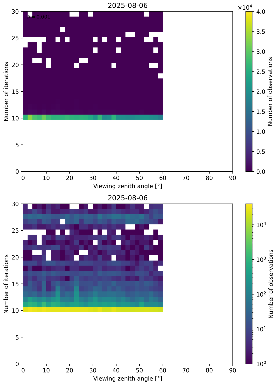
Figure 113: Scatter density plot of “Viewing zenith angle” against “Number of iterations” for 2025-08-05 to 2025-08-07.
