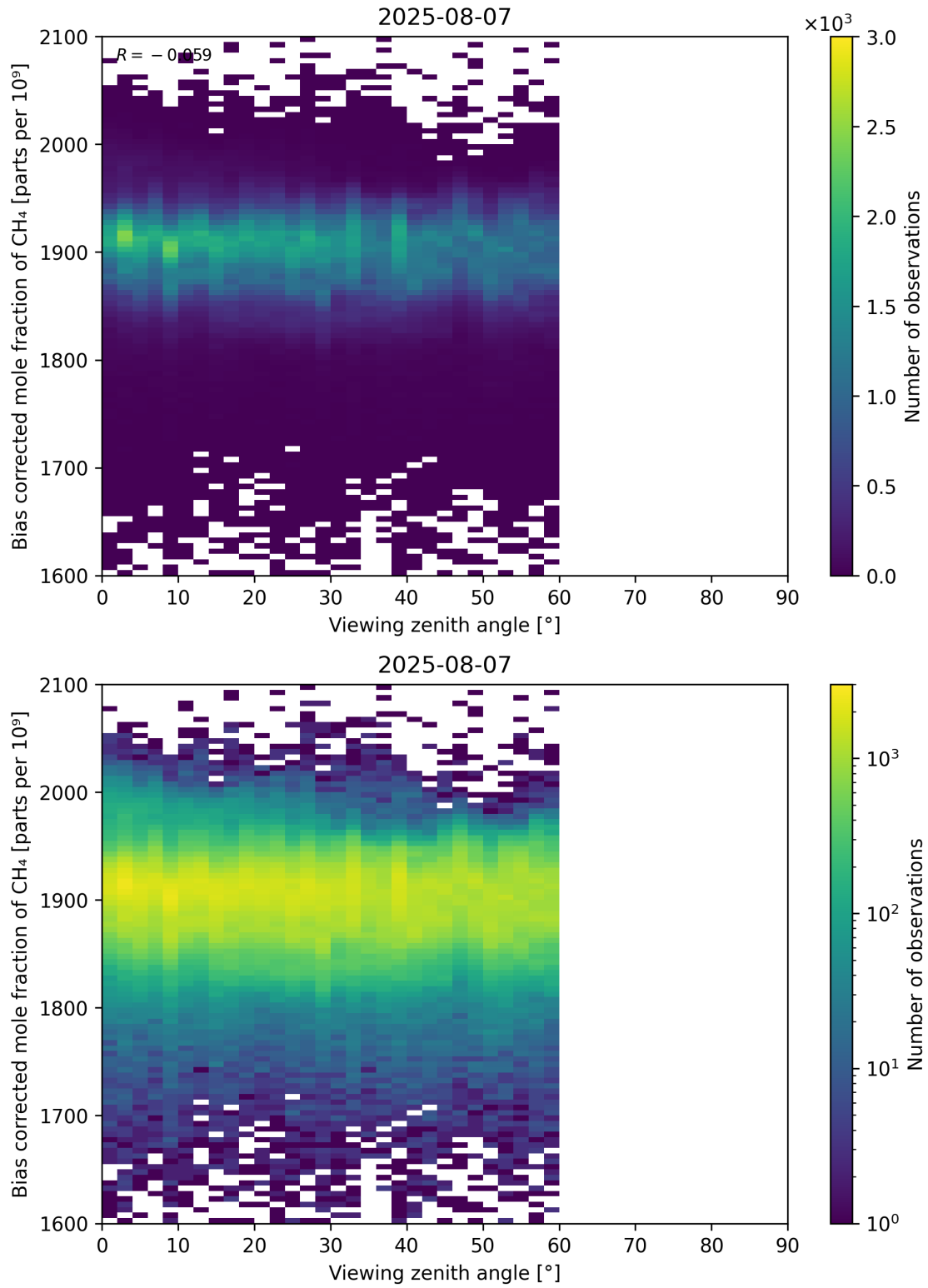
Figure 111: Scatter density plot of “Viewing zenith angle” against “Bias corrected mole fraction of CH 4 ” for 2025-08-06 to 2025-08-08.
