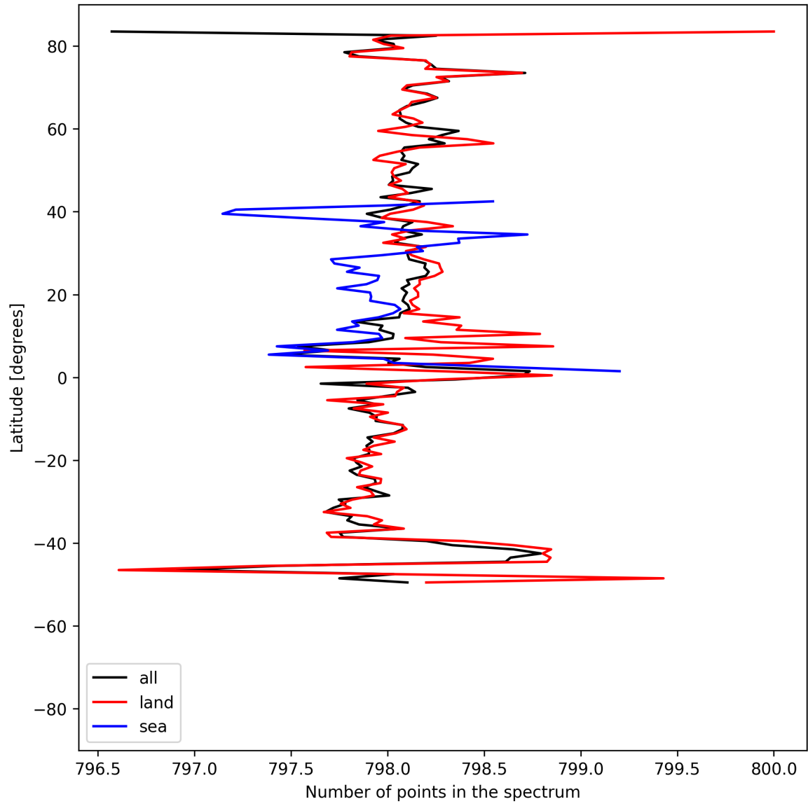
Figure 15: Zonal average of “Number of points in the spectrum” for 2025-08-06 to 2025-08-08.
