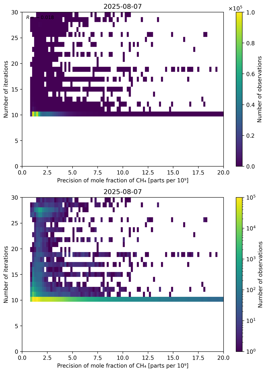
Figure 83: Scatter density plot of “Precision of mole fraction of CH 4 ” against “Number of iterations” for 2025-08-06 to 2025-08-08.
