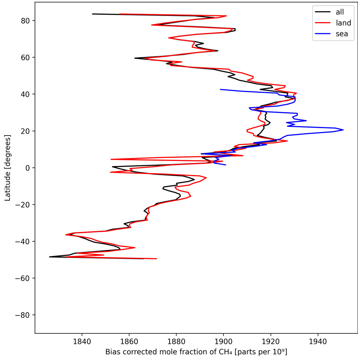
Figure 14: Zonal average of “Bias corrected mole fraction of CH 4 ” for 2025-08-06 to 2025-08-08.
