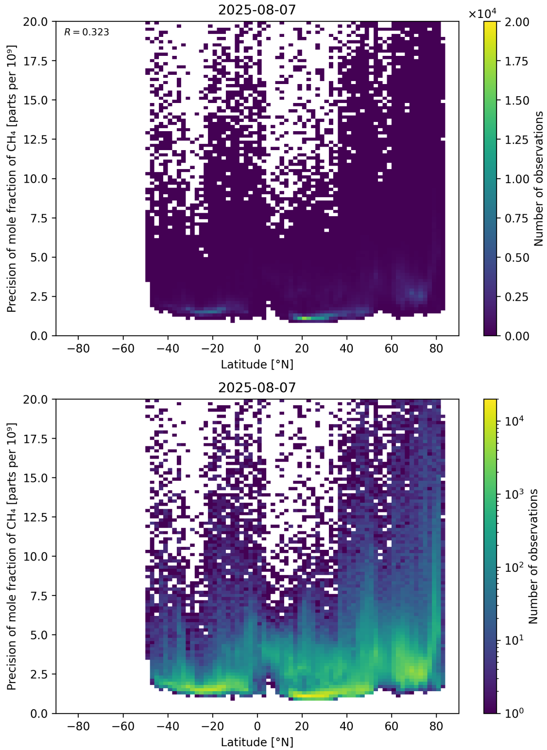
Figure 59: Scatter density plot of “Latitude” against “Precision of mole fraction of \text{CH}_4 ” for 2025-08-06 to 2025-08-08.
