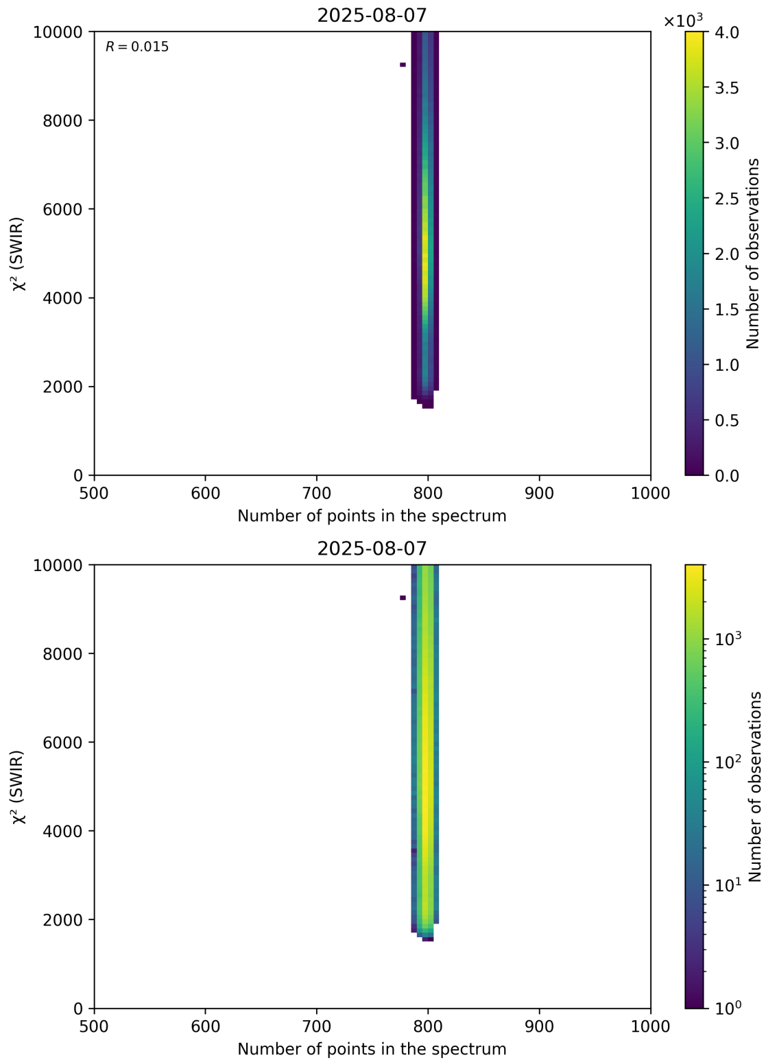
Figure 89: Scatter density plot of “Number of points in the spectrum” against “ \chi^2 (SWIR)” for 2025-08-06 to 2025-08-08.
