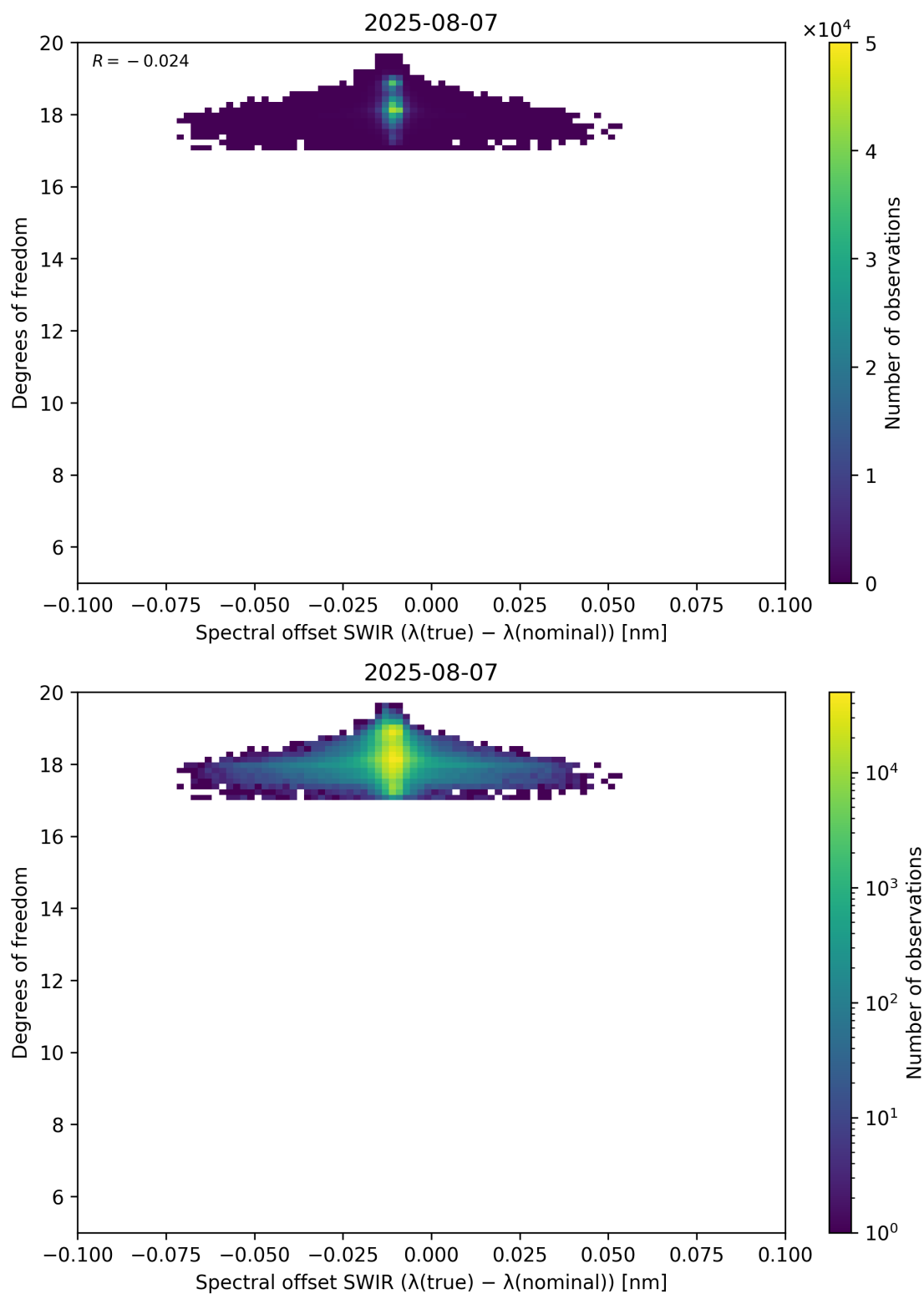
Figure 119: Scatter density plot of “Spectral offset SWIR ( \lambda_{\text{true}} - \lambda_{\text{nominal}} )” against “Degrees of freedom” for 2025-08-06 to 2025-08-08.
