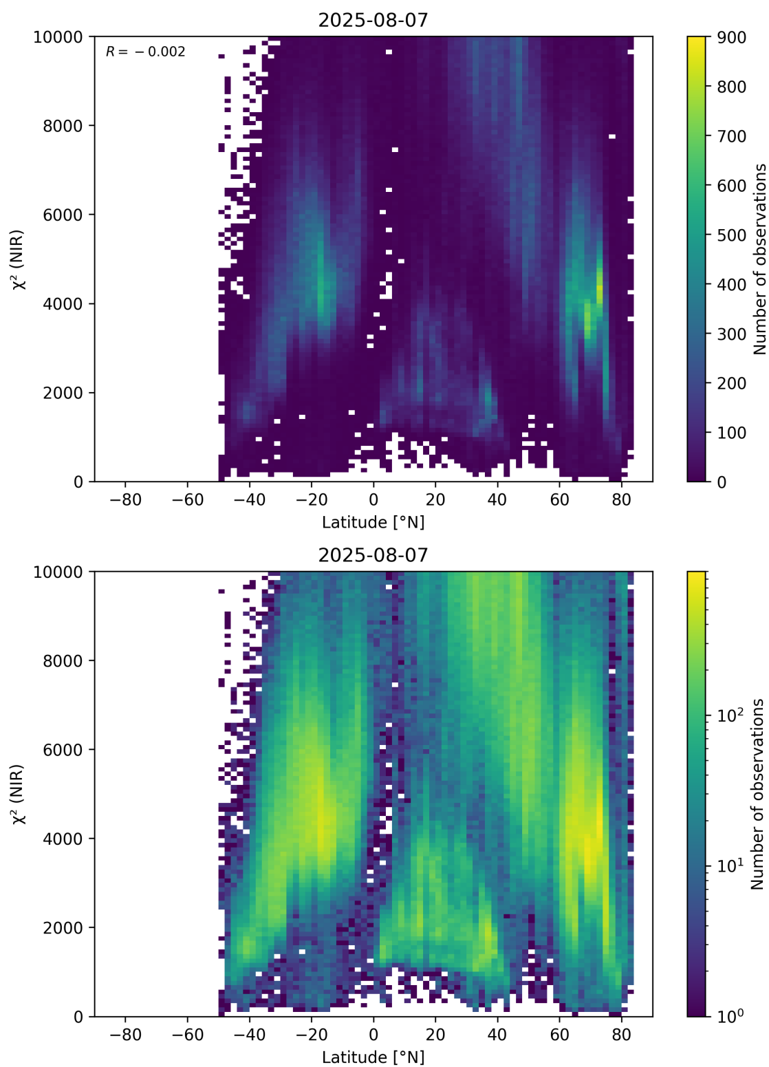
Figure 53: Scatter density plot of “Latitude” against “ \chi^2 (NIR)” for 2025-08-06 to 2025-08-08.
