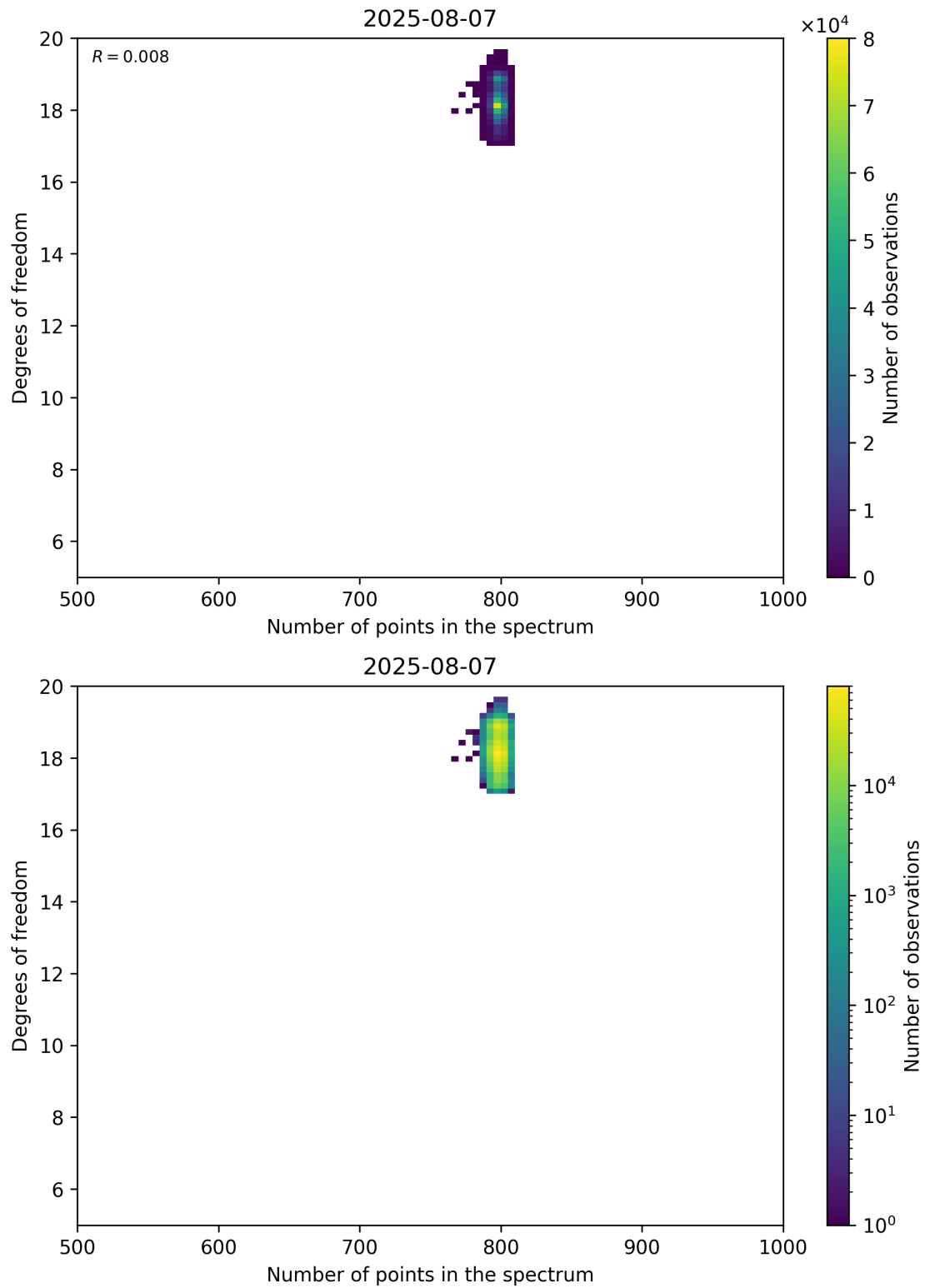
Figure 90: Scatter density plot of “Number of points in the spectrum” against “Degrees of freedom” for 2025-08-06 to 2025-08-08.
