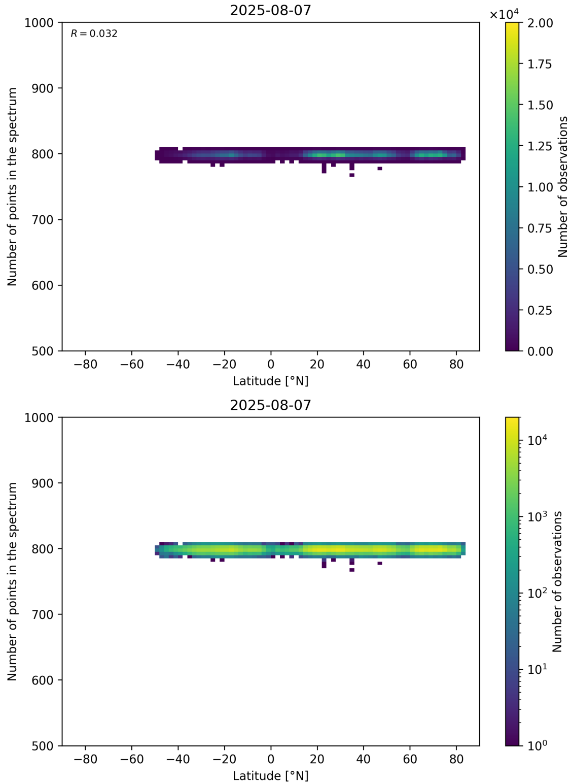
Figure 61: Scatter density plot of “Latitude” against “Number of points in the spectrum” for 2025-08-06 to 2025-08-08.
