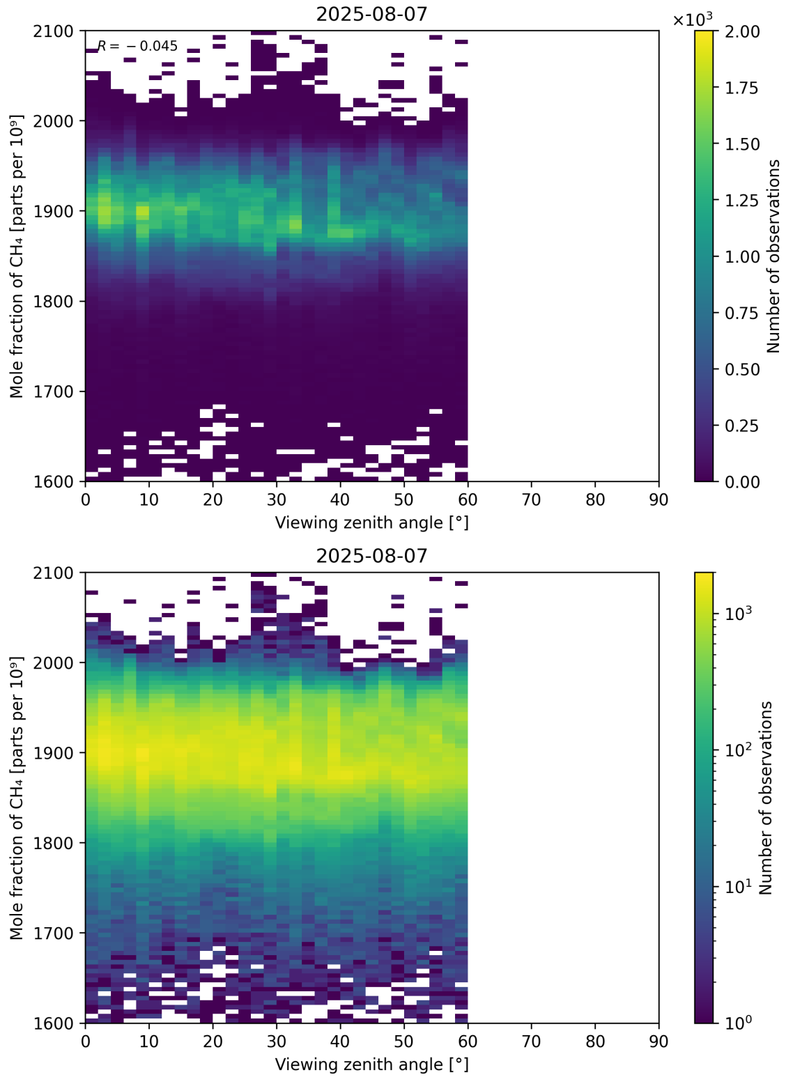
Figure 110: Scatter density plot of “Viewing zenith angle” against “Mole fraction of CH 4 ” for 2025-08-06 to 2025-08-08.
