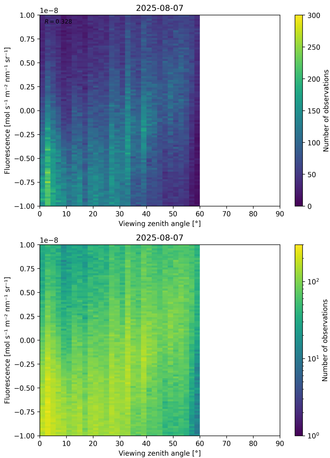
Figure 108: Scatter density plot of “Viewing zenith angle” against “Fluorescence” for 2025-08-06 to 2025-08-08.
