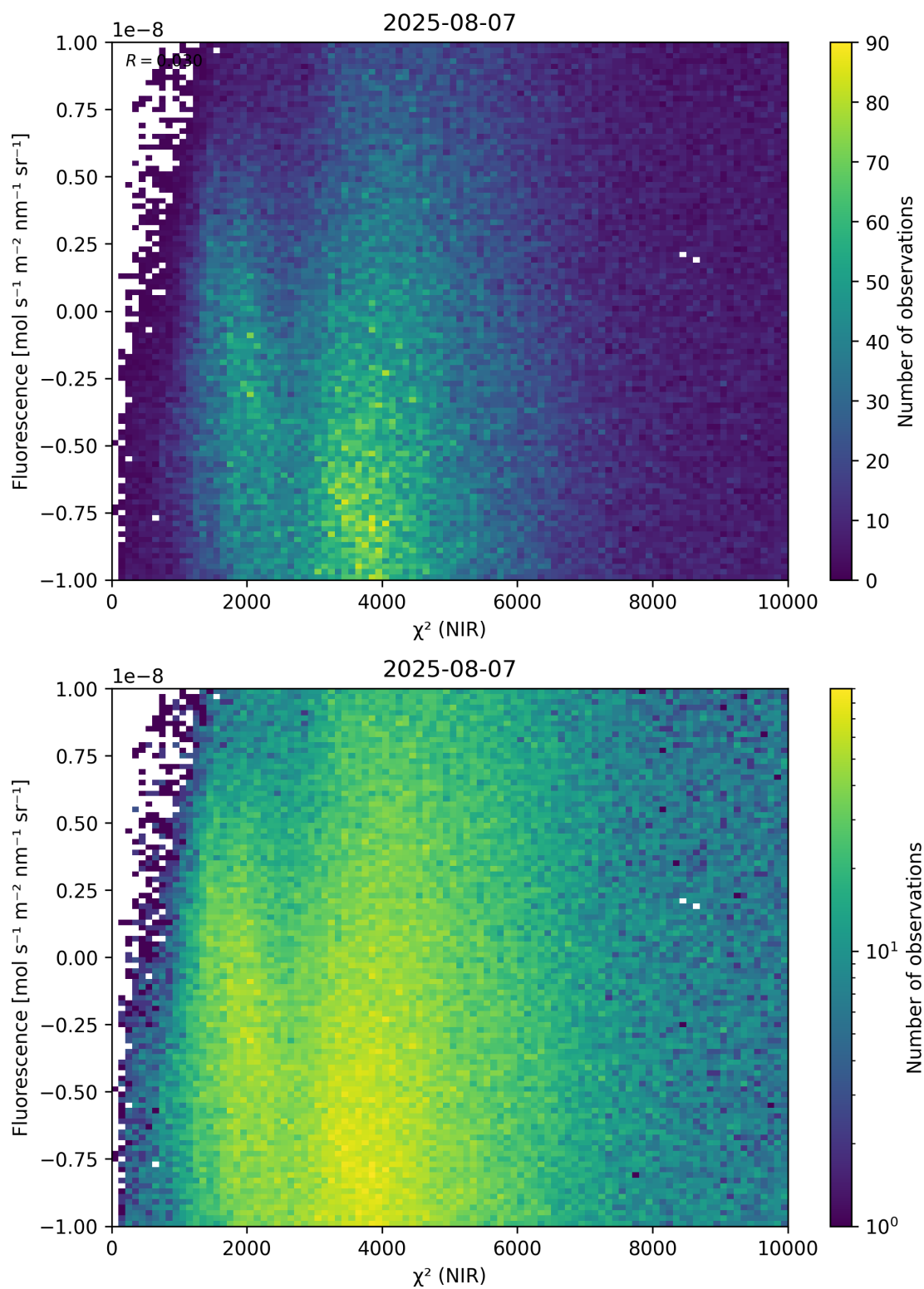
Figure 45: Scatter density plot of “ \chi^2 (NIR)” against “Fluorescence” for 2025-08-06 to 2025-08-08.
