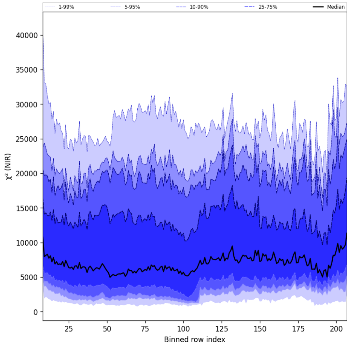
Figure 40: Along track statistics of " \chi^2 (NIR)" for 2025-08-06 to 2025-08-08
