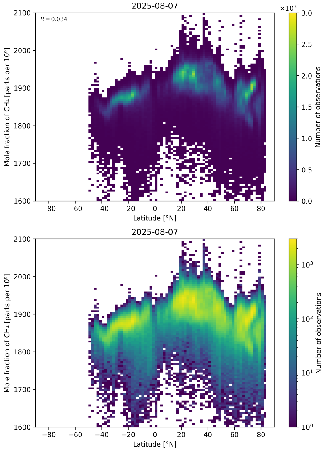
Figure 57: Scatter density plot of “Latitude” against “Mole fraction of \text{CH}_4 ” for 2025-08-06 to 2025-08-08.
