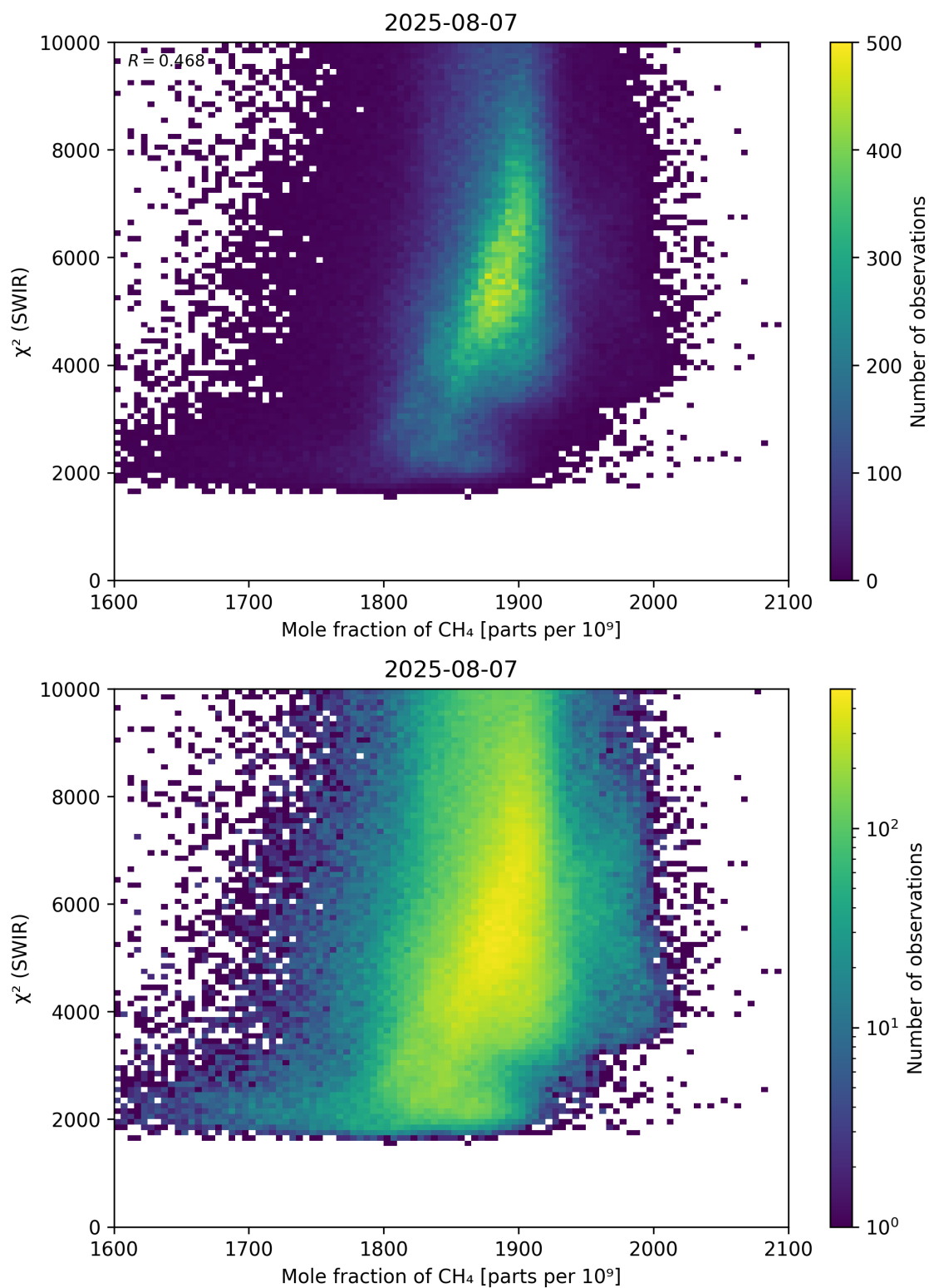
Figure 71: Scatter density plot of “Mole fraction of \text{CH}_4 ” against “ \chi^2 (SWIR)” for 2025-08-06 to 2025-08-08.
