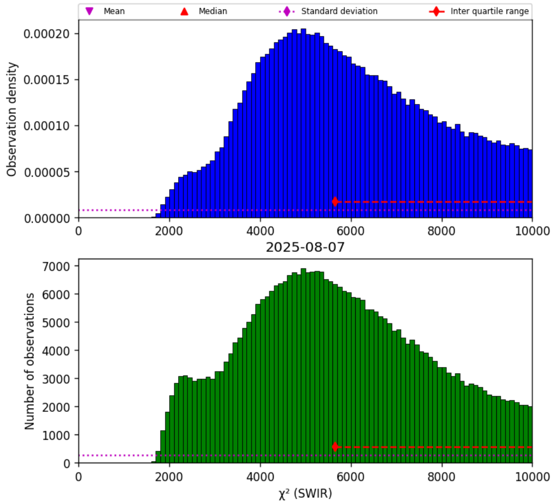
Figure 28: Histogram of “ \chi^2 (SWIR)” for 2025-08-06 to 2025-08-08
