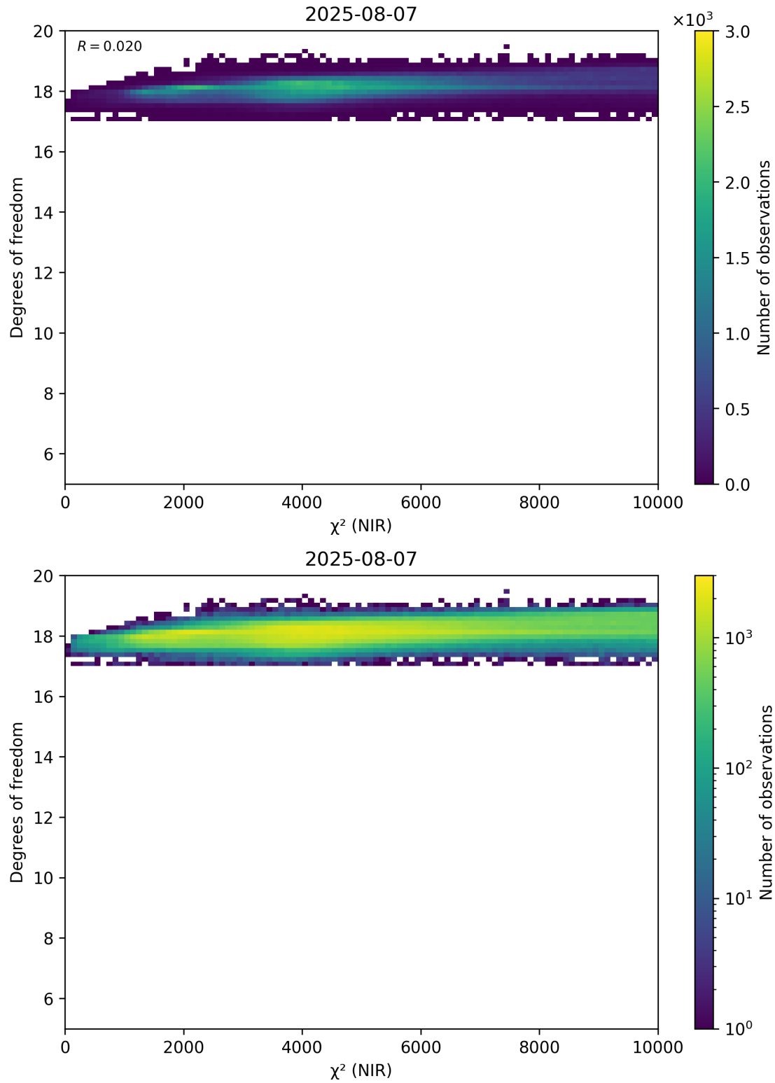
Figure 44: Scatter density plot of “ \chi^2 (NIR)” against “Degrees of freedom” for 2025-08-06 to 2025-08-08.
