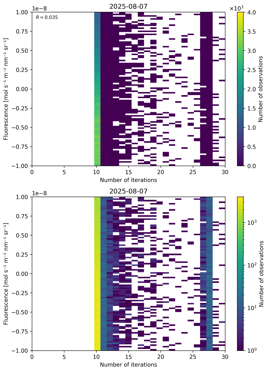
Figure 87: Scatter density plot of “Number of iterations” against “Fluorescence” for 2025-08-06 to 2025-08-08.
