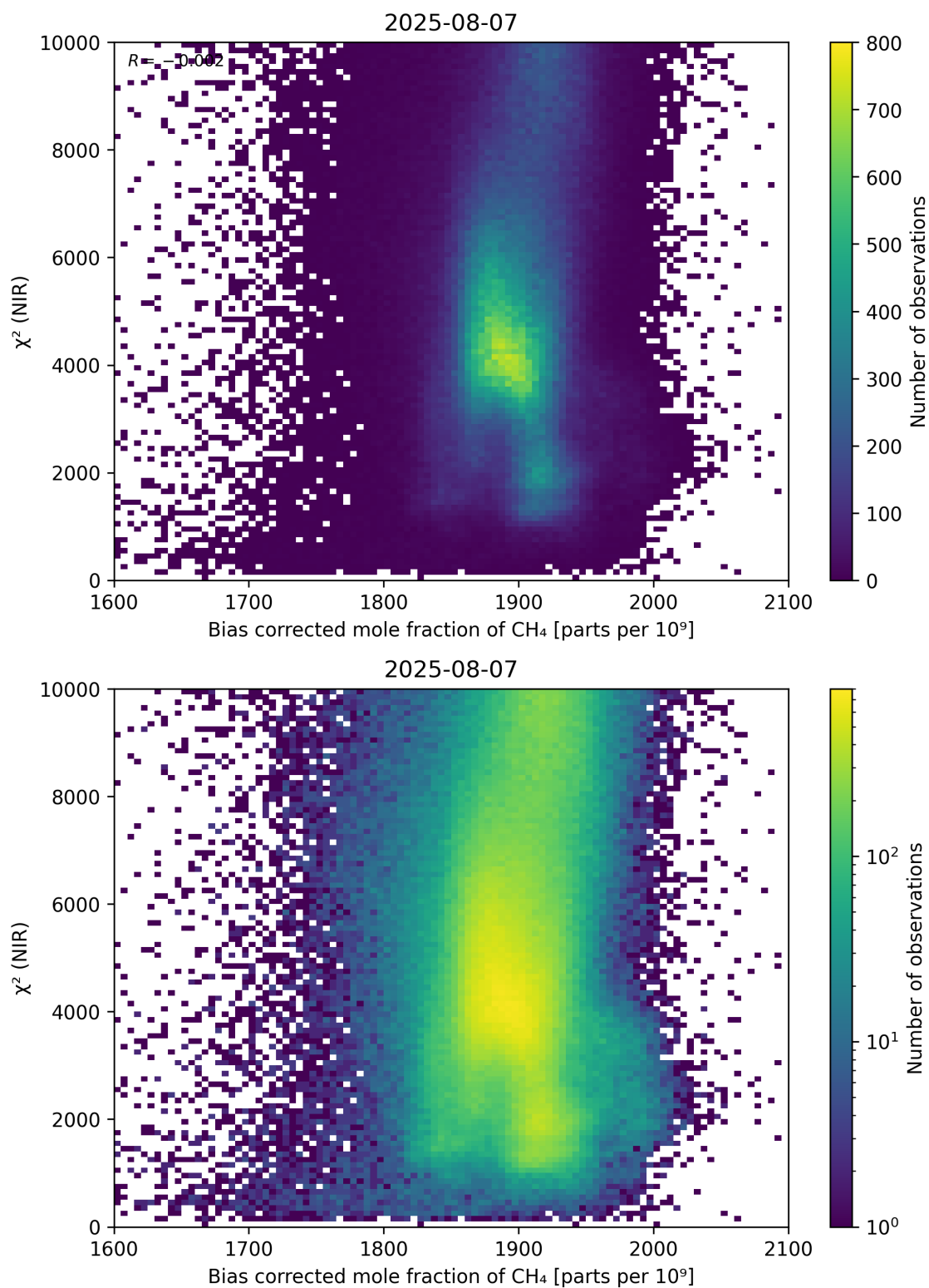
Figure 63: Scatter density plot of “Bias corrected mole fraction of \text{CH}_4 ” against “ \chi^2 (NIR)” for 2025-08-06 to 2025-08-08.
