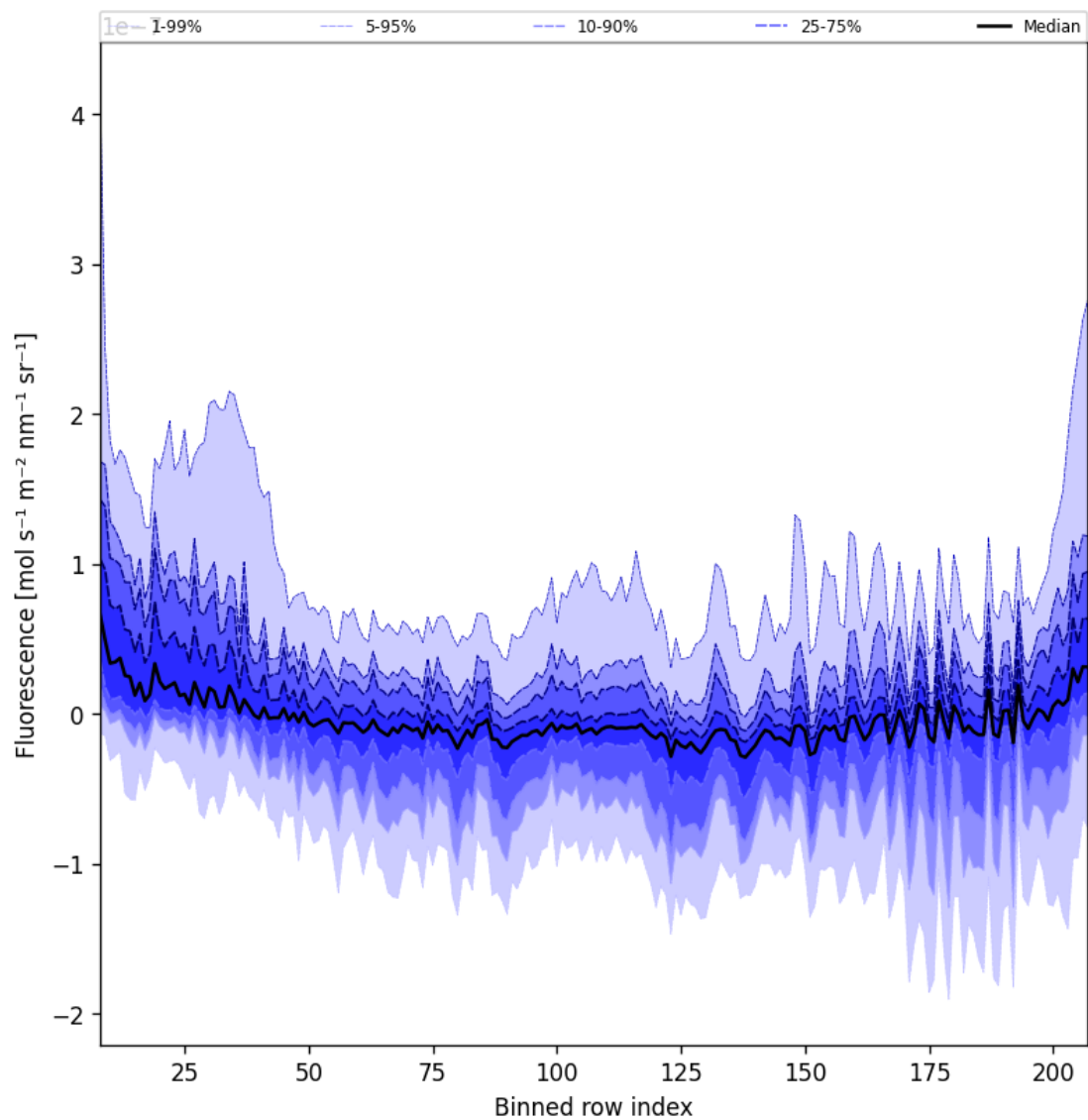
Figure 43: Along track statistics of “Fluorescence” for 2025-08-06 to 2025-08-08
