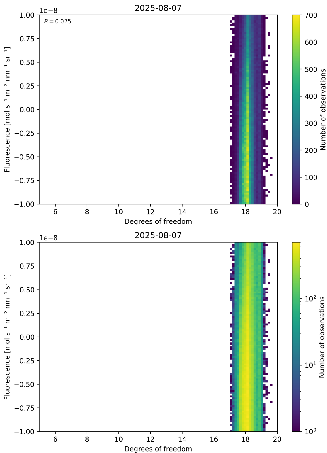
Figure 51: Scatter density plot of “Degrees of freedom” against “Fluorescence” for 2025-08-06 to 2025-08-08.
