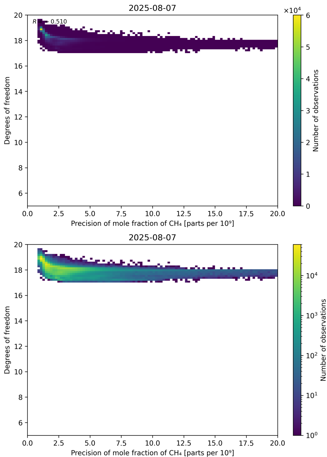
Figure 80: Scatter density plot of “Precision of mole fraction of CH 4 ” against “Degrees of freedom” for 2025-08-06 to 2025-08-08.
