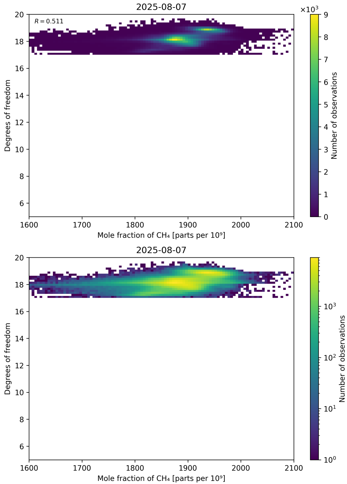
Figure 72: Scatter density plot of “Mole fraction of CH 4 ” against “Degrees of freedom” for 2025-08-06 to 2025-08-08.
