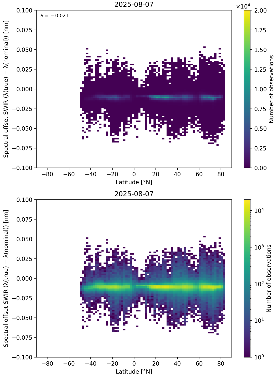
Figure 62: Scatter density plot of “Latitude” against “Spectral offset SWIR ( \lambda_{\text{true}} - \lambda_{\text{nominal}} )” for 2025-08-06 to 2025-08-08.
