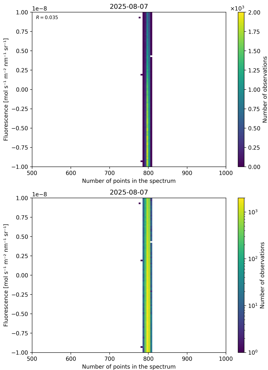
Figure 91: Scatter density plot of “Number of points in the spectrum” against “Fluorescence” for 2025-08-06 to 2025-08-08.
