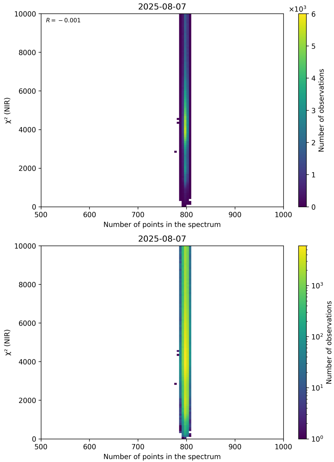
Figure 88: Scatter density plot of “Number of points in the spectrum” against “ \chi^2 (NIR)” for 2025-08-06 to 2025-08-08.
