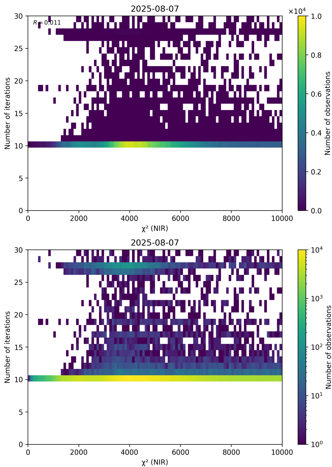
Figure 46: Scatter density plot of “ \chi^2 (NIR)” against “Number of iterations” for 2025-08-06 to 2025-08-08.
