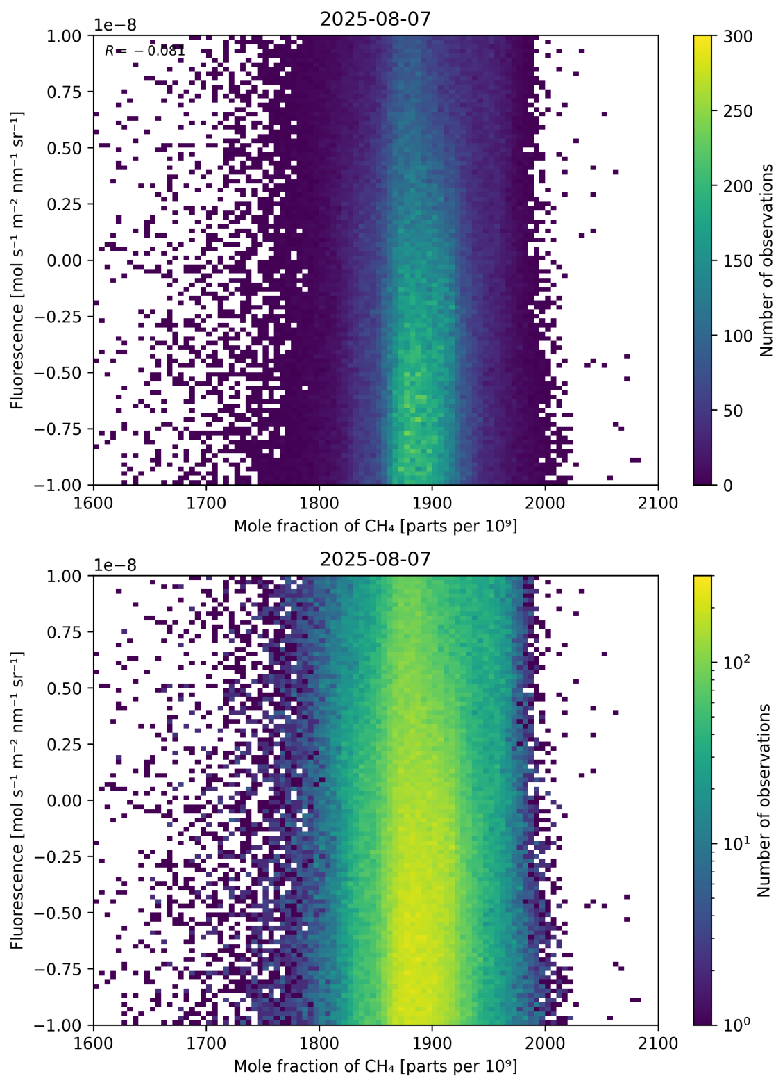
Figure 73: Scatter density plot of “Mole fraction of \text{CH}_4 ” against “Fluorescence” for 2025-08-06 to 2025-08-08.
