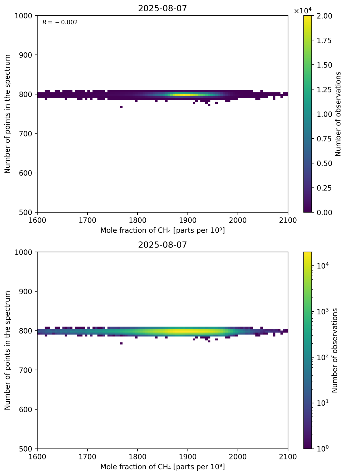
Figure 77: Scatter density plot of “Mole fraction of CH 4 ” against “Number of points in the spectrum” for 2025-08-06 to 2025-08-08.
