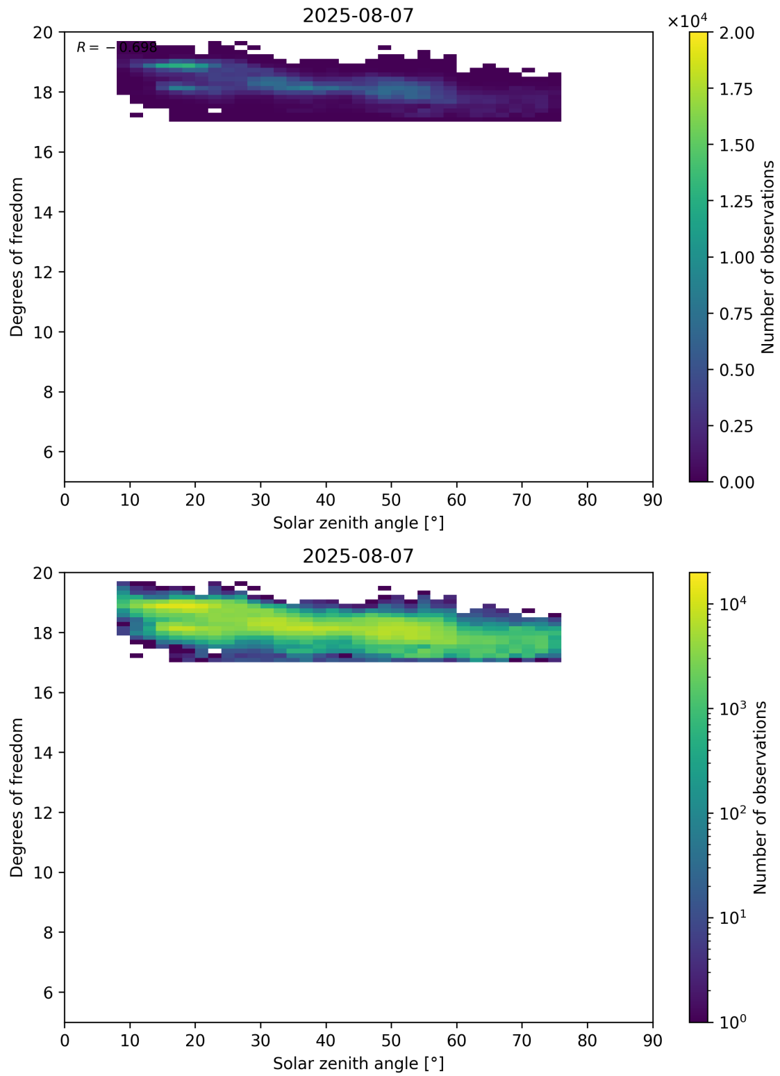
Figure 96: Scatter density plot of “Solar zenith angle” against “Degrees of freedom” for 2025-08-06 to 2025-08-08.
