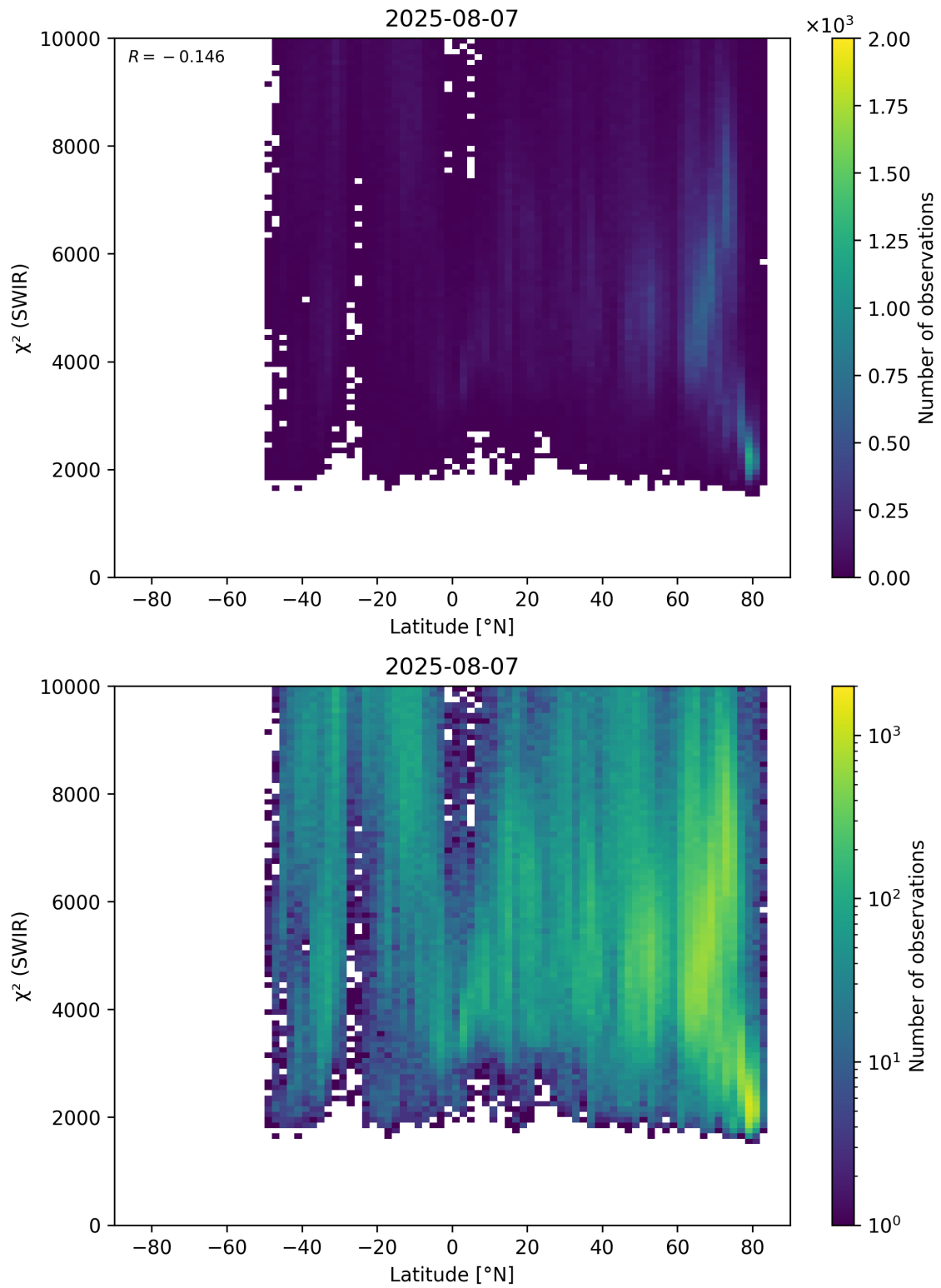
Figure 54: Scatter density plot of “Latitude” against “ \chi^2 (SWIR)” for 2025-08-06 to 2025-08-08.
