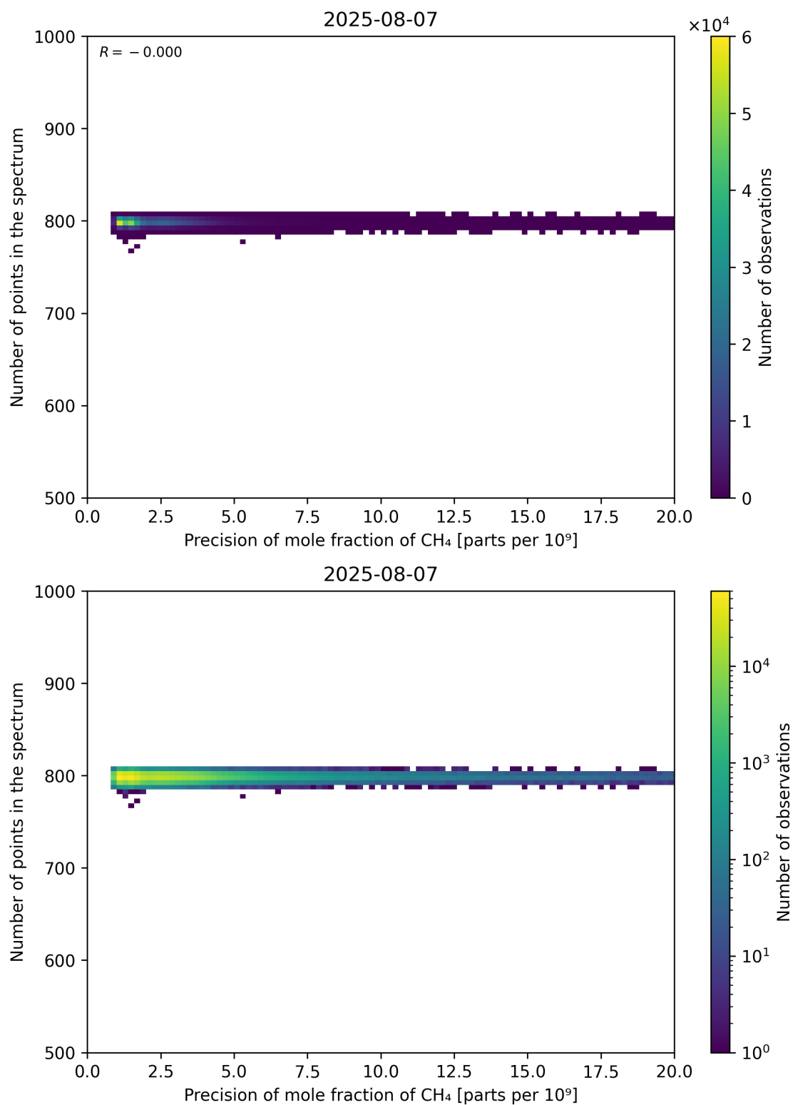
Figure 84: Scatter density plot of “Precision of mole fraction of CH 4 ” against “Number of points in the spectrum” for 2025-08-06 to 2025-08-08.
