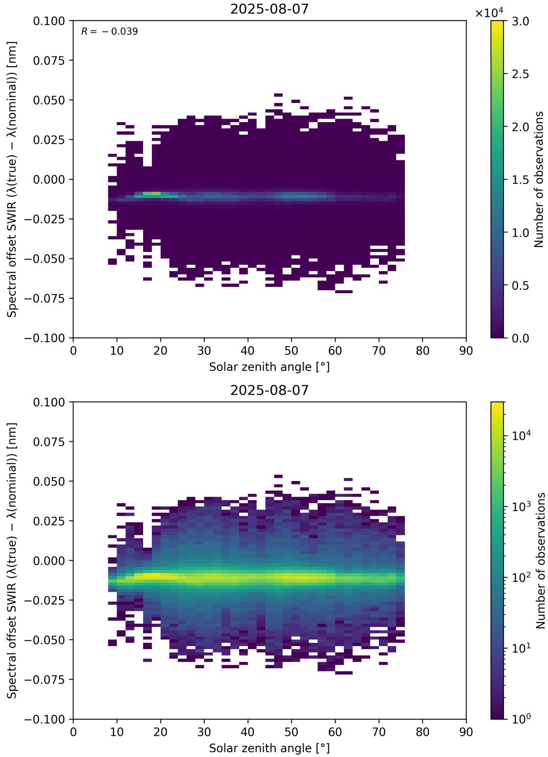
Figure 104: Scatter density plot of “Solar zenith angle” against “Spectral offset SWIR ( \lambda_{\text{true}} - \lambda_{\text{nominal}} )” for 2025-08-06 to 2025-08-08.
