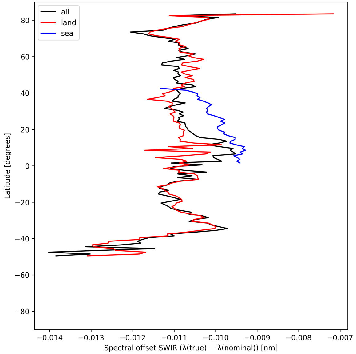
Figure 16: Zonal average of “Spectral offset SWIR ( \lambda_{\text{true}} - \lambda_{\text{nominal}} )” for 2025-08-06 to 2025-08-08.
