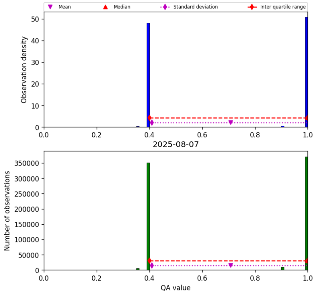
Figure 22: Histogram of “QA value” for 2025-08-06 to 2025-08-08
