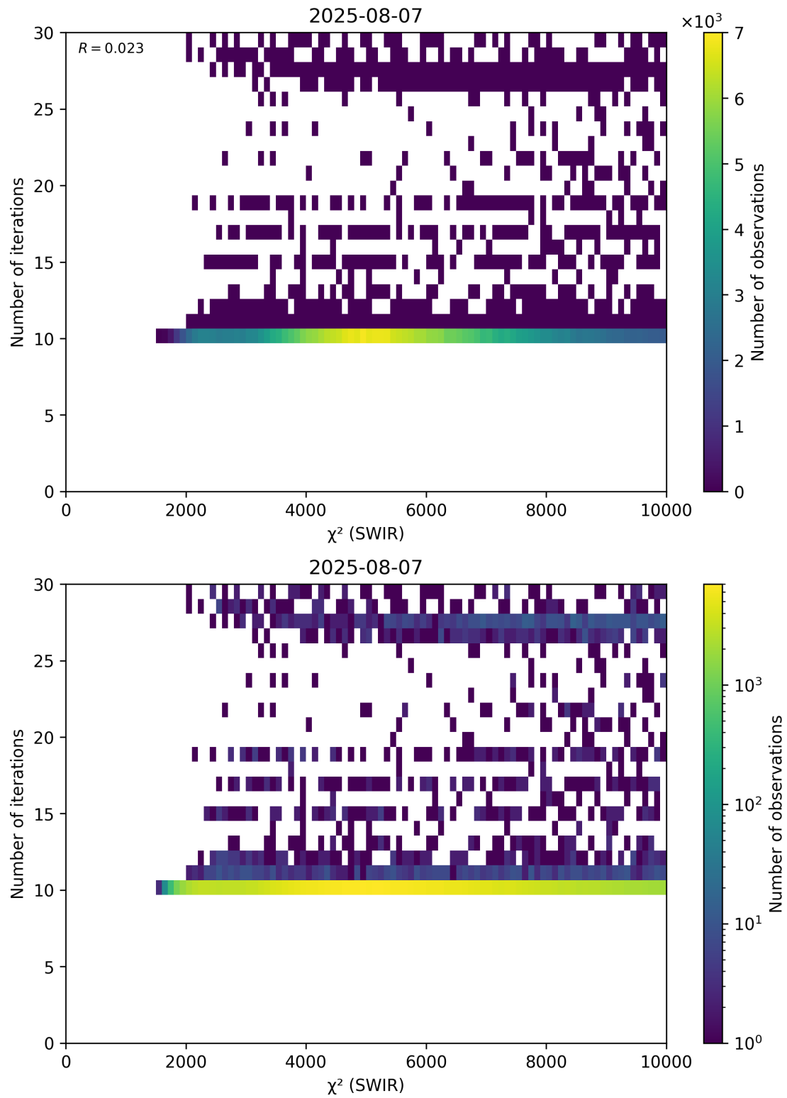
Figure 50: Scatter density plot of “ \chi^2 (SWIR)” against “Number of iterations” for 2025-08-06 to 2025-08-08.
