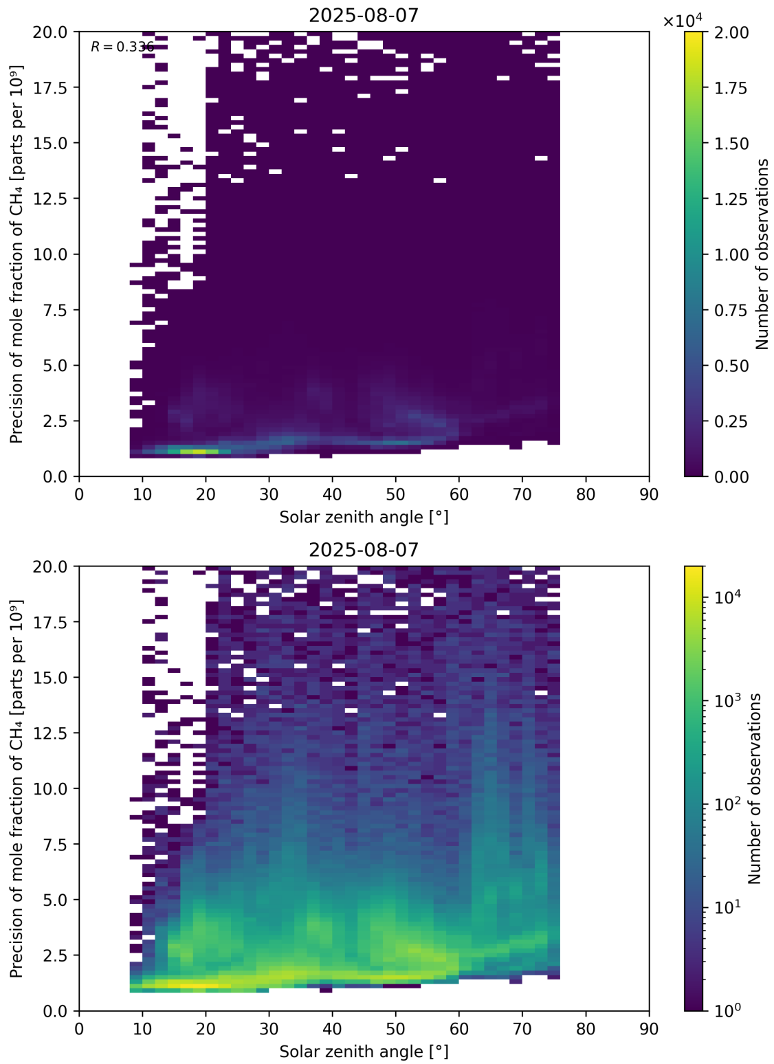
Figure 101: Scatter density plot of “Solar zenith angle” against “Precision of mole fraction of CH 4 ” for 2025-08-06 to 2025-08-08.
