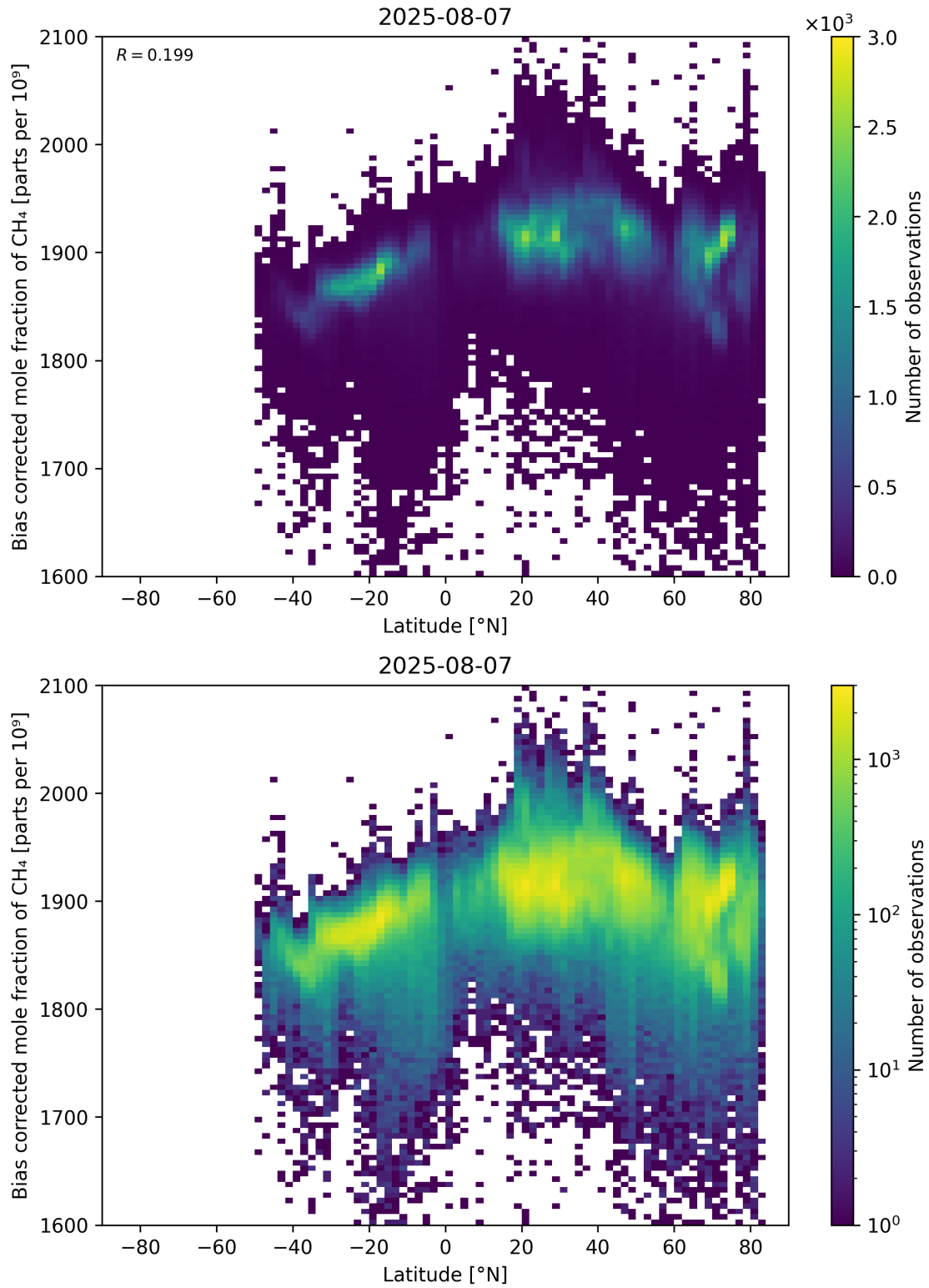
Figure 58: Scatter density plot of “Latitude” against “Bias corrected mole fraction of CH 4 ” for 2025-08-06 to 2025-08-08.
