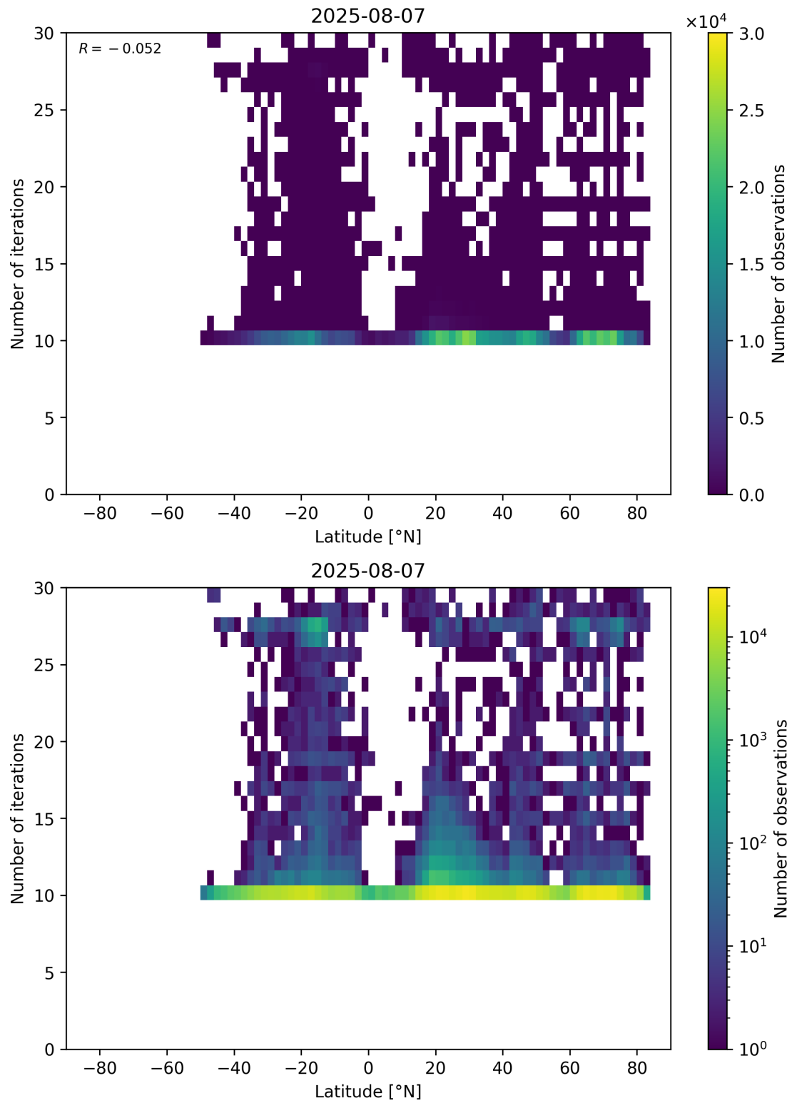
Figure 60: Scatter density plot of “Latitude” against “Number of iterations” for 2025-08-06 to 2025-08-08.
