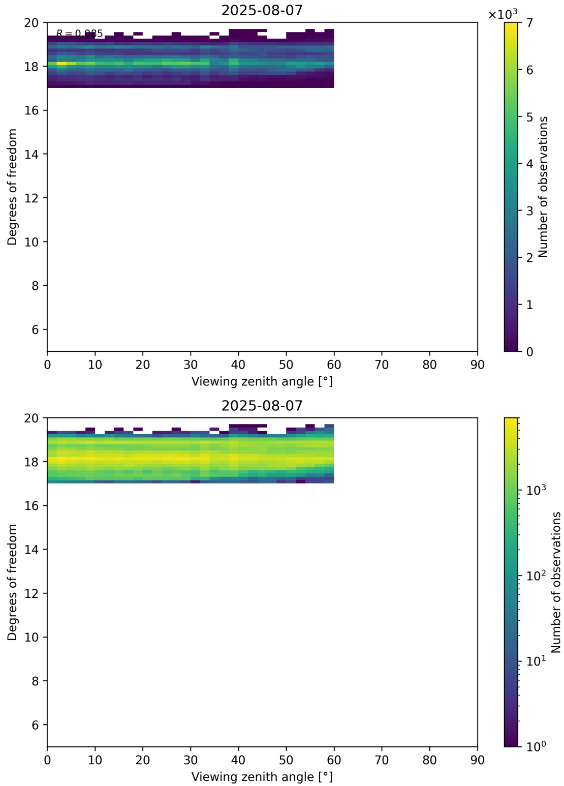
Figure 107: Scatter density plot of “Viewing zenith angle” against “Degrees of freedom” for 2025-08-06 to 2025-08-08.
