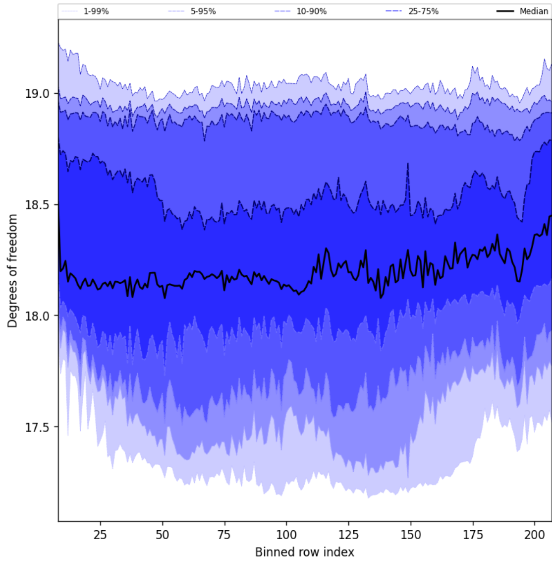
Figure 41: Along track statistics of “Degrees of freedom” for 2025-08-06 to 2025-08-08
