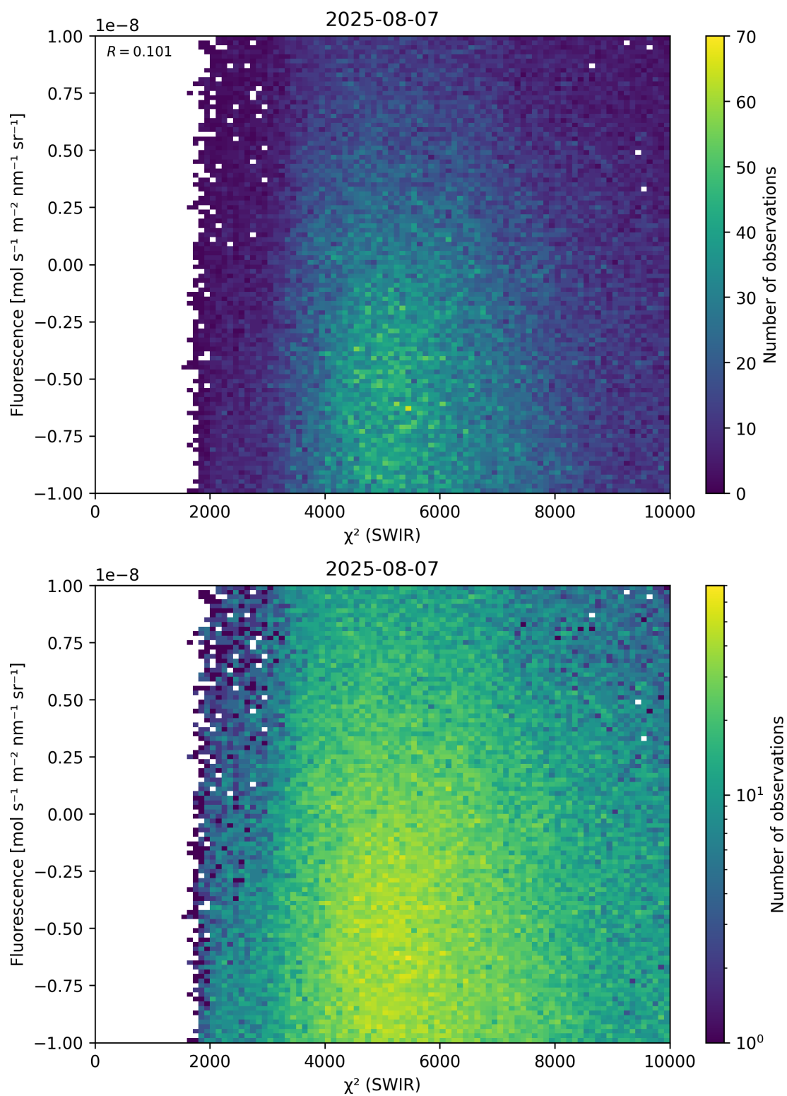
Figure 49: Scatter density plot of “ \chi^2 (SWIR)” against “Fluorescence” for 2025-08-06 to 2025-08-08.
