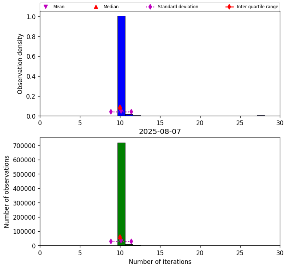
Figure 31: Histogram of “Number of iterations” for 2025-08-06 to 2025-08-08
