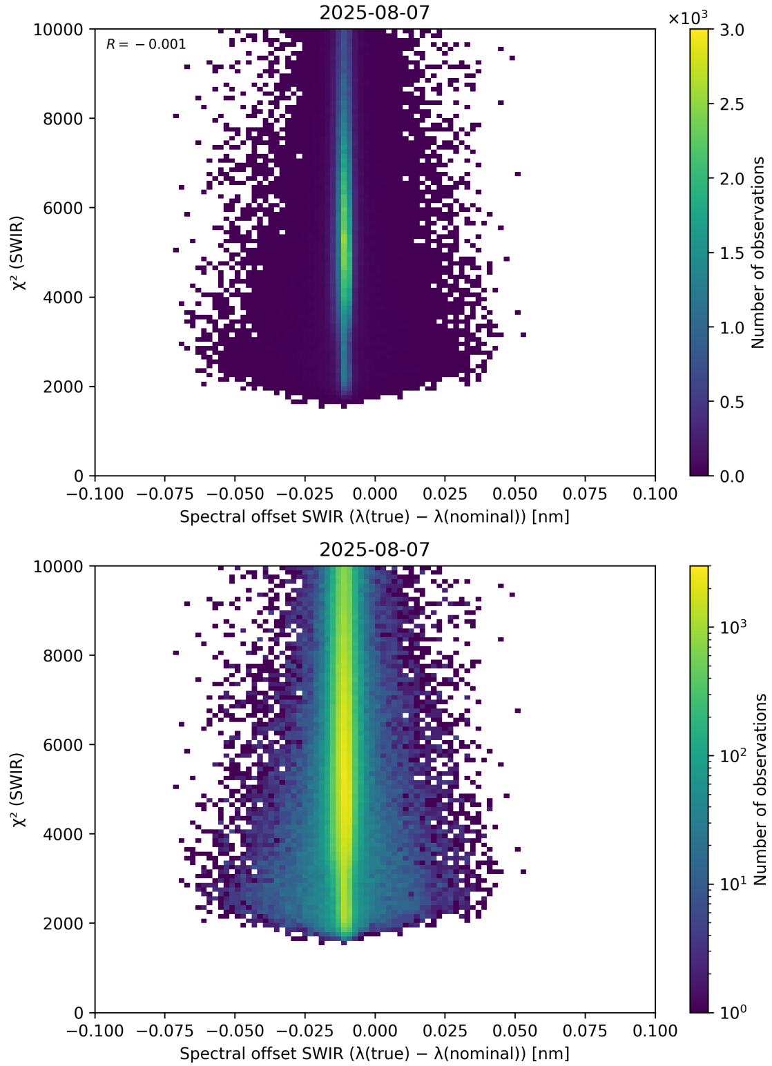
Figure 118: Scatter density plot of “Spectral offset SWIR ( \lambda_{\text{true}} - \lambda_{\text{nominal}} )” against “ \chi^2 (SWIR)” for 2025-08-06 to 2025-08-08.
