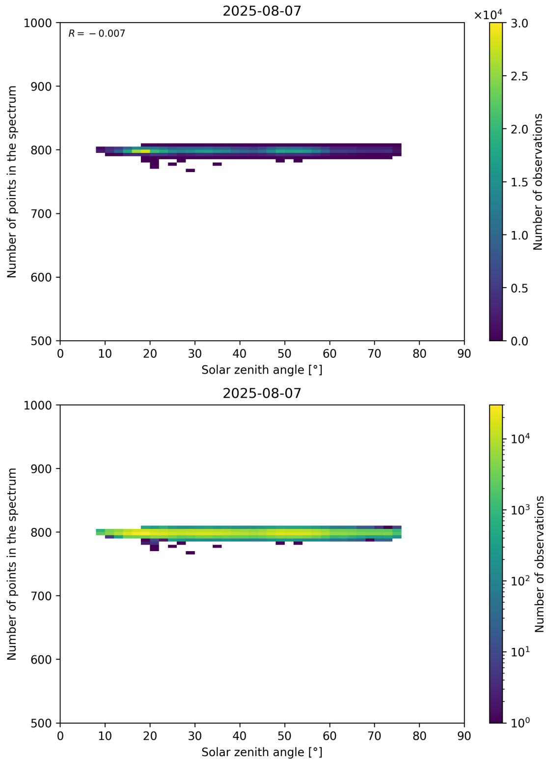
Figure 103: Scatter density plot of “Solar zenith angle” against “Number of points in the spectrum” for 2025-08-06 to 2025-08-08.
