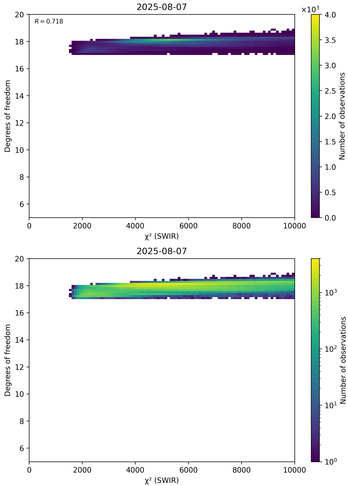
Figure 48: Scatter density plot of “ \chi^2 (SWIR)” against “Degrees of freedom” for 2025-08-06 to 2025-08-08.
