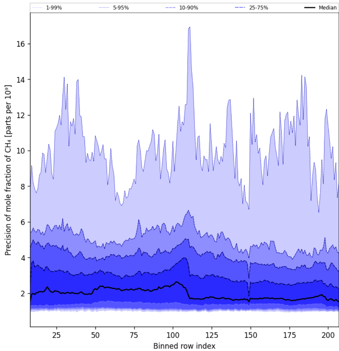
Figure 35: Along track statistics of “Precision of mole fraction of CH 4 ” for 2025-08-06 to 2025-08-08
