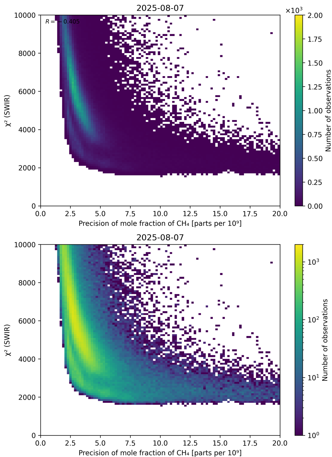
Figure 79: Scatter density plot of “Precision of mole fraction of \text{CH}_4 ” against “ \chi^2 (SWIR)” for 2025-08-06 to 2025-08-08.
