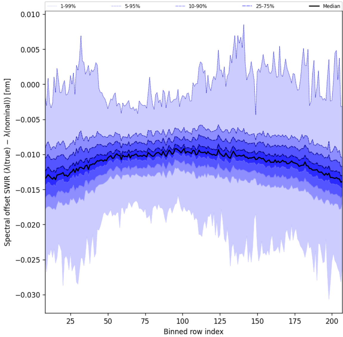
Figure 38: Along track statistics of “Spectral offset SWIR ( \lambda_{\text{true}} - \lambda_{\text{nominal}} )” for 2025-08-06 to 2025-08-08
