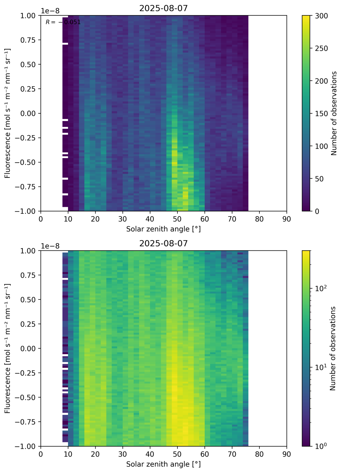
Figure 97: Scatter density plot of “Solar zenith angle” against “Fluorescence” for 2025-08-06 to 2025-08-08.
