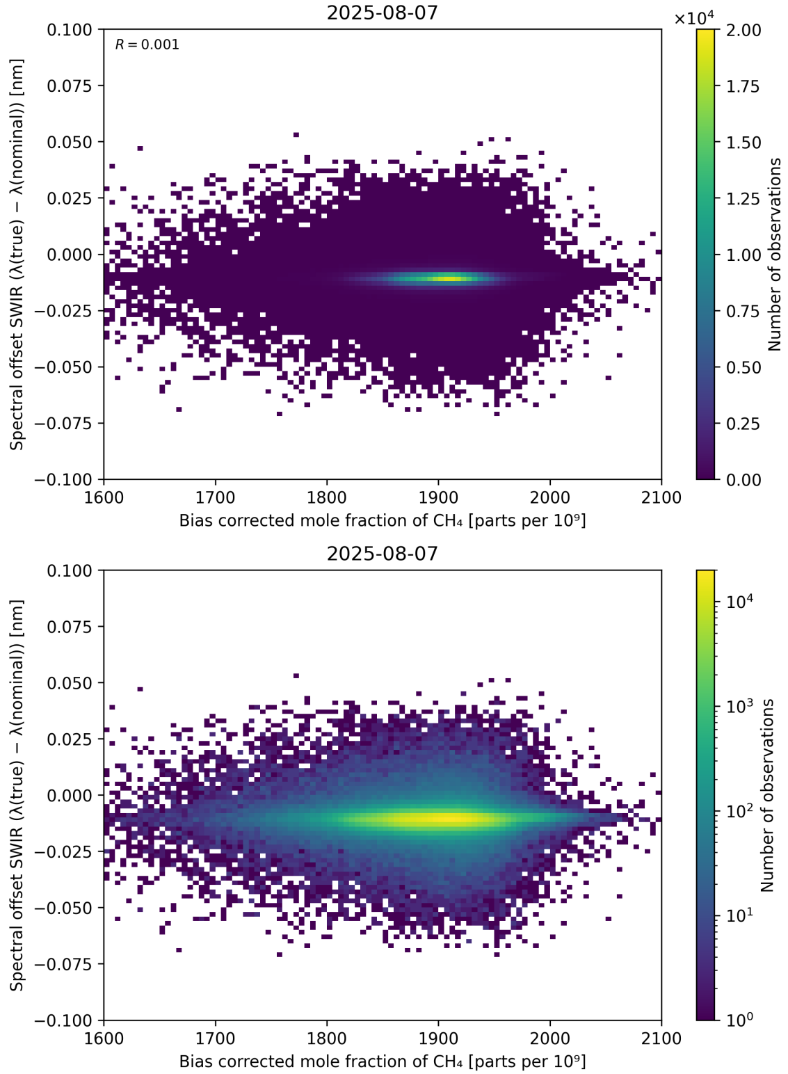
Figure 69: Scatter density plot of “Bias corrected mole fraction of \text{CH}_4 ” against “Spectral offset SWIR ( \lambda_{\text{true}} - \lambda_{\text{nominal}} )” for 2025-08-06 to 2025-08-08.
