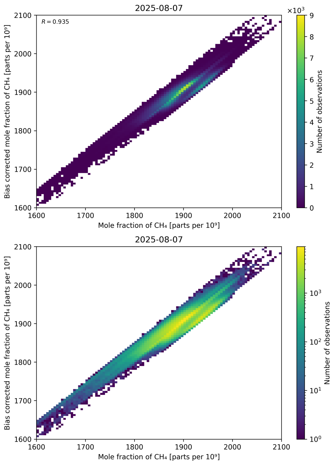
Figure 74: Scatter density plot of “Mole fraction of CH 4 ” against “Bias corrected mole fraction of CH 4 ” for 2025-08-06 to 2025-08-08.
