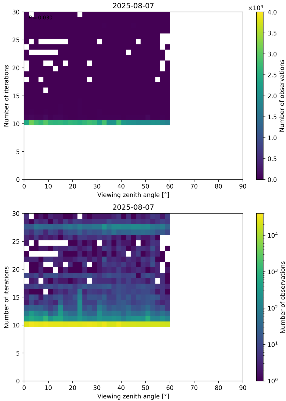
Figure 113: Scatter density plot of “Viewing zenith angle” against “Number of iterations” for 2025-08-06 to 2025-08-08.
