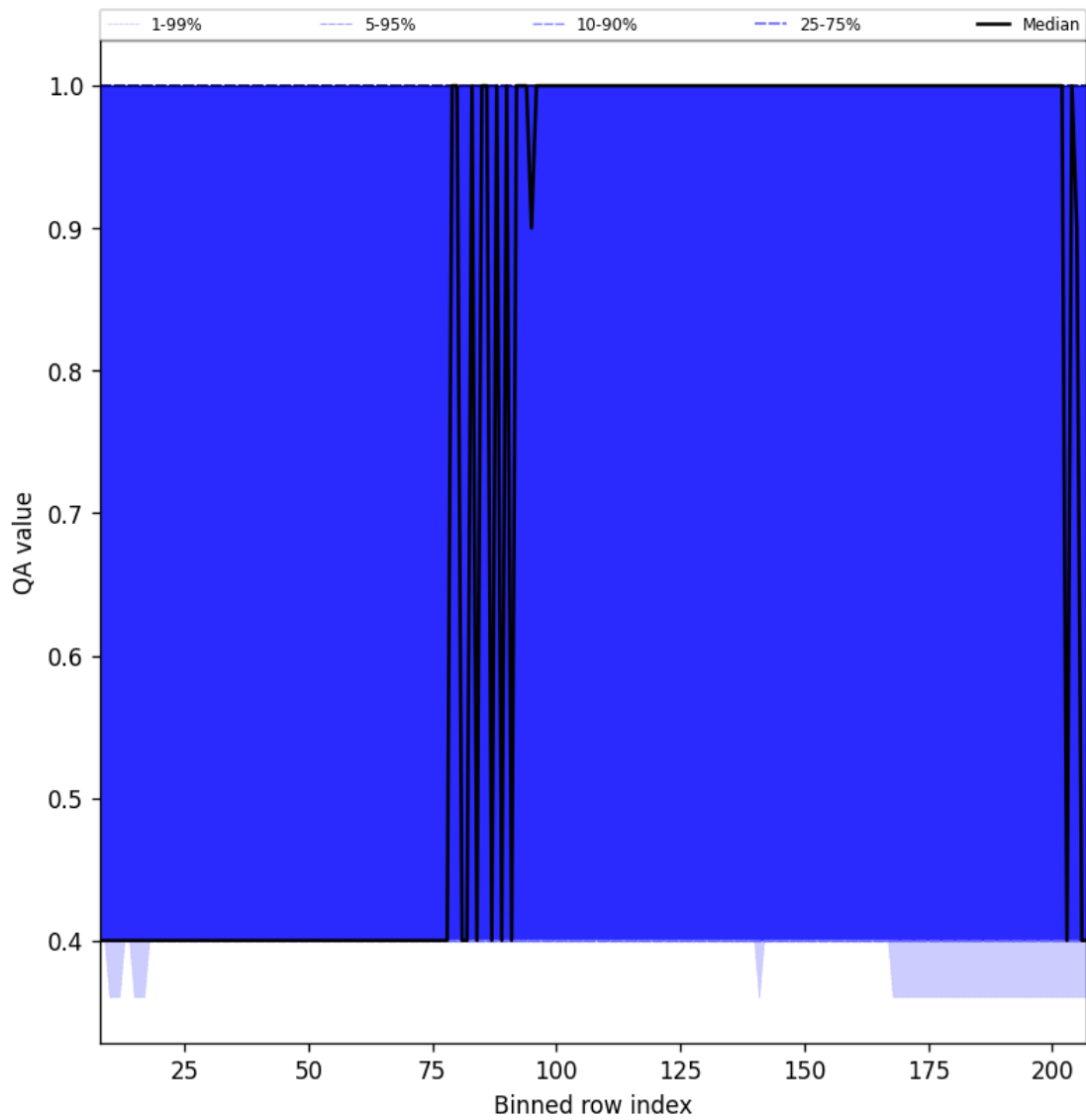
Figure 33: Along track statistics of “QA value” for 2025-08-06 to 2025-08-08
