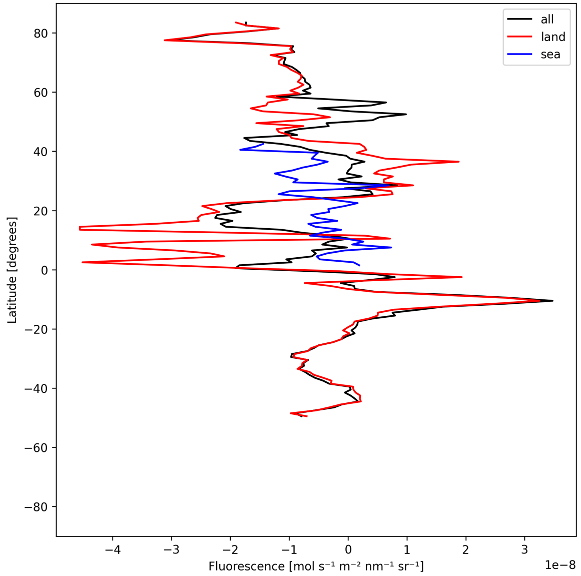
Figure 21: Zonal average of “Fluorescence” for 2025-08-06 to 2025-08-08.
