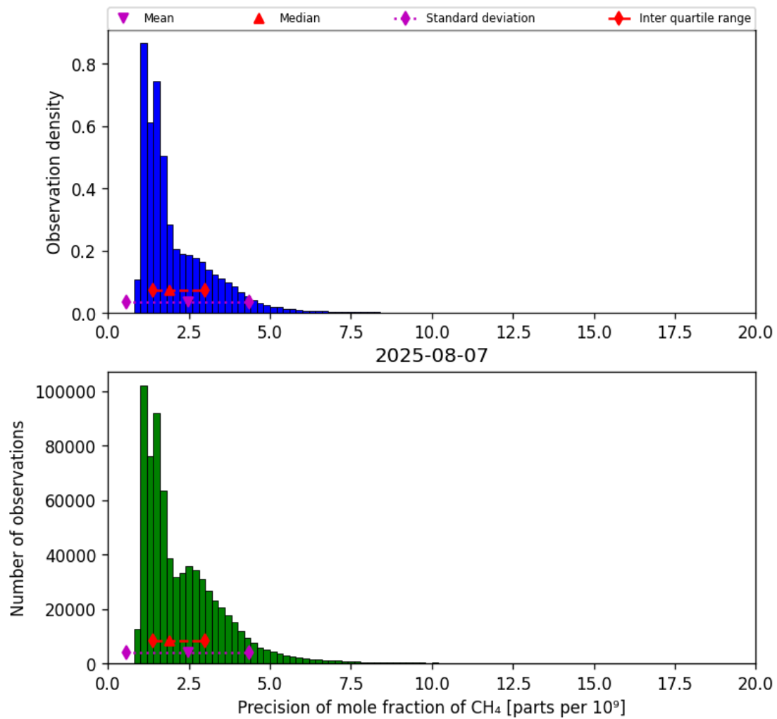
Figure 24: Histogram of “Precision of mole fraction of CH 4 ” for 2025-08-06 to 2025-08-08
