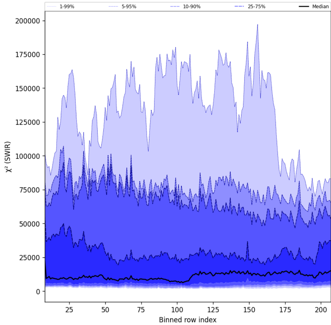
Figure 39: Along track statistics of “ \chi^2 (SWIR)” for 2025-08-06 to 2025-08-08
