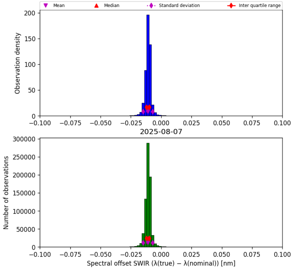
Figure 27: Histogram of “Spectral offset SWIR ( \lambda_{\text{true}} - \lambda_{\text{nominal}} )” for 2025-08-06 to 2025-08-08
