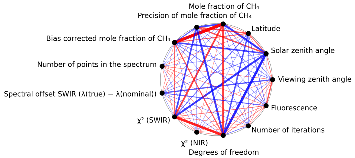
Figure 1: Map of correlation graph for 2025-08-06 to 2025-08-08.
