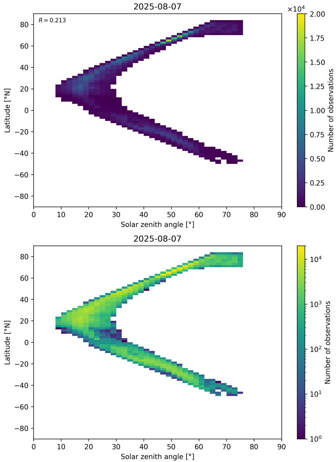
Figure 98: Scatter density plot of “Solar zenith angle” against “Latitude” for 2025-08-06 to 2025-08-08.
