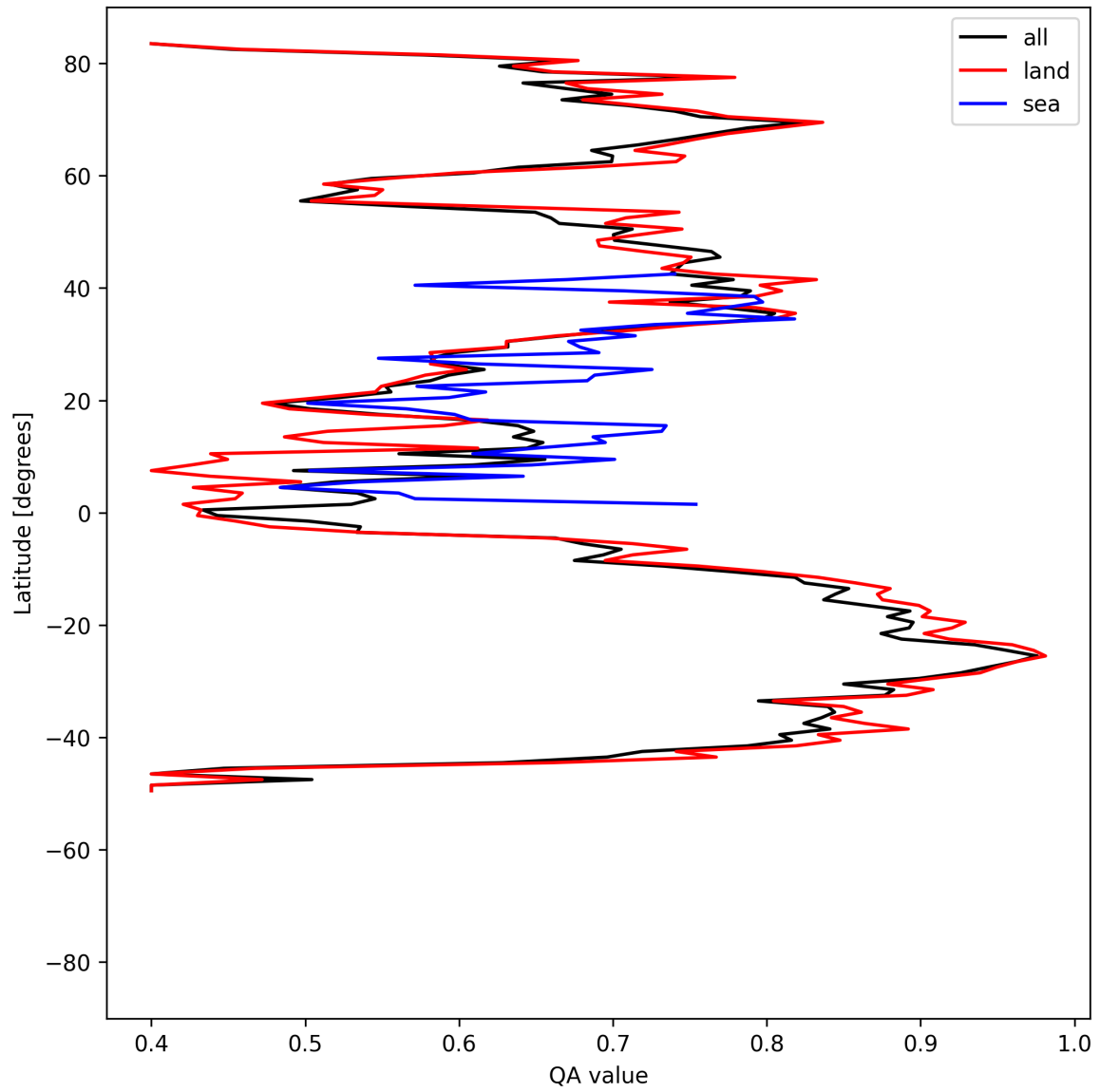
Figure 11: Zonal average of “QA value” for 2025-08-06 to 2025-08-08.
