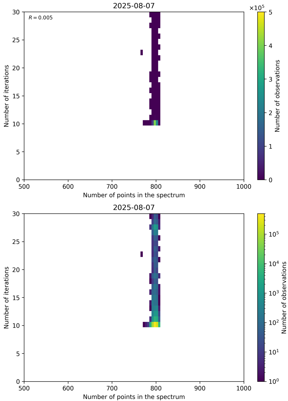
Figure 92: Scatter density plot of “Number of points in the spectrum” against “Number of iterations” for 2025-08-06 to 2025-08-08.
