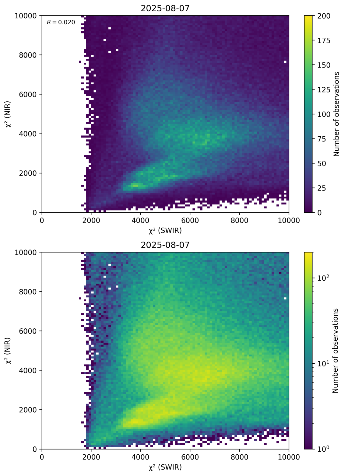
Figure 47: Scatter density plot of “ \chi^2 (SWIR)” against “ \chi^2 (NIR)” for 2025-08-06 to 2025-08-08.
