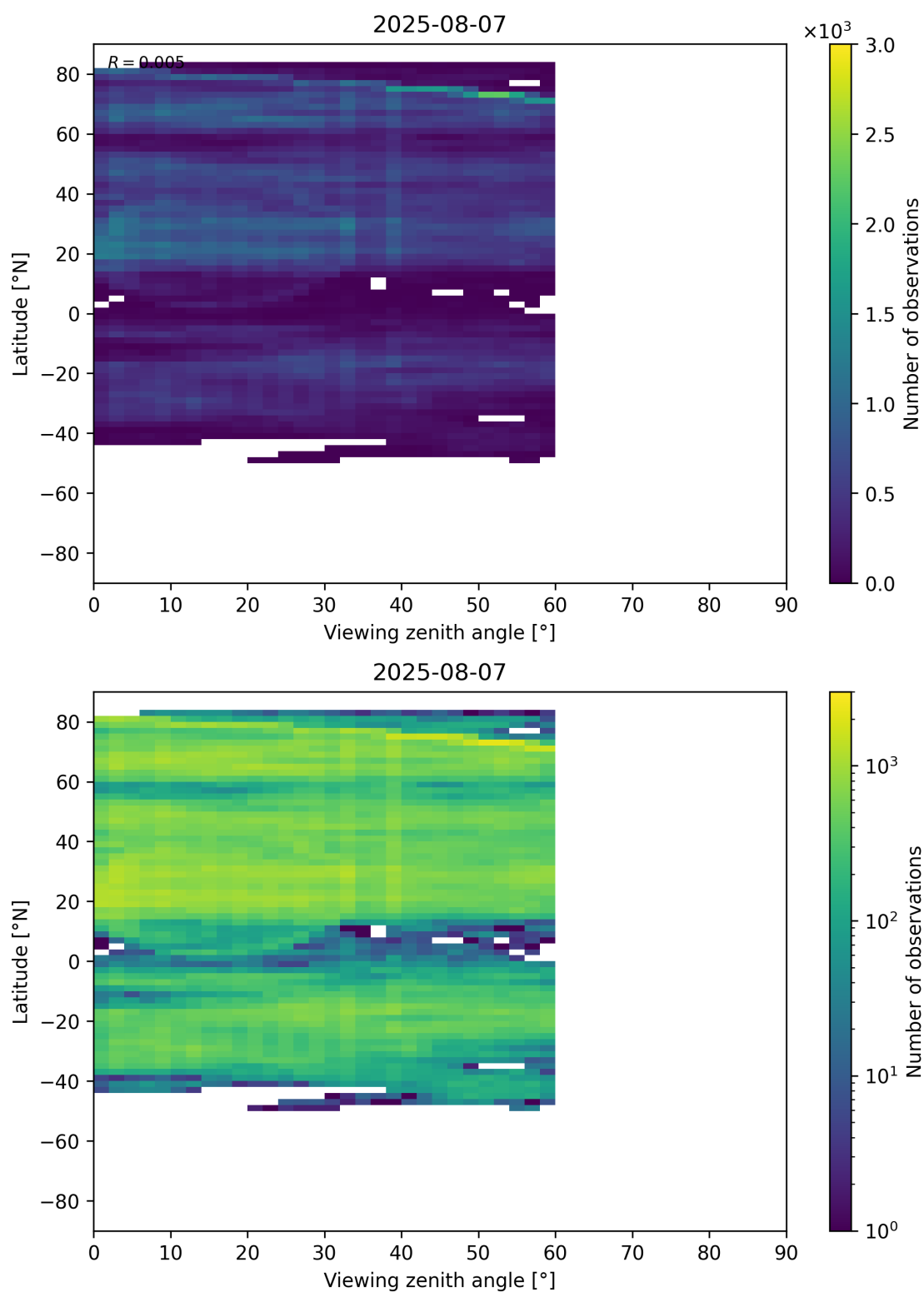
Figure 109: Scatter density plot of “Viewing zenith angle” against “Latitude” for 2025-08-06 to 2025-08-08.
