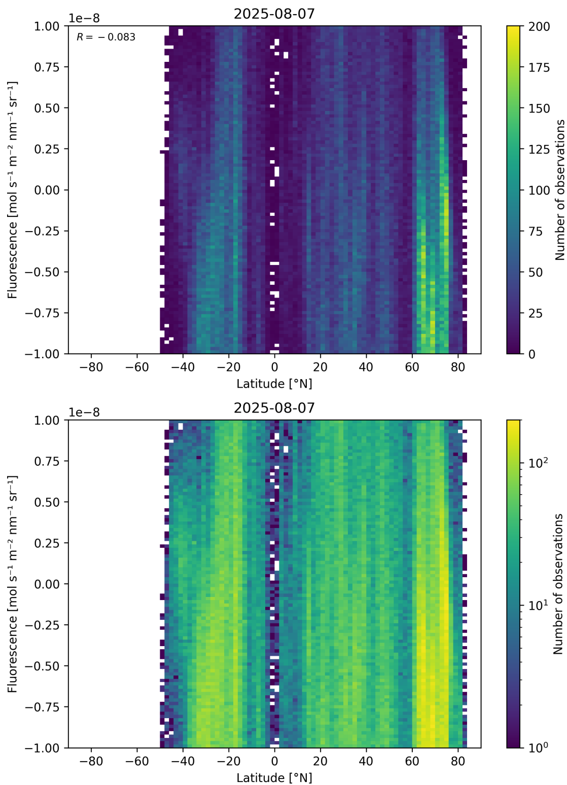
Figure 56: Scatter density plot of “Latitude” against “Fluorescence” for 2025-08-06 to 2025-08-08.
