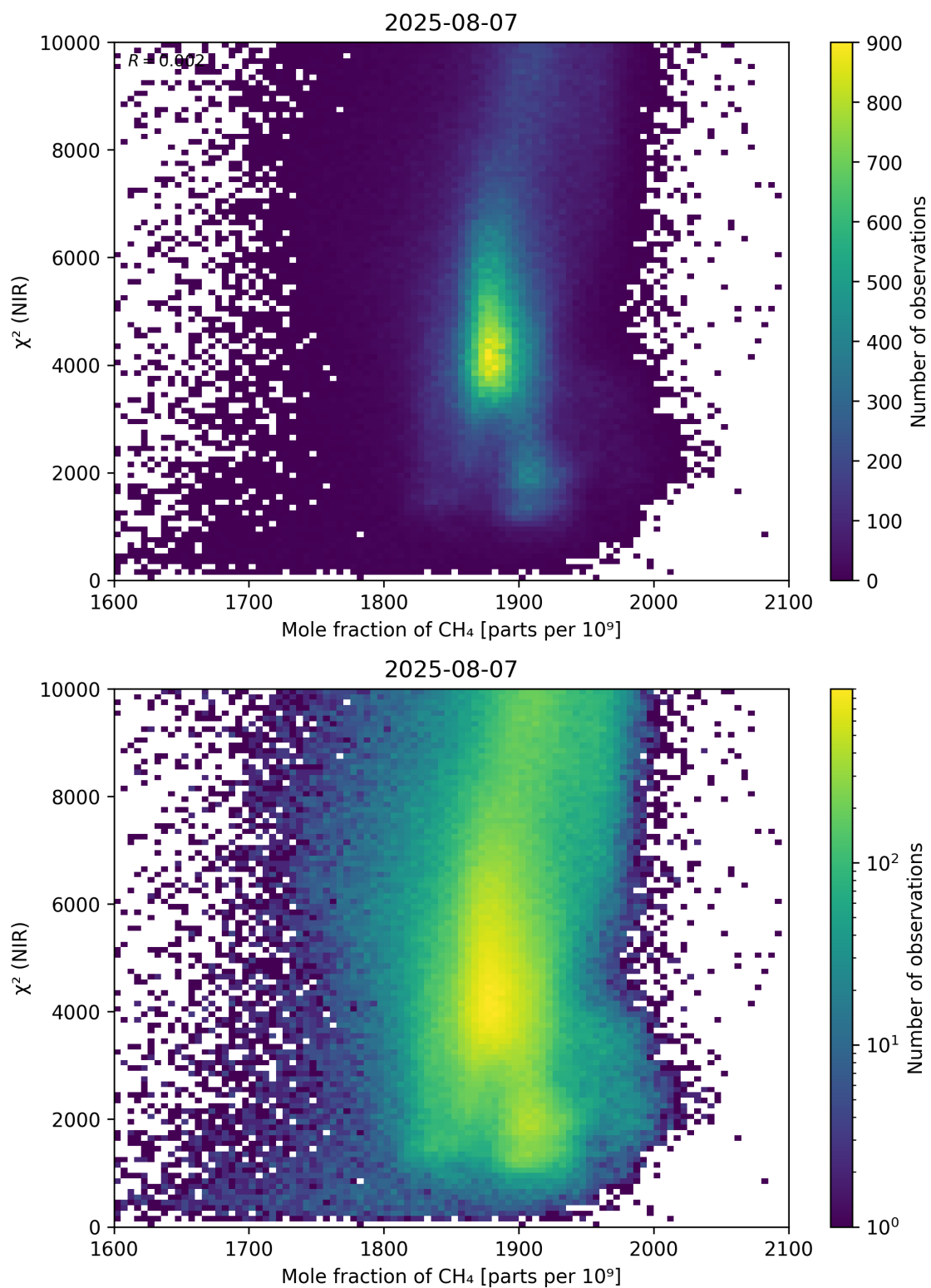
Figure 70: Scatter density plot of “Mole fraction of \text{CH}_4 ” against “ \chi^2 (NIR)” for 2025-08-06 to 2025-08-08.
