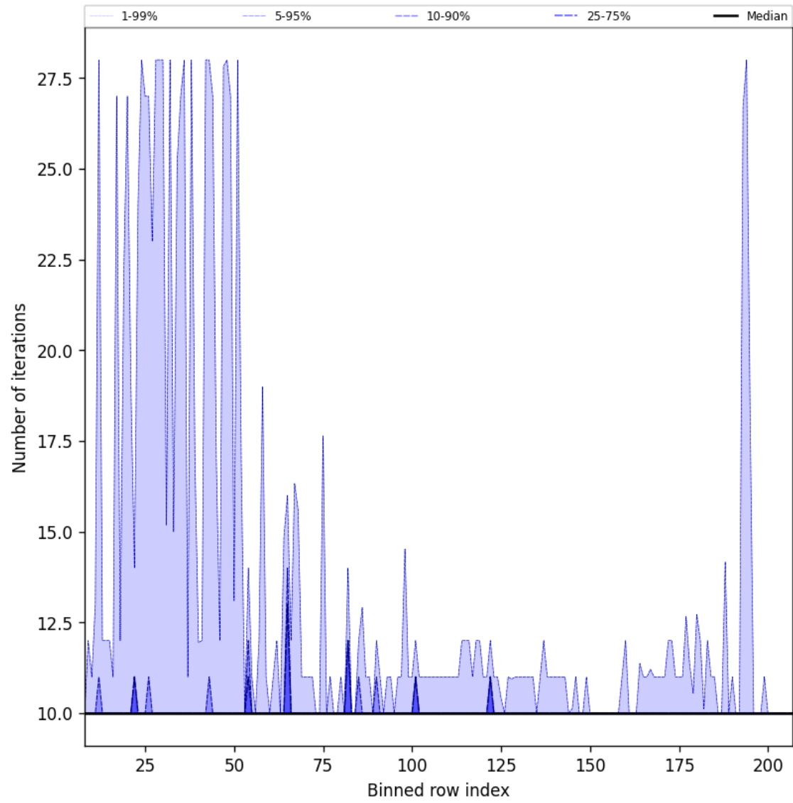
Figure 42: Along track statistics of “Number of iterations” for 2025-08-06 to 2025-08-08
