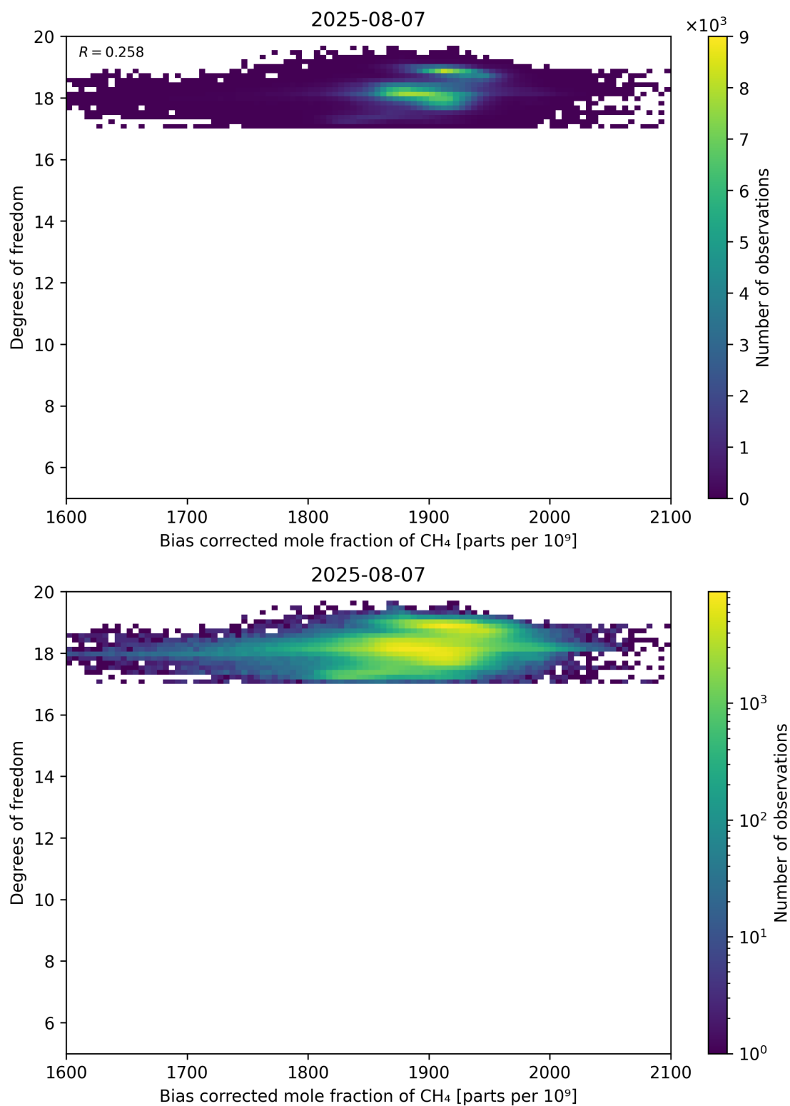
Figure 65: Scatter density plot of “Bias corrected mole fraction of CH 4 ” against “Degrees of freedom” for 2025-08-06 to 2025-08-08.
