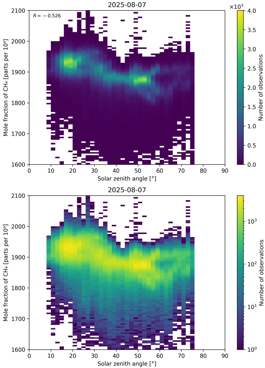
Figure 99: Scatter density plot of “Solar zenith angle” against “Mole fraction of CH 4 ” for 2025-08-06 to 2025-08-08.
