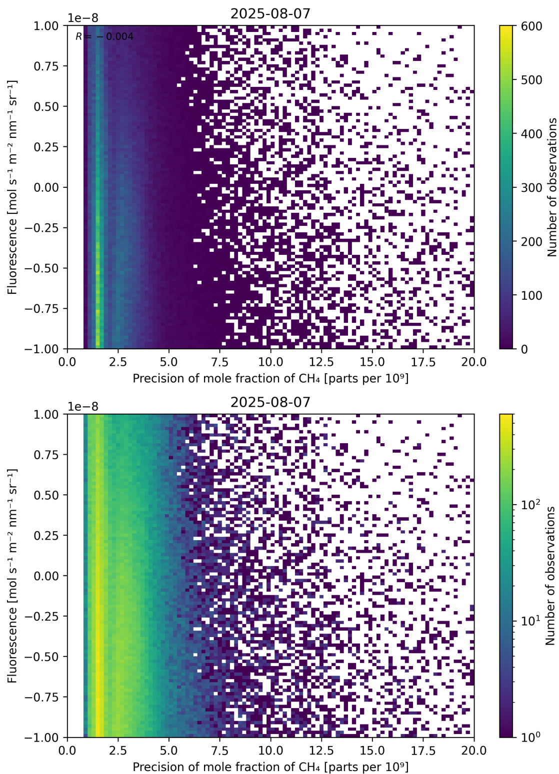
Figure 81: Scatter density plot of “Precision of mole fraction of \text{CH}_4 ” against “Fluorescence” for 2025-08-06 to 2025-08-08.
