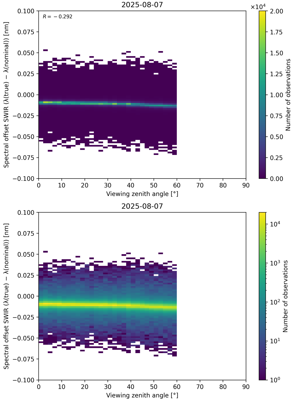
Figure 116: Scatter density plot of “Viewing zenith angle” against “Spectral offset SWIR ( \lambda_{\text{true}} - \lambda_{\text{nominal}} )” for 2025-08-06 to 2025-08-08.
