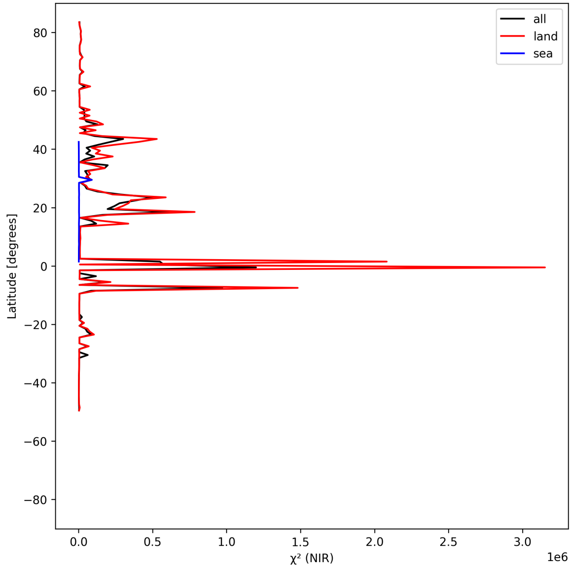
Figure 18: Zonal average of “ \chi^2 (NIR)” for 2025-08-06 to 2025-08-08.
