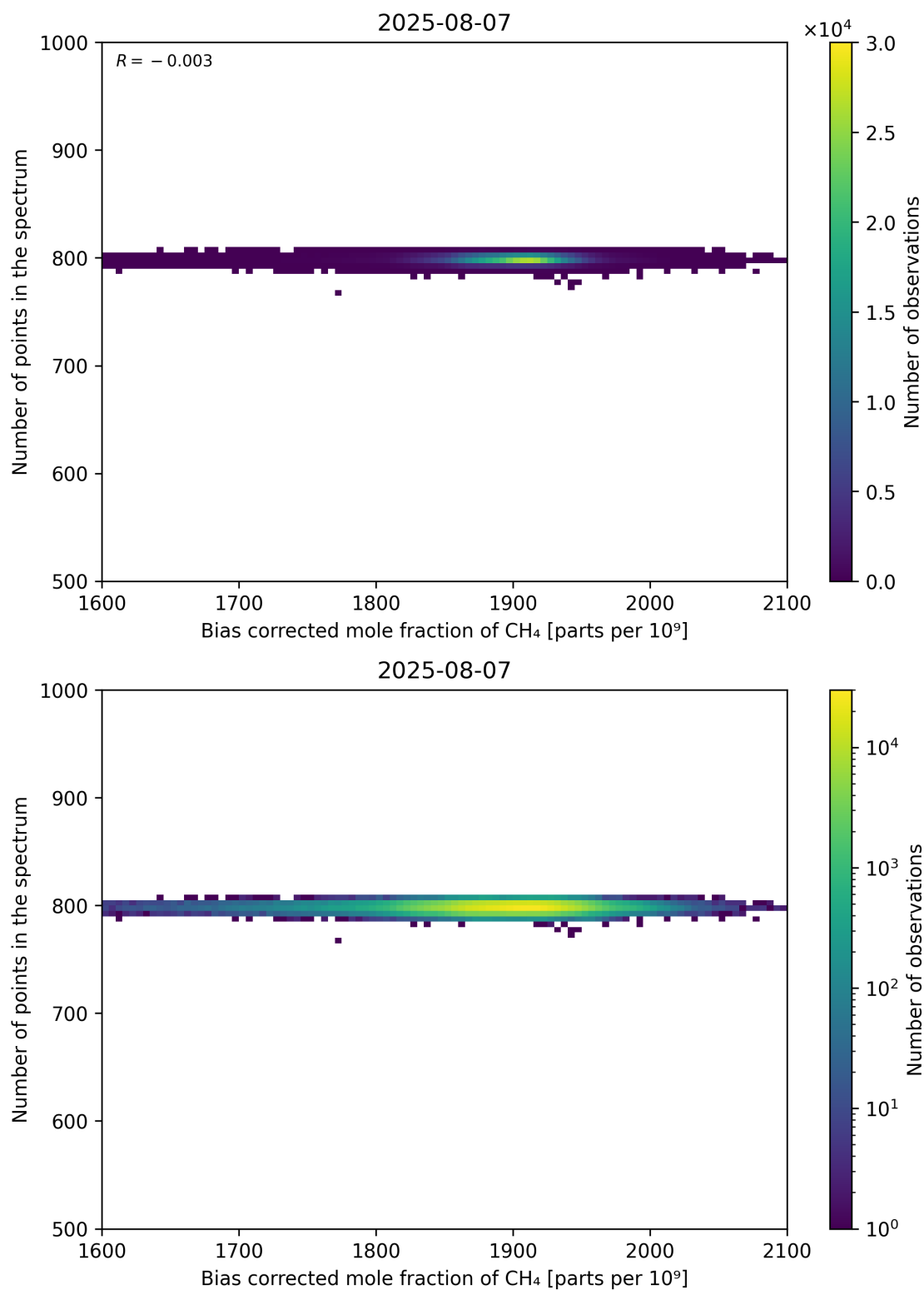
Figure 68: Scatter density plot of “Bias corrected mole fraction of CH 4 ” against “Number of points in the spectrum” for 2025-08-06 to 2025-08-08.
