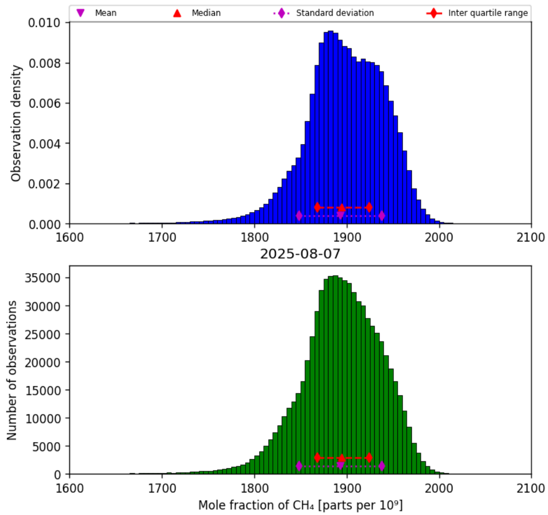
Figure 23: Histogram of “Mole fraction of CH 4 ” for 2025-08-06 to 2025-08-08
