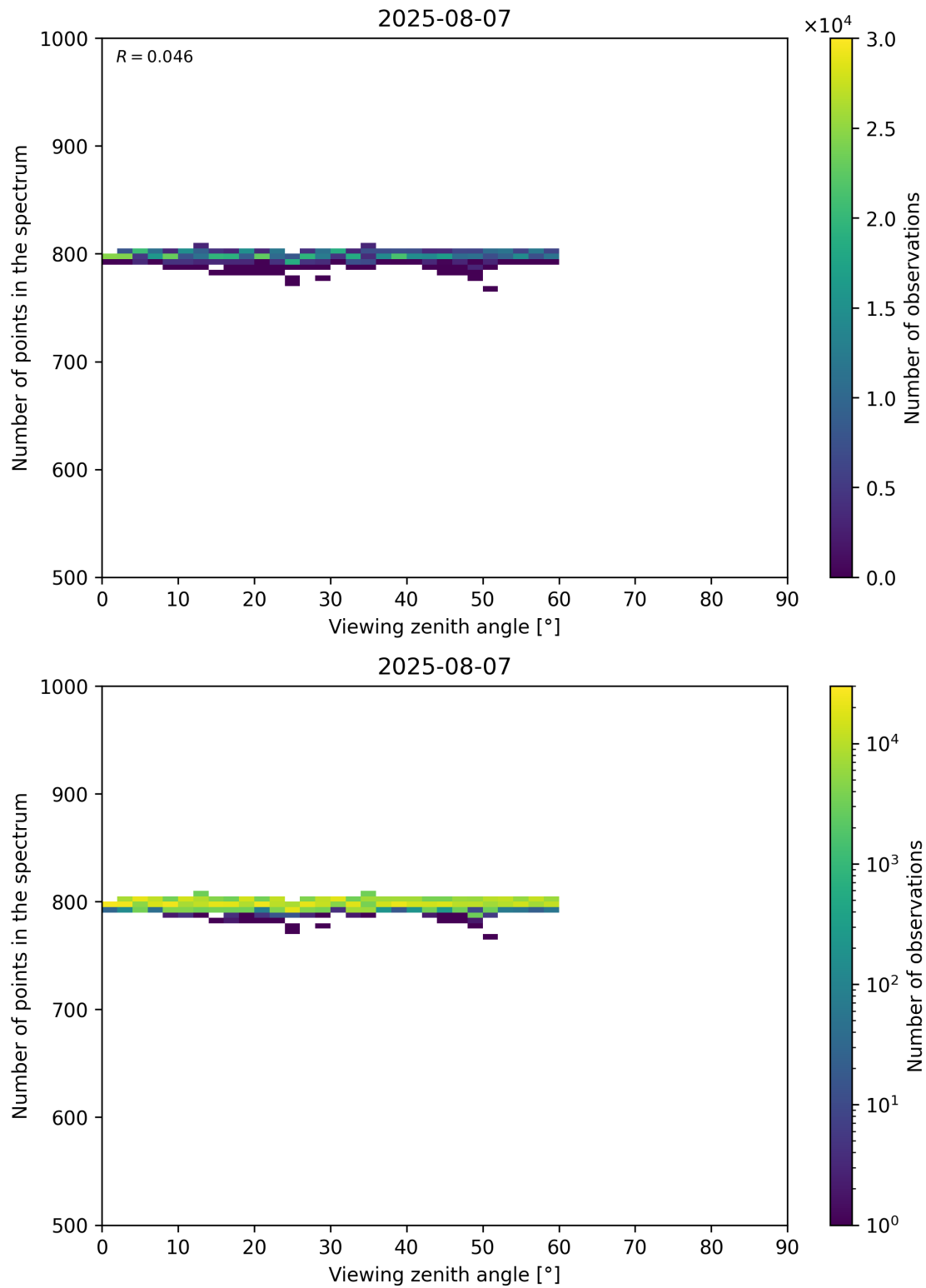
Figure 114: Scatter density plot of “Viewing zenith angle” against “Number of points in the spectrum” for 2025-08-06 to 2025-08-08.
