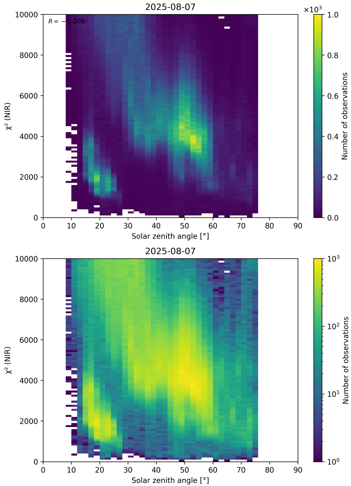
Figure 94: Scatter density plot of “Solar zenith angle” against “ \chi^2 (NIR)” for 2025-08-06 to 2025-08-08.
