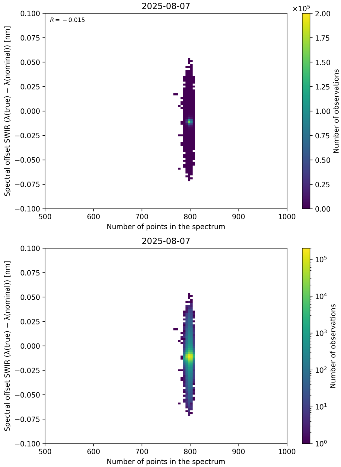
Figure 93: Scatter density plot of “Number of points in the spectrum” against “Spectral offset SWIR ( \lambda_{\text{true}} - \lambda_{\text{nominal}} )” for 2025-08-06 to 2025-08-08.
