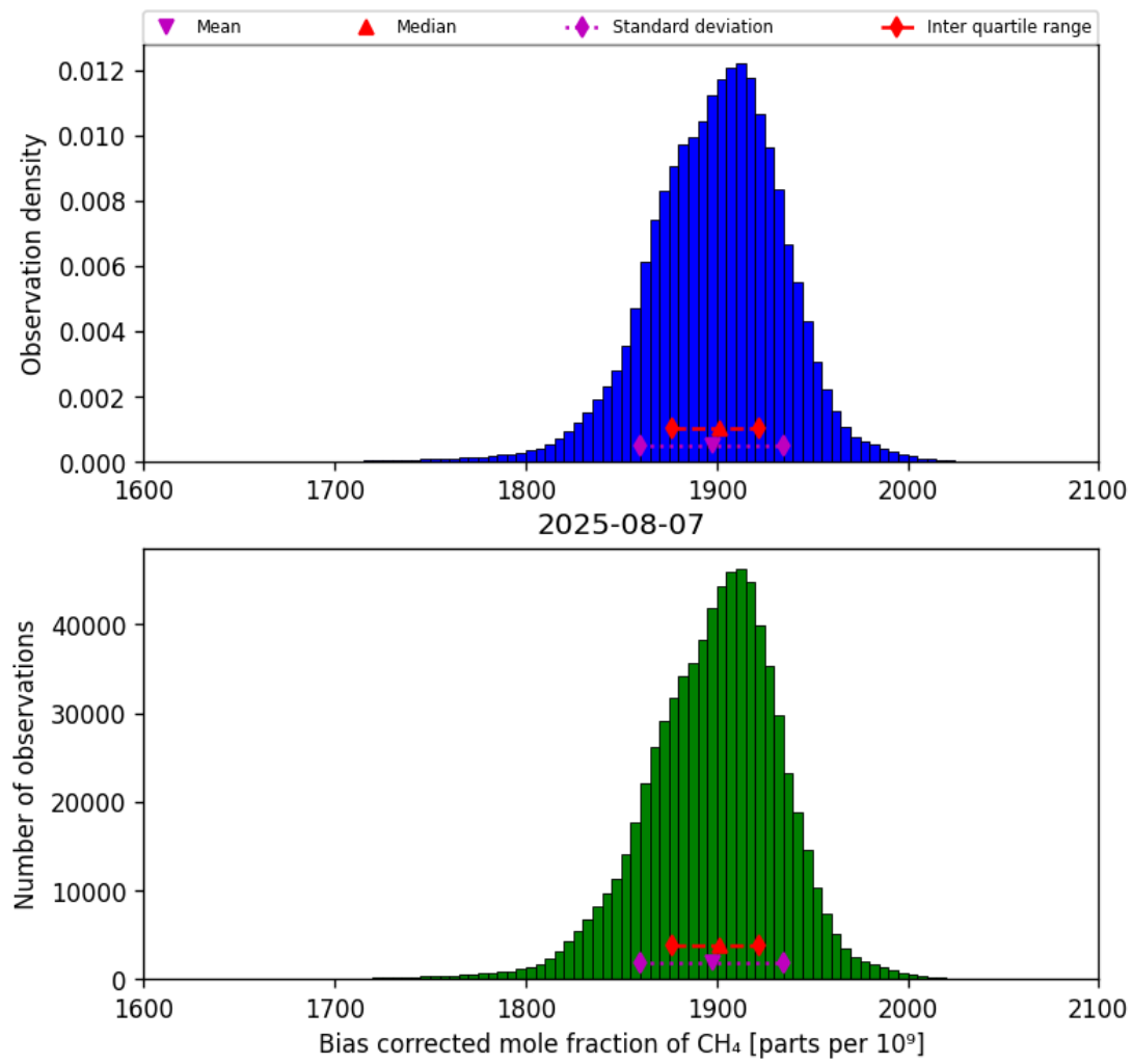
Figure 25: Histogram of “Bias corrected mole fraction of CH 4 ” for 2025-08-06 to 2025-08-08
