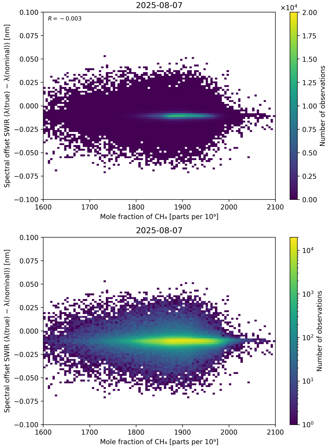
Figure 86: Scatter density plot of “Mole fraction of CH 4 ” against “Spectral offset SWIR ( \lambda_{\text{true}} - \lambda_{\text{nominal}} )” for 2025-08-06 to 2025-08-08.
