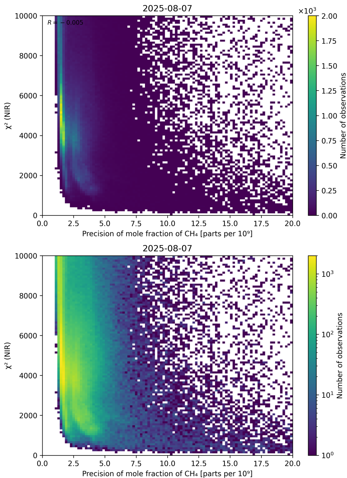
Figure 78: Scatter density plot of “Precision of mole fraction of CH 4 ” against “ \chi^2 (NIR)” for 2025-08-06 to 2025-08-08.
