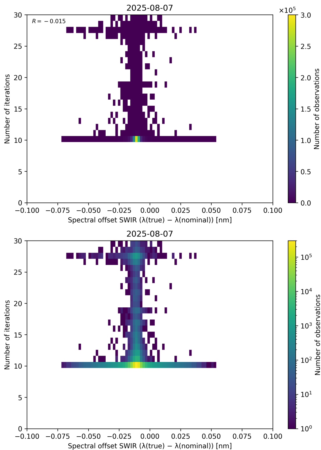
Figure 121: Scatter density plot of “Spectral offset SWIR ( \lambda_{\text{true}} - \lambda_{\text{nominal}} )” against “Number of iterations” for 2025-08-06 to 2025-08-08.
