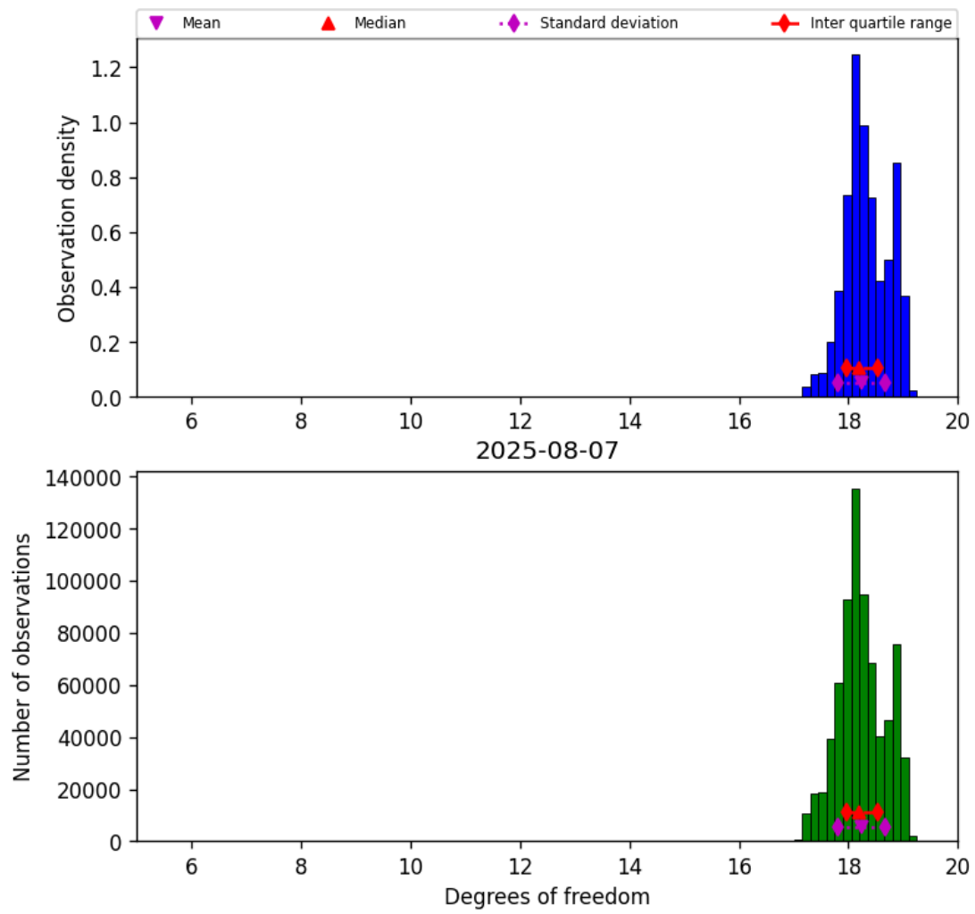
Figure 30: Histogram of “Degrees of freedom” for 2025-08-06 to 2025-08-08
