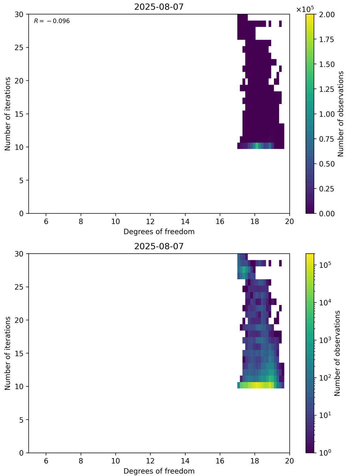
Figure 52: Scatter density plot of “Degrees of freedom” against “Number of iterations” for 2025-08-06 to 2025-08-08.
