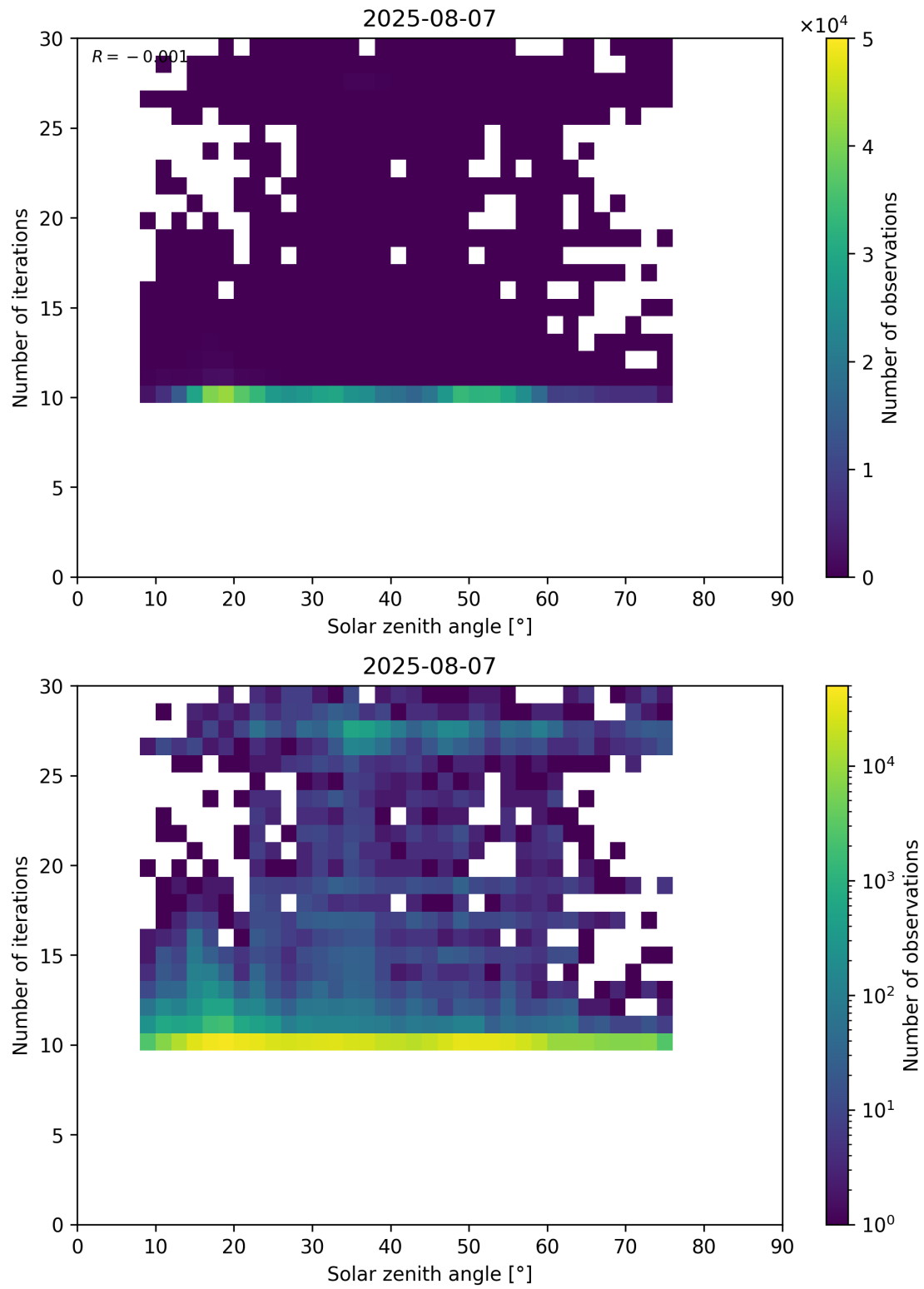
Figure 102: Scatter density plot of “Solar zenith angle” against “Number of iterations” for 2025-08-06 to 2025-08-08.
