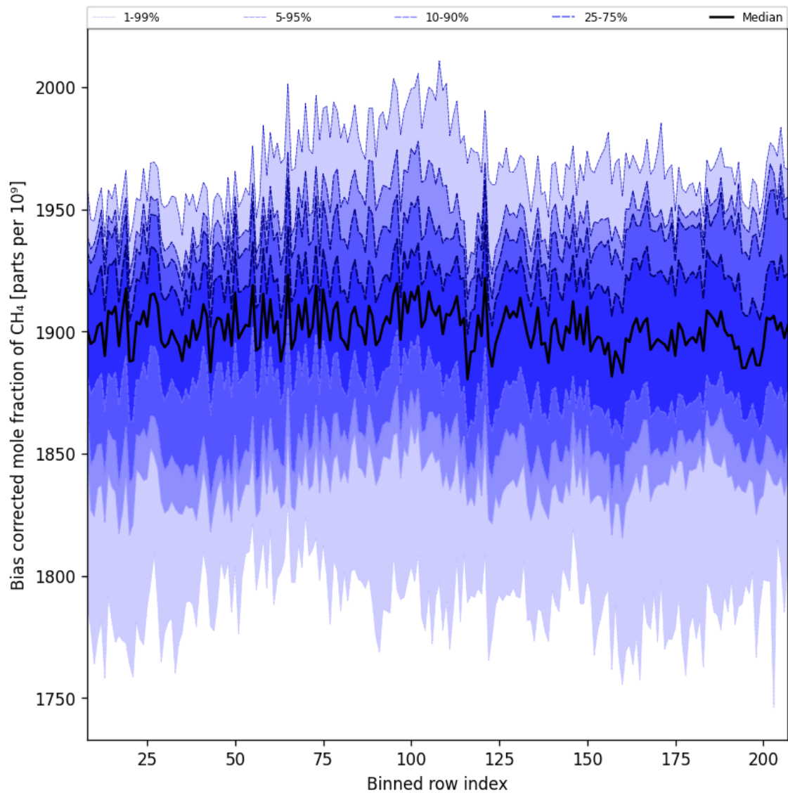
Figure 36: Along track statistics of “Bias corrected mole fraction of CH 4 ” for 2025-08-06 to 2025-08-08
