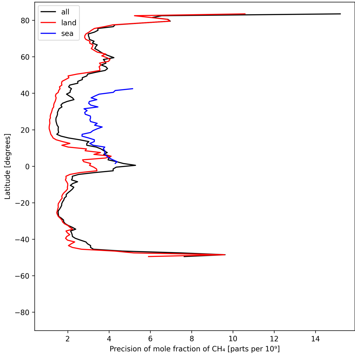
Figure 13: Zonal average of “Precision of mole fraction of CH 4 ” for 2025-08-06 to 2025-08-08.
