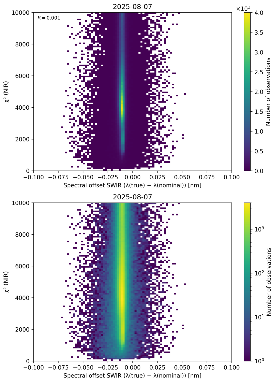
Figure 117: Scatter density plot of “Spectral offset SWIR ( \lambda_{\text{true}} - \lambda_{\text{nominal}} )” against “ \chi^2 (NIR)” for 2025-08-06 to 2025-08-08.
