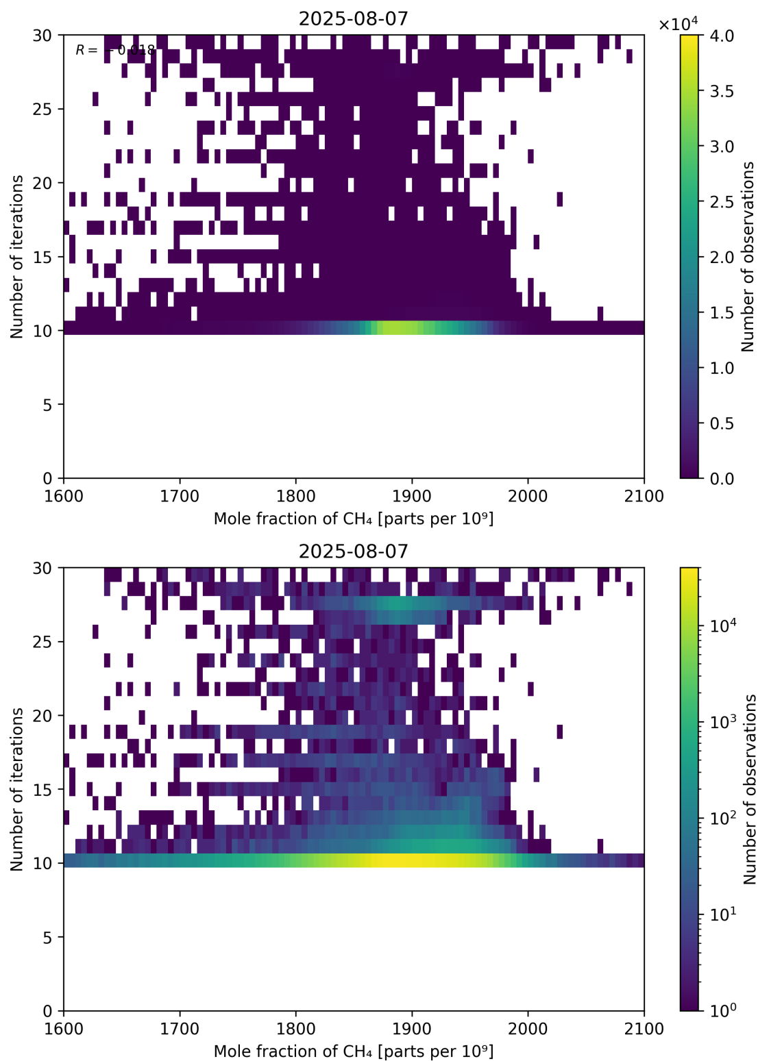
Figure 76: Scatter density plot of “Mole fraction of CH 4 ” against “Number of iterations” for 2025-08-06 to 2025-08-08.
