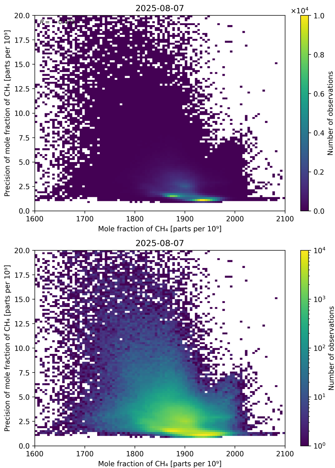
Figure 75: Scatter density plot of “Mole fraction of CH 4 ” against “Precision of mole fraction of CH 4 ” for 2025-08-06 to 2025-08-08.
