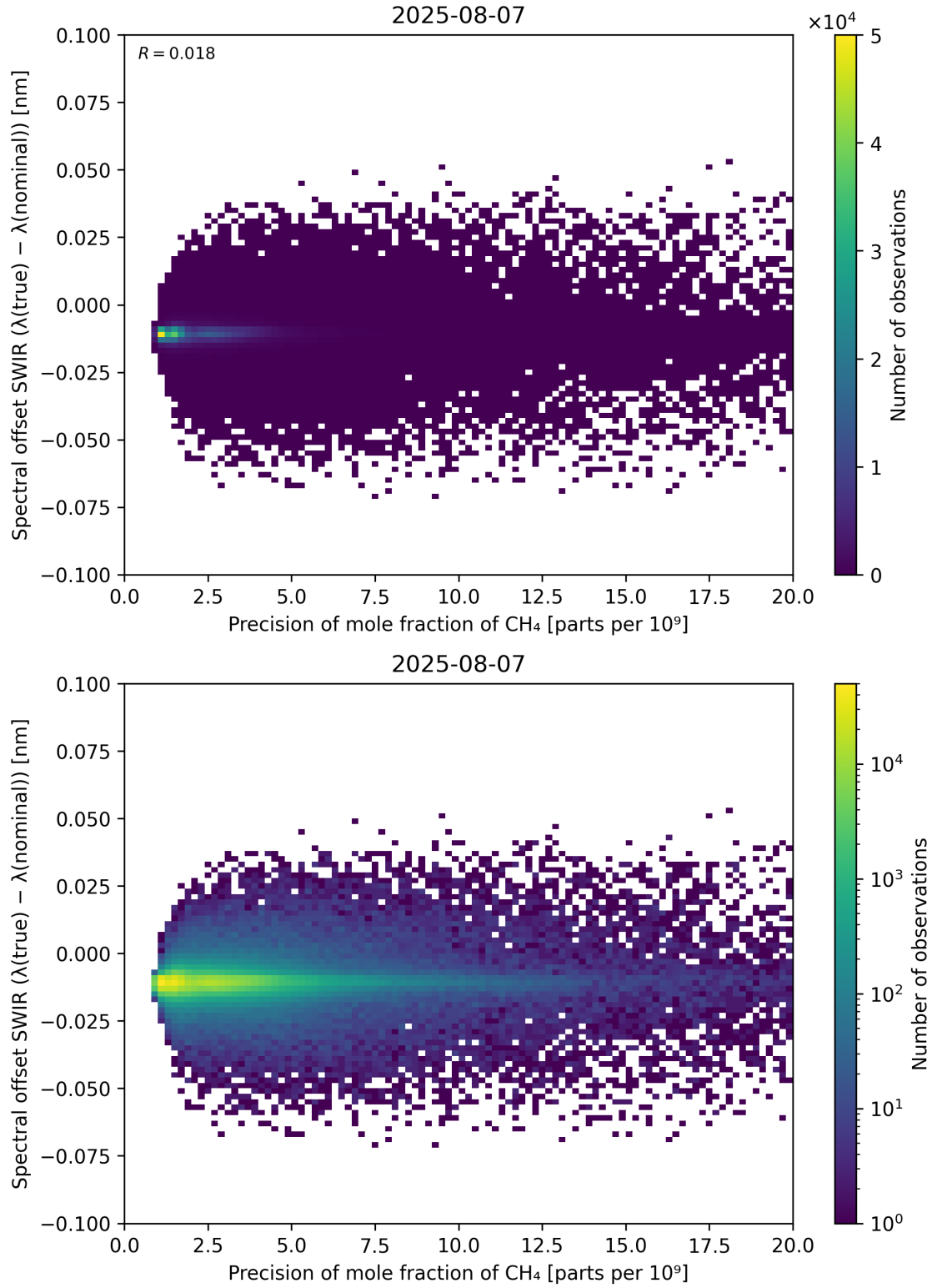
Figure 85: Scatter density plot of “Precision of mole fraction of CH 4 ” against “Spectral offset SWIR ( \lambda_{\text{true}} - \lambda_{\text{nominal}} )” for 2025-08-06 to 2025-08-08.
