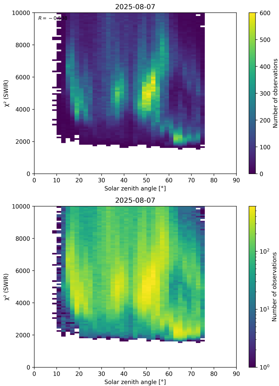
Figure 95: Scatter density plot of “Solar zenith angle” against “ \chi^2 (SWIR)” for 2025-08-06 to 2025-08-08.
