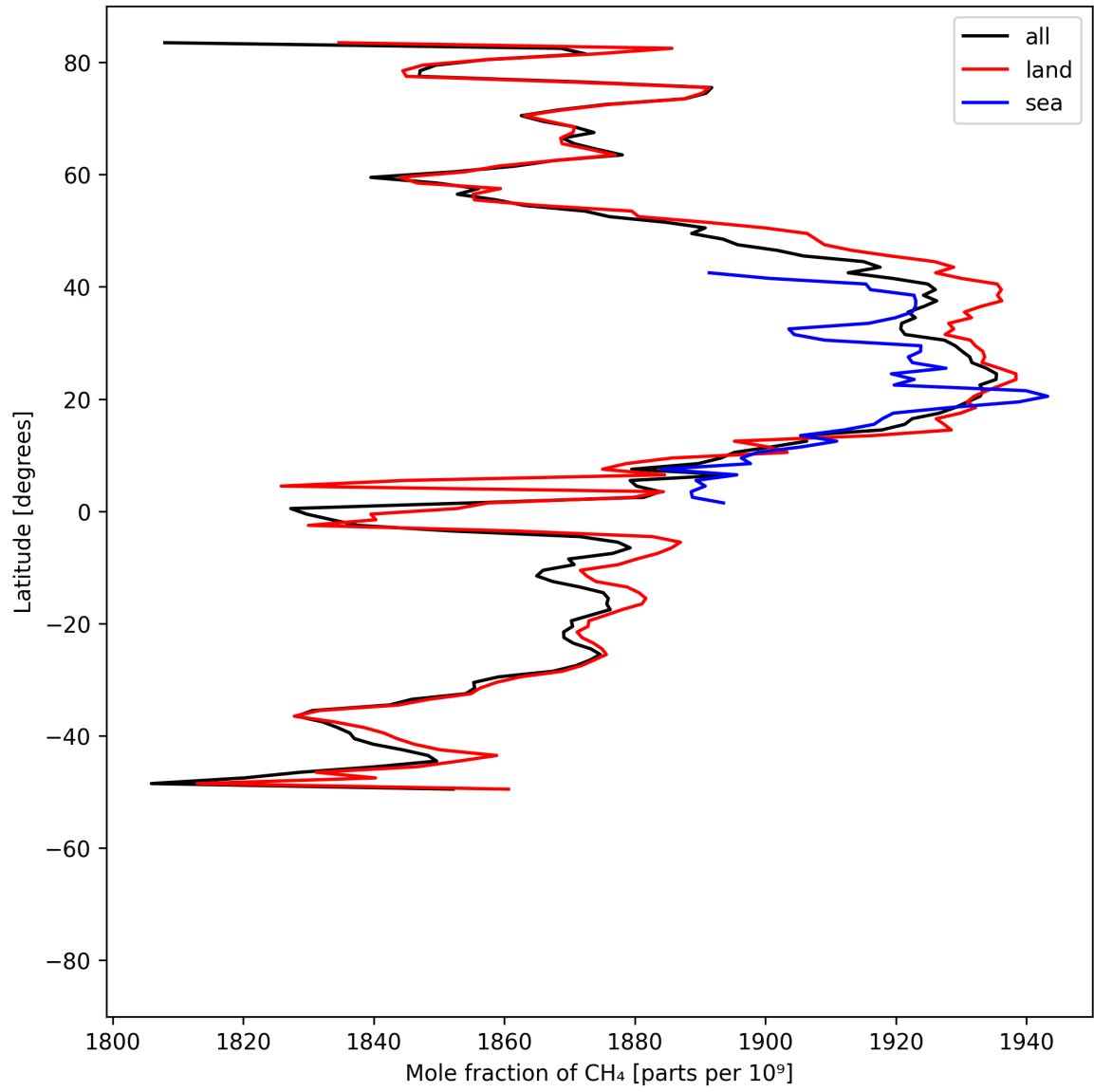
Figure 12: Zonal average of “Mole fraction of CH 4 ” for 2025-08-06 to 2025-08-08.
