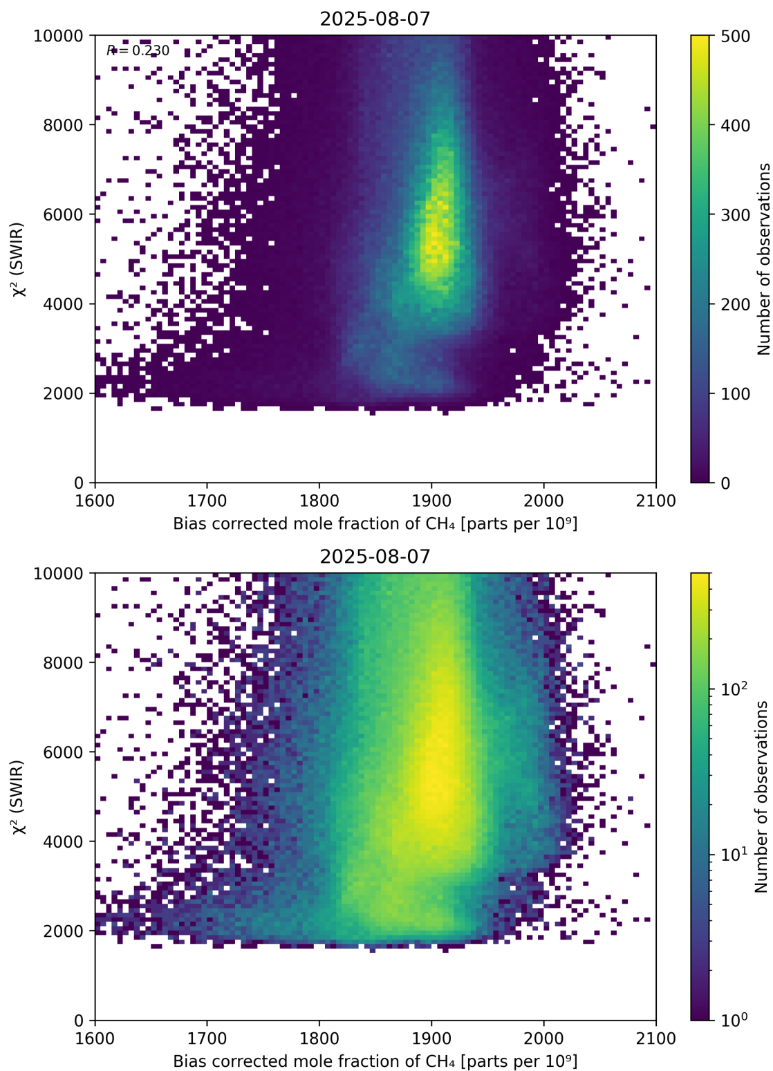
Figure 64: Scatter density plot of “Bias corrected mole fraction of \text{CH}_4 ” against “ \chi^2 (SWIR)” for 2025-08-06 to 2025-08-08.
