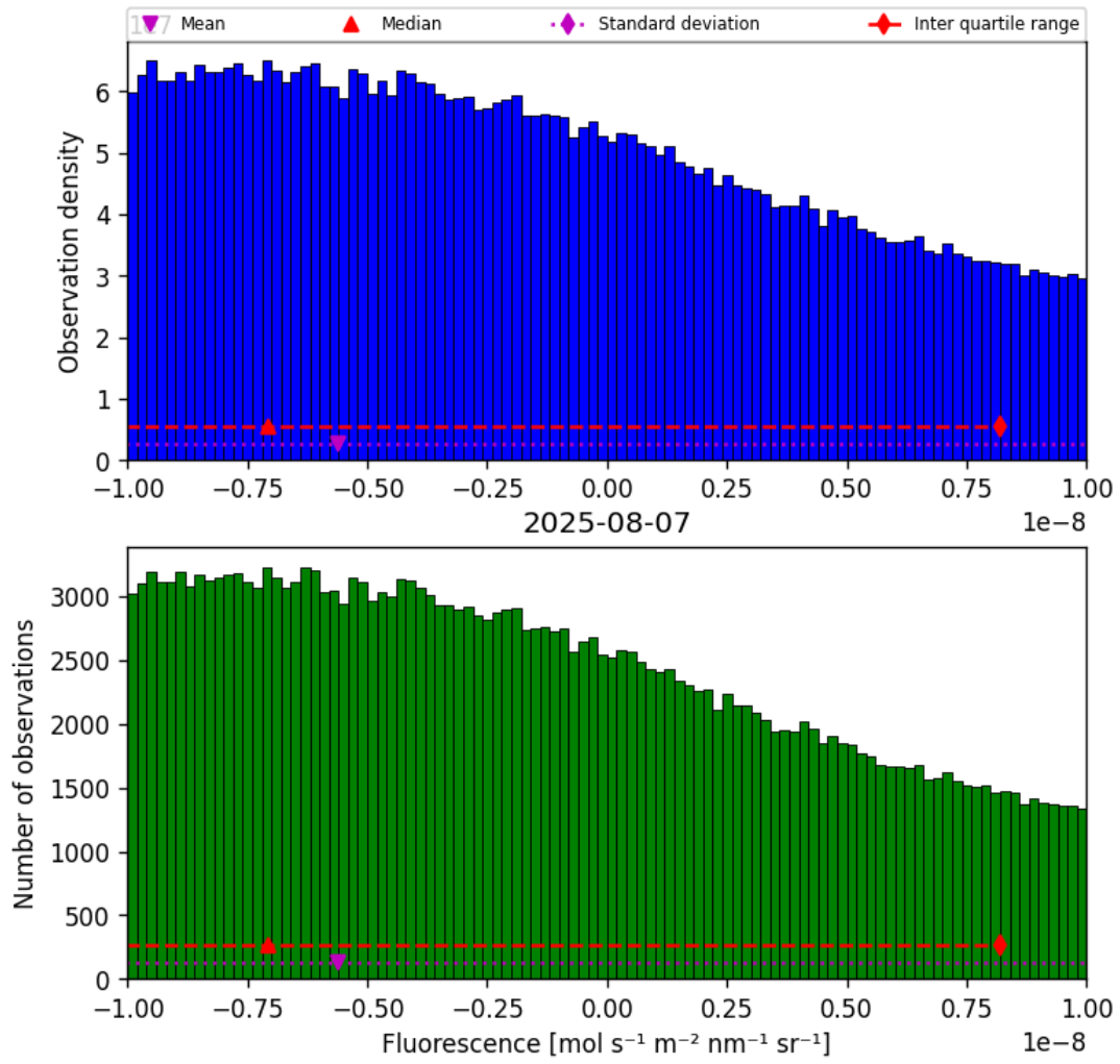
Figure 32: Histogram of “Fluorescence” for 2025-08-06 to 2025-08-08
