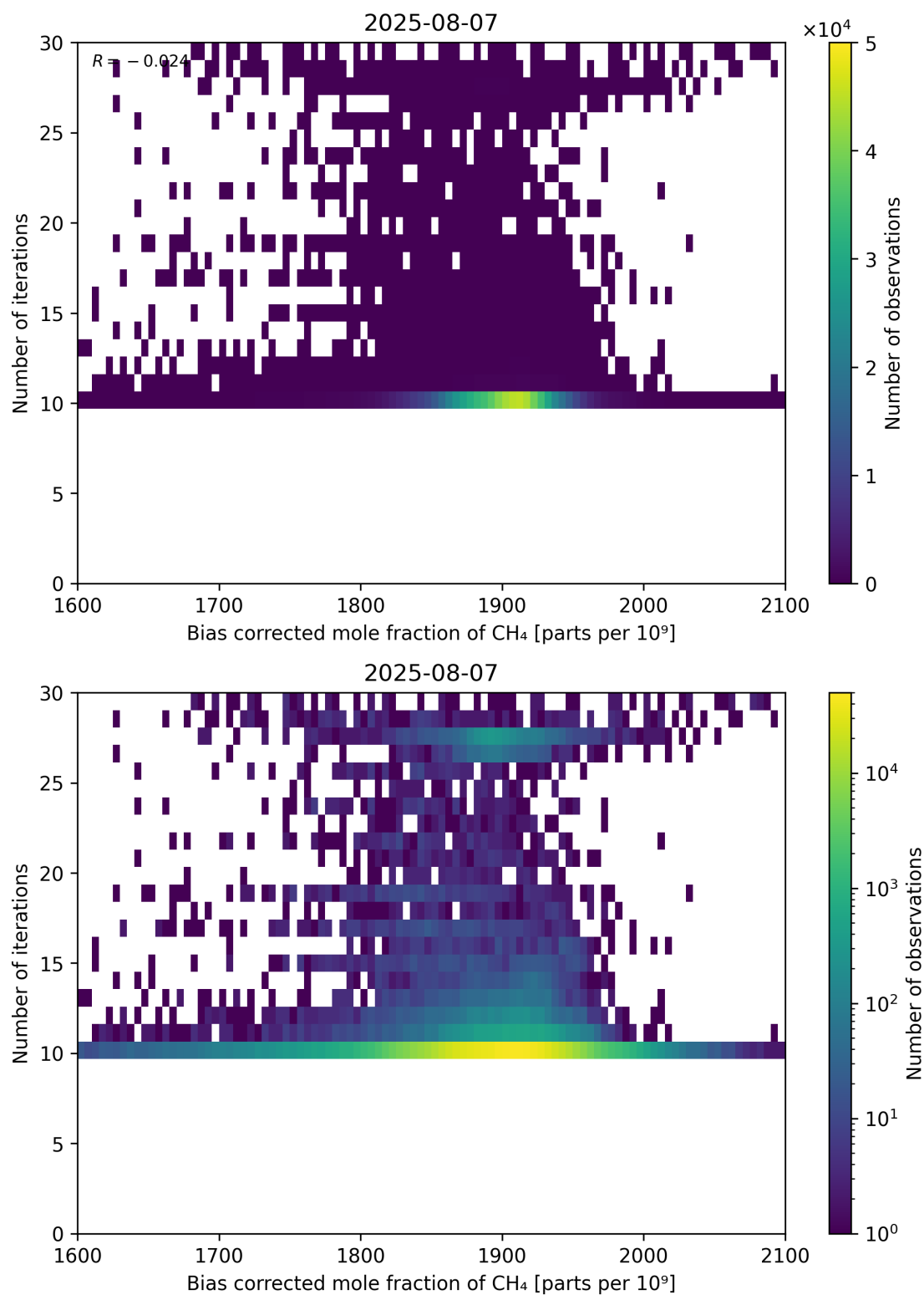
Figure 67: Scatter density plot of “Bias corrected mole fraction of CH 4 ” against “Number of iterations” for 2025-08-06 to 2025-08-08.
