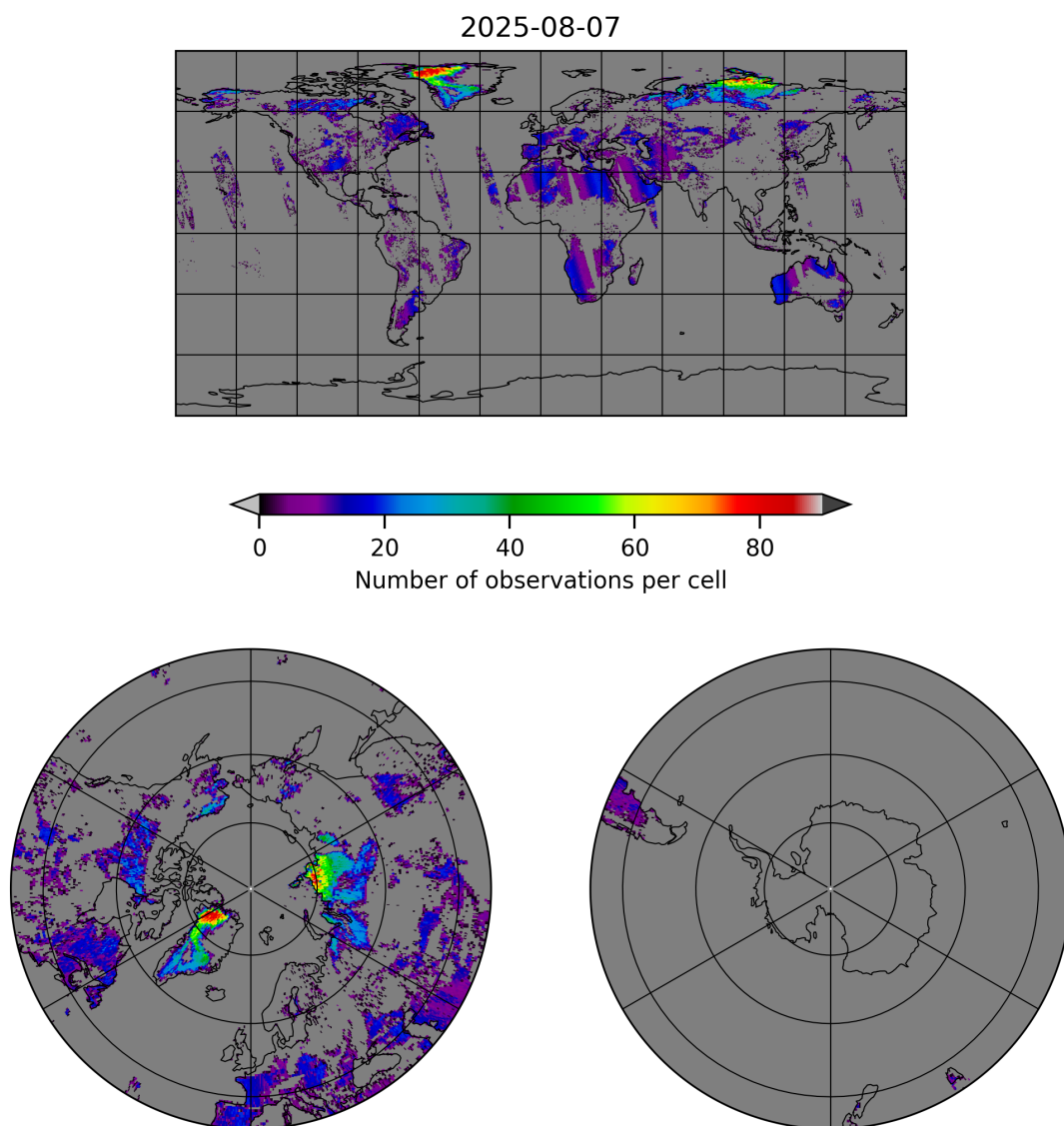
Figure 10: Map of the number of observations for 2025-08-06 to 2025-08-08
