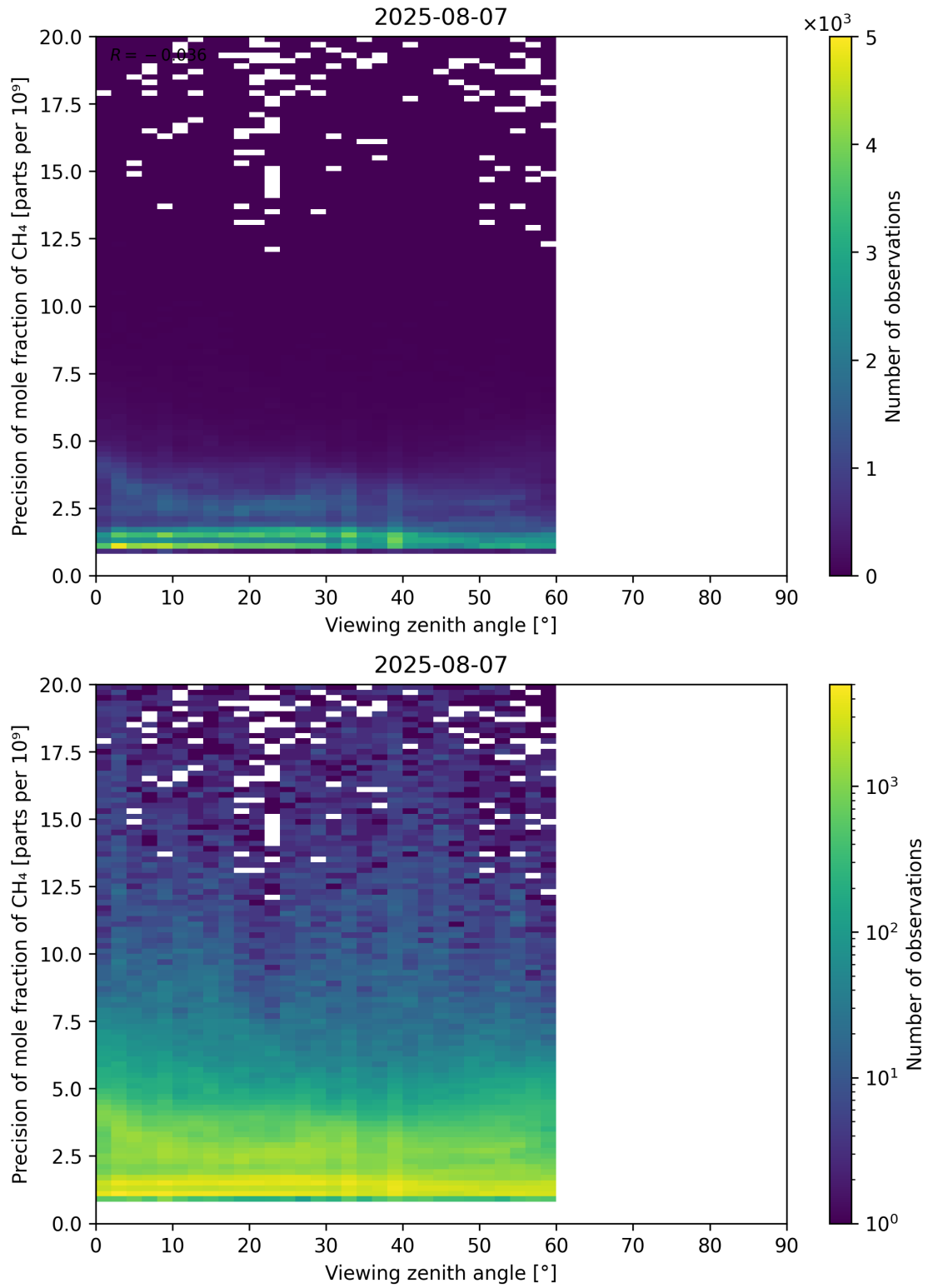
Figure 112: Scatter density plot of “Viewing zenith angle” against “Precision of mole fraction of CH 4 ” for 2025-08-06 to 2025-08-08.
