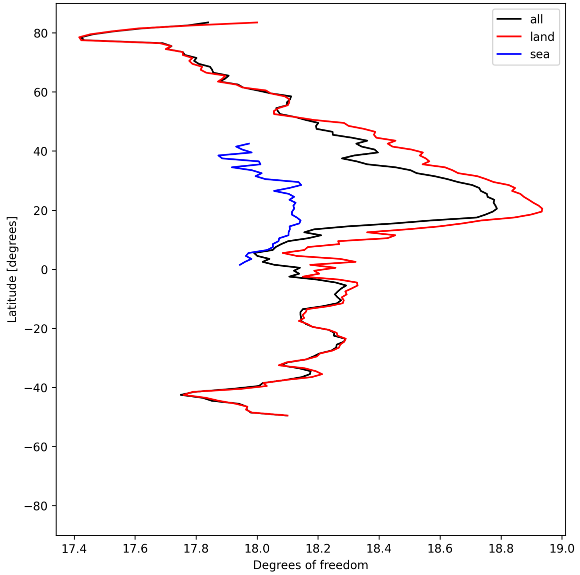
Figure 19: Zonal average of “Degrees of freedom” for 2025-08-06 to 2025-08-08.
