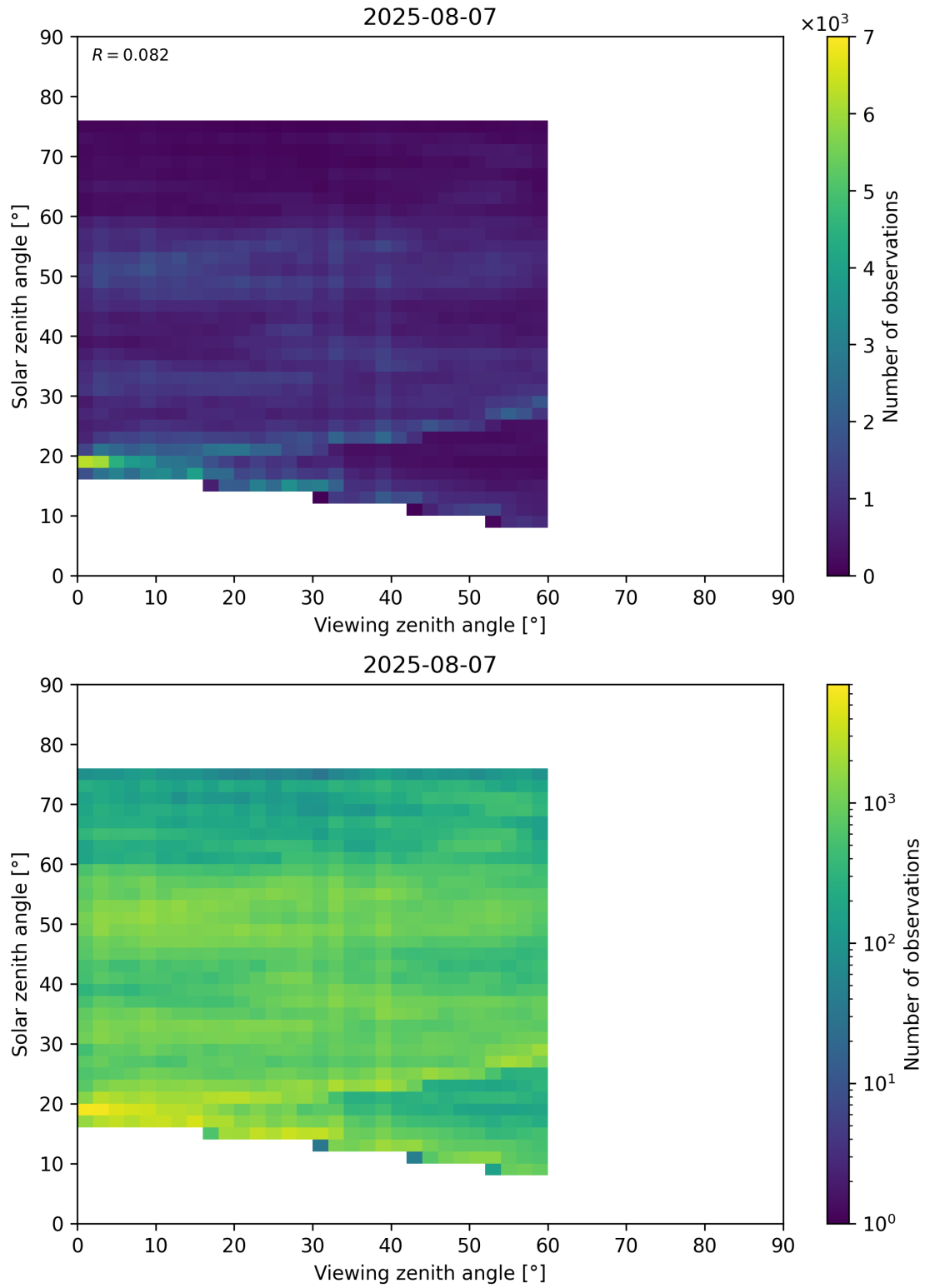
Figure 115: Scatter density plot of “Viewing zenith angle” against “Solar zenith angle” for 2025-08-06 to 2025-08-08.
