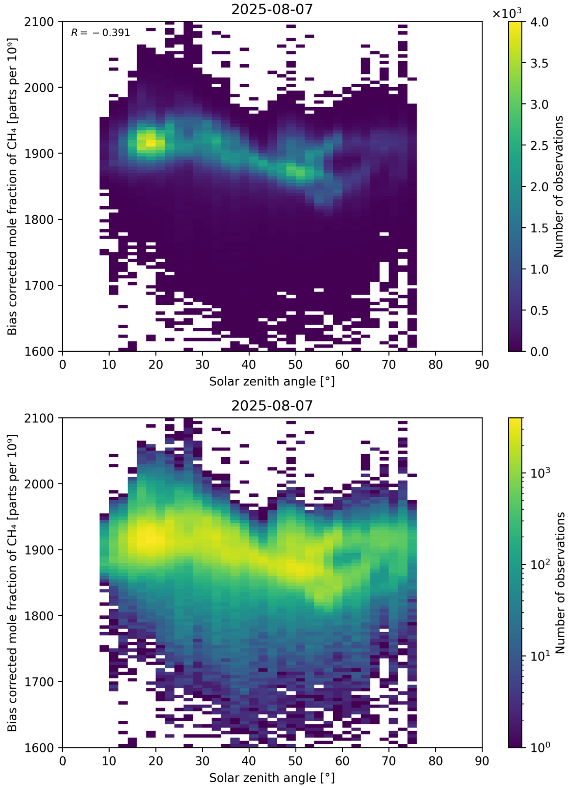
Figure 100: Scatter density plot of “Solar zenith angle” against “Bias corrected mole fraction of \text{CH}_4 ” for 2025-08-06 to 2025-08-08.
