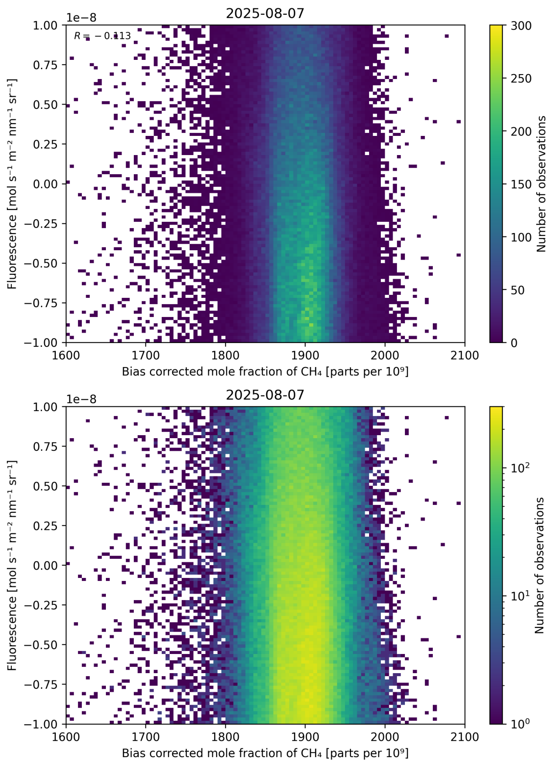
Figure 66: Scatter density plot of “Bias corrected mole fraction of \text{CH}_4 ” against “Fluorescence” for 2025-08-06 to 2025-08-08.
