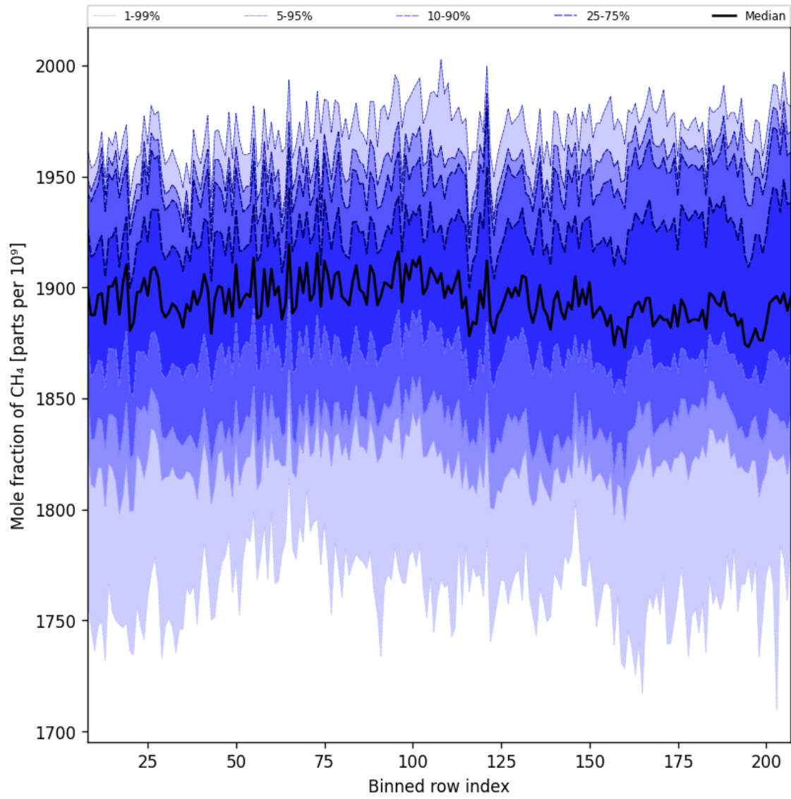
Figure 34: Along track statistics of “Mole fraction of CH 4 ” for 2025-08-06 to 2025-08-08
