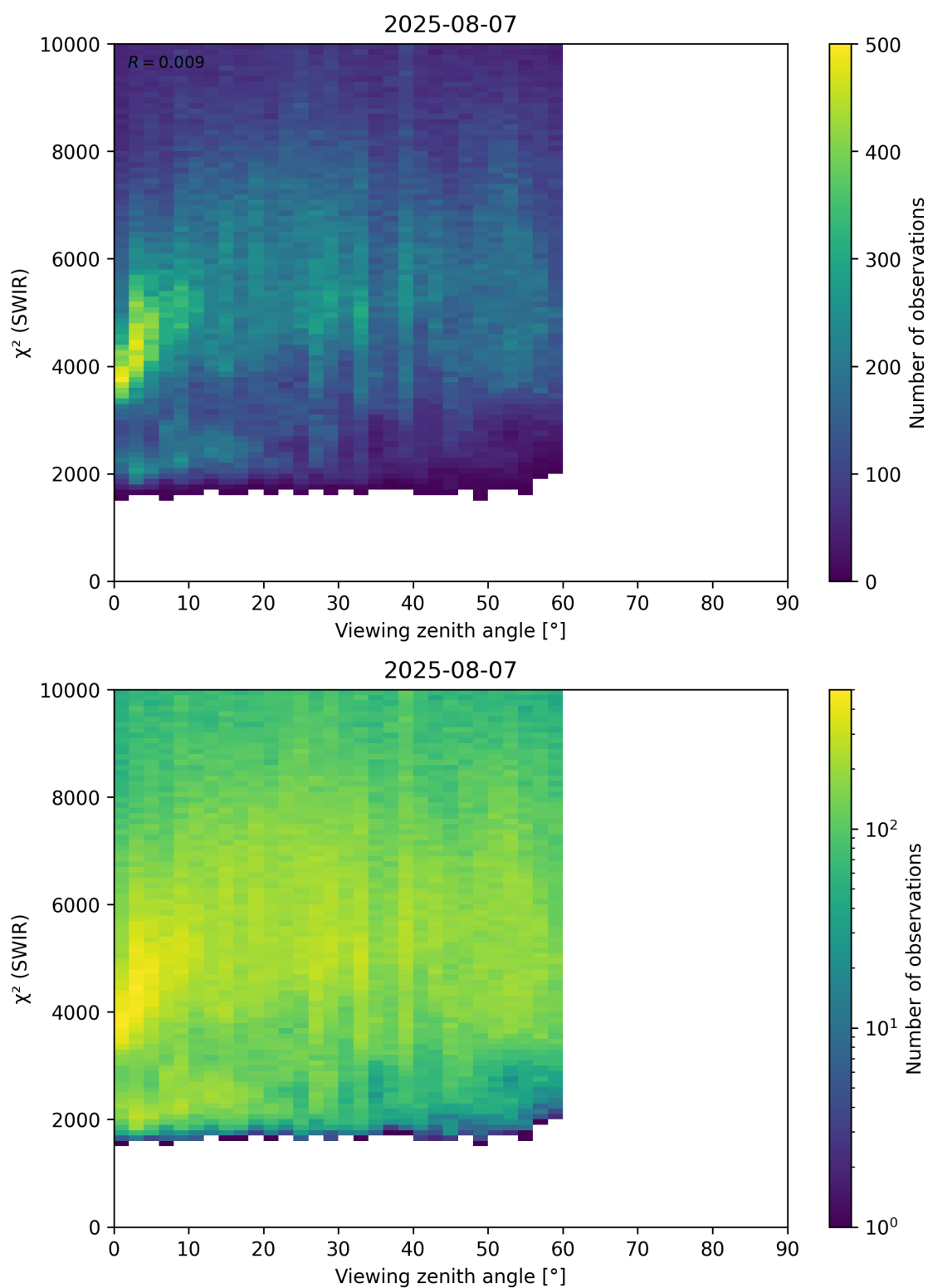
Figure 106: Scatter density plot of “Viewing zenith angle” against “ \chi^2 (SWIR)” for 2025-08-06 to 2025-08-08.
