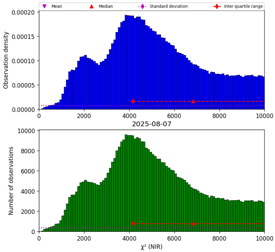
Figure 29: Histogram of " \chi^2 (NIR)" for 2025-08-06 to 2025-08-08
