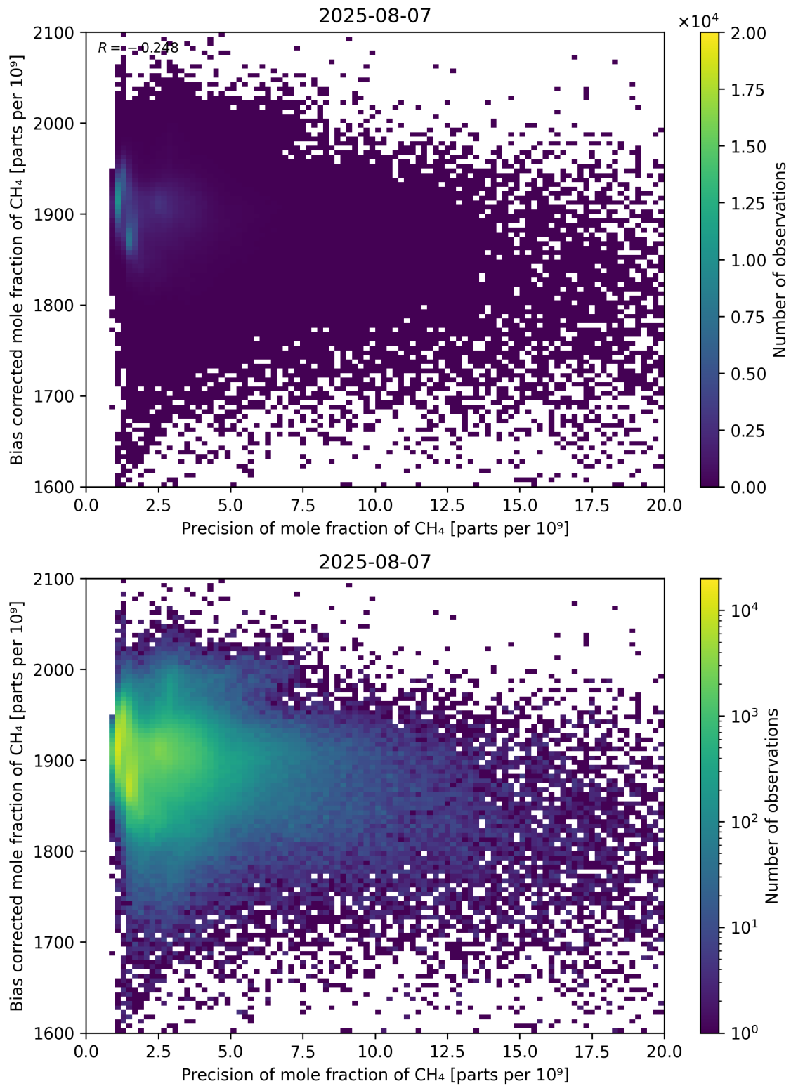
Figure 82: Scatter density plot of “Precision of mole fraction of CH 4 ” against “Bias corrected mole fraction of CH 4 ” for 2025-08-06 to 2025-08-08.
