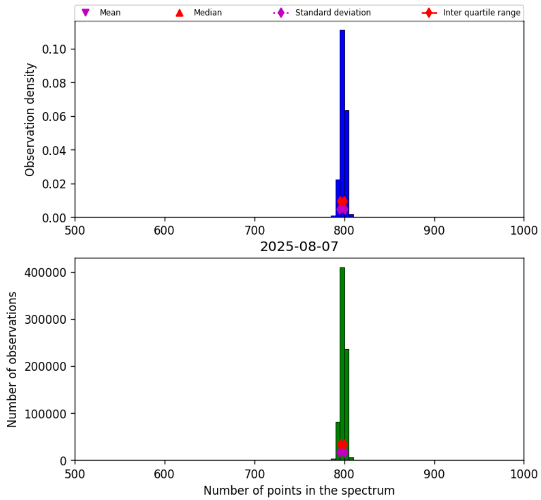
Figure 26: Histogram of “Number of points in the spectrum” for 2025-08-06 to 2025-08-08
