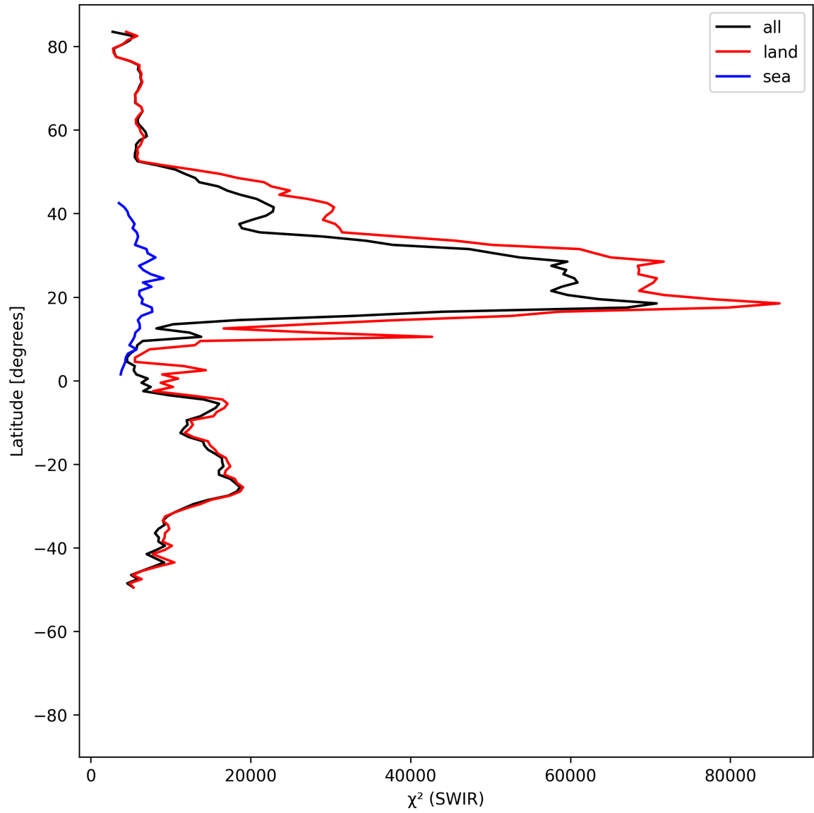
Figure 17: Zonal average of “ \chi^2 (SWIR)” for 2025-08-06 to 2025-08-08.
