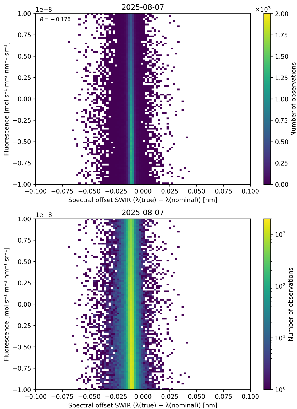
Figure 120: Scatter density plot of “Spectral offset SWIR ( \lambda_{\text{true}} - \lambda_{\text{nominal}} )” against “Fluorescence” for 2025-08-06 to 2025-08-08.
