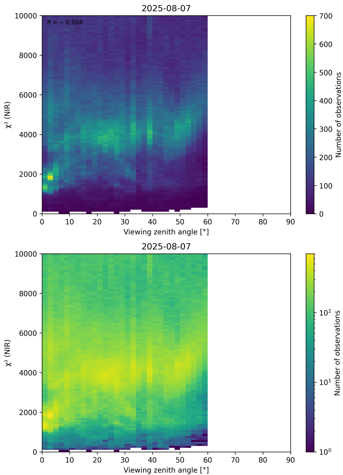
Figure 105: Scatter density plot of “Viewing zenith angle” against “ \chi^2 (NIR)” for 2025-08-06 to 2025-08-08.
