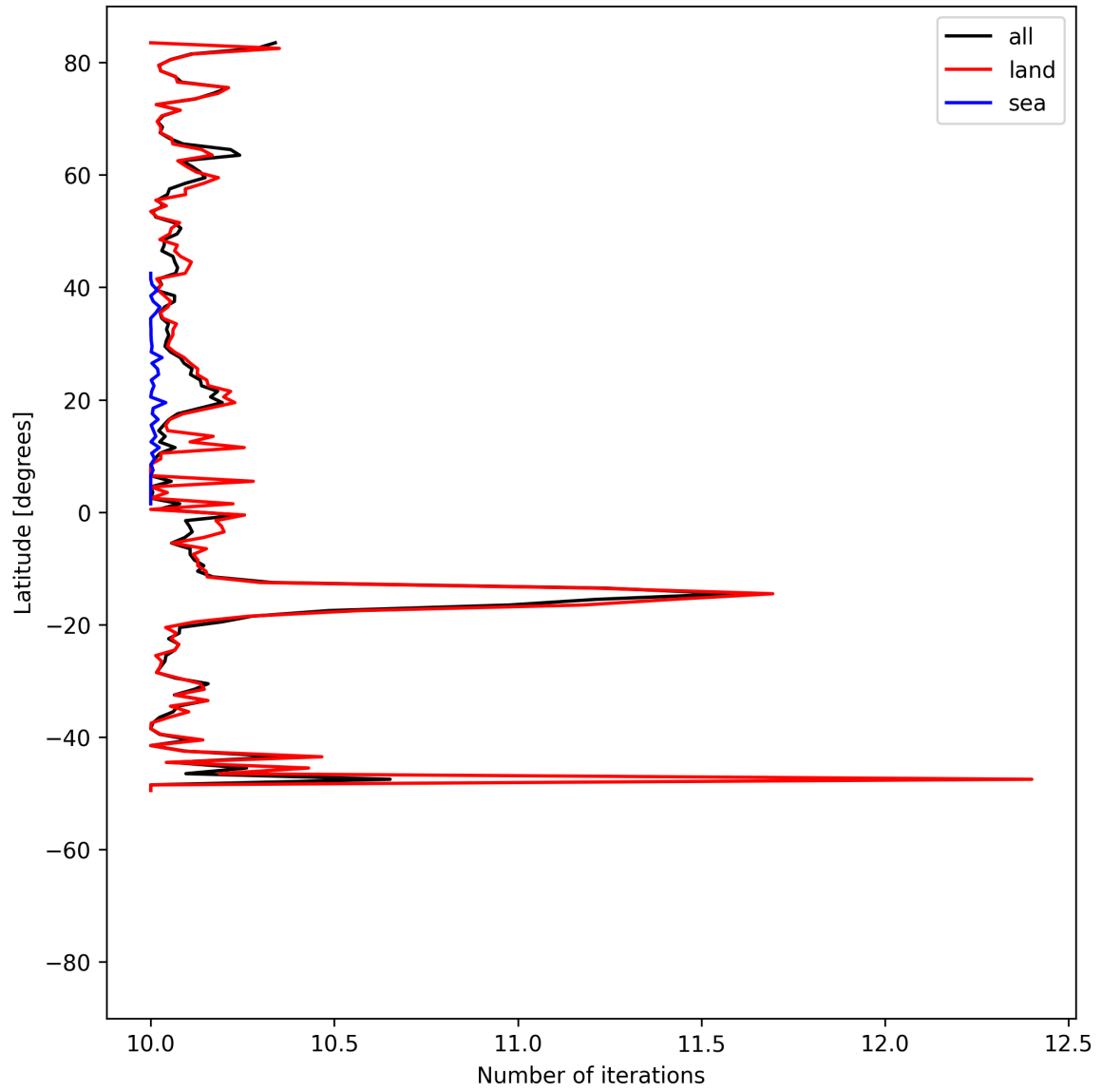
Figure 20: Zonal average of “Number of iterations” for 2025-08-06 to 2025-08-08.
