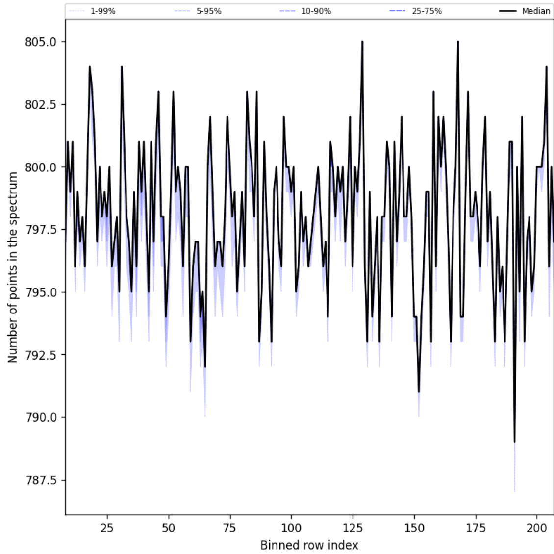
Figure 37: Along track statistics of “Number of points in the spectrum” for 2025-08-06 to 2025-08-08
