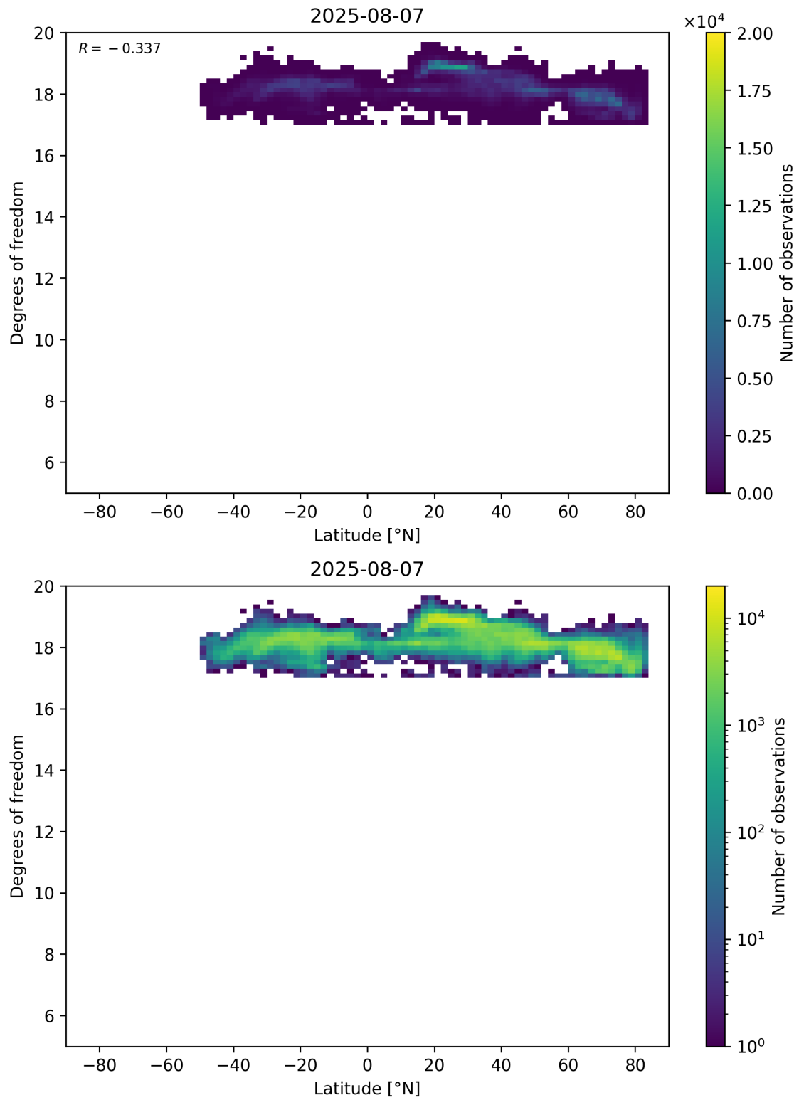
Figure 55: Scatter density plot of “Latitude” against “Degrees of freedom” for 2025-08-06 to 2025-08-08.
