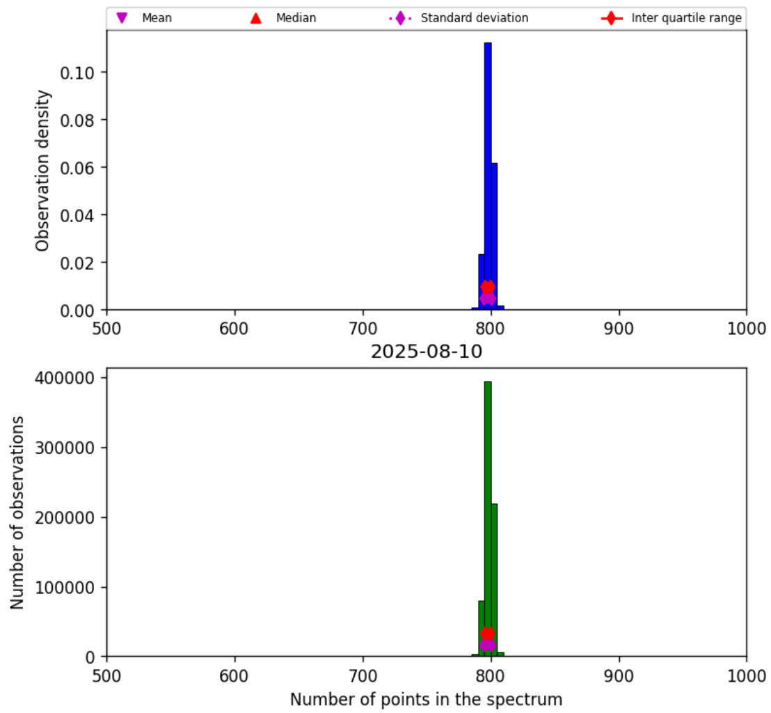
Figure 26: Histogram of “Number of points in the spectrum” for 2025-08-09 to 2025-08-11
