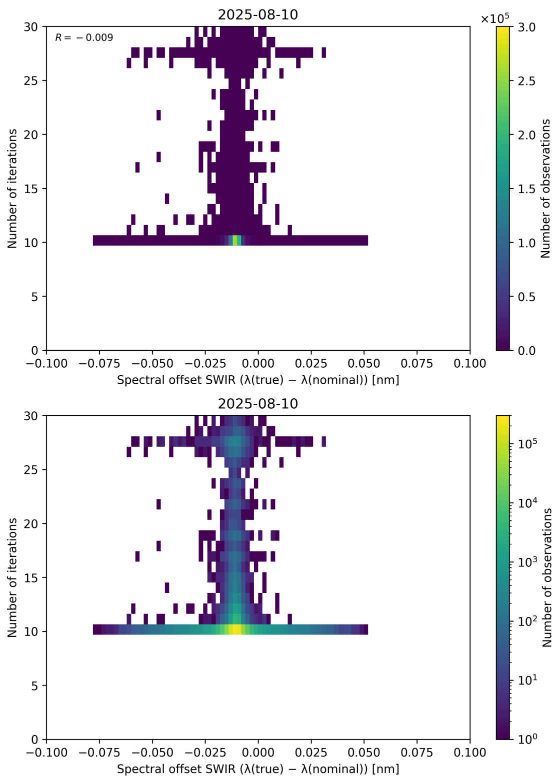
Figure 121: Scatter density plot of “Spectral offset SWIR ( \lambda_{\text{true}} - \lambda_{\text{nominal}} )” against “Number of iterations” for 2025-08-09 to 2025-08-11.
