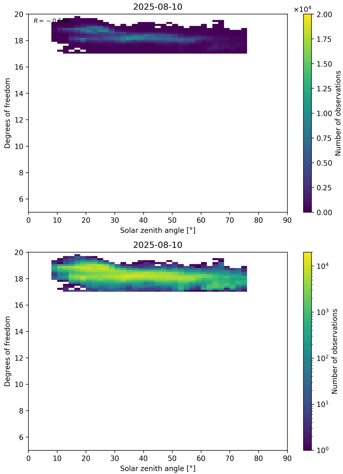
Figure 96: Scatter density plot of “Solar zenith angle” against “Degrees of freedom” for 2025-08-09 to 2025-08-11.
