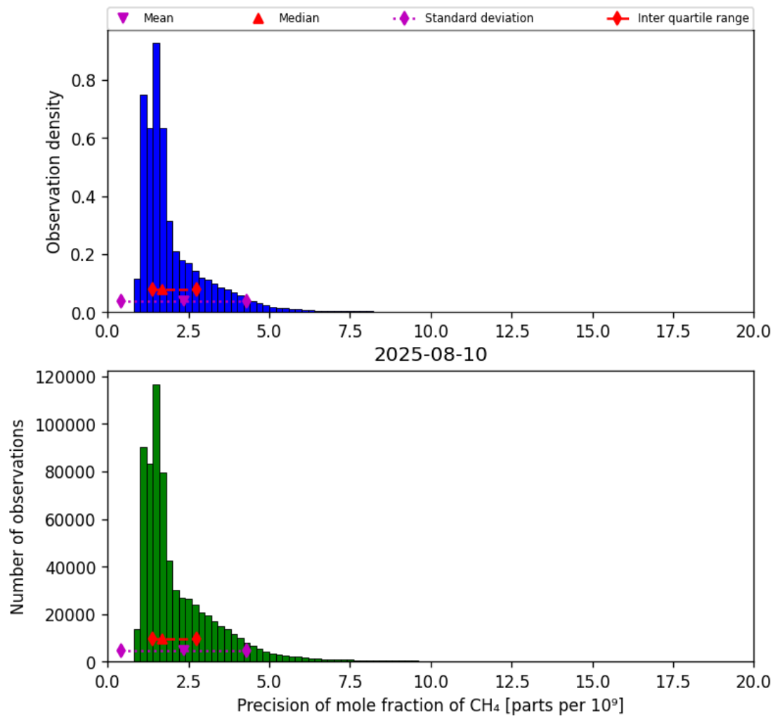
Figure 24: Histogram of “Precision of mole fraction of CH 4 ” for 2025-08-09 to 2025-08-11
