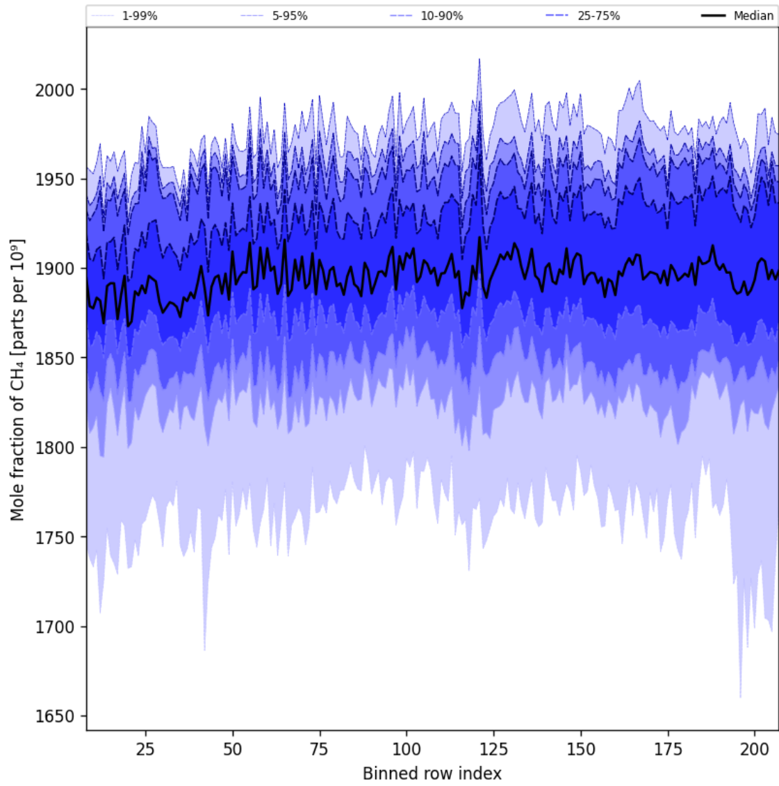
Figure 34: Along track statistics of “Mole fraction of CH 4 ” for 2025-08-09 to 2025-08-11
