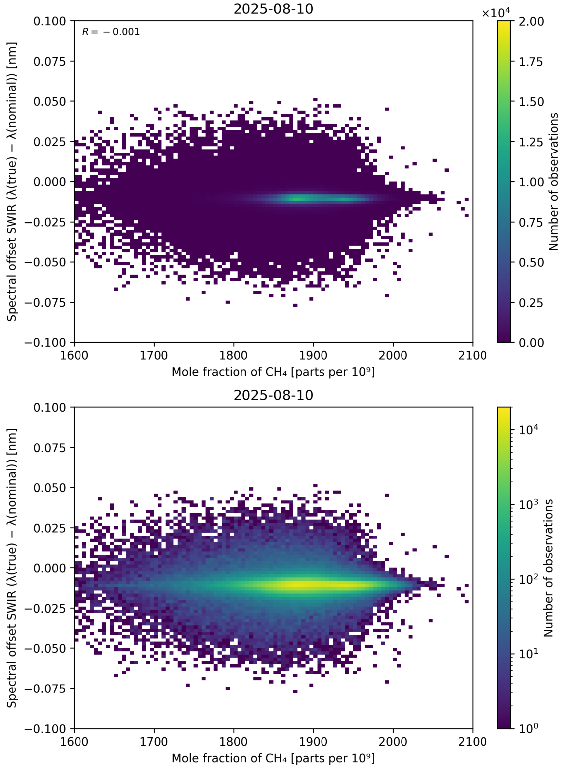
Figure 86: Scatter density plot of “Mole fraction of CH 4 ” against “Spectral offset SWIR ( \lambda_{\text{true}} - \lambda_{\text{nominal}} )” for 2025-08-09 to 2025-08-11.
