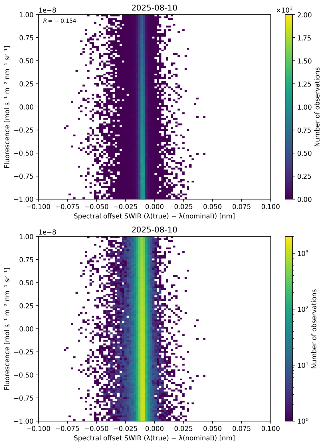
Figure 120: Scatter density plot of “Spectral offset SWIR ( \lambda_{\text{true}} - \lambda_{\text{nominal}} )” against “Fluorescence” for 2025-08-09 to 2025-08-11.
