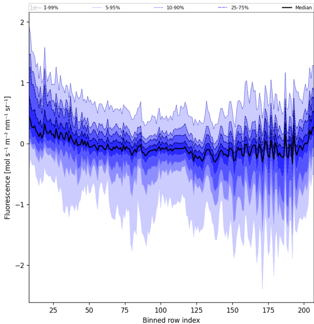
Figure 43: Along track statistics of "Fluorescence" for 2025-08-09 to 2025-08-11
