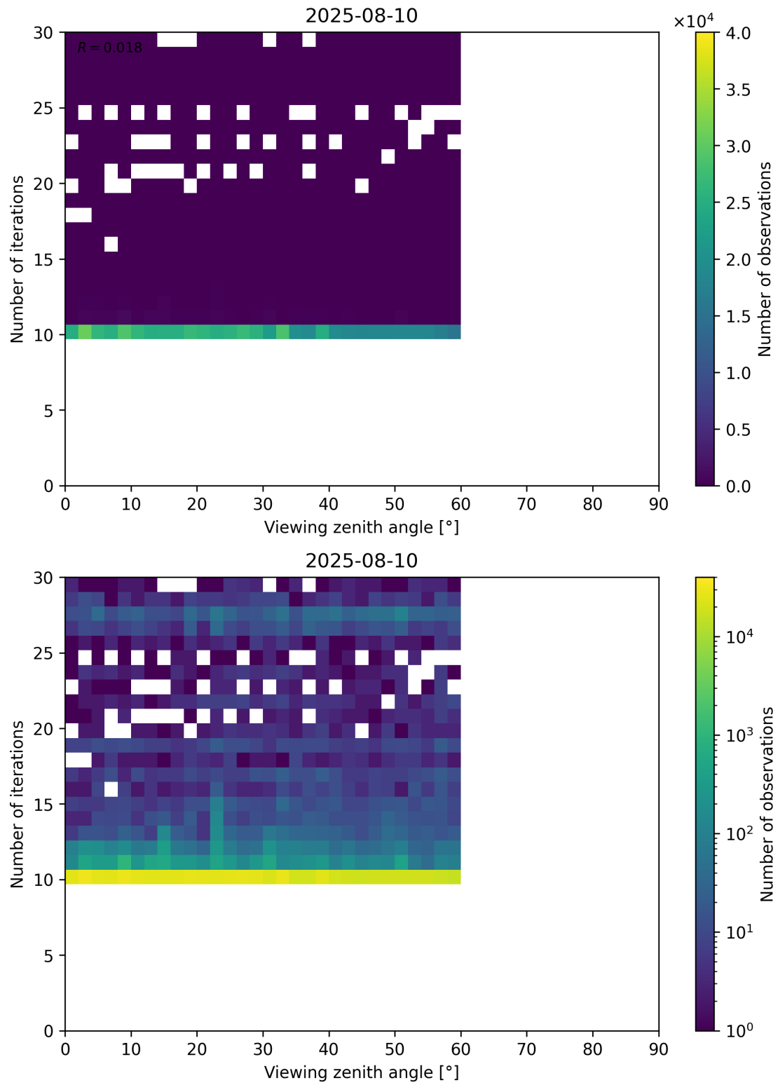
Figure 113: Scatter density plot of “Viewing zenith angle” against “Number of iterations” for 2025-08-09 to 2025-08-11.
