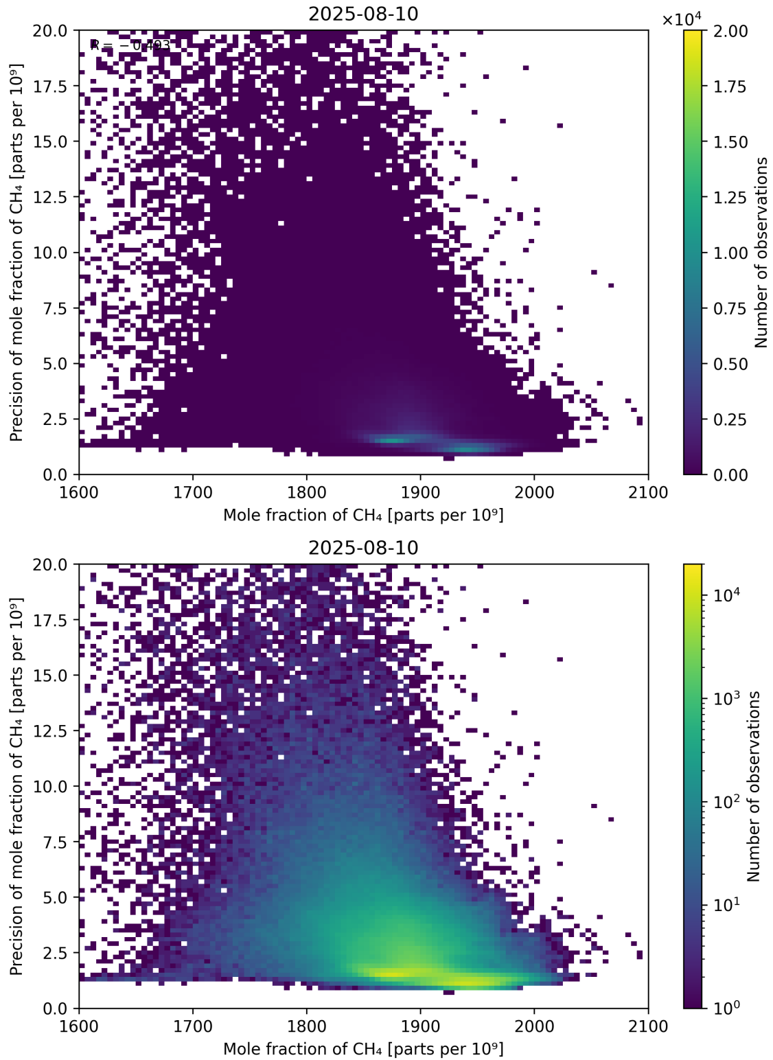
Figure 75: Scatter density plot of “Mole fraction of CH 4 ” against “Precision of mole fraction of CH 4 ” for 2025-08-09 to 2025-08-11.
