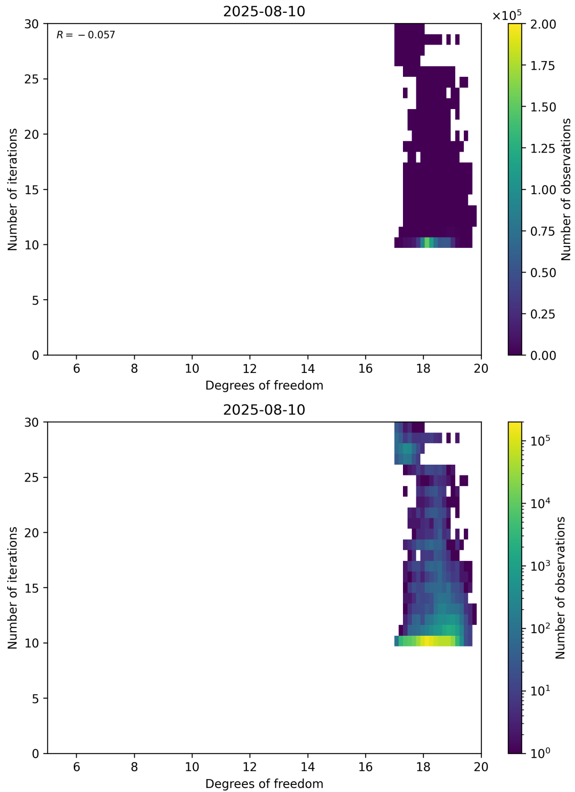
Figure 52: Scatter density plot of “Degrees of freedom” against “Number of iterations” for 2025-08-09 to 2025-08-11.
