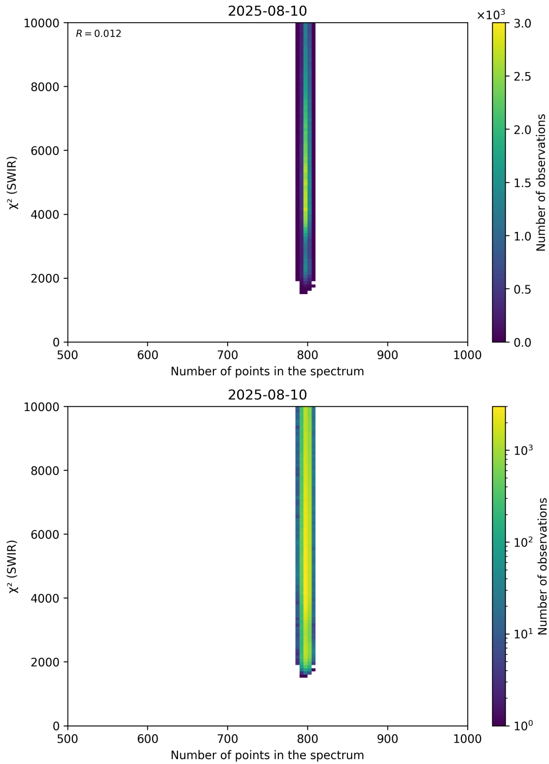
Figure 89: Scatter density plot of “Number of points in the spectrum” against “ \chi^2 (SWIR)” for 2025-08-09 to 2025-08-11.
