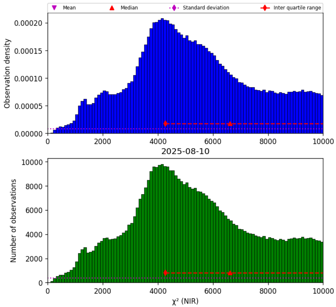
Figure 29: Histogram of " \chi^2 (NIR)" for 2025-08-09 to 2025-08-11
