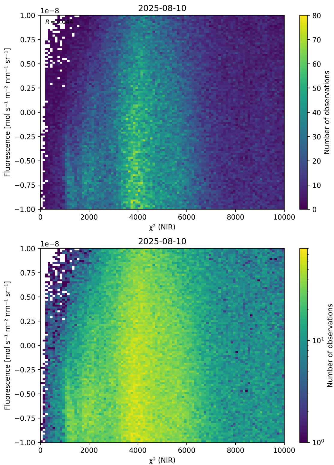
Figure 45: Scatter density plot of “ \chi^2 (NIR)” against “Fluorescence” for 2025-08-09 to 2025-08-11.
