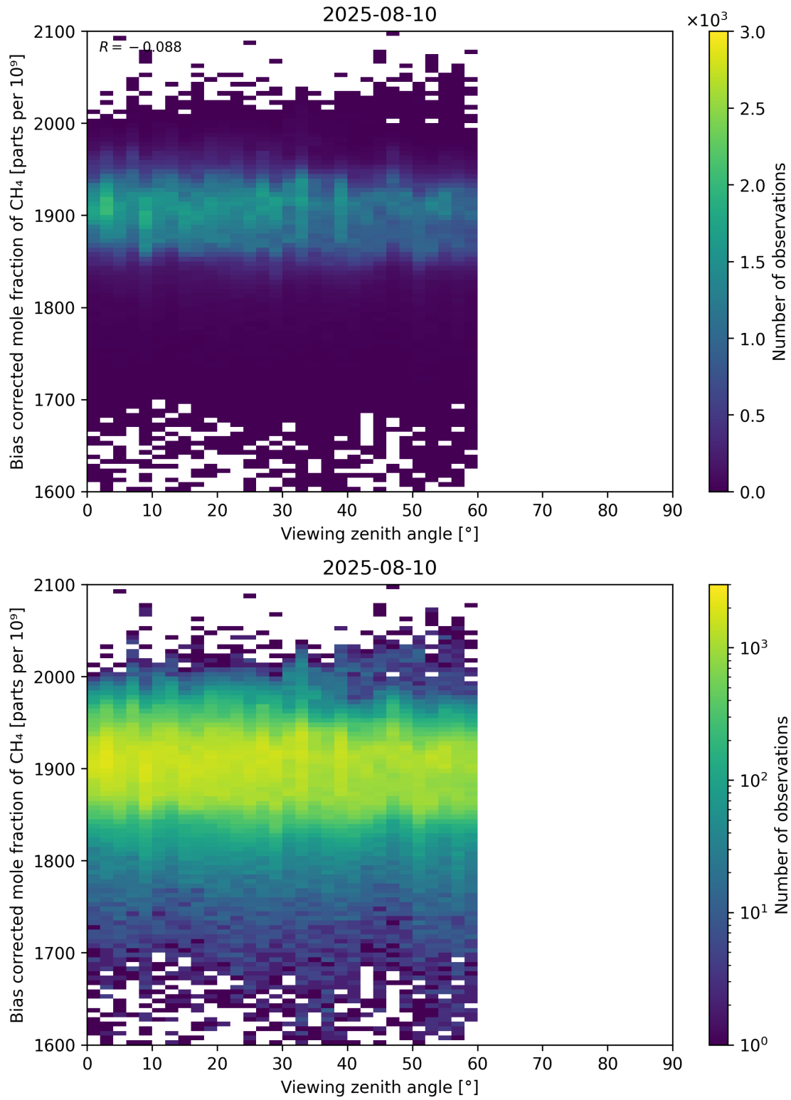
Figure 111: Scatter density plot of “Viewing zenith angle” against “Bias corrected mole fraction of CH 4 ” for 2025-08-09 to 2025-08-11.
