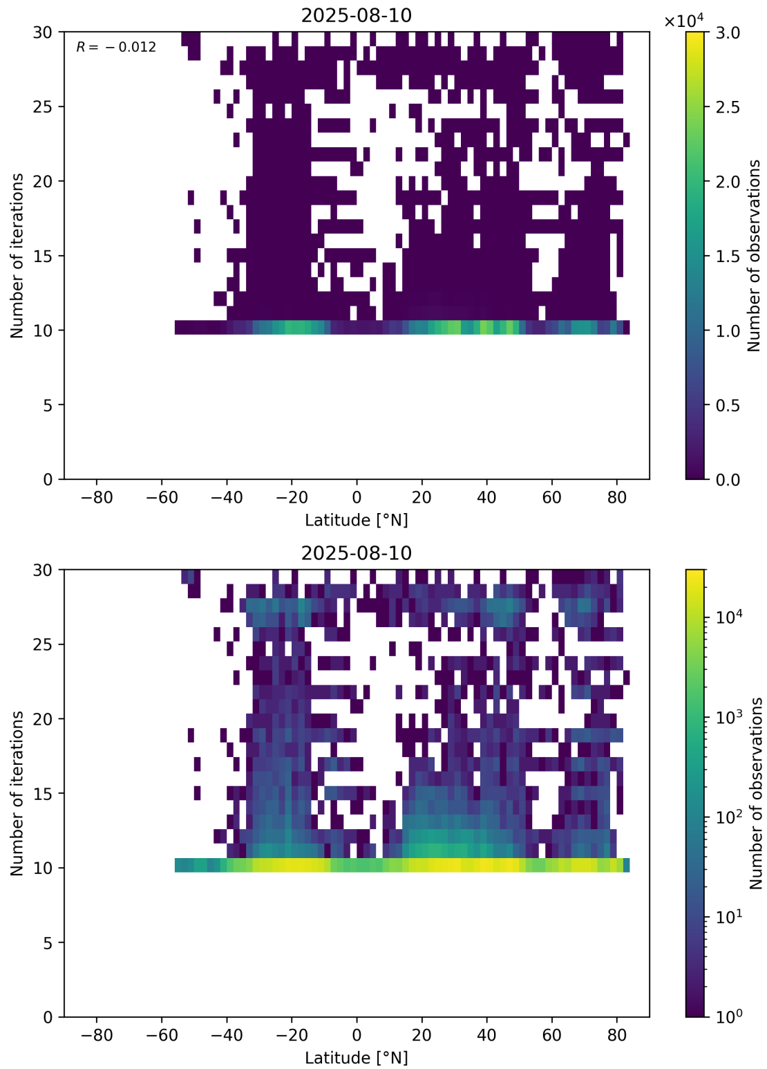
Figure 60: Scatter density plot of “Latitude” against “Number of iterations” for 2025-08-09 to 2025-08-11.
