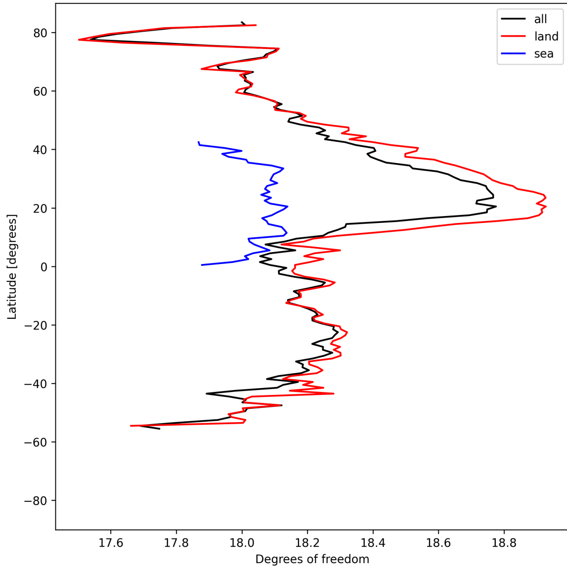
Figure 19: Zonal average of “Degrees of freedom” for 2025-08-09 to 2025-08-11.
