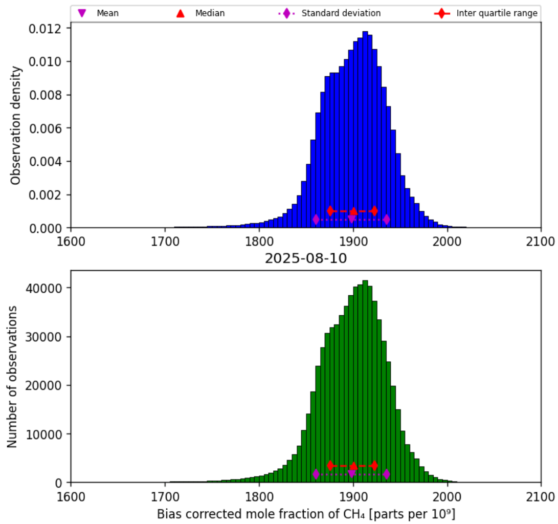
Figure 25: Histogram of “Bias corrected mole fraction of CH 4 ” for 2025-08-09 to 2025-08-11
