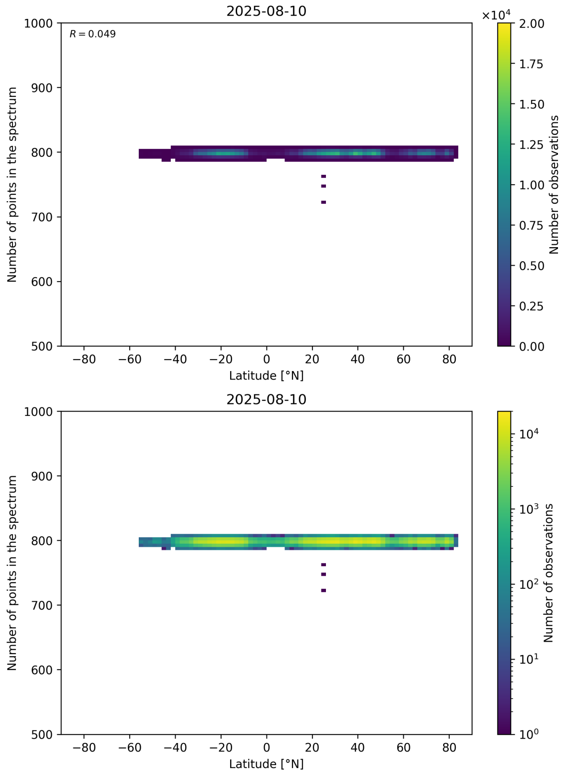
Figure 61: Scatter density plot of “Latitude” against “Number of points in the spectrum” for 2025-08-09 to 2025-08-11.
