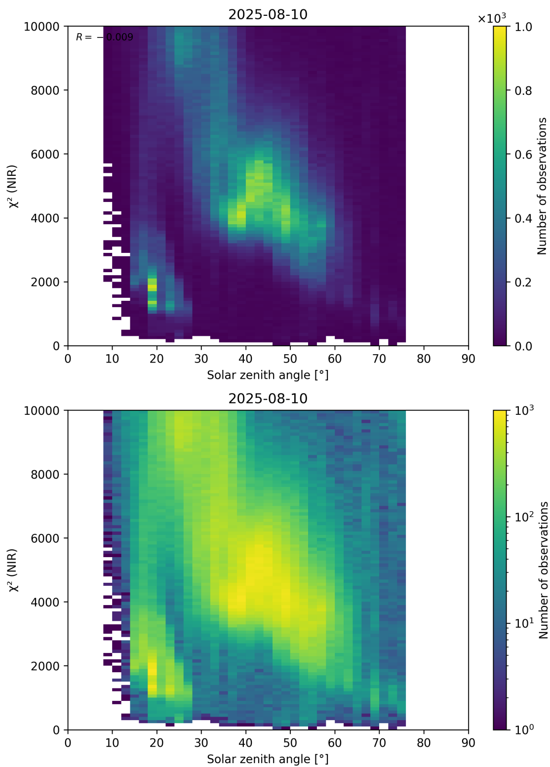
Figure 94: Scatter density plot of “Solar zenith angle” against “ \chi^2 (NIR)” for 2025-08-09 to 2025-08-11.
