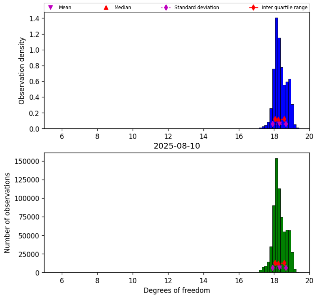
Figure 30: Histogram of “Degrees of freedom” for 2025-08-09 to 2025-08-11
