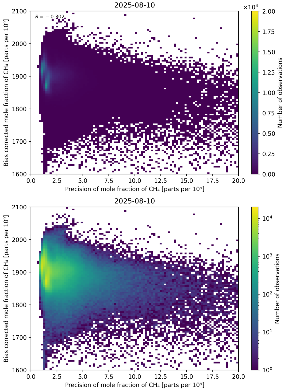
Figure 82: Scatter density plot of “Precision of mole fraction of CH 4 ” against “Bias corrected mole fraction of CH 4 ” for 2025-08-09 to 2025-08-11.
