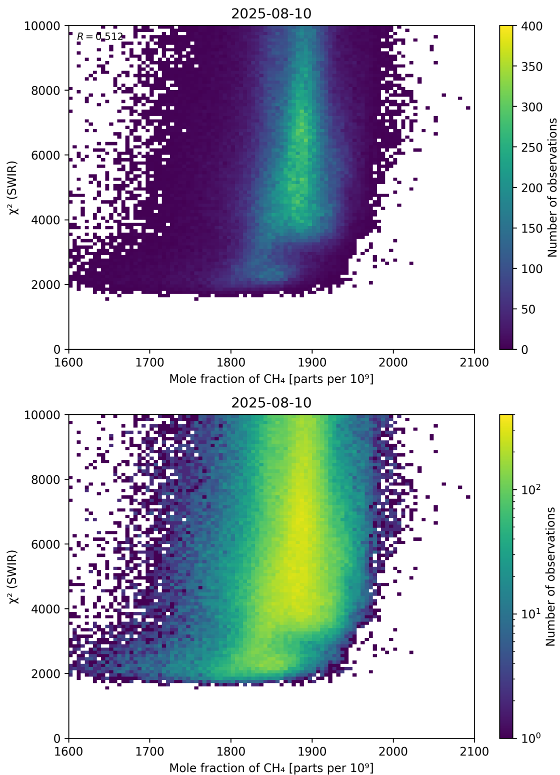
Figure 71: Scatter density plot of “Mole fraction of CH 4 ” against “ \chi^2 (SWIR)” for 2025-08-09 to 2025-08-11.
