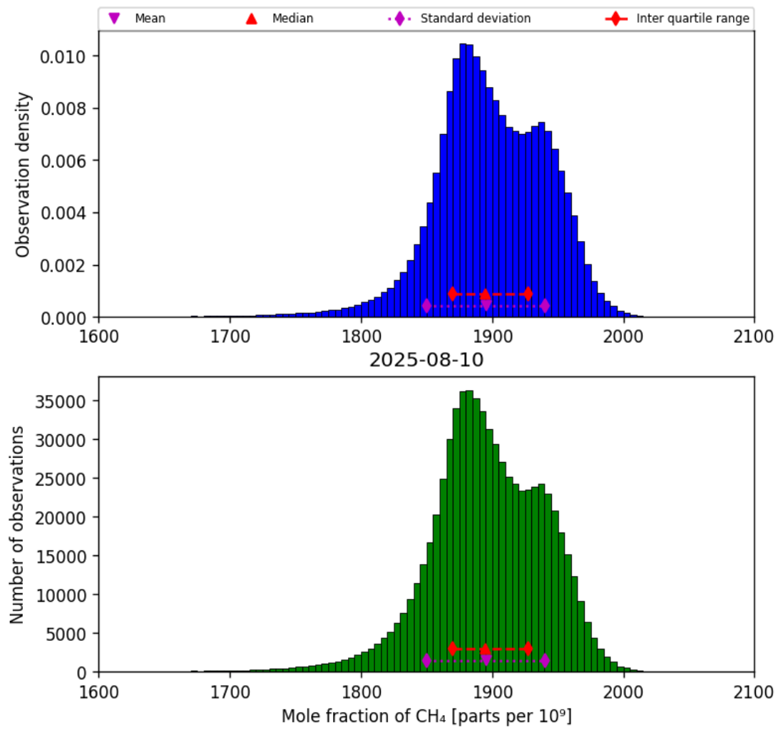
Figure 23: Histogram of “Mole fraction of CH 4 ” for 2025-08-09 to 2025-08-11
