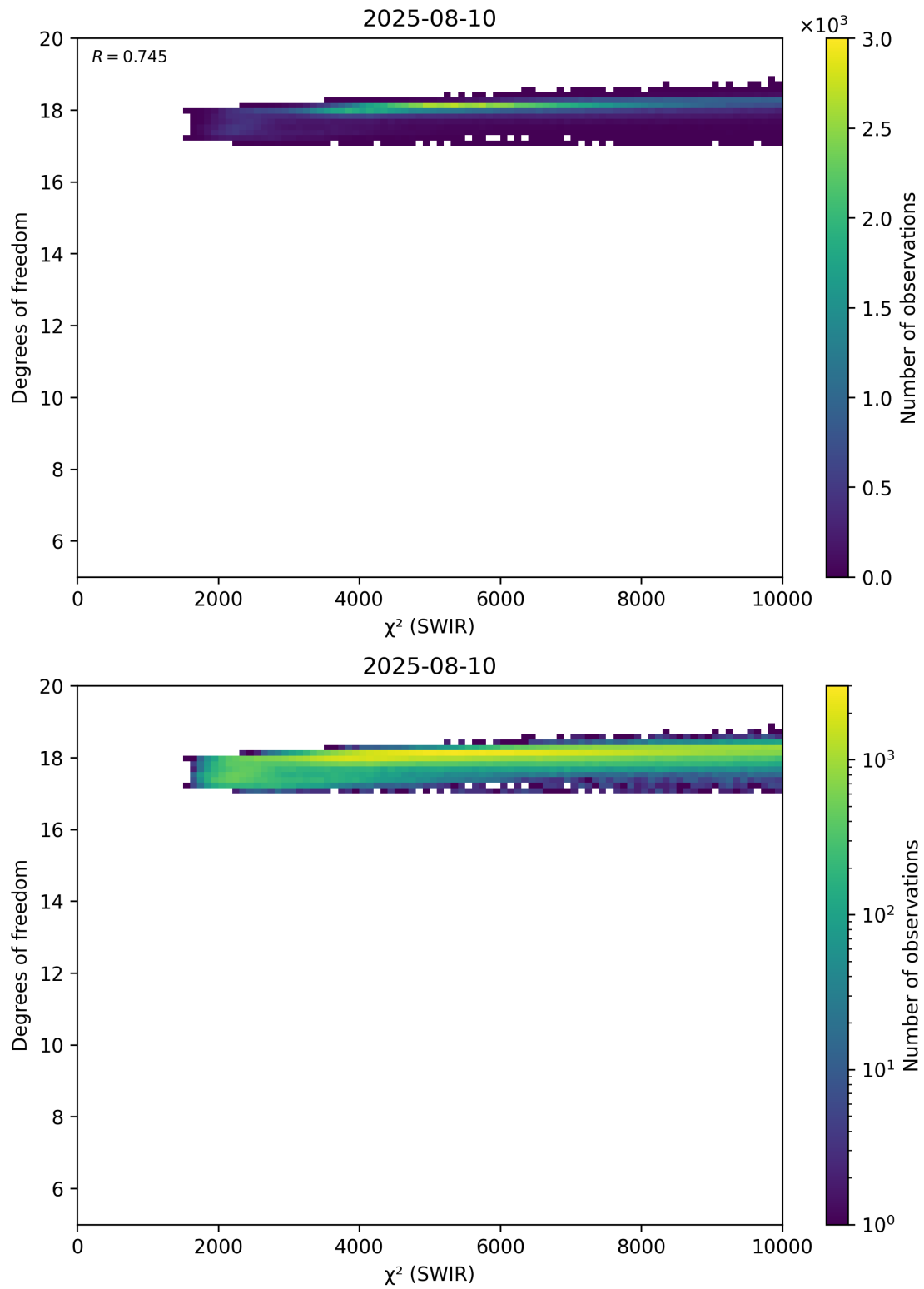
Figure 48: Scatter density plot of “ \chi^2 (SWIR)” against “Degrees of freedom” for 2025-08-09 to 2025-08-11.
