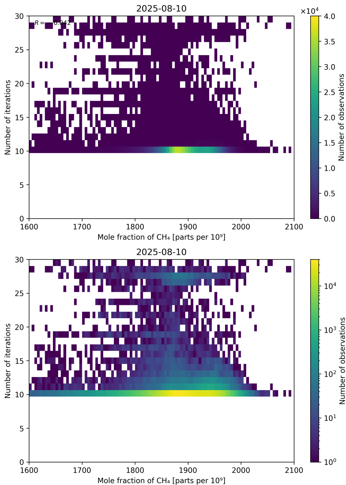
Figure 76: Scatter density plot of “Mole fraction of CH 4 ” against “Number of iterations” for 2025-08-09 to 2025-08-11.
