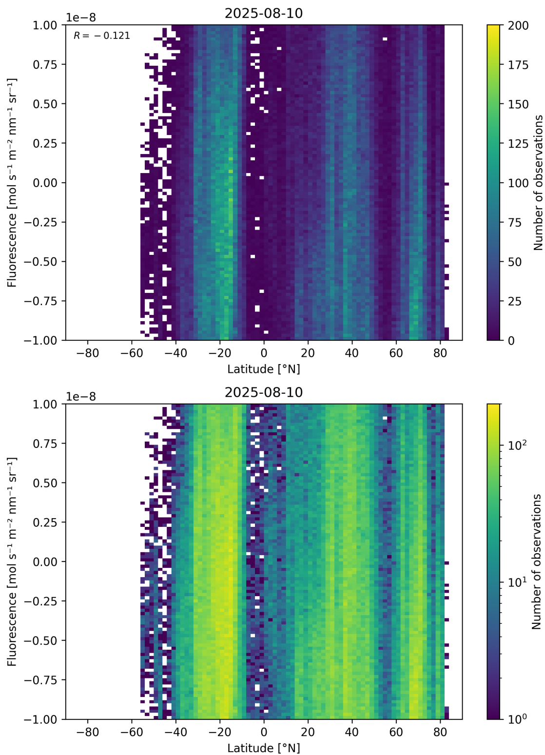
Figure 56: Scatter density plot of “Latitude” against “Fluorescence” for 2025-08-09 to 2025-08-11.
