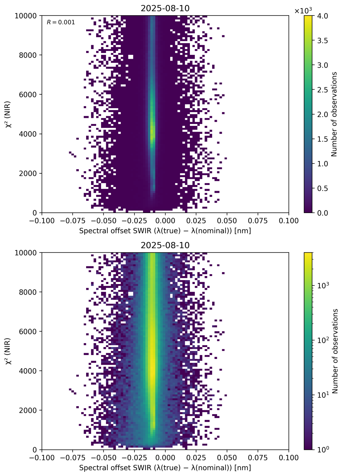
Figure 117: Scatter density plot of “Spectral offset SWIR ( \lambda_{\text{true}} - \lambda_{\text{nominal}} )” against “ \chi^2 (NIR)” for 2025-08-09 to 2025-08-11.
