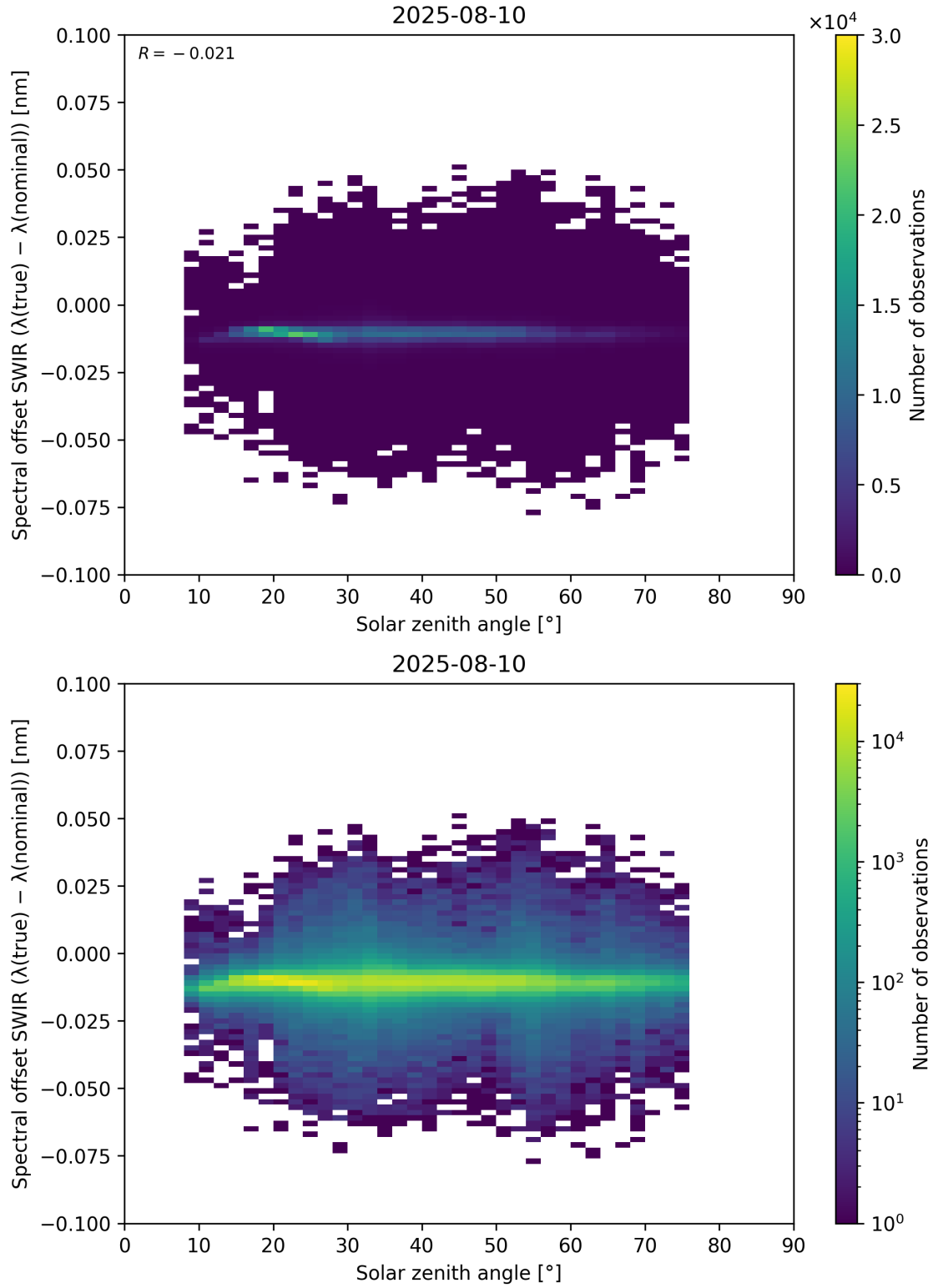
Figure 104: Scatter density plot of “Solar zenith angle” against “Spectral offset SWIR ( \lambda_{\text{true}} - \lambda_{\text{nominal}} )” for 2025-08-09 to 2025-08-11.
