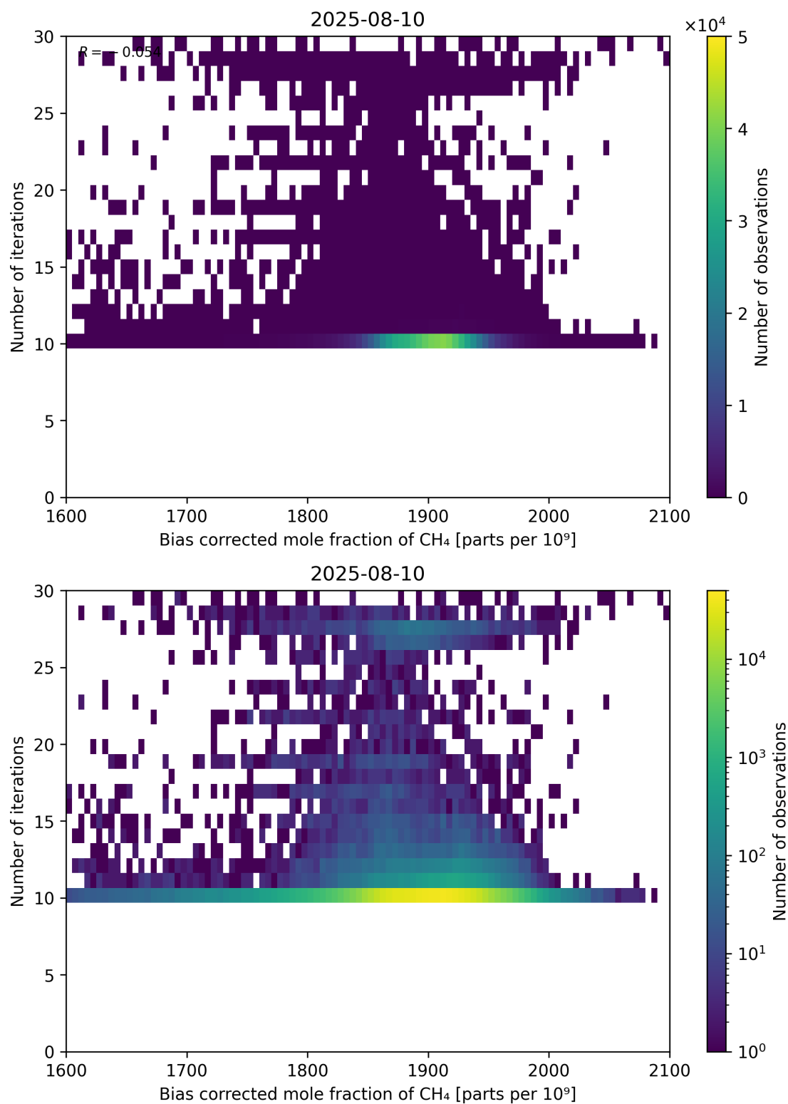
Figure 67: Scatter density plot of “Bias corrected mole fraction of CH 4 ” against “Number of iterations” for 2025-08-09 to 2025-08-11.
