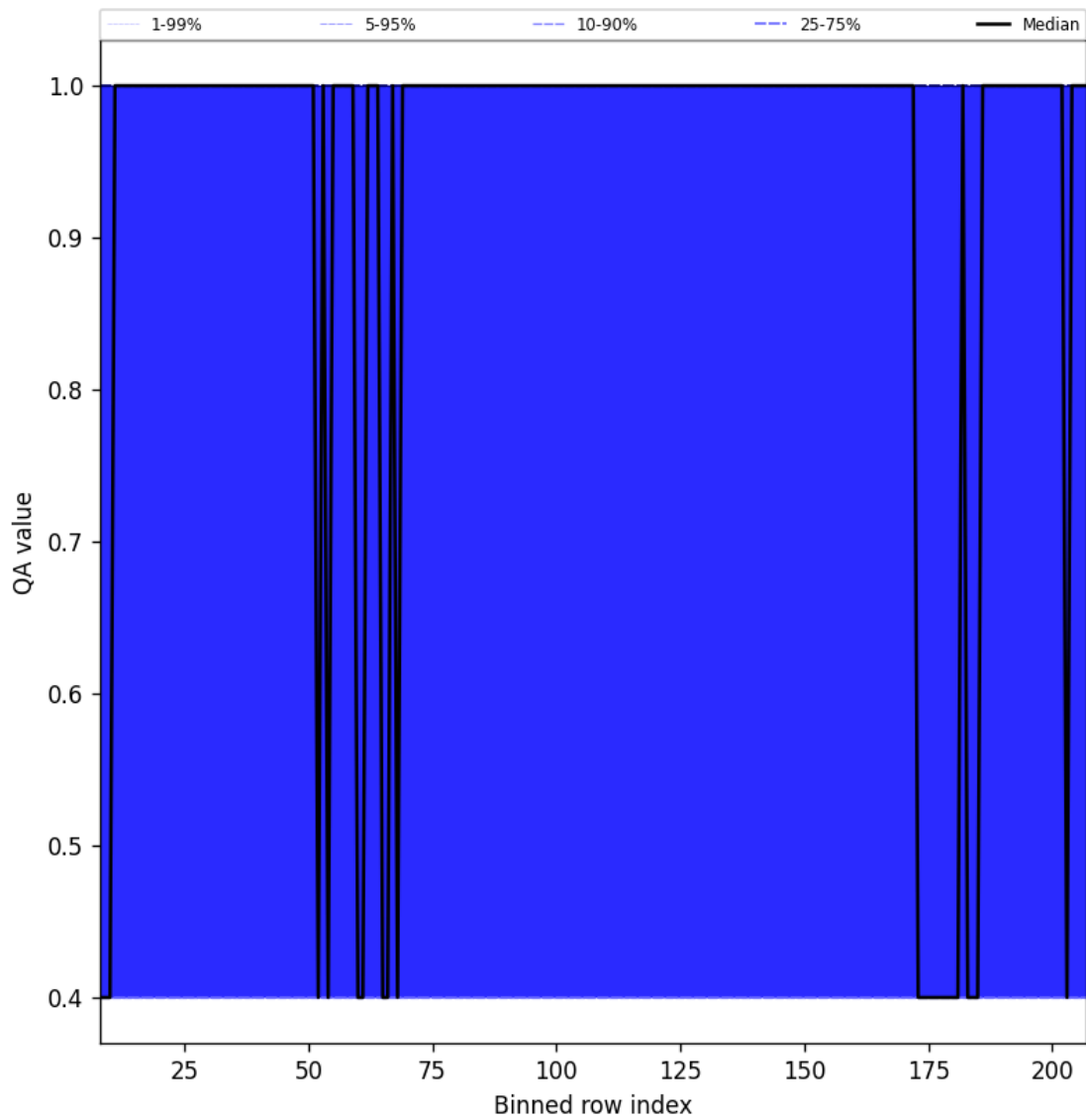
Figure 33: Along track statistics of “QA value” for 2025-08-09 to 2025-08-11
