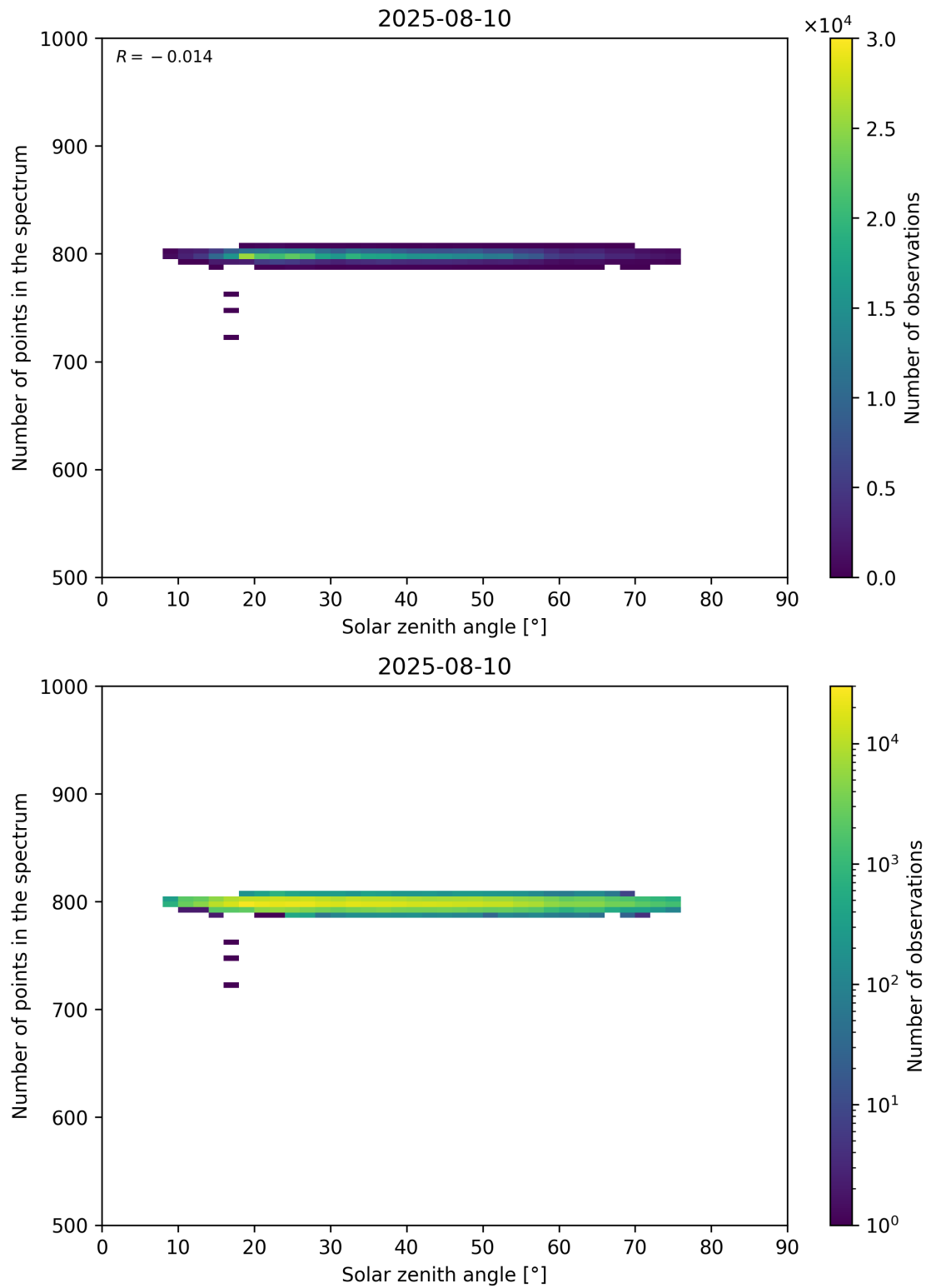
Figure 103: Scatter density plot of “Solar zenith angle” against “Number of points in the spectrum” for 2025-08-09 to 2025-08-11.
