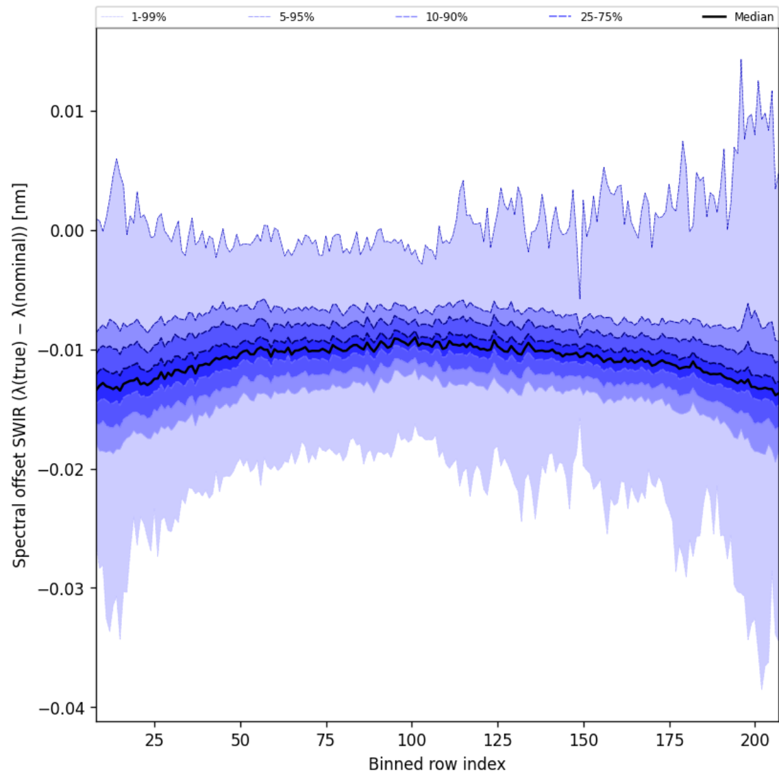
Figure 38: Along track statistics of “Spectral offset SWIR ( \lambda_{\text{true}} - \lambda_{\text{nominal}} )” for 2025-08-09 to 2025-08-11
