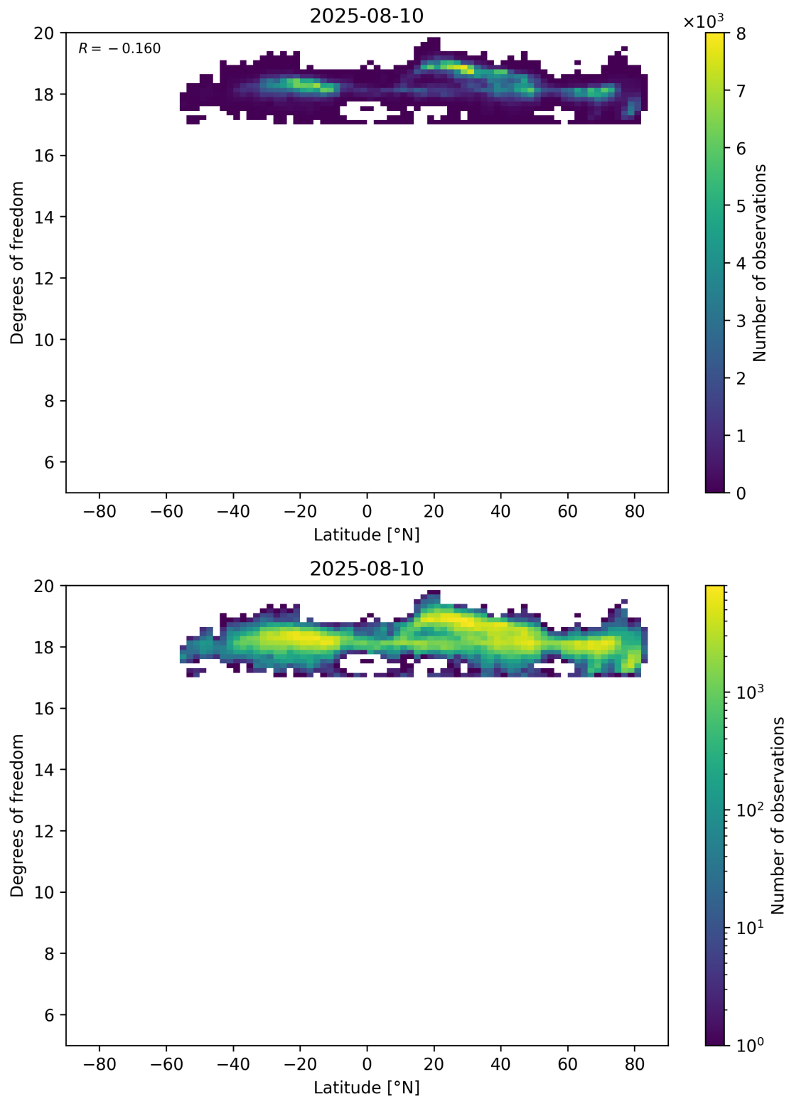
Figure 55: Scatter density plot of “Latitude” against “Degrees of freedom” for 2025-08-09 to 2025-08-11.
