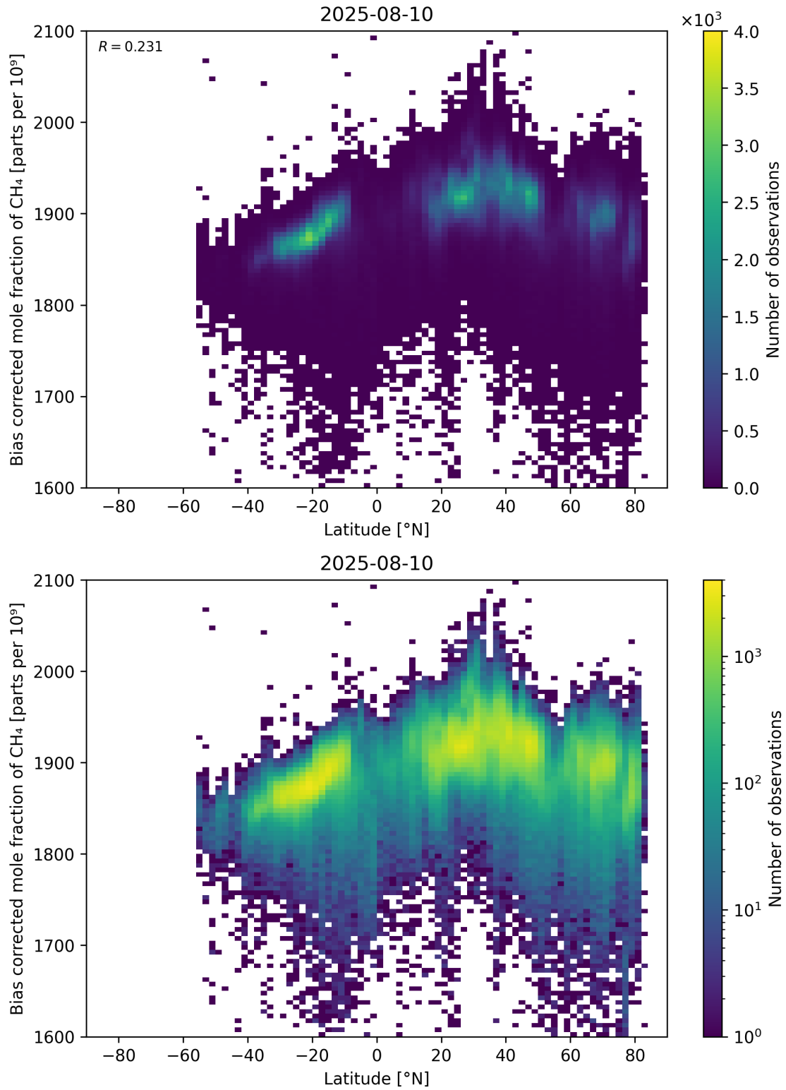
Figure 58: Scatter density plot of “Latitude” against “Bias corrected mole fraction of \text{CH}_4 ” for 2025-08-09 to 2025-08-11.
