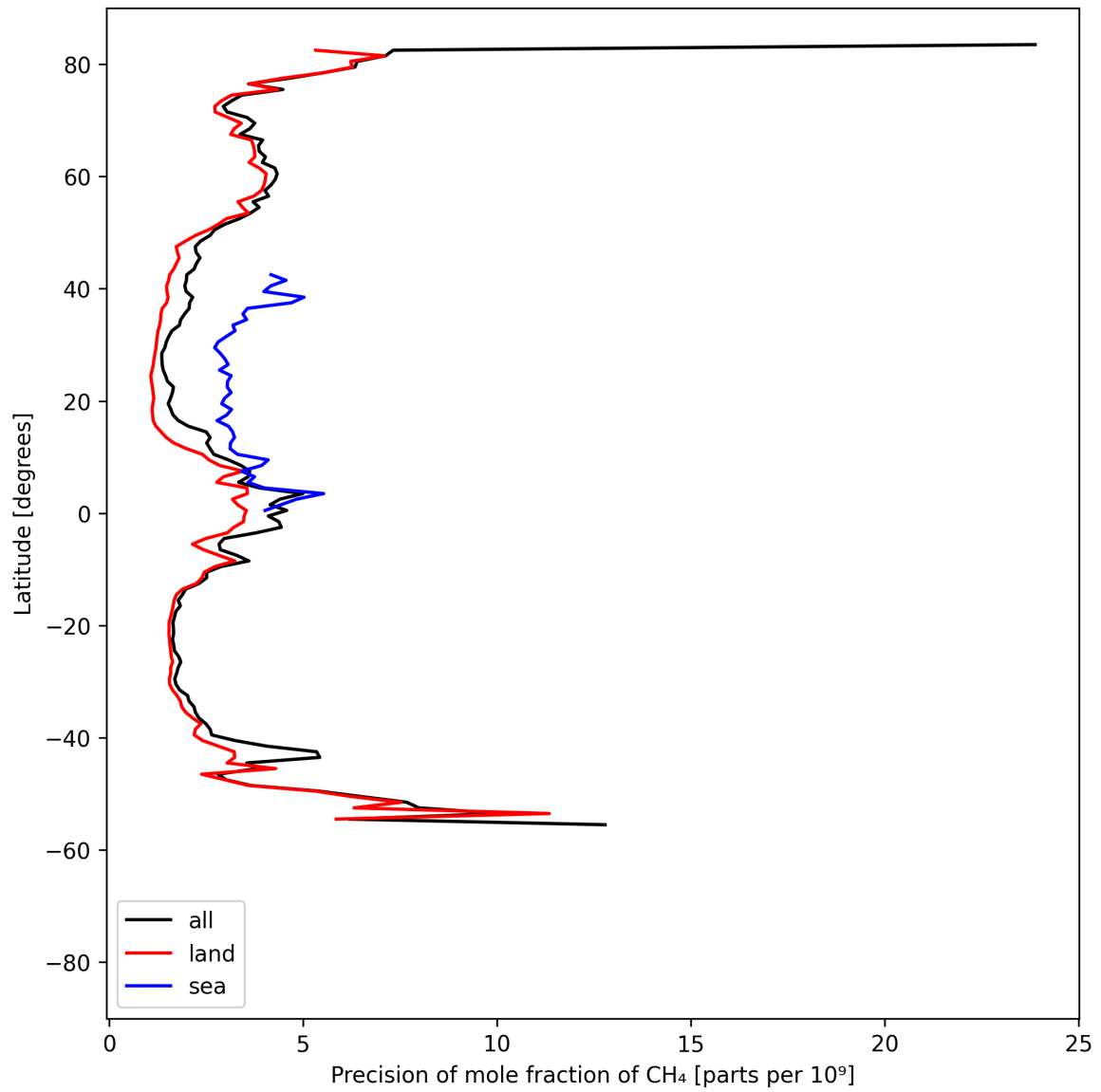
Figure 13: Zonal average of “Precision of mole fraction of CH 4 ” for 2025-08-09 to 2025-08-11.
