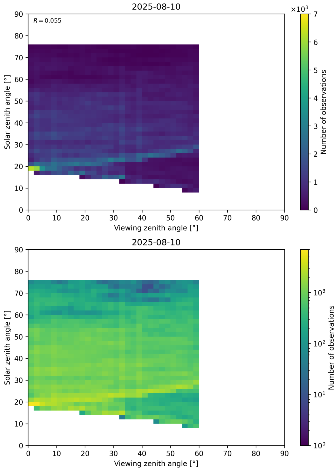
Figure 115: Scatter density plot of “Viewing zenith angle” against “Solar zenith angle” for 2025-08-09 to 2025-08-11.
