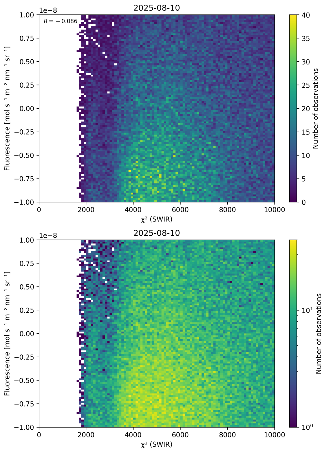
Figure 49: Scatter density plot of “ \chi^2 (SWIR)” against “Fluorescence” for 2025-08-09 to 2025-08-11.
