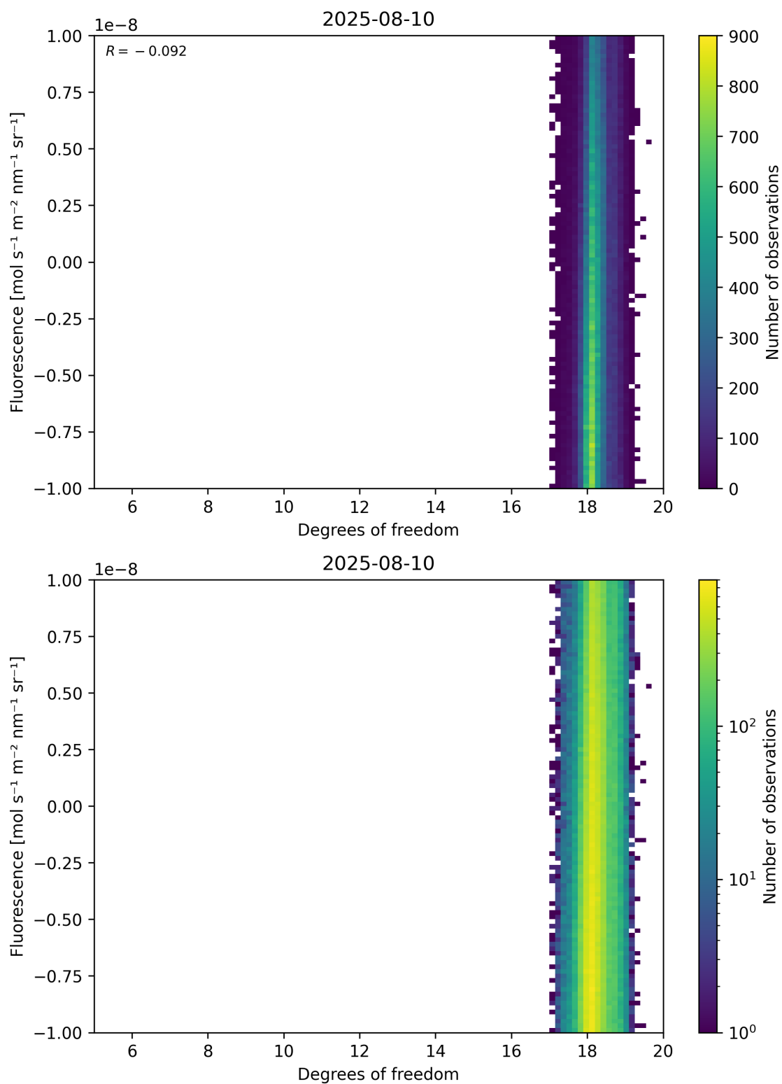
Figure 51: Scatter density plot of “Degrees of freedom” against “Fluorescence” for 2025-08-09 to 2025-08-11.
