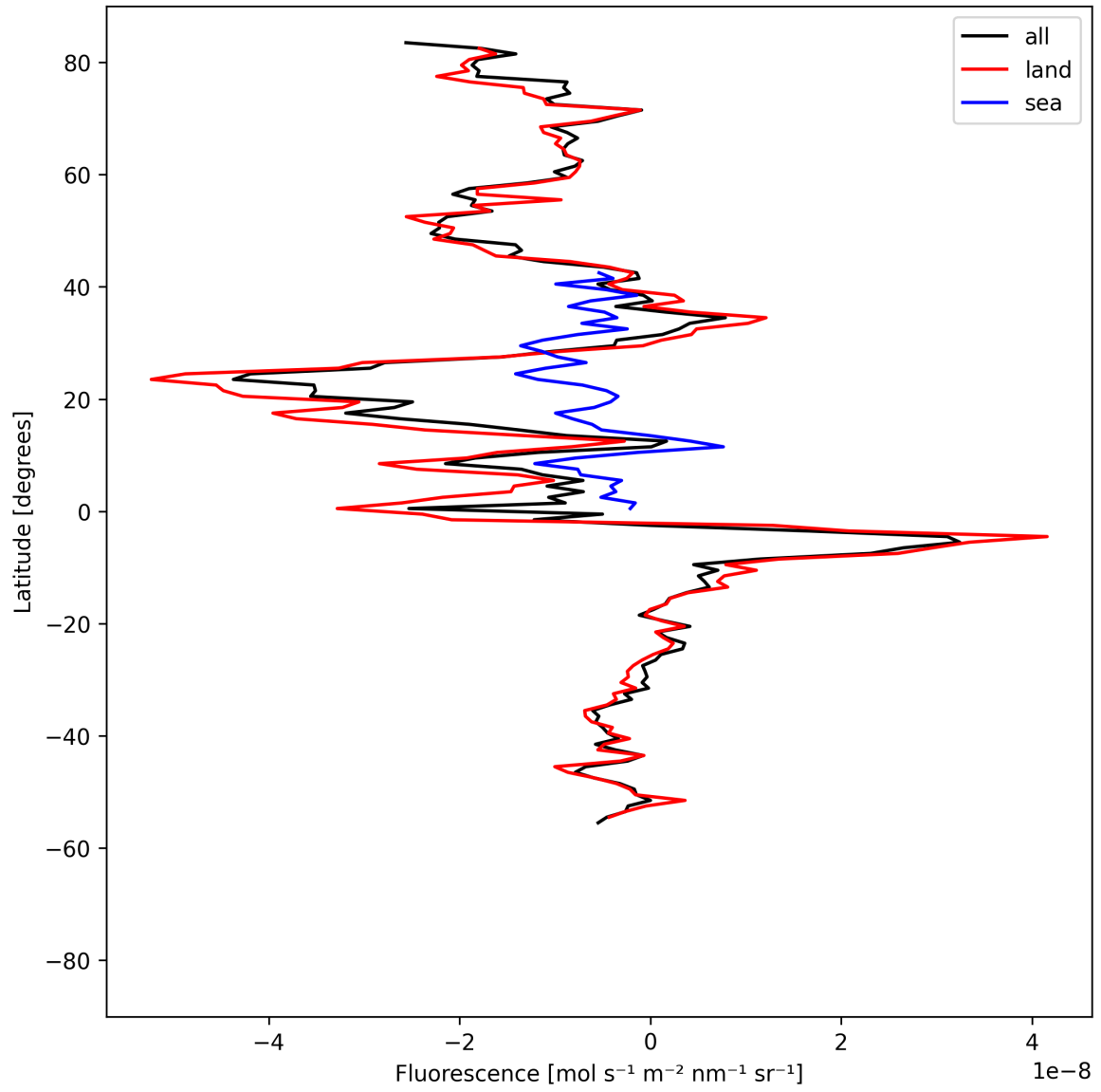
Figure 21: Zonal average of “Fluorescence” for 2025-08-09 to 2025-08-11.
