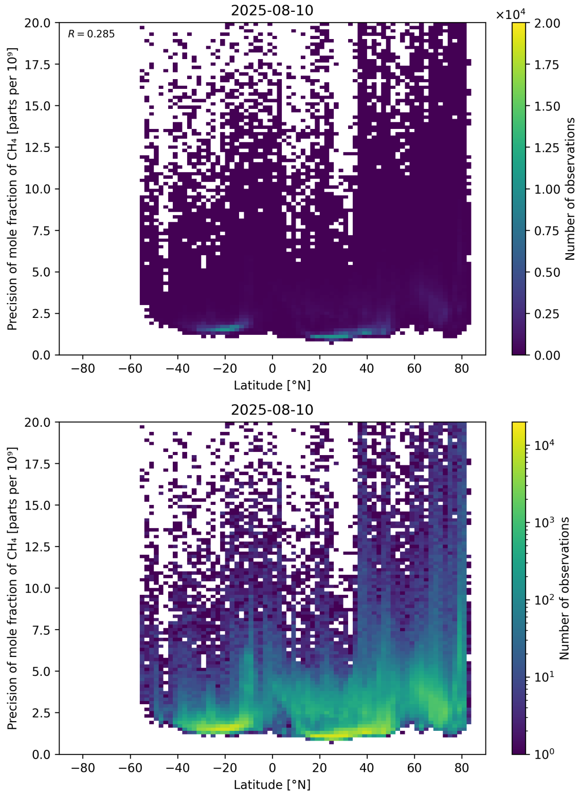
Figure 59: Scatter density plot of “Latitude” against “Precision of mole fraction of \text{CH}_4 ” for 2025-08-09 to 2025-08-11.
