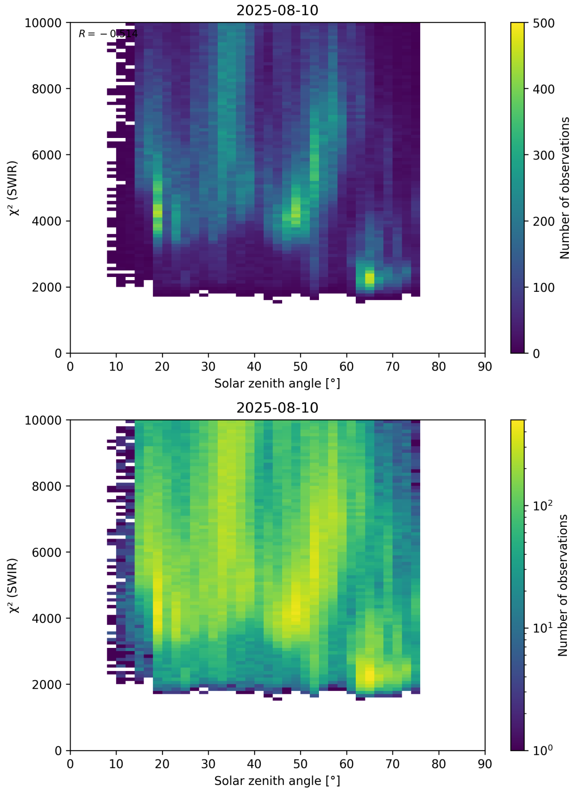
Figure 95: Scatter density plot of “Solar zenith angle” against “ \chi^2 (SWIR)” for 2025-08-09 to 2025-08-11.
