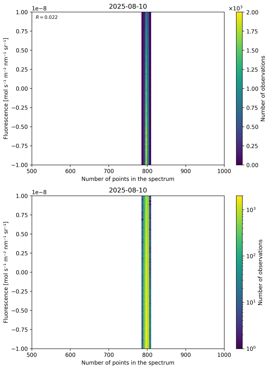
Figure 91: Scatter density plot of “Number of points in the spectrum” against “Fluorescence” for 2025-08-09 to 2025-08-11.
