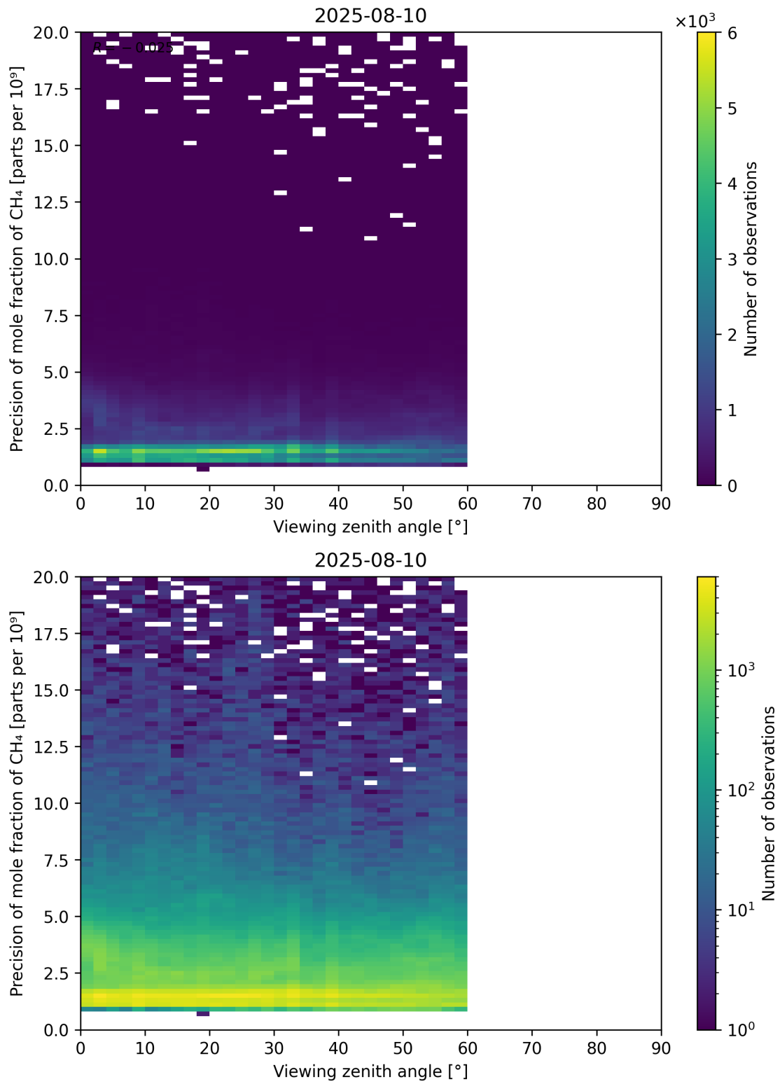
Figure 112: Scatter density plot of “Viewing zenith angle” against “Precision of mole fraction of CH 4 ” for 2025-08-09 to 2025-08-11.
