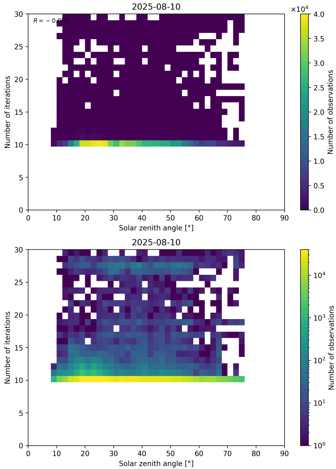
Figure 102: Scatter density plot of “Solar zenith angle” against “Number of iterations” for 2025-08-09 to 2025-08-11.
