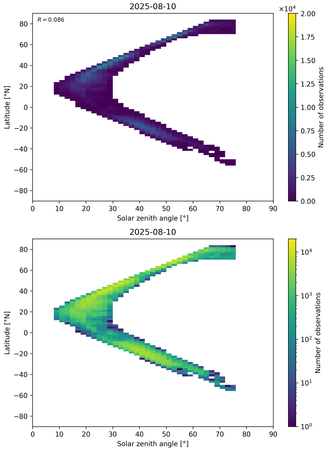
Figure 98: Scatter density plot of “Solar zenith angle” against “Latitude” for 2025-08-09 to 2025-08-11.
