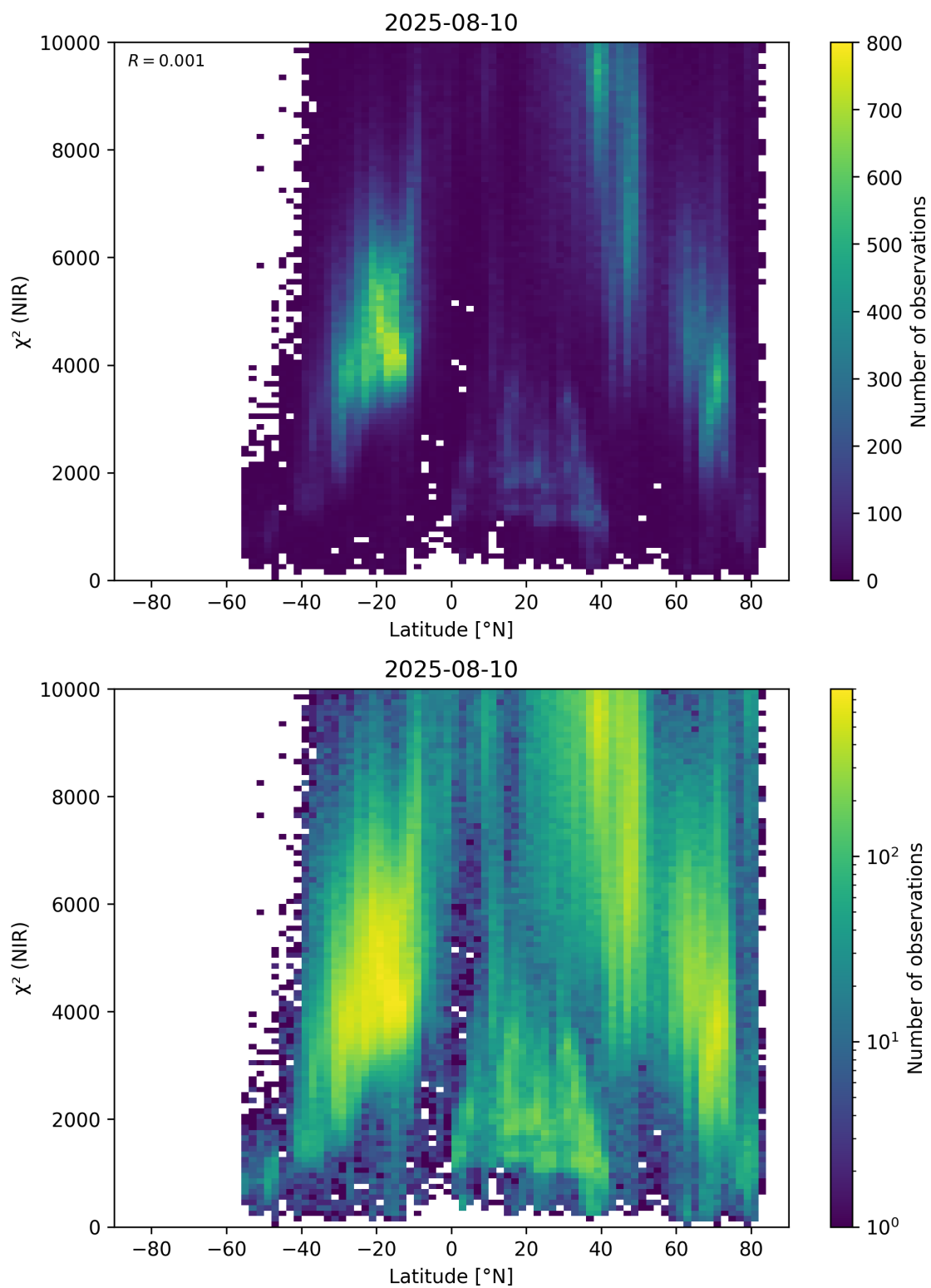
Figure 53: Scatter density plot of “Latitude” against “ \chi^2 (NIR)” for 2025-08-09 to 2025-08-11.
