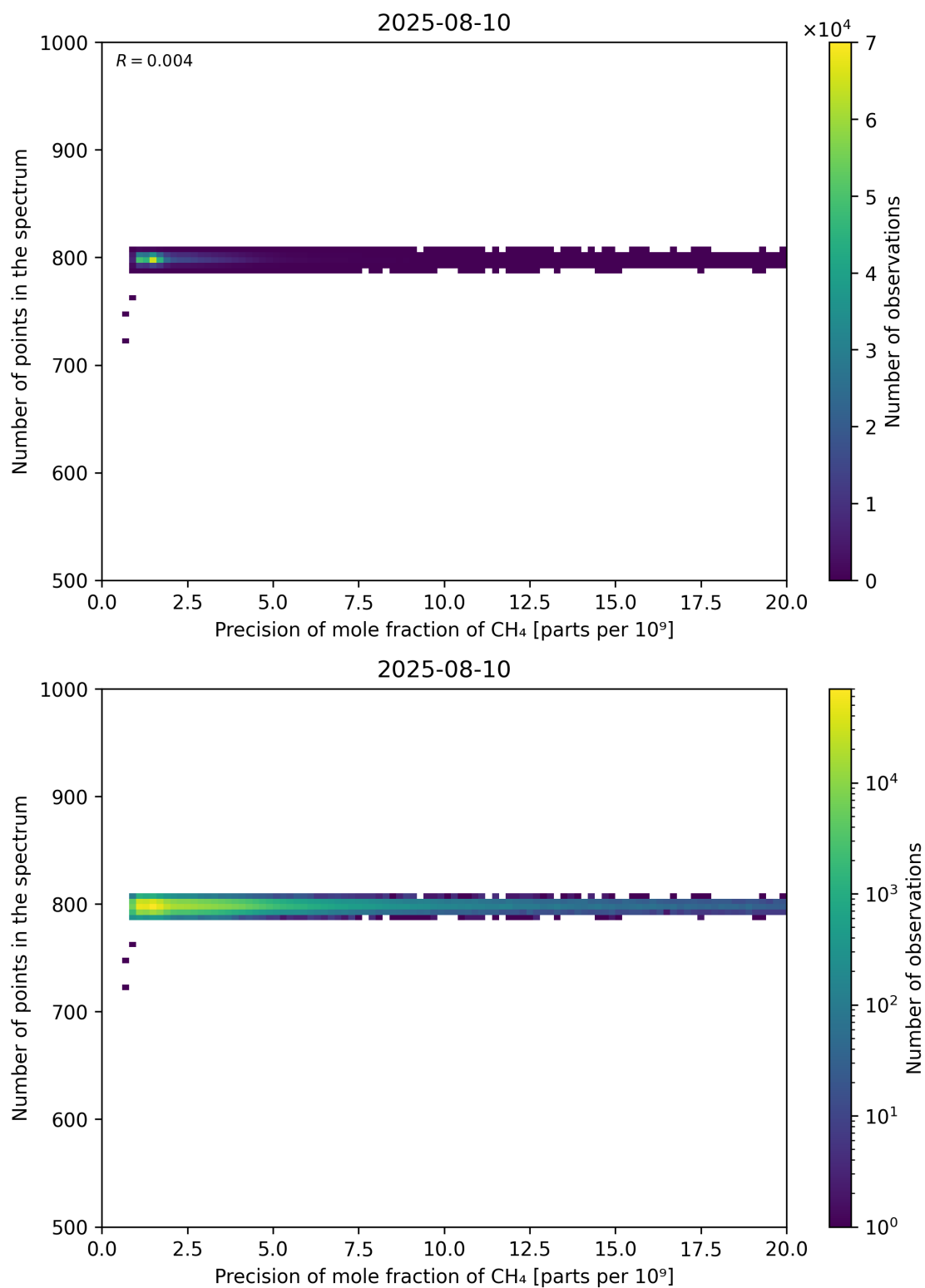
Figure 84: Scatter density plot of “Precision of mole fraction of CH 4 ” against “Number of points in the spectrum” for 2025-08-09 to 2025-08-11.
