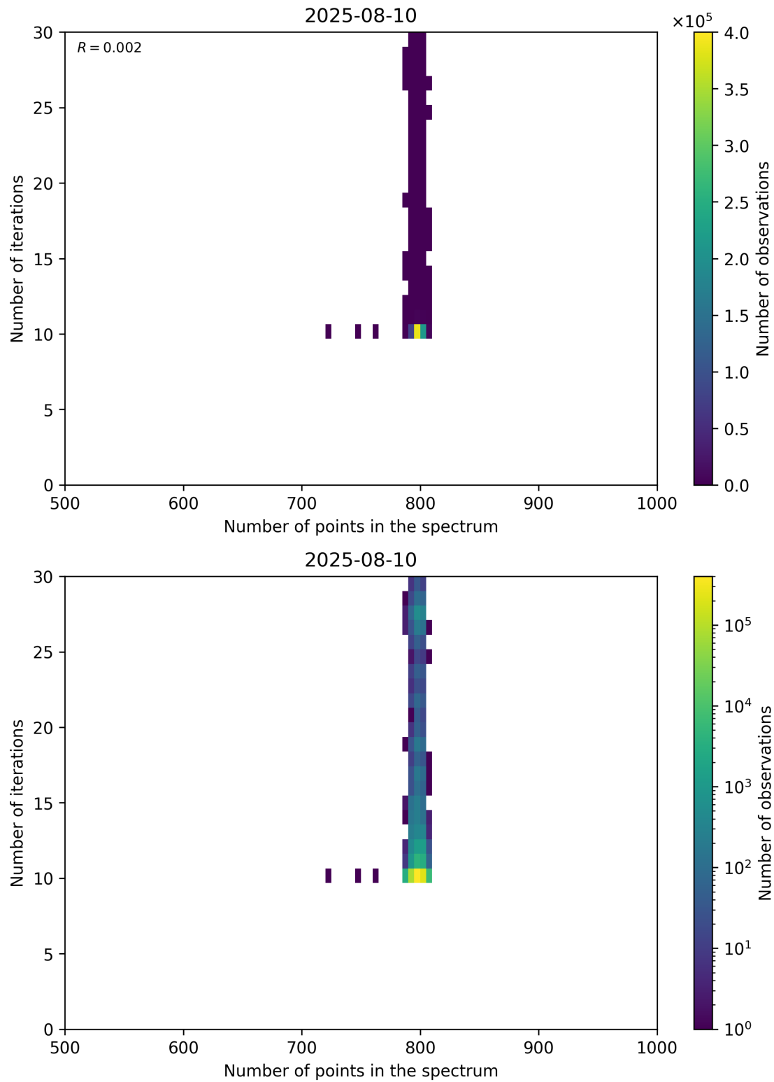
Figure 92: Scatter density plot of “Number of points in the spectrum” against “Number of iterations” for 2025-08-09 to 2025-08-11.
