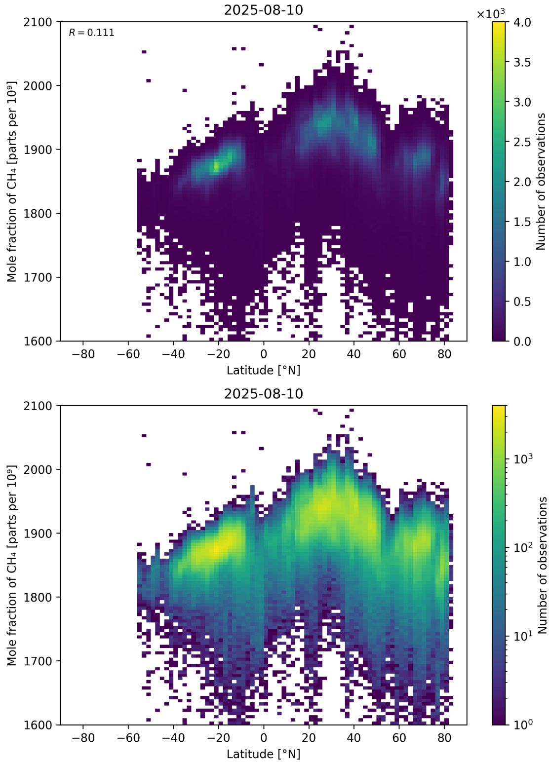
Figure 57: Scatter density plot of “Latitude” against “Mole fraction of CH 4 ” for 2025-08-09 to 2025-08-11.
