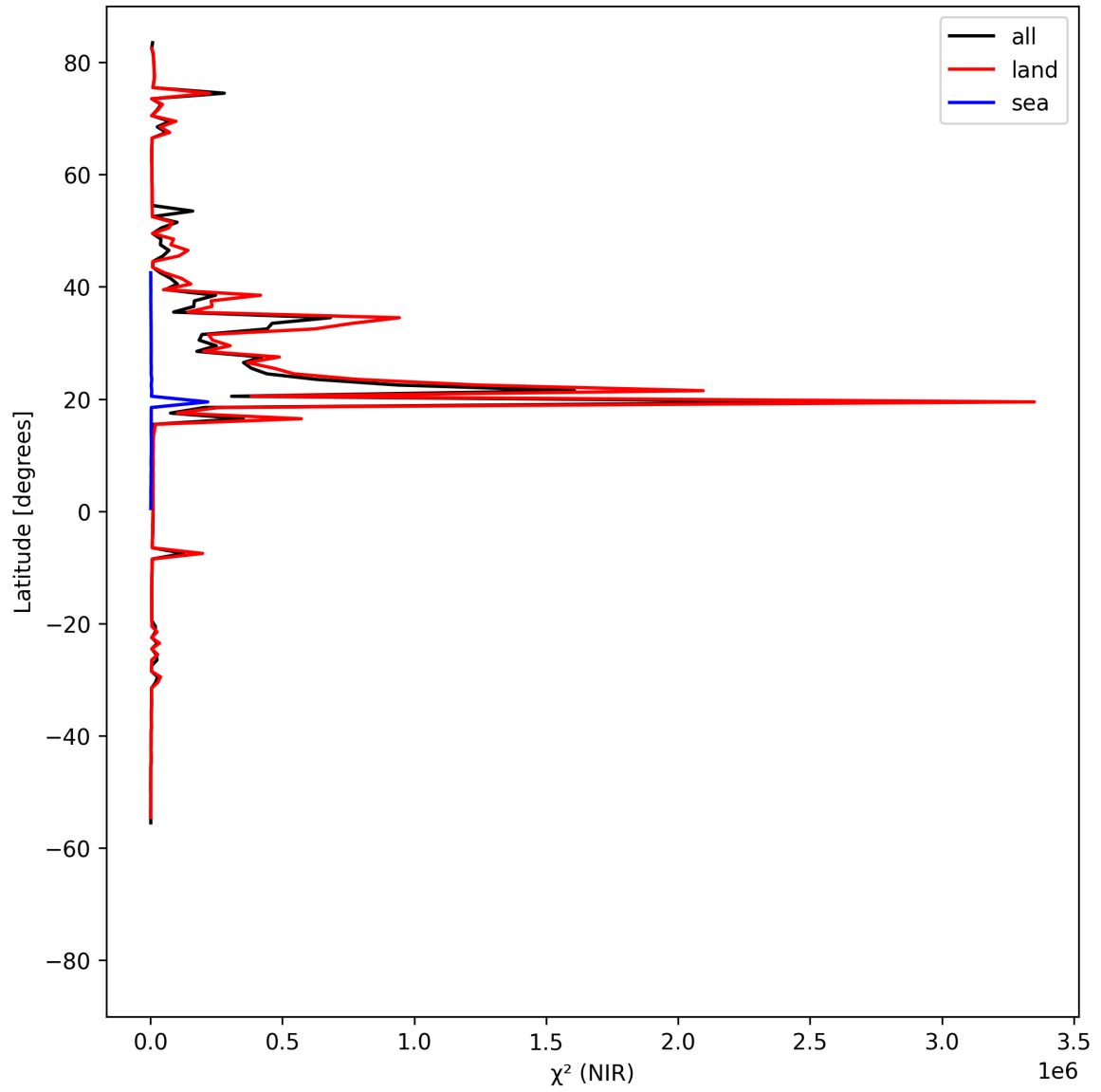
Figure 18: Zonal average of “ \chi^2 (NIR)” for 2025-08-09 to 2025-08-11.
