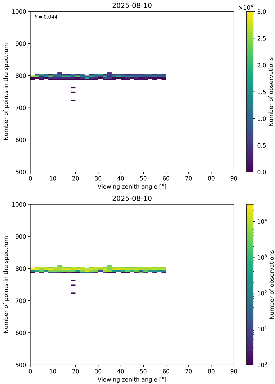
Figure 114: Scatter density plot of “Viewing zenith angle” against “Number of points in the spectrum” for 2025-08-09 to 2025-08-11.
