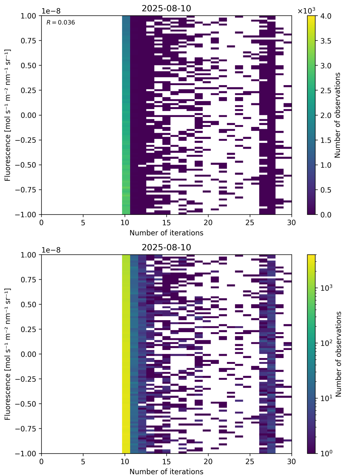
Figure 87: Scatter density plot of “Number of iterations” against “Fluorescence” for 2025-08-09 to 2025-08-11.
