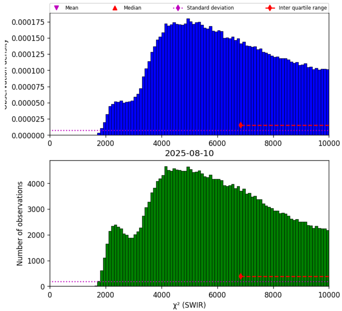
Figure 28: Histogram of “ \chi^2 (SWIR)” for 2025-08-09 to 2025-08-11
