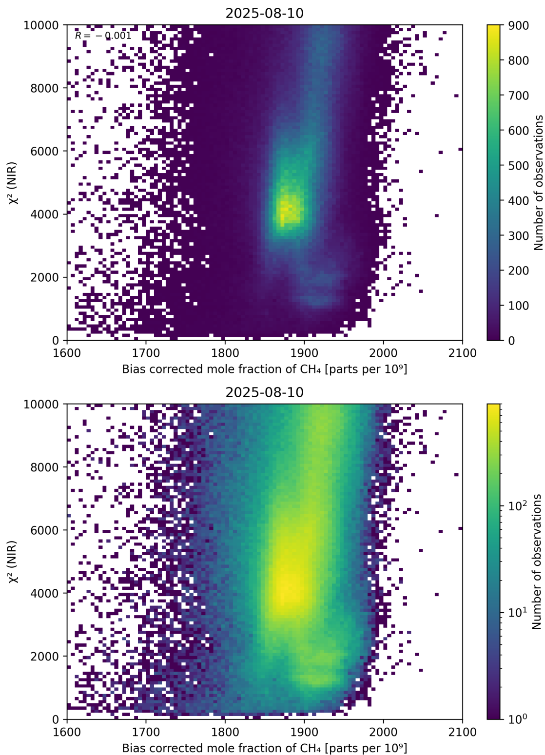
Figure 63: Scatter density plot of “Bias corrected mole fraction of CH 4 ” against “ \chi^2 (NIR)” for 2025-08-09 to 2025-08-11.
