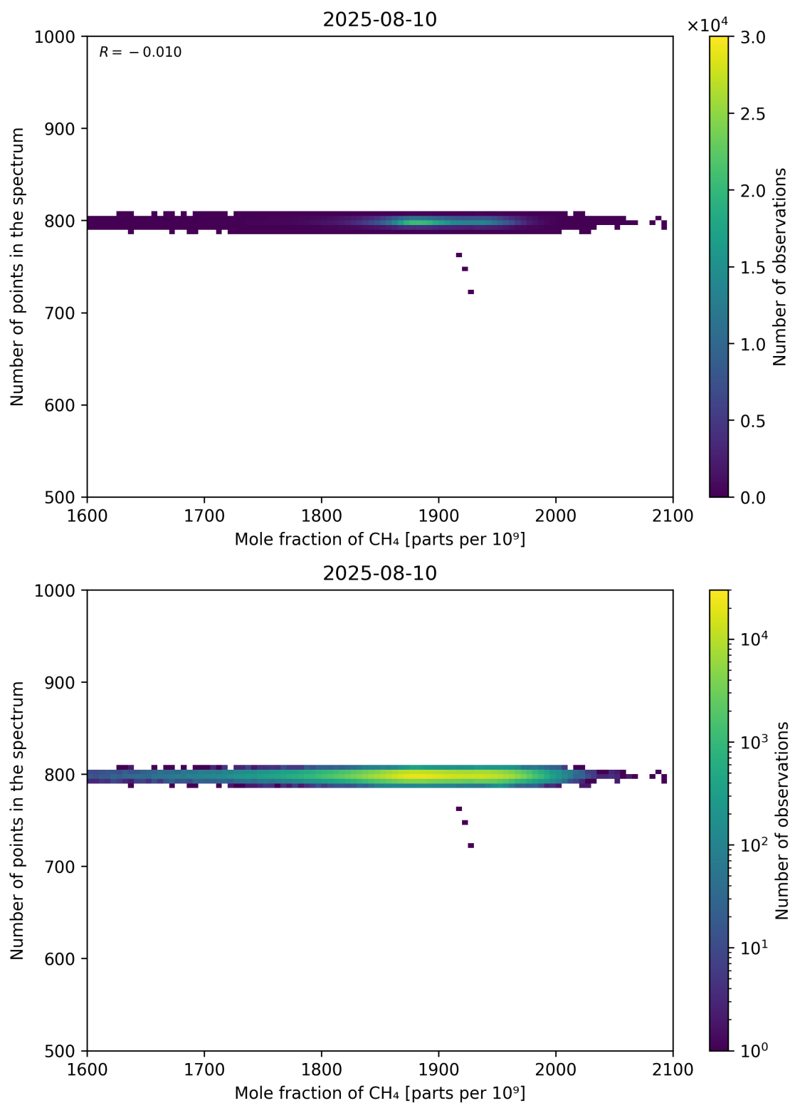
Figure 77: Scatter density plot of “Mole fraction of CH 4 ” against “Number of points in the spectrum” for 2025-08-09 to 2025-08-11.
