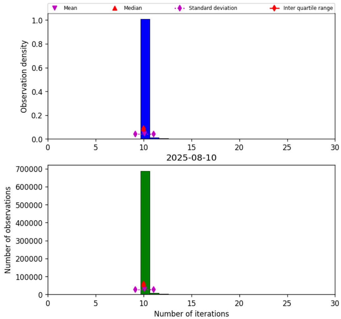
Figure 31: Histogram of “Number of iterations” for 2025-08-09 to 2025-08-11
