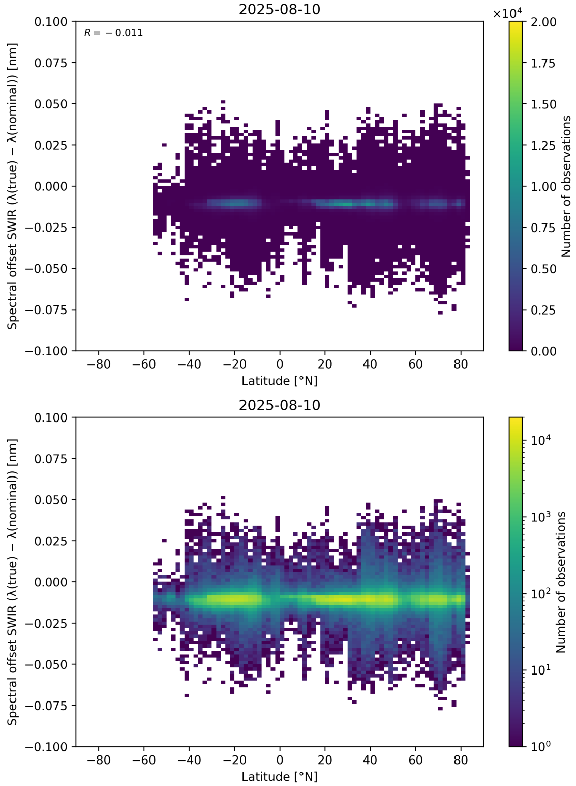
Figure 62: Scatter density plot of “Latitude” against “Spectral offset SWIR ( \lambda_{\text{true}} - \lambda_{\text{nominal}} )” for 2025-08-09 to 2025-08-11.
