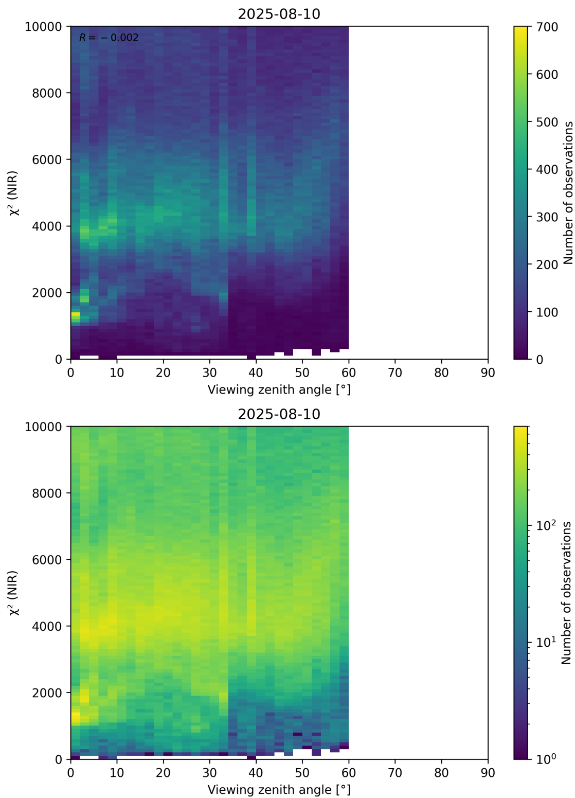
Figure 105: Scatter density plot of “Viewing zenith angle” against “ \chi^2 (NIR)” for 2025-08-09 to 2025-08-11.
