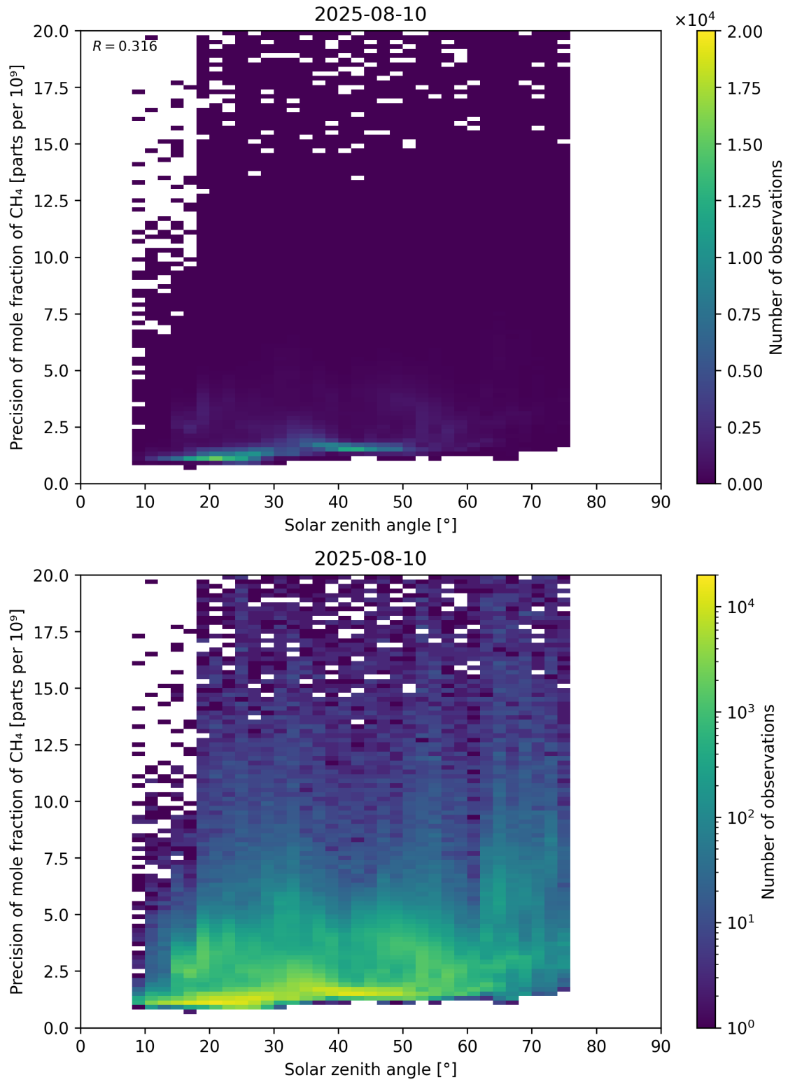
Figure 101: Scatter density plot of “Solar zenith angle” against “Precision of mole fraction of CH 4 ” for 2025-08-09 to 2025-08-11.
