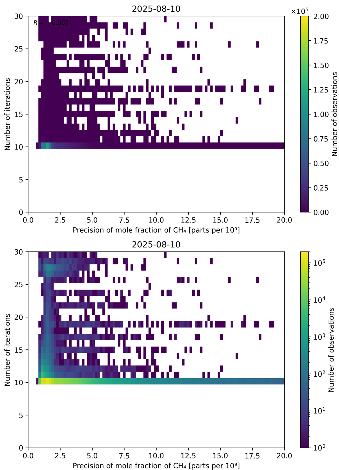
Figure 83: Scatter density plot of “Precision of mole fraction of CH 4 ” against “Number of iterations” for 2025-08-09 to 2025-08-11.
