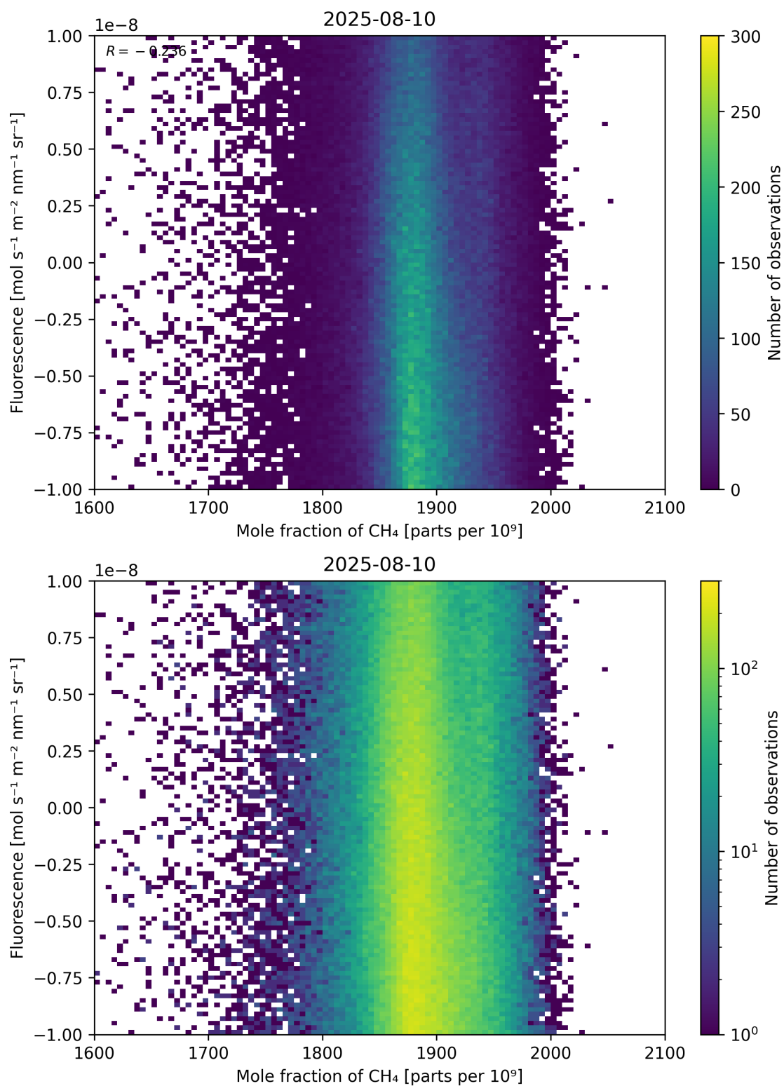
Figure 73: Scatter density plot of “Mole fraction of CH 4 ” against “Fluorescence” for 2025-08-09 to 2025-08-11.
