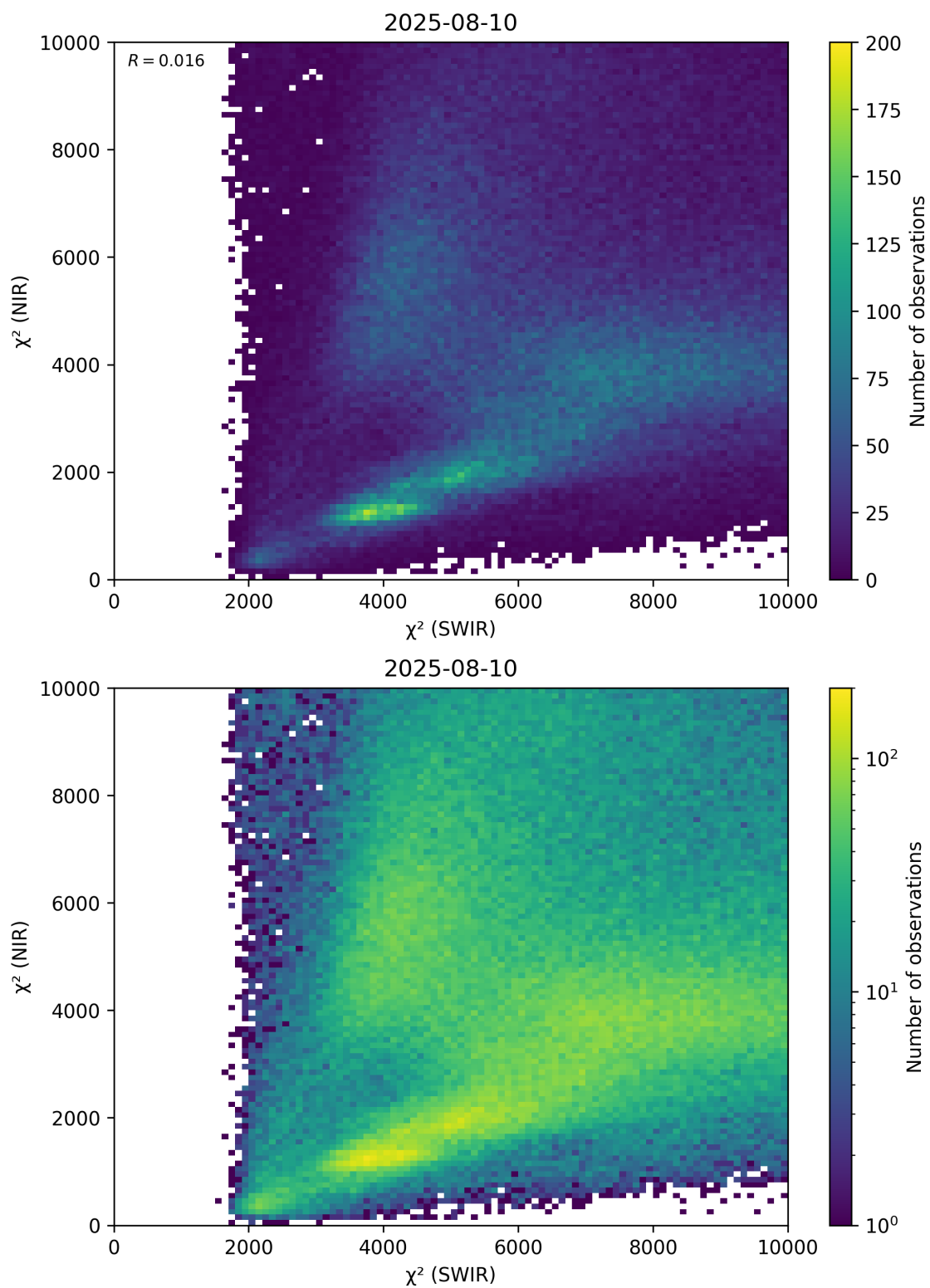
Figure 47: Scatter density plot of “ \chi^2 (SWIR)” against “ \chi^2 (NIR)” for 2025-08-09 to 2025-08-11.
