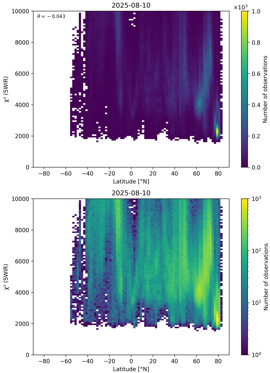
Figure 54: Scatter density plot of “Latitude” against “ \chi^2 (SWIR)” for 2025-08-09 to 2025-08-11.
