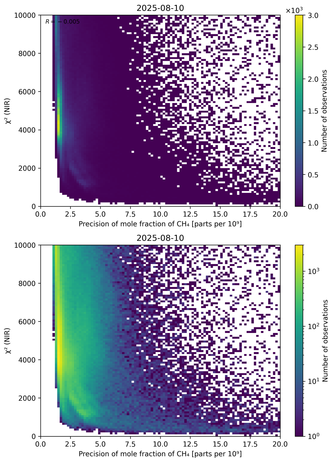
Figure 78: Scatter density plot of “Precision of mole fraction of CH 4 ” against “ \chi^2 (NIR)” for 2025-08-09 to 2025-08-11.
