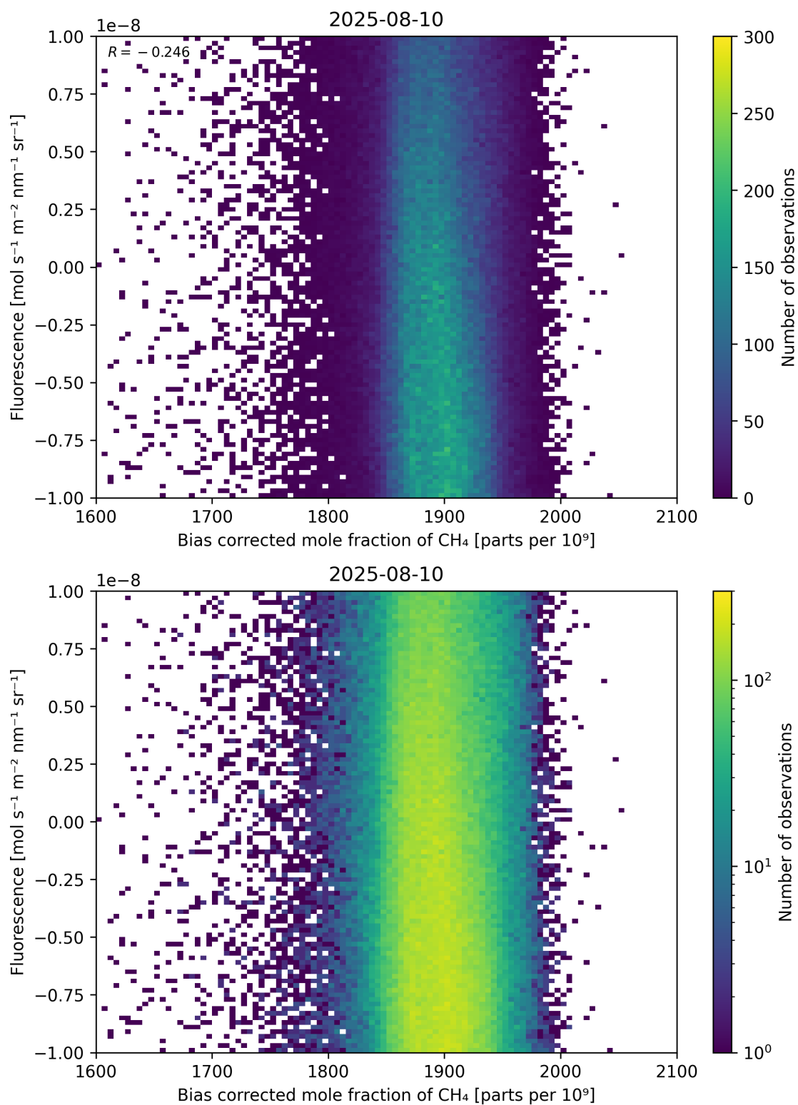
Figure 66: Scatter density plot of “Bias corrected mole fraction of \text{CH}_4 ” against “Fluorescence” for 2025-08-09 to 2025-08-11.
