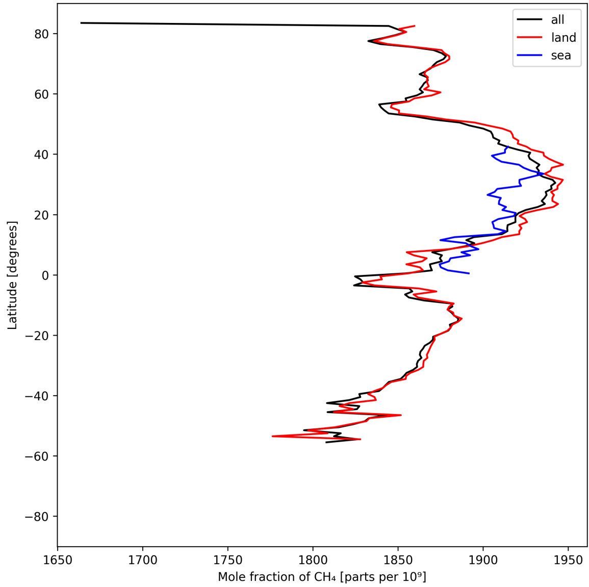
Figure 12: Zonal average of “Mole fraction of \text{CH}_4 ” for 2025-08-09 to 2025-08-11.
