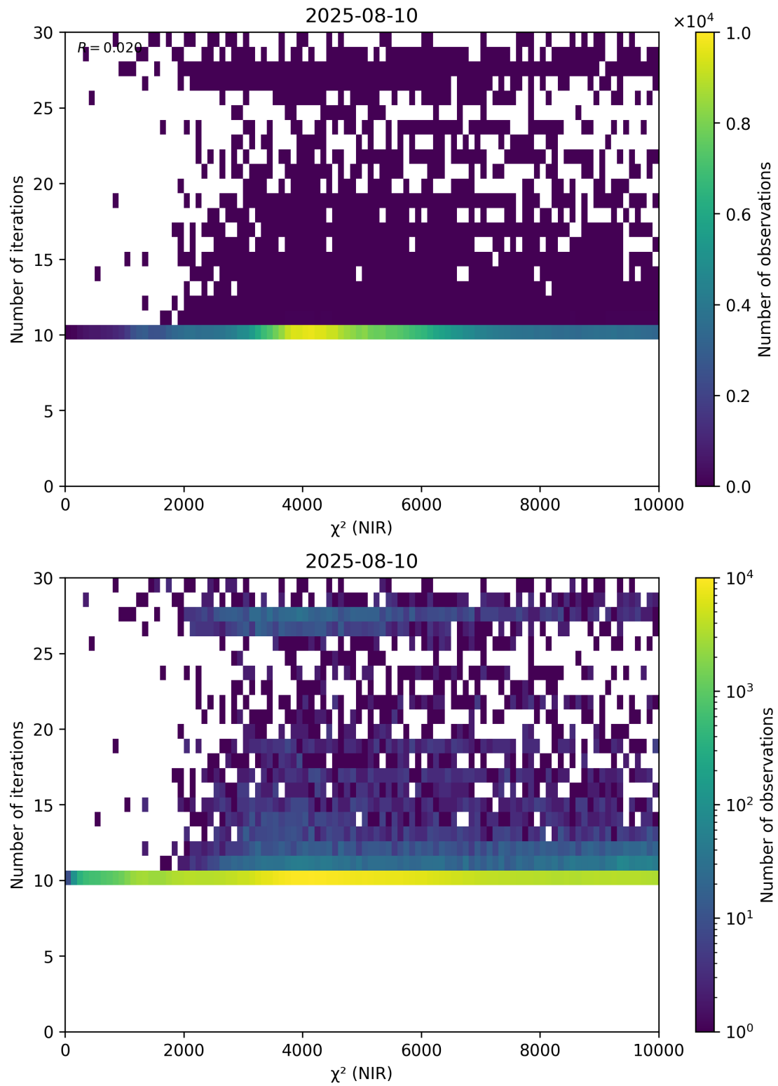
Figure 46: Scatter density plot of “ \chi^2 (NIR)” against “Number of iterations” for 2025-08-09 to 2025-08-11.
