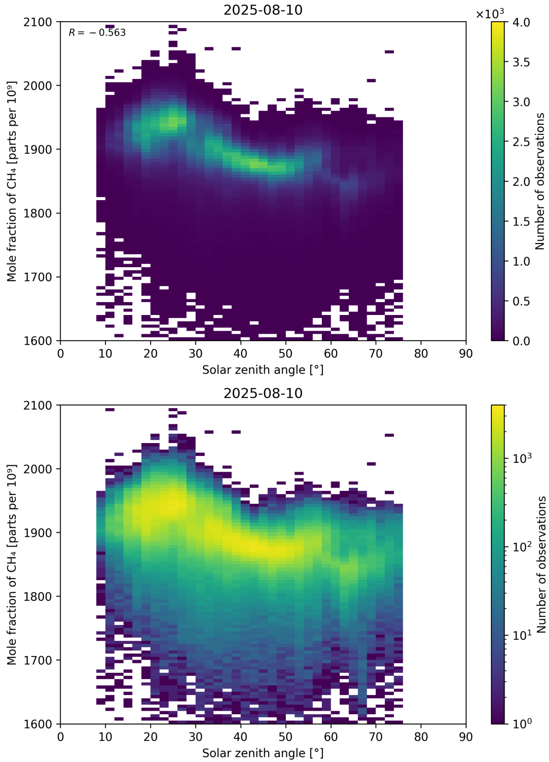
Figure 99: Scatter density plot of “Solar zenith angle” against “Mole fraction of \text{CH}_4 ” for 2025-08-09 to 2025-08-11.
