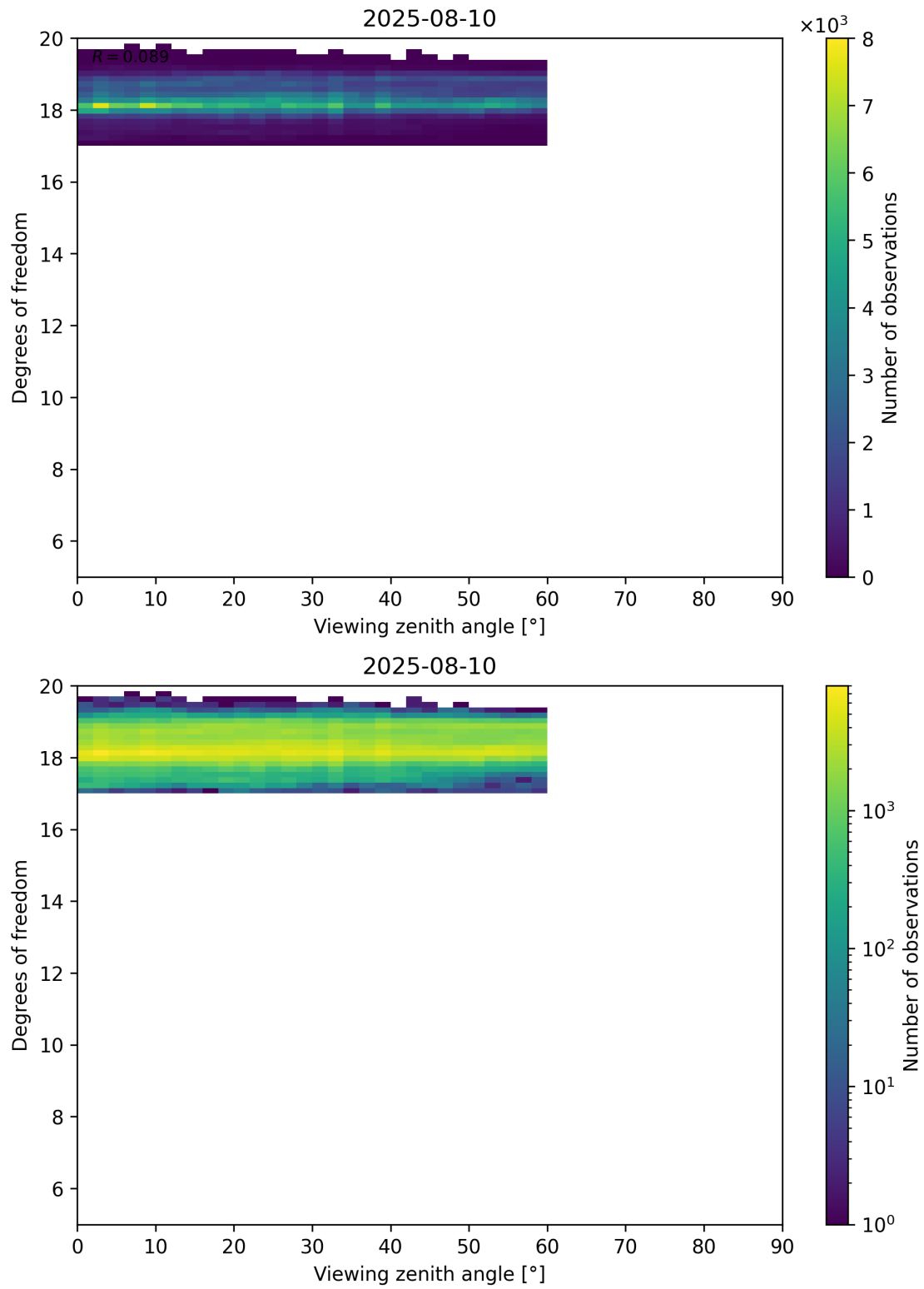
Figure 107: Scatter density plot of “Viewing zenith angle” against “Degrees of freedom” for 2025-08-09 to 2025-08-11.
