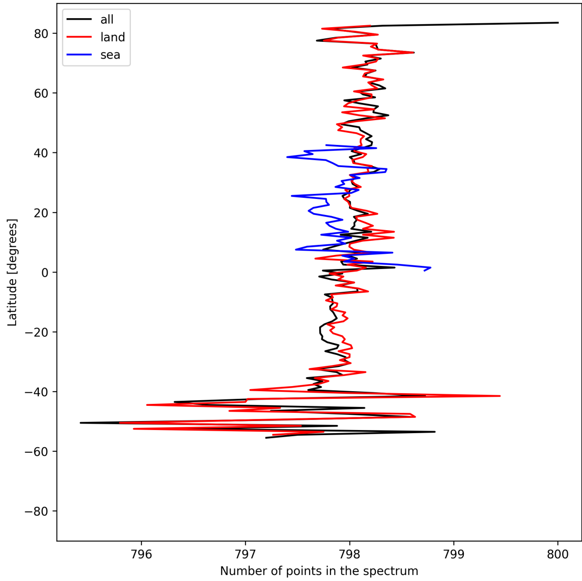
Figure 15: Zonal average of “Number of points in the spectrum” for 2025-08-09 to 2025-08-11.
