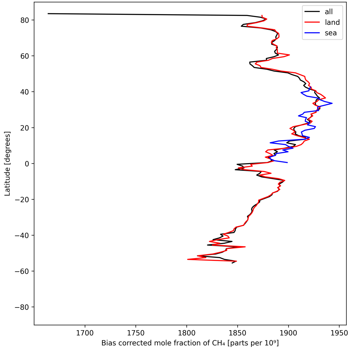
Figure 14: Zonal average of “Bias corrected mole fraction of \text{CH}_4 ” for 2025-08-09 to 2025-08-11.
