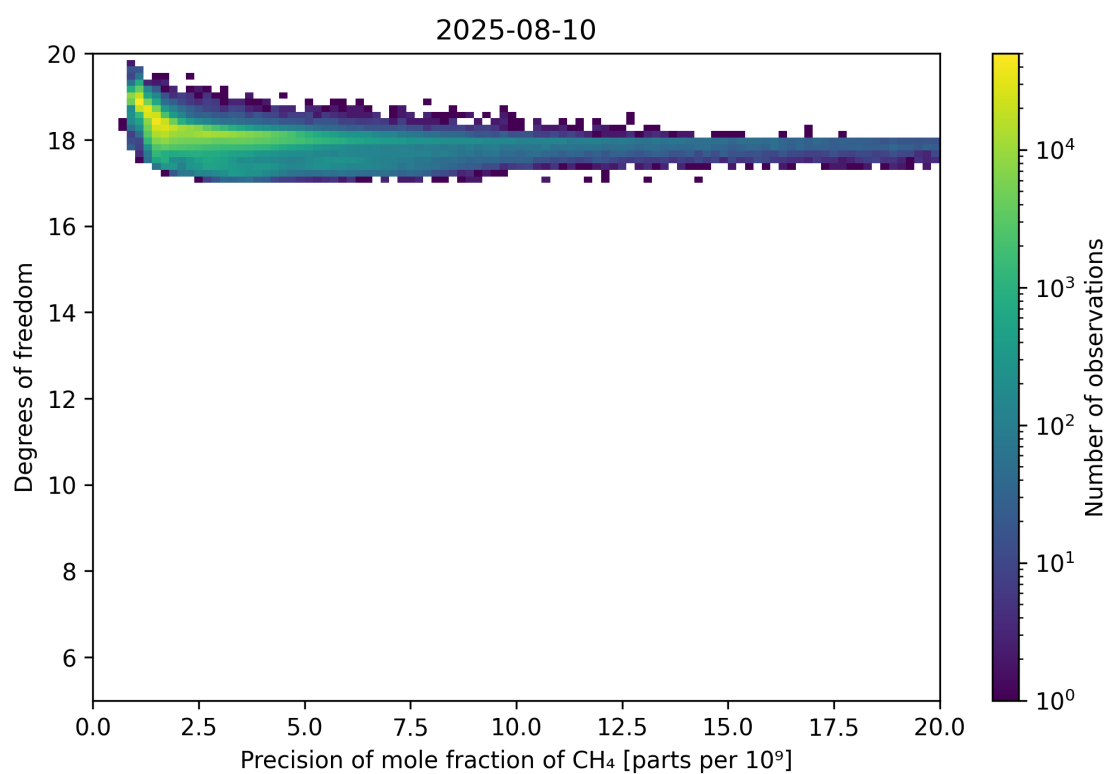
Figure 80: Scatter density plot of “Precision of mole fraction of CH 4 ” against “Degrees of freedom” for 2025-08-09 to 2025-08-11.
