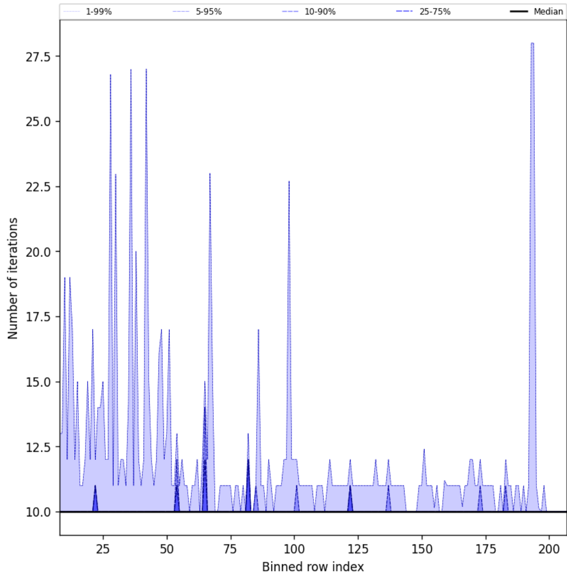
Figure 42: Along track statistics of “Number of iterations” for 2025-08-09 to 2025-08-11
