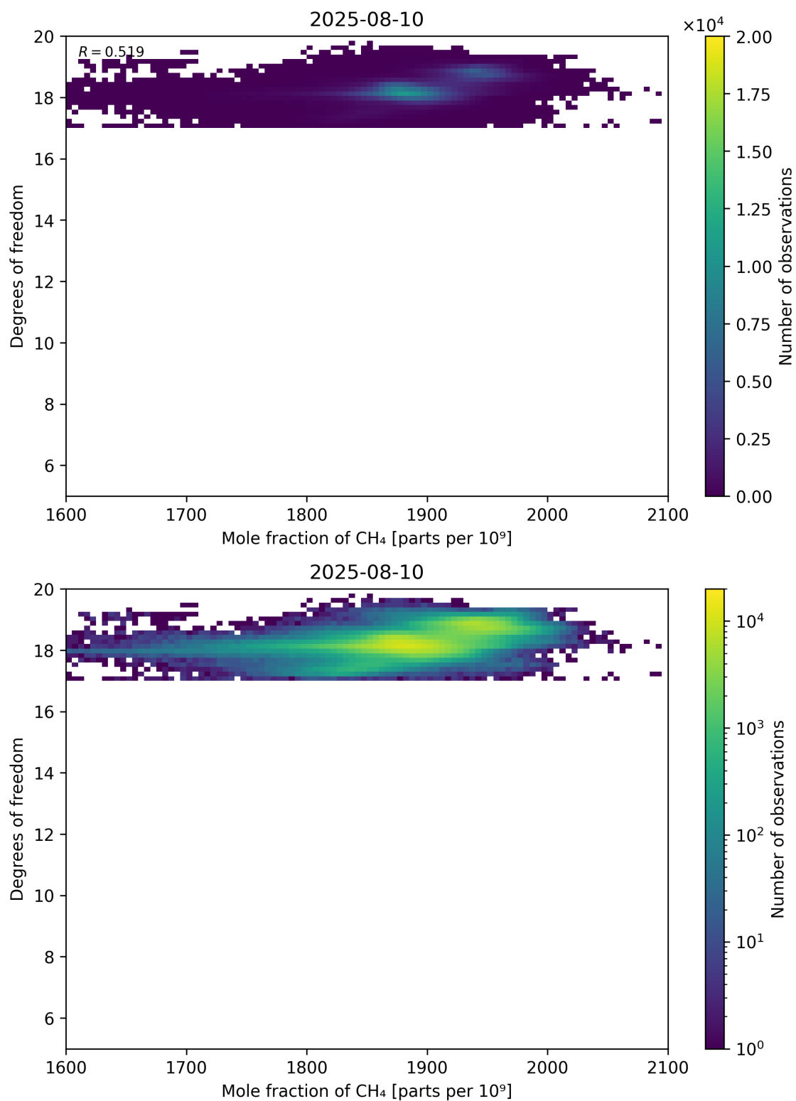
Figure 72: Scatter density plot of “Mole fraction of CH 4 ” against “Degrees of freedom” for 2025-08-09 to 2025-08-11.
