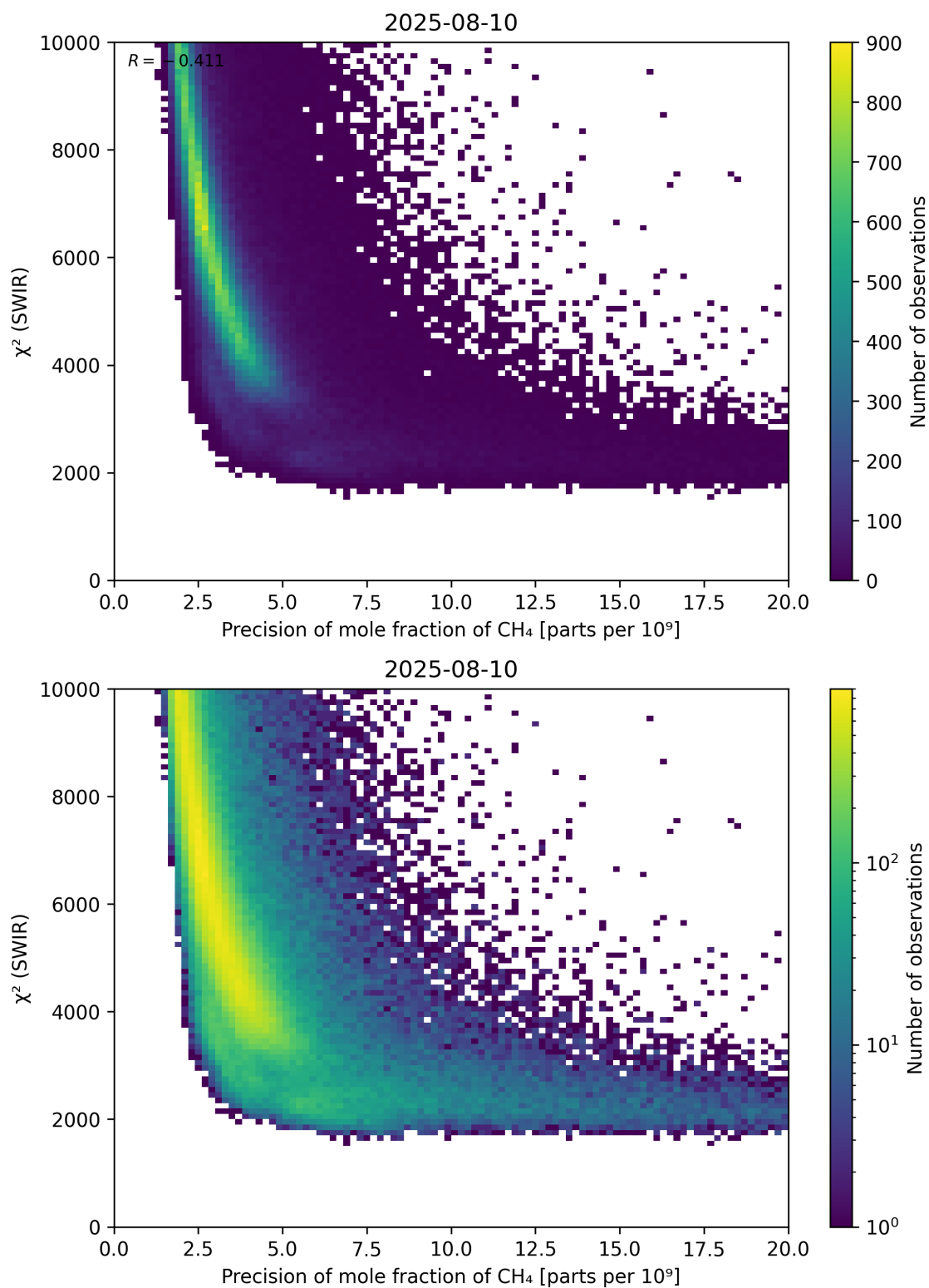
Figure 79: Scatter density plot of “Precision of mole fraction of CH 4 ” against “ \chi^2 (SWIR)” for 2025-08-09 to 2025-08-11.
