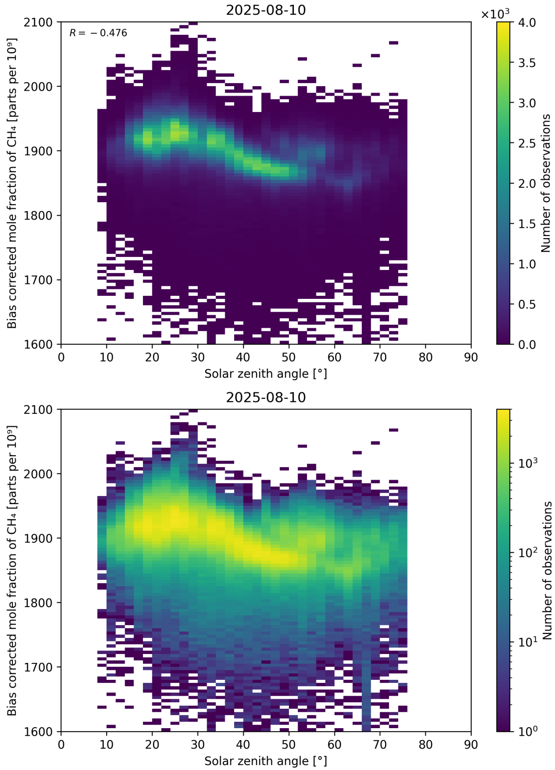
Figure 100: Scatter density plot of “Solar zenith angle” against “Bias corrected mole fraction of CH 4 ” for 2025-08-09 to 2025-08-11.
