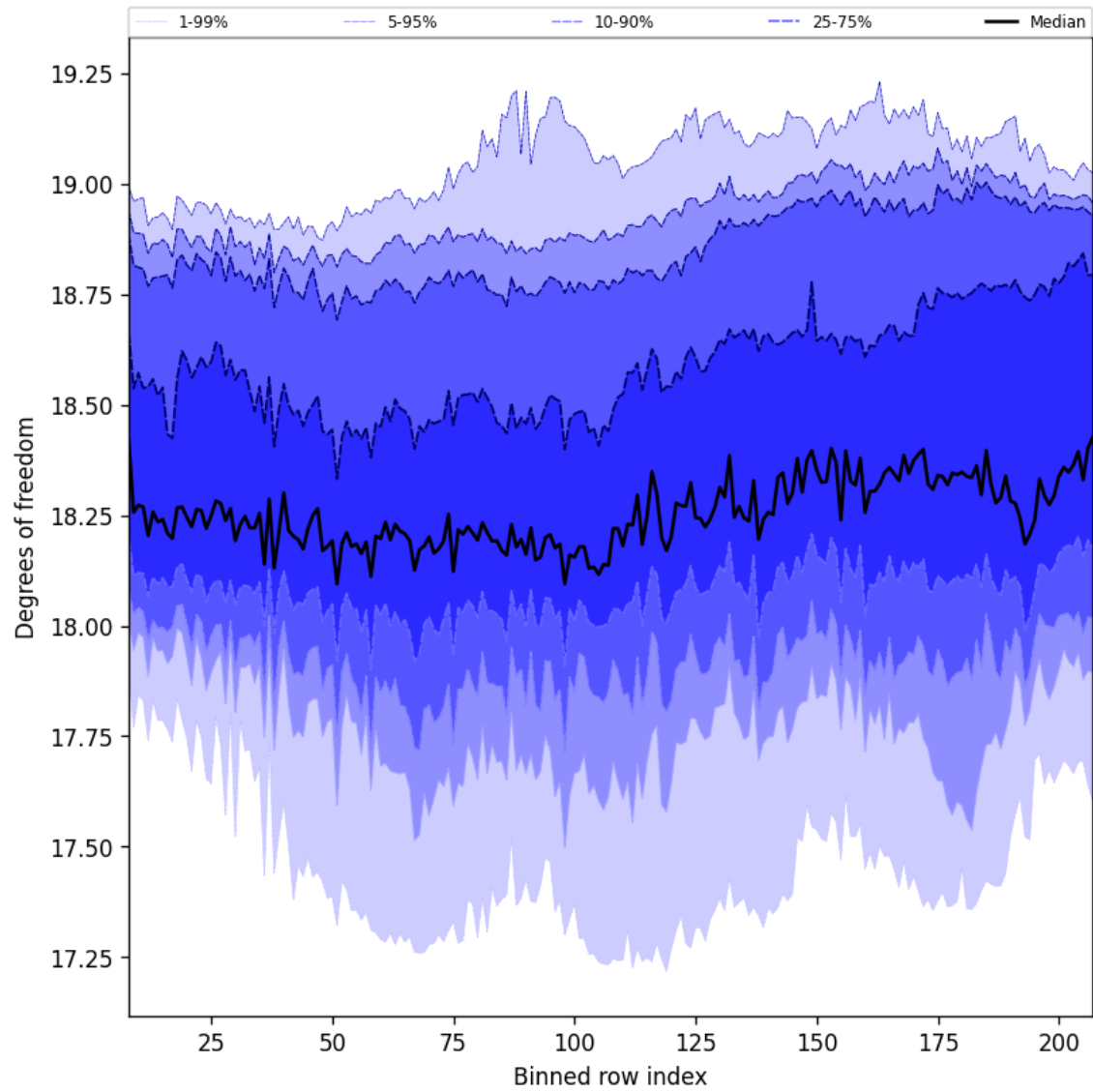
Figure 41: Along track statistics of “Degrees of freedom” for 2025-08-09 to 2025-08-11
