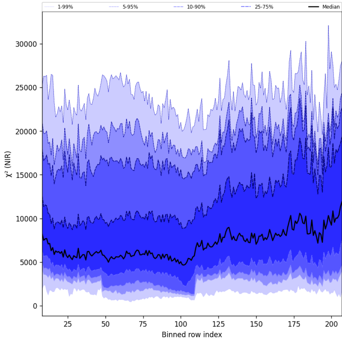
Figure 40: Along track statistics of “ \chi^2 (NIR)” for 2025-08-09 to 2025-08-11
