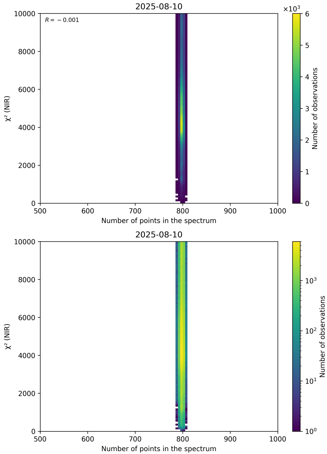
Figure 88: Scatter density plot of “Number of points in the spectrum” against “ \chi^2 (NIR)” for 2025-08-09 to 2025-08-11.
