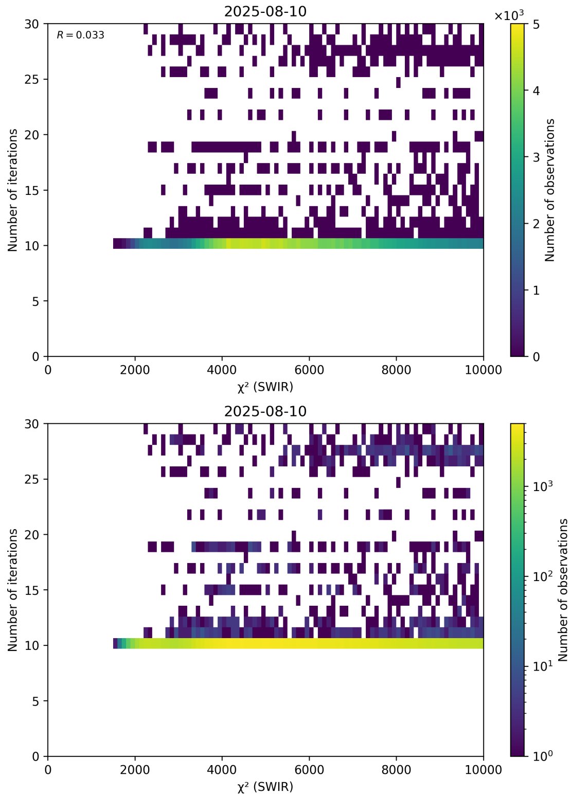
Figure 50: Scatter density plot of “ \chi^2 (SWIR)” against “Number of iterations” for 2025-08-09 to 2025-08-11.
