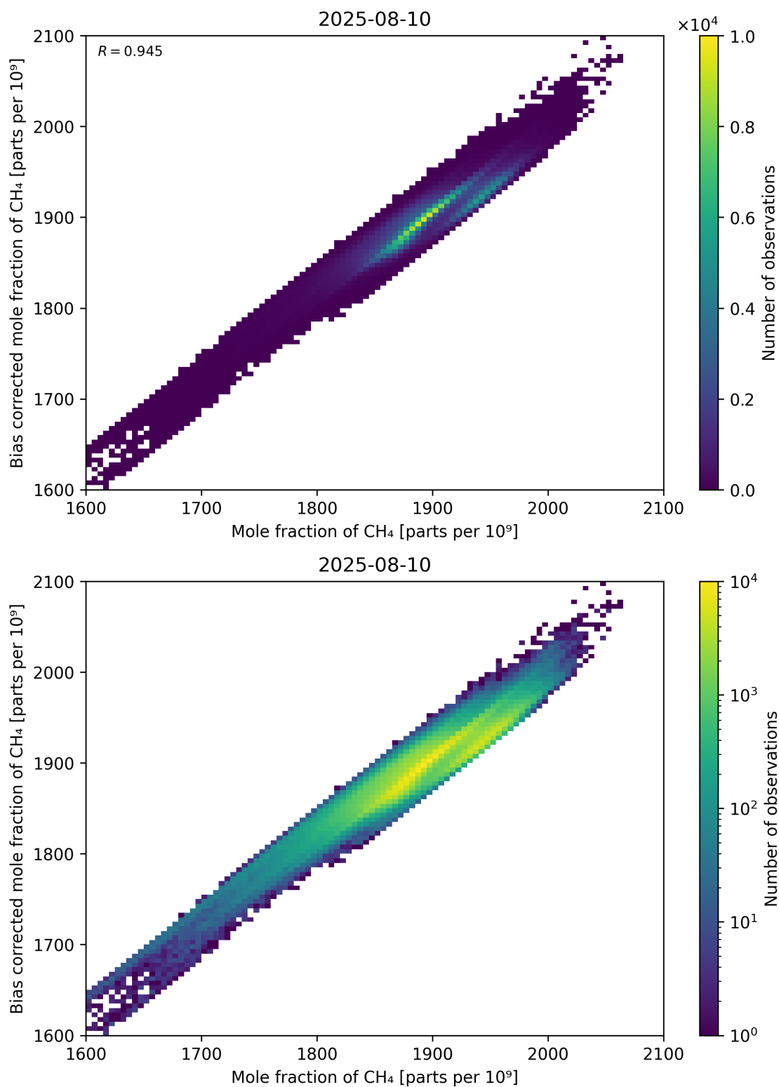
Figure 74: Scatter density plot of “Mole fraction of CH 4 ” against “Bias corrected mole fraction of CH 4 ” for 2025-08-09 to 2025-08-11.
