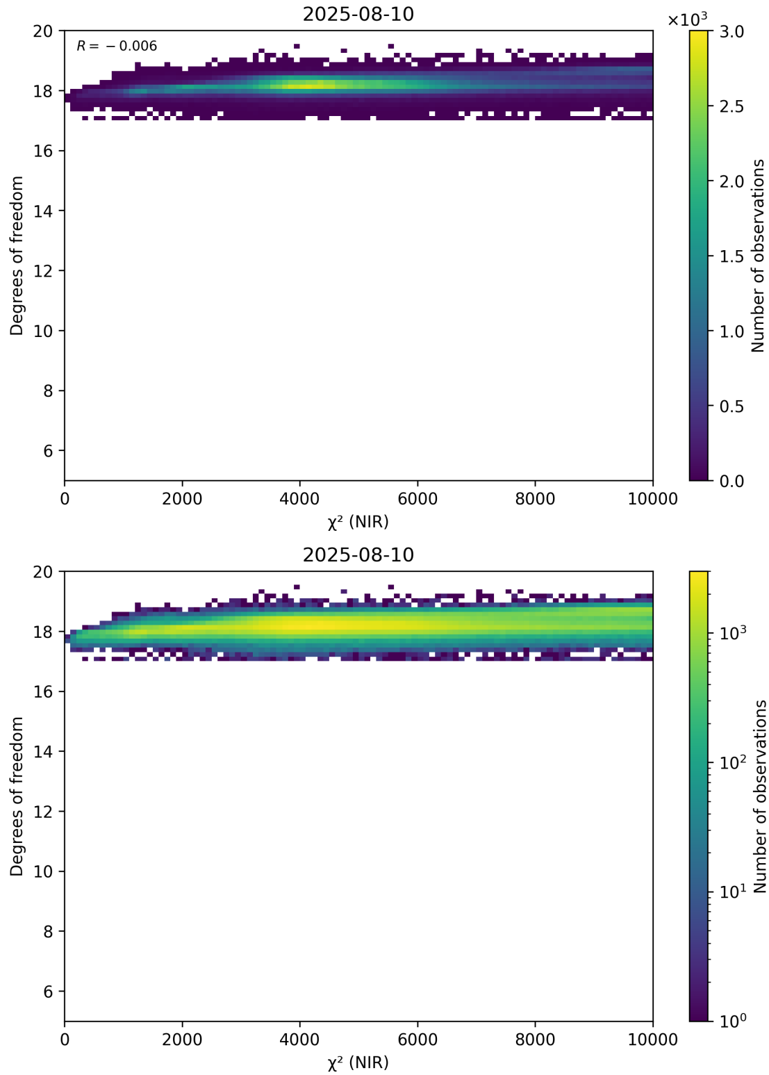
Figure 44: Scatter density plot of “ \chi^2 (NIR)” against “Degrees of freedom” for 2025-08-09 to 2025-08-11.
