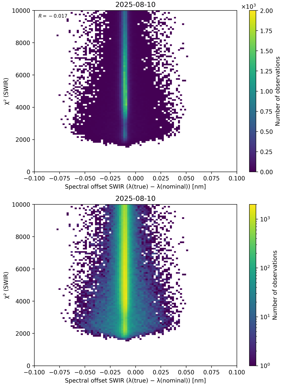
Figure 118: Scatter density plot of “Spectral offset SWIR ( \lambda_{\text{true}} - \lambda_{\text{nominal}} )” against “ \chi^2 (SWIR)” for 2025-08-09 to 2025-08-11.
