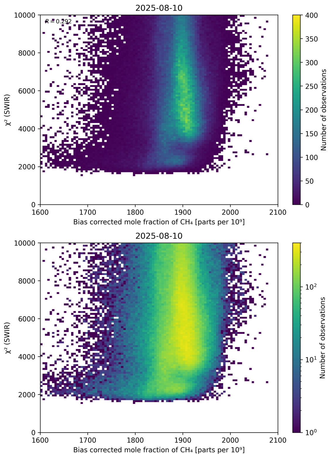
Figure 64: Scatter density plot of “Bias corrected mole fraction of \text{CH}_4 ” against “ \chi^2 (SWIR)” for 2025-08-09 to 2025-08-11.
