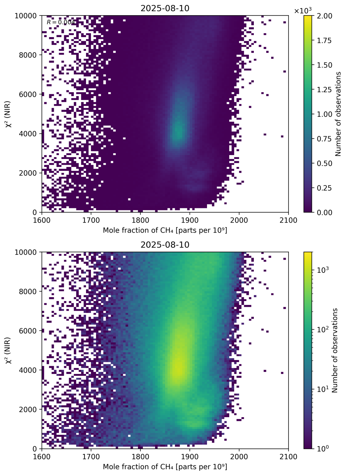
Figure 70: Scatter density plot of “Mole fraction of \text{CH}_4 ” against “ \chi^2 (NIR)” for 2025-08-09 to 2025-08-11.
