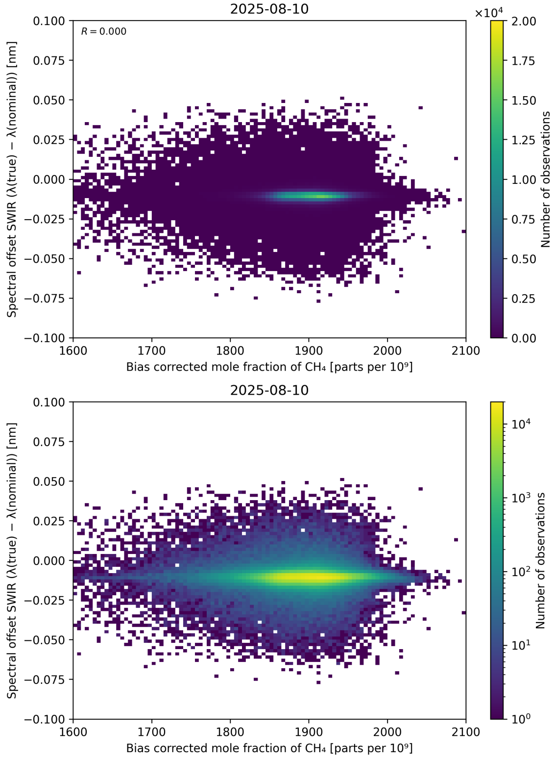
Figure 69: Scatter density plot of “Bias corrected mole fraction of \text{CH}_4 ” against “Spectral offset SWIR ( \lambda_{\text{true}} - \lambda_{\text{nominal}} )” for 2025-08-09 to 2025-08-11.
