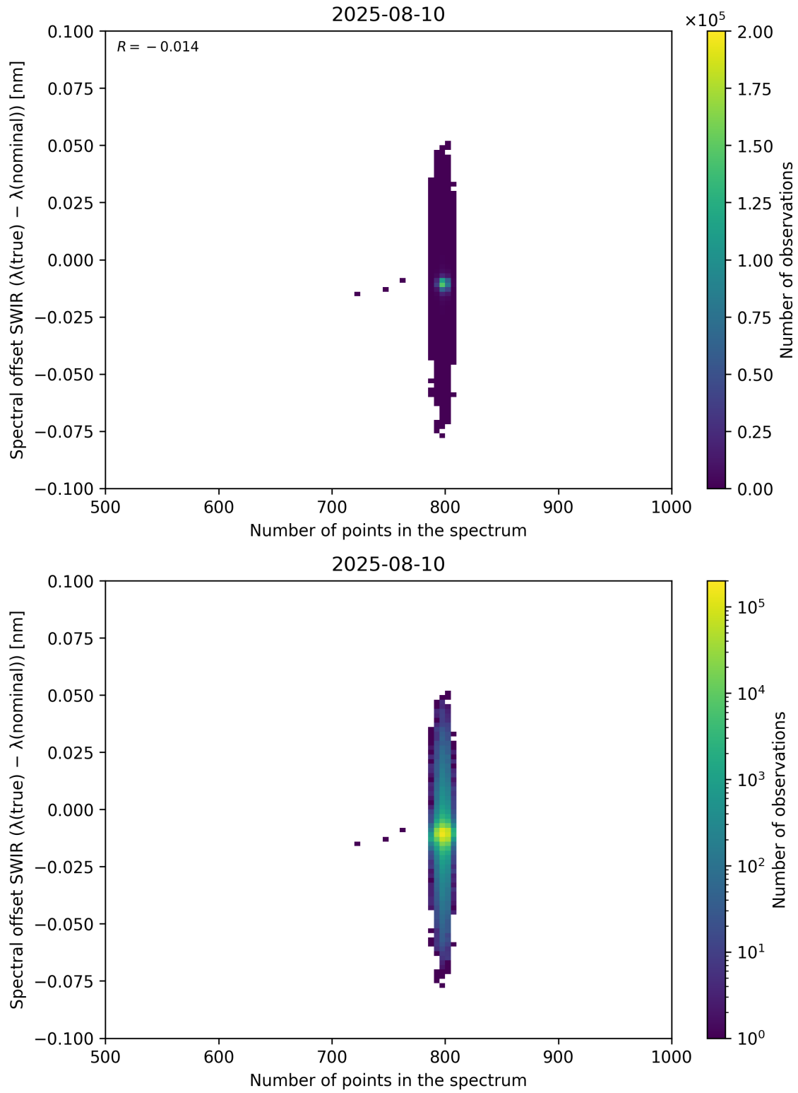
Figure 93: Scatter density plot of “Number of points in the spectrum” against “Spectral offset SWIR ( \lambda_{\text{true}} - \lambda_{\text{nominal}} )” for 2025-08-09 to 2025-08-11.
