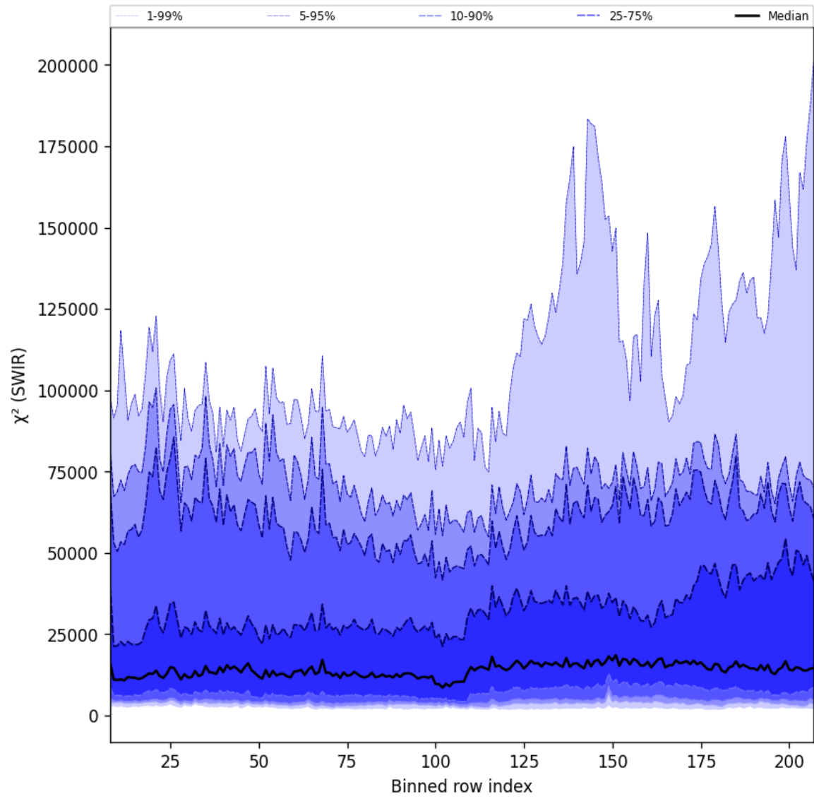
Figure 39: Along track statistics of “ \chi^2 (SWIR)” for 2025-08-09 to 2025-08-11
