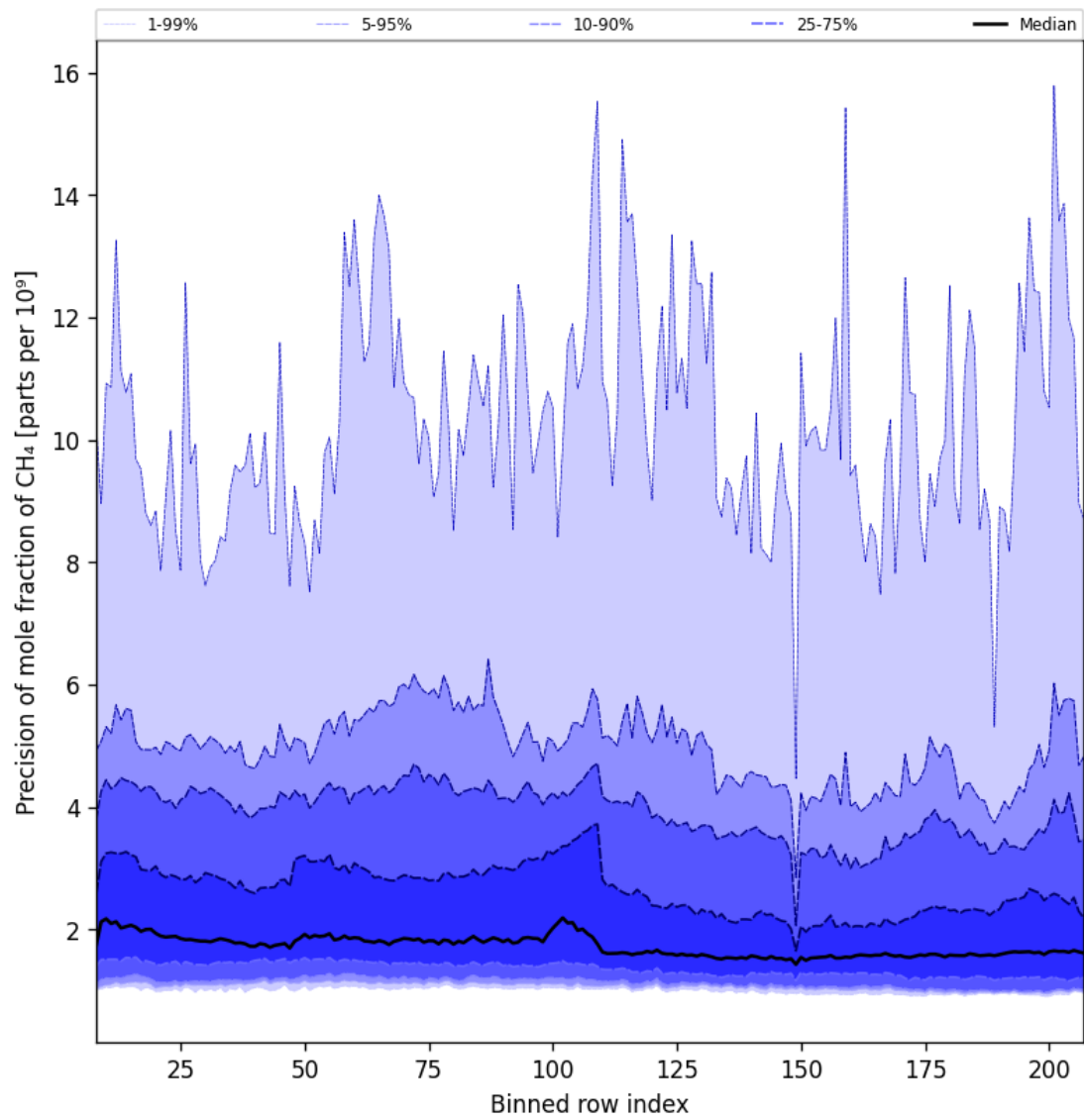
Figure 35: Along track statistics of “Precision of mole fraction of CH 4 ” for 2025-08-09 to 2025-08-11
