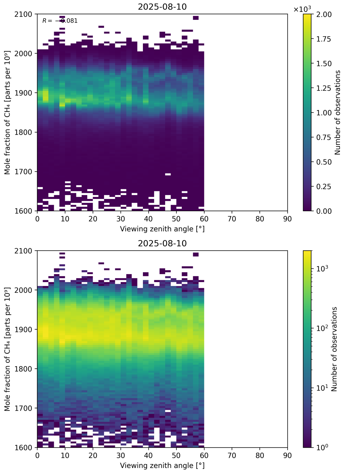
Figure 110: Scatter density plot of “Viewing zenith angle” against “Mole fraction of CH 4 ” for 2025-08-09 to 2025-08-11.
