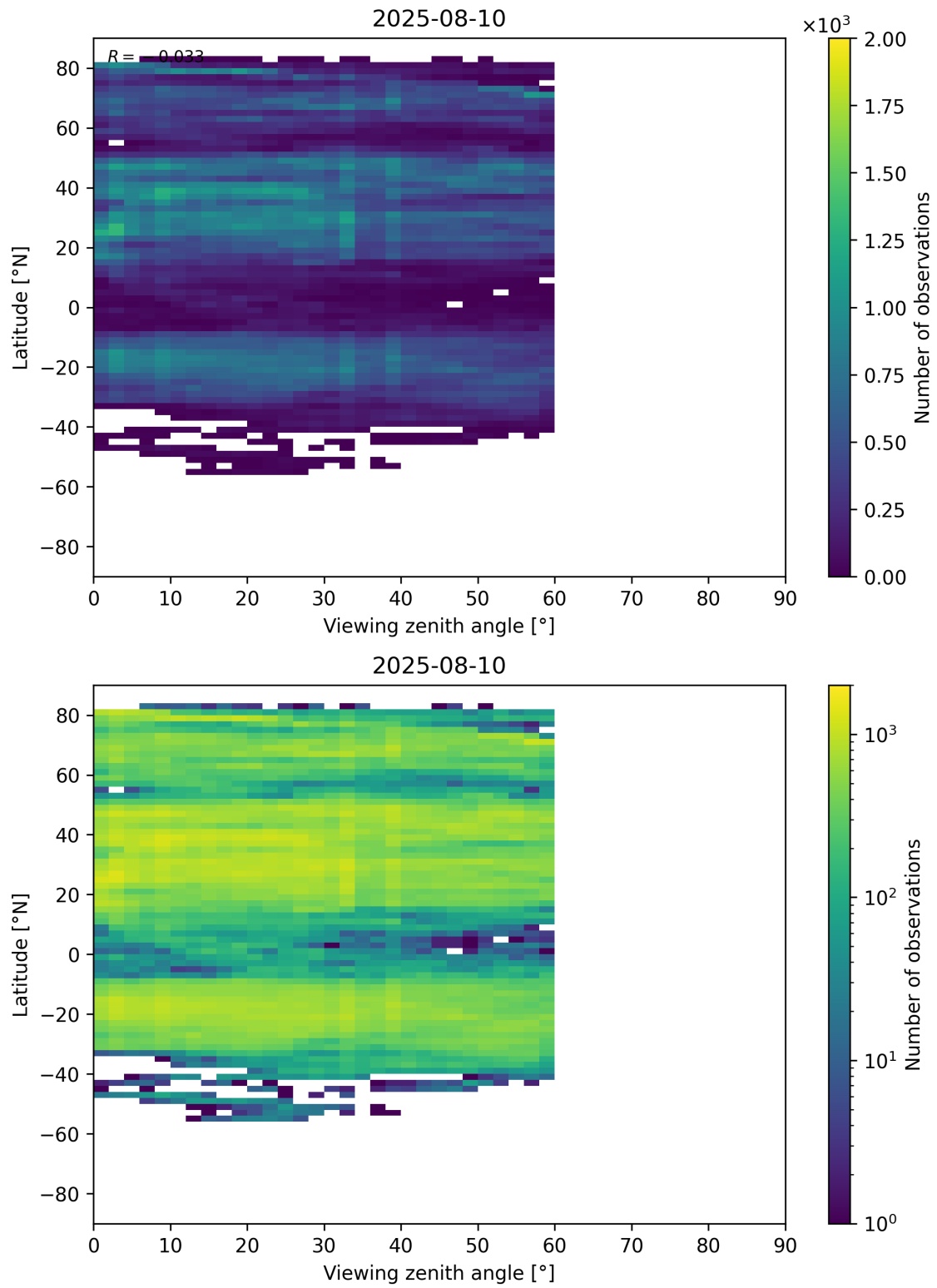
Figure 109: Scatter density plot of “Viewing zenith angle” against “Latitude” for 2025-08-09 to 2025-08-11.
