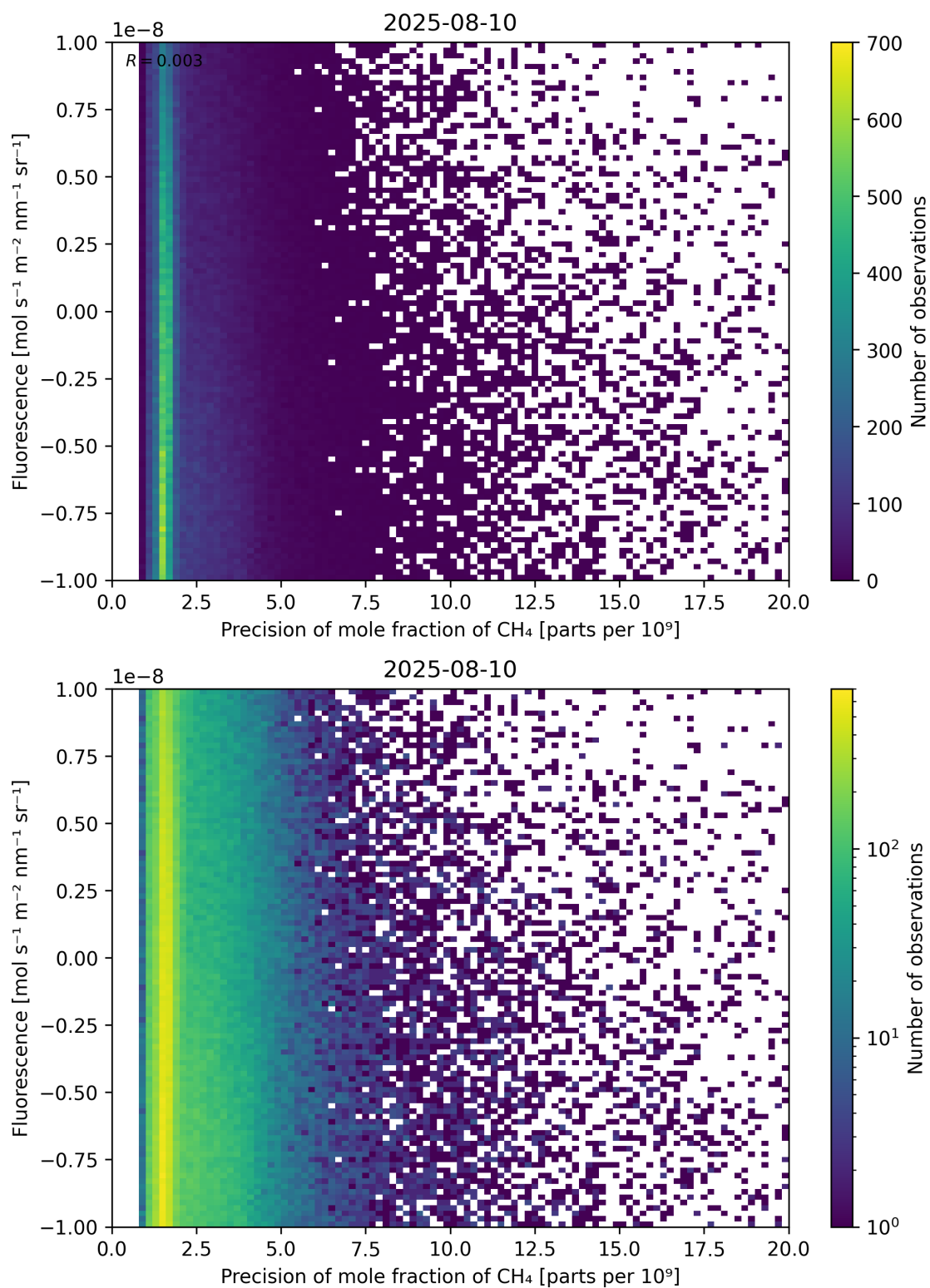
Figure 81: Scatter density plot of “Precision of mole fraction of \text{CH}_4 ” against “Fluorescence” for 2025-08-09 to 2025-08-11.
