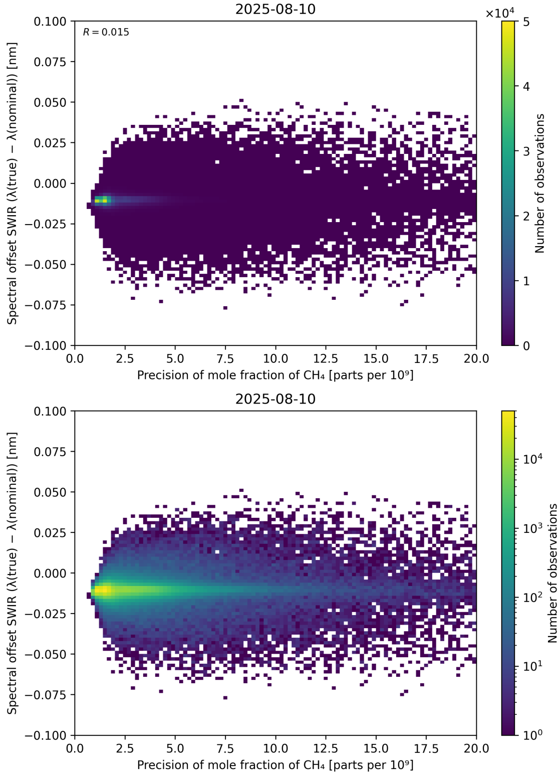
Figure 85: Scatter density plot of “Precision of mole fraction of \text{CH}_4 ” against “Spectral offset SWIR ( \lambda_{\text{true}} - \lambda_{\text{nominal}} )” for 2025-08-09 to 2025-08-11.
