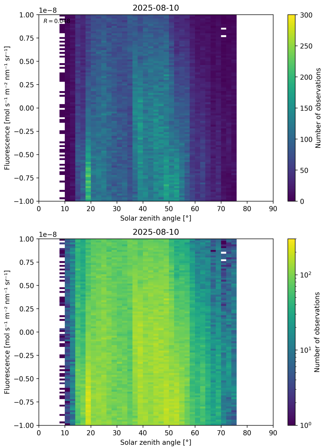
Figure 97: Scatter density plot of “Solar zenith angle” against “Fluorescence” for 2025-08-09 to 2025-08-11.
