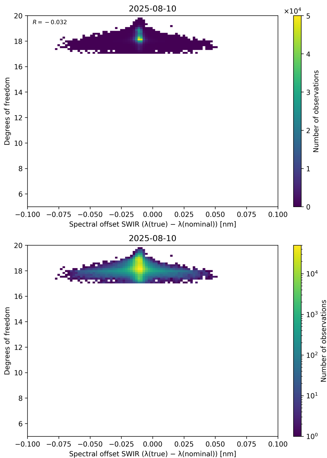
Figure 119: Scatter density plot of “Spectral offset SWIR ( \lambda_{\text{true}} - \lambda_{\text{nominal}} )” against “Degrees of freedom” for 2025-08-09 to 2025-08-11.
