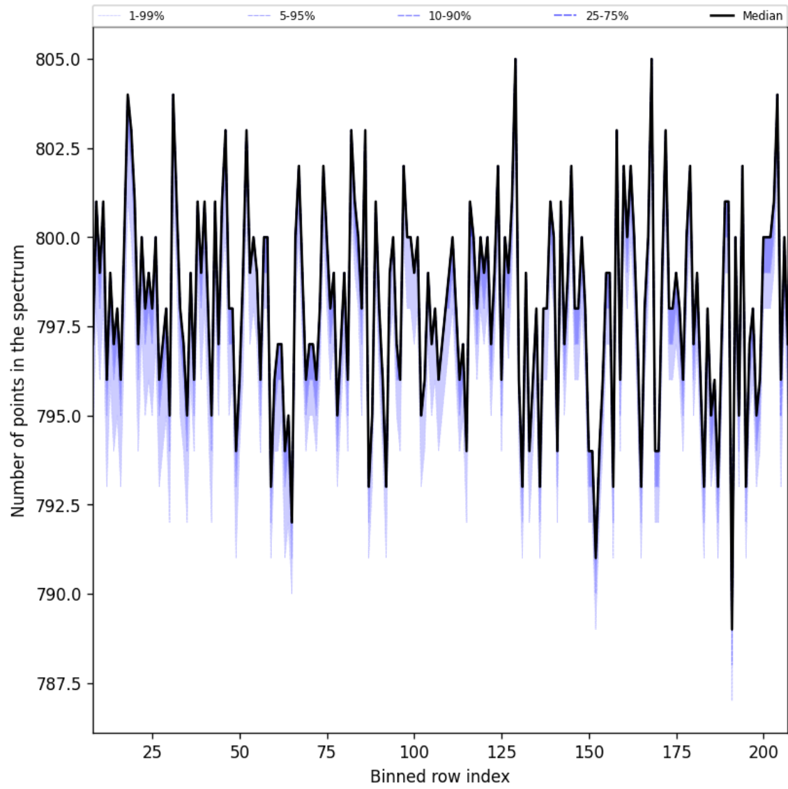
Figure 37: Along track statistics of “Number of points in the spectrum” for 2025-08-09 to 2025-08-11
