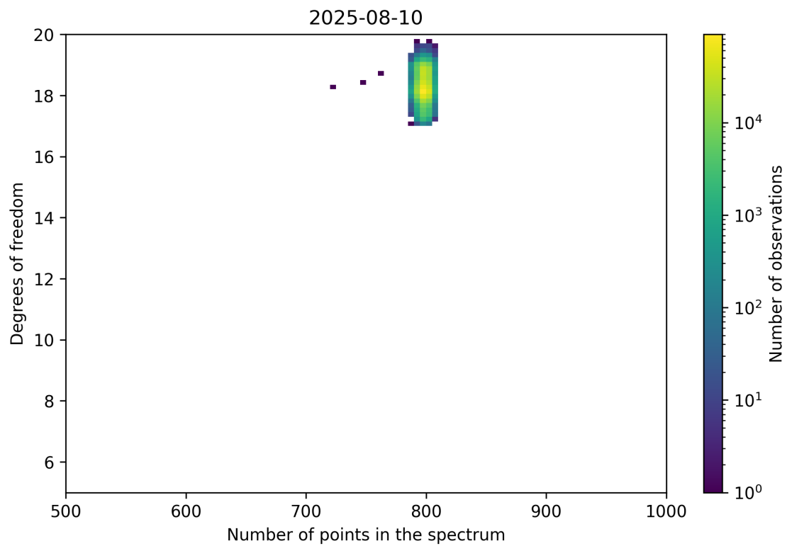
Figure 90: Scatter density plot of “Number of points in the spectrum” against “Degrees of freedom” for 2025-08-09 to 2025-08-11.
