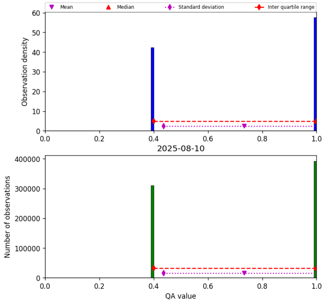
Figure 22: Histogram of “QA value” for 2025-08-09 to 2025-08-11
