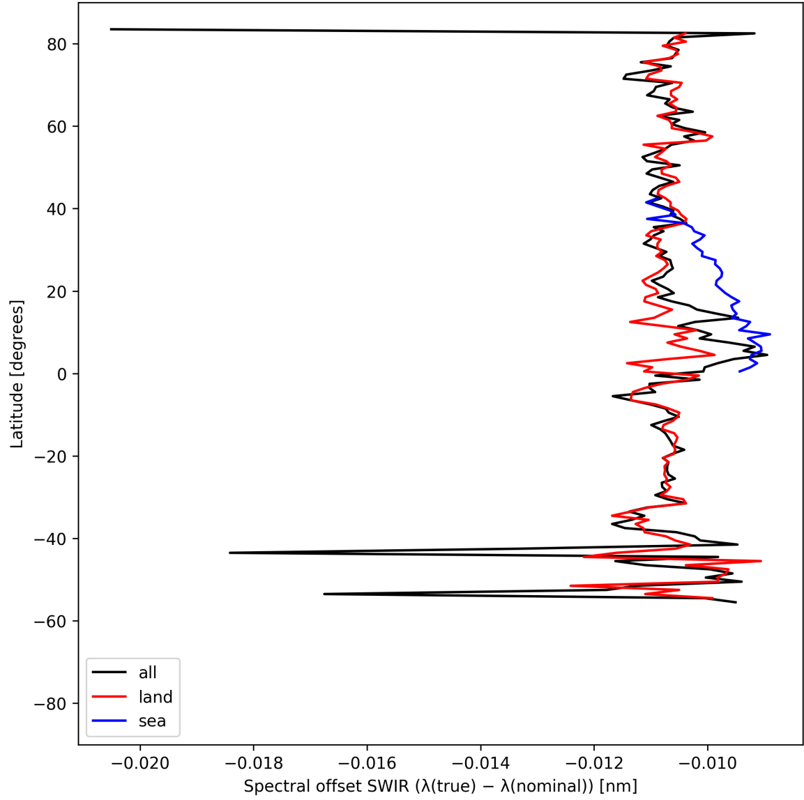
Figure 16: Zonal average of “Spectral offset SWIR ( \lambda_{\text{true}} - \lambda_{\text{nominal}} )” for 2025-08-09 to 2025-08-11.
