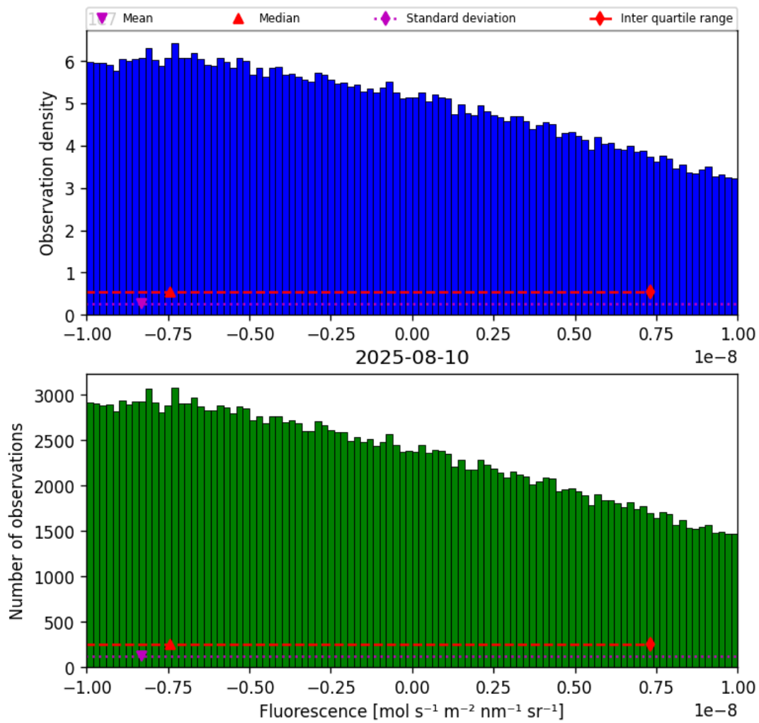
Figure 32: Histogram of “Fluorescence” for 2025-08-09 to 2025-08-11
