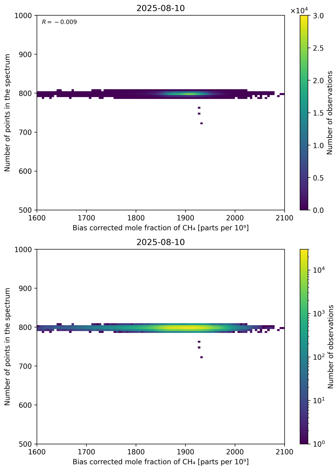
Figure 68: Scatter density plot of “Bias corrected mole fraction of CH 4 ” against “Number of points in the spectrum” for 2025-08-09 to 2025-08-11.
