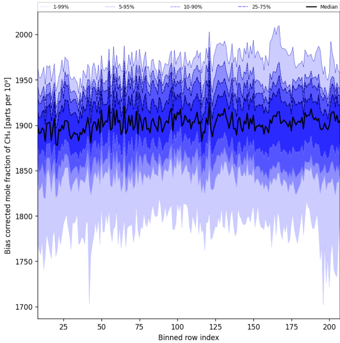
Figure 36: Along track statistics of “Bias corrected mole fraction of CH 4 ” for 2025-08-09 to 2025-08-11
