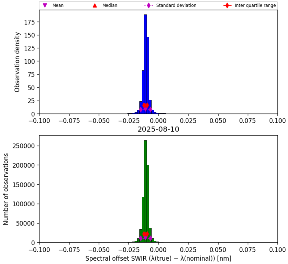
Figure 27: Histogram of “Spectral offset SWIR ( \lambda_{\text{true}} - \lambda_{\text{nominal}} )” for 2025-08-09 to 2025-08-11
