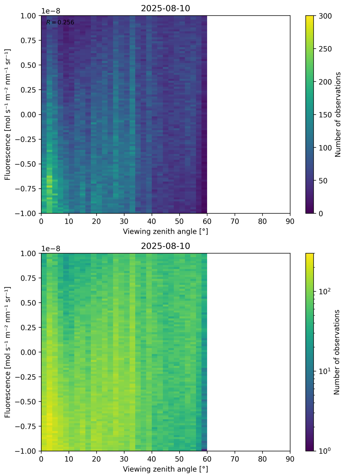
Figure 108: Scatter density plot of “Viewing zenith angle” against “Fluorescence” for 2025-08-09 to 2025-08-11.
