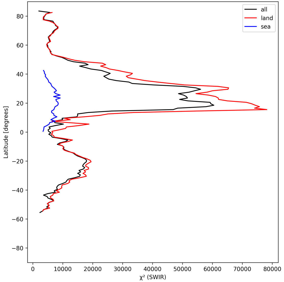
Figure 17: Zonal average of “ \chi^2 (SWIR)” for 2025-08-09 to 2025-08-11.
