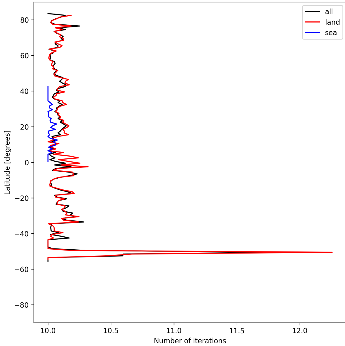
Figure 20: Zonal average of “Number of iterations” for 2025-08-09 to 2025-08-11.
