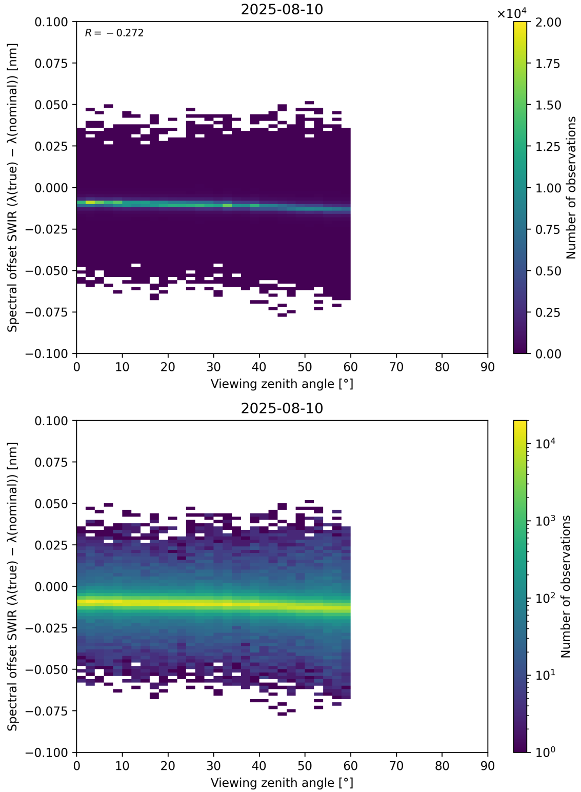
Figure 116: Scatter density plot of “Viewing zenith angle” against “Spectral offset SWIR ( \lambda_{\text{true}} - \lambda_{\text{nominal}} )” for 2025-08-09 to 2025-08-11.
