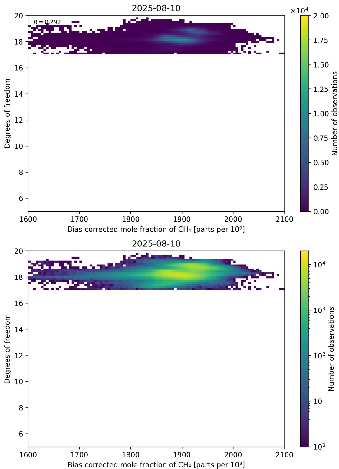
Figure 65: Scatter density plot of “Bias corrected mole fraction of CH 4 ” against “Degrees of freedom” for 2025-08-09 to 2025-08-11.
