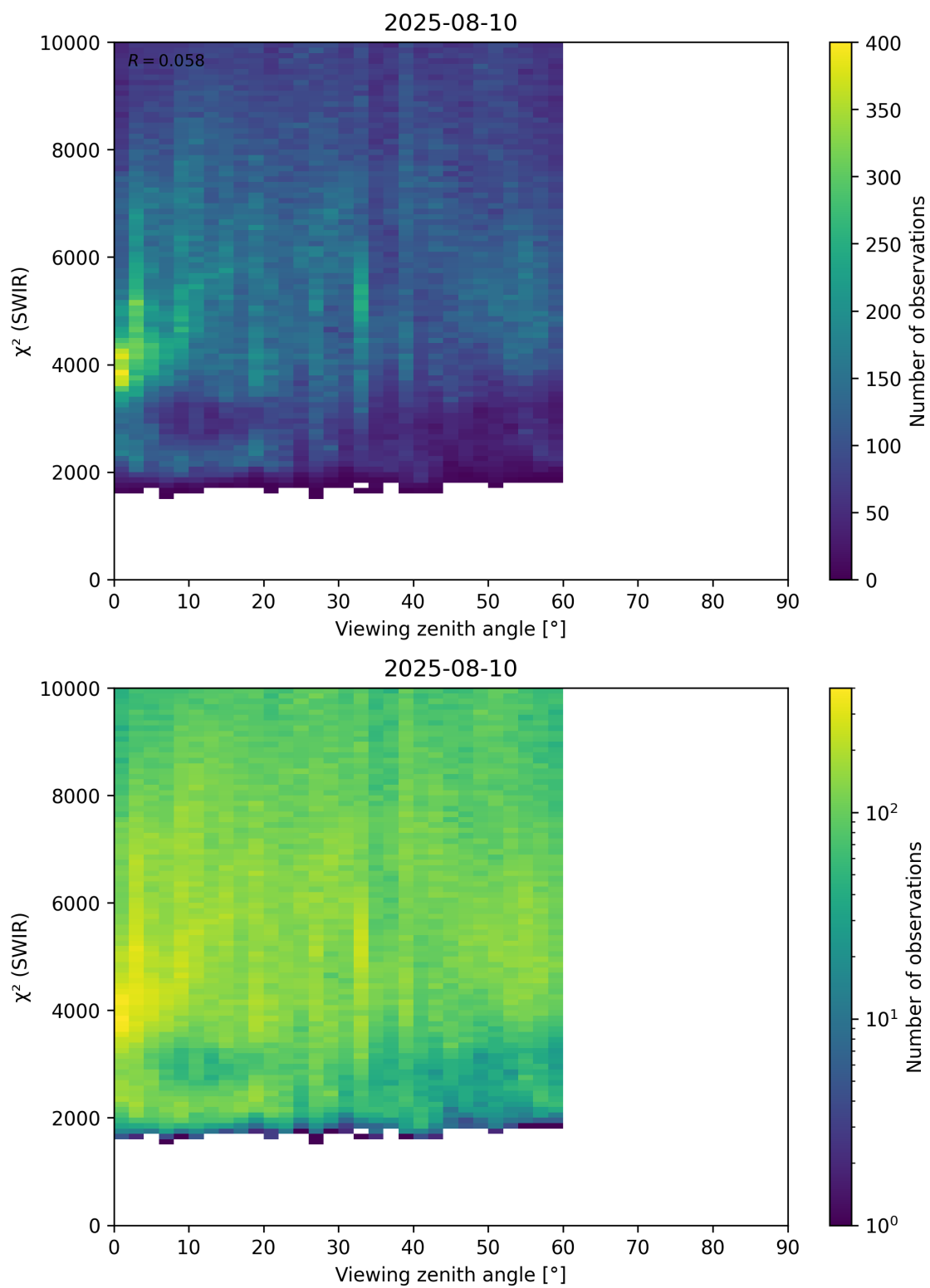
Figure 106: Scatter density plot of “Viewing zenith angle” against “ \chi^2 (SWIR)” for 2025-08-09 to 2025-08-11.
