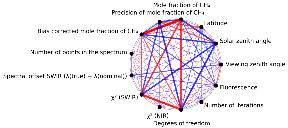
Figure 1: Map of correlation graph for 2025-08-09 to 2025-08-11.
