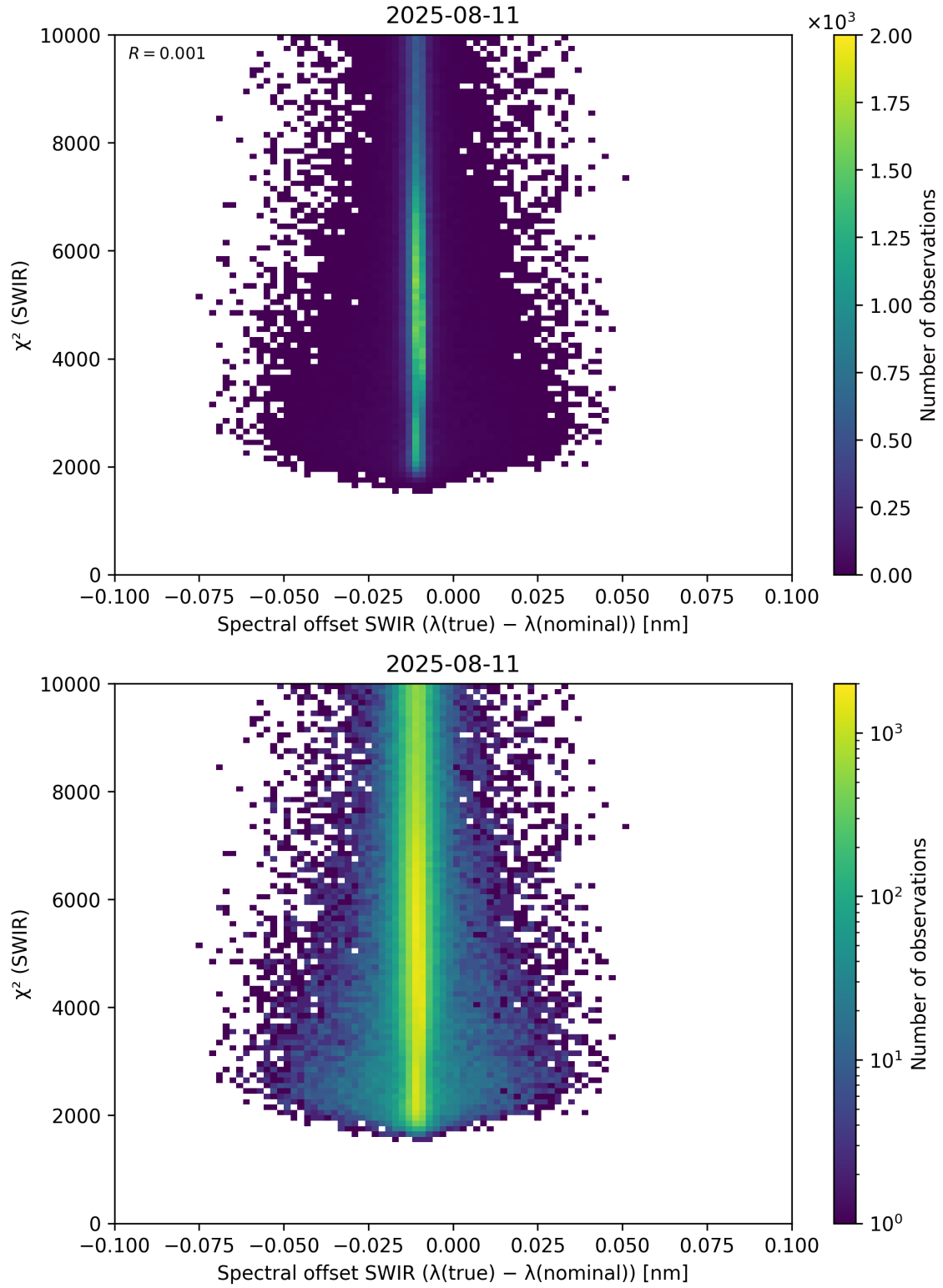
Figure 118: Scatter density plot of “Spectral offset SWIR ( \lambda_{\text{true}} - \lambda_{\text{nominal}} )” against “ \chi^2 (SWIR)” for 2025-08-10 to 2025-08-12.
