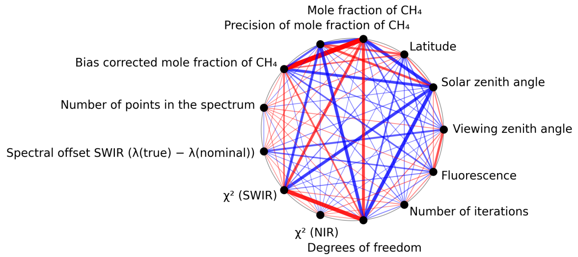
Figure 1: Map of correlation graph for 2025-08-10 to 2025-08-12.
