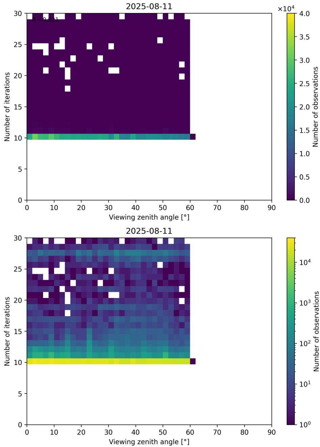
Figure 113: Scatter density plot of “Viewing zenith angle” against “Number of iterations” for 2025-08-10 to 2025-08-12.
