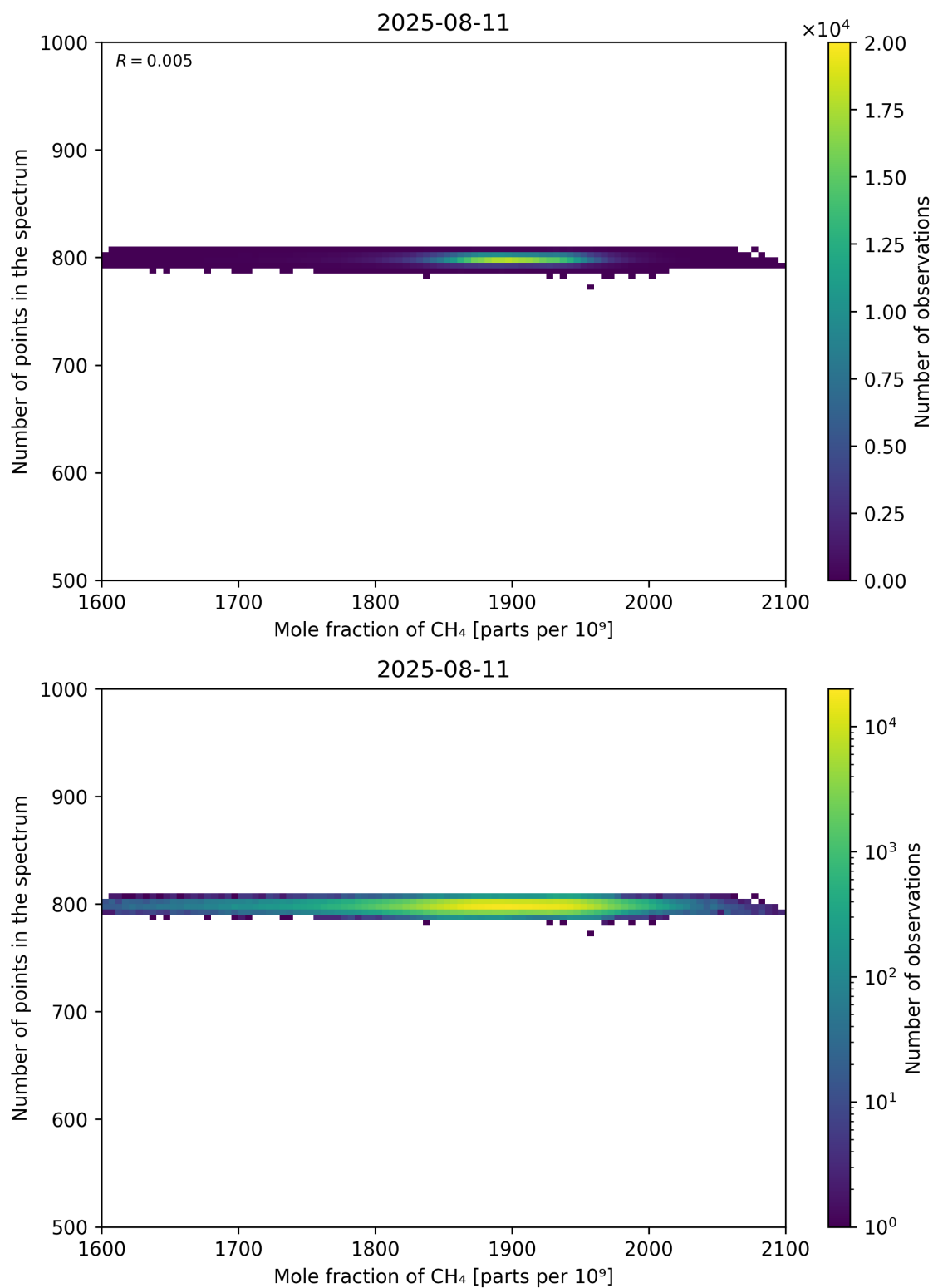
Figure 77: Scatter density plot of “Mole fraction of CH 4 ” against “Number of points in the spectrum” for 2025-08-10 to 2025-08-12.
