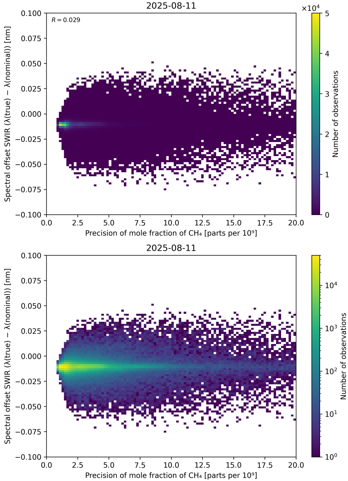
Figure 85: Scatter density plot of “Precision of mole fraction of CH 4 ” against “Spectral offset SWIR ( \lambda_{\text{true}} - \lambda_{\text{nominal}} )” for 2025-08-10 to 2025-08-12.
