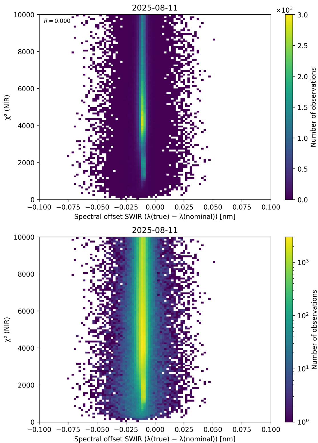
Figure 117: Scatter density plot of “Spectral offset SWIR ( \lambda_{\text{true}} - \lambda_{\text{nominal}} )” against “ \chi^2 (NIR)” for 2025-08-10 to 2025-08-12.
