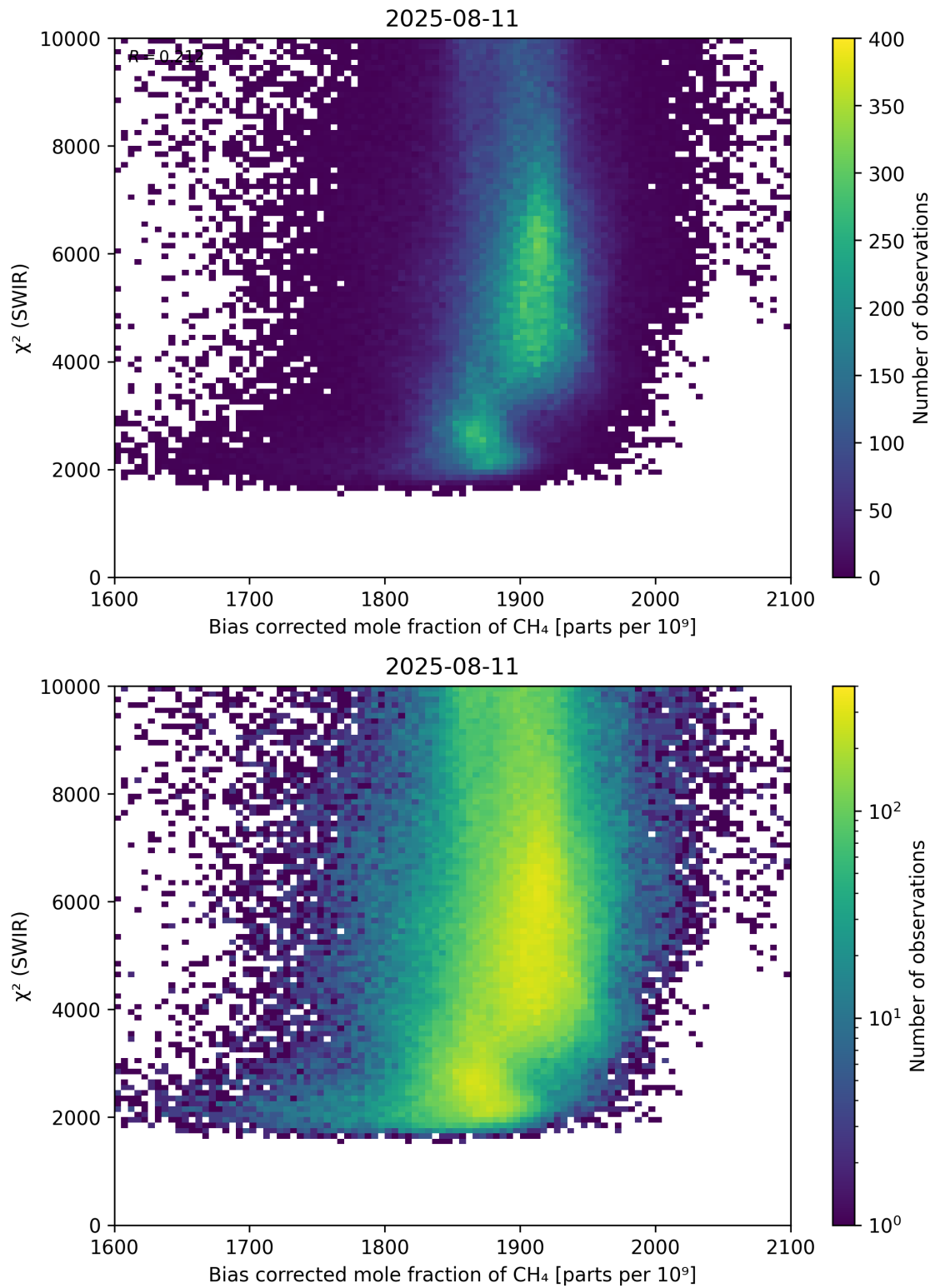
Figure 64: Scatter density plot of “Bias corrected mole fraction of CH 4 ” against “ \chi^2 (SWIR)” for 2025-08-10 to 2025-08-12.
