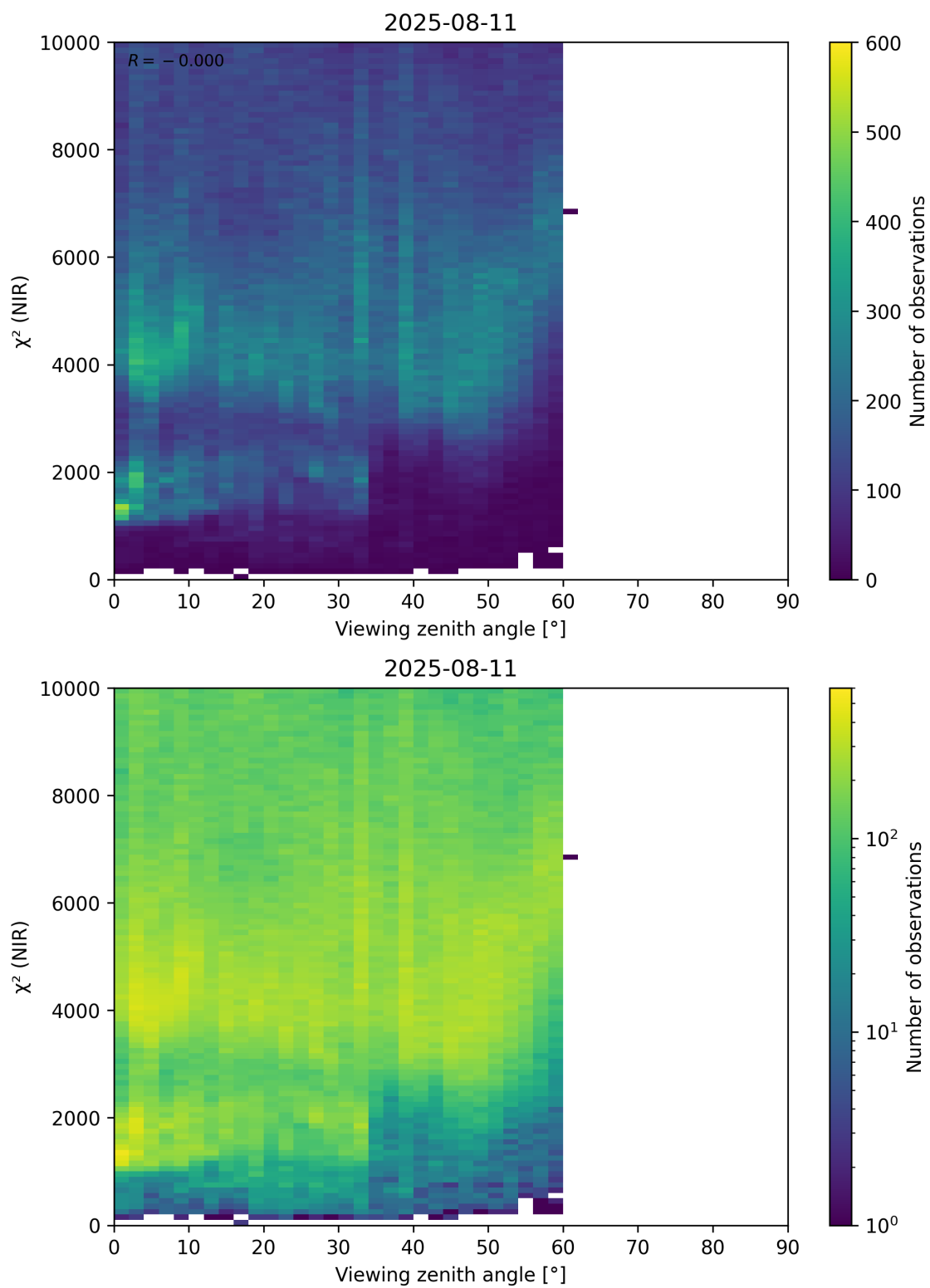
Figure 105: Scatter density plot of “Viewing zenith angle” against “ \chi^2 (NIR)” for 2025-08-10 to 2025-08-12.
