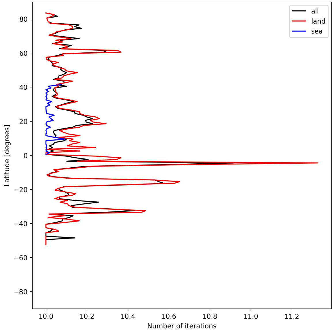
Figure 20: Zonal average of “Number of iterations” for 2025-08-10 to 2025-08-12.
