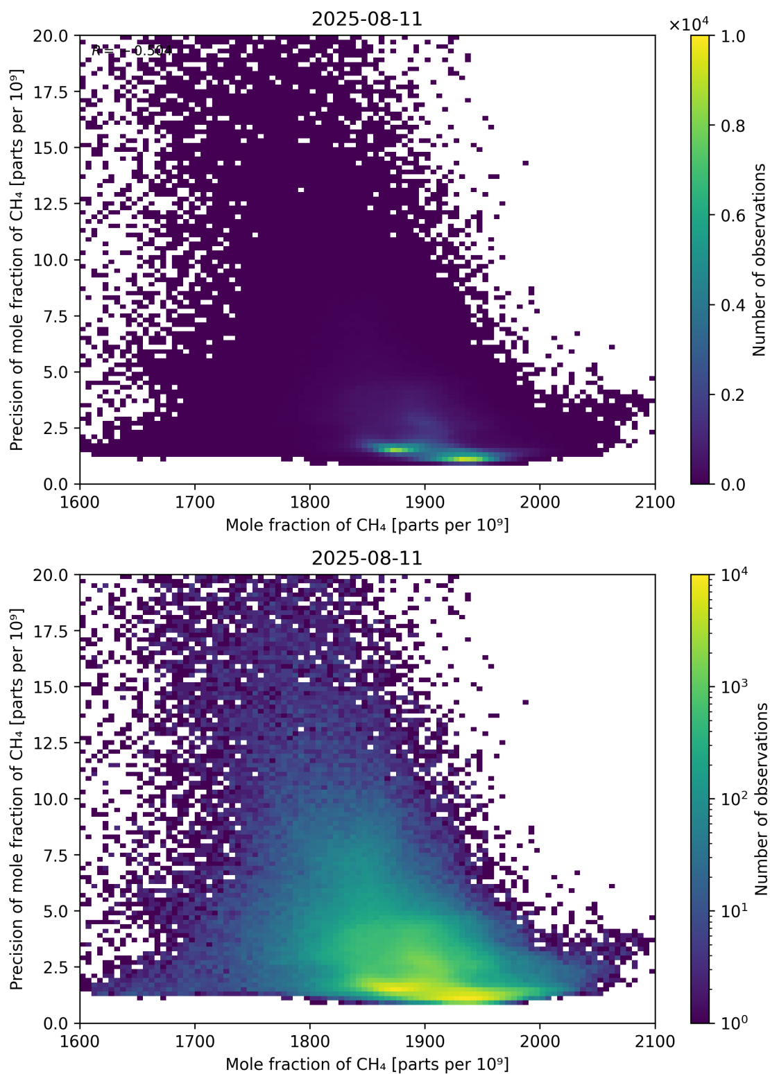
Figure 75: Scatter density plot of “Mole fraction of CH 4 ” against “Precision of mole fraction of CH 4 ” for 2025-08-10 to 2025-08-12.
