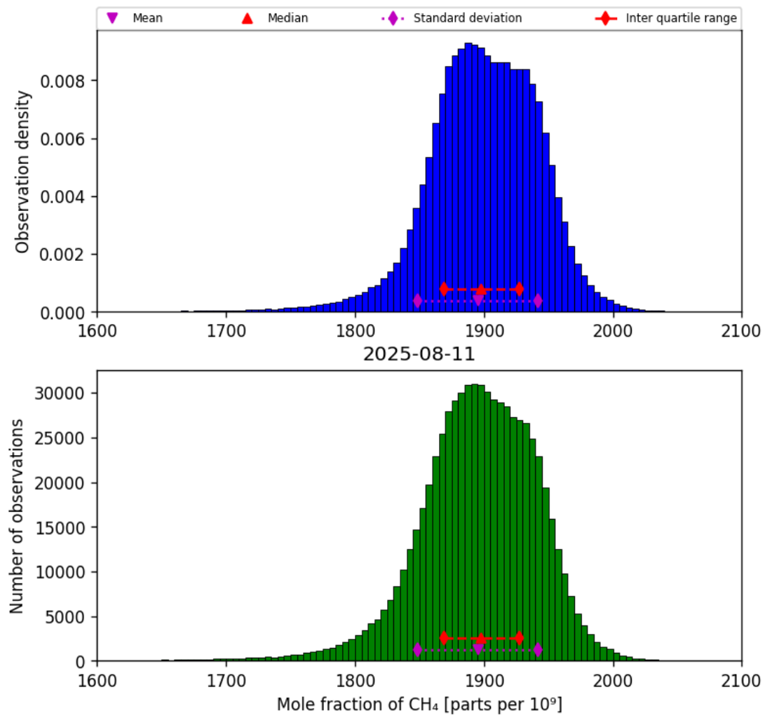
Figure 23: Histogram of “Mole fraction of CH 4 ” for 2025-08-10 to 2025-08-12
