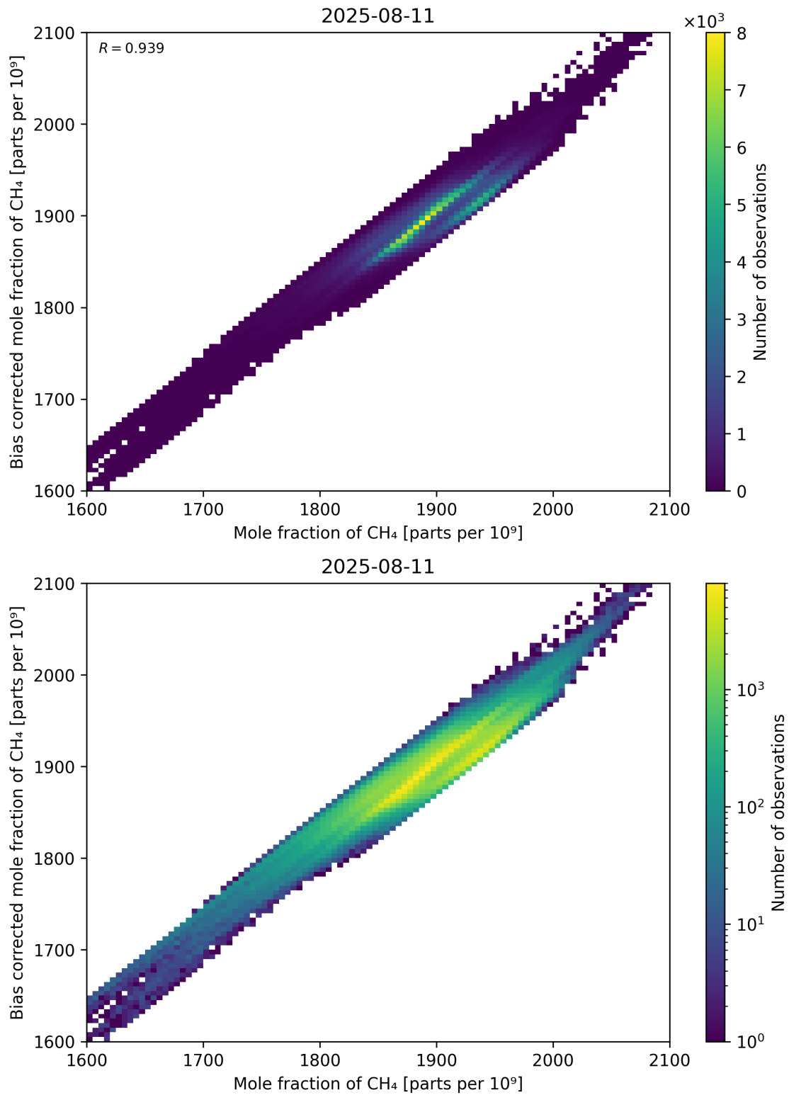
Figure 74: Scatter density plot of “Mole fraction of CH 4 ” against “Bias corrected mole fraction of CH 4 ” for 2025-08-10 to 2025-08-12.
