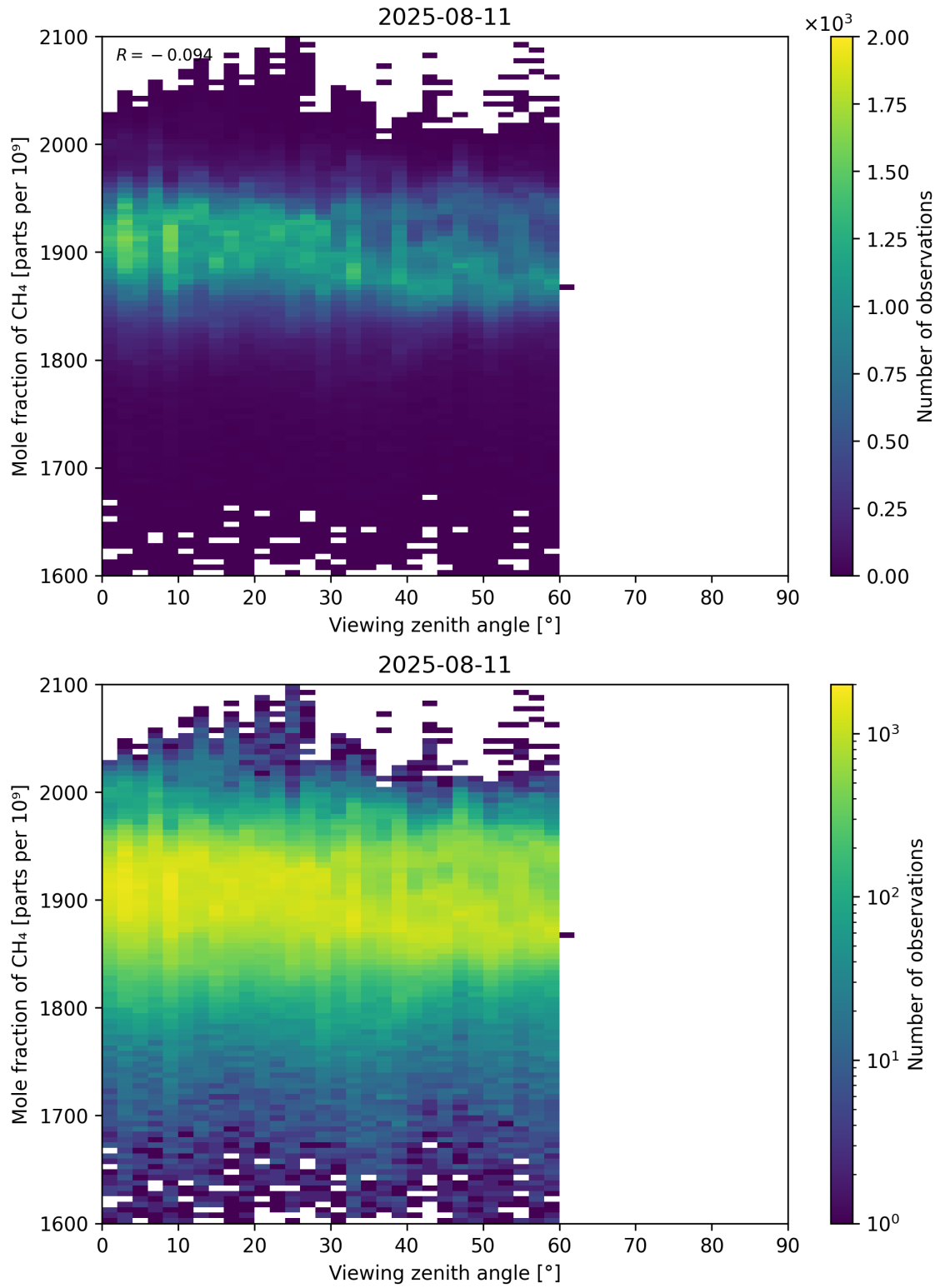
Figure 110: Scatter density plot of “Viewing zenith angle” against “Mole fraction of CH 4 ” for 2025-08-10 to 2025-08-12.
