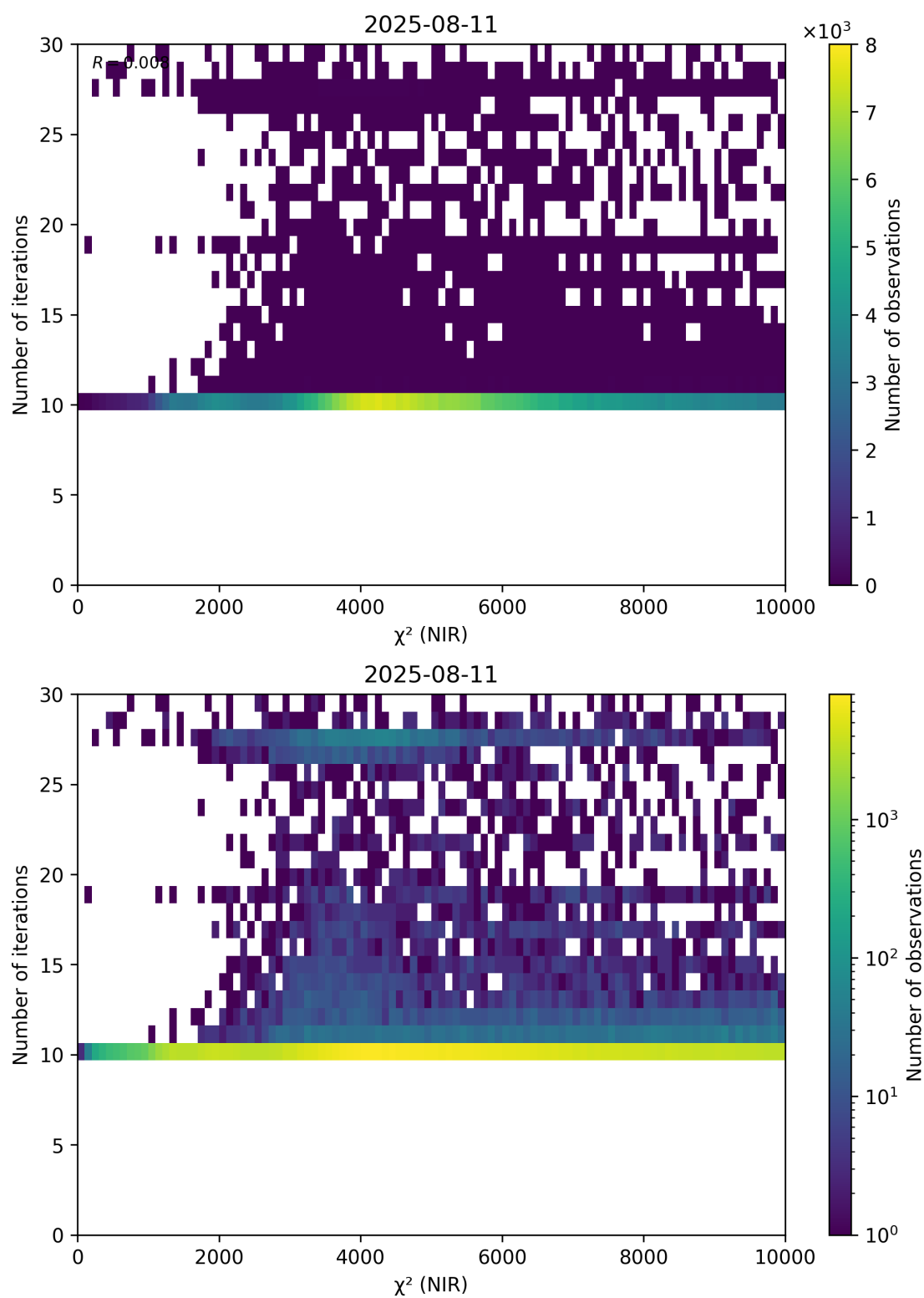
Figure 46: Scatter density plot of “ \chi^2 (NIR)” against “Number of iterations” for 2025-08-10 to 2025-08-12.
