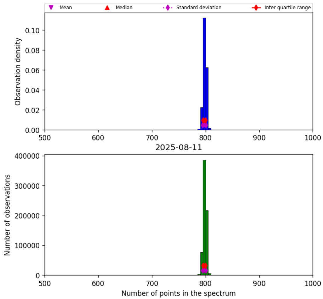
Figure 26: Histogram of “Number of points in the spectrum” for 2025-08-10 to 2025-08-12
