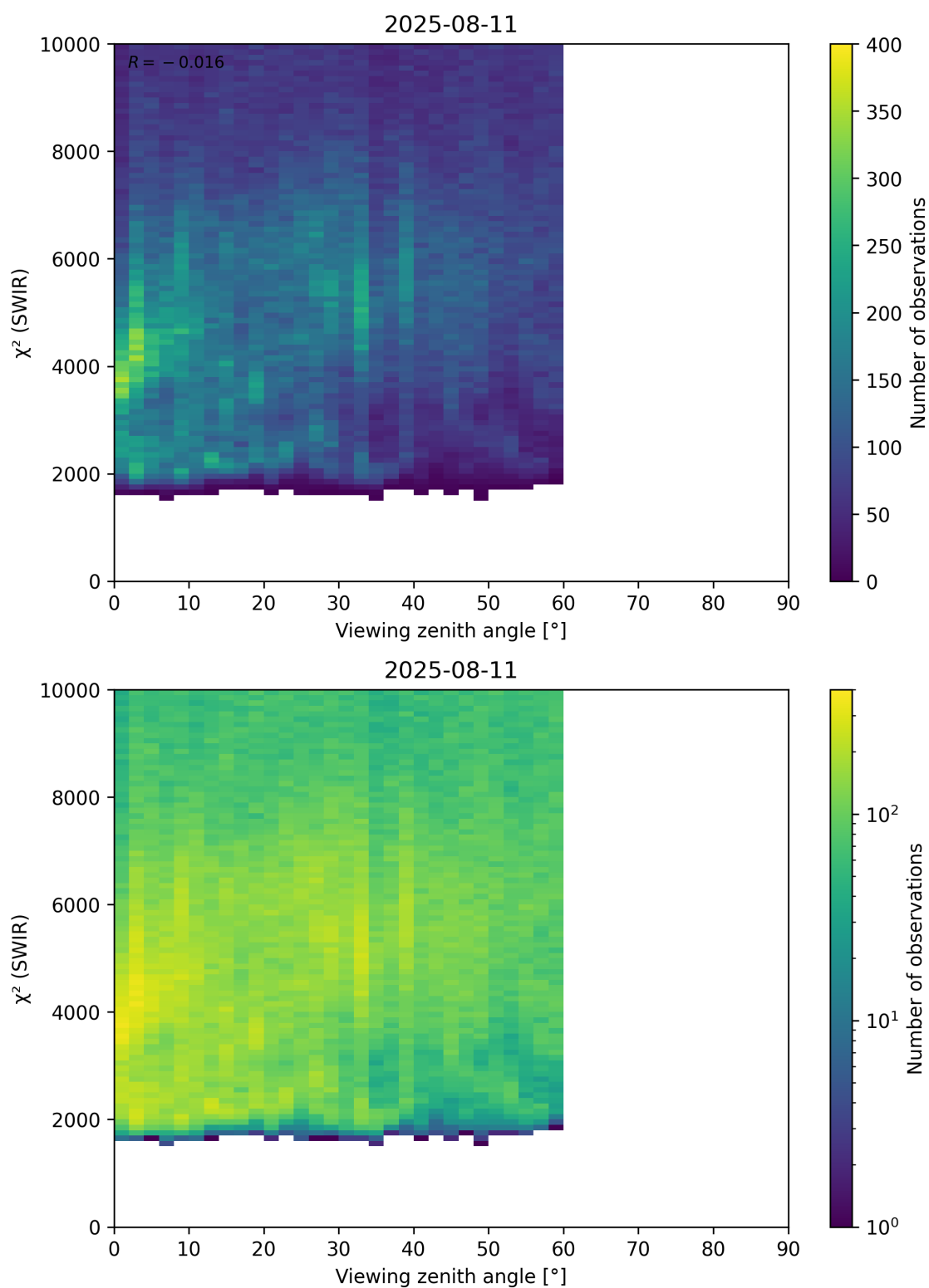
Figure 106: Scatter density plot of “Viewing zenith angle” against “ \chi^2 (SWIR)” for 2025-08-10 to 2025-08-12.
