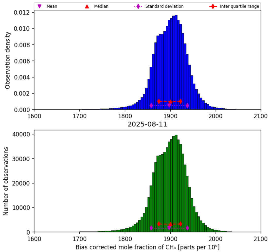
Figure 25: Histogram of “Bias corrected mole fraction of CH 4 ” for 2025-08-10 to 2025-08-12
