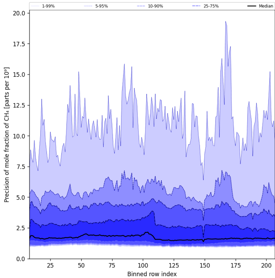
Figure 35: Along track statistics of “Precision of mole fraction of CH 4 ” for 2025-08-10 to 2025-08-12
