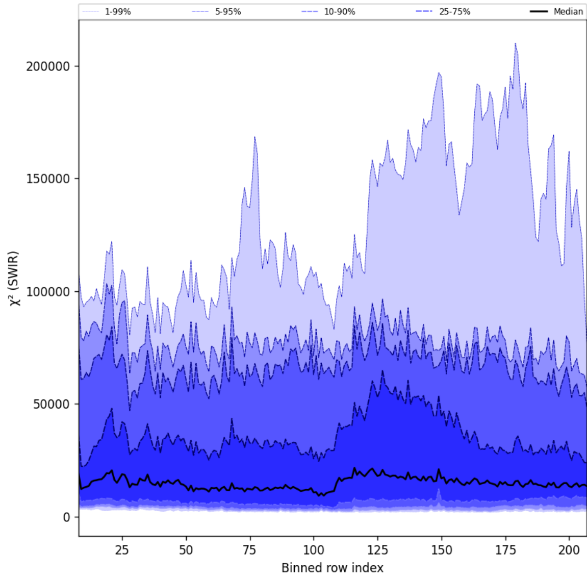
Figure 39: Along track statistics of “ \chi^2 (SWIR)” for 2025-08-10 to 2025-08-12
