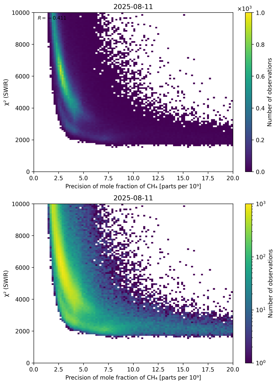
Figure 79: Scatter density plot of “Precision of mole fraction of \text{CH}_4 ” against “ \chi^2 (SWIR)” for 2025-08-10 to 2025-08-12.
