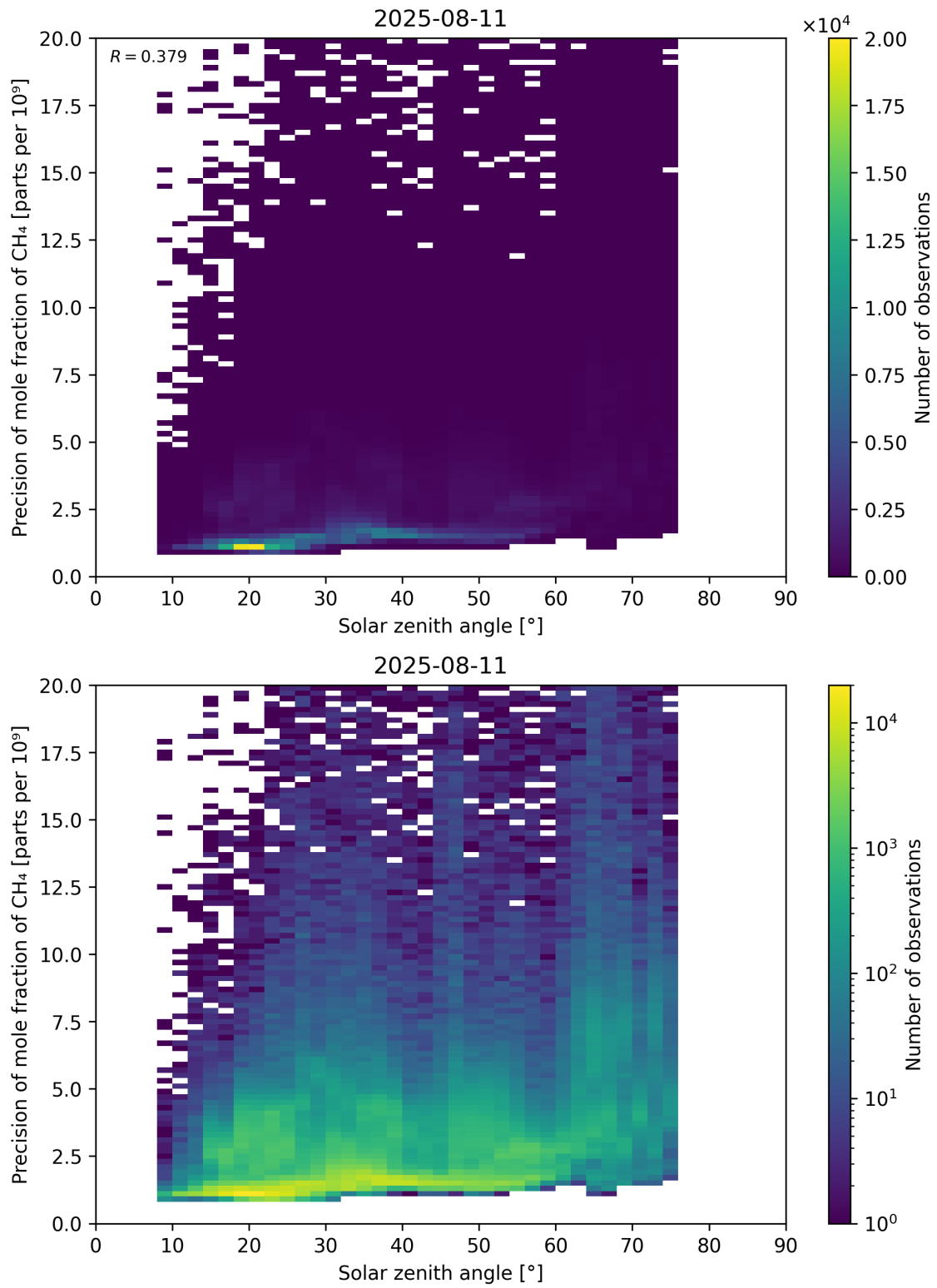
Figure 101: Scatter density plot of “Solar zenith angle” against “Precision of mole fraction of \text{CH}_4 ” for 2025-08-10 to 2025-08-12.
