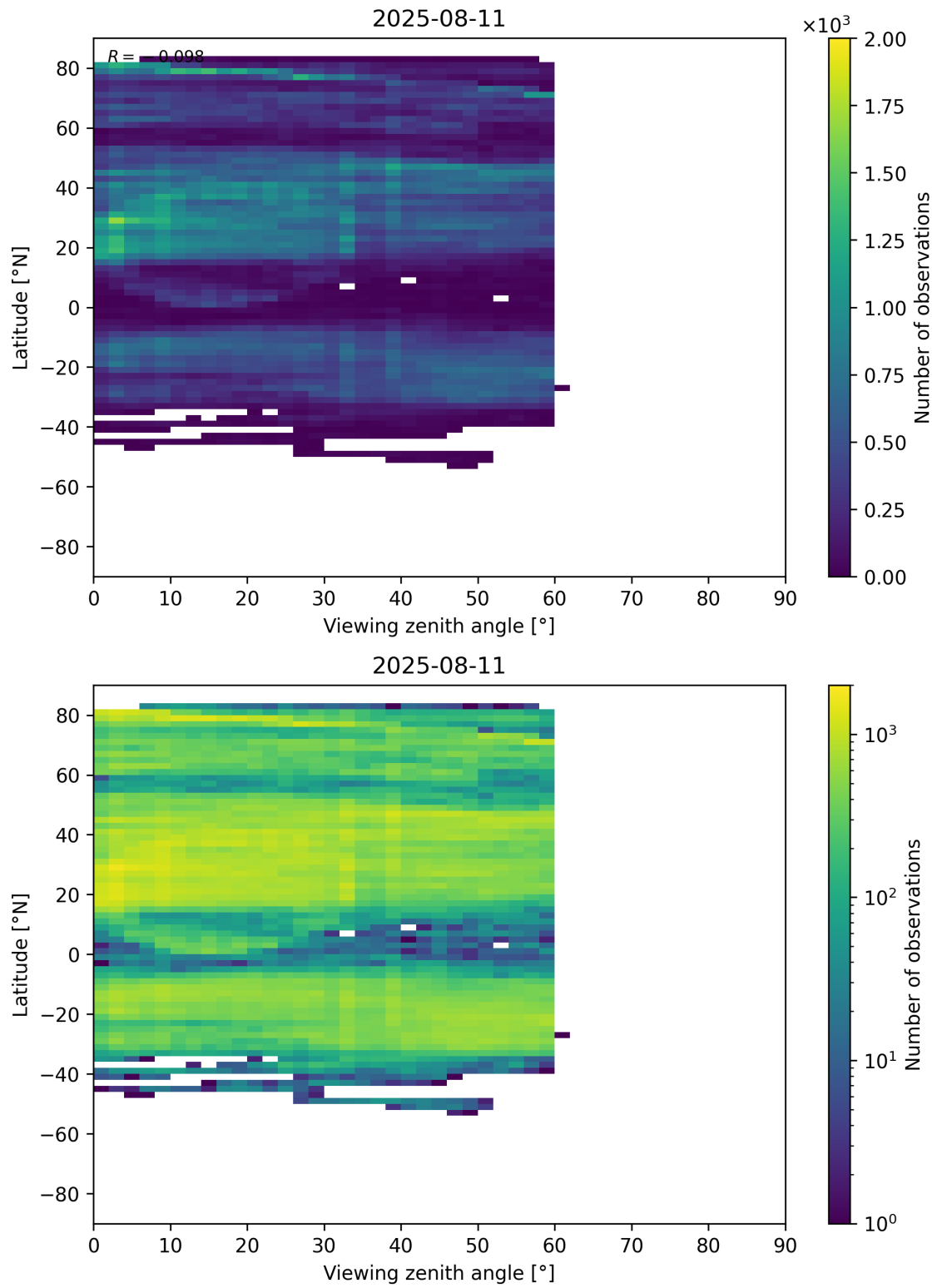
Figure 109: Scatter density plot of “Viewing zenith angle” against “Latitude” for 2025-08-10 to 2025-08-12.
