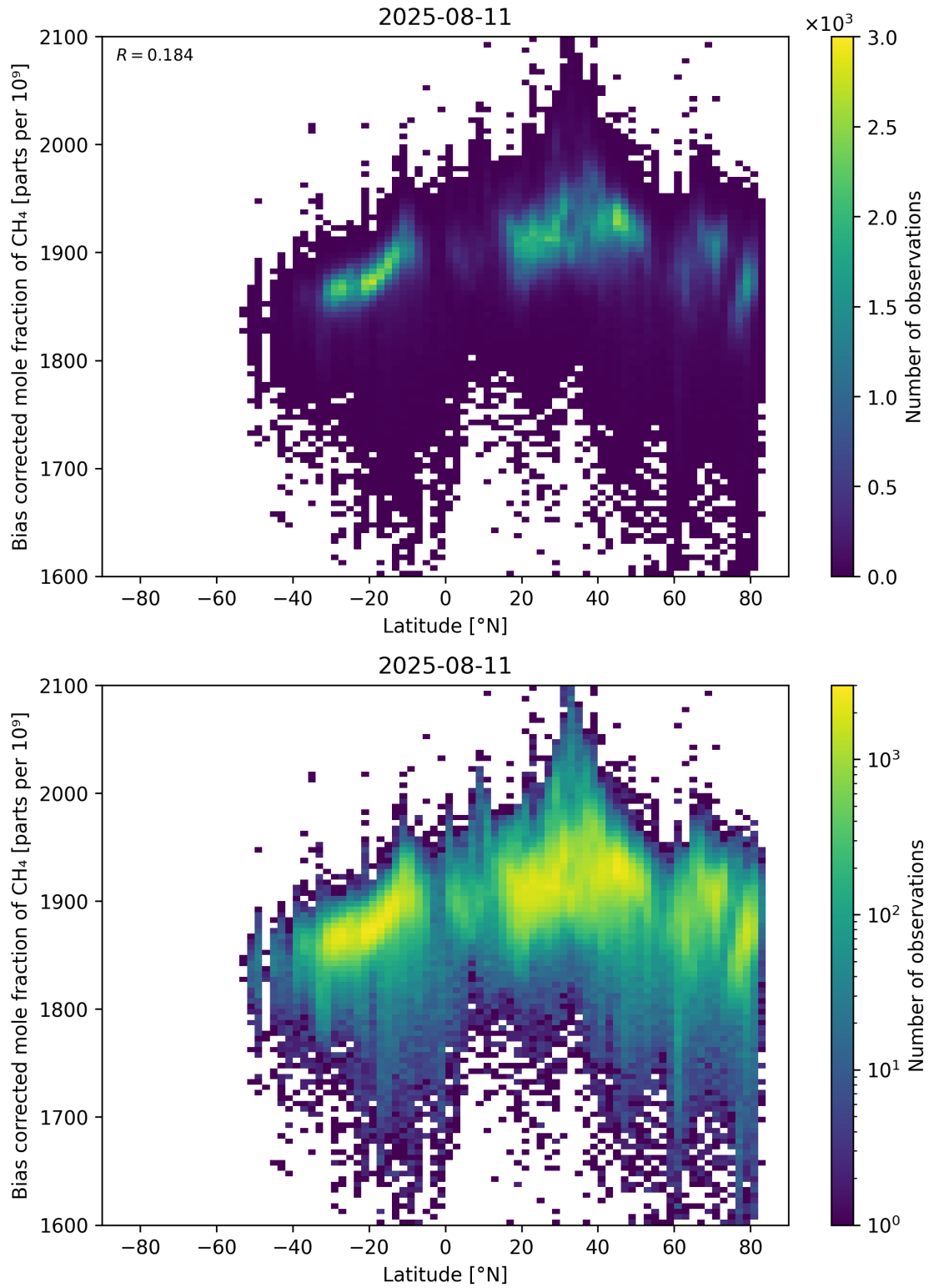
Figure 58: Scatter density plot of “Latitude” against “Bias corrected mole fraction of \text{CH}_4 ” for 2025-08-10 to 2025-08-12.
