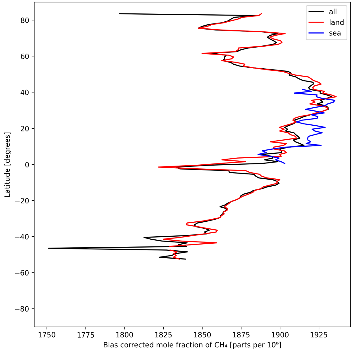
Figure 14: Zonal average of “Bias corrected mole fraction of \text{CH}_4 ” for 2025-08-10 to 2025-08-12.
