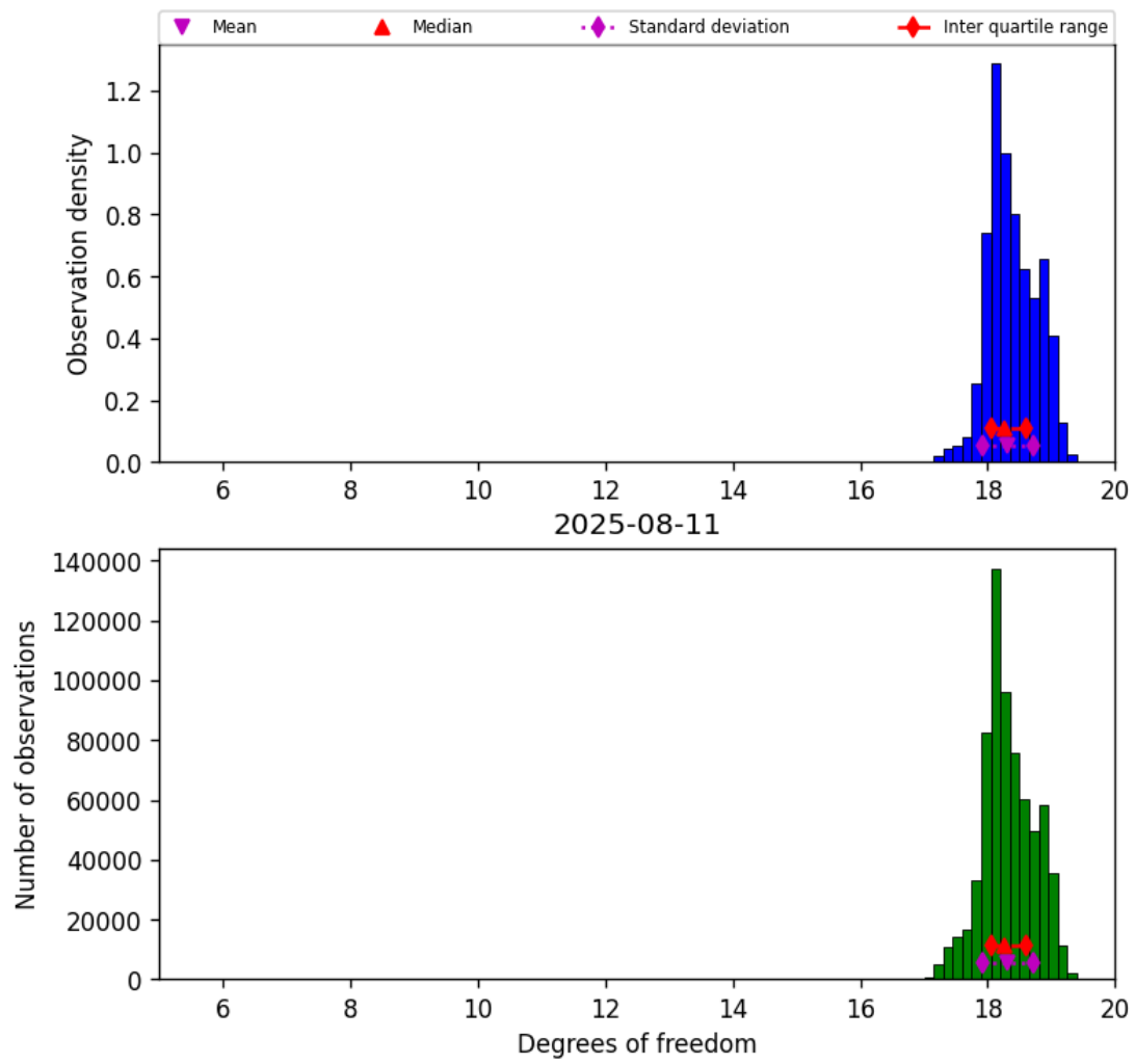
Figure 30: Histogram of “Degrees of freedom” for 2025-08-10 to 2025-08-12
