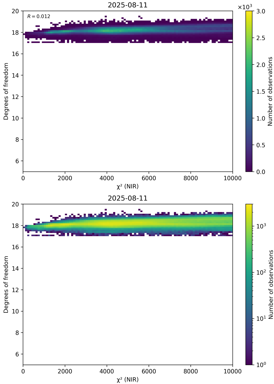
Figure 44: Scatter density plot of “ \chi^2 (NIR)” against “Degrees of freedom” for 2025-08-10 to 2025-08-12.
