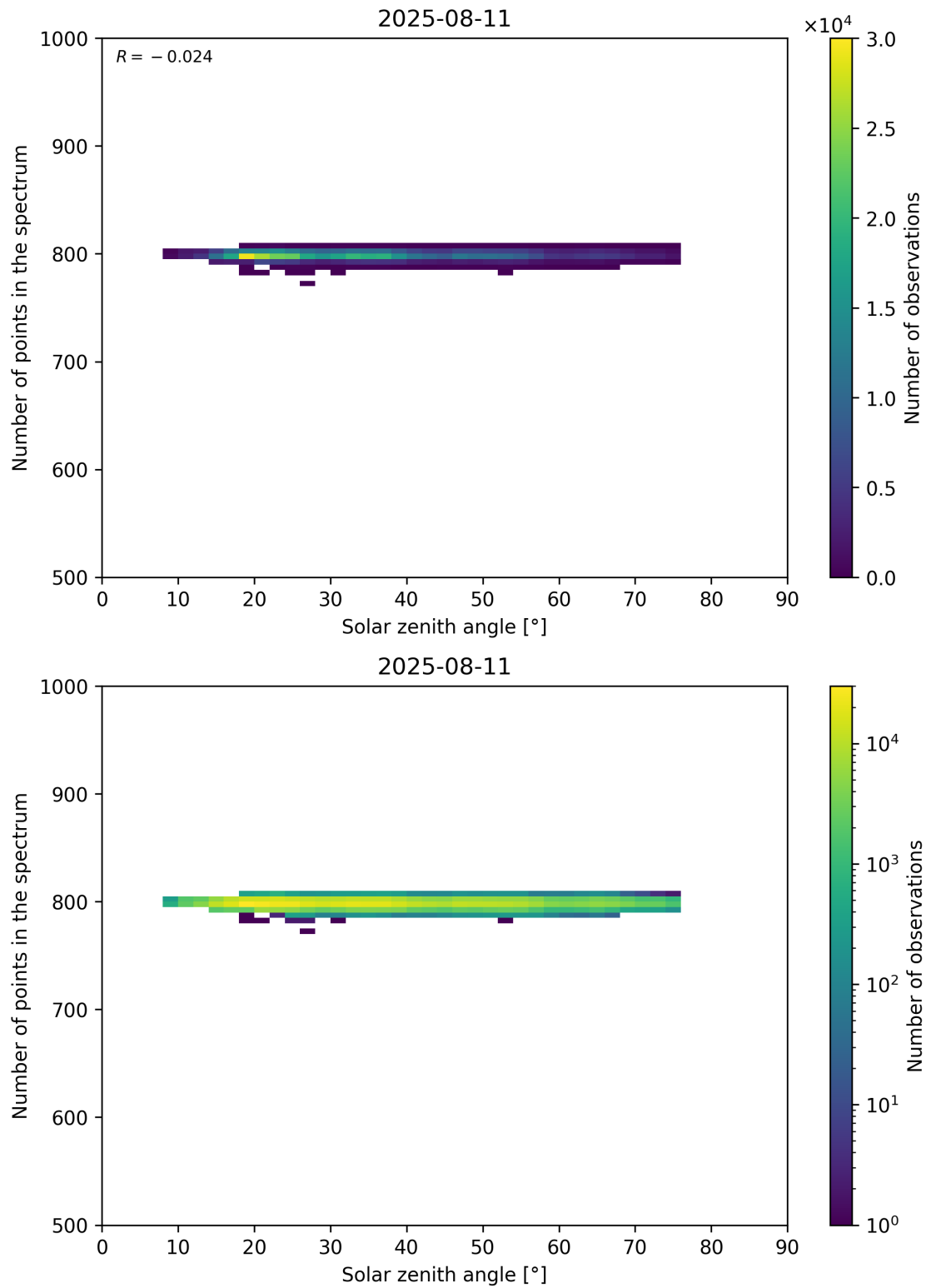
Figure 103: Scatter density plot of “Solar zenith angle” against “Number of points in the spectrum” for 2025-08-10 to 2025-08-12.
