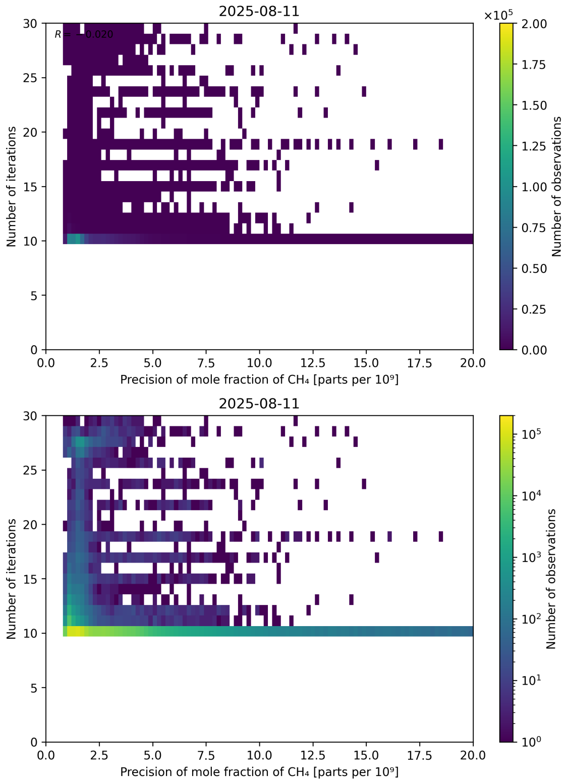
Figure 83: Scatter density plot of “Precision of mole fraction of CH 4 ” against “Number of iterations” for 2025-08-10 to 2025-08-12.
