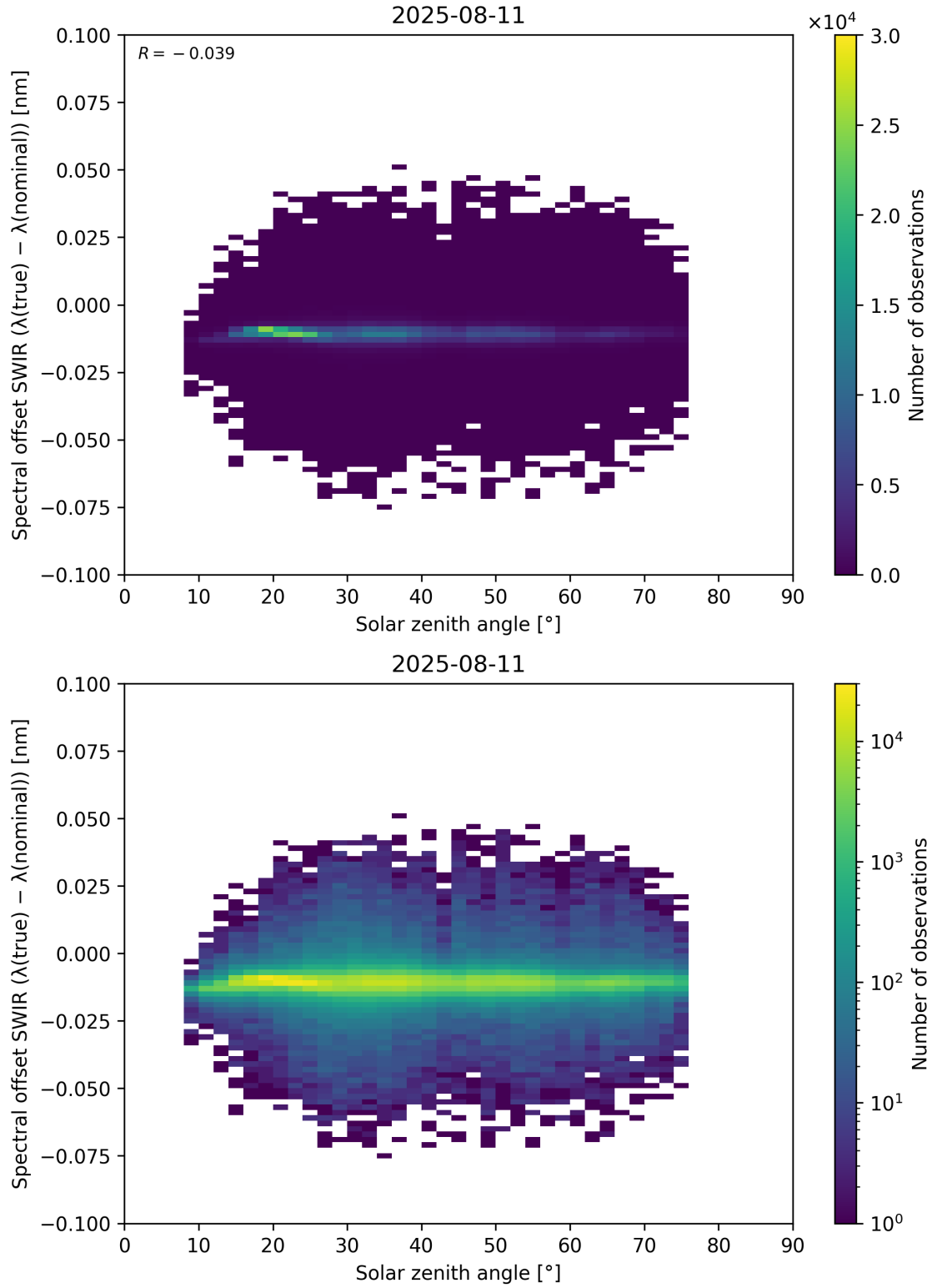
Figure 104: Scatter density plot of “Solar zenith angle” against “Spectral offset SWIR ( \lambda_{\text{true}} - \lambda_{\text{nominal}} )” for 2025-08-10 to 2025-08-12.
