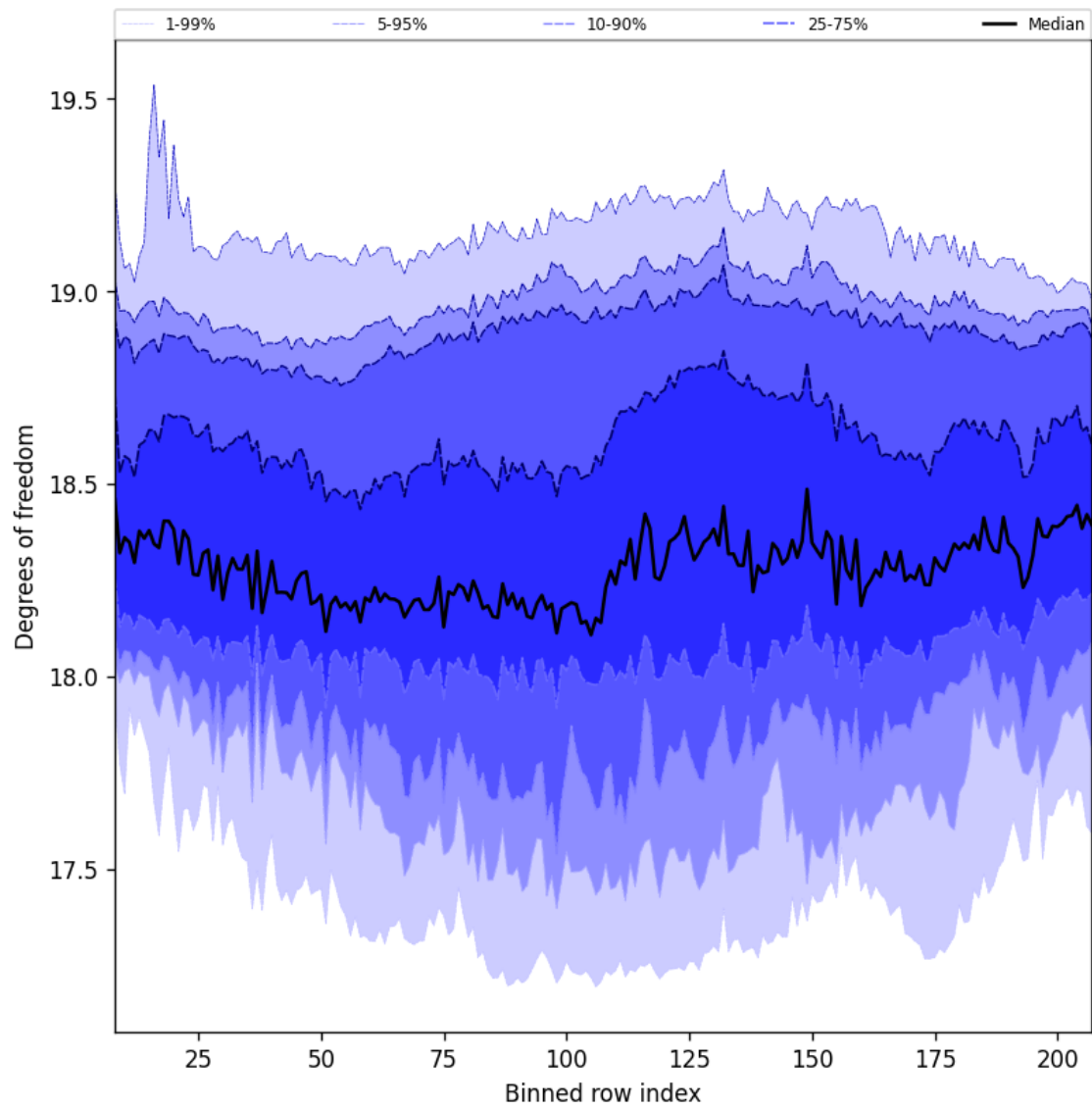
Figure 41: Along track statistics of “Degrees of freedom” for 2025-08-10 to 2025-08-12
