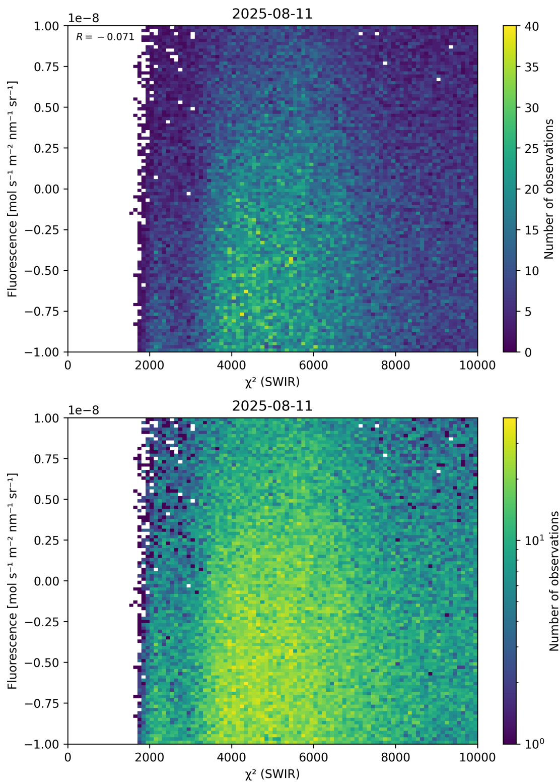
Figure 49: Scatter density plot of “ \chi^2 (SWIR)” against “Fluorescence” for 2025-08-10 to 2025-08-12.
