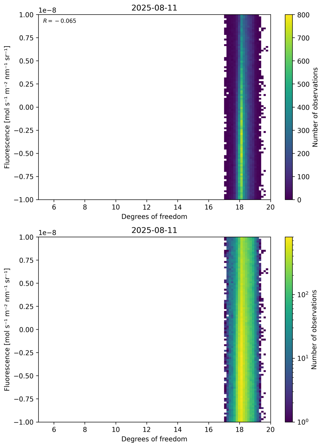
Figure 51: Scatter density plot of “Degrees of freedom” against “Fluorescence” for 2025-08-10 to 2025-08-12.
