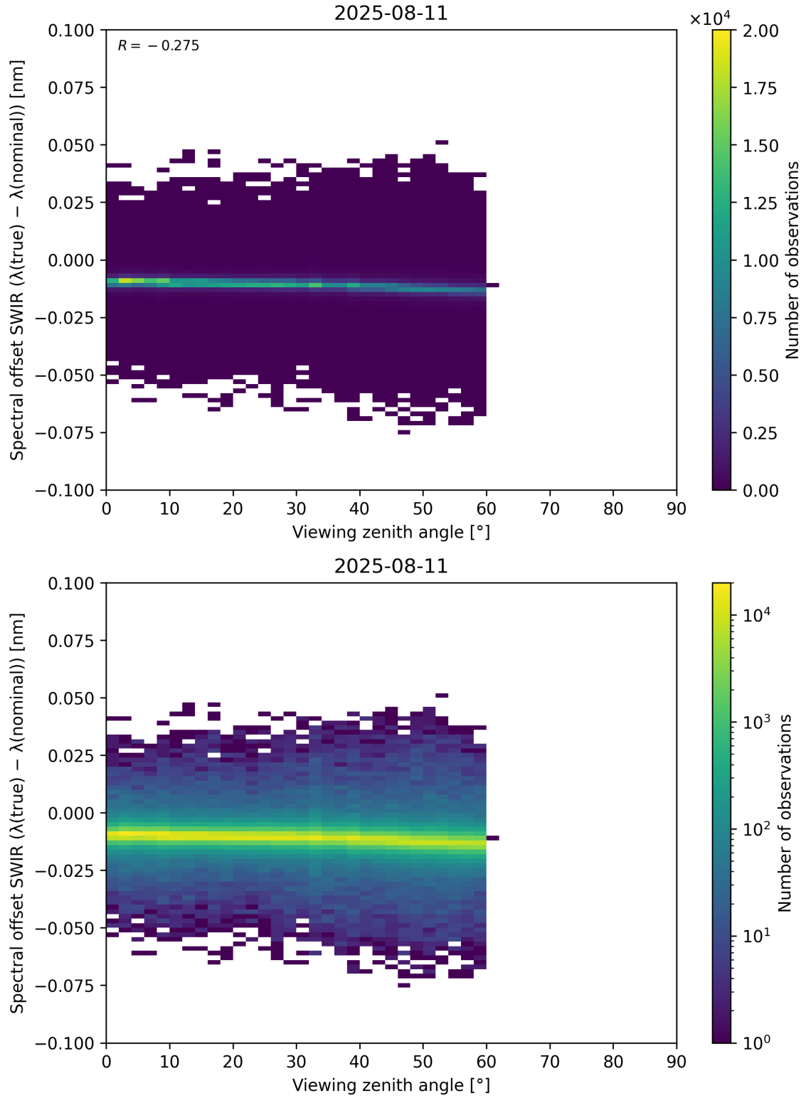
Figure 116: Scatter density plot of “Viewing zenith angle” against “Spectral offset SWIR ( \lambda_{\text{true}} - \lambda_{\text{nominal}} )” for 2025-08-10 to 2025-08-12.
