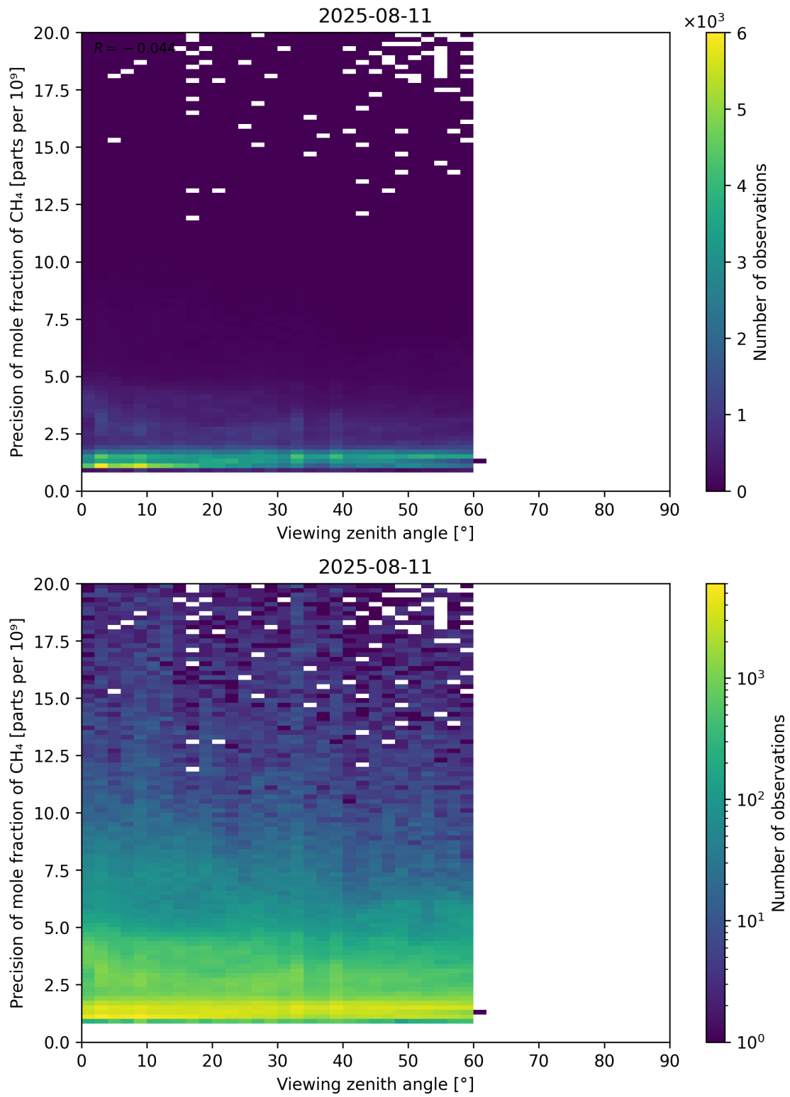
Figure 112: Scatter density plot of “Viewing zenith angle” against “Precision of mole fraction of CH 4 ” for 2025-08-10 to 2025-08-12.
