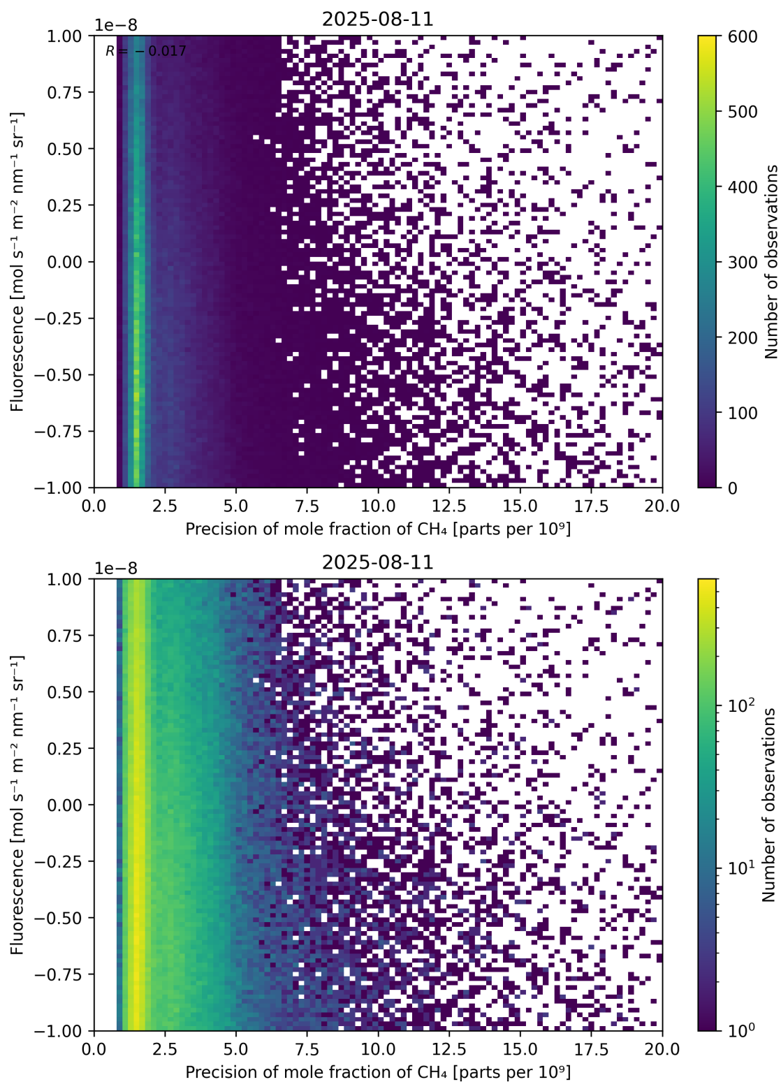
Figure 81: Scatter density plot of “Precision of mole fraction of \text{CH}_4 ” against “Fluorescence” for 2025-08-10 to 2025-08-12.
