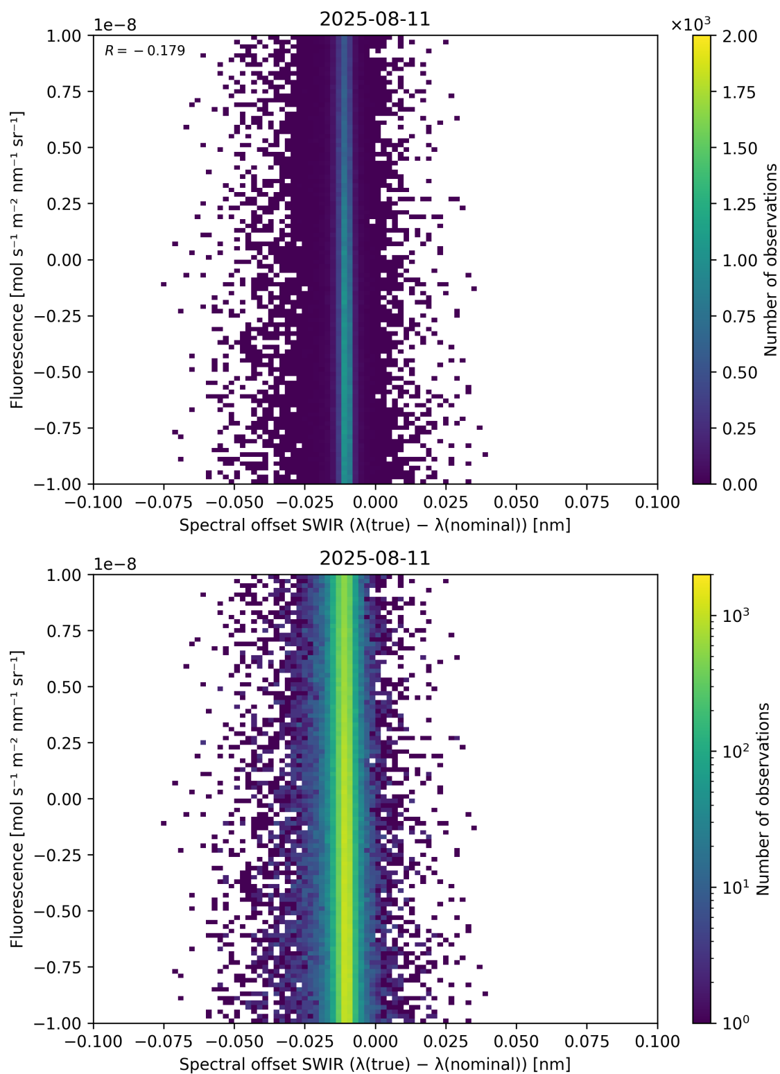
Figure 120: Scatter density plot of “Spectral offset SWIR ( \lambda_{\text{true}} - \lambda_{\text{nominal}} )” against “Fluorescence” for 2025-08-10 to 2025-08-12.
