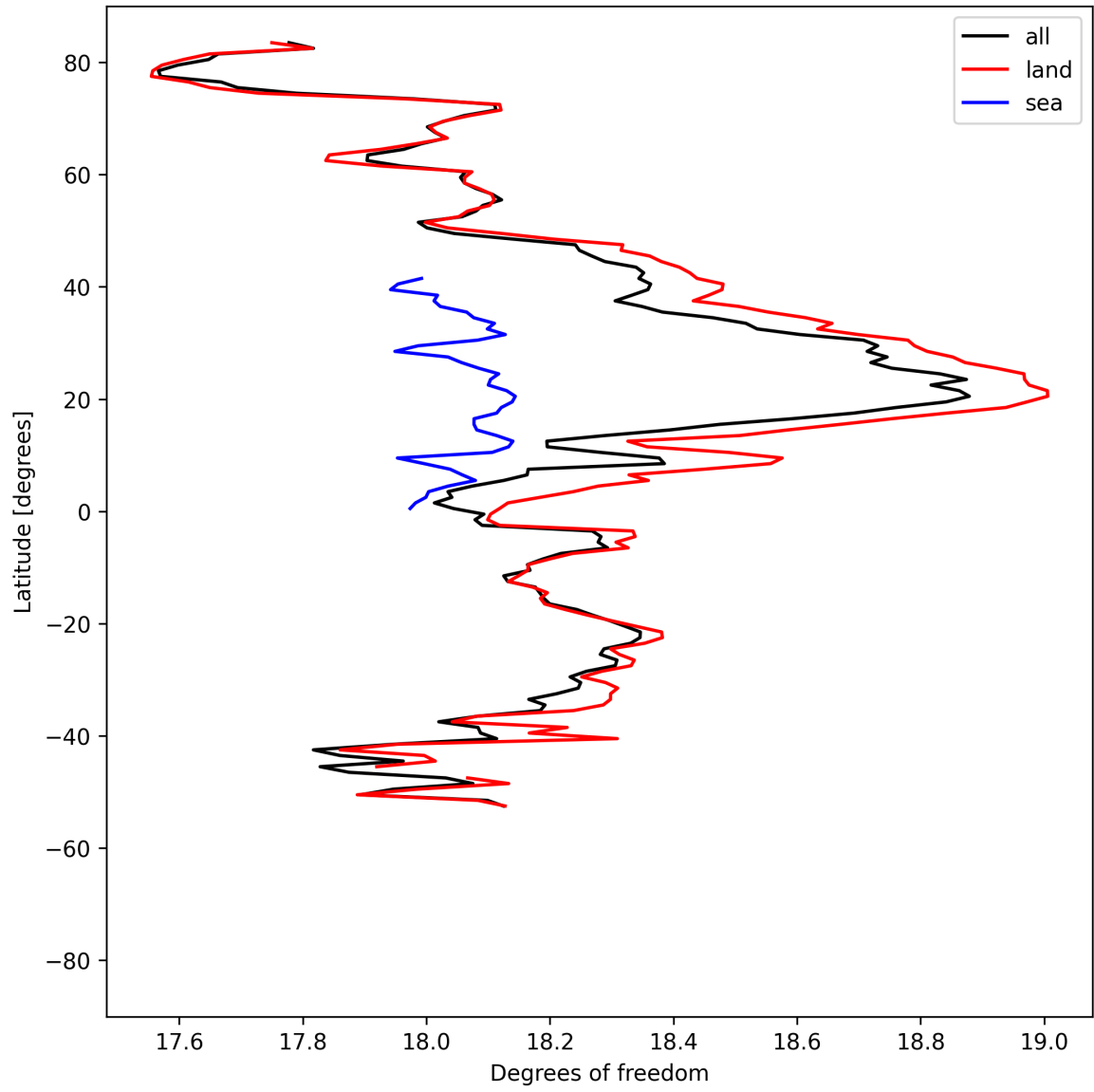
Figure 19: Zonal average of “Degrees of freedom” for 2025-08-10 to 2025-08-12.
