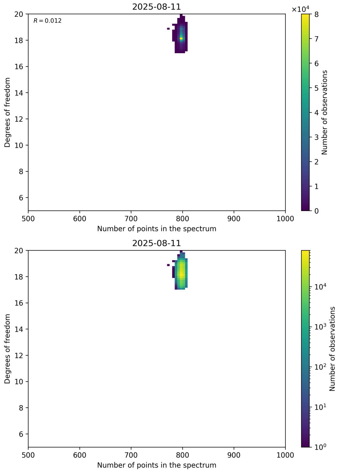
Figure 90: Scatter density plot of “Number of points in the spectrum” against “Degrees of freedom” for 2025-08-10 to 2025-08-12.
