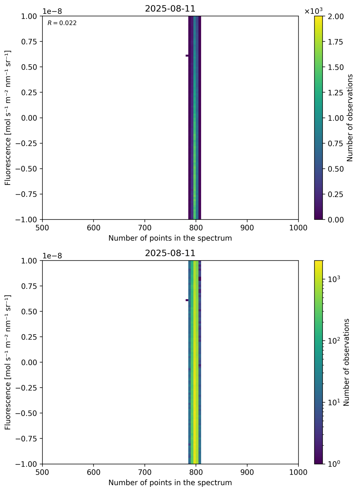
Figure 91: Scatter density plot of “Number of points in the spectrum” against “Fluorescence” for 2025-08-10 to 2025-08-12.
