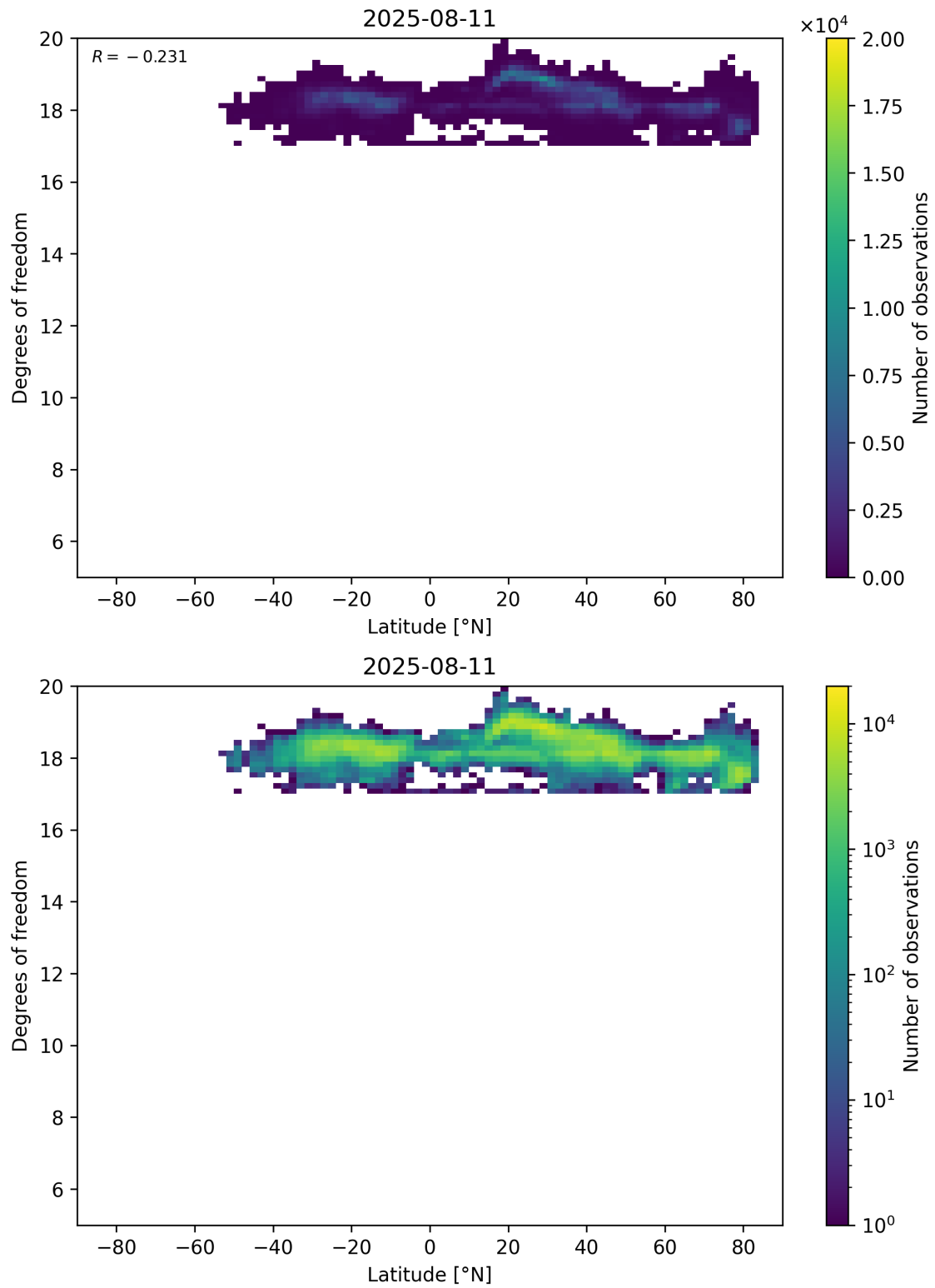
Figure 55: Scatter density plot of “Latitude” against “Degrees of freedom” for 2025-08-10 to 2025-08-12.
