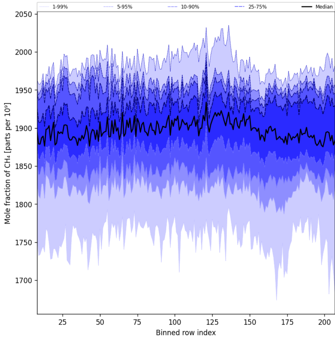
Figure 34: Along track statistics of “Mole fraction of CH 4 ” for 2025-08-10 to 2025-08-12
