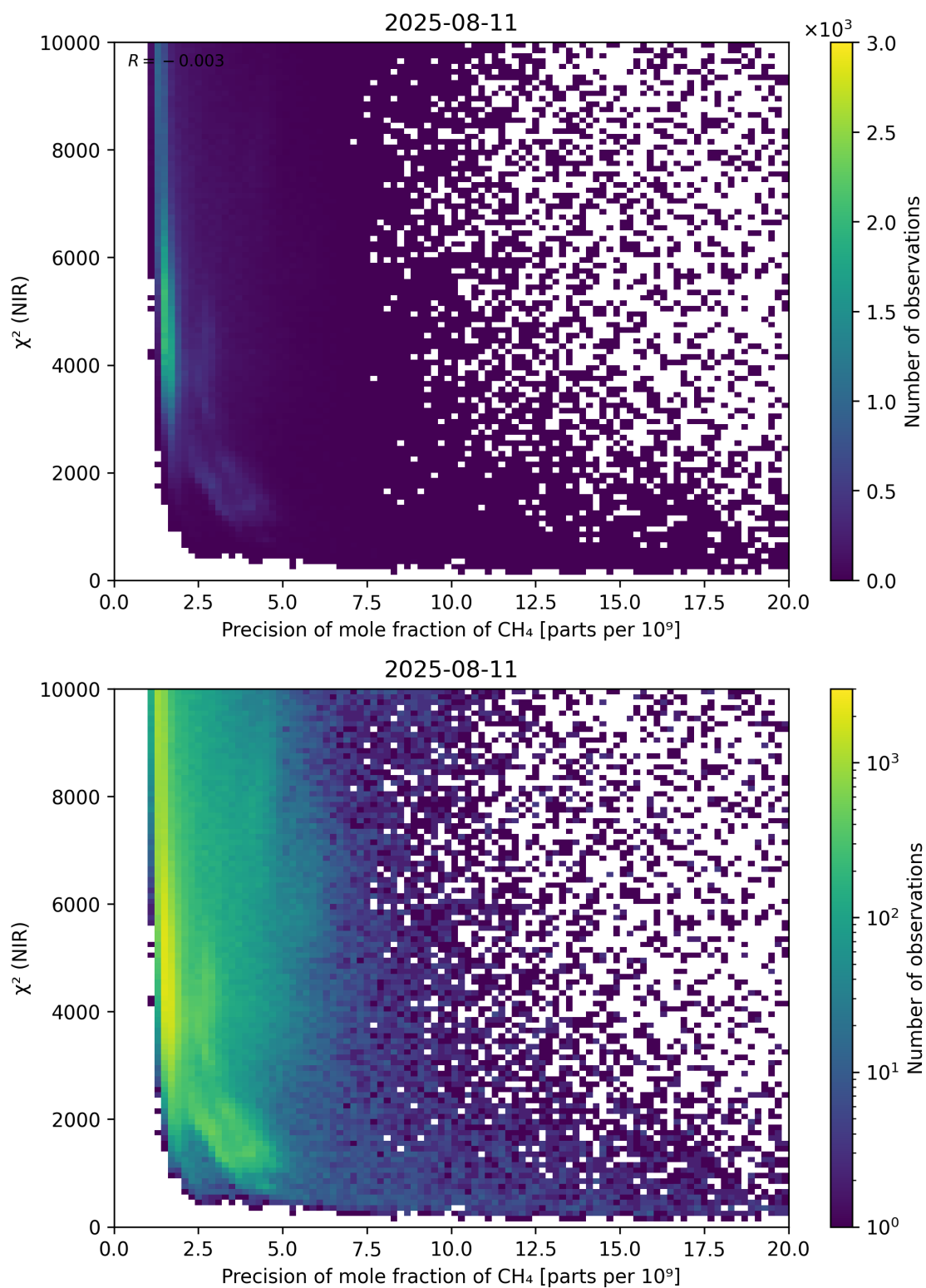
Figure 78: Scatter density plot of “Precision of mole fraction of CH 4 ” against “ \chi^2 (NIR)” for 2025-08-10 to 2025-08-12.
