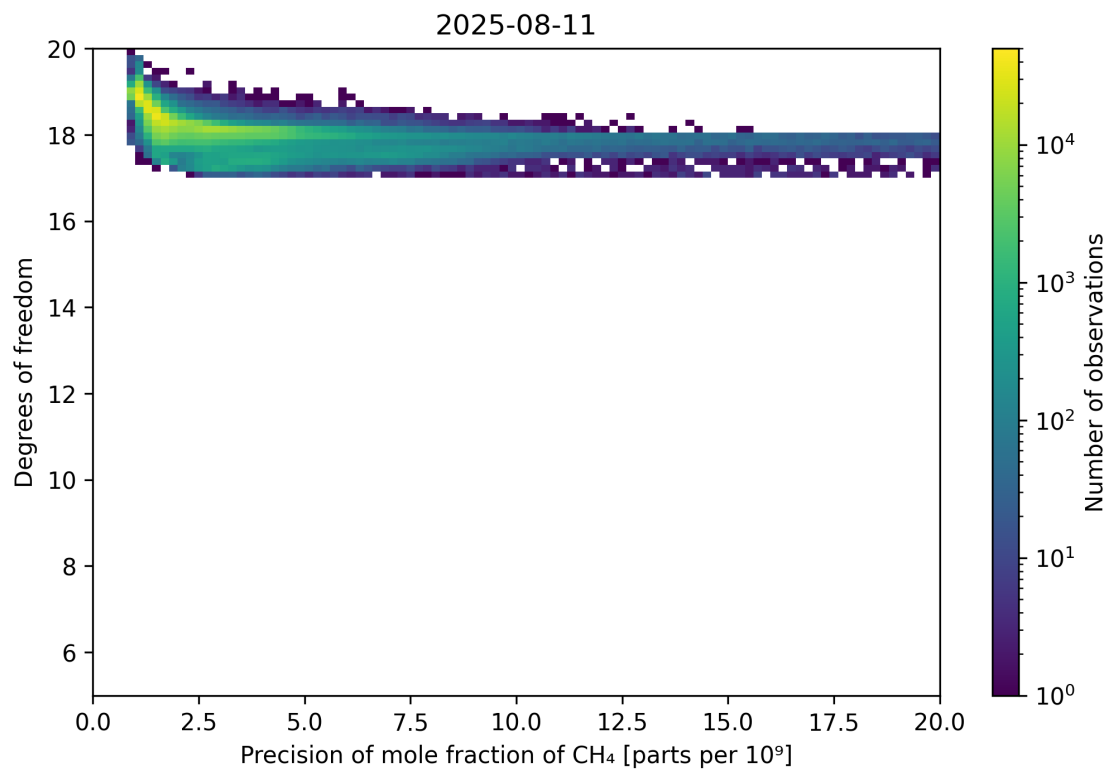
Figure 80: Scatter density plot of “Precision of mole fraction of CH 4 ” against “Degrees of freedom” for 2025-08-10 to 2025-08-12.
