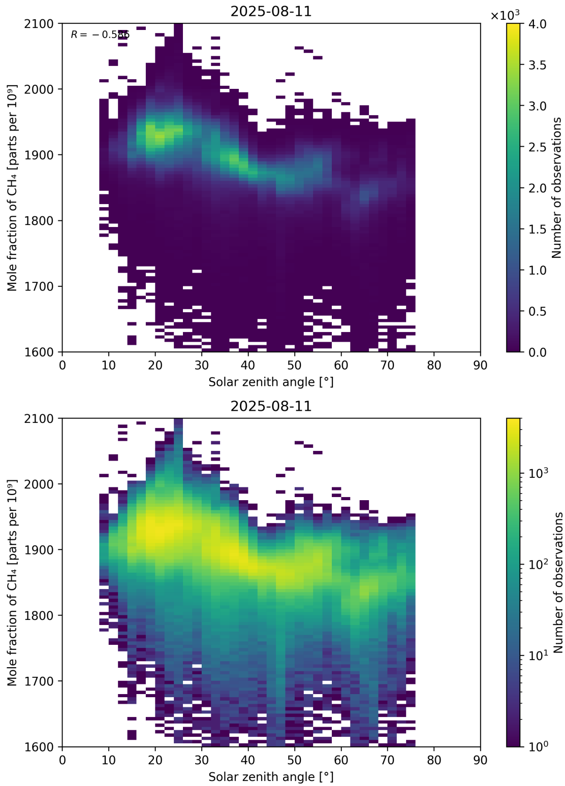
Figure 99: Scatter density plot of “Solar zenith angle” against “Mole fraction of CH 4 ” for 2025-08-10 to 2025-08-12.
