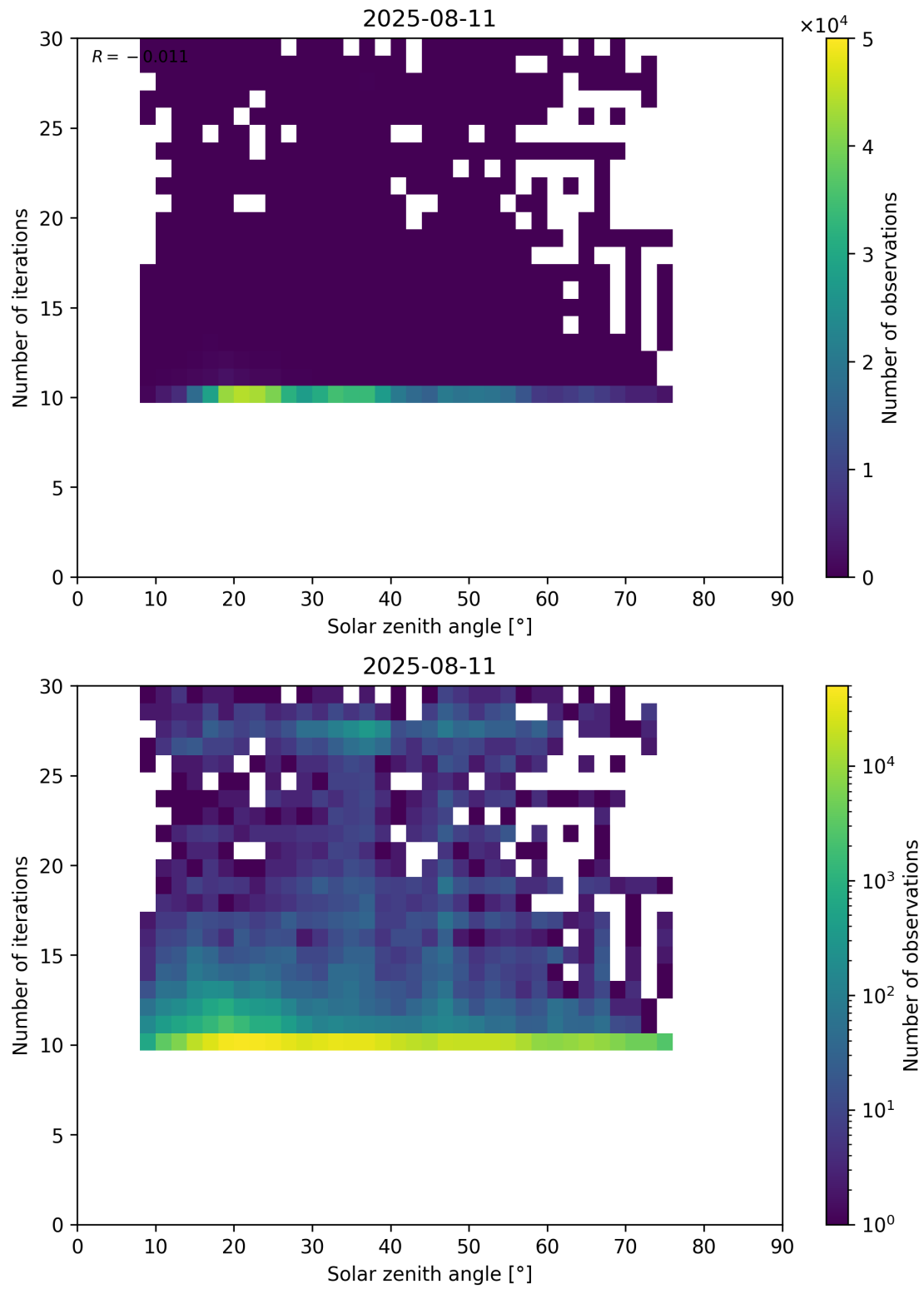
Figure 102: Scatter density plot of “Solar zenith angle” against “Number of iterations” for 2025-08-10 to 2025-08-12.
