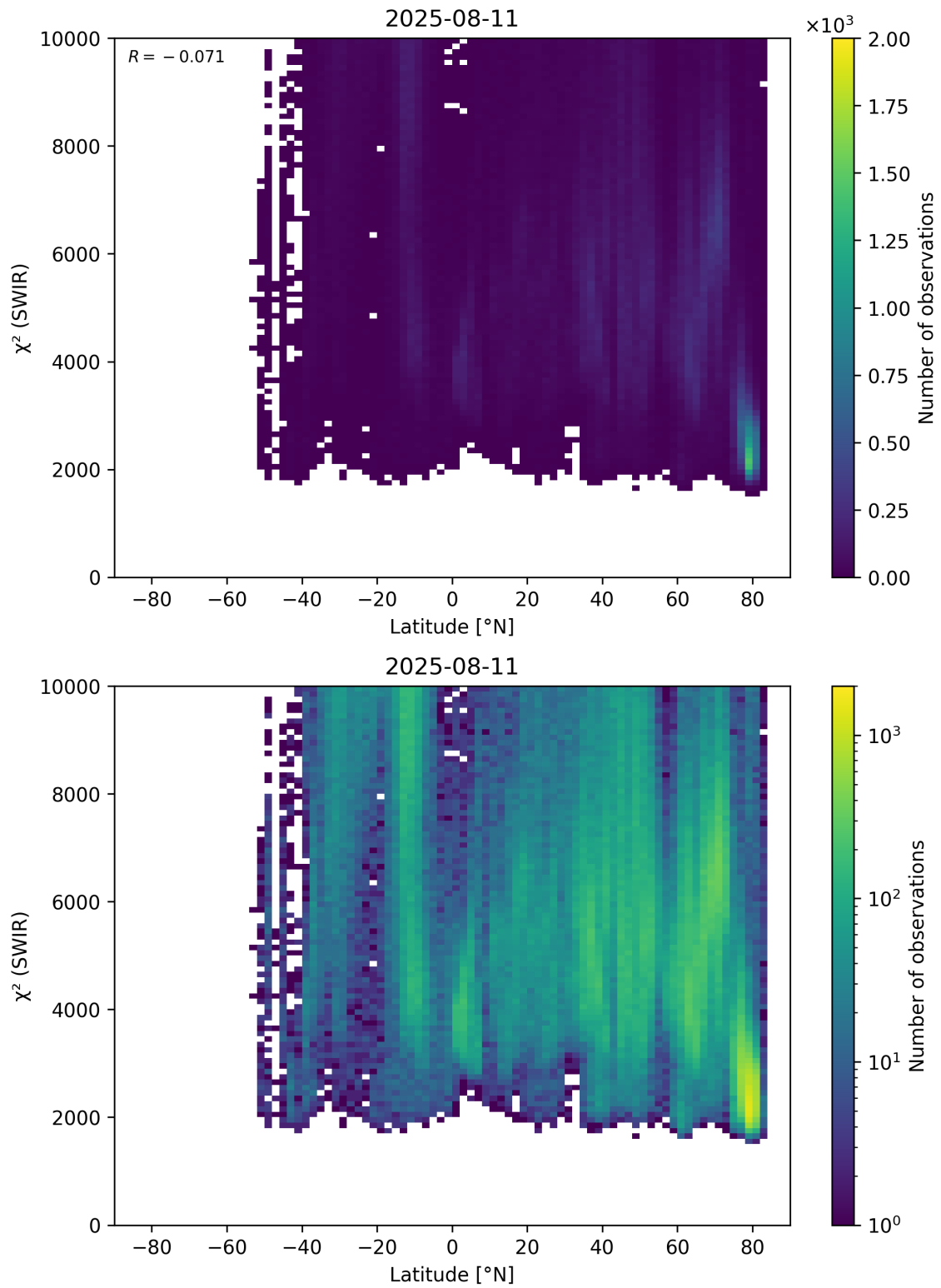
Figure 54: Scatter density plot of “Latitude” against “ \chi^2 (SWIR)” for 2025-08-10 to 2025-08-12.
