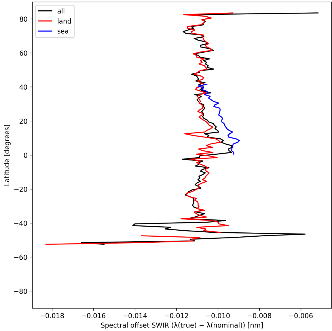
Figure 16: Zonal average of “Spectral offset SWIR ( \lambda_{\text{true}} - \lambda_{\text{nominal}} )” for 2025-08-10 to 2025-08-12.
