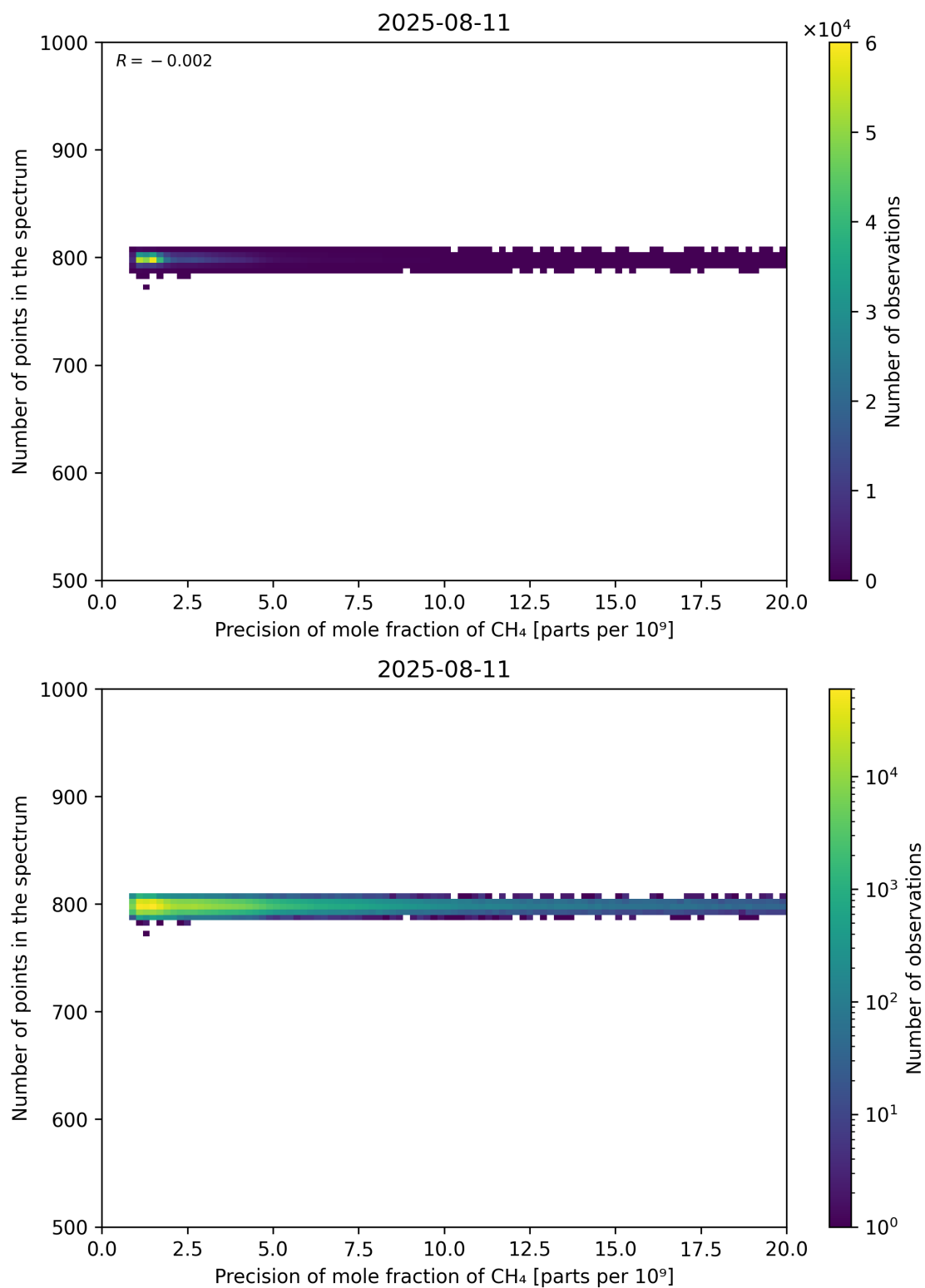
Figure 84: Scatter density plot of “Precision of mole fraction of CH 4 ” against “Number of points in the spectrum” for 2025-08-10 to 2025-08-12.
