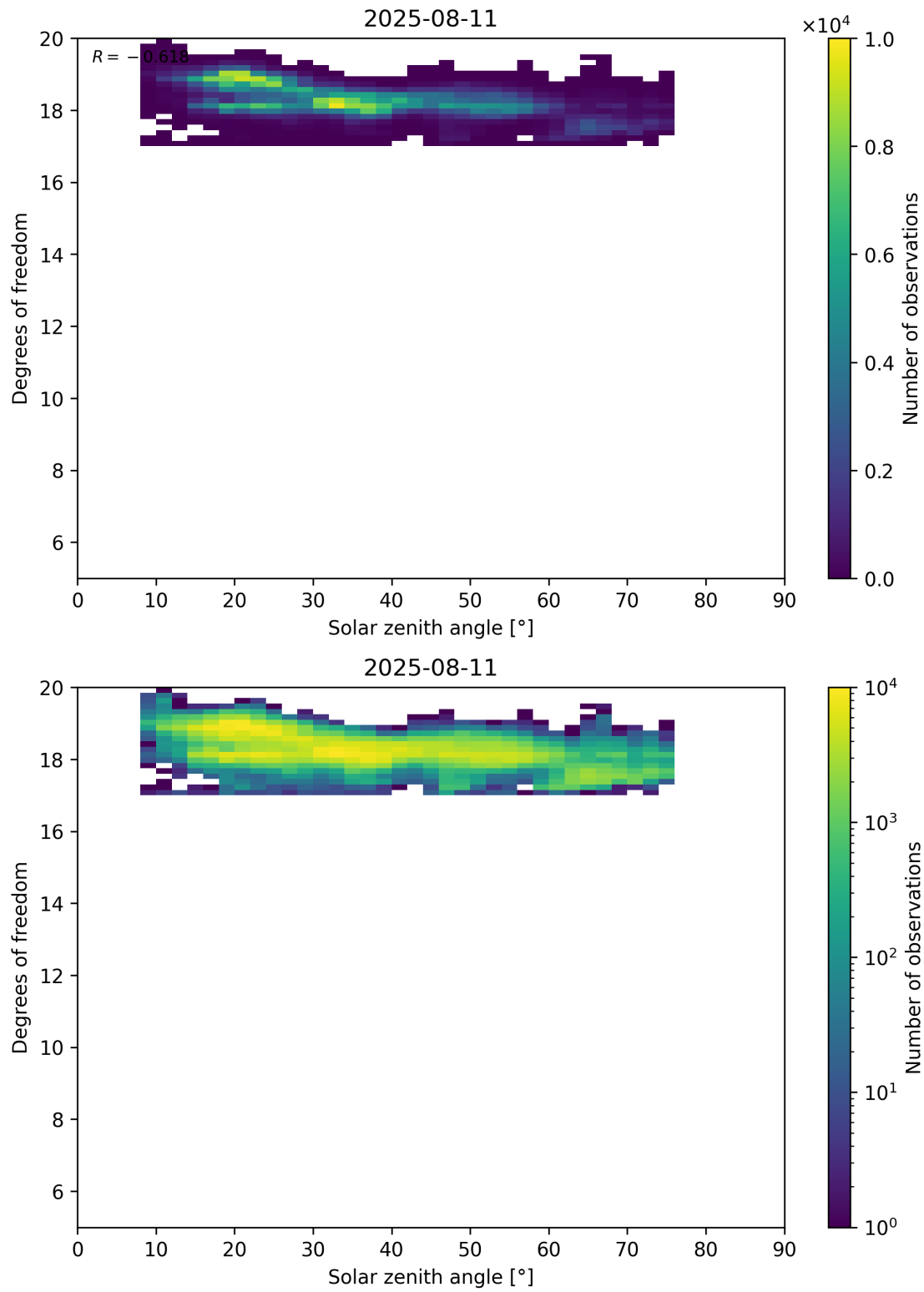
Figure 96: Scatter density plot of “Solar zenith angle” against “Degrees of freedom” for 2025-08-10 to 2025-08-12.
