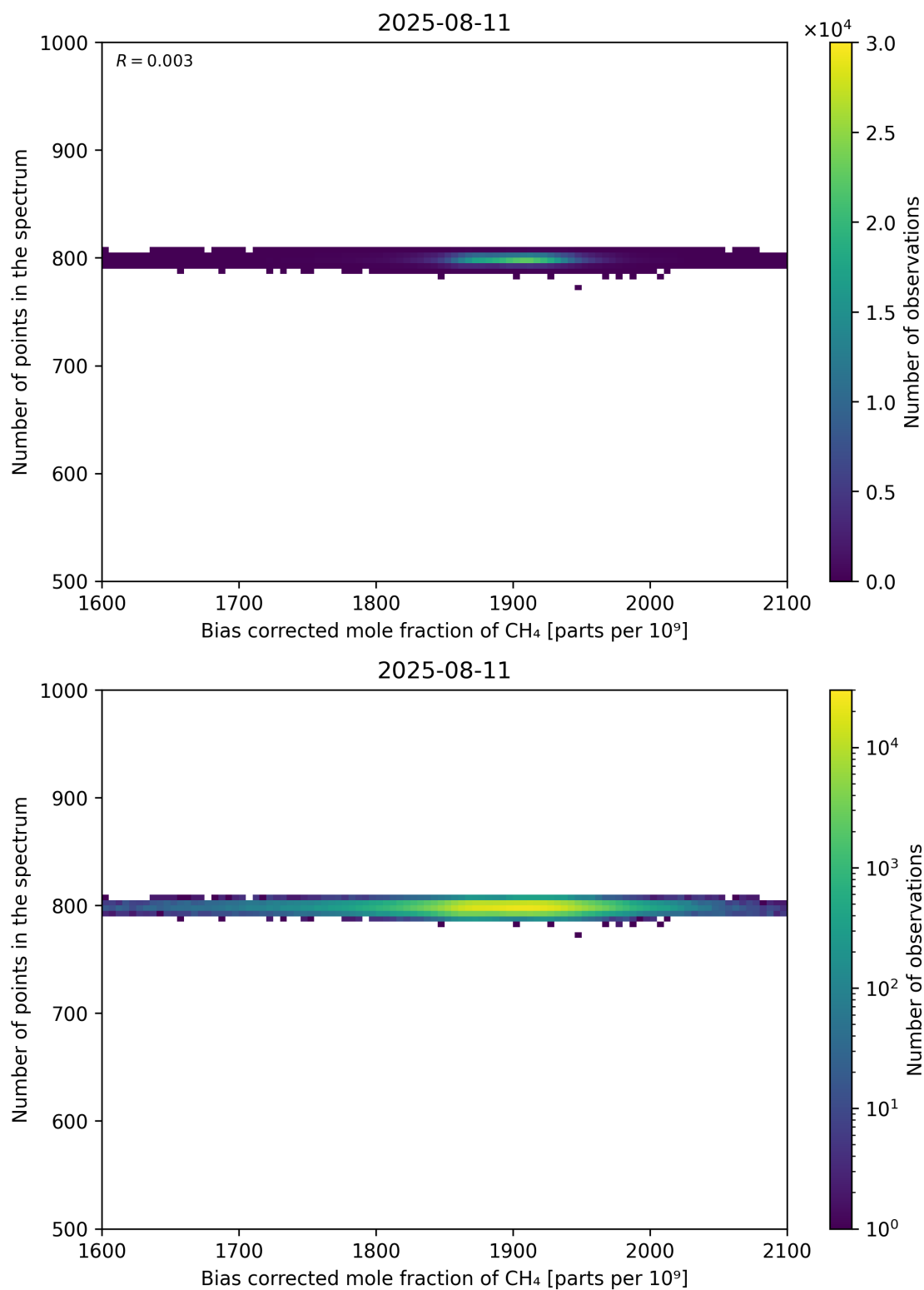
Figure 68: Scatter density plot of “Bias corrected mole fraction of CH 4 ” against “Number of points in the spectrum” for 2025-08-10 to 2025-08-12.
