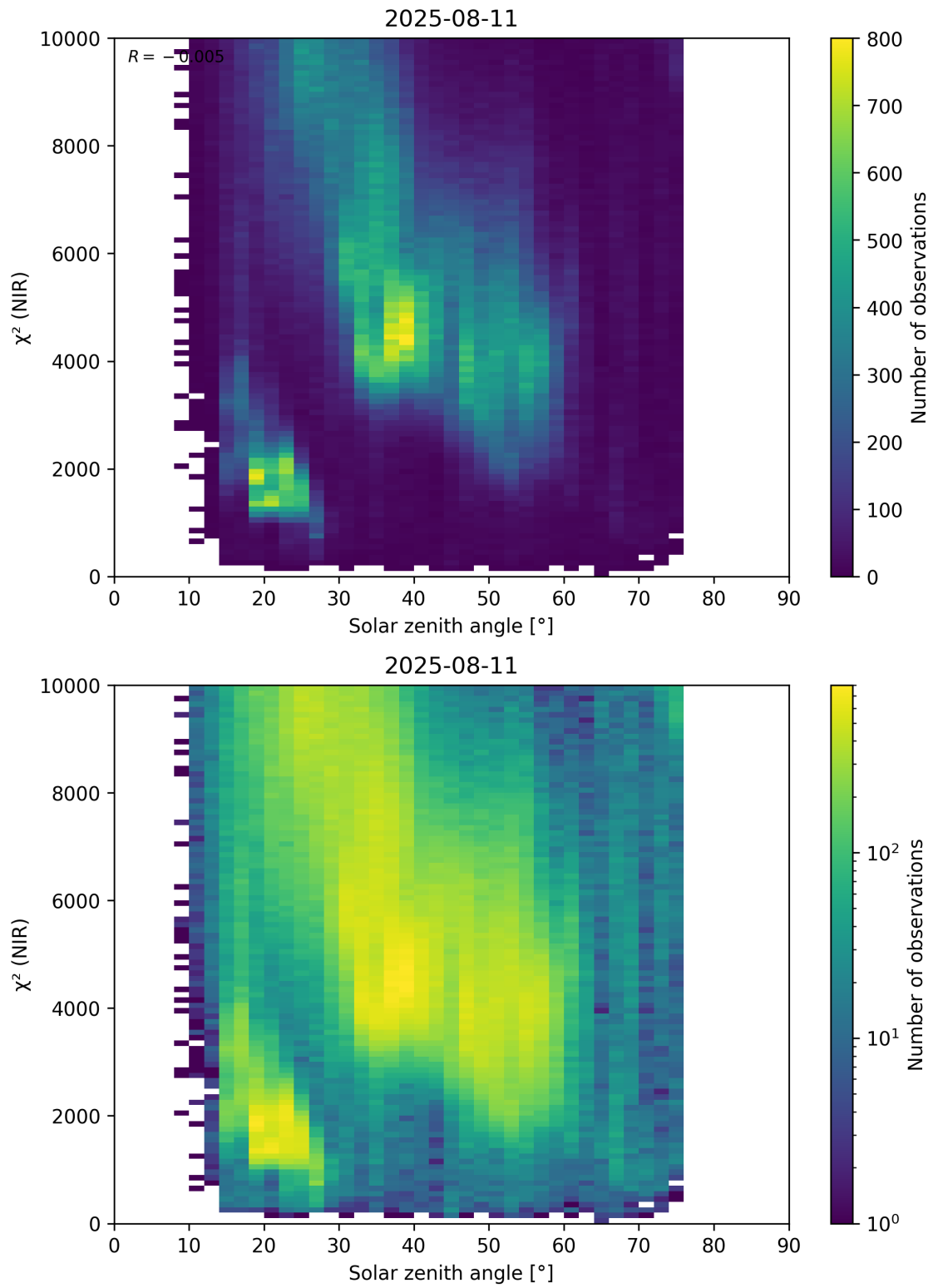
Figure 94: Scatter density plot of “Solar zenith angle” against “ \chi^2 (NIR)” for 2025-08-10 to 2025-08-12.
