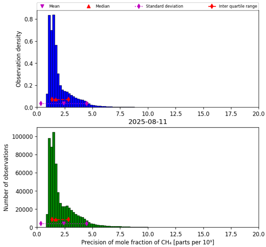
Figure 24: Histogram of “Precision of mole fraction of CH 4 ” for 2025-08-10 to 2025-08-12
