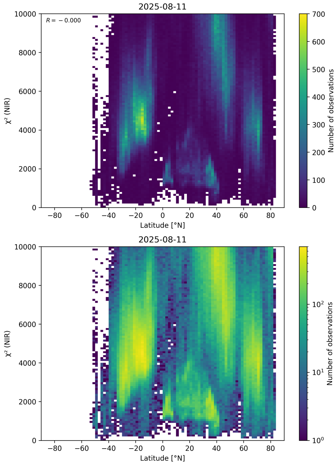
Figure 53: Scatter density plot of “Latitude” against “ \chi^2 (NIR)” for 2025-08-10 to 2025-08-12.
