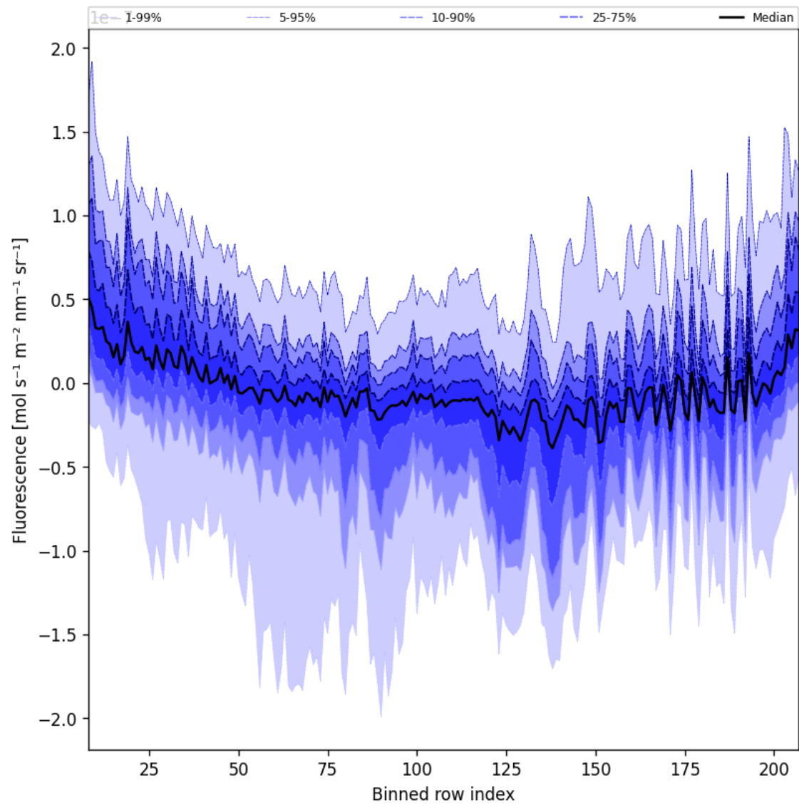
Figure 43: Along track statistics of “Fluorescence” for 2025-08-10 to 2025-08-12
