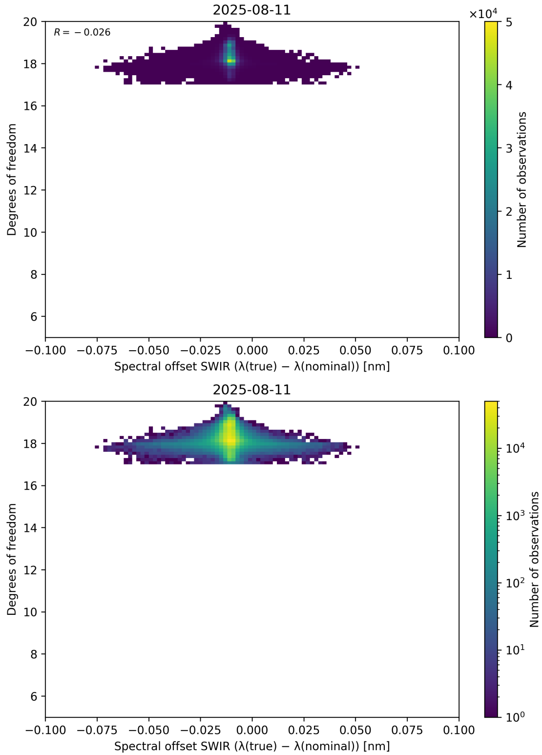
Figure 119: Scatter density plot of “Spectral offset SWIR ( \lambda_{\text{true}} - \lambda_{\text{nominal}} )” against “Degrees of freedom” for 2025-08-10 to 2025-08-12.
