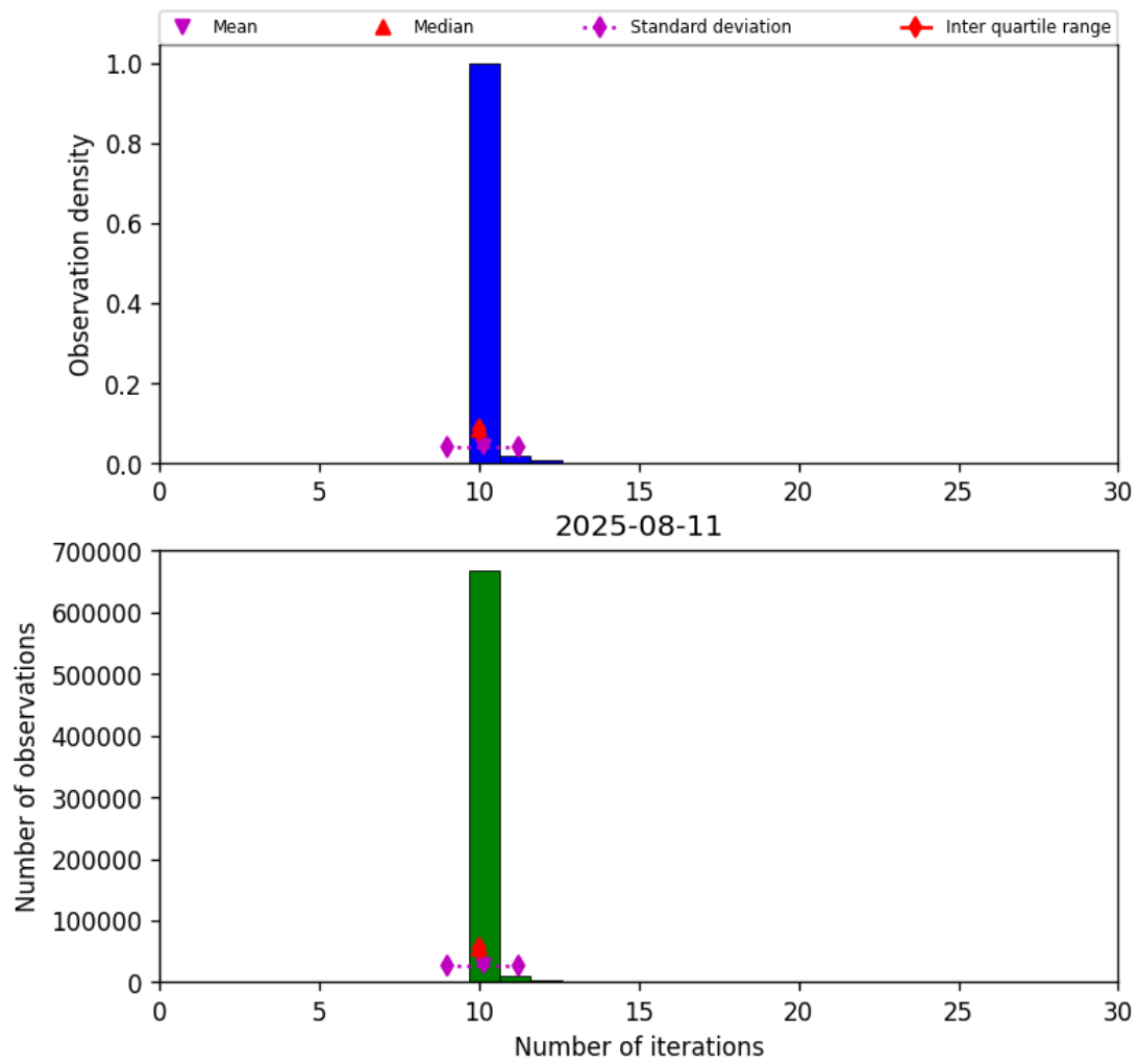
Figure 31: Histogram of “Number of iterations” for 2025-08-10 to 2025-08-12
