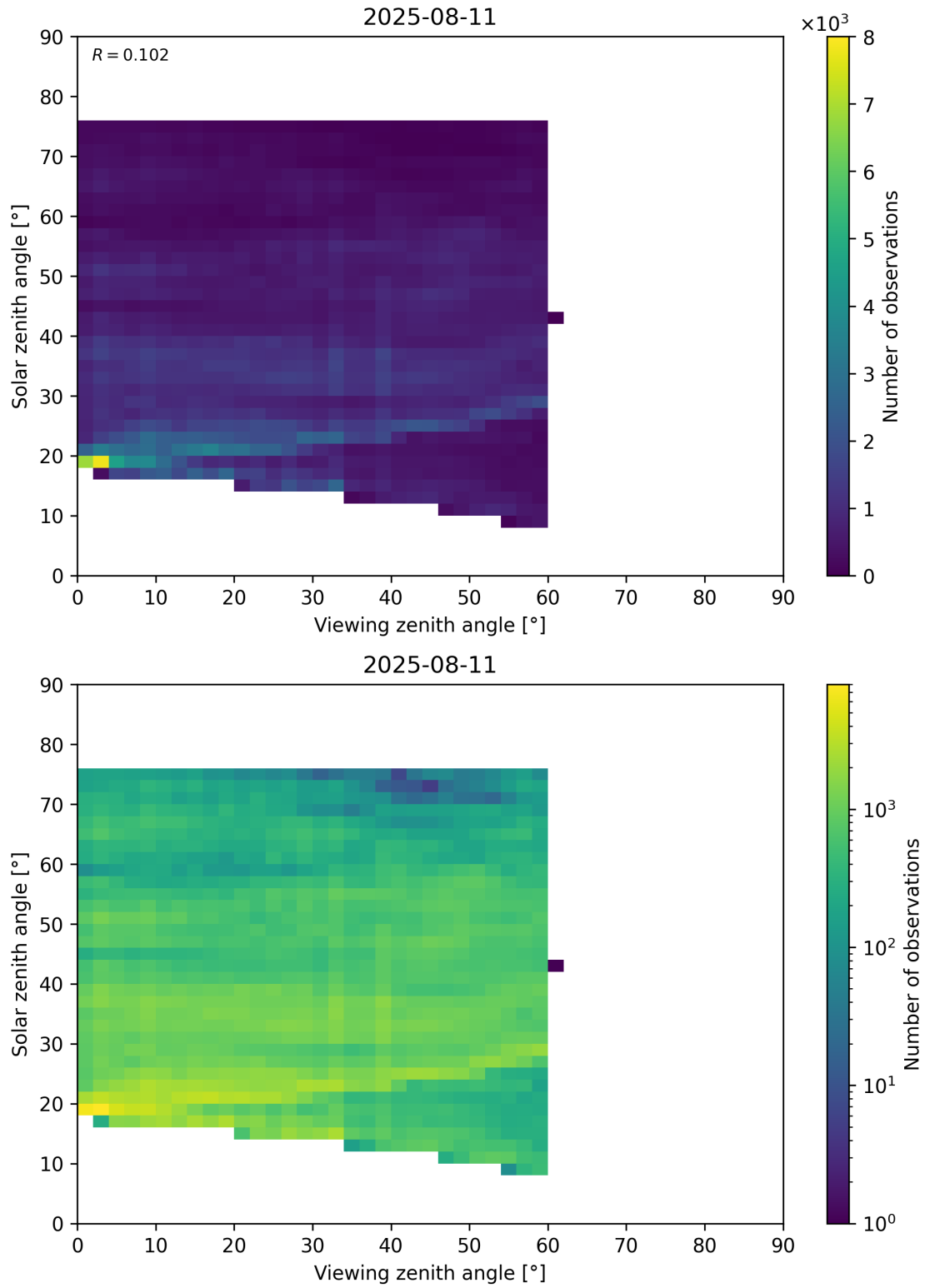
Figure 115: Scatter density plot of “Viewing zenith angle” against “Solar zenith angle” for 2025-08-10 to 2025-08-12.
