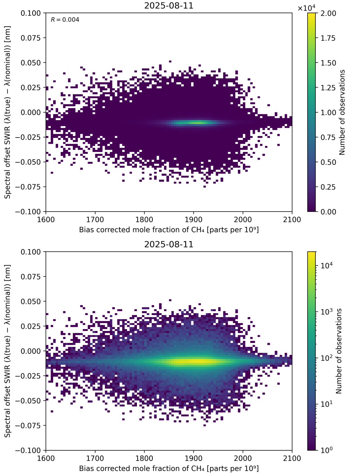
Figure 69: Scatter density plot of “Bias corrected mole fraction of \text{CH}_4 ” against “Spectral offset SWIR ( \lambda_{\text{true}} - \lambda_{\text{nominal}} )” for 2025-08-10 to 2025-08-12.
