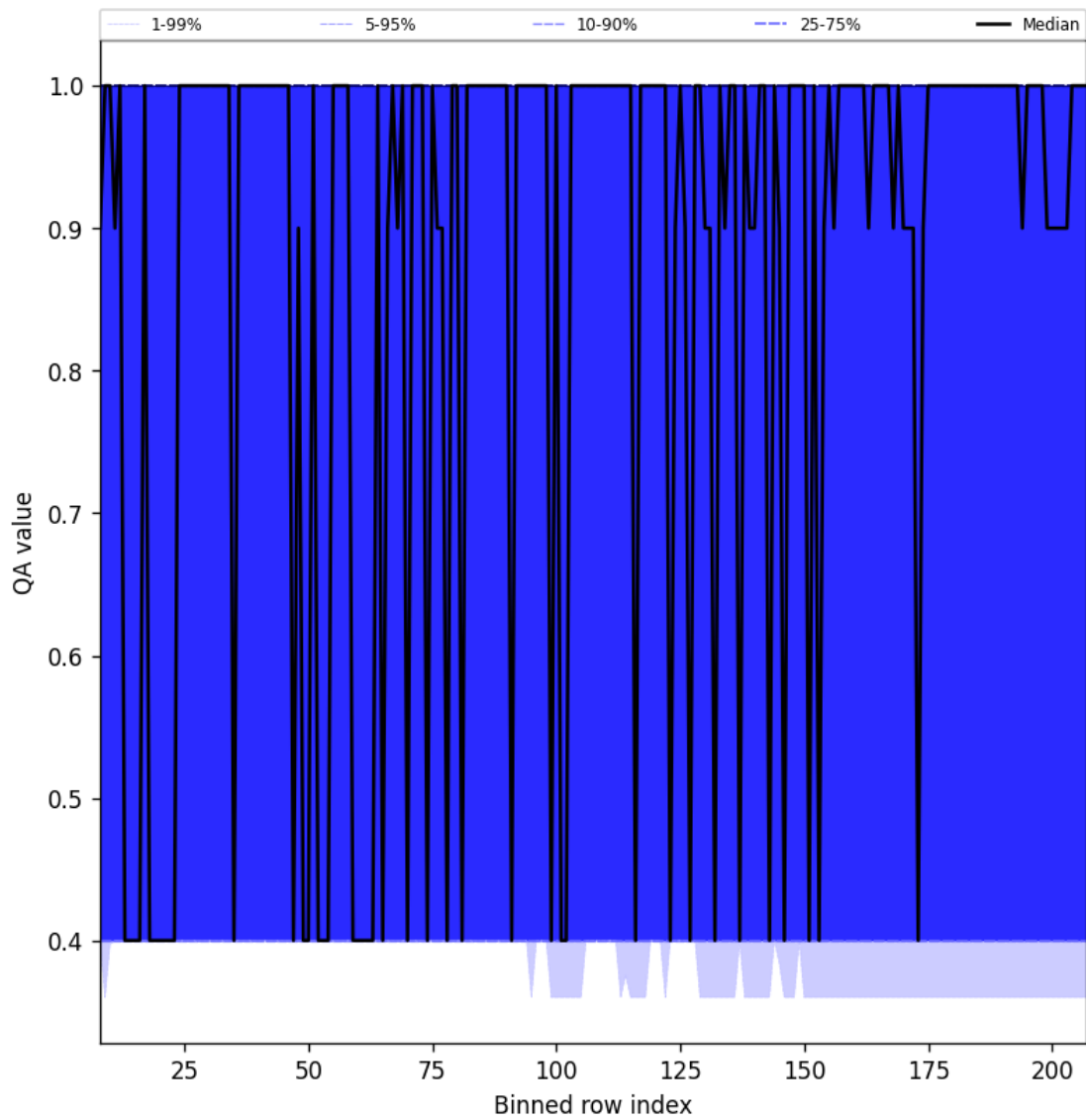
Figure 33: Along track statistics of “QA value” for 2025-08-10 to 2025-08-12
