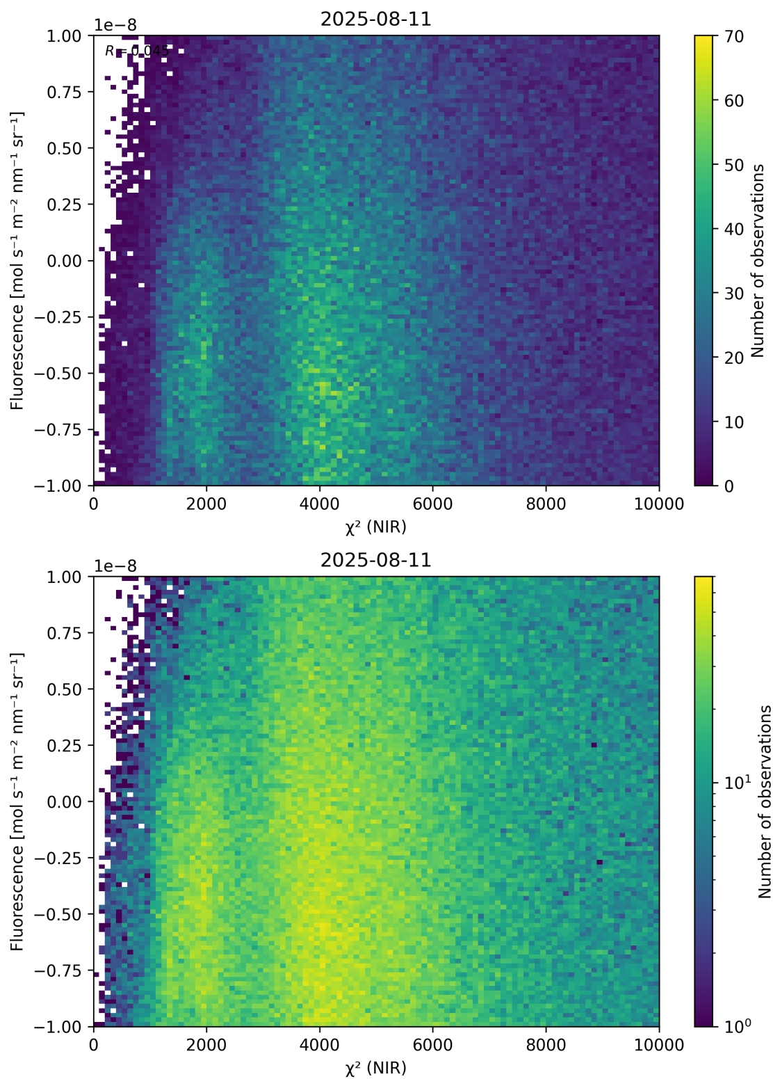
Figure 45: Scatter density plot of “ \chi^2 (NIR)” against “Fluorescence” for 2025-08-10 to 2025-08-12.
