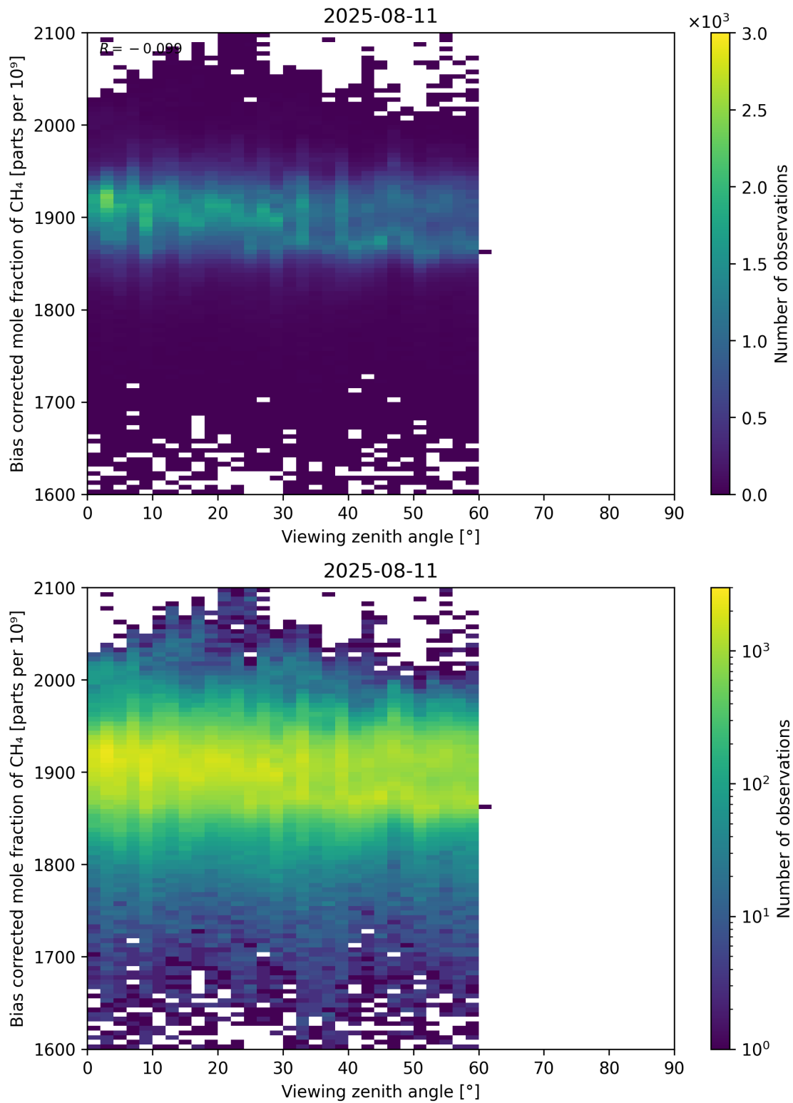
Figure 111: Scatter density plot of “Viewing zenith angle” against “Bias corrected mole fraction of CH 4 ” for 2025-08-10 to 2025-08-12.
