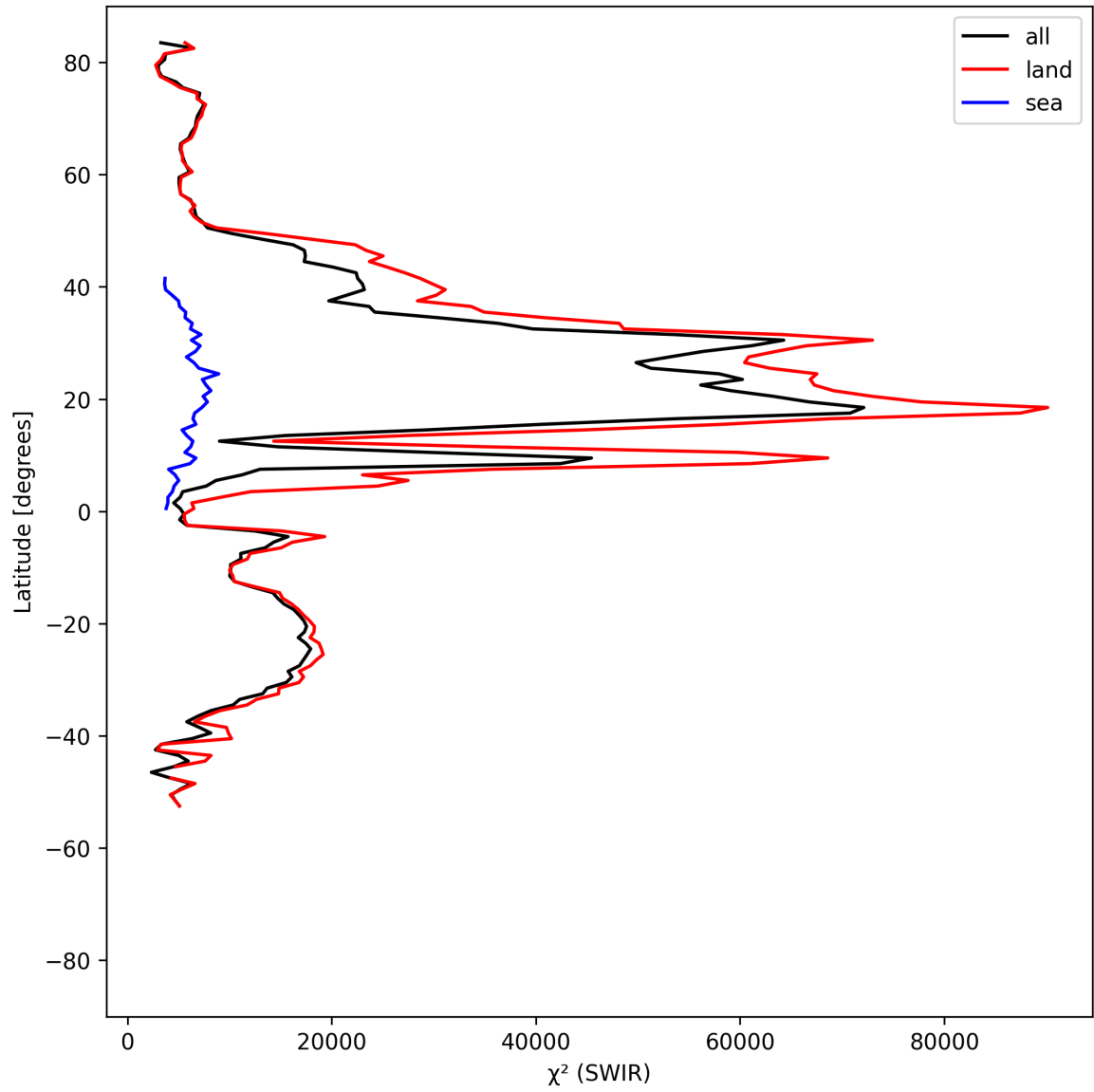
Figure 17: Zonal average of “ \chi^2 (SWIR)” for 2025-08-10 to 2025-08-12.
