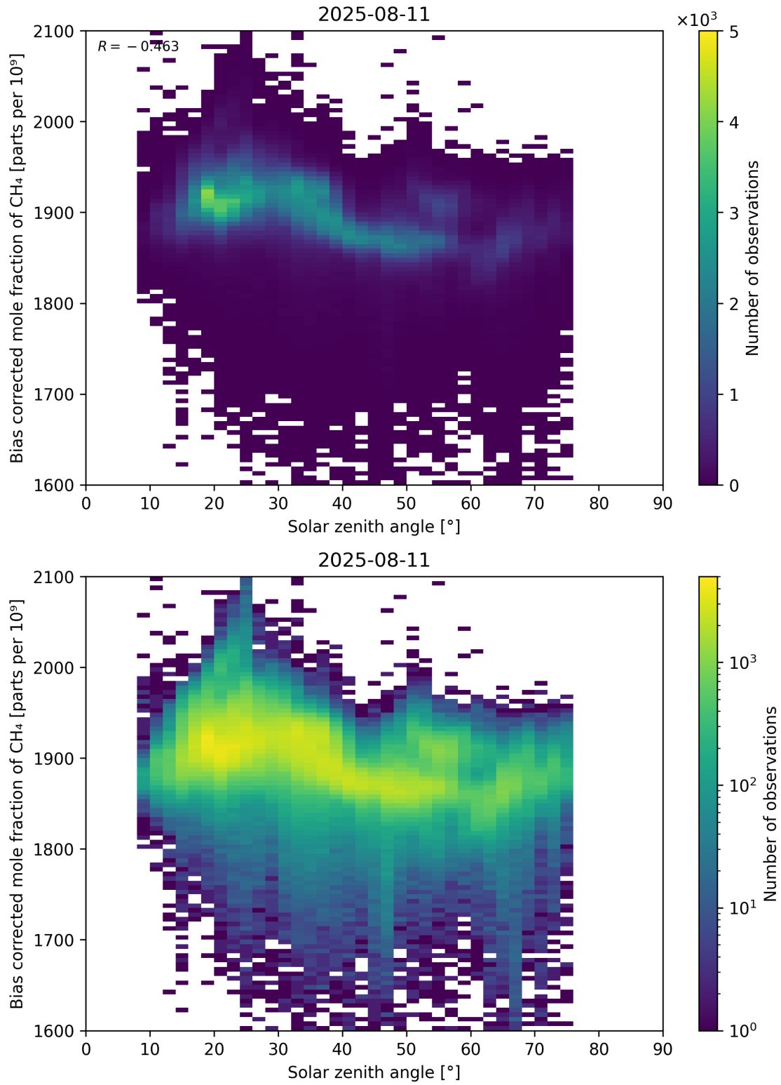
Figure 100: Scatter density plot of “Solar zenith angle” against “Bias corrected mole fraction of CH 4 ” for 2025-08-10 to 2025-08-12.
