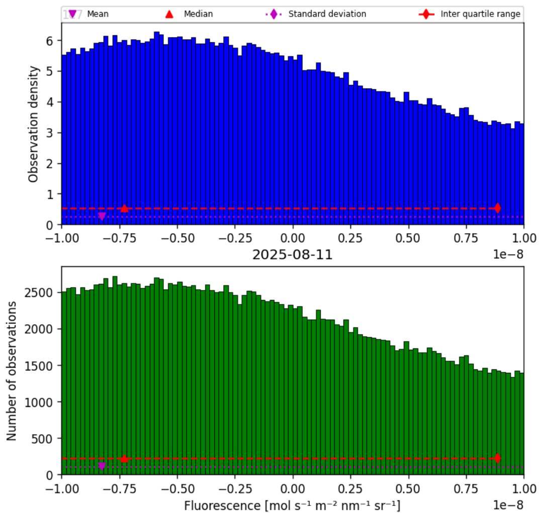
Figure 32: Histogram of “Fluorescence” for 2025-08-10 to 2025-08-12
