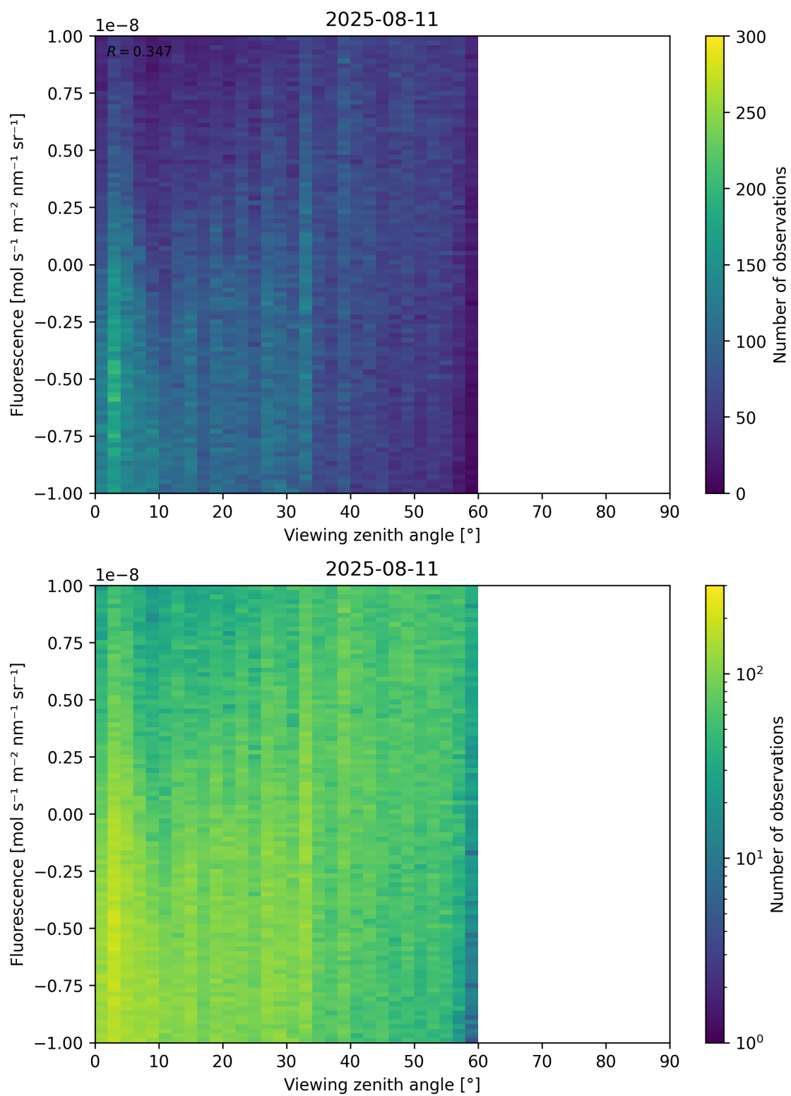
Figure 108: Scatter density plot of “Viewing zenith angle” against “Fluorescence” for 2025-08-10 to 2025-08-12.
