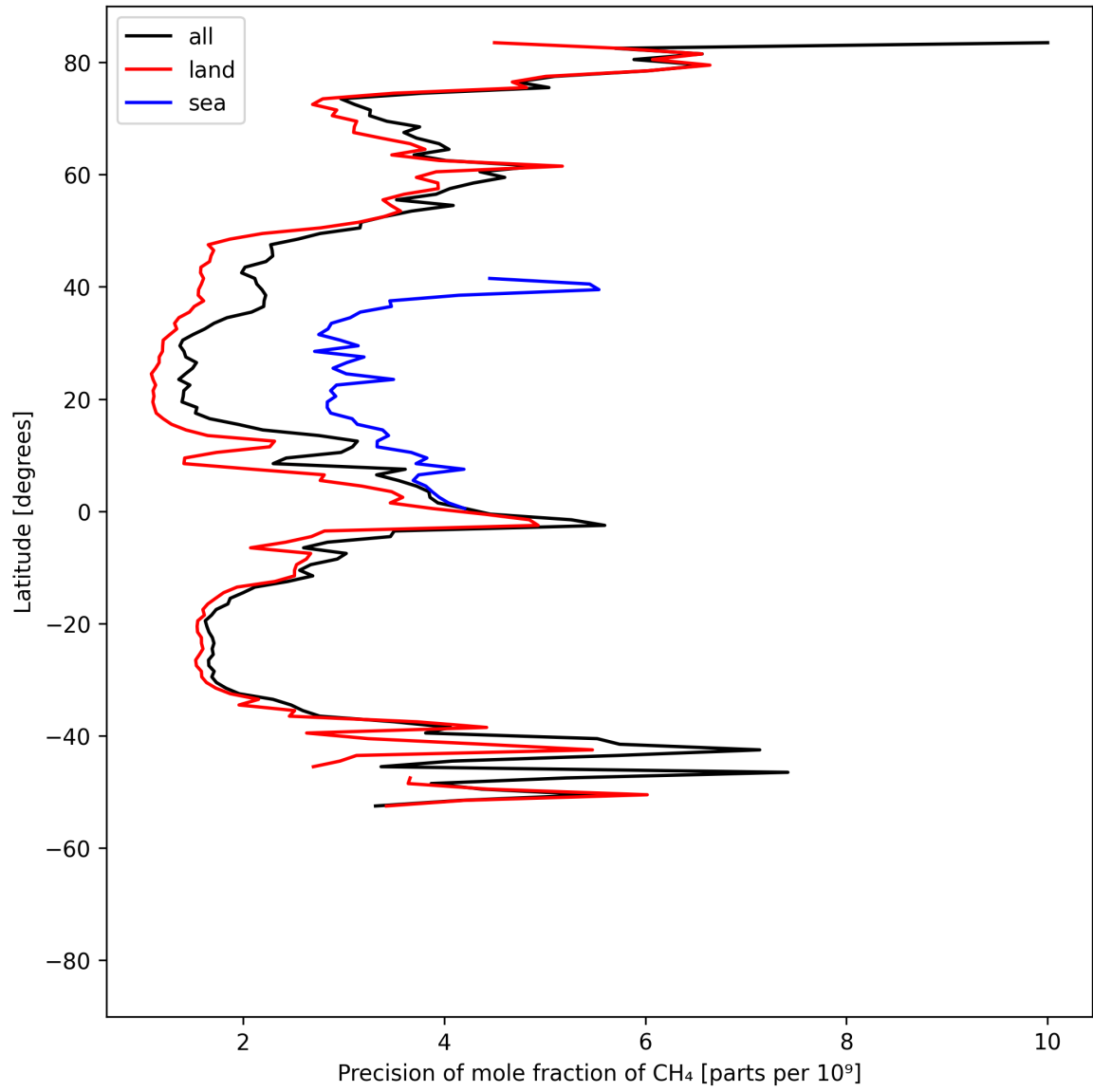
Figure 13: Zonal average of “Precision of mole fraction of CH 4 ” for 2025-08-10 to 2025-08-12.
