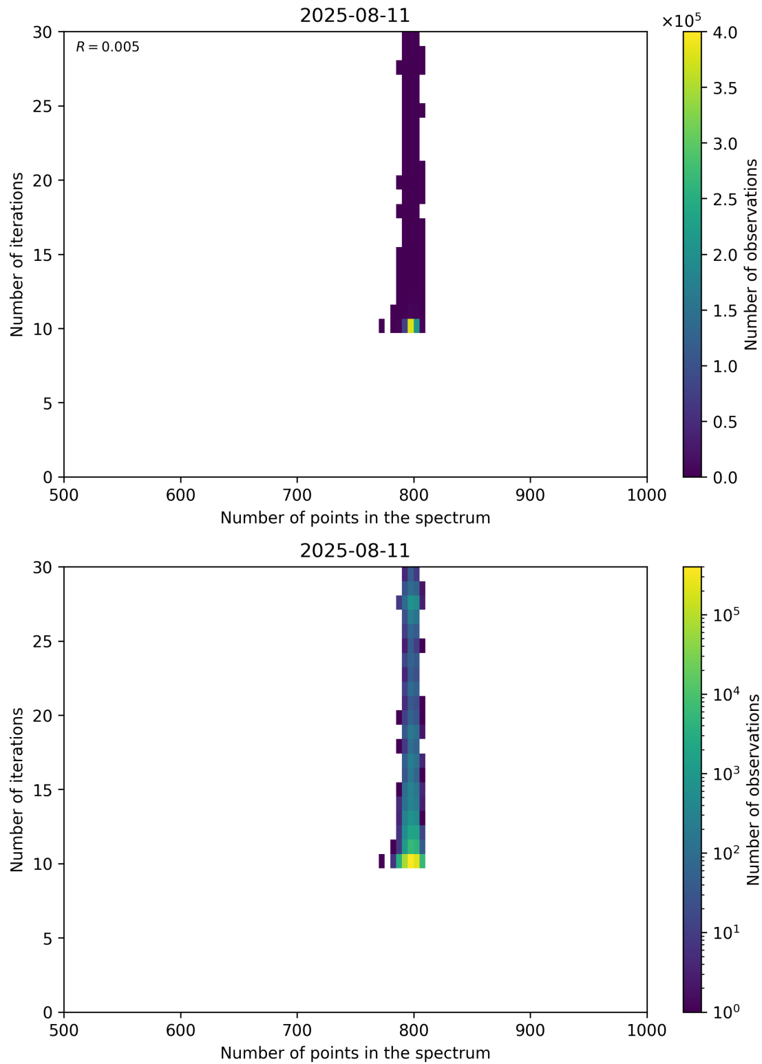
Figure 92: Scatter density plot of “Number of points in the spectrum” against “Number of iterations” for 2025-08-10 to 2025-08-12.
