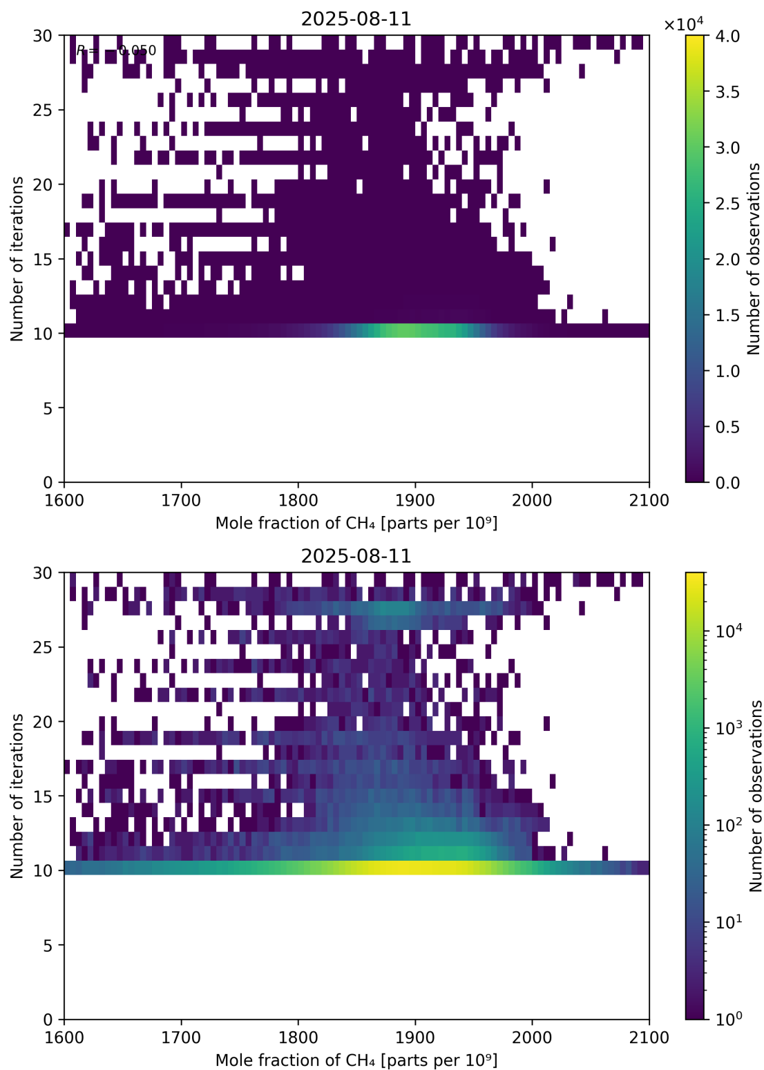
Figure 76: Scatter density plot of “Mole fraction of CH 4 ” against “Number of iterations” for 2025-08-10 to 2025-08-12.
