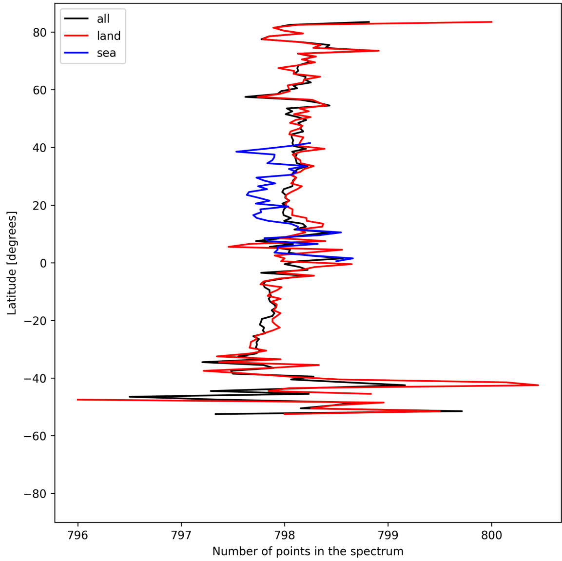
Figure 15: Zonal average of “Number of points in the spectrum” for 2025-08-10 to 2025-08-12.
