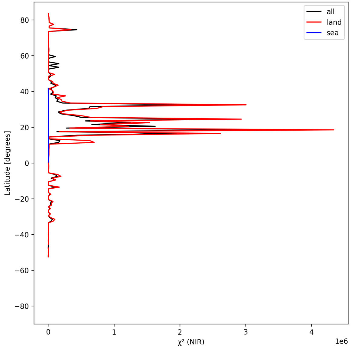
Figure 18: Zonal average of “ \chi^2 (NIR)” for 2025-08-10 to 2025-08-12.
