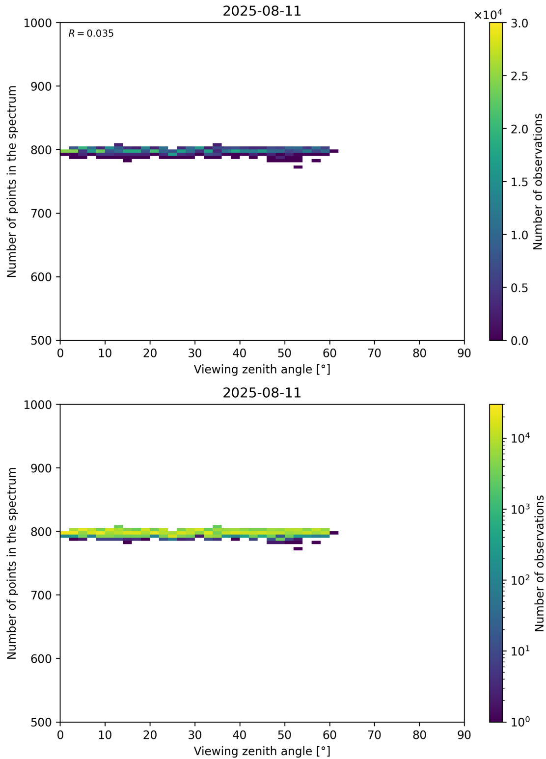
Figure 114: Scatter density plot of “Viewing zenith angle” against “Number of points in the spectrum” for 2025-08-10 to 2025-08-12.
