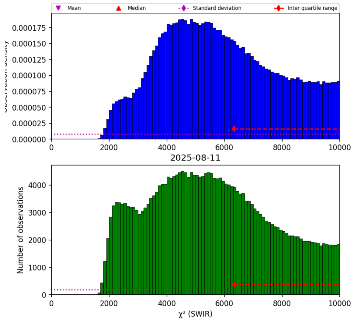
Figure 28: Histogram of “ \chi^2 (SWIR)” for 2025-08-10 to 2025-08-12
