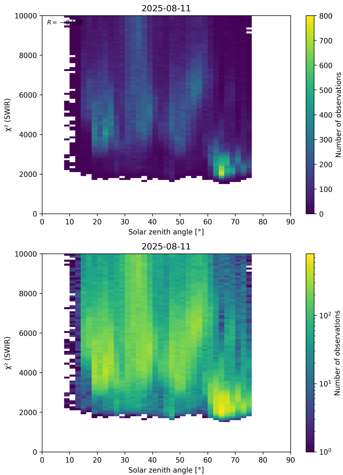
Figure 95: Scatter density plot of “Solar zenith angle” against “ \chi^2 (SWIR)” for 2025-08-10 to 2025-08-12.
