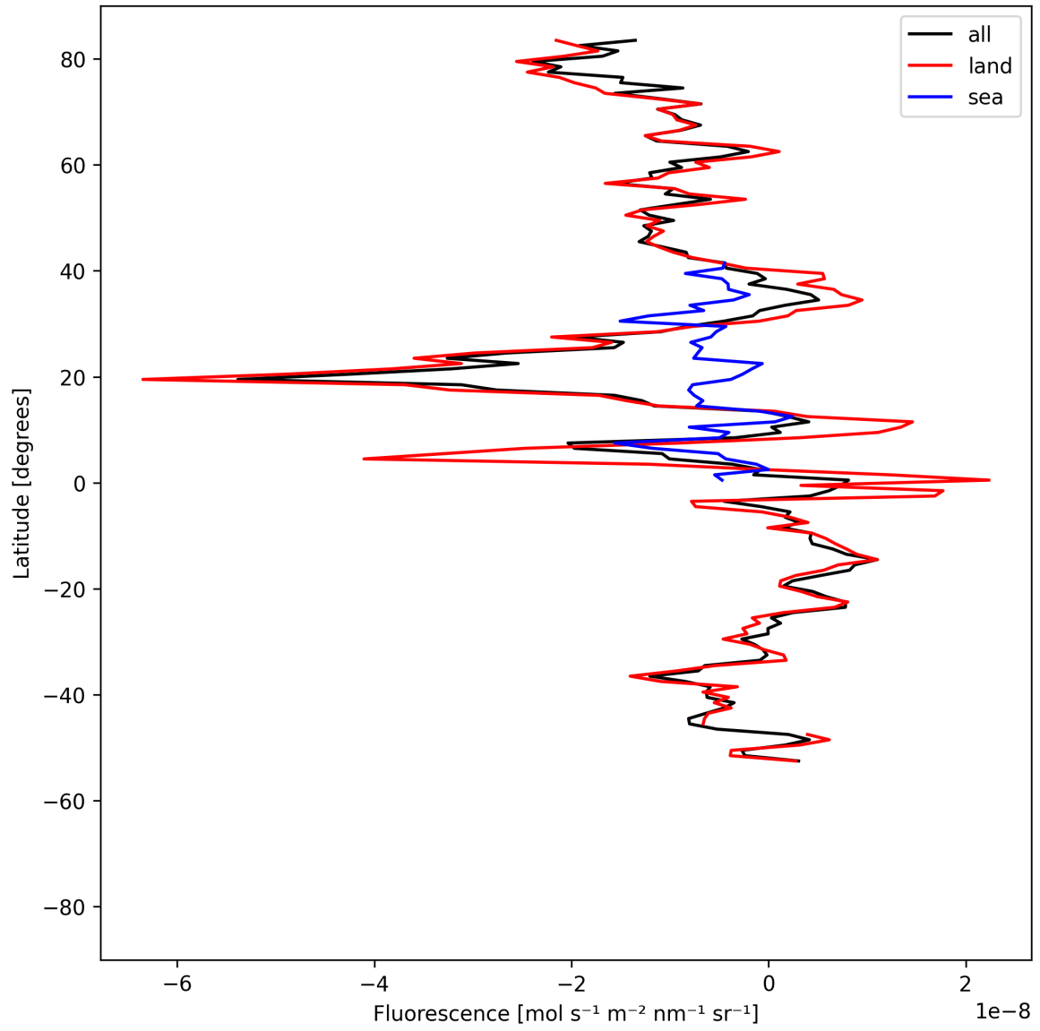
Figure 21: Zonal average of “Fluorescence” for 2025-08-10 to 2025-08-12.
