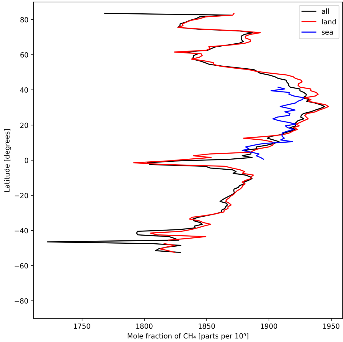
Figure 12: Zonal average of “Mole fraction of \text{CH}_4 ” for 2025-08-10 to 2025-08-12.
