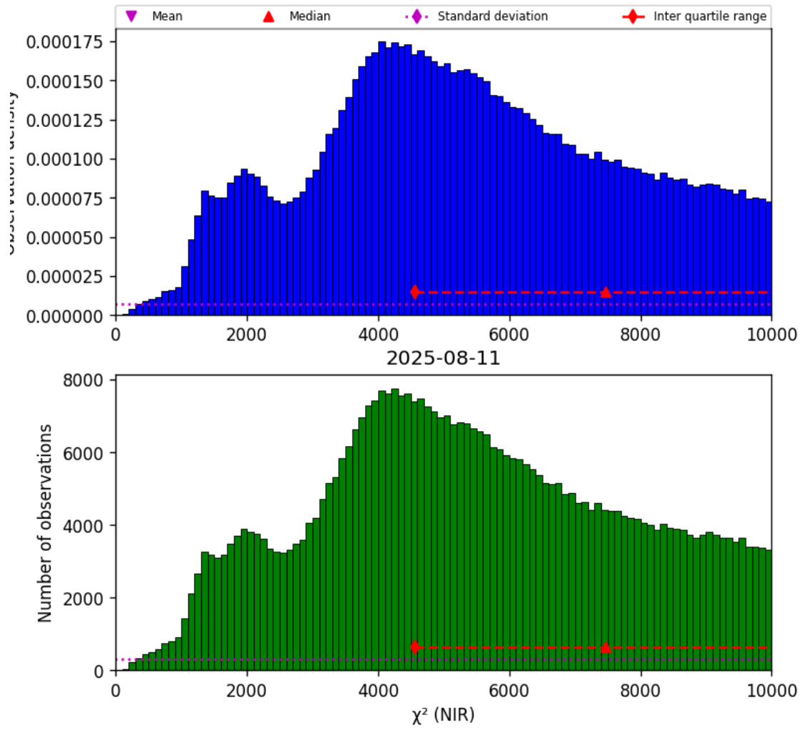
Figure 29: Histogram of “ \chi^2 (NIR)” for 2025-08-10 to 2025-08-12
