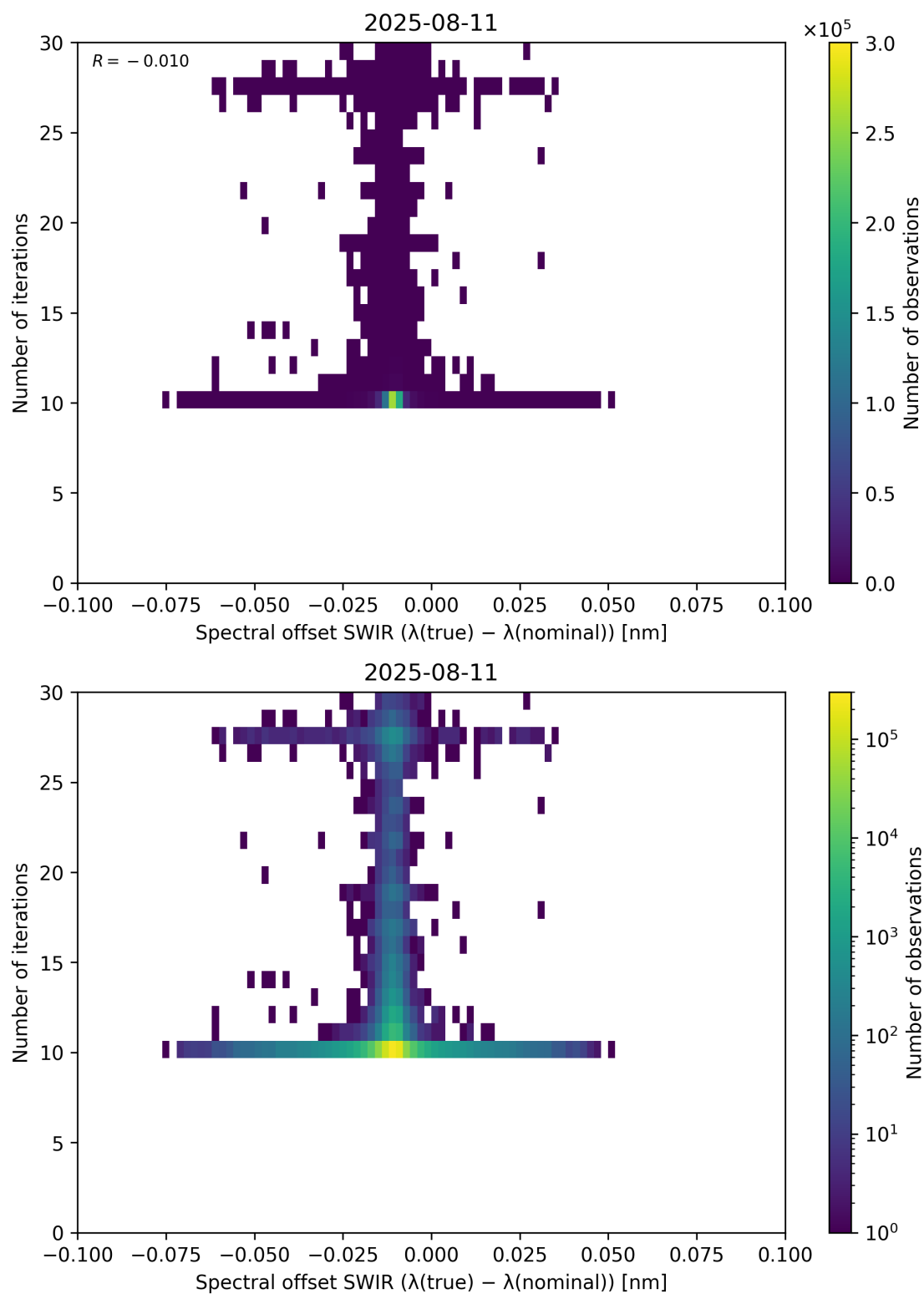
Figure 121: Scatter density plot of “Spectral offset SWIR ( \lambda_{\text{true}} - \lambda_{\text{nominal}} )” against “Number of iterations” for 2025-08-10 to 2025-08-12.
