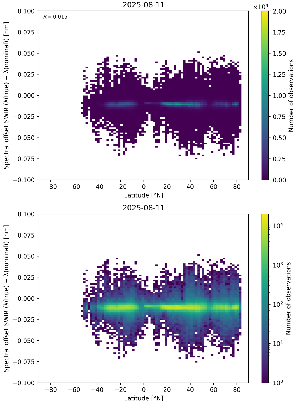
Figure 62: Scatter density plot of “Latitude” against “Spectral offset SWIR ( \lambda_{\text{true}} - \lambda_{\text{nominal}} )” for 2025-08-10 to 2025-08-12.
