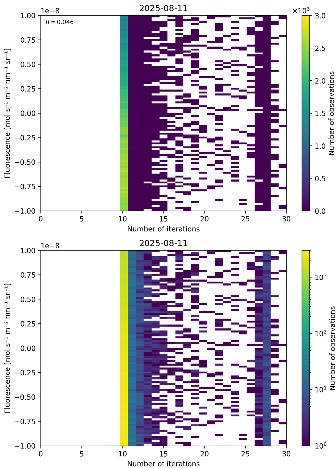
Figure 87: Scatter density plot of “Number of iterations” against “Fluorescence” for 2025-08-10 to 2025-08-12.
