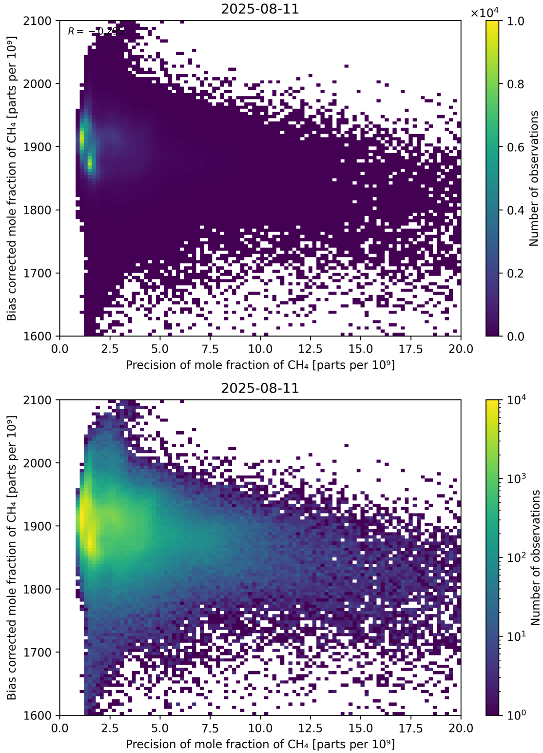
Figure 82: Scatter density plot of “Precision of mole fraction of CH 4 ” against “Bias corrected mole fraction of CH 4 ” for 2025-08-10 to 2025-08-12.
