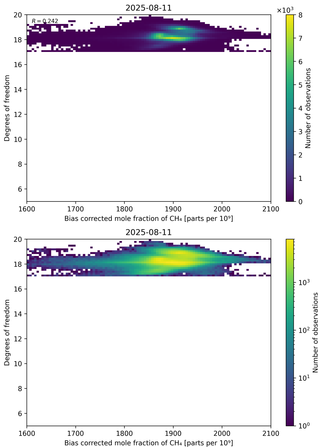
Figure 65: Scatter density plot of “Bias corrected mole fraction of CH 4 ” against “Degrees of freedom” for 2025-08-10 to 2025-08-12.
