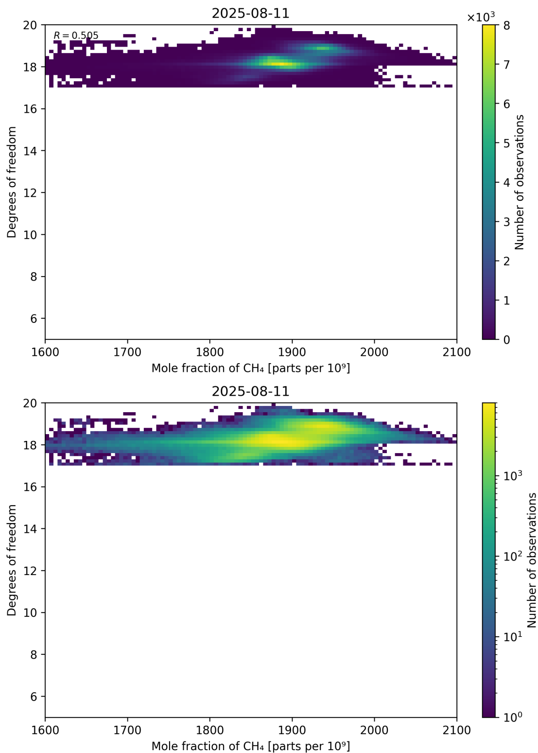
Figure 72: Scatter density plot of “Mole fraction of CH 4 ” against “Degrees of freedom” for 2025-08-10 to 2025-08-12.
