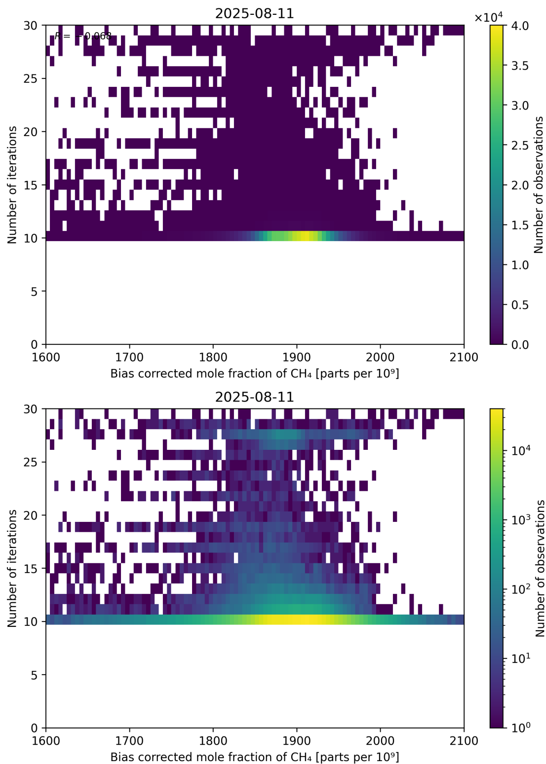
Figure 67: Scatter density plot of “Bias corrected mole fraction of CH 4 ” against “Number of iterations” for 2025-08-10 to 2025-08-12.
