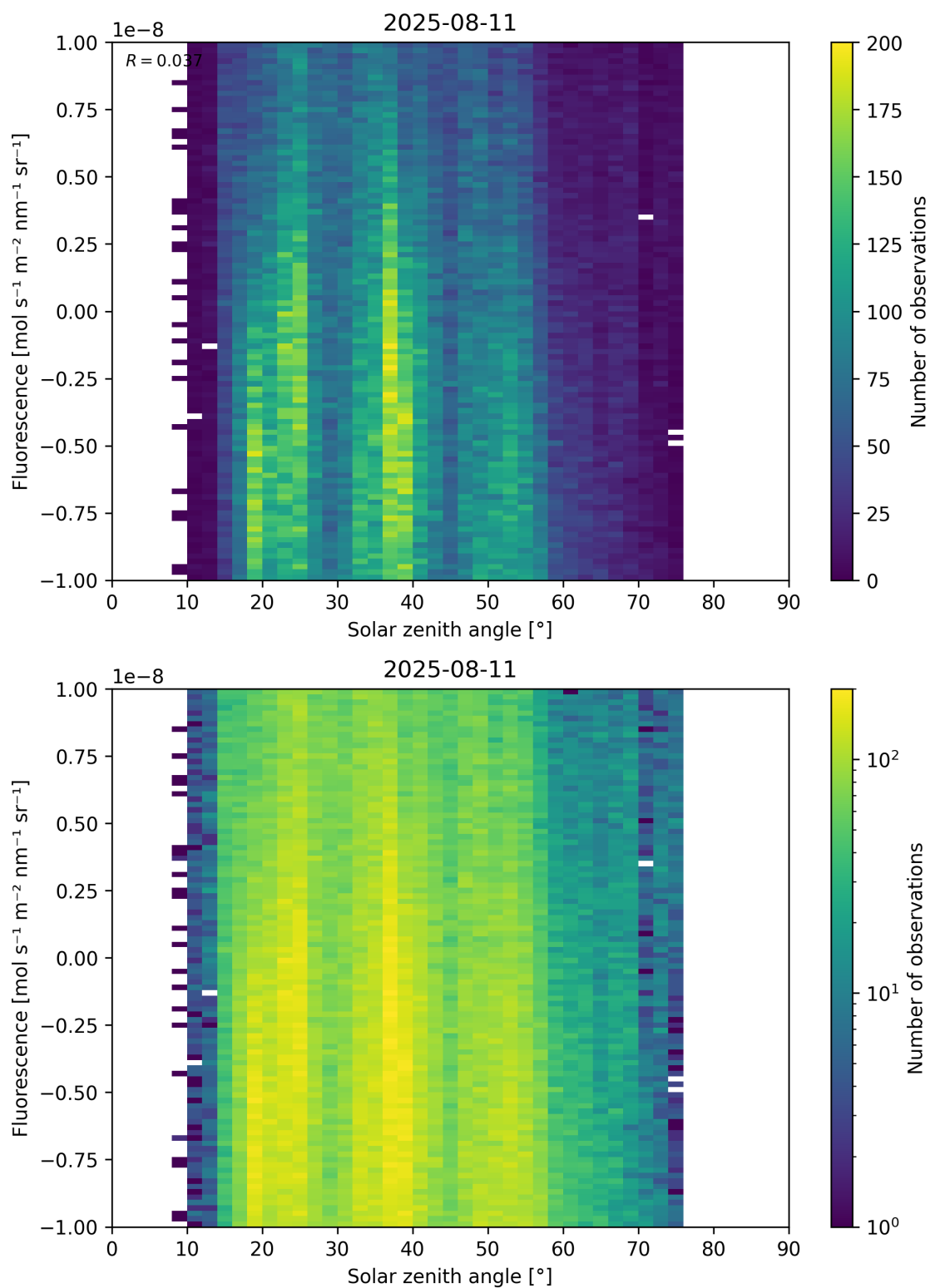
Figure 97: Scatter density plot of “Solar zenith angle” against “Fluorescence” for 2025-08-10 to 2025-08-12.
