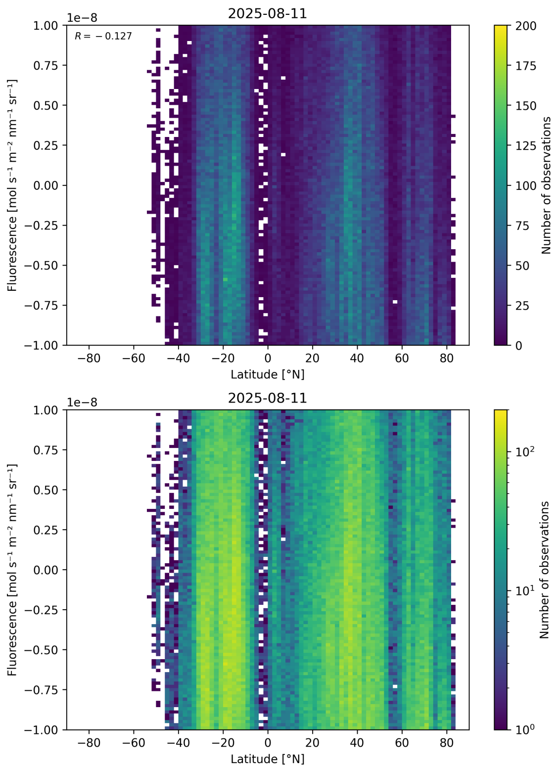
Figure 56: Scatter density plot of “Latitude” against “Fluorescence” for 2025-08-10 to 2025-08-12.
