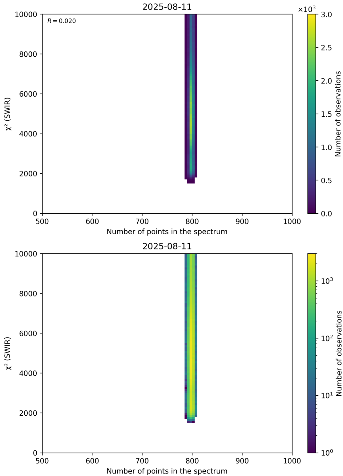
Figure 89: Scatter density plot of “Number of points in the spectrum” against “ \chi^2 (SWIR)” for 2025-08-10 to 2025-08-12.
