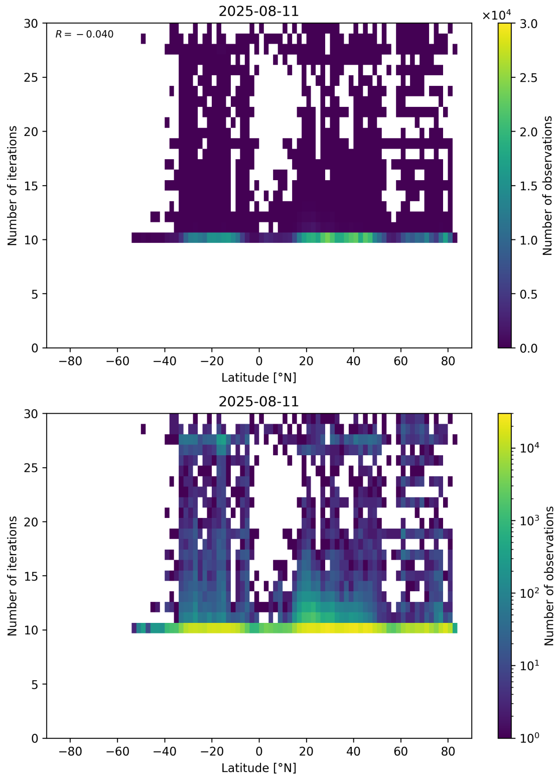
Figure 60: Scatter density plot of “Latitude” against “Number of iterations” for 2025-08-10 to 2025-08-12.
