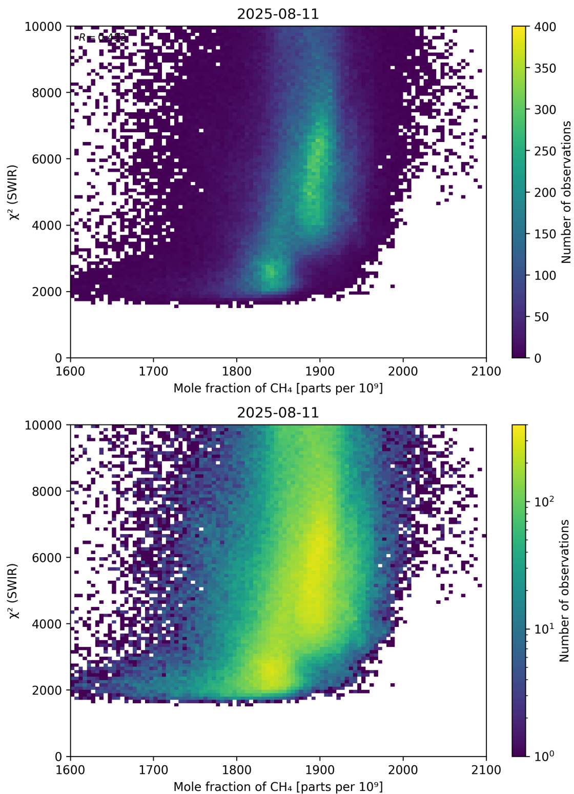
Figure 71: Scatter density plot of “Mole fraction of \text{CH}_4 ” against “ \chi^2 (SWIR)” for 2025-08-10 to 2025-08-12.
