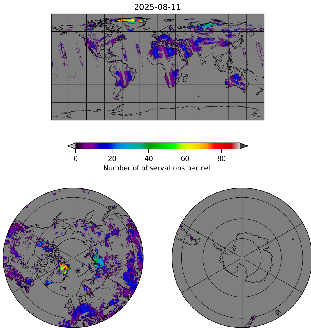
Figure 10: Map of the number of observations for 2025-08-10 to 2025-08-12
