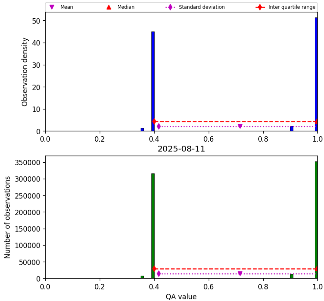
Figure 22: Histogram of “QA value” for 2025-08-10 to 2025-08-12
