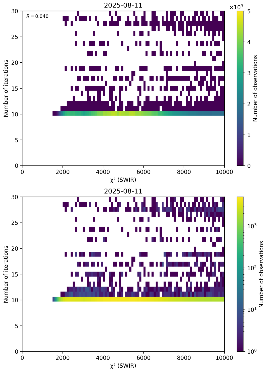
Figure 50: Scatter density plot of “ \chi^2 (SWIR)” against “Number of iterations” for 2025-08-10 to 2025-08-12.
