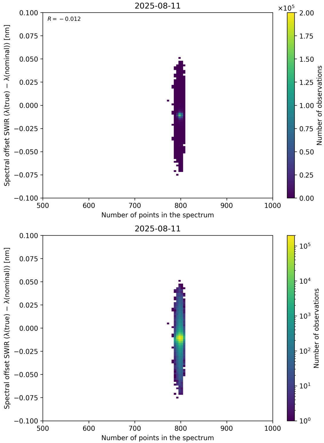
Figure 93: Scatter density plot of “Number of points in the spectrum” against “Spectral offset SWIR ( \lambda_{\text{true}} - \lambda_{\text{nominal}} )” for 2025-08-10 to 2025-08-12.
