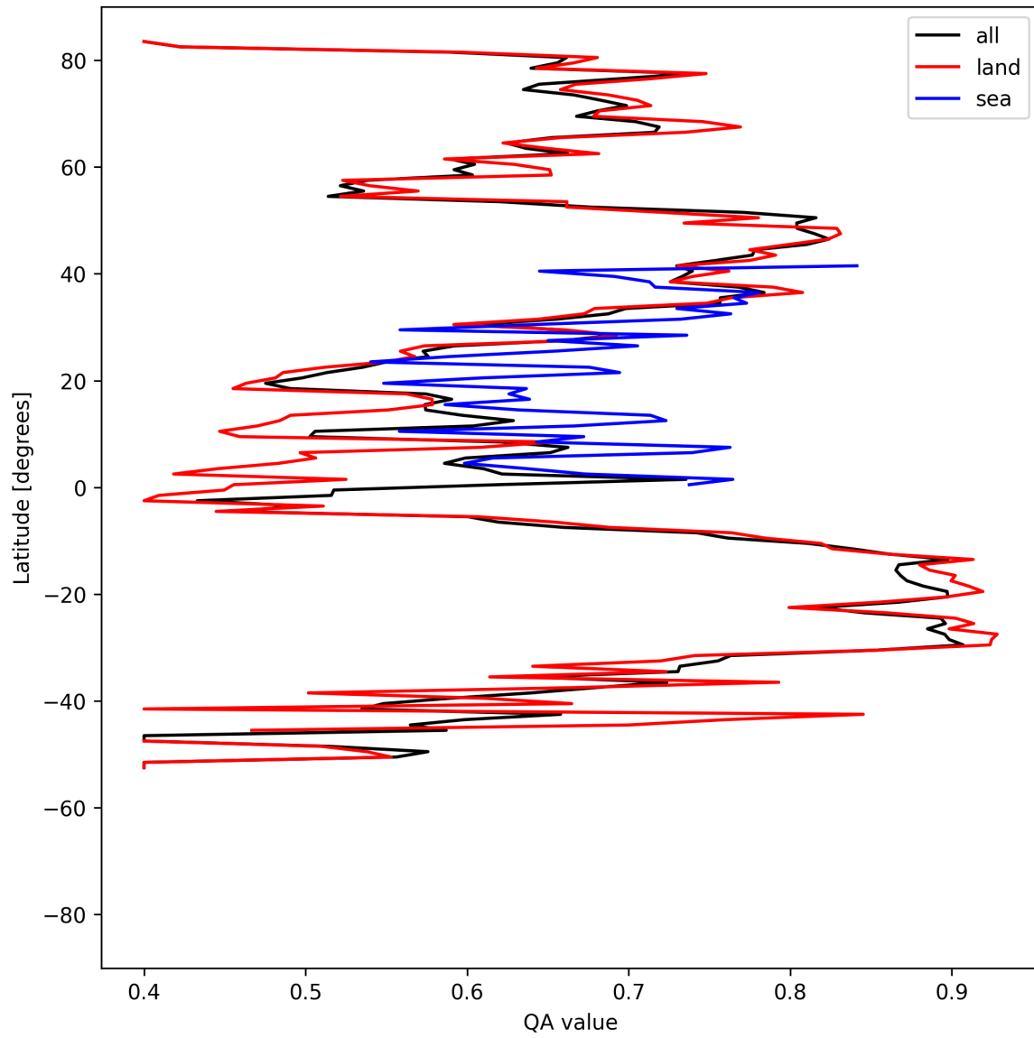
Figure 11: Zonal average of “QA value” for 2025-08-10 to 2025-08-12.
