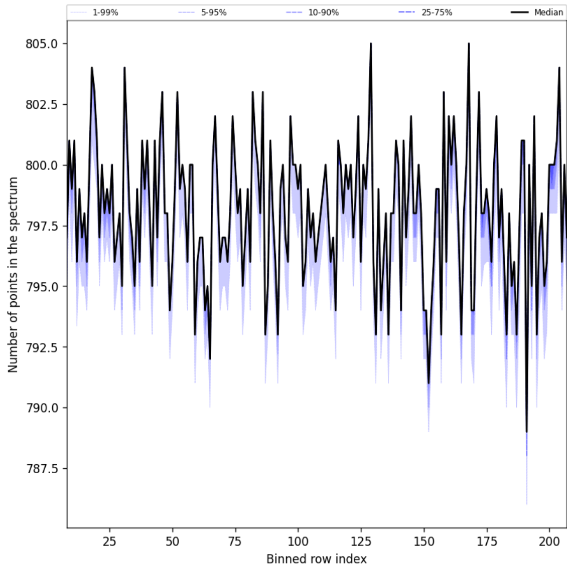
Figure 37: Along track statistics of “Number of points in the spectrum” for 2025-08-10 to 2025-08-12
