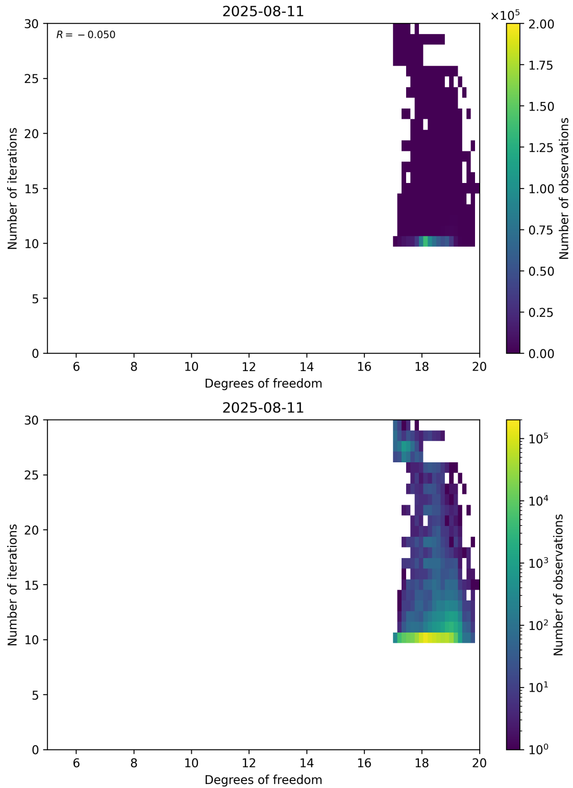
Figure 52: Scatter density plot of “Degrees of freedom” against “Number of iterations” for 2025-08-10 to 2025-08-12.
