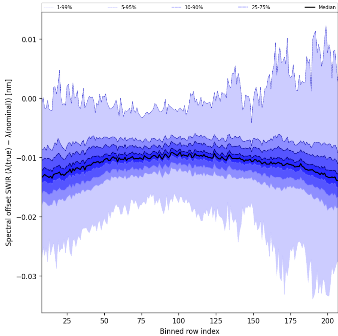
Figure 38: Along track statistics of “Spectral offset SWIR ( \lambda_{\text{true}} - \lambda_{\text{nominal}} )” for 2025-08-10 to 2025-08-12
