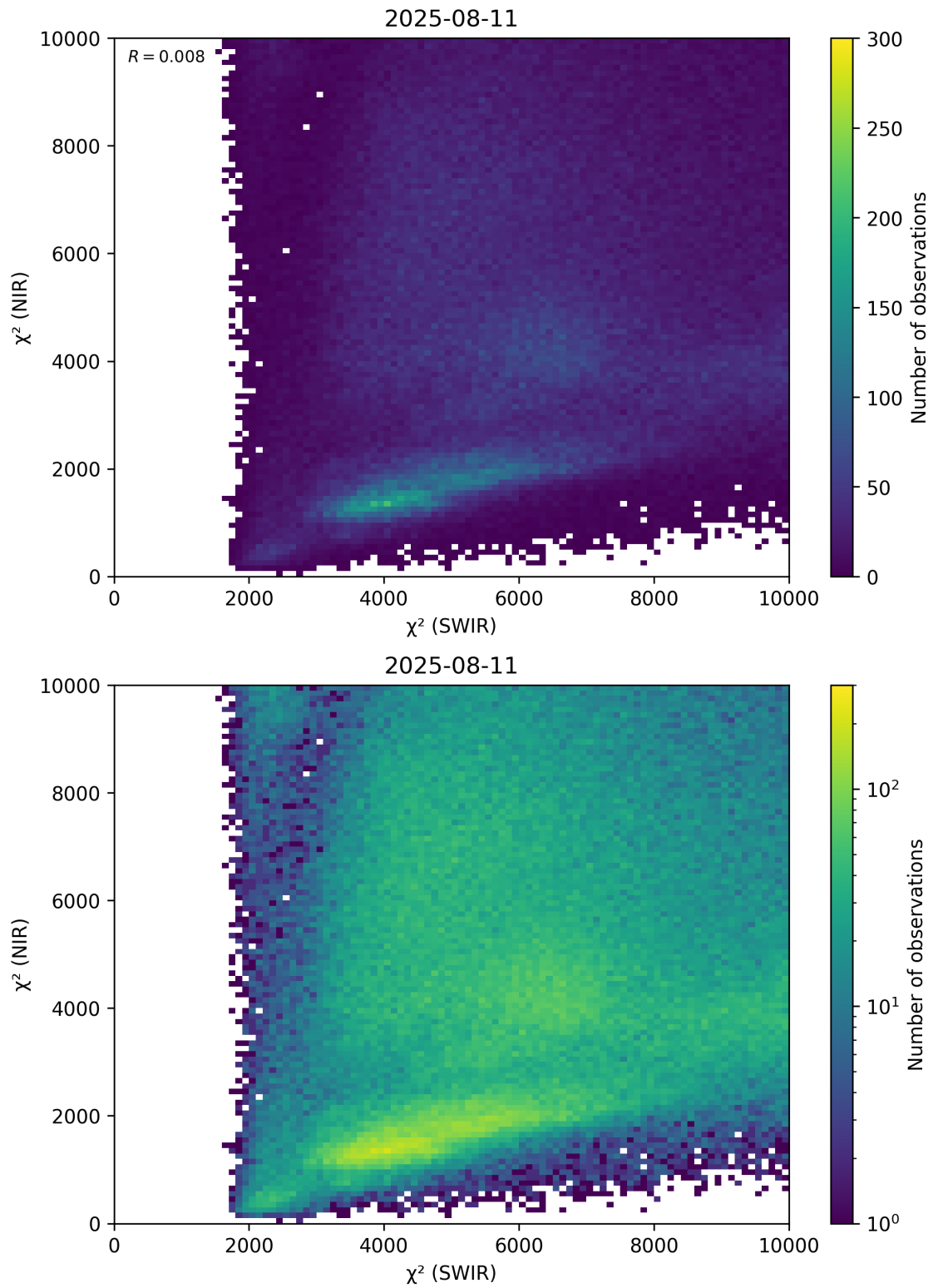
Figure 47: Scatter density plot of “ \chi^2 (SWIR)” against “ \chi^2 (NIR)” for 2025-08-10 to 2025-08-12.
