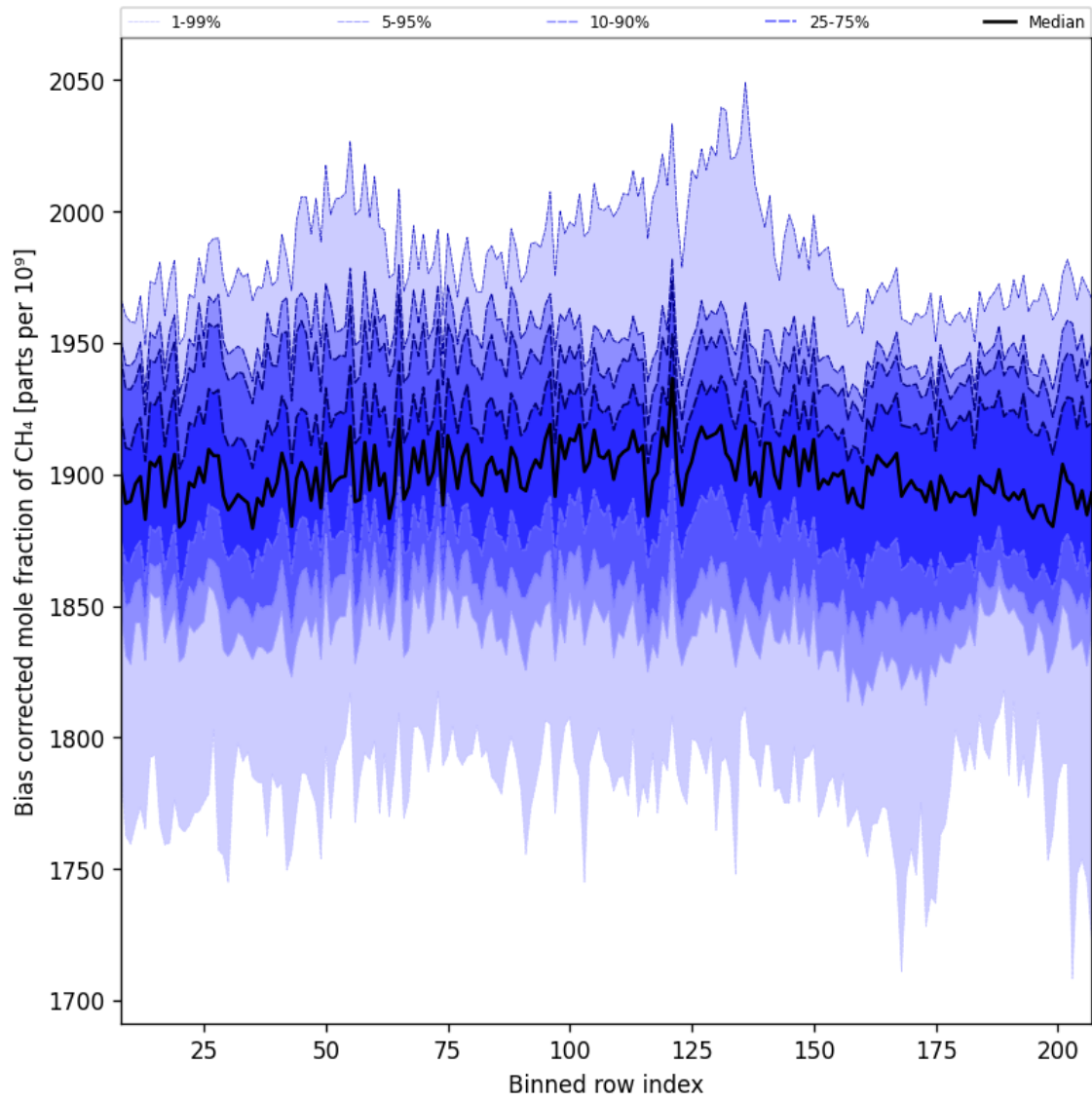
Figure 36: Along track statistics of “Bias corrected mole fraction of CH 4 ” for 2025-08-10 to 2025-08-12
