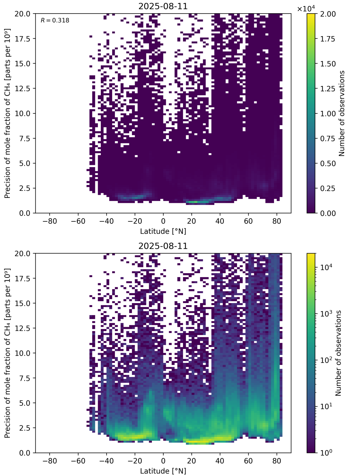
Figure 59: Scatter density plot of “Latitude” against “Precision of mole fraction of \text{CH}_4 ” for 2025-08-10 to 2025-08-12.
