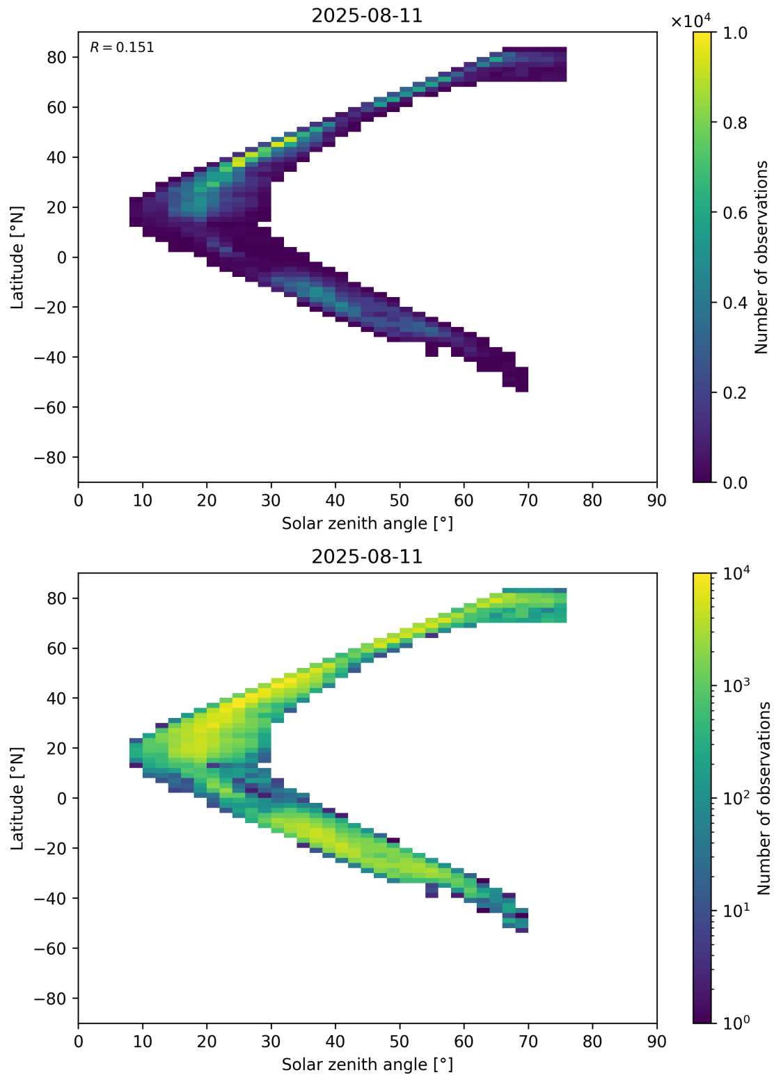
Figure 98: Scatter density plot of “Solar zenith angle” against “Latitude” for 2025-08-10 to 2025-08-12.
