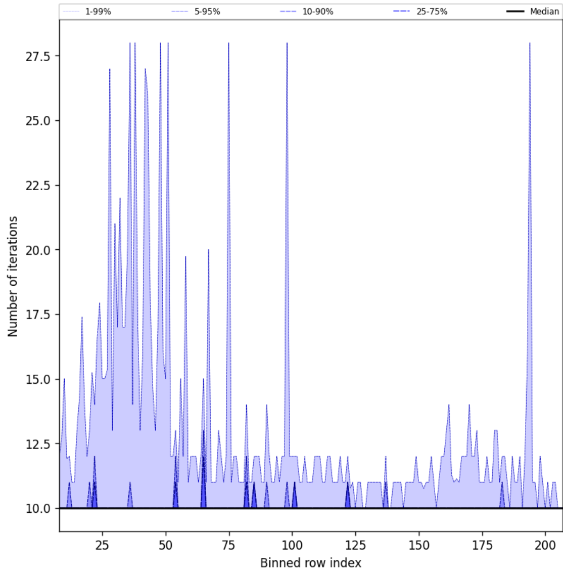
Figure 42: Along track statistics of “Number of iterations” for 2025-08-10 to 2025-08-12
