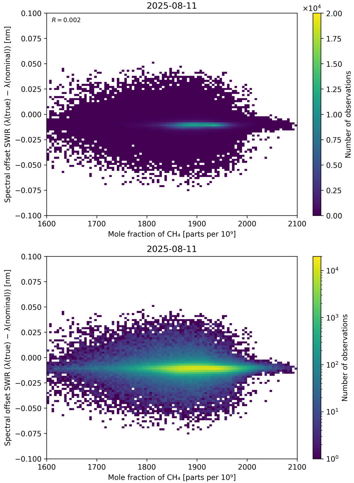
Figure 86: Scatter density plot of “Mole fraction of CH 4 ” against “Spectral offset SWIR ( \lambda_{\text{true}} - \lambda_{\text{nominal}} )” for 2025-08-10 to 2025-08-12.
