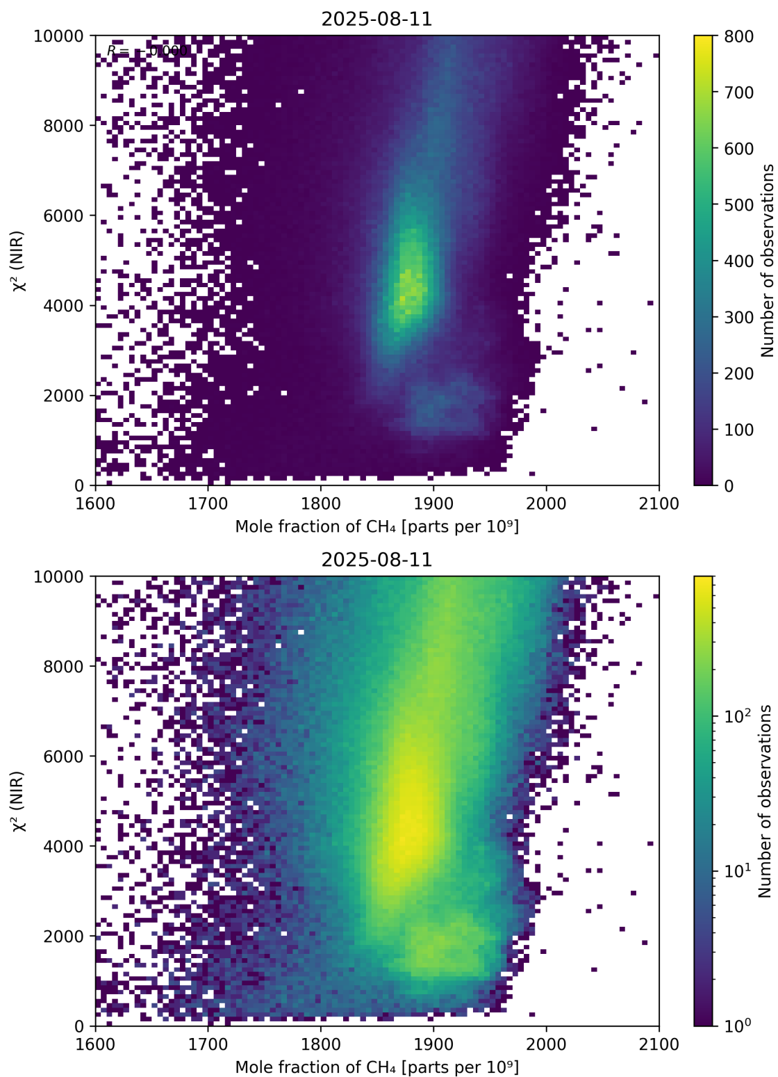
Figure 70: Scatter density plot of “Mole fraction of CH 4 ” against “ \chi^2 (NIR)” for 2025-08-10 to 2025-08-12.
