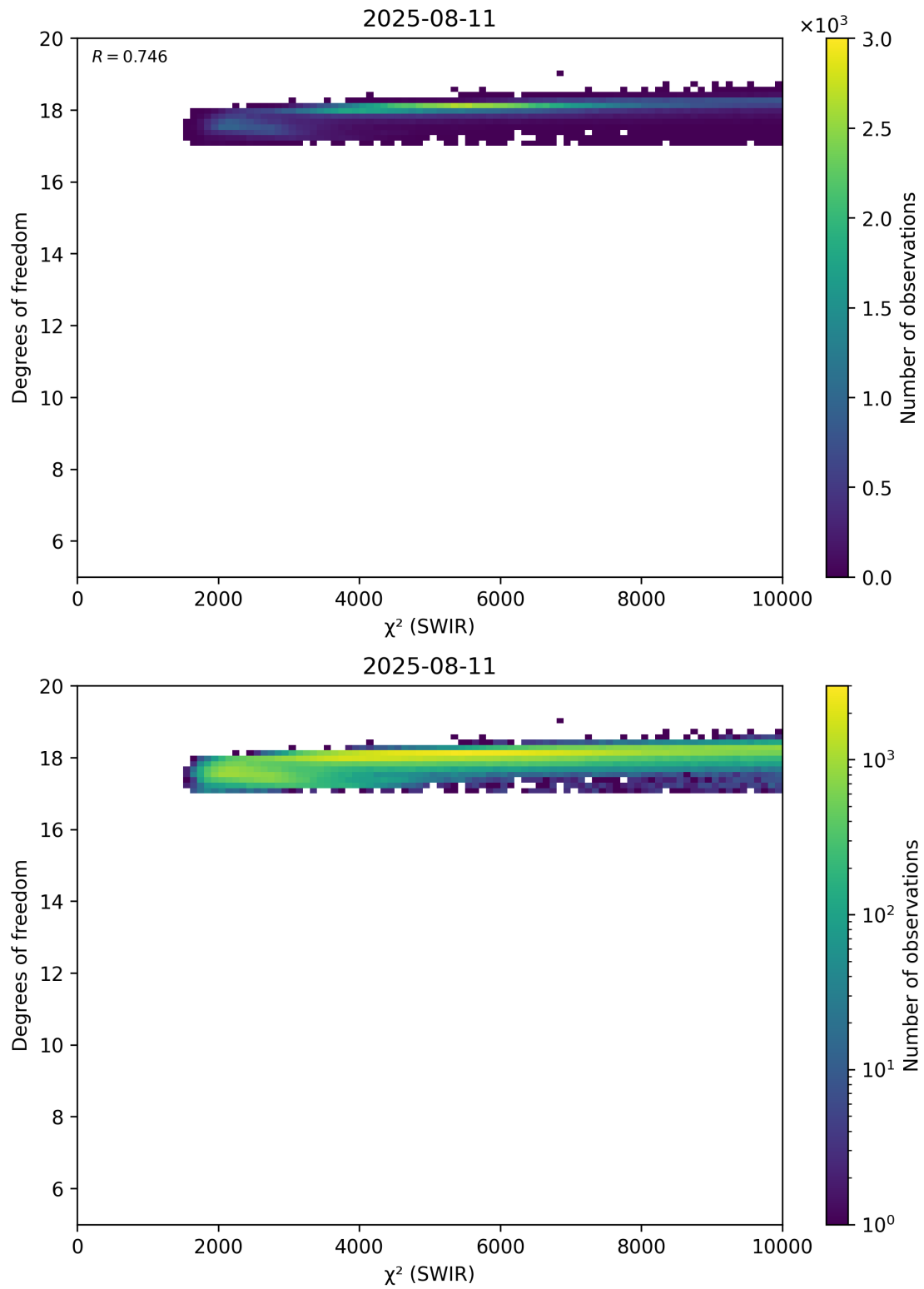
Figure 48: Scatter density plot of “ \chi^2 (SWIR)” against “Degrees of freedom” for 2025-08-10 to 2025-08-12.
