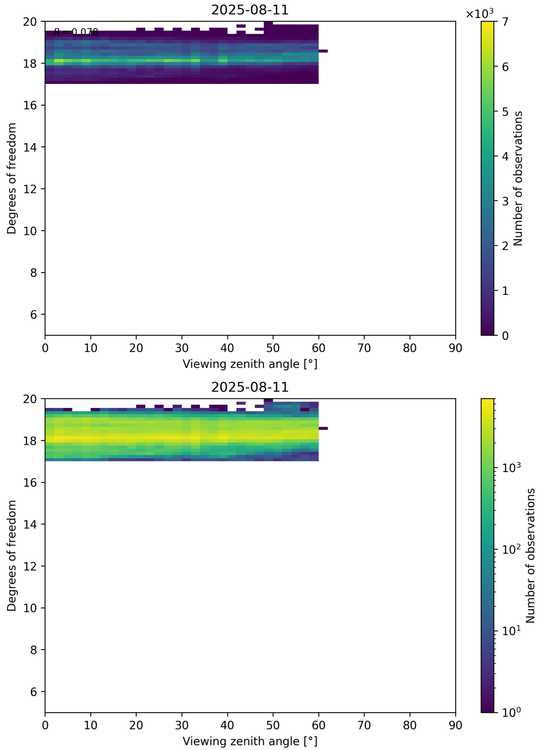
Figure 107: Scatter density plot of “Viewing zenith angle” against “Degrees of freedom” for 2025-08-10 to 2025-08-12.
