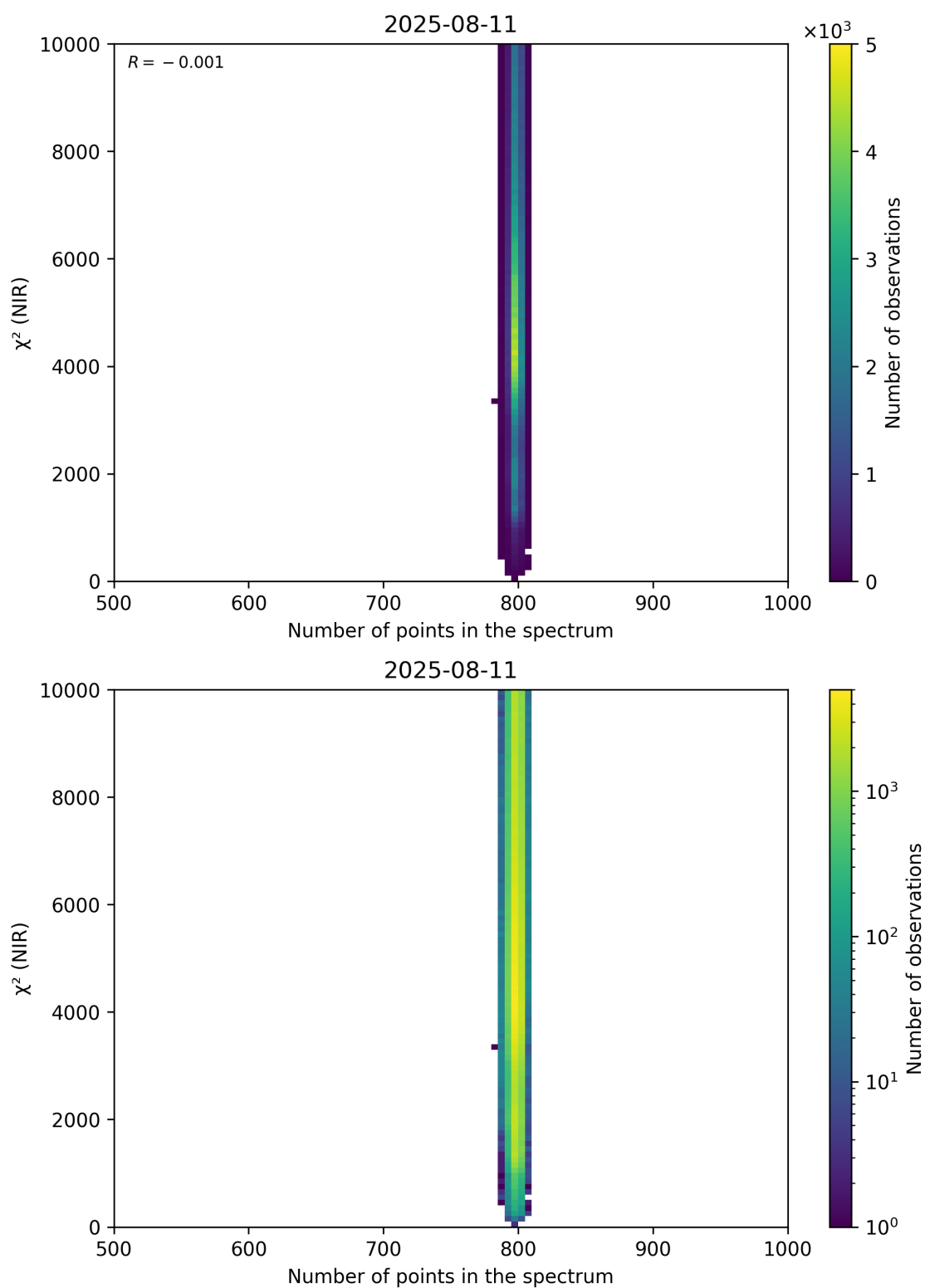
Figure 88: Scatter density plot of “Number of points in the spectrum” against “ \chi^2 (NIR)” for 2025-08-10 to 2025-08-12.
