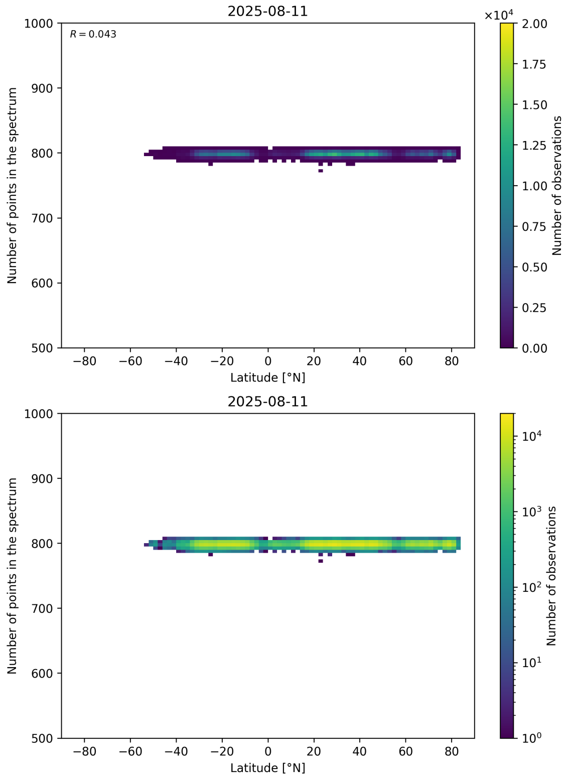
Figure 61: Scatter density plot of “Latitude” against “Number of points in the spectrum” for 2025-08-10 to 2025-08-12.
