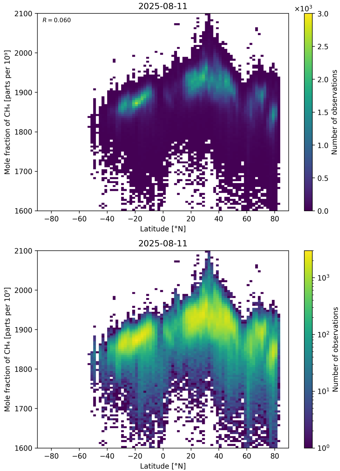
Figure 57: Scatter density plot of “Latitude” against “Mole fraction of \text{CH}_4 ” for 2025-08-10 to 2025-08-12.
