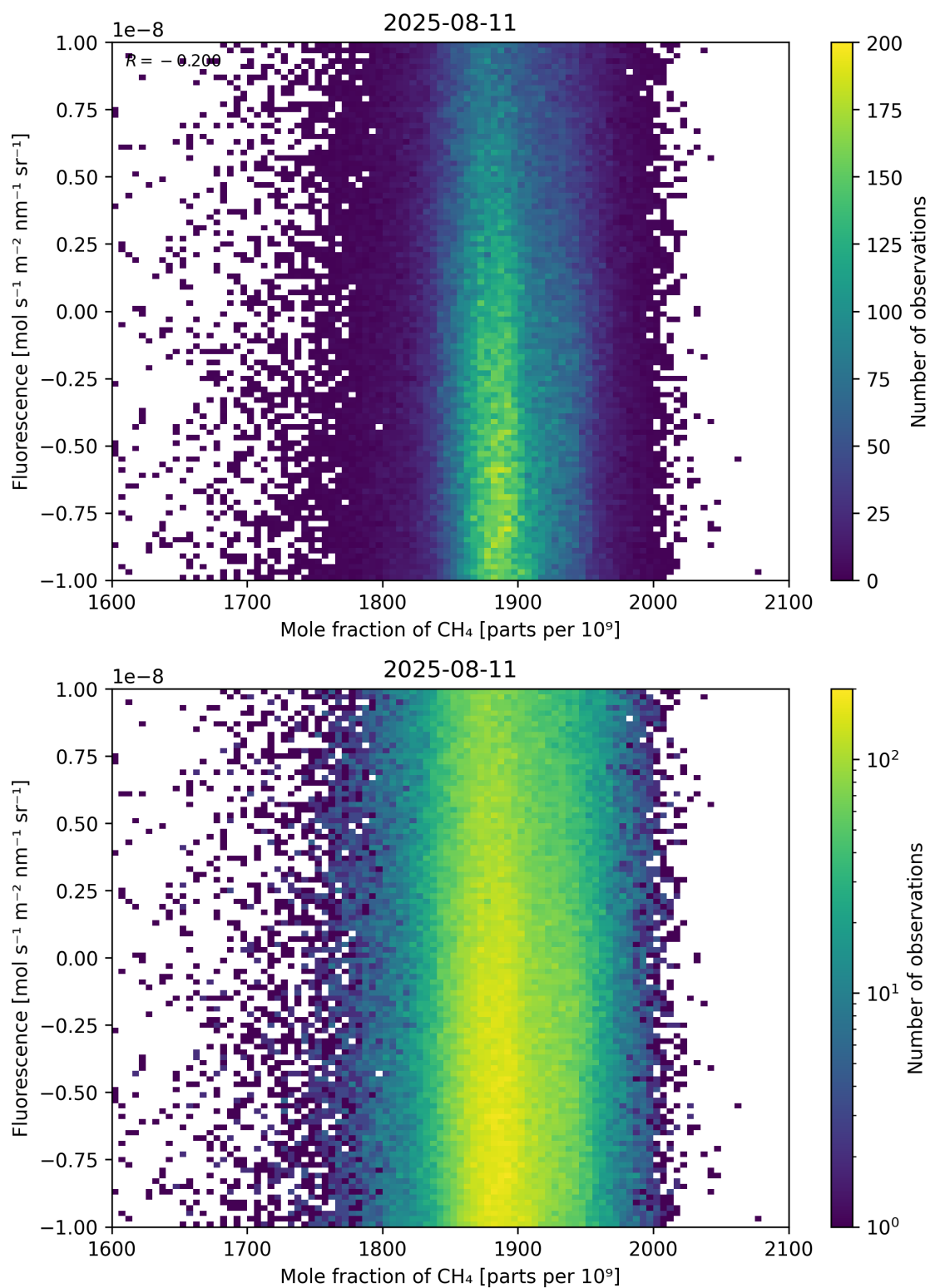
Figure 73: Scatter density plot of “Mole fraction of \text{CH}_4 ” against “Fluorescence” for 2025-08-10 to 2025-08-12.
