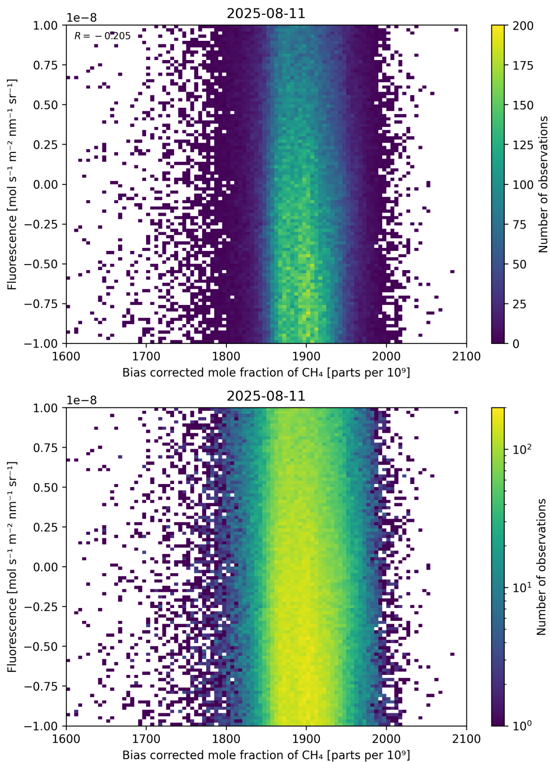
Figure 66: Scatter density plot of “Bias corrected mole fraction of \text{CH}_4 ” against “Fluorescence” for 2025-08-10 to 2025-08-12.
