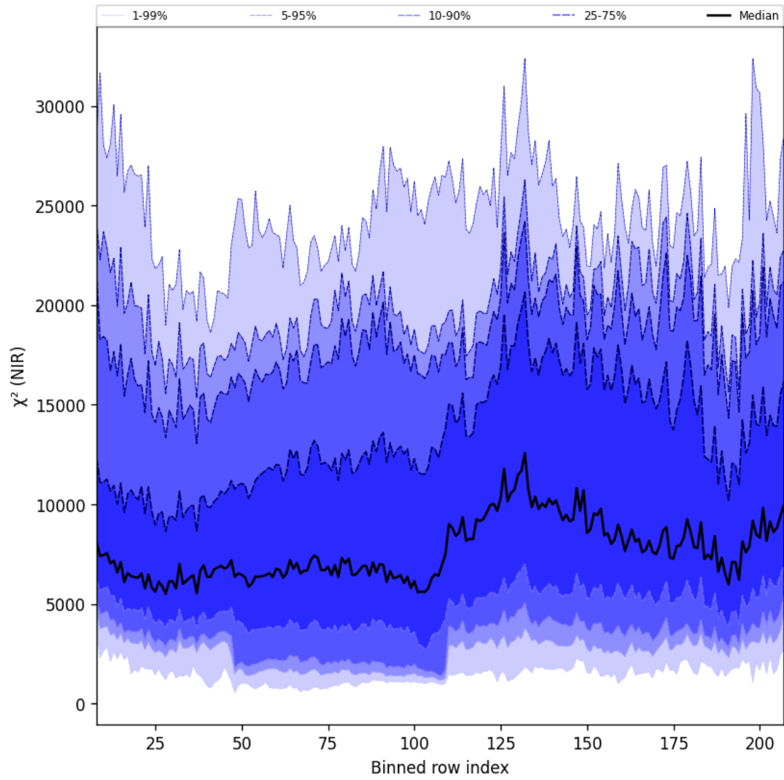
Figure 40: Along track statistics of “ \chi^2 (NIR)” for 2025-08-10 to 2025-08-12
