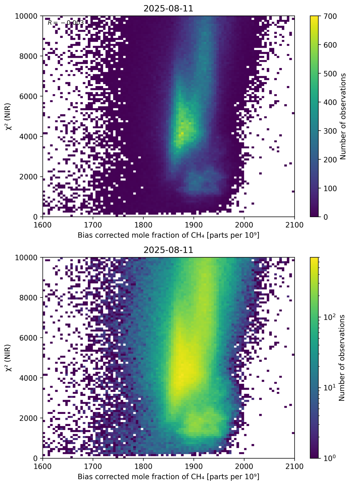
Figure 63: Scatter density plot of “Bias corrected mole fraction of CH 4 ” against “ \chi^2 (NIR)” for 2025-08-10 to 2025-08-12.
