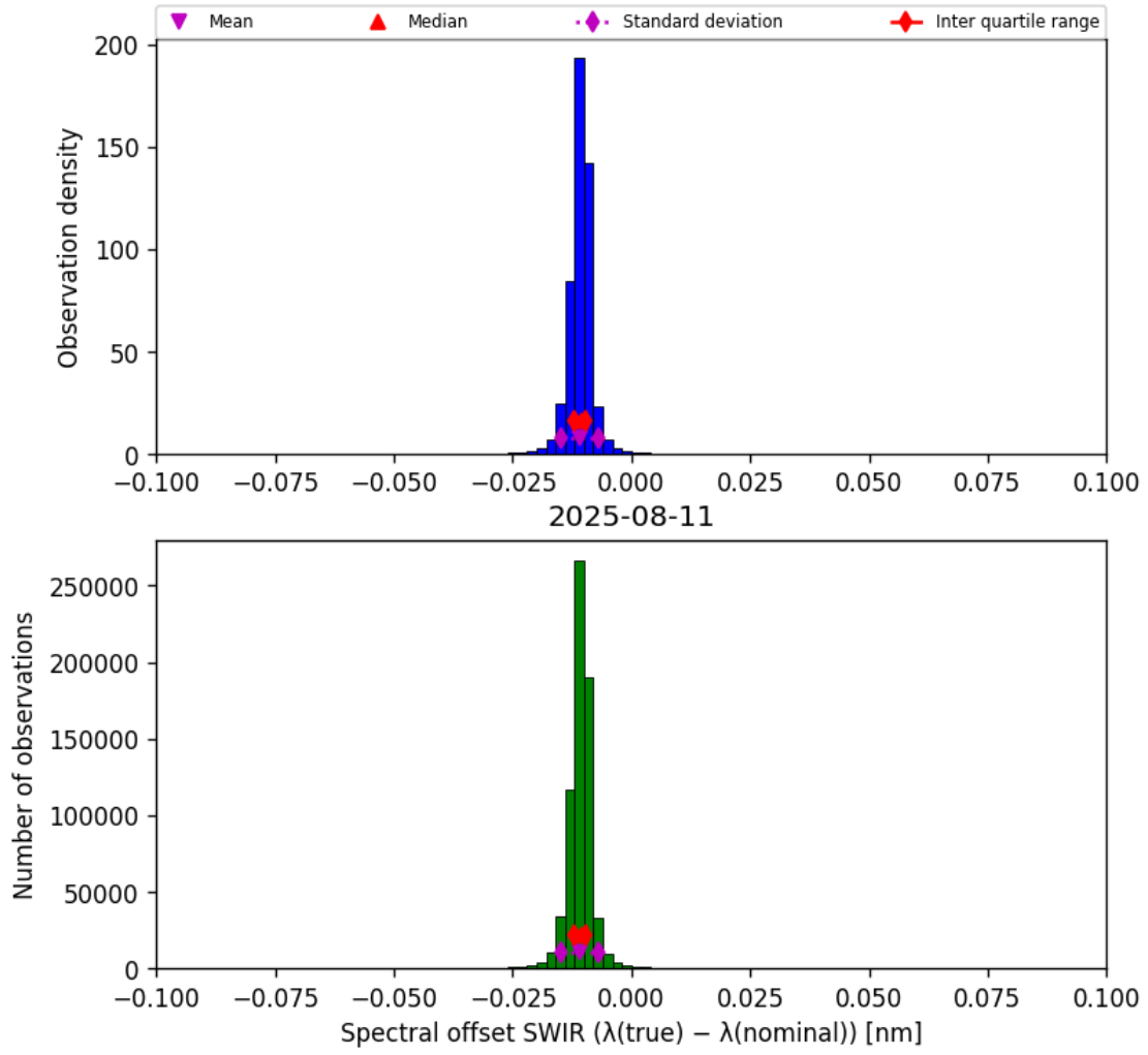
Figure 27: Histogram of “Spectral offset SWIR ( \lambda_{\text{true}} - \lambda_{\text{nominal}} )” for 2025-08-10 to 2025-08-12
