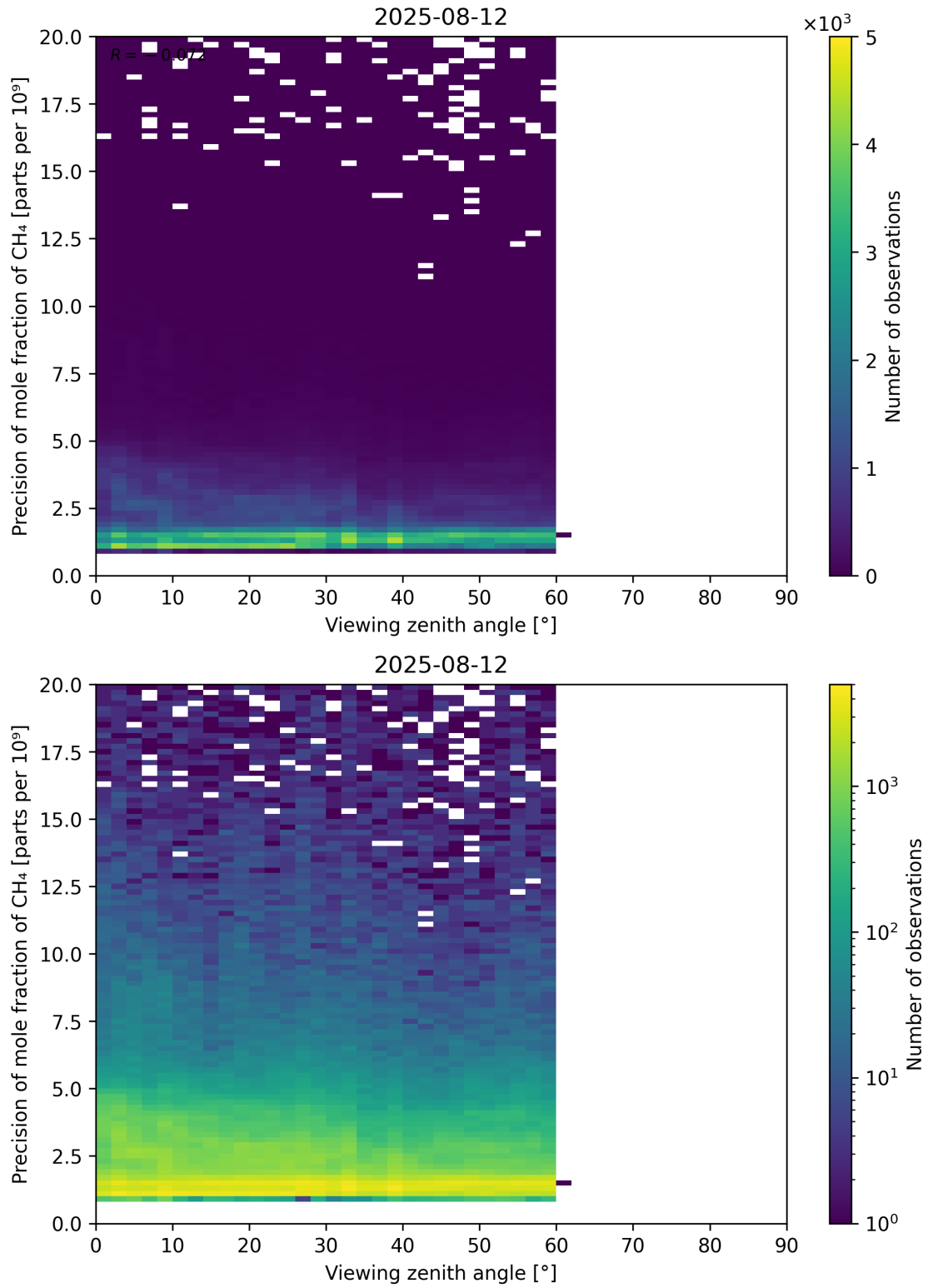
Figure 112: Scatter density plot of “Viewing zenith angle” against “Precision of mole fraction of CH 4 ” for 2025-08-11 to 2025-08-13.
