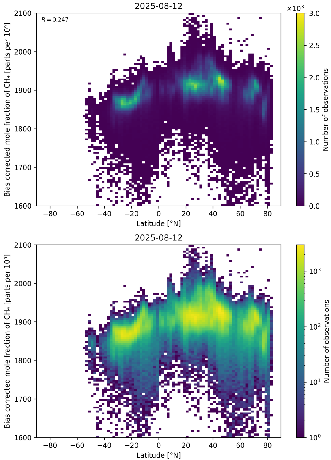
Figure 58: Scatter density plot of “Latitude” against “Bias corrected mole fraction of \text{CH}_4 ” for 2025-08-11 to 2025-08-13.
