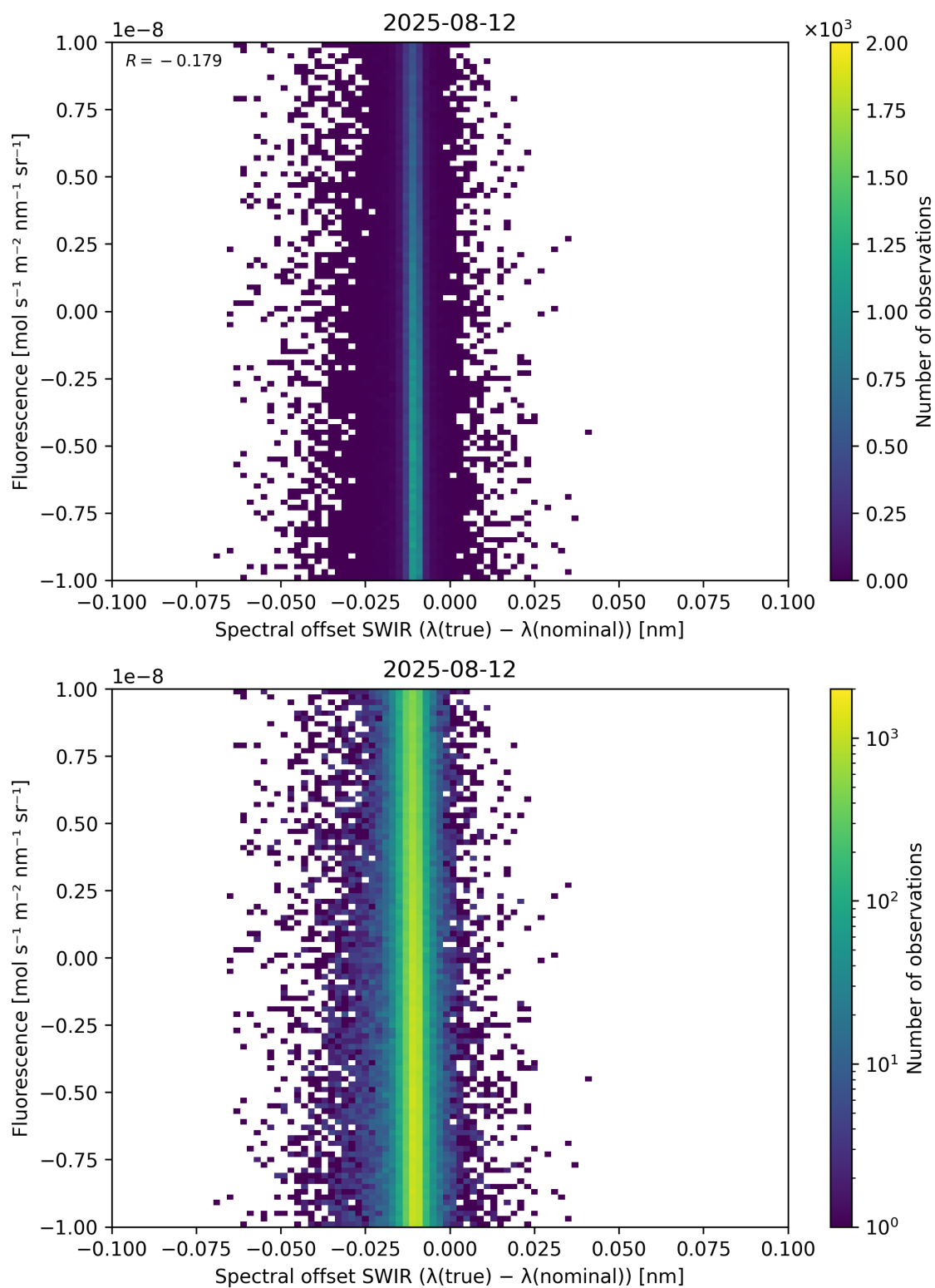
Figure 120: Scatter density plot of “Spectral offset SWIR ( \lambda_{\text{true}} - \lambda_{\text{nominal}} )” against “Fluorescence” for 2025-08-11 to 2025-08-13.
