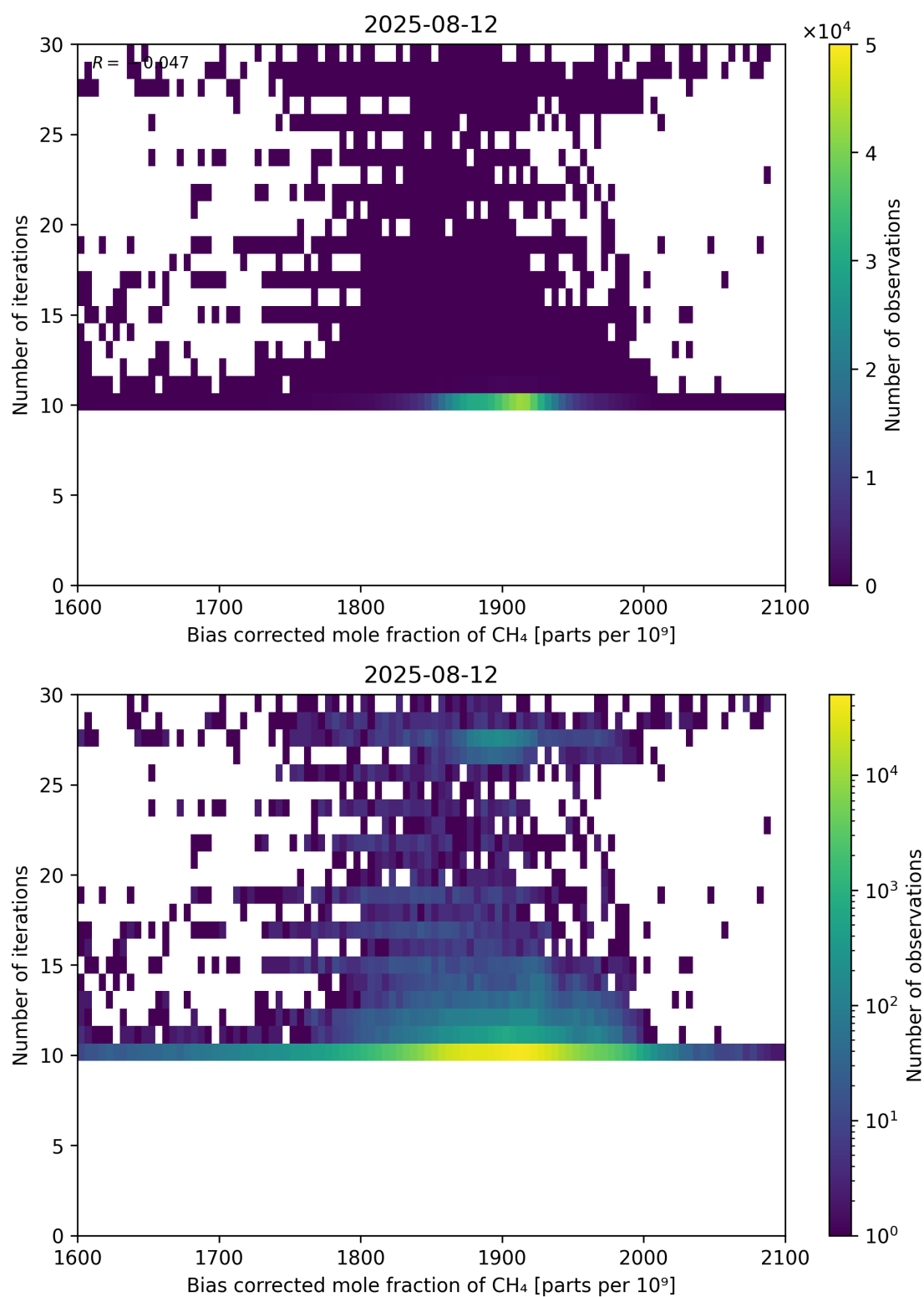
Figure 67: Scatter density plot of “Bias corrected mole fraction of CH 4 ” against “Number of iterations” for 2025-08-11 to 2025-08-13.
