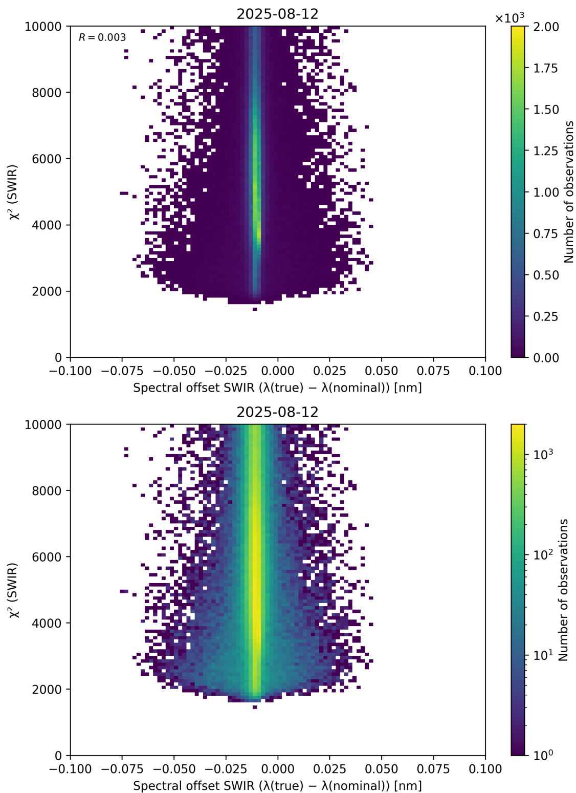
Figure 118: Scatter density plot of “Spectral offset SWIR ( \lambda_{\text{true}} - \lambda_{\text{nominal}} )” against “ \chi^2 (SWIR)” for 2025-08-11 to 2025-08-13.
