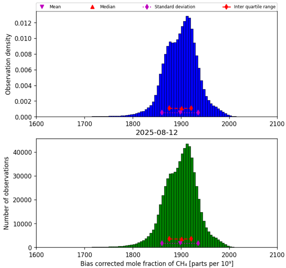
Figure 25: Histogram of “Bias corrected mole fraction of CH 4 ” for 2025-08-11 to 2025-08-13
