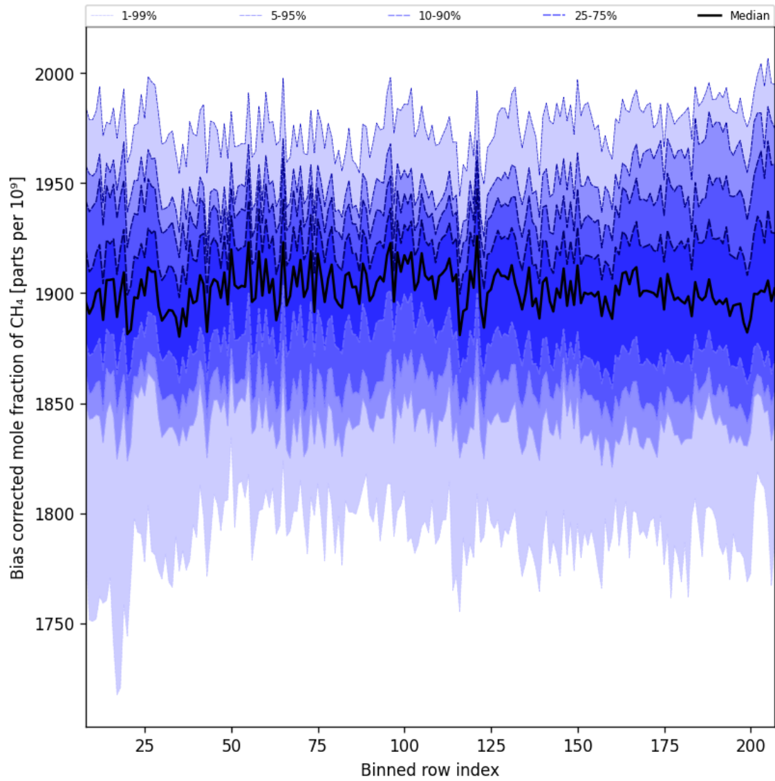
Figure 36: Along track statistics of “Bias corrected mole fraction of CH 4 ” for 2025-08-11 to 2025-08-13
