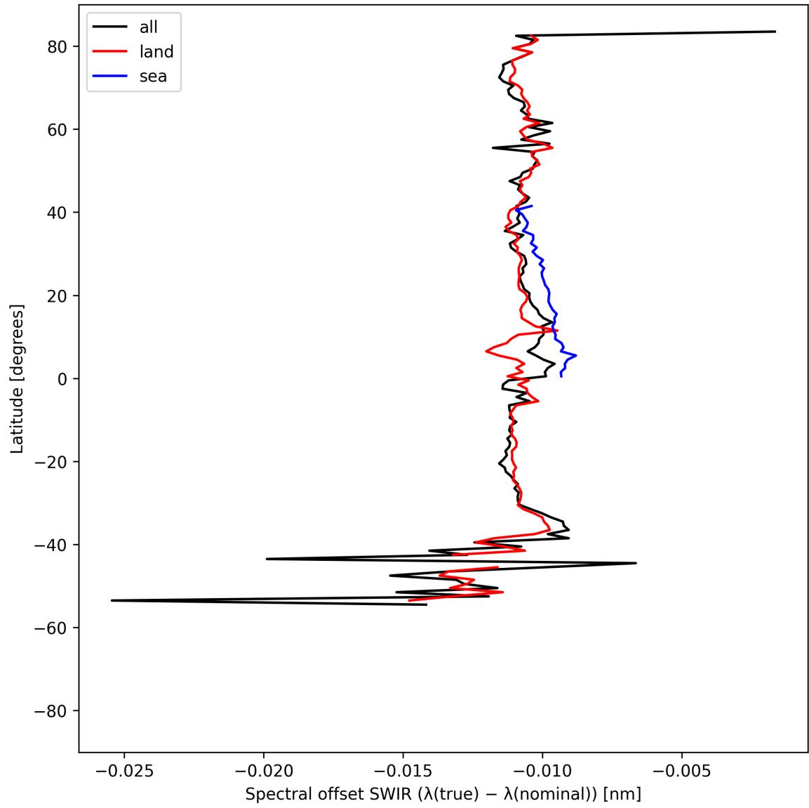
Figure 16: Zonal average of “Spectral offset SWIR ( \lambda_{\text{true}} - \lambda_{\text{nominal}} )” for 2025-08-11 to 2025-08-13.
