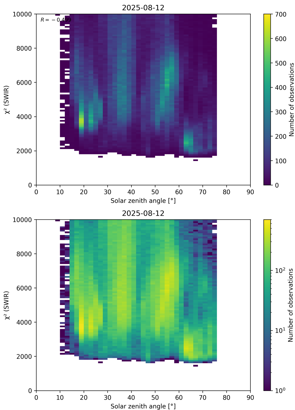
Figure 95: Scatter density plot of “Solar zenith angle” against “ \chi^2 (SWIR)” for 2025-08-11 to 2025-08-13.
