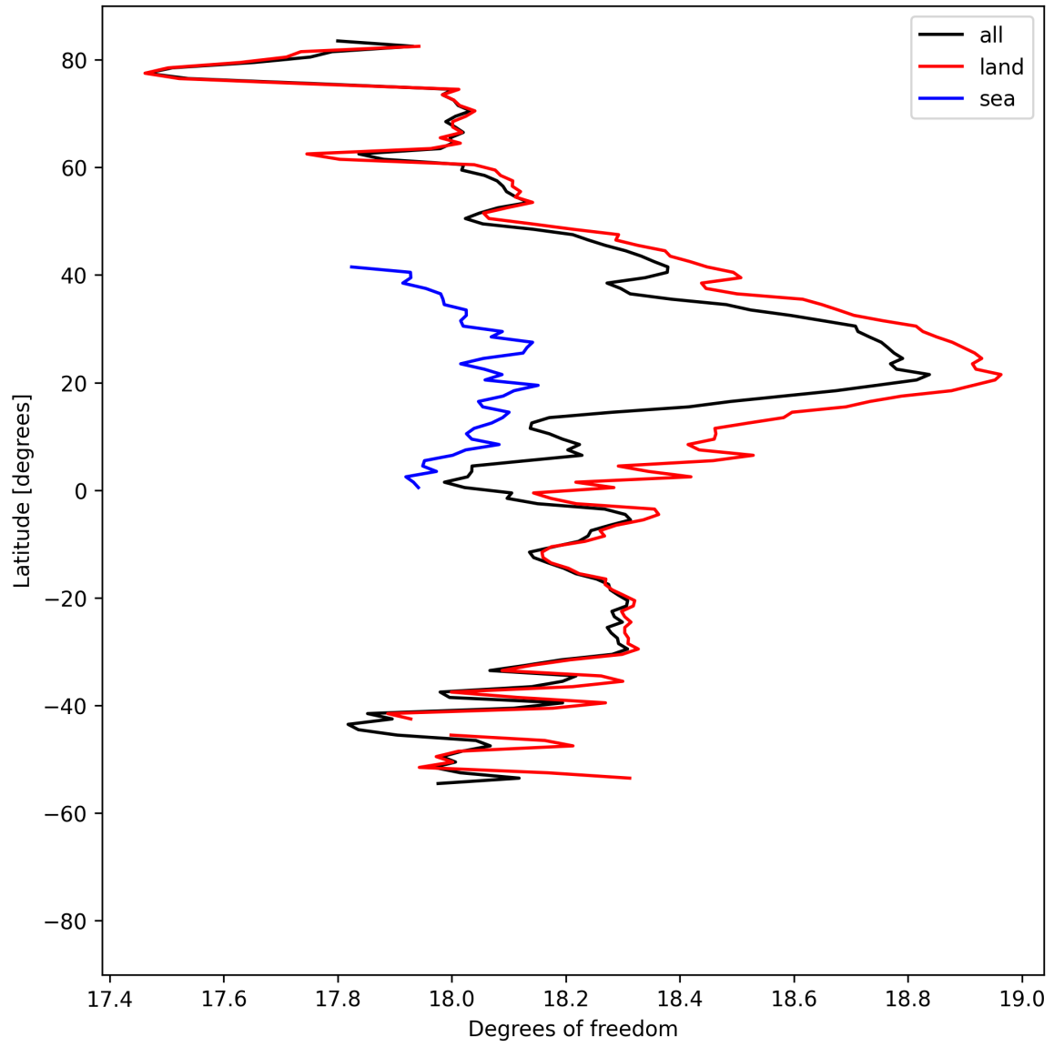
Figure 19: Zonal average of “Degrees of freedom” for 2025-08-11 to 2025-08-13.
