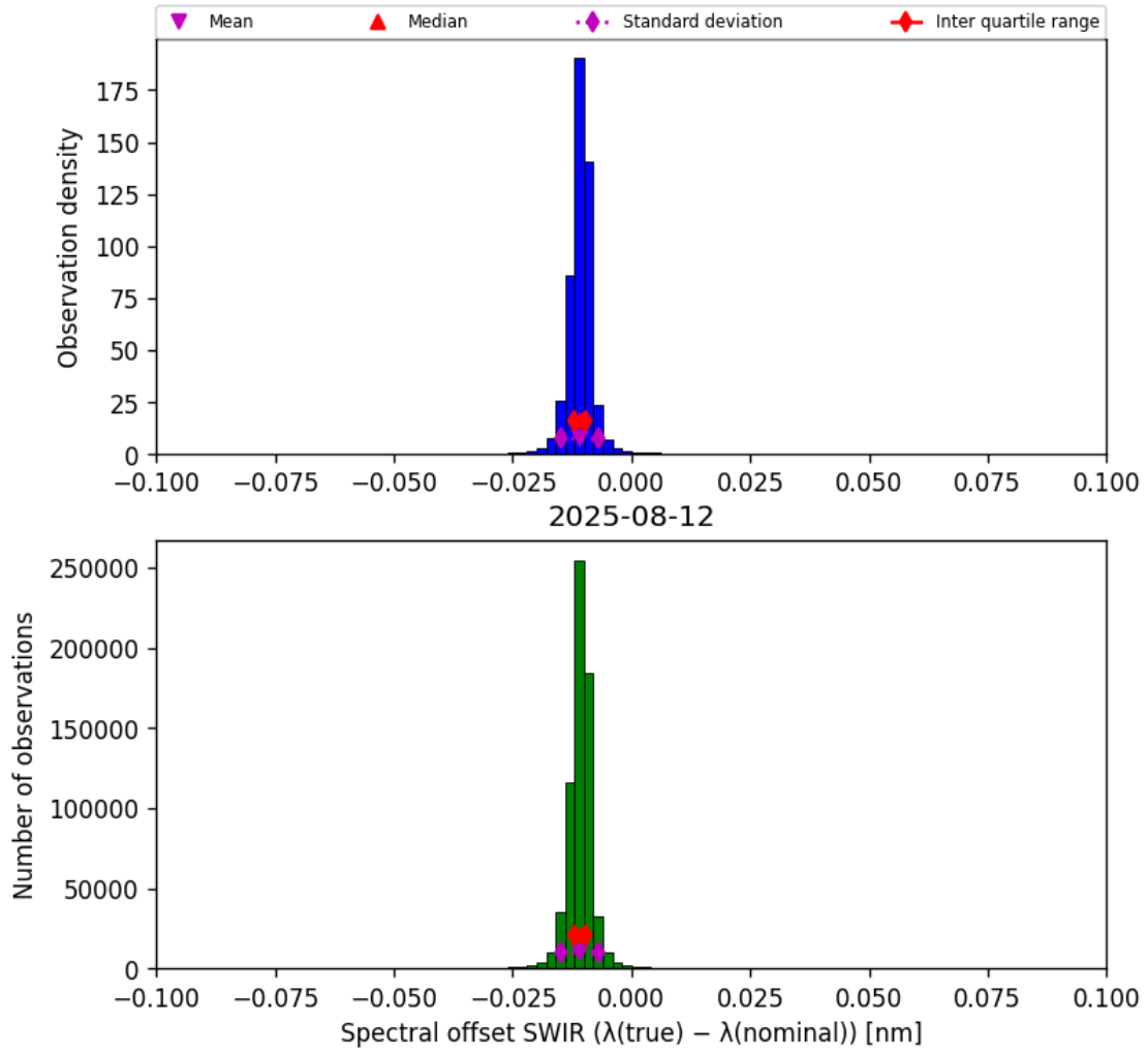
Figure 27: Histogram of “Spectral offset SWIR ( \lambda_{\text{true}} - \lambda_{\text{nominal}} )” for 2025-08-11 to 2025-08-13
