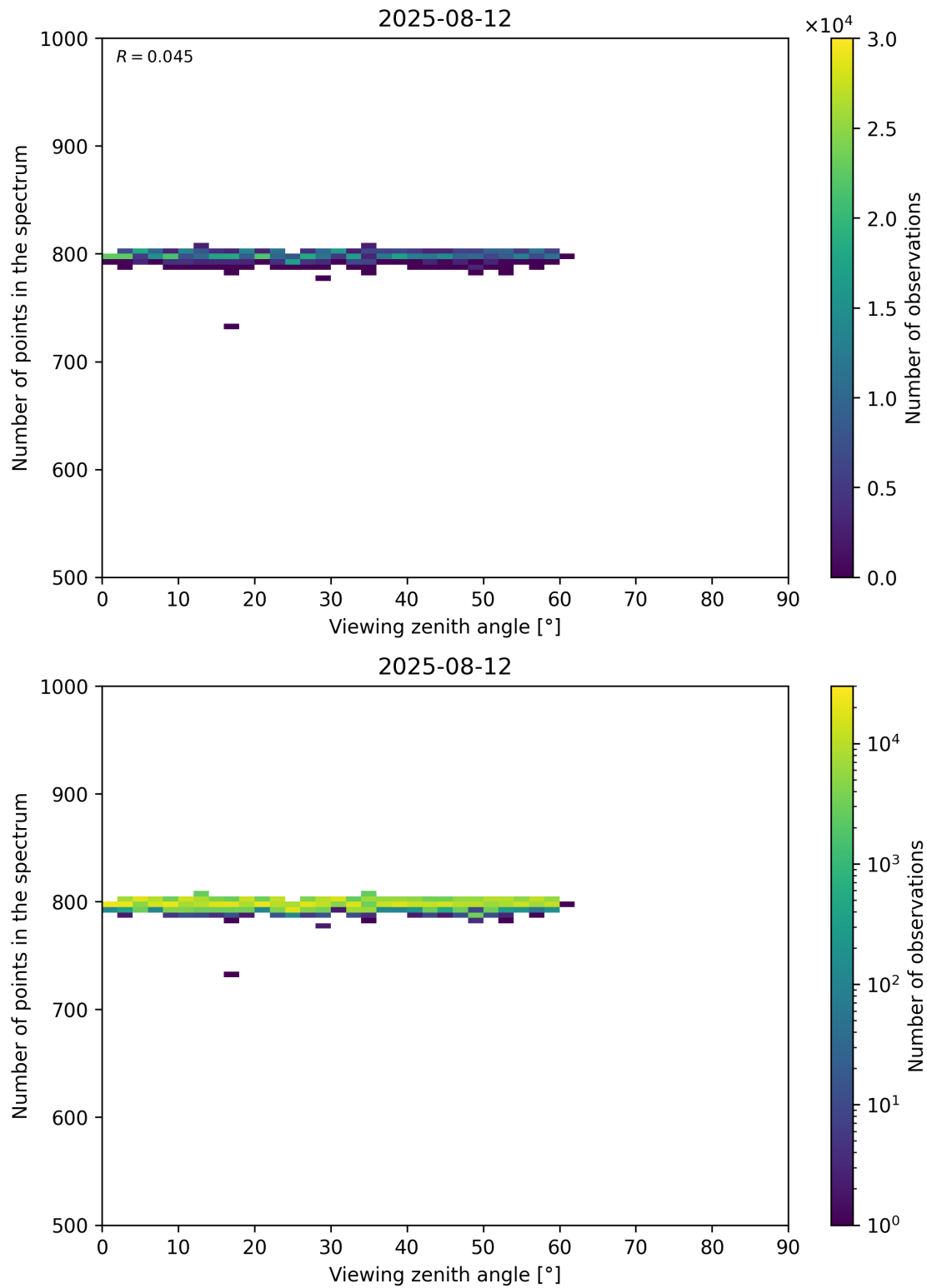
Figure 114: Scatter density plot of “Viewing zenith angle” against “Number of points in the spectrum” for 2025-08-11 to 2025-08-13.
