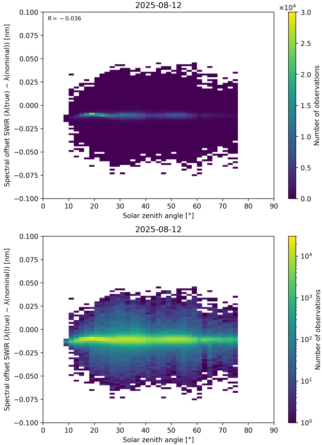
Figure 104: Scatter density plot of “Solar zenith angle” against “Spectral offset SWIR ( \lambda_{\text{true}} - \lambda_{\text{nominal}} )” for 2025-08-11 to 2025-08-13.
