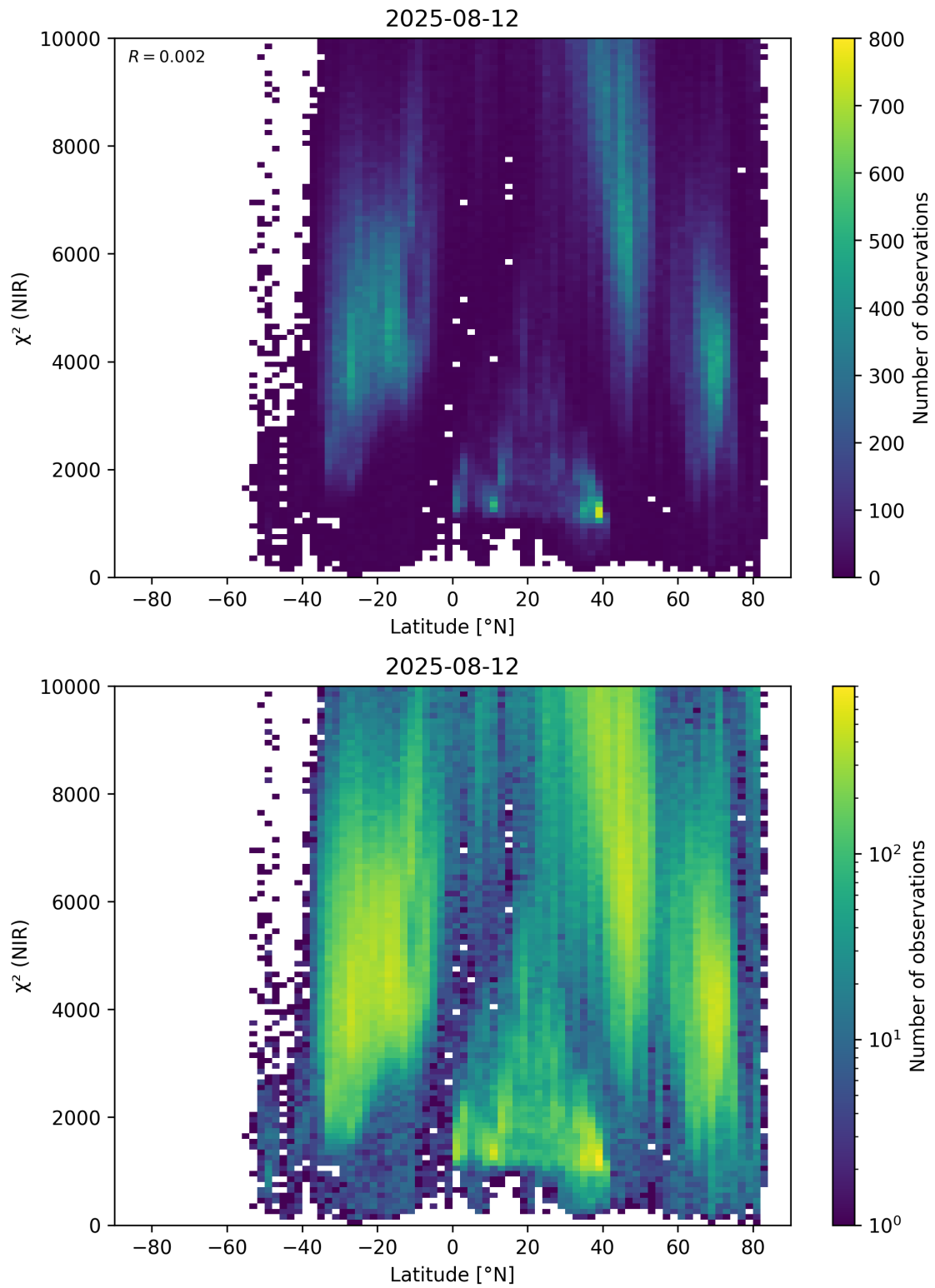
Figure 53: Scatter density plot of “Latitude” against “ \chi^2 (NIR)” for 2025-08-11 to 2025-08-13.
