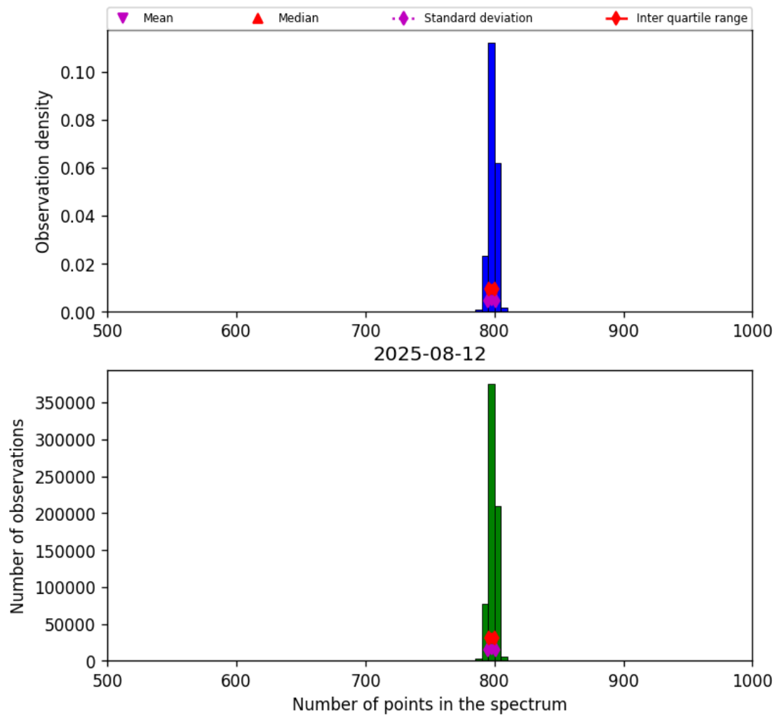
Figure 26: Histogram of “Number of points in the spectrum” for 2025-08-11 to 2025-08-13
