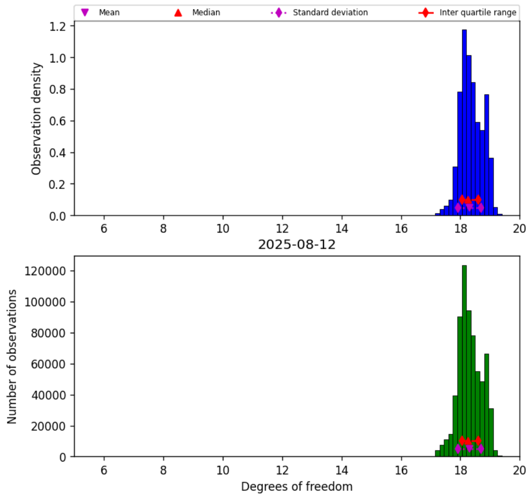
Figure 30: Histogram of “Degrees of freedom” for 2025-08-11 to 2025-08-13
