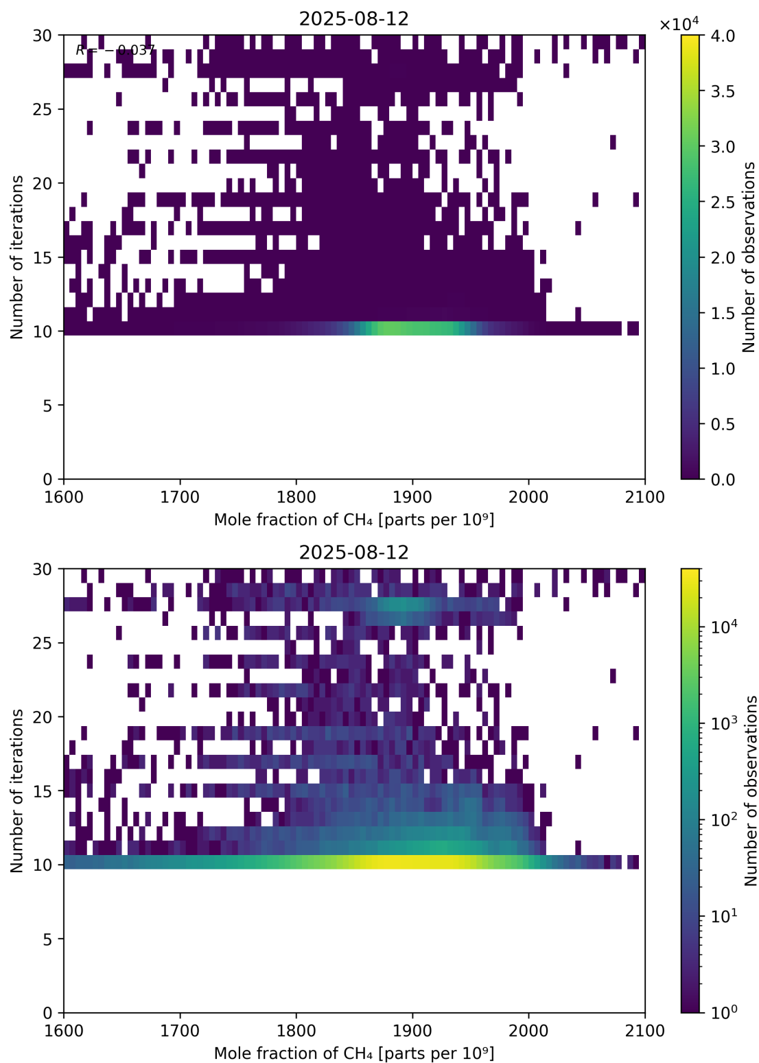
Figure 76: Scatter density plot of “Mole fraction of CH 4 ” against “Number of iterations” for 2025-08-11 to 2025-08-13.
