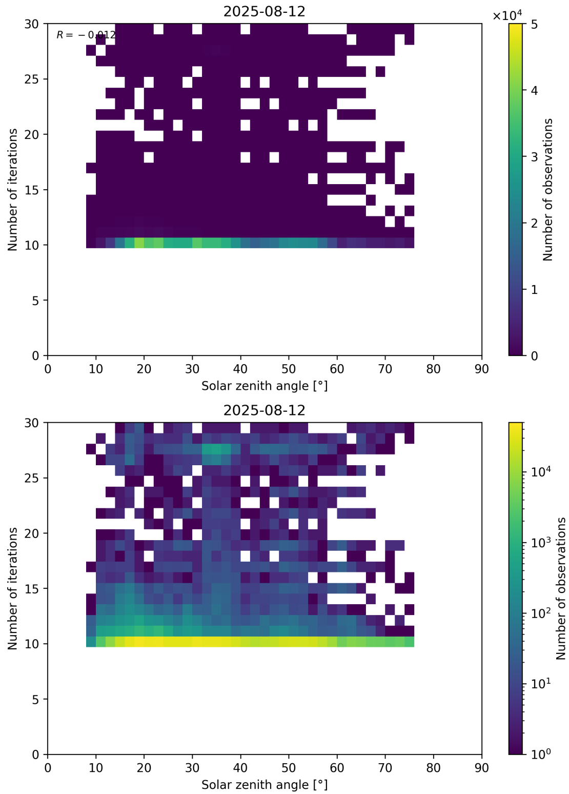
Figure 102: Scatter density plot of “Solar zenith angle” against “Number of iterations” for 2025-08-11 to 2025-08-13.
