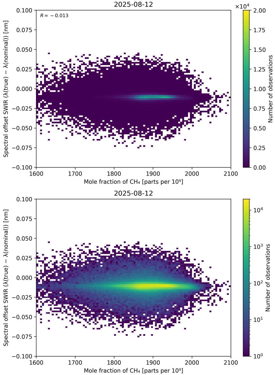
Figure 86: Scatter density plot of “Mole fraction of CH 4 ” against “Spectral offset SWIR ( \lambda_{\text{true}} - \lambda_{\text{nominal}} )” for 2025-08-11 to 2025-08-13.
