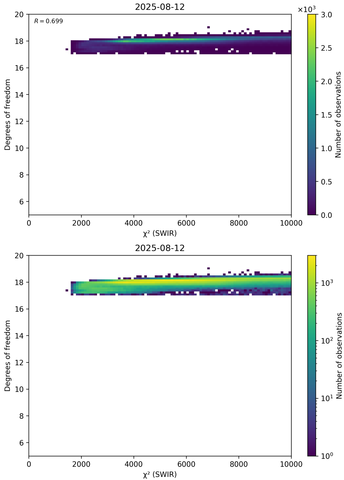
Figure 48: Scatter density plot of “ \chi^2 (SWIR)” against “Degrees of freedom” for 2025-08-11 to 2025-08-13.
