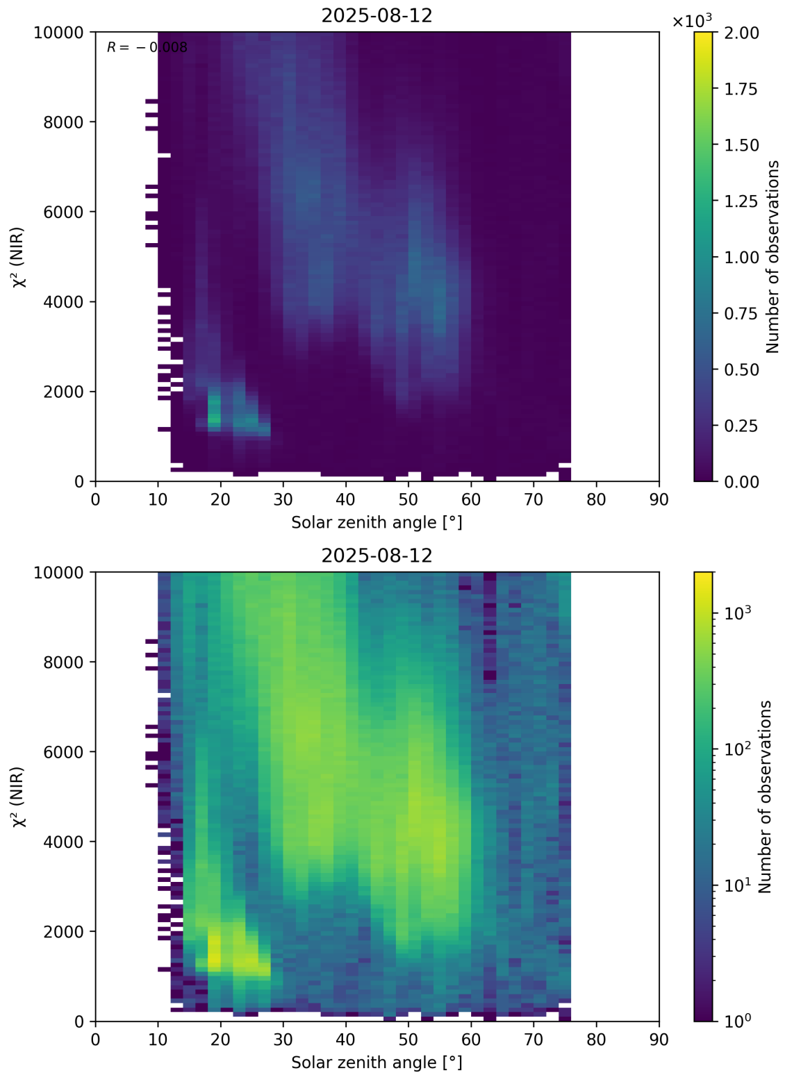
Figure 94: Scatter density plot of “Solar zenith angle” against “ \chi^2 (NIR)” for 2025-08-11 to 2025-08-13.
