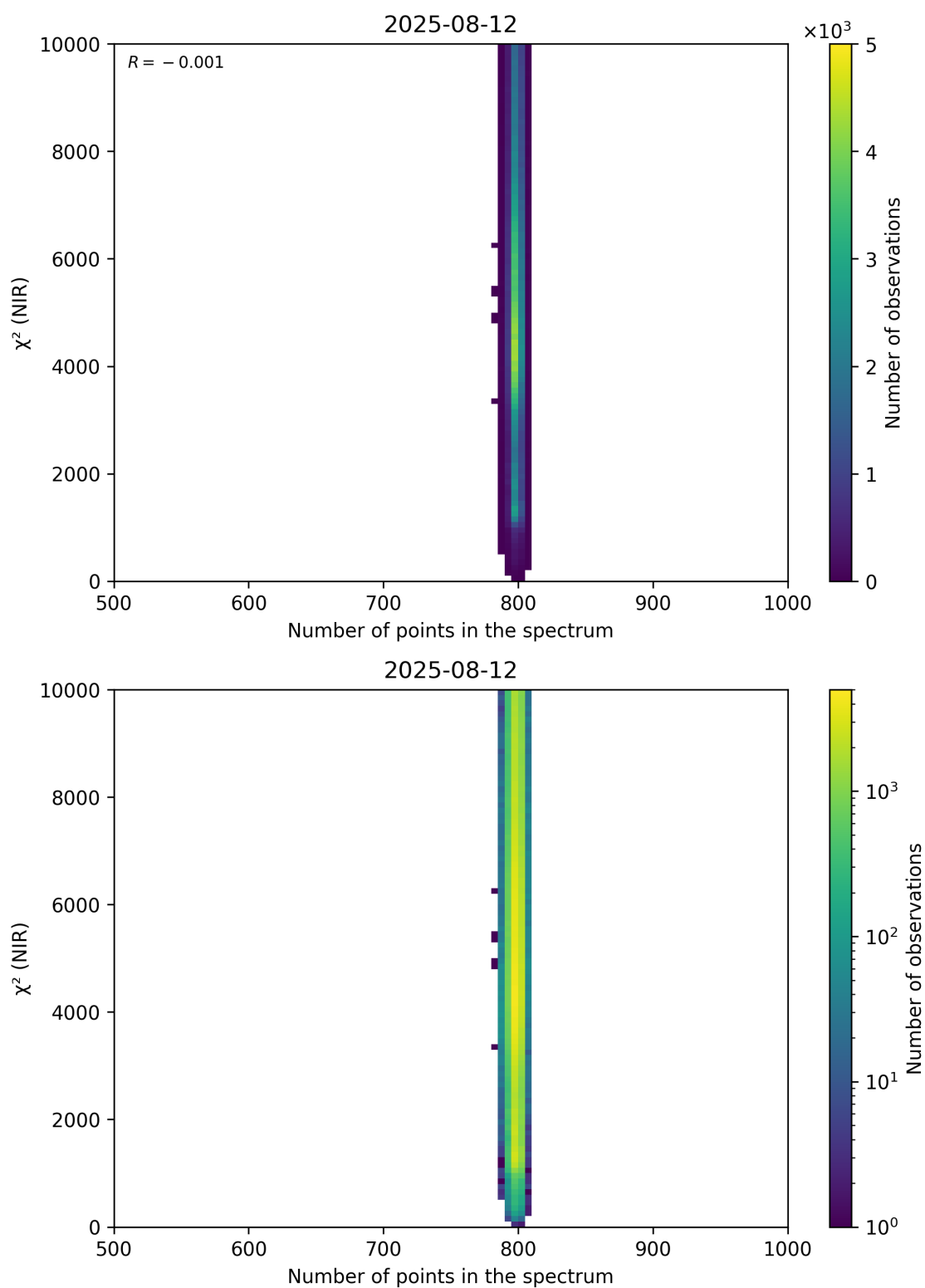
Figure 88: Scatter density plot of “Number of points in the spectrum” against “ \chi^2 (NIR)” for 2025-08-11 to 2025-08-13.
