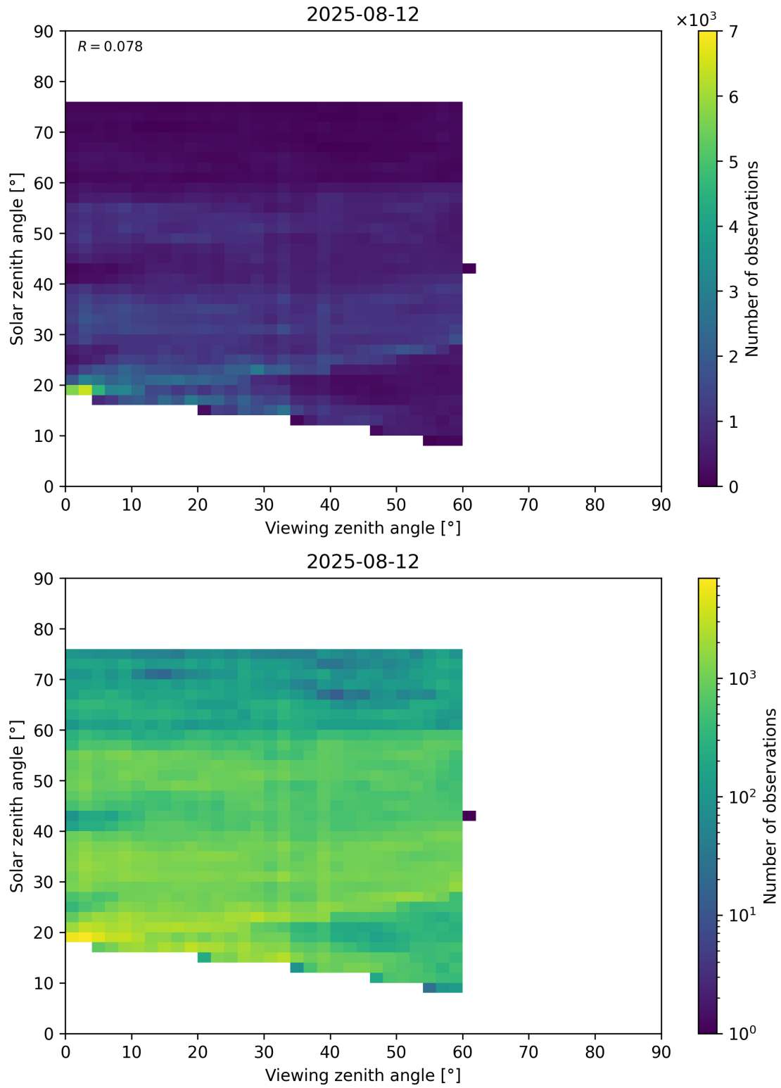
Figure 115: Scatter density plot of “Viewing zenith angle” against “Solar zenith angle” for 2025-08-11 to 2025-08-13.
