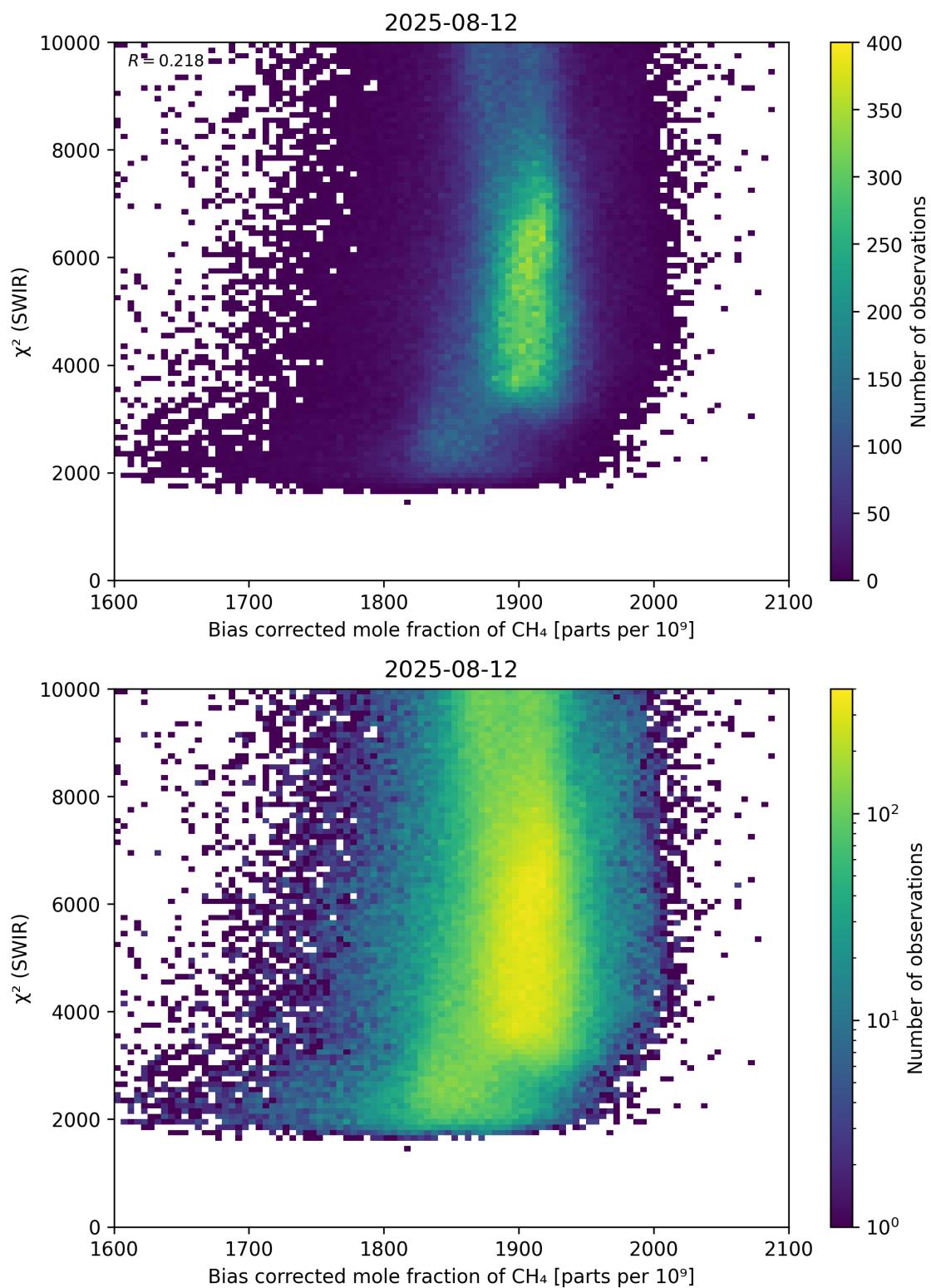
Figure 64: Scatter density plot of “Bias corrected mole fraction of \text{CH}_4 ” against “ \chi^2 (SWIR)” for 2025-08-11 to 2025-08-13.
