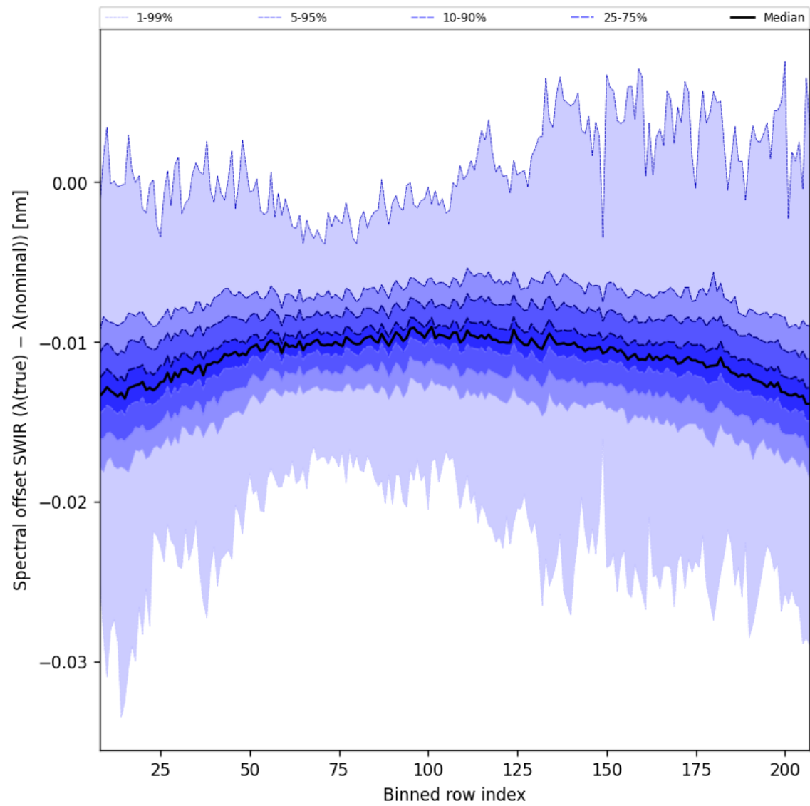
Figure 38: Along track statistics of “Spectral offset SWIR ( \lambda_{\text{true}} - \lambda_{\text{nominal}} )” for 2025-08-11 to 2025-08-13
