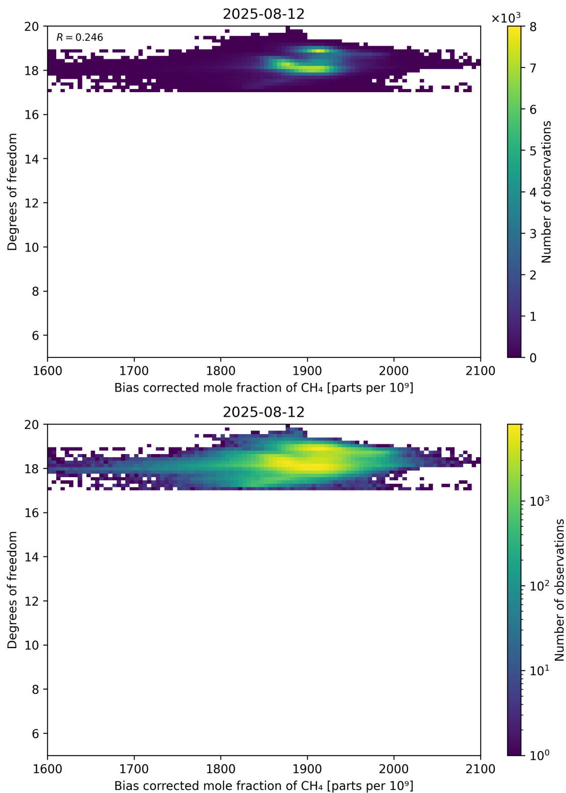
Figure 65: Scatter density plot of “Bias corrected mole fraction of CH 4 ” against “Degrees of freedom” for 2025-08-11 to 2025-08-13.
