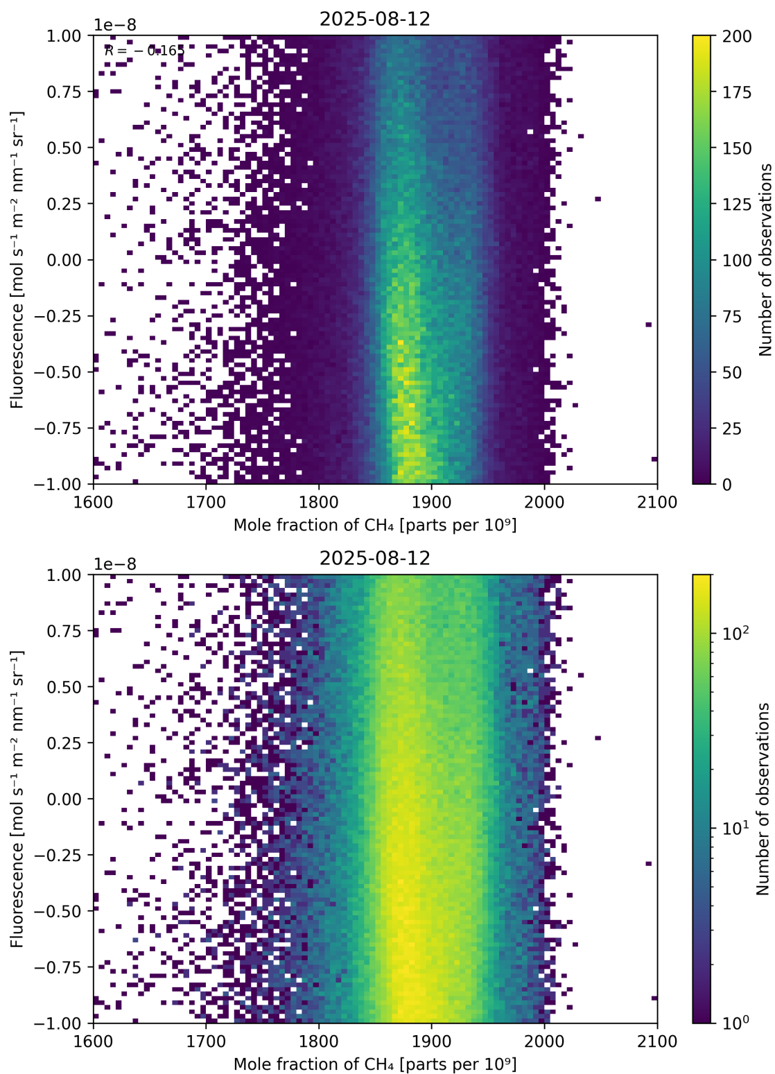
Figure 73: Scatter density plot of “Mole fraction of \text{CH}_4 ” against “Fluorescence” for 2025-08-11 to 2025-08-13.
