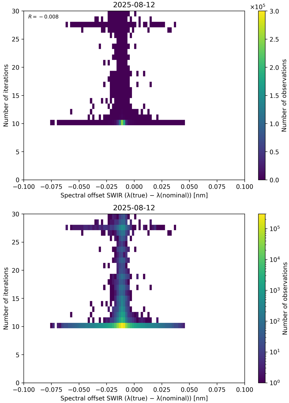
Figure 121: Scatter density plot of “Spectral offset SWIR ( \lambda_{\text{true}} - \lambda_{\text{nominal}} )” against “Number of iterations” for 2025-08-11 to 2025-08-13.
