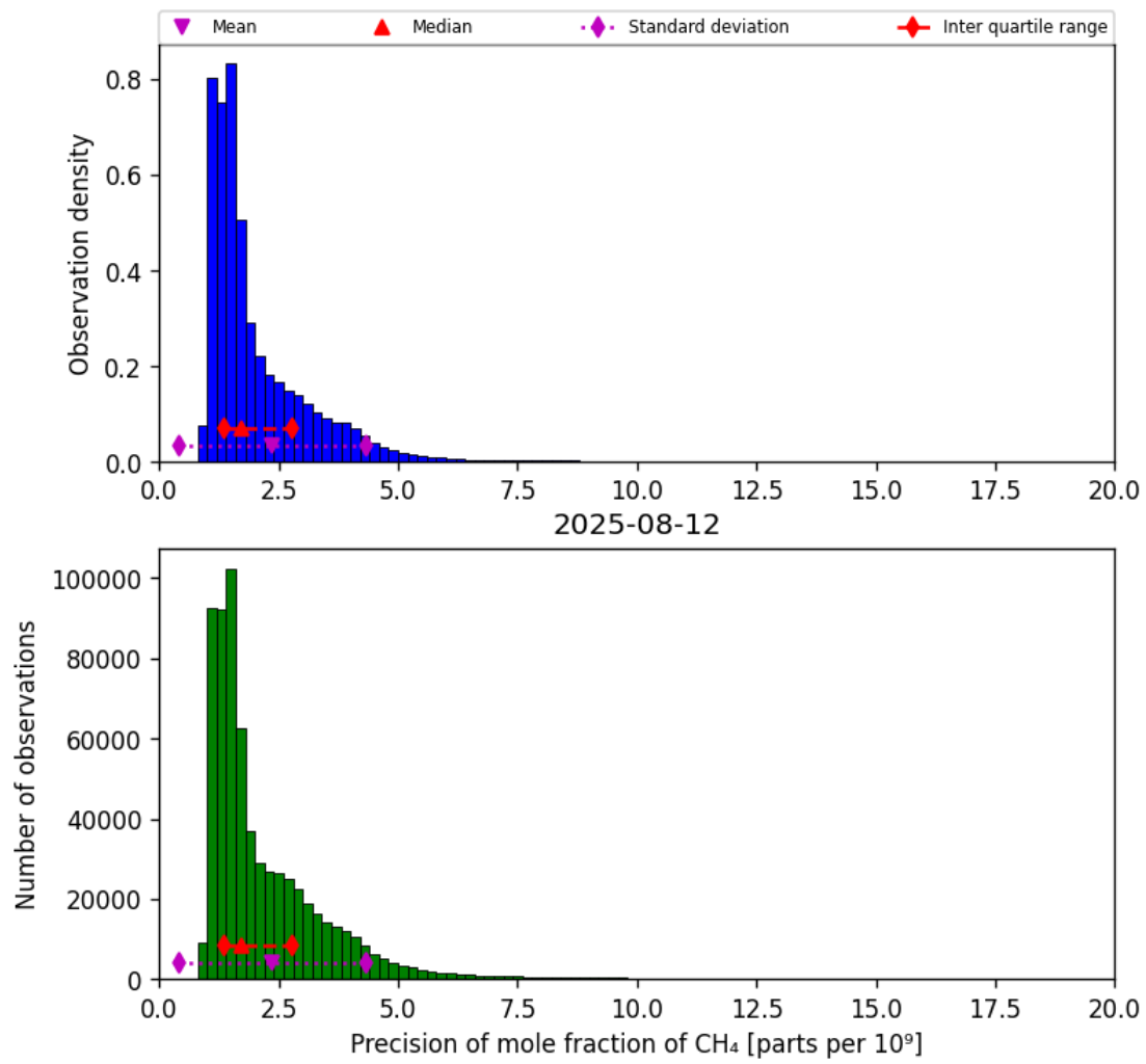
Figure 24: Histogram of “Precision of mole fraction of CH 4 ” for 2025-08-11 to 2025-08-13
