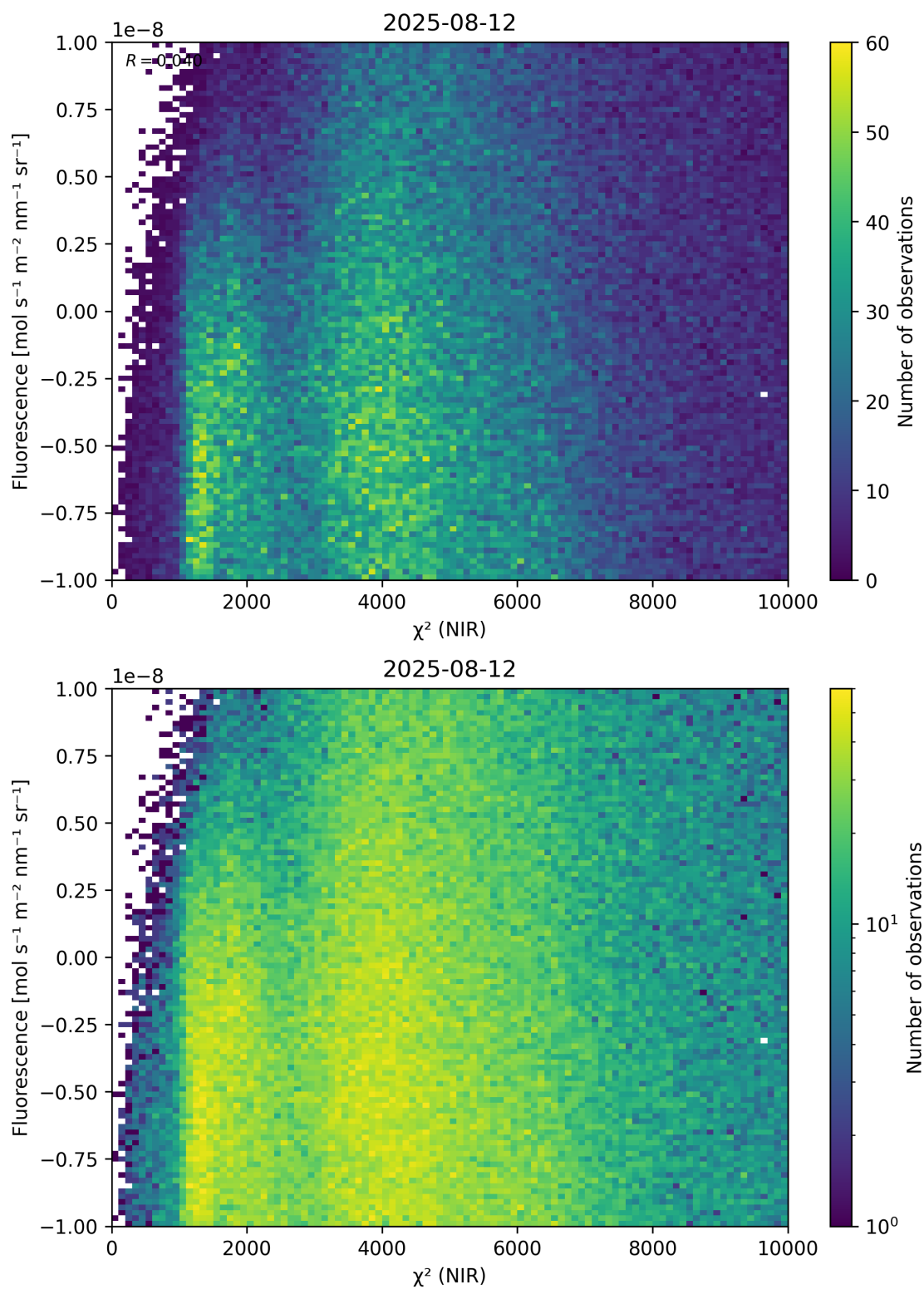
Figure 45: Scatter density plot of “ \chi^2 (NIR)” against “Fluorescence” for 2025-08-11 to 2025-08-13.
