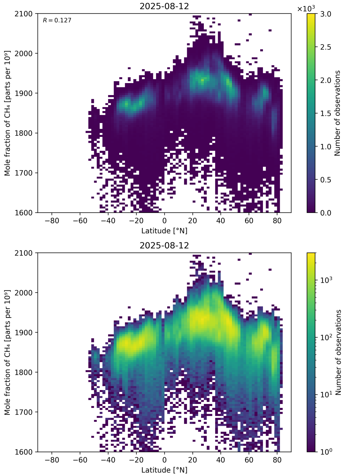
Figure 57: Scatter density plot of “Latitude” against “Mole fraction of CH 4 ” for 2025-08-11 to 2025-08-13.
