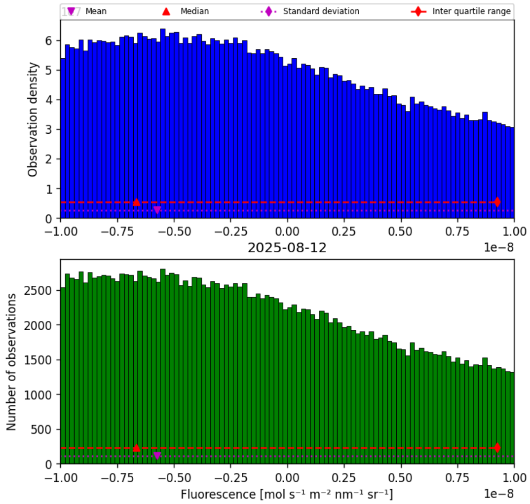
Figure 32: Histogram of “Fluorescence” for 2025-08-11 to 2025-08-13
