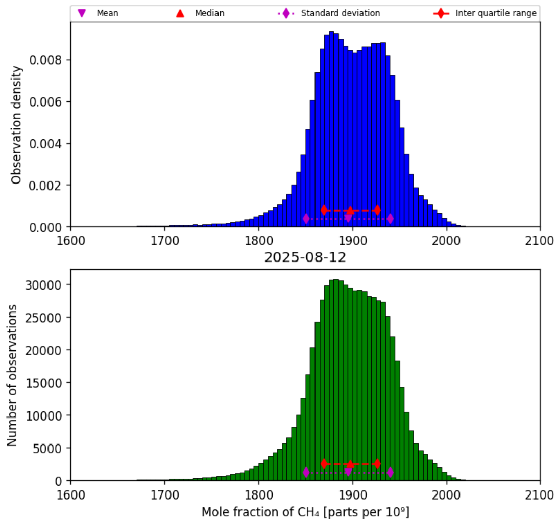
Figure 23: Histogram of “Mole fraction of CH 4 ” for 2025-08-11 to 2025-08-13
