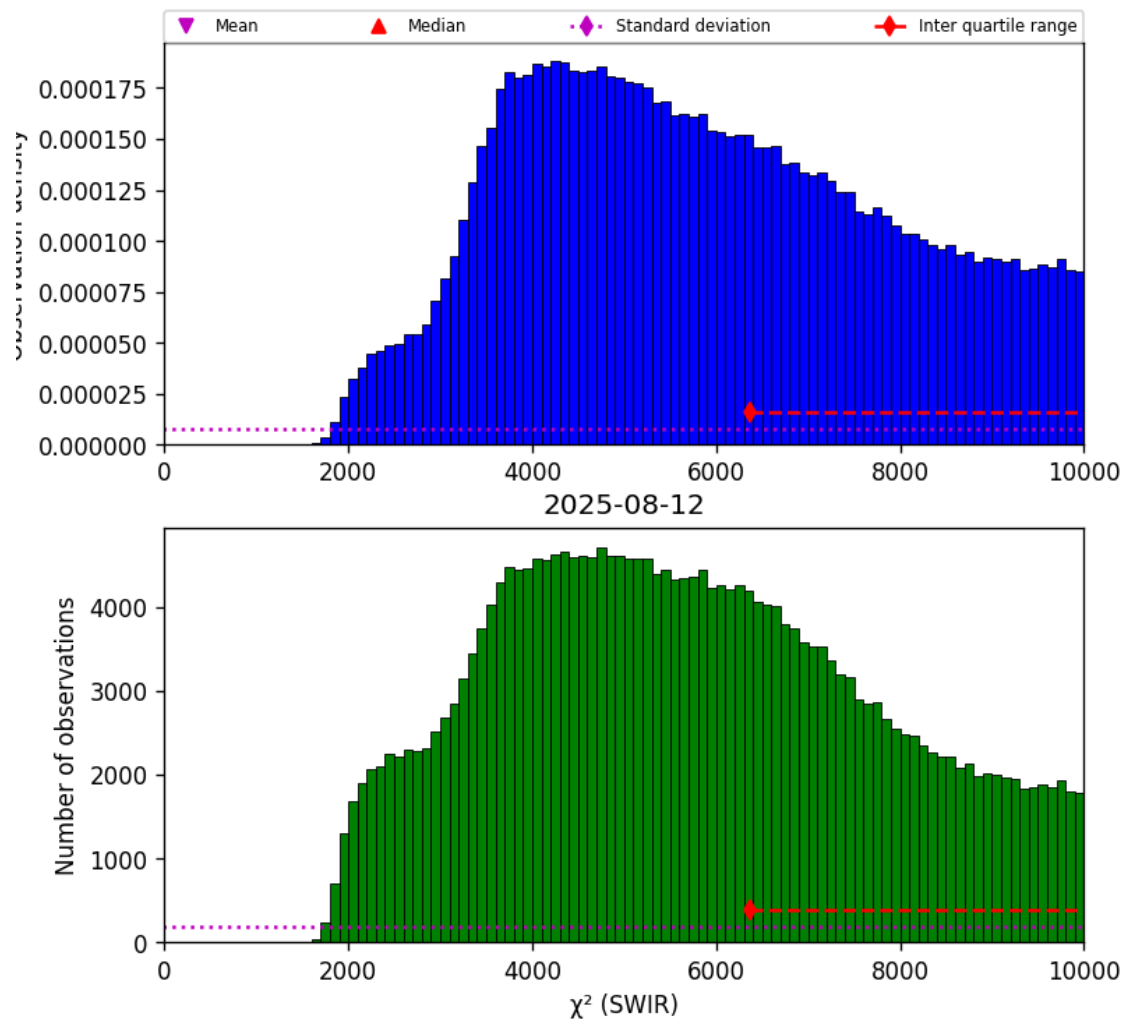
Figure 28: Histogram of “ \chi^2 (SWIR)” for 2025-08-11 to 2025-08-13
