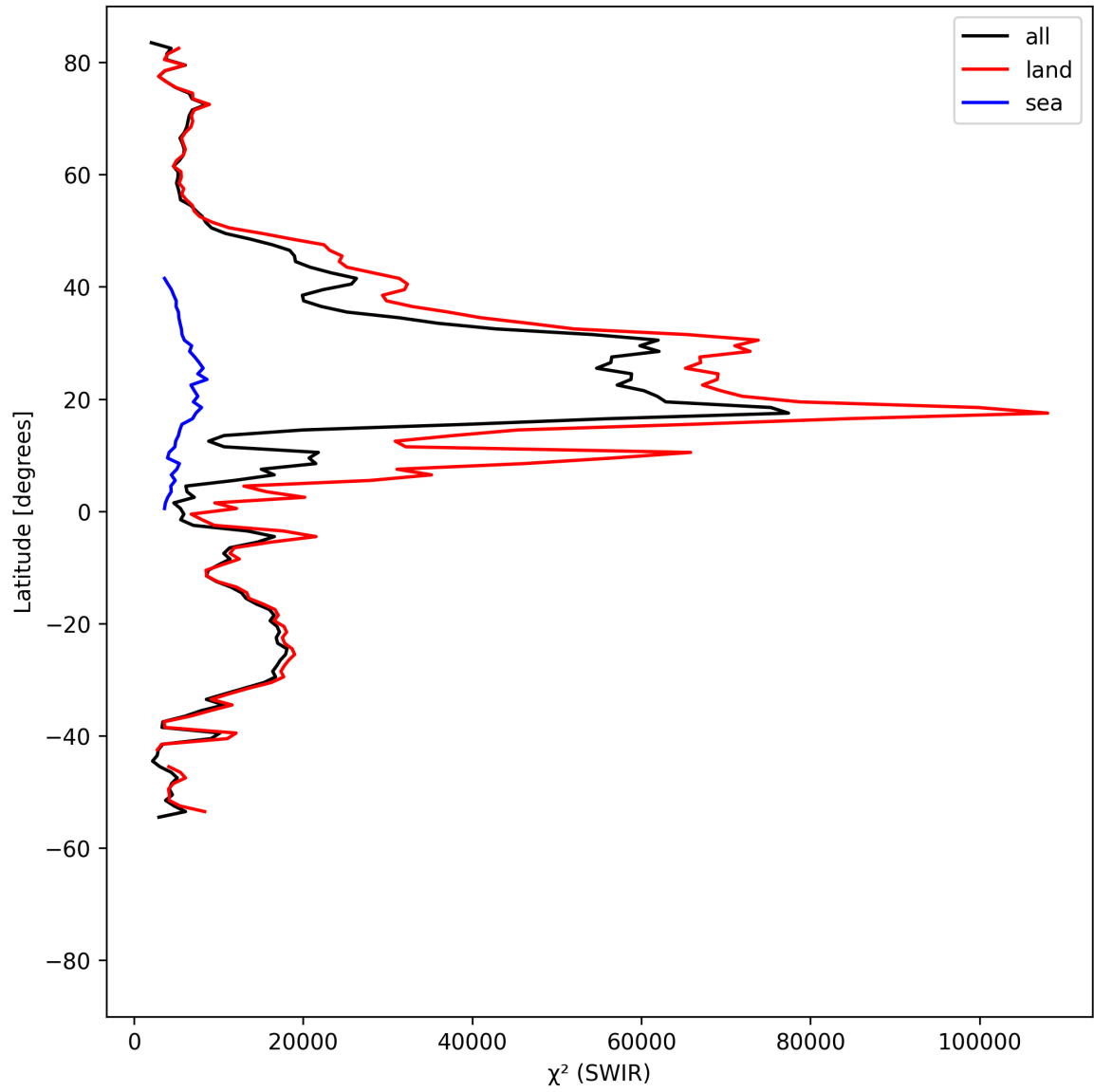
Figure 17: Zonal average of “ \chi^2 (SWIR)” for 2025-08-11 to 2025-08-13.
