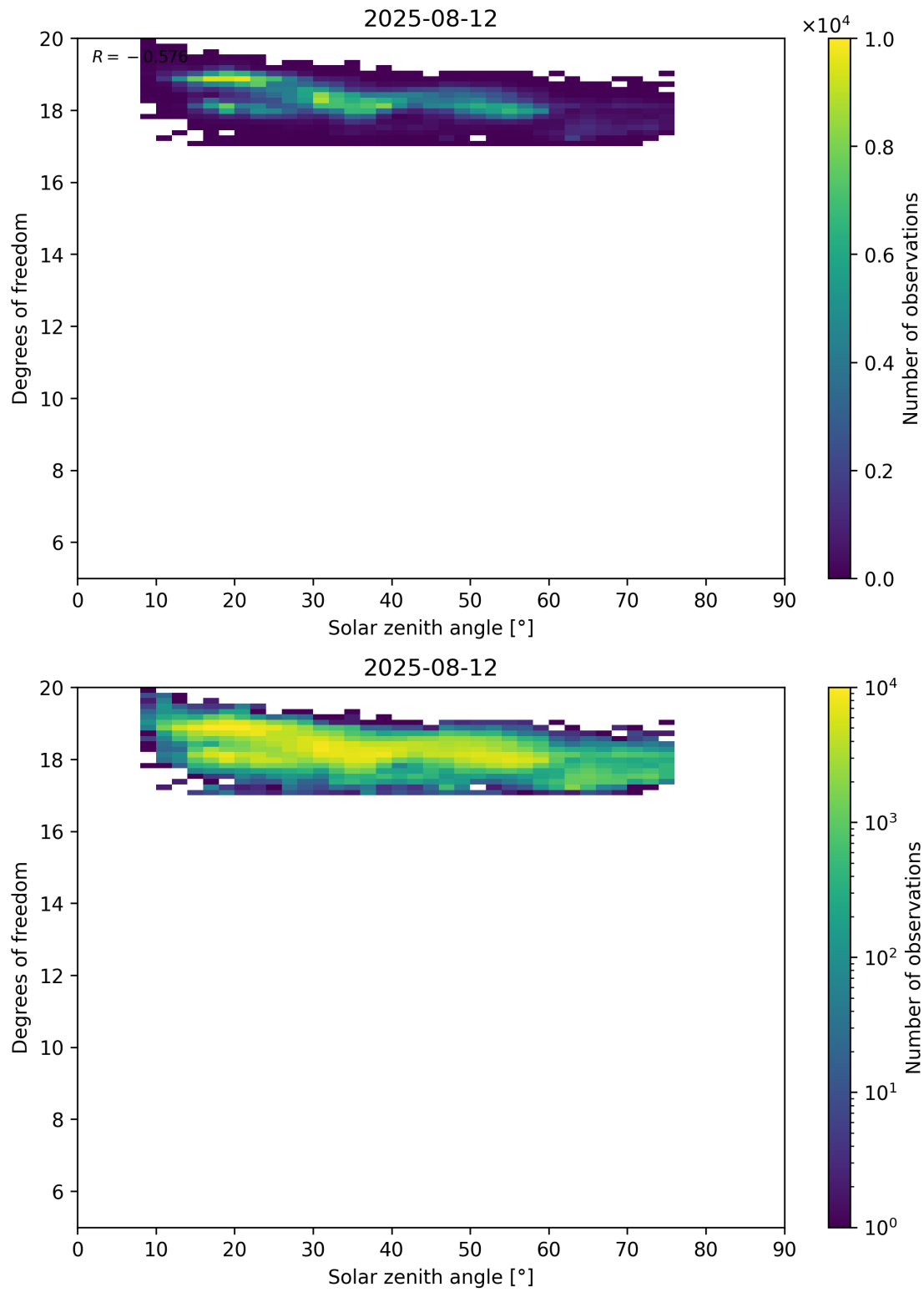
Figure 96: Scatter density plot of “Solar zenith angle” against “Degrees of freedom” for 2025-08-11 to 2025-08-13.
