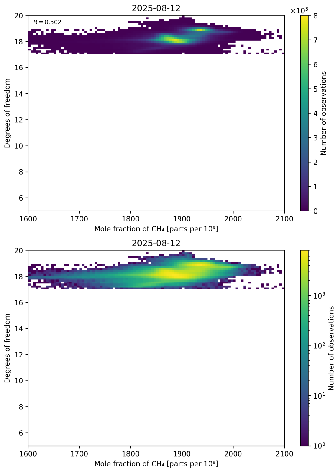
Figure 72: Scatter density plot of “Mole fraction of CH 4 ” against “Degrees of freedom” for 2025-08-11 to 2025-08-13.
