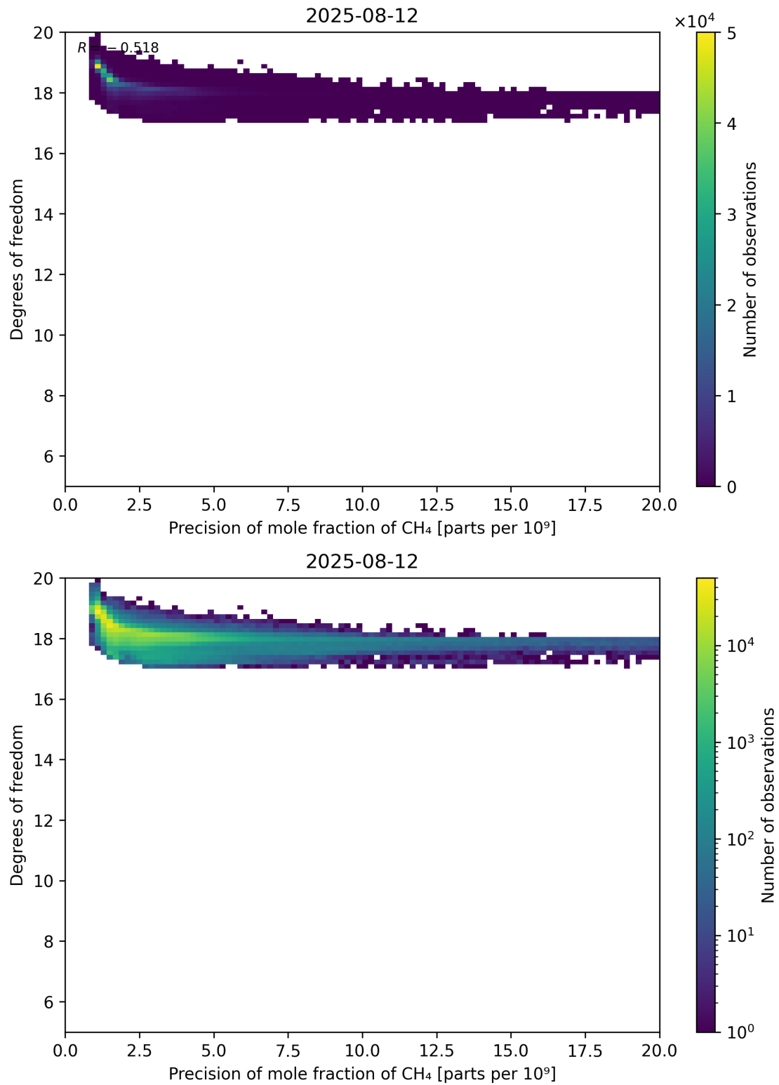
Figure 80: Scatter density plot of “Precision of mole fraction of CH 4 ” against “Degrees of freedom” for 2025-08-11 to 2025-08-13.
