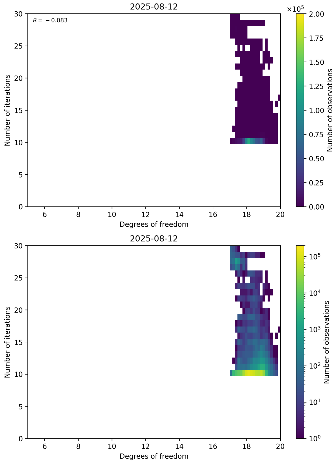
Figure 52: Scatter density plot of “Degrees of freedom” against “Number of iterations” for 2025-08-11 to 2025-08-13.
