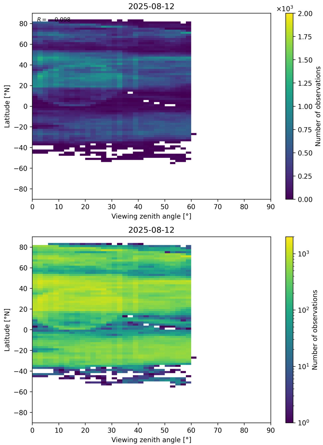
Figure 109: Scatter density plot of “Viewing zenith angle” against “Latitude” for 2025-08-11 to 2025-08-13.
