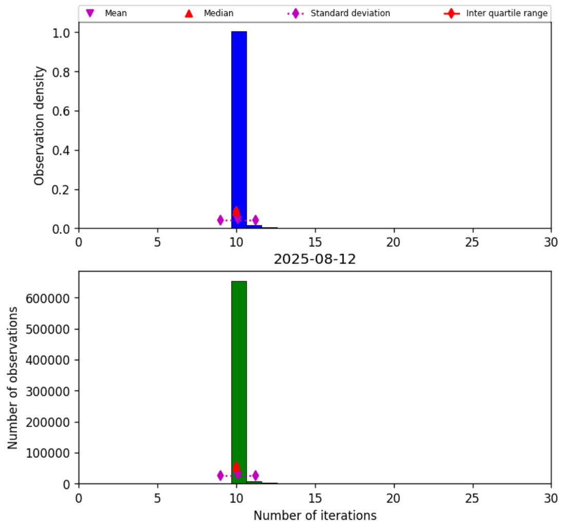
Figure 31: Histogram of “Number of iterations” for 2025-08-11 to 2025-08-13
