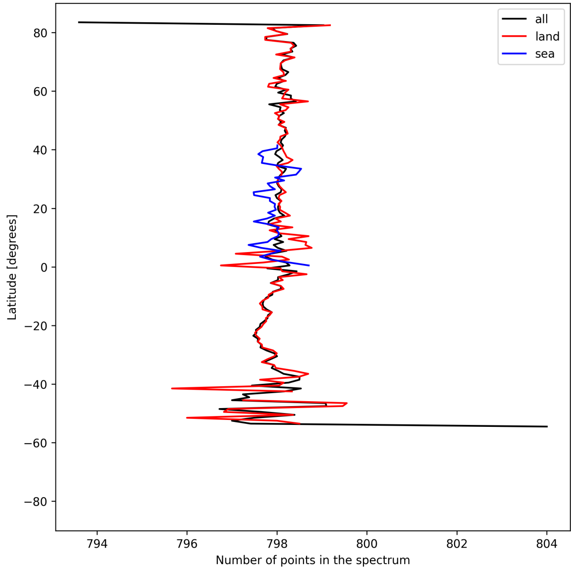
Figure 15: Zonal average of “Number of points in the spectrum” for 2025-08-11 to 2025-08-13.
