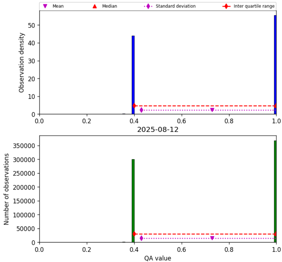
Figure 22: Histogram of “QA value” for 2025-08-11 to 2025-08-13
