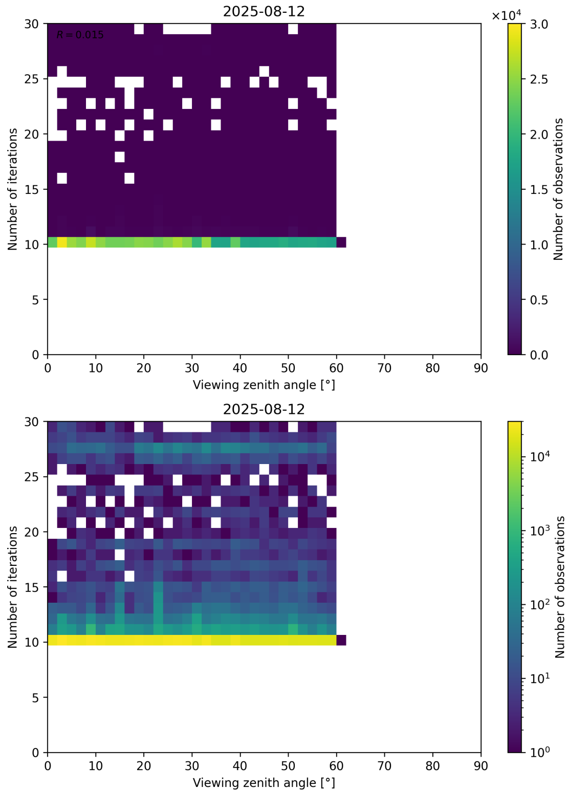
Figure 113: Scatter density plot of “Viewing zenith angle” against “Number of iterations” for 2025-08-11 to 2025-08-13.
