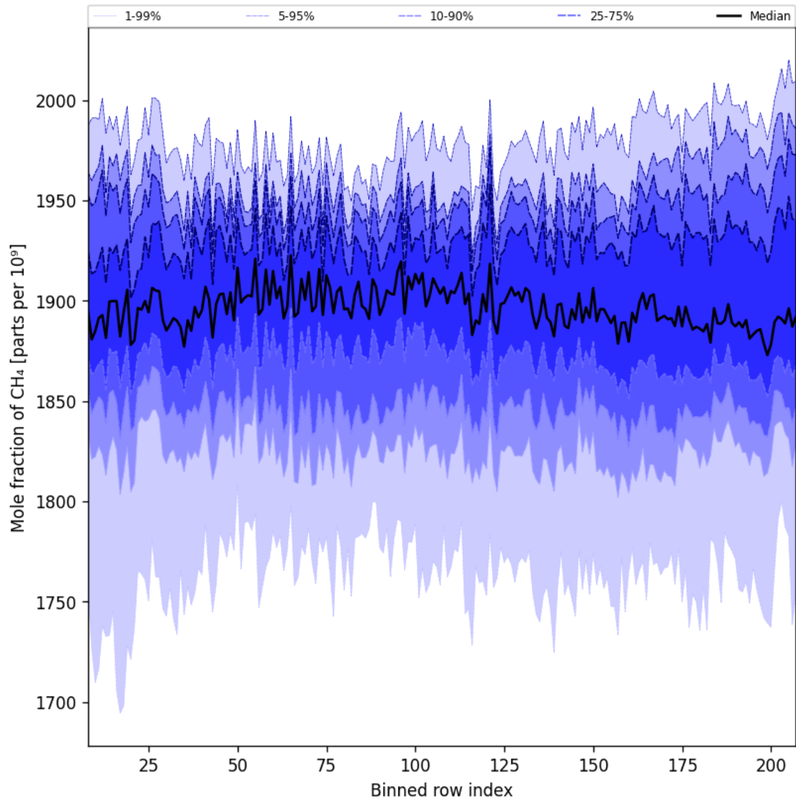
Figure 34: Along track statistics of “Mole fraction of CH 4 ” for 2025-08-11 to 2025-08-13
