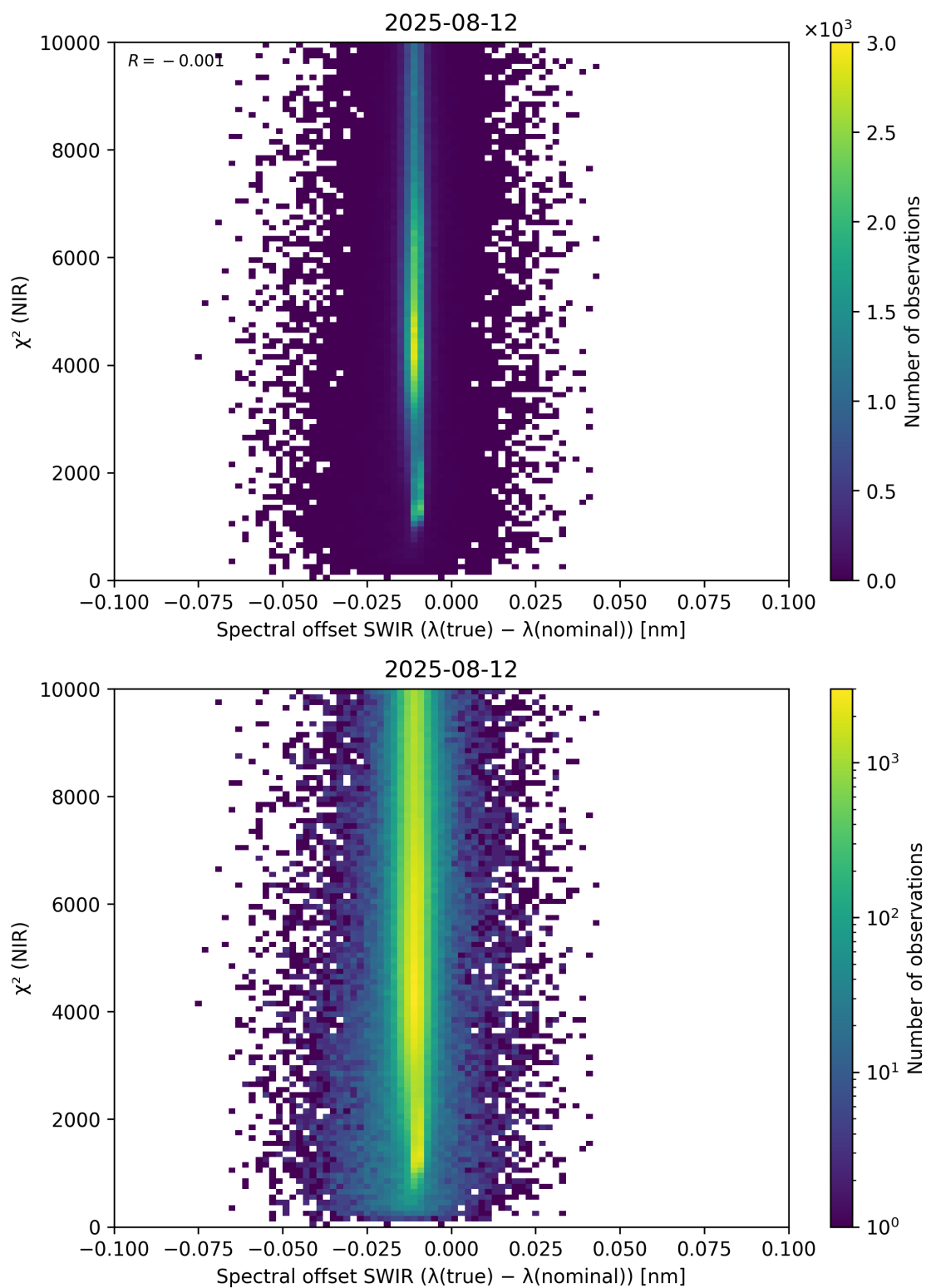
Figure 117: Scatter density plot of “Spectral offset SWIR ( \lambda_{\text{true}} - \lambda_{\text{nominal}} )” against “ \chi^2 (NIR)” for 2025-08-11 to 2025-08-13.
