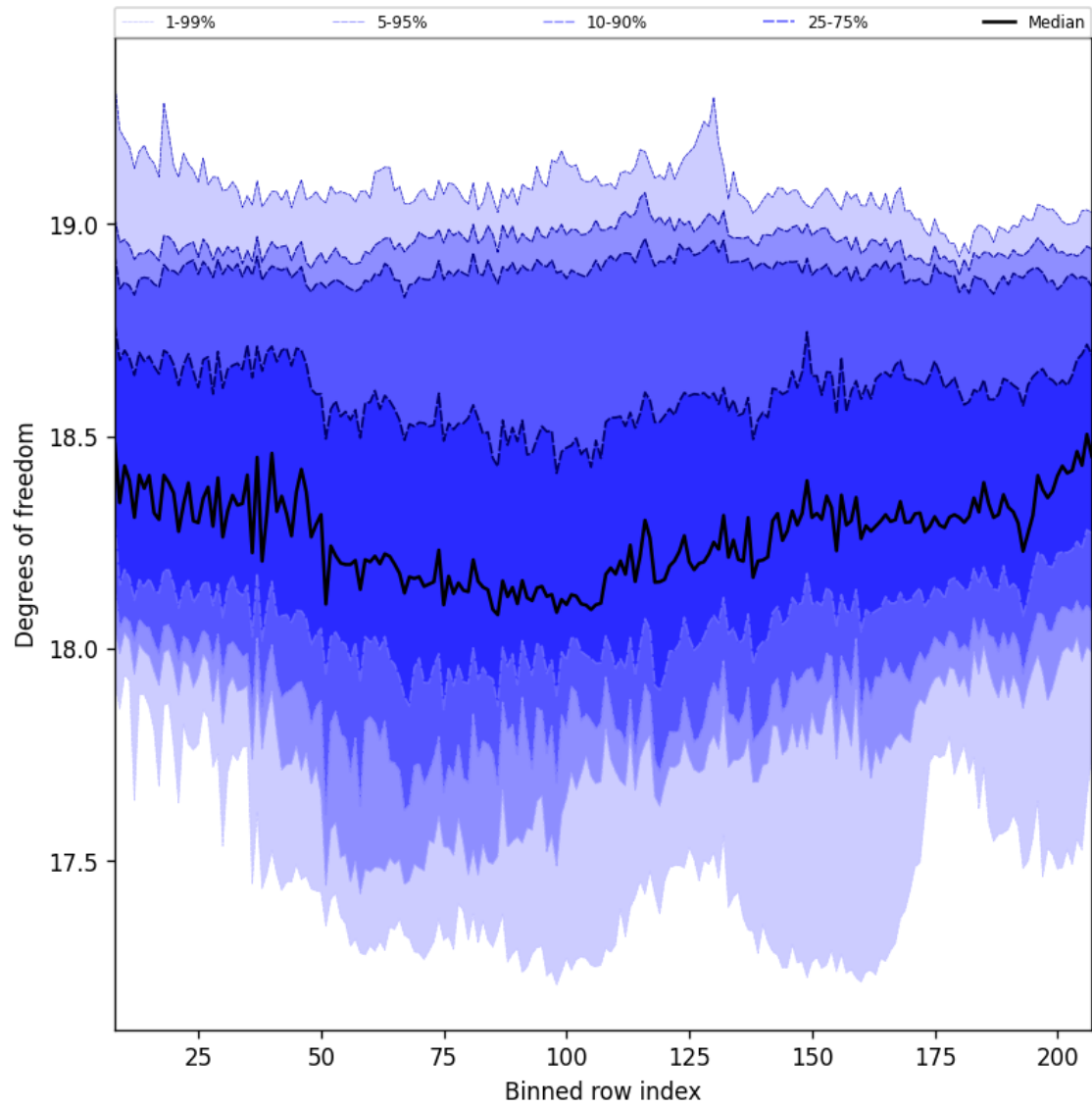
Figure 41: Along track statistics of “Degrees of freedom” for 2025-08-11 to 2025-08-13
