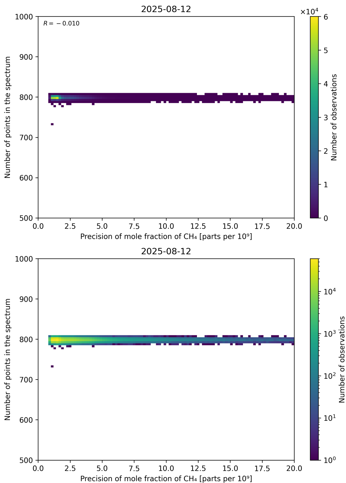
Figure 84: Scatter density plot of “Precision of mole fraction of CH 4 ” against “Number of points in the spectrum” for 2025-08-11 to 2025-08-13.
