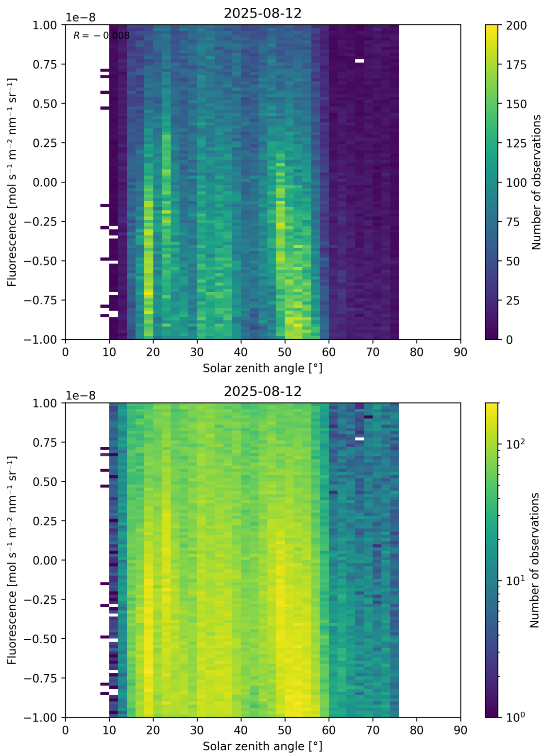
Figure 97: Scatter density plot of “Solar zenith angle” against “Fluorescence” for 2025-08-11 to 2025-08-13.
