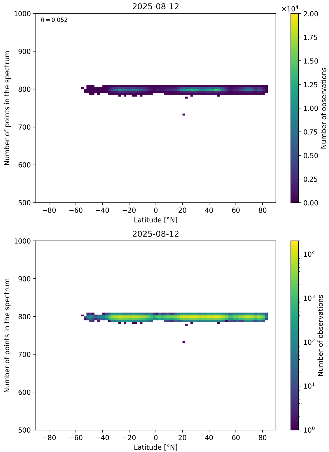
Figure 61: Scatter density plot of “Latitude” against “Number of points in the spectrum” for 2025-08-11 to 2025-08-13.
