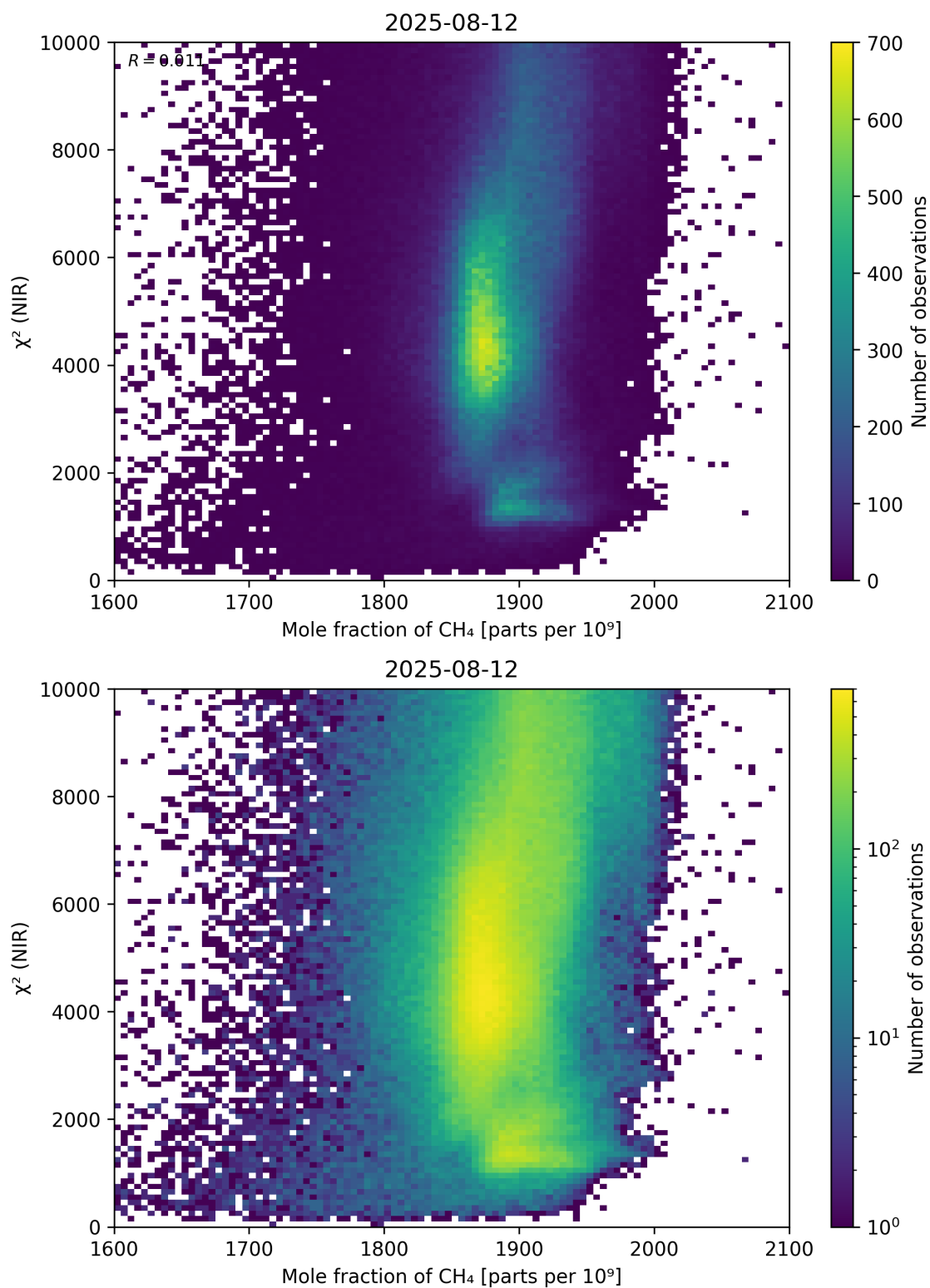
Figure 70: Scatter density plot of “Mole fraction of \text{CH}_4 ” against “ \chi^2 (NIR)” for 2025-08-11 to 2025-08-13.
