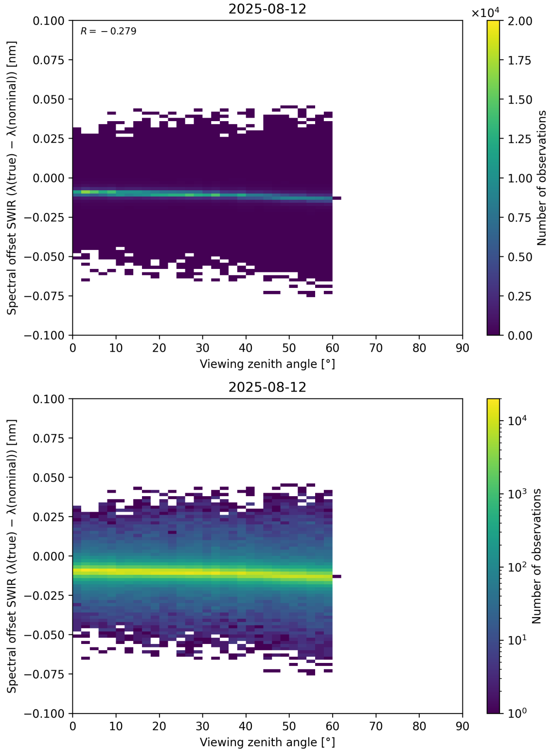
Figure 116: Scatter density plot of “Viewing zenith angle” against “Spectral offset SWIR ( \lambda_{\text{true}} - \lambda_{\text{nominal}} )” for 2025-08-11 to 2025-08-13.
