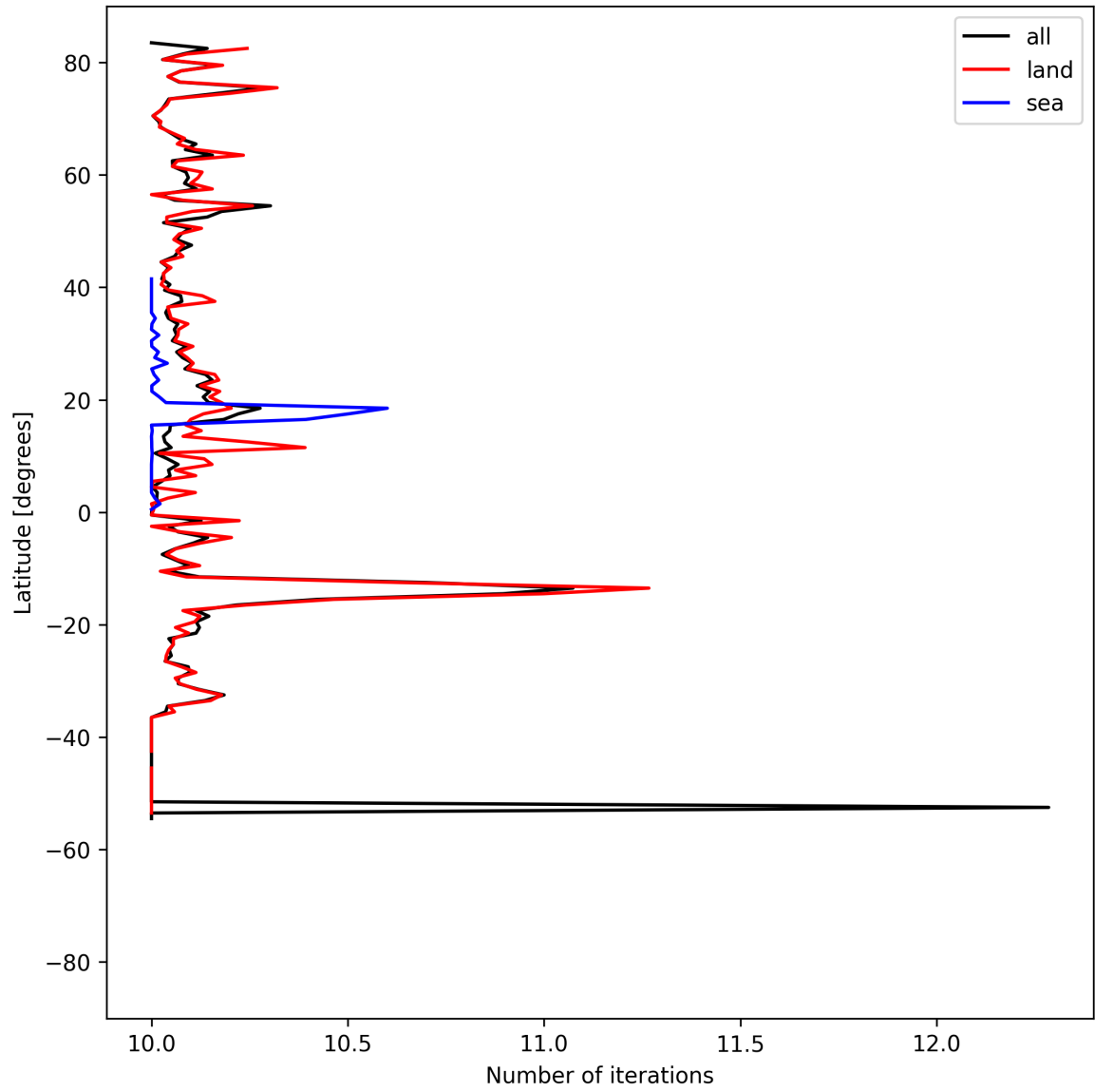
Figure 20: Zonal average of “Number of iterations” for 2025-08-11 to 2025-08-13.
