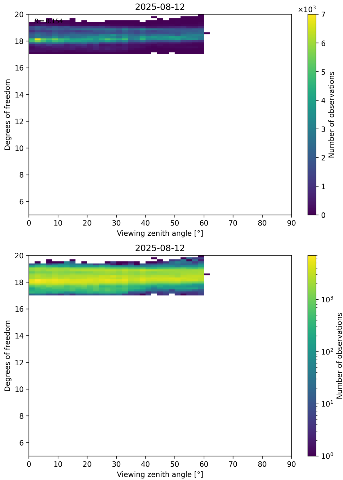
Figure 107: Scatter density plot of “Viewing zenith angle” against “Degrees of freedom” for 2025-08-11 to 2025-08-13.
