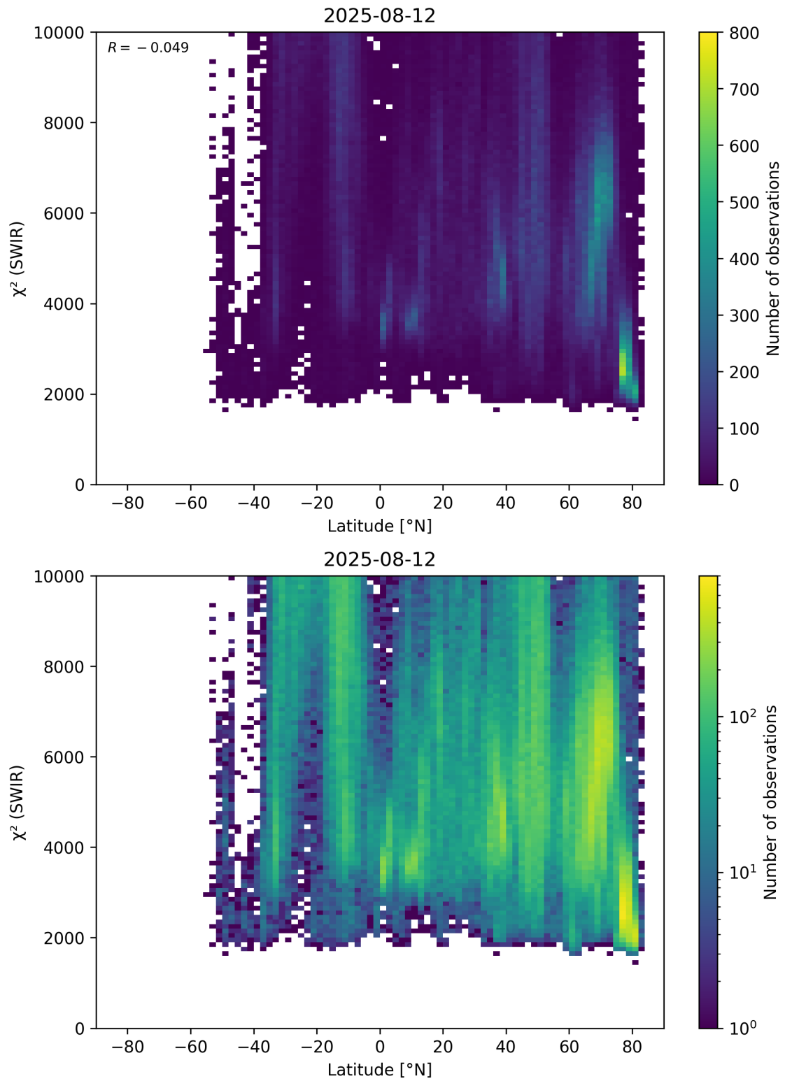
Figure 54: Scatter density plot of “Latitude” against “ \chi^2 (SWIR)” for 2025-08-11 to 2025-08-13.
