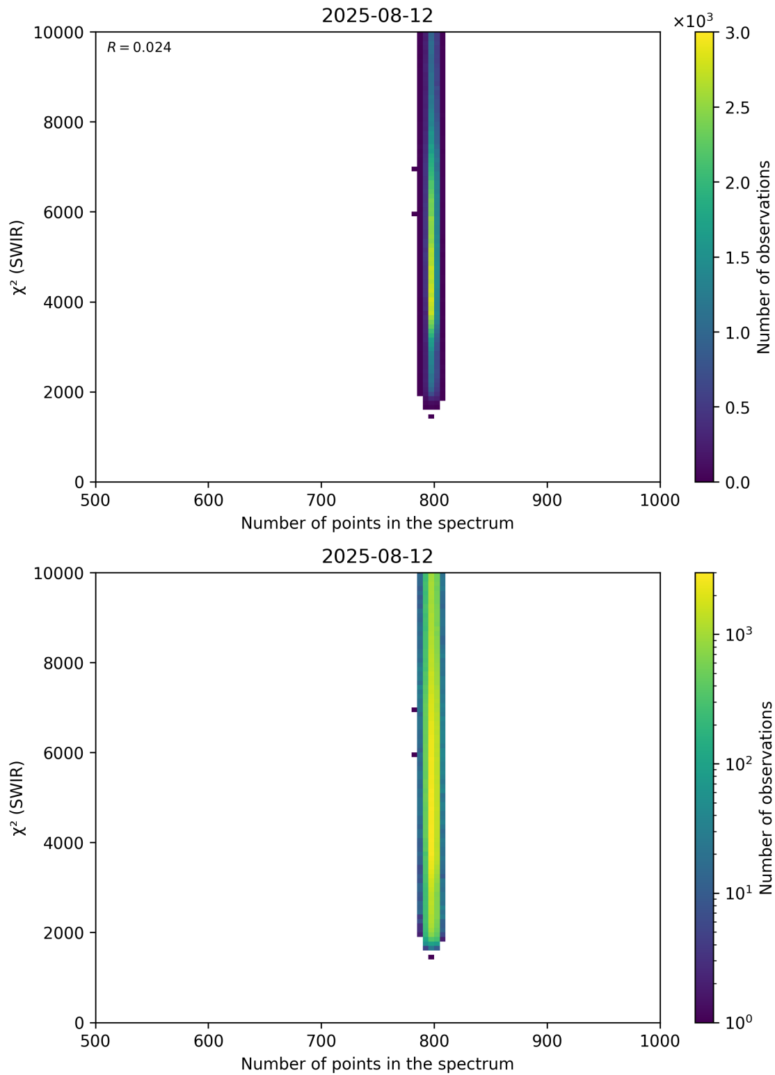
Figure 89: Scatter density plot of “Number of points in the spectrum” against “ \chi^2 (SWIR)” for 2025-08-11 to 2025-08-13.
