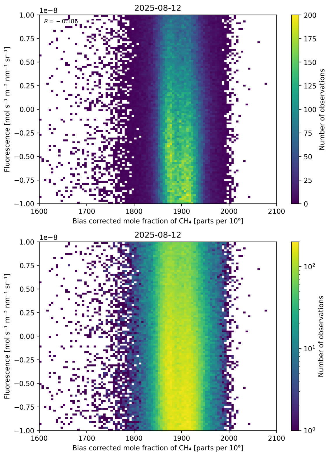
Figure 66: Scatter density plot of “Bias corrected mole fraction of \text{CH}_4 ” against “Fluorescence” for 2025-08-11 to 2025-08-13.
