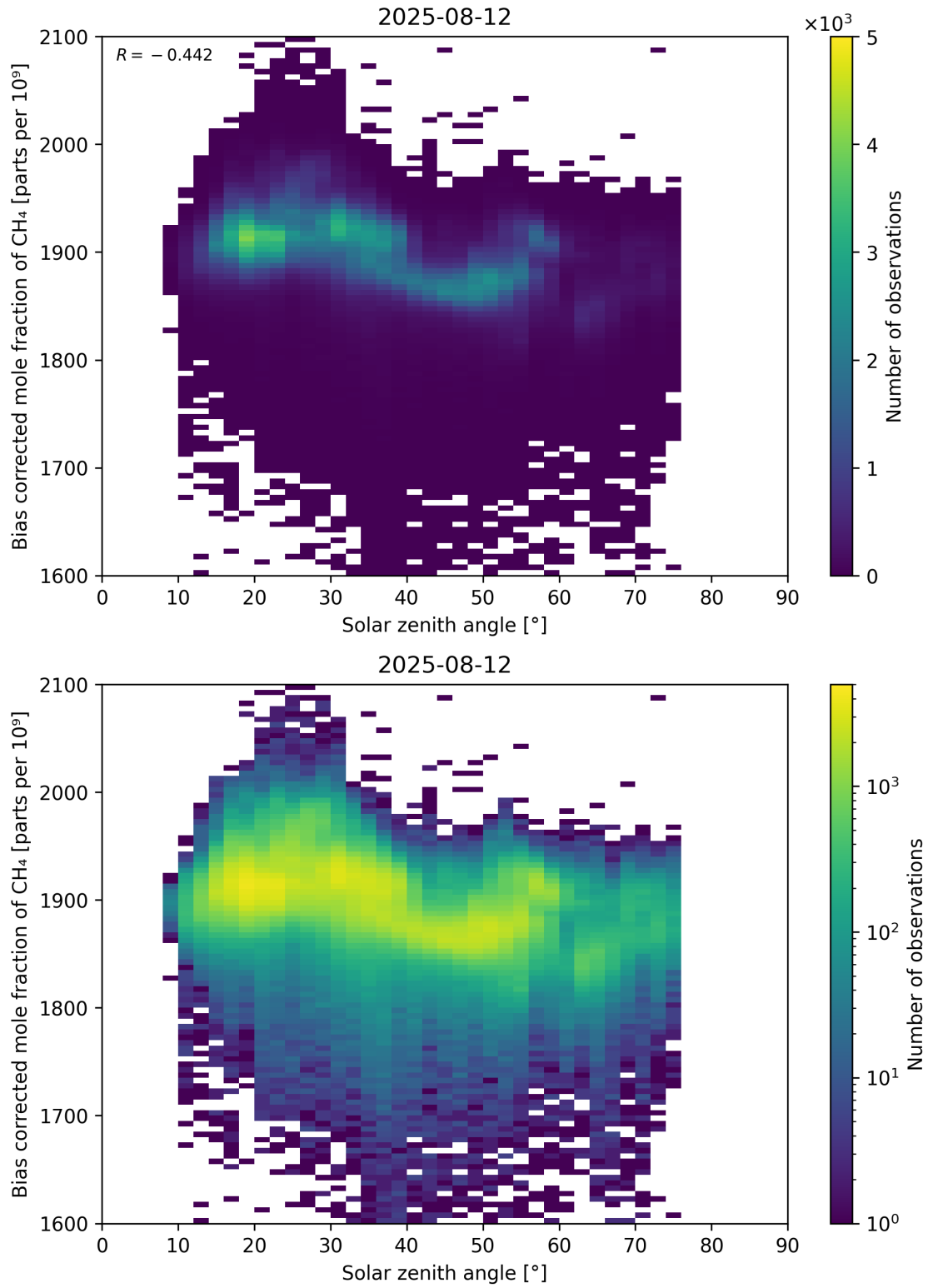
Figure 100: Scatter density plot of “Solar zenith angle” against “Bias corrected mole fraction of CH 4 ” for 2025-08-11 to 2025-08-13.
