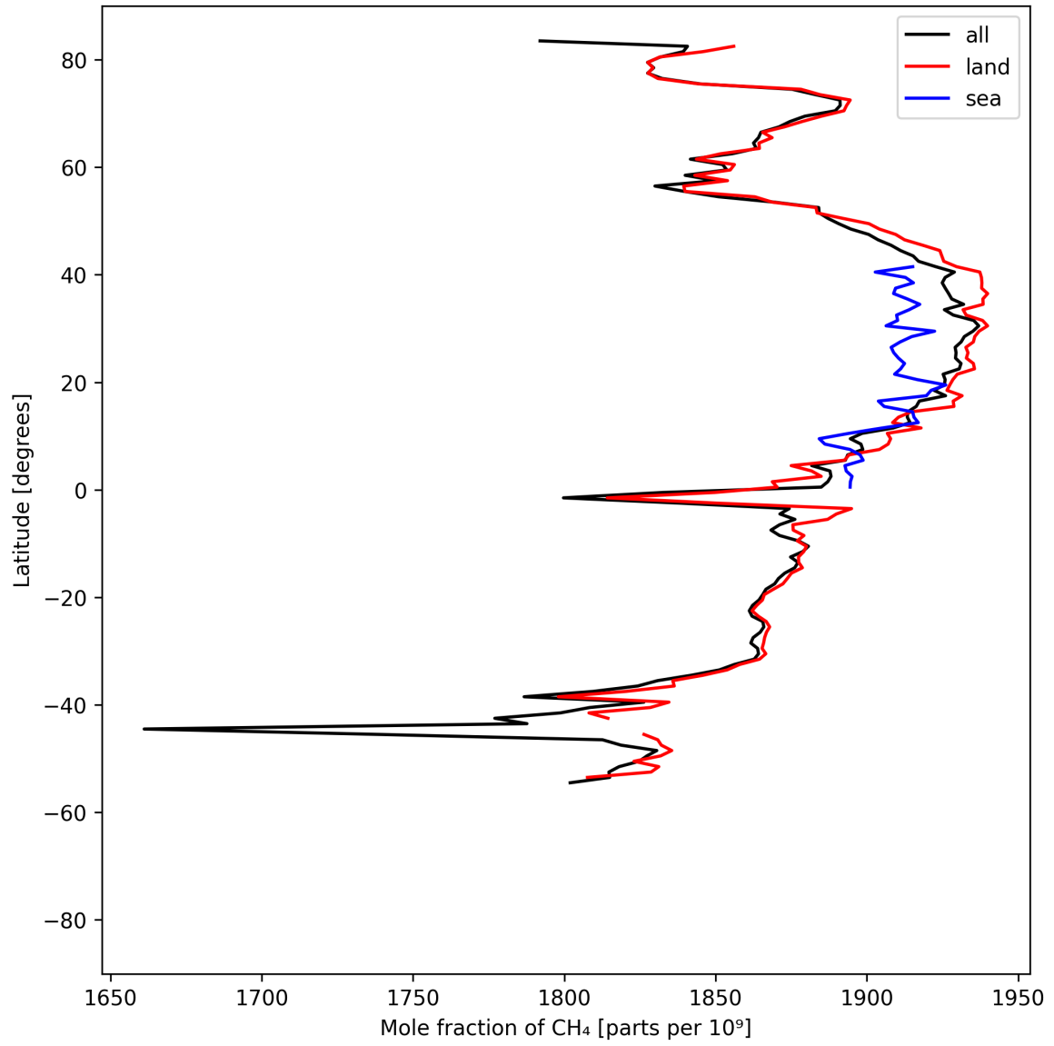
Figure 12: Zonal average of “Mole fraction of \text{CH}_4 ” for 2025-08-11 to 2025-08-13.
