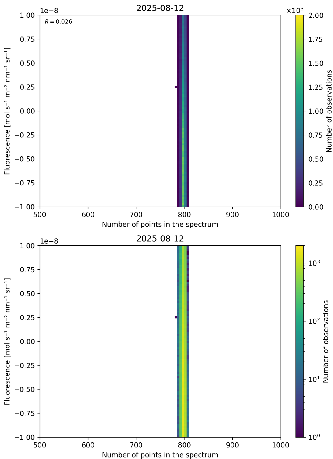
Figure 91: Scatter density plot of “Number of points in the spectrum” against “Fluorescence” for 2025-08-11 to 2025-08-13.
