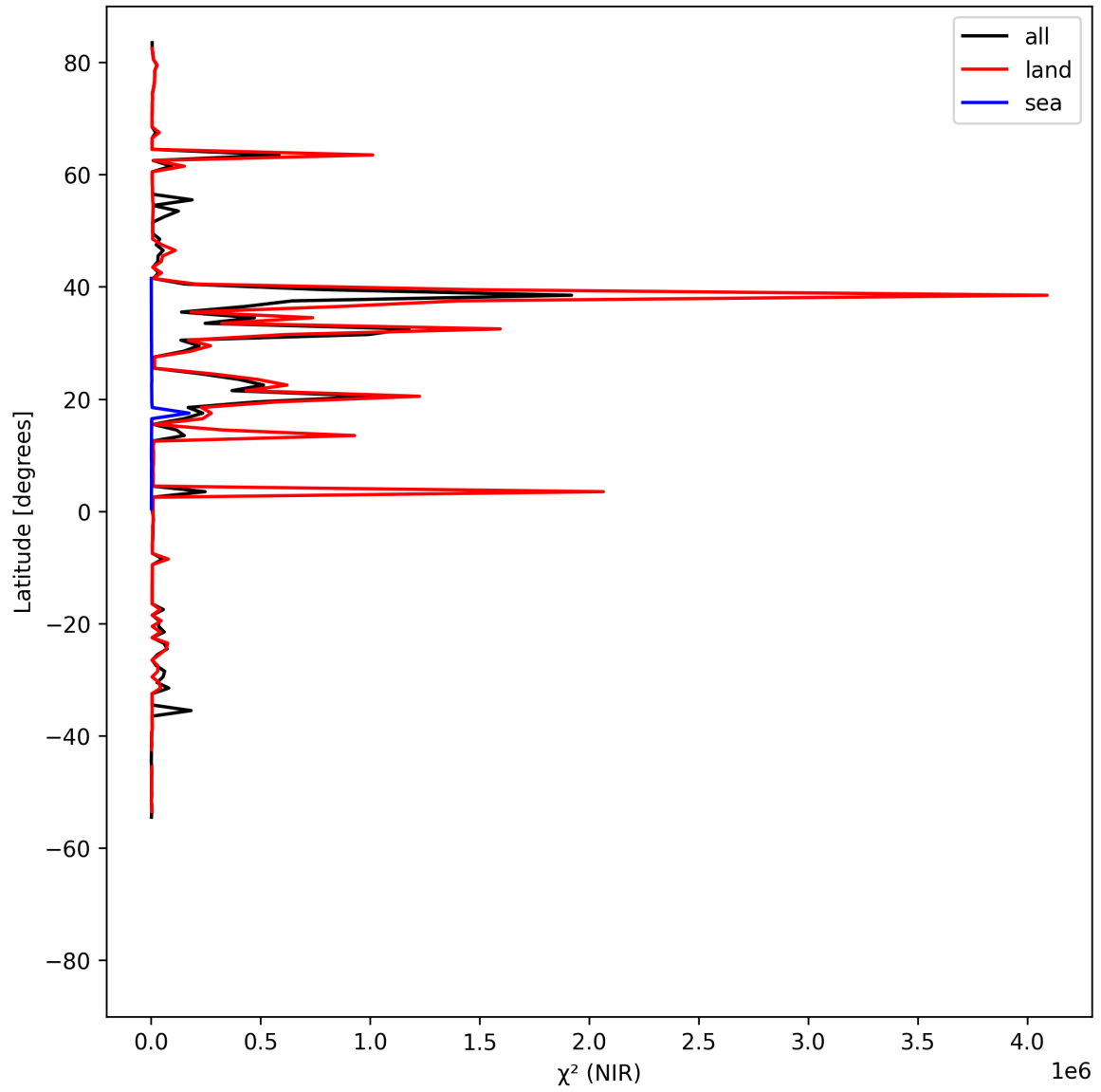
Figure 18: Zonal average of “ \chi^2 (NIR)” for 2025-08-11 to 2025-08-13.
