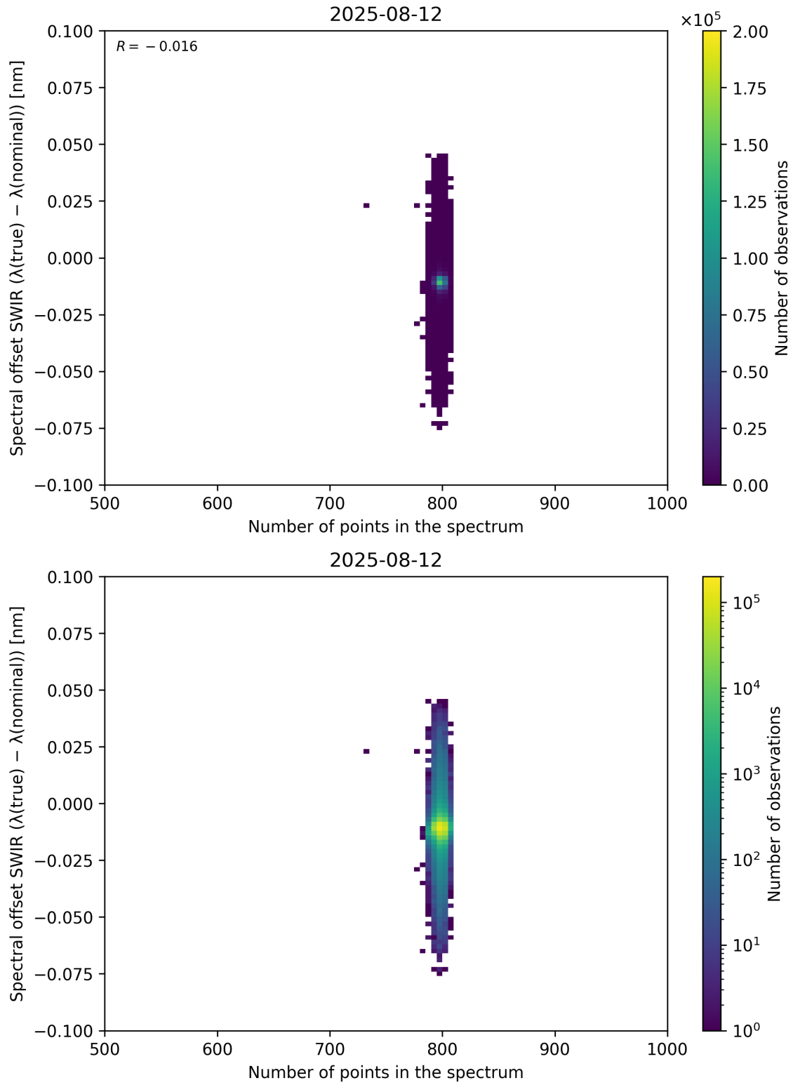
Figure 93: Scatter density plot of “Number of points in the spectrum” against “Spectral offset SWIR ( \lambda_{\text{true}} - \lambda_{\text{nominal}} )” for 2025-08-11 to 2025-08-13.
