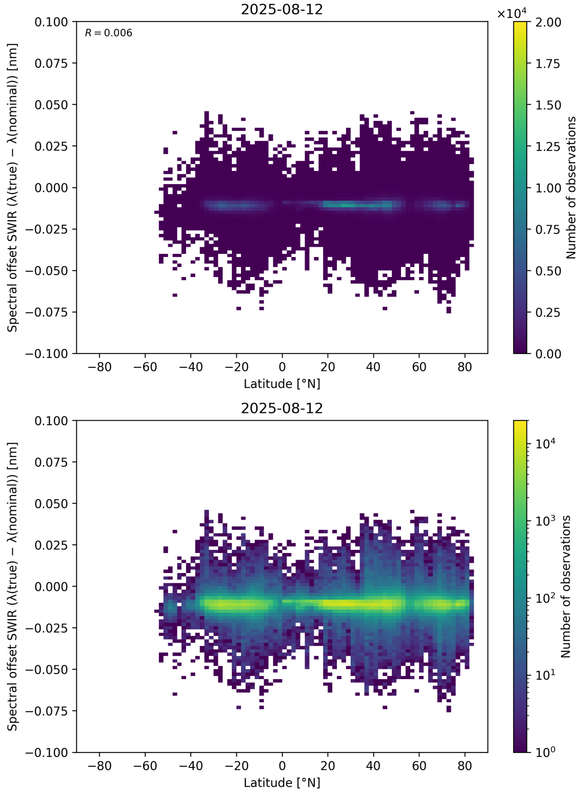
Figure 62: Scatter density plot of “Latitude” against “Spectral offset SWIR ( \lambda_{\text{true}} - \lambda_{\text{nominal}} )” for 2025-08-11 to 2025-08-13.
