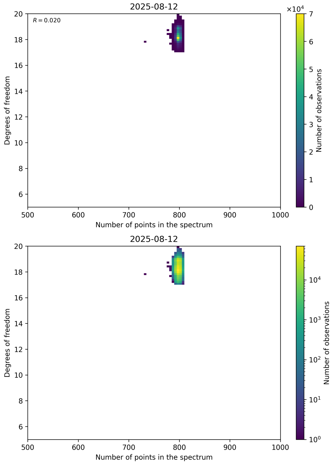
Figure 90: Scatter density plot of “Number of points in the spectrum” against “Degrees of freedom” for 2025-08-11 to 2025-08-13.
