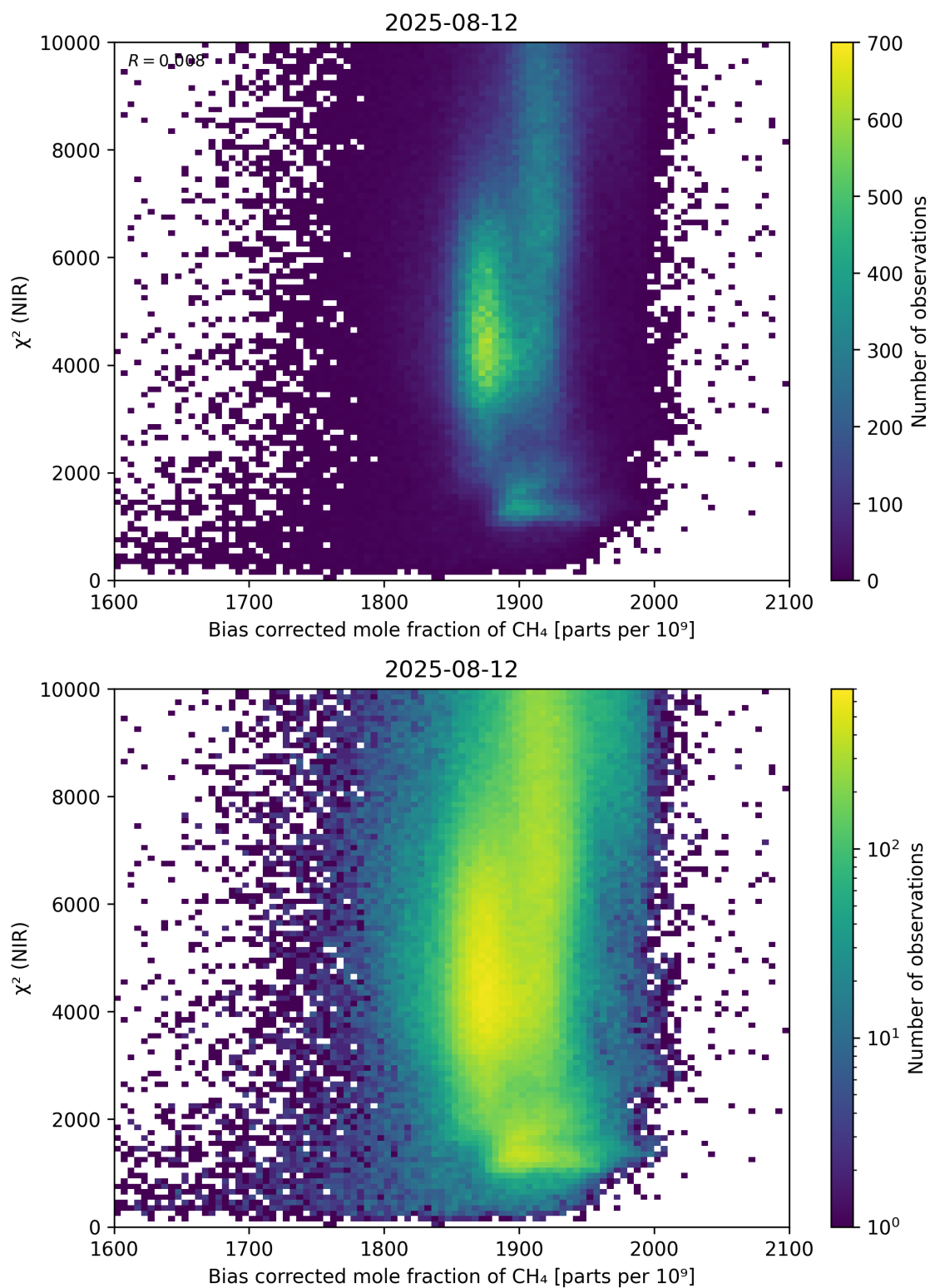
Figure 63: Scatter density plot of “Bias corrected mole fraction of CH 4 ” against “ \chi^2 (NIR)” for 2025-08-11 to 2025-08-13.
