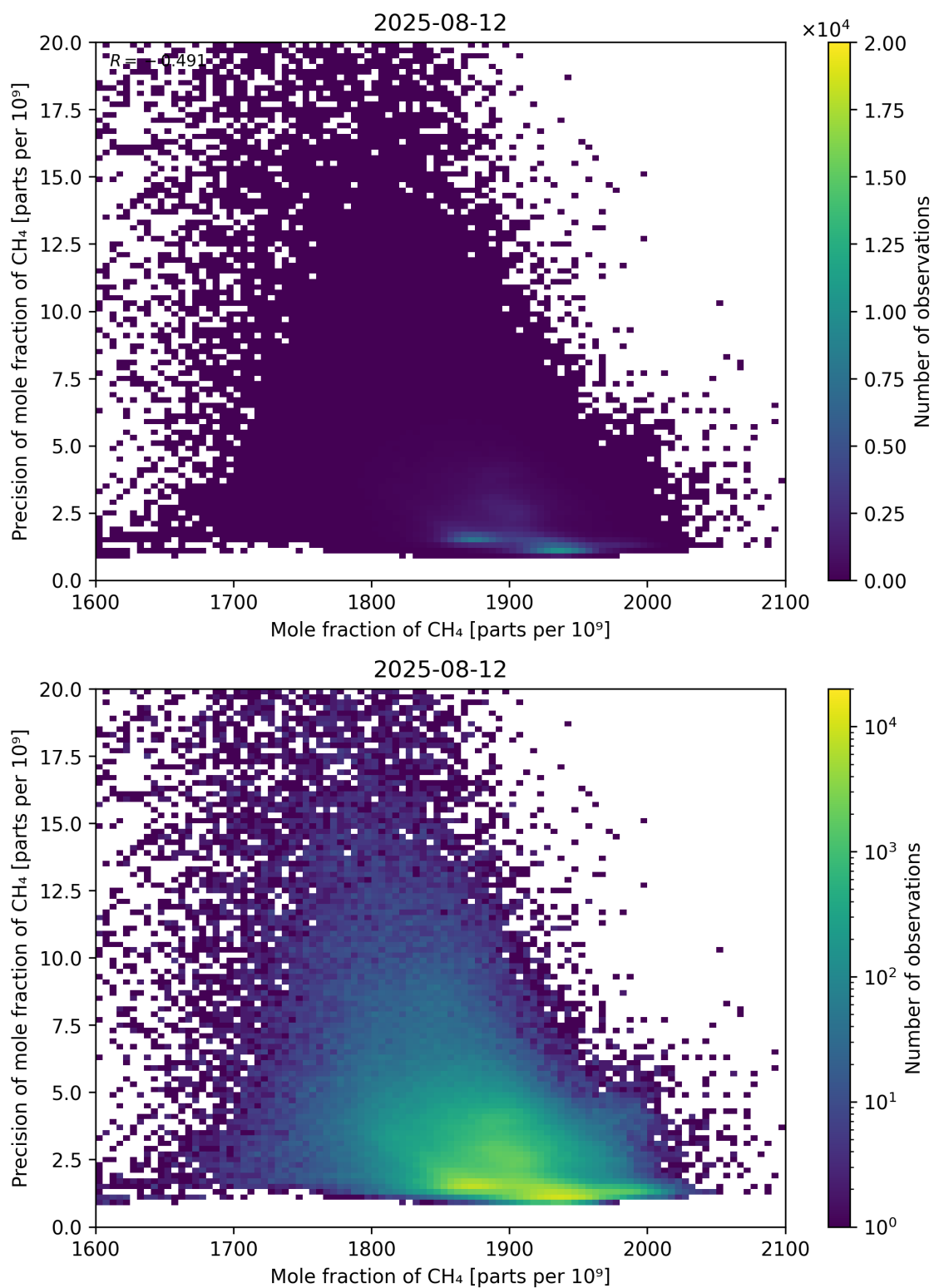
Figure 75: Scatter density plot of “Mole fraction of CH 4 ” against “Precision of mole fraction of CH 4 ” for 2025-08-11 to 2025-08-13.
