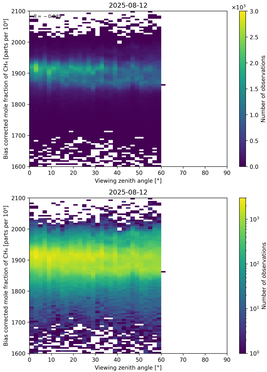
Figure 111: Scatter density plot of “Viewing zenith angle” against “Bias corrected mole fraction of CH 4 ” for 2025-08-11 to 2025-08-13.
