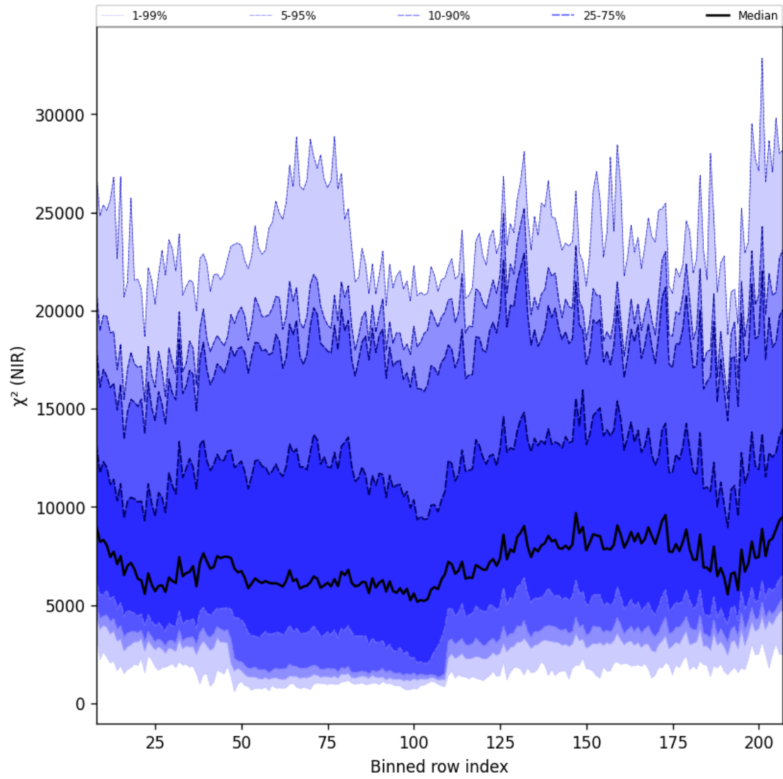
Figure 40: Along track statistics of “ \chi^2 (NIR)” for 2025-08-11 to 2025-08-13
