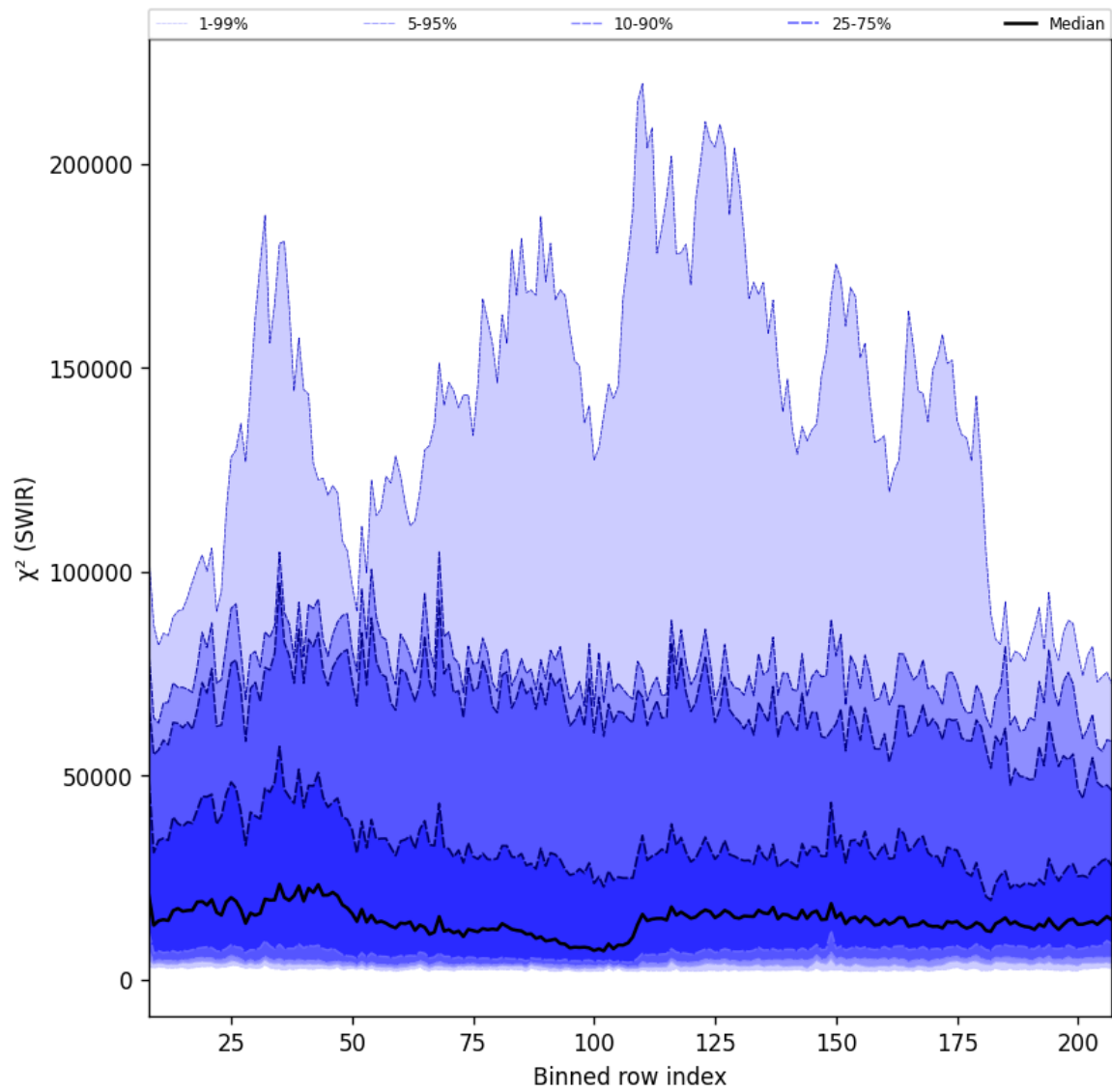
Figure 39: Along track statistics of “ \chi^2 (SWIR)” for 2025-08-11 to 2025-08-13
