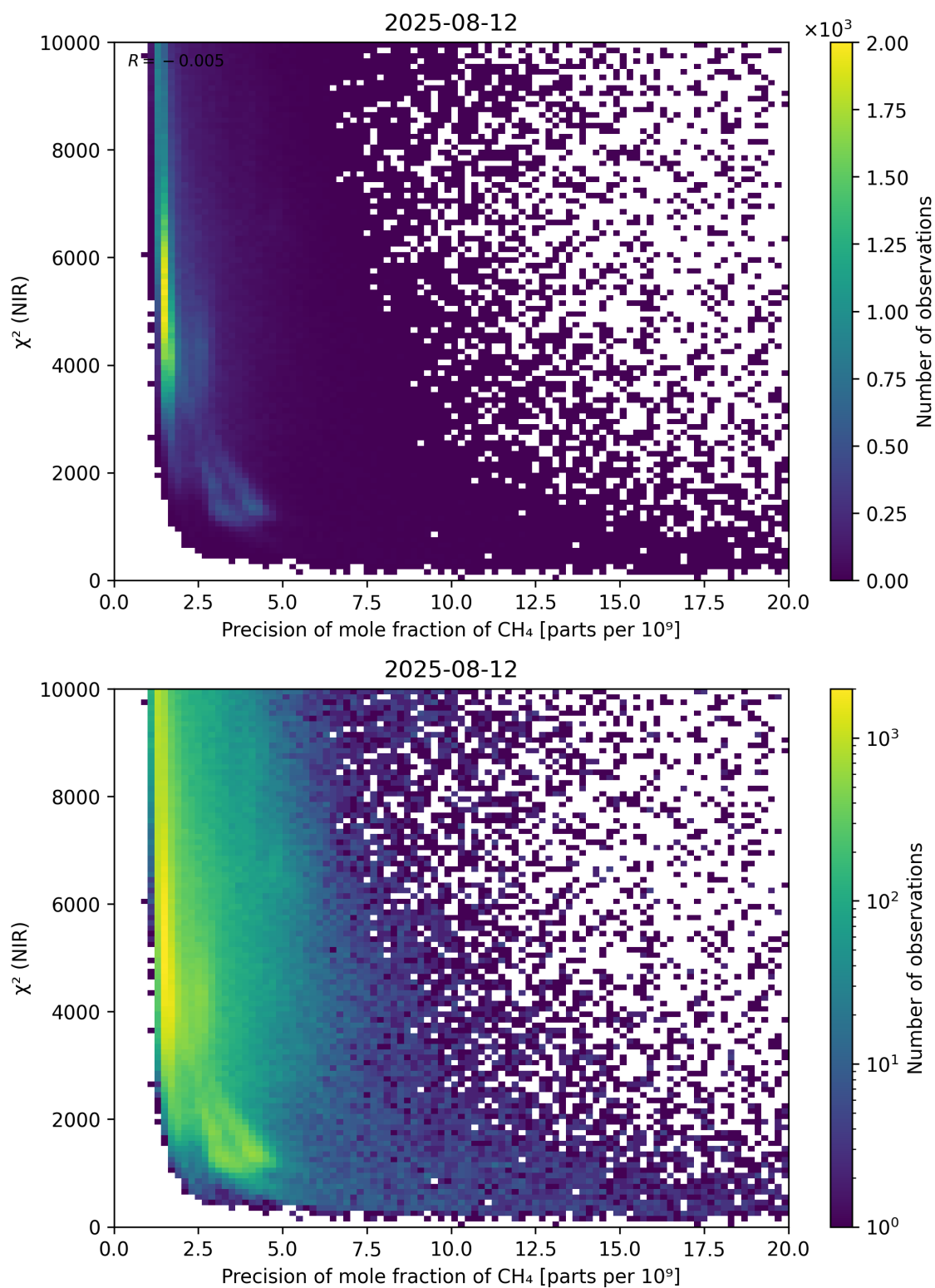
Figure 78: Scatter density plot of “Precision of mole fraction of \text{CH}_4 ” against “ \chi^2 (NIR)” for 2025-08-11 to 2025-08-13.
