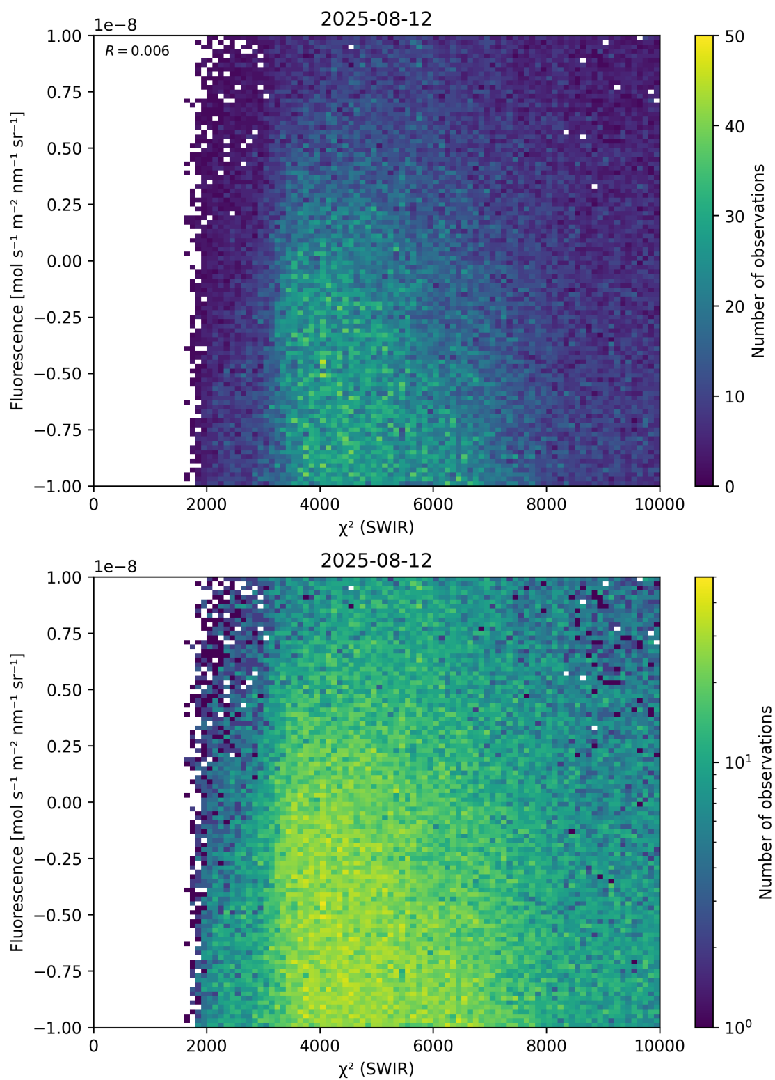
Figure 49: Scatter density plot of “ \chi^2 (SWIR)” against “Fluorescence” for 2025-08-11 to 2025-08-13.
