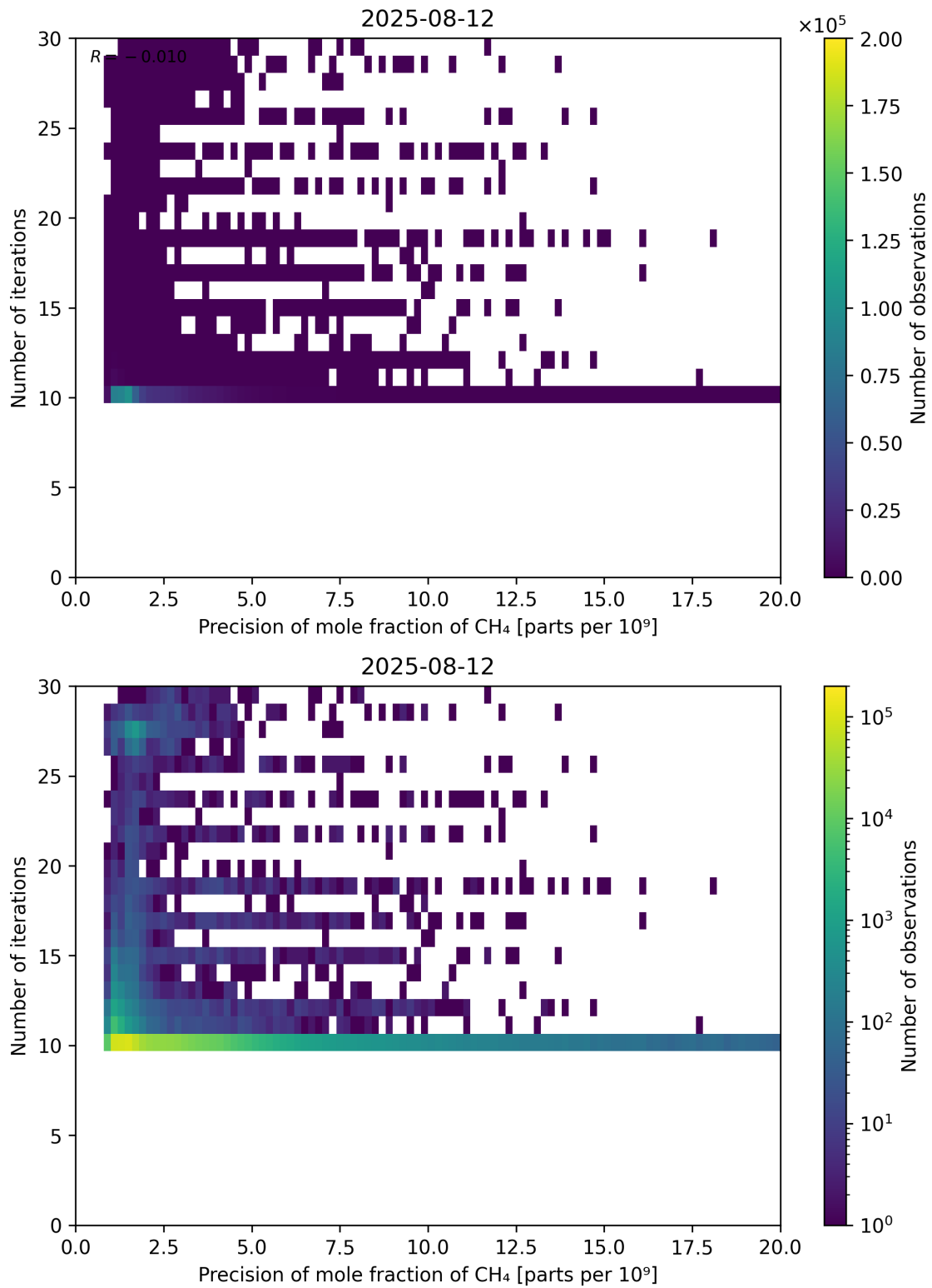
Figure 83: Scatter density plot of “Precision of mole fraction of CH 4 ” against “Number of iterations” for 2025-08-11 to 2025-08-13.
