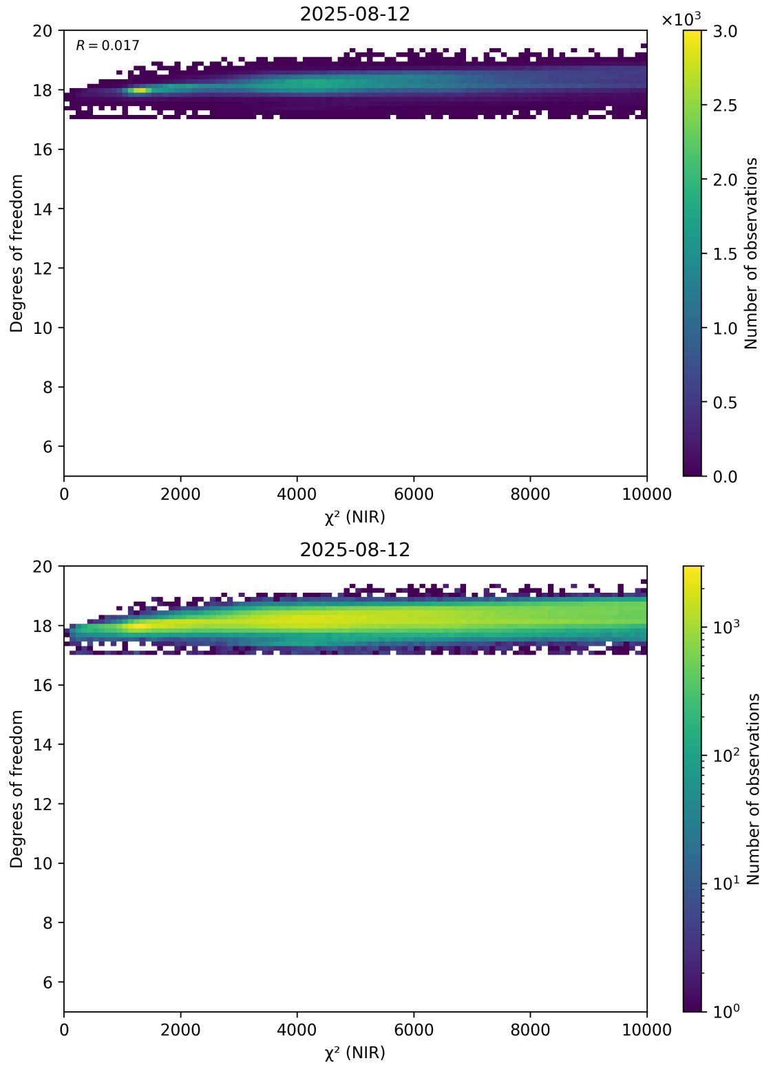
Figure 44: Scatter density plot of “ \chi^2 (NIR)” against “Degrees of freedom” for 2025-08-11 to 2025-08-13.
