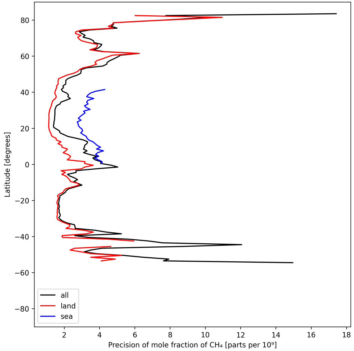
Figure 13: Zonal average of “Precision of mole fraction of \text{CH}_4 ” for 2025-08-11 to 2025-08-13.
