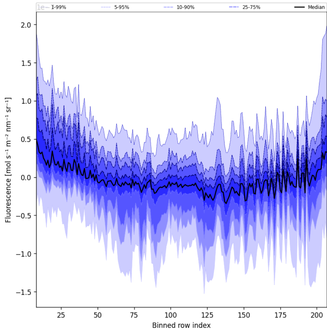
Figure 43: Along track statistics of “Fluorescence” for 2025-08-11 to 2025-08-13
