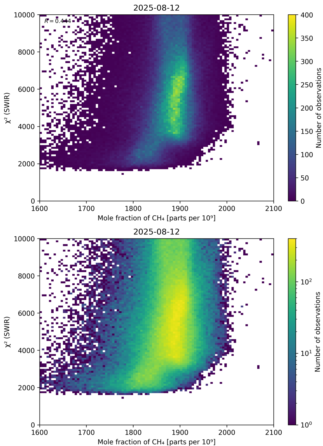
Figure 71: Scatter density plot of “Mole fraction of \text{CH}_4 ” against “ \chi^2 (SWIR)” for 2025-08-11 to 2025-08-13.
