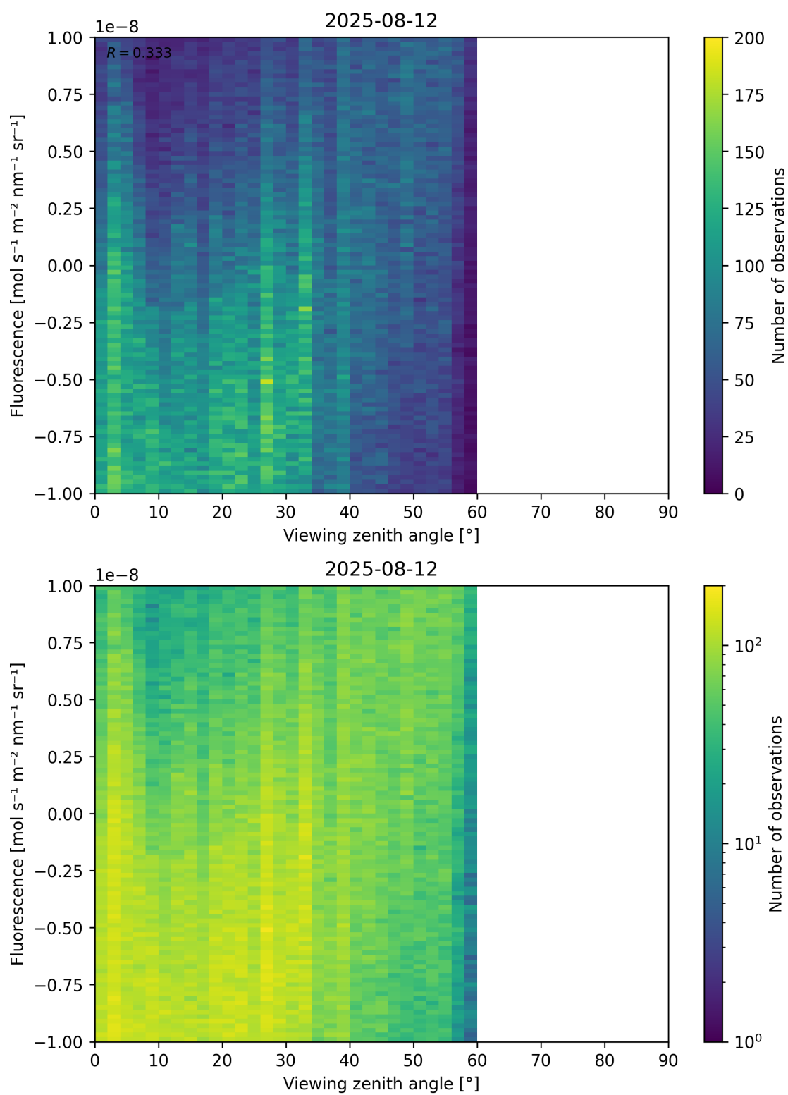
Figure 108: Scatter density plot of “Viewing zenith angle” against “Fluorescence” for 2025-08-11 to 2025-08-13.
