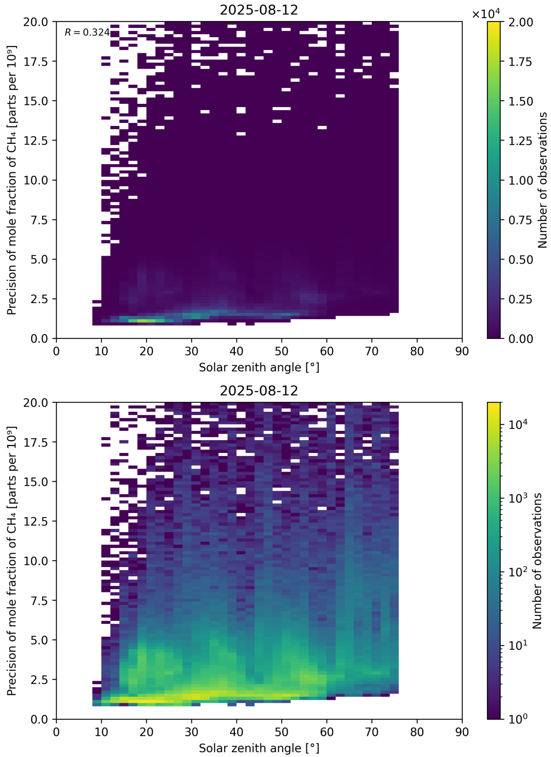
Figure 101: Scatter density plot of “Solar zenith angle” against “Precision of mole fraction of CH 4 ” for 2025-08-11 to 2025-08-13.
