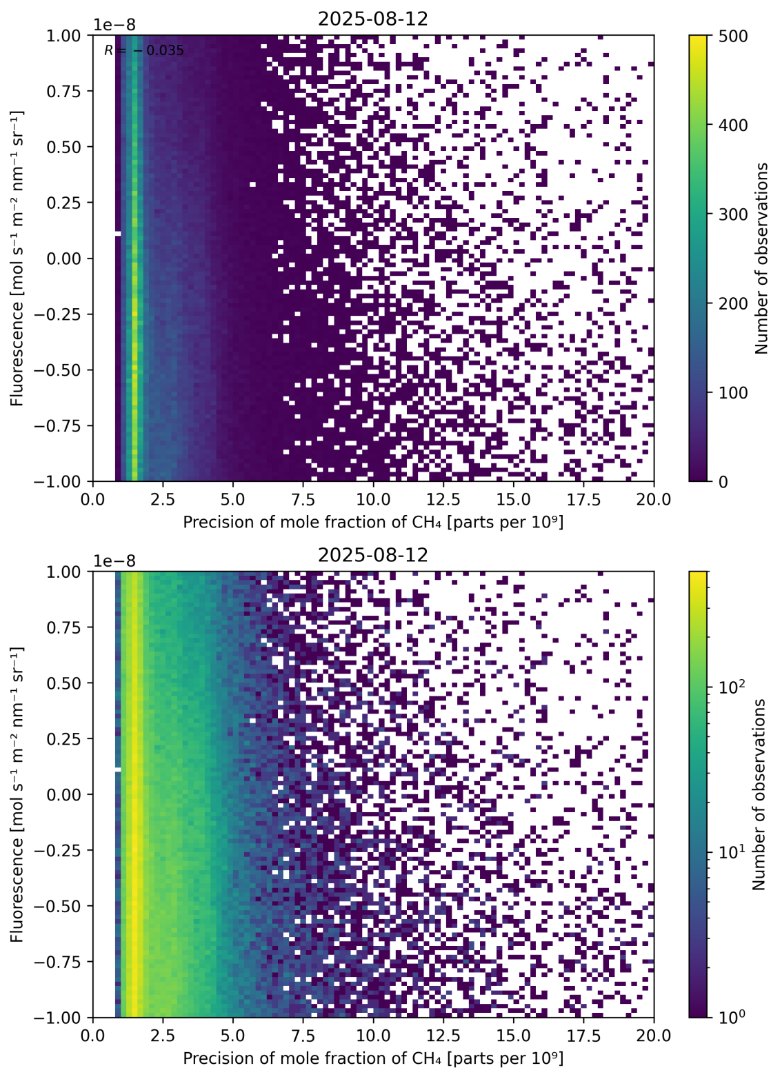
Figure 81: Scatter density plot of “Precision of mole fraction of CH 4 ” against “Fluorescence” for 2025-08-11 to 2025-08-13.
