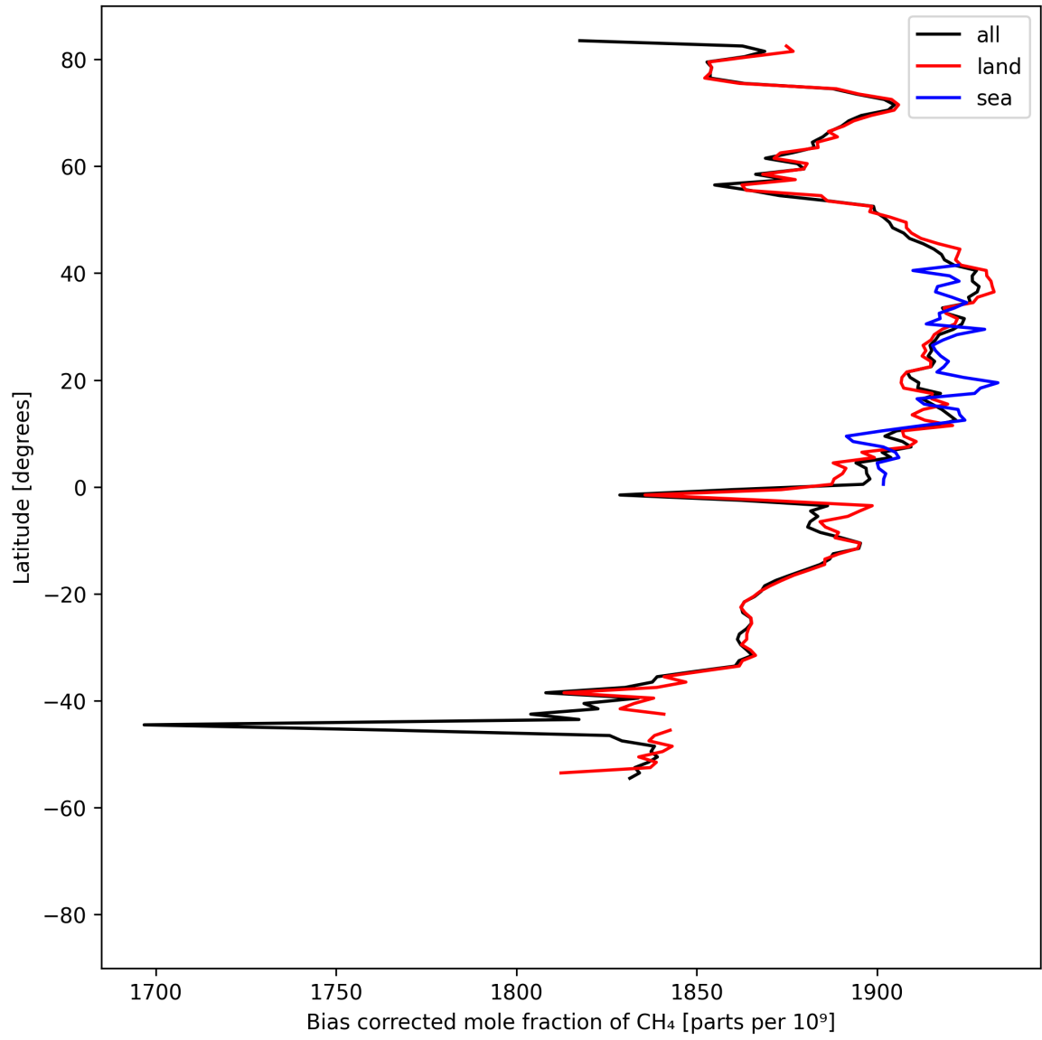
Figure 14: Zonal average of “Bias corrected mole fraction of \text{CH}_4 ” for 2025-08-11 to 2025-08-13.
