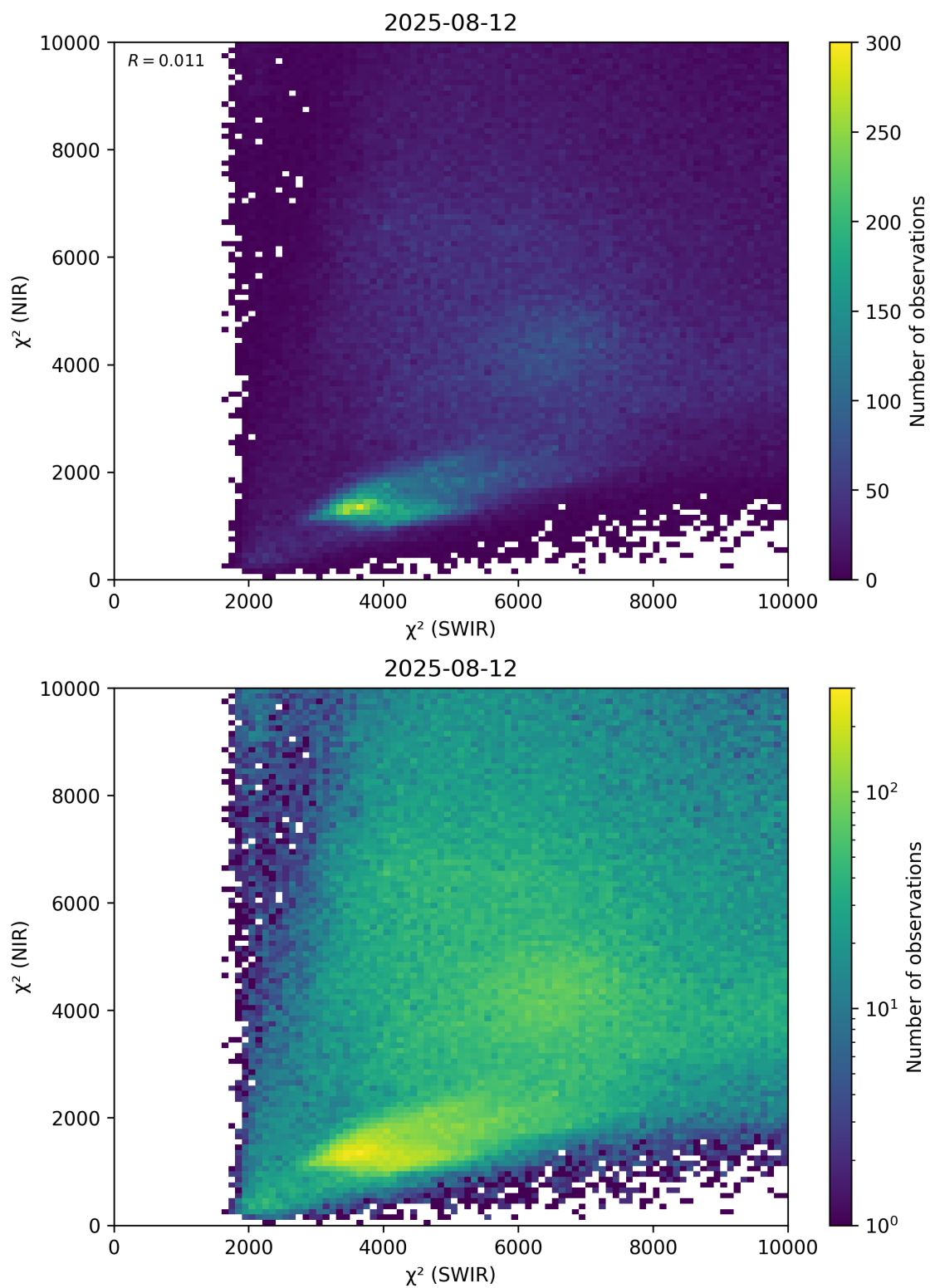
Figure 47: Scatter density plot of “ \chi^2 (SWIR)” against “ \chi^2 (NIR)” for 2025-08-11 to 2025-08-13.
