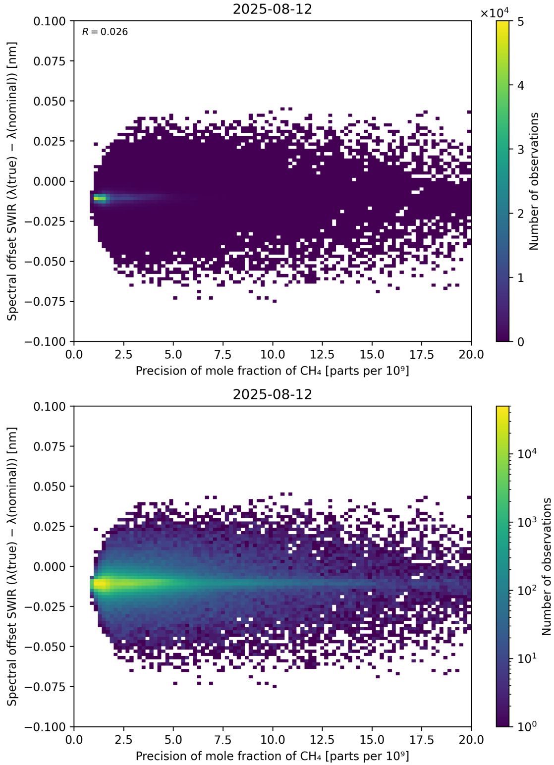
Figure 85: Scatter density plot of “Precision of mole fraction of CH 4 ” against “Spectral offset SWIR ( \lambda_{\text{true}} - \lambda_{\text{nominal}} )” for 2025-08-11 to 2025-08-13.
