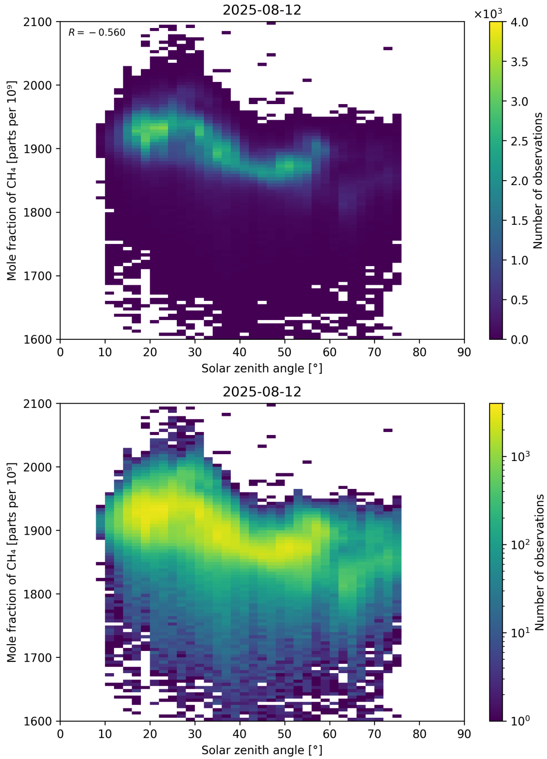
Figure 99: Scatter density plot of “Solar zenith angle” against “Mole fraction of CH 4 ” for 2025-08-11 to 2025-08-13.
