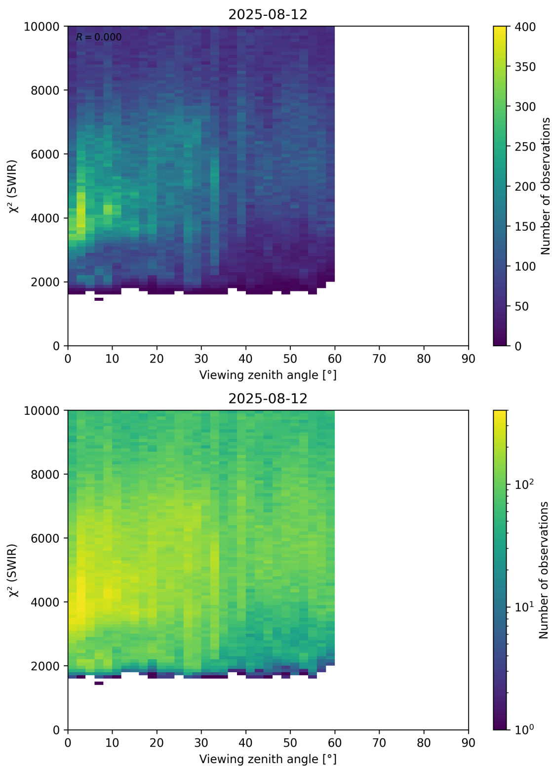
Figure 106: Scatter density plot of “Viewing zenith angle” against “ \chi^2 (SWIR)” for 2025-08-11 to 2025-08-13.
