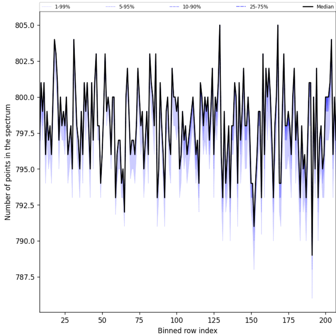
Figure 37: Along track statistics of “Number of points in the spectrum” for 2025-08-11 to 2025-08-13
