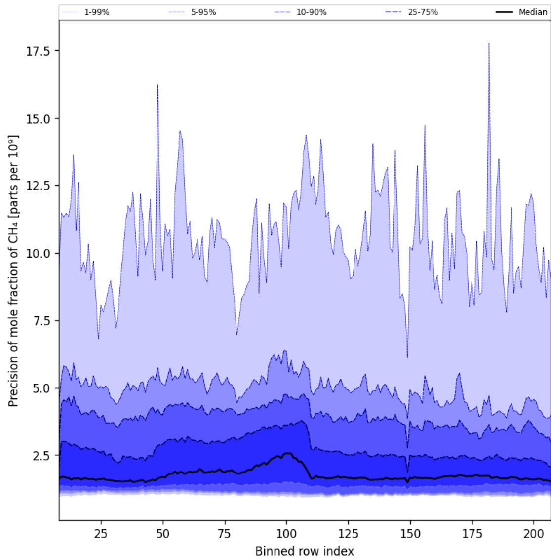
Figure 35: Along track statistics of “Precision of mole fraction of CH 4 ” for 2025-08-11 to 2025-08-13
