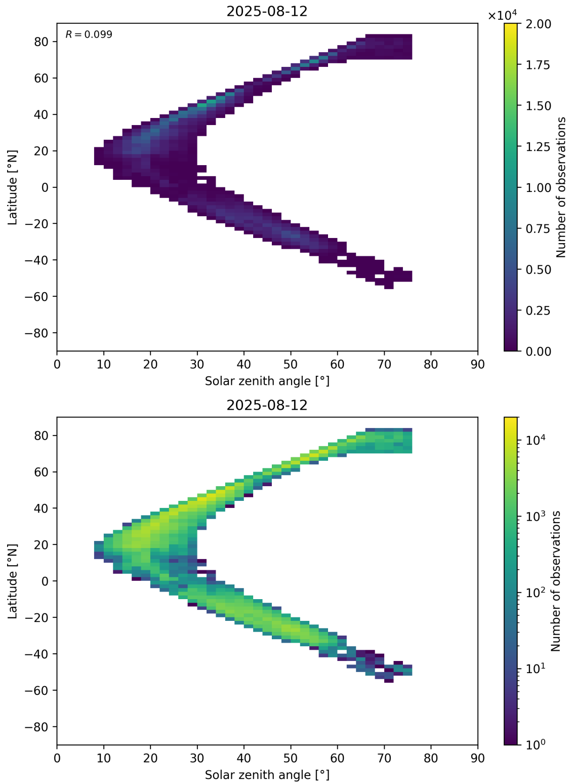
Figure 98: Scatter density plot of “Solar zenith angle” against “Latitude” for 2025-08-11 to 2025-08-13.
