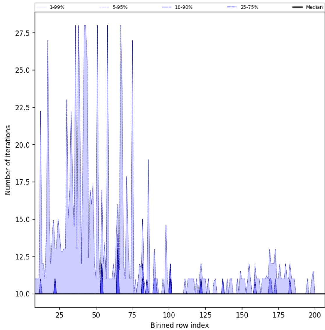
Figure 42: Along track statistics of “Number of iterations” for 2025-08-11 to 2025-08-13
