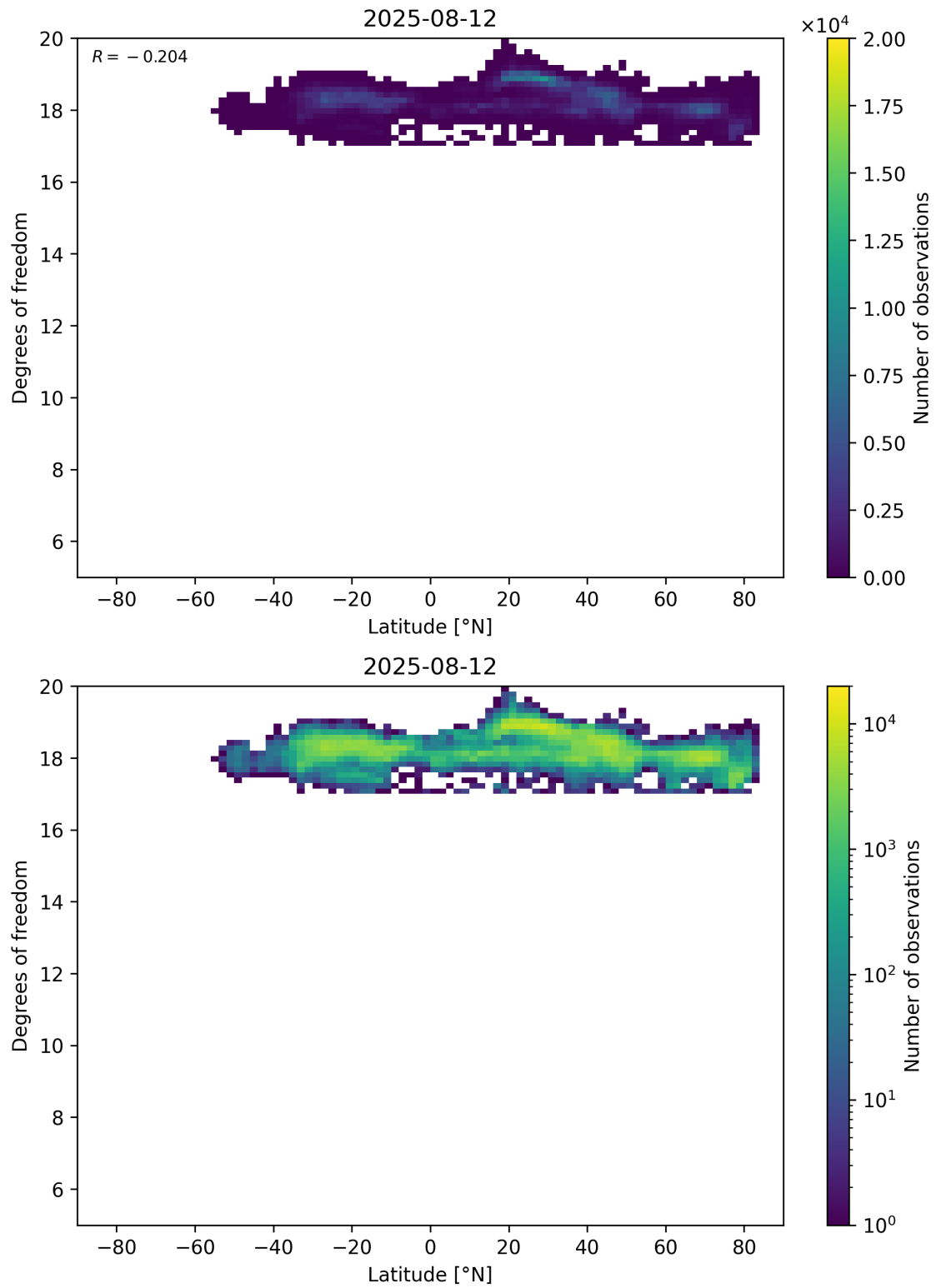
Figure 55: Scatter density plot of “Latitude” against “Degrees of freedom” for 2025-08-11 to 2025-08-13.
