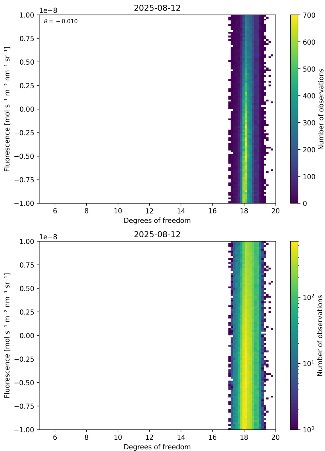
Figure 51: Scatter density plot of “Degrees of freedom” against “Fluorescence” for 2025-08-11 to 2025-08-13.
