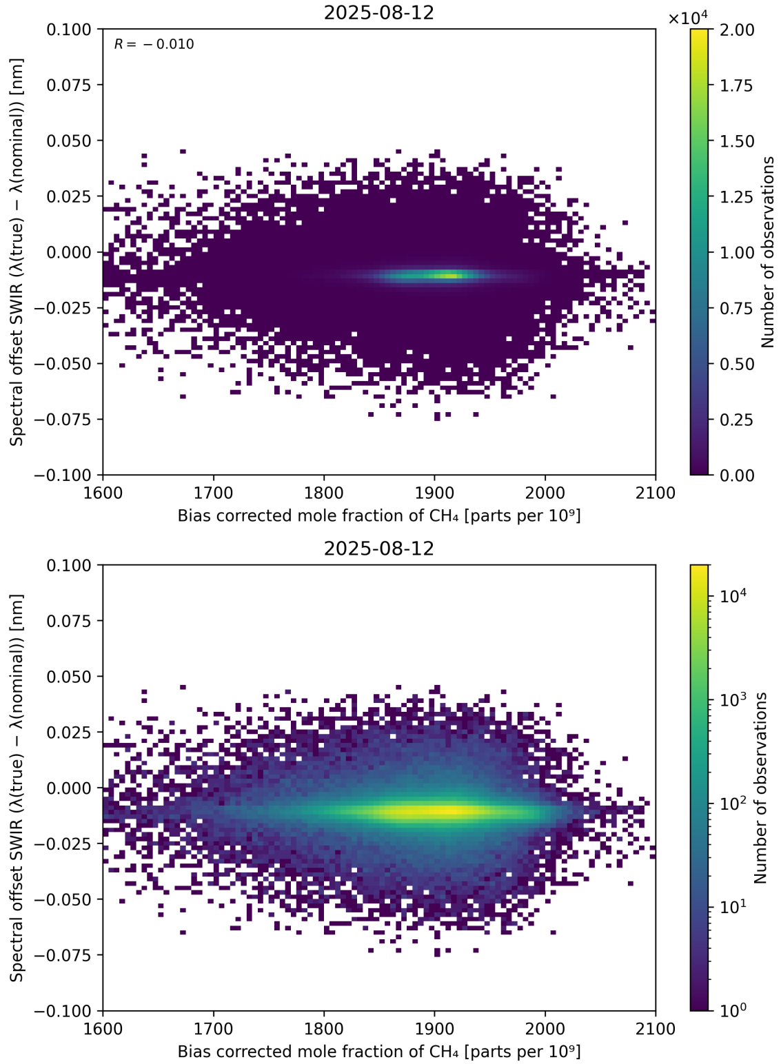
Figure 69: Scatter density plot of “Bias corrected mole fraction of \text{CH}_4 ” against “Spectral offset SWIR ( \lambda_{\text{true}} - \lambda_{\text{nominal}} )” for 2025-08-11 to 2025-08-13.
