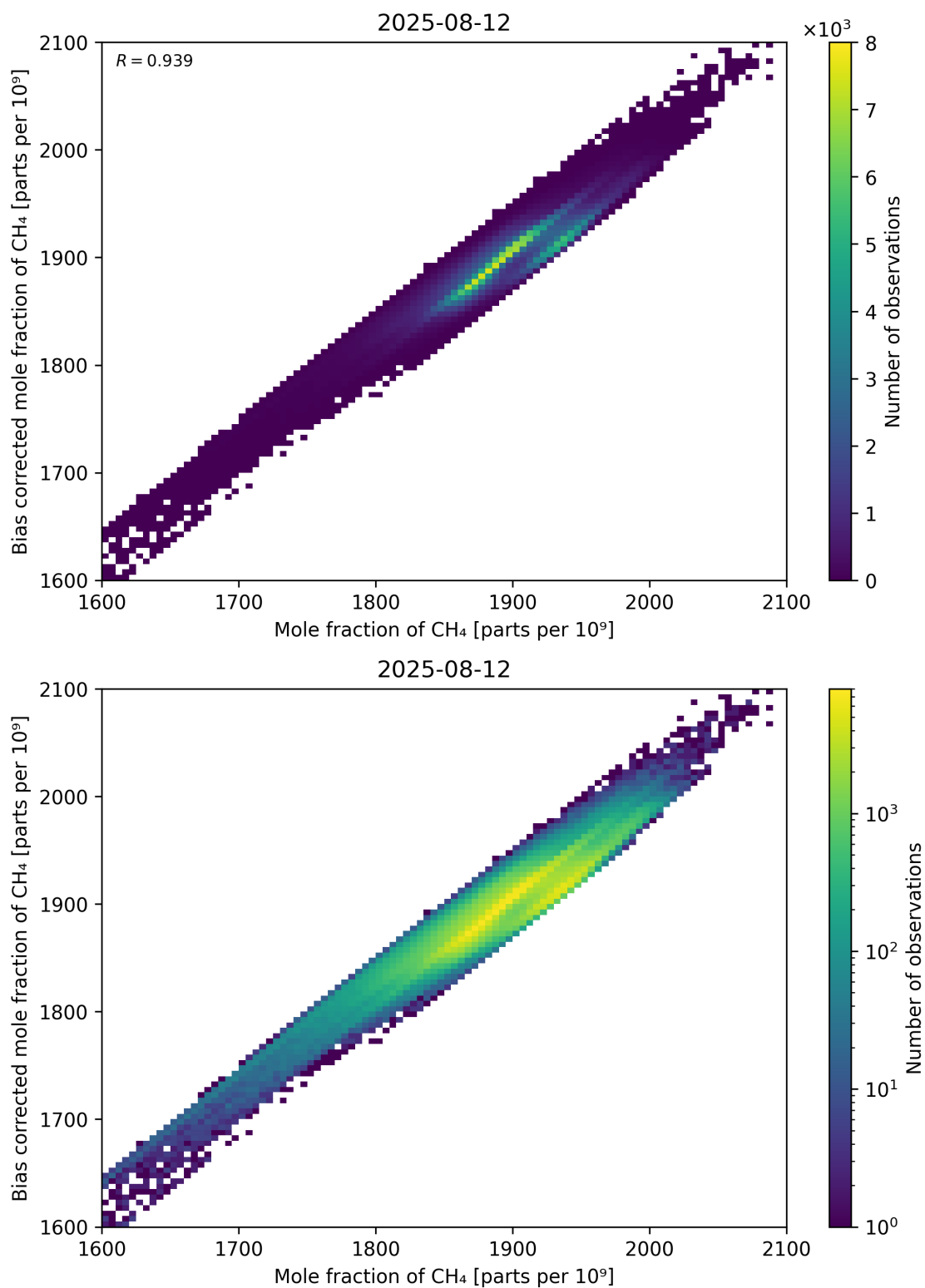
Figure 74: Scatter density plot of “Mole fraction of CH 4 ” against “Bias corrected mole fraction of CH 4 ” for 2025-08-11 to 2025-08-13.
