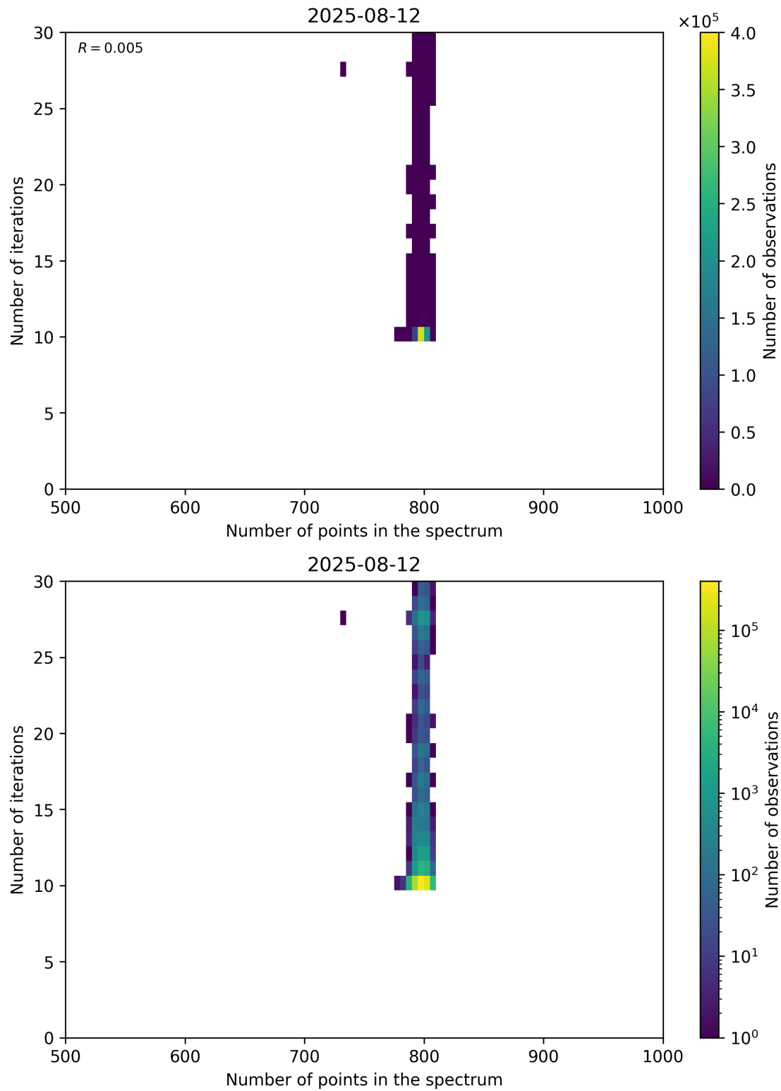
Figure 92: Scatter density plot of “Number of points in the spectrum” against “Number of iterations” for 2025-08-11 to 2025-08-13.
