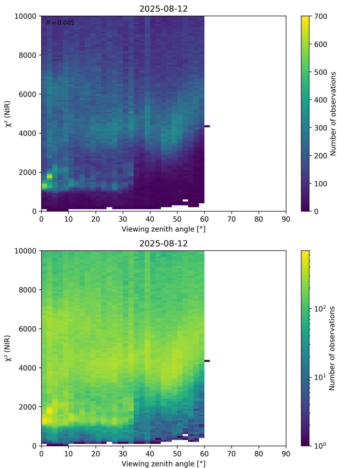
Figure 105: Scatter density plot of “Viewing zenith angle” against “ \chi^2 (NIR)” for 2025-08-11 to 2025-08-13.
