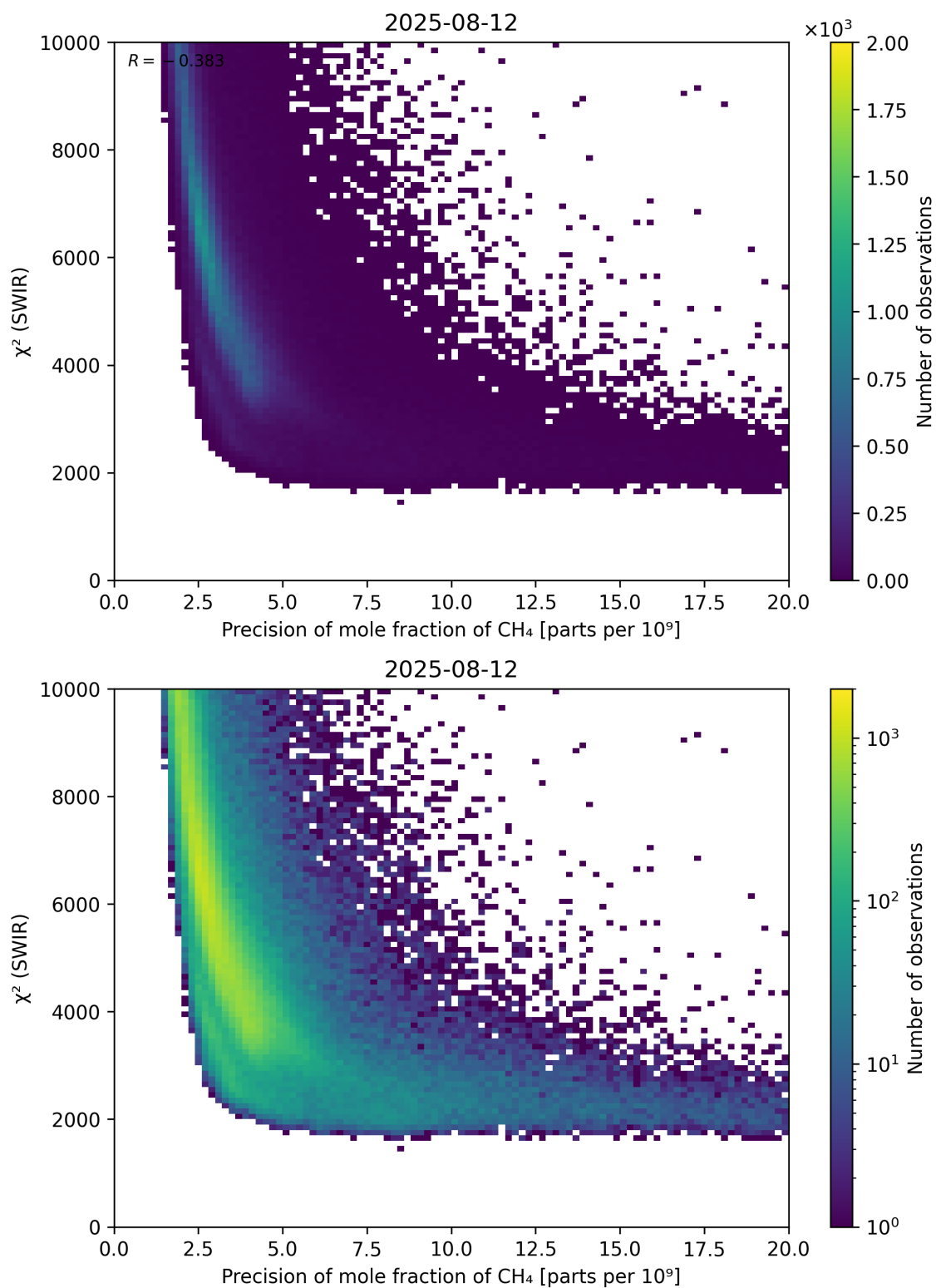
Figure 79: Scatter density plot of “Precision of mole fraction of \text{CH}_4 ” against “ \chi^2 (SWIR)” for 2025-08-11 to 2025-08-13.
