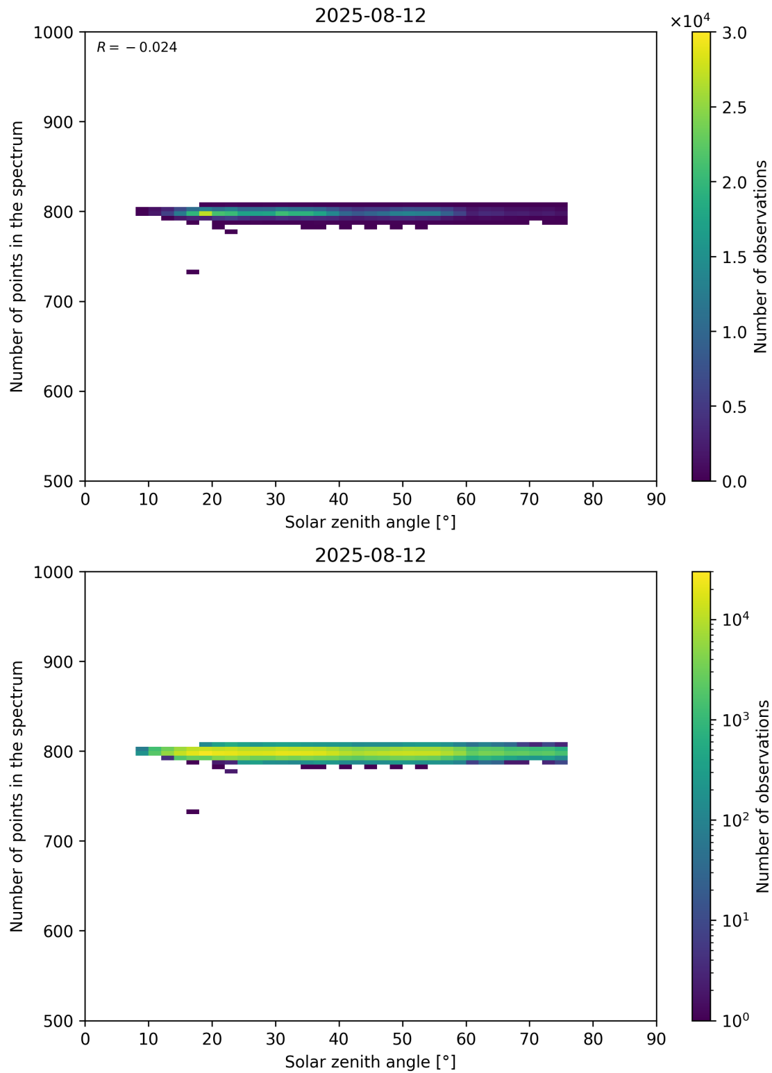
Figure 103: Scatter density plot of “Solar zenith angle” against “Number of points in the spectrum” for 2025-08-11 to 2025-08-13.
