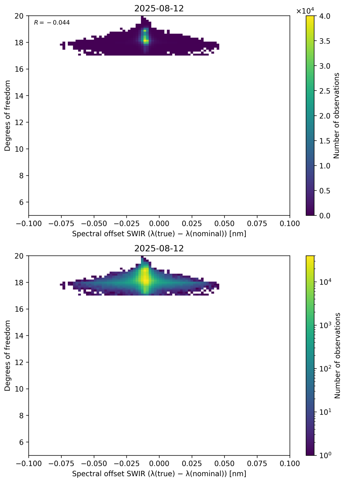
Figure 119: Scatter density plot of “Spectral offset SWIR ( \lambda_{\text{true}} - \lambda_{\text{nominal}} )” against “Degrees of freedom” for 2025-08-11 to 2025-08-13.
