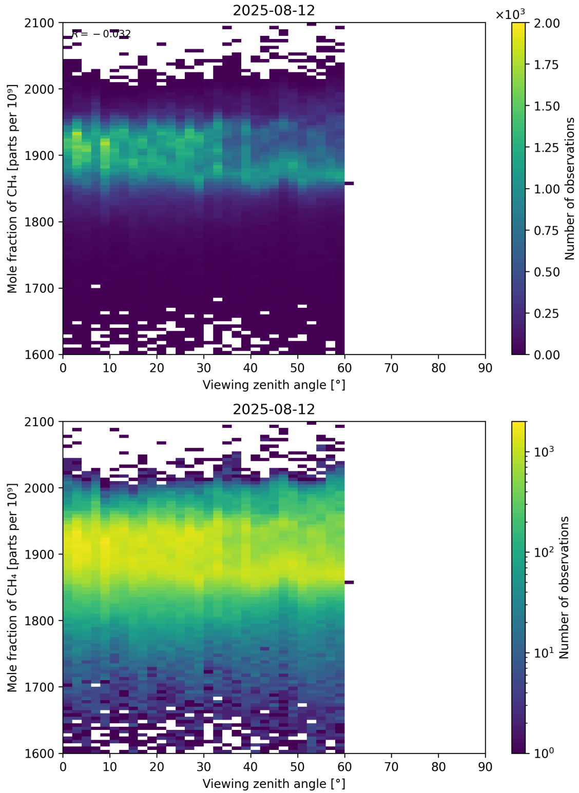
Figure 110: Scatter density plot of “Viewing zenith angle” against “Mole fraction of CH 4 ” for 2025-08-11 to 2025-08-13.
