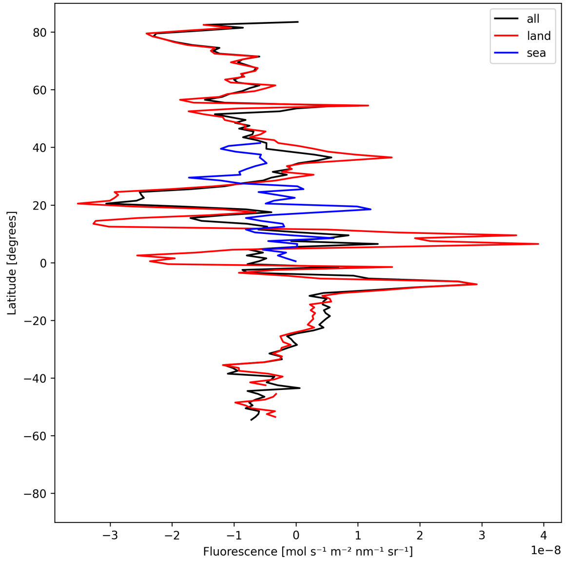
Figure 21: Zonal average of “Fluorescence” for 2025-08-11 to 2025-08-13.
