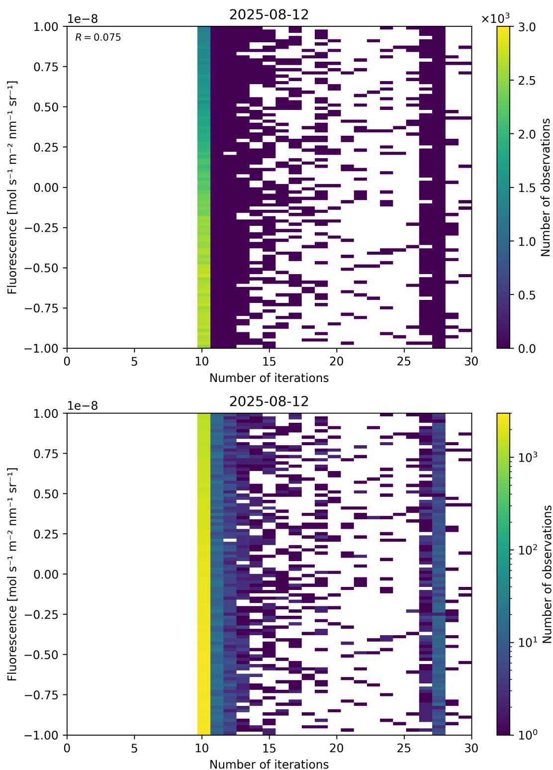
Figure 87: Scatter density plot of “Number of iterations” against “Fluorescence” for 2025-08-11 to 2025-08-13.
