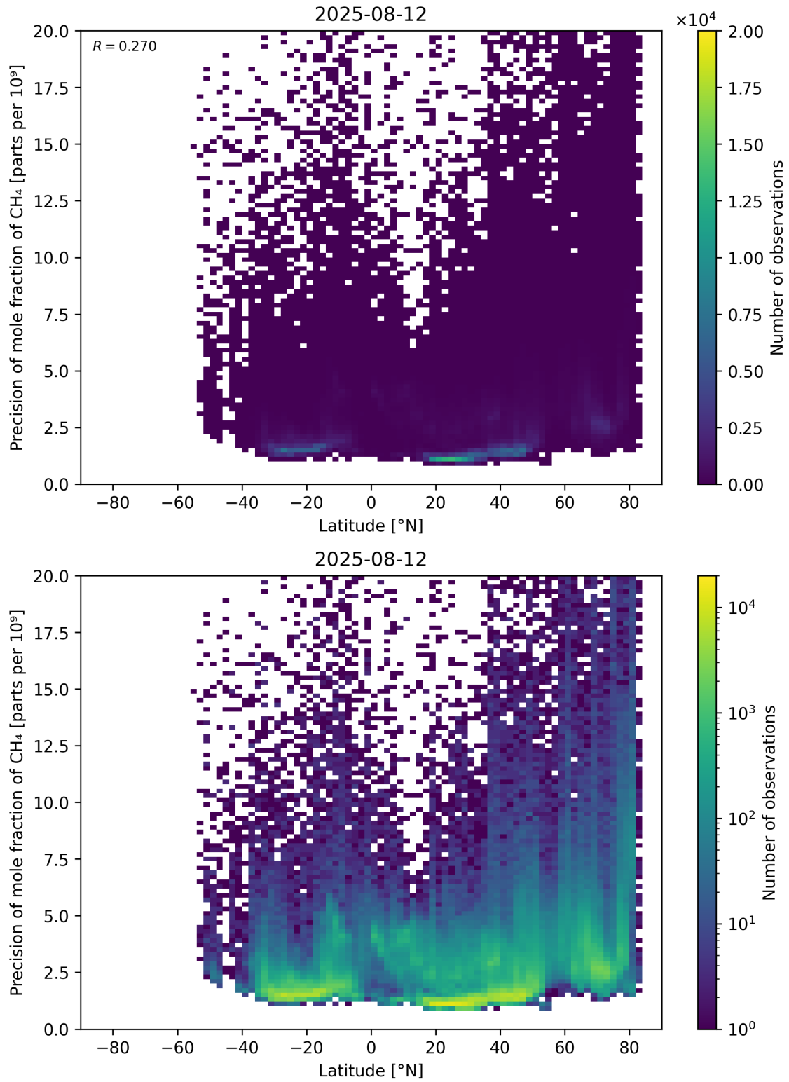
Figure 59: Scatter density plot of “Latitude” against “Precision of mole fraction of \text{CH}_4 ” for 2025-08-11 to 2025-08-13.
