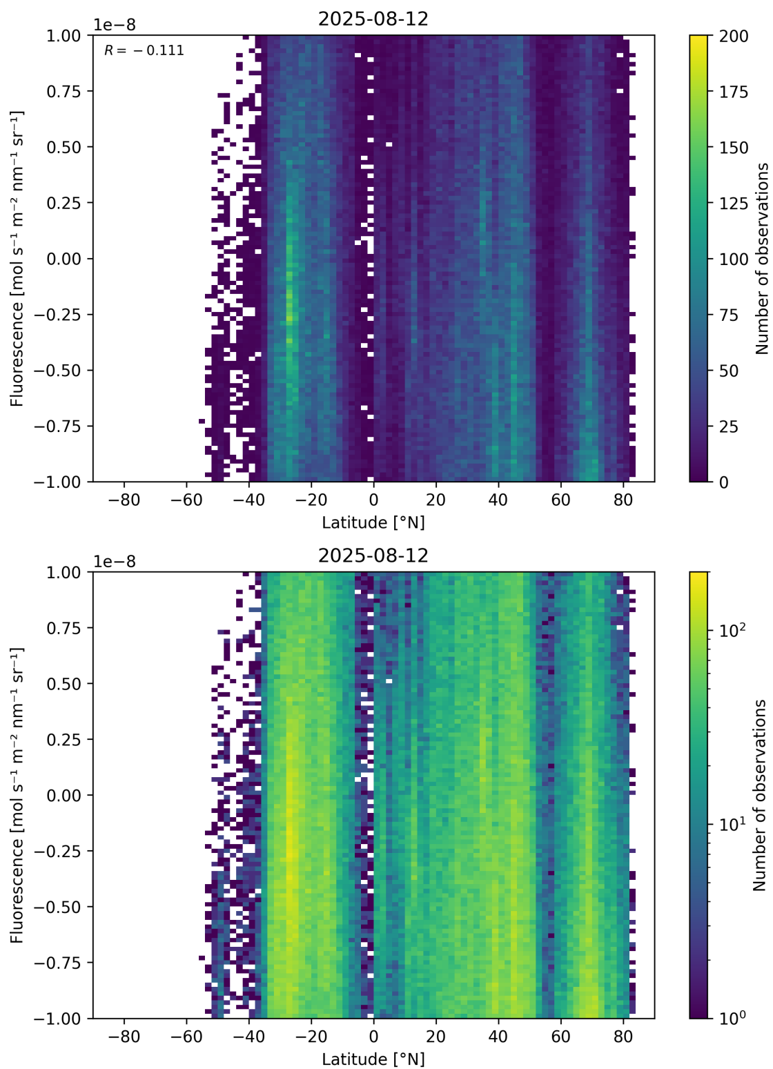
Figure 56: Scatter density plot of “Latitude” against “Fluorescence” for 2025-08-11 to 2025-08-13.
