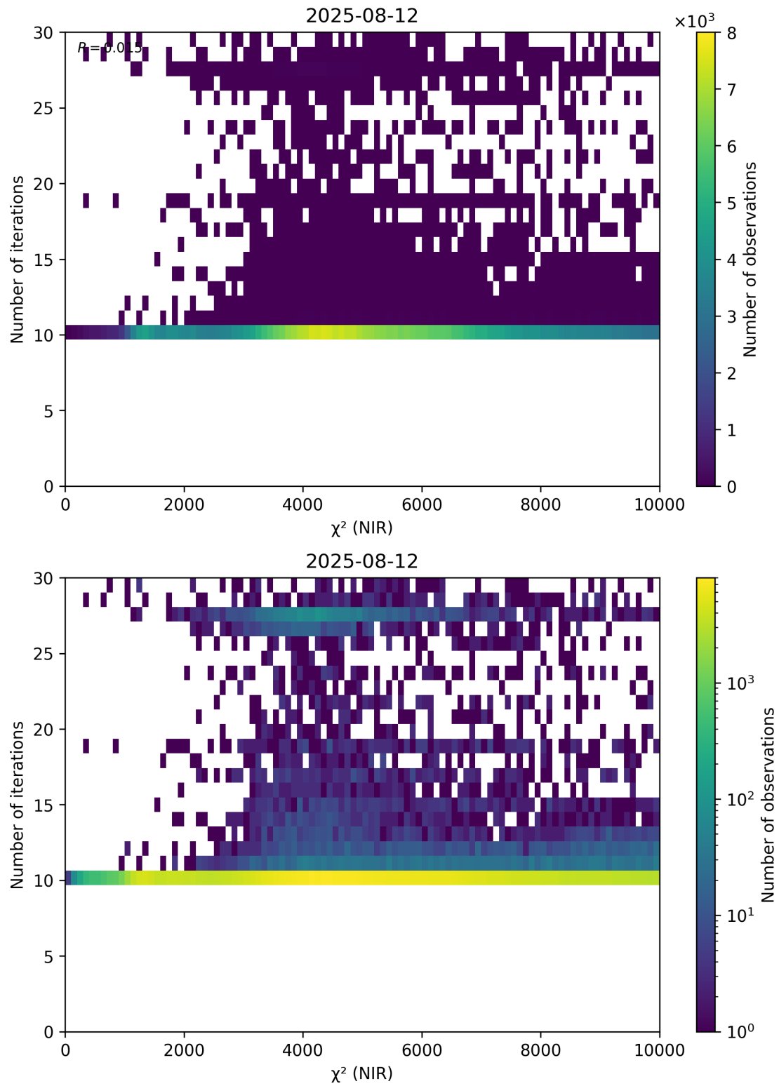
Figure 46: Scatter density plot of “ \chi^2 (NIR)” against “Number of iterations” for 2025-08-11 to 2025-08-13.
