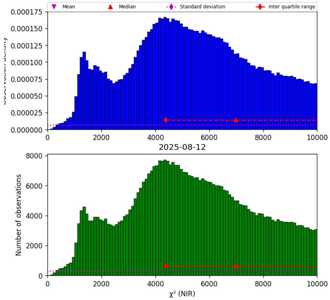
Figure 29: Histogram of “ \chi^2 (NIR)” for 2025-08-11 to 2025-08-13
