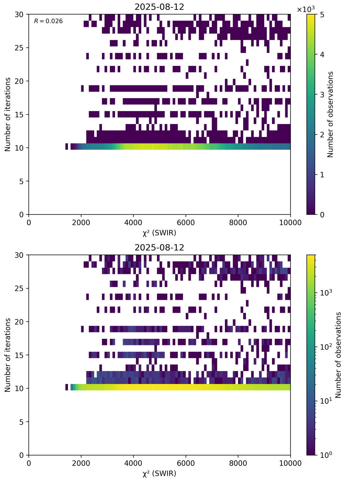
Figure 50: Scatter density plot of “ \chi^2 (SWIR)” against “Number of iterations” for 2025-08-11 to 2025-08-13.
