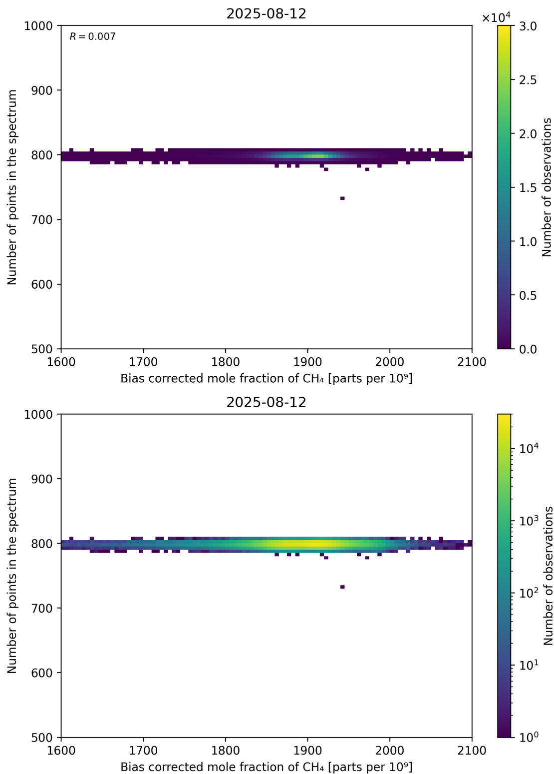
Figure 68: Scatter density plot of “Bias corrected mole fraction of CH 4 ” against “Number of points in the spectrum” for 2025-08-11 to 2025-08-13.
