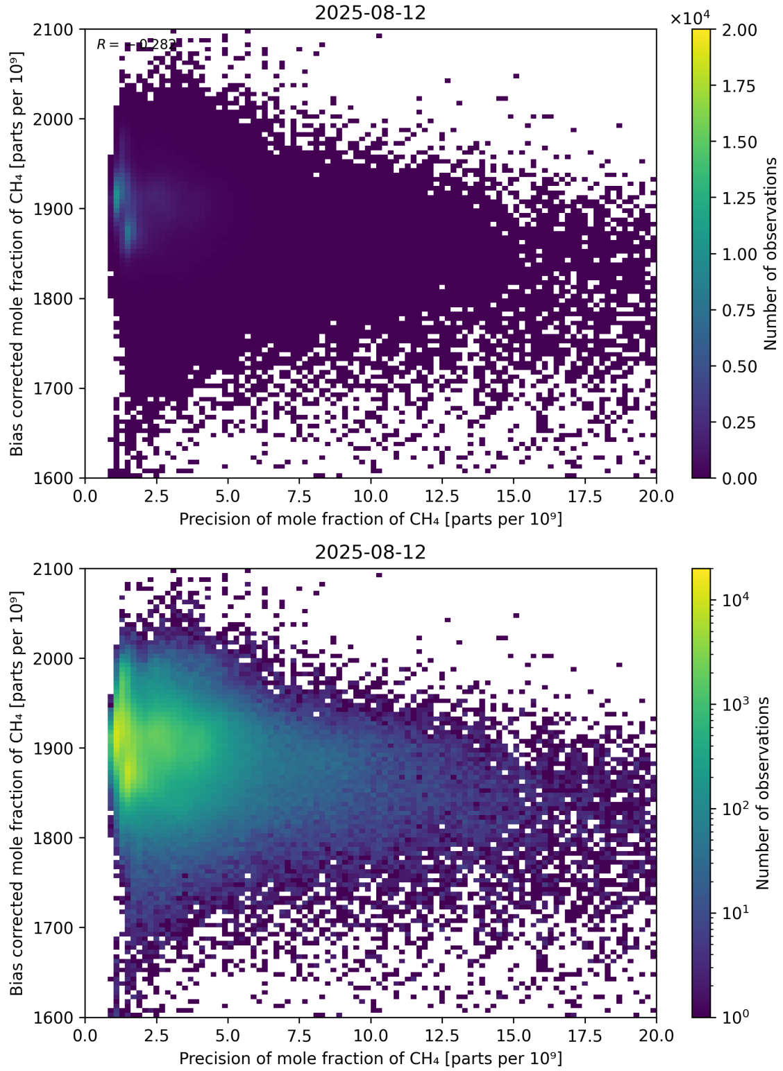
Figure 82: Scatter density plot of “Precision of mole fraction of CH 4 ” against “Bias corrected mole fraction of CH 4 ” for 2025-08-11 to 2025-08-13.
