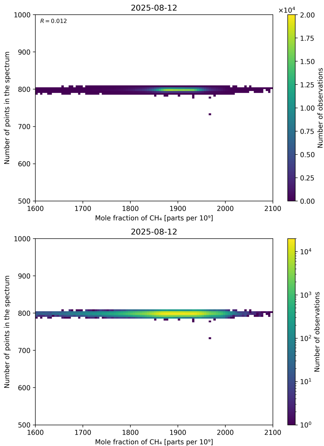
Figure 77: Scatter density plot of “Mole fraction of CH 4 ” against “Number of points in the spectrum” for 2025-08-11 to 2025-08-13.
