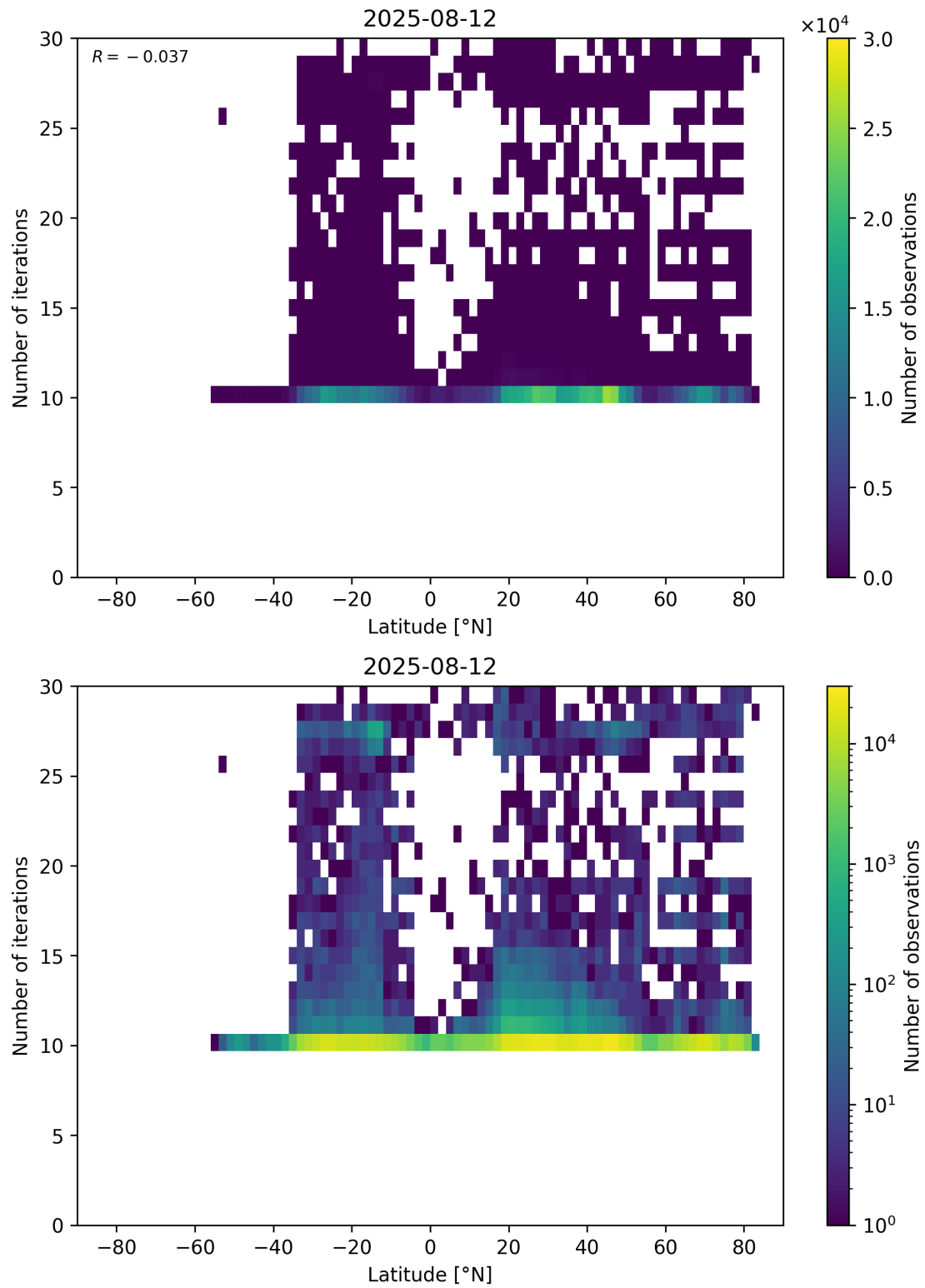
Figure 60: Scatter density plot of “Latitude” against “Number of iterations” for 2025-08-11 to 2025-08-13.
