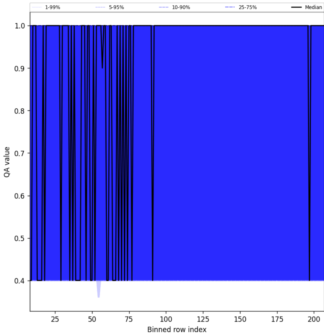
Figure 33: Along track statistics of “QA value” for 2025-08-11 to 2025-08-13
