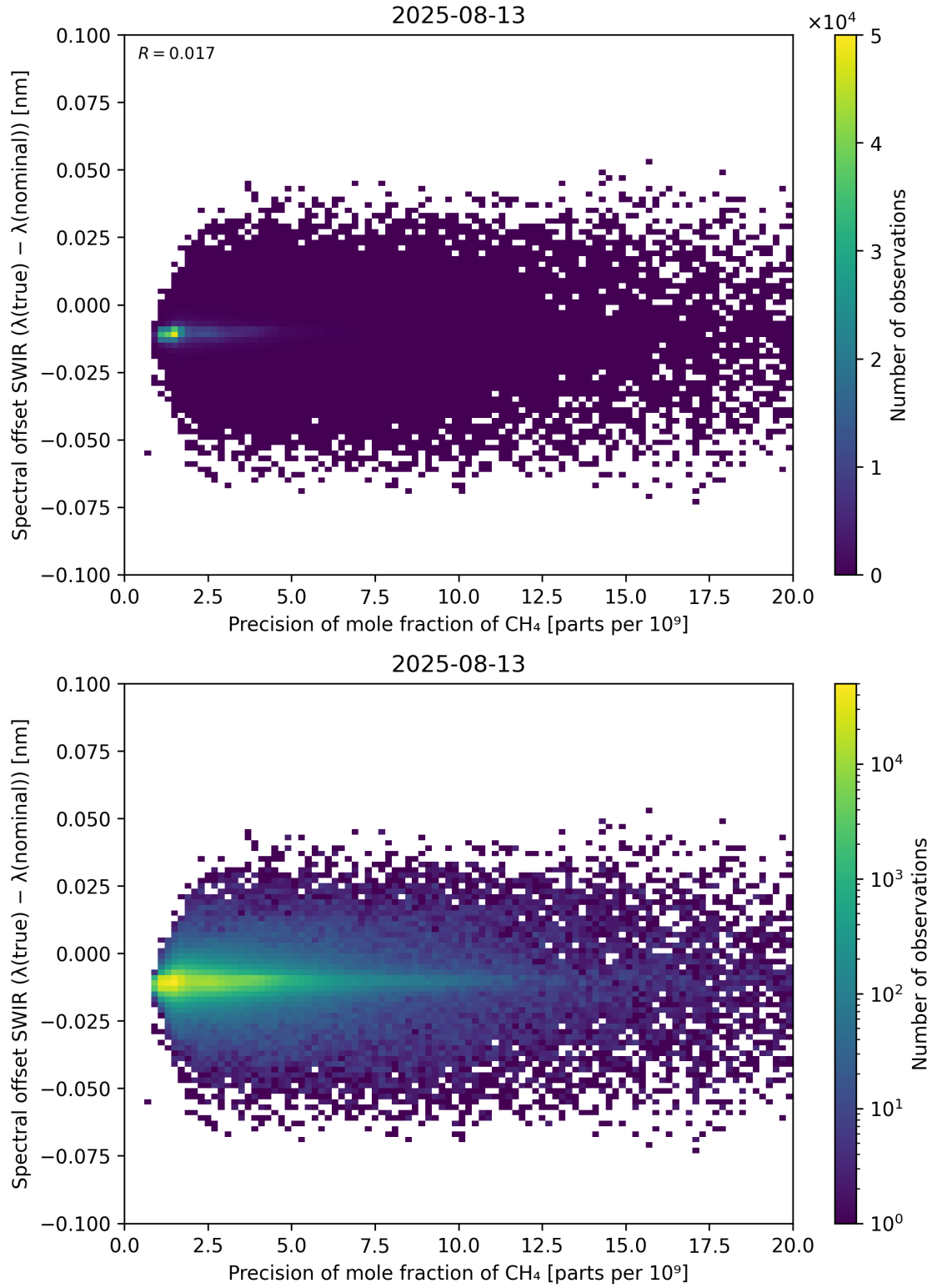
Figure 85: Scatter density plot of “Precision of mole fraction of CH 4 ” against “Spectral offset SWIR ( \lambda_{\text{true}} - \lambda_{\text{nominal}} )” for 2025-08-12 to 2025-08-14.
