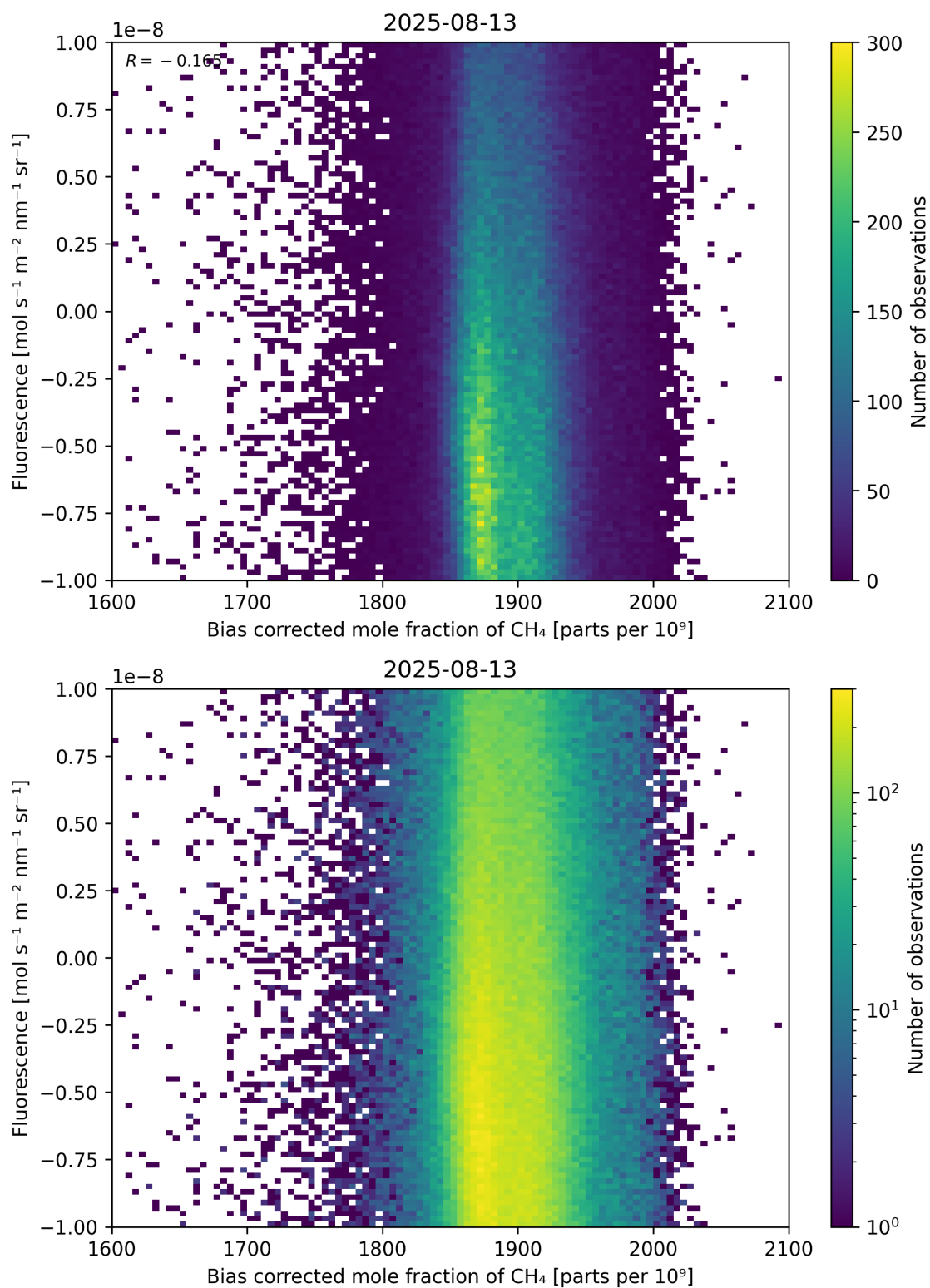
Figure 66: Scatter density plot of “Bias corrected mole fraction of \text{CH}_4 ” against “Fluorescence” for 2025-08-12 to 2025-08-14.
