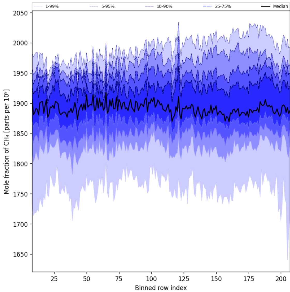
Figure 34: Along track statistics of “Mole fraction of CH 4 ” for 2025-08-12 to 2025-08-14
