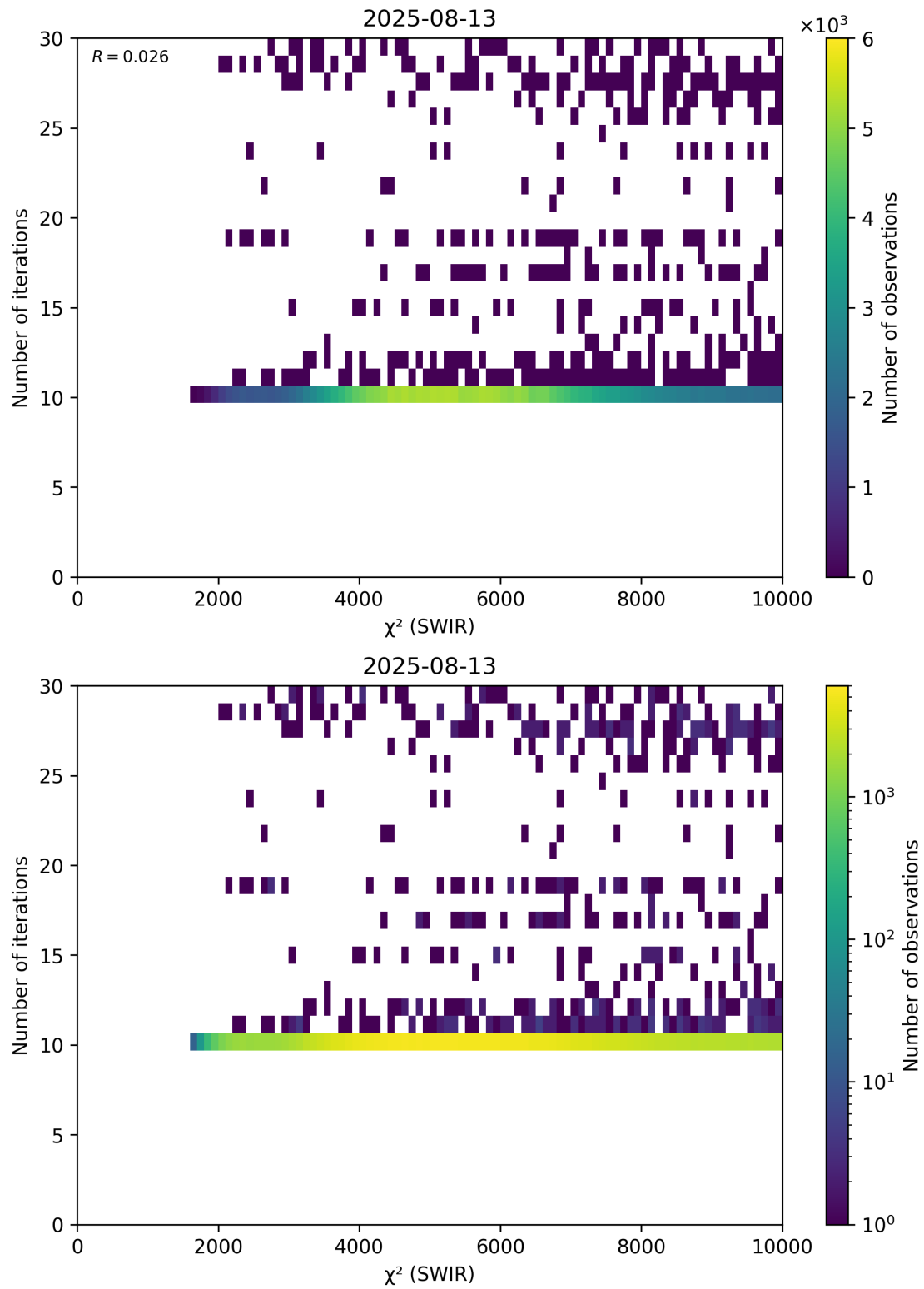
Figure 50: Scatter density plot of “ \chi^2 (SWIR)” against “Number of iterations” for 2025-08-12 to 2025-08-14.
