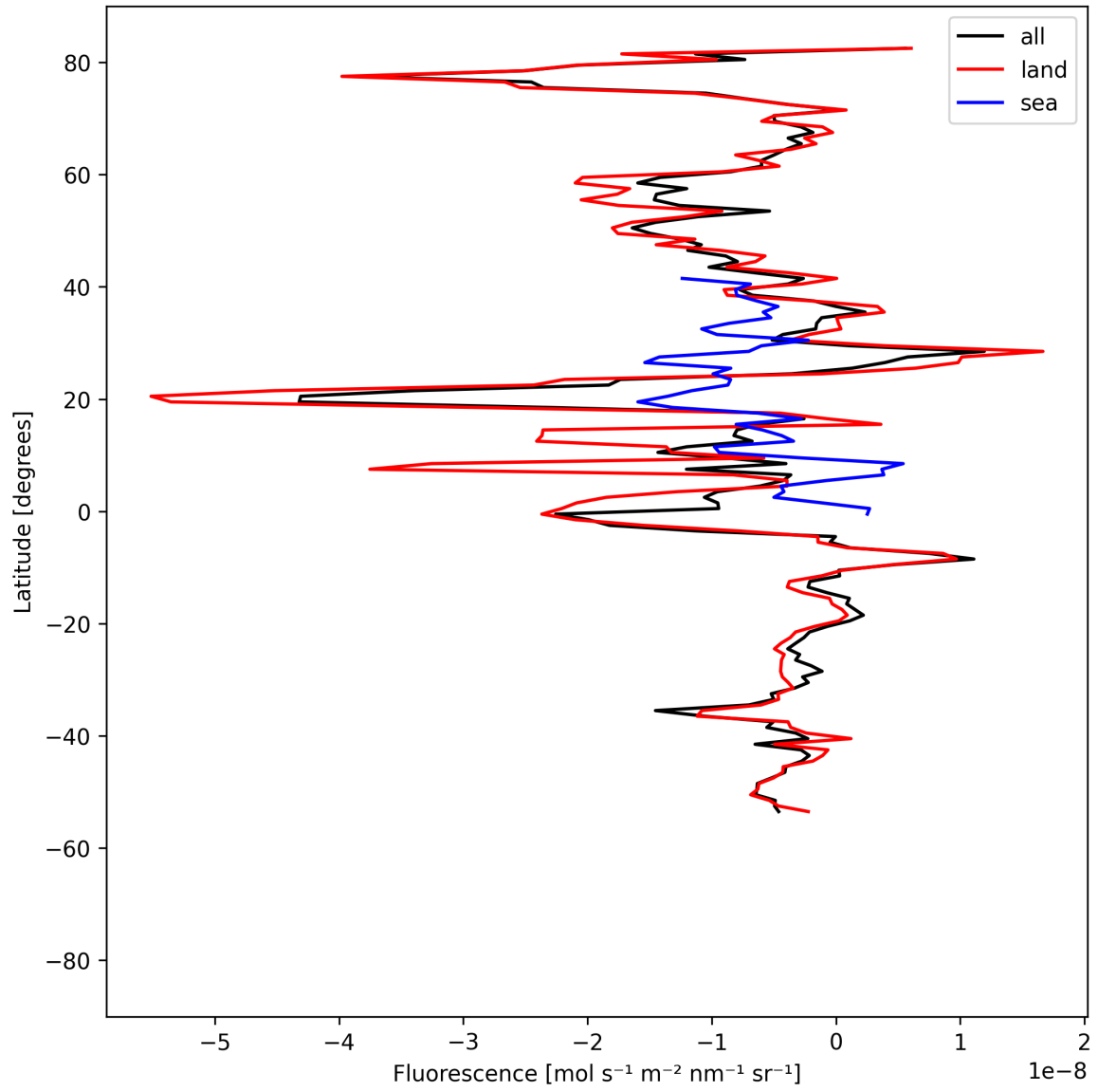
Figure 21: Zonal average of “Fluorescence” for 2025-08-12 to 2025-08-14.
