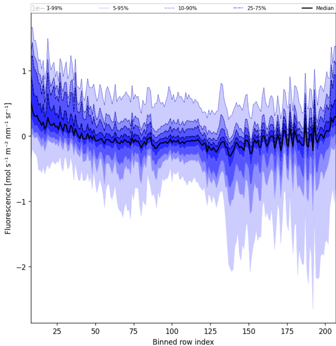
Figure 43: Along track statistics of “Fluorescence” for 2025-08-12 to 2025-08-14
