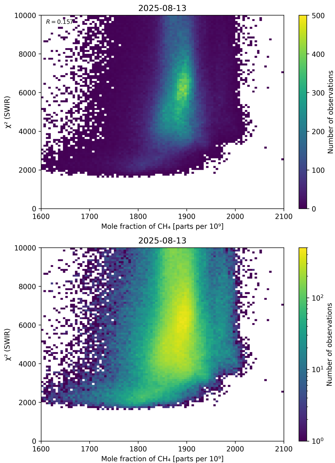
Figure 71: Scatter density plot of “Mole fraction of \text{CH}_4 ” against “ \chi^2 (SWIR)” for 2025-08-12 to 2025-08-14.
