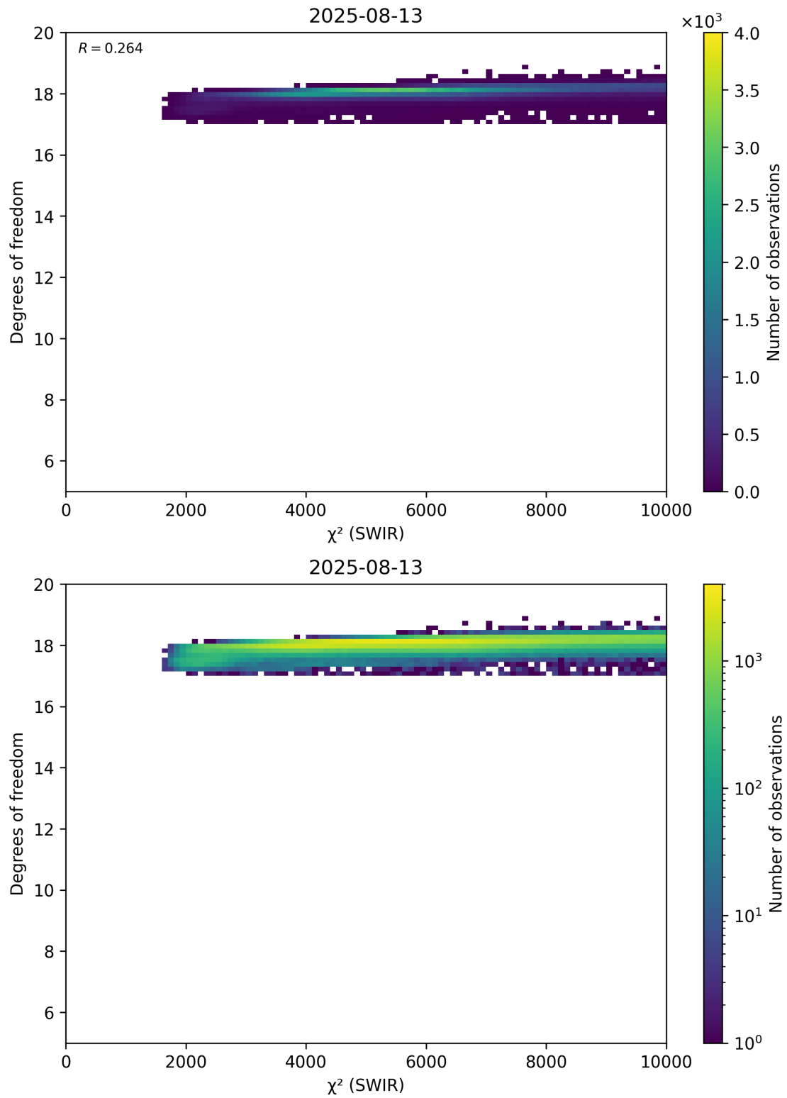
Figure 48: Scatter density plot of “ \chi^2 (SWIR)” against “Degrees of freedom” for 2025-08-12 to 2025-08-14.
