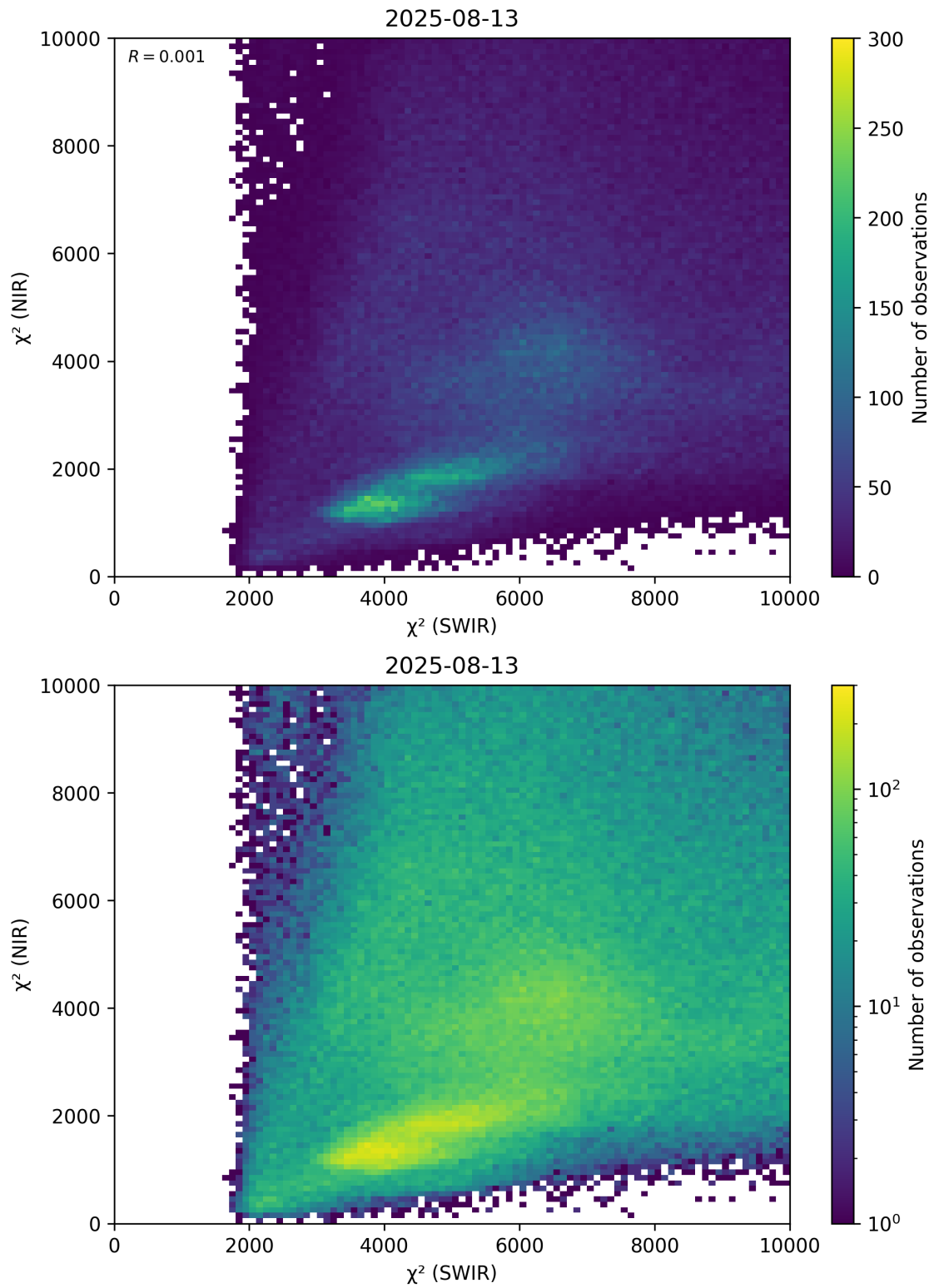
Figure 47: Scatter density plot of “ \chi^2 (SWIR)” against “ \chi^2 (NIR)” for 2025-08-12 to 2025-08-14.
