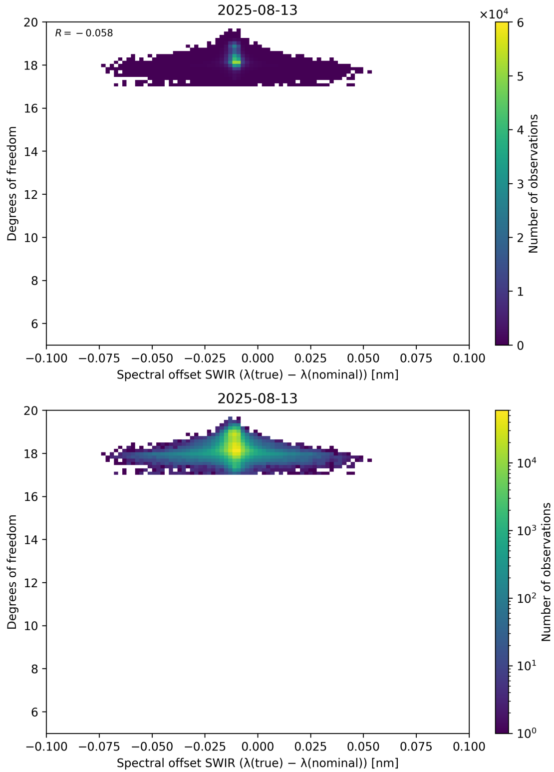
Figure 119: Scatter density plot of “Spectral offset SWIR ( \lambda_{\text{true}} - \lambda_{\text{nominal}} )” against “Degrees of freedom” for 2025-08-12 to 2025-08-14.
