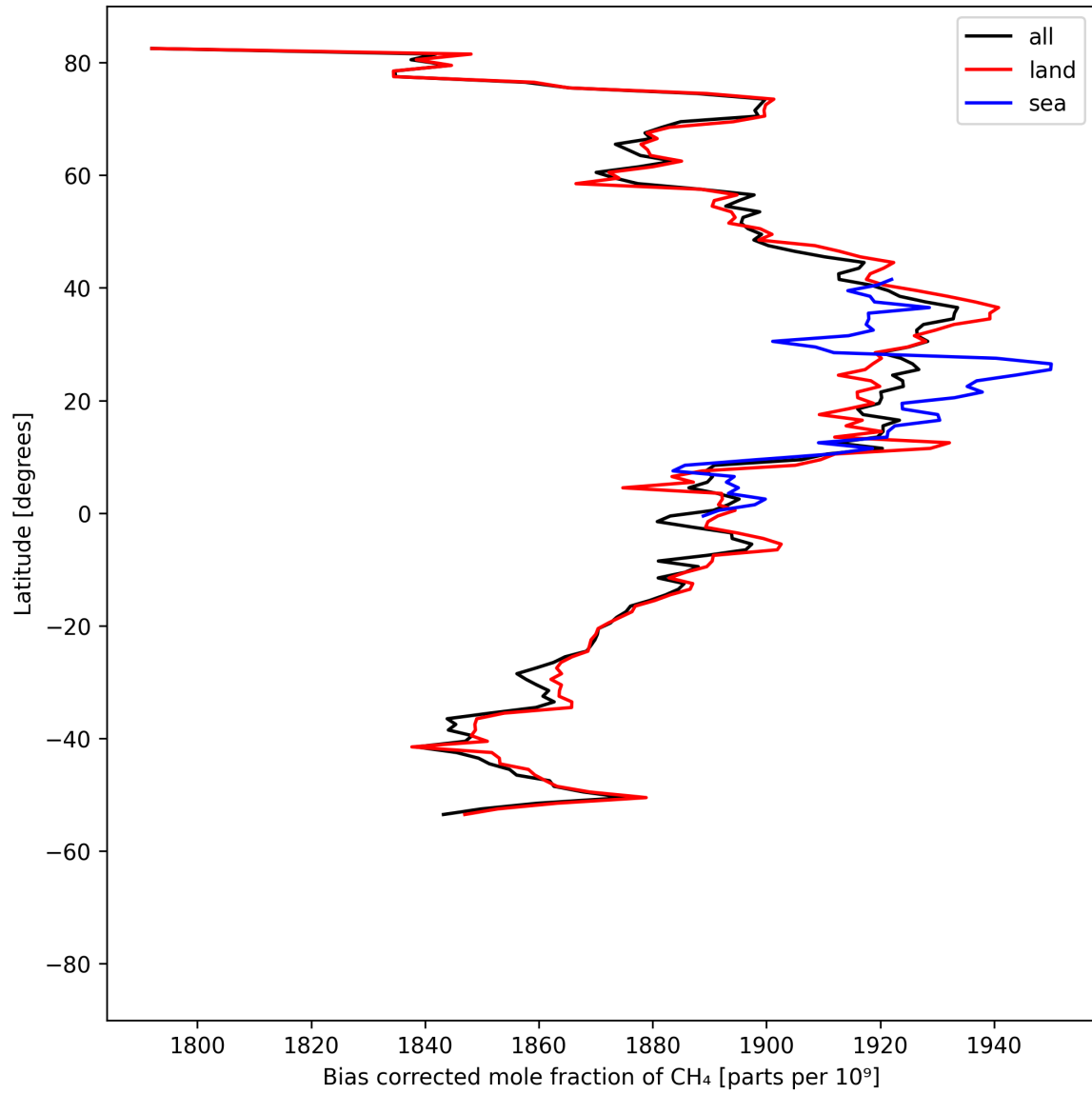
Figure 14: Zonal average of “Bias corrected mole fraction of \text{CH}_4 ” for 2025-08-12 to 2025-08-14.
