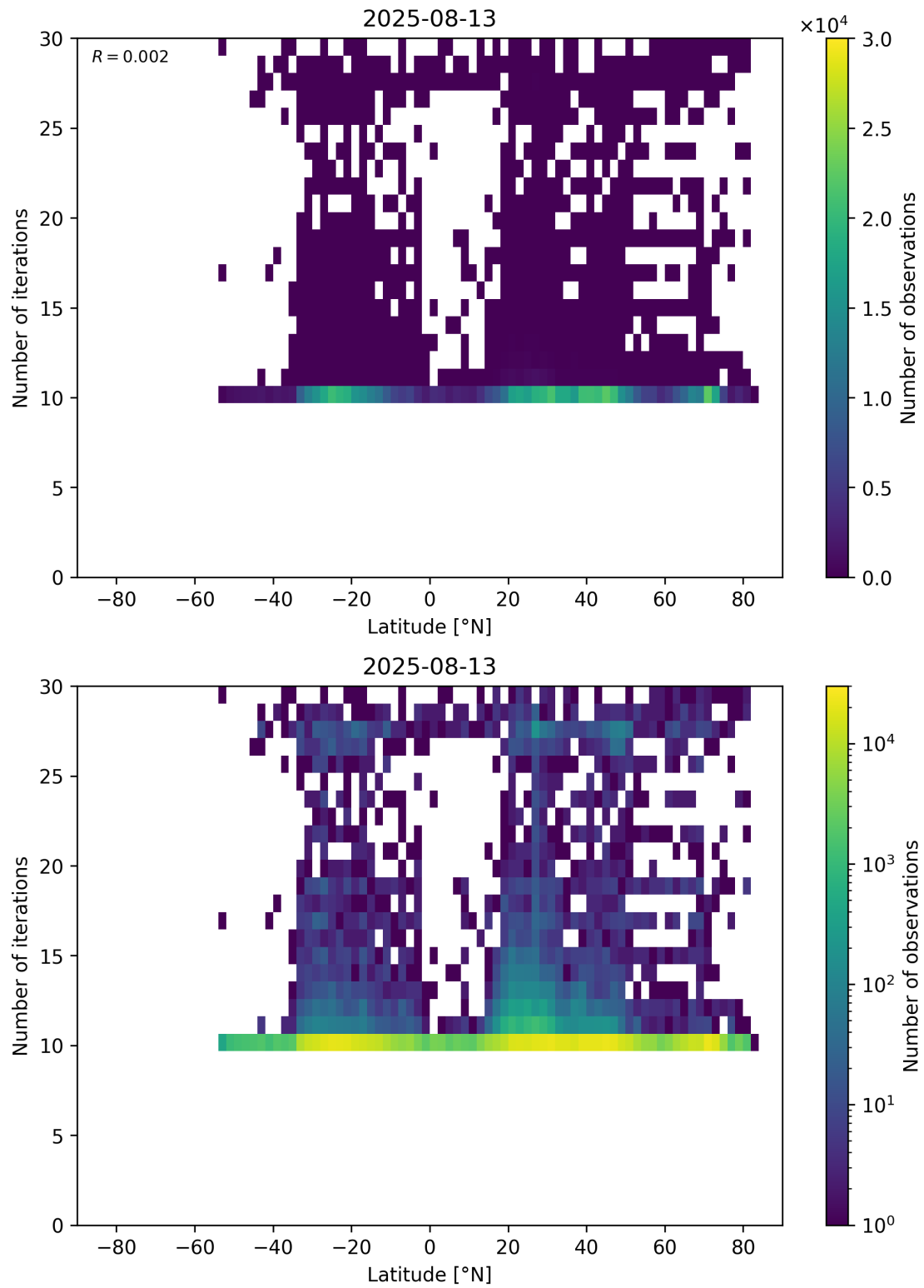
Figure 60: Scatter density plot of “Latitude” against “Number of iterations” for 2025-08-12 to 2025-08-14.
