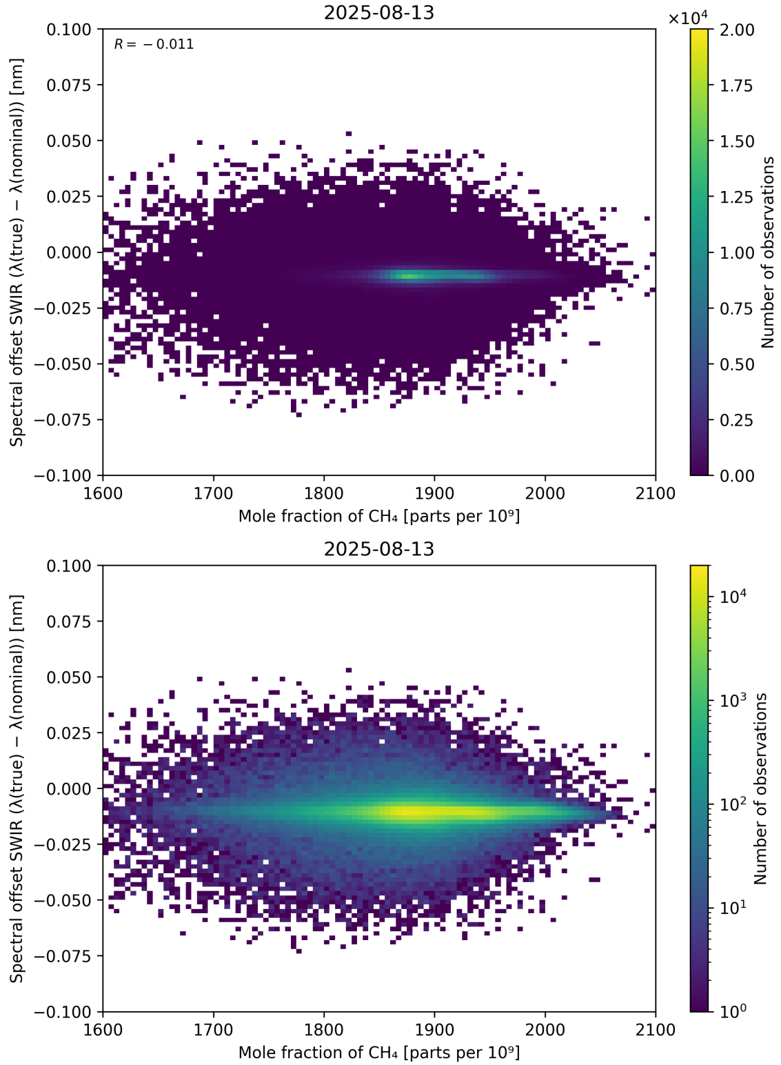
Figure 86: Scatter density plot of “Mole fraction of CH 4 ” against “Spectral offset SWIR ( \lambda_{\text{true}} - \lambda_{\text{nominal}} )” for 2025-08-12 to 2025-08-14.
