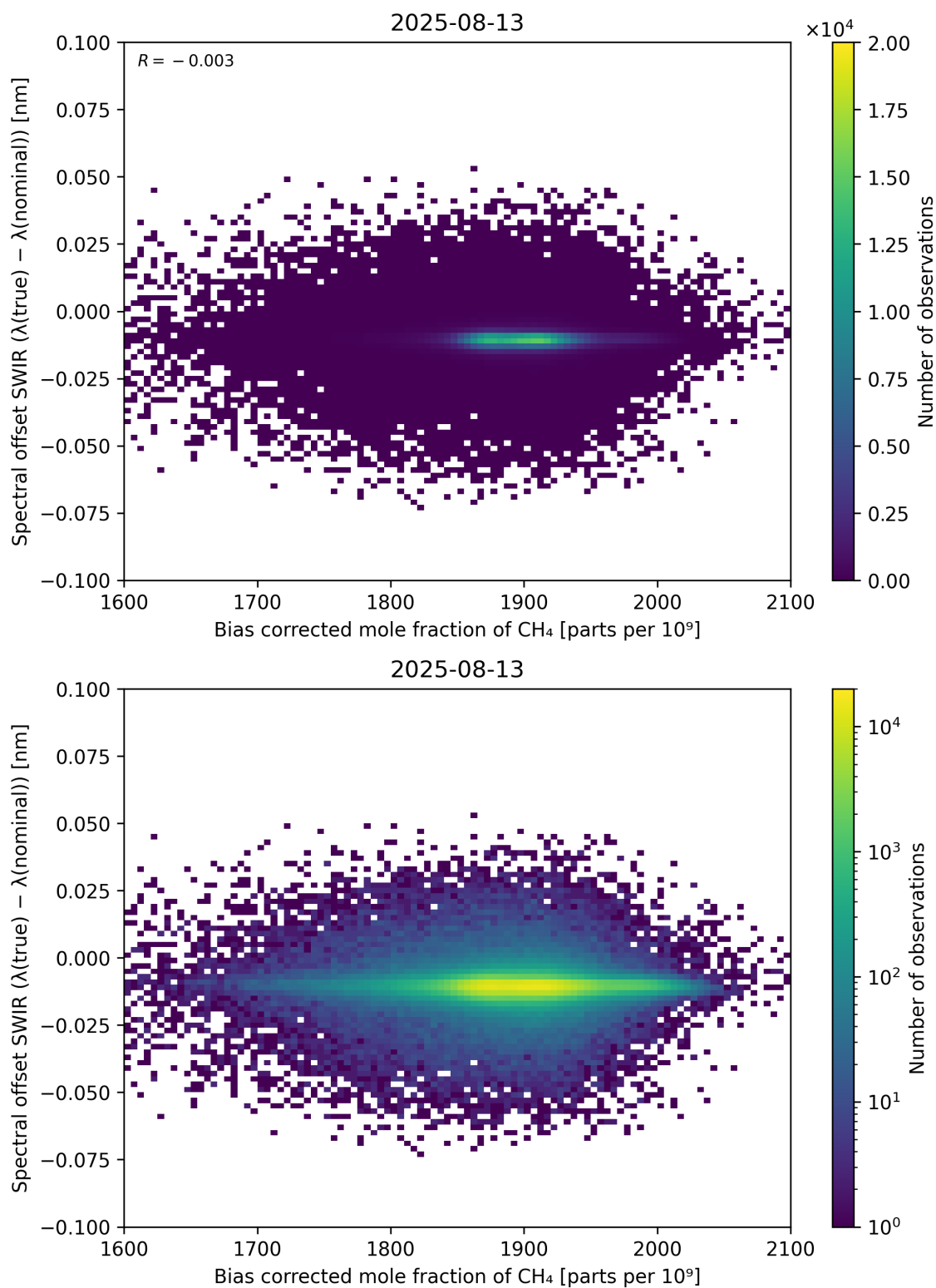
Figure 69: Scatter density plot of “Bias corrected mole fraction of \text{CH}_4 ” against “Spectral offset SWIR ( \lambda_{\text{true}} - \lambda_{\text{nominal}} )” for 2025-08-12 to 2025-08-14.
