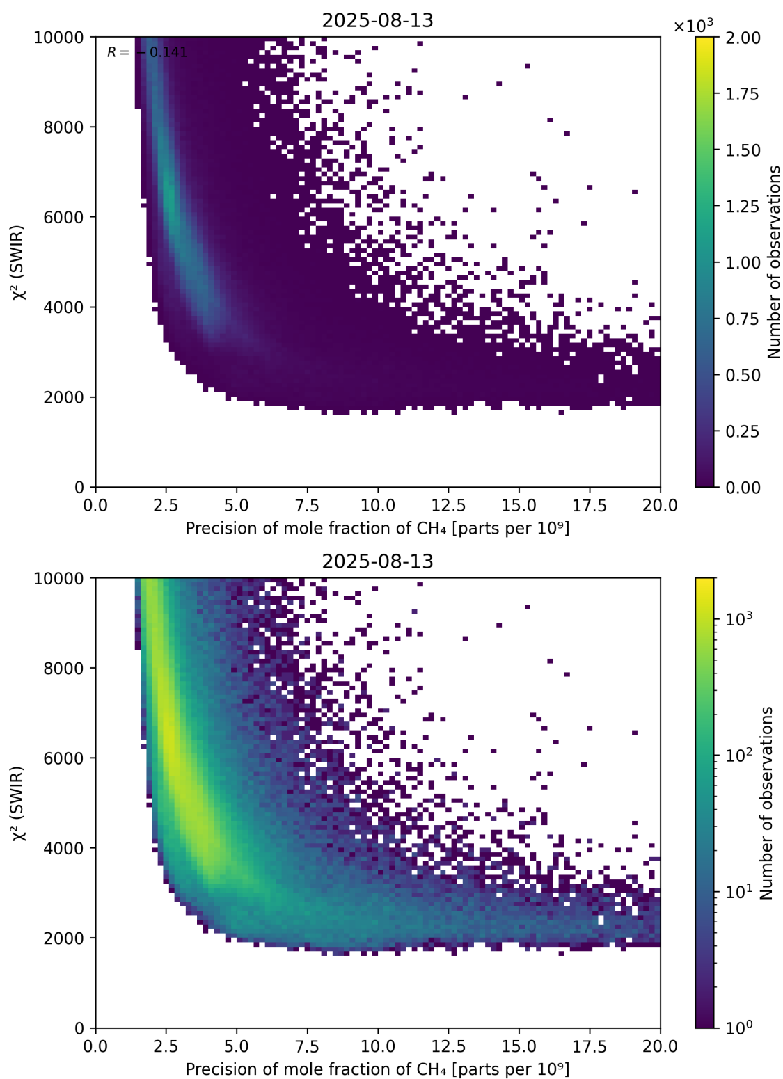
Figure 79: Scatter density plot of “Precision of mole fraction of CH 4 ” against “ \chi^2 (SWIR)” for 2025-08-12 to 2025-08-14.
