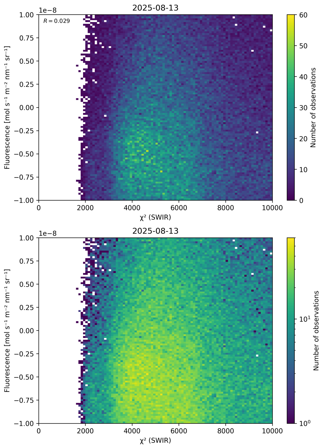
Figure 49: Scatter density plot of “ \chi^2 (SWIR)” against “Fluorescence” for 2025-08-12 to 2025-08-14.
