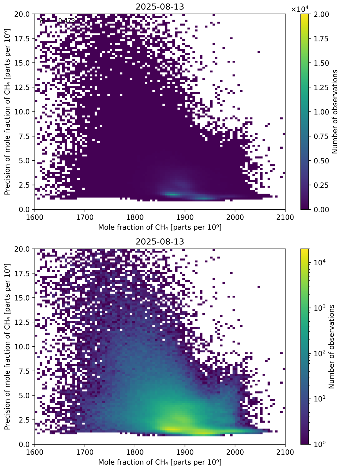
Figure 75: Scatter density plot of “Mole fraction of CH 4 ” against “Precision of mole fraction of CH 4 ” for 2025-08-12 to 2025-08-14.
