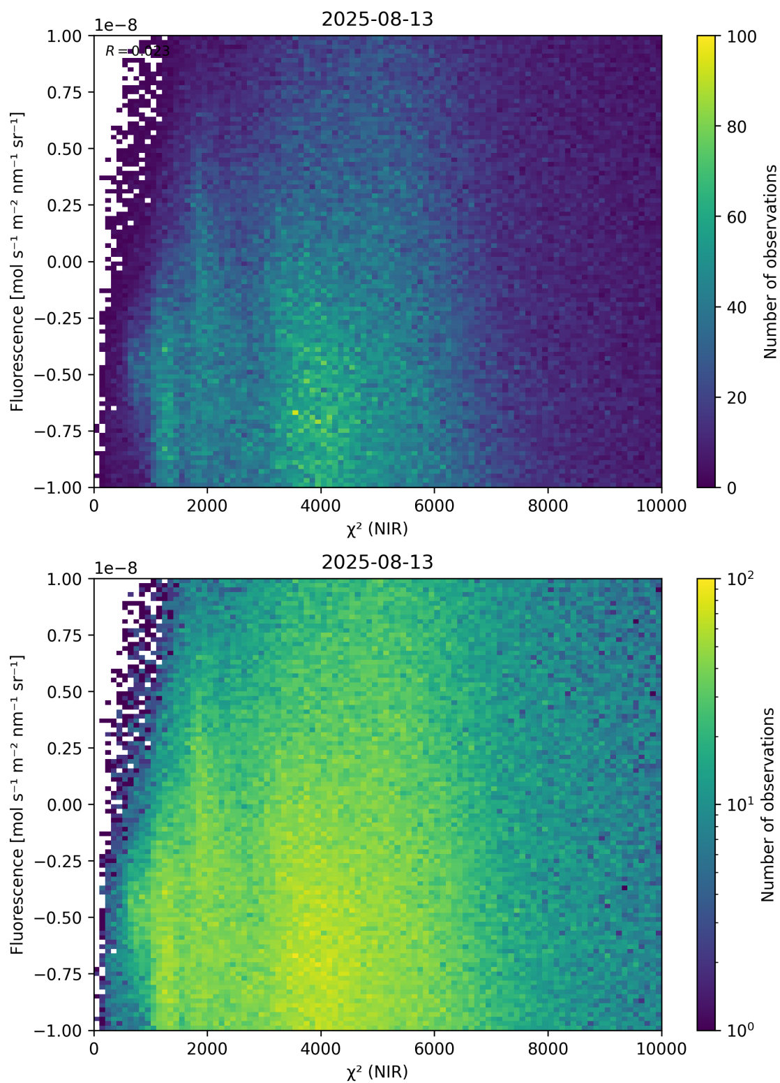
Figure 45: Scatter density plot of “ \chi^2 (NIR)” against “Fluorescence” for 2025-08-12 to 2025-08-14.
