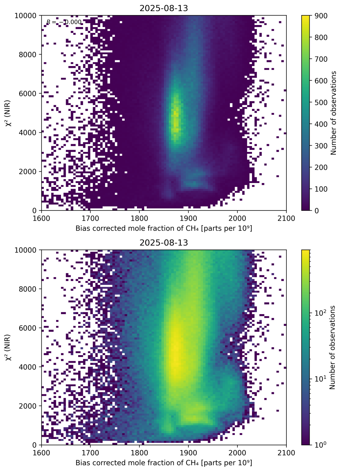
Figure 63: Scatter density plot of “Bias corrected mole fraction of CH 4 ” against “ \chi^2 (NIR)” for 2025-08-12 to 2025-08-14.
