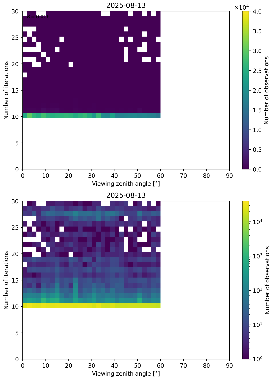
Figure 113: Scatter density plot of “Viewing zenith angle” against “Number of iterations” for 2025-08-12 to 2025-08-14.
