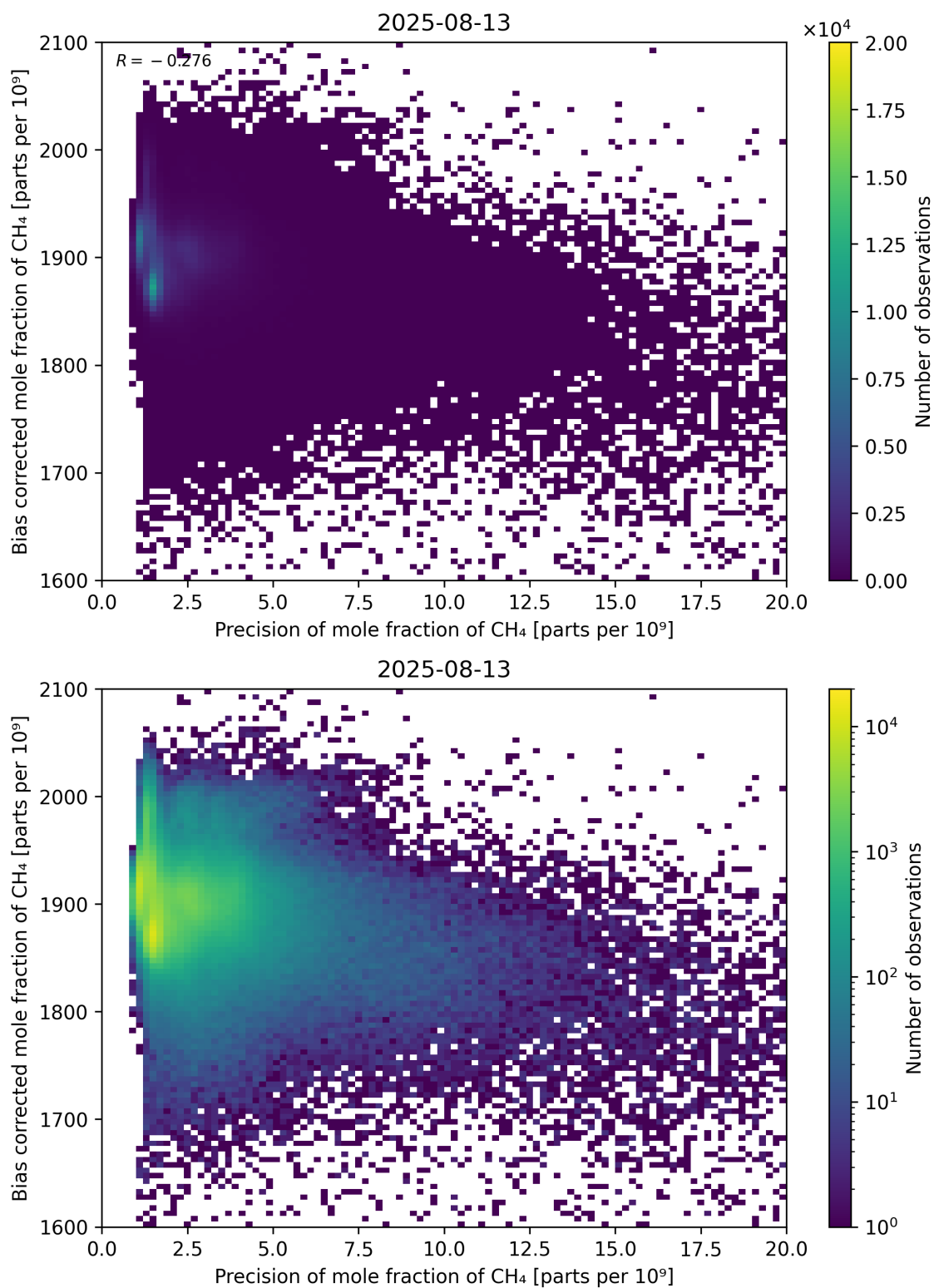
Figure 82: Scatter density plot of “Precision of mole fraction of CH 4 ” against “Bias corrected mole fraction of CH 4 ” for 2025-08-12 to 2025-08-14.
