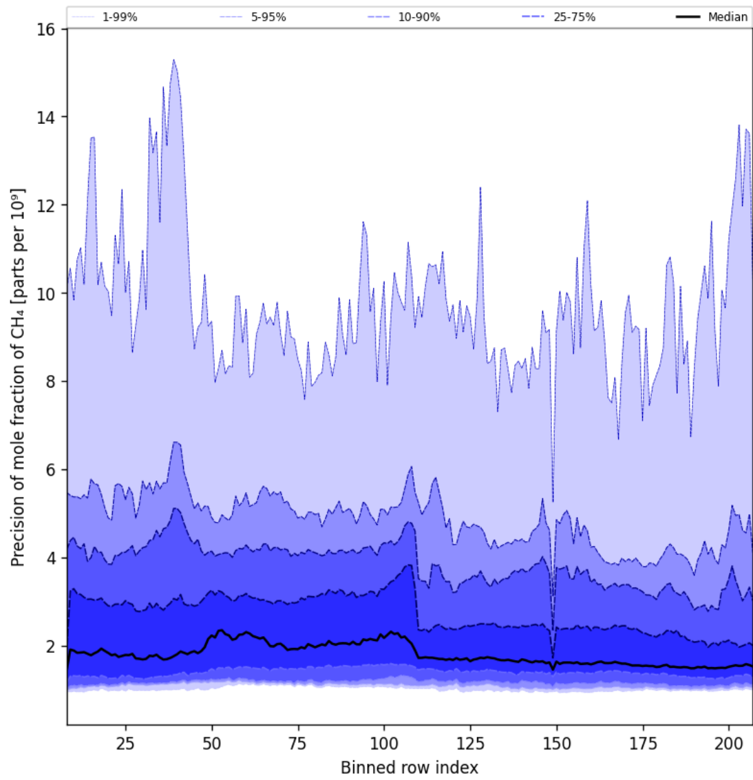
Figure 35: Along track statistics of “Precision of mole fraction of CH 4 ” for 2025-08-12 to 2025-08-14
