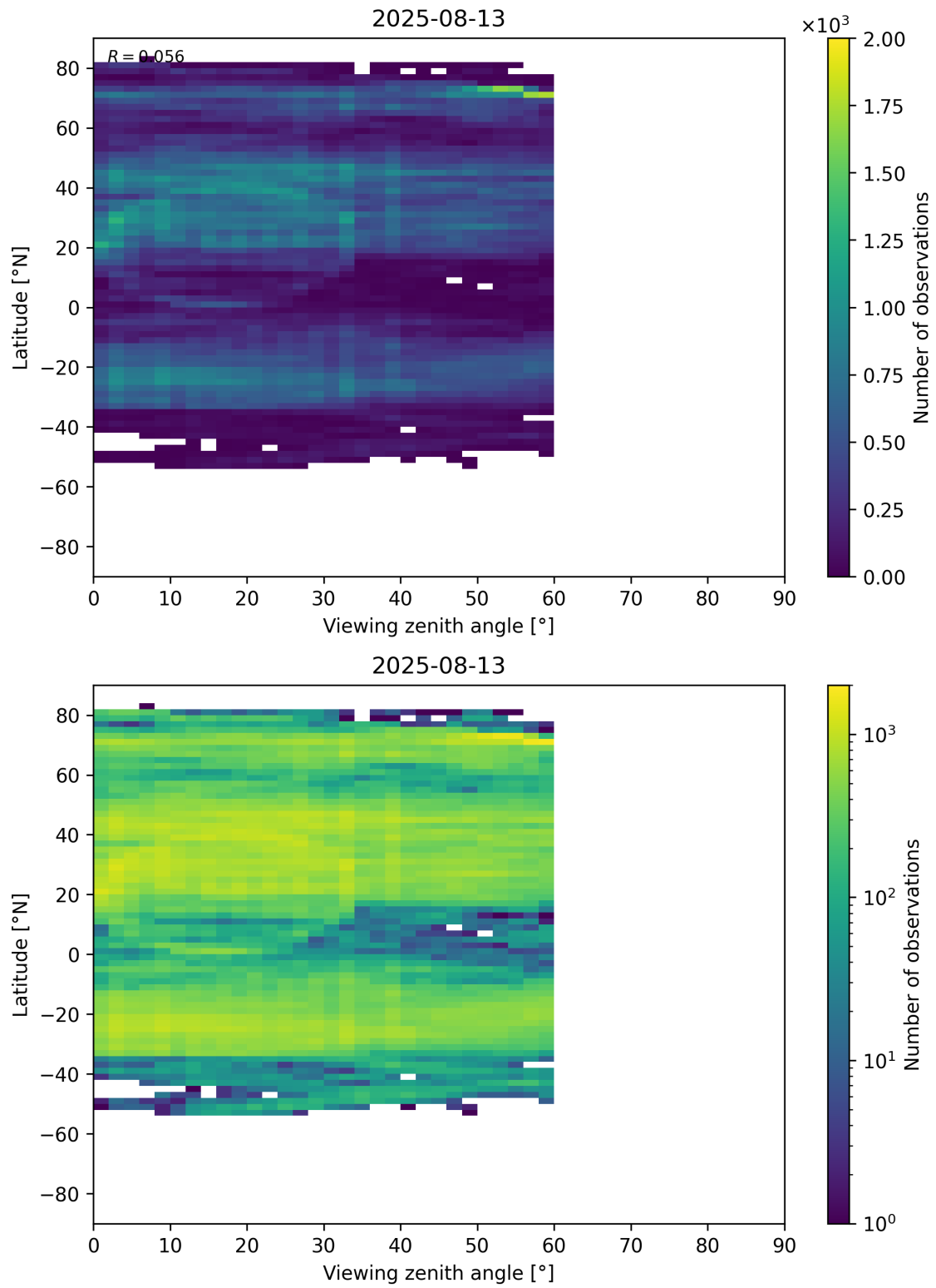
Figure 109: Scatter density plot of “Viewing zenith angle” against “Latitude” for 2025-08-12 to 2025-08-14.
