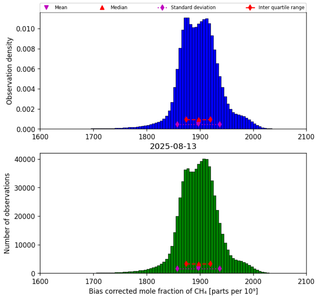
Figure 25: Histogram of “Bias corrected mole fraction of CH 4 ” for 2025-08-12 to 2025-08-14
