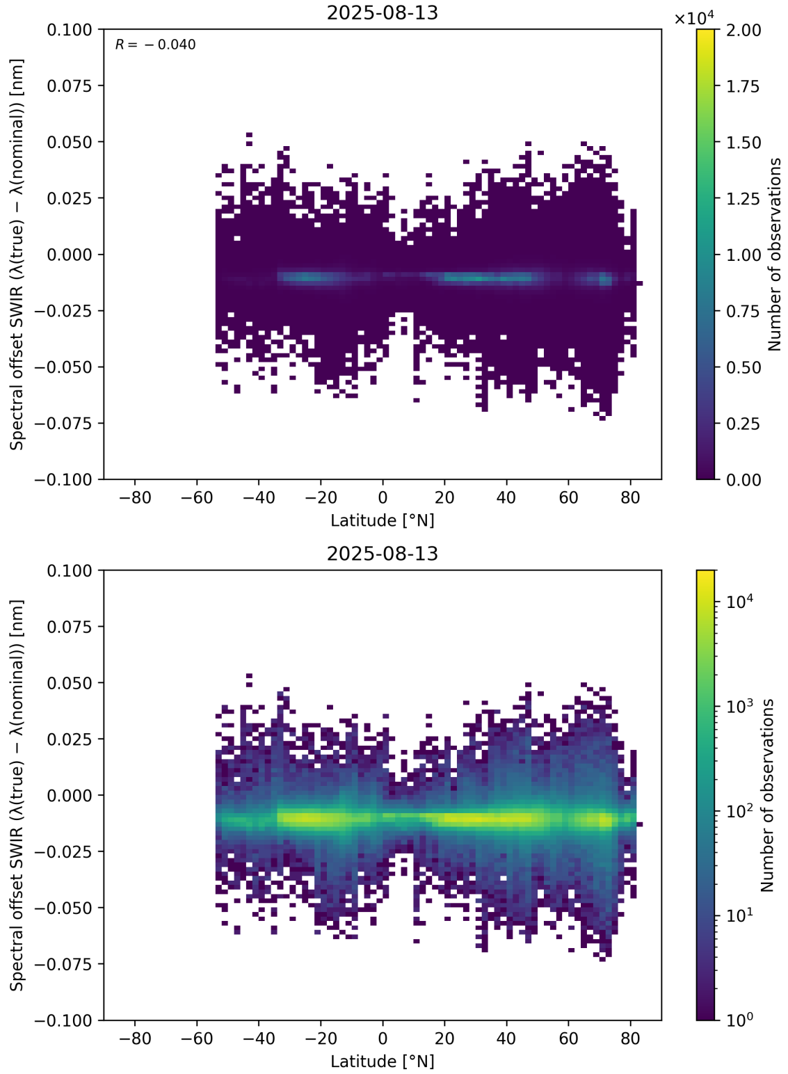
Figure 62: Scatter density plot of “Latitude” against “Spectral offset SWIR ( \lambda_{\text{true}} - \lambda_{\text{nominal}} )” for 2025-08-12 to 2025-08-14.
