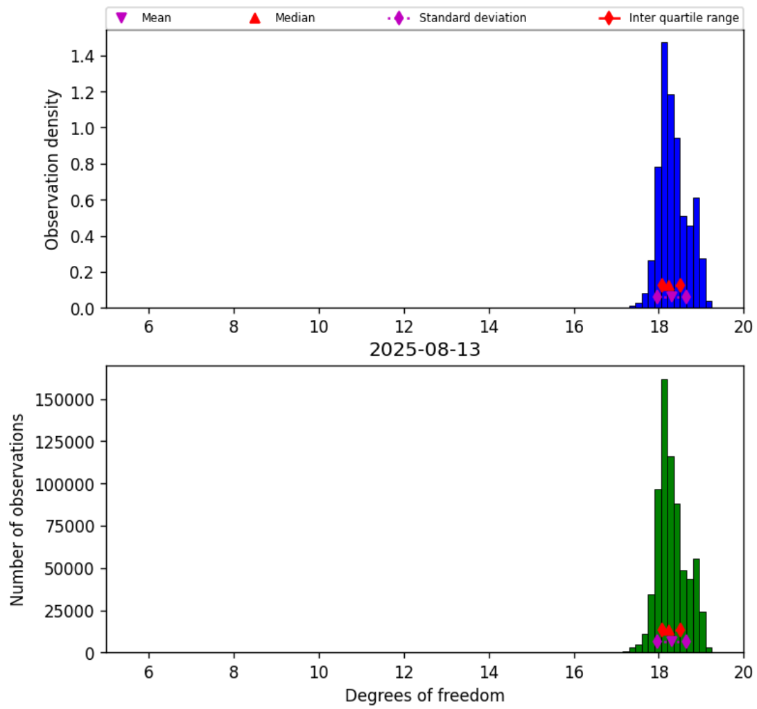
Figure 30: Histogram of “Degrees of freedom” for 2025-08-12 to 2025-08-14
