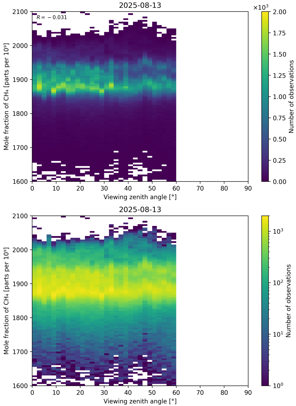
Figure 110: Scatter density plot of “Viewing zenith angle” against “Mole fraction of CH 4 ” for 2025-08-12 to 2025-08-14.
