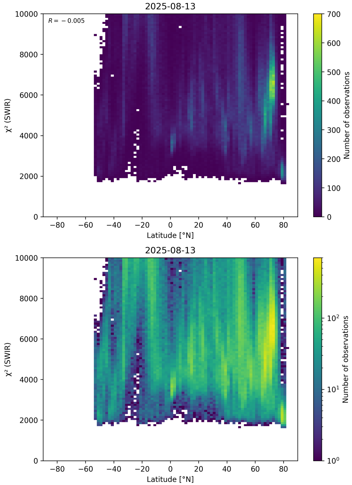
Figure 54: Scatter density plot of “Latitude” against “ \chi^2 (SWIR)” for 2025-08-12 to 2025-08-14.
