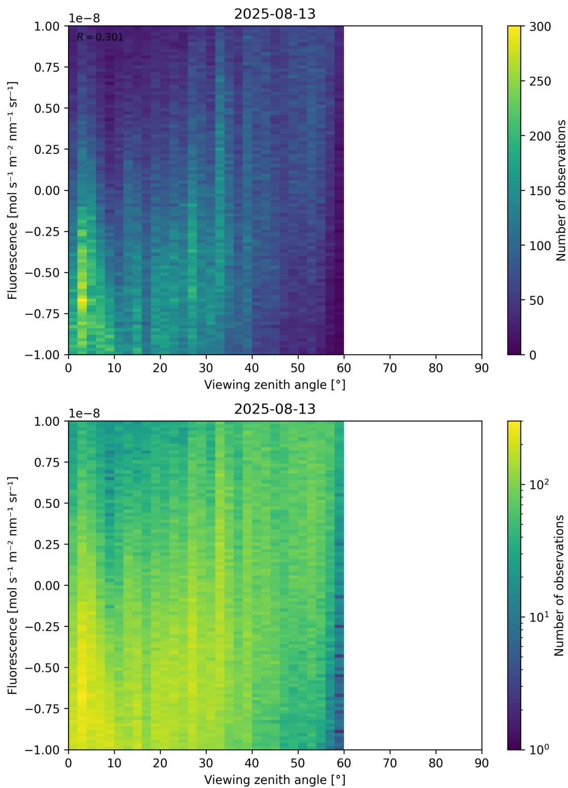
Figure 108: Scatter density plot of “Viewing zenith angle” against “Fluorescence” for 2025-08-12 to 2025-08-14.
