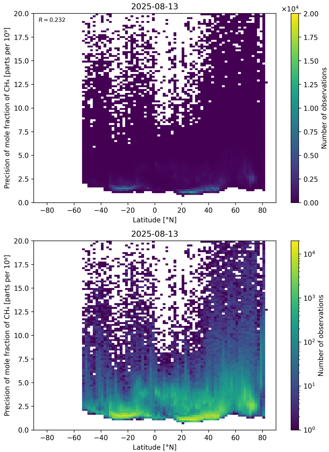
Figure 59: Scatter density plot of “Latitude” against “Precision of mole fraction of \text{CH}_4 ” for 2025-08-12 to 2025-08-14.
