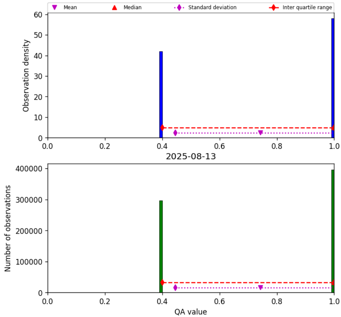
Figure 22: Histogram of “QA value” for 2025-08-12 to 2025-08-14
