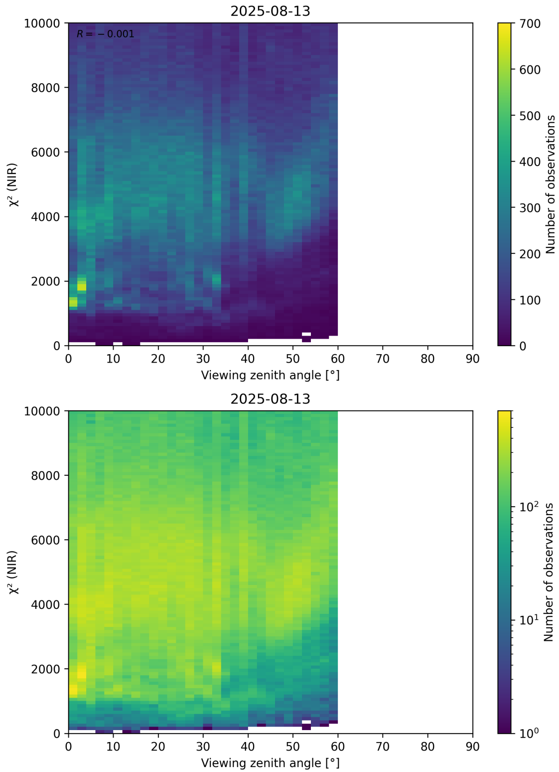
Figure 105: Scatter density plot of “Viewing zenith angle” against “ \chi^2 (NIR)” for 2025-08-12 to 2025-08-14.
