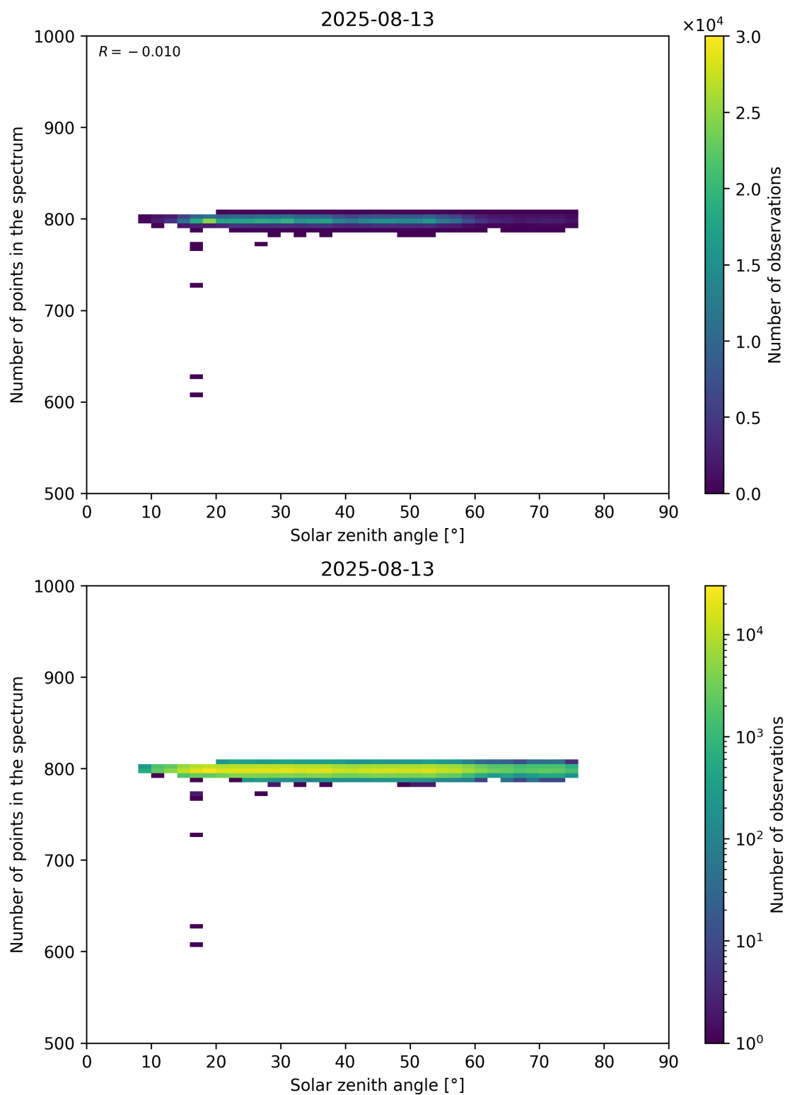
Figure 103: Scatter density plot of “Solar zenith angle” against “Number of points in the spectrum” for 2025-08-12 to 2025-08-14.
