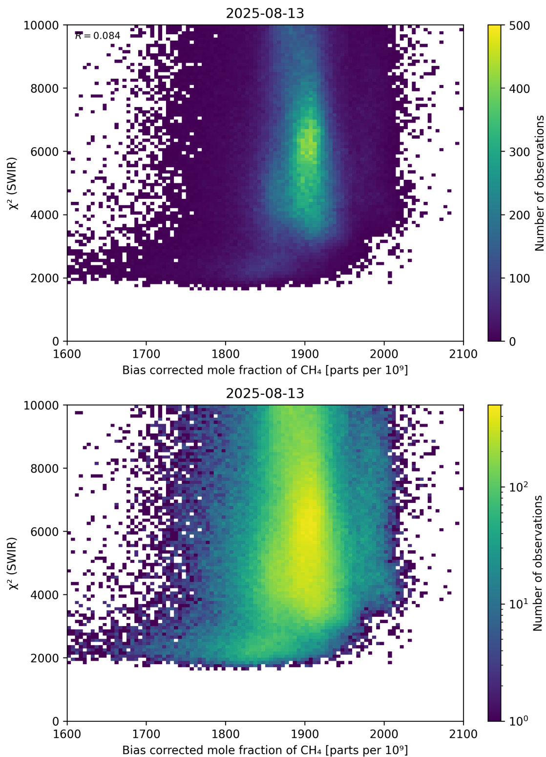
Figure 64: Scatter density plot of “Bias corrected mole fraction of \text{CH}_4 ” against “ \chi^2 (SWIR)” for 2025-08-12 to 2025-08-14.
