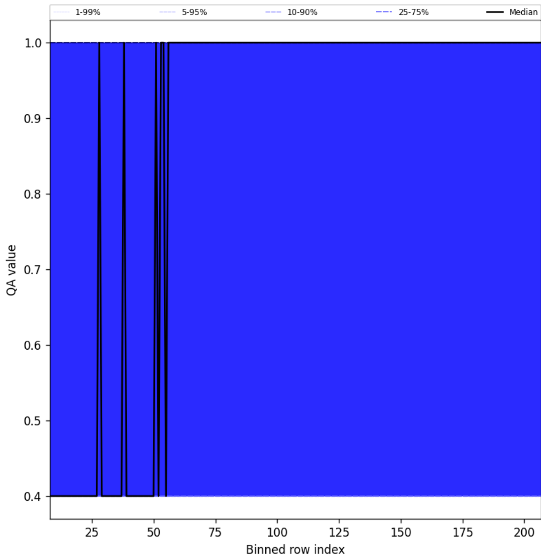
Figure 33: Along track statistics of “QA value” for 2025-08-12 to 2025-08-14
