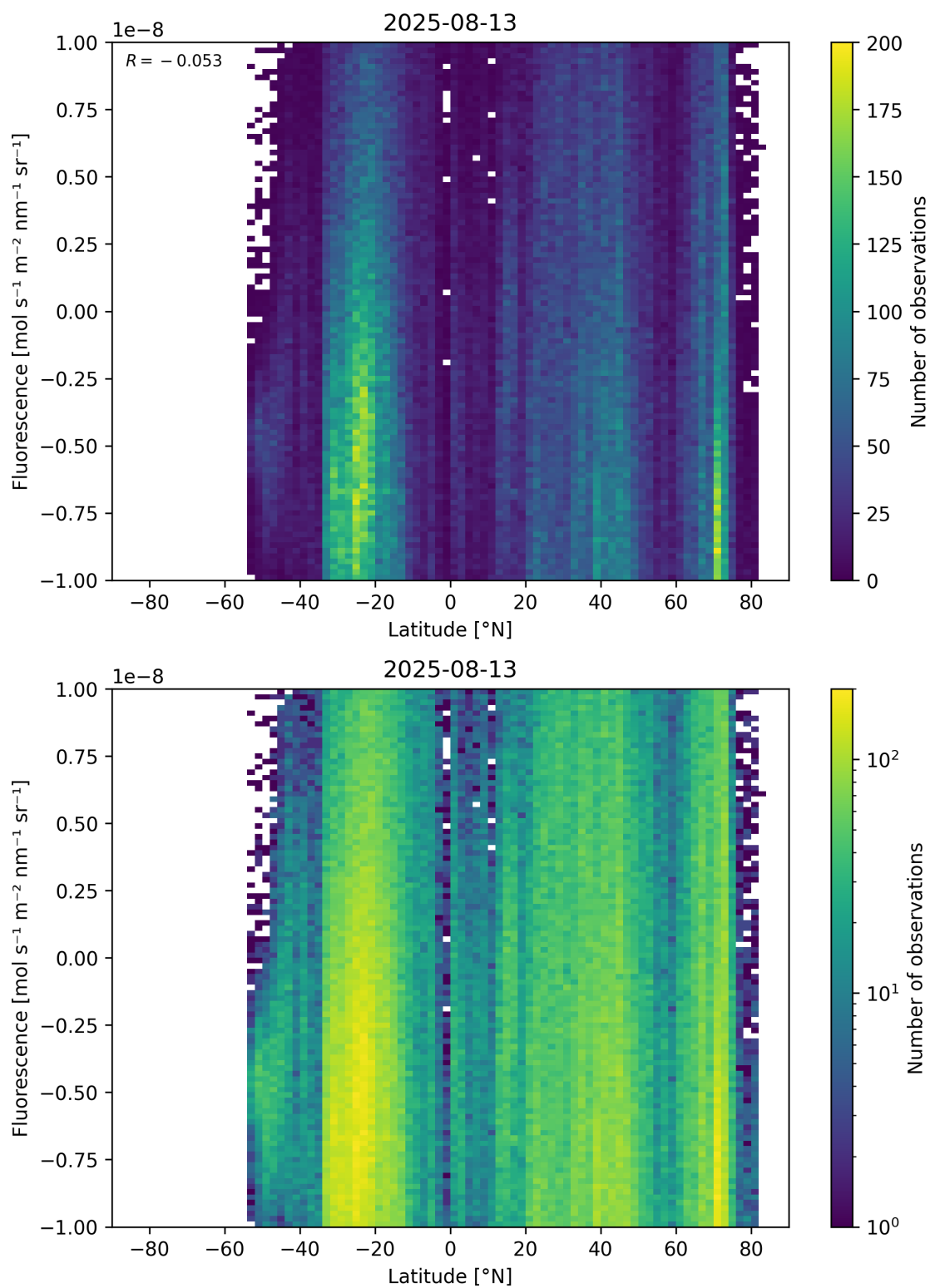
Figure 56: Scatter density plot of “Latitude” against “Fluorescence” for 2025-08-12 to 2025-08-14.
