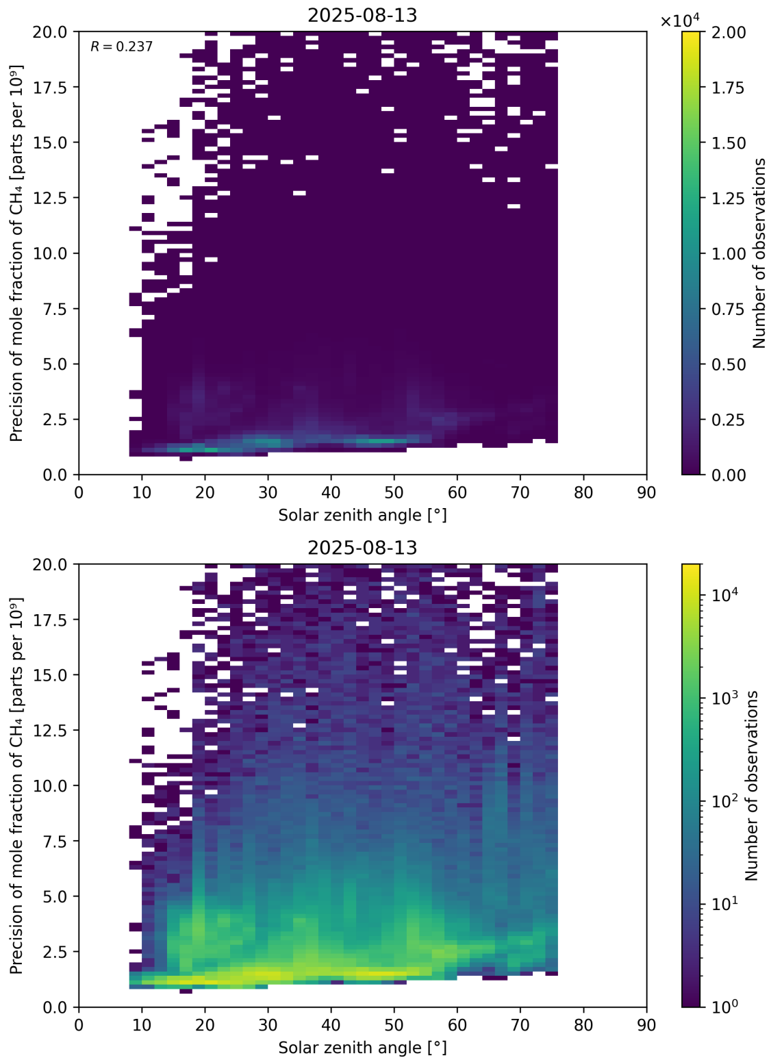
Figure 101: Scatter density plot of “Solar zenith angle” against “Precision of mole fraction of CH 4 ” for 2025-08-12 to 2025-08-14.
