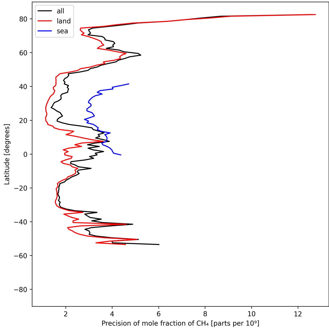
Figure 13: Zonal average of “Precision of mole fraction of CH 4 ” for 2025-08-12 to 2025-08-14.
