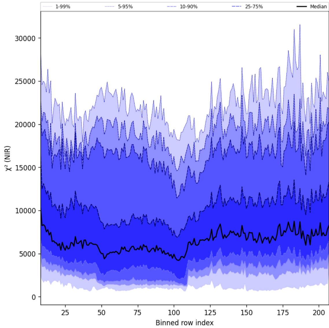
Figure 40: Along track statistics of “ \chi^2 (NIR)” for 2025-08-12 to 2025-08-14
