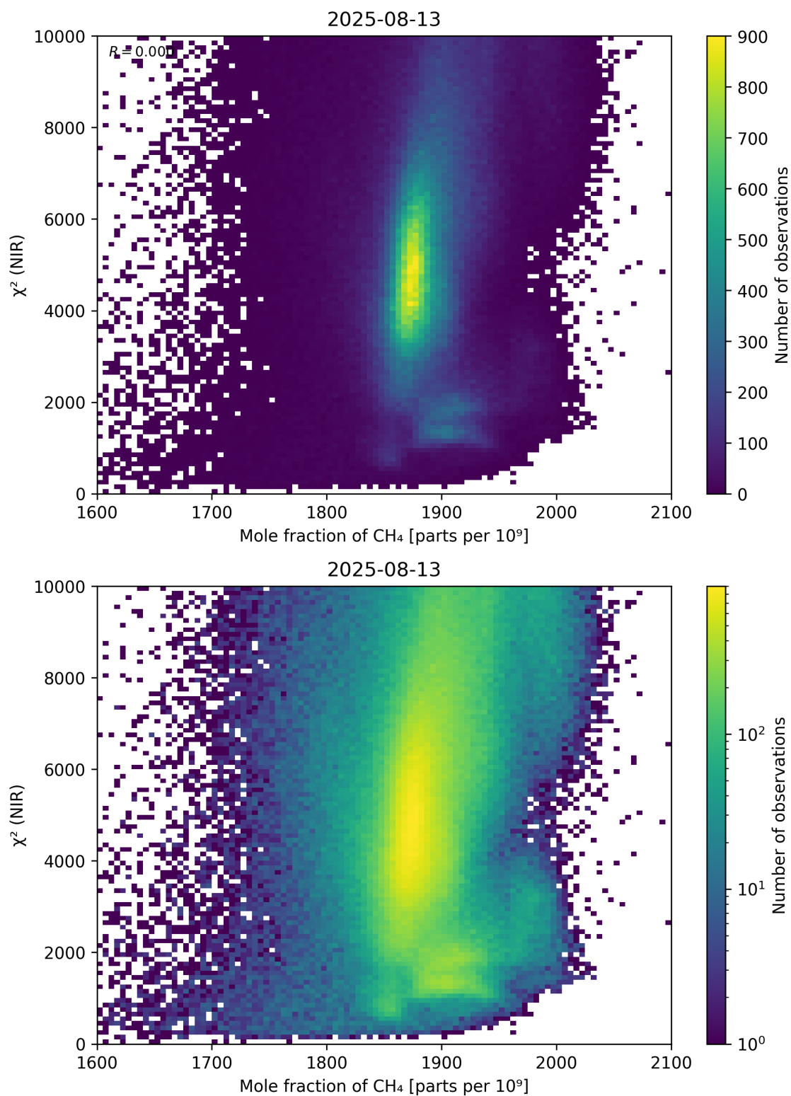
Figure 70: Scatter density plot of “Mole fraction of \text{CH}_4 ” against “ \chi^2 (NIR)” for 2025-08-12 to 2025-08-14.
