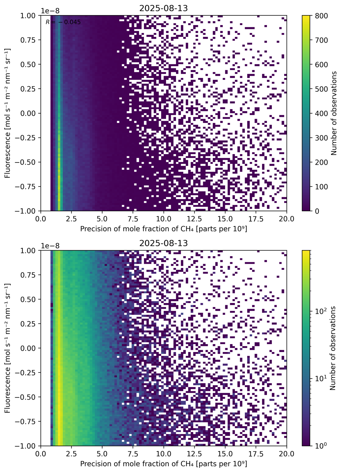
Figure 81: Scatter density plot of “Precision of mole fraction of \text{CH}_4 ” against “Fluorescence” for 2025-08-12 to 2025-08-14.
