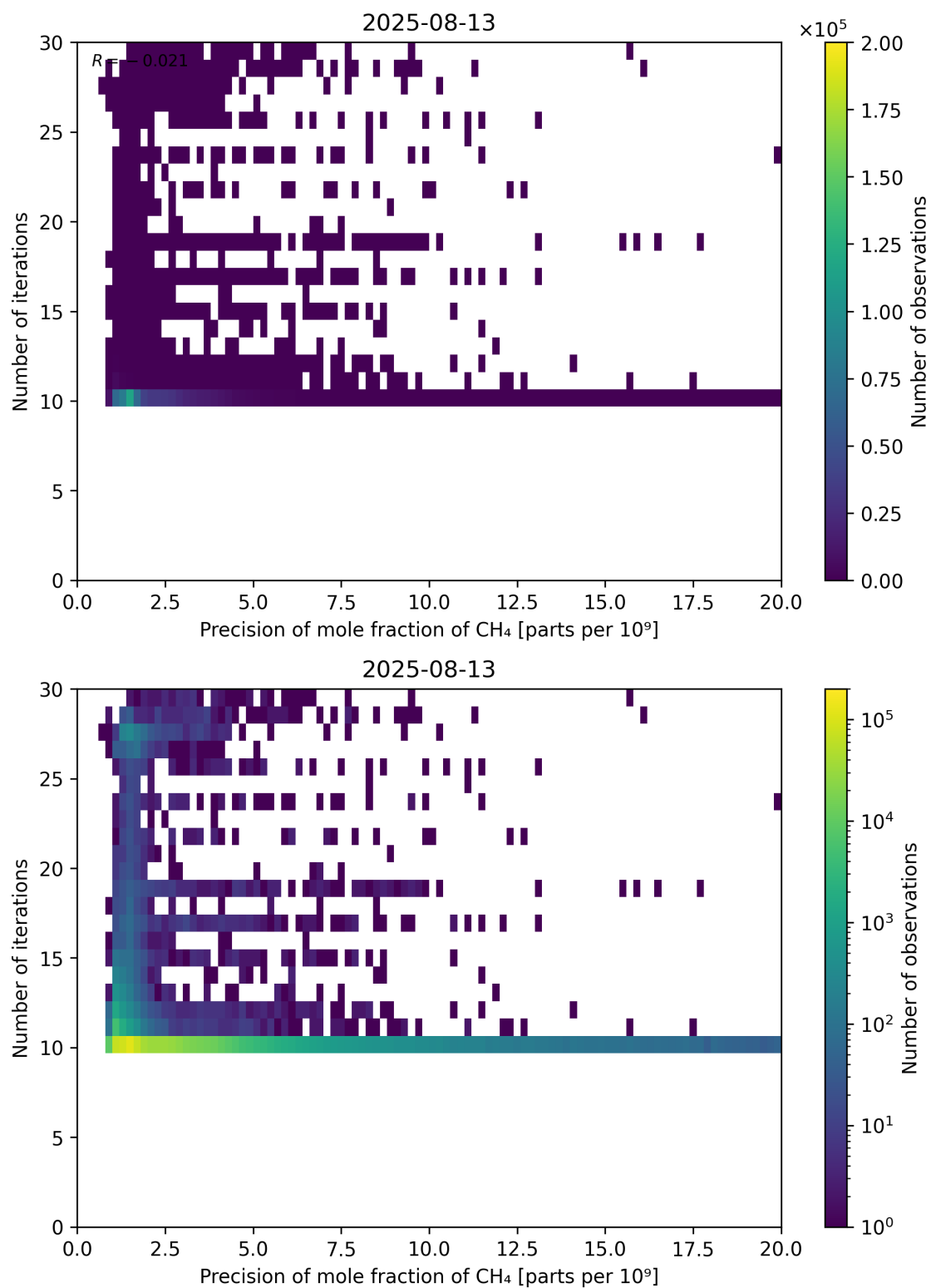
Figure 83: Scatter density plot of “Precision of mole fraction of CH 4 ” against “Number of iterations” for 2025-08-12 to 2025-08-14.
