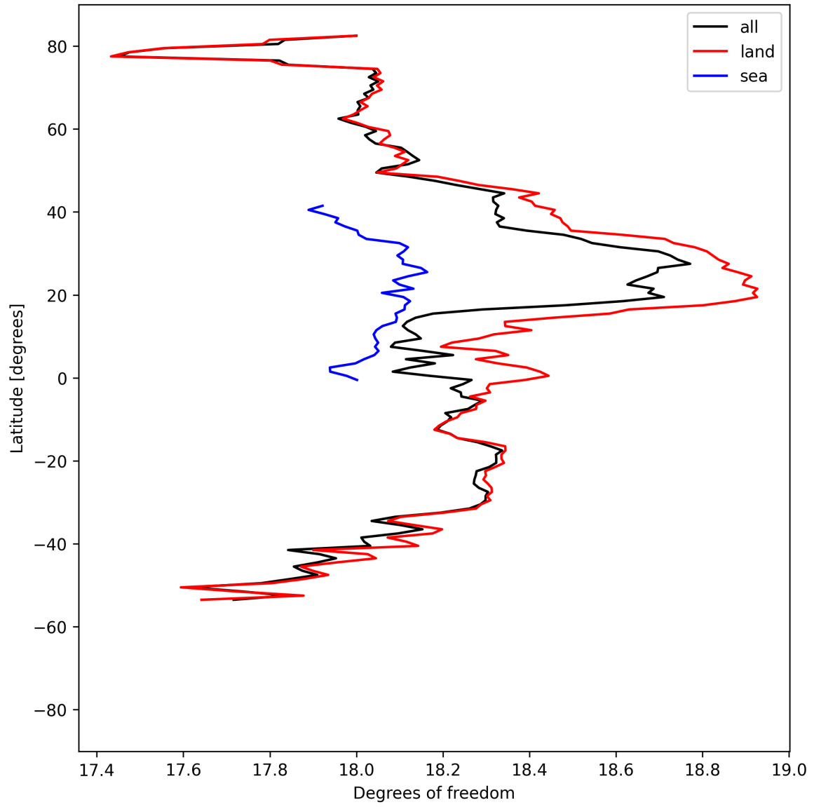
Figure 19: Zonal average of “Degrees of freedom” for 2025-08-12 to 2025-08-14.
