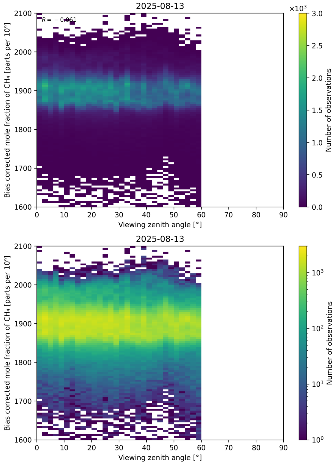
Figure 111: Scatter density plot of “Viewing zenith angle” against “Bias corrected mole fraction of CH 4 ” for 2025-08-12 to 2025-08-14.
