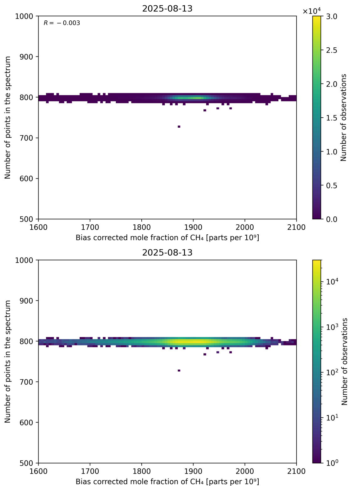
Figure 68: Scatter density plot of “Bias corrected mole fraction of CH 4 ” against “Number of points in the spectrum” for 2025-08-12 to 2025-08-14.
