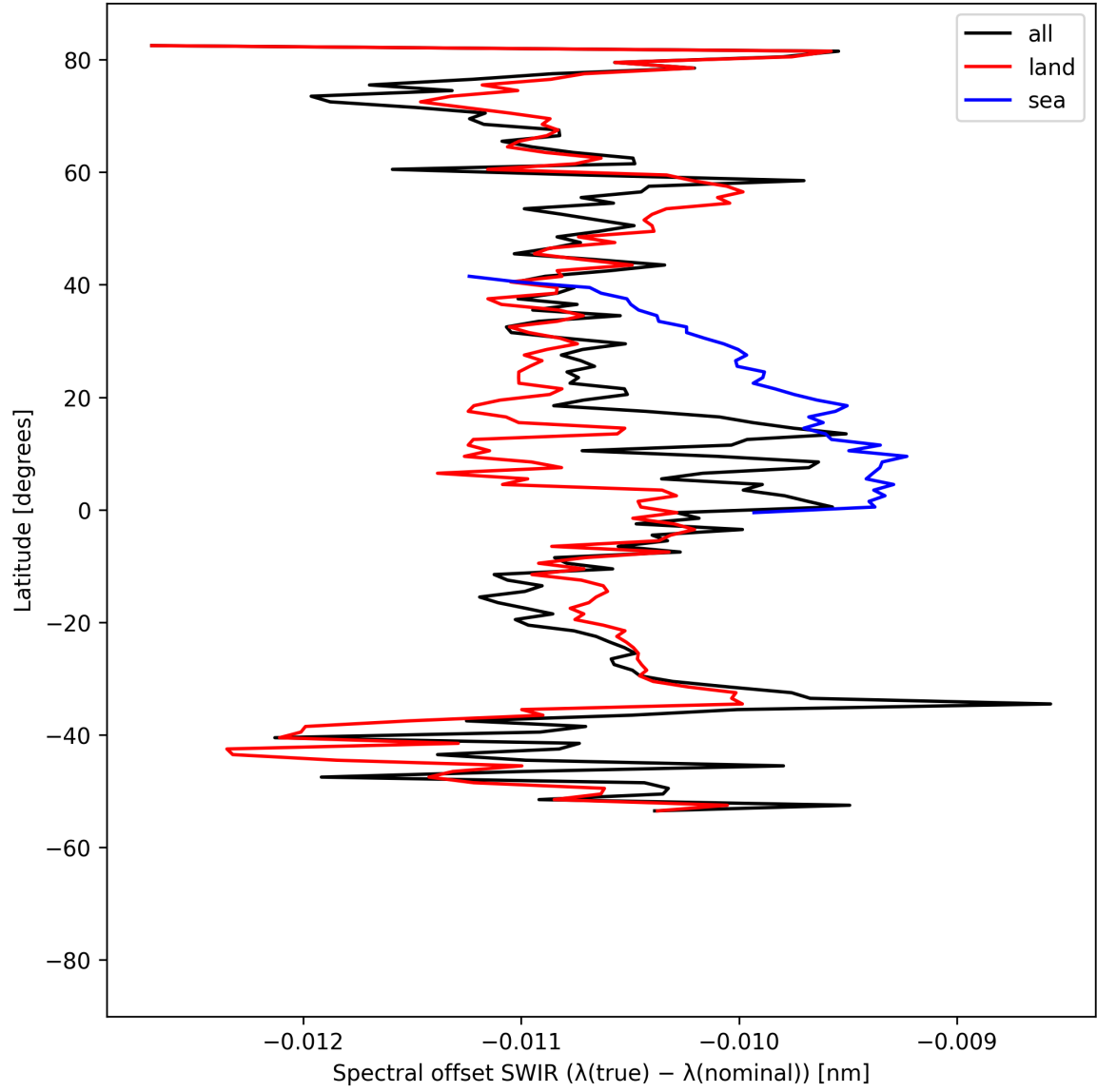
Figure 16: Zonal average of “Spectral offset SWIR ( \lambda_{\text{true}} - \lambda_{\text{nominal}} )” for 2025-08-12 to 2025-08-14.
