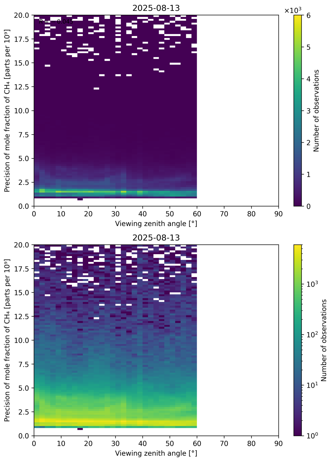
Figure 112: Scatter density plot of “Viewing zenith angle” against “Precision of mole fraction of CH 4 ” for 2025-08-12 to 2025-08-14.
