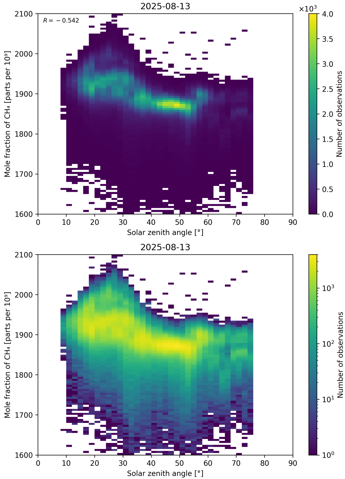
Figure 99: Scatter density plot of “Solar zenith angle” against “Mole fraction of \text{CH}_4 ” for 2025-08-12 to 2025-08-14.
