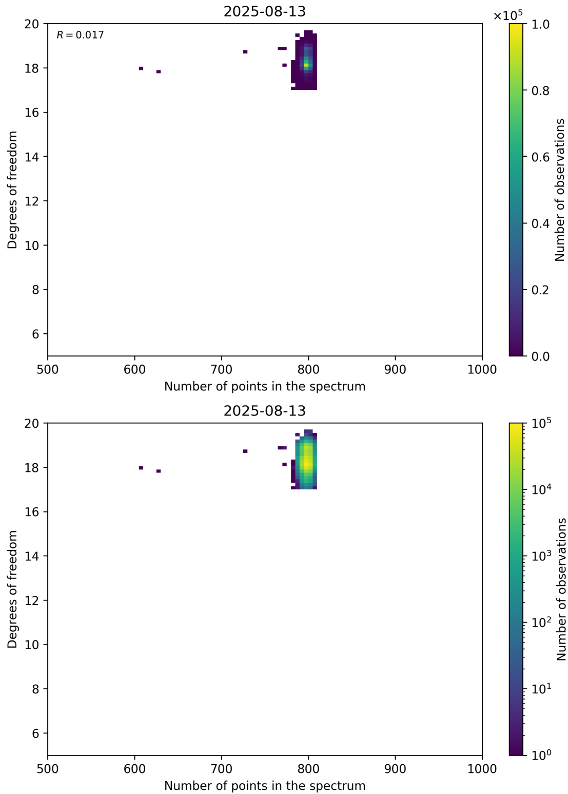
Figure 90: Scatter density plot of “Number of points in the spectrum” against “Degrees of freedom” for 2025-08-12 to 2025-08-14.
