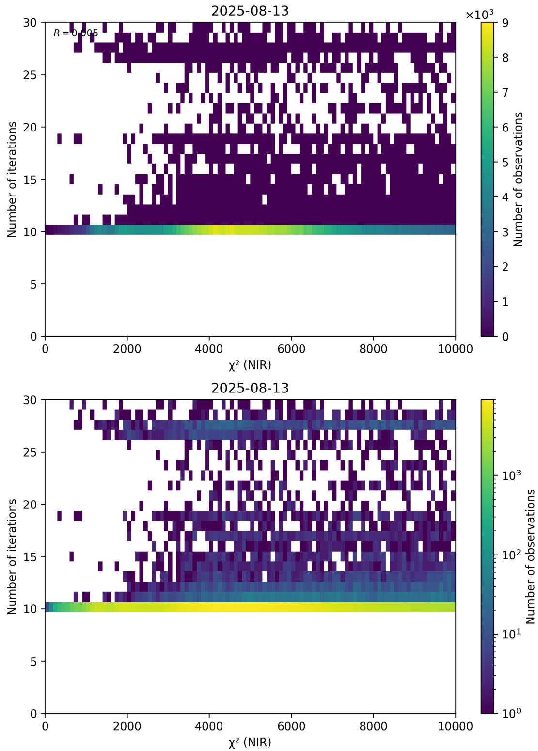
Figure 46: Scatter density plot of “ \chi^2 (NIR)” against “Number of iterations” for 2025-08-12 to 2025-08-14.
