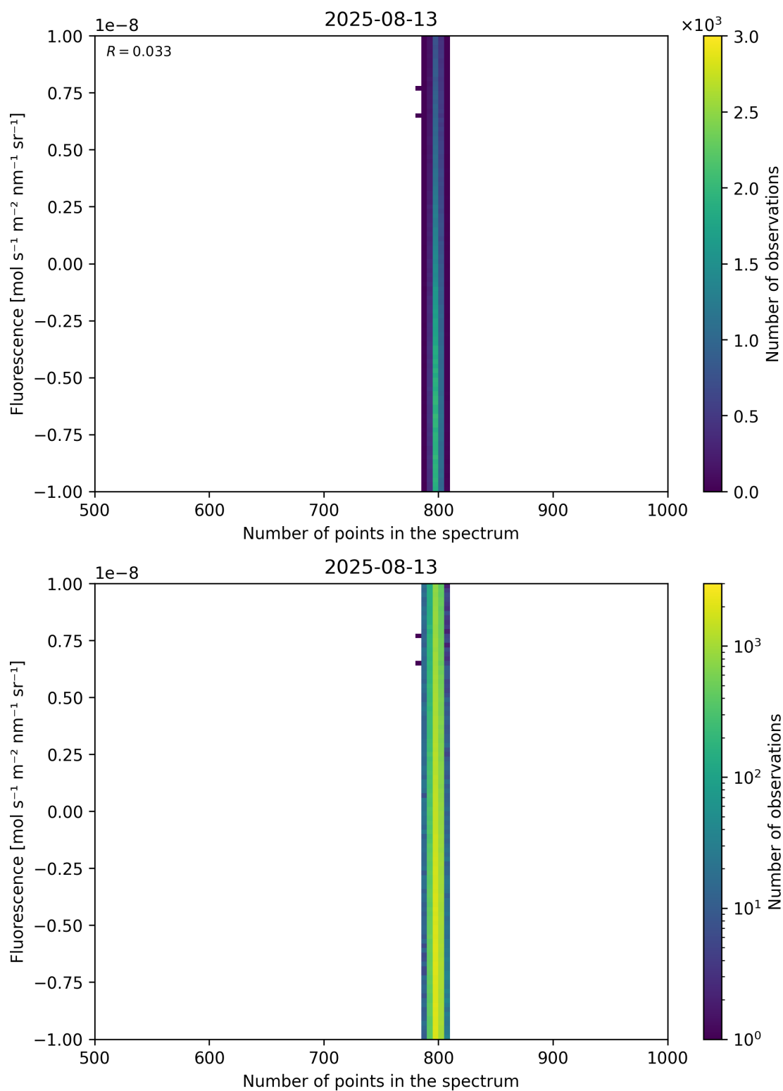
Figure 91: Scatter density plot of “Number of points in the spectrum” against “Fluorescence” for 2025-08-12 to 2025-08-14.
