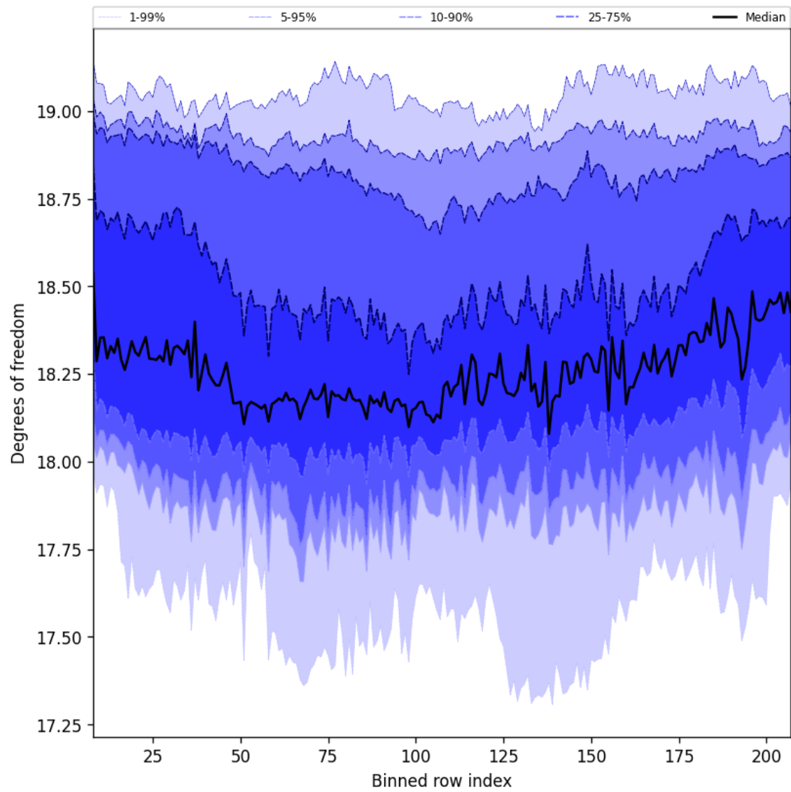
Figure 41: Along track statistics of “Degrees of freedom” for 2025-08-12 to 2025-08-14
