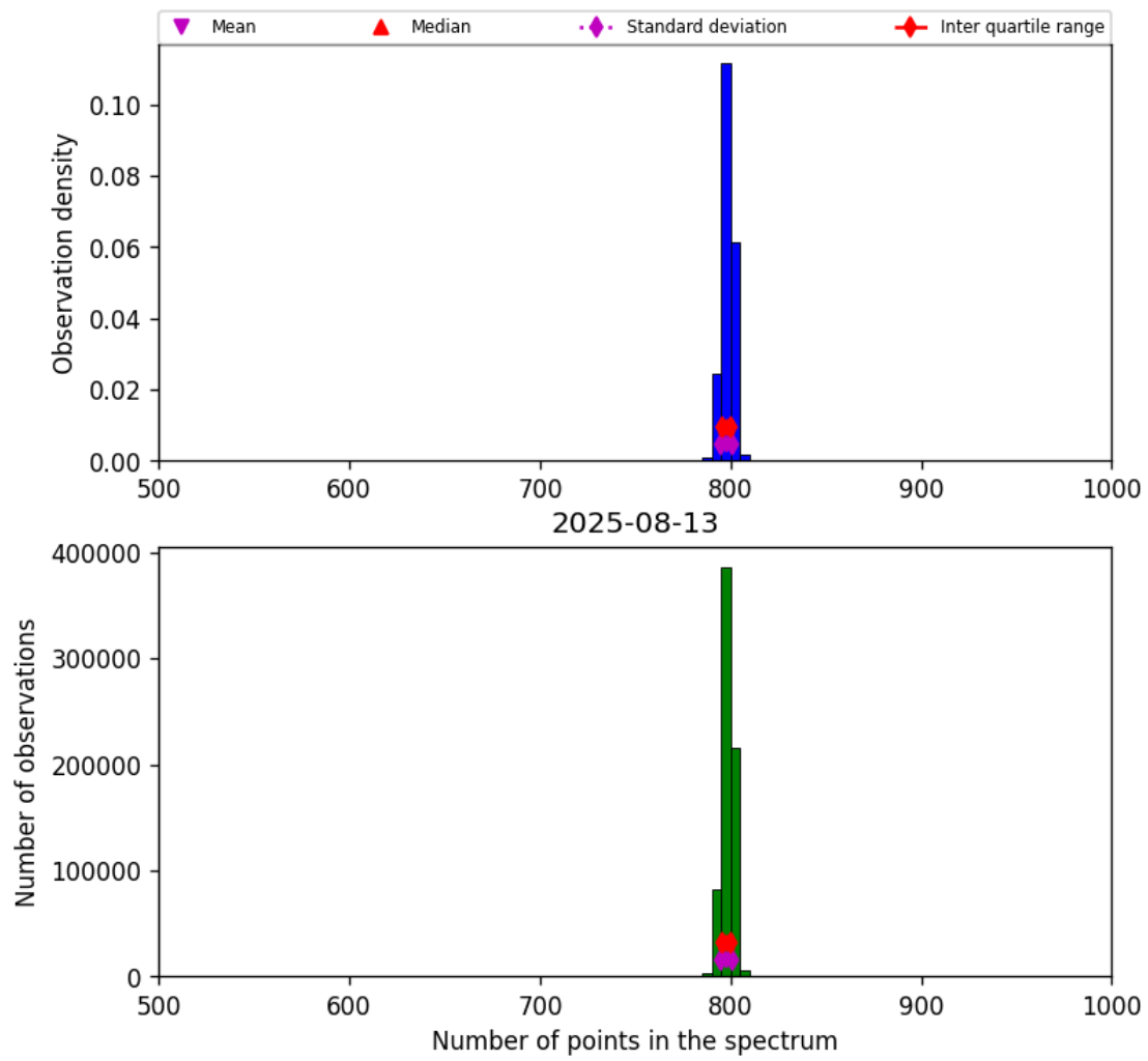
Figure 26: Histogram of “Number of points in the spectrum” for 2025-08-12 to 2025-08-14
