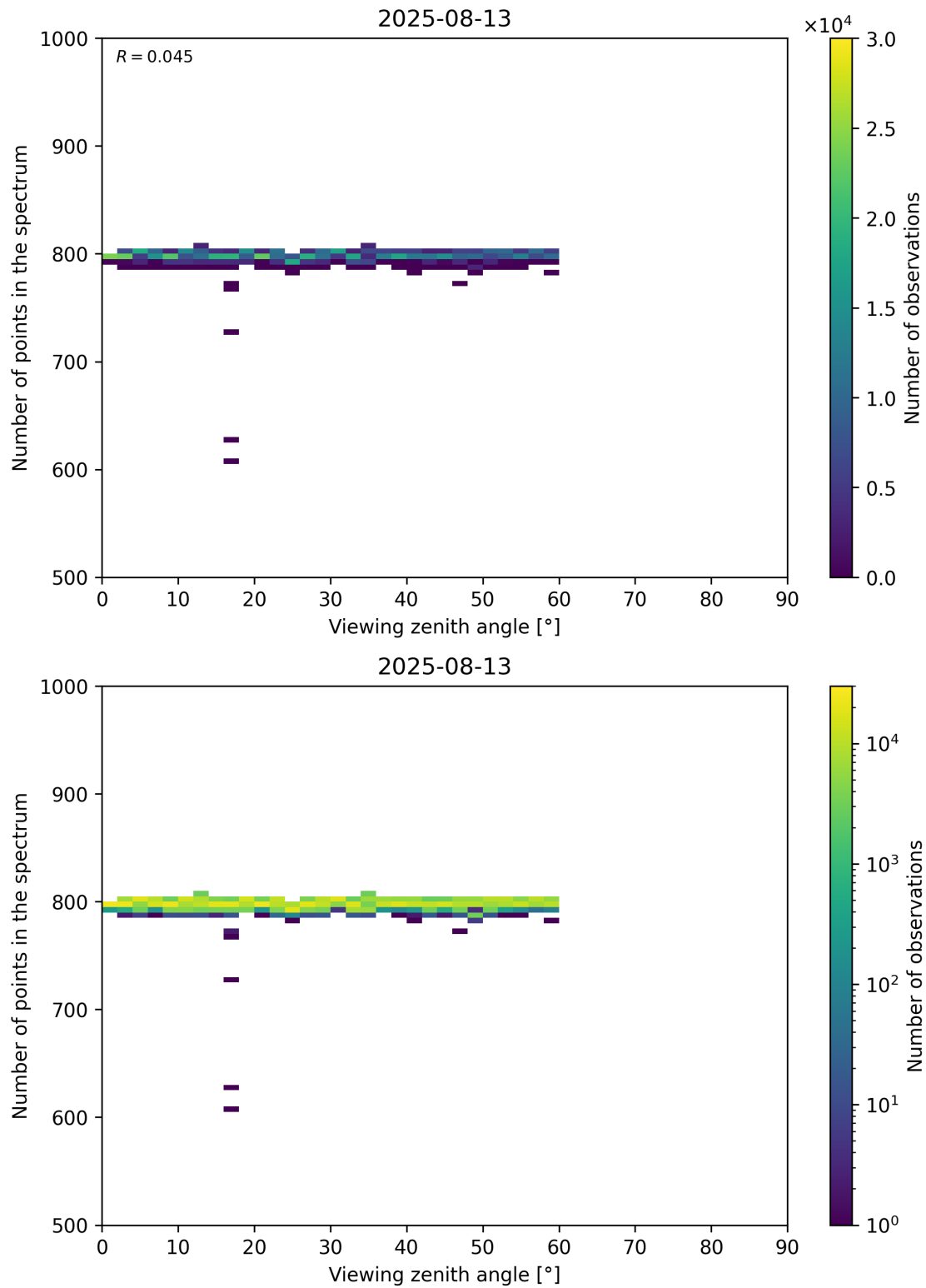
Figure 114: Scatter density plot of “Viewing zenith angle” against “Number of points in the spectrum” for 2025-08-12 to 2025-08-14.
