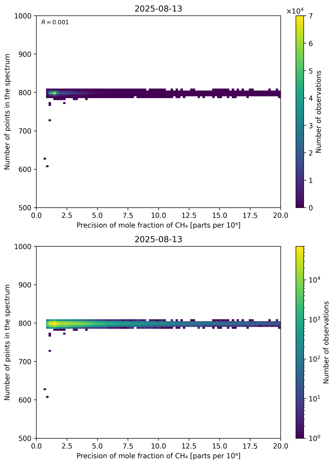
Figure 84: Scatter density plot of “Precision of mole fraction of CH 4 ” against “Number of points in the spectrum” for 2025-08-12 to 2025-08-14.
