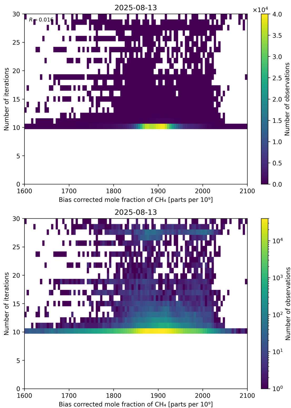
Figure 67: Scatter density plot of “Bias corrected mole fraction of \text{CH}_4 ” against “Number of iterations” for 2025-08-12 to 2025-08-14.
