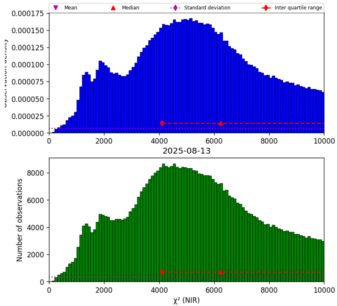
Figure 29: Histogram of “ \chi^2 (NIR)” for 2025-08-12 to 2025-08-14
