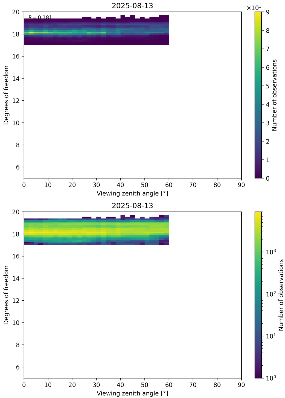
Figure 107: Scatter density plot of “Viewing zenith angle” against “Degrees of freedom” for 2025-08-12 to 2025-08-14.
