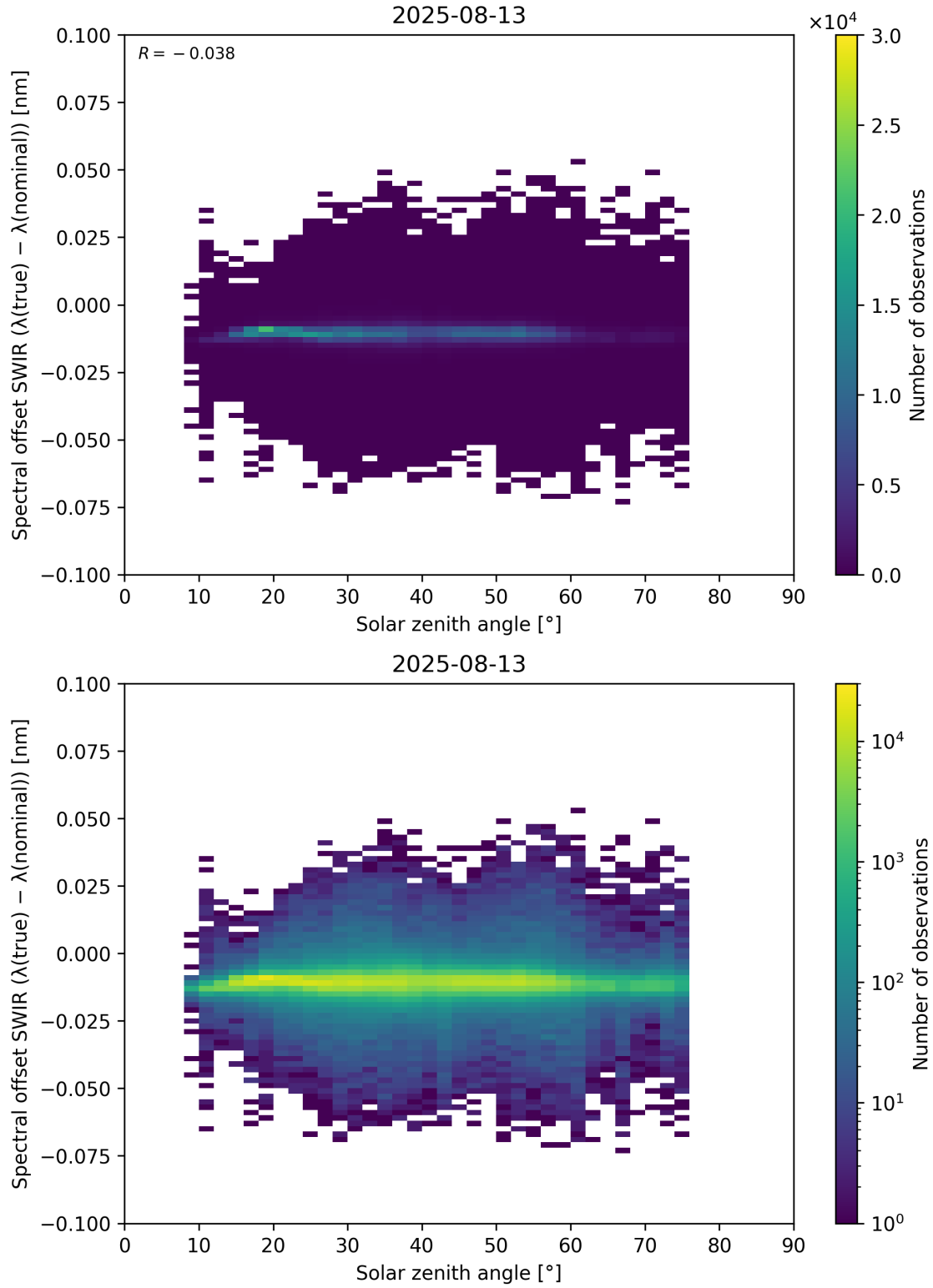
Figure 104: Scatter density plot of “Solar zenith angle” against “Spectral offset SWIR ( \lambda_{\text{true}} - \lambda_{\text{nominal}} )” for 2025-08-12 to 2025-08-14.
