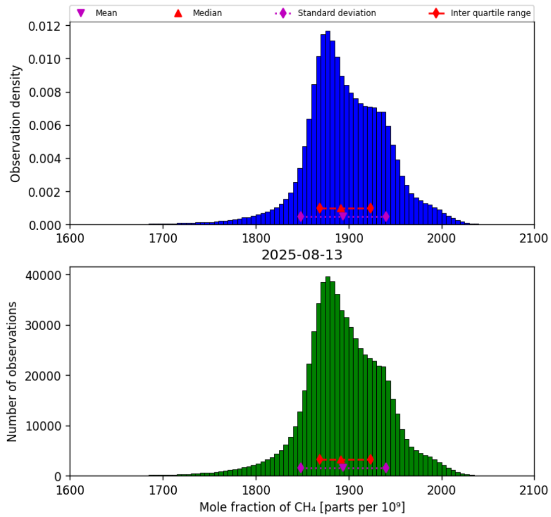
Figure 23: Histogram of “Mole fraction of CH 4 ” for 2025-08-12 to 2025-08-14
