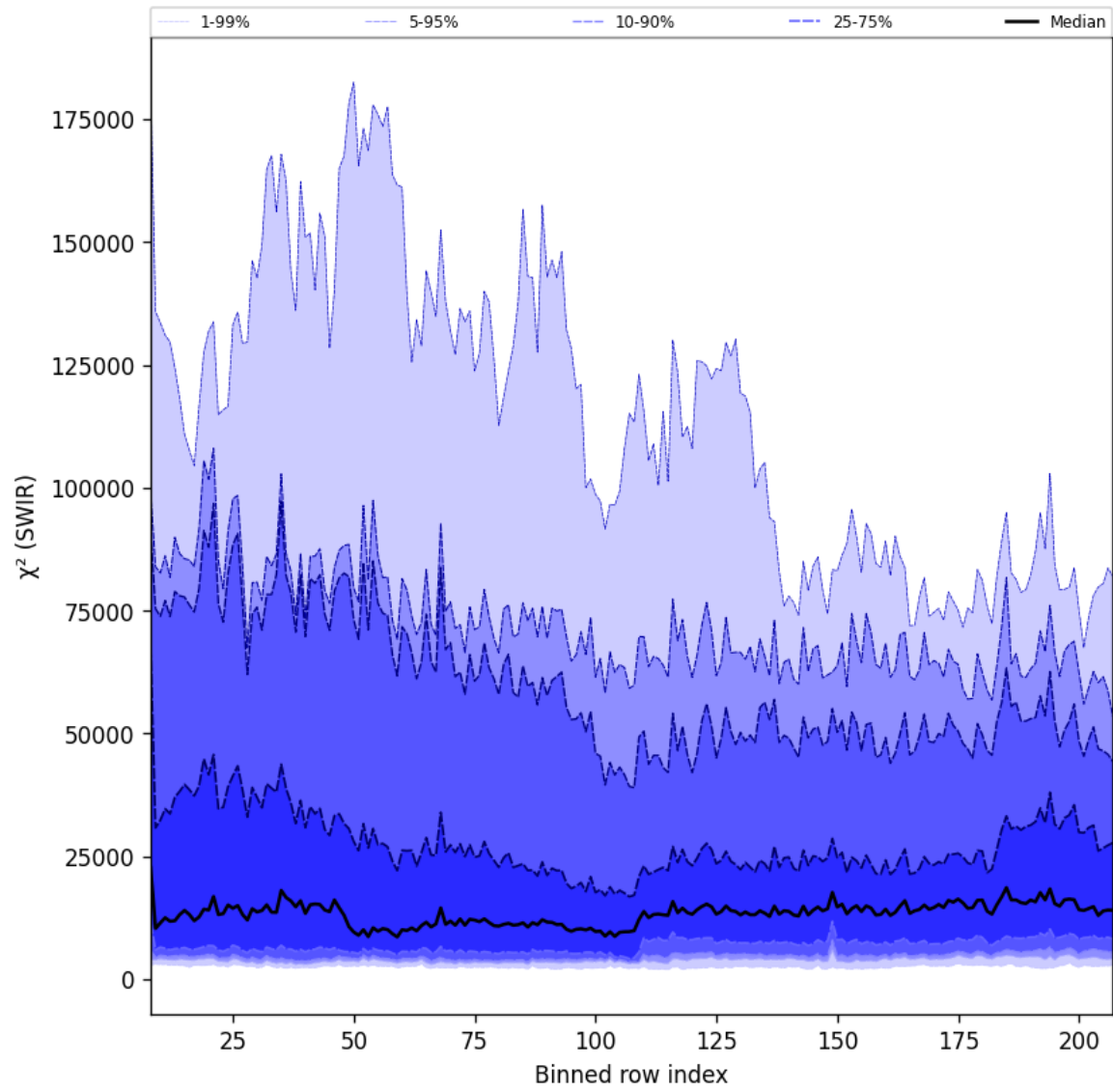
Figure 39: Along track statistics of “ \chi^2 (SWIR)” for 2025-08-12 to 2025-08-14
