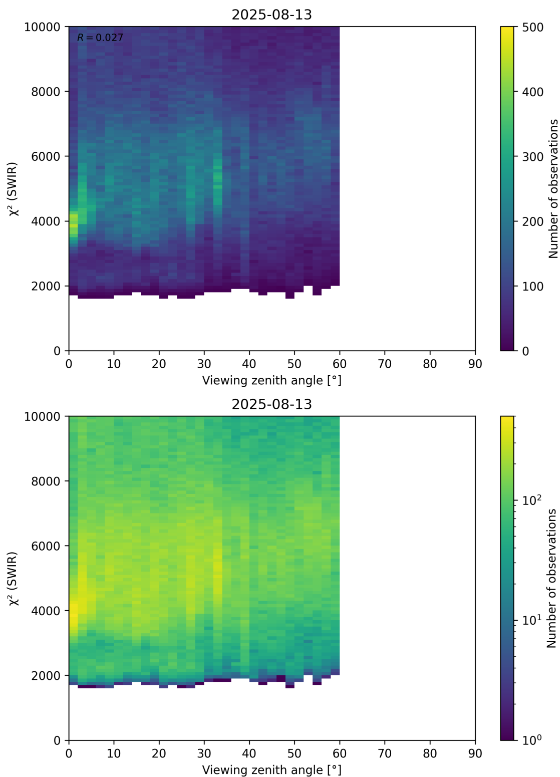
Figure 106: Scatter density plot of “Viewing zenith angle” against “ \chi^2 (SWIR)” for 2025-08-12 to 2025-08-14.
