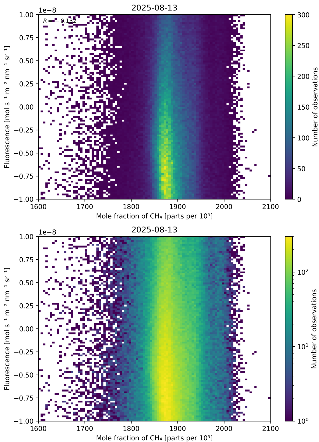
Figure 73: Scatter density plot of “Mole fraction of \text{CH}_4 ” against “Fluorescence” for 2025-08-12 to 2025-08-14.
