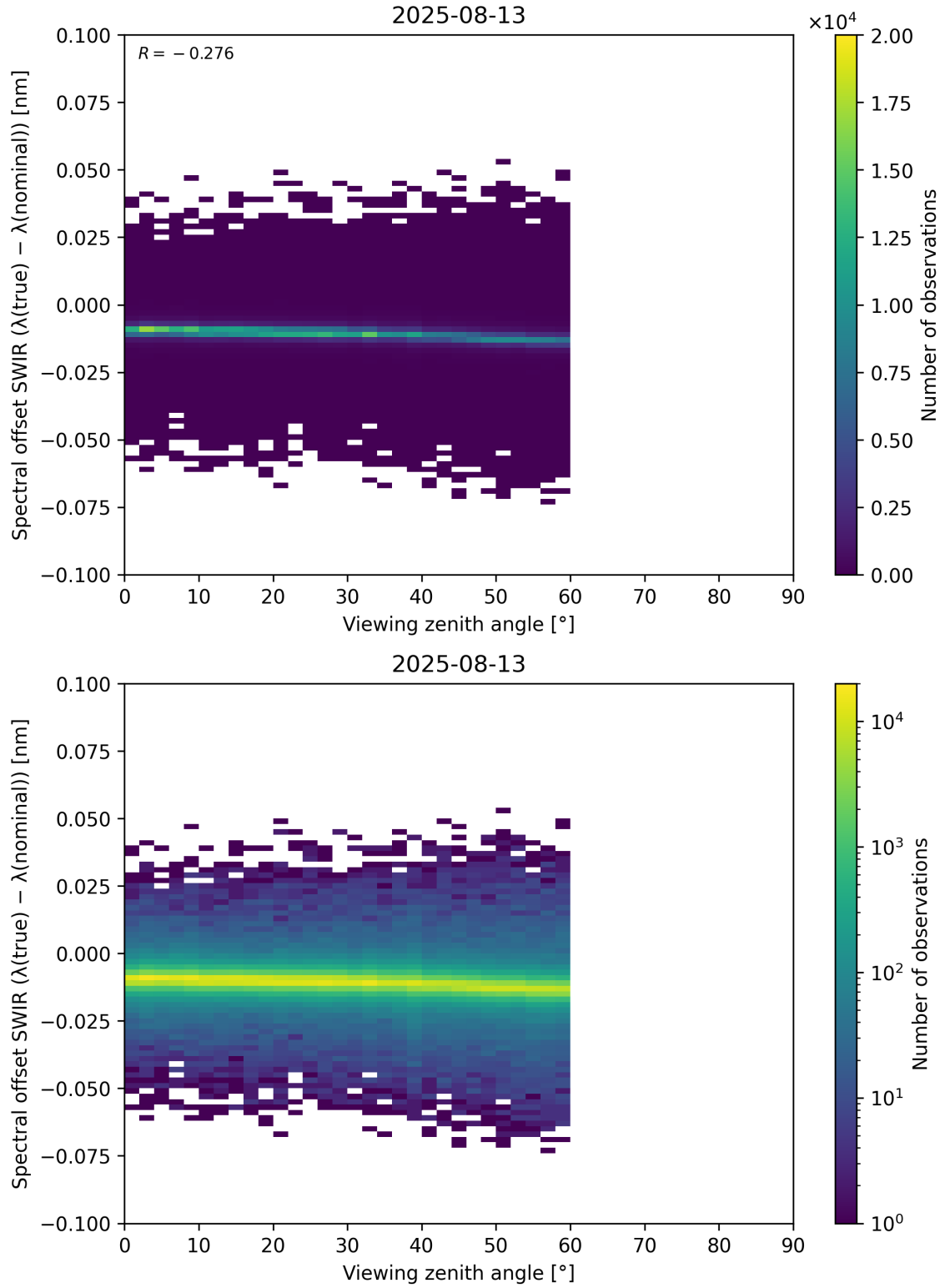
Figure 116: Scatter density plot of “Viewing zenith angle” against “Spectral offset SWIR ( \lambda_{\text{true}} - \lambda_{\text{nominal}} )” for 2025-08-12 to 2025-08-14.
