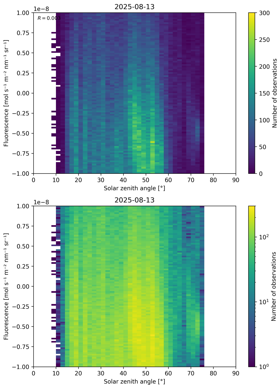
Figure 97: Scatter density plot of “Solar zenith angle” against “Fluorescence” for 2025-08-12 to 2025-08-14.
