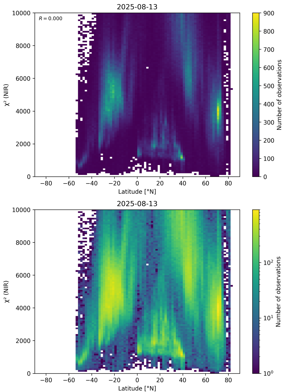
Figure 53: Scatter density plot of “Latitude” against “ \chi^2 (NIR)” for 2025-08-12 to 2025-08-14.
