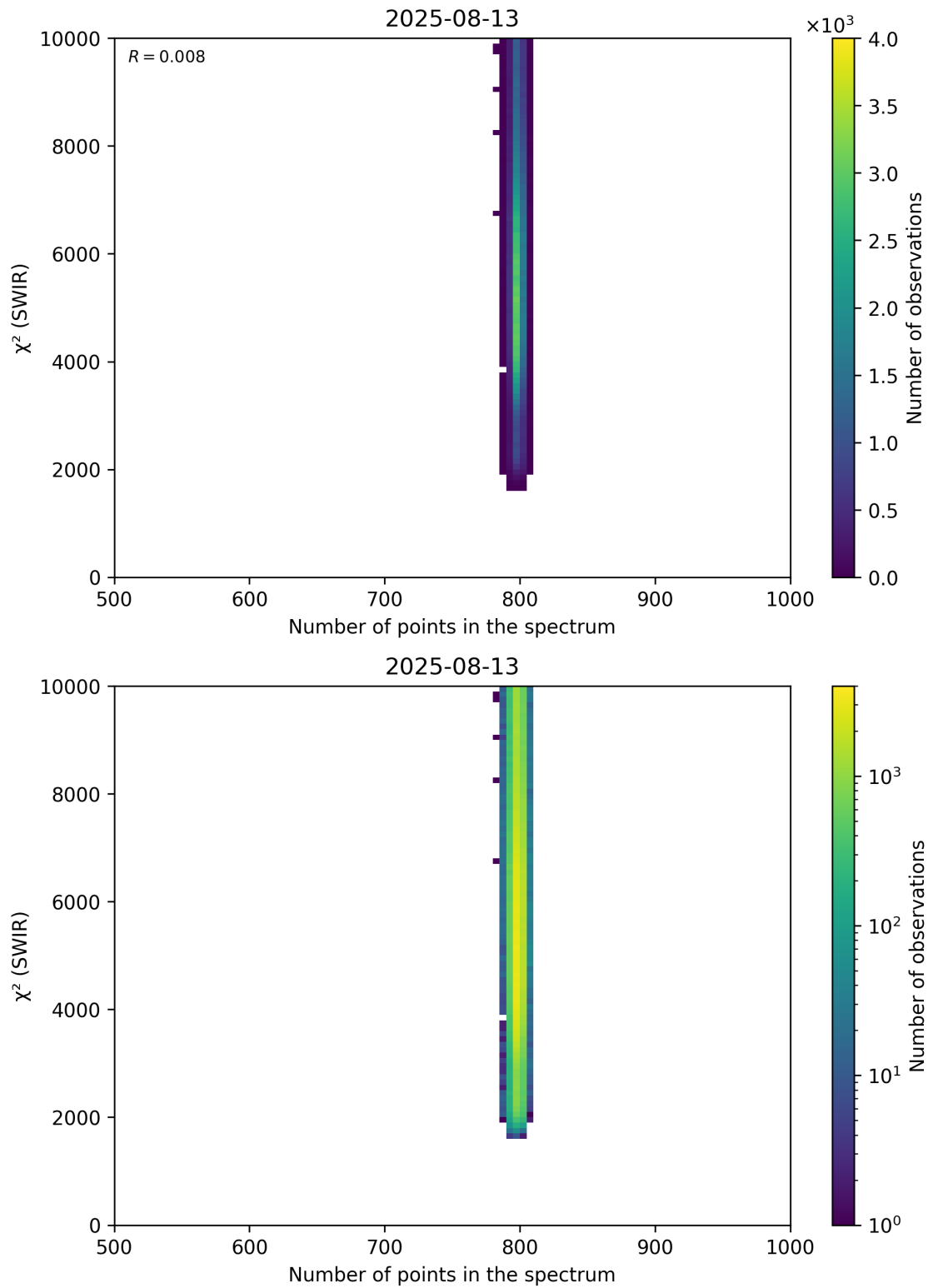
Figure 89: Scatter density plot of “Number of points in the spectrum” against “ \chi^2 (SWIR)” for 2025-08-12 to 2025-08-14.
