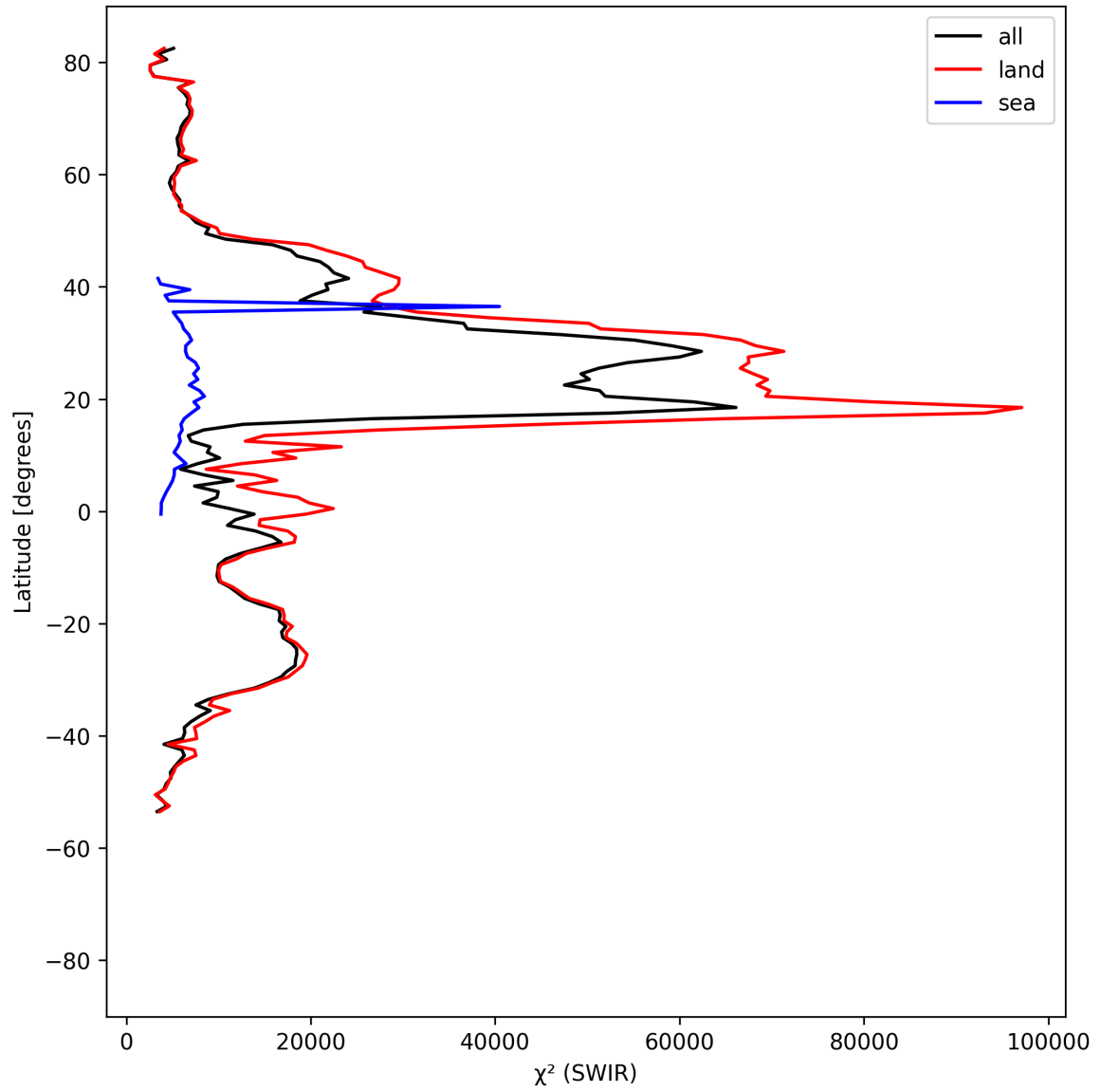
Figure 17: Zonal average of “ \chi^2 (SWIR)” for 2025-08-12 to 2025-08-14.
