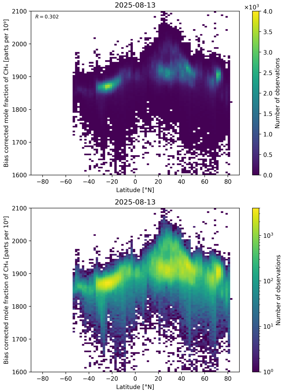
Figure 58: Scatter density plot of “Latitude” against “Bias corrected mole fraction of CH 4 ” for 2025-08-12 to 2025-08-14.
