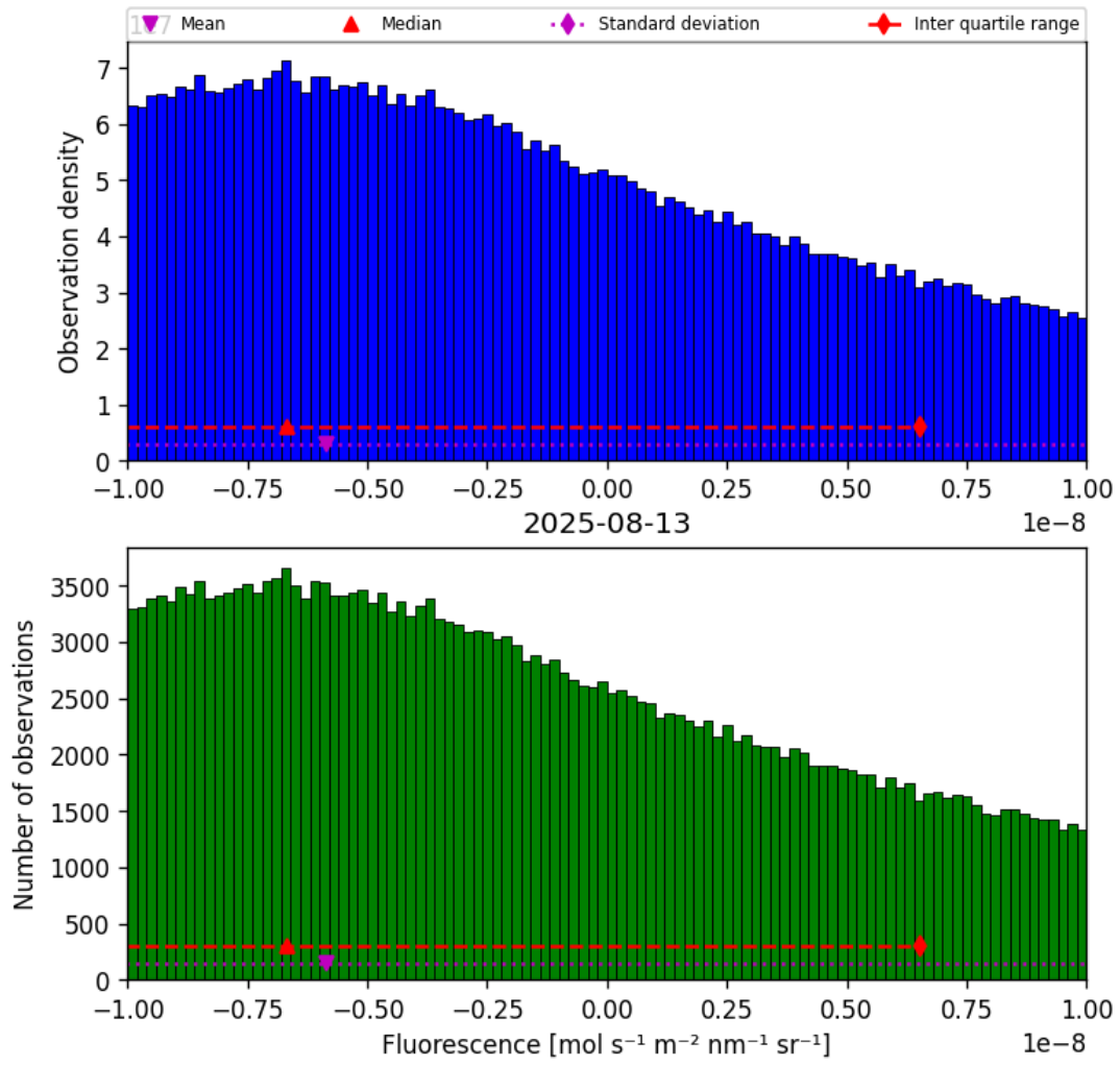
Figure 32: Histogram of “Fluorescence” for 2025-08-12 to 2025-08-14
