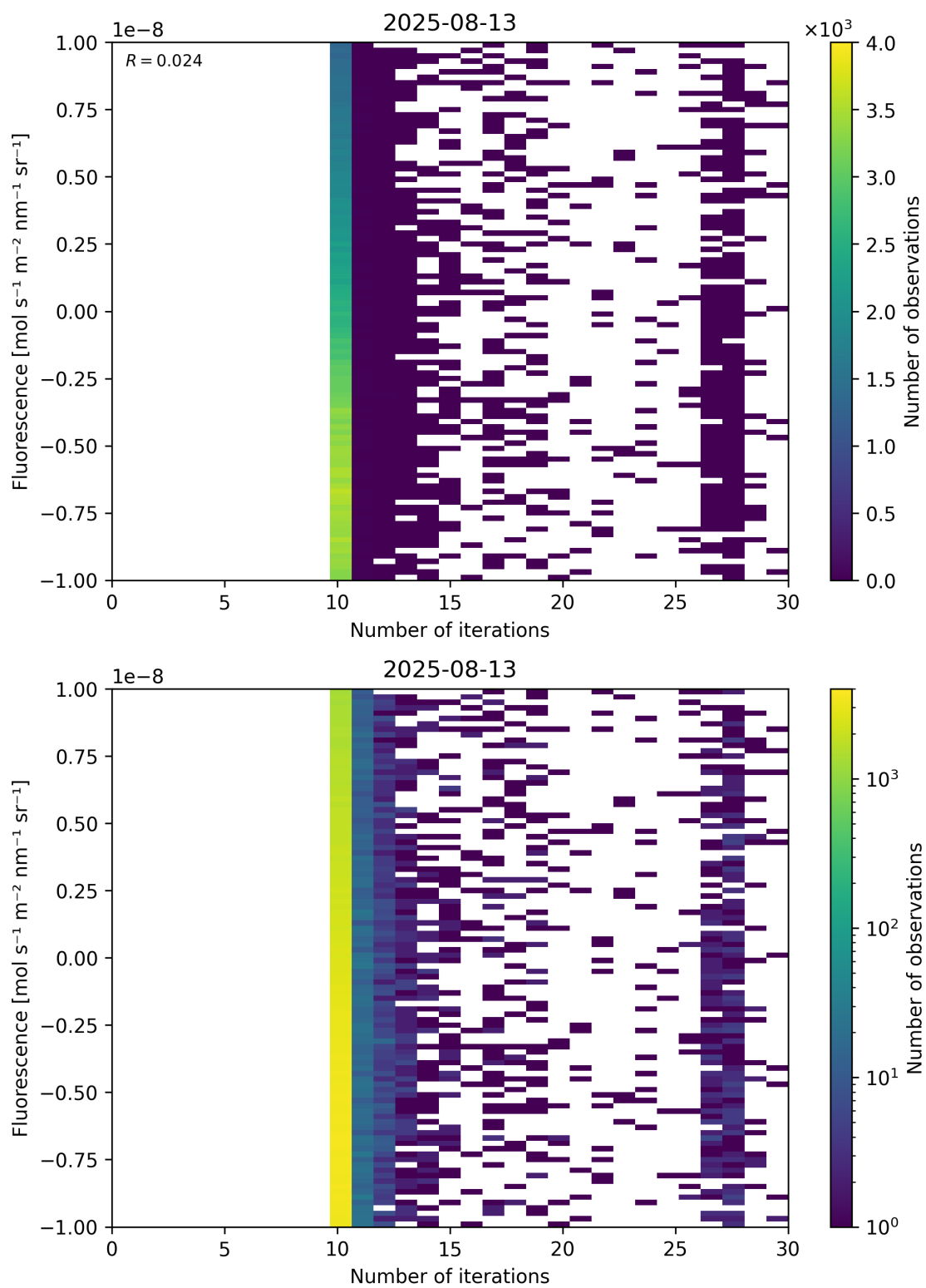
Figure 87: Scatter density plot of “Number of iterations” against “Fluorescence” for 2025-08-12 to 2025-08-14.
