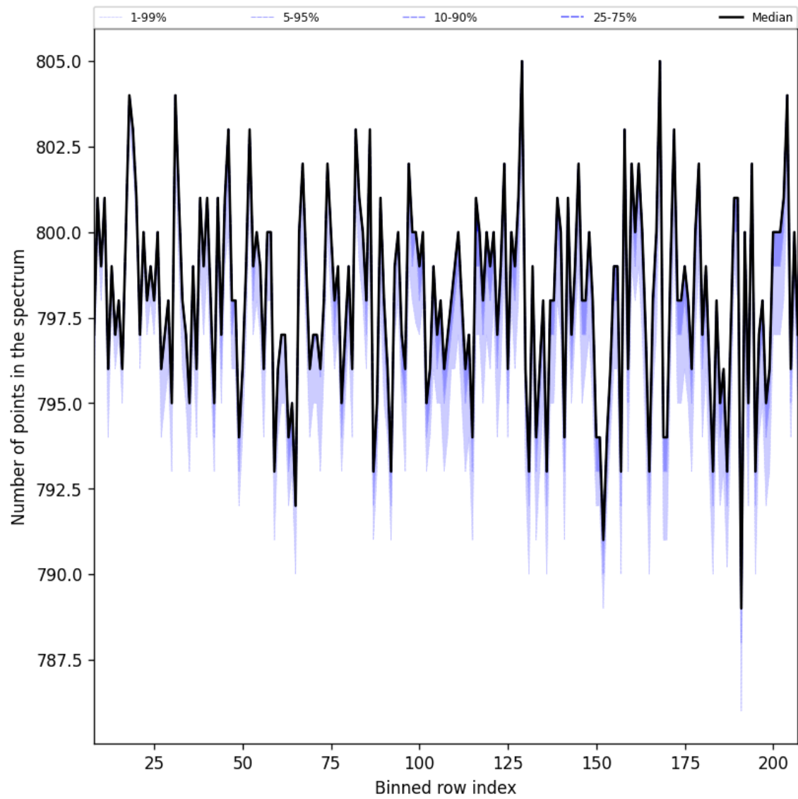
Figure 37: Along track statistics of “Number of points in the spectrum” for 2025-08-12 to 2025-08-14
