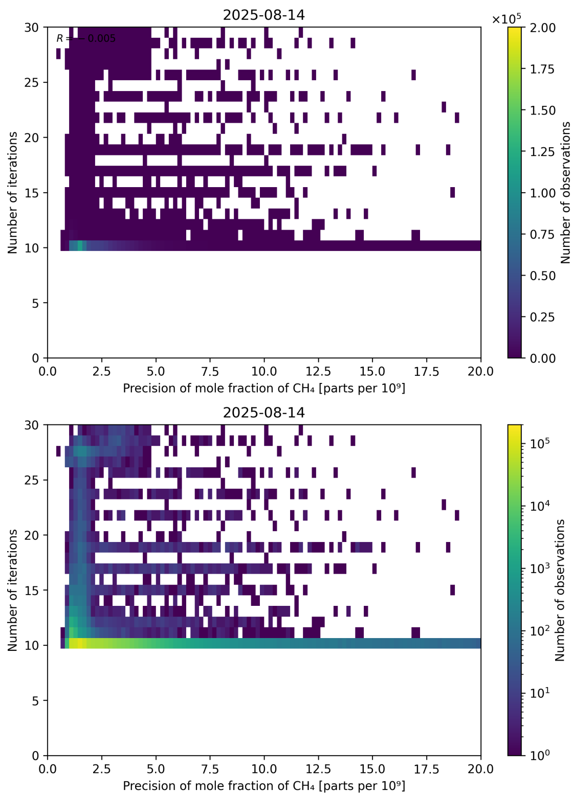
Figure 83: Scatter density plot of “Precision of mole fraction of CH 4 ” against “Number of iterations” for 2025-08-14 to 2025-08-15.
