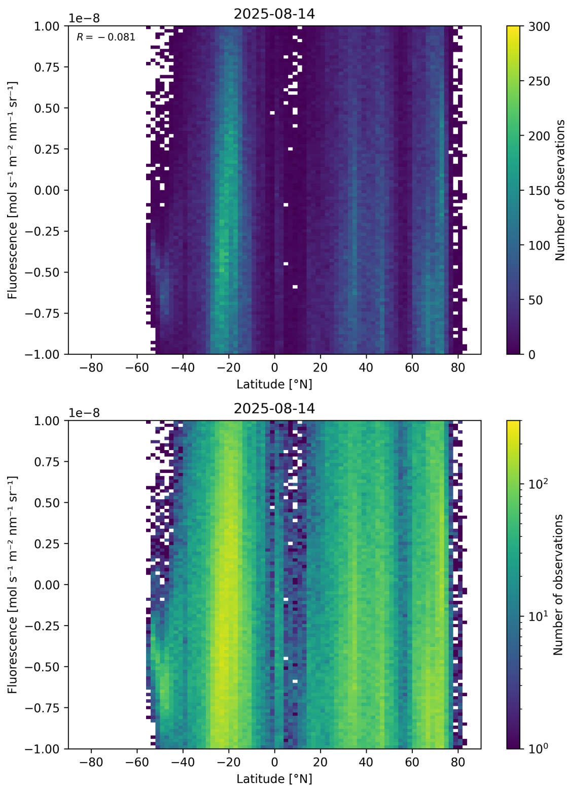
Figure 56: Scatter density plot of “Latitude” against “Fluorescence” for 2025-08-14 to 2025-08-15.
