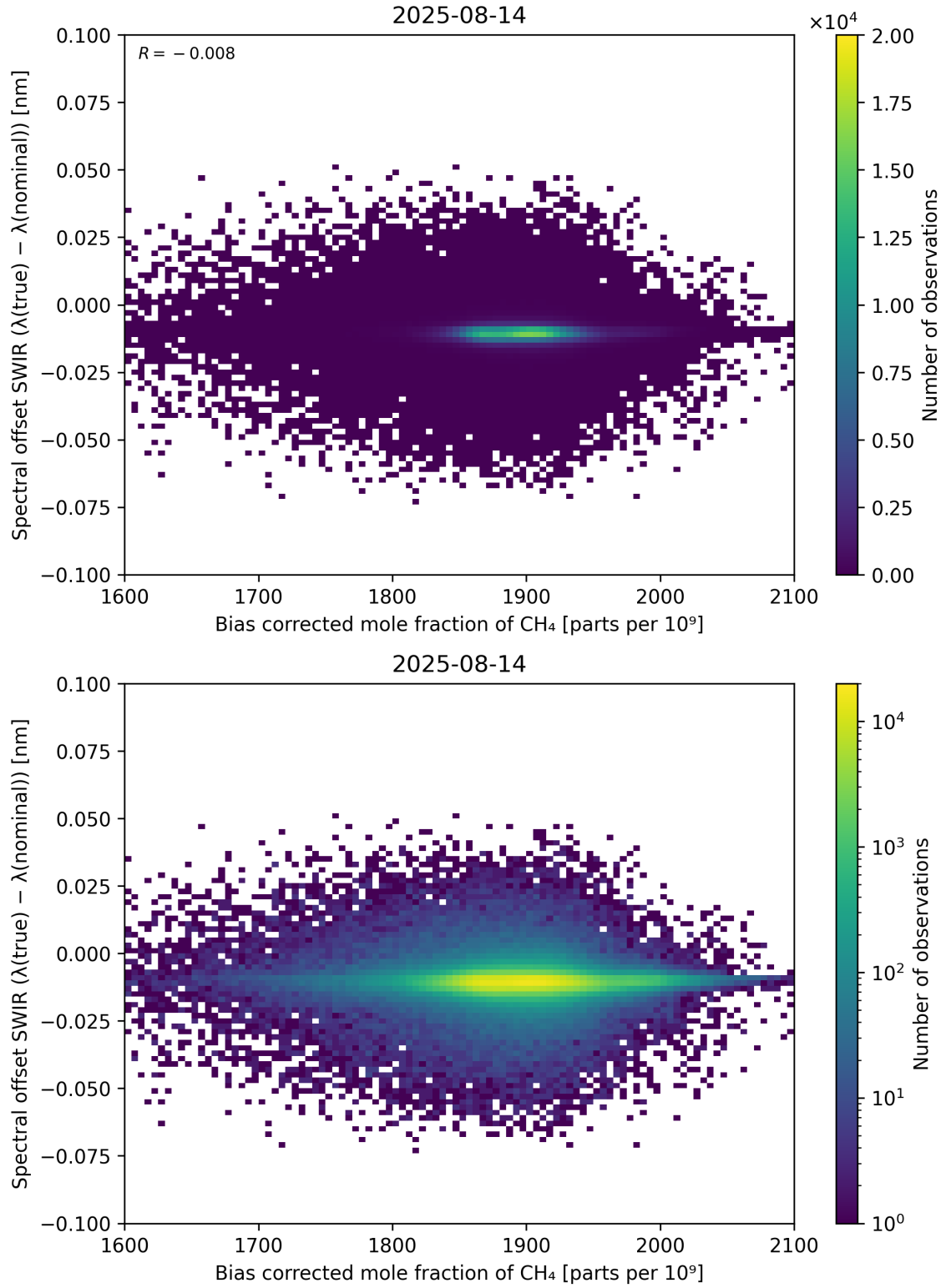
Figure 69: Scatter density plot of “Bias corrected mole fraction of \text{CH}_4 ” against “Spectral offset SWIR ( \lambda_{\text{true}} - \lambda_{\text{nominal}} )” for 2025-08-14 to 2025-08-15.
