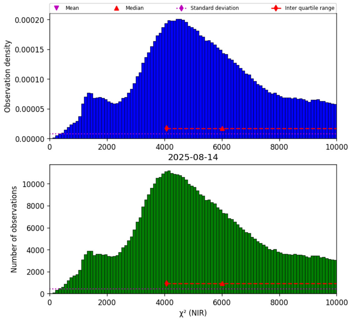
Figure 29: Histogram of " \chi^2 (NIR)" for 2025-08-14 to 2025-08-15
