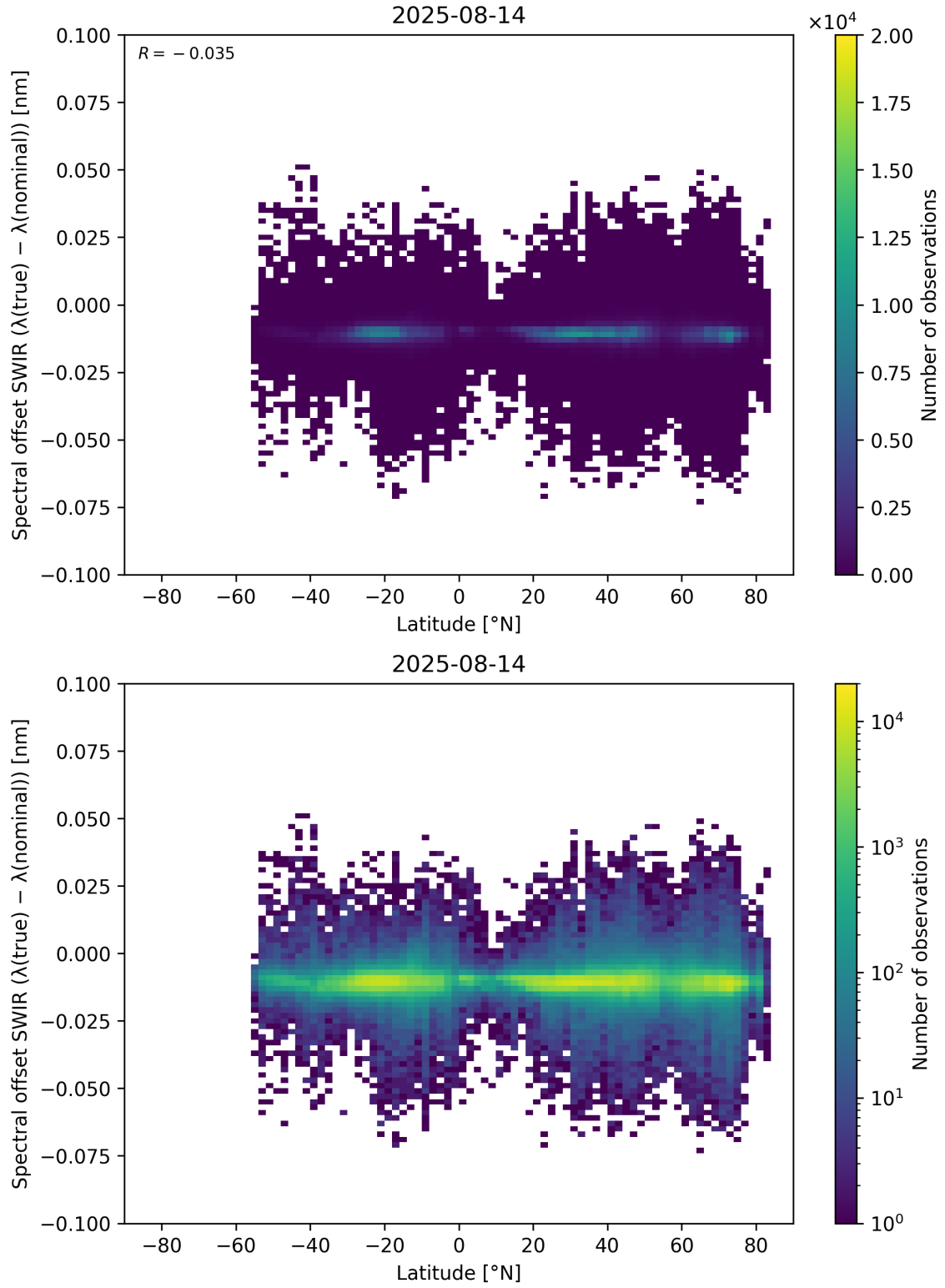
Figure 62: Scatter density plot of “Latitude” against “Spectral offset SWIR ( \lambda_{\text{true}} - \lambda_{\text{nominal}} )” for 2025-08-14 to 2025-08-15.
