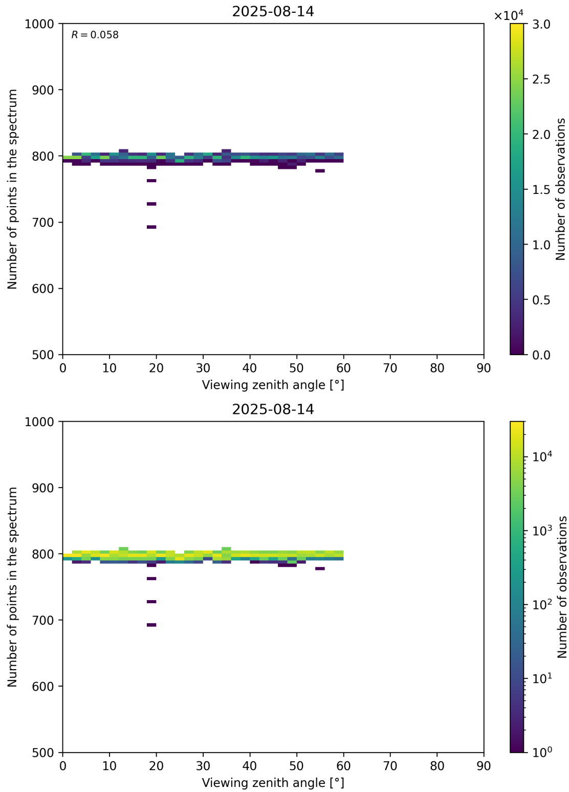
Figure 114: Scatter density plot of “Viewing zenith angle” against “Number of points in the spectrum” for 2025-08-14 to 2025-08-15.
