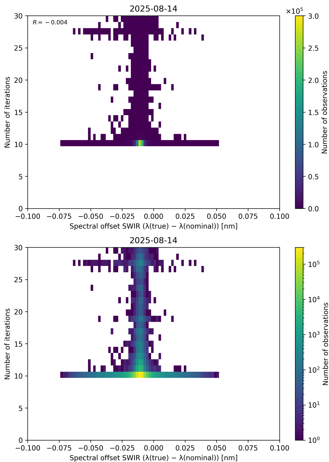
Figure 121: Scatter density plot of “Spectral offset SWIR ( \lambda_{\text{true}} - \lambda_{\text{nominal}} )” against “Number of iterations” for 2025-08-14 to 2025-08-15.
