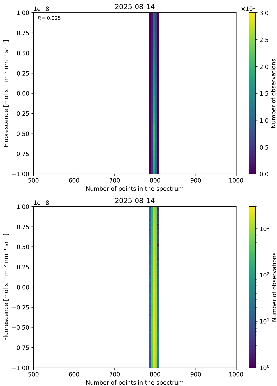
Figure 91: Scatter density plot of “Number of points in the spectrum” against “Fluorescence” for 2025-08-14 to 2025-08-15.
