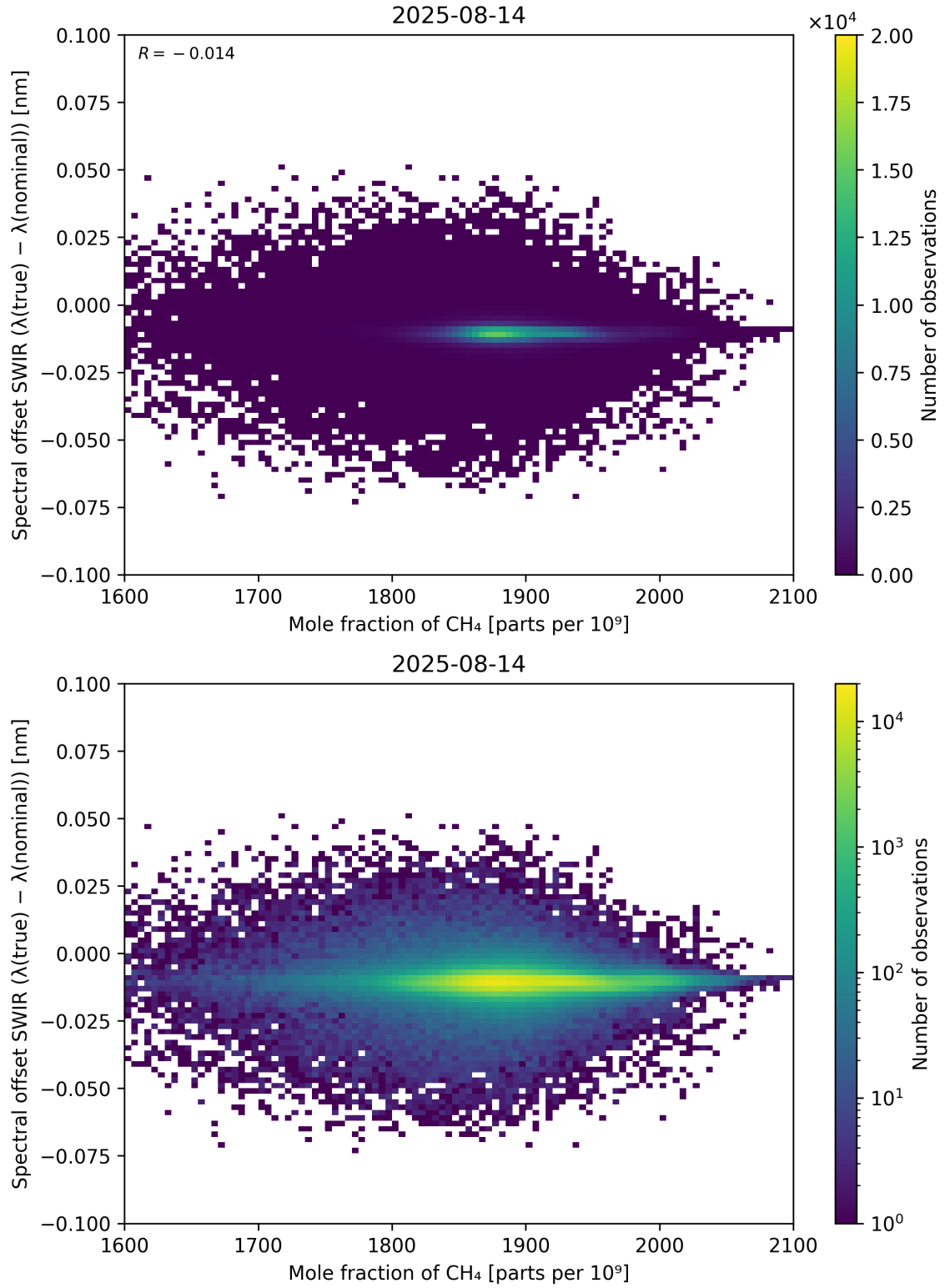
Figure 86: Scatter density plot of “Mole fraction of \text{CH}_4 ” against “Spectral offset SWIR ( \lambda_{\text{true}} - \lambda_{\text{nominal}} )” for 2025-08-14 to 2025-08-15.
