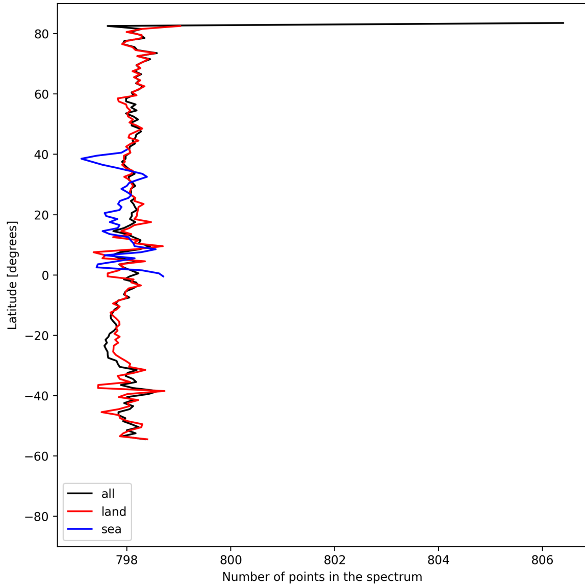
Figure 15: Zonal average of “Number of points in the spectrum” for 2025-08-14 to 2025-08-15.
