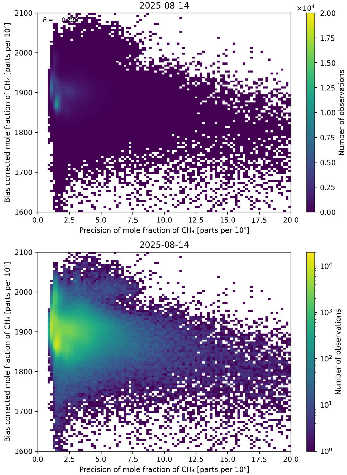
Figure 82: Scatter density plot of “Precision of mole fraction of CH 4 ” against “Bias corrected mole fraction of CH 4 ” for 2025-08-14 to 2025-08-15.
