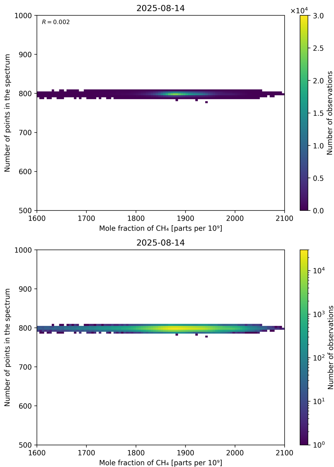
Figure 77: Scatter density plot of “Mole fraction of CH 4 ” against “Number of points in the spectrum” for 2025-08-14 to 2025-08-15.
