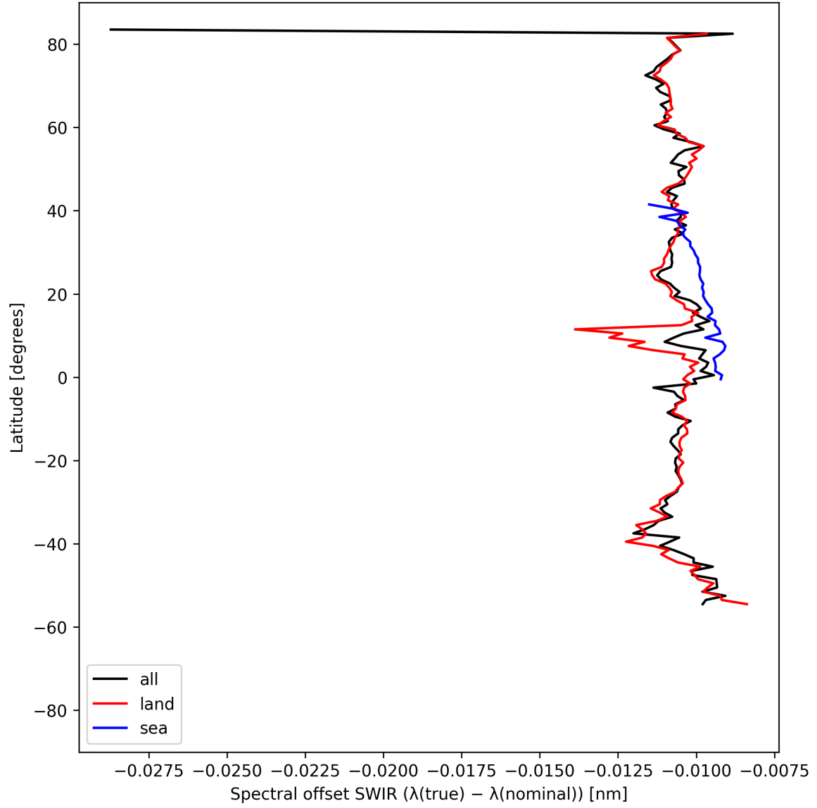
Figure 16: Zonal average of “Spectral offset SWIR ( \lambda_{\text{true}} - \lambda_{\text{nominal}} )” for 2025-08-14 to 2025-08-15.
