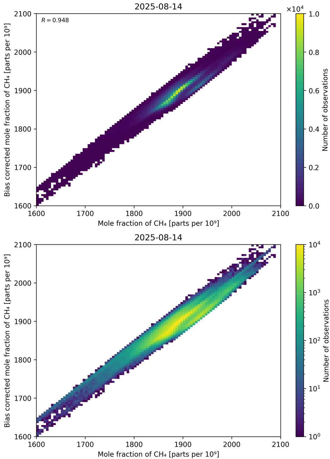
Figure 74: Scatter density plot of “Mole fraction of CH 4 ” against “Bias corrected mole fraction of CH 4 ” for 2025-08-14 to 2025-08-15.
