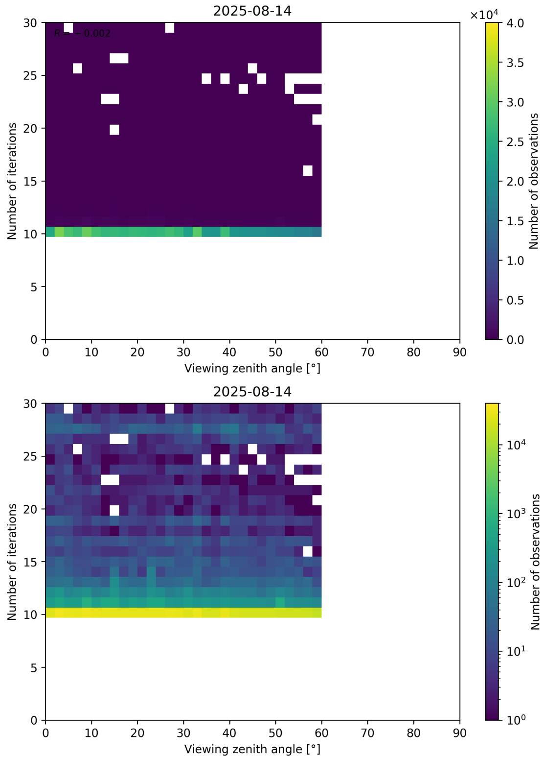
Figure 113: Scatter density plot of “Viewing zenith angle” against “Number of iterations” for 2025-08-14 to 2025-08-15.
