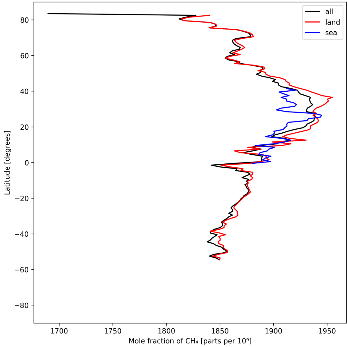
Figure 12: Zonal average of “Mole fraction of \text{CH}_4 ” for 2025-08-14 to 2025-08-15.
