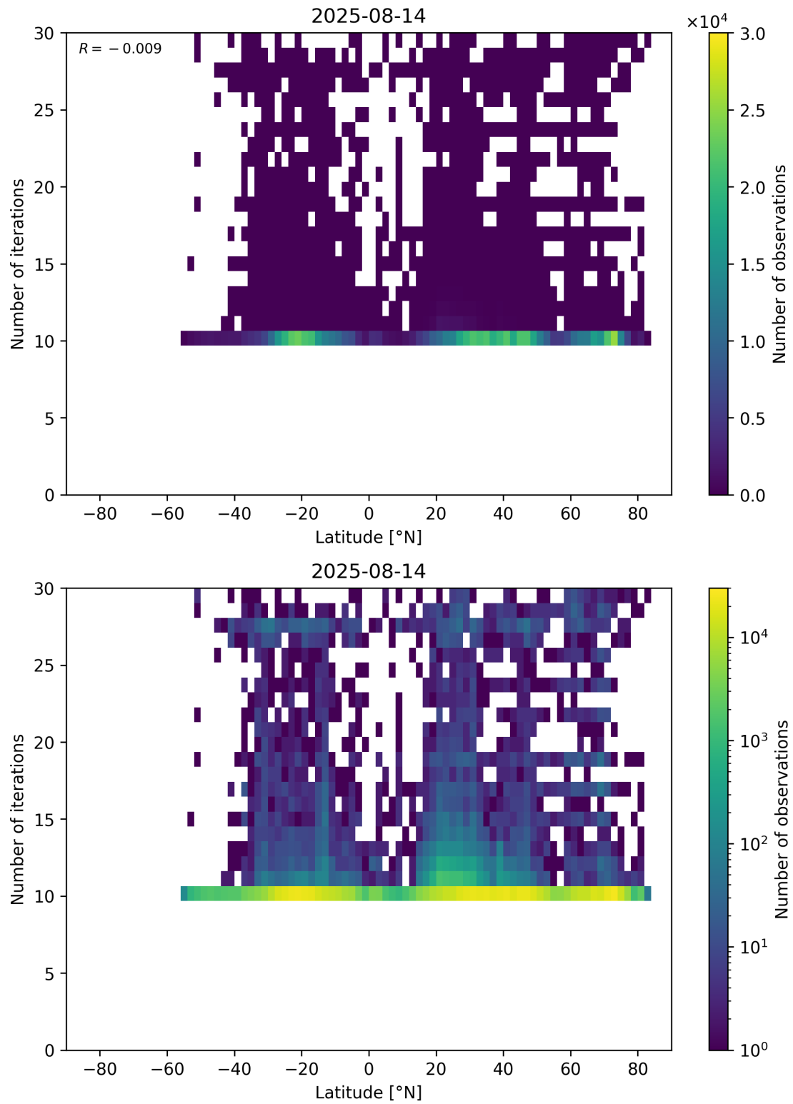
Figure 60: Scatter density plot of “Latitude” against “Number of iterations” for 2025-08-14 to 2025-08-15.
