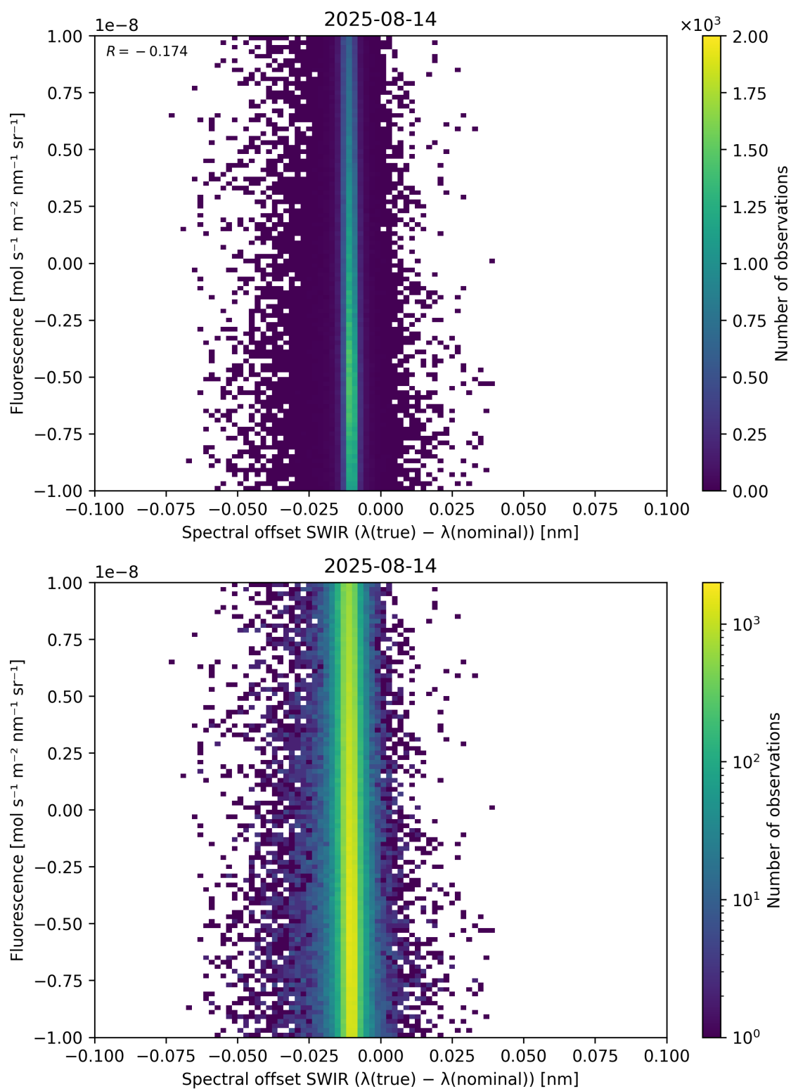
Figure 120: Scatter density plot of “Spectral offset SWIR ( \lambda_{\text{true}} - \lambda_{\text{nominal}} )” against “Fluorescence” for 2025-08-14 to 2025-08-15.
