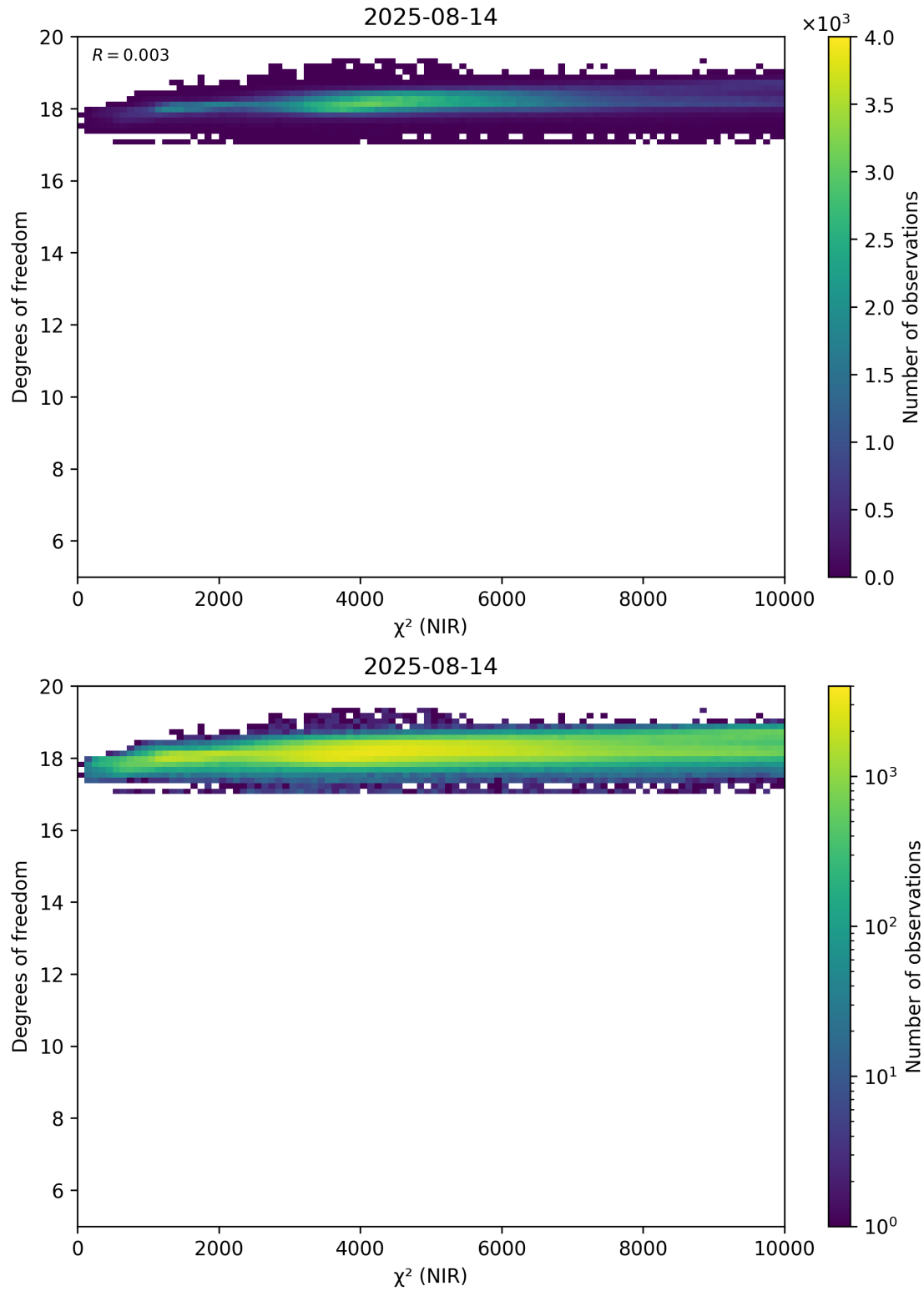
Figure 44: Scatter density plot of “ \chi^2 (NIR)” against “Degrees of freedom” for 2025-08-14 to 2025-08-15.
