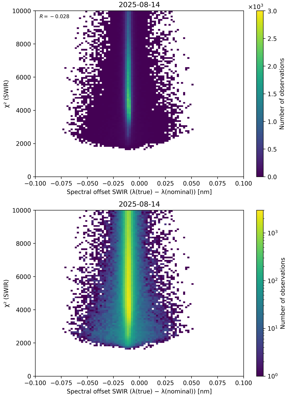
Figure 118: Scatter density plot of “Spectral offset SWIR ( \lambda_{\text{true}} - \lambda_{\text{nominal}} )” against “ \chi^2 (SWIR)” for 2025-08-14 to 2025-08-15.
