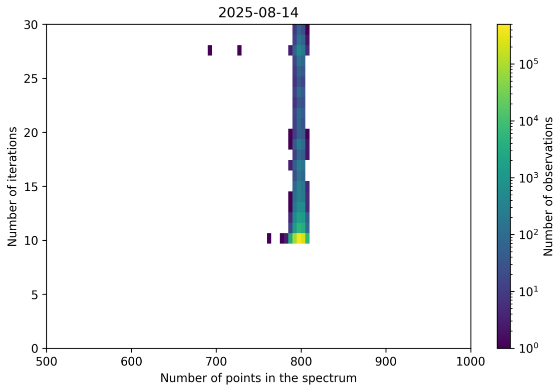
Figure 92: Scatter density plot of “Number of points in the spectrum” against “Number of iterations” for 2025-08-14 to 2025-08-15.
