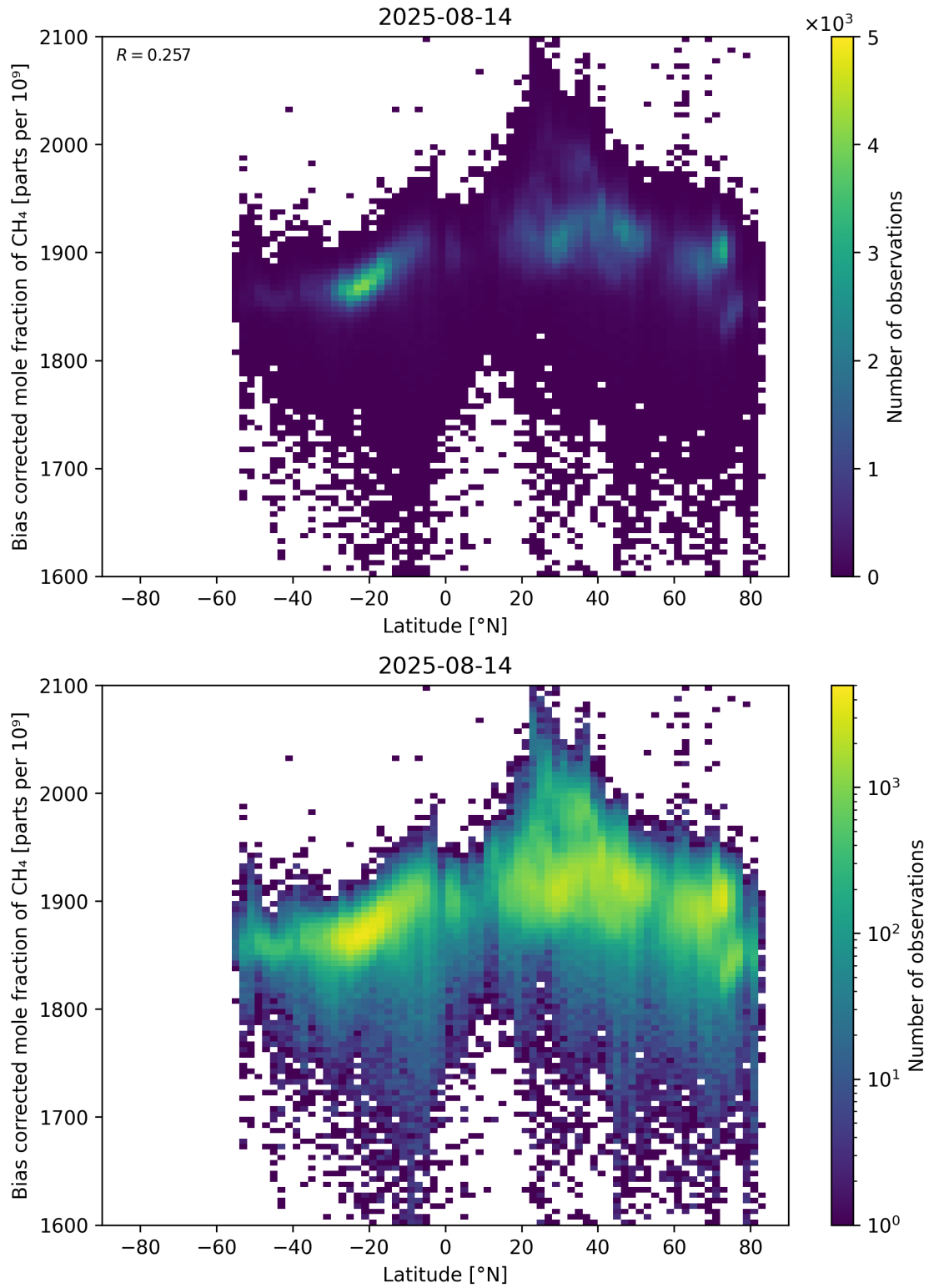
Figure 58: Scatter density plot of “Latitude” against “Bias corrected mole fraction of CH 4 ” for 2025-08-14 to 2025-08-15.
