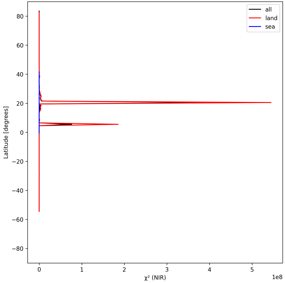
Figure 18: Zonal average of “ \chi^2 (NIR)” for 2025-08-14 to 2025-08-15.
