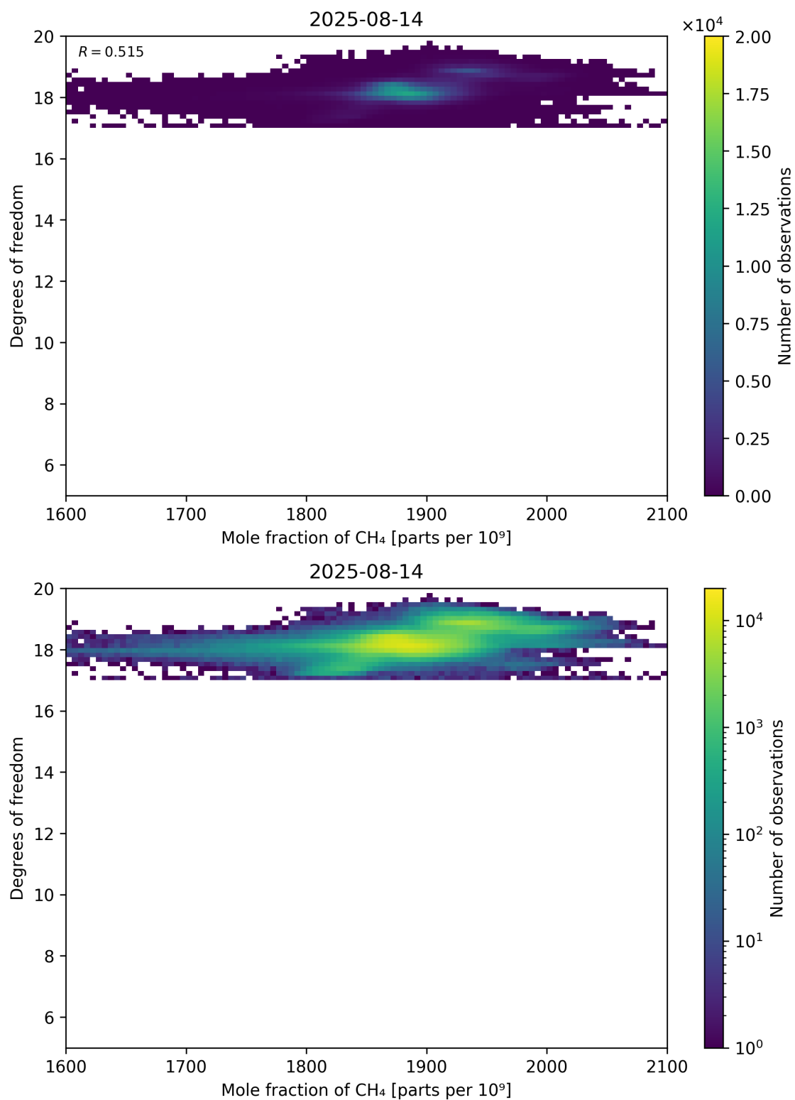
Figure 72: Scatter density plot of “Mole fraction of CH 4 ” against “Degrees of freedom” for 2025-08-14 to 2025-08-15.
