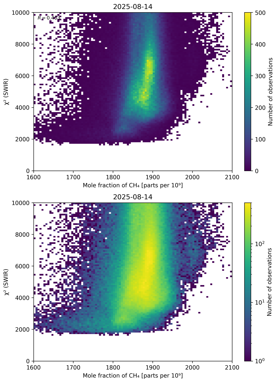
Figure 71: Scatter density plot of “Mole fraction of CH 4 ” against “ \chi^2 (SWIR)” for 2025-08-14 to 2025-08-15.
