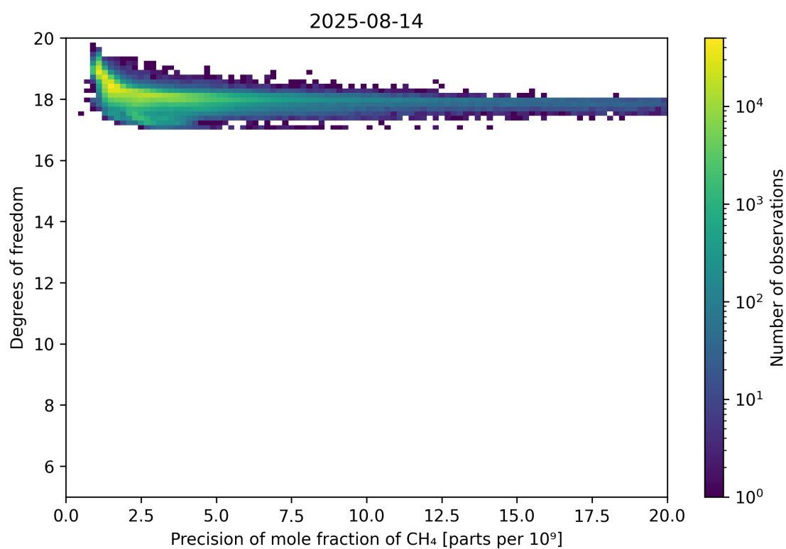
Figure 80: Scatter density plot of “Precision of mole fraction of CH 4 ” against “Degrees of freedom” for 2025-08-14 to 2025-08-15.
