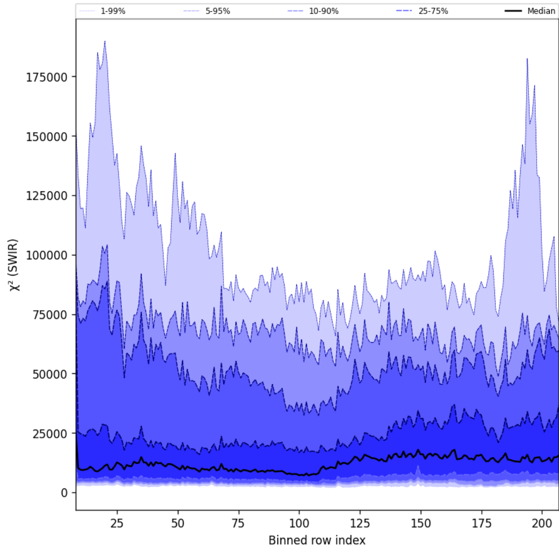
Figure 39: Along track statistics of " \chi^2 (SWIR)" for 2025-08-14 to 2025-08-15
