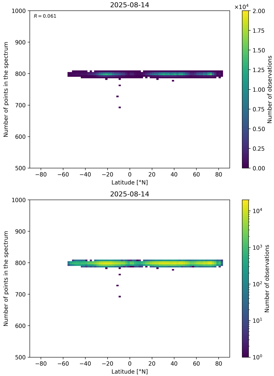
Figure 61: Scatter density plot of “Latitude” against “Number of points in the spectrum” for 2025-08-14 to 2025-08-15.
