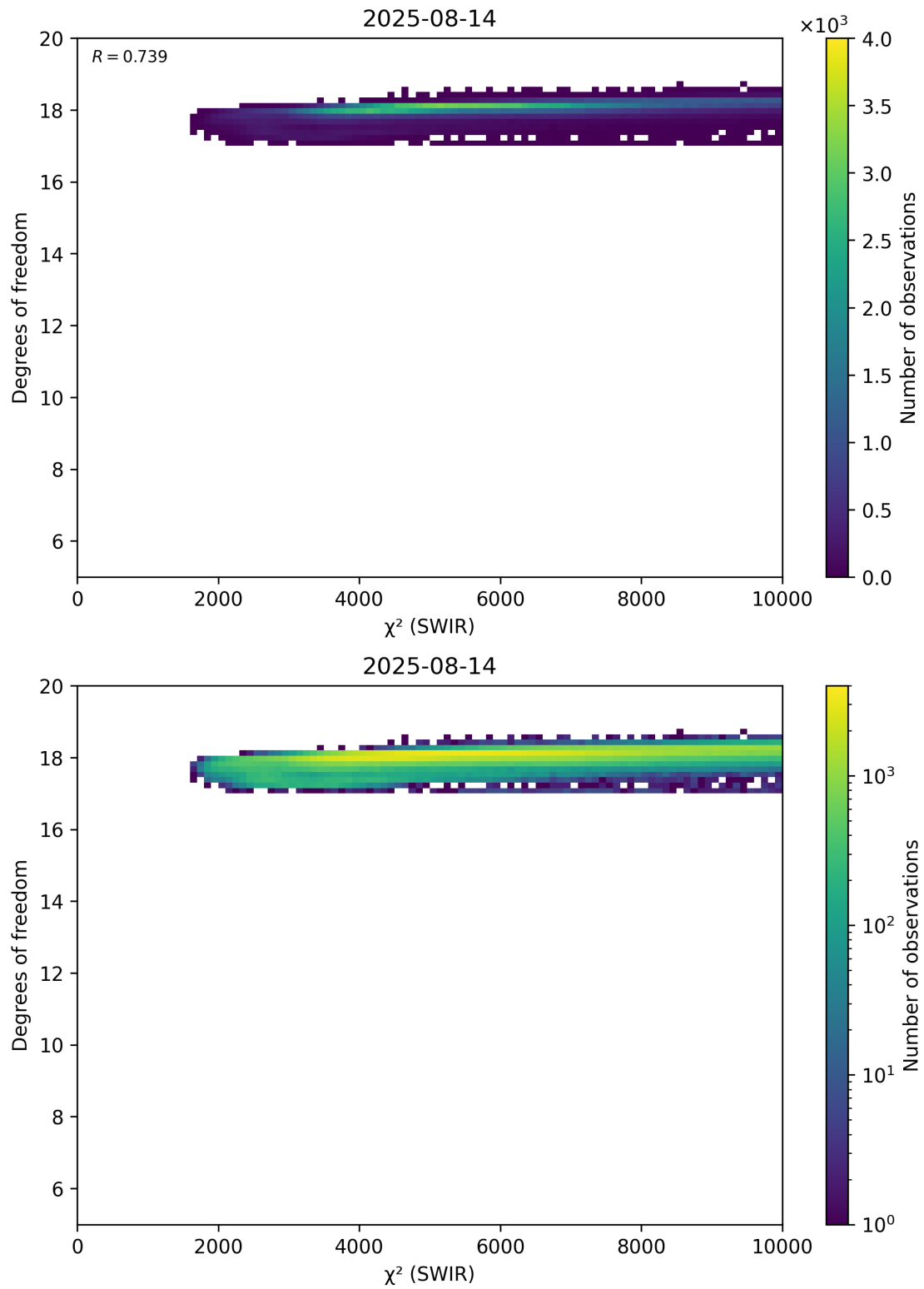
Figure 48: Scatter density plot of " \chi^2 (SWIR)" against "Degrees of freedom" for 2025-08-14 to 2025-08-15.
