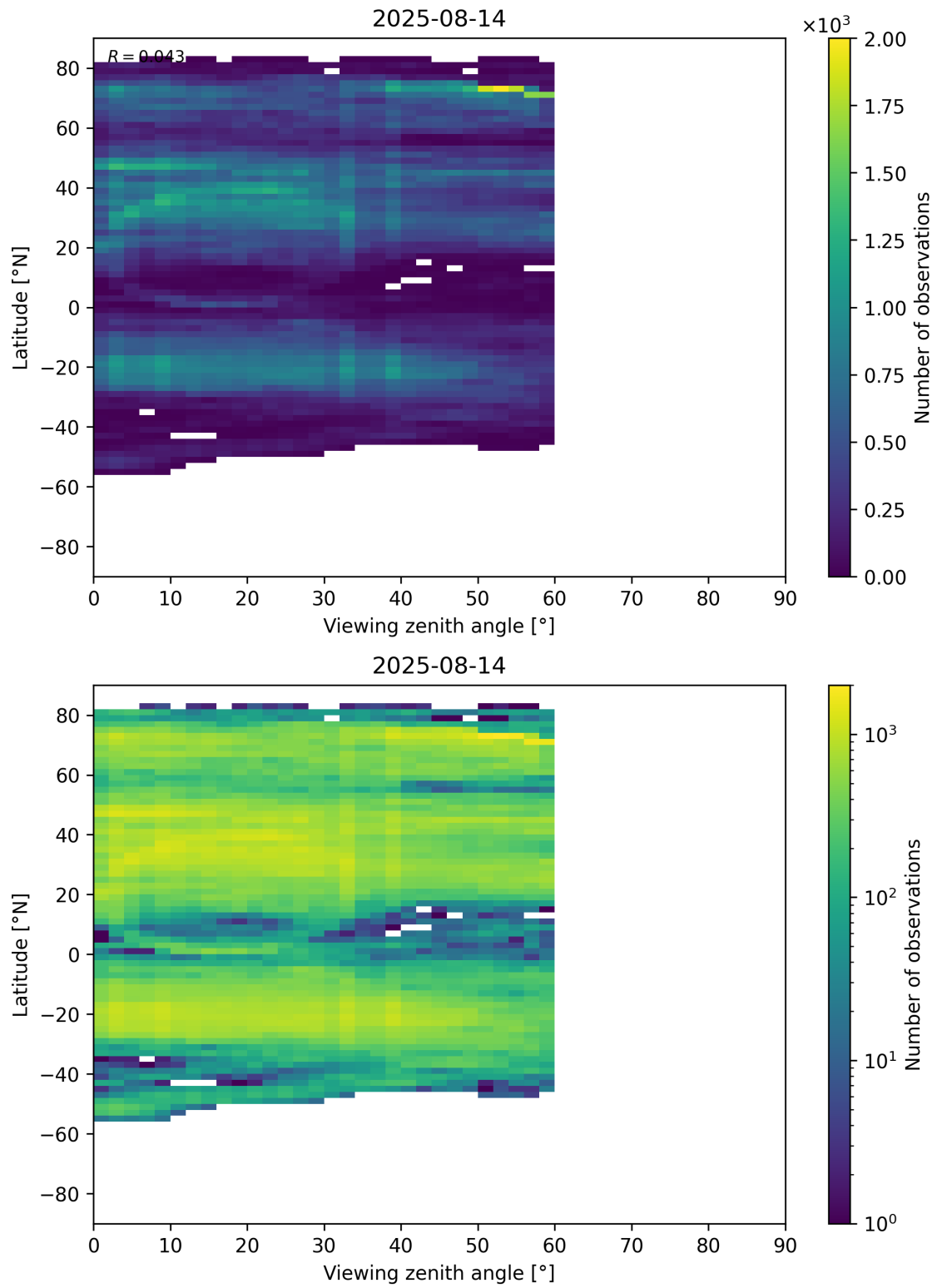
Figure 109: Scatter density plot of “Viewing zenith angle” against “Latitude” for 2025-08-14 to 2025-08-15.
