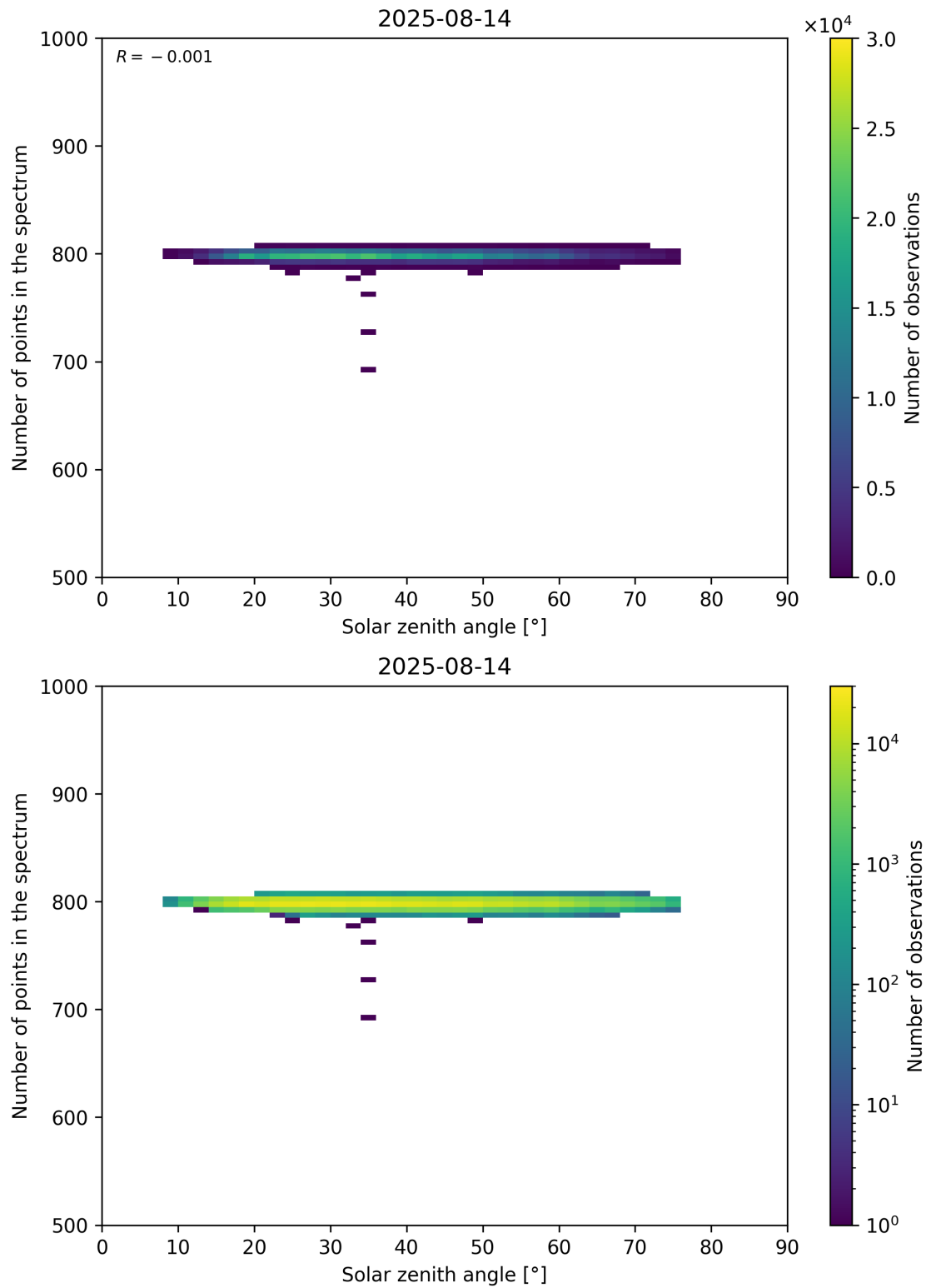
Figure 103: Scatter density plot of “Solar zenith angle” against “Number of points in the spectrum” for 2025-08-14 to 2025-08-15.
