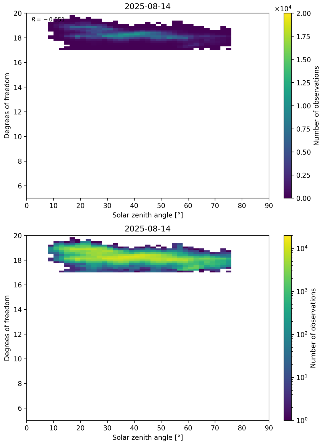
Figure 96: Scatter density plot of “Solar zenith angle” against “Degrees of freedom” for 2025-08-14 to 2025-08-15.
