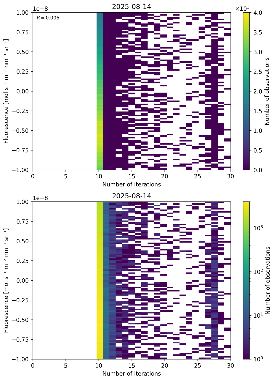
Figure 87: Scatter density plot of "Number of iterations" against "Fluorescence" for 2025-08-14 to 2025-08-15.
