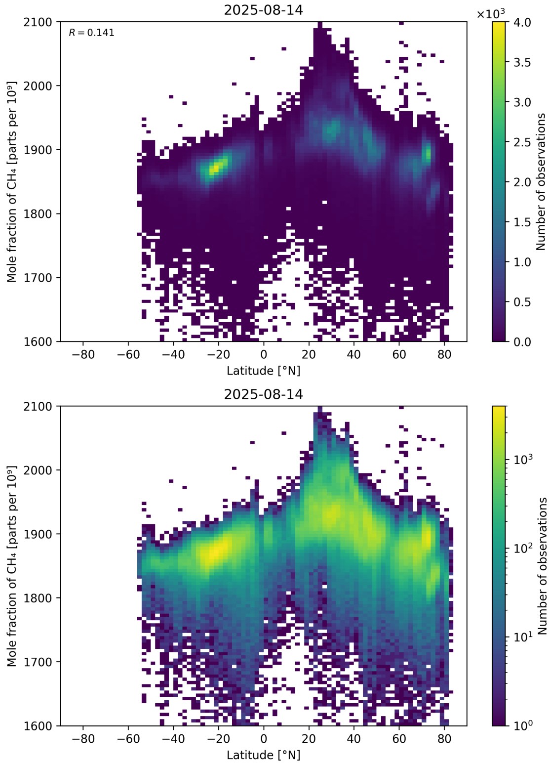
Figure 57: Scatter density plot of “Latitude” against “Mole fraction of CH 4 ” for 2025-08-14 to 2025-08-15.
