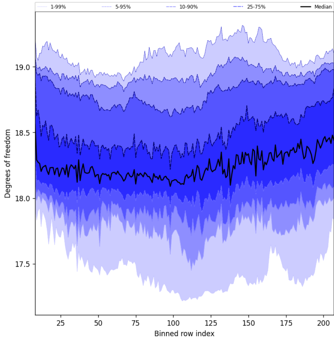
Figure 41: Along track statistics of “Degrees of freedom” for 2025-08-14 to 2025-08-15
