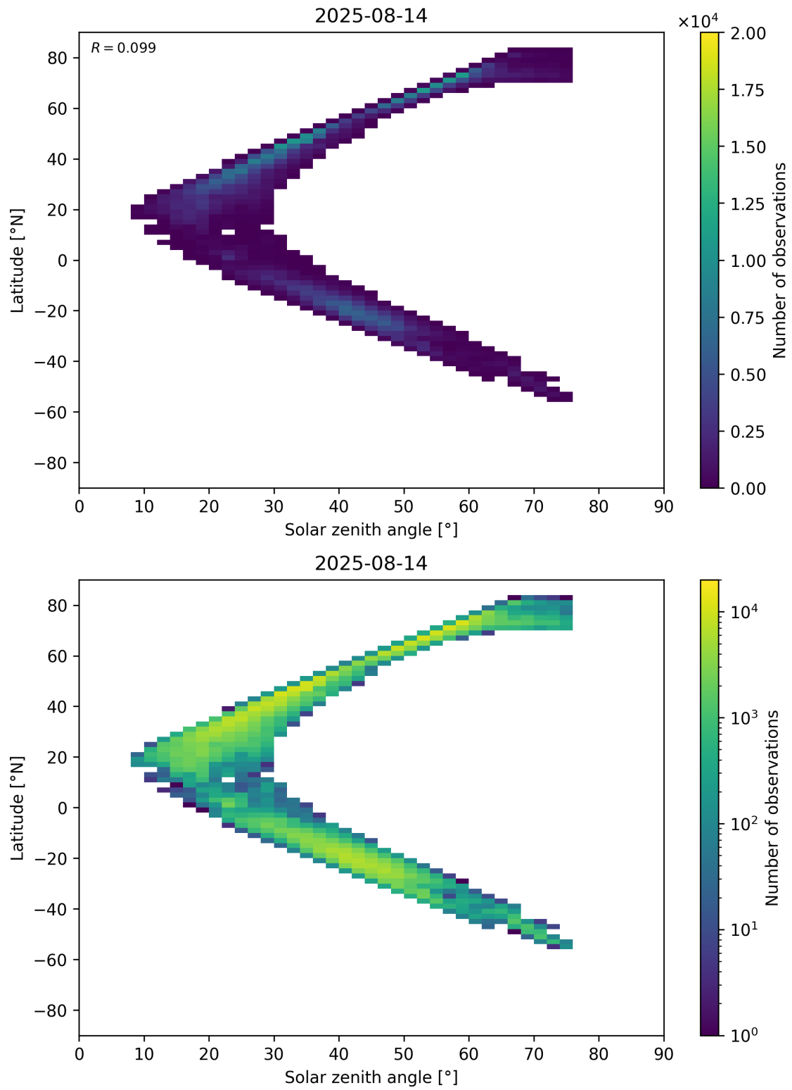
Figure 98: Scatter density plot of “Solar zenith angle” against “Latitude” for 2025-08-14 to 2025-08-15.
