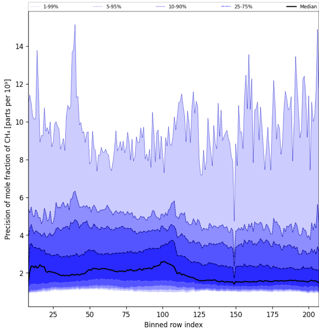
Figure 35: Along track statistics of “Precision of mole fraction of CH 4 ” for 2025-08-14 to 2025-08-15
