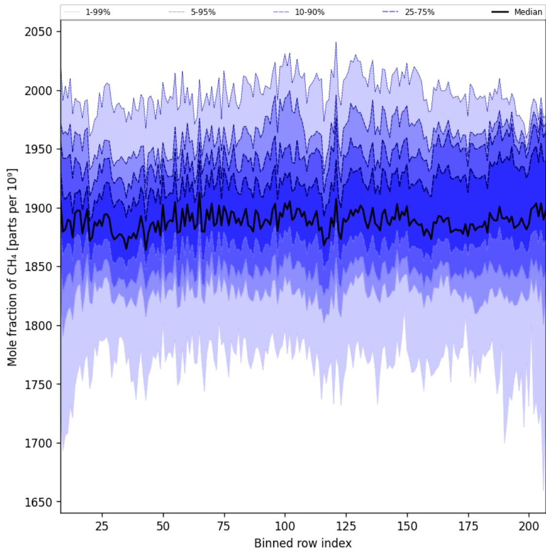
Figure 34: Along track statistics of “Mole fraction of CH 4 ” for 2025-08-14 to 2025-08-15
