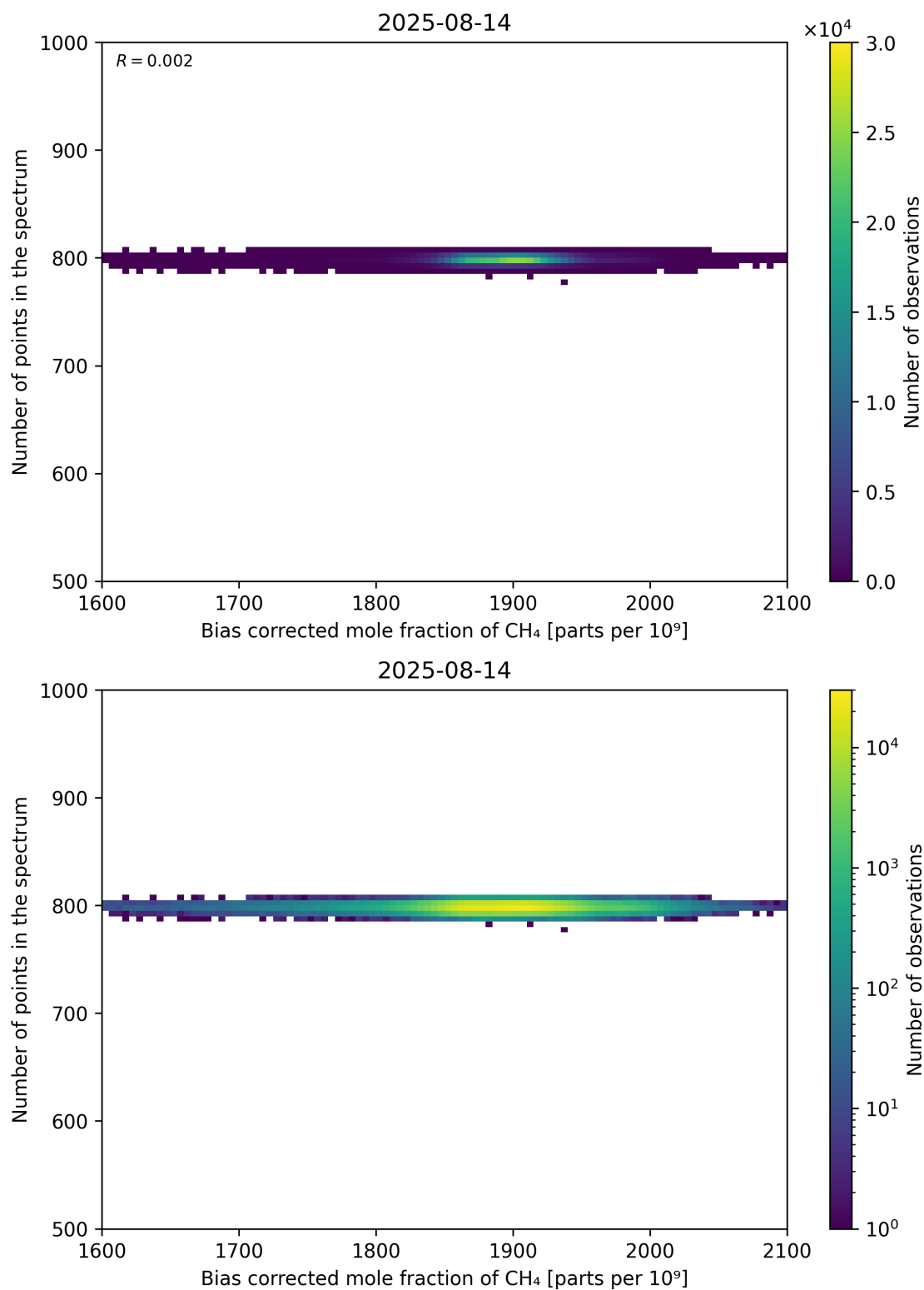
Figure 68: Scatter density plot of “Bias corrected mole fraction of CH 4 ” against “Number of points in the spectrum” for 2025-08-14 to 2025-08-15.
