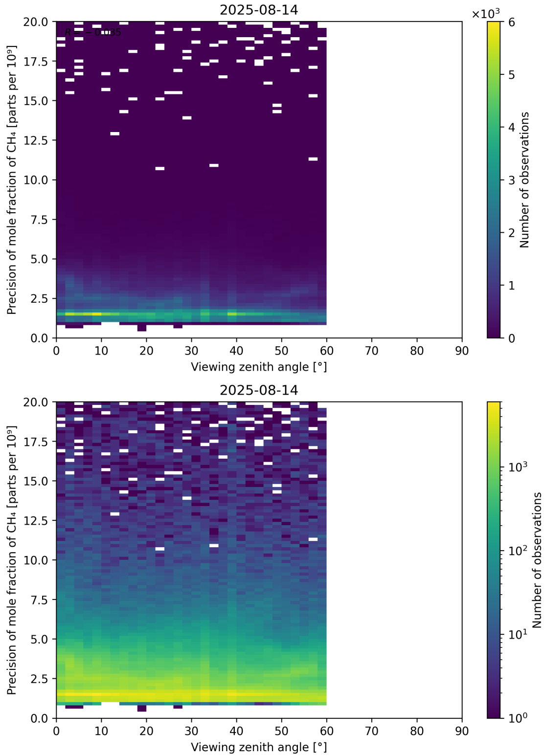
Figure 112: Scatter density plot of “Viewing zenith angle” against “Precision of mole fraction of CH 4 ” for 2025-08-14 to 2025-08-15.
