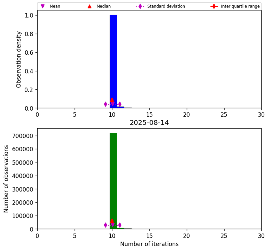
Figure 31: Histogram of “Number of iterations” for 2025-08-14 to 2025-08-15
