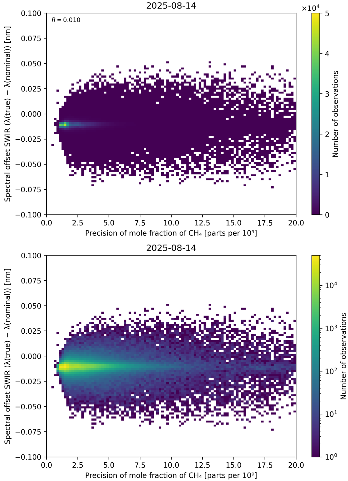
Figure 85: Scatter density plot of “Precision of mole fraction of CH 4 ” against “Spectral offset SWIR ( \lambda_{\text{true}} - \lambda_{\text{nominal}} )” for 2025-08-14 to 2025-08-15.
