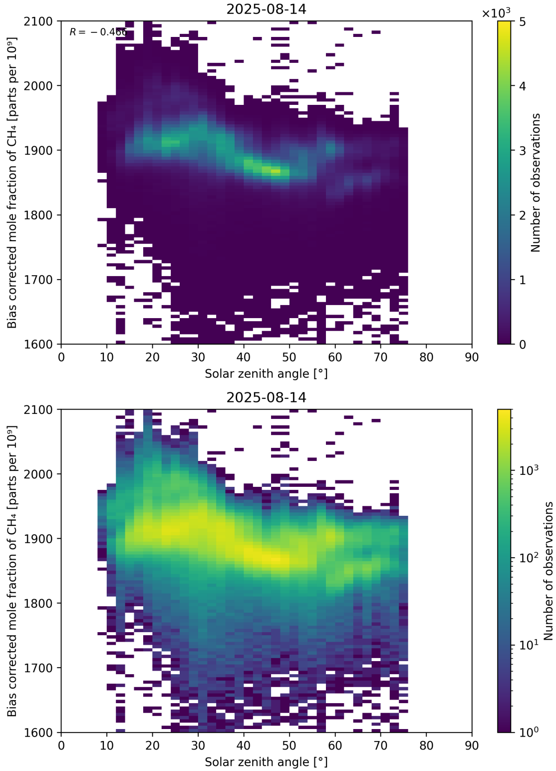
Figure 100: Scatter density plot of “Solar zenith angle” against “Bias corrected mole fraction of CH 4 ” for 2025-08-14 to 2025-08-15.
