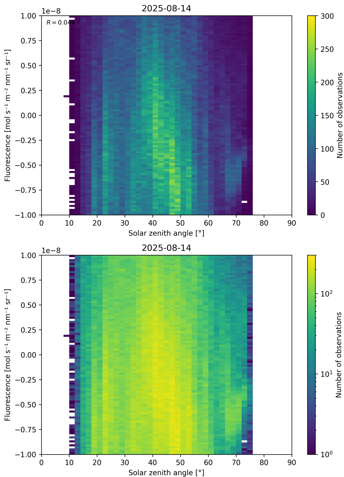
Figure 97: Scatter density plot of “Solar zenith angle” against “Fluorescence” for 2025-08-14 to 2025-08-15.
