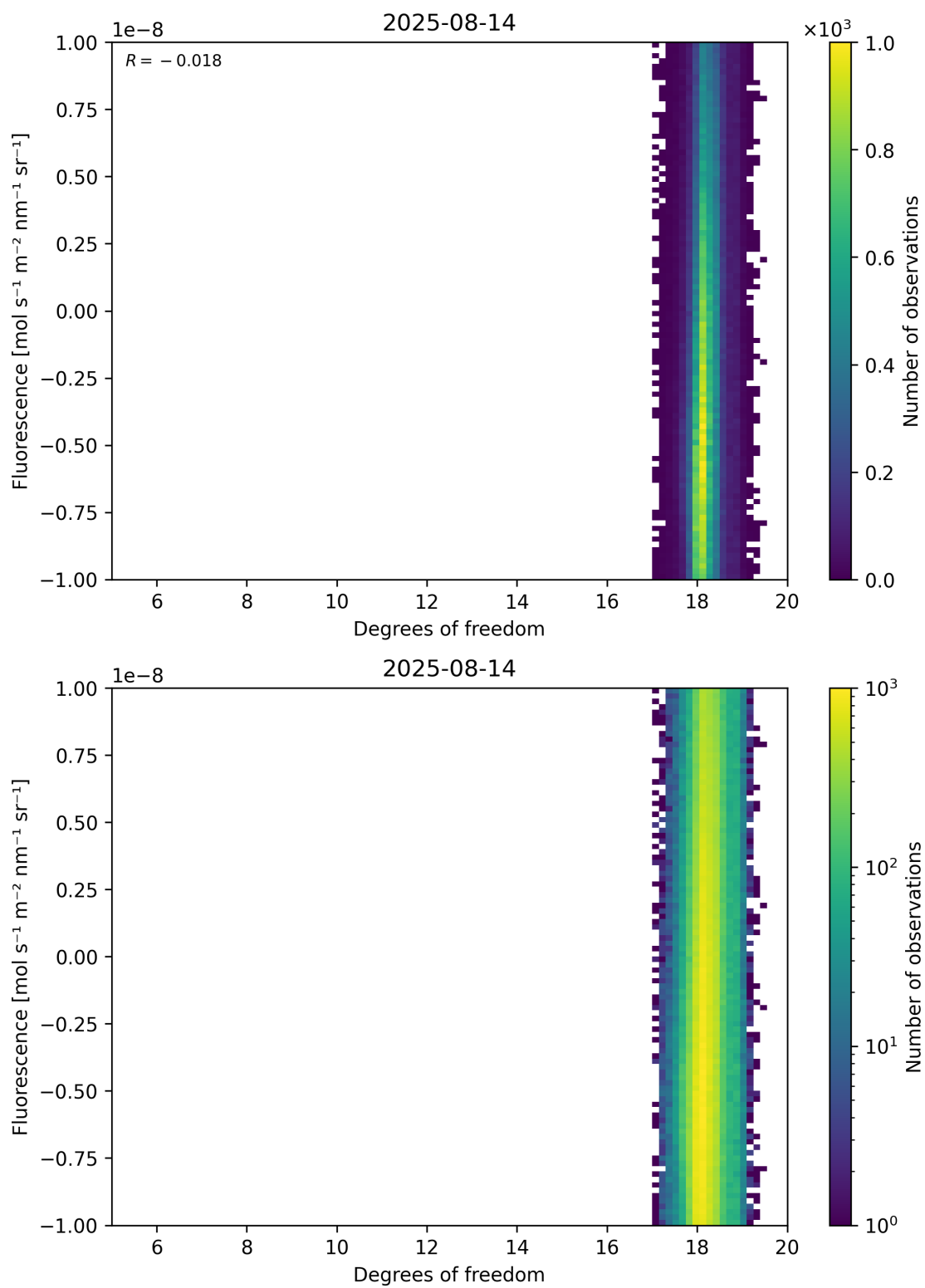
Figure 51: Scatter density plot of “Degrees of freedom” against “Fluorescence” for 2025-08-14 to 2025-08-15.
