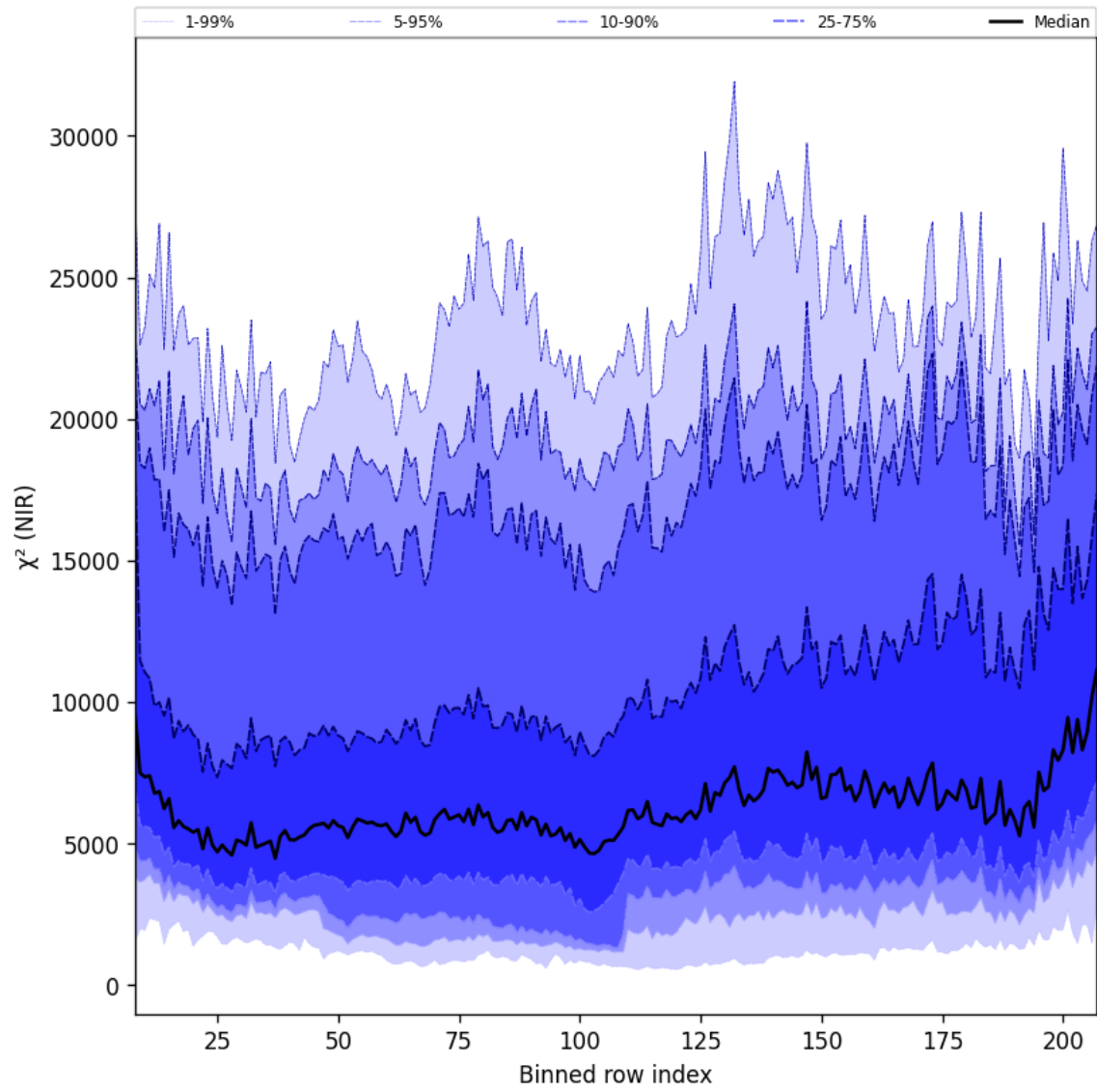
Figure 40: Along track statistics of “ \chi^2 (NIR)” for 2025-08-14 to 2025-08-15
