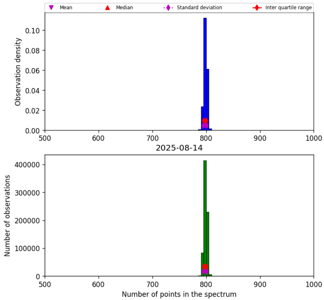
Figure 26: Histogram of “Number of points in the spectrum” for 2025-08-14 to 2025-08-15
