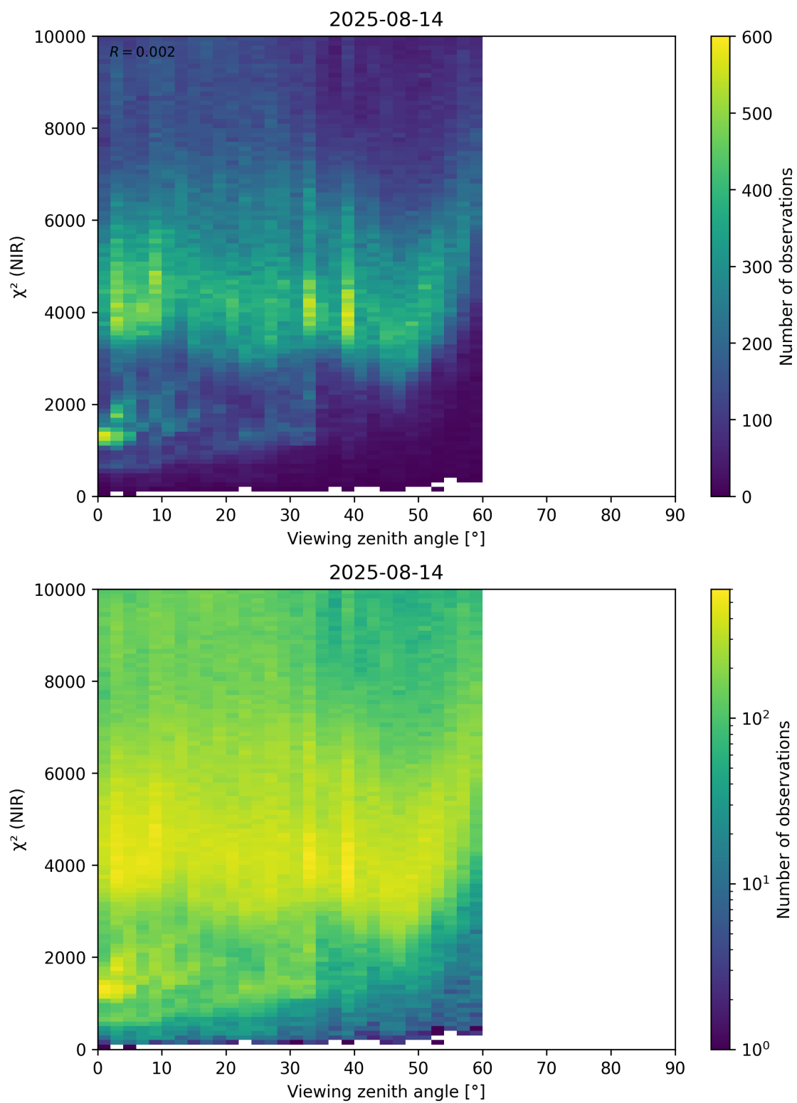
Figure 105: Scatter density plot of “Viewing zenith angle” against “ \chi^2 (NIR)” for 2025-08-14 to 2025-08-15.
