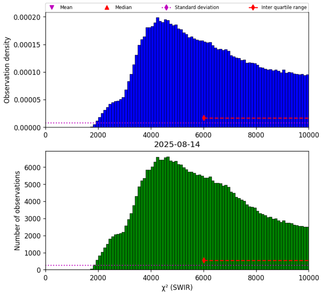
Figure 28: Histogram of “ \chi^2 (SWIR)” for 2025-08-14 to 2025-08-15
