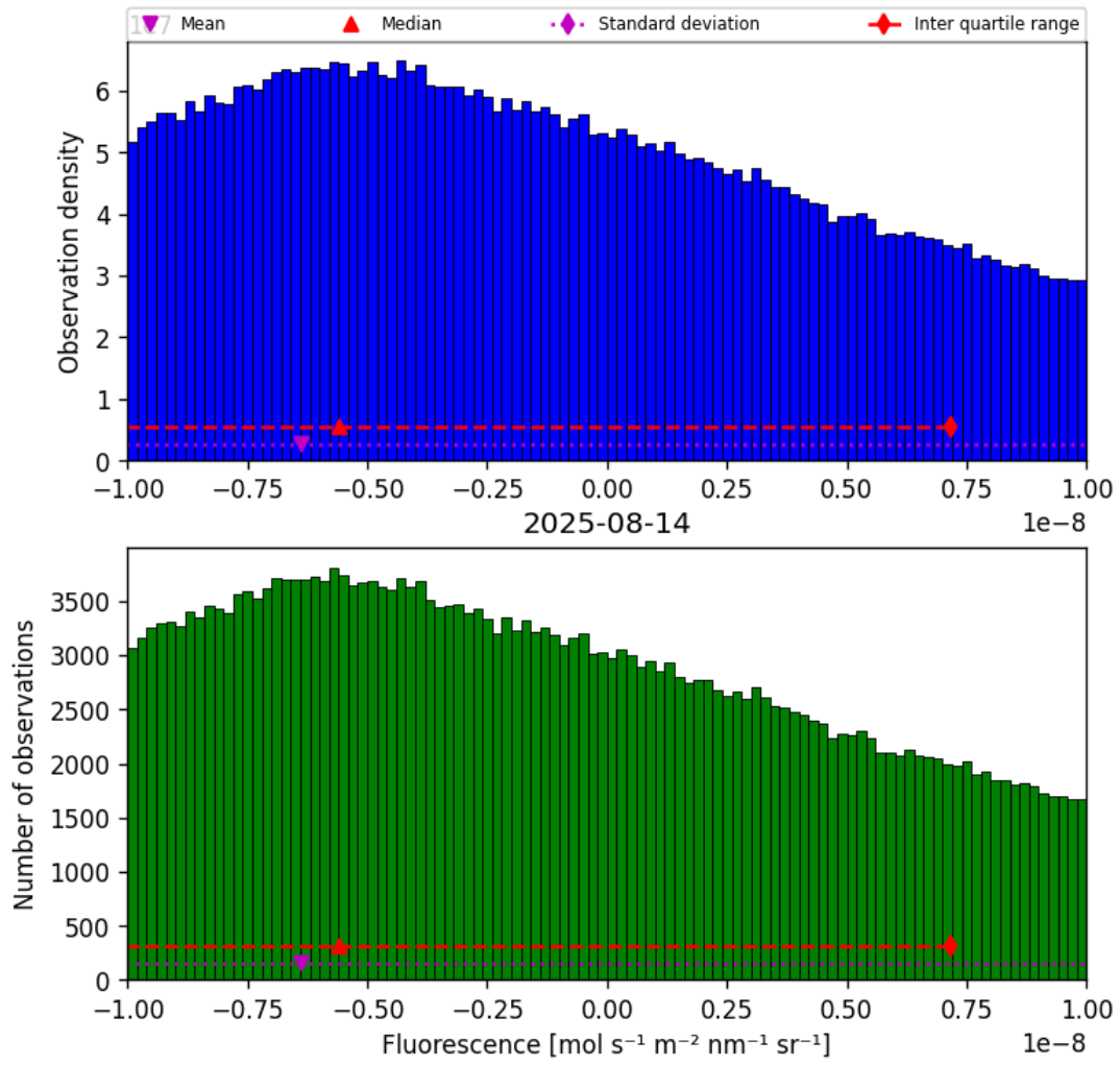
Figure 32: Histogram of “Fluorescence” for 2025-08-14 to 2025-08-15
