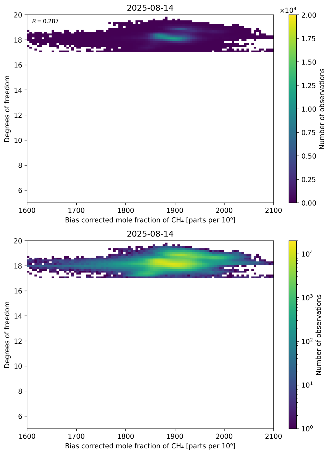
Figure 65: Scatter density plot of “Bias corrected mole fraction of CH 4 ” against “Degrees of freedom” for 2025-08-14 to 2025-08-15.
