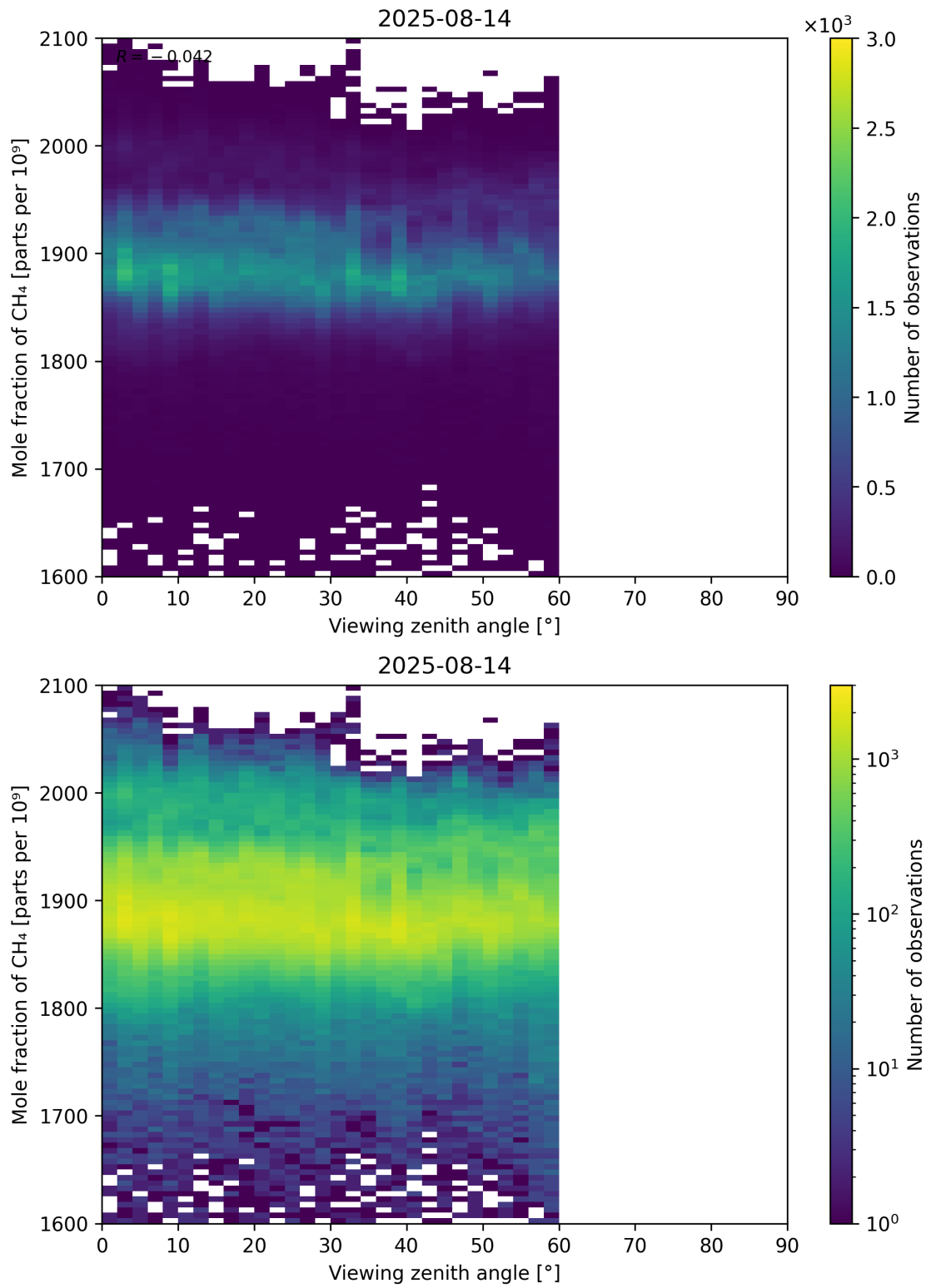
Figure 110: Scatter density plot of “Viewing zenith angle” against “Mole fraction of CH 4 ” for 2025-08-14 to 2025-08-15.
