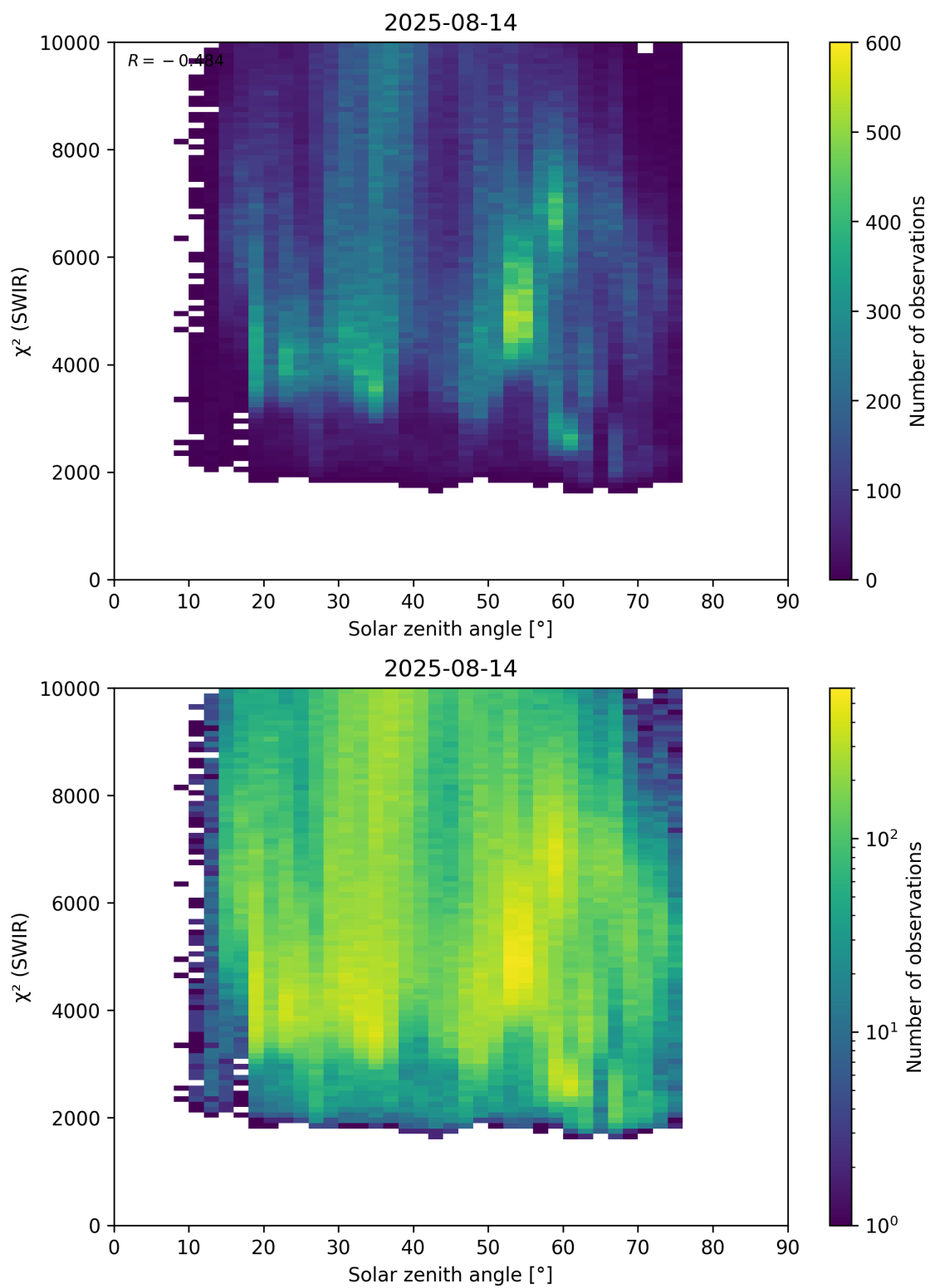
Figure 95: Scatter density plot of “Solar zenith angle” against “ \chi^2 (SWIR)” for 2025-08-14 to 2025-08-15.
