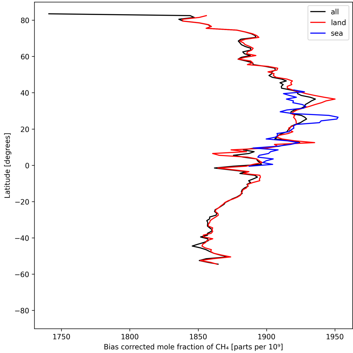
Figure 14: Zonal average of “Bias corrected mole fraction of CH 4 ” for 2025-08-14 to 2025-08-15.
