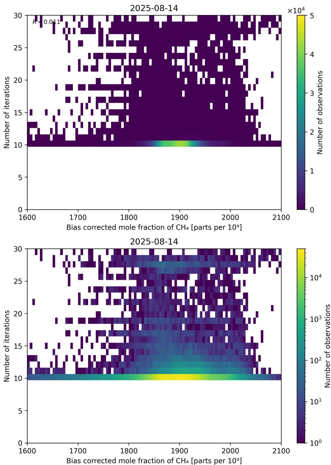
Figure 67: Scatter density plot of “Bias corrected mole fraction of CH 4 ” against “Number of iterations” for 2025-08-14 to 2025-08-15.
