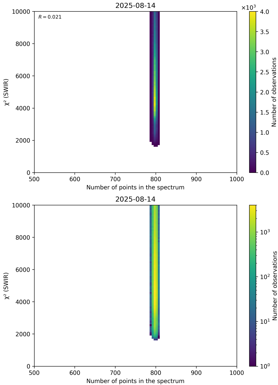
Figure 89: Scatter density plot of “Number of points in the spectrum” against “ \chi^2 (SWIR)” for 2025-08-14 to 2025-08-15.
