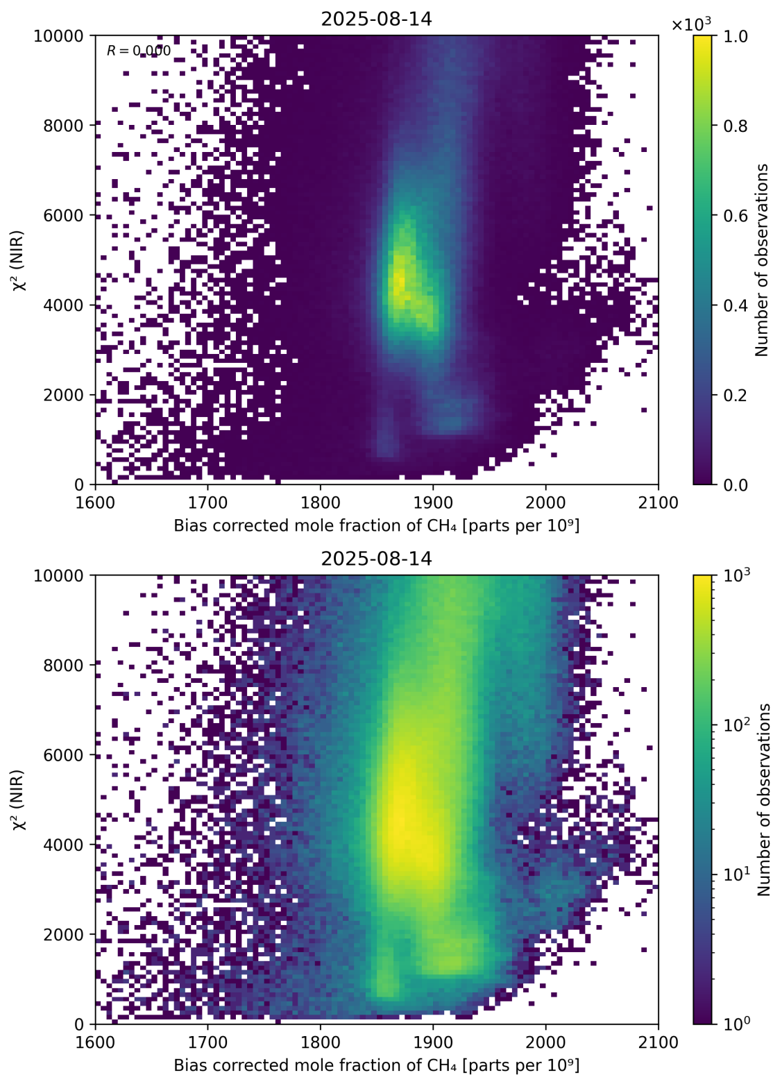
Figure 63: Scatter density plot of “Bias corrected mole fraction of \text{CH}_4 ” against “ \chi^2 (NIR)” for 2025-08-14 to 2025-08-15.
