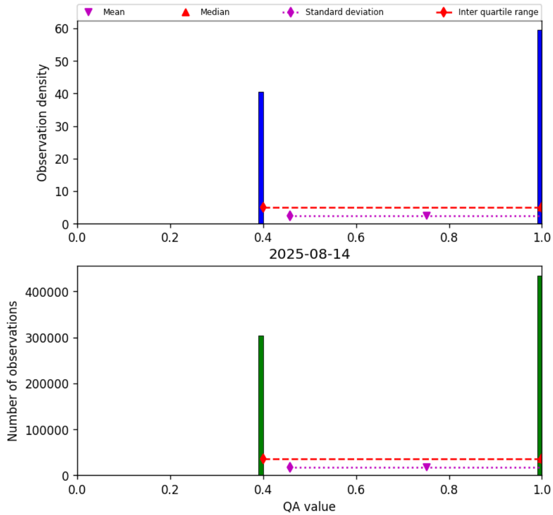
Figure 22: Histogram of “QA value” for 2025-08-14 to 2025-08-15
