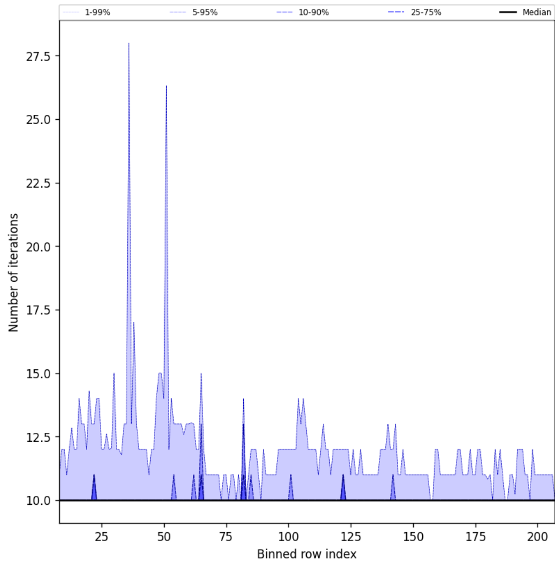
Figure 42: Along track statistics of “Number of iterations” for 2025-08-14 to 2025-08-15
