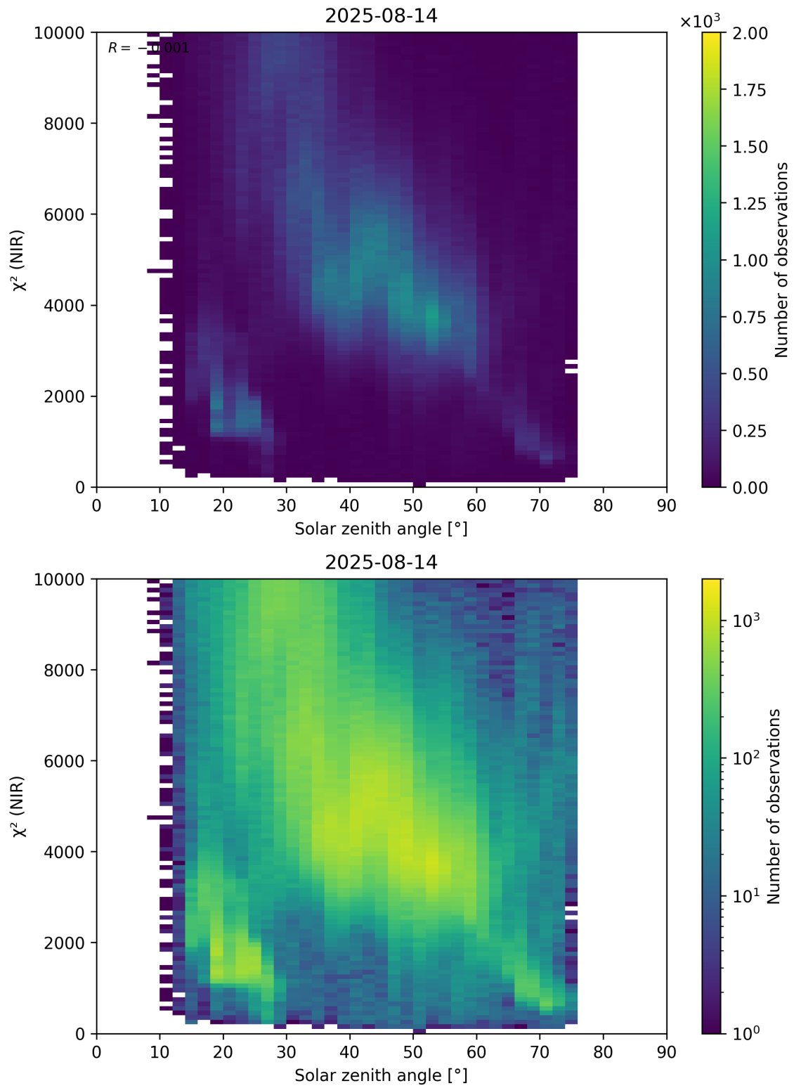
Figure 94: Scatter density plot of “Solar zenith angle” against “ \chi^2 (NIR)” for 2025-08-14 to 2025-08-15.
