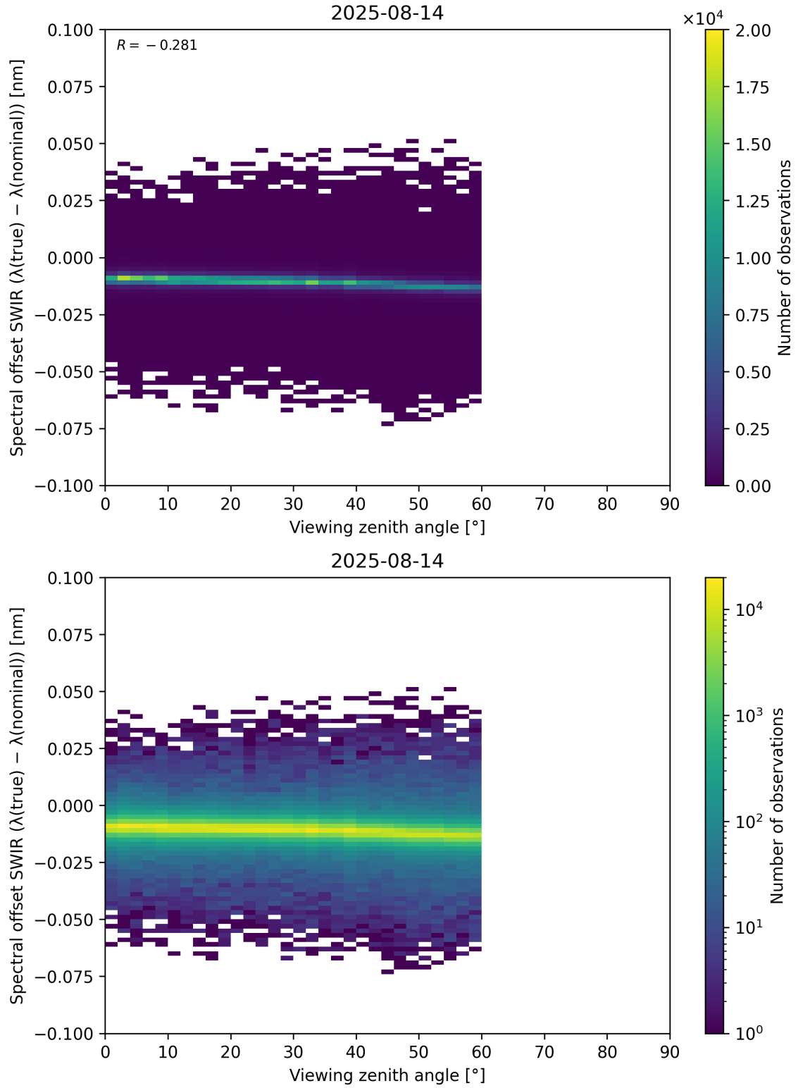
Figure 116: Scatter density plot of “Viewing zenith angle” against “Spectral offset SWIR ( \lambda_{\text{true}} - \lambda_{\text{nominal}} )” for 2025-08-14 to 2025-08-15.
