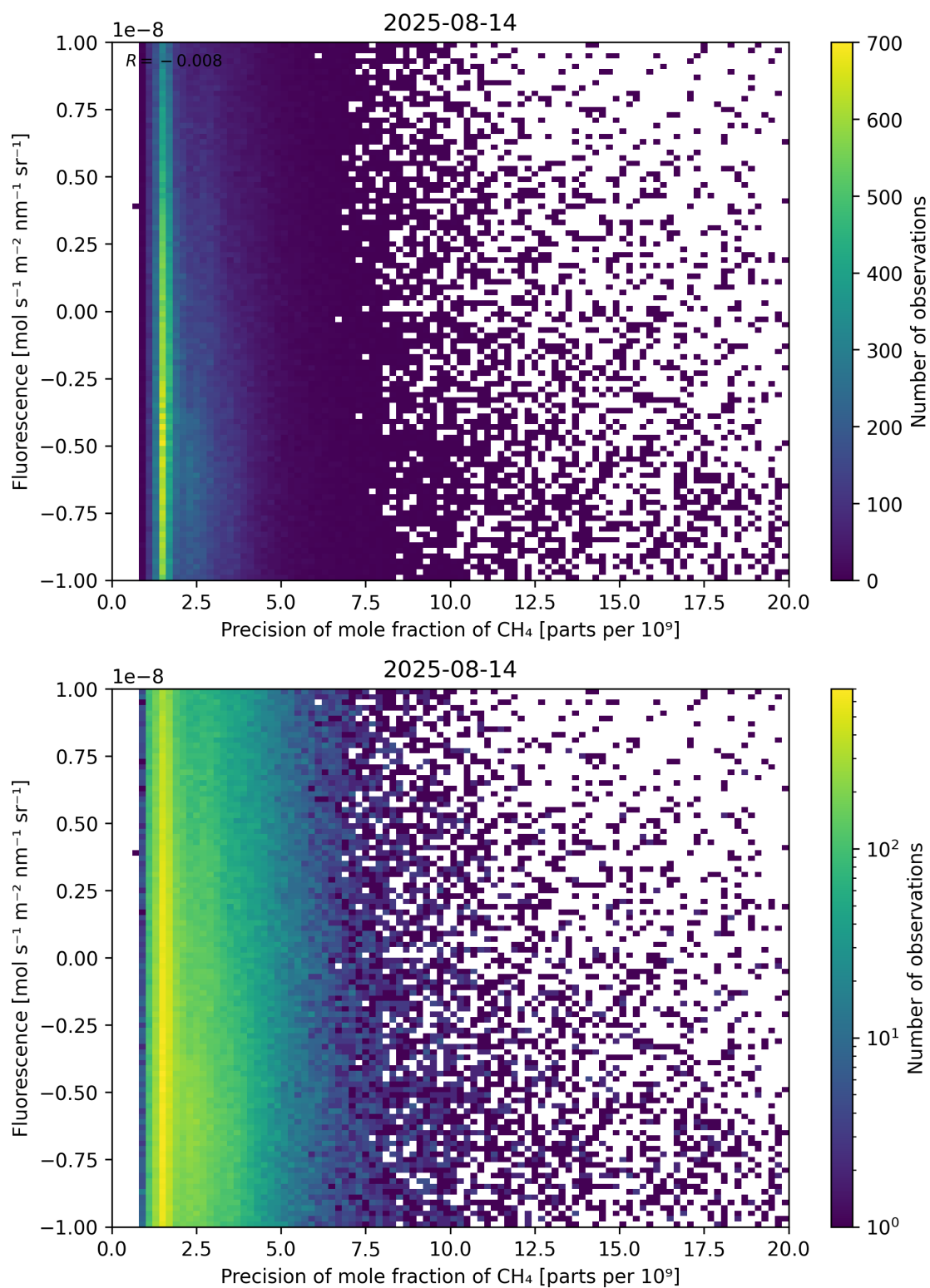
Figure 81: Scatter density plot of “Precision of mole fraction of CH 4 ” against “Fluorescence” for 2025-08-14 to 2025-08-15.
