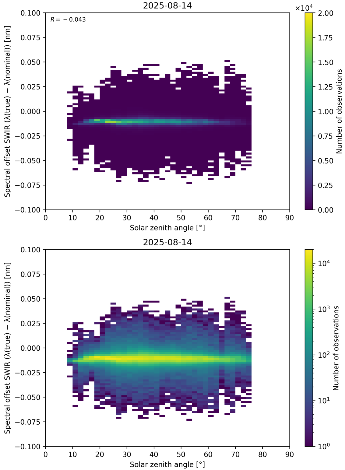
Figure 104: Scatter density plot of “Solar zenith angle” against “Spectral offset SWIR ( \lambda_{\text{true}} - \lambda_{\text{nominal}} )” for 2025-08-14 to 2025-08-15.
