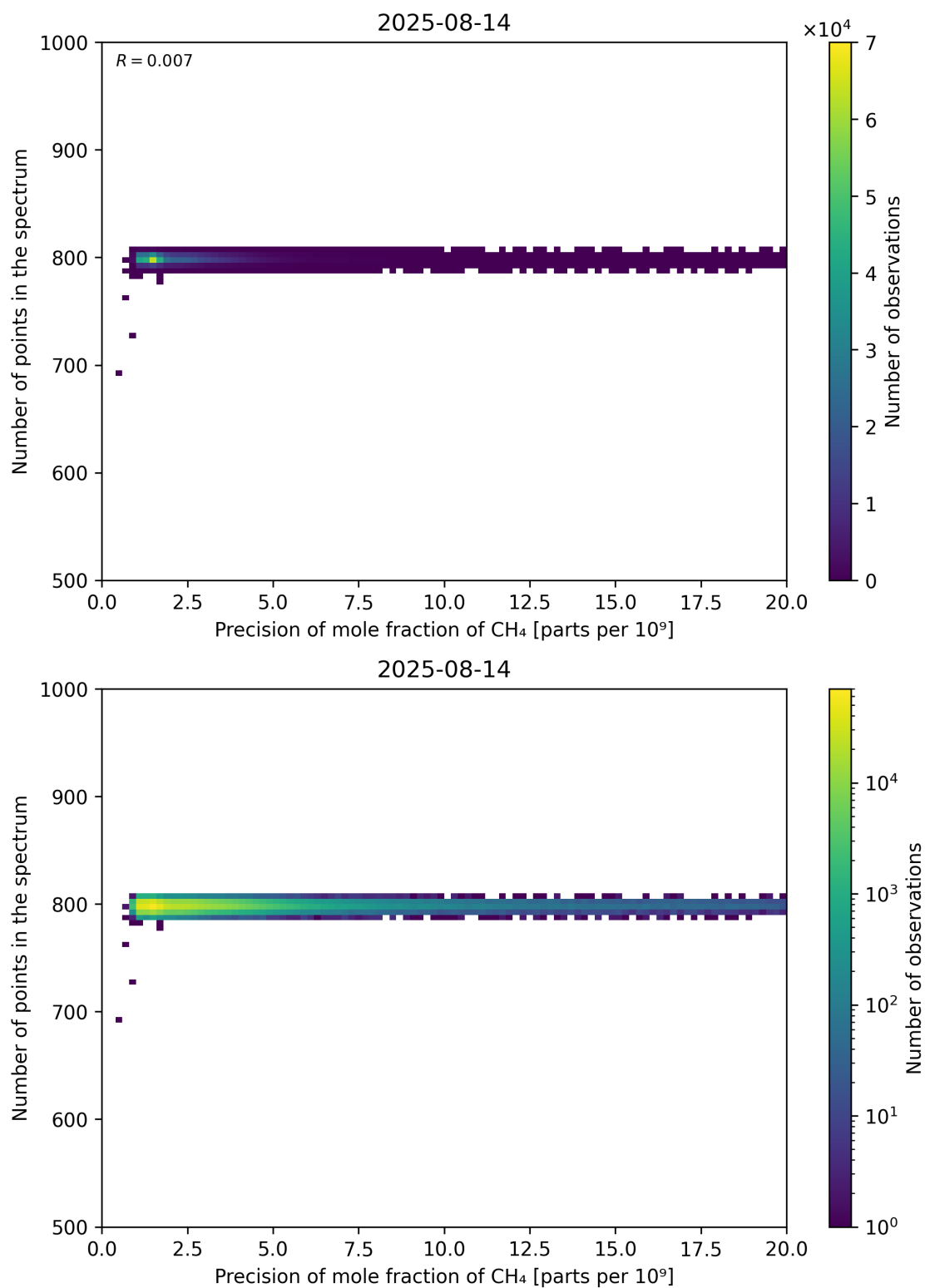
Figure 84: Scatter density plot of “Precision of mole fraction of CH 4 ” against “Number of points in the spectrum” for 2025-08-14 to 2025-08-15.
