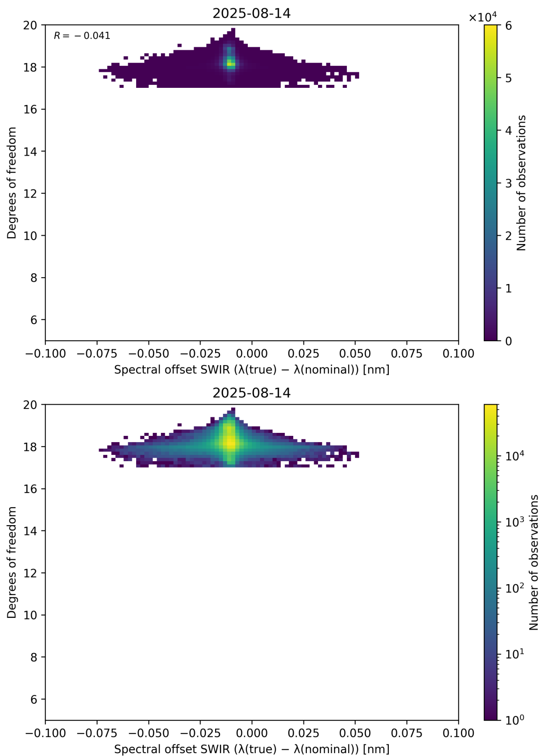
Figure 119: Scatter density plot of “Spectral offset SWIR ( \lambda_{\text{true}} - \lambda_{\text{nominal}} )” against “Degrees of freedom” for 2025-08-14 to 2025-08-15.
