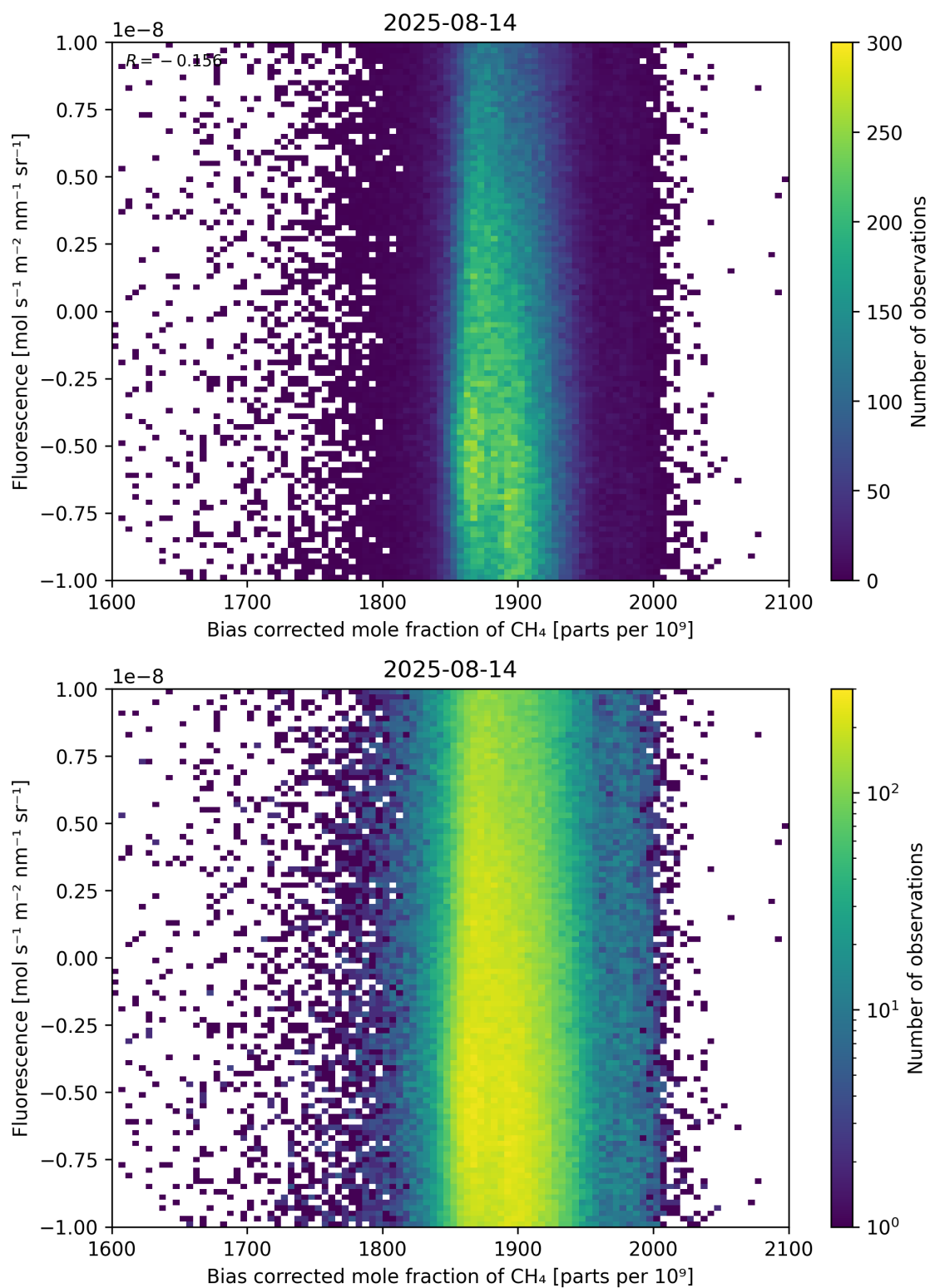
Figure 66: Scatter density plot of “Bias corrected mole fraction of \text{CH}_4 ” against “Fluorescence” for 2025-08-14 to 2025-08-15.
