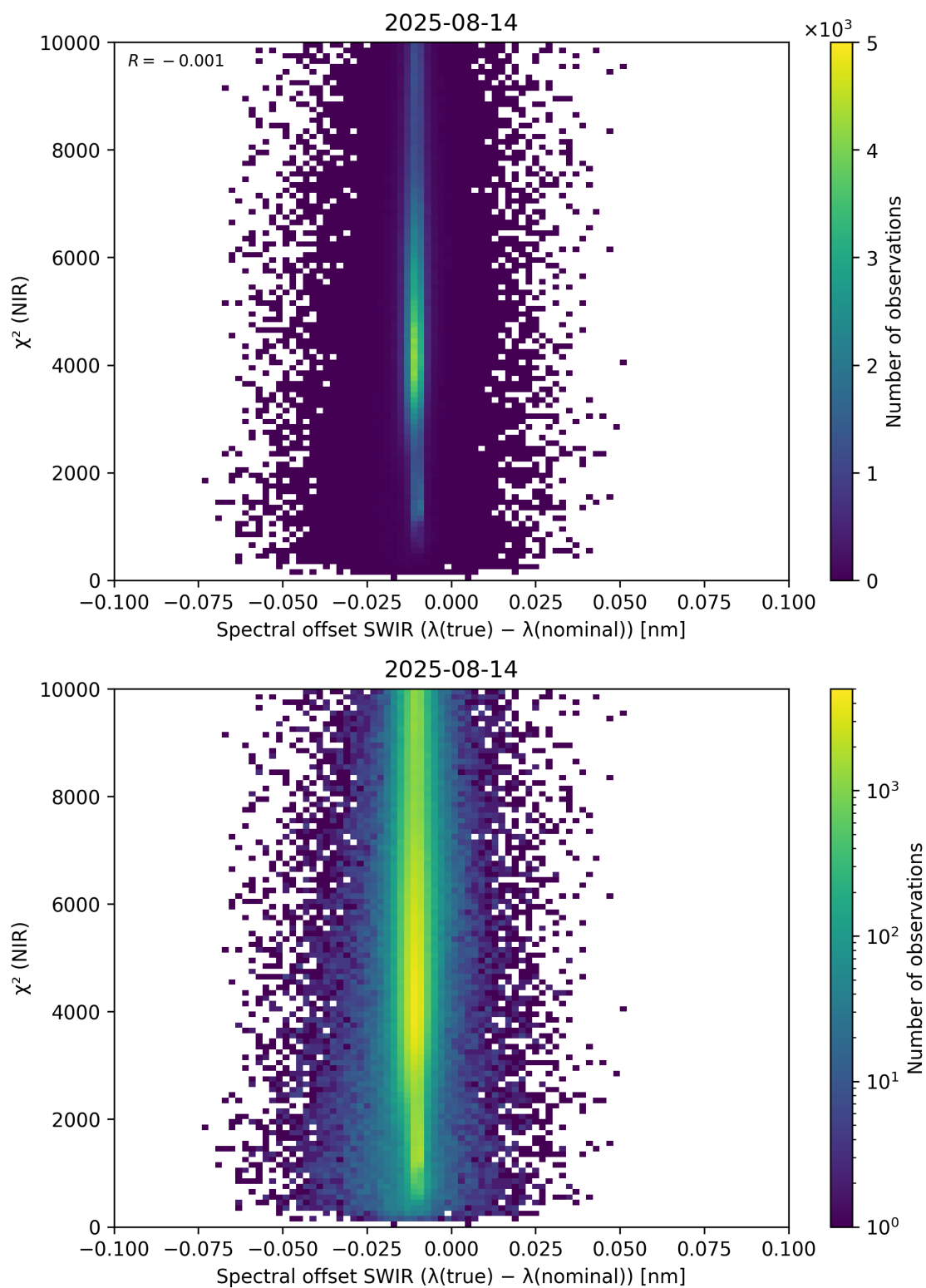
Figure 117: Scatter density plot of “Spectral offset SWIR ( \lambda_{\text{true}} - \lambda_{\text{nominal}} )” against “ \chi^2 (NIR)” for 2025-08-14 to 2025-08-15.
