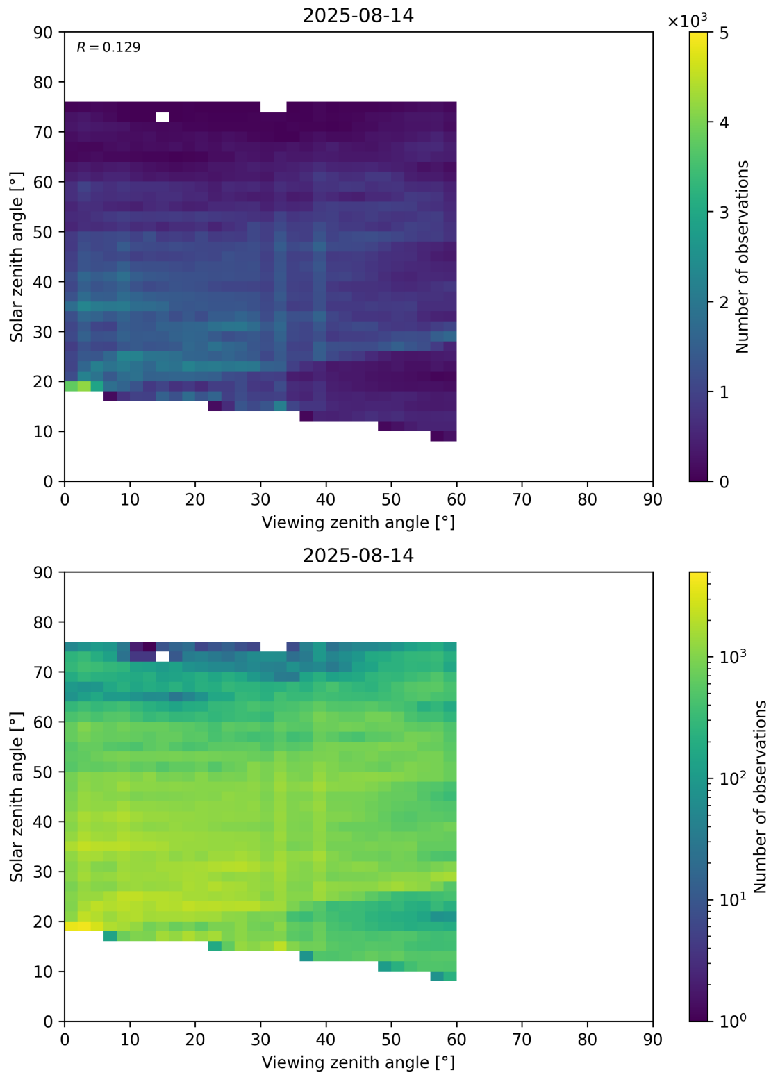
Figure 115: Scatter density plot of “Viewing zenith angle” against “Solar zenith angle” for 2025-08-14 to 2025-08-15.
