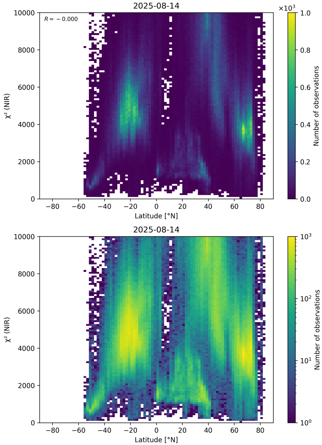
Figure 53: Scatter density plot of “Latitude” against “ \chi^2 (NIR)” for 2025-08-14 to 2025-08-15.
