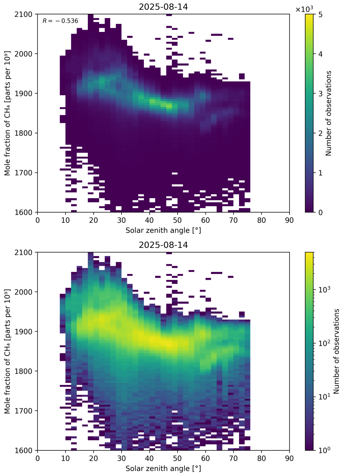
Figure 99: Scatter density plot of “Solar zenith angle” against “Mole fraction of \text{CH}_4 ” for 2025-08-14 to 2025-08-15.
