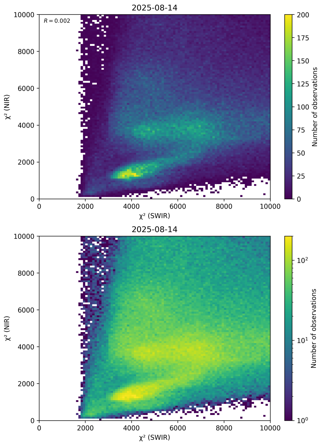
Figure 47: Scatter density plot of “ \chi^2 (SWIR)” against “ \chi^2 (NIR)” for 2025-08-14 to 2025-08-15.
