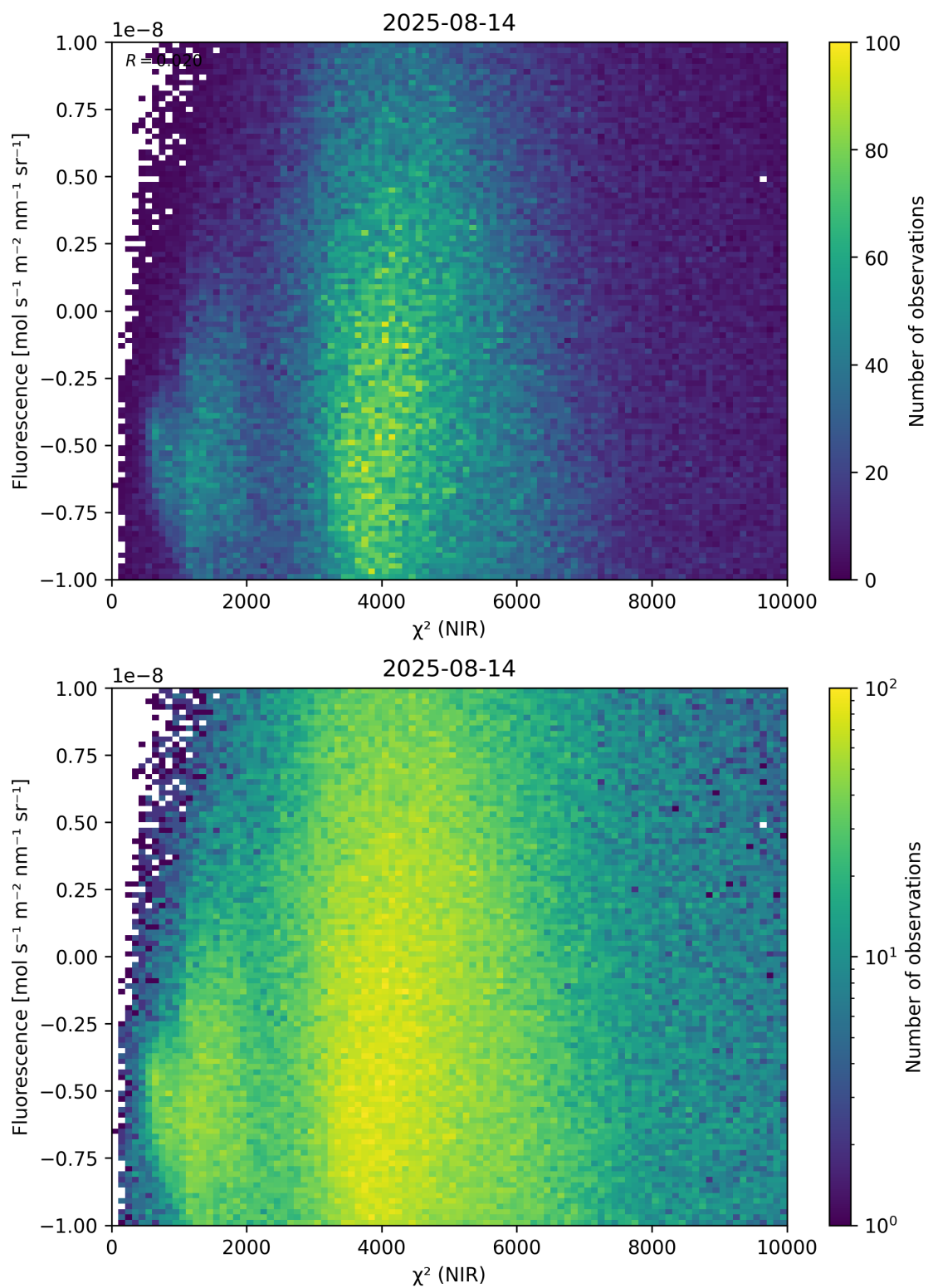
Figure 45: Scatter density plot of “ \chi^2 (NIR)” against “Fluorescence” for 2025-08-14 to 2025-08-15.
