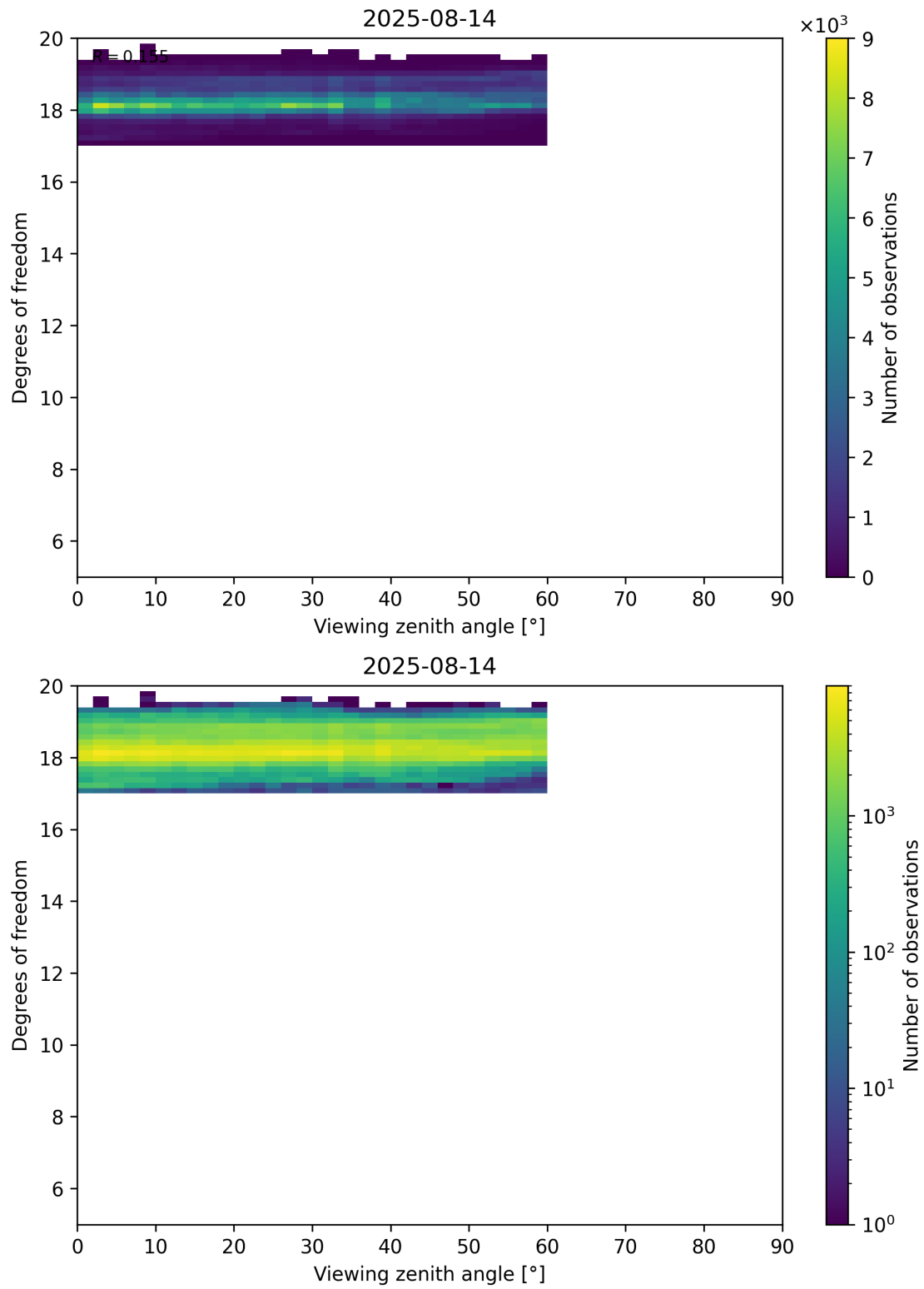
Figure 107: Scatter density plot of “Viewing zenith angle” against “Degrees of freedom” for 2025-08-14 to 2025-08-15.
