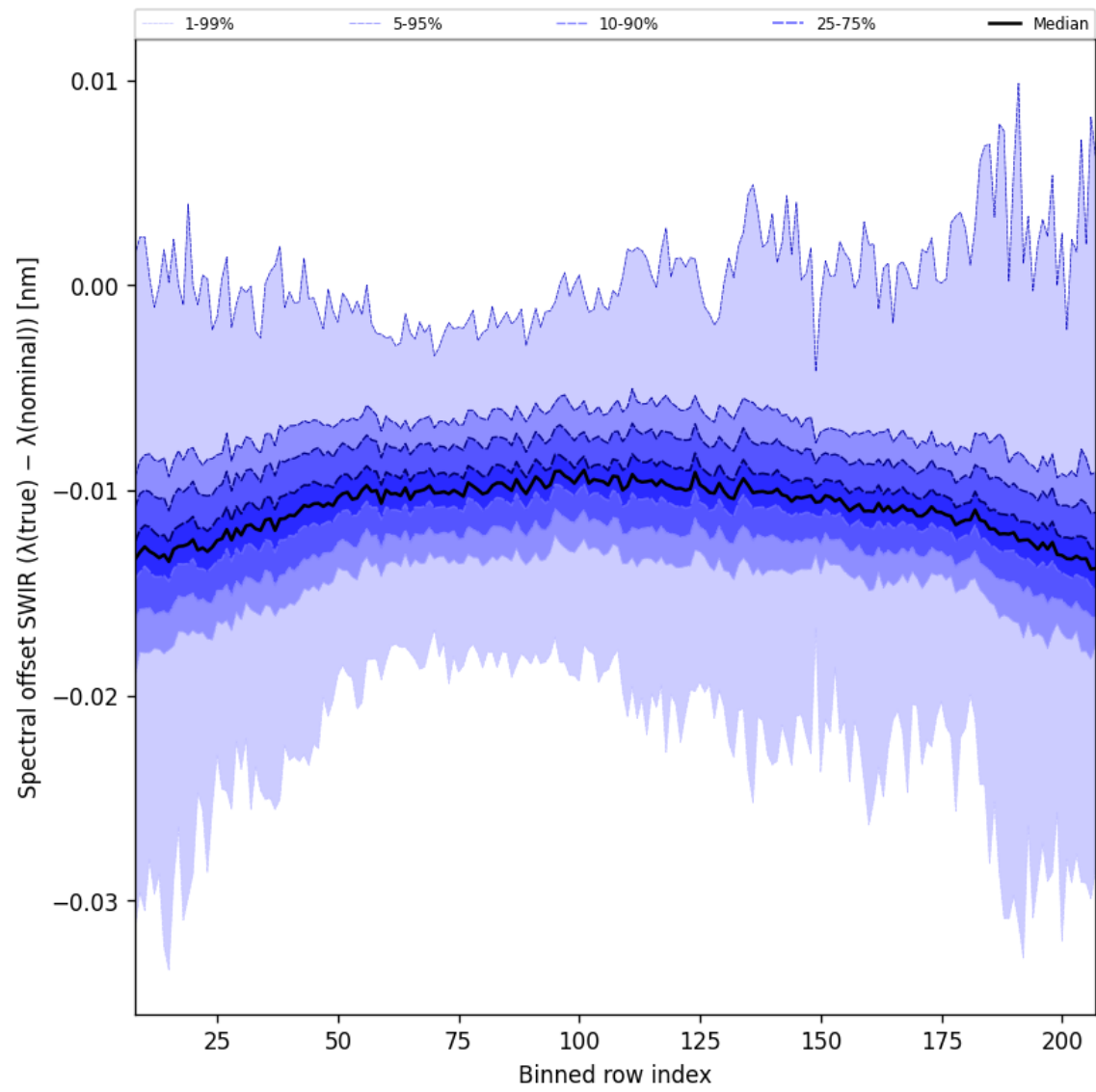
Figure 38: Along track statistics of “Spectral offset SWIR ( \lambda_{\text{true}} - \lambda_{\text{nominal}} )” for 2025-08-14 to 2025-08-15
