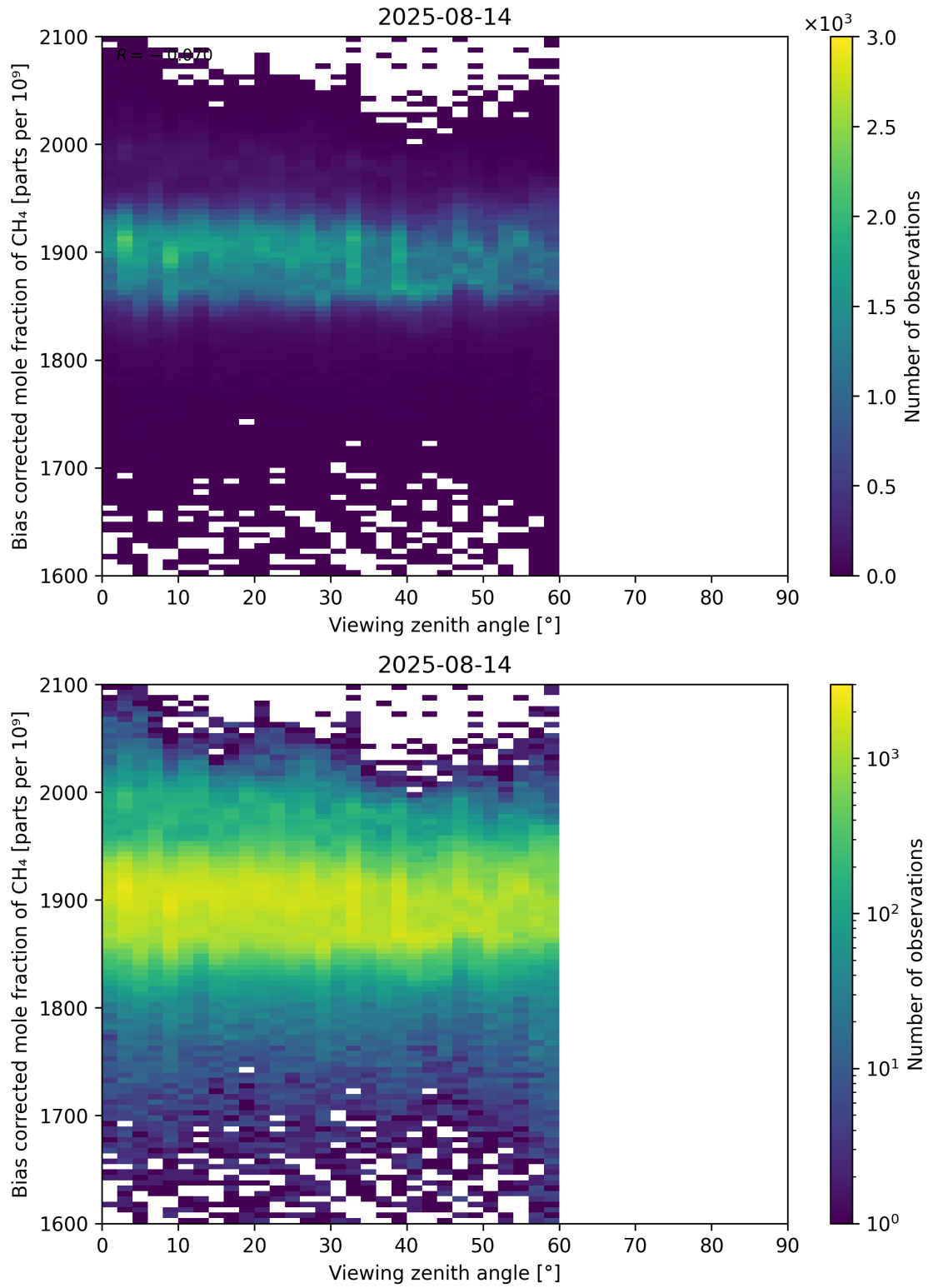
Figure 111: Scatter density plot of “Viewing zenith angle” against “Bias corrected mole fraction of CH 4 ” for 2025-08-14 to 2025-08-15.
