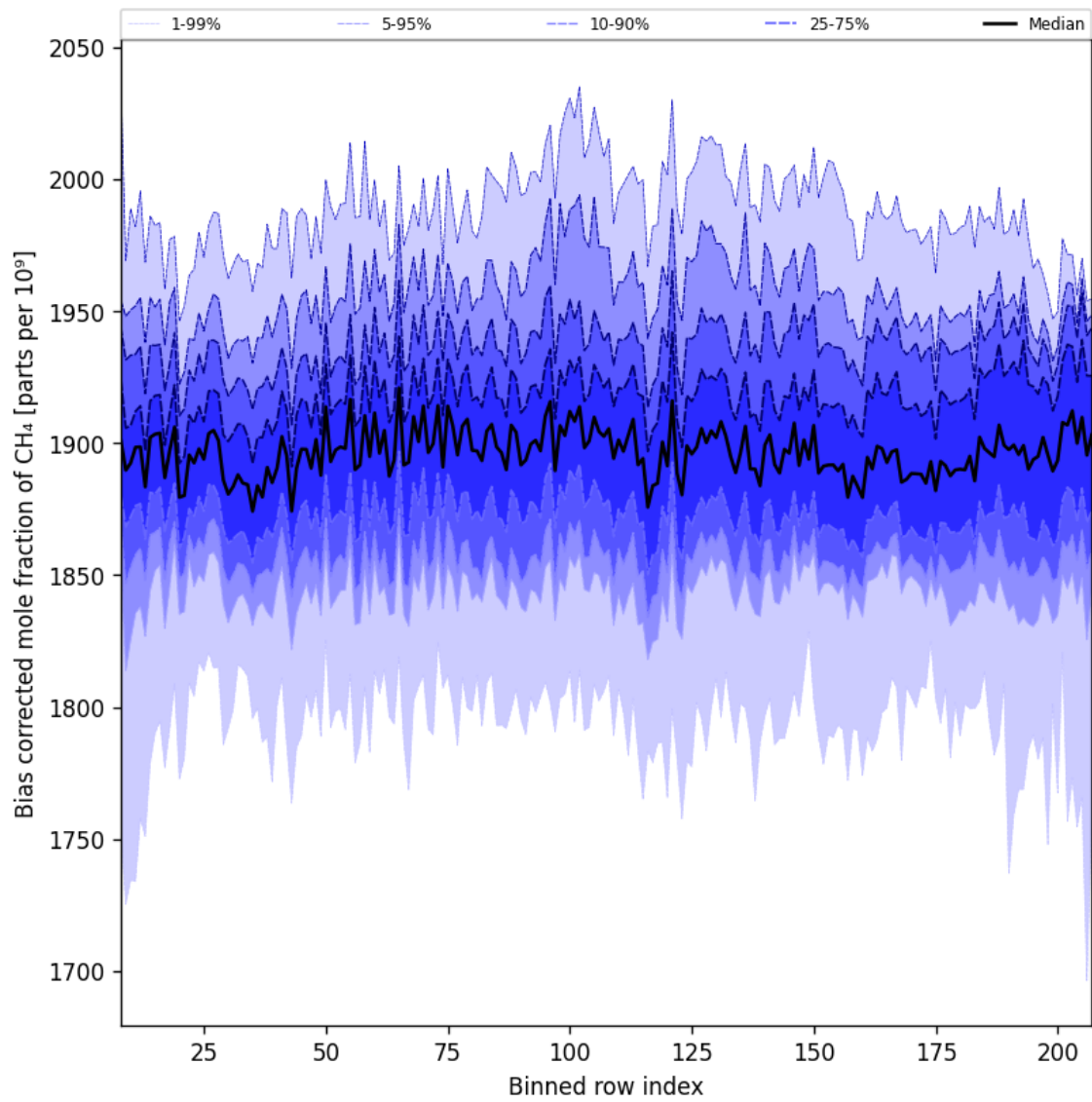
Figure 36: Along track statistics of “Bias corrected mole fraction of CH 4 ” for 2025-08-14 to 2025-08-15
