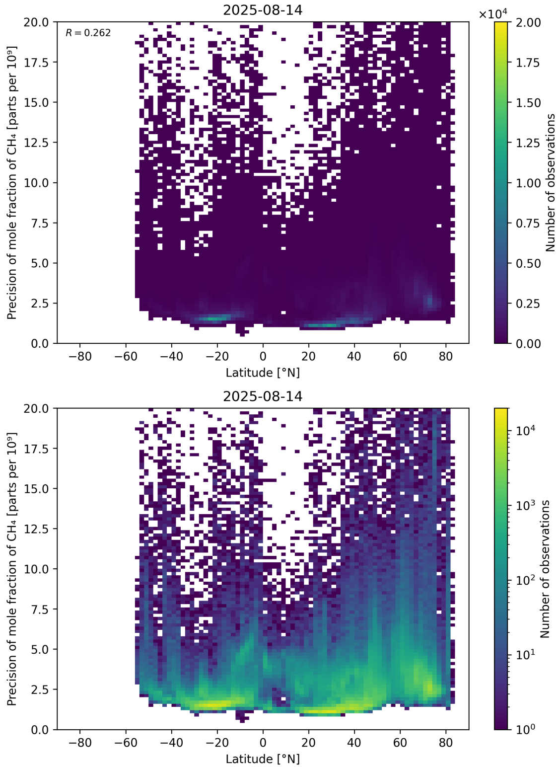
Figure 59: Scatter density plot of “Latitude” against “Precision of mole fraction of \text{CH}_4 ” for 2025-08-14 to 2025-08-15.
