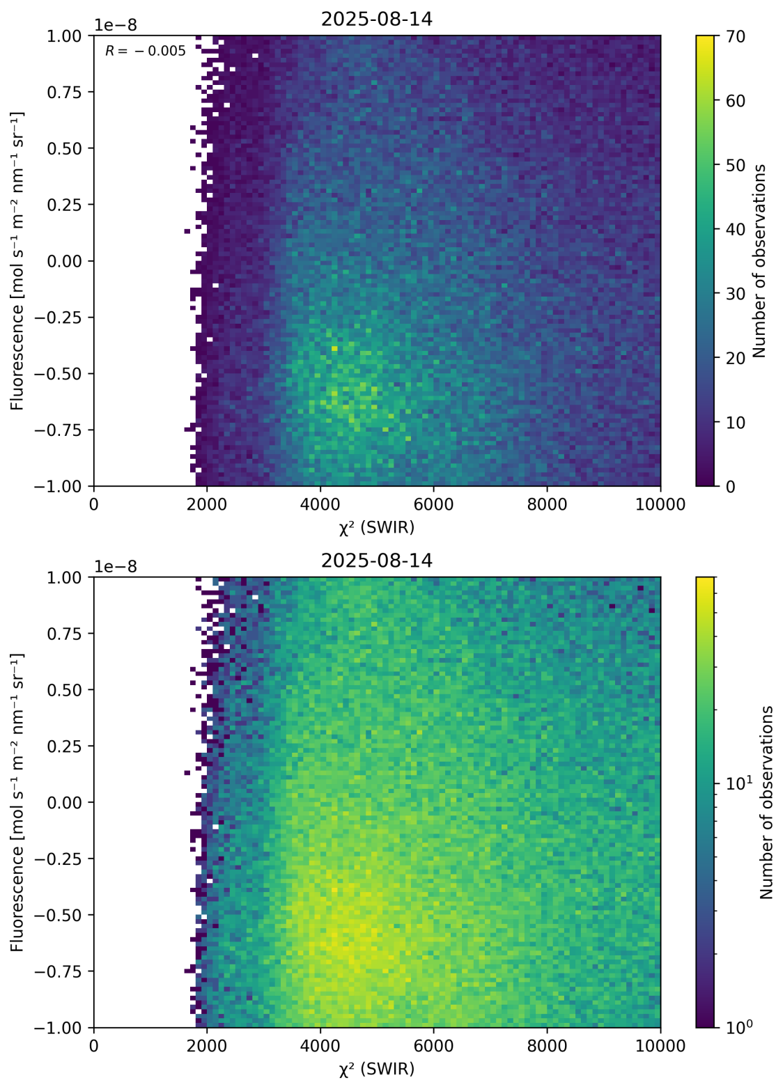
Figure 49: Scatter density plot of “ \chi^2 (SWIR)” against “Fluorescence” for 2025-08-14 to 2025-08-15.
