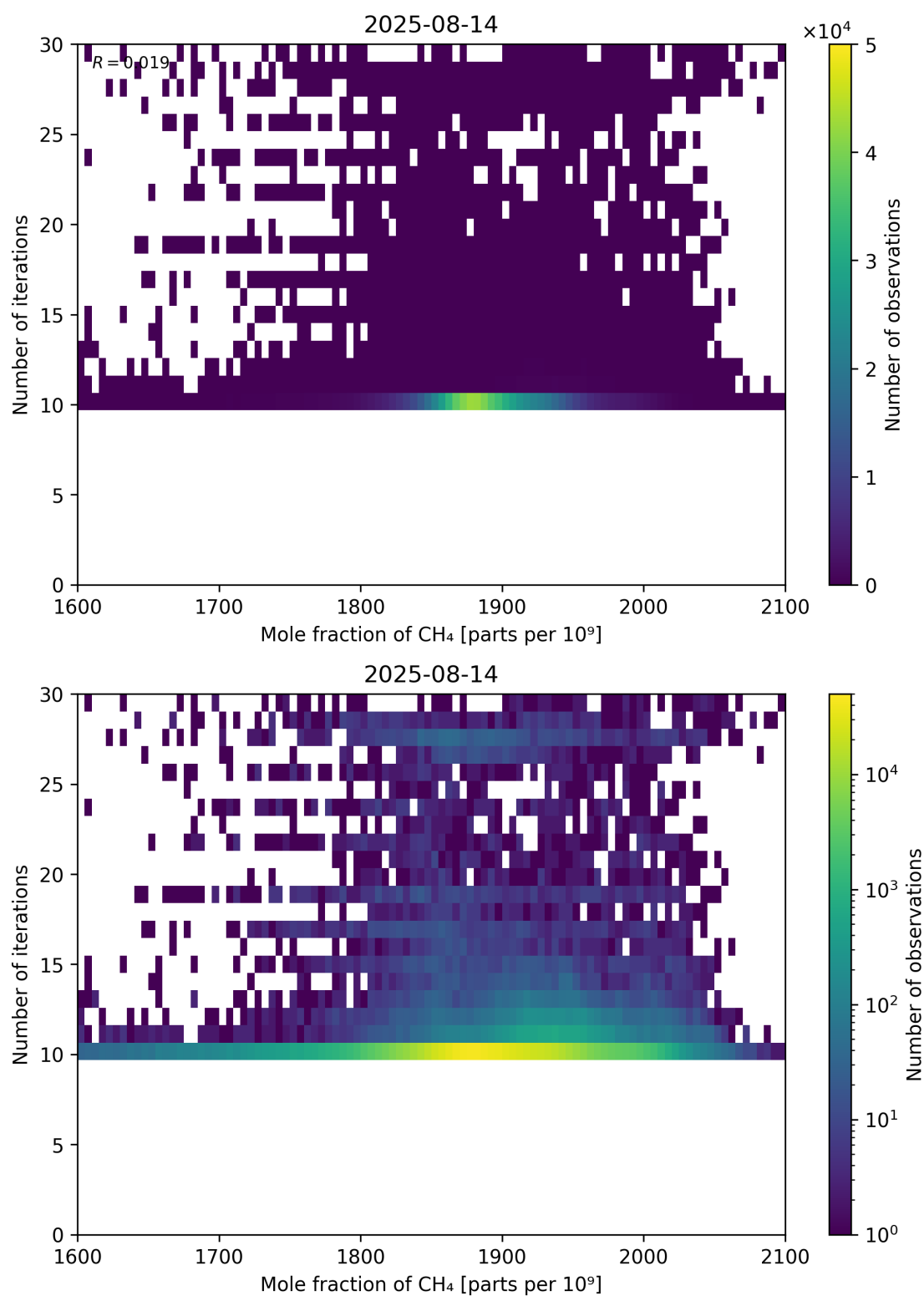
Figure 76: Scatter density plot of “Mole fraction of CH 4 ” against “Number of iterations” for 2025-08-14 to 2025-08-15.
