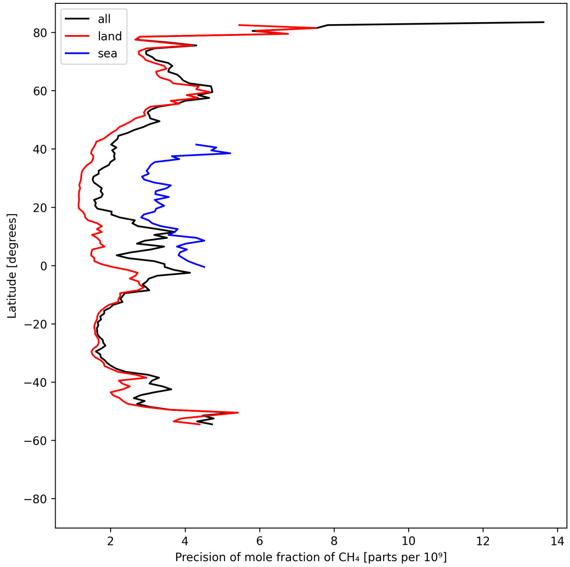
Figure 13: Zonal average of “Precision of mole fraction of CH 4 ” for 2025-08-14 to 2025-08-15.
