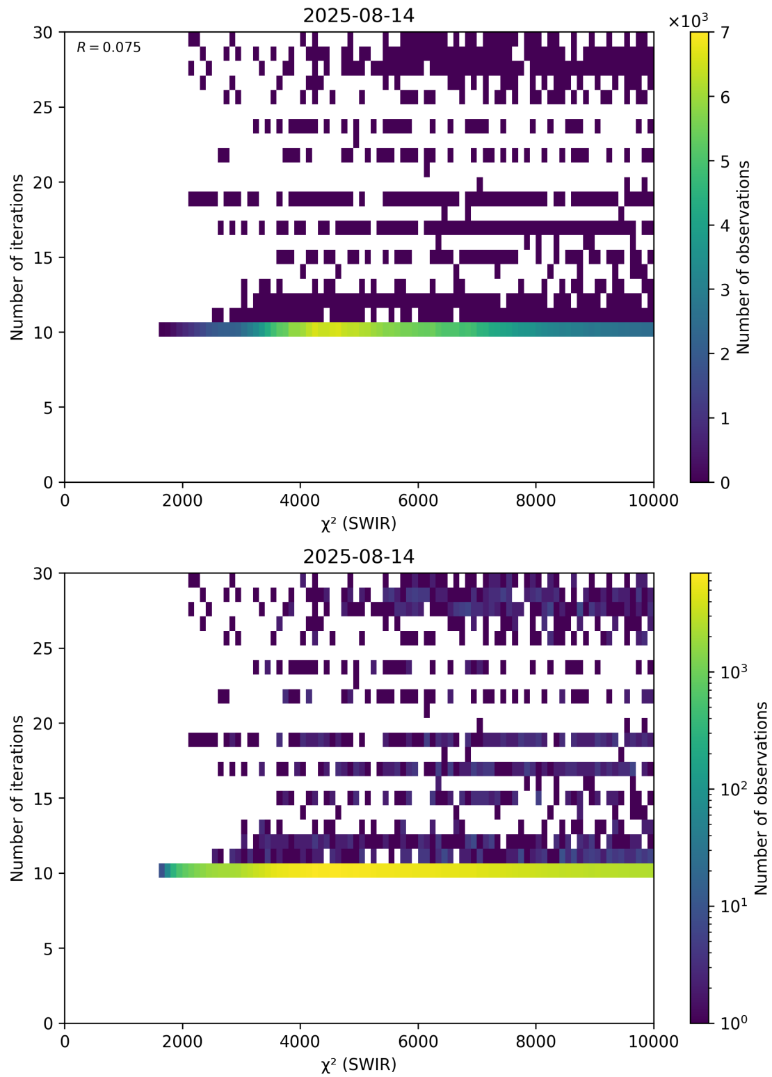
Figure 50: Scatter density plot of “ \chi^2 (SWIR)” against “Number of iterations” for 2025-08-14 to 2025-08-15.
