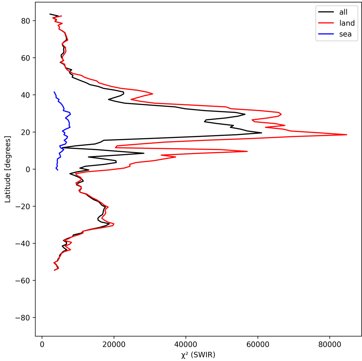
Figure 17: Zonal average of “ \chi^2 (SWIR)” for 2025-08-14 to 2025-08-15.
