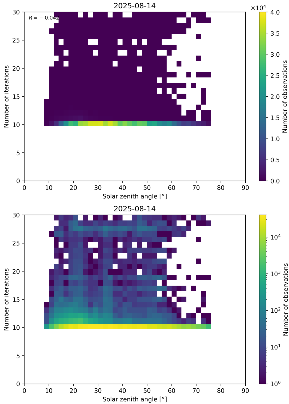
Figure 102: Scatter density plot of “Solar zenith angle” against “Number of iterations” for 2025-08-14 to 2025-08-15.
