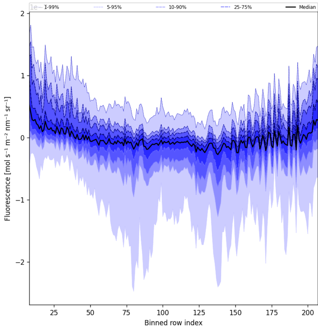
Figure 43: Along track statistics of “Fluorescence” for 2025-08-14 to 2025-08-15
