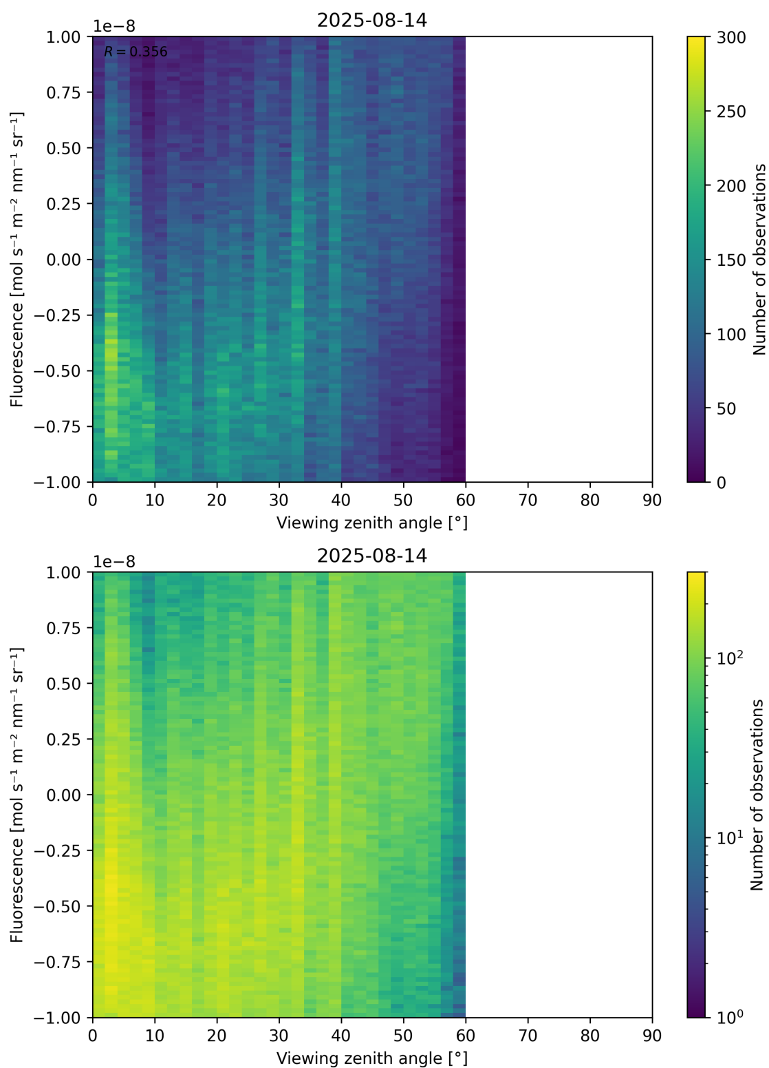
Figure 108: Scatter density plot of “Viewing zenith angle” against “Fluorescence” for 2025-08-14 to 2025-08-15.
