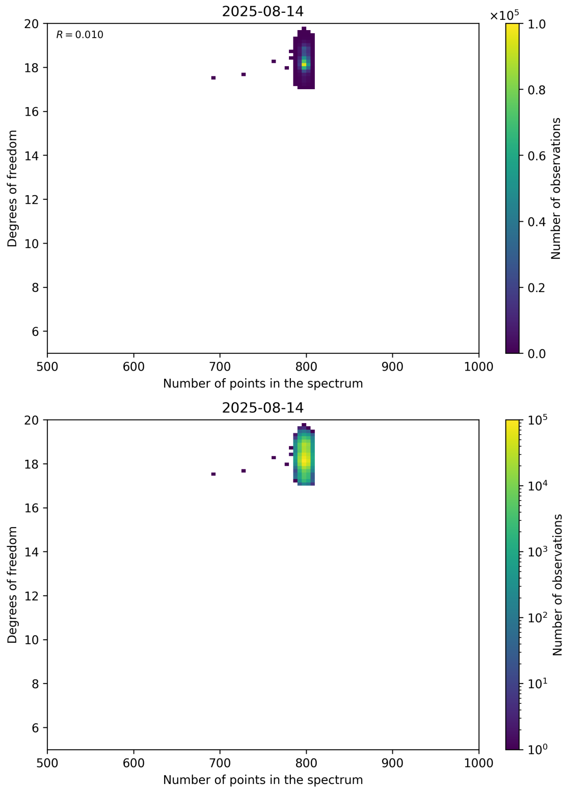
Figure 90: Scatter density plot of “Number of points in the spectrum” against “Degrees of freedom” for 2025-08-14 to 2025-08-15.
