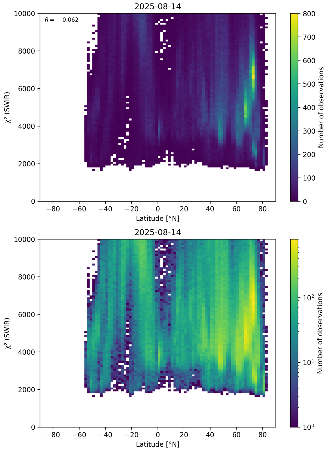
Figure 54: Scatter density plot of “Latitude” against “ \chi^2 (SWIR)” for 2025-08-14 to 2025-08-15.
