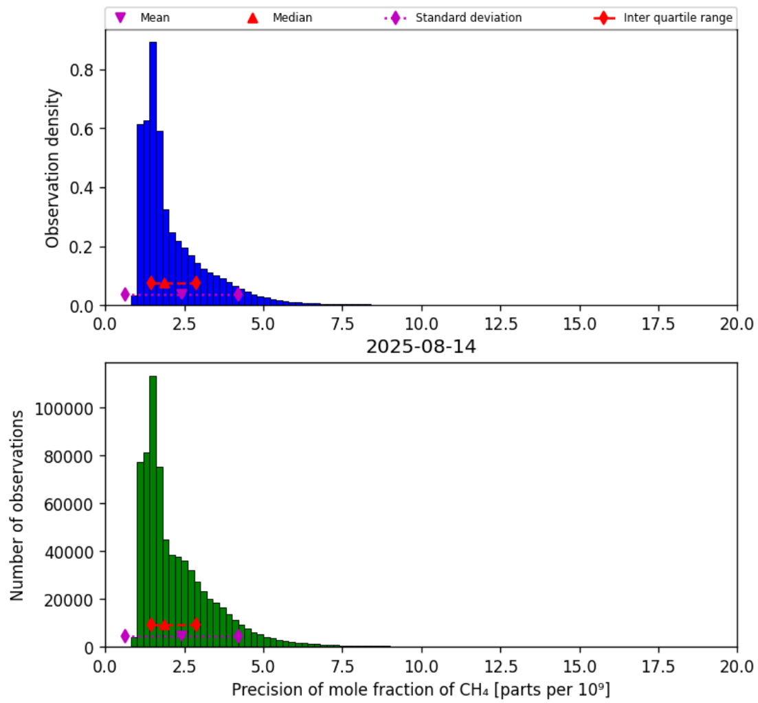
Figure 24: Histogram of “Precision of mole fraction of CH 4 ” for 2025-08-14 to 2025-08-15
