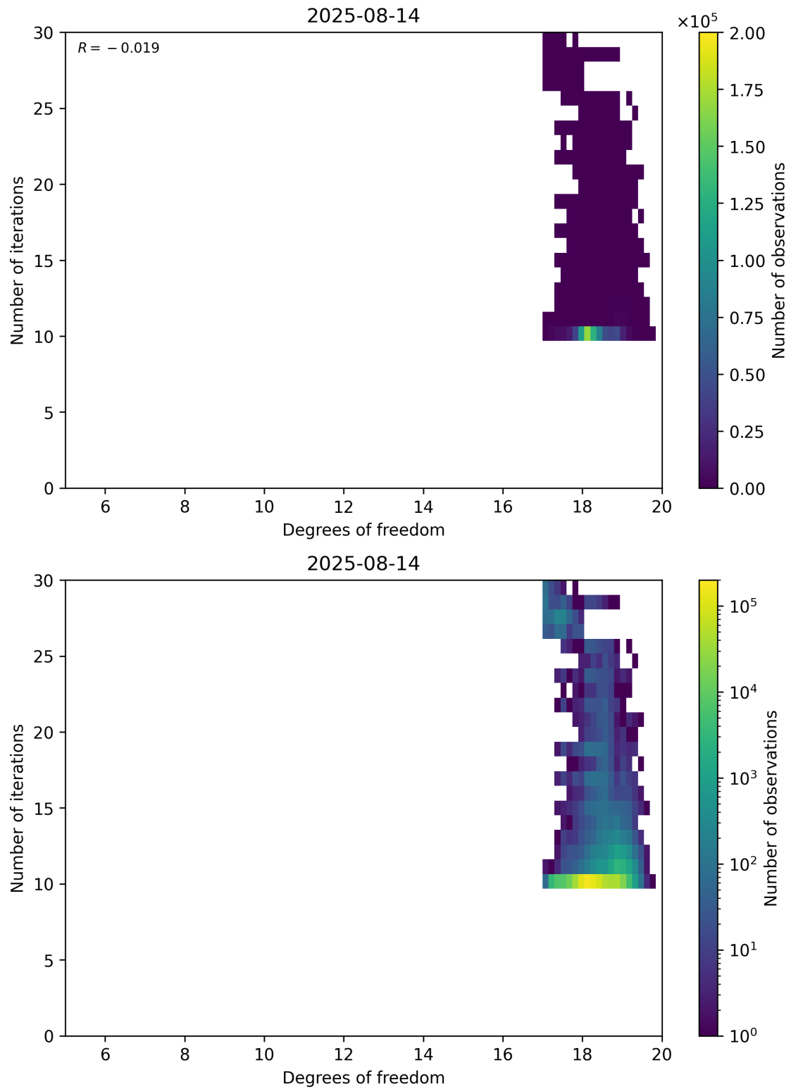
Figure 52: Scatter density plot of “Degrees of freedom” against “Number of iterations” for 2025-08-14 to 2025-08-15.
