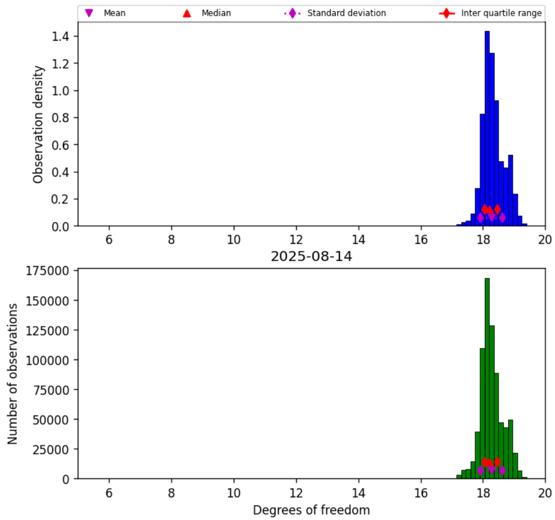
Figure 30: Histogram of “Degrees of freedom” for 2025-08-14 to 2025-08-15
