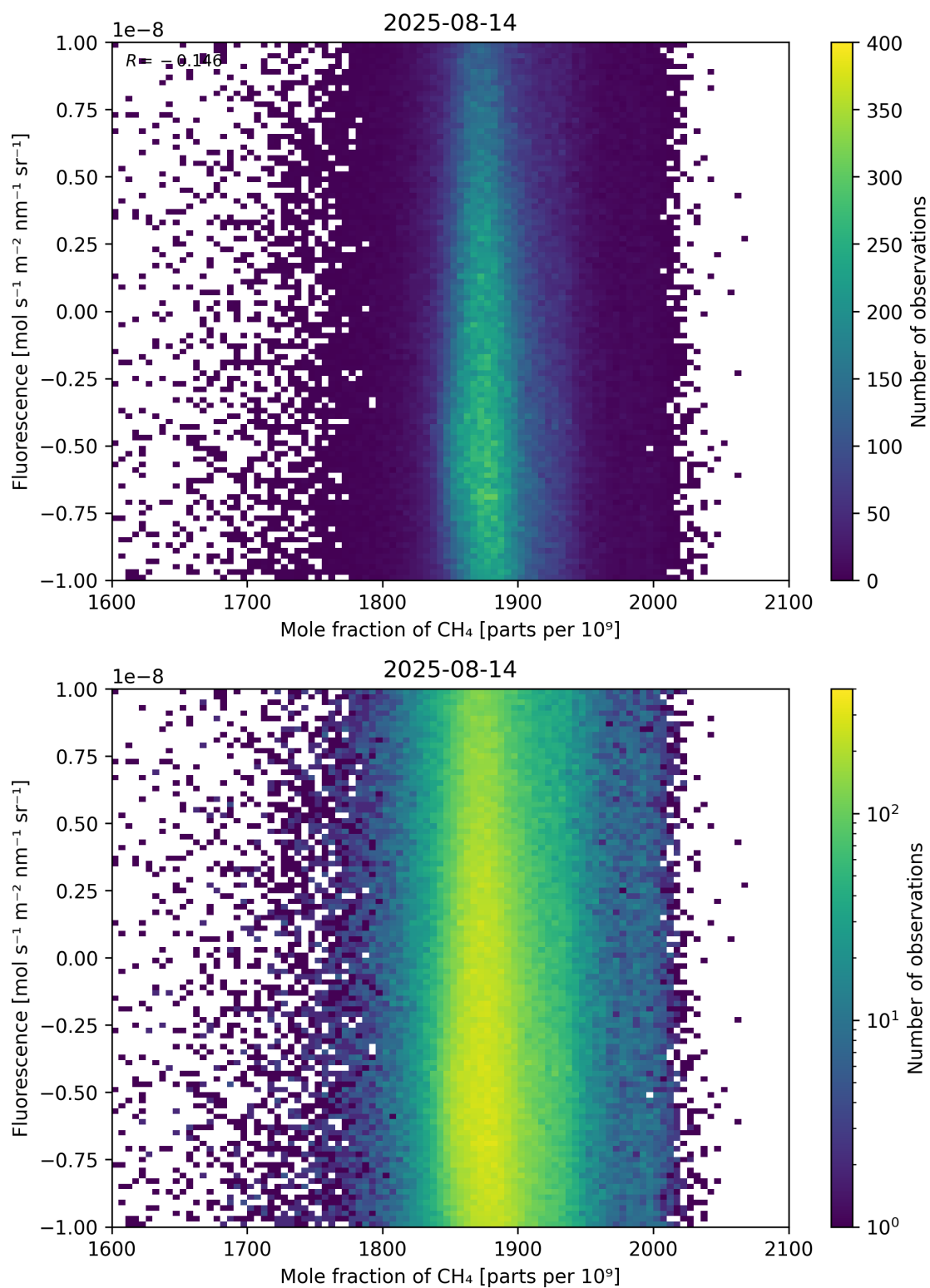
Figure 73: Scatter density plot of “Mole fraction of \text{CH}_4 ” against “Fluorescence” for 2025-08-14 to 2025-08-15.
