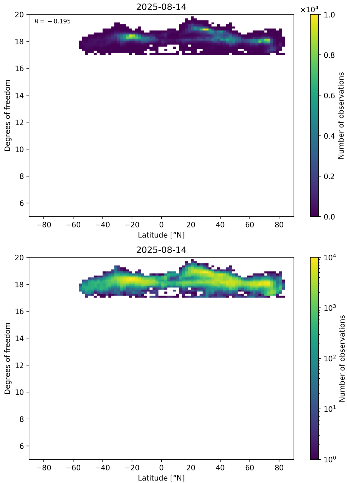
Figure 55: Scatter density plot of “Latitude” against “Degrees of freedom” for 2025-08-14 to 2025-08-15.
