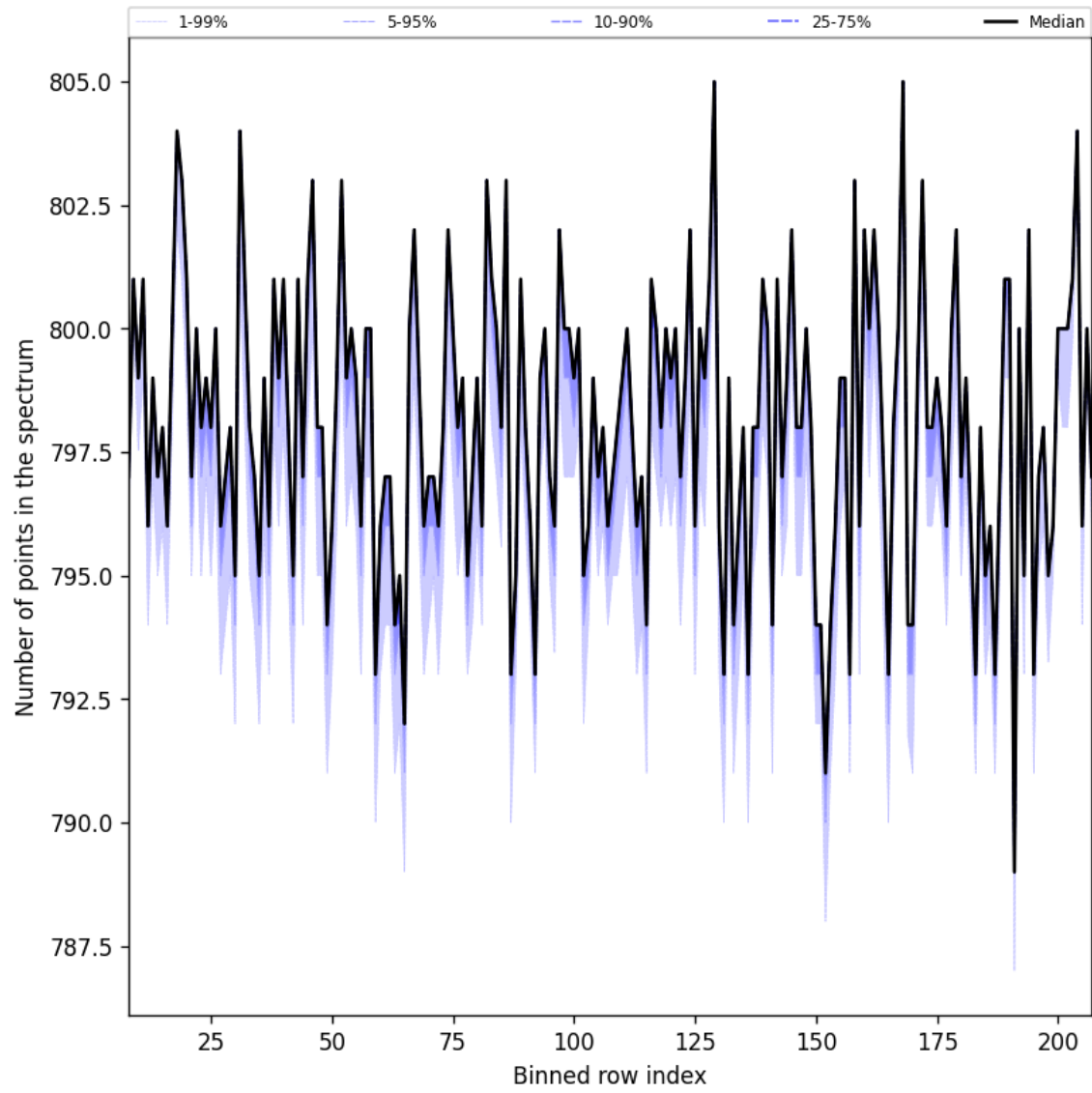
Figure 37: Along track statistics of “Number of points in the spectrum” for 2025-08-14 to 2025-08-15
