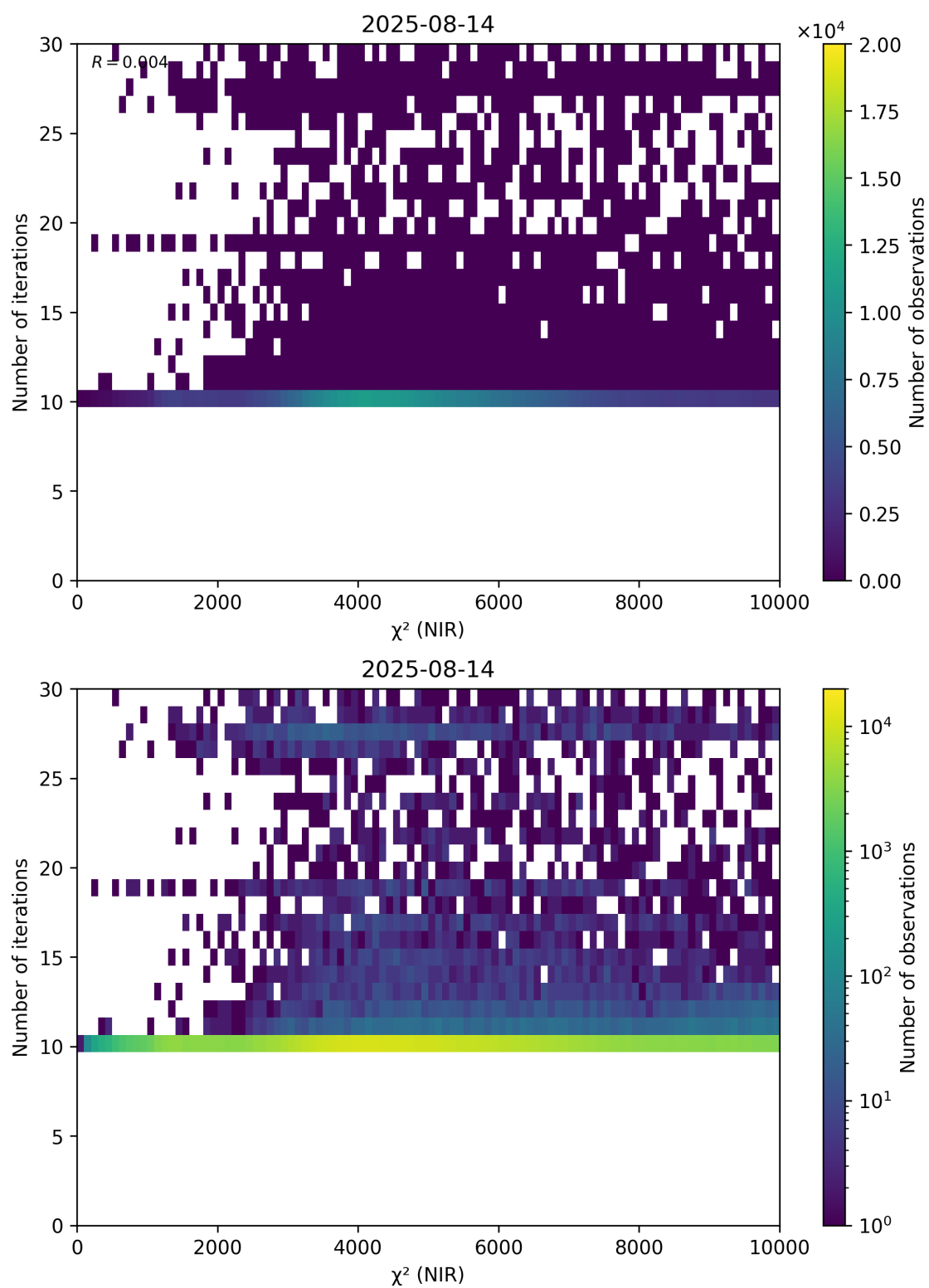
Figure 46: Scatter density plot of “ \chi^2 (NIR)” against “Number of iterations” for 2025-08-14 to 2025-08-15.
