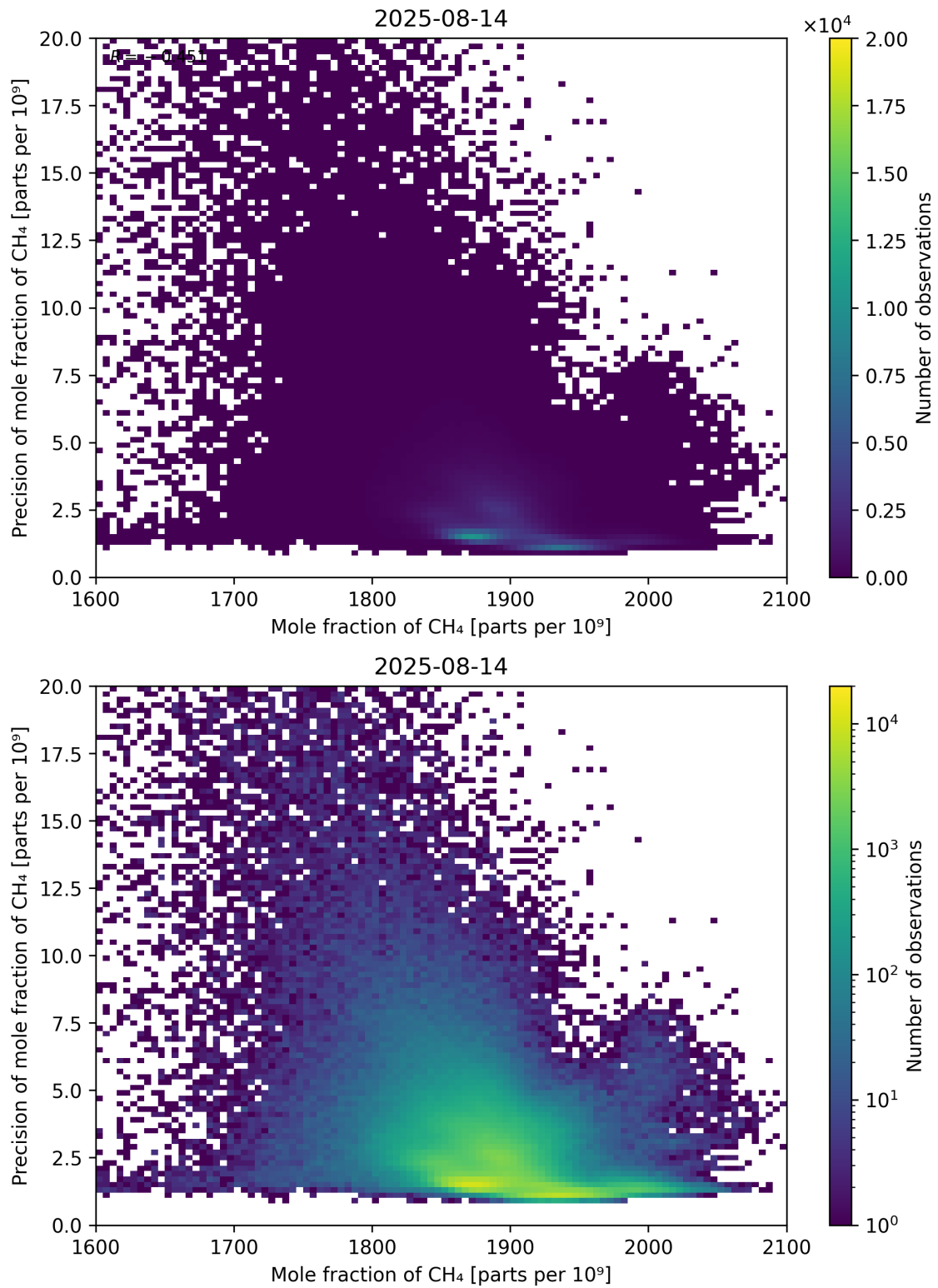
Figure 75: Scatter density plot of “Mole fraction of CH 4 ” against “Precision of mole fraction of CH 4 ” for 2025-08-14 to 2025-08-15.
