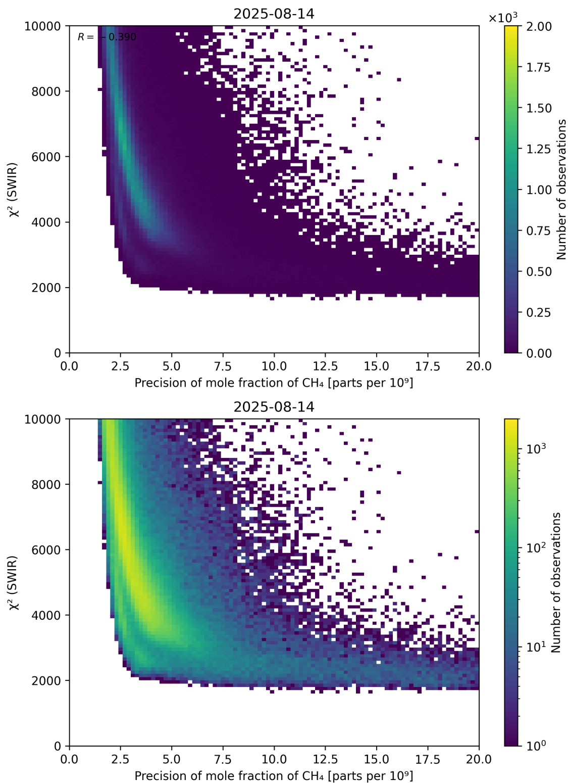
Figure 79: Scatter density plot of “Precision of mole fraction of \text{CH}_4 ” against “ \chi^2 (SWIR)” for 2025-08-14 to 2025-08-15.
