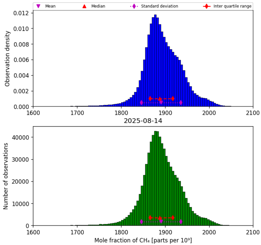
Figure 23: Histogram of “Mole fraction of CH 4 ” for 2025-08-14 to 2025-08-15
