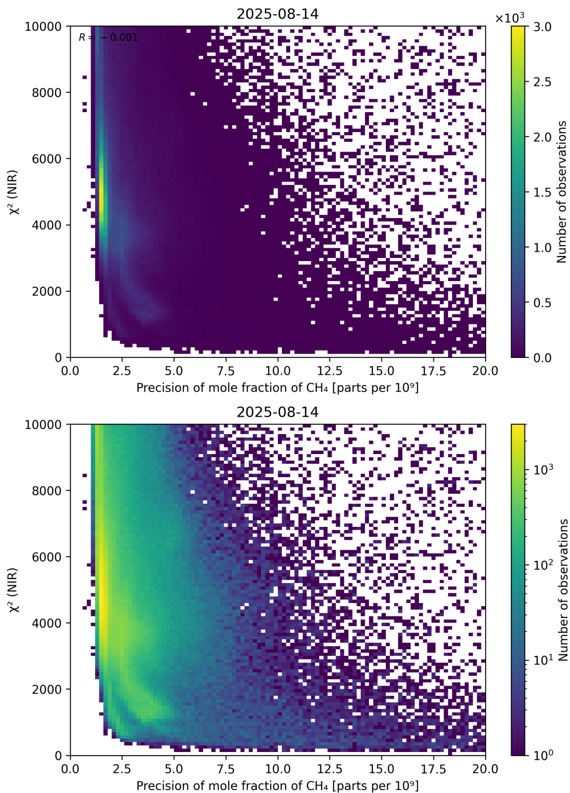
Figure 78: Scatter density plot of “Precision of mole fraction of CH 4 ” against “ \chi^2 (NIR)” for 2025-08-14 to 2025-08-15.
