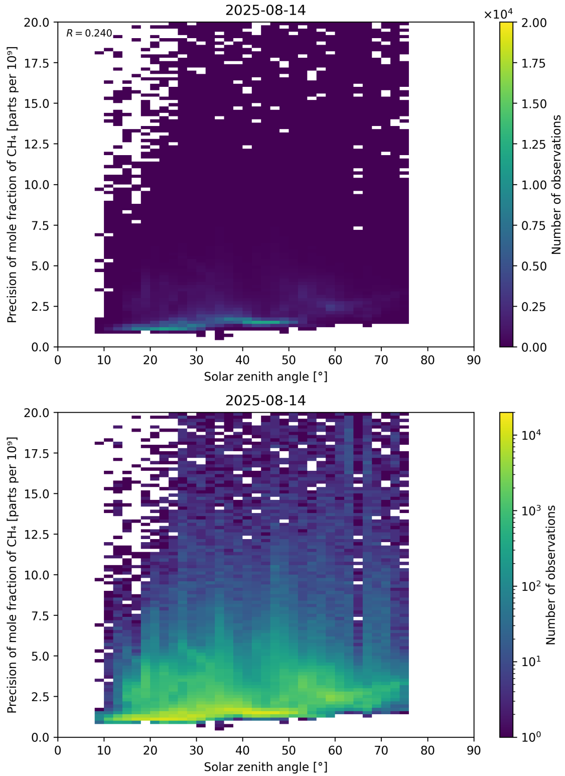
Figure 101: Scatter density plot of “Solar zenith angle” against “Precision of mole fraction of CH 4 ” for 2025-08-14 to 2025-08-15.
