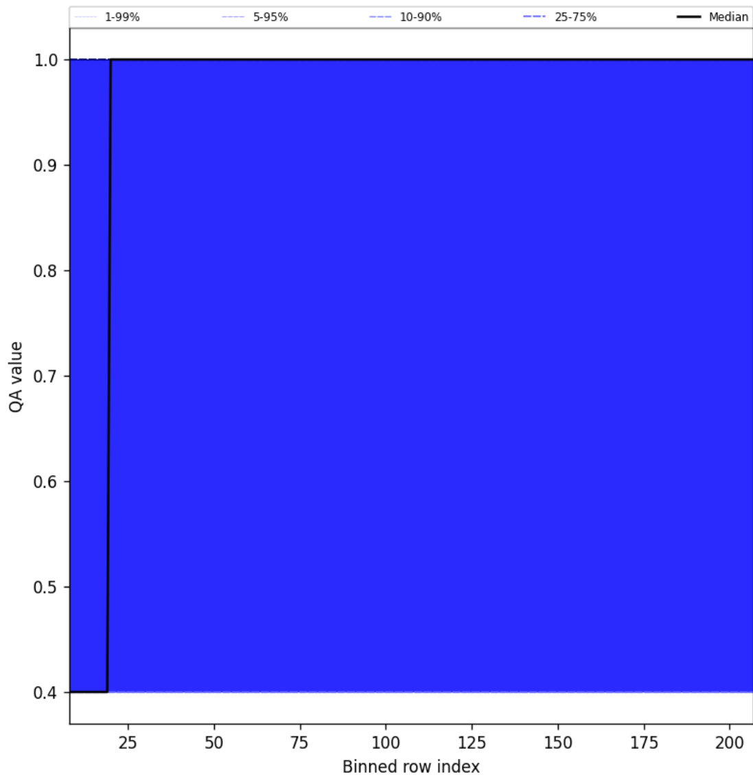
Figure 33: Along track statistics of “QA value” for 2025-08-14 to 2025-08-15
