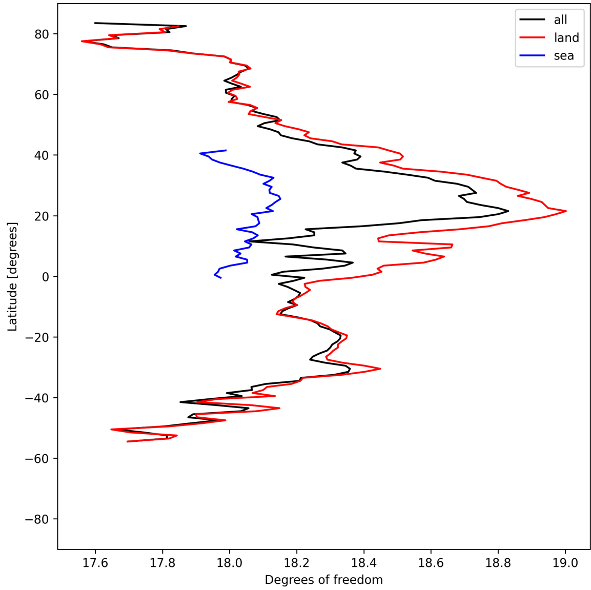
Figure 19: Zonal average of “Degrees of freedom” for 2025-08-14 to 2025-08-15.
