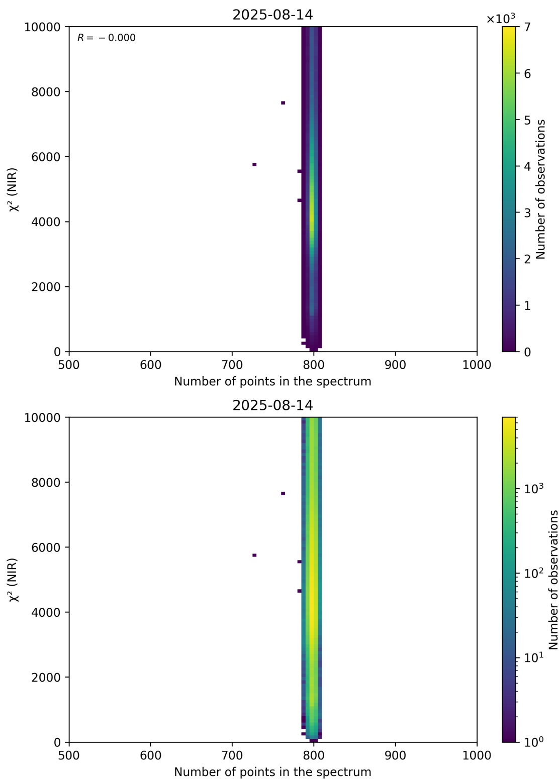
Figure 88: Scatter density plot of “Number of points in the spectrum” against “ \chi^2 (NIR)” for 2025-08-14 to 2025-08-15.
