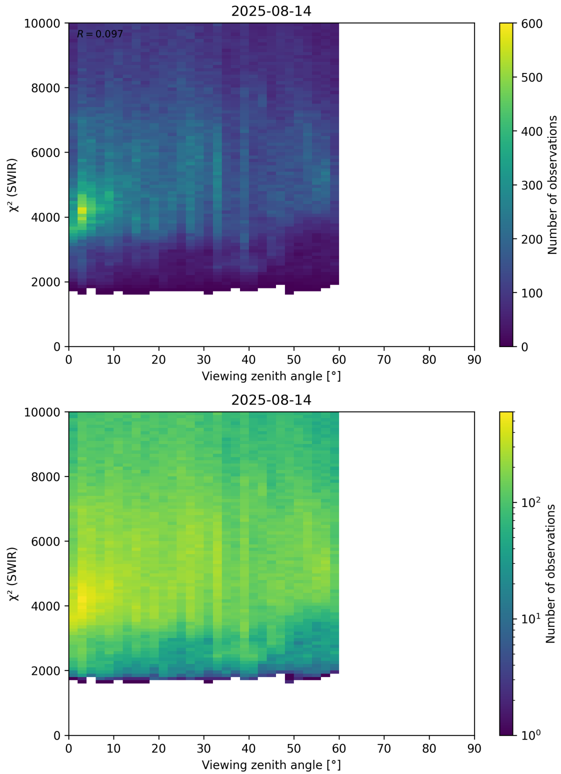
Figure 106: Scatter density plot of “Viewing zenith angle” against “ \chi^2 (SWIR)” for 2025-08-14 to 2025-08-15.
