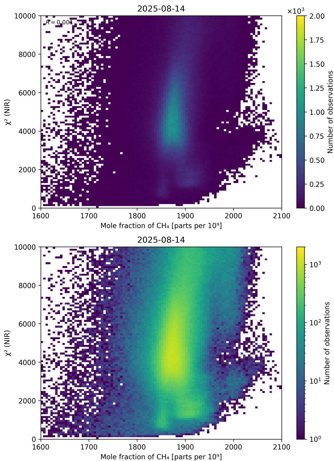
Figure 70: Scatter density plot of “Mole fraction of CH 4 ” against “ \chi^2 (NIR)” for 2025-08-14 to 2025-08-15.
