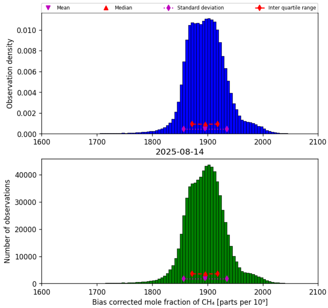
Figure 25: Histogram of “Bias corrected mole fraction of CH 4 ” for 2025-08-14 to 2025-08-15
