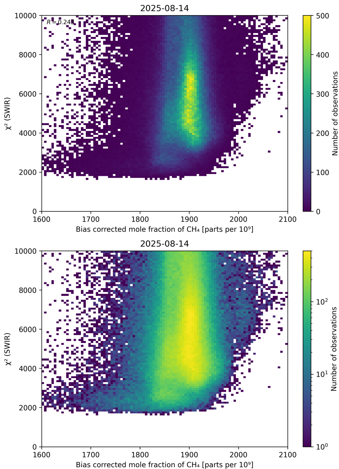
Figure 64: Scatter density plot of “Bias corrected mole fraction of \text{CH}_4 ” against “ \chi^2 (SWIR)” for 2025-08-14 to 2025-08-15.
