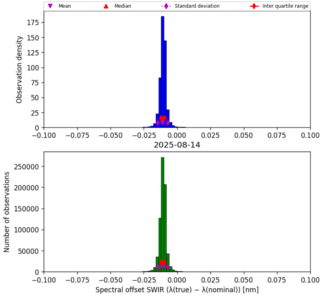
Figure 27: Histogram of “Spectral offset SWIR ( \lambda_{\text{true}} - \lambda_{\text{nominal}} )” for 2025-08-14 to 2025-08-15
