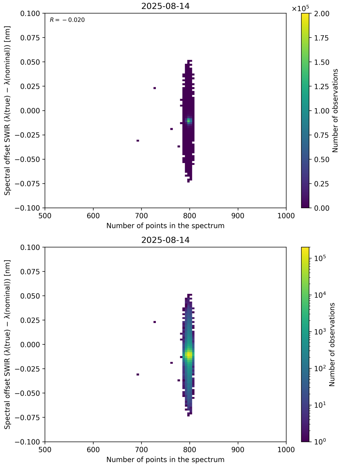
Figure 93: Scatter density plot of “Number of points in the spectrum” against “Spectral offset SWIR ( \lambda_{\text{true}} - \lambda_{\text{nominal}} )” for 2025-08-14 to 2025-08-15.
