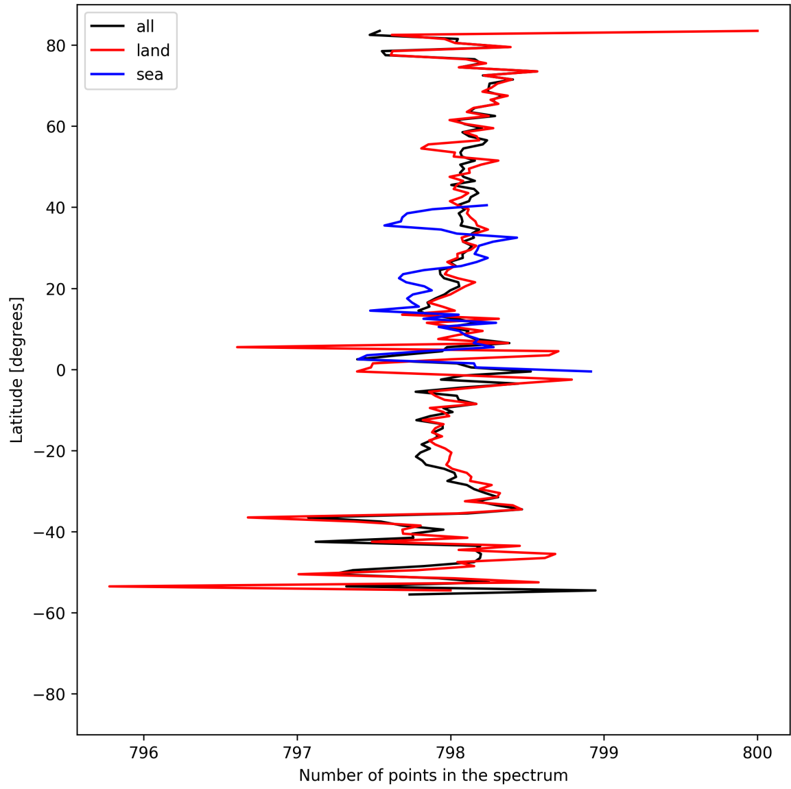
Figure 15: Zonal average of “Number of points in the spectrum” for 2025-08-14 to 2025-08-16.
