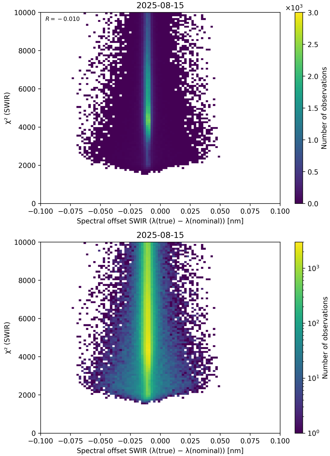
Figure 118: Scatter density plot of “Spectral offset SWIR ( \lambda_{\text{true}} - \lambda_{\text{nominal}} )” against “ \chi^2 (SWIR)” for 2025-08-14 to 2025-08-16.
