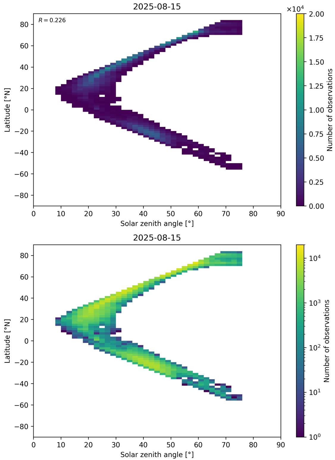
Figure 98: Scatter density plot of “Solar zenith angle” against “Latitude” for 2025-08-14 to 2025-08-16.
