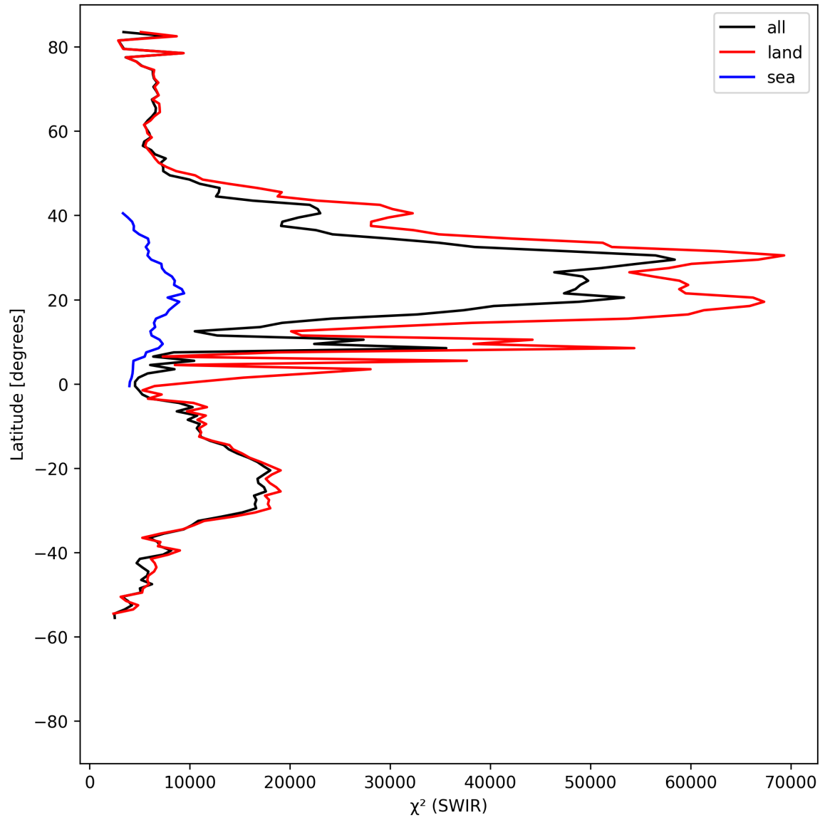
Figure 17: Zonal average of “ \chi^2 (SWIR)” for 2025-08-14 to 2025-08-16.
