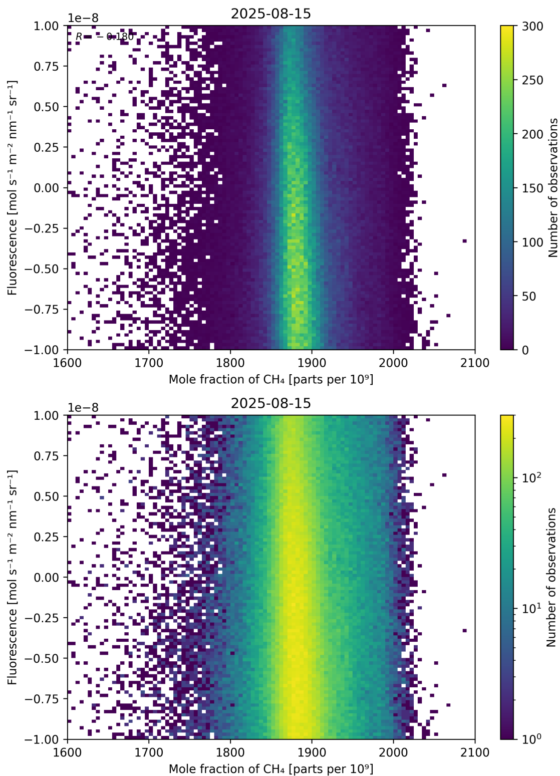
Figure 73: Scatter density plot of “Mole fraction of \text{CH}_4 ” against “Fluorescence” for 2025-08-14 to 2025-08-16.
