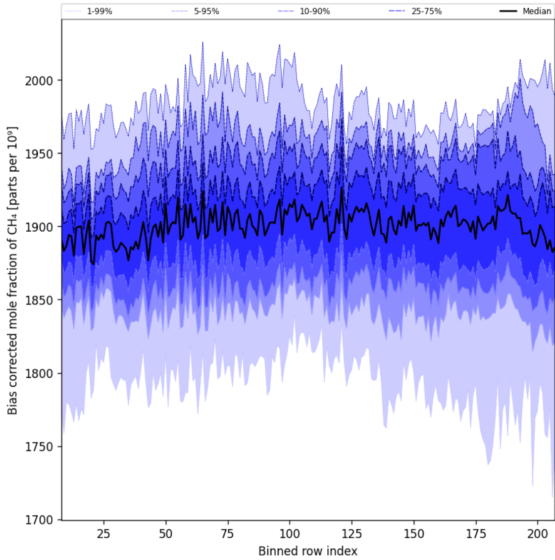
Figure 36: Along track statistics of “Bias corrected mole fraction of CH 4 ” for 2025-08-14 to 2025-08-16
