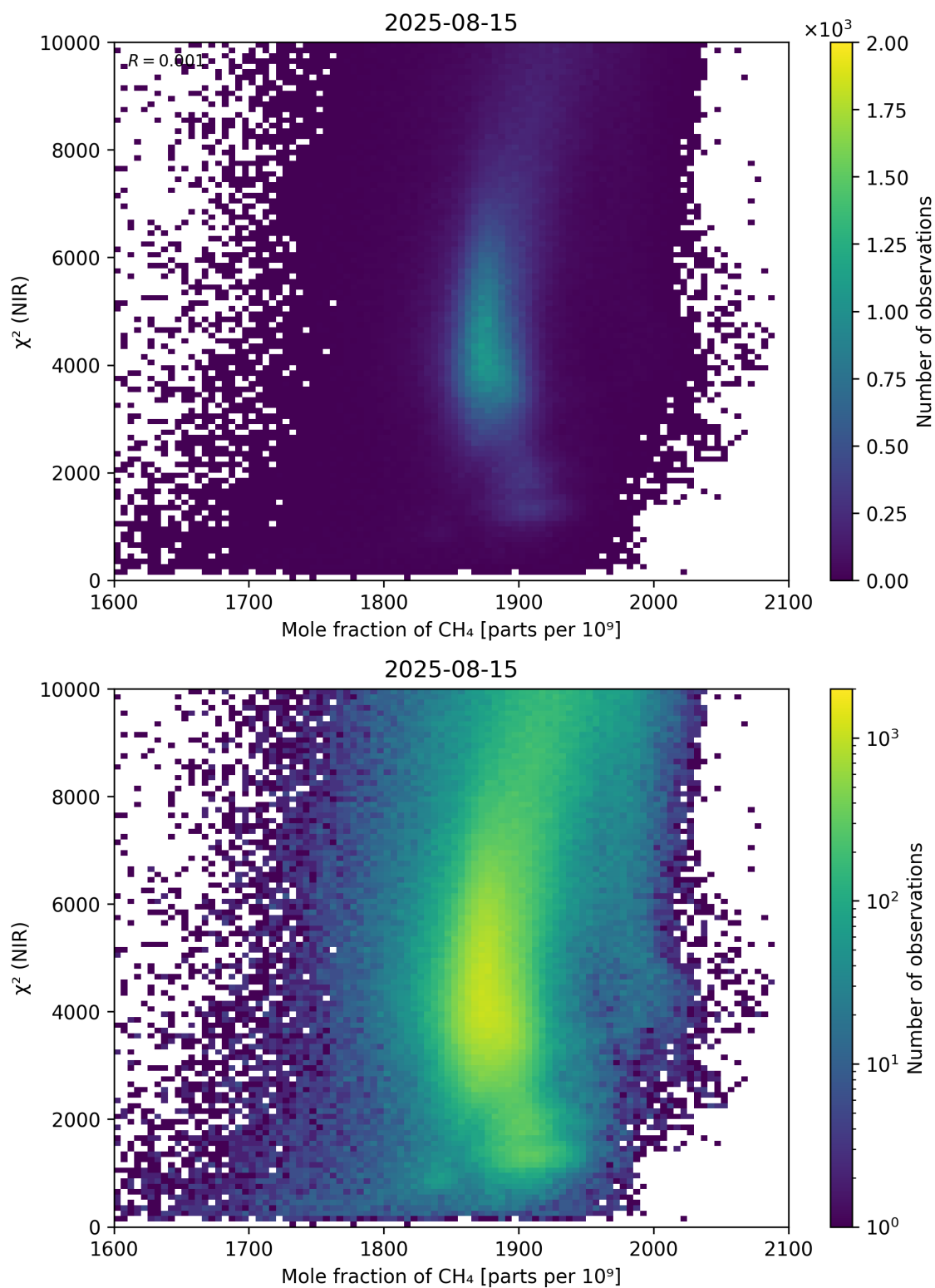
Figure 70: Scatter density plot of “Mole fraction of \text{CH}_4 ” against “ \chi^2 (NIR)” for 2025-08-14 to 2025-08-16.
