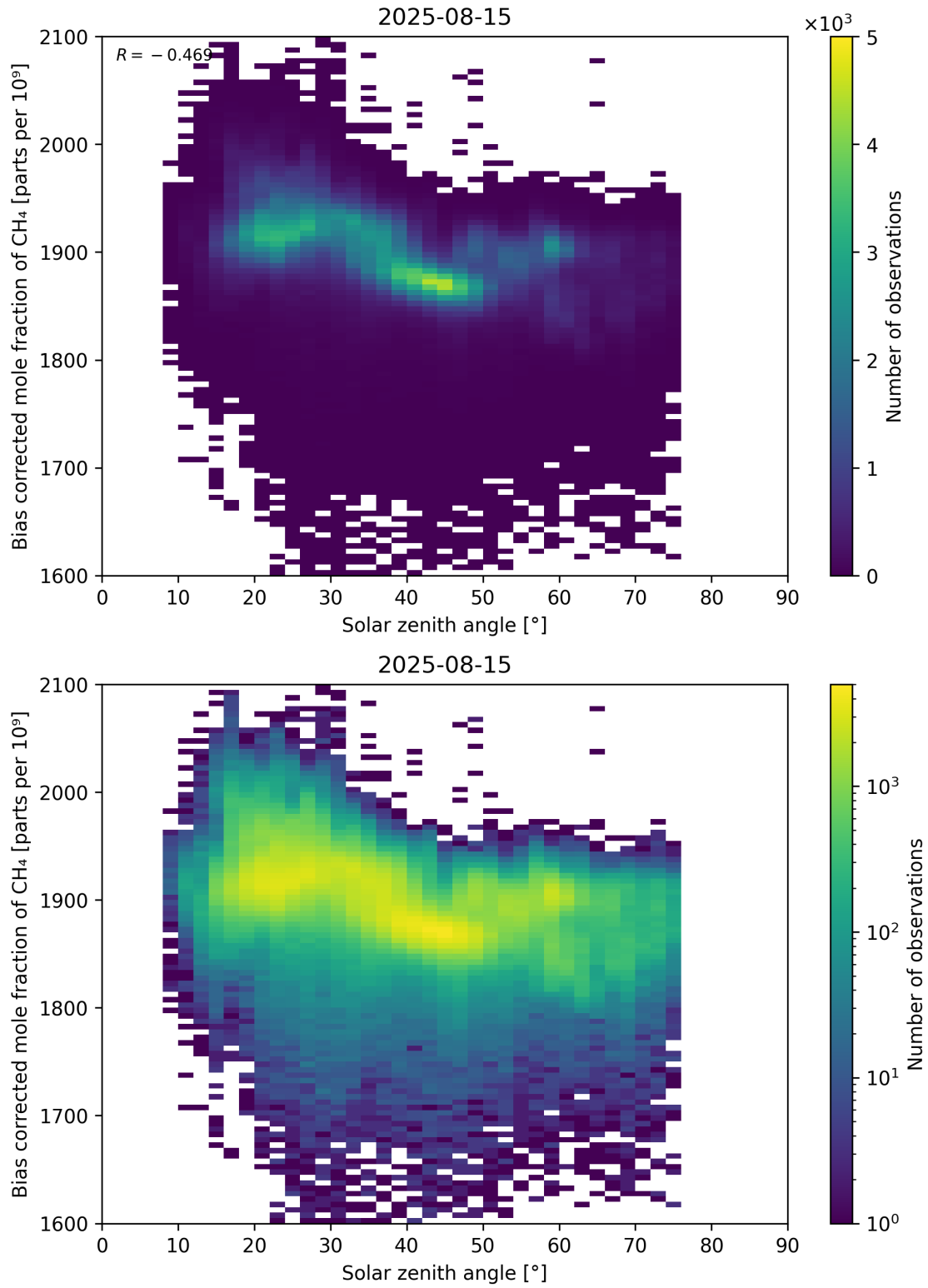
Figure 100: Scatter density plot of “Solar zenith angle” against “Bias corrected mole fraction of \text{CH}_4 ” for 2025-08-14 to 2025-08-16.
