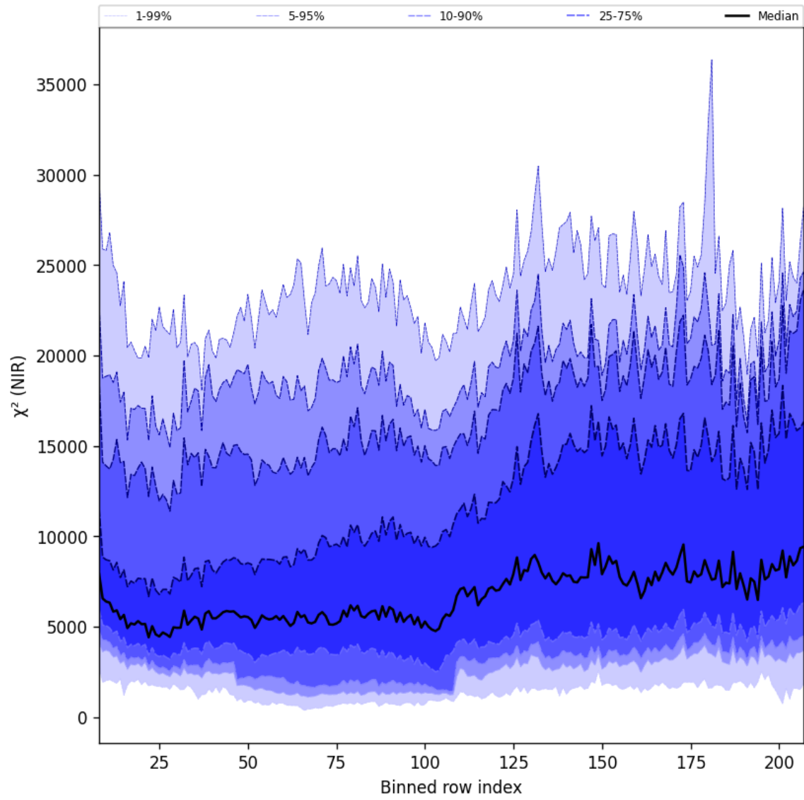
Figure 40: Along track statistics of “ \chi^2 (NIR)” for 2025-08-14 to 2025-08-16
