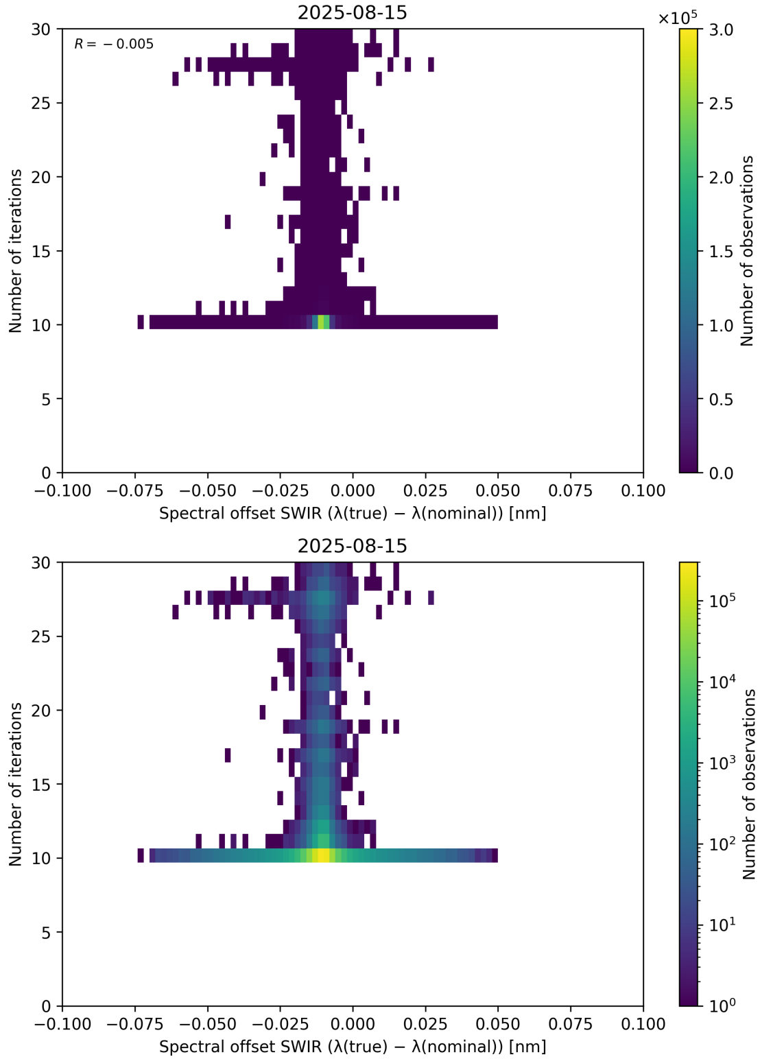
Figure 121: Scatter density plot of “Spectral offset SWIR ( \lambda_{\text{true}} - \lambda_{\text{nominal}} )” against “Number of iterations” for 2025-08-14 to 2025-08-16.
