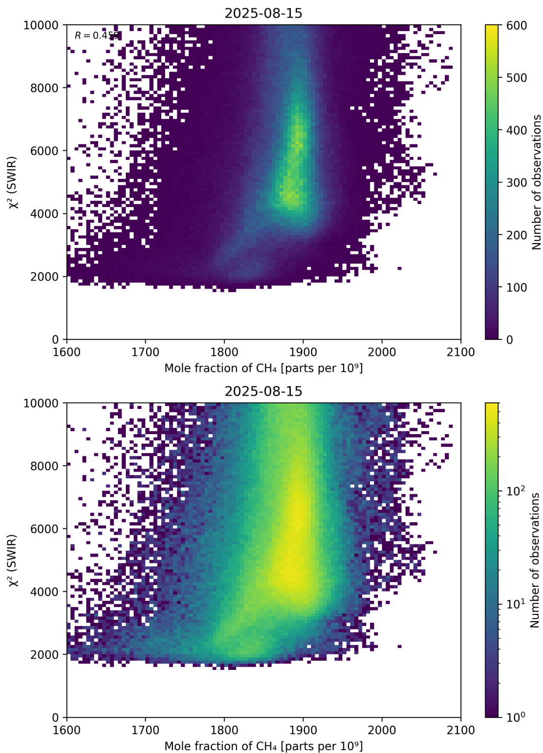
Figure 71: Scatter density plot of “Mole fraction of \text{CH}_4 ” against “ \chi^2 (SWIR)” for 2025-08-14 to 2025-08-16.
