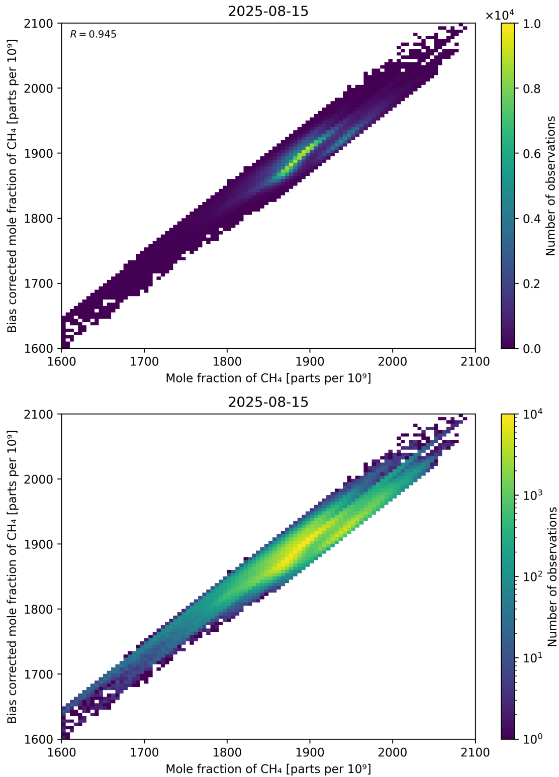
Figure 74: Scatter density plot of “Mole fraction of CH 4 ” against “Bias corrected mole fraction of CH 4 ” for 2025-08-14 to 2025-08-16.
