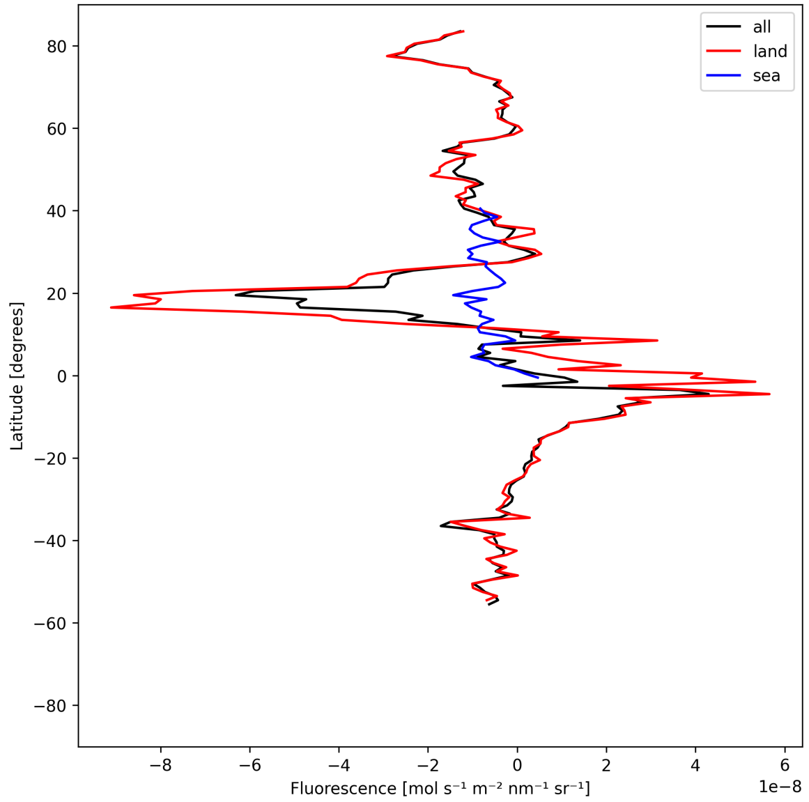
Figure 21: Zonal average of “Fluorescence” for 2025-08-14 to 2025-08-16.
