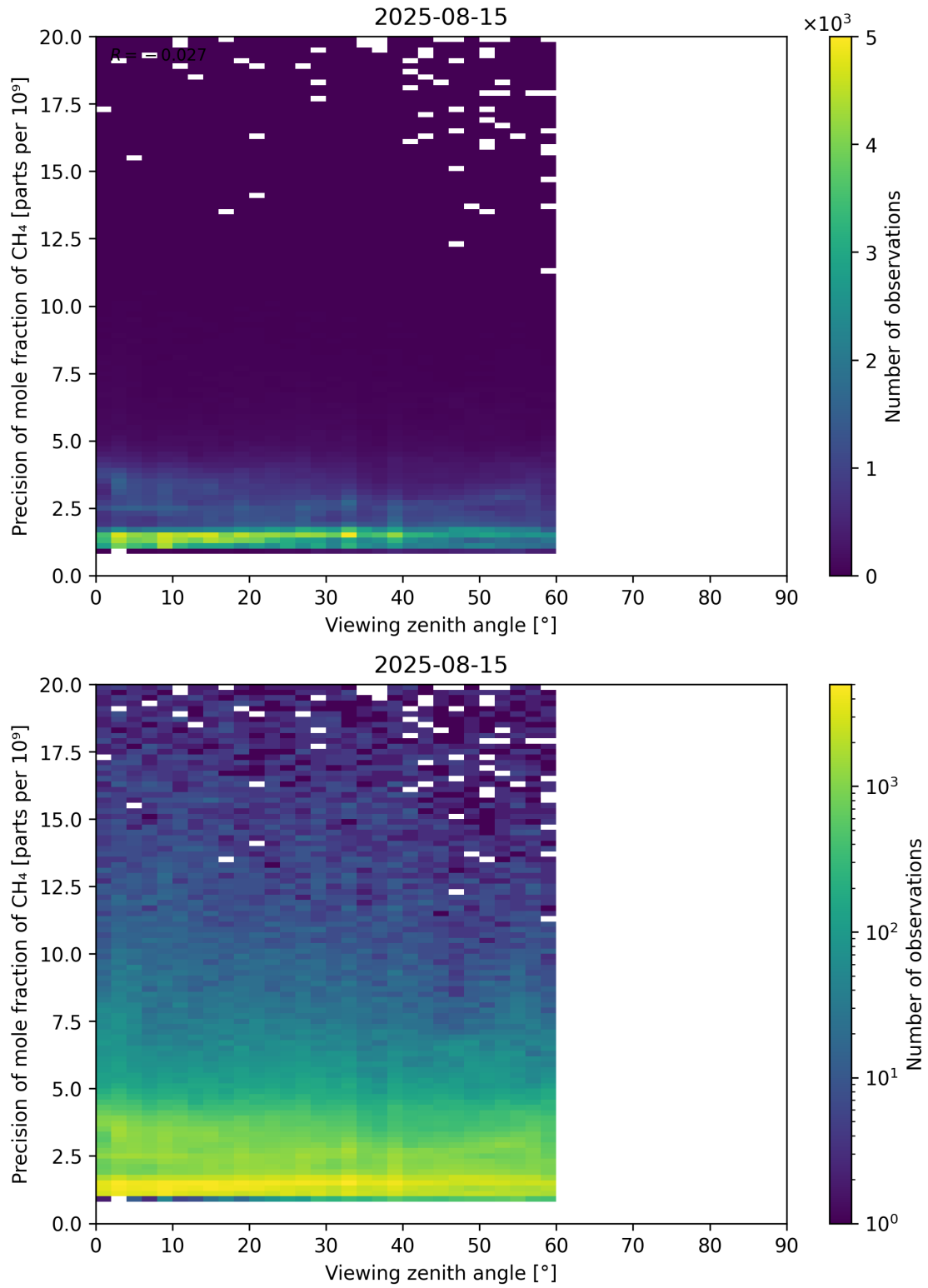
Figure 112: Scatter density plot of “Viewing zenith angle” against “Precision of mole fraction of CH 4 ” for 2025-08-14 to 2025-08-16.
