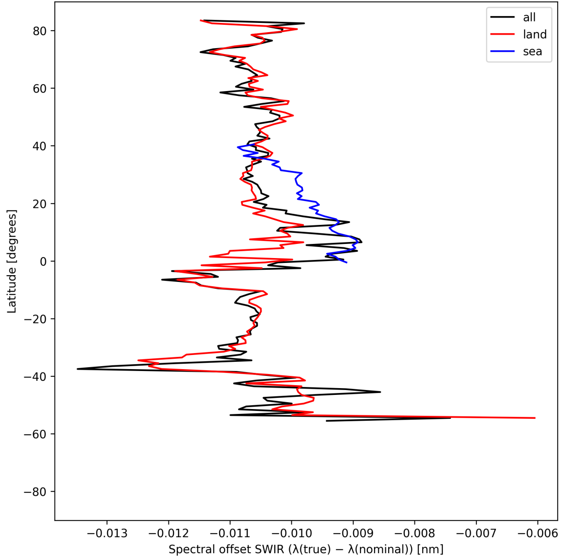
Figure 16: Zonal average of “Spectral offset SWIR ( \lambda_{\text{true}} - \lambda_{\text{nominal}} )” for 2025-08-14 to 2025-08-16.
