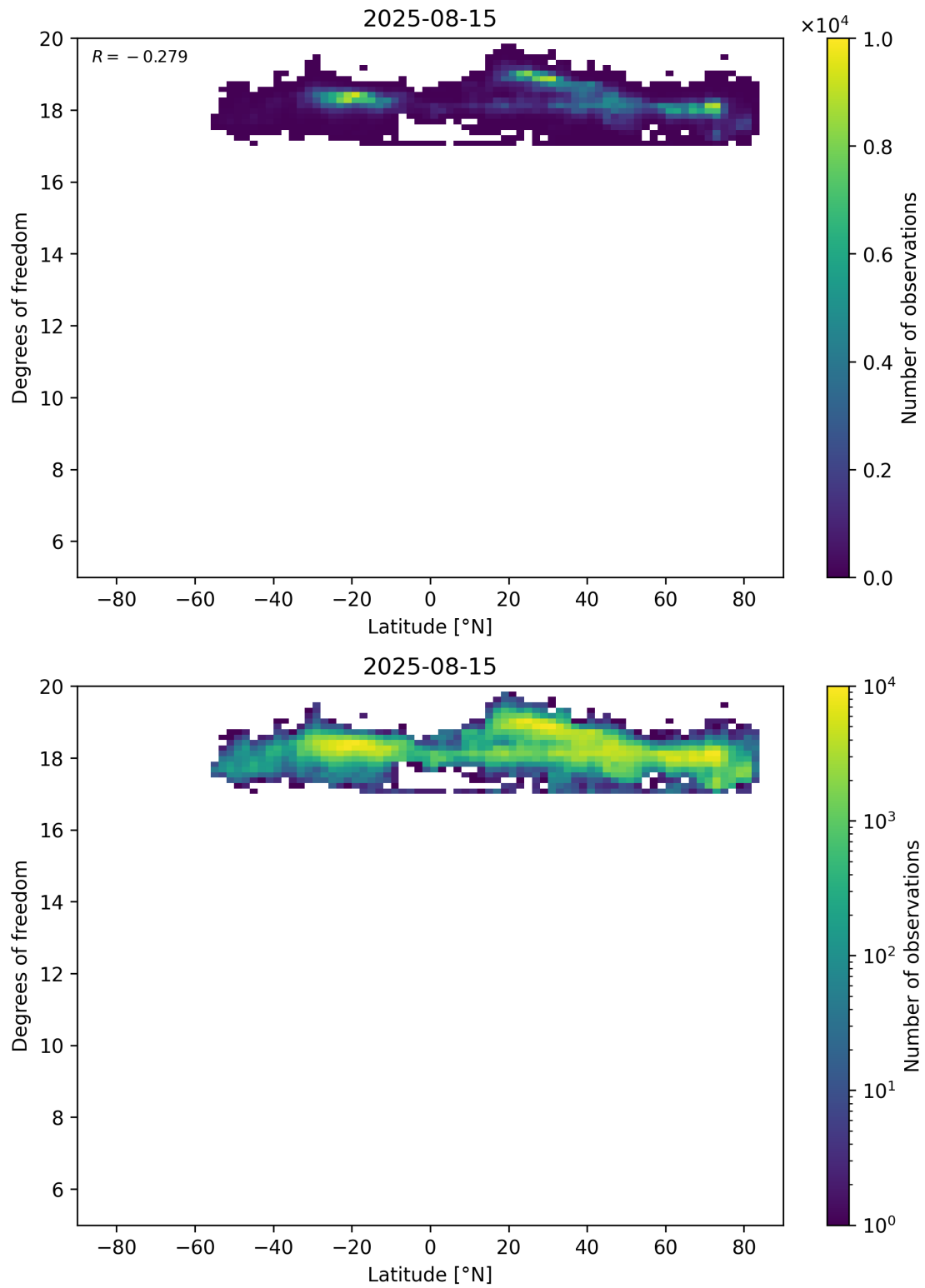
Figure 55: Scatter density plot of “Latitude” against “Degrees of freedom” for 2025-08-14 to 2025-08-16.
