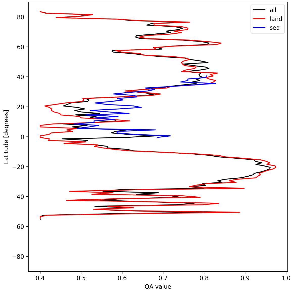
Figure 11: Zonal average of “QA value” for 2025-08-14 to 2025-08-16.
