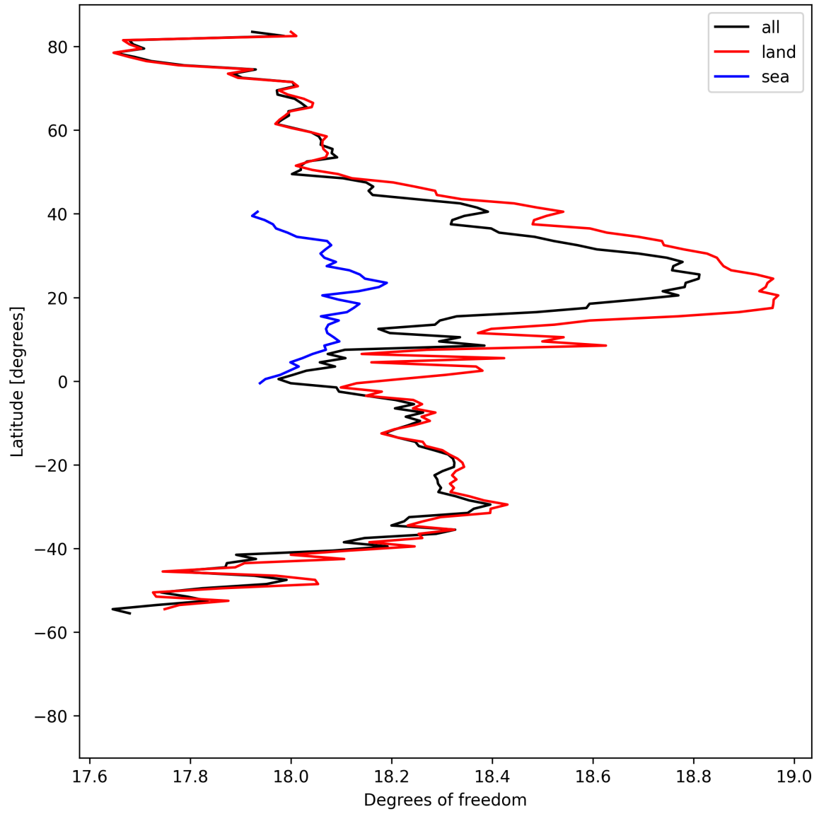
Figure 19: Zonal average of “Degrees of freedom” for 2025-08-14 to 2025-08-16.
