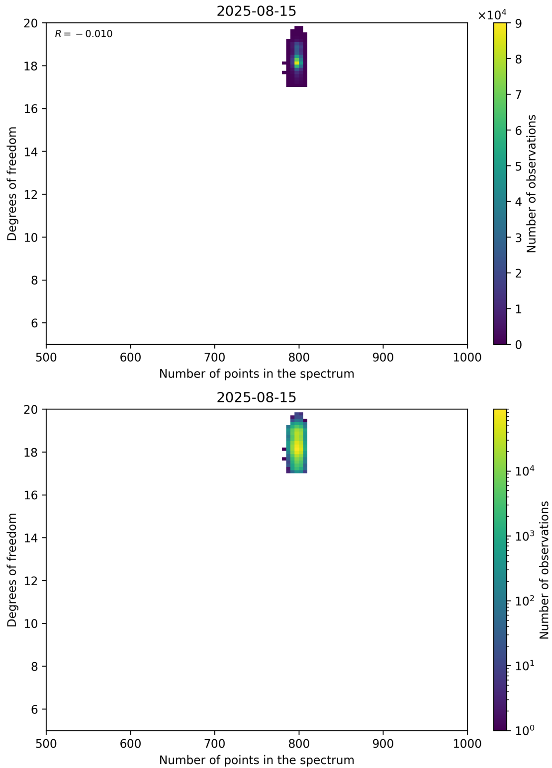
Figure 90: Scatter density plot of “Number of points in the spectrum” against “Degrees of freedom” for 2025-08-14 to 2025-08-16.
