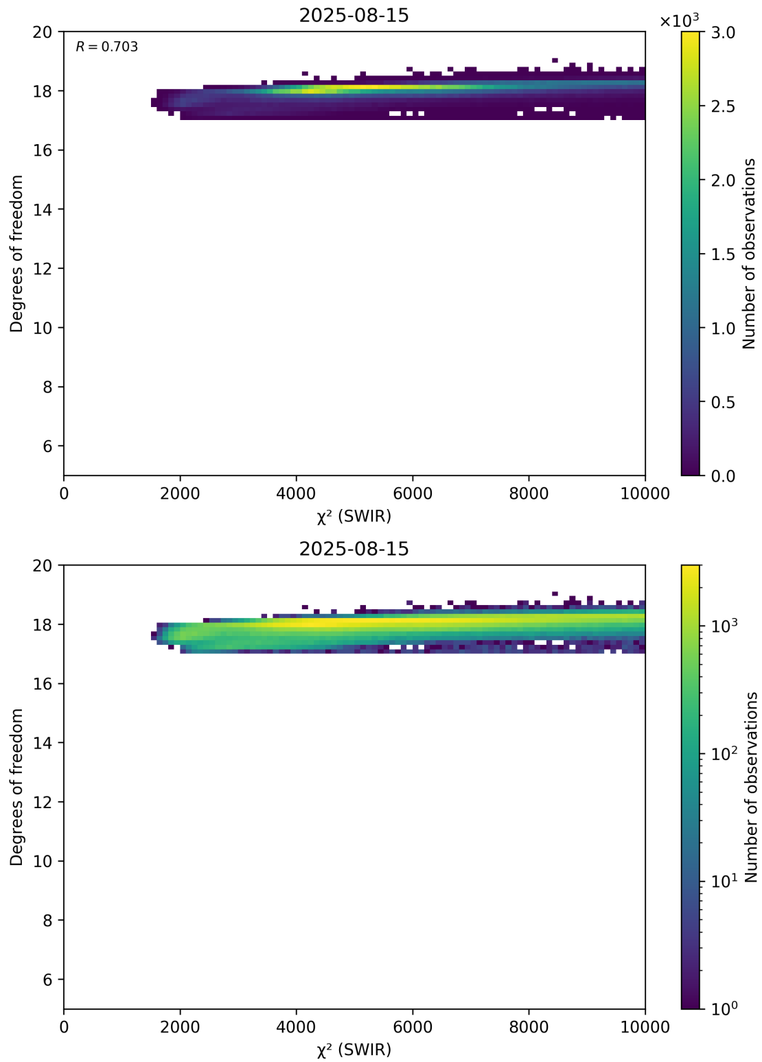
Figure 48: Scatter density plot of “ \chi^2 (SWIR)” against “Degrees of freedom” for 2025-08-14 to 2025-08-16.
