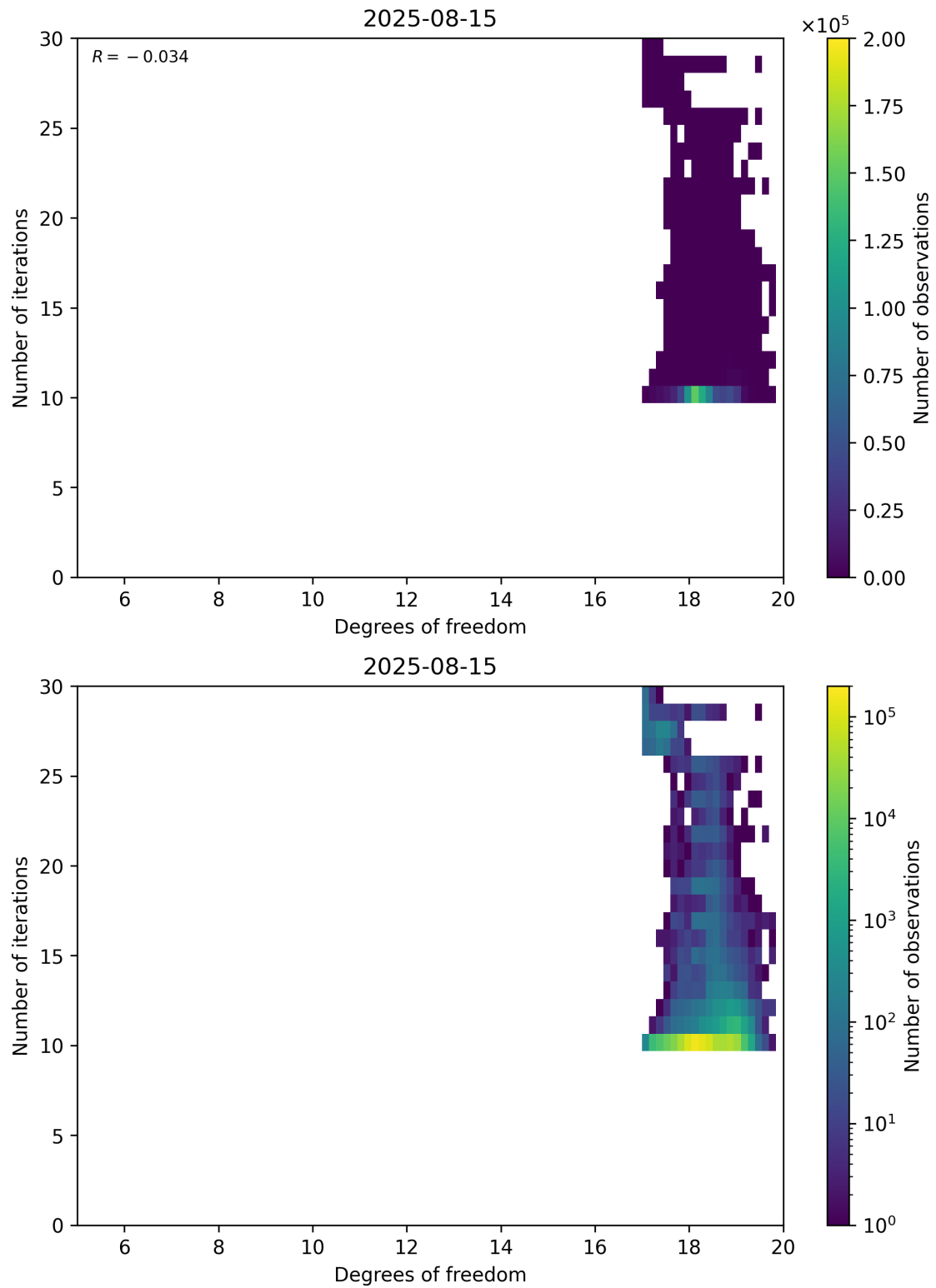
Figure 52: Scatter density plot of “Degrees of freedom” against “Number of iterations” for 2025-08-14 to 2025-08-16.
