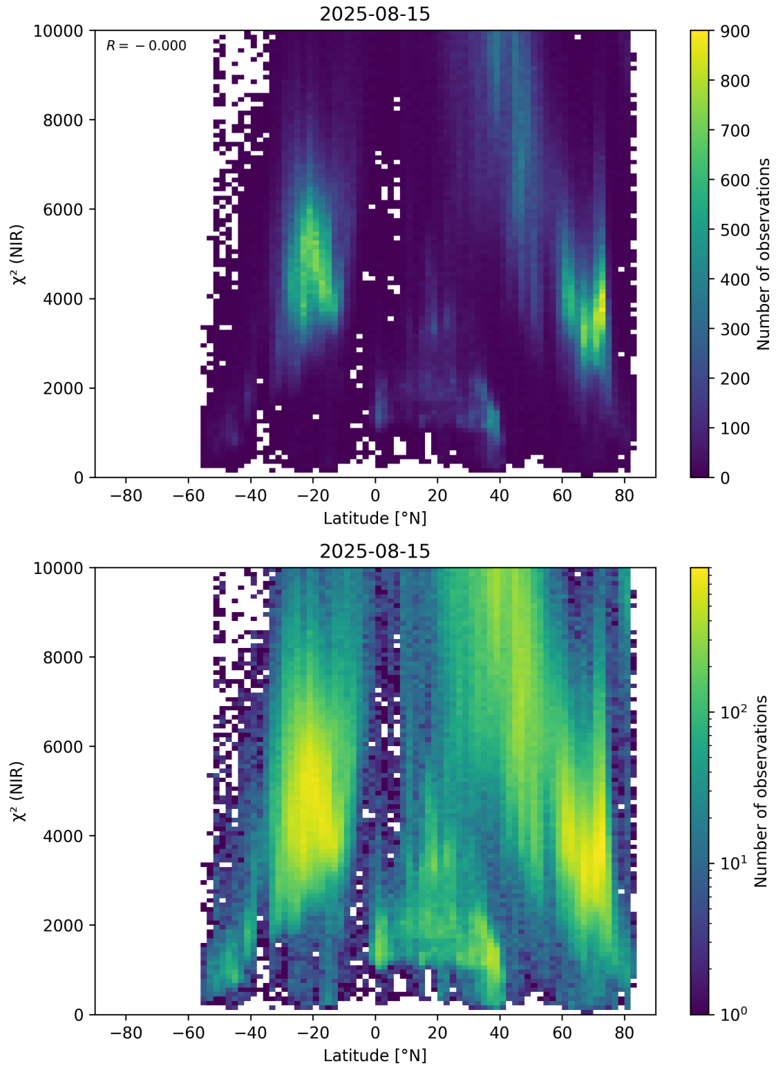
Figure 53: Scatter density plot of “Latitude” against “ \chi^2 (NIR)” for 2025-08-14 to 2025-08-16.
