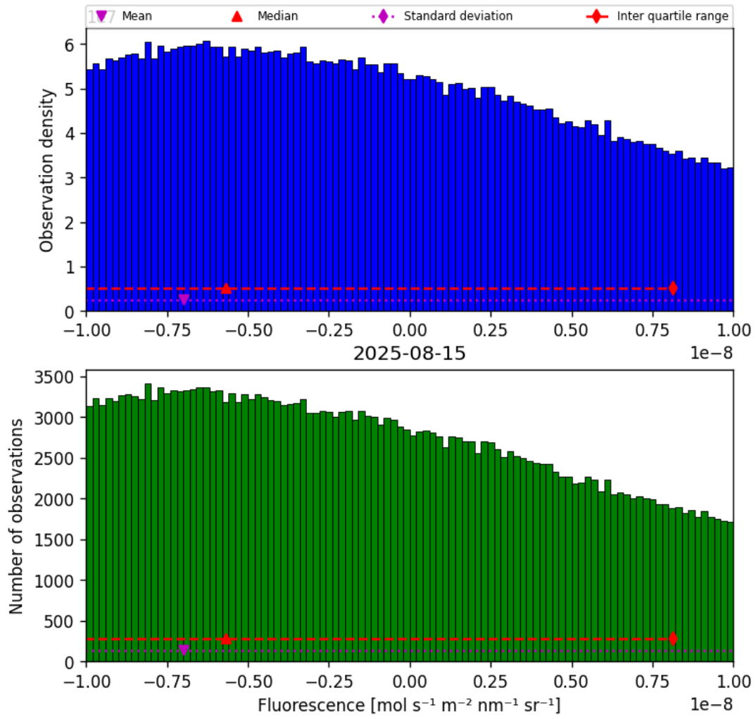
Figure 32: Histogram of “Fluorescence” for 2025-08-14 to 2025-08-16
