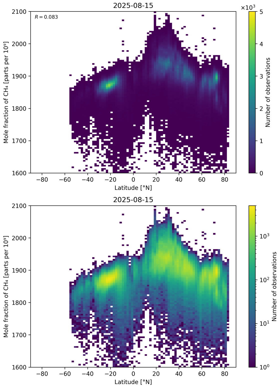
Figure 57: Scatter density plot of “Latitude” against “Mole fraction of \text{CH}_4 ” for 2025-08-14 to 2025-08-16.
