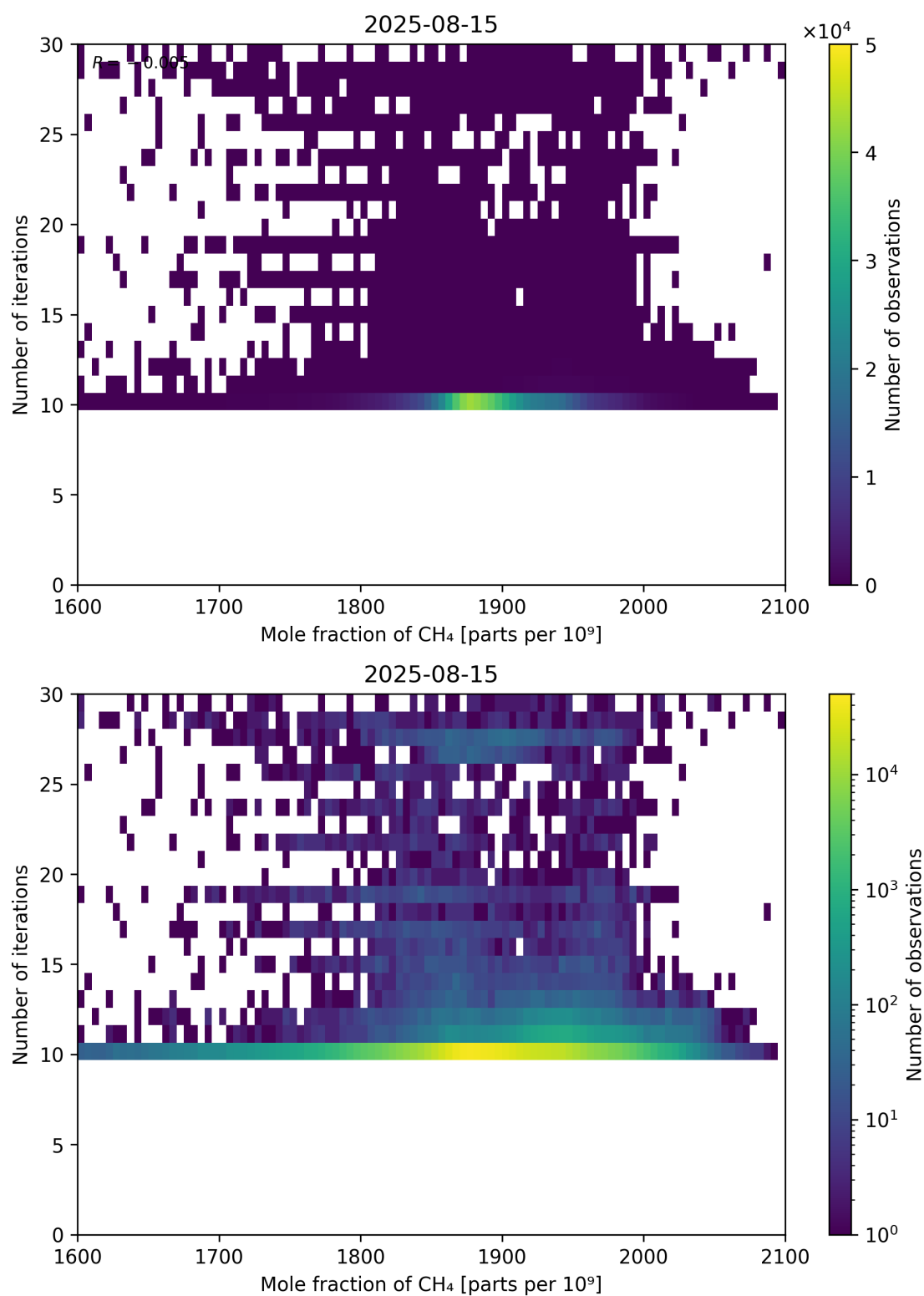
Figure 76: Scatter density plot of “Mole fraction of CH 4 ” against “Number of iterations” for 2025-08-14 to 2025-08-16.
