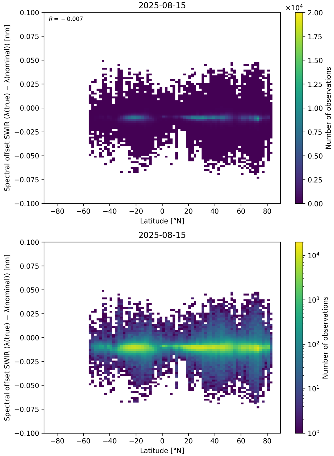
Figure 62: Scatter density plot of “Latitude” against “Spectral offset SWIR ( \lambda_{\text{true}} - \lambda_{\text{nominal}} )” for 2025-08-14 to 2025-08-16.
