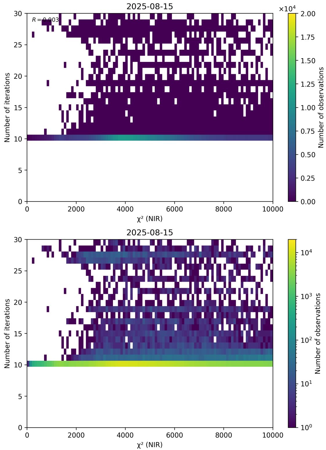
Figure 46: Scatter density plot of “ \chi^2 (NIR)” against “Number of iterations” for 2025-08-14 to 2025-08-16.
