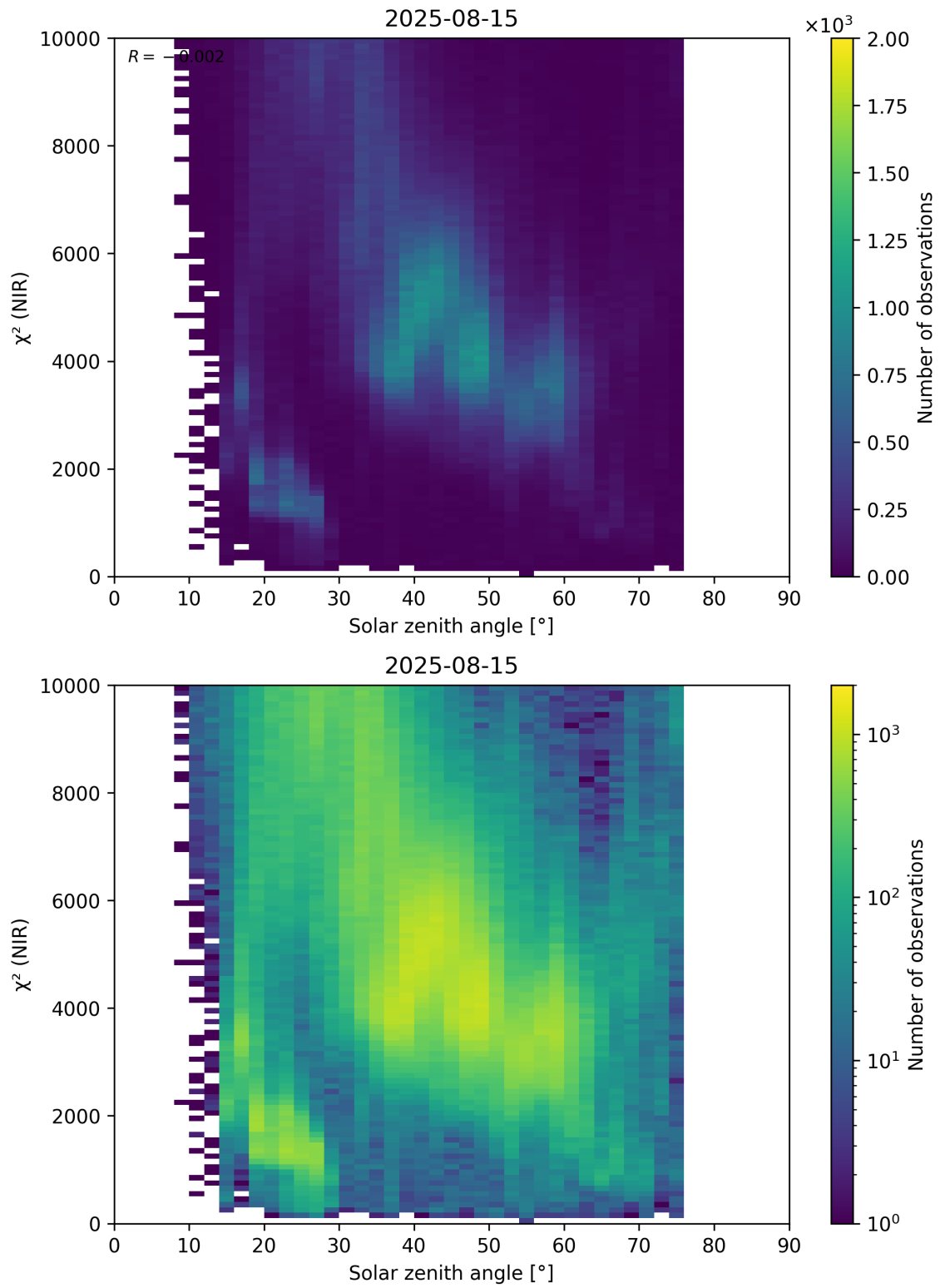
Figure 94: Scatter density plot of “Solar zenith angle” against “ \chi^2 (NIR)” for 2025-08-14 to 2025-08-16.
