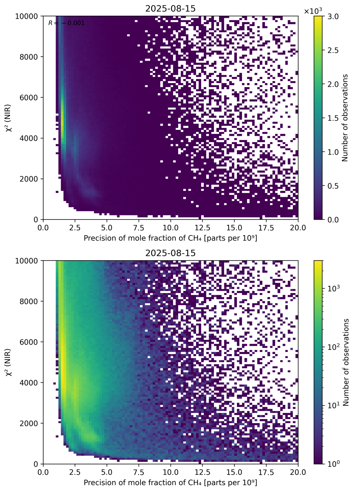
Figure 78: Scatter density plot of “Precision of mole fraction of CH 4 ” against “ \chi^2 (NIR)” for 2025-08-14 to 2025-08-16.
