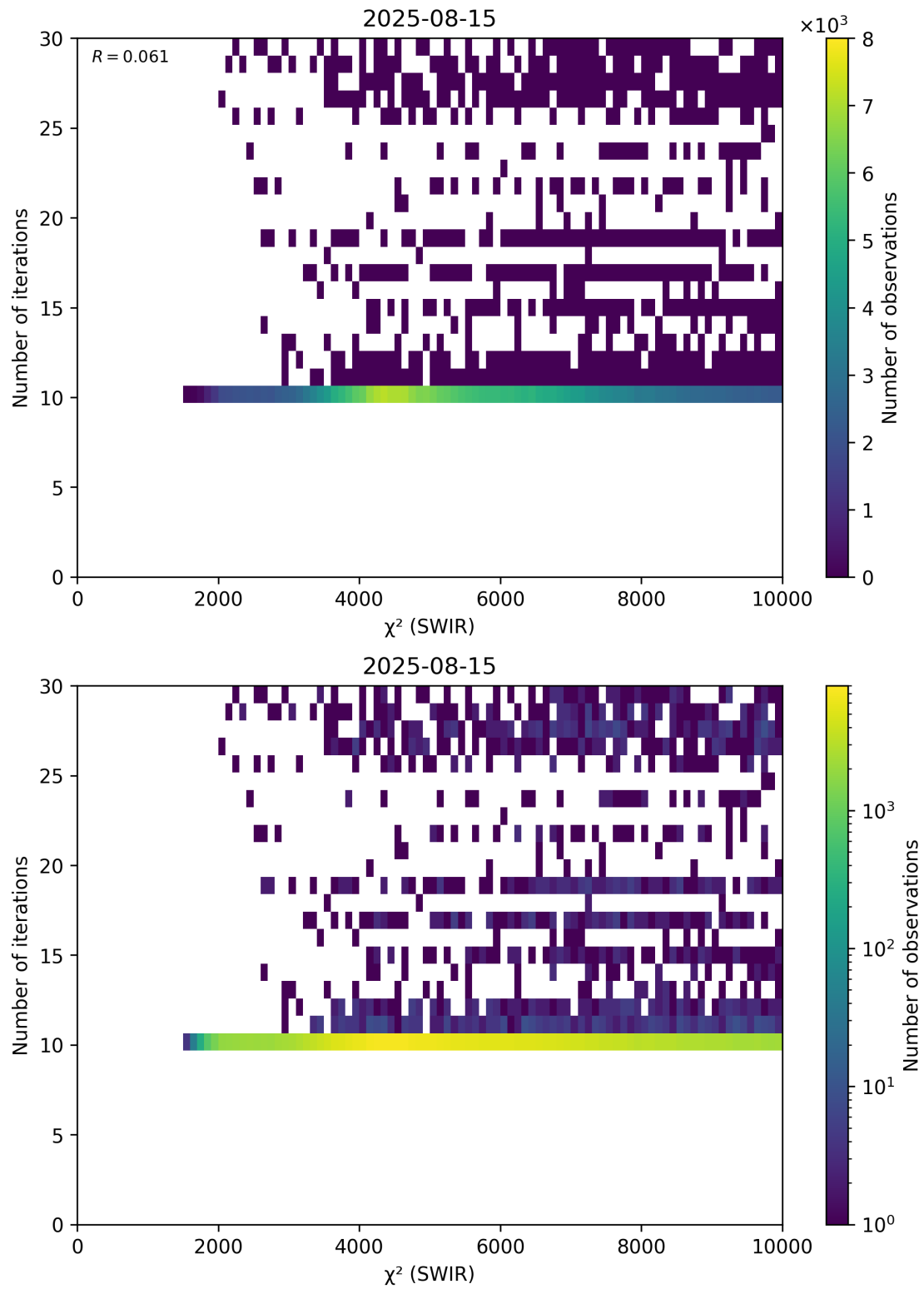
Figure 50: Scatter density plot of “ \chi^2 (SWIR)” against “Number of iterations” for 2025-08-14 to 2025-08-16.
