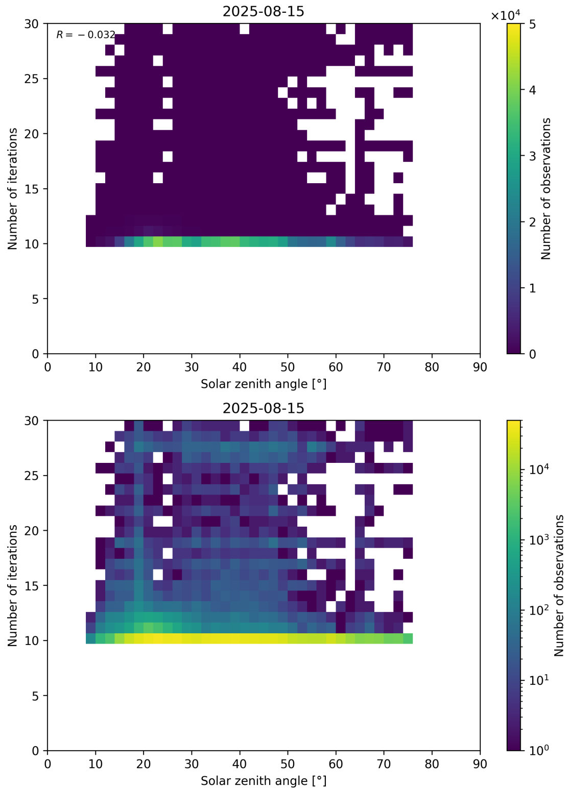
Figure 102: Scatter density plot of “Solar zenith angle” against “Number of iterations” for 2025-08-14 to 2025-08-16.
