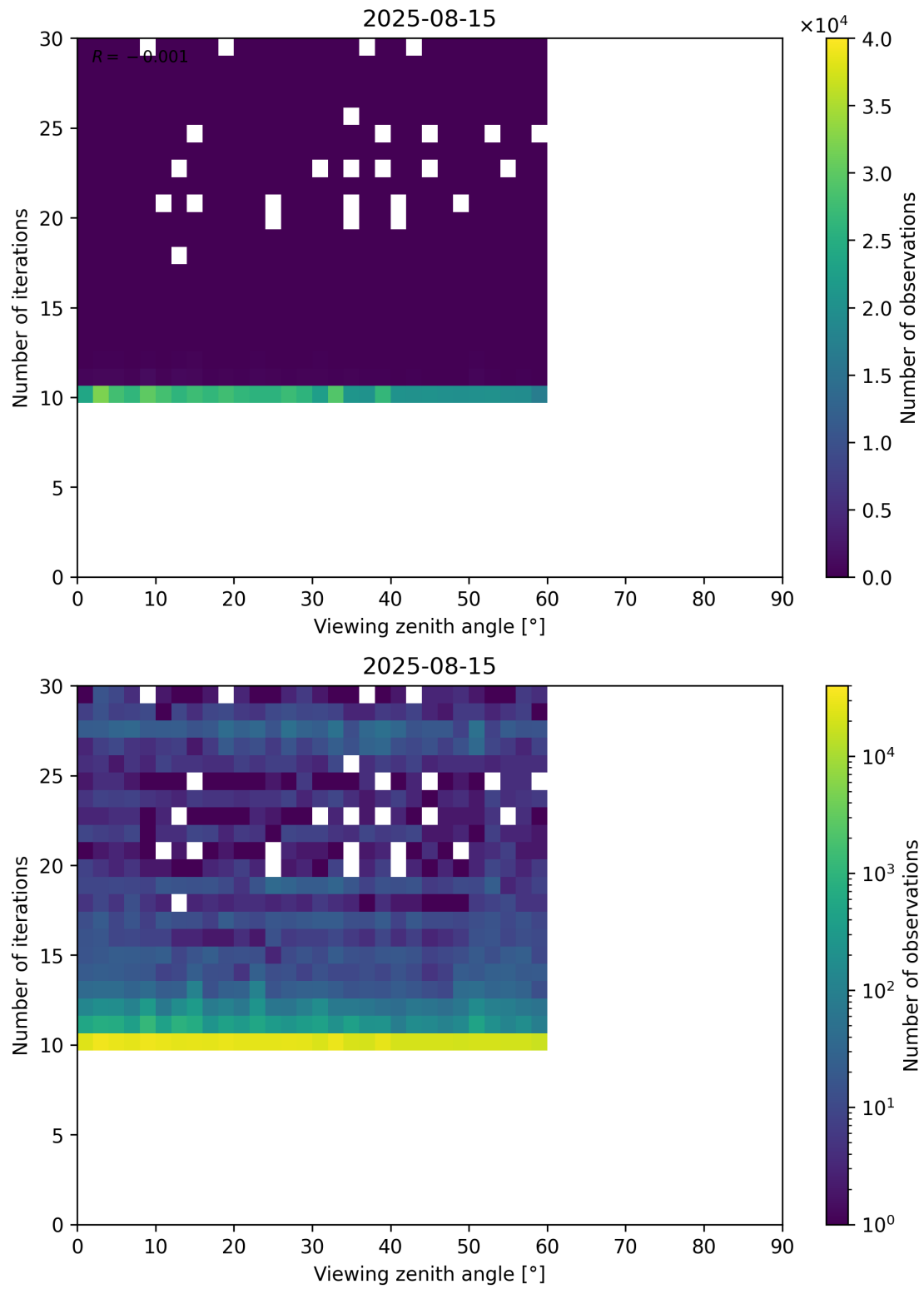
Figure 113: Scatter density plot of “Viewing zenith angle” against “Number of iterations” for 2025-08-14 to 2025-08-16.
