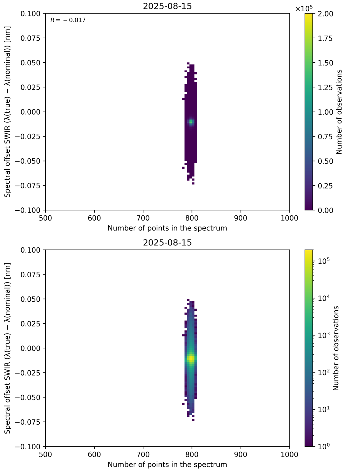
Figure 93: Scatter density plot of “Number of points in the spectrum” against “Spectral offset SWIR ( \lambda_{\text{true}} - \lambda_{\text{nominal}} )” for 2025-08-14 to 2025-08-16.
