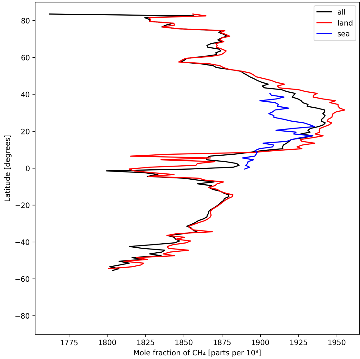
Figure 12: Zonal average of “Mole fraction of CH 4 ” for 2025-08-14 to 2025-08-16.
