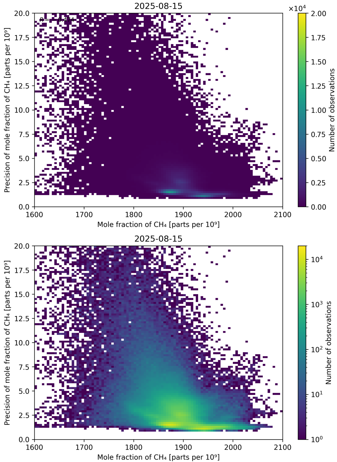
Figure 75: Scatter density plot of “Mole fraction of CH 4 ” against “Precision of mole fraction of CH 4 ” for 2025-08-14 to 2025-08-16.
