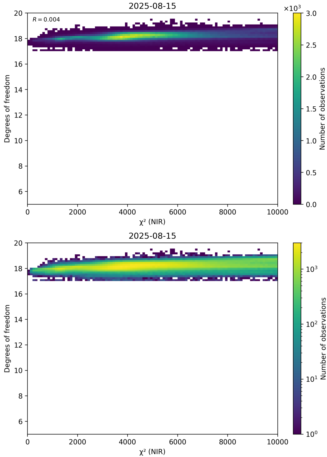
Figure 44: Scatter density plot of “ \chi^2 (NIR)” against “Degrees of freedom” for 2025-08-14 to 2025-08-16.
