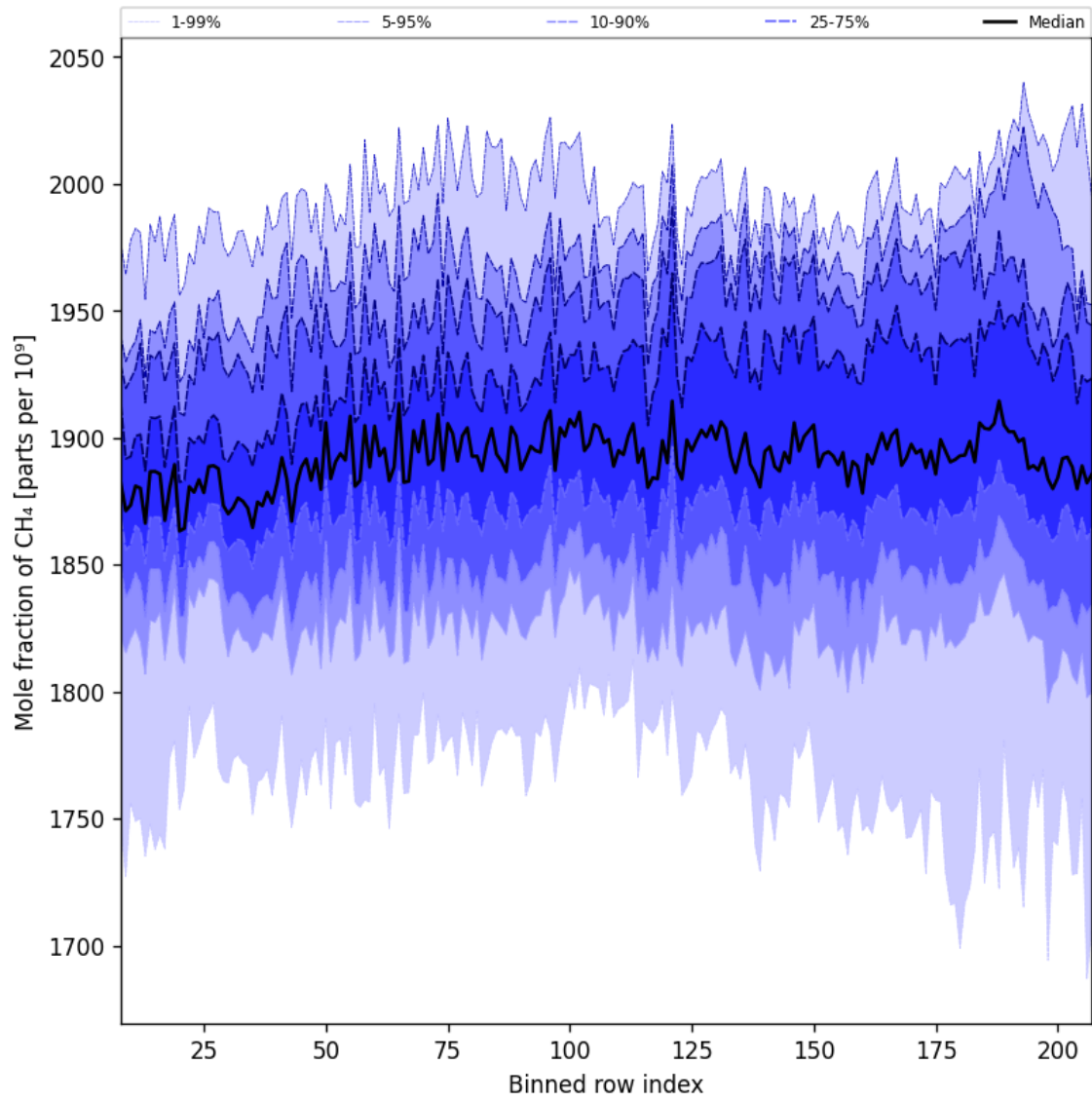
Figure 34: Along track statistics of “Mole fraction of CH 4 ” for 2025-08-14 to 2025-08-16
