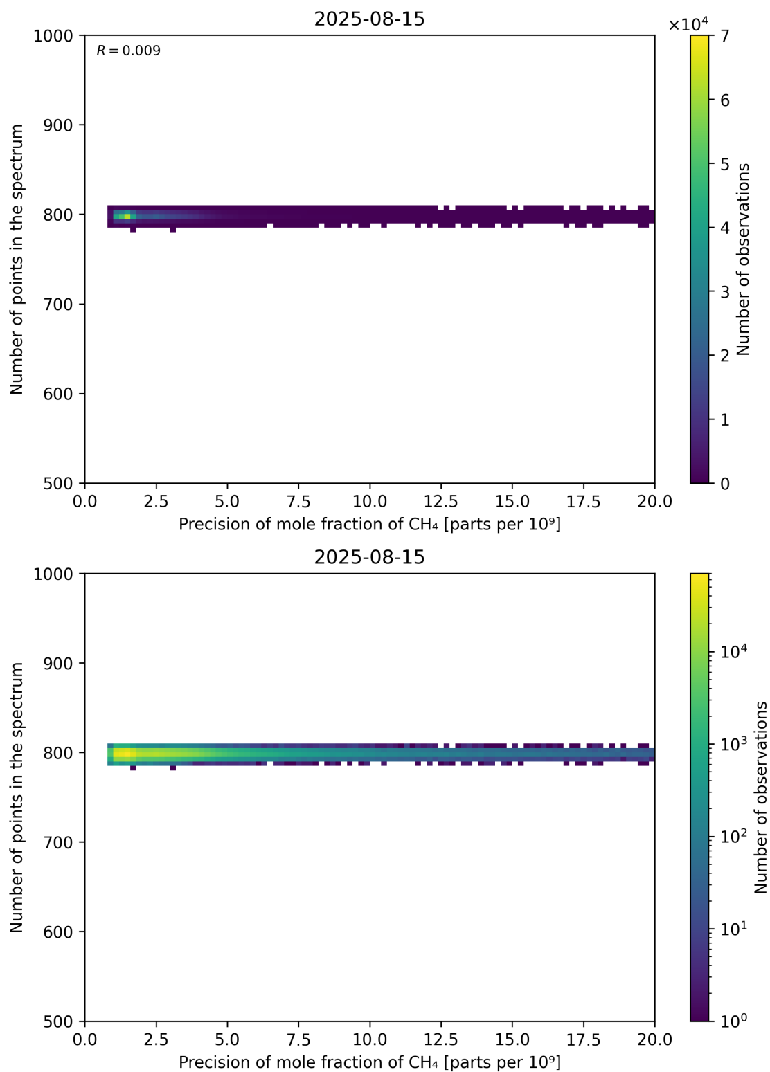
Figure 84: Scatter density plot of “Precision of mole fraction of CH 4 ” against “Number of points in the spectrum” for 2025-08-14 to 2025-08-16.
