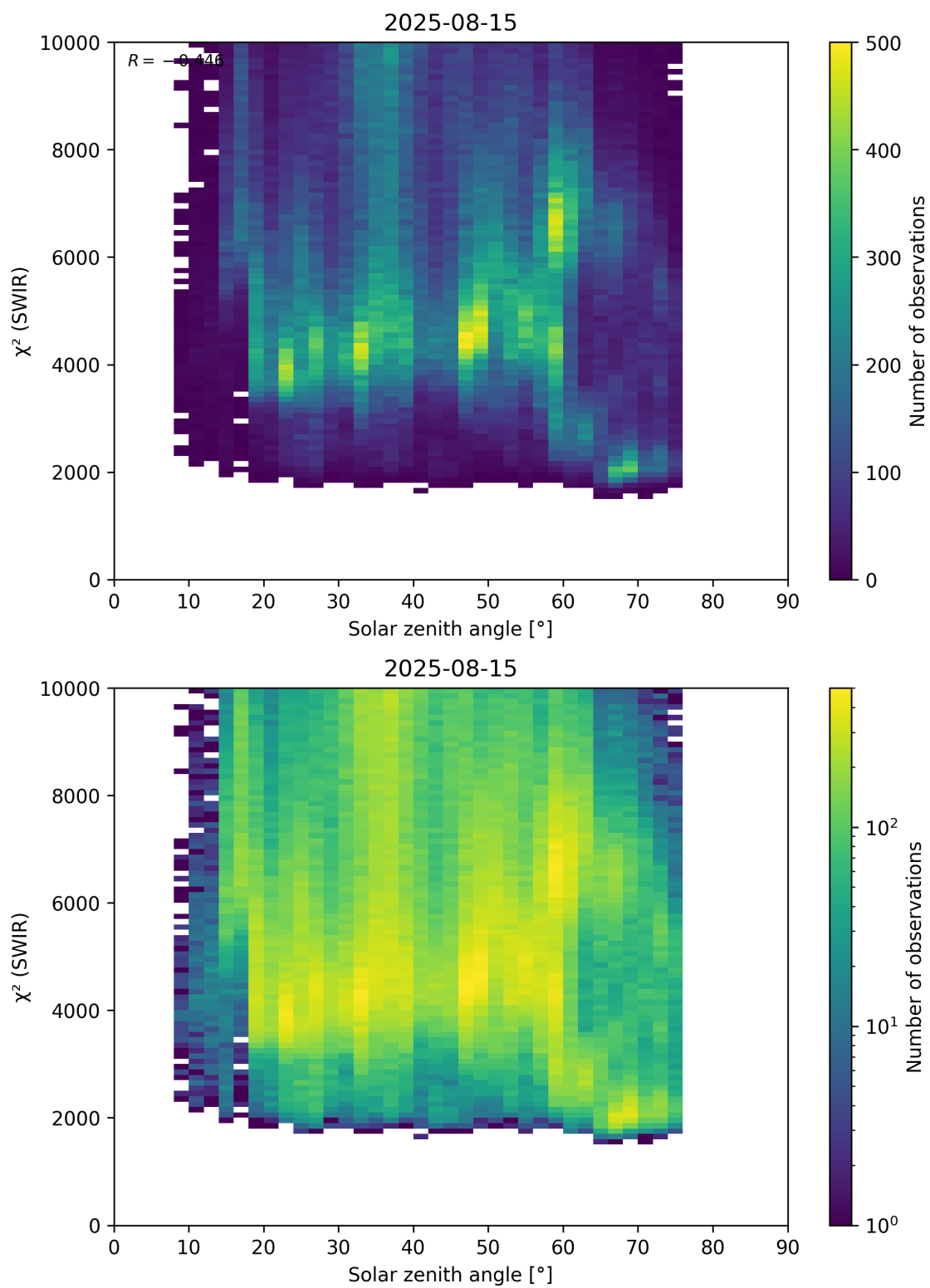
Figure 95: Scatter density plot of “Solar zenith angle” against “ \chi^2 (SWIR)” for 2025-08-14 to 2025-08-16.
