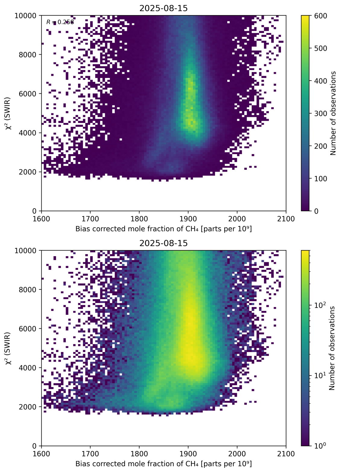
Figure 64: Scatter density plot of “Bias corrected mole fraction of \text{CH}_4 ” against “ \chi^2 (SWIR)” for 2025-08-14 to 2025-08-16.
