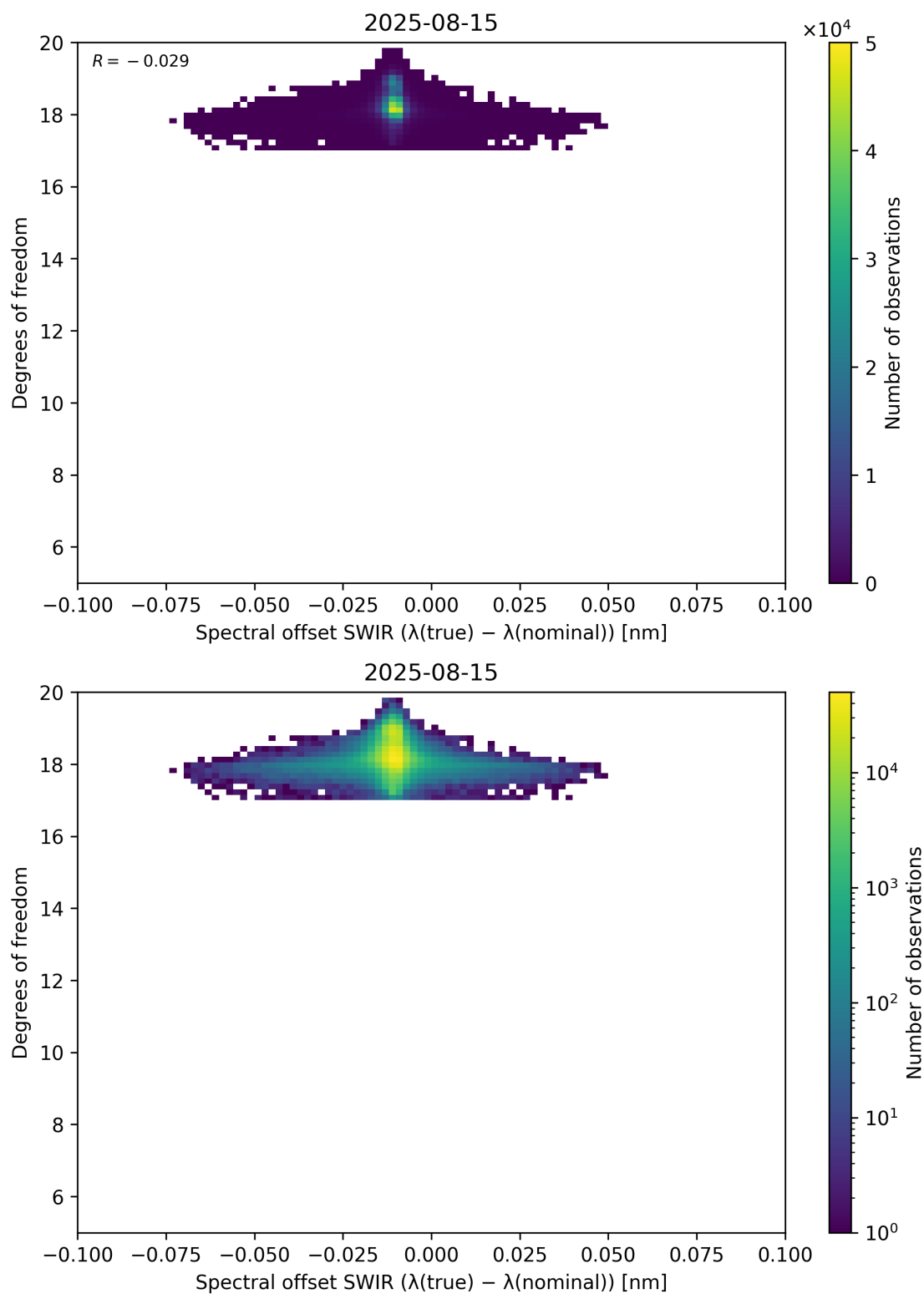
Figure 119: Scatter density plot of “Spectral offset SWIR ( \lambda_{\text{true}} - \lambda_{\text{nominal}} )” against “Degrees of freedom” for 2025-08-14 to 2025-08-16.
