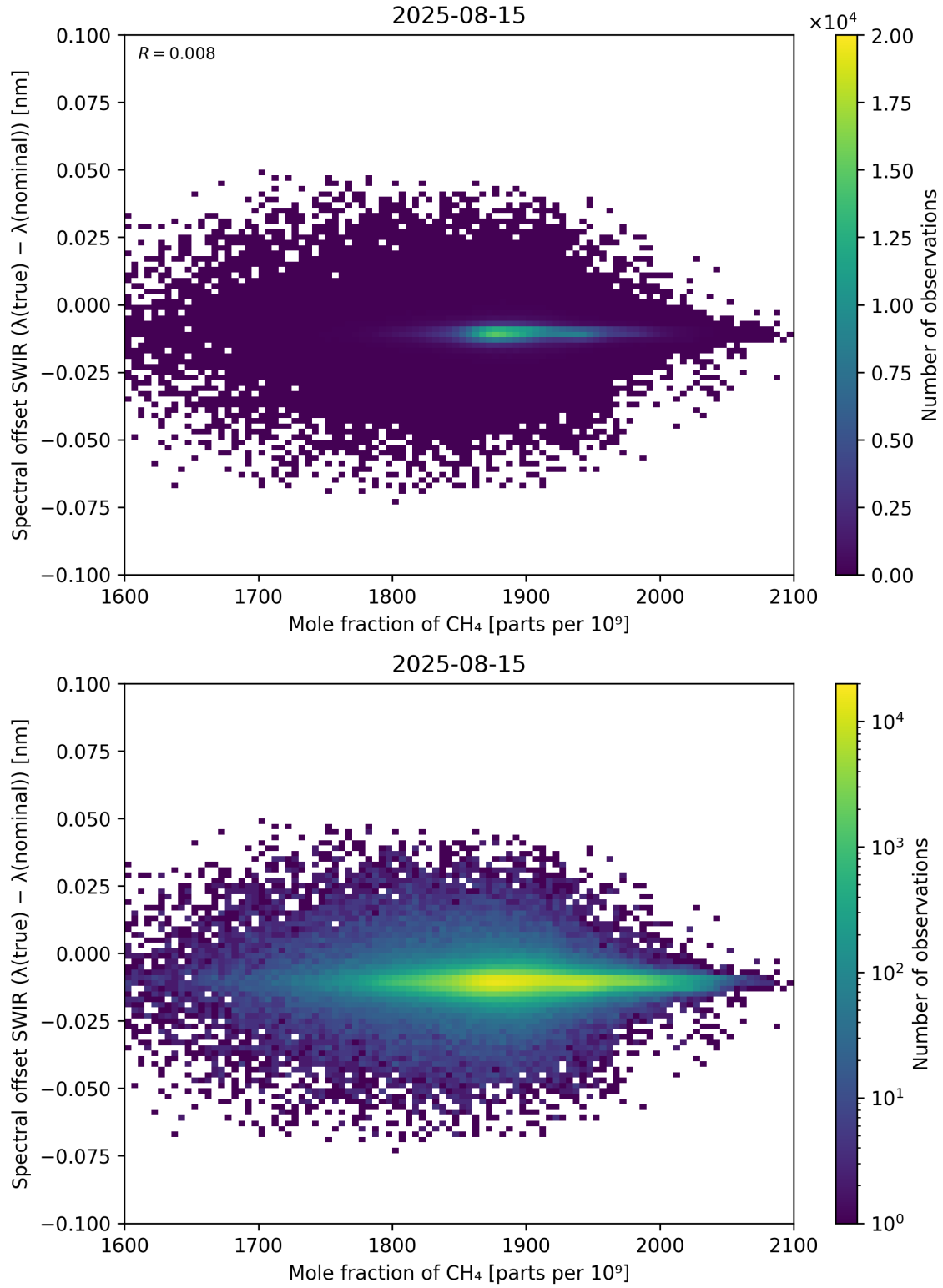
Figure 86: Scatter density plot of “Mole fraction of CH 4 ” against “Spectral offset SWIR ( \lambda_{\text{true}} - \lambda_{\text{nominal}} )” for 2025-08-14 to 2025-08-16.
