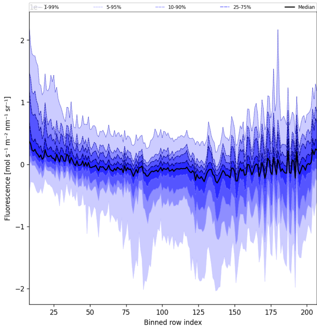
Figure 43: Along track statistics of “Fluorescence” for 2025-08-14 to 2025-08-16
