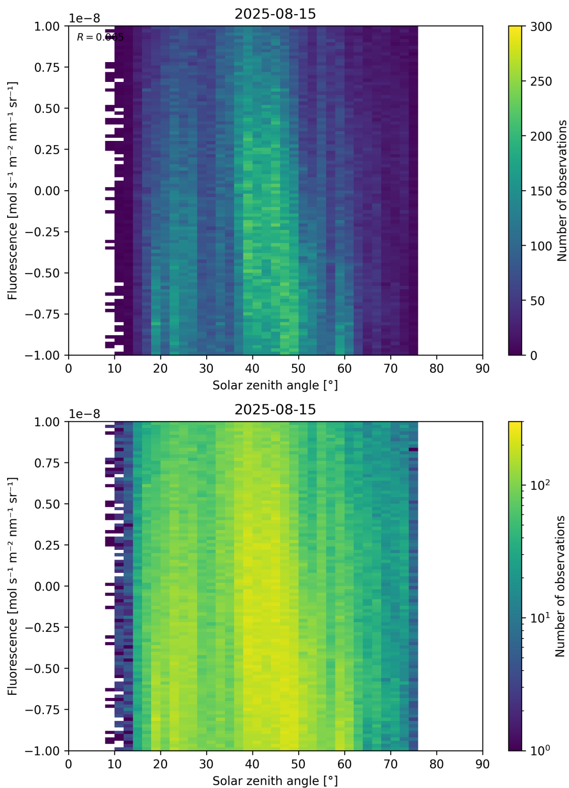
Figure 97: Scatter density plot of “Solar zenith angle” against “Fluorescence” for 2025-08-14 to 2025-08-16.
