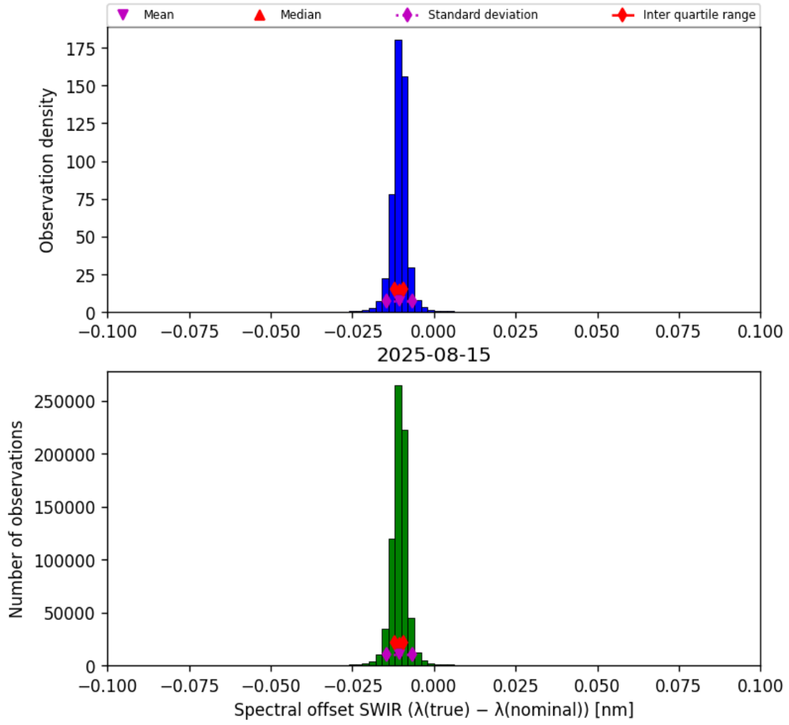
Figure 27: Histogram of “Spectral offset SWIR ( \lambda_{\text{true}} - \lambda_{\text{nominal}} )” for 2025-08-14 to 2025-08-16
