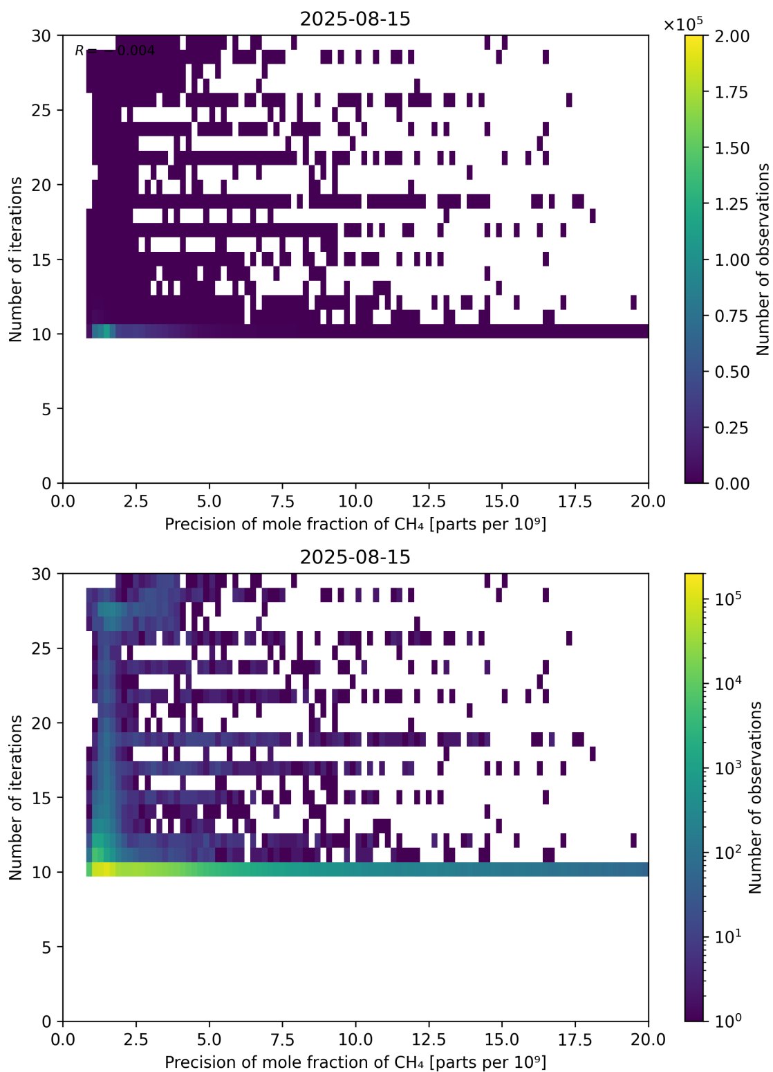
Figure 83: Scatter density plot of “Precision of mole fraction of CH 4 ” against “Number of iterations” for 2025-08-14 to 2025-08-16.
