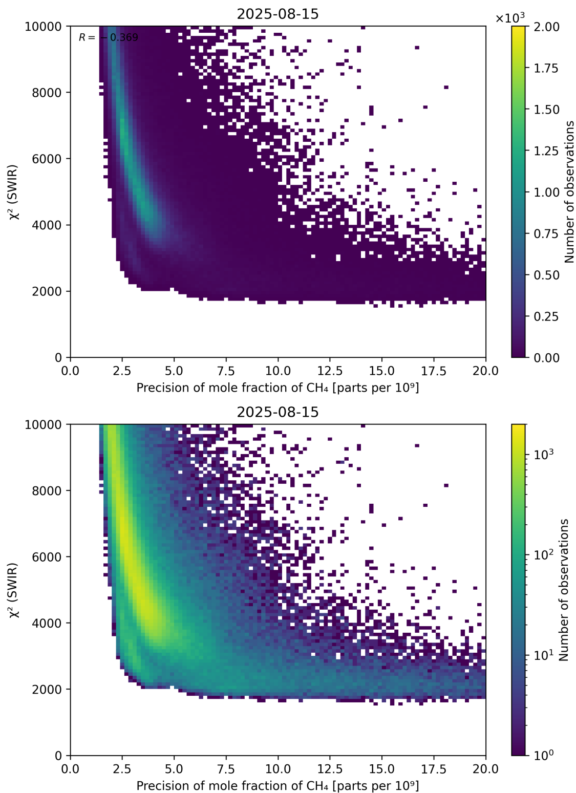
Figure 79: Scatter density plot of “Precision of mole fraction of \text{CH}_4 ” against “ \chi^2 (SWIR)” for 2025-08-14 to 2025-08-16.
