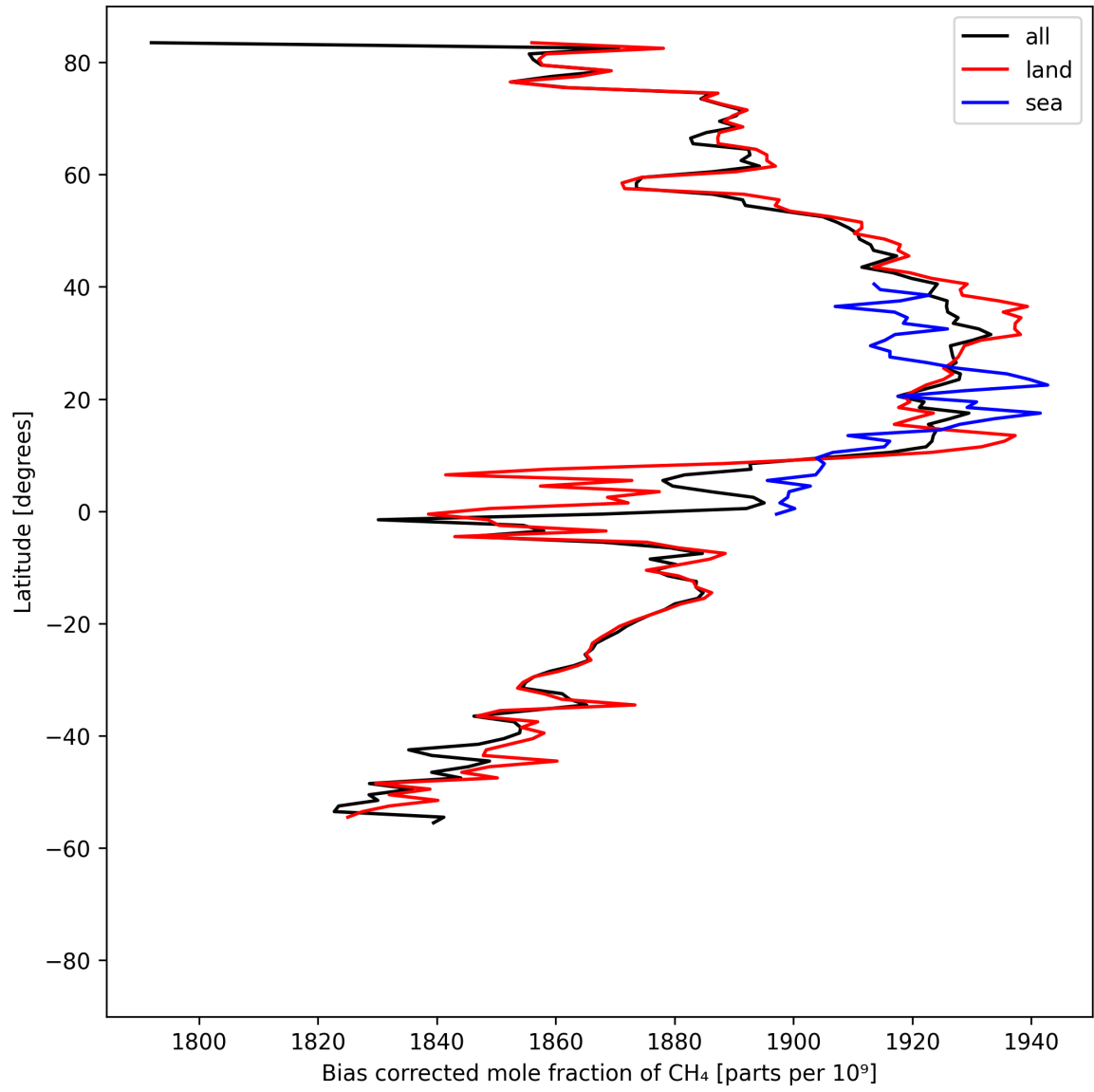
Figure 14: Zonal average of “Bias corrected mole fraction of CH 4 ” for 2025-08-14 to 2025-08-16.
