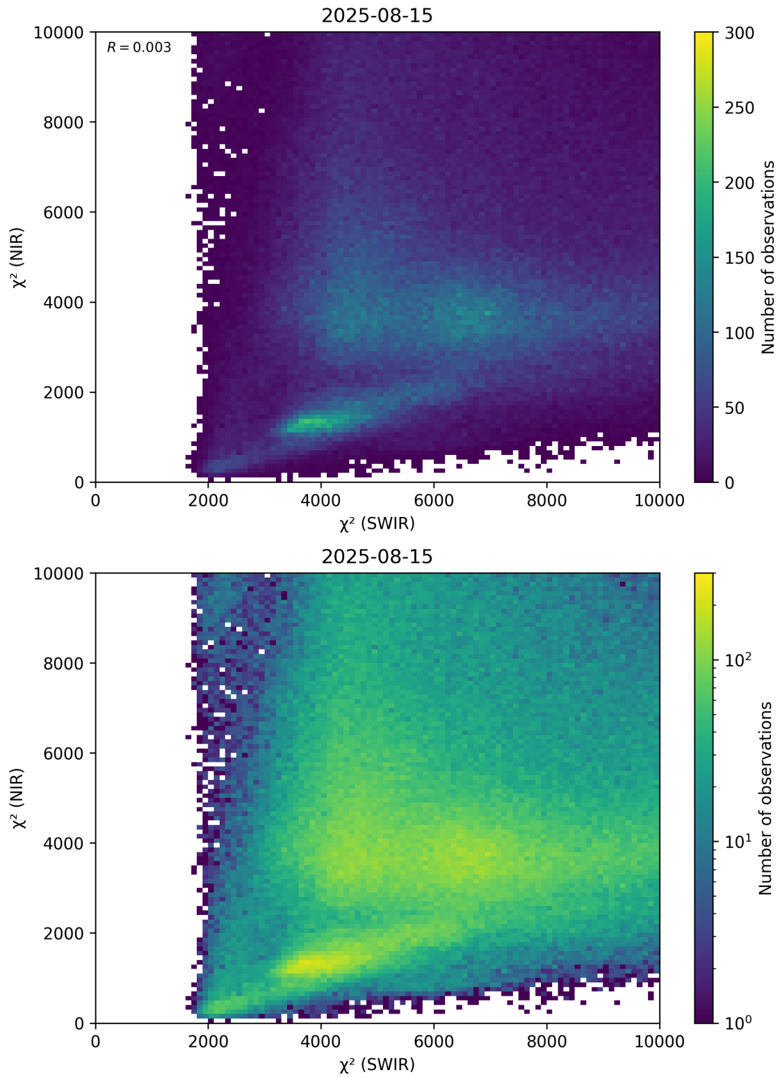
Figure 47: Scatter density plot of “ \chi^2 (SWIR)” against “ \chi^2 (NIR)” for 2025-08-14 to 2025-08-16.
