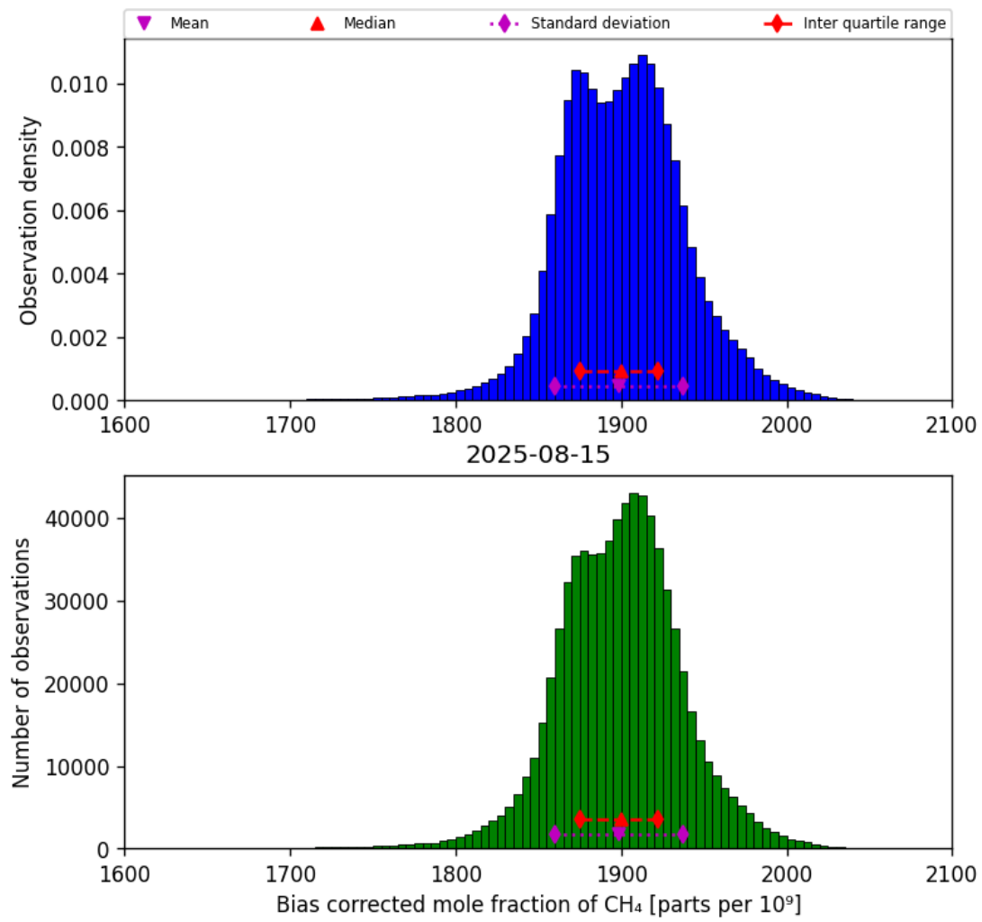
Figure 25: Histogram of “Bias corrected mole fraction of CH 4 ” for 2025-08-14 to 2025-08-16
