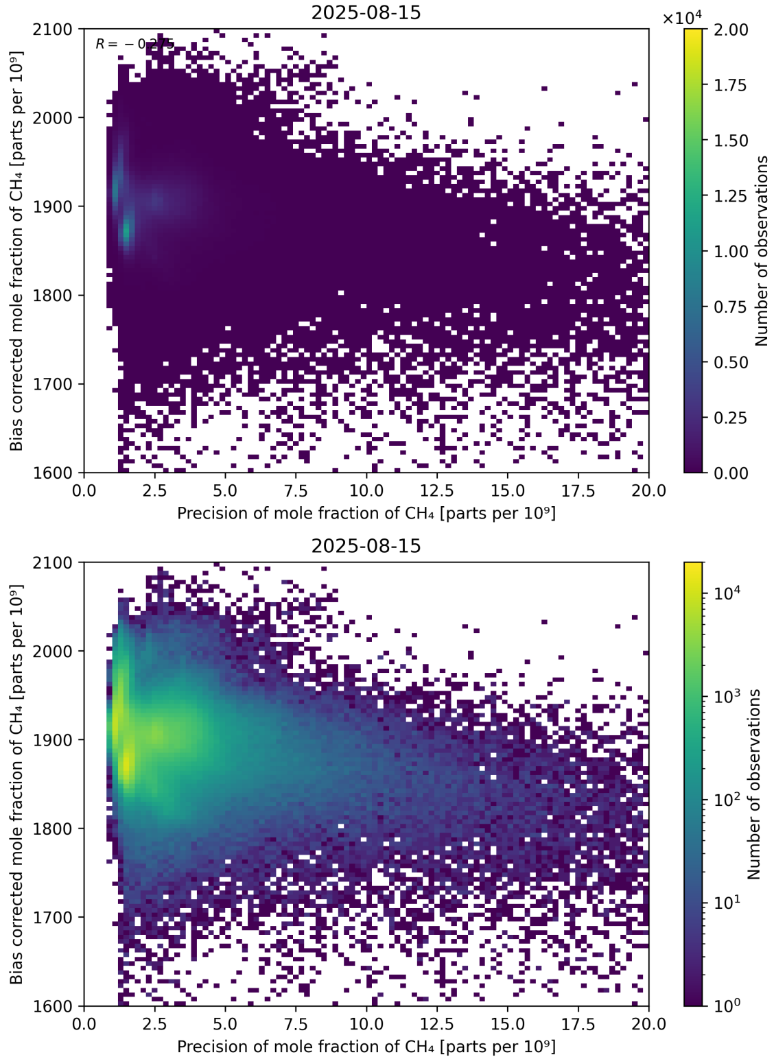
Figure 82: Scatter density plot of “Precision of mole fraction of CH 4 ” against “Bias corrected mole fraction of CH 4 ” for 2025-08-14 to 2025-08-16.
