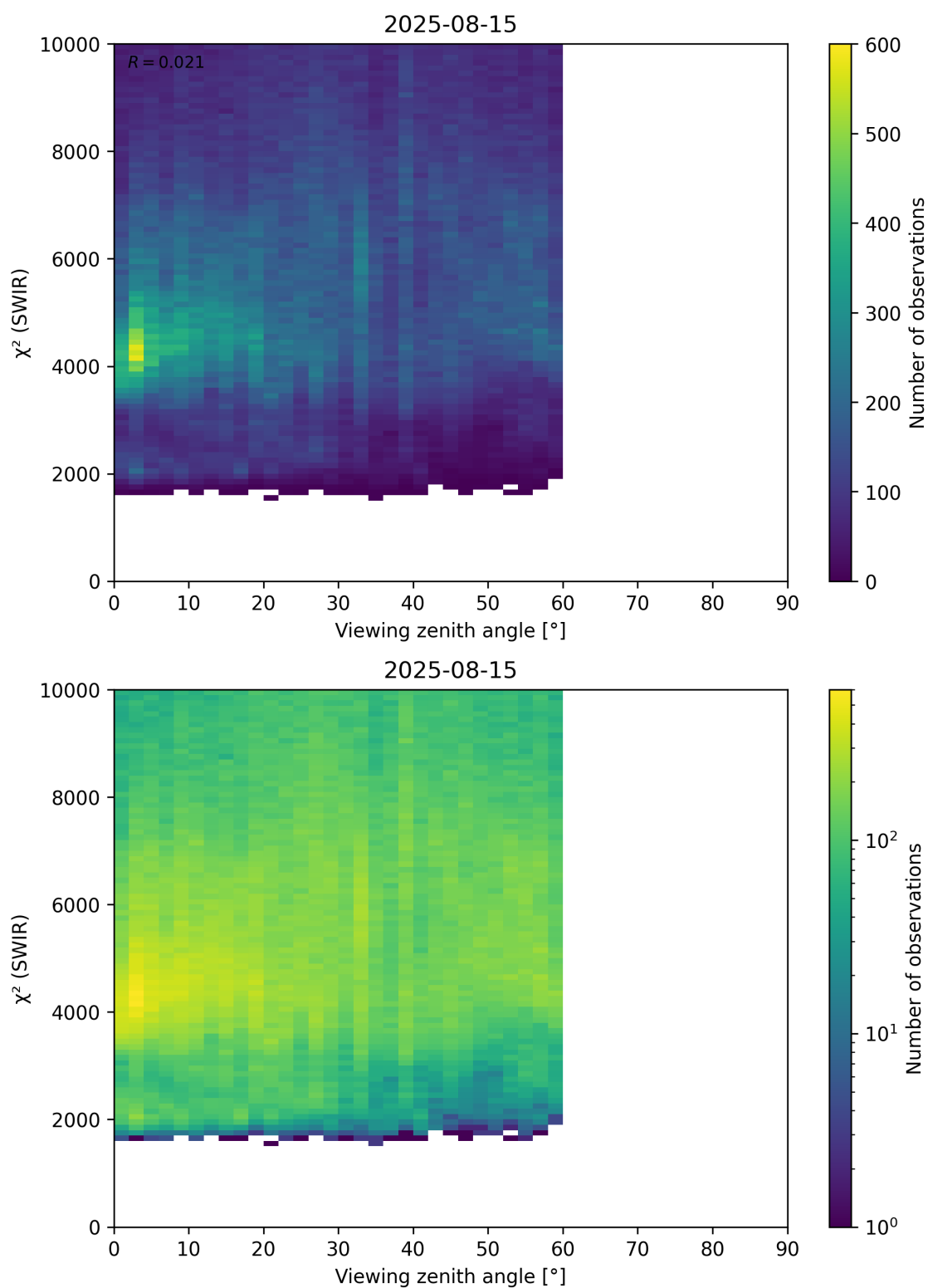
Figure 106: Scatter density plot of “Viewing zenith angle” against “ \chi^2 (SWIR)” for 2025-08-14 to 2025-08-16.
