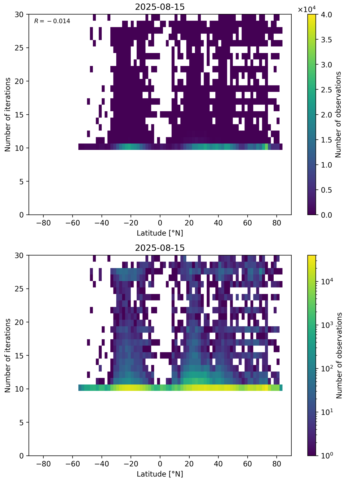
Figure 60: Scatter density plot of “Latitude” against “Number of iterations” for 2025-08-14 to 2025-08-16.
