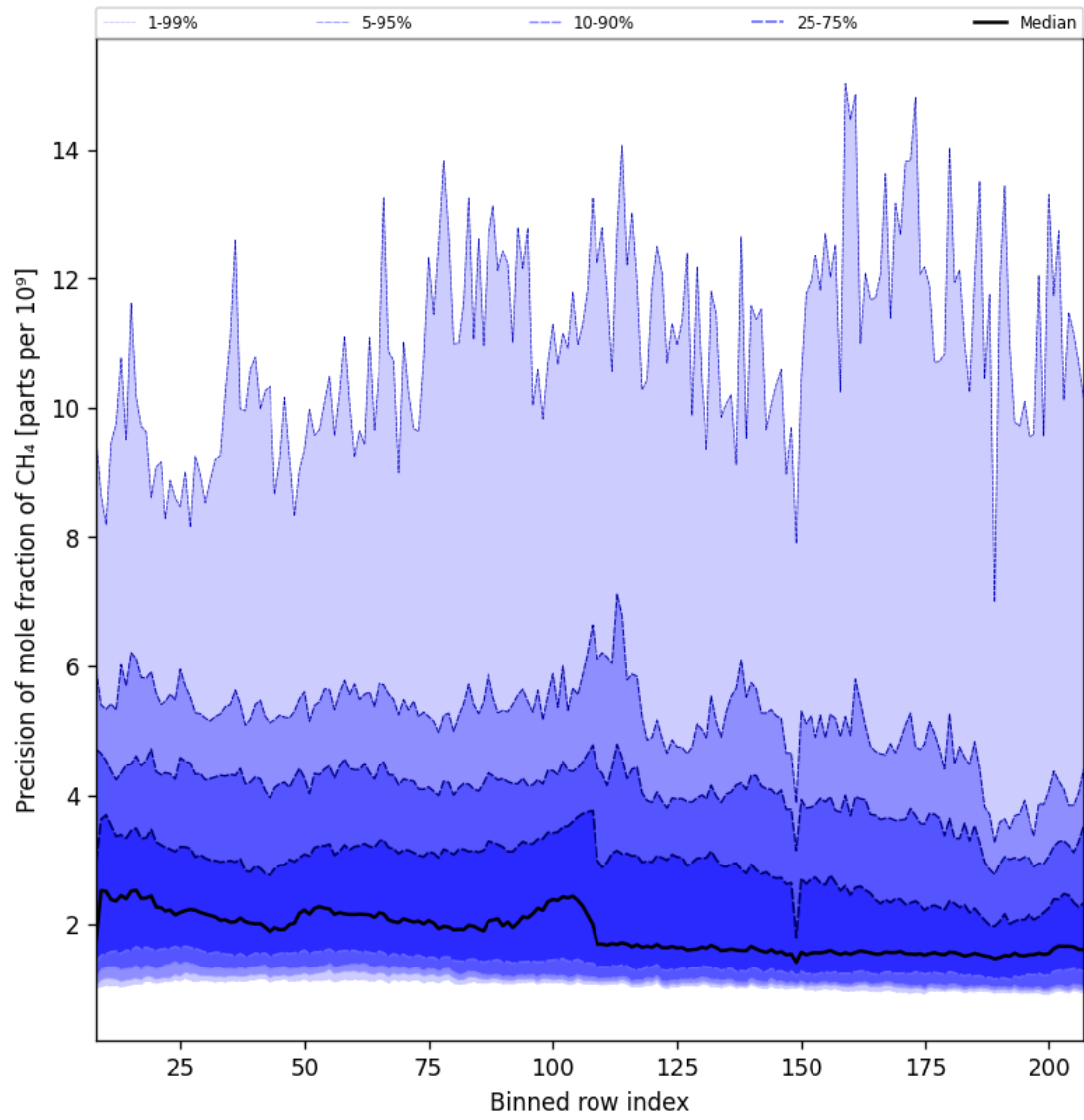
Figure 35: Along track statistics of “Precision of mole fraction of CH 4 ” for 2025-08-14 to 2025-08-16
