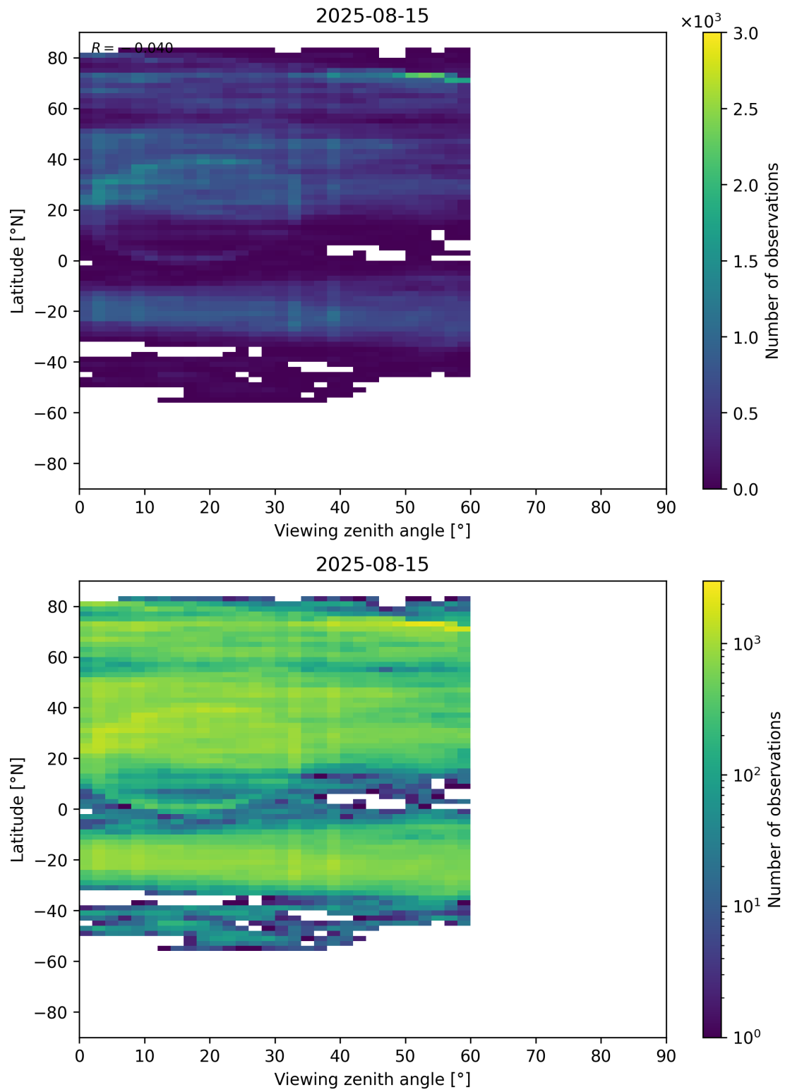
Figure 109: Scatter density plot of “Viewing zenith angle” against “Latitude” for 2025-08-14 to 2025-08-16.
