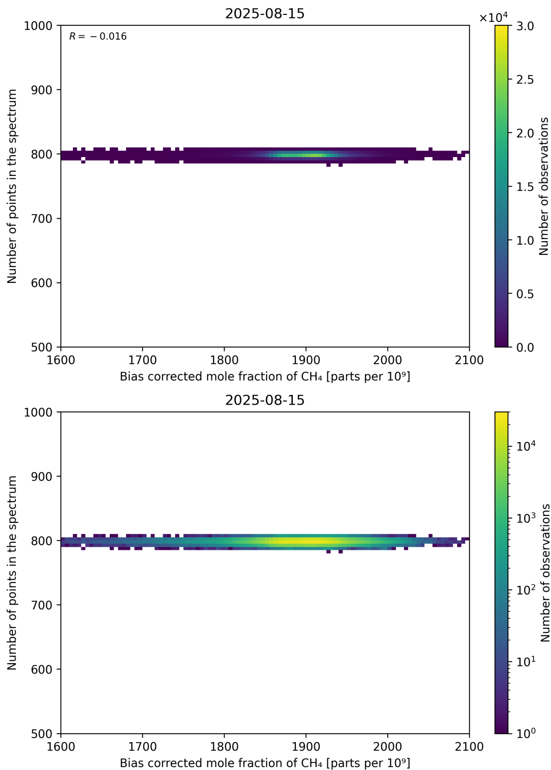
Figure 68: Scatter density plot of “Bias corrected mole fraction of CH 4 ” against “Number of points in the spectrum” for 2025-08-14 to 2025-08-16.
