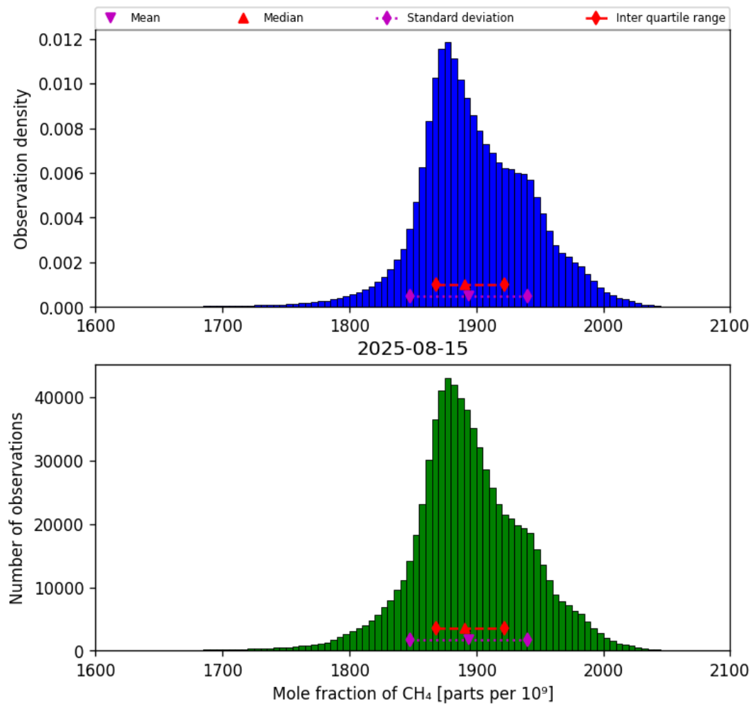
Figure 23: Histogram of “Mole fraction of CH 4 ” for 2025-08-14 to 2025-08-16
