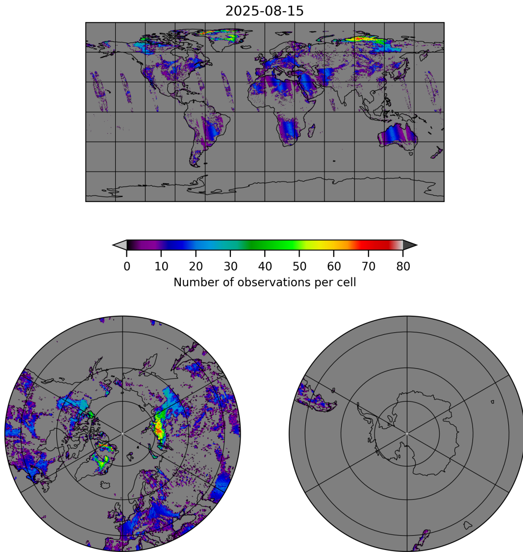
Figure 10: Map of the number of observations for 2025-08-14 to 2025-08-16
