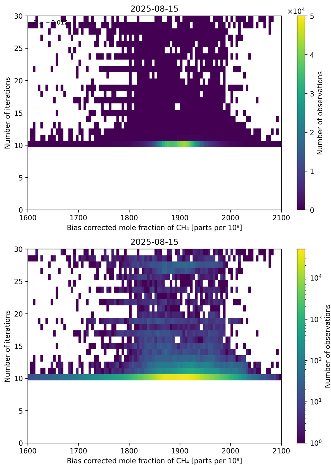
Figure 67: Scatter density plot of “Bias corrected mole fraction of CH 4 ” against “Number of iterations” for 2025-08-14 to 2025-08-16.
