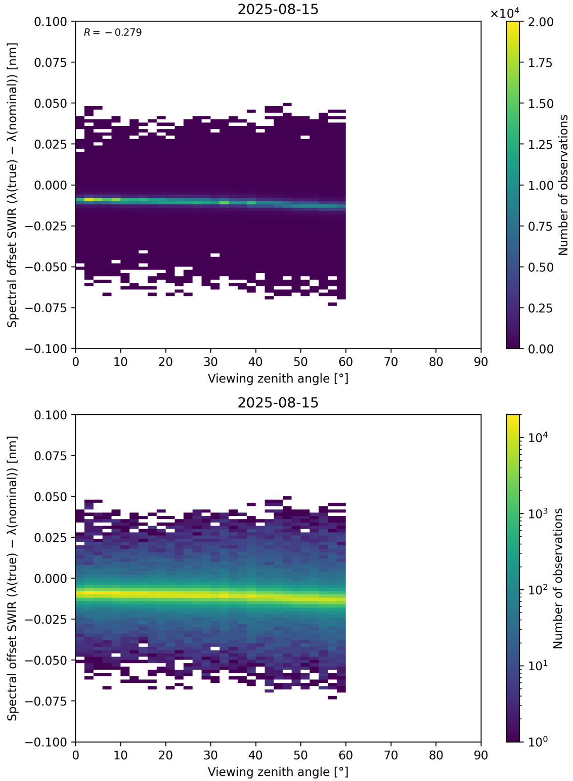
Figure 116: Scatter density plot of “Viewing zenith angle” against “Spectral offset SWIR ( \lambda_{\text{true}} - \lambda_{\text{nominal}} )” for 2025-08-14 to 2025-08-16.
