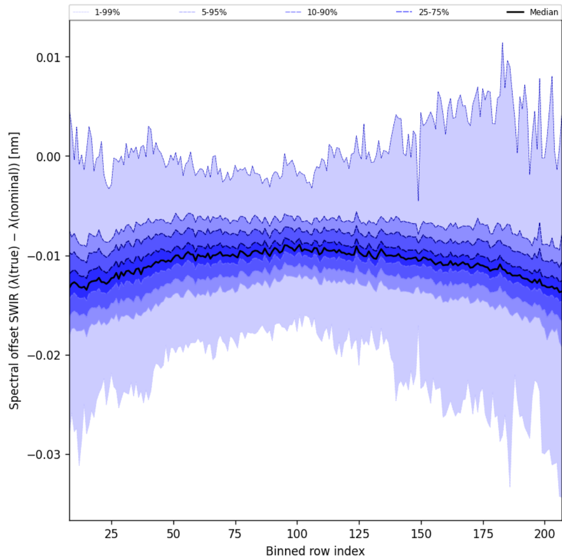
Figure 38: Along track statistics of “Spectral offset SWIR ( \lambda_{\text{true}} - \lambda_{\text{nominal}} )” for 2025-08-14 to 2025-08-16
