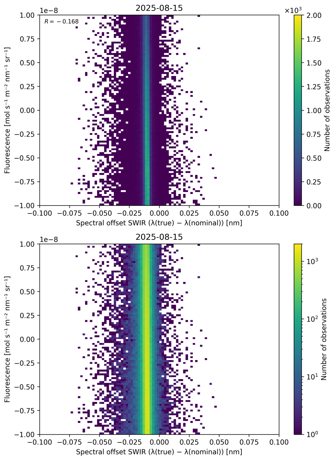
Figure 120: Scatter density plot of “Spectral offset SWIR ( \lambda_{\text{true}} - \lambda_{\text{nominal}} )” against “Fluorescence” for 2025-08-14 to 2025-08-16.
