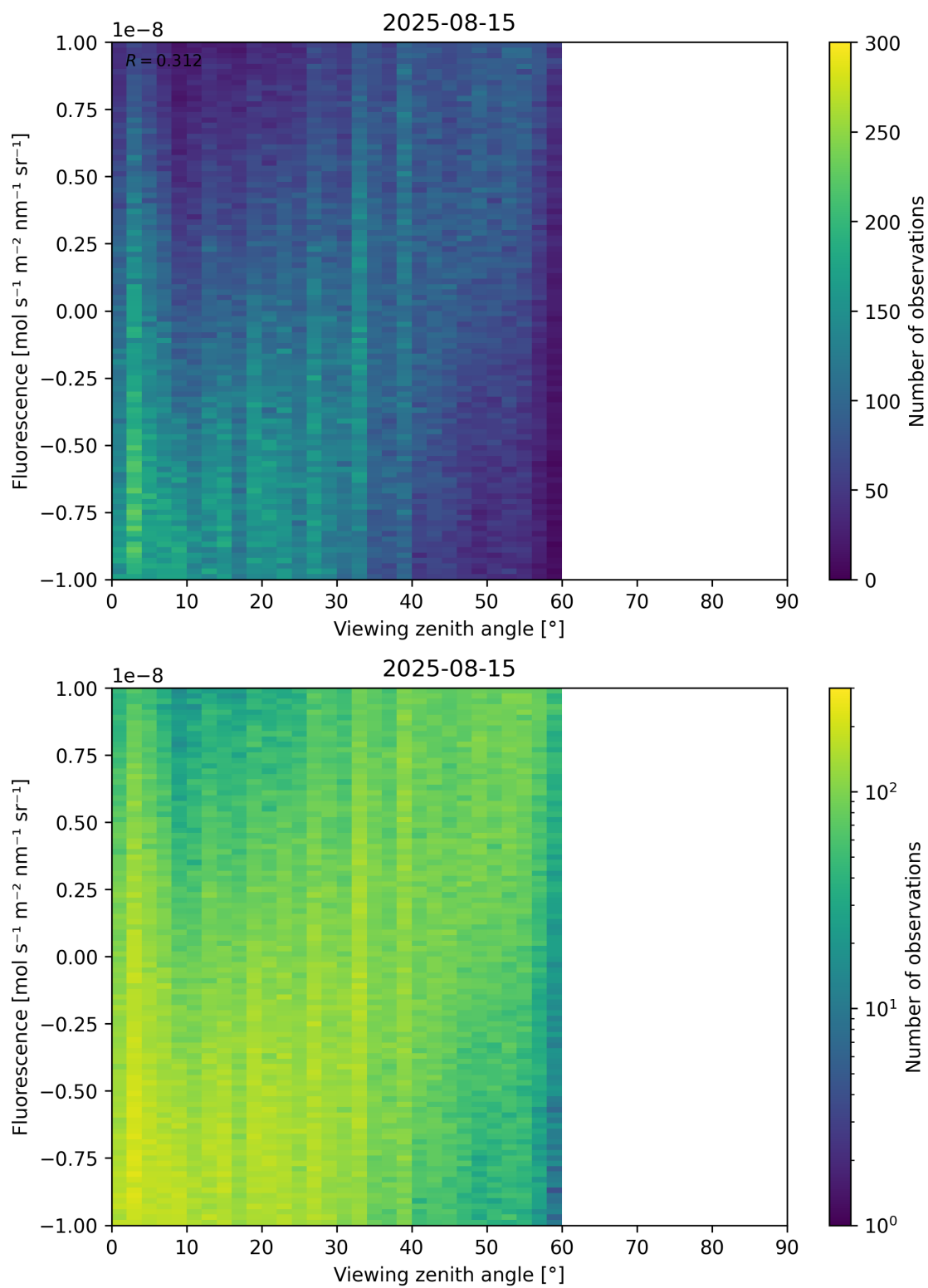
Figure 108: Scatter density plot of “Viewing zenith angle” against “Fluorescence” for 2025-08-14 to 2025-08-16.
