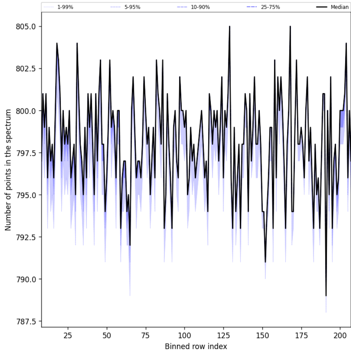
Figure 37: Along track statistics of “Number of points in the spectrum” for 2025-08-14 to 2025-08-16
