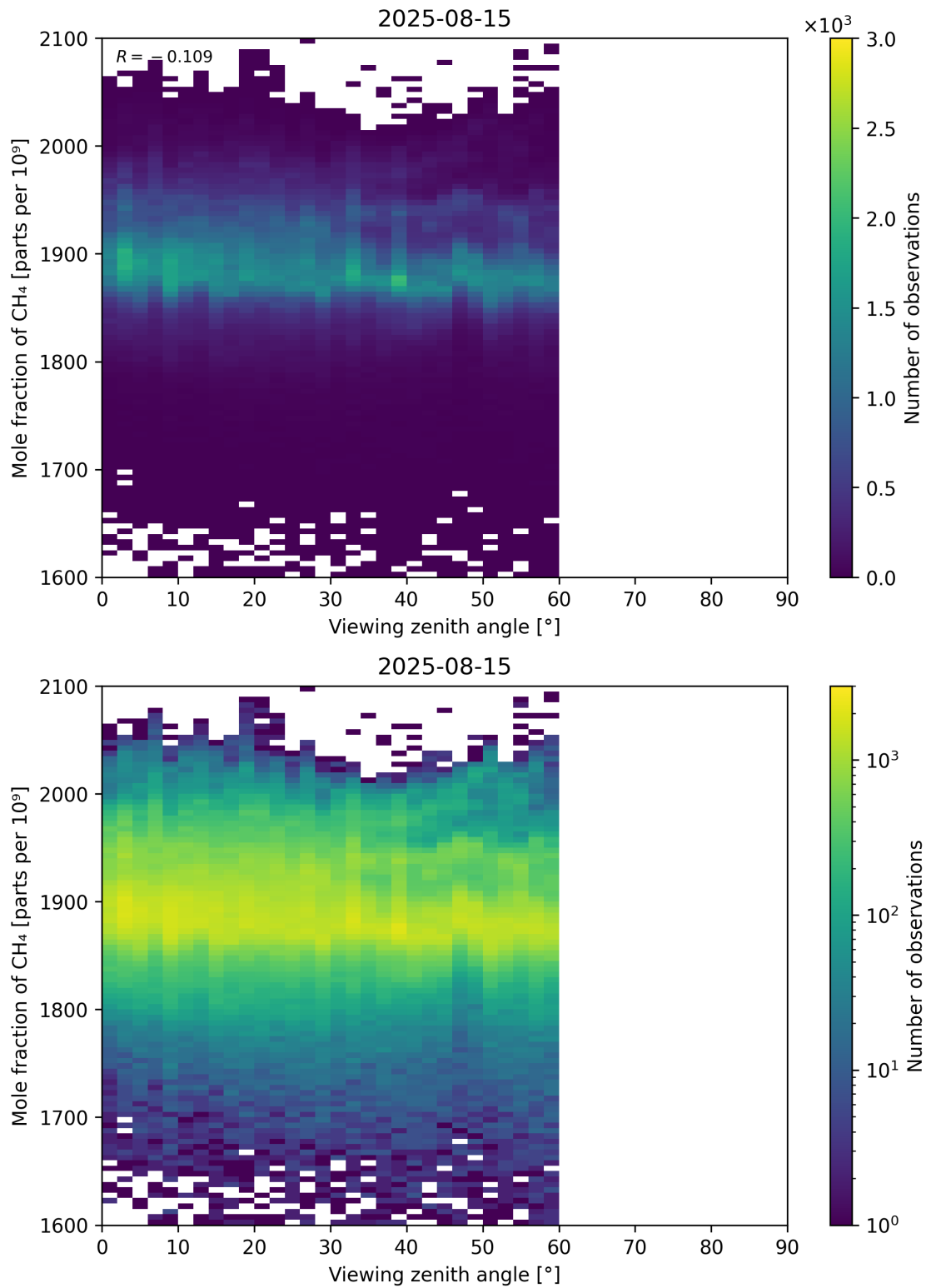
Figure 110: Scatter density plot of “Viewing zenith angle” against “Mole fraction of CH 4 ” for 2025-08-14 to 2025-08-16.
