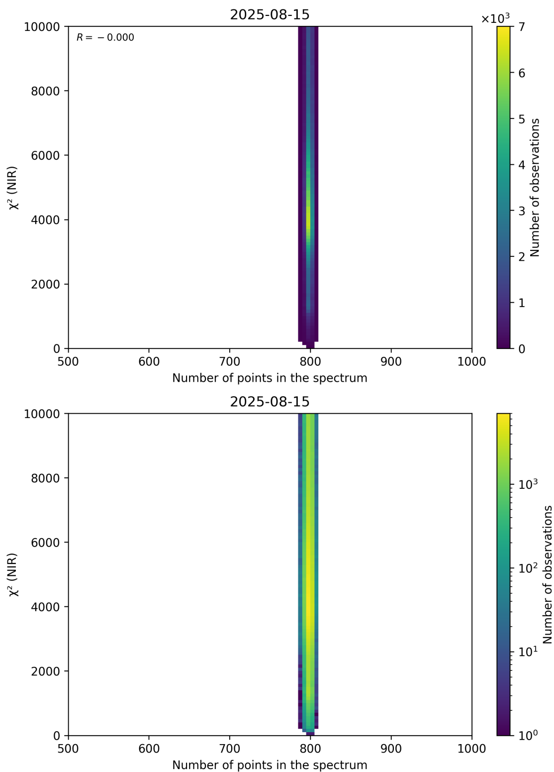
Figure 88: Scatter density plot of “Number of points in the spectrum” against “ \chi^2 (NIR)” for 2025-08-14 to 2025-08-16.
