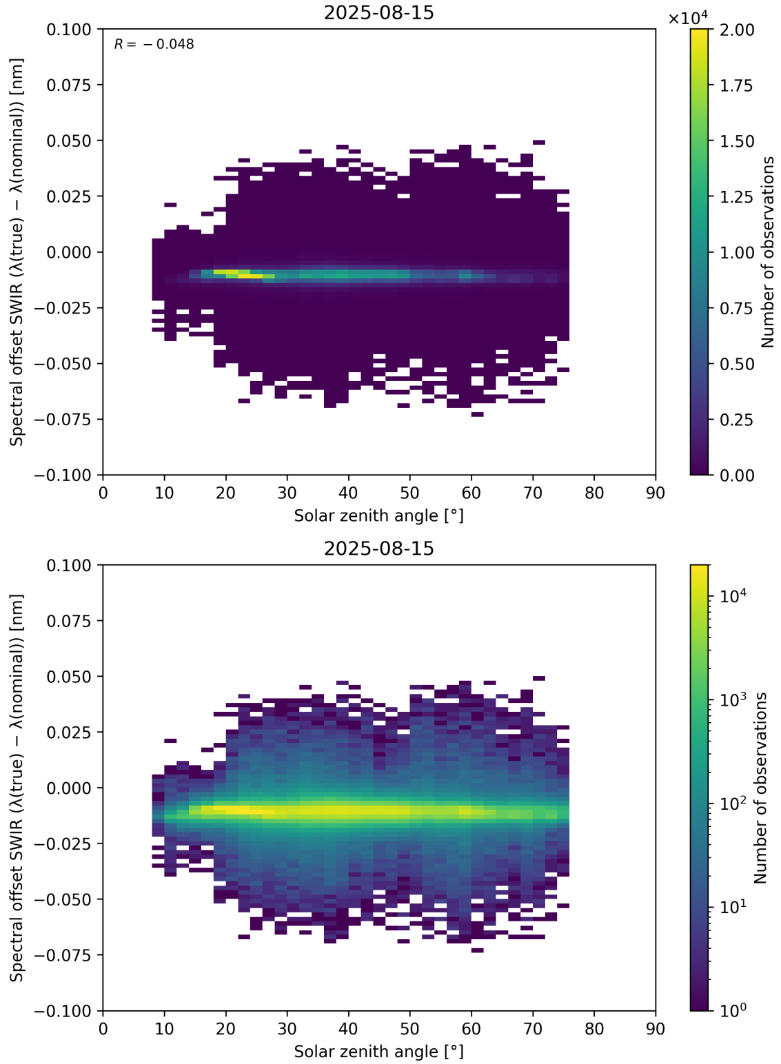
Figure 104: Scatter density plot of “Solar zenith angle” against “Spectral offset SWIR ( \lambda_{\text{true}} - \lambda_{\text{nominal}} )” for 2025-08-14 to 2025-08-16.
