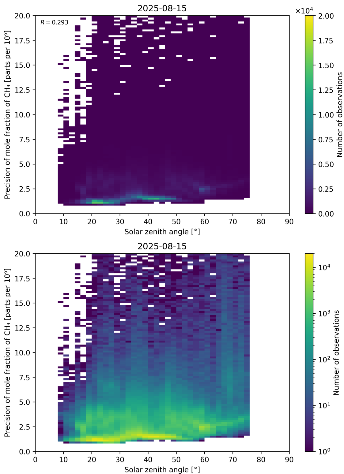
Figure 101: Scatter density plot of “Solar zenith angle” against “Precision of mole fraction of CH 4 ” for 2025-08-14 to 2025-08-16.
