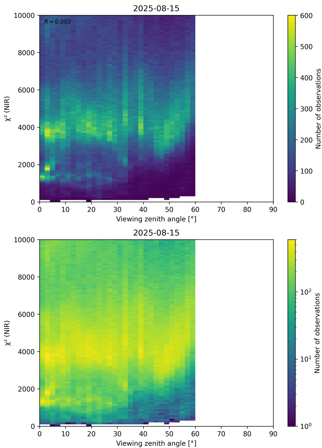
Figure 105: Scatter density plot of “Viewing zenith angle” against “ \chi^2 (NIR)” for 2025-08-14 to 2025-08-16.
