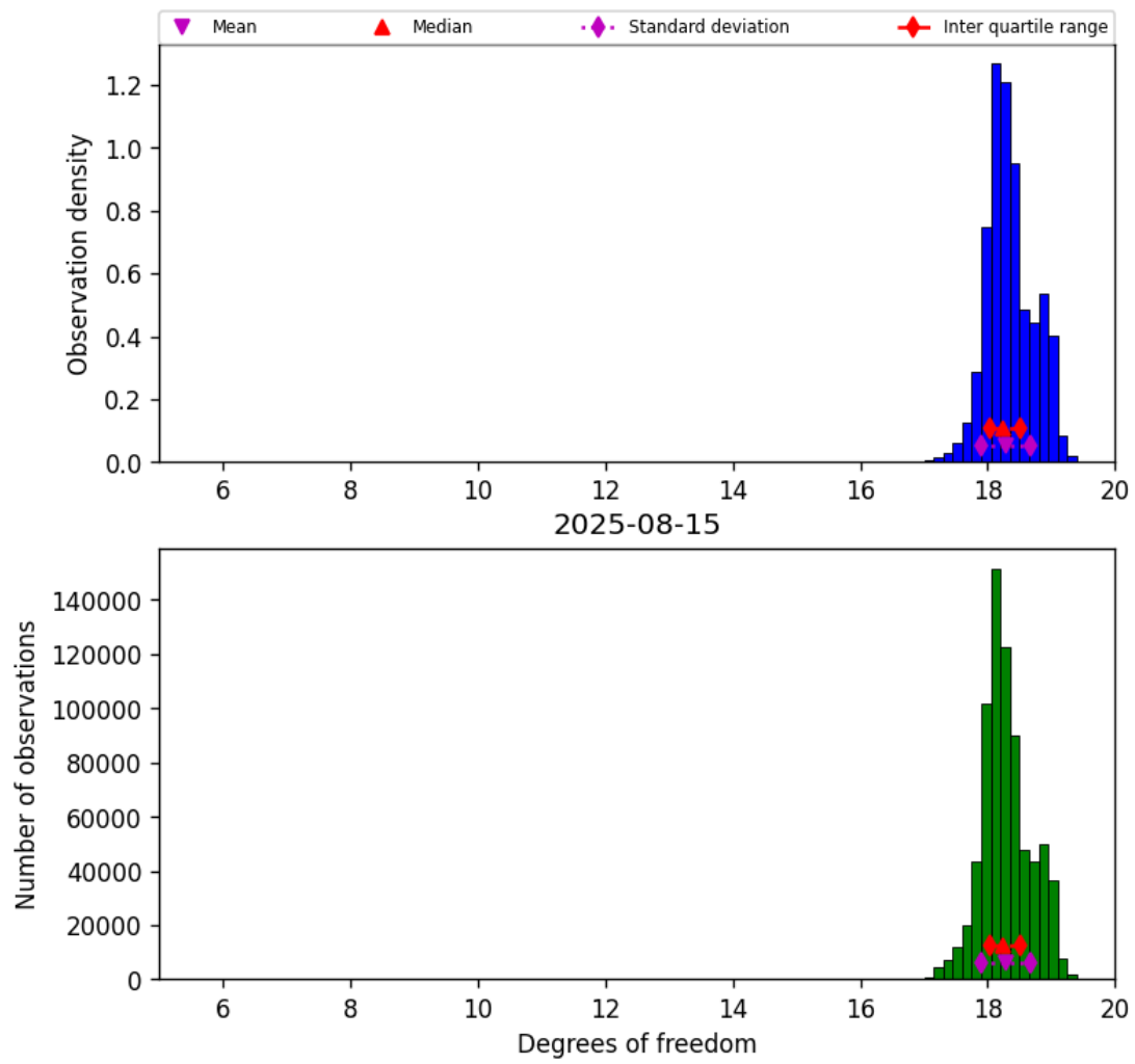
Figure 30: Histogram of “Degrees of freedom” for 2025-08-14 to 2025-08-16
