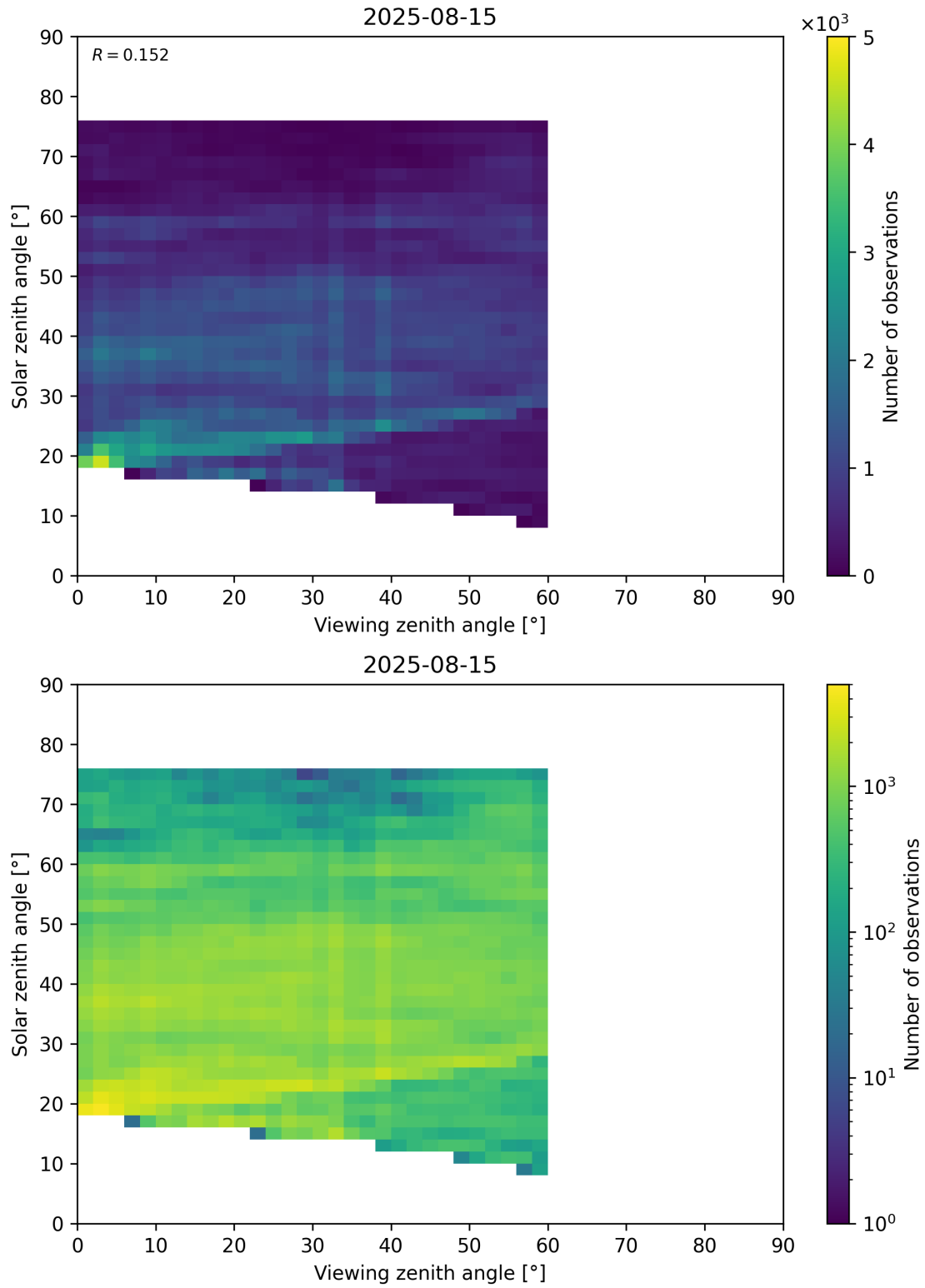
Figure 115: Scatter density plot of “Viewing zenith angle” against “Solar zenith angle” for 2025-08-14 to 2025-08-16.
