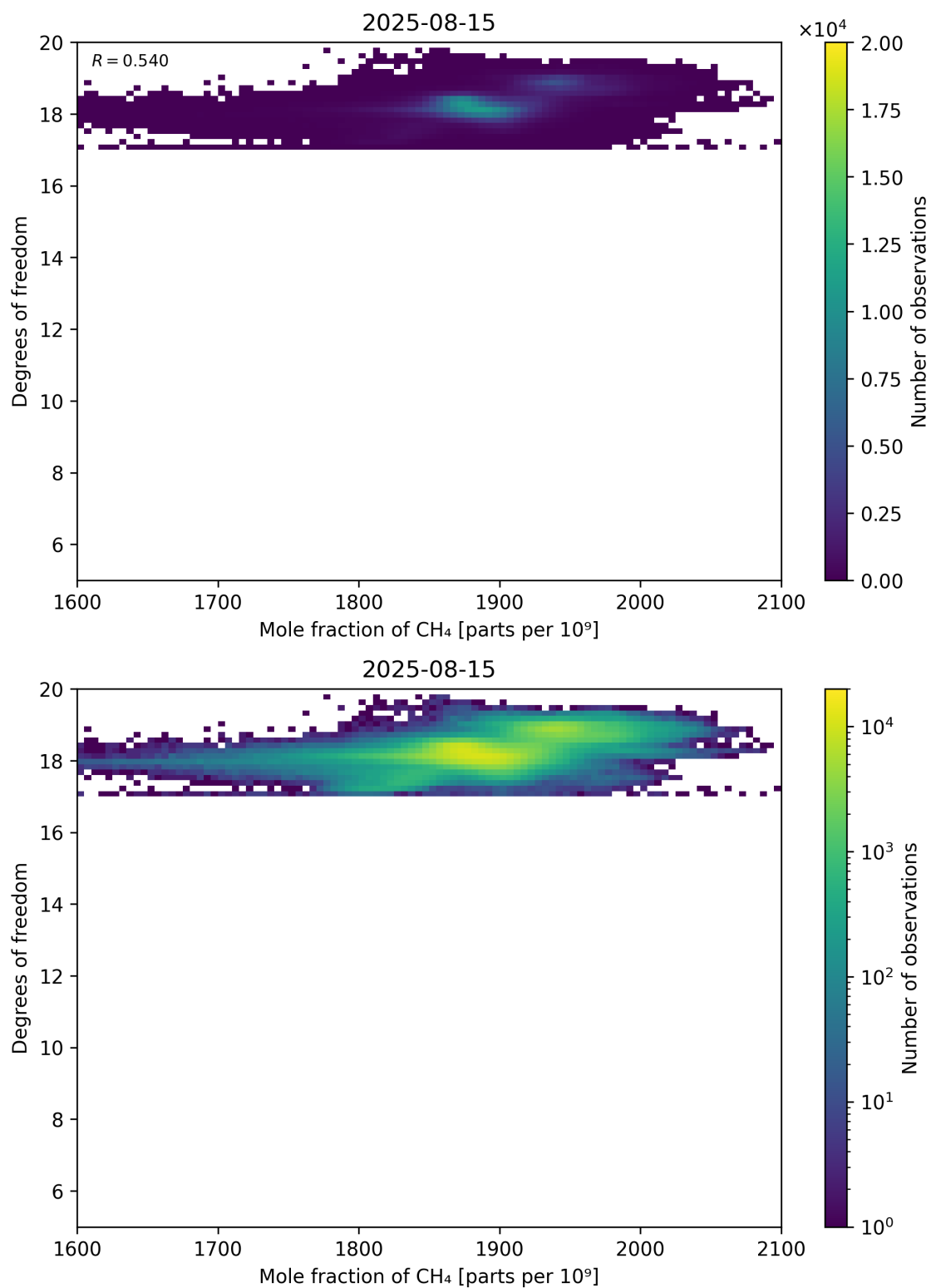
Figure 72: Scatter density plot of “Mole fraction of CH 4 ” against “Degrees of freedom” for 2025-08-14 to 2025-08-16.
