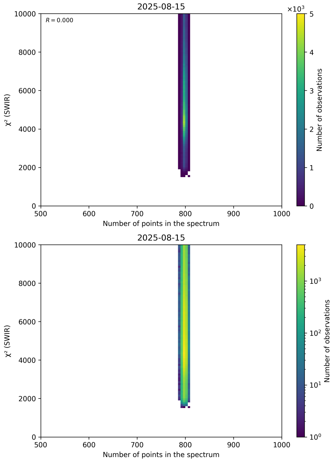
Figure 89: Scatter density plot of “Number of points in the spectrum” against “ \chi^2 (SWIR)” for 2025-08-14 to 2025-08-16.
