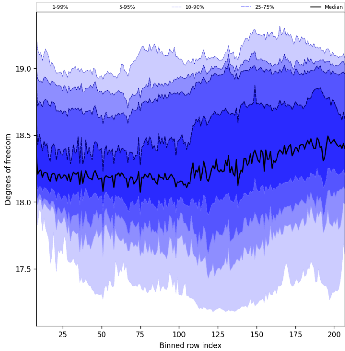
Figure 41: Along track statistics of “Degrees of freedom” for 2025-08-14 to 2025-08-16
