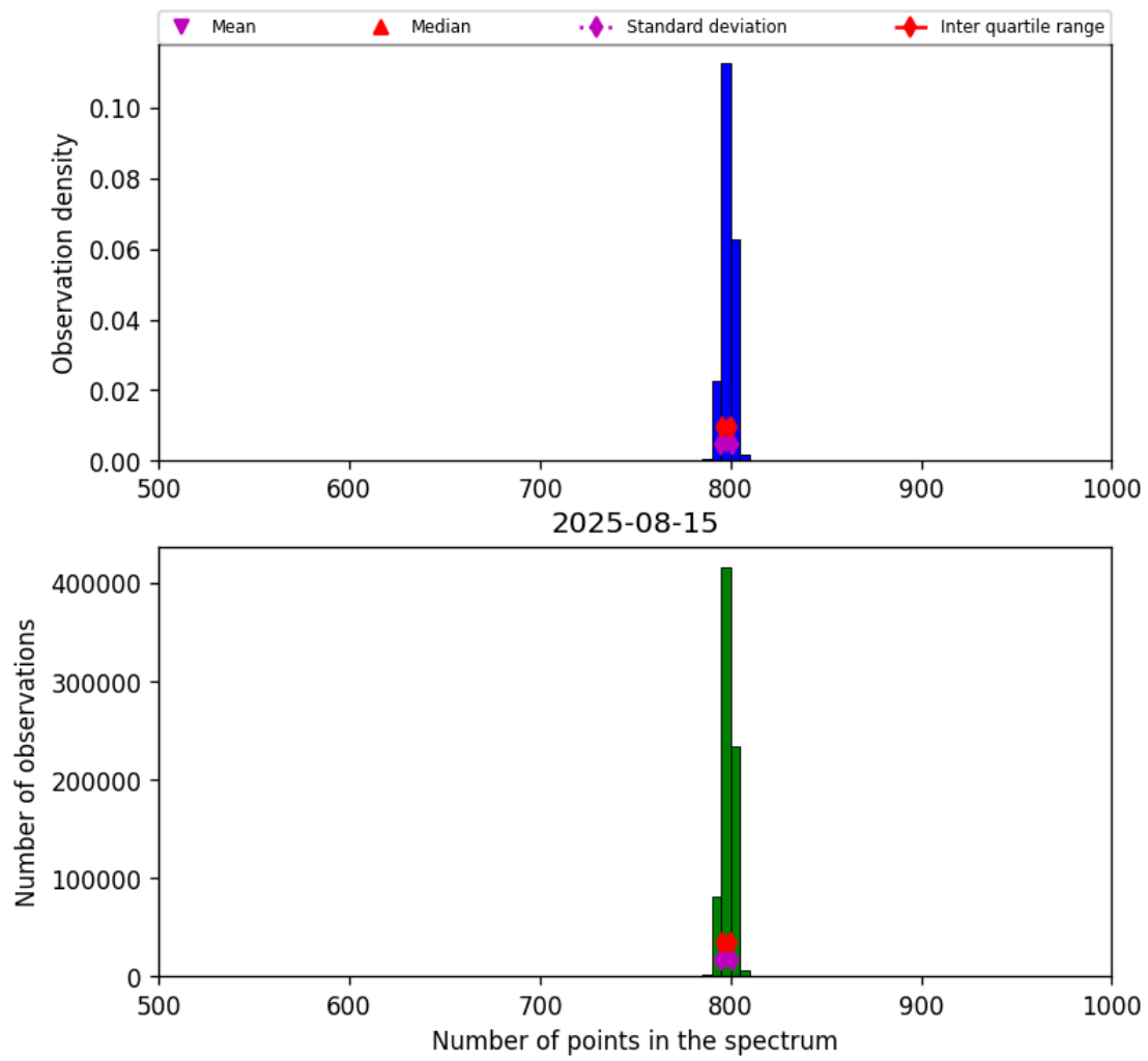
Figure 26: Histogram of “Number of points in the spectrum” for 2025-08-14 to 2025-08-16
