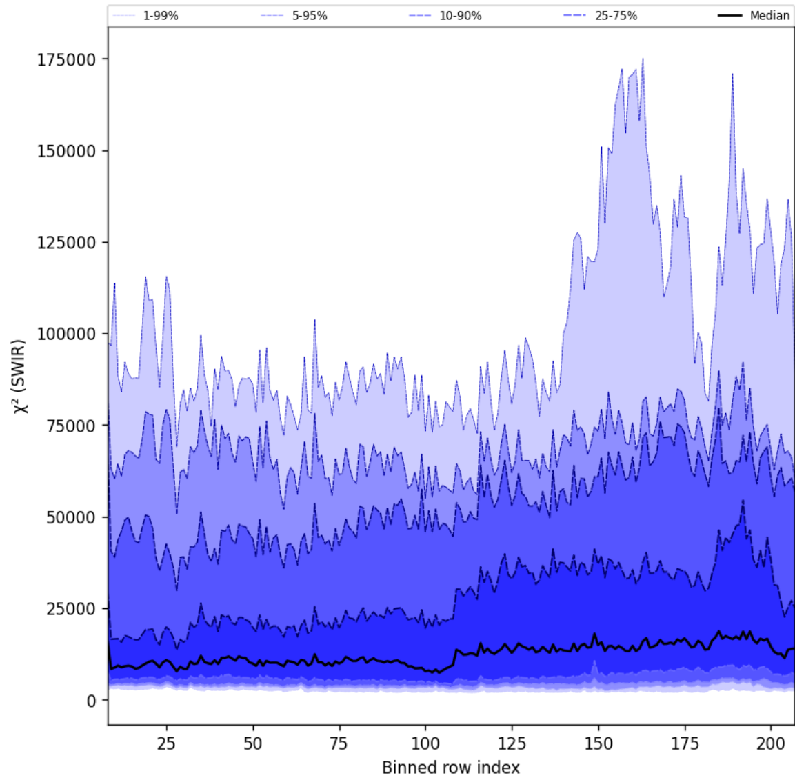
Figure 39: Along track statistics of “ \chi^2 (SWIR)” for 2025-08-14 to 2025-08-16
