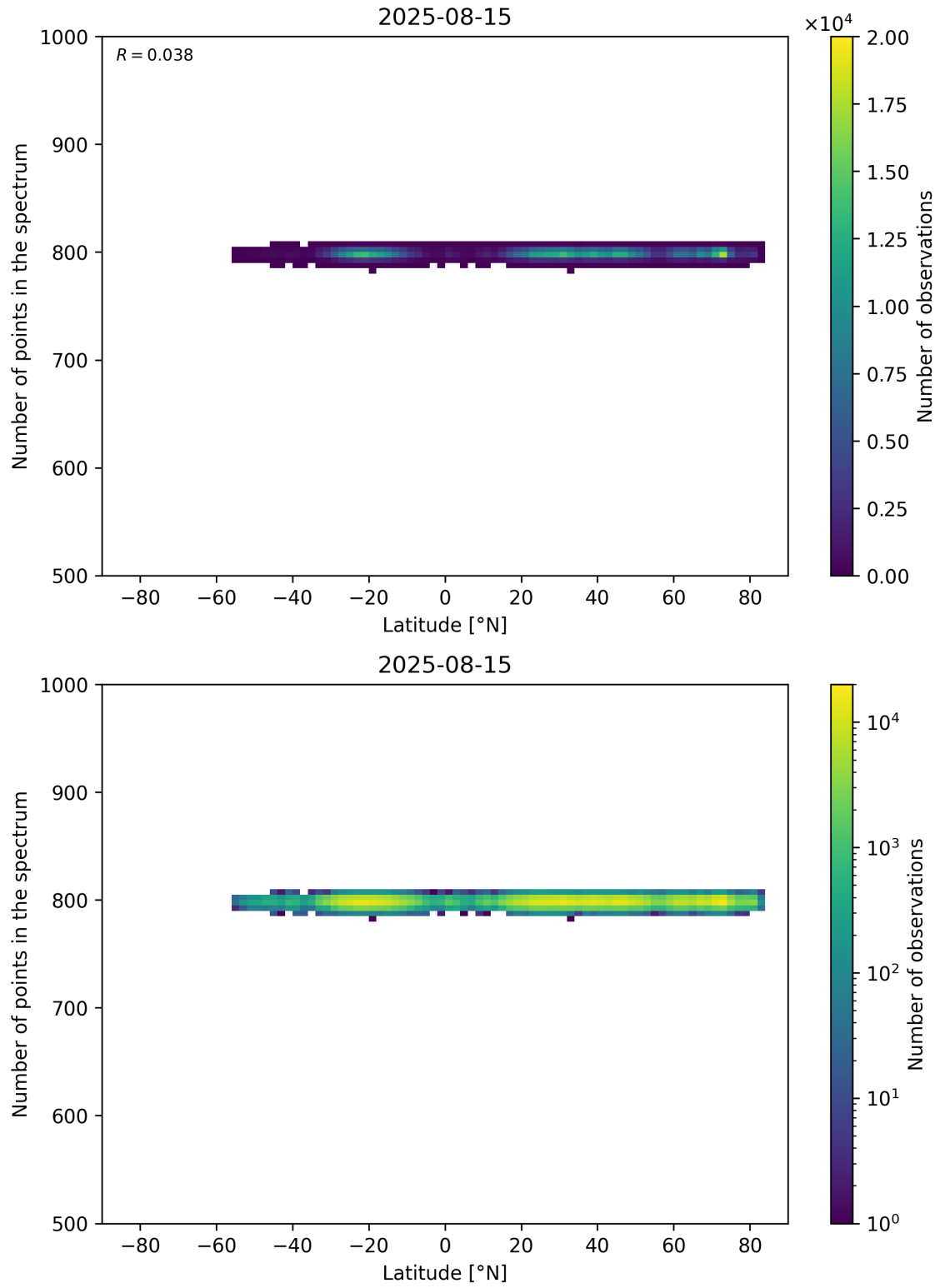
Figure 61: Scatter density plot of “Latitude” against “Number of points in the spectrum” for 2025-08-14 to 2025-08-16.
