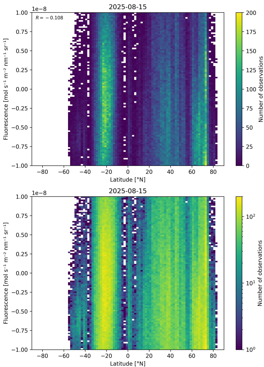
Figure 56: Scatter density plot of “Latitude” against “Fluorescence” for 2025-08-14 to 2025-08-16.
