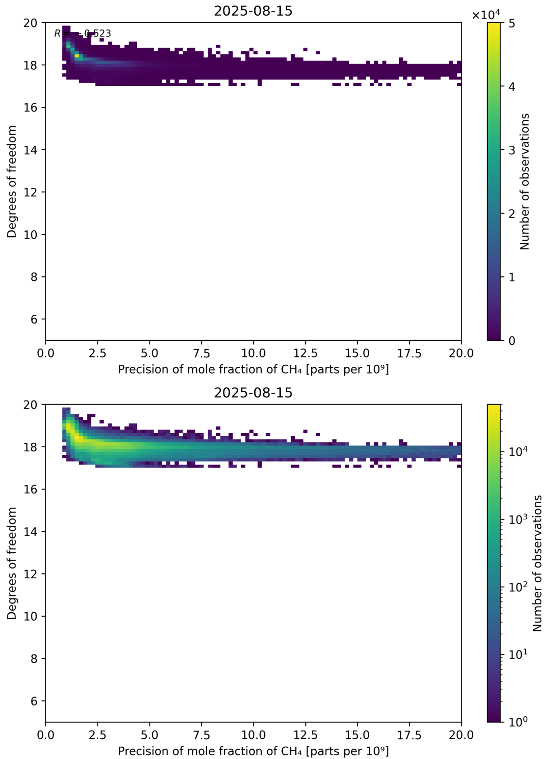
Figure 80: Scatter density plot of “Precision of mole fraction of CH 4 ” against “Degrees of freedom” for 2025-08-14 to 2025-08-16.
