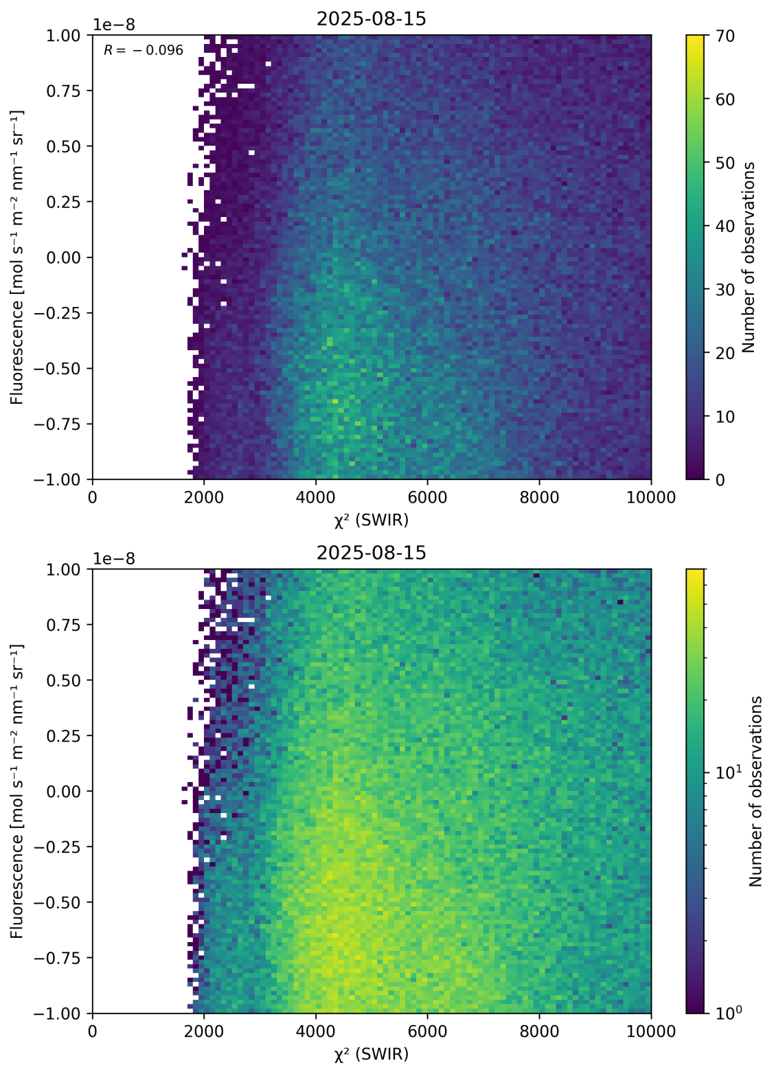
Figure 49: Scatter density plot of “ \chi^2 (SWIR)” against “Fluorescence” for 2025-08-14 to 2025-08-16.
