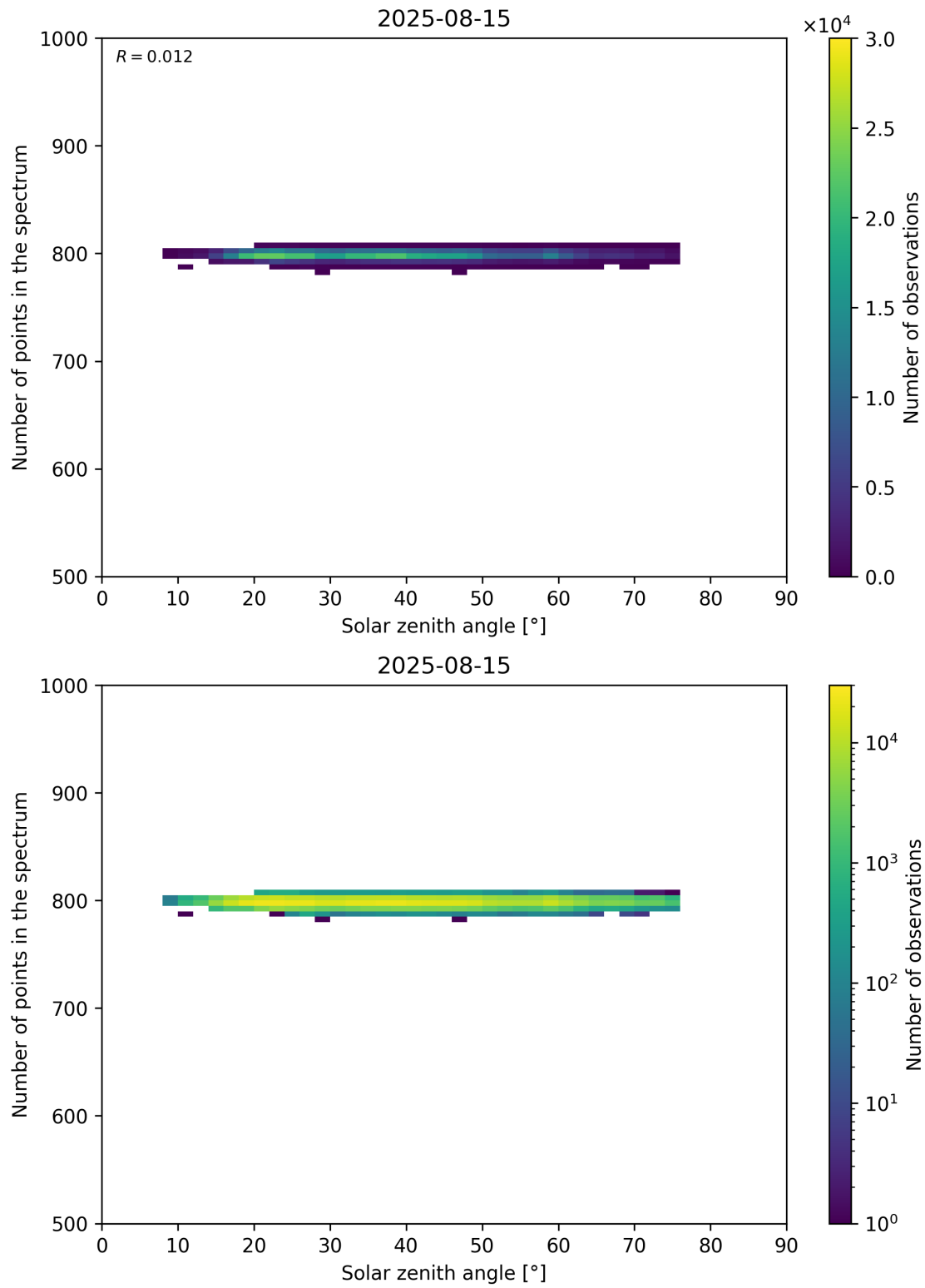
Figure 103: Scatter density plot of “Solar zenith angle” against “Number of points in the spectrum” for 2025-08-14 to 2025-08-16.
