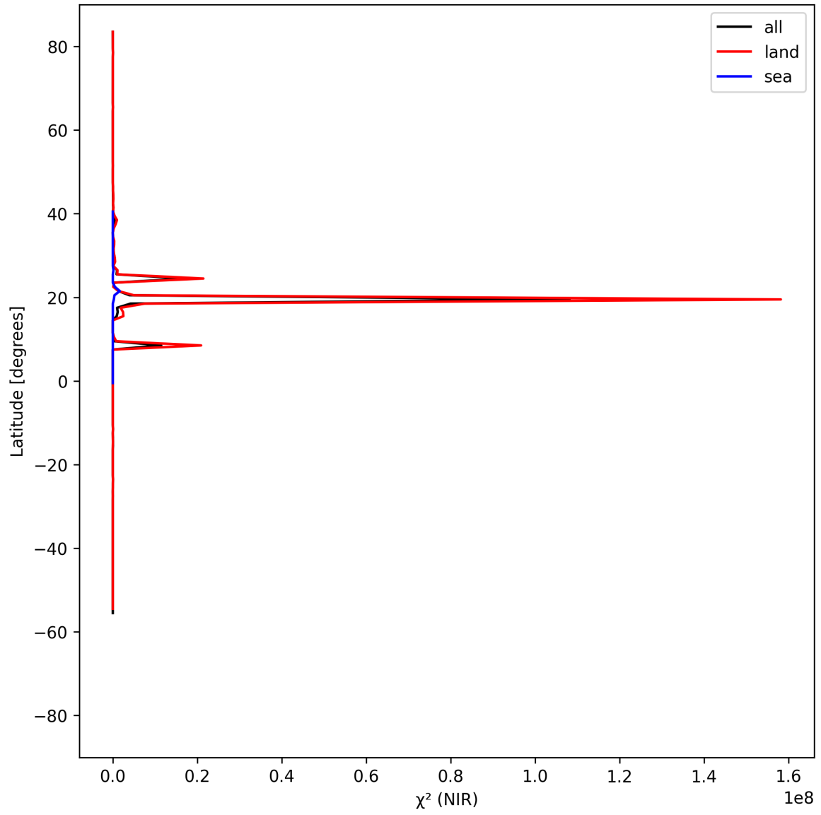
Figure 18: Zonal average of “ \chi^2 (NIR)” for 2025-08-14 to 2025-08-16.
