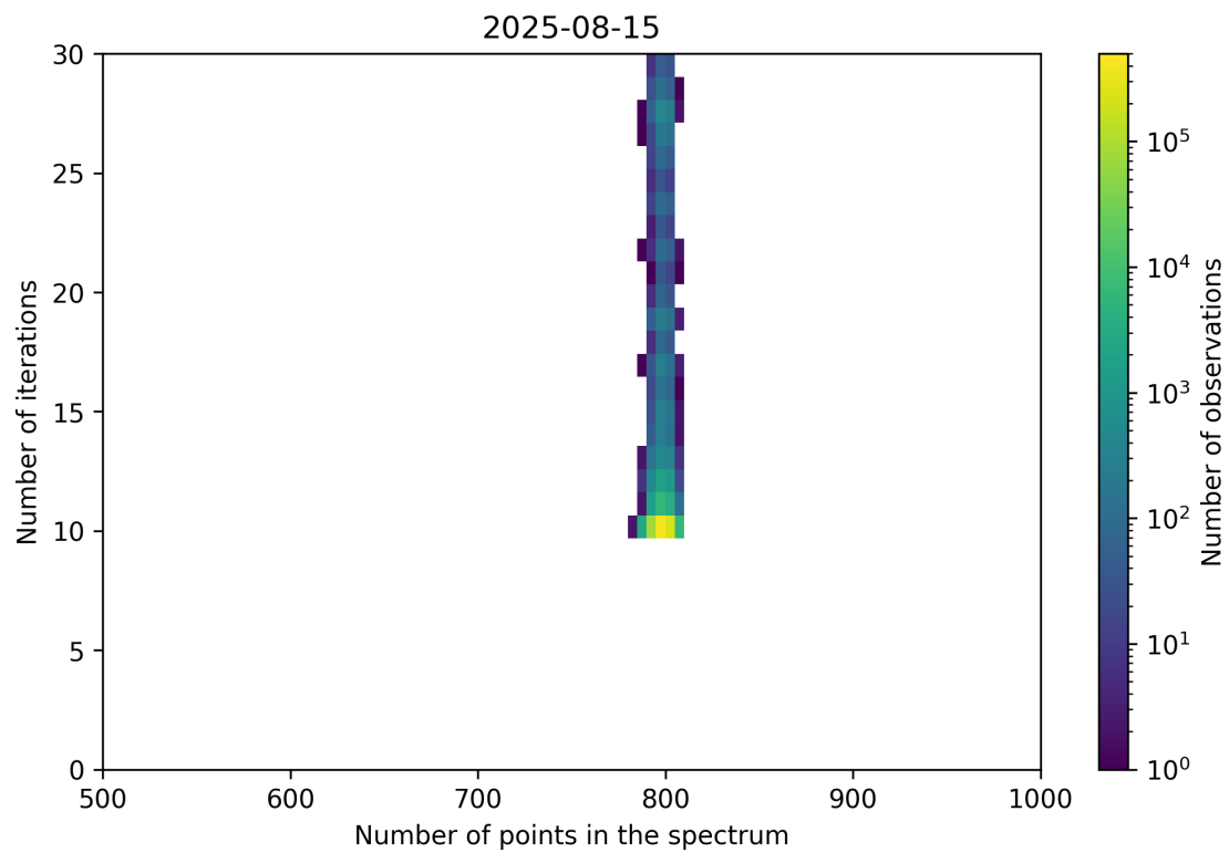
Figure 92: Scatter density plot of “Number of points in the spectrum” against “Number of iterations” for 2025-08-14 to 2025-08-16.
