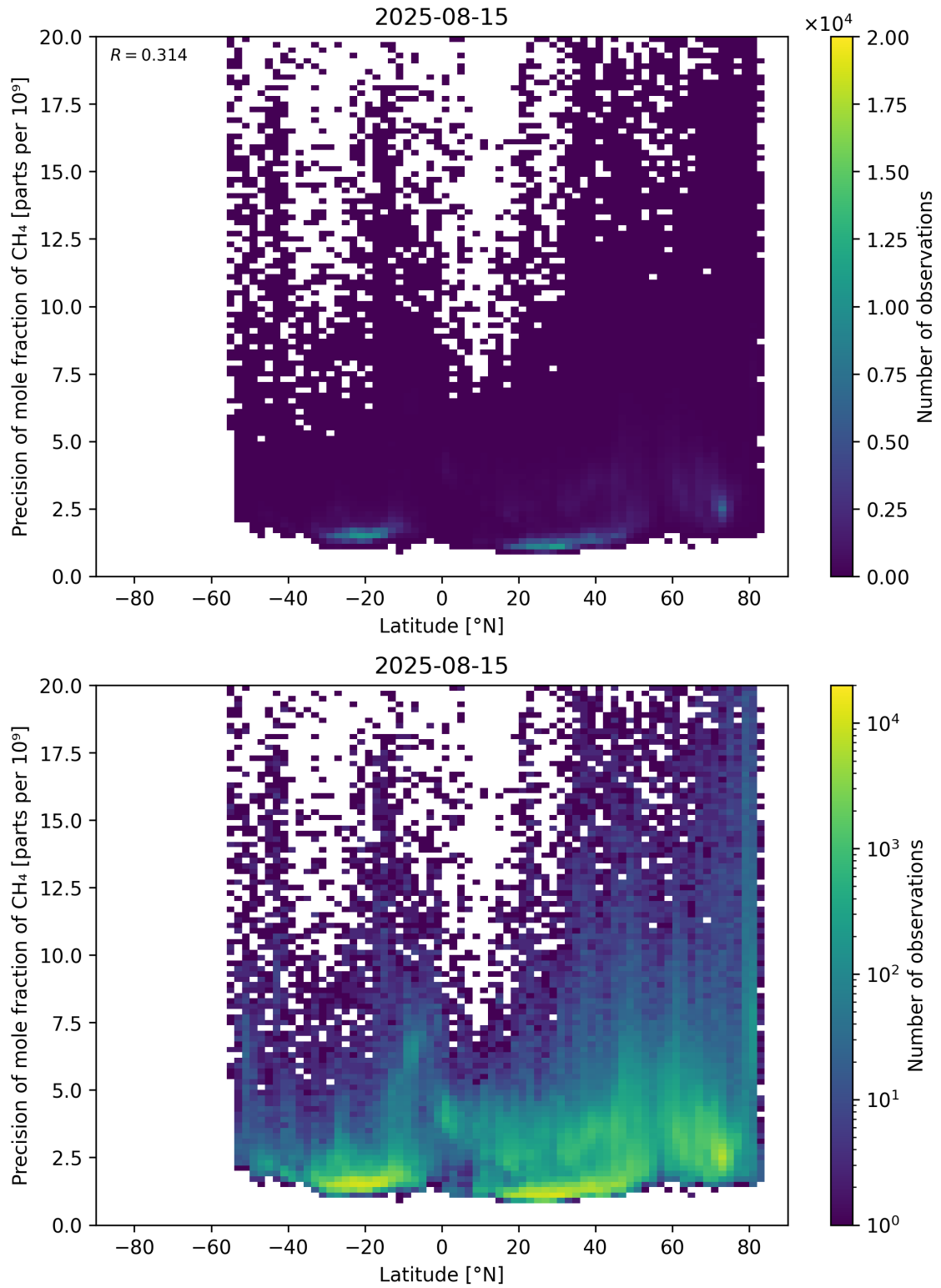
Figure 59: Scatter density plot of “Latitude” against “Precision of mole fraction of \text{CH}_4 ” for 2025-08-14 to 2025-08-16.
