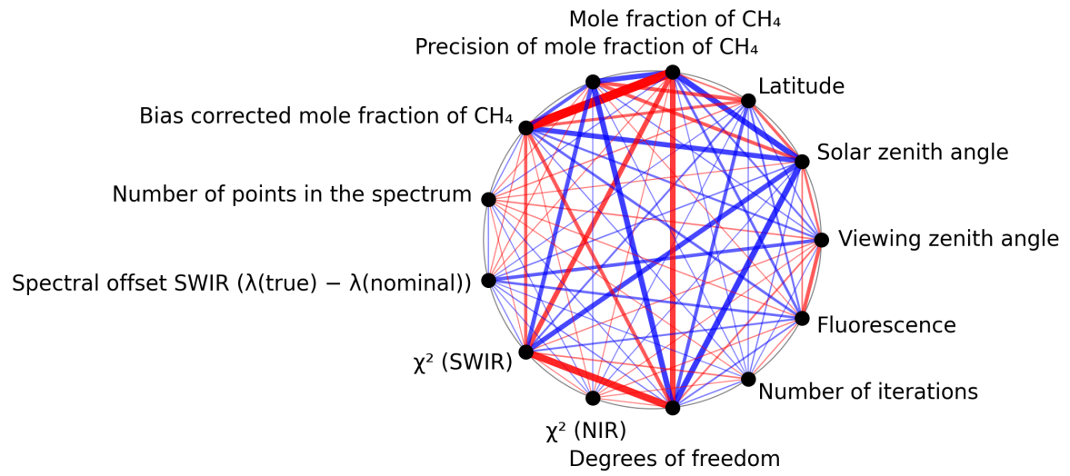
Figure 1: Map of correlation graph for 2025-08-14 to 2025-08-16.
