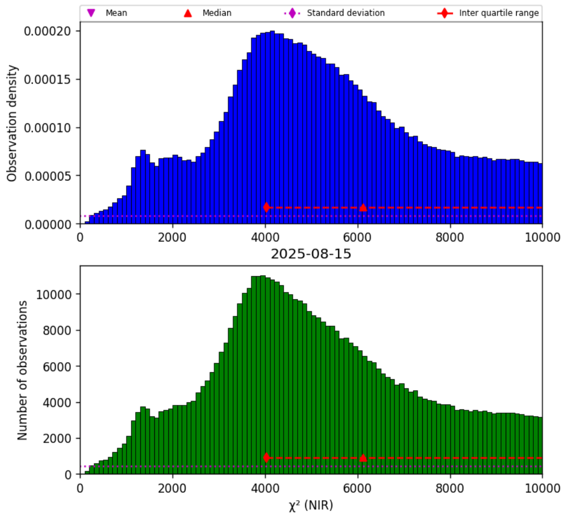
Figure 29: Histogram of " \chi^2 (NIR)" for 2025-08-14 to 2025-08-16
