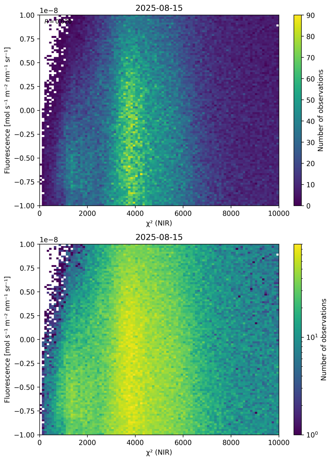
Figure 45: Scatter density plot of “ \chi^2 (NIR)” against “Fluorescence” for 2025-08-14 to 2025-08-16.
