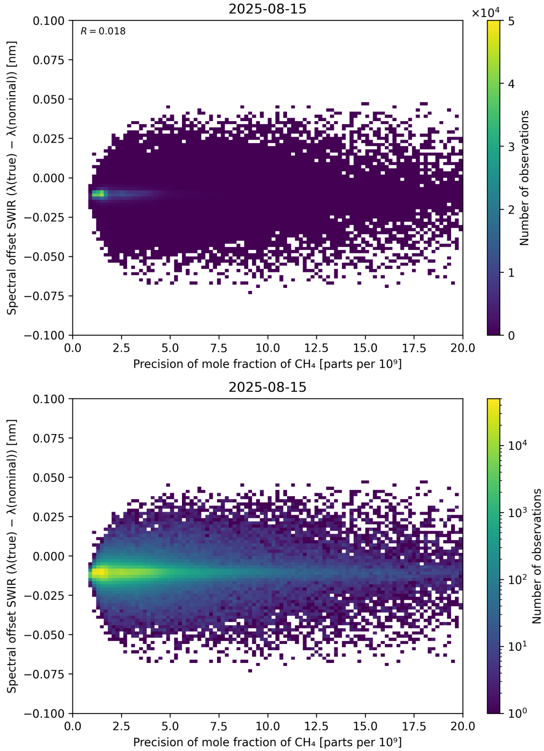
Figure 85: Scatter density plot of “Precision of mole fraction of \text{CH}_4 ” against “Spectral offset SWIR ( \lambda_{\text{true}} - \lambda_{\text{nominal}} )” for 2025-08-14 to 2025-08-16.
