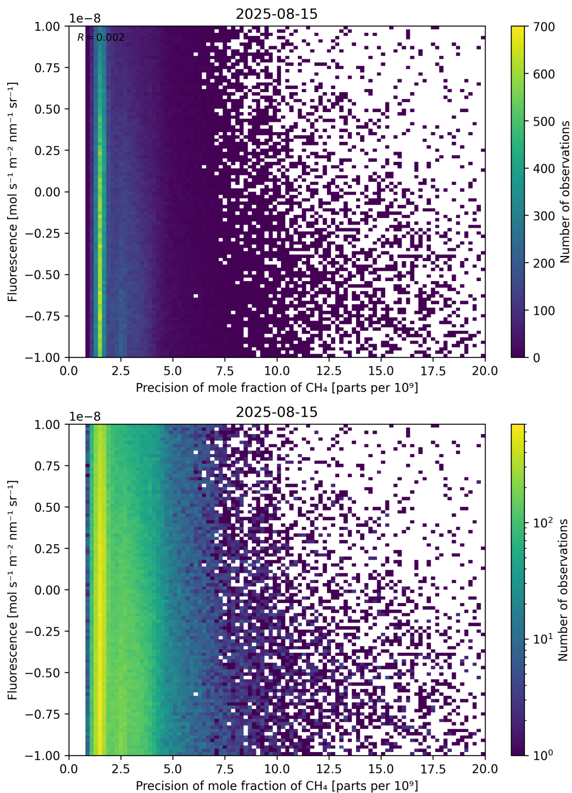
Figure 81: Scatter density plot of “Precision of mole fraction of \text{CH}_4 ” against “Fluorescence” for 2025-08-14 to 2025-08-16.
