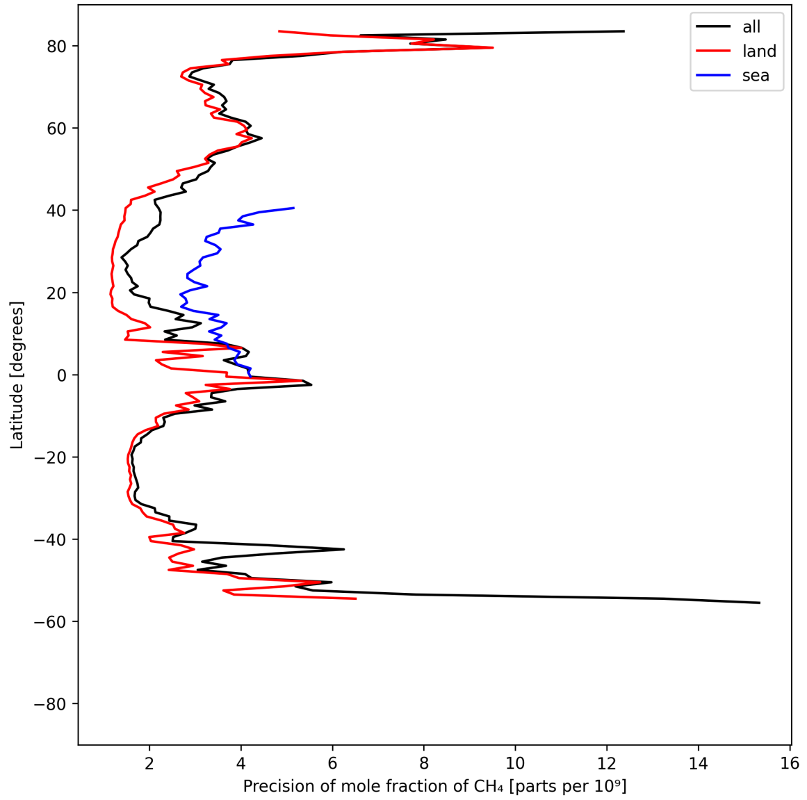
Figure 13: Zonal average of “Precision of mole fraction of CH 4 ” for 2025-08-14 to 2025-08-16.
