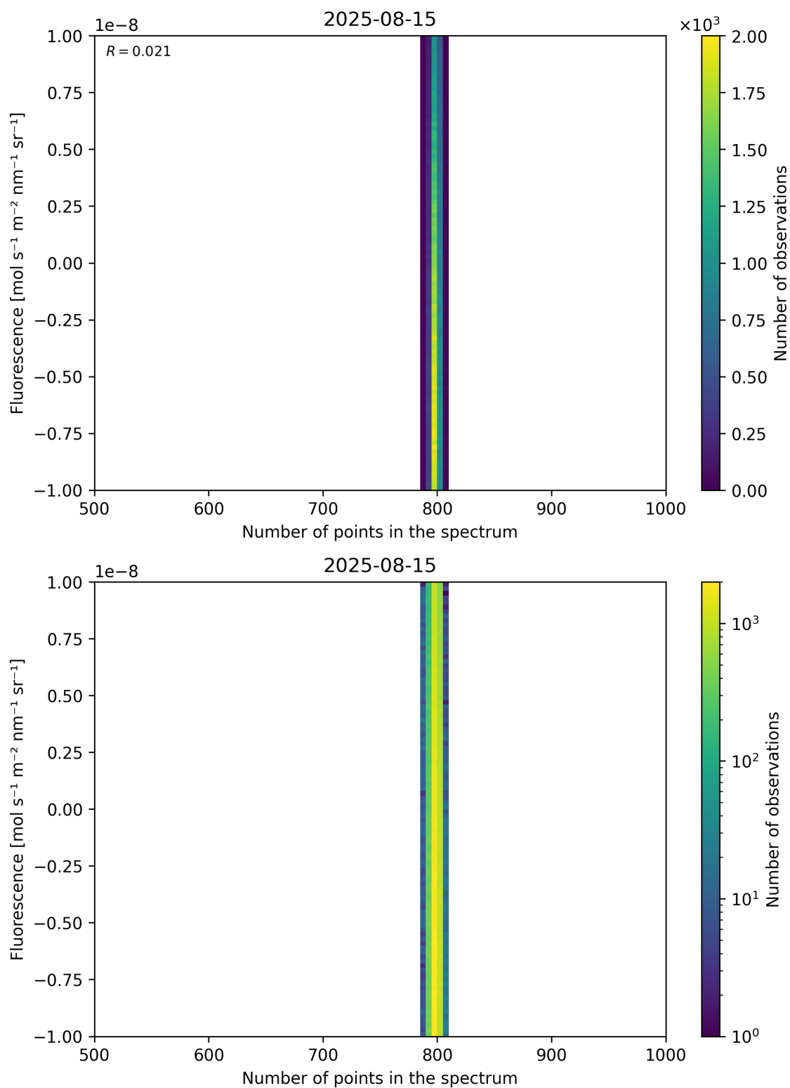
Figure 91: Scatter density plot of “Number of points in the spectrum” against “Fluorescence” for 2025-08-14 to 2025-08-16.
