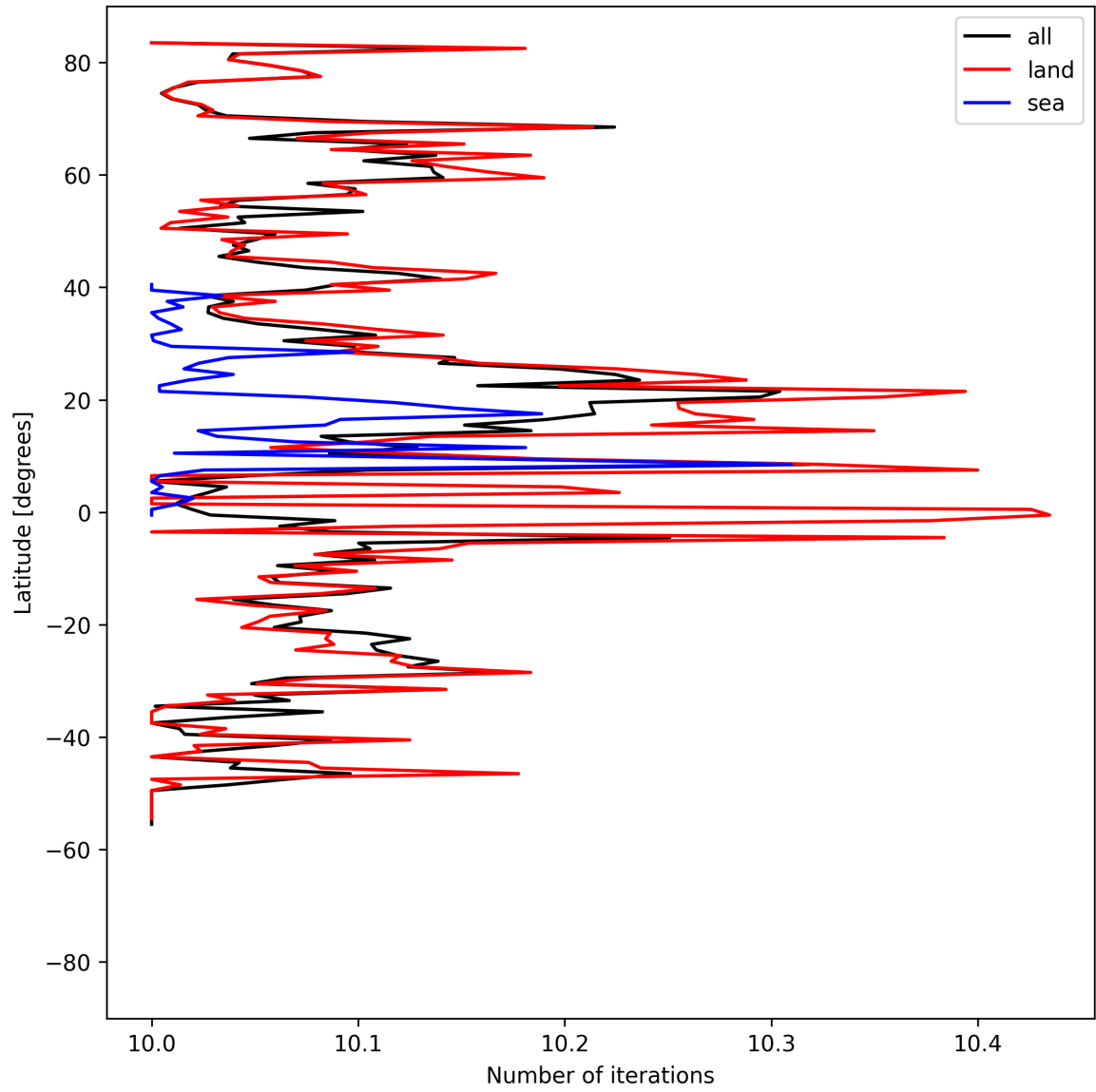
Figure 20: Zonal average of “Number of iterations” for 2025-08-14 to 2025-08-16.
