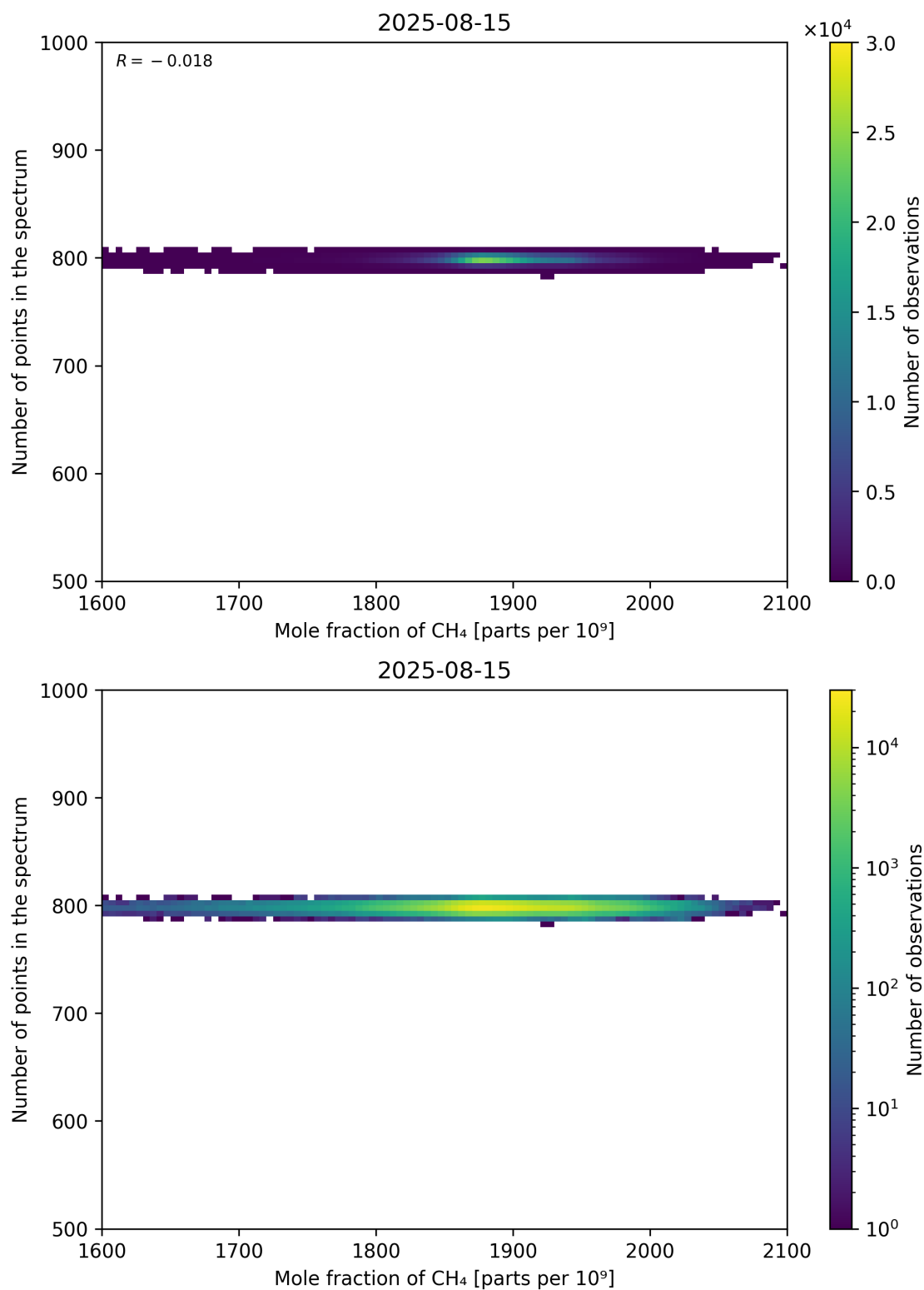
Figure 77: Scatter density plot of “Mole fraction of CH 4 ” against “Number of points in the spectrum” for 2025-08-14 to 2025-08-16.
