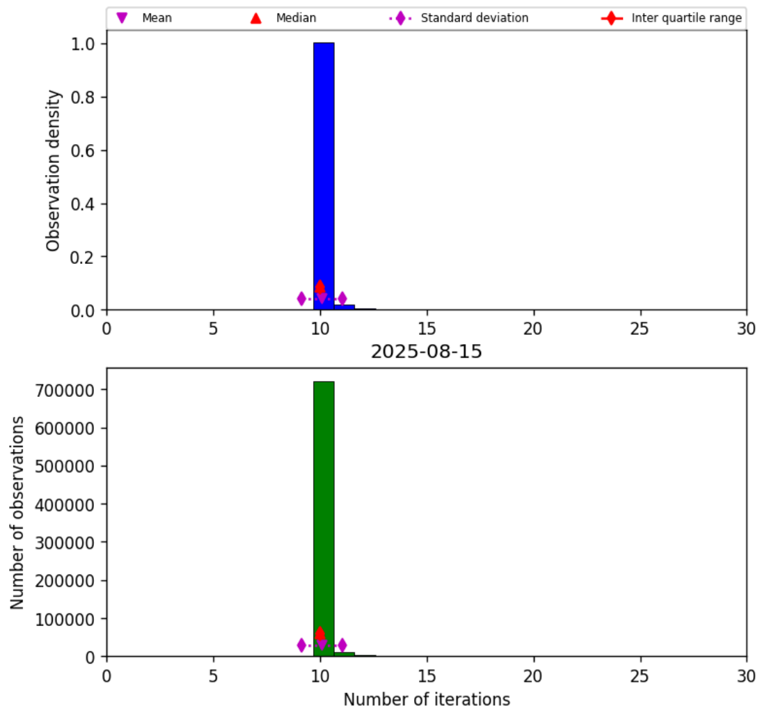
Figure 31: Histogram of “Number of iterations” for 2025-08-14 to 2025-08-16
