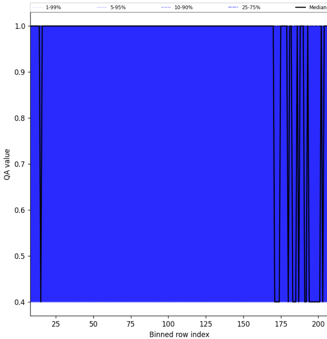
Figure 33: Along track statistics of “QA value” for 2025-08-14 to 2025-08-16
