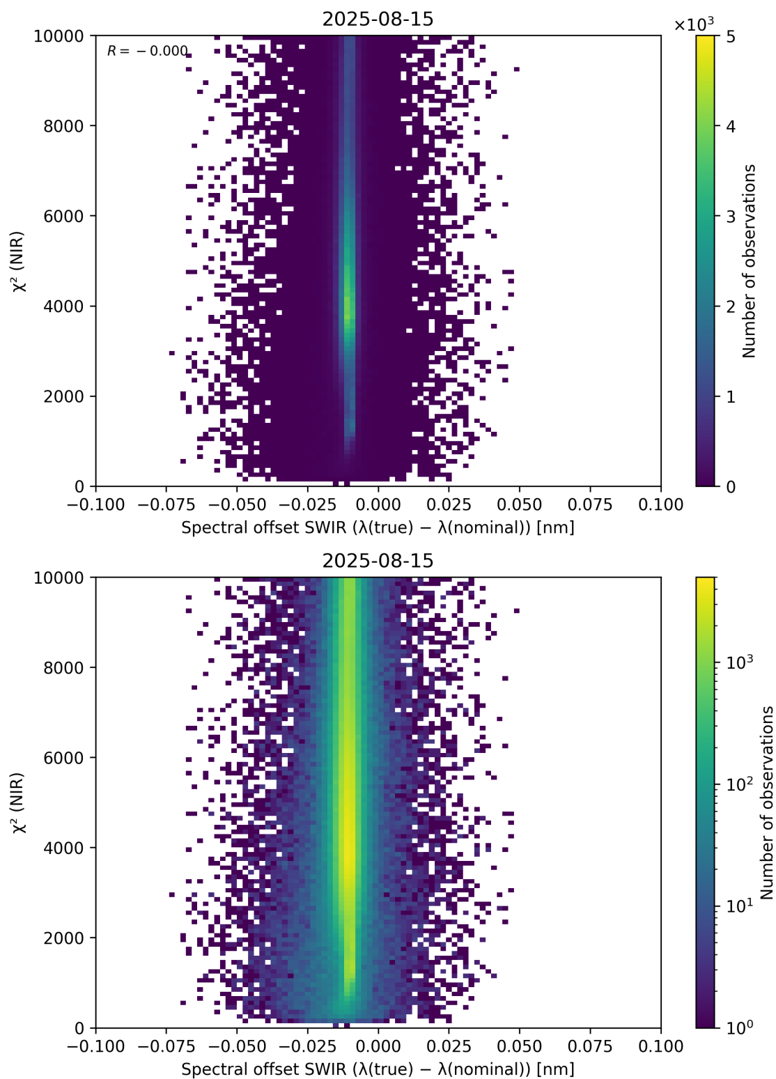
Figure 117: Scatter density plot of “Spectral offset SWIR ( \lambda_{\text{true}} - \lambda_{\text{nominal}} )” against “ \chi^2 (NIR)” for 2025-08-14 to 2025-08-16.
