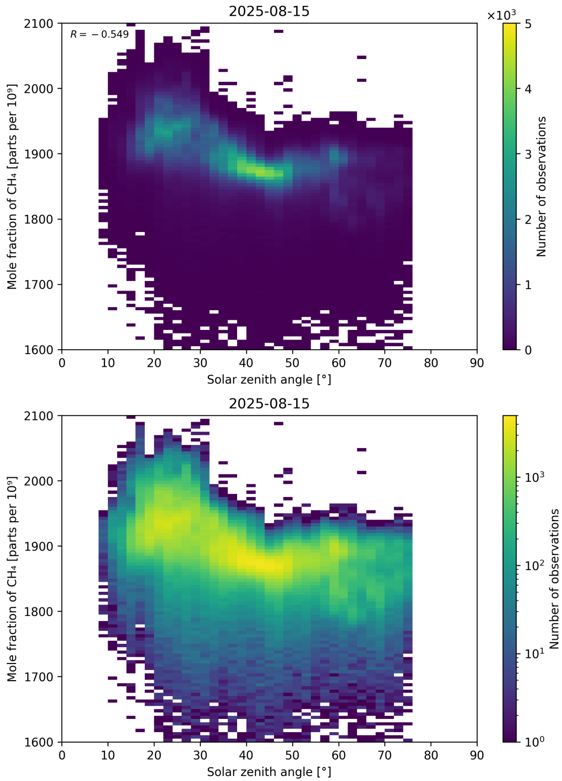
Figure 99: Scatter density plot of “Solar zenith angle” against “Mole fraction of \text{CH}_4 ” for 2025-08-14 to 2025-08-16.
