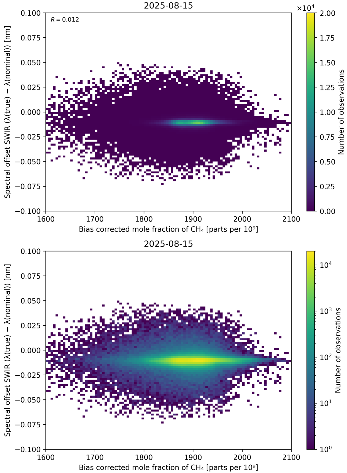
Figure 69: Scatter density plot of “Bias corrected mole fraction of \text{CH}_4 ” against “Spectral offset SWIR ( \lambda_{\text{true}} - \lambda_{\text{nominal}} )” for 2025-08-14 to 2025-08-16.
