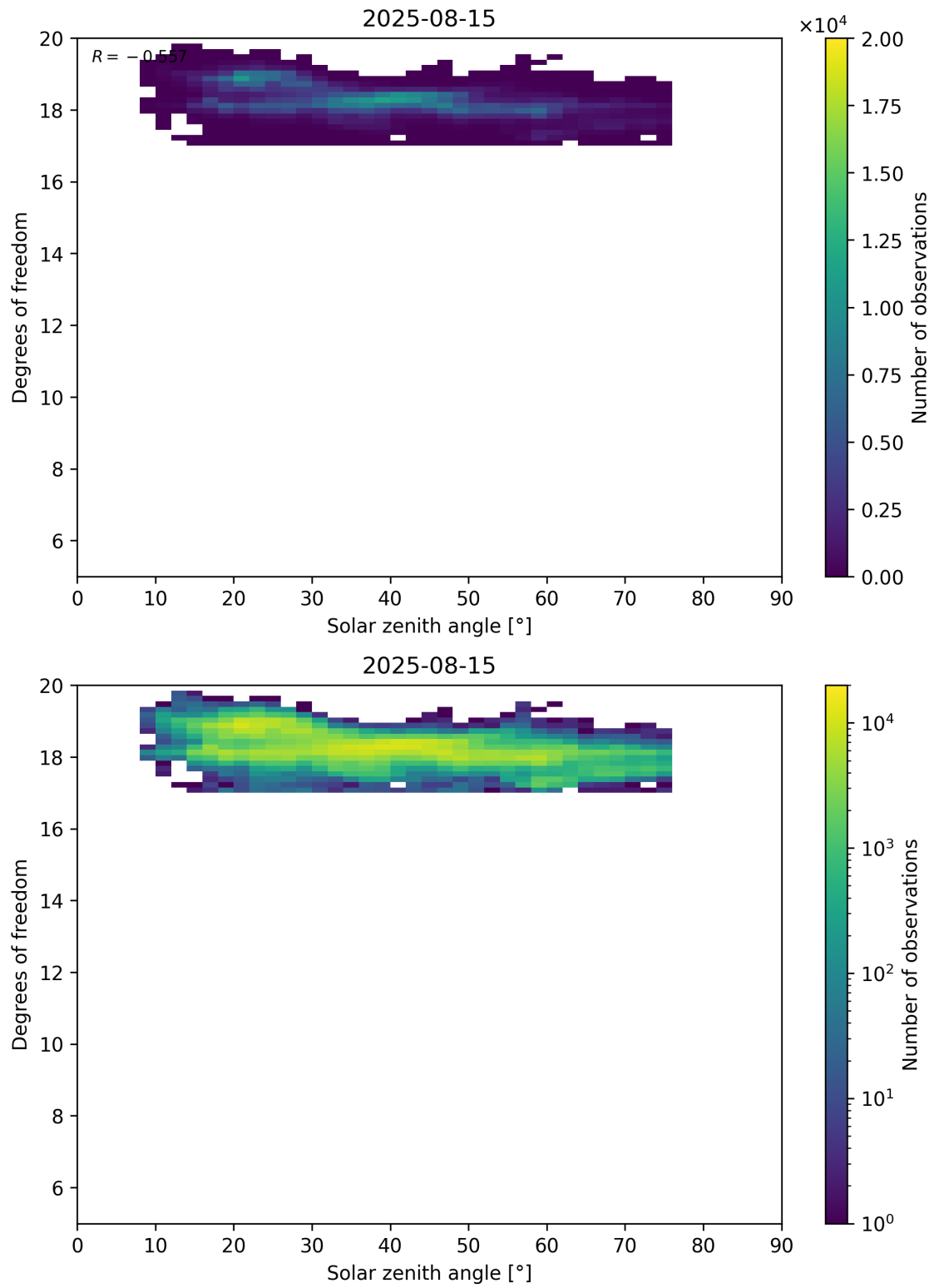
Figure 96: Scatter density plot of “Solar zenith angle” against “Degrees of freedom” for 2025-08-14 to 2025-08-16.
