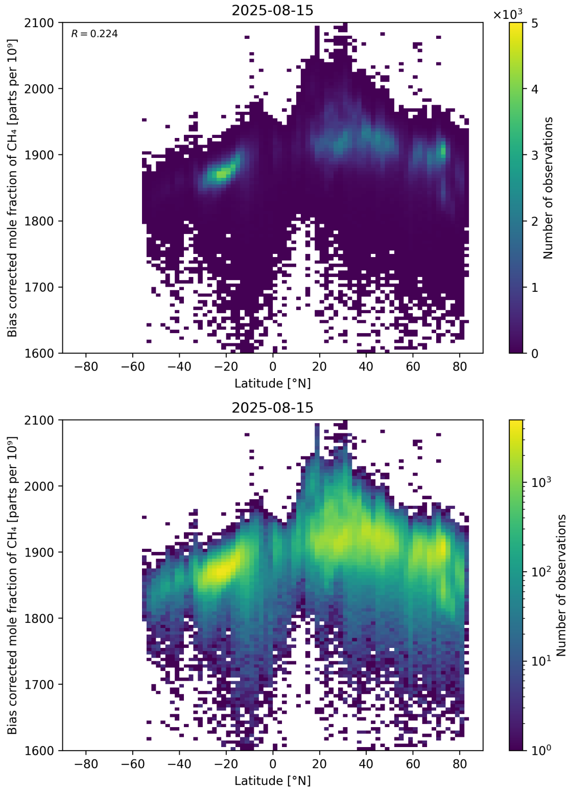
Figure 58: Scatter density plot of “Latitude” against “Bias corrected mole fraction of CH 4 ” for 2025-08-14 to 2025-08-16.
