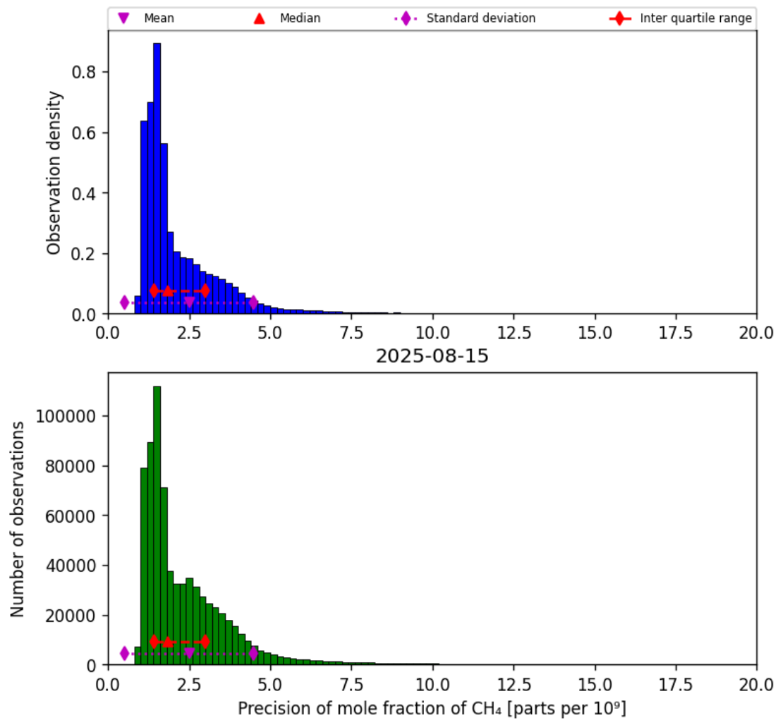
Figure 24: Histogram of “Precision of mole fraction of CH 4 ” for 2025-08-14 to 2025-08-16
