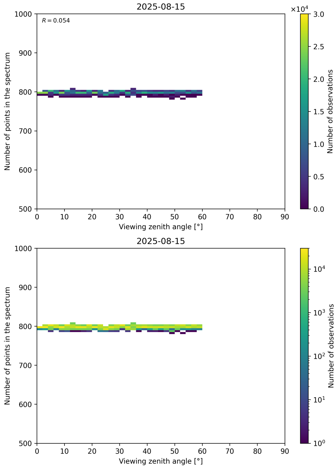
Figure 114: Scatter density plot of “Viewing zenith angle” against “Number of points in the spectrum” for 2025-08-14 to 2025-08-16.
