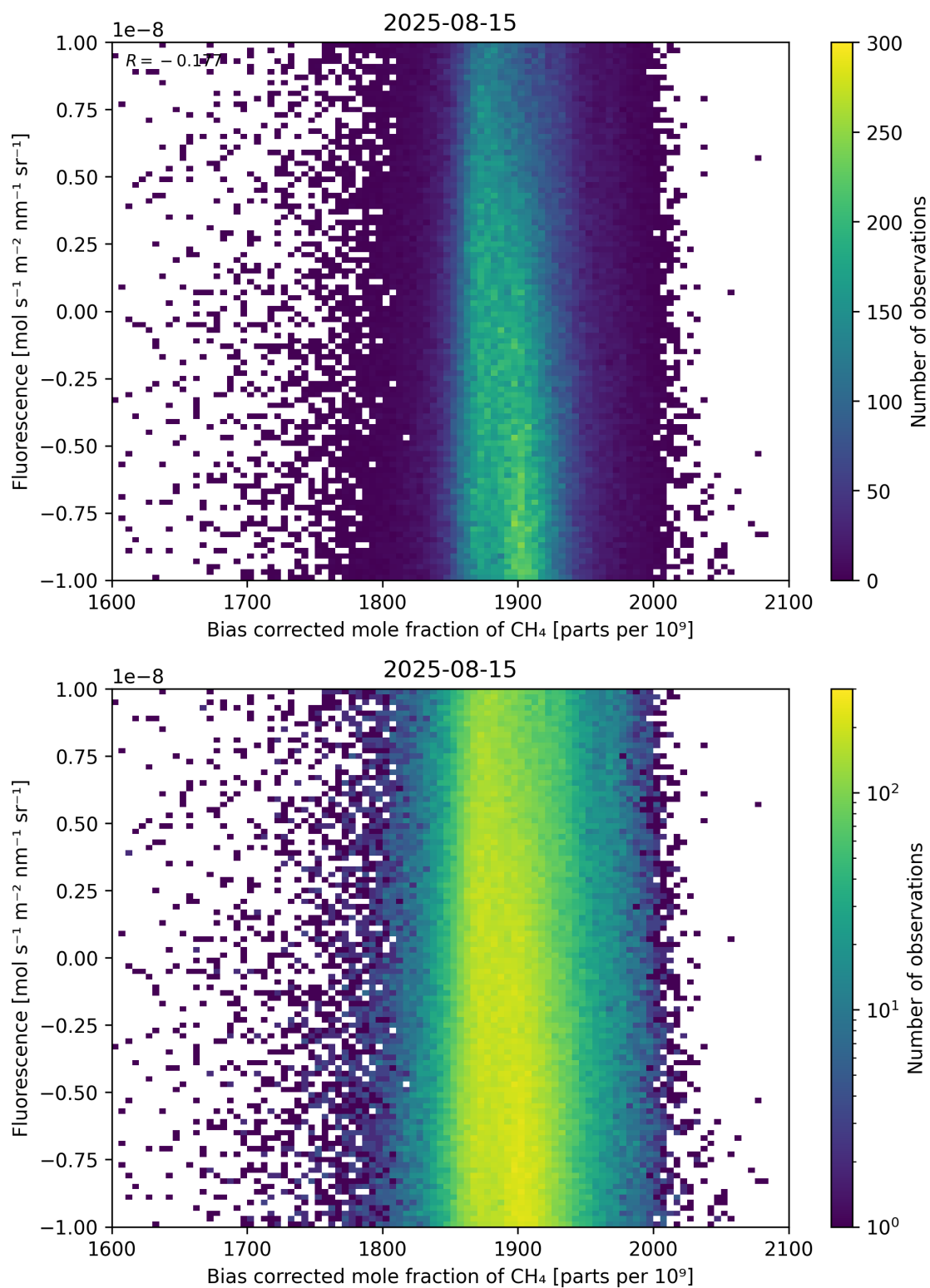
Figure 66: Scatter density plot of “Bias corrected mole fraction of \text{CH}_4 ” against “Fluorescence” for 2025-08-14 to 2025-08-16.
