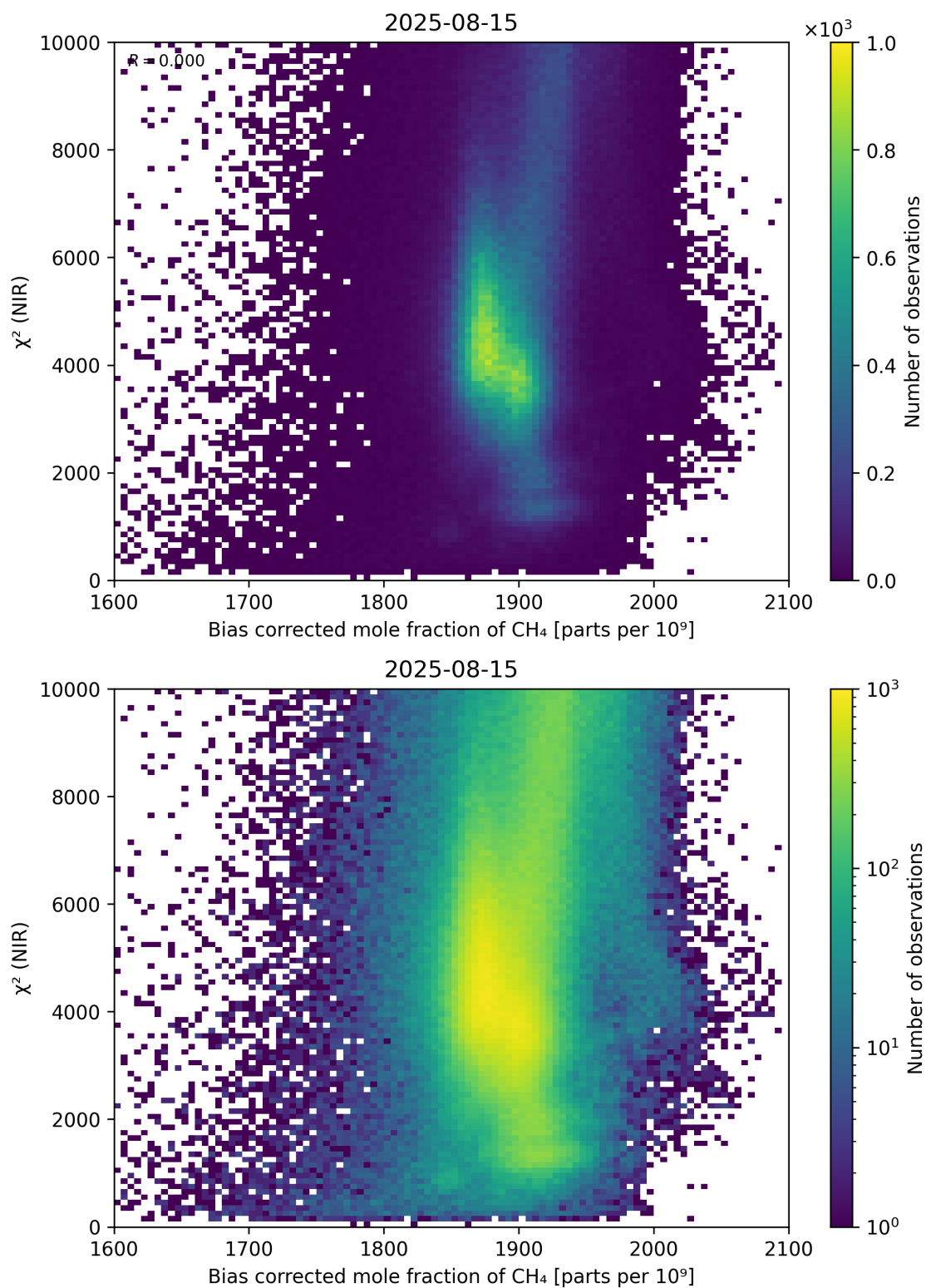
Figure 63: Scatter density plot of “Bias corrected mole fraction of \text{CH}_4 ” against “ \chi^2 (NIR)” for 2025-08-14 to 2025-08-16.
