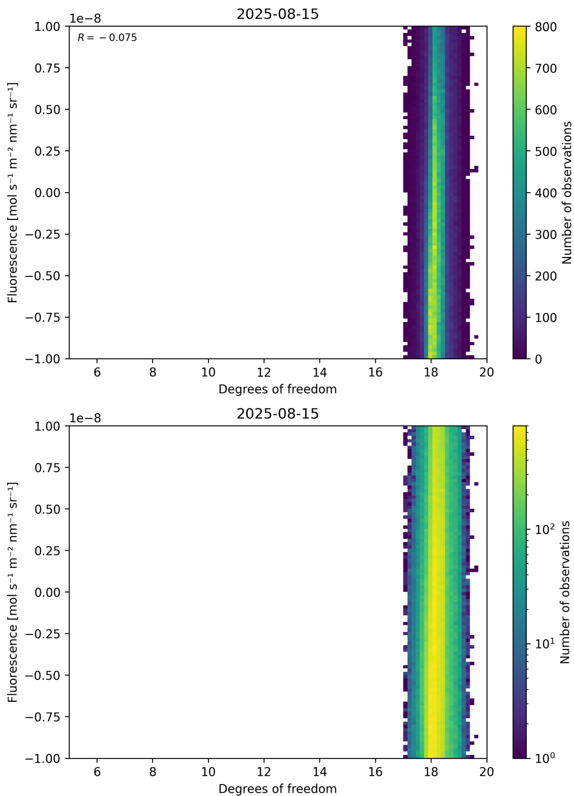
Figure 51: Scatter density plot of “Degrees of freedom” against “Fluorescence” for 2025-08-14 to 2025-08-16.
