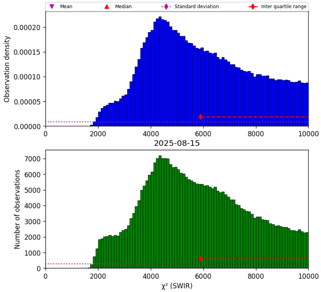
Figure 28: Histogram of " \chi^2 (SWIR)" for 2025-08-14 to 2025-08-16
