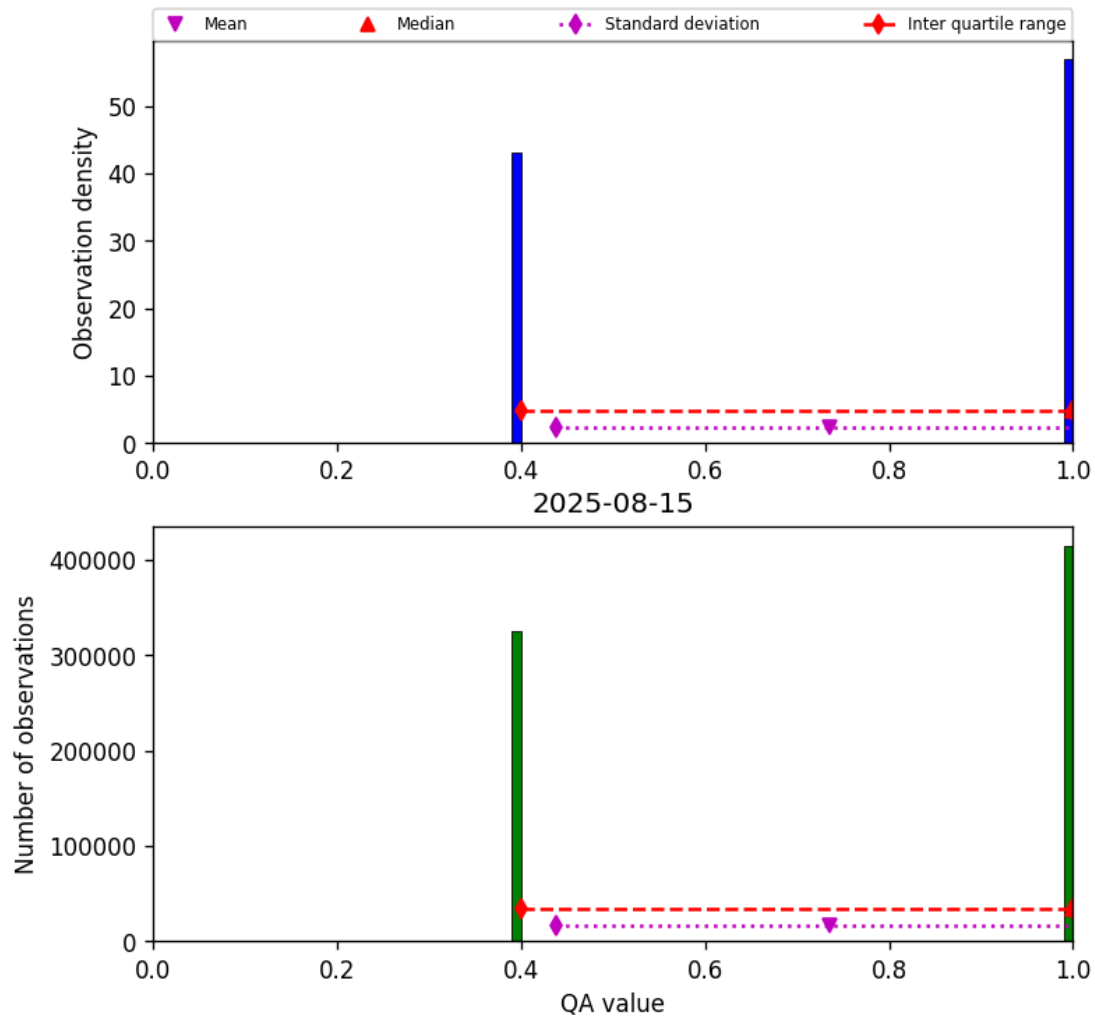
Figure 22: Histogram of “QA value” for 2025-08-14 to 2025-08-16
