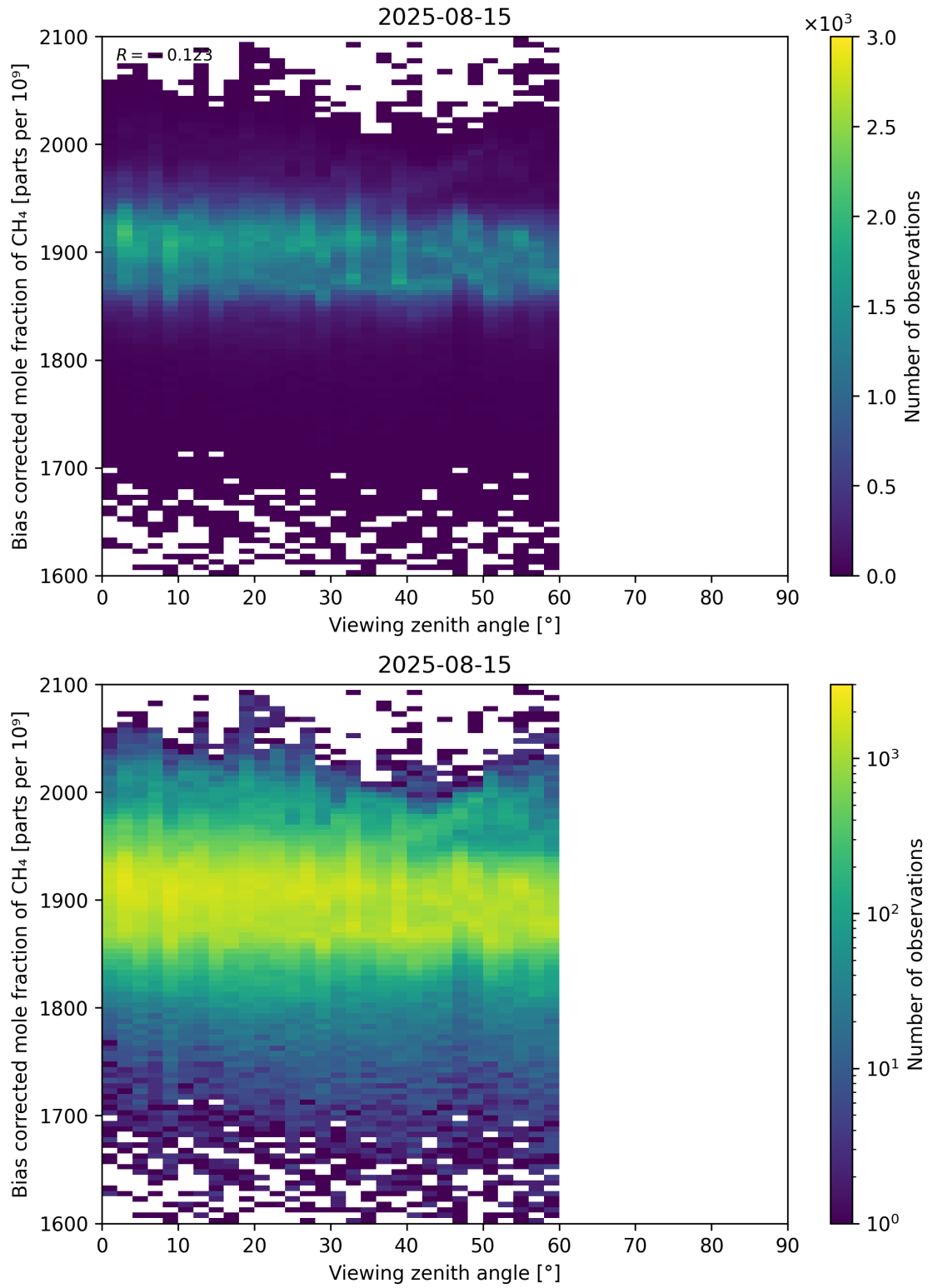
Figure 111: Scatter density plot of “Viewing zenith angle” against “Bias corrected mole fraction of CH 4 ” for 2025-08-14 to 2025-08-16.
