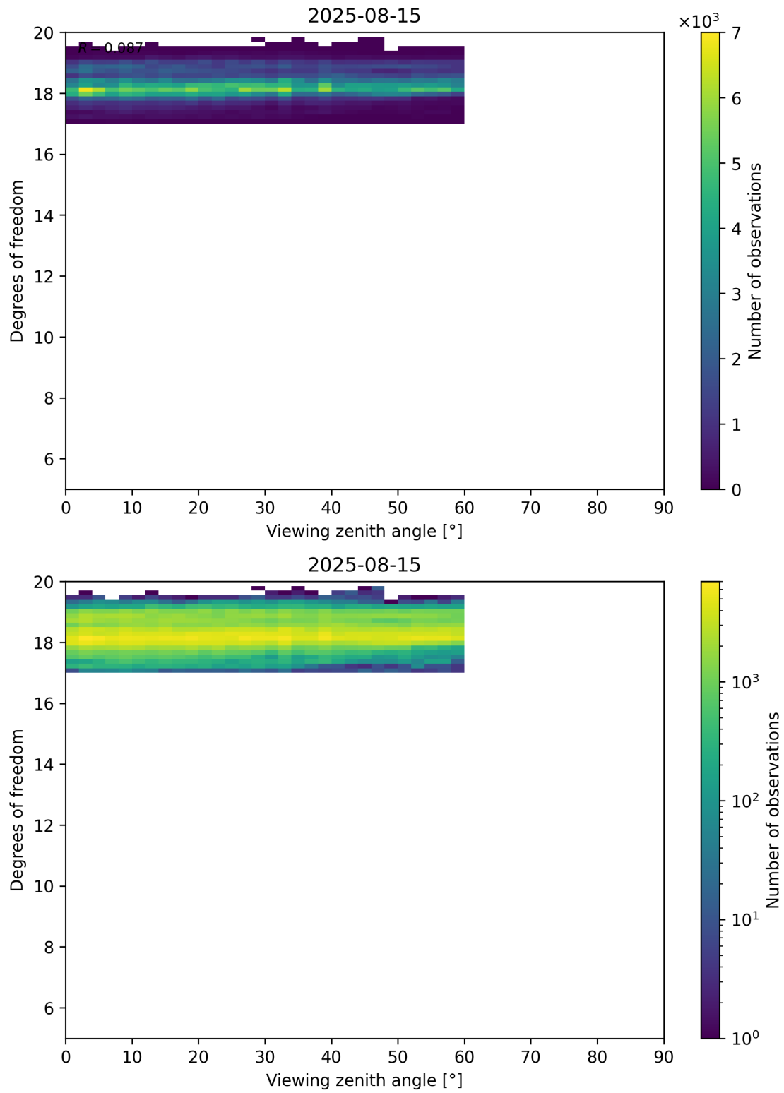
Figure 107: Scatter density plot of “Viewing zenith angle” against “Degrees of freedom” for 2025-08-14 to 2025-08-16.
