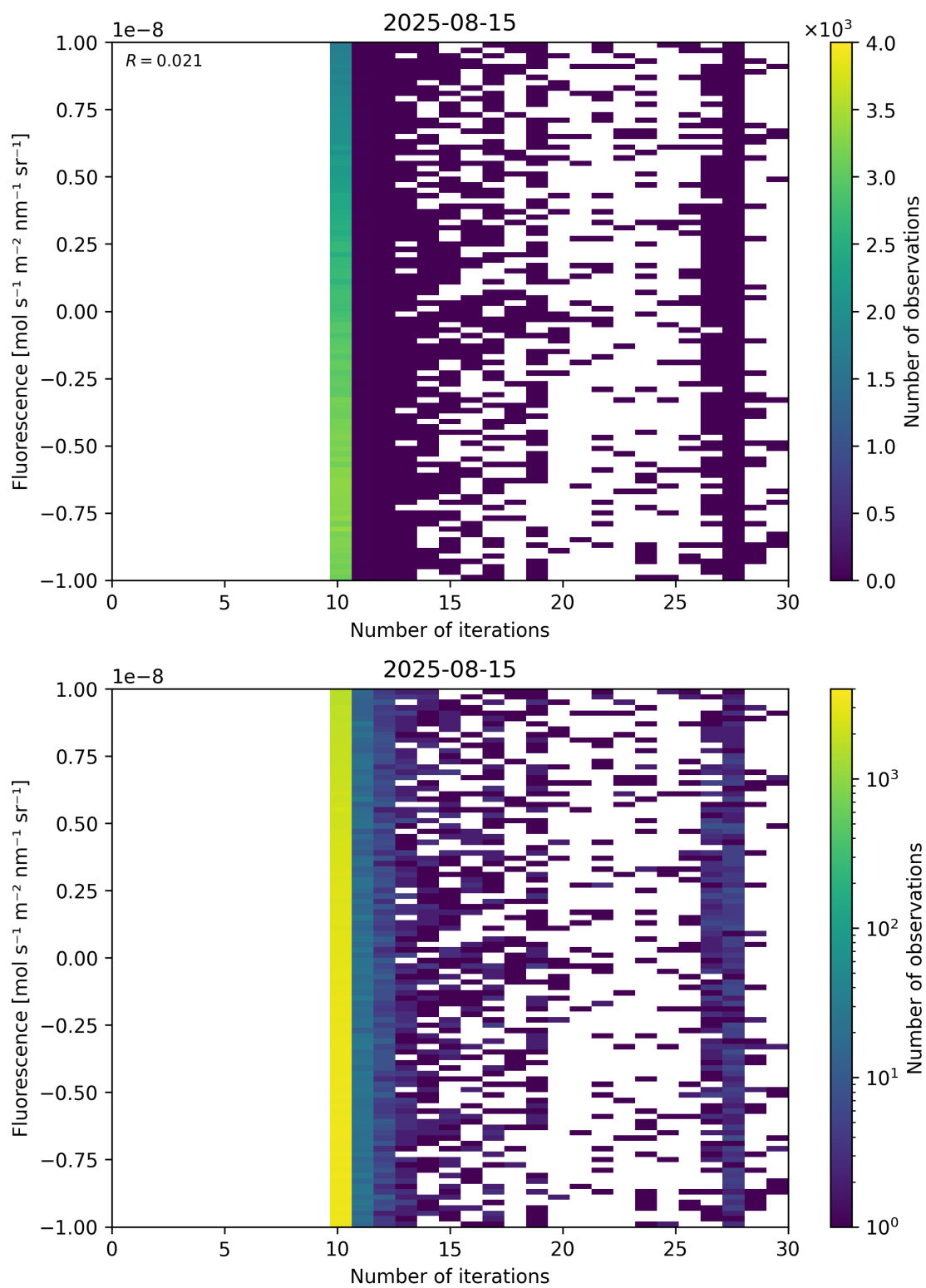
Figure 87: Scatter density plot of “Number of iterations” against “Fluorescence” for 2025-08-14 to 2025-08-16.
