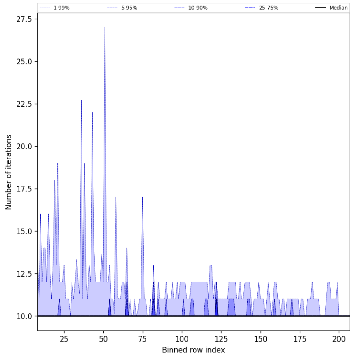
Figure 42: Along track statistics of “Number of iterations” for 2025-08-14 to 2025-08-16
