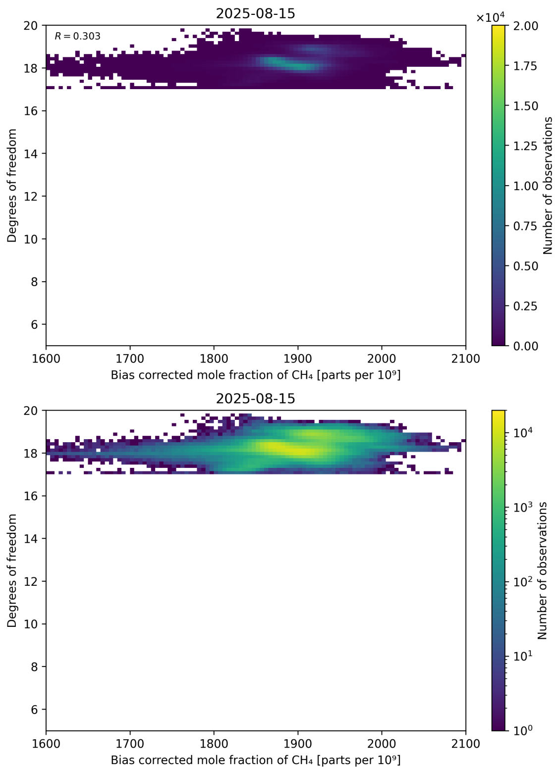
Figure 65: Scatter density plot of “Bias corrected mole fraction of CH 4 ” against “Degrees of freedom” for 2025-08-14 to 2025-08-16.
