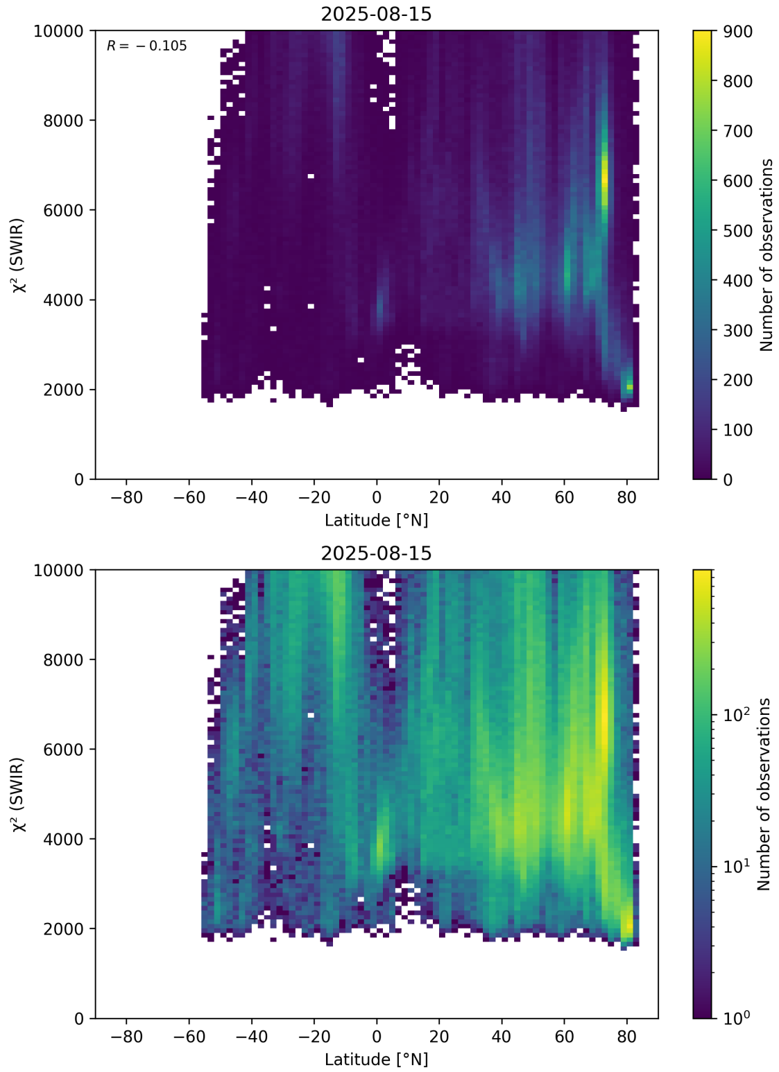
Figure 54: Scatter density plot of “Latitude” against “ \chi^2 (SWIR)” for 2025-08-14 to 2025-08-16.
