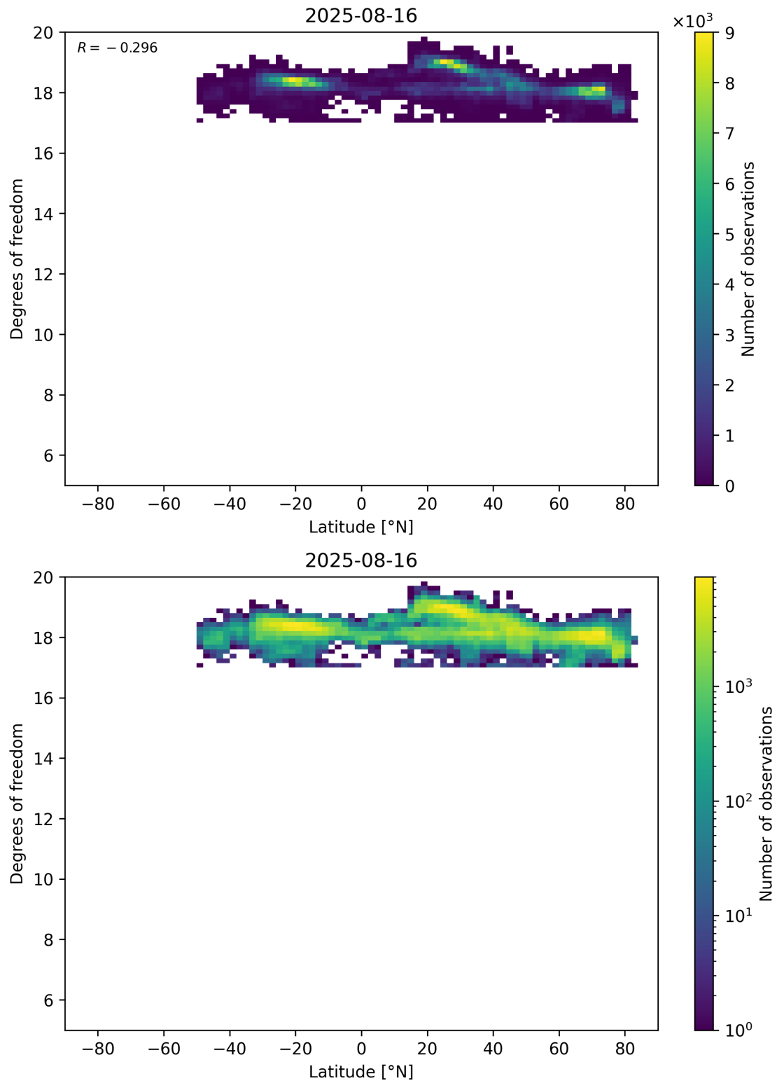
Figure 55: Scatter density plot of “Latitude” against “Degrees of freedom” for 2025-08-15 to 2025-08-17.
