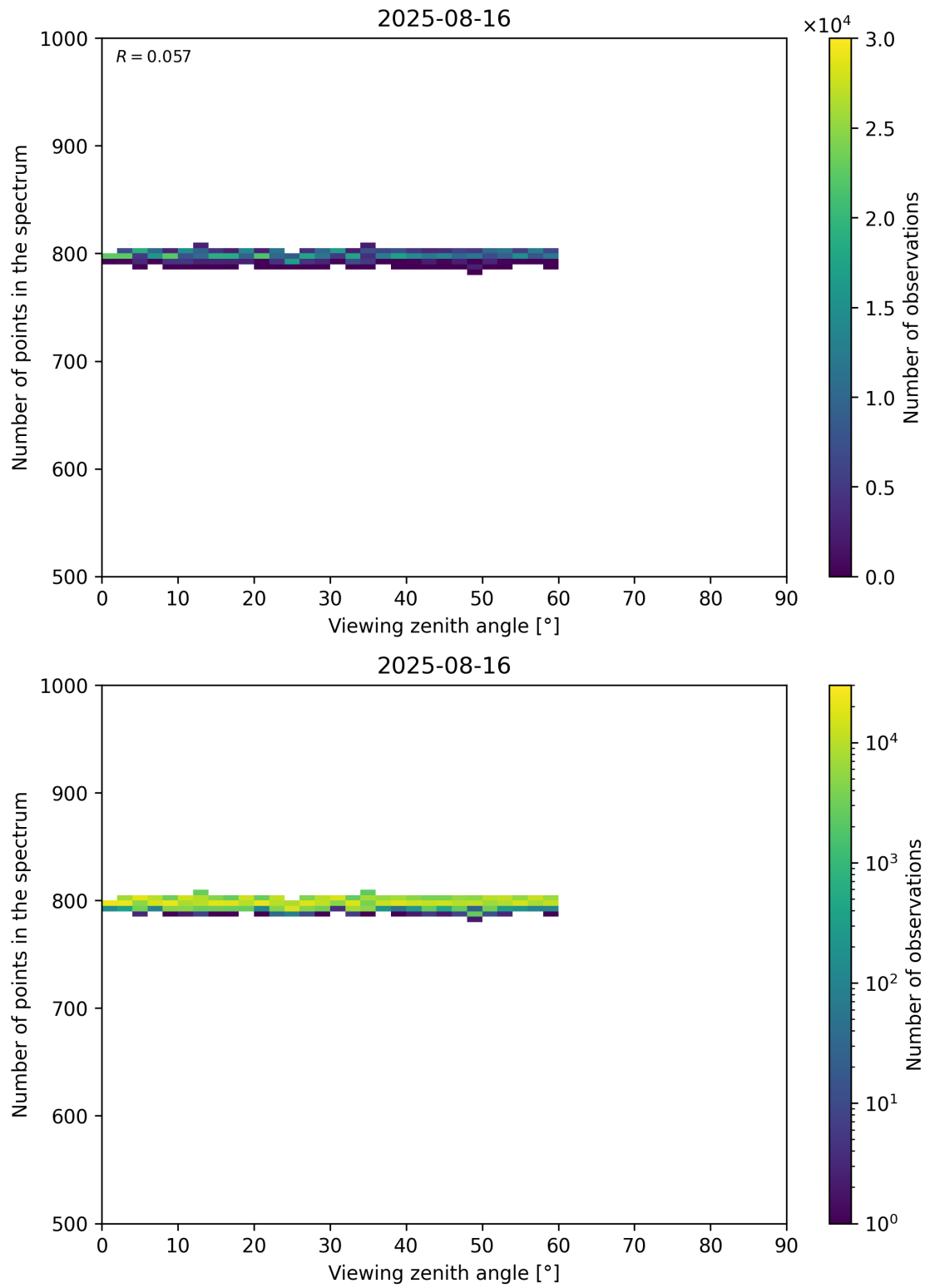
Figure 114: Scatter density plot of “Viewing zenith angle” against “Number of points in the spectrum” for 2025-08-15 to 2025-08-17.
