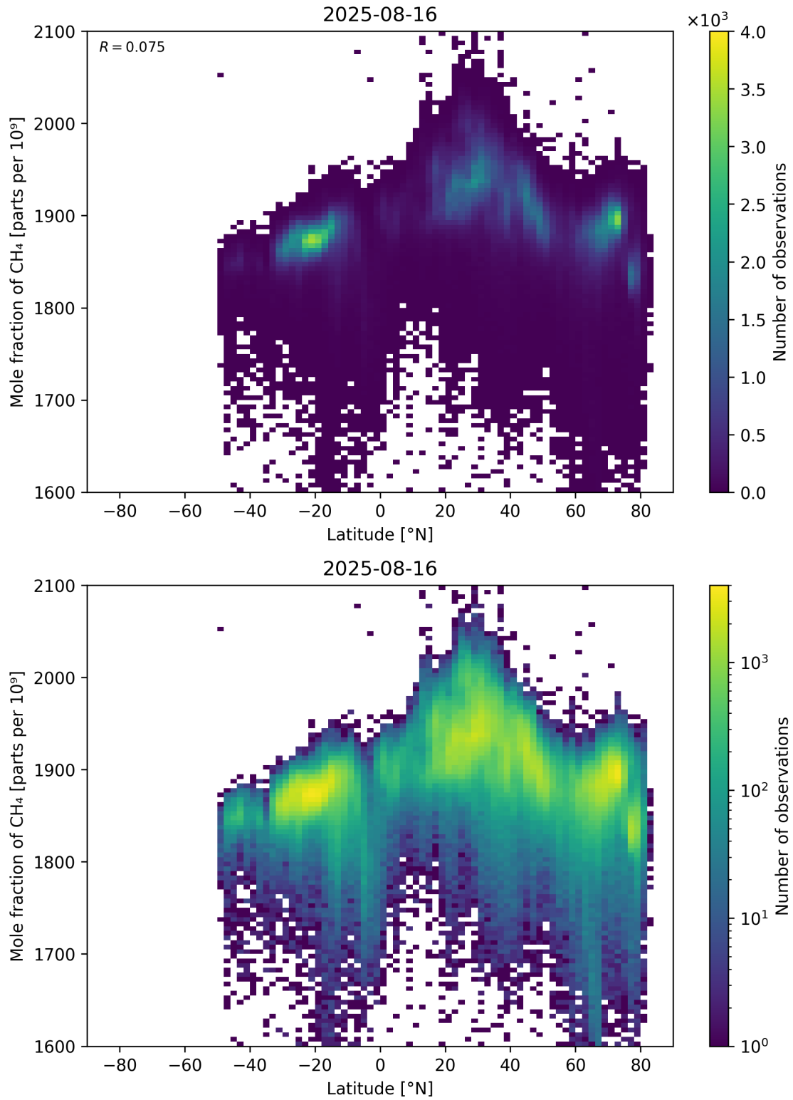
Figure 57: Scatter density plot of “Latitude” against “Mole fraction of CH 4 ” for 2025-08-15 to 2025-08-17.
