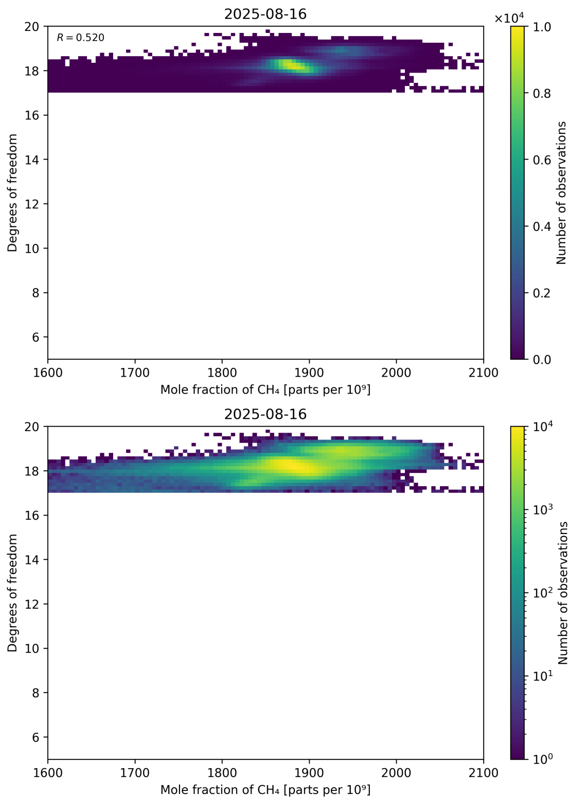
Figure 72: Scatter density plot of “Mole fraction of CH 4 ” against “Degrees of freedom” for 2025-08-15 to 2025-08-17.
