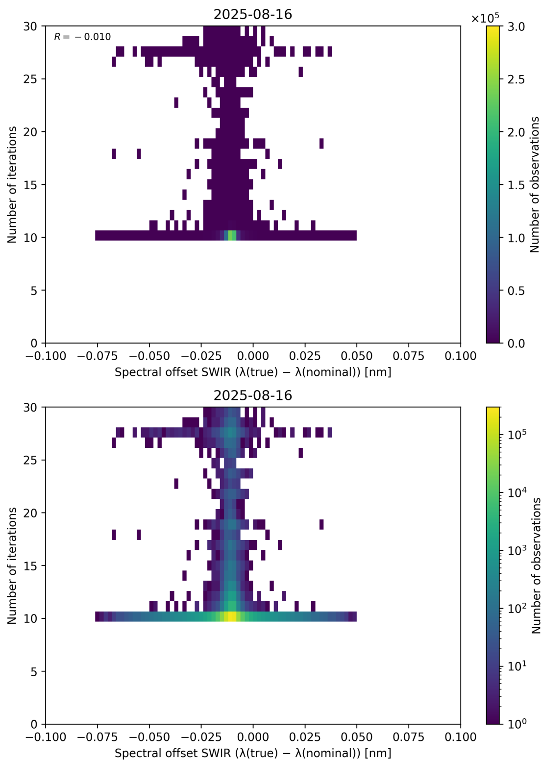
Figure 121: Scatter density plot of “Spectral offset SWIR ( \lambda_{\text{true}} - \lambda_{\text{nominal}} )” against “Number of iterations” for 2025-08-15 to 2025-08-17.
