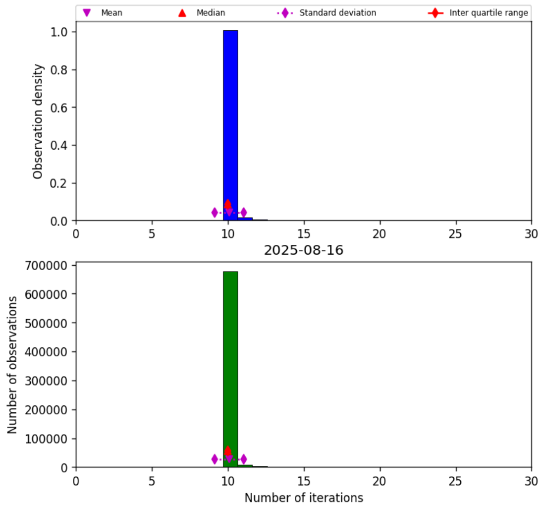
Figure 31: Histogram of “Number of iterations” for 2025-08-15 to 2025-08-17
