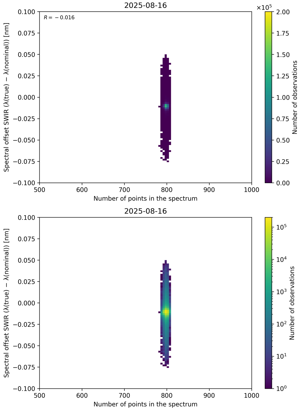
Figure 93: Scatter density plot of “Number of points in the spectrum” against “Spectral offset SWIR ( \lambda_{\text{true}} - \lambda_{\text{nominal}} )” for 2025-08-15 to 2025-08-17.
