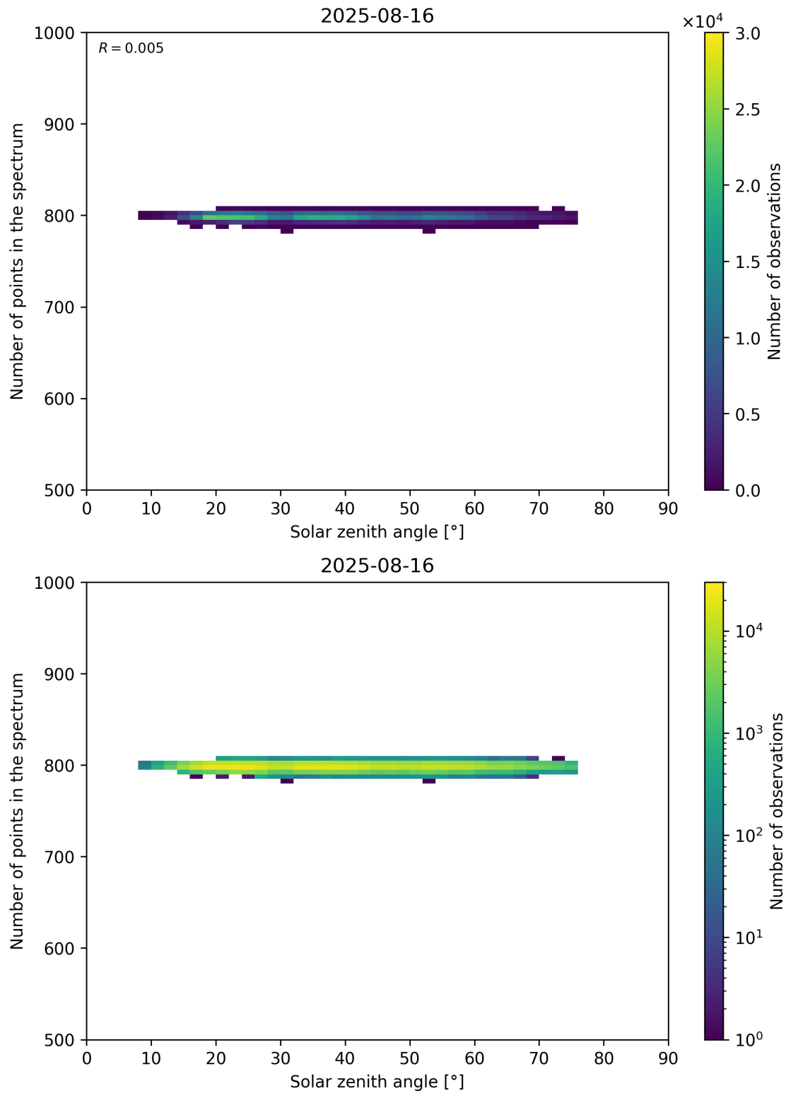
Figure 103: Scatter density plot of “Solar zenith angle” against “Number of points in the spectrum” for 2025-08-15 to 2025-08-17.
