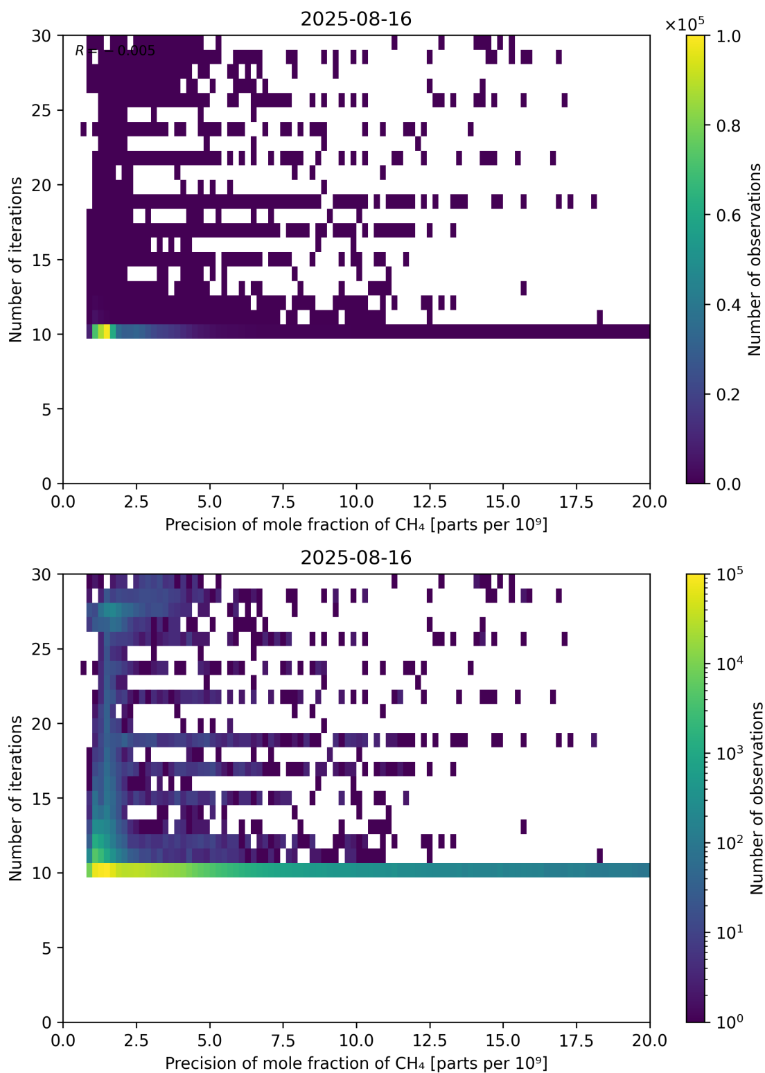
Figure 83: Scatter density plot of “Precision of mole fraction of CH 4 ” against “Number of iterations” for 2025-08-15 to 2025-08-17.
