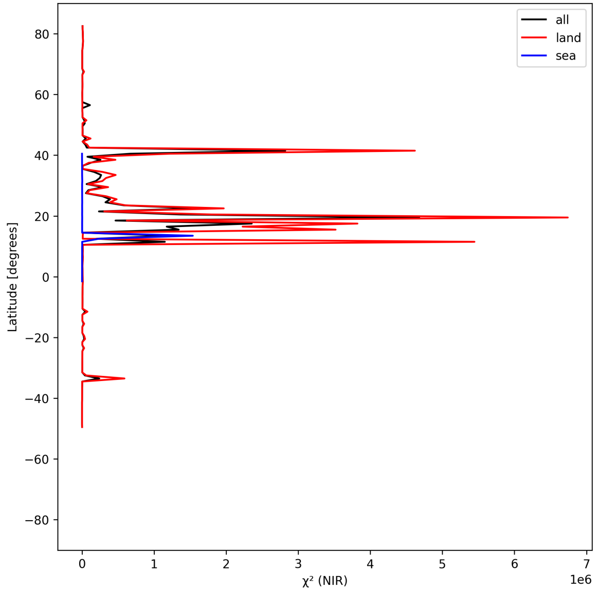
Figure 18: Zonal average of “ \chi^2 (NIR)” for 2025-08-15 to 2025-08-17.
