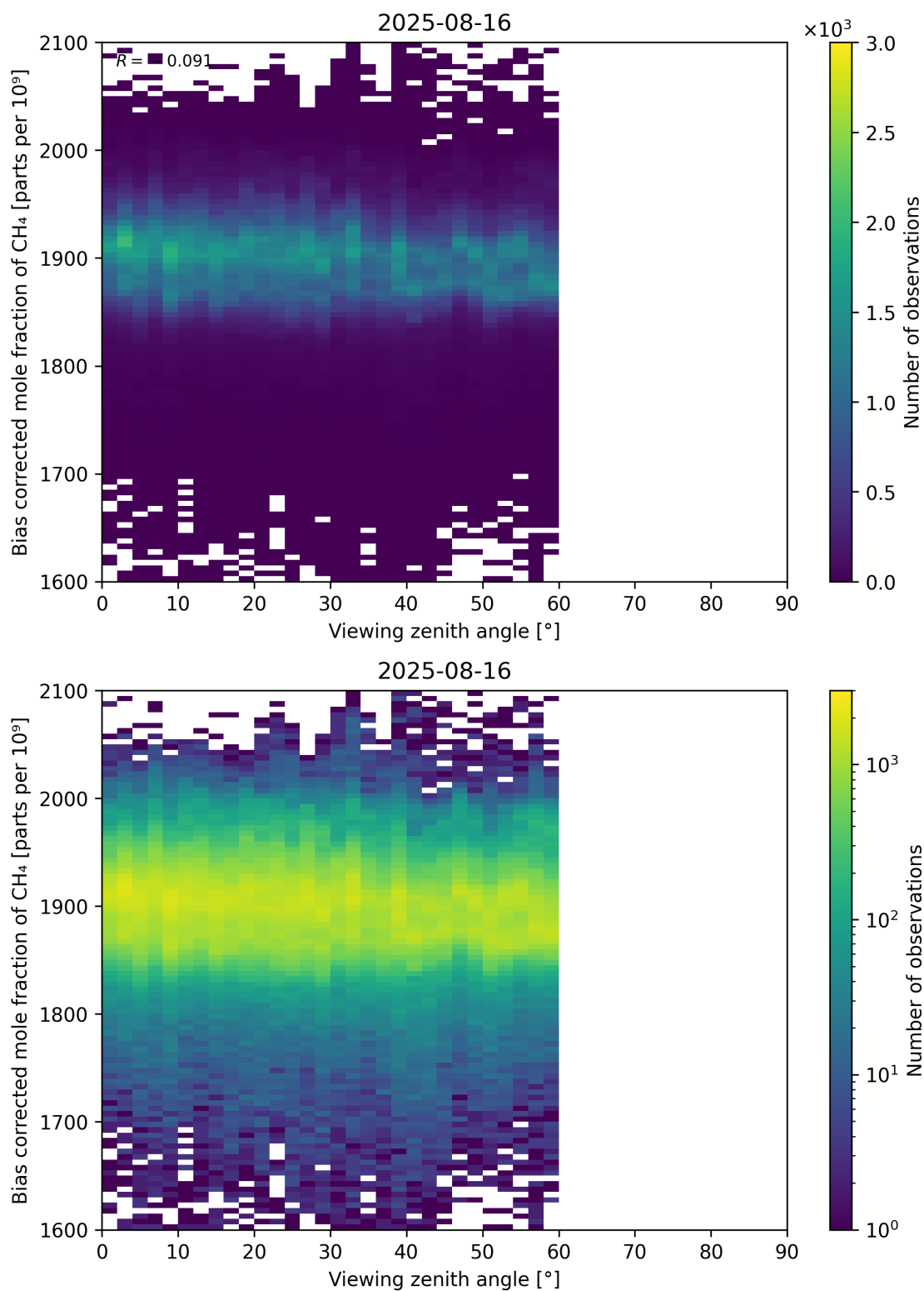
Figure 111: Scatter density plot of “Viewing zenith angle” against “Bias corrected mole fraction of CH 4 ” for 2025-08-15 to 2025-08-17.
