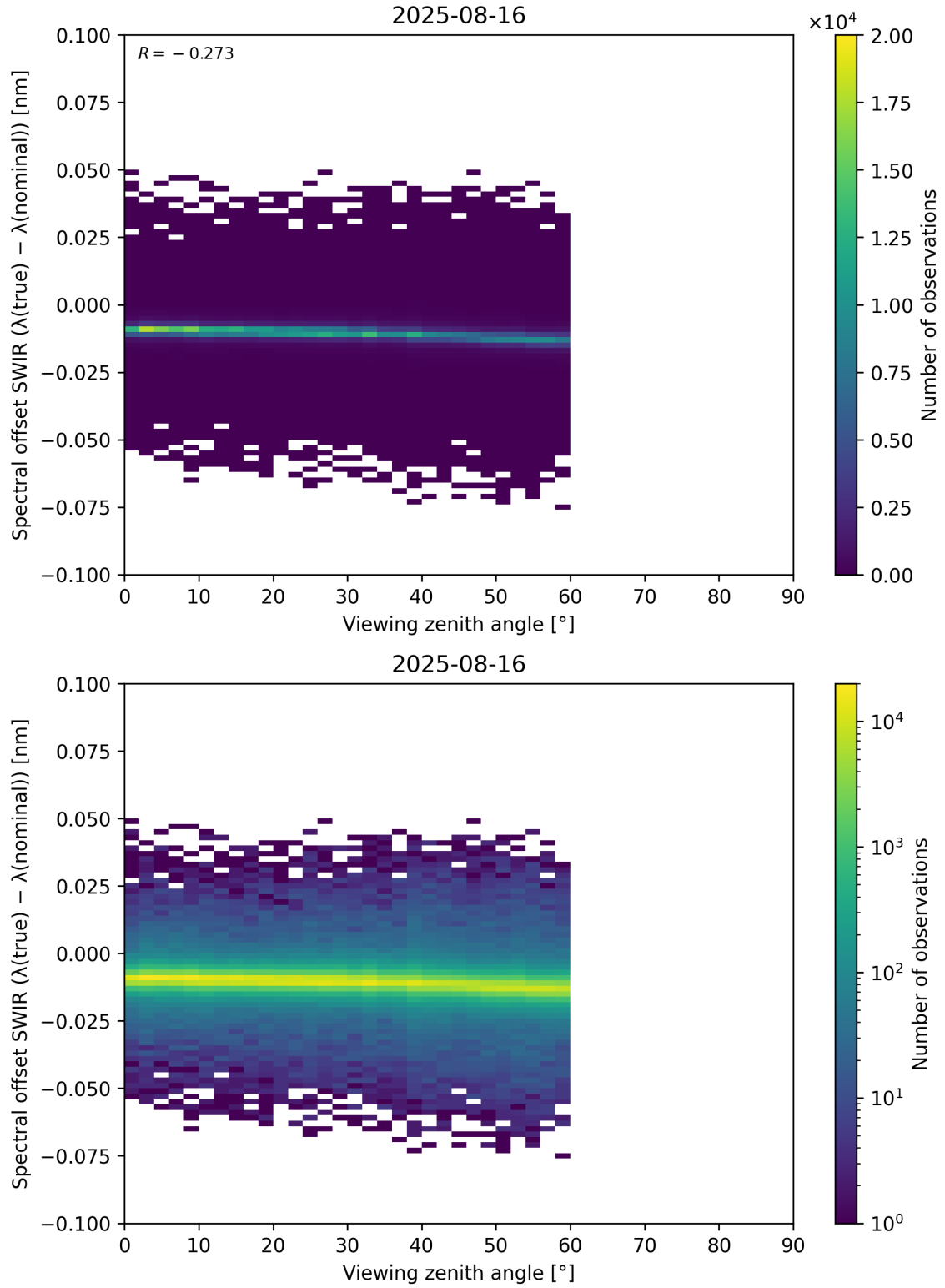
Figure 116: Scatter density plot of “Viewing zenith angle” against “Spectral offset SWIR ( \lambda_{\text{true}} - \lambda_{\text{nominal}} )” for 2025-08-15 to 2025-08-17.
