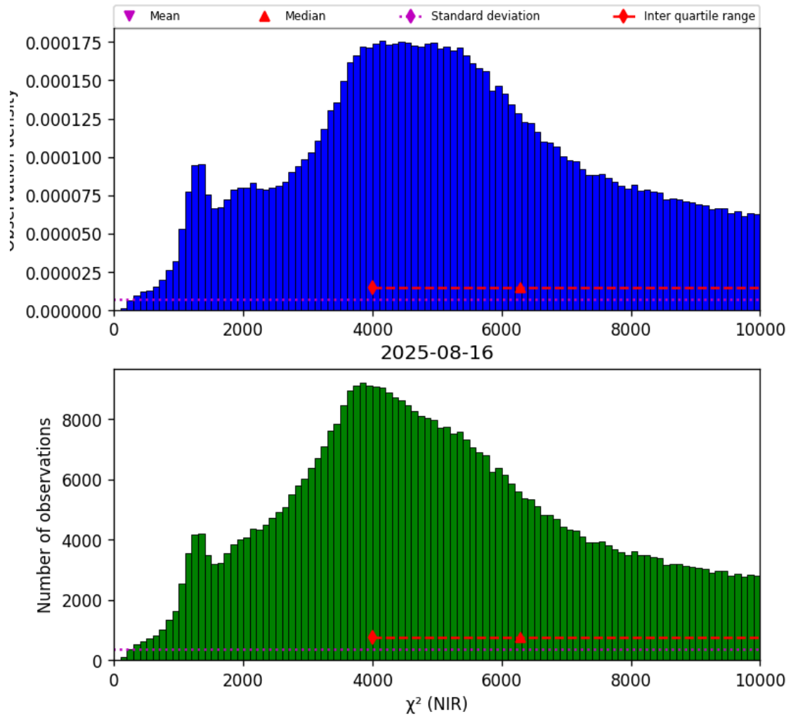
Figure 29: Histogram of “ \chi^2 (NIR)” for 2025-08-15 to 2025-08-17
