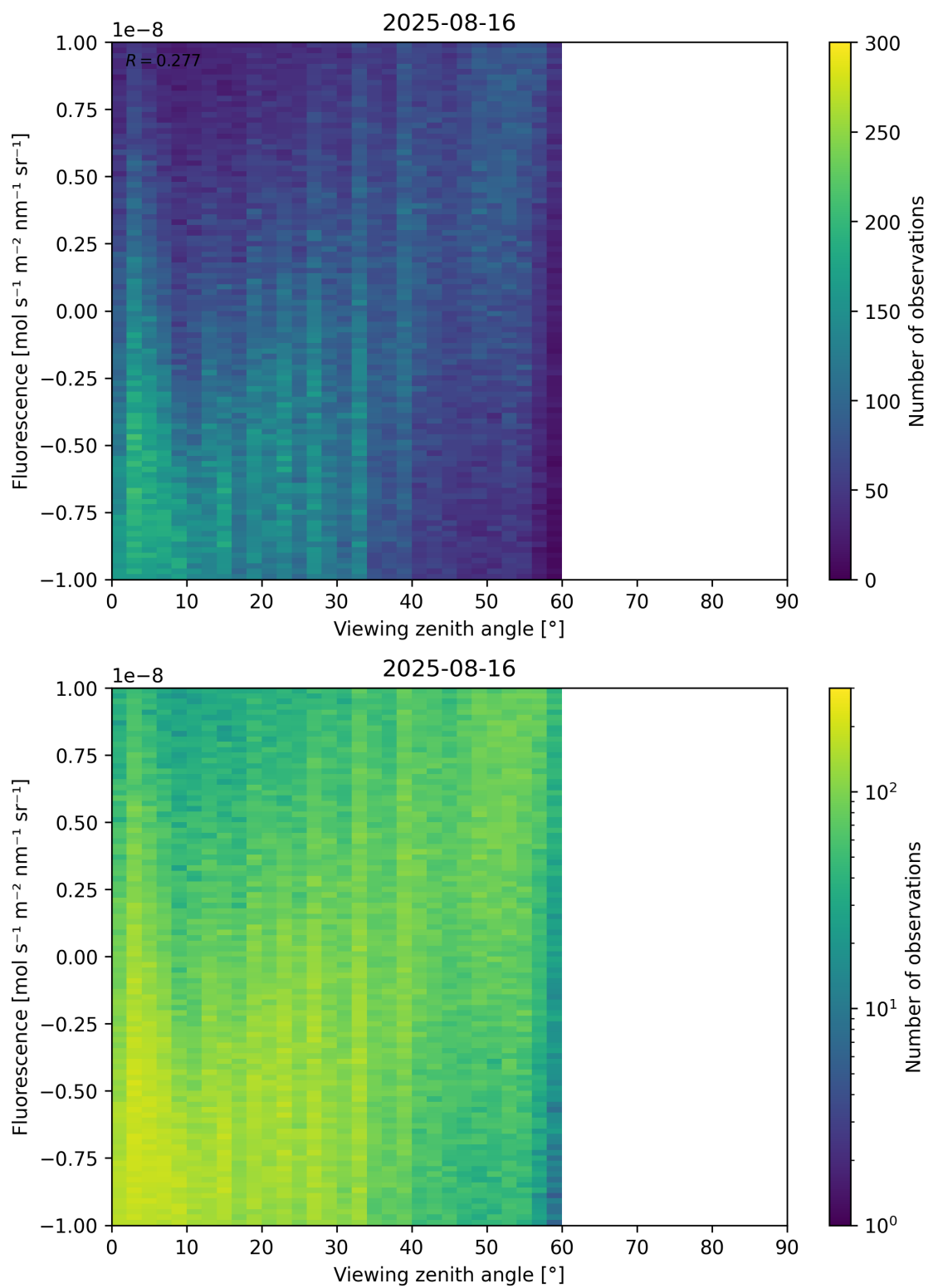
Figure 108: Scatter density plot of “Viewing zenith angle” against “Fluorescence” for 2025-08-15 to 2025-08-17.
