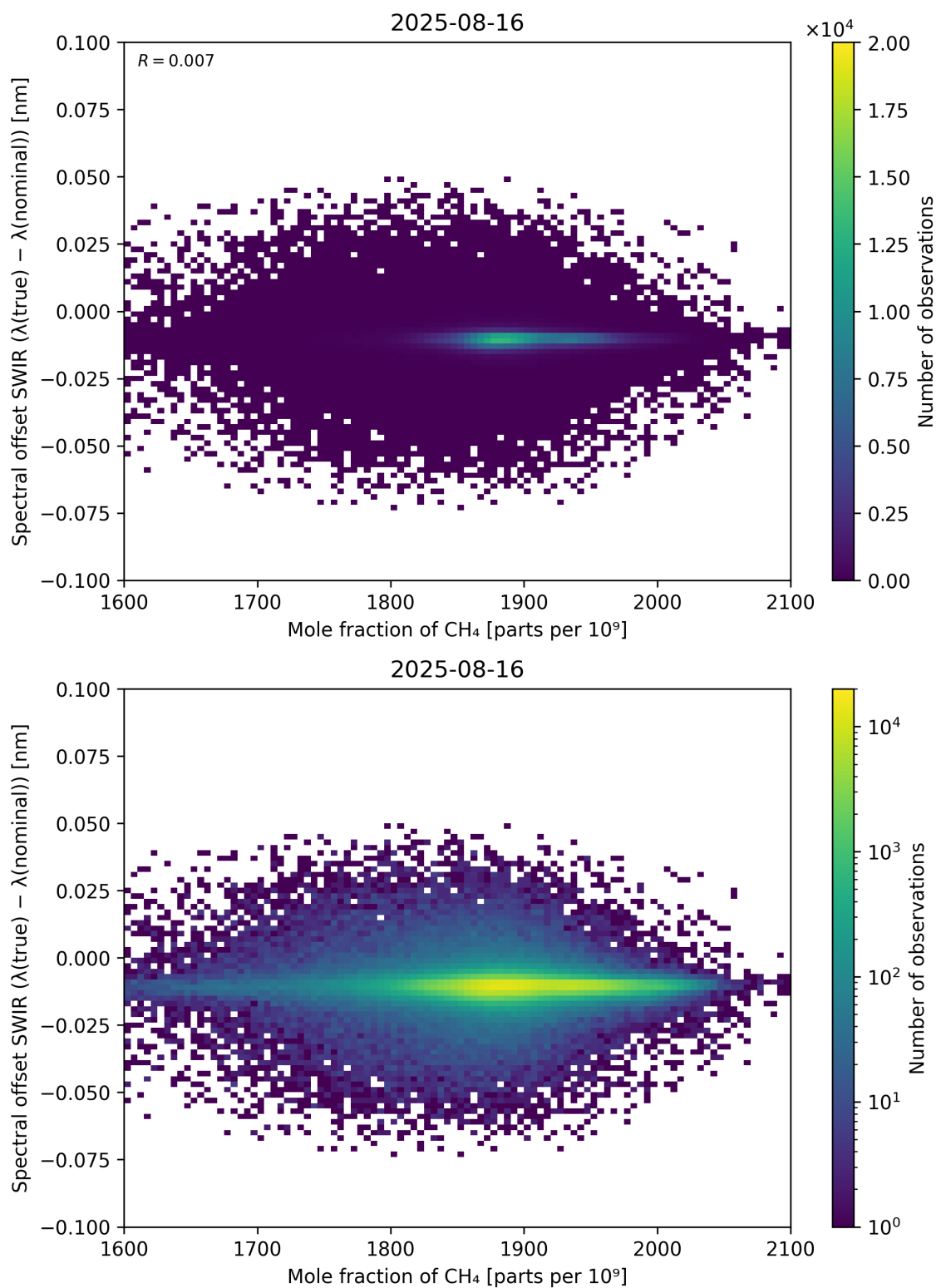
Figure 86: Scatter density plot of “Mole fraction of CH 4 ” against “Spectral offset SWIR ( \lambda_{\text{true}} - \lambda_{\text{nominal}} )” for 2025-08-15 to 2025-08-17.
