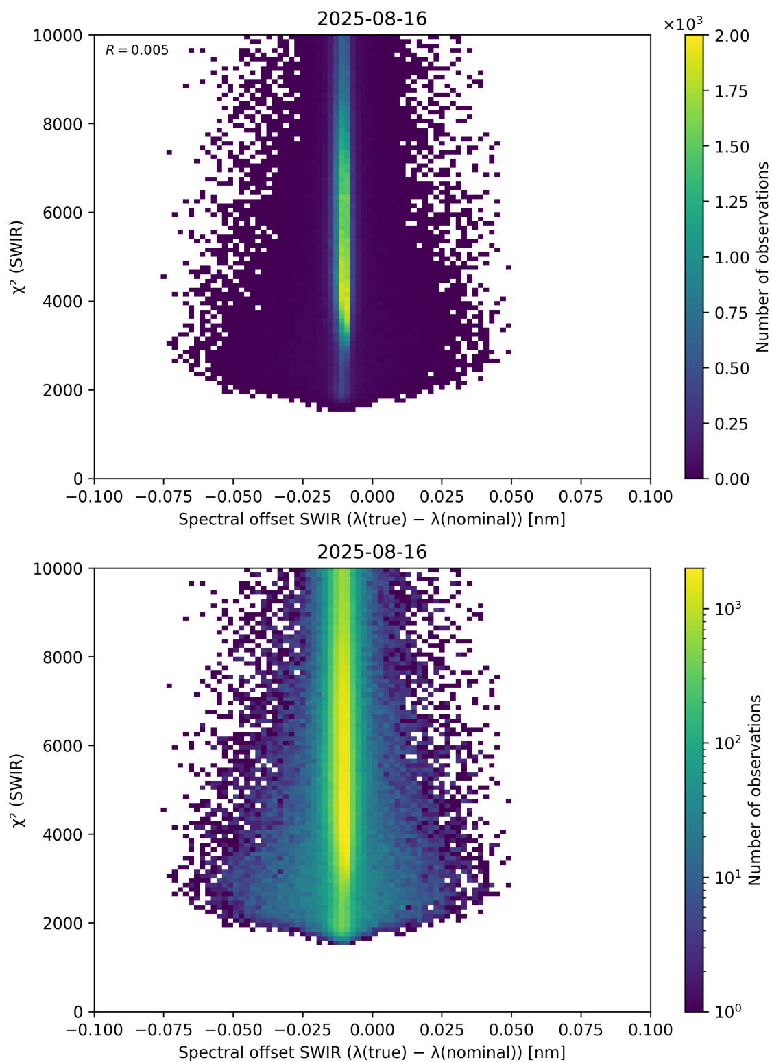
Figure 118: Scatter density plot of “Spectral offset SWIR ( \lambda_{\text{true}} - \lambda_{\text{nominal}} )” against “ \chi^2 (SWIR)” for 2025-08-15 to 2025-08-17.
