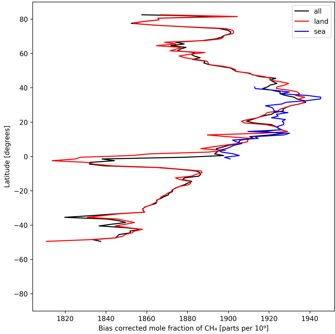
Figure 14: Zonal average of “Bias corrected mole fraction of \text{CH}_4 ” for 2025-08-15 to 2025-08-17.
