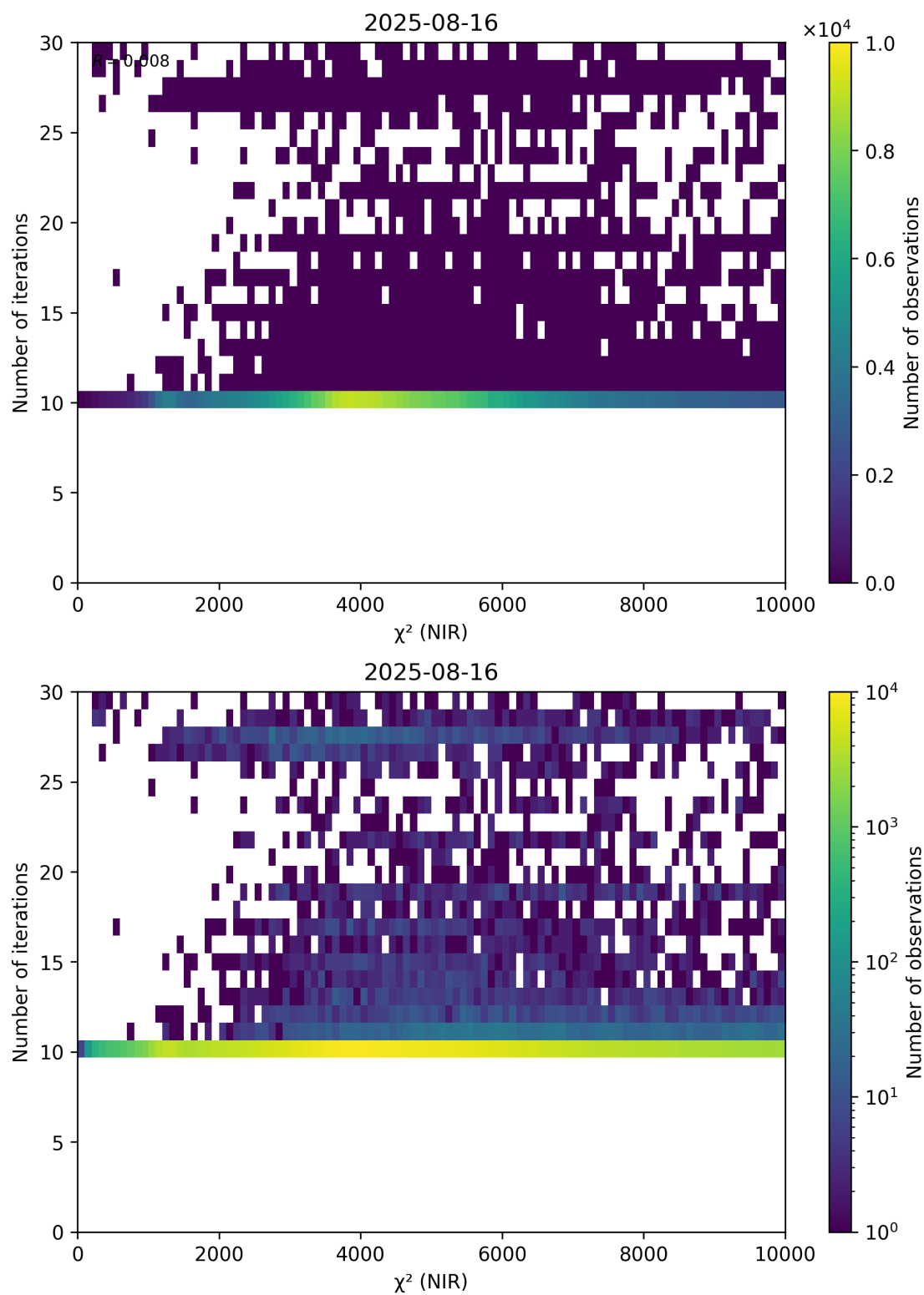
Figure 46: Scatter density plot of “ \chi^2 (NIR)” against “Number of iterations” for 2025-08-15 to 2025-08-17.
