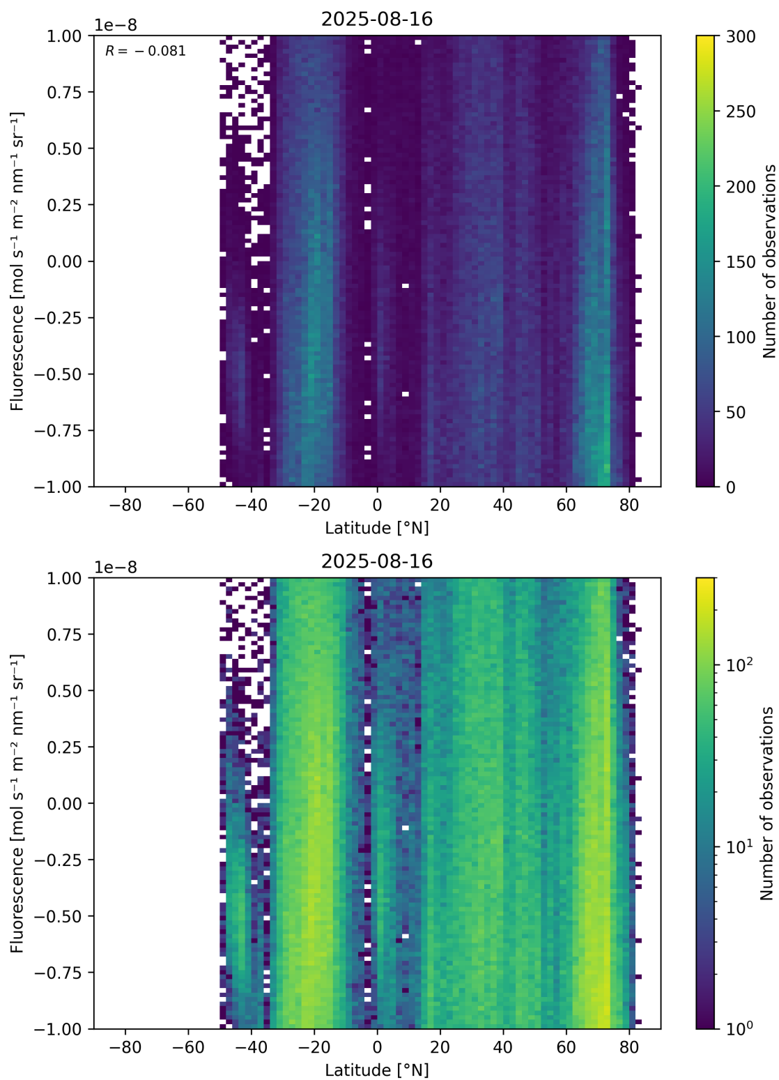
Figure 56: Scatter density plot of “Latitude” against “Fluorescence” for 2025-08-15 to 2025-08-17.
