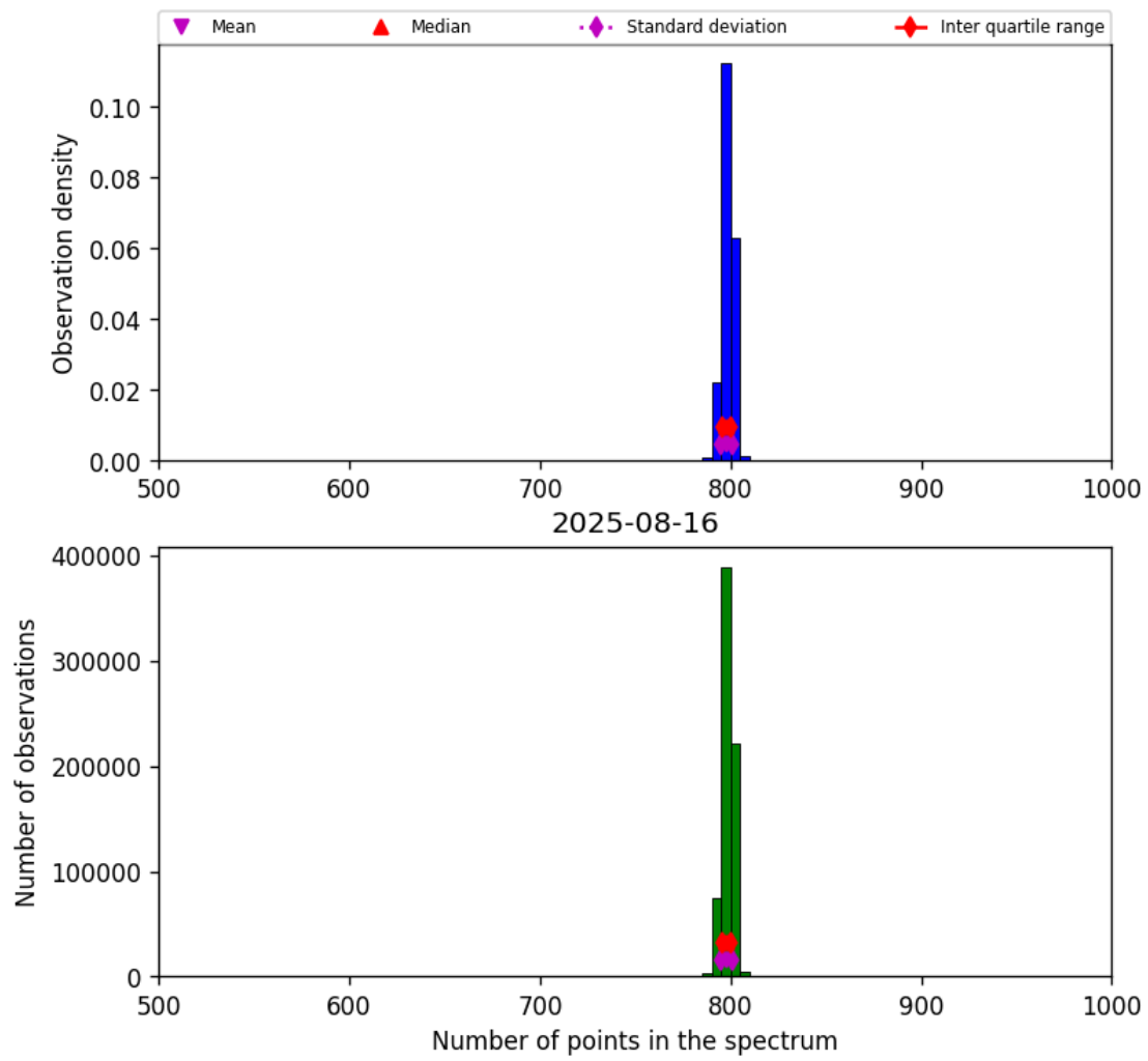
Figure 26: Histogram of “Number of points in the spectrum” for 2025-08-15 to 2025-08-17
