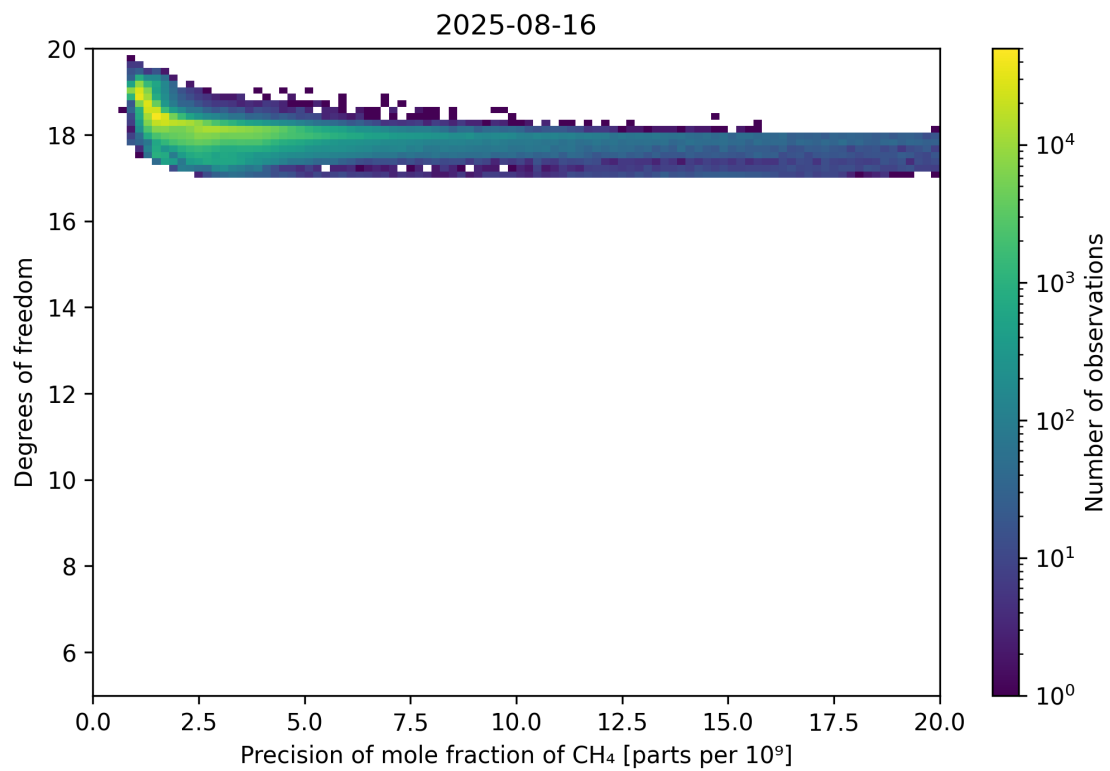
Figure 80: Scatter density plot of “Precision of mole fraction of CH 4 ” against “Degrees of freedom” for 2025-08-15 to 2025-08-17.
