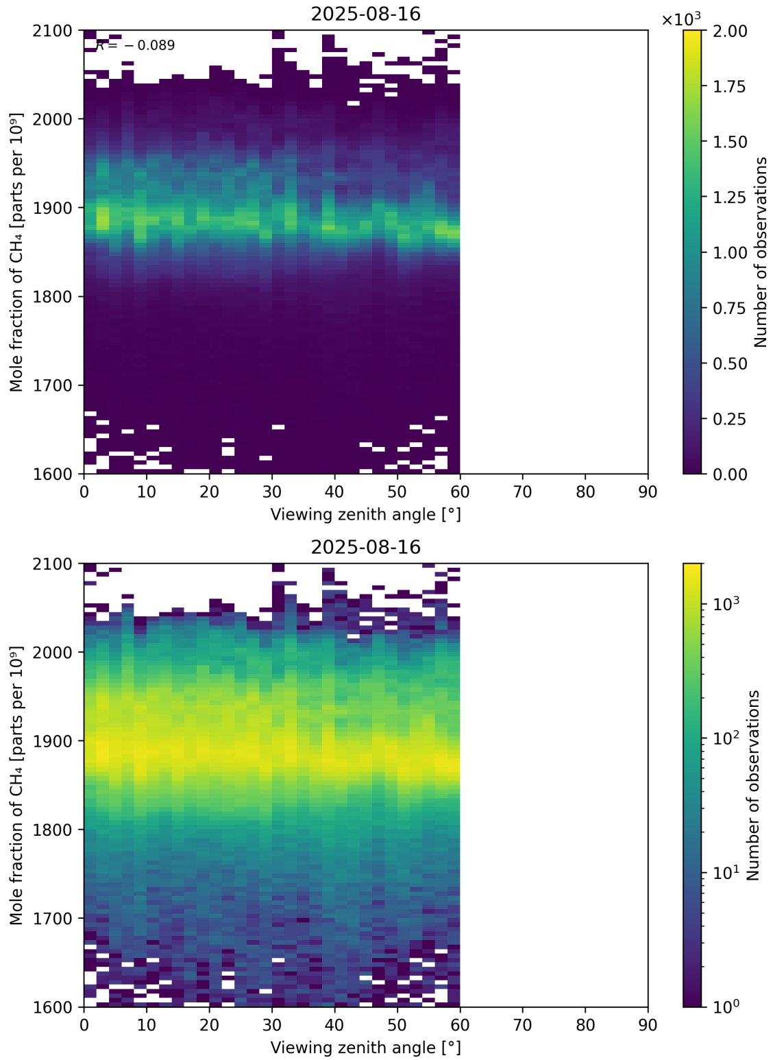
Figure 110: Scatter density plot of “Viewing zenith angle” against “Mole fraction of CH 4 ” for 2025-08-15 to 2025-08-17.
