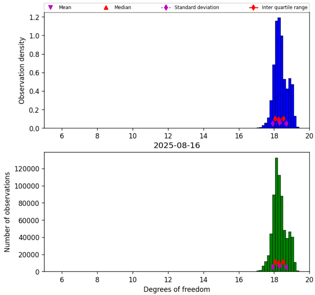
Figure 30: Histogram of “Degrees of freedom” for 2025-08-15 to 2025-08-17
