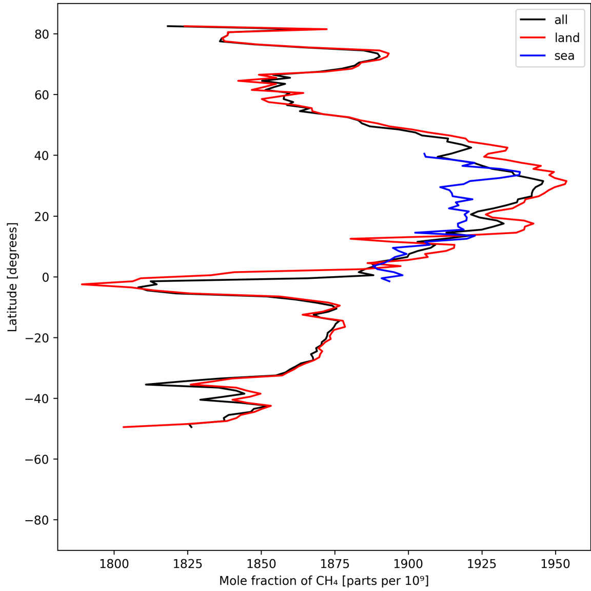
Figure 12: Zonal average of “Mole fraction of \text{CH}_4 ” for 2025-08-15 to 2025-08-17.
