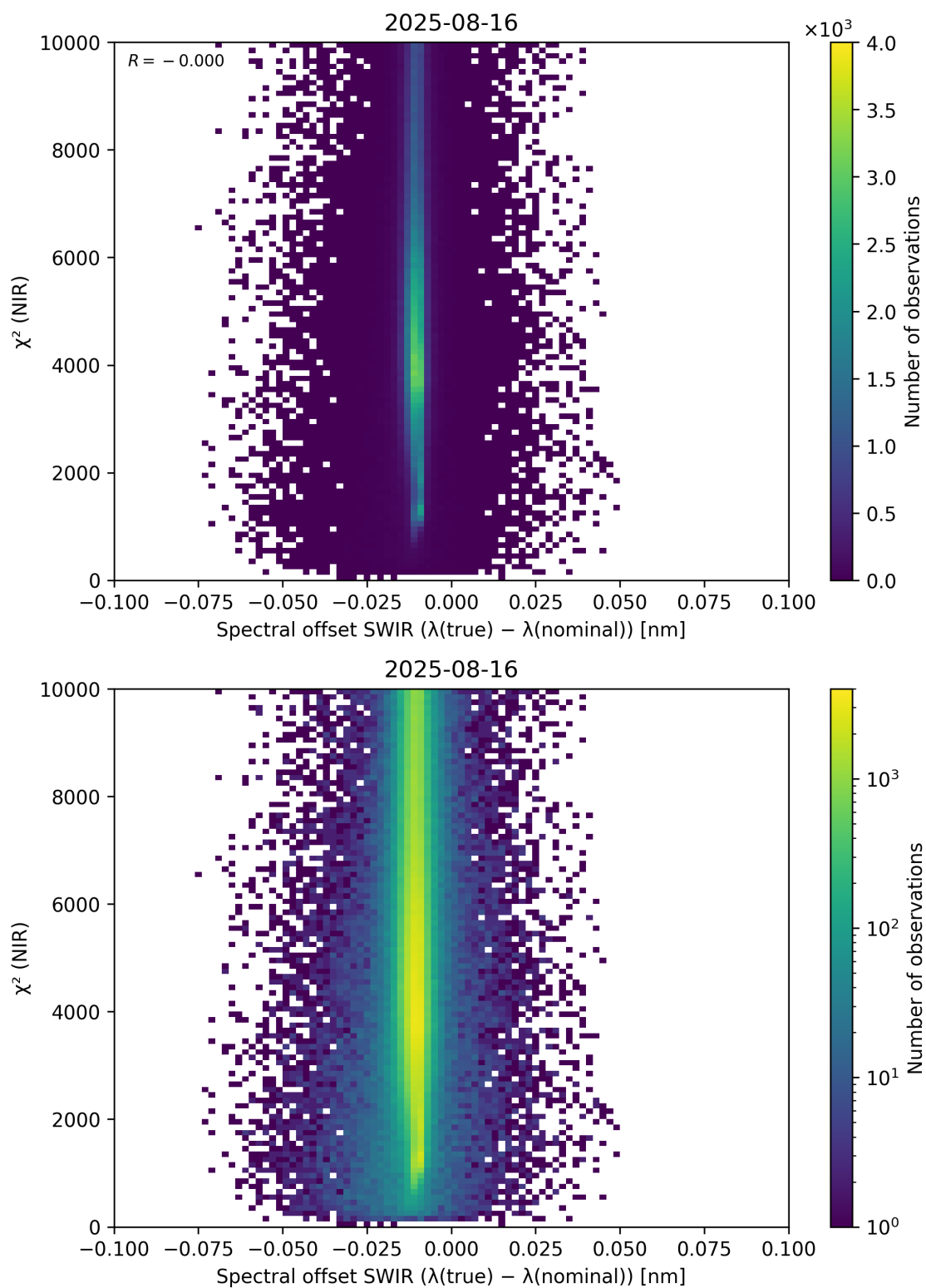
Figure 117: Scatter density plot of “Spectral offset SWIR ( \lambda_{\text{true}} - \lambda_{\text{nominal}} )” against “ \chi^2 (NIR)” for 2025-08-15 to 2025-08-17.
