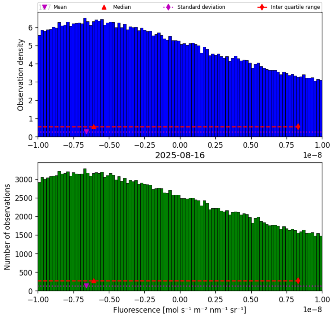
Figure 32: Histogram of “Fluorescence” for 2025-08-15 to 2025-08-17
