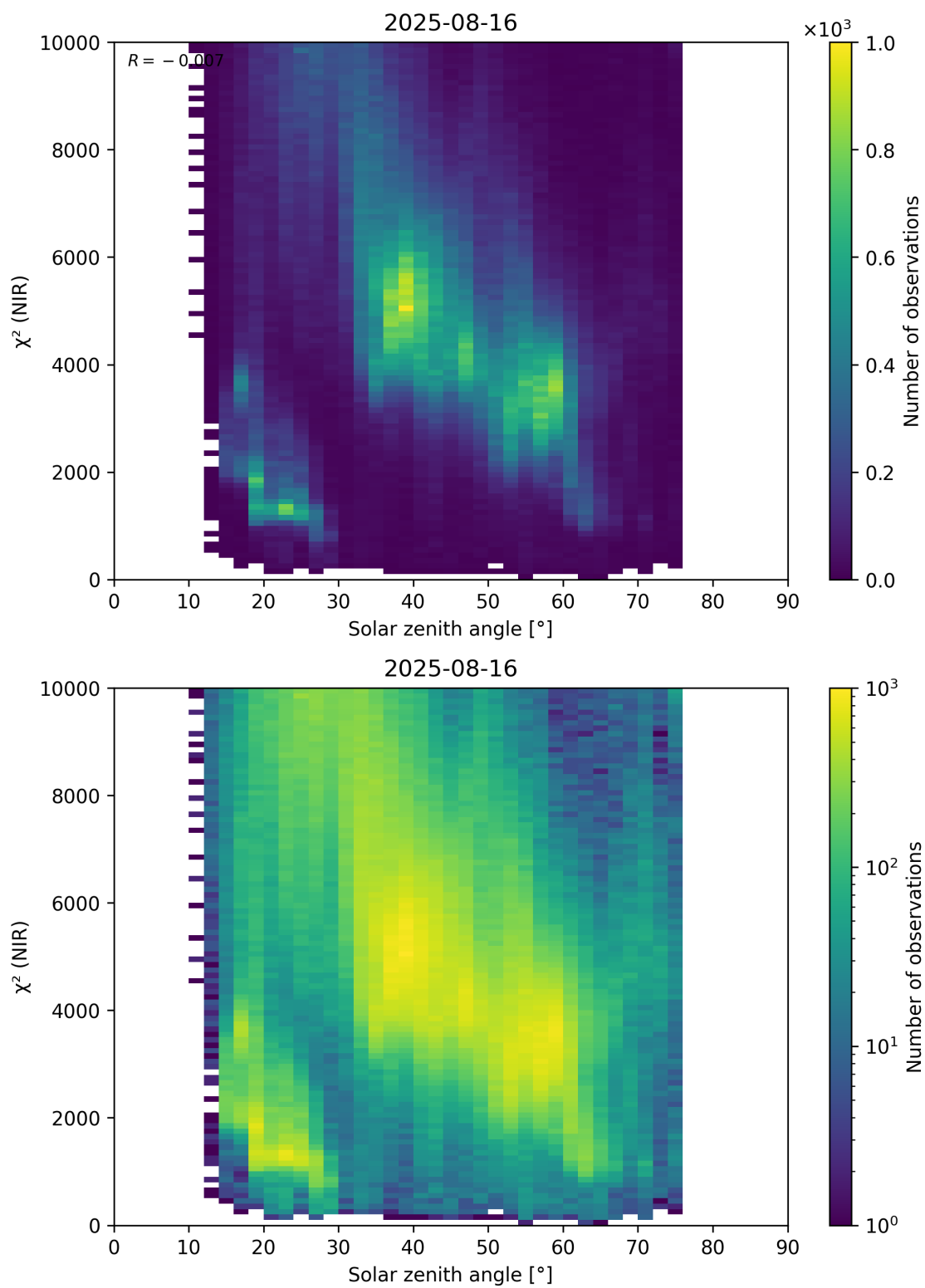
Figure 94: Scatter density plot of “Solar zenith angle” against “ \chi^2 (NIR)” for 2025-08-15 to 2025-08-17.
