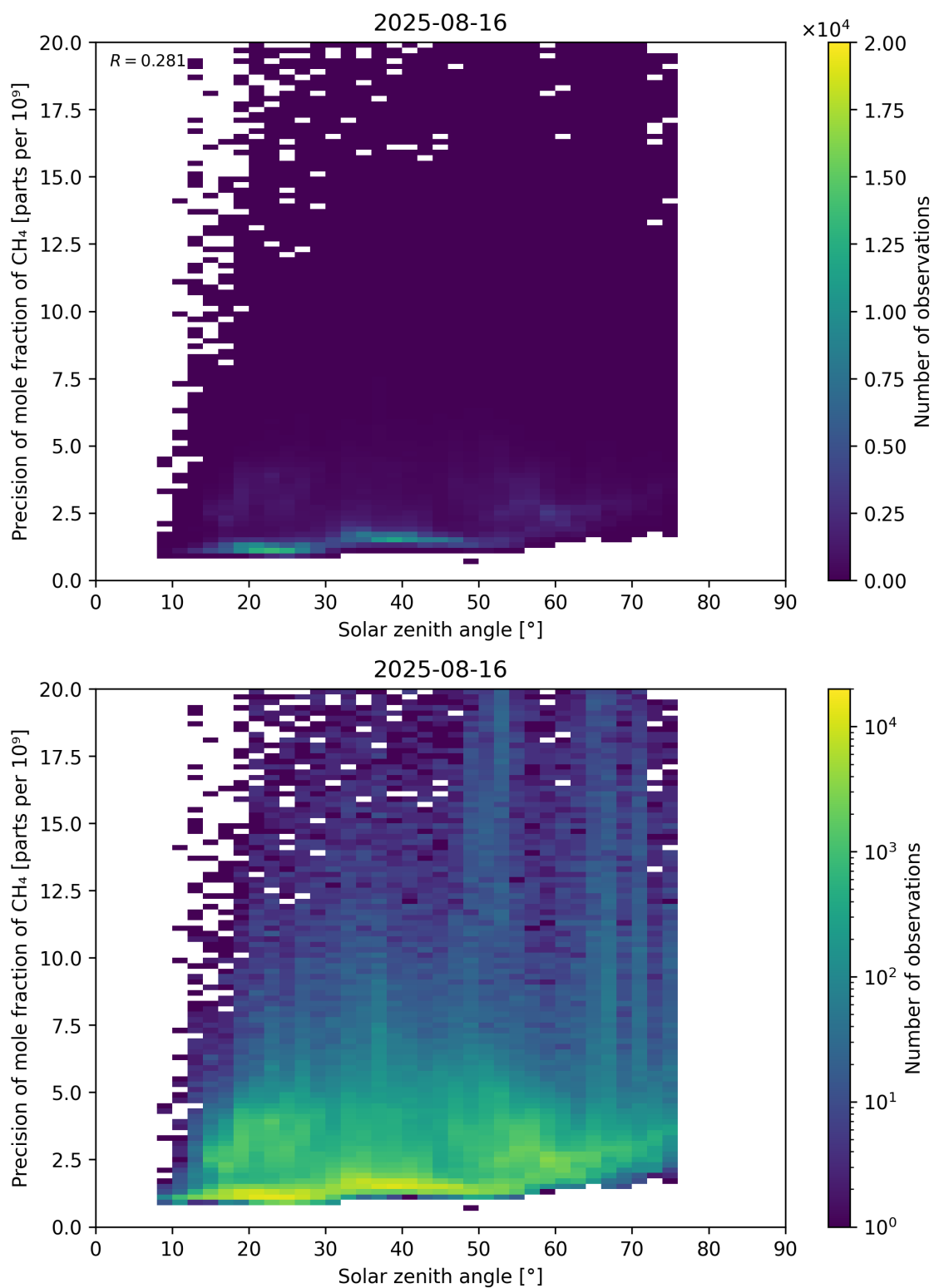
Figure 101: Scatter density plot of “Solar zenith angle” against “Precision of mole fraction of CH 4 ” for 2025-08-15 to 2025-08-17.
