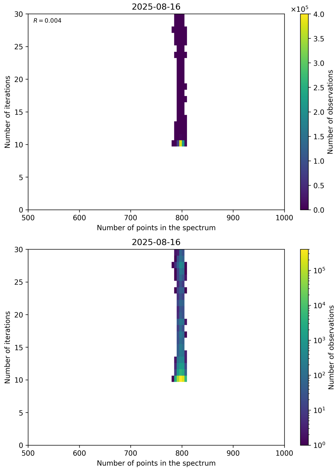
Figure 92: Scatter density plot of “Number of points in the spectrum” against “Number of iterations” for 2025-08-15 to 2025-08-17.
