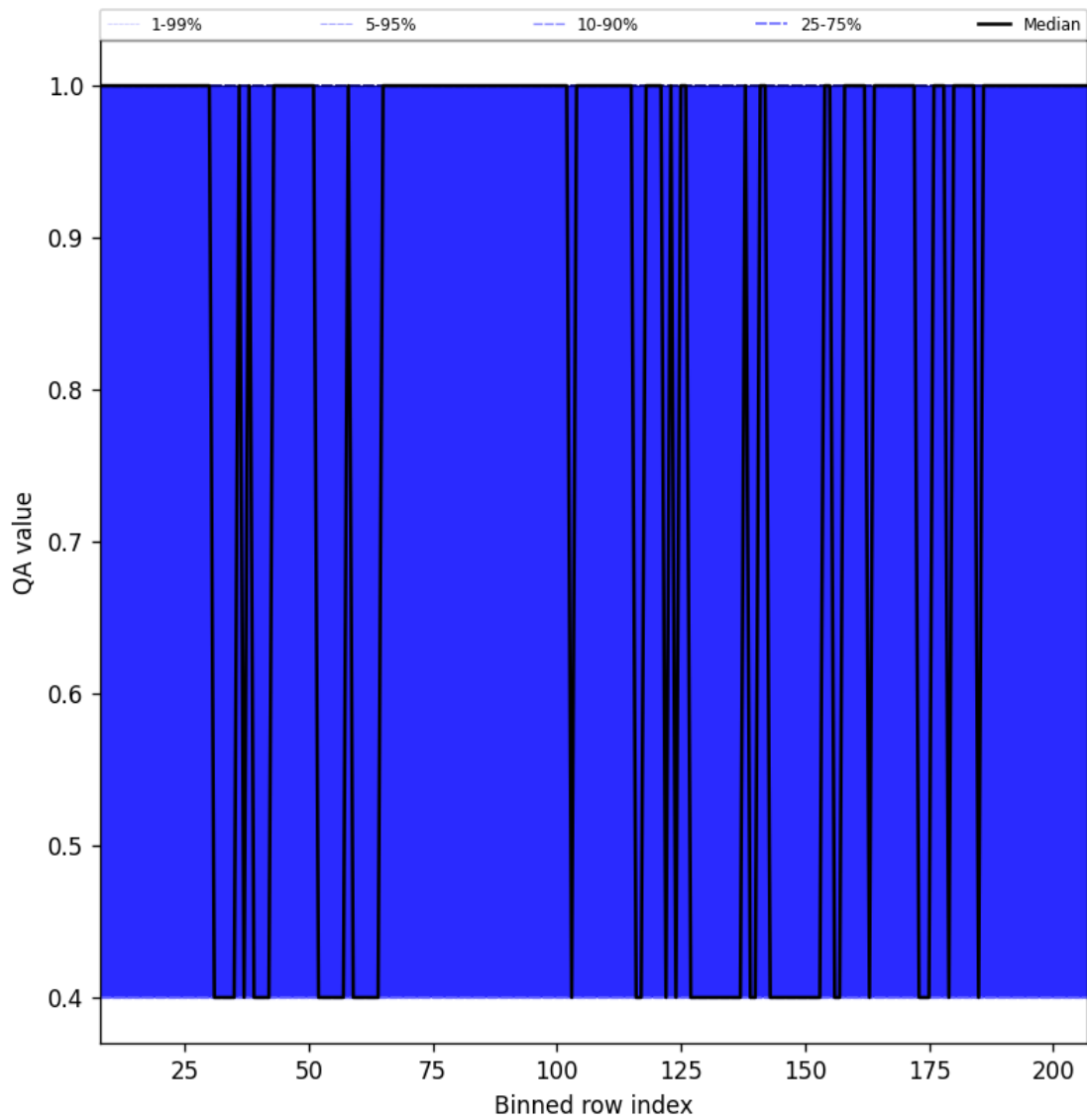
Figure 33: Along track statistics of “QA value” for 2025-08-15 to 2025-08-17
