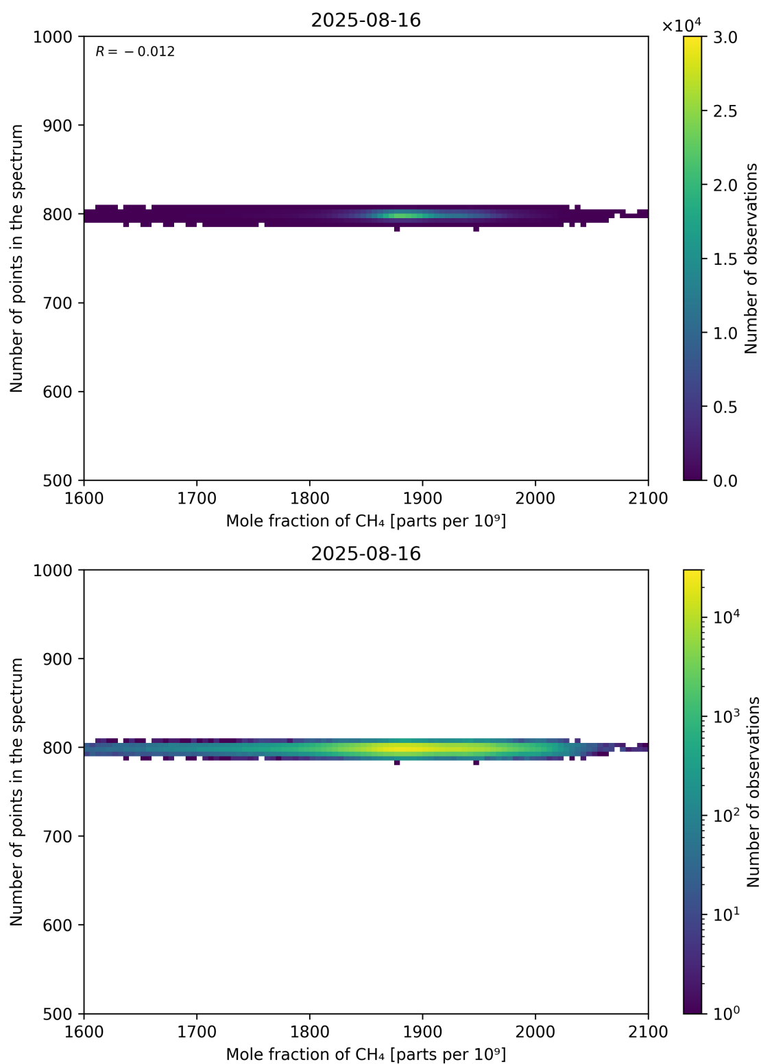
Figure 77: Scatter density plot of “Mole fraction of CH 4 ” against “Number of points in the spectrum” for 2025-08-15 to 2025-08-17.
