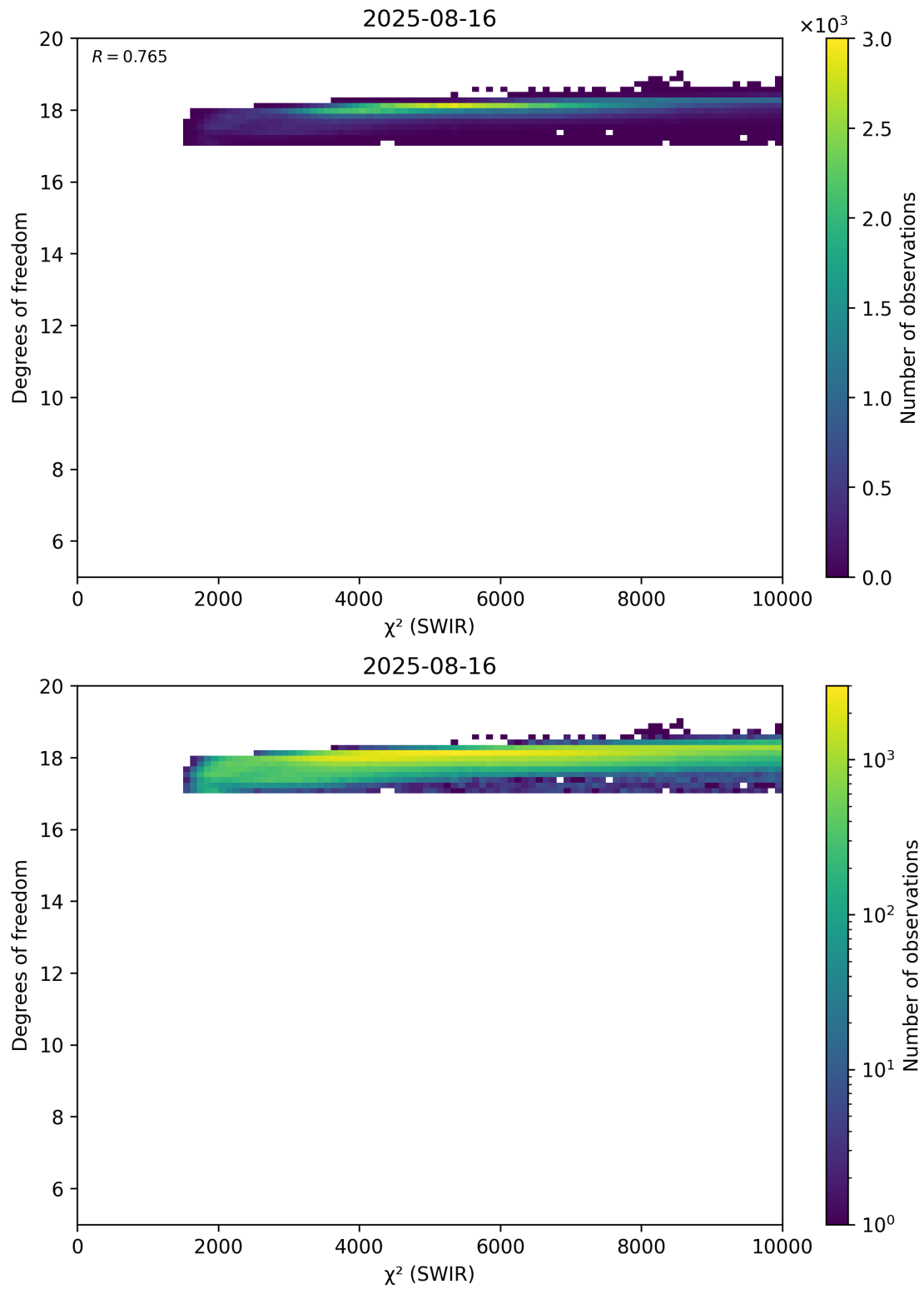
Figure 48: Scatter density plot of “ \chi^2 (SWIR)” against “Degrees of freedom” for 2025-08-15 to 2025-08-17.
