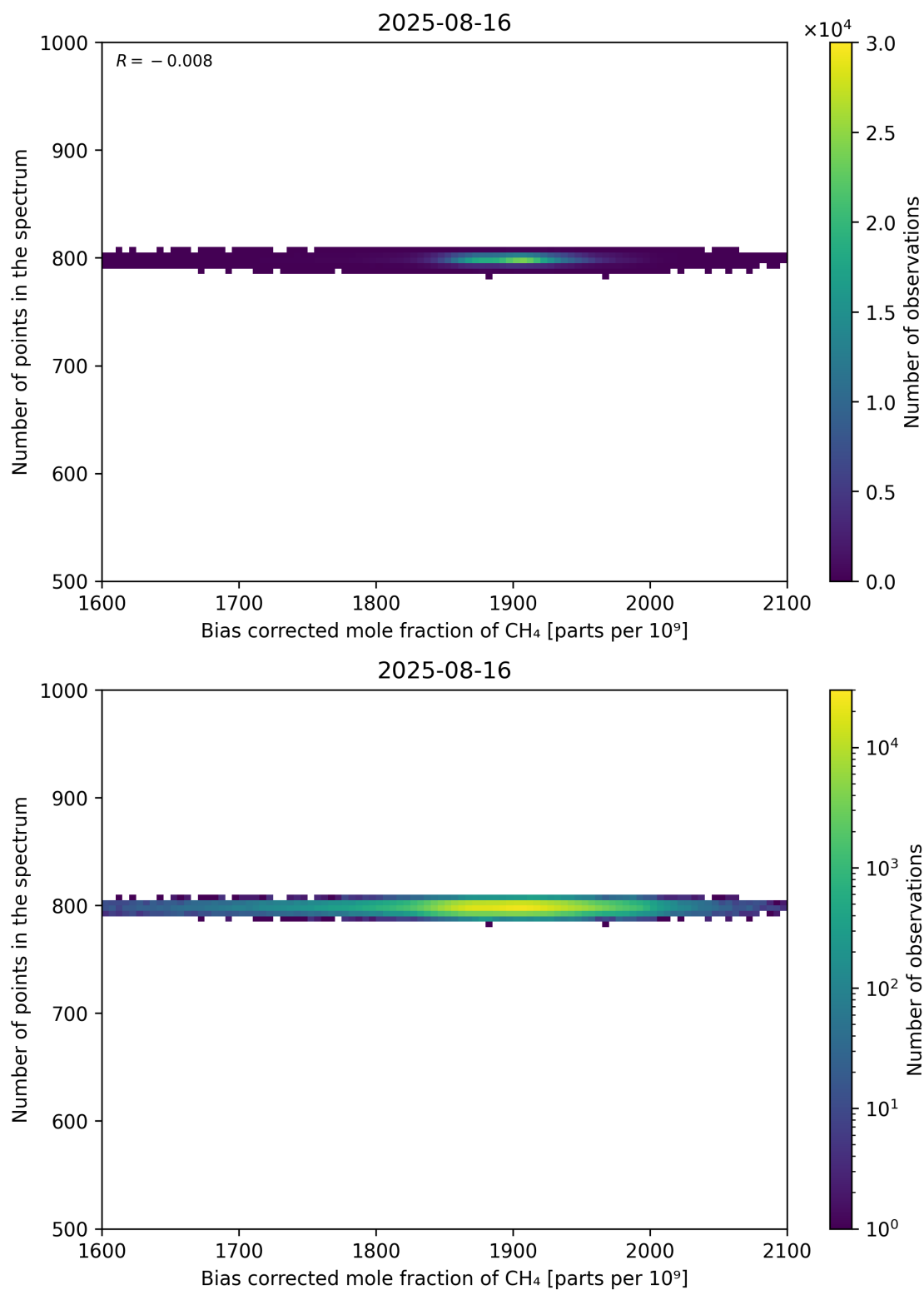
Figure 68: Scatter density plot of “Bias corrected mole fraction of CH 4 ” against “Number of points in the spectrum” for 2025-08-15 to 2025-08-17.
