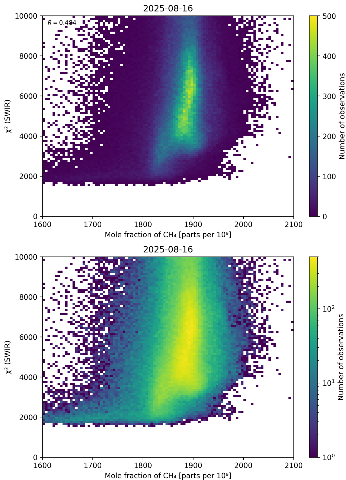
Figure 71: Scatter density plot of “Mole fraction of \text{CH}_4 ” against “ \chi^2 (SWIR)” for 2025-08-15 to 2025-08-17.
