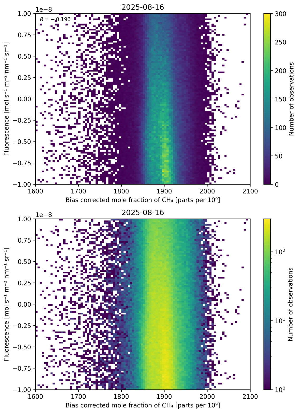
Figure 66: Scatter density plot of “Bias corrected mole fraction of \text{CH}_4 ” against “Fluorescence” for 2025-08-15 to 2025-08-17.
