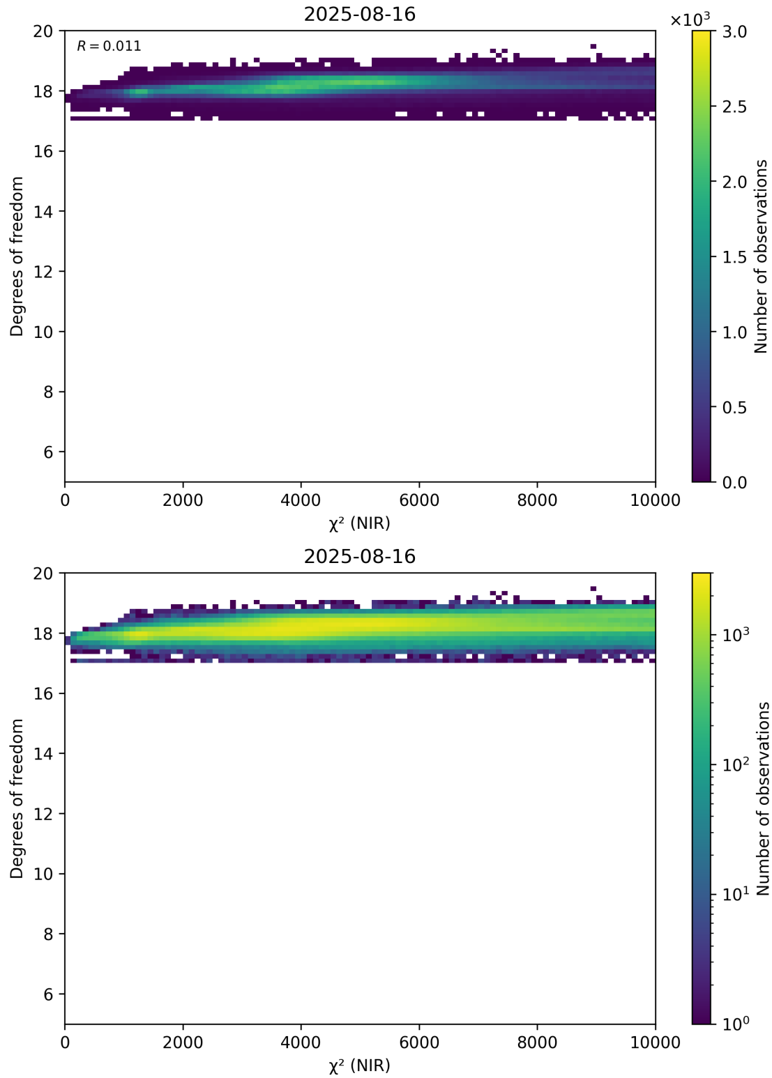
Figure 44: Scatter density plot of “ \chi^2 (NIR)” against “Degrees of freedom” for 2025-08-15 to 2025-08-17.
