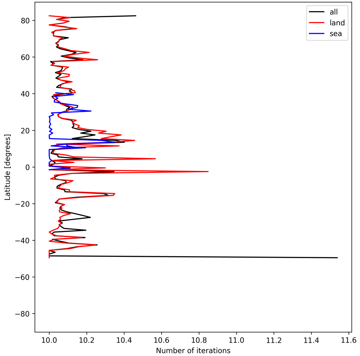
Figure 20: Zonal average of “Number of iterations” for 2025-08-15 to 2025-08-17.
