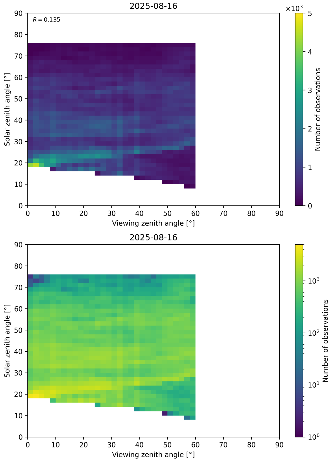
Figure 115: Scatter density plot of “Viewing zenith angle” against “Solar zenith angle” for 2025-08-15 to 2025-08-17.
