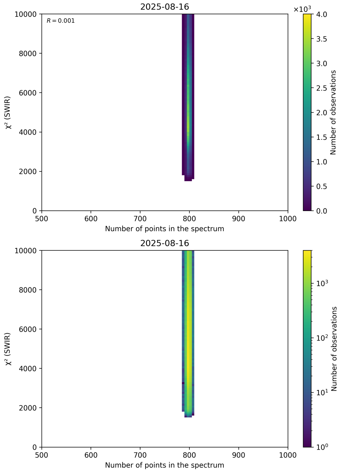
Figure 89: Scatter density plot of “Number of points in the spectrum” against “ \chi^2 (SWIR)” for 2025-08-15 to 2025-08-17.
