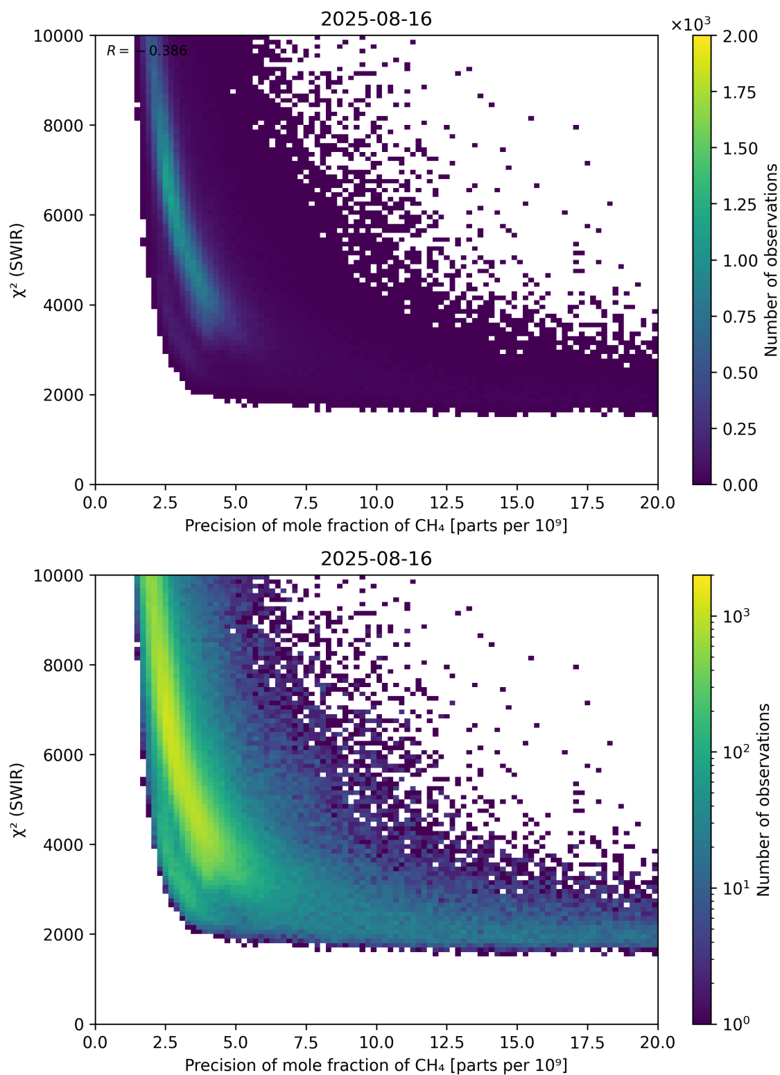
Figure 79: Scatter density plot of “Precision of mole fraction of \text{CH}_4 ” against “ \chi^2 (SWIR)” for 2025-08-15 to 2025-08-17.
