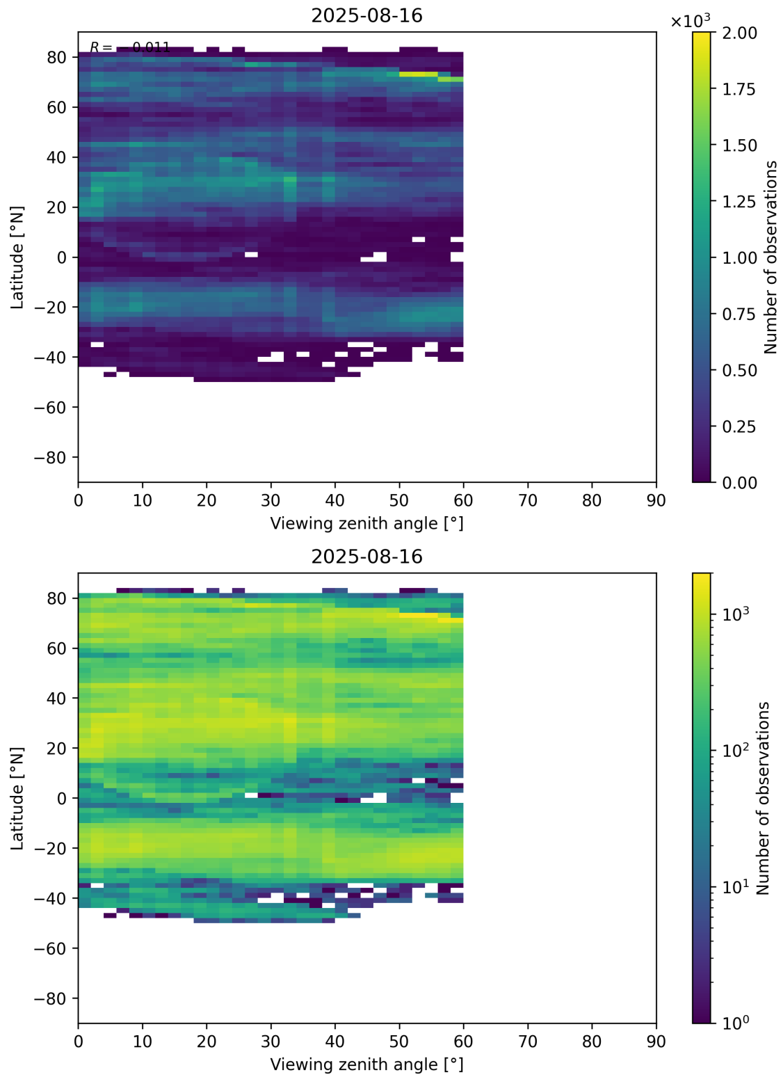
Figure 109: Scatter density plot of “Viewing zenith angle” against “Latitude” for 2025-08-15 to 2025-08-17.
