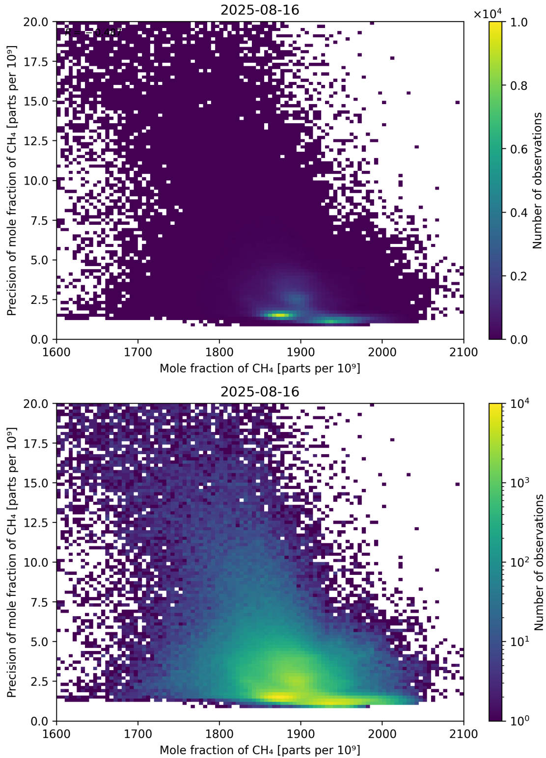
Figure 75: Scatter density plot of “Mole fraction of CH 4 ” against “Precision of mole fraction of CH 4 ” for 2025-08-15 to 2025-08-17.
