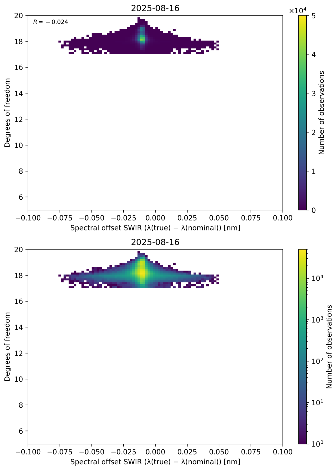
Figure 119: Scatter density plot of “Spectral offset SWIR ( \lambda_{\text{true}} - \lambda_{\text{nominal}} )” against “Degrees of freedom” for 2025-08-15 to 2025-08-17.
