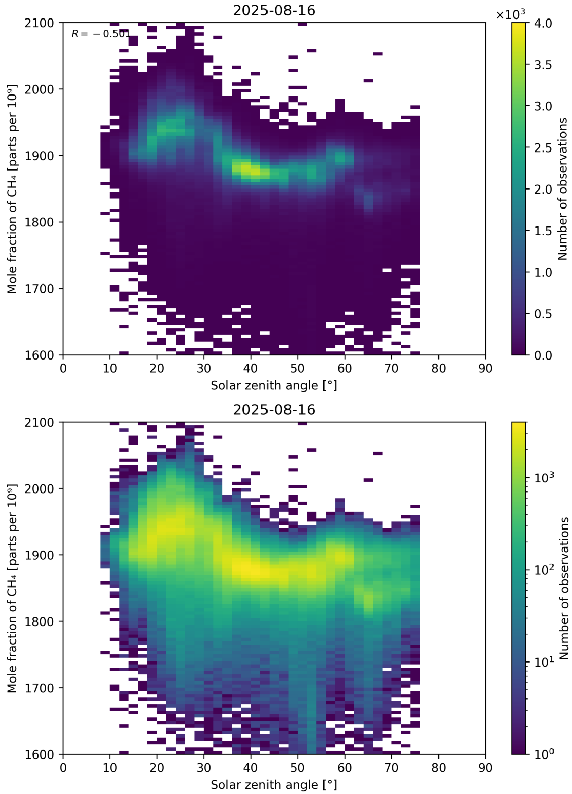
Figure 99: Scatter density plot of “Solar zenith angle” against “Mole fraction of CH 4 ” for 2025-08-15 to 2025-08-17.
