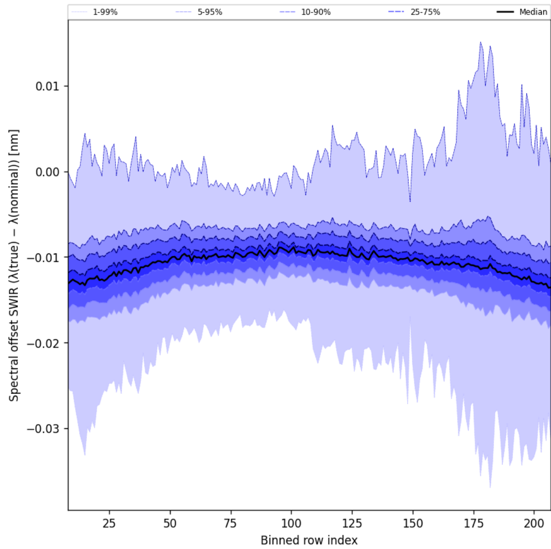
Figure 38: Along track statistics of “Spectral offset SWIR ( \lambda_{\text{true}} - \lambda_{\text{nominal}} )” for 2025-08-15 to 2025-08-17
