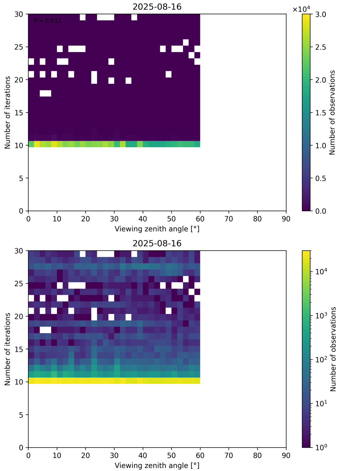
Figure 113: Scatter density plot of “Viewing zenith angle” against “Number of iterations” for 2025-08-15 to 2025-08-17.
