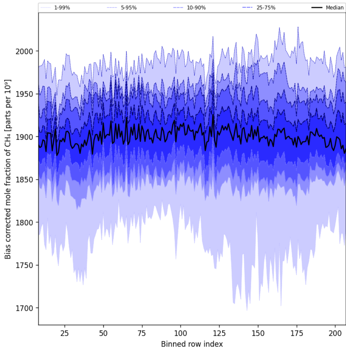
Figure 36: Along track statistics of “Bias corrected mole fraction of CH 4 ” for 2025-08-15 to 2025-08-17
