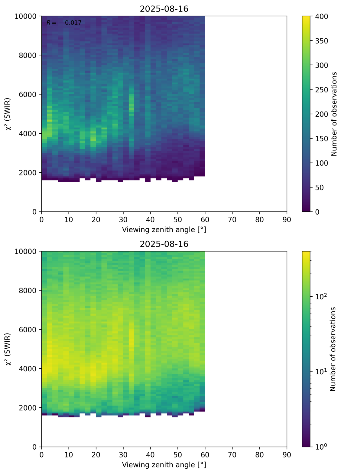
Figure 106: Scatter density plot of “Viewing zenith angle” against “ \chi^2 (SWIR)” for 2025-08-15 to 2025-08-17.
