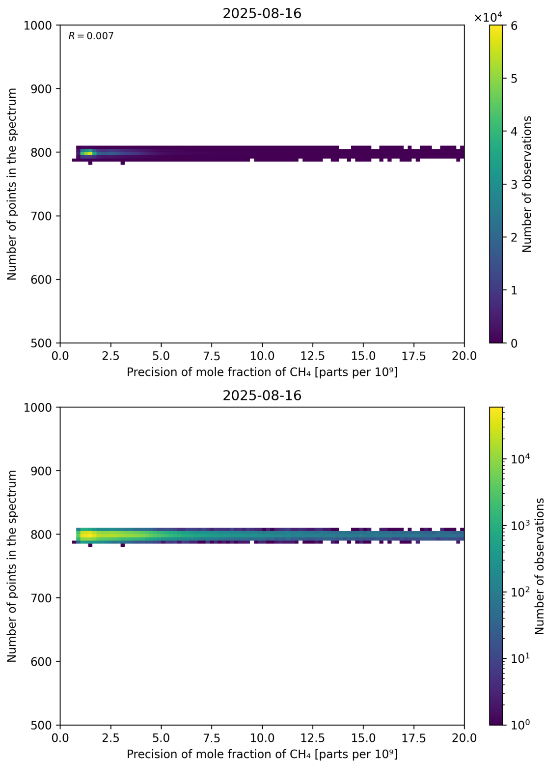
Figure 84: Scatter density plot of “Precision of mole fraction of CH 4 ” against “Number of points in the spectrum” for 2025-08-15 to 2025-08-17.
