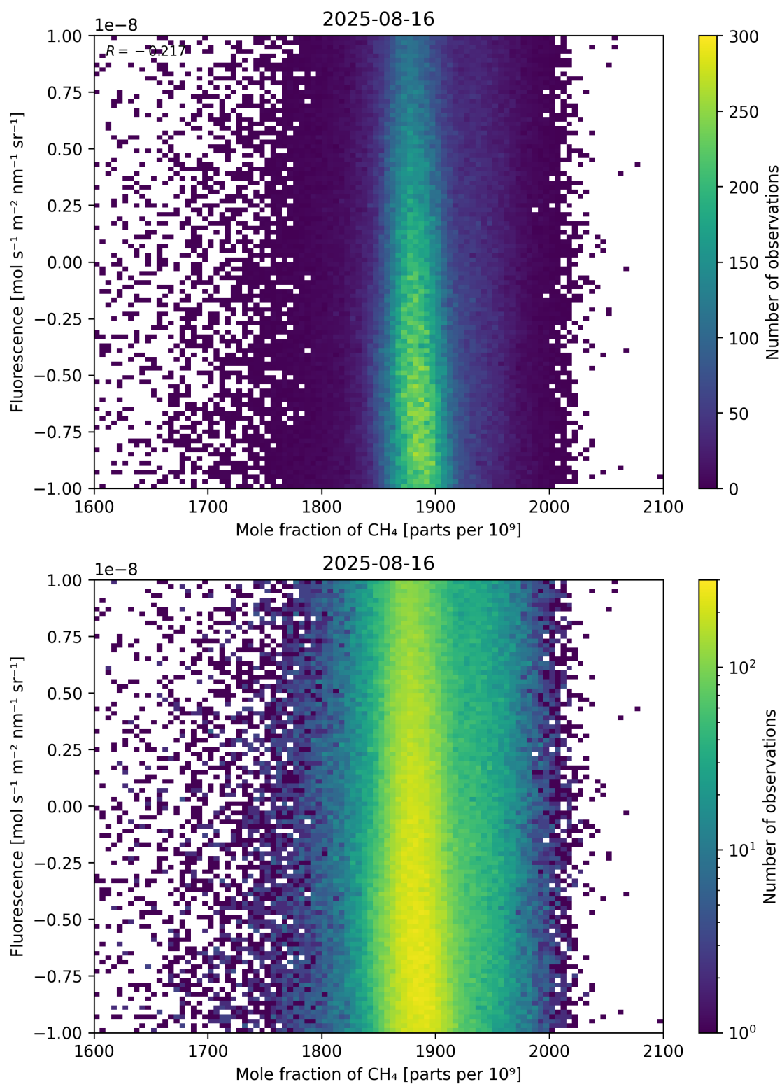
Figure 73: Scatter density plot of “Mole fraction of \text{CH}_4 ” against “Fluorescence” for 2025-08-15 to 2025-08-17.
