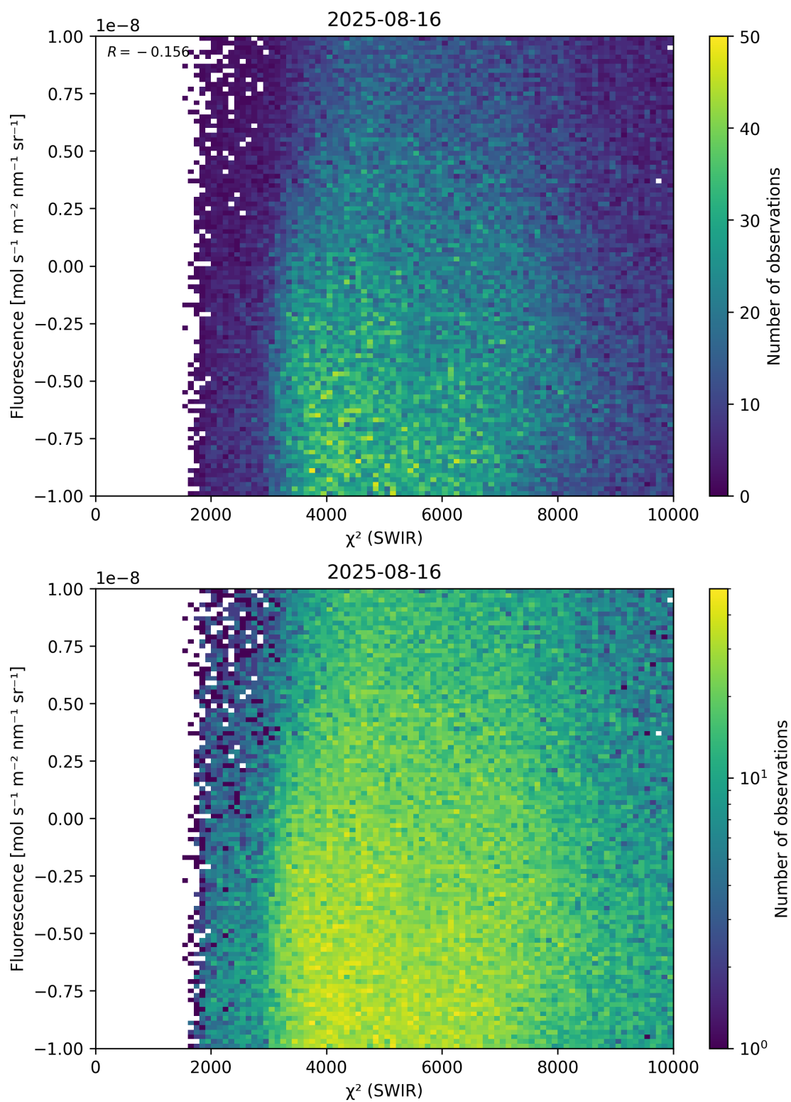
Figure 49: Scatter density plot of “ \chi^2 (SWIR)” against “Fluorescence” for 2025-08-15 to 2025-08-17.
