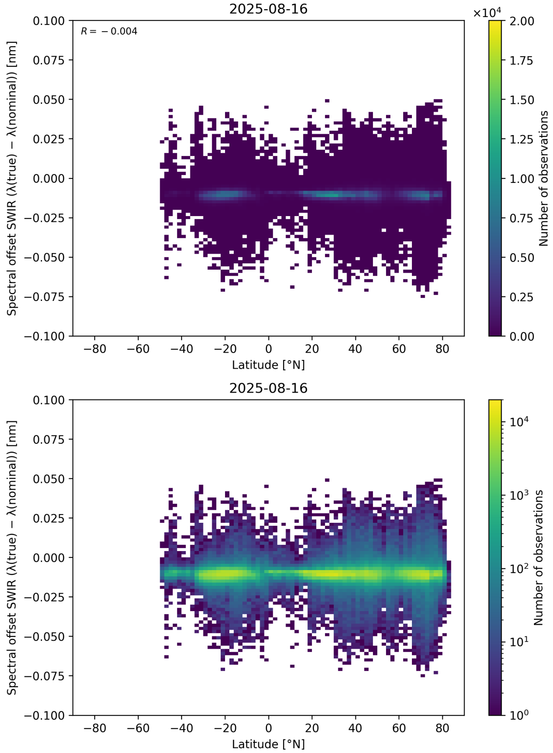
Figure 62: Scatter density plot of “Latitude” against “Spectral offset SWIR ( \lambda_{\text{true}} - \lambda_{\text{nominal}} )” for 2025-08-15 to 2025-08-17.
