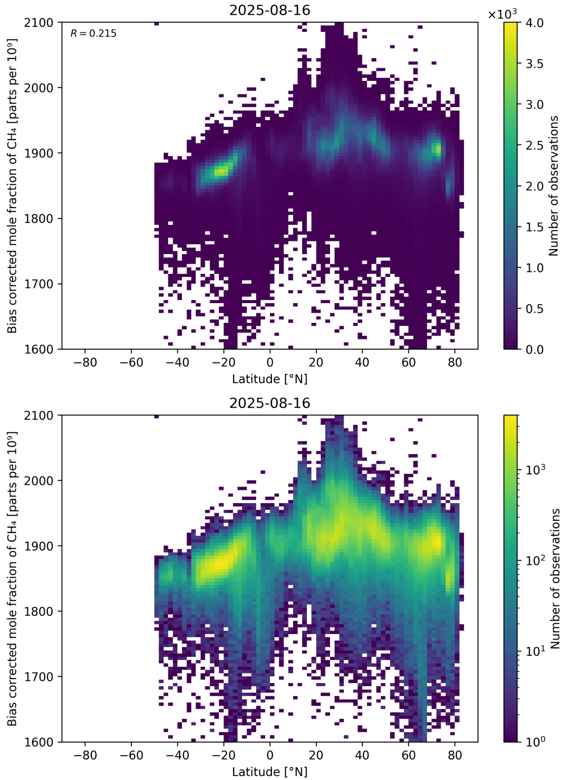
Figure 58: Scatter density plot of “Latitude” against “Bias corrected mole fraction of CH 4 ” for 2025-08-15 to 2025-08-17.
