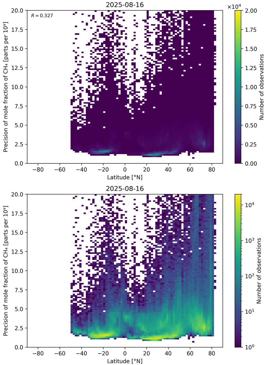
Figure 59: Scatter density plot of “Latitude” against “Precision of mole fraction of \text{CH}_4 ” for 2025-08-15 to 2025-08-17.
