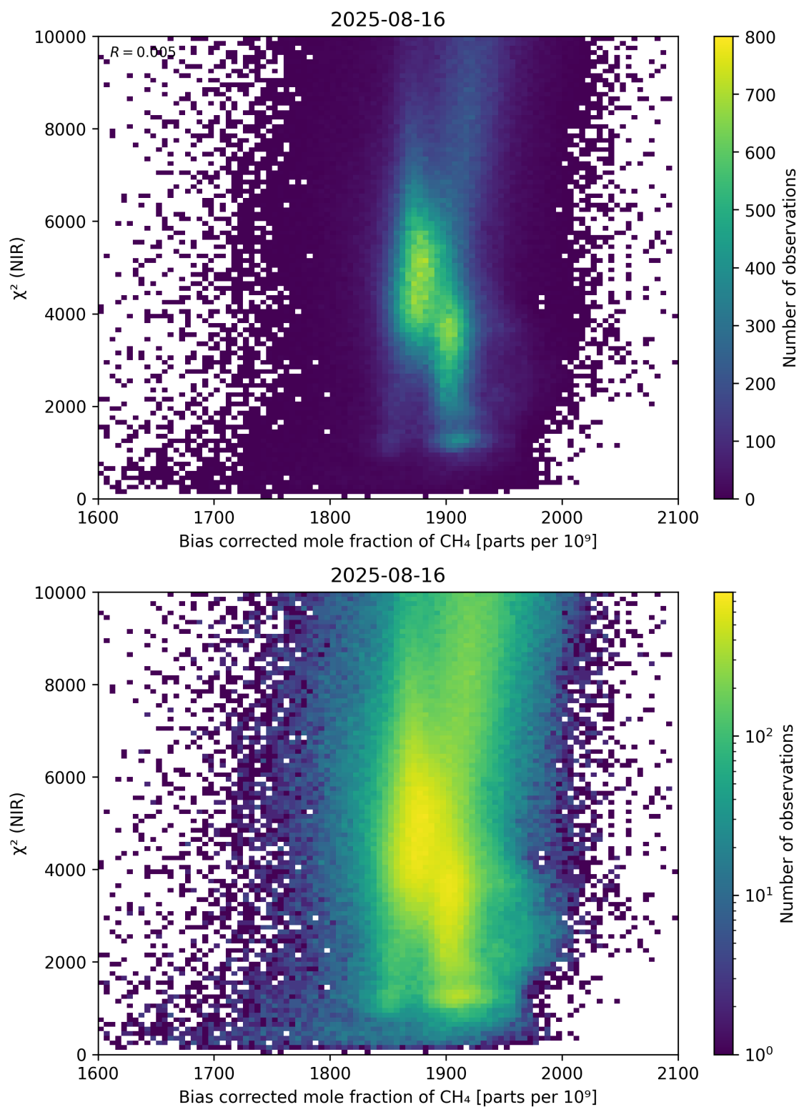
Figure 63: Scatter density plot of “Bias corrected mole fraction of CH 4 ” against “ \chi^2 (NIR)” for 2025-08-15 to 2025-08-17.
