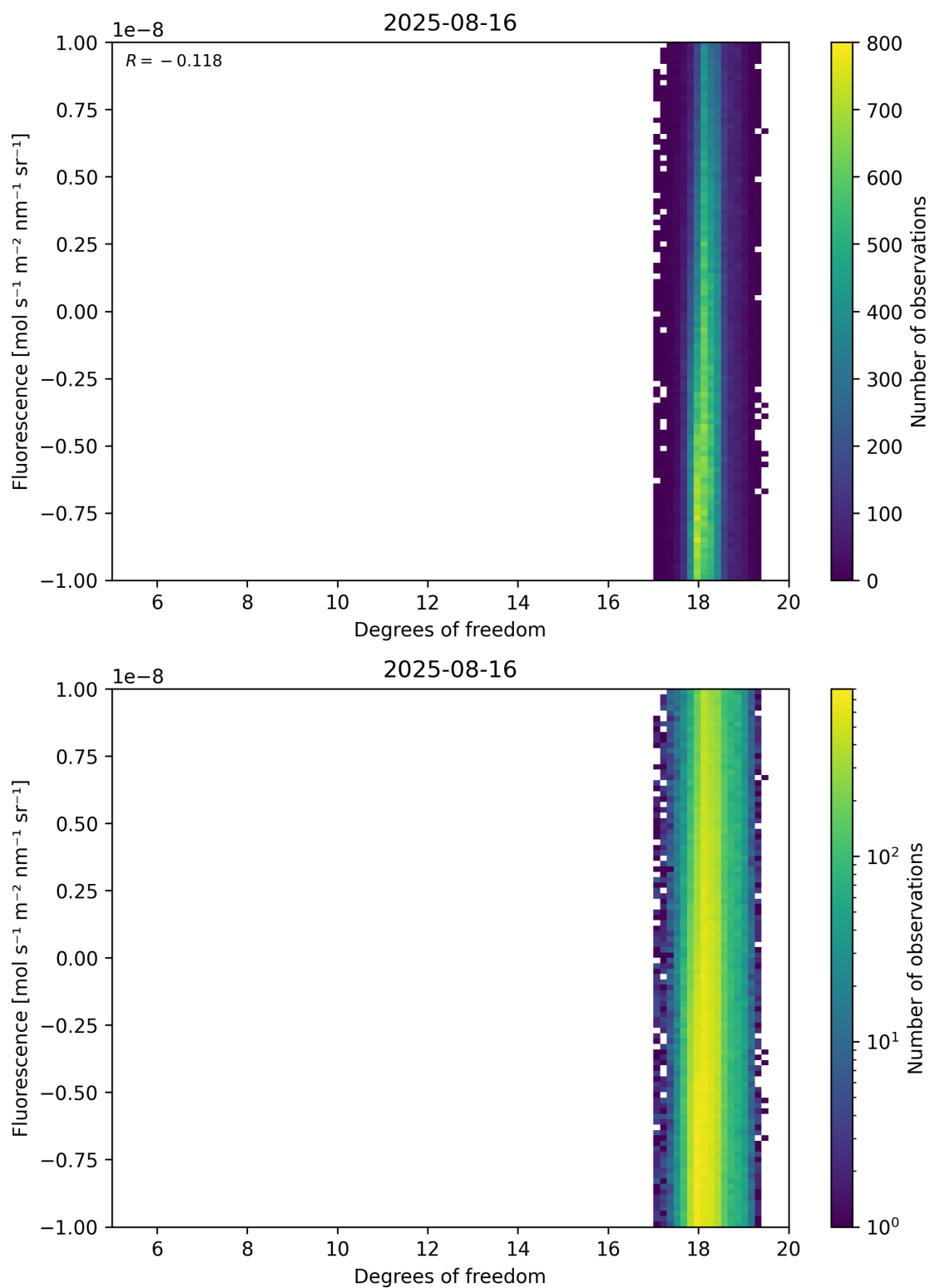
Figure 51: Scatter density plot of “Degrees of freedom” against “Fluorescence” for 2025-08-15 to 2025-08-17.
