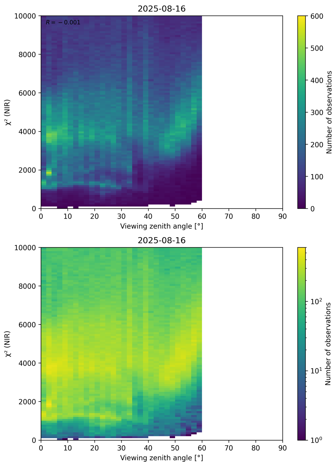
Figure 105: Scatter density plot of “Viewing zenith angle” against “ \chi^2 (NIR)” for 2025-08-15 to 2025-08-17.
