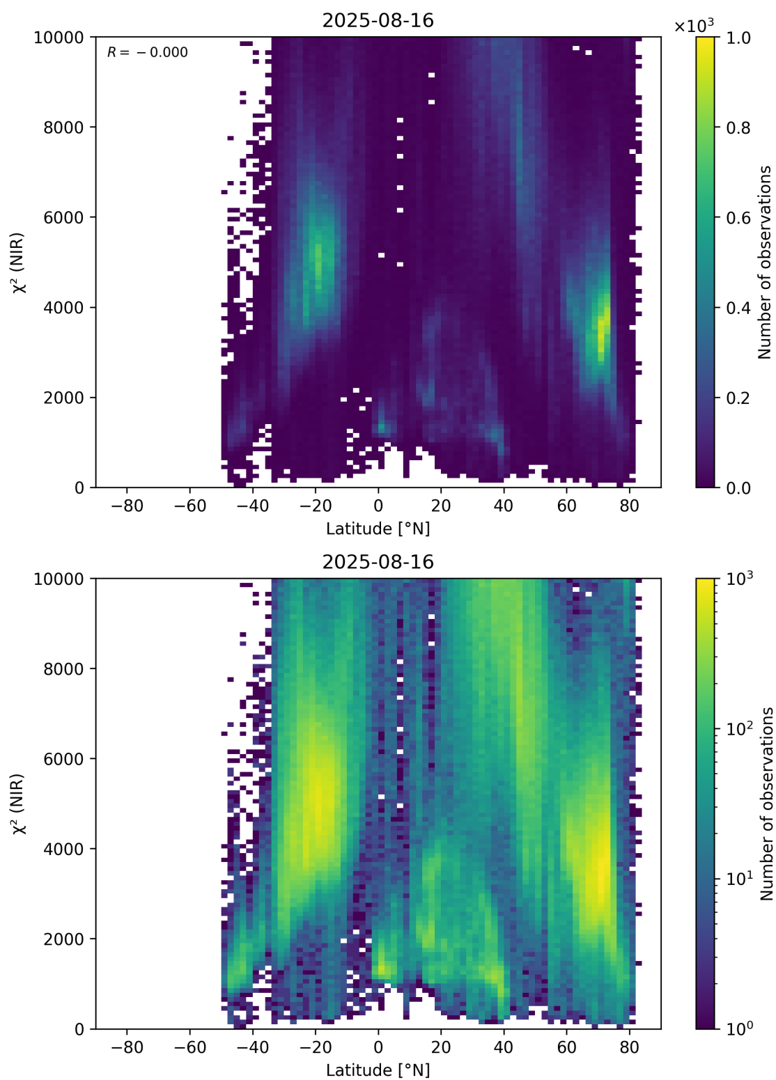
Figure 53: Scatter density plot of “Latitude” against “ \chi^2 (NIR)” for 2025-08-15 to 2025-08-17.
