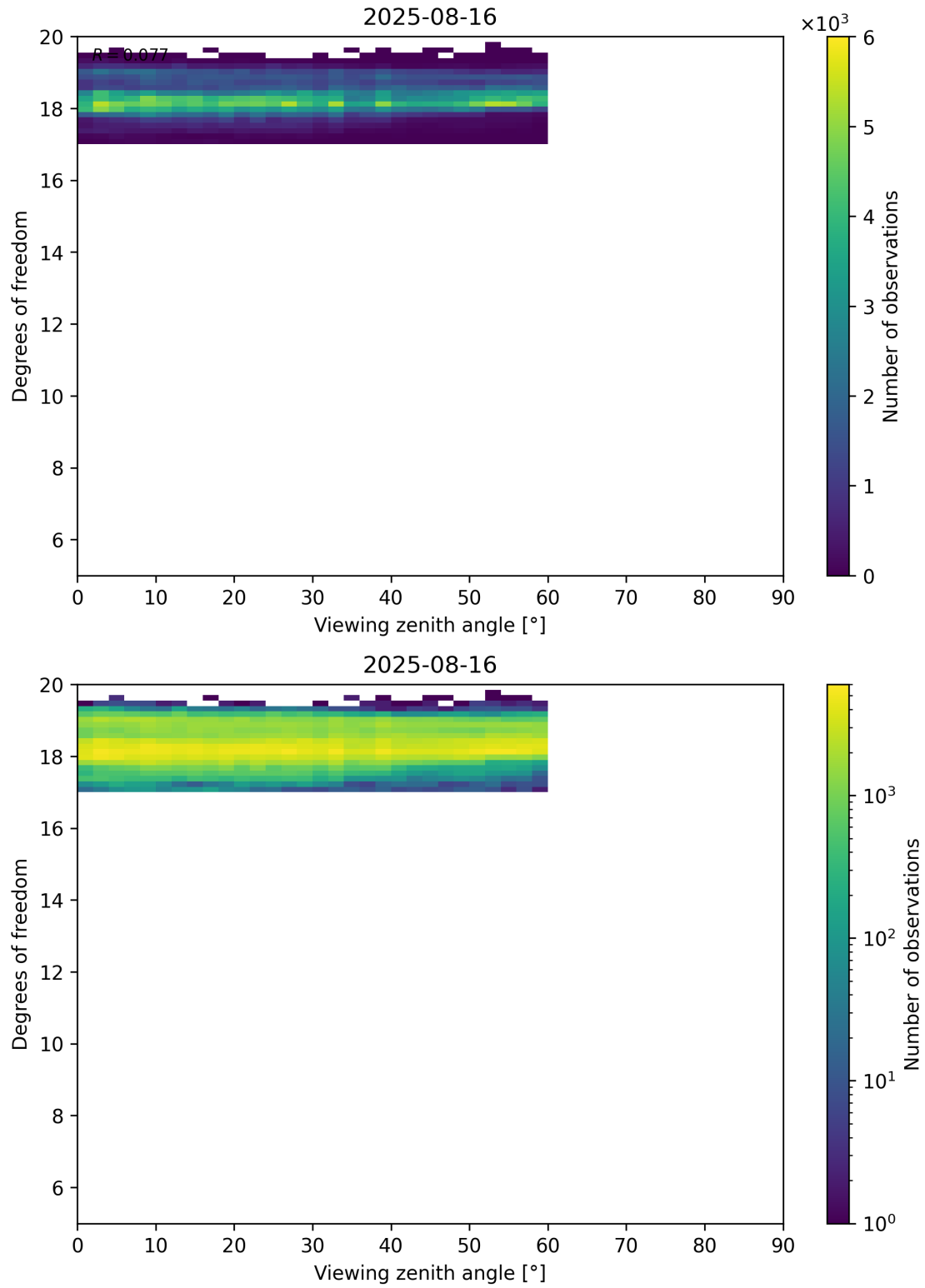
Figure 107: Scatter density plot of “Viewing zenith angle” against “Degrees of freedom” for 2025-08-15 to 2025-08-17.
