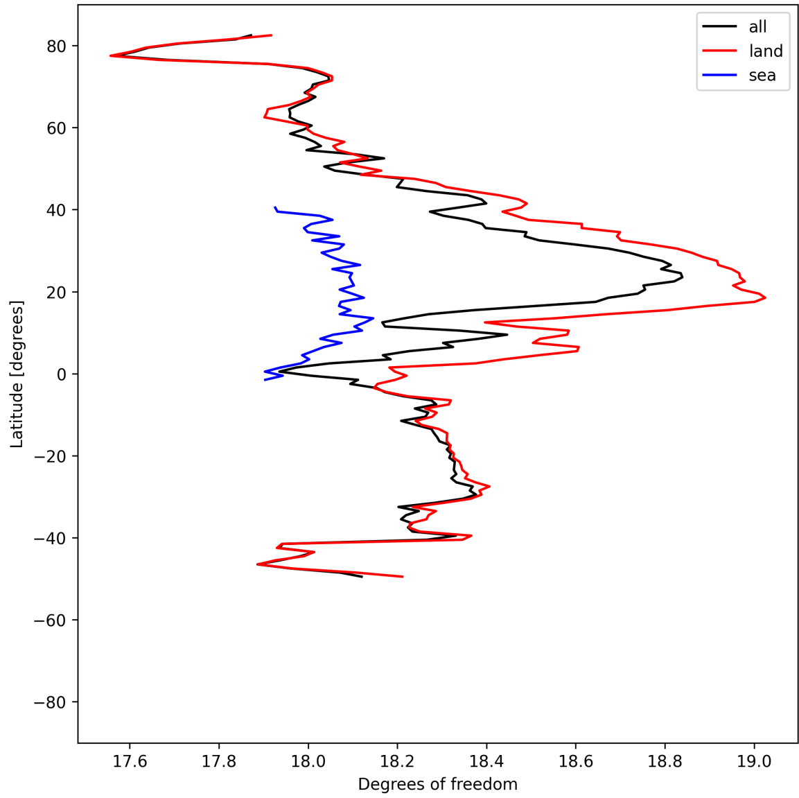
Figure 19: Zonal average of “Degrees of freedom” for 2025-08-15 to 2025-08-17.
