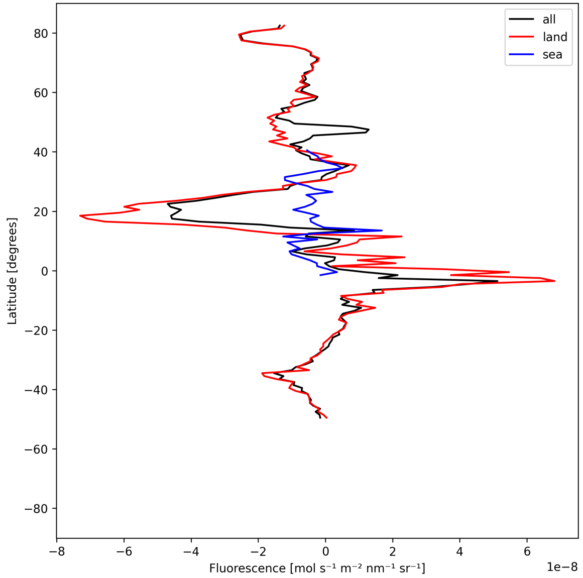
Figure 21: Zonal average of “Fluorescence” for 2025-08-15 to 2025-08-17.
