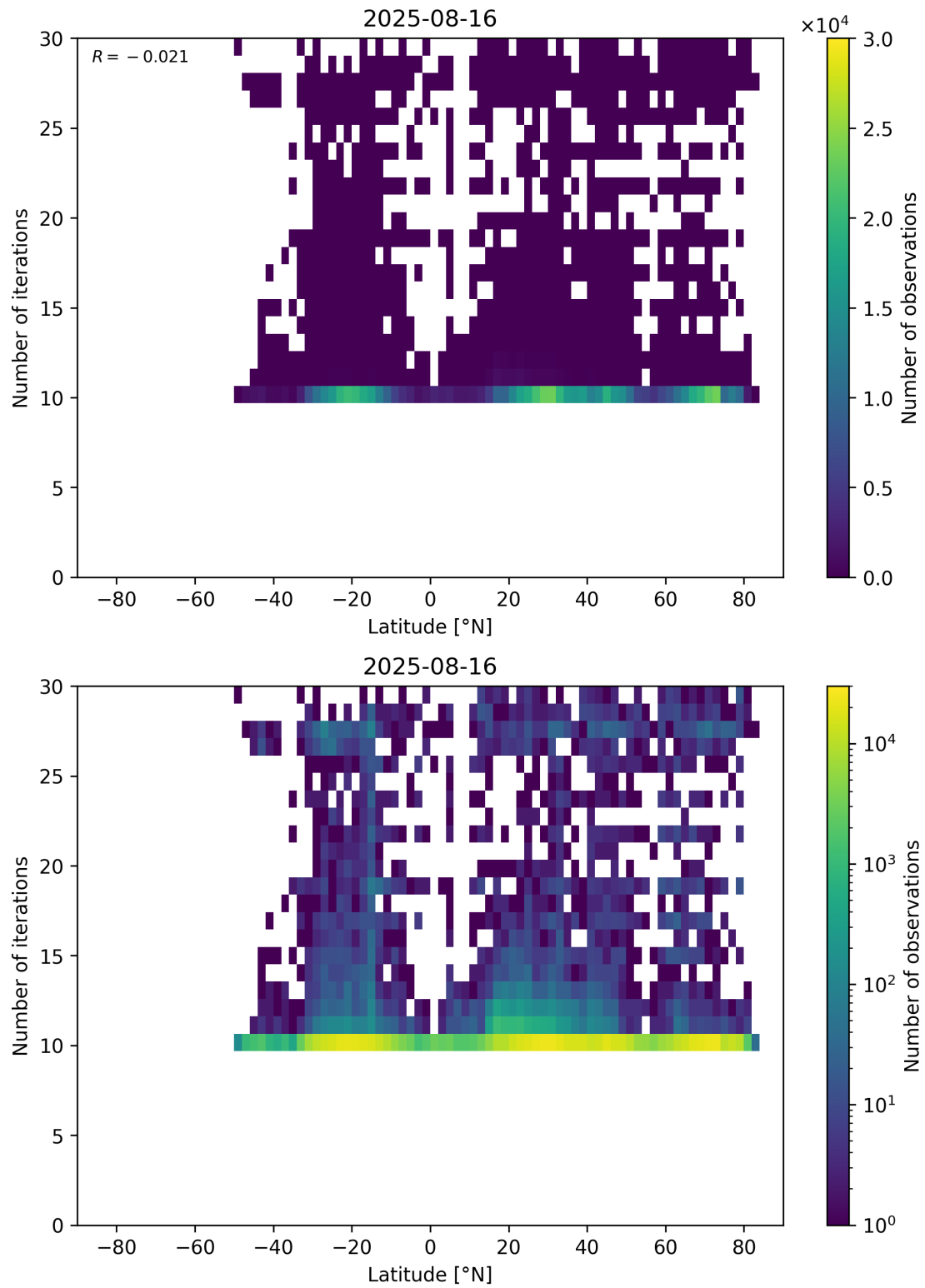
Figure 60: Scatter density plot of “Latitude” against “Number of iterations” for 2025-08-15 to 2025-08-17.
