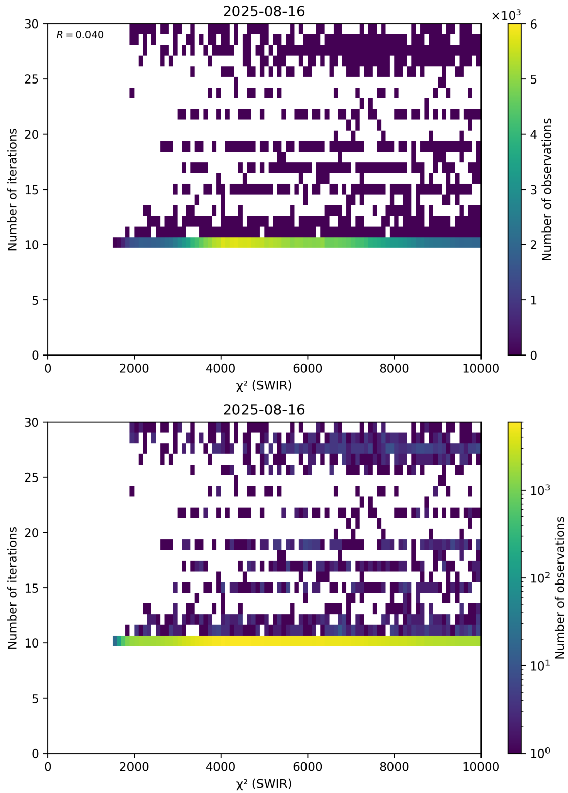
Figure 50: Scatter density plot of “ \chi^2 (SWIR)” against “Number of iterations” for 2025-08-15 to 2025-08-17.
