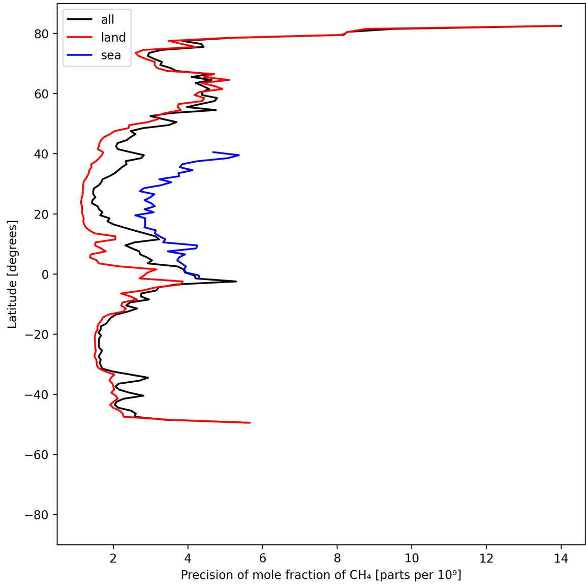
Figure 13: Zonal average of “Precision of mole fraction of CH 4 ” for 2025-08-15 to 2025-08-17.
