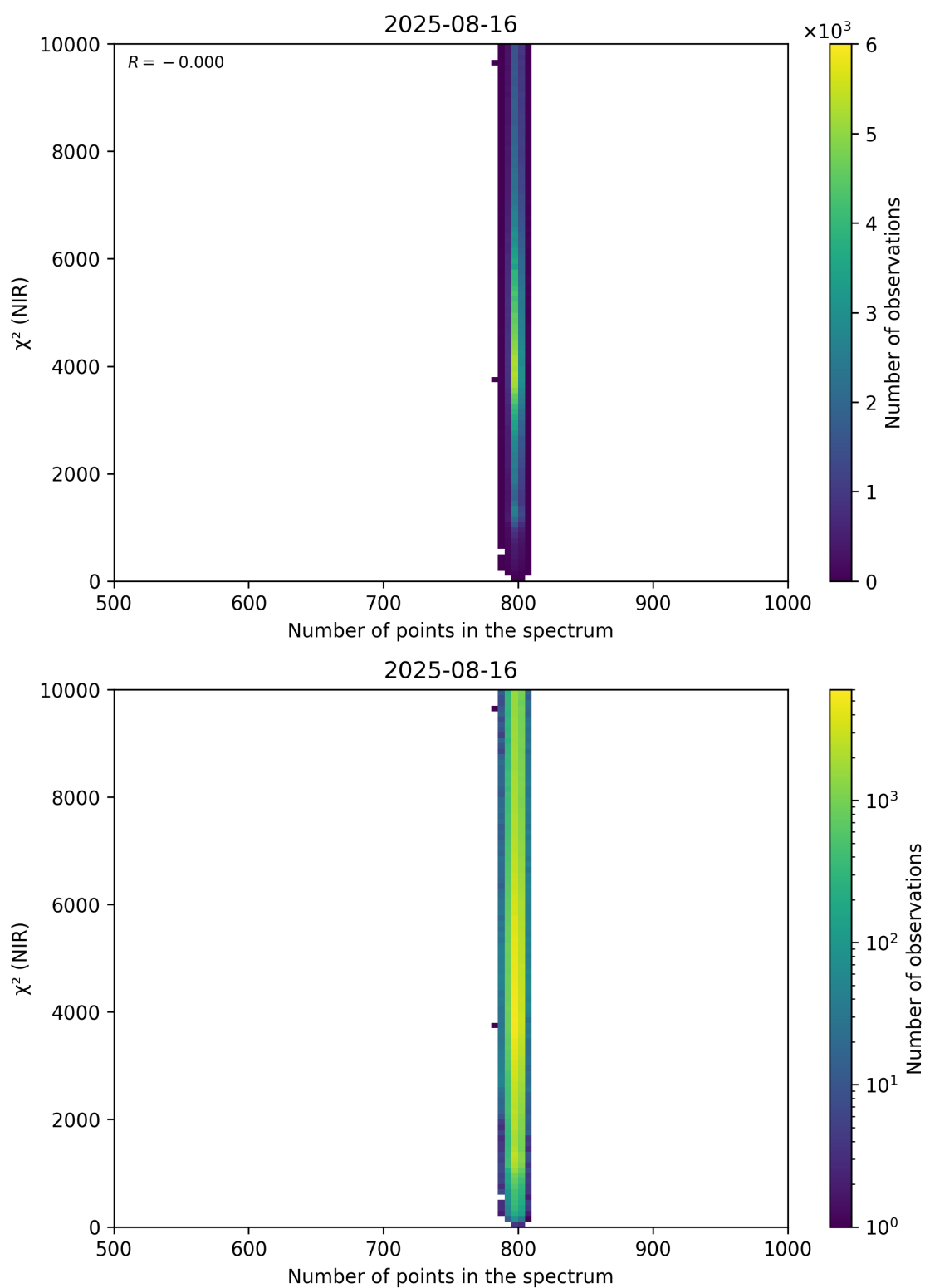
Figure 88: Scatter density plot of “Number of points in the spectrum” against “ \chi^2 (NIR)” for 2025-08-15 to 2025-08-17.
