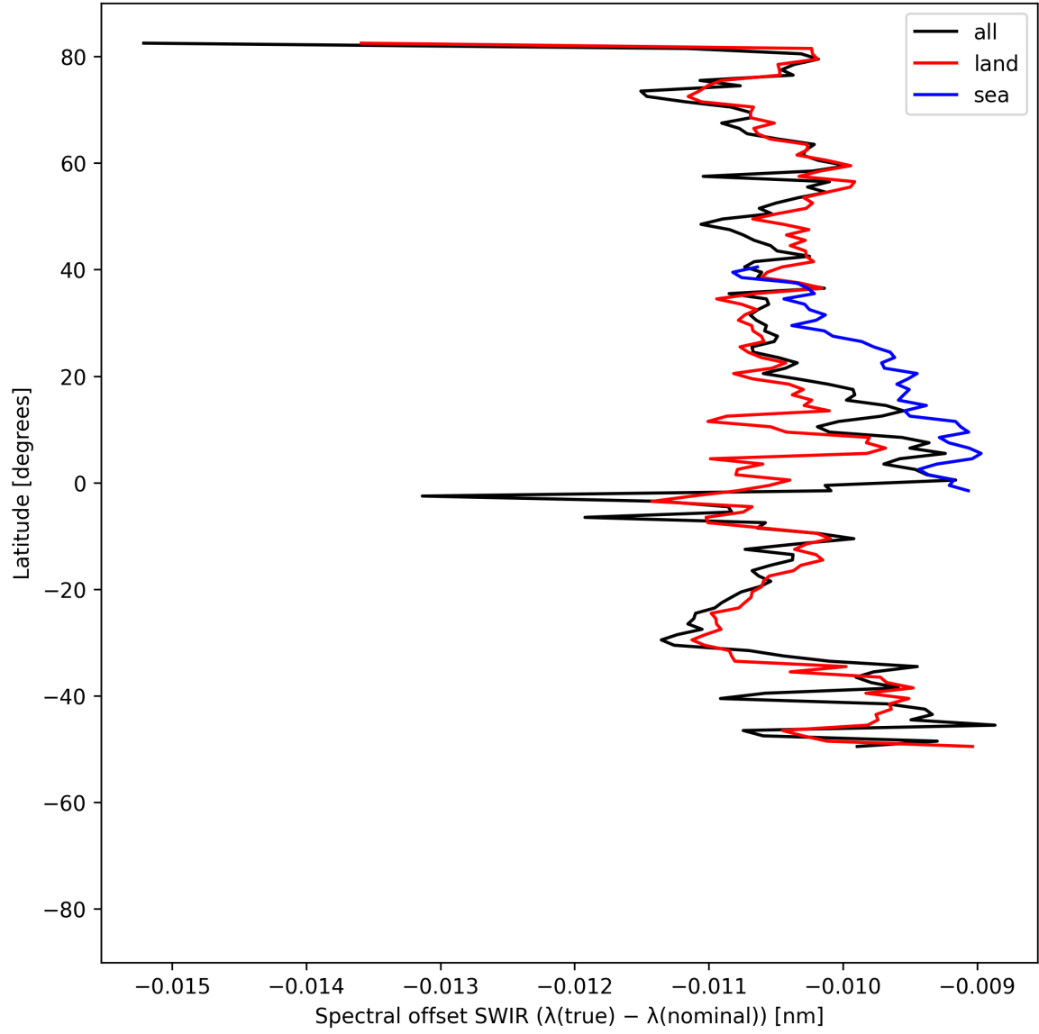
Figure 16: Zonal average of “Spectral offset SWIR ( \lambda_{\text{true}} - \lambda_{\text{nominal}} )” for 2025-08-15 to 2025-08-17.
