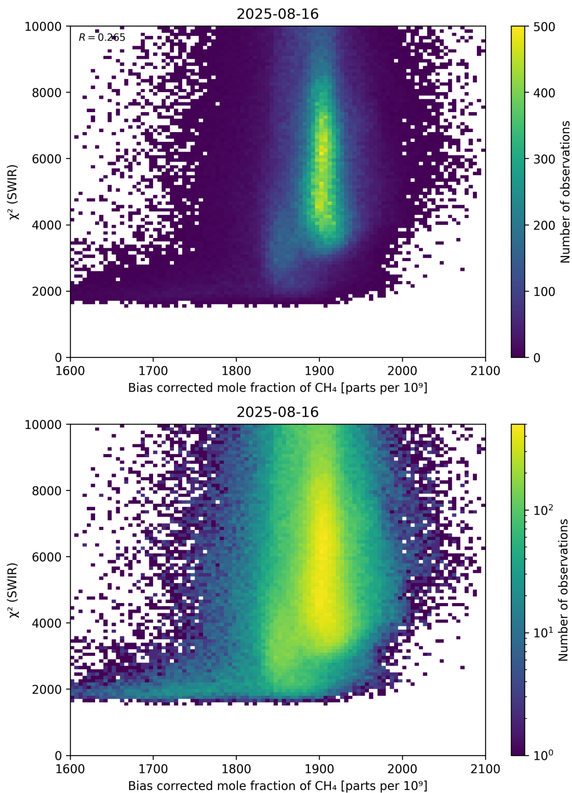
Figure 64: Scatter density plot of “Bias corrected mole fraction of \text{CH}_4 ” against “ \chi^2 (SWIR)” for 2025-08-15 to 2025-08-17.
