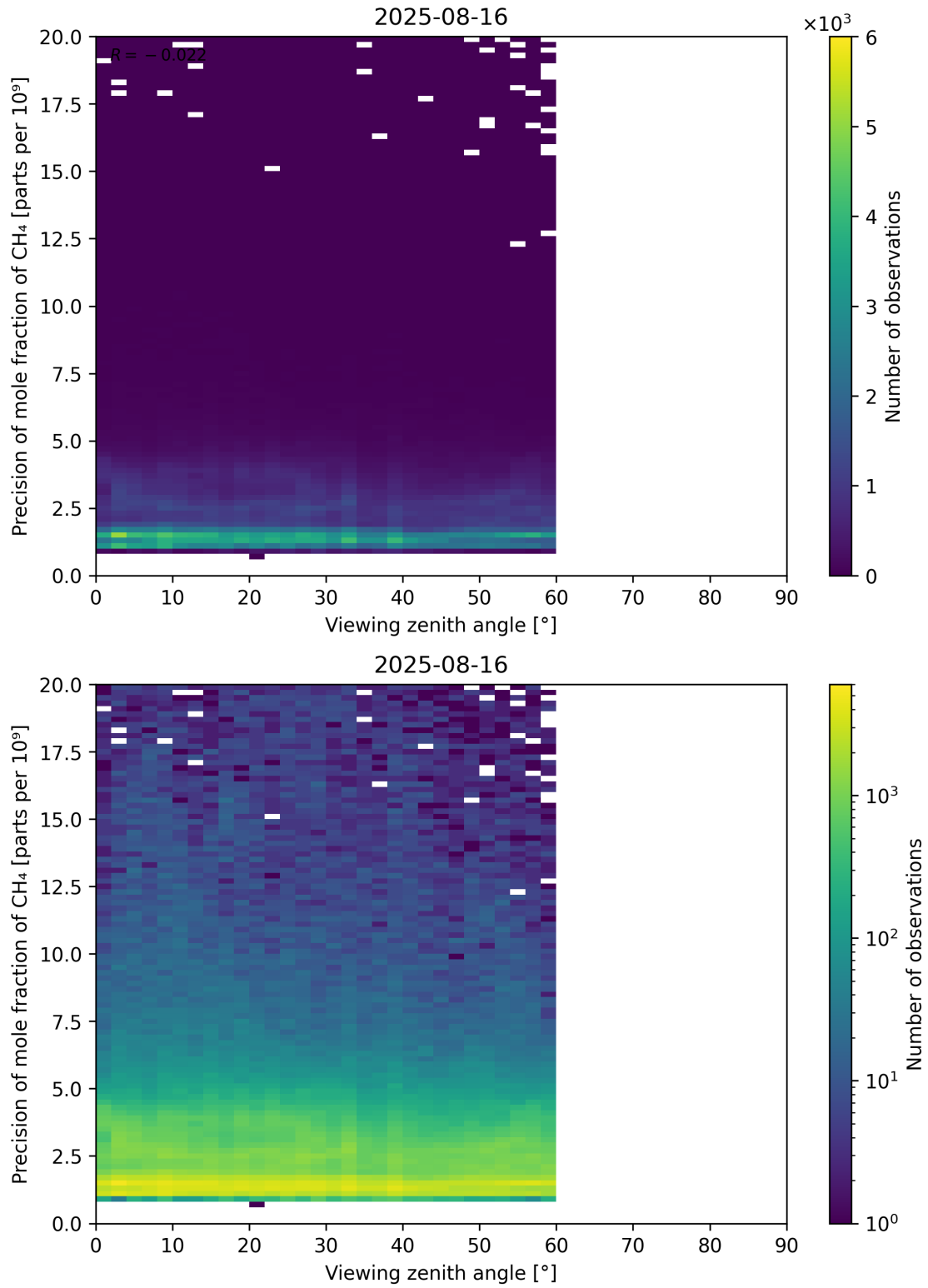
Figure 112: Scatter density plot of “Viewing zenith angle” against “Precision of mole fraction of CH 4 ” for 2025-08-15 to 2025-08-17.
