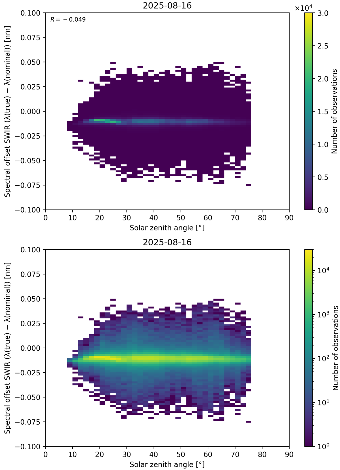
Figure 104: Scatter density plot of “Solar zenith angle” against “Spectral offset SWIR ( \lambda_{\text{true}} - \lambda_{\text{nominal}} )” for 2025-08-15 to 2025-08-17.
