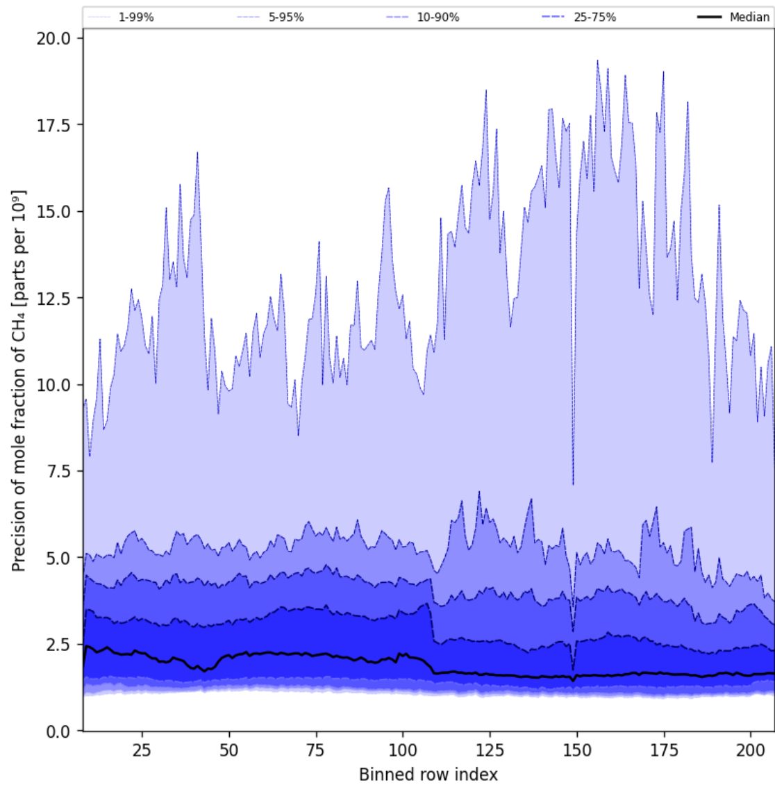
Figure 35: Along track statistics of “Precision of mole fraction of CH 4 ” for 2025-08-15 to 2025-08-17
