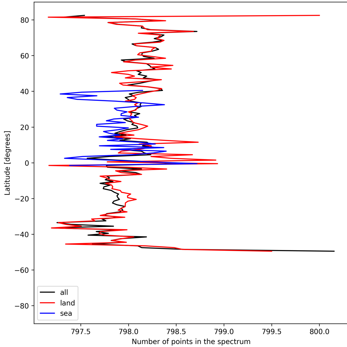
Figure 15: Zonal average of “Number of points in the spectrum” for 2025-08-15 to 2025-08-17.
