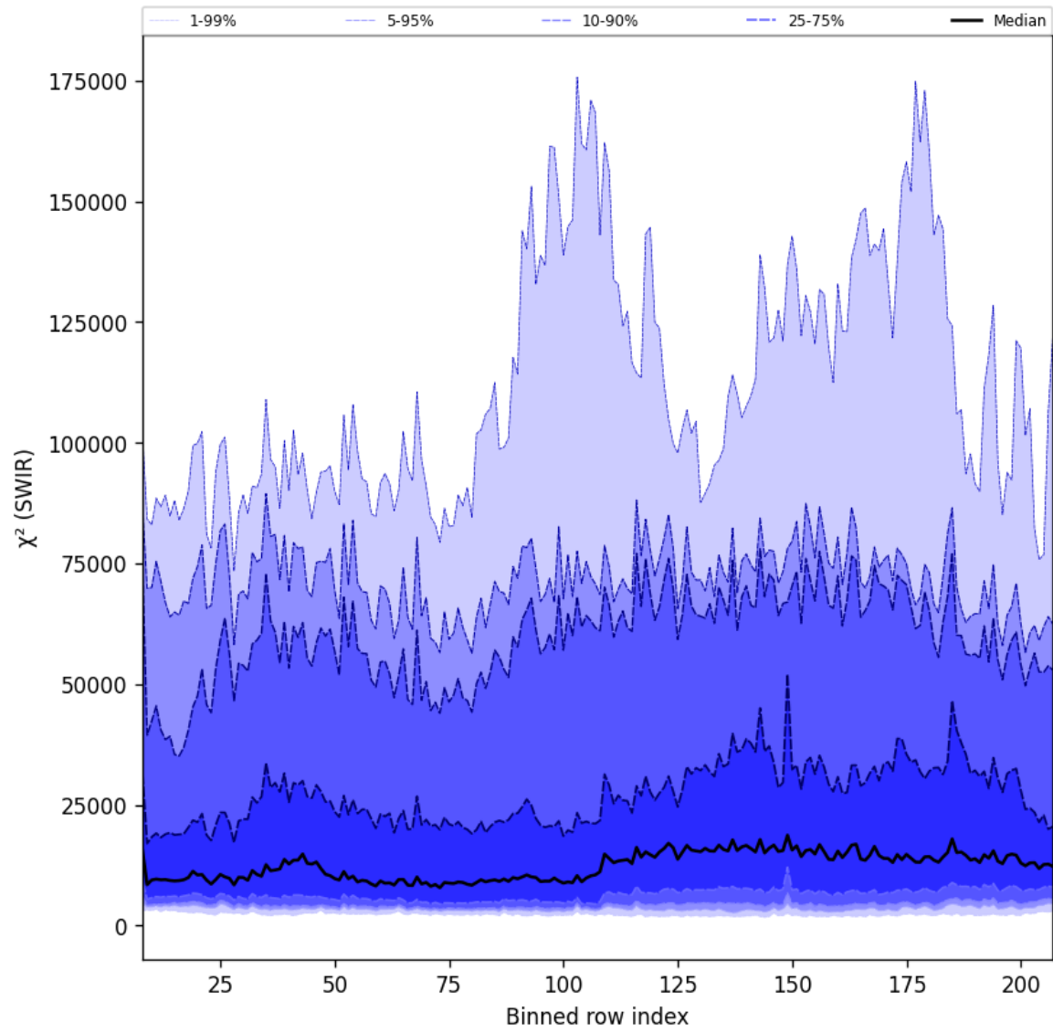
Figure 39: Along track statistics of “ \chi^2 (SWIR)” for 2025-08-15 to 2025-08-17
