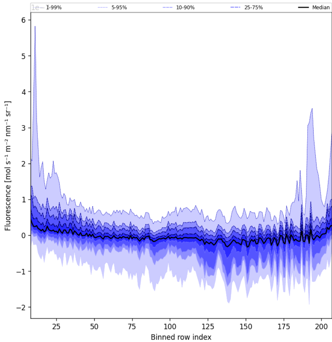
Figure 43: Along track statistics of “Fluorescence” for 2025-08-15 to 2025-08-17
