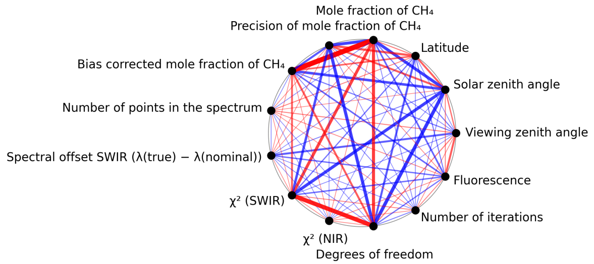
Figure 1: Map of correlation graph for 2025-08-15 to 2025-08-17.
