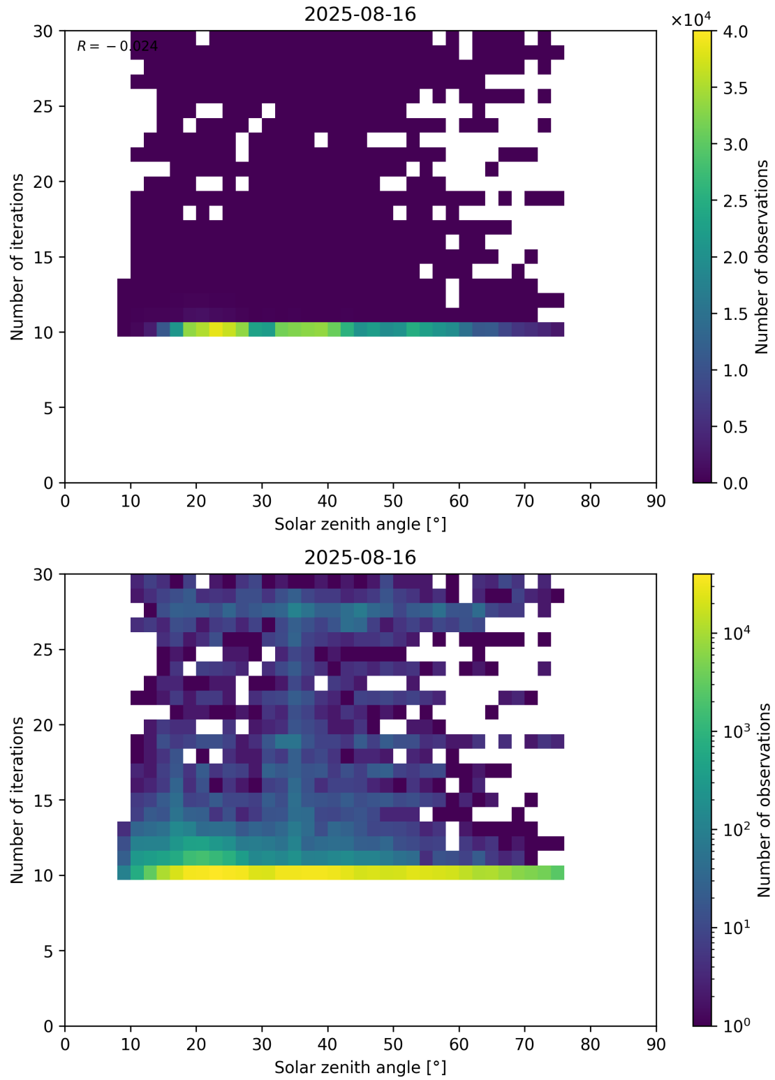
Figure 102: Scatter density plot of “Solar zenith angle” against “Number of iterations” for 2025-08-15 to 2025-08-17.
