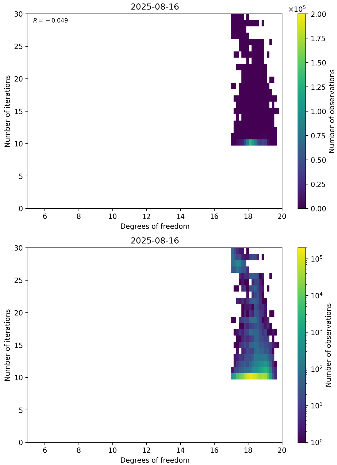
Figure 52: Scatter density plot of “Degrees of freedom” against “Number of iterations” for 2025-08-15 to 2025-08-17.
