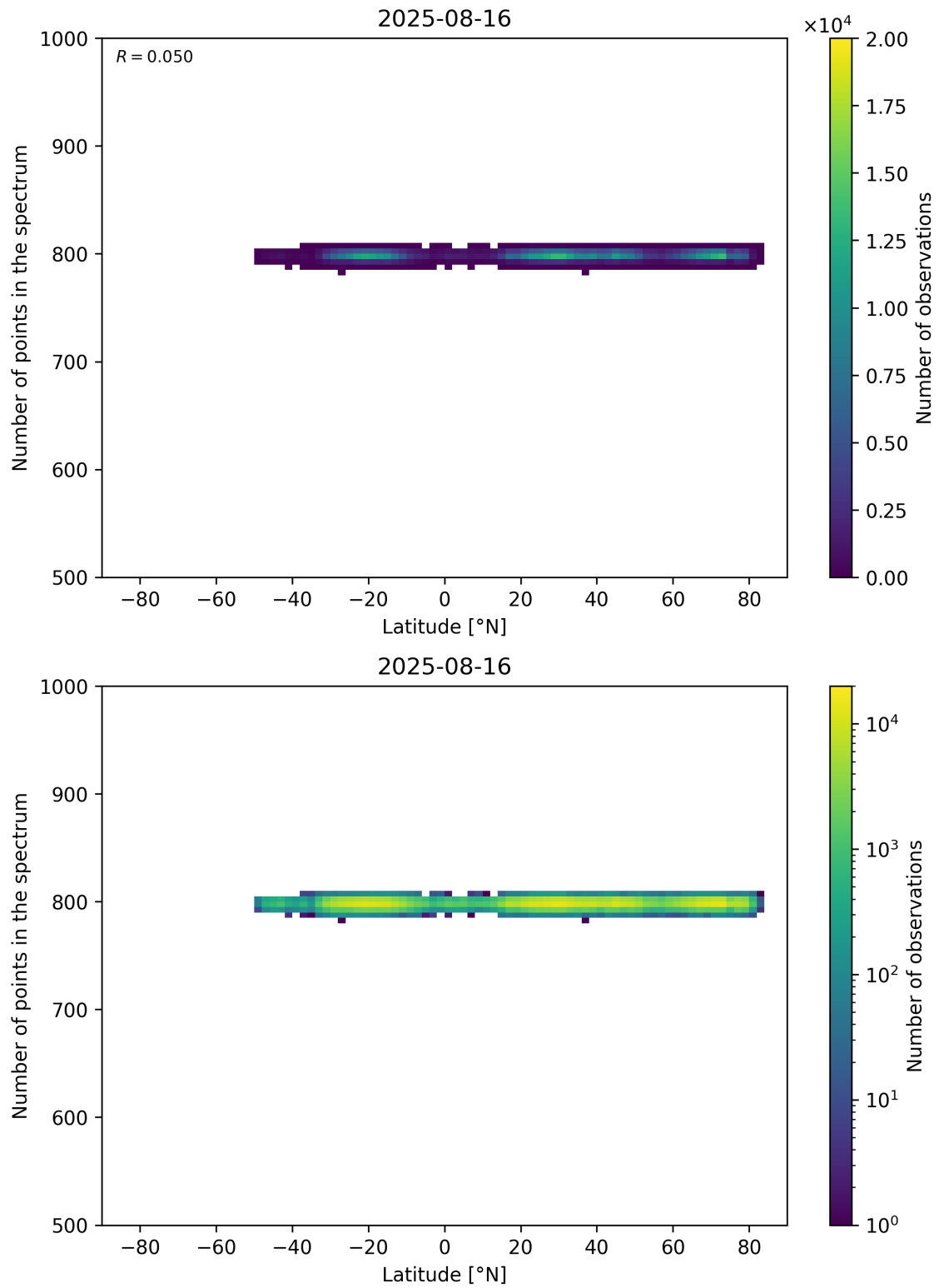
Figure 61: Scatter density plot of “Latitude” against “Number of points in the spectrum” for 2025-08-15 to 2025-08-17.
