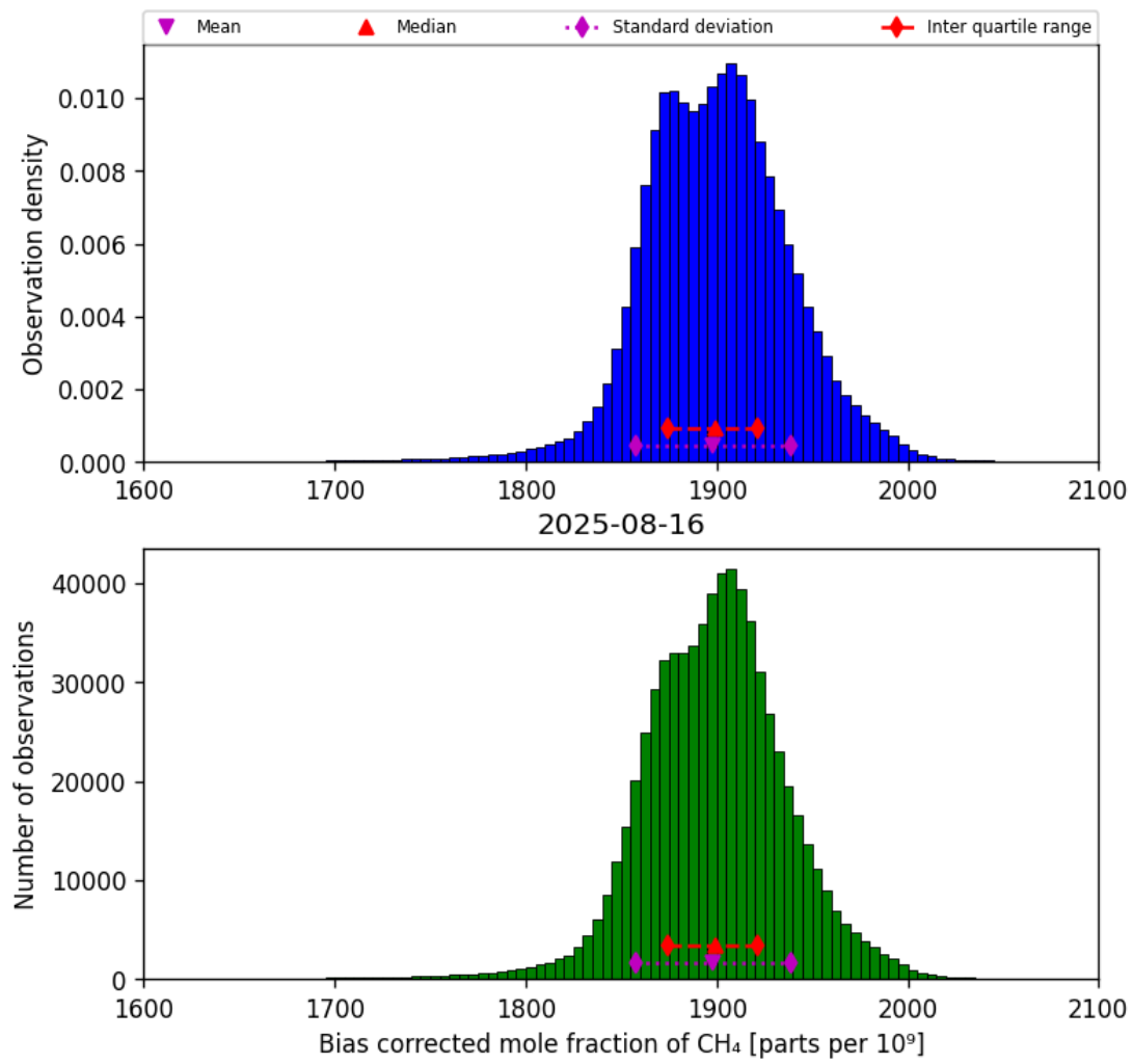
Figure 25: Histogram of “Bias corrected mole fraction of CH 4 ” for 2025-08-15 to 2025-08-17
