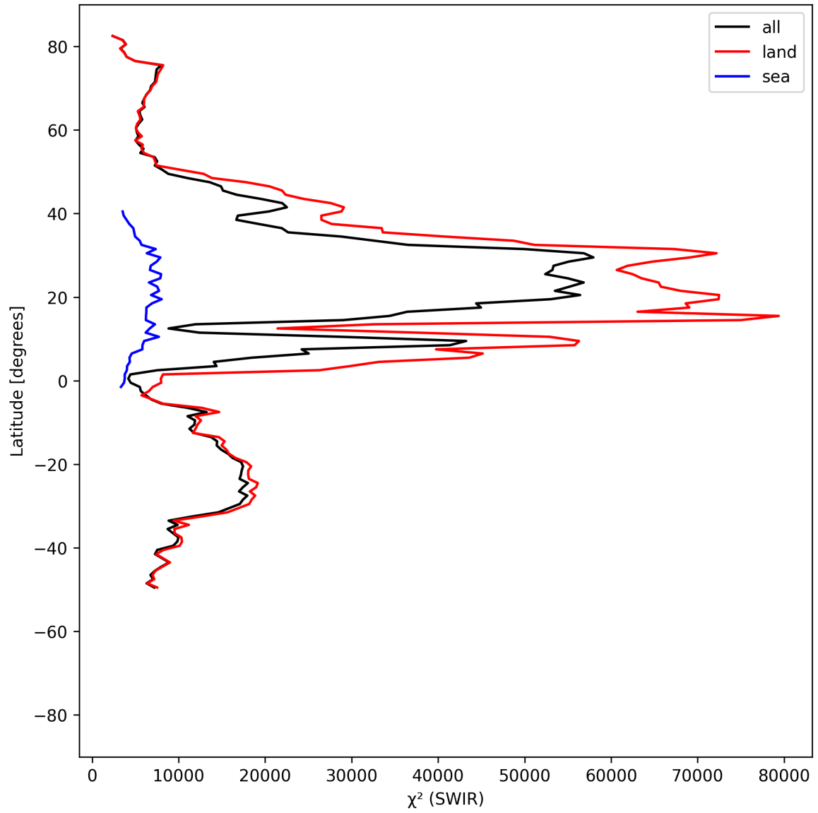
Figure 17: Zonal average of “ \chi^2 (SWIR)” for 2025-08-15 to 2025-08-17.
