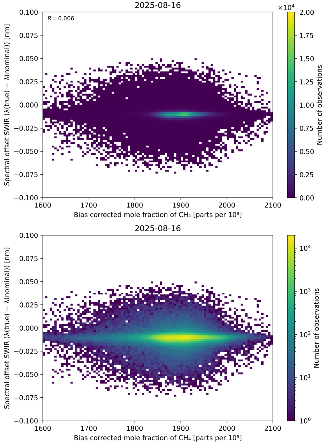
Figure 69: Scatter density plot of “Bias corrected mole fraction of \text{CH}_4 ” against “Spectral offset SWIR ( \lambda_{\text{true}} - \lambda_{\text{nominal}} )” for 2025-08-15 to 2025-08-17.
