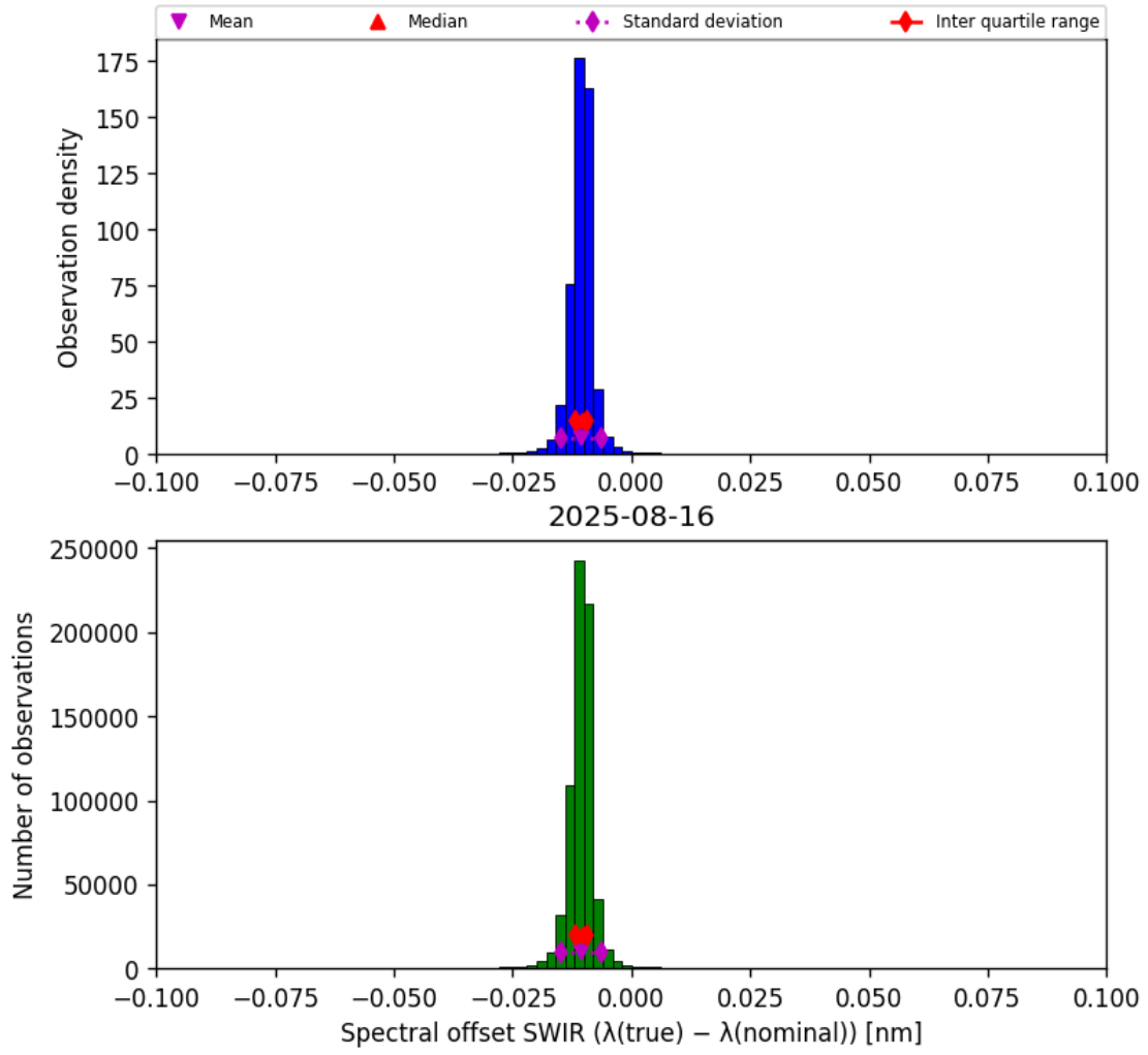
Figure 27: Histogram of “Spectral offset SWIR ( \lambda_{\text{true}} - \lambda_{\text{nominal}} )” for 2025-08-15 to 2025-08-17
