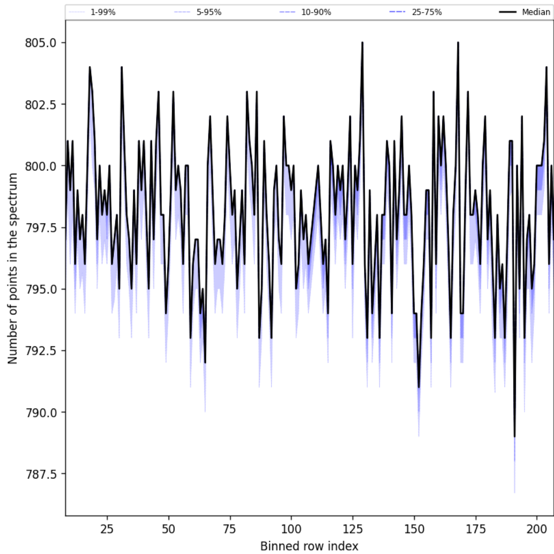
Figure 37: Along track statistics of “Number of points in the spectrum” for 2025-08-15 to 2025-08-17
