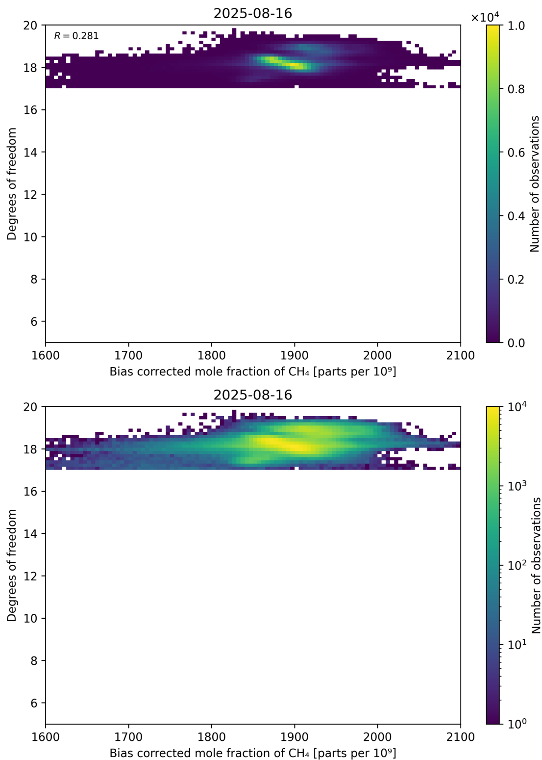
Figure 65: Scatter density plot of “Bias corrected mole fraction of CH 4 ” against “Degrees of freedom” for 2025-08-15 to 2025-08-17.
