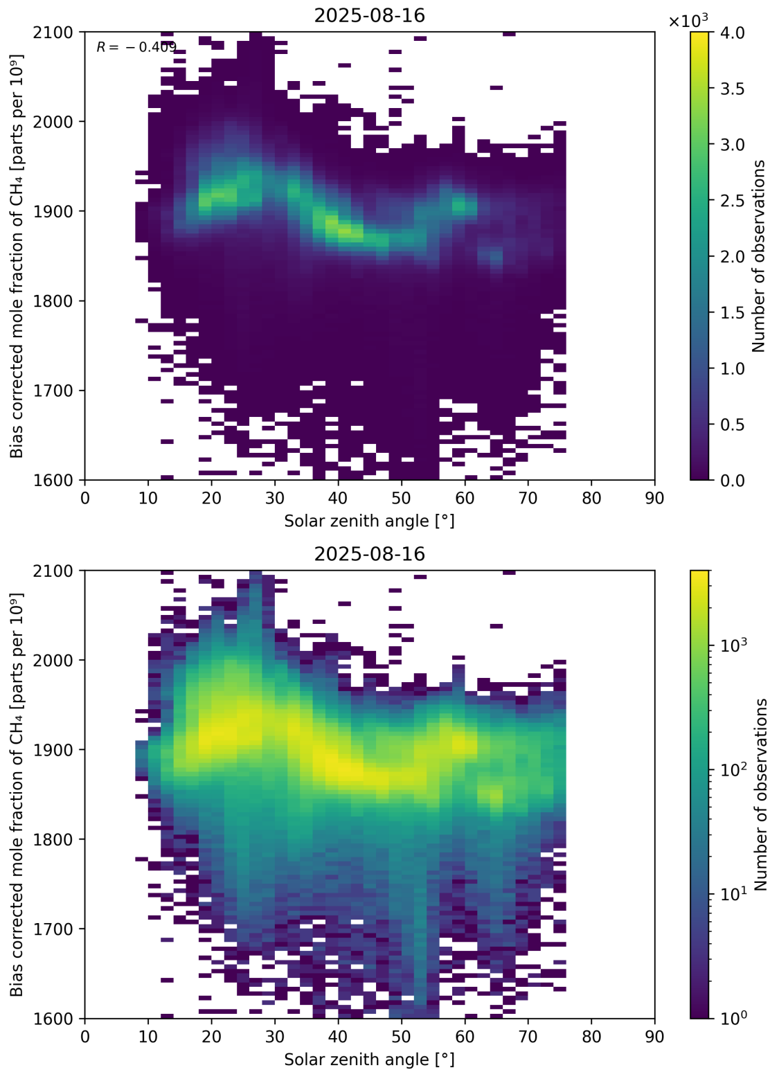
Figure 100: Scatter density plot of “Solar zenith angle” against “Bias corrected mole fraction of CH 4 ” for 2025-08-15 to 2025-08-17.
