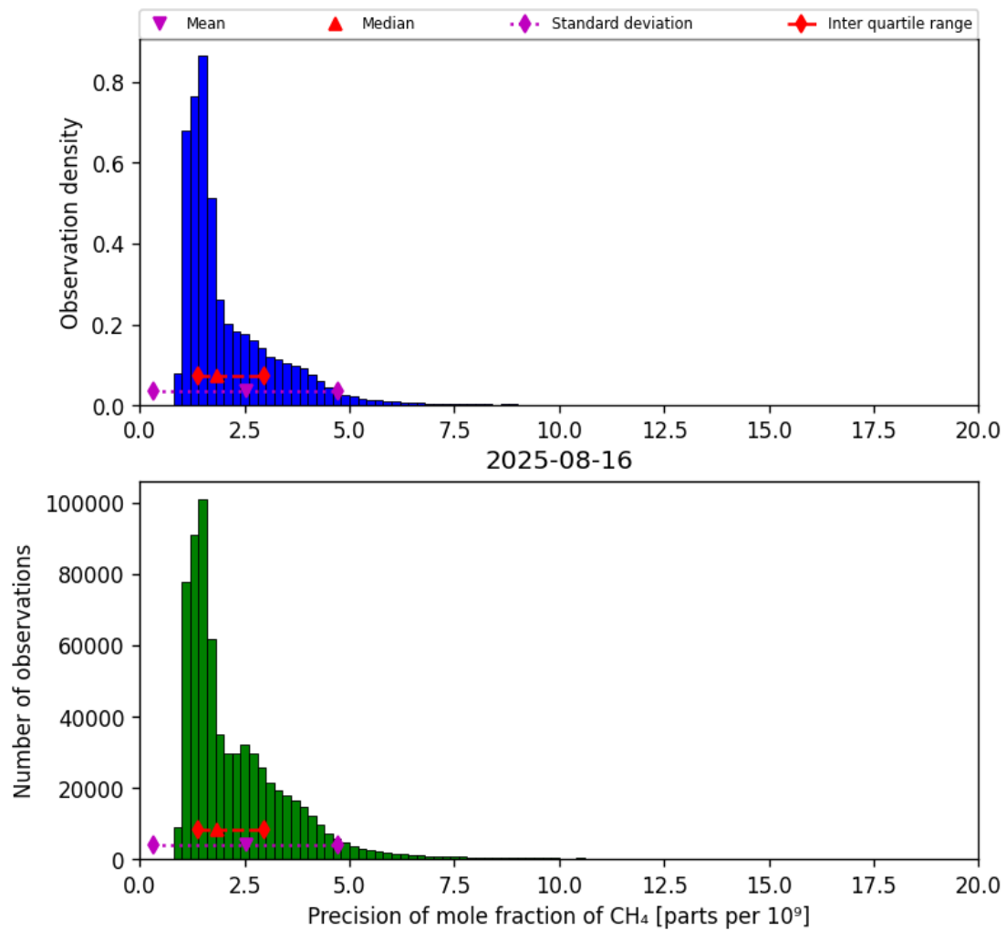
Figure 24: Histogram of “Precision of mole fraction of CH 4 ” for 2025-08-15 to 2025-08-17
