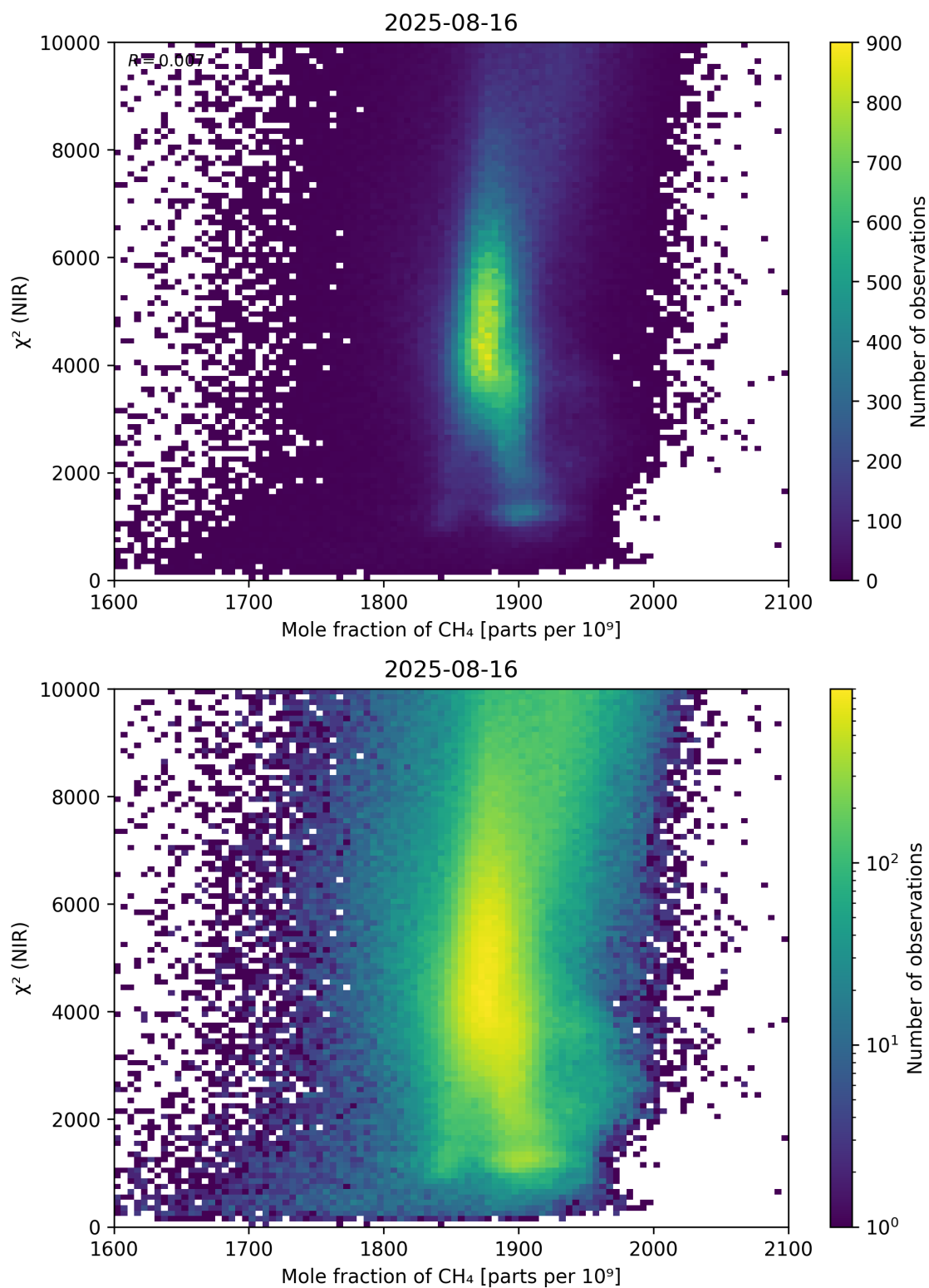
Figure 70: Scatter density plot of “Mole fraction of \text{CH}_4 ” against “ \chi^2 (NIR)” for 2025-08-15 to 2025-08-17.
