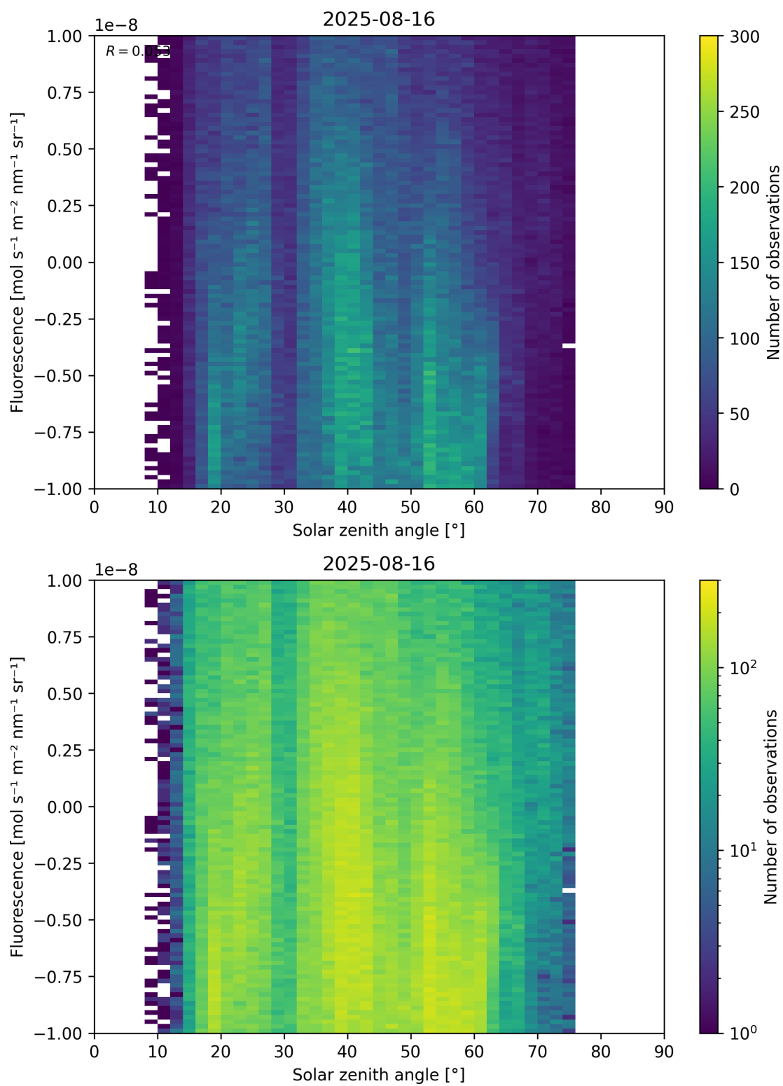
Figure 97: Scatter density plot of “Solar zenith angle” against “Fluorescence” for 2025-08-15 to 2025-08-17.
