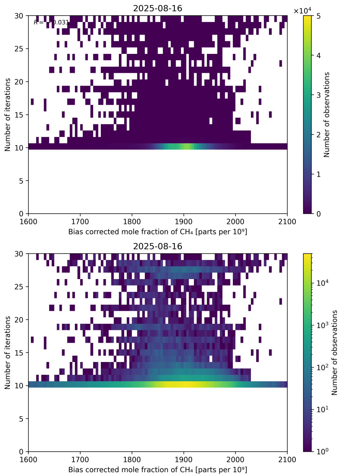
Figure 67: Scatter density plot of “Bias corrected mole fraction of CH 4 ” against “Number of iterations” for 2025-08-15 to 2025-08-17.
