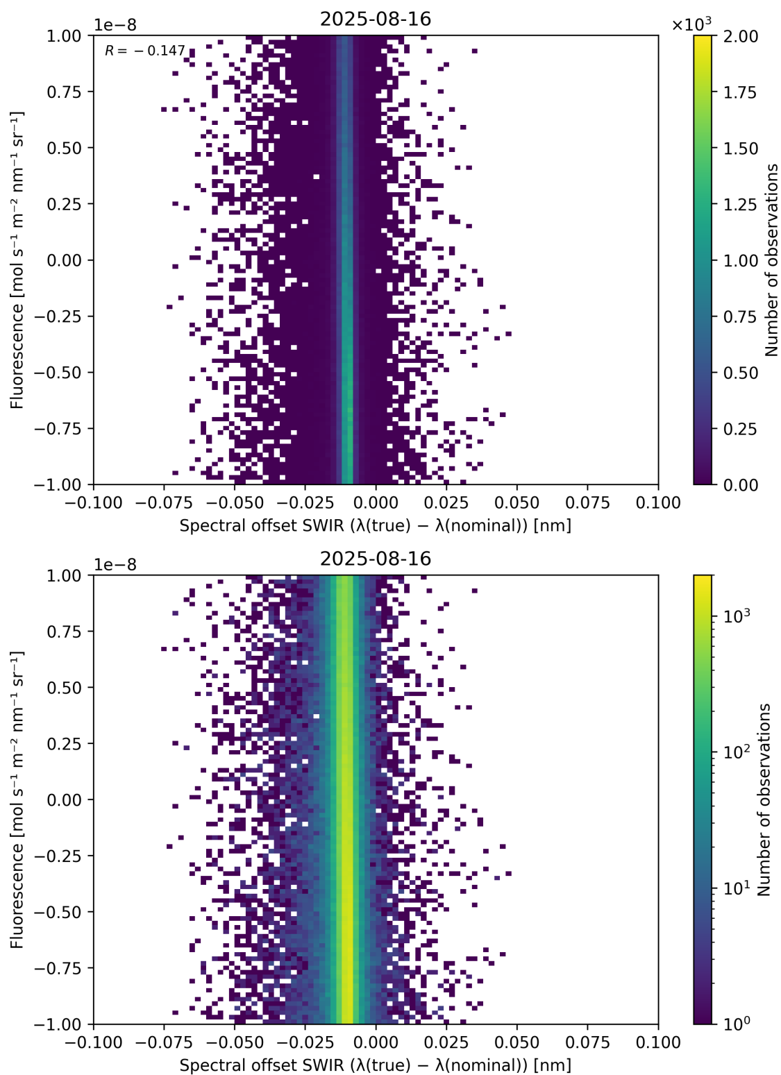
Figure 120: Scatter density plot of “Spectral offset SWIR ( \lambda_{\text{true}} - \lambda_{\text{nominal}} )” against “Fluorescence” for 2025-08-15 to 2025-08-17.
