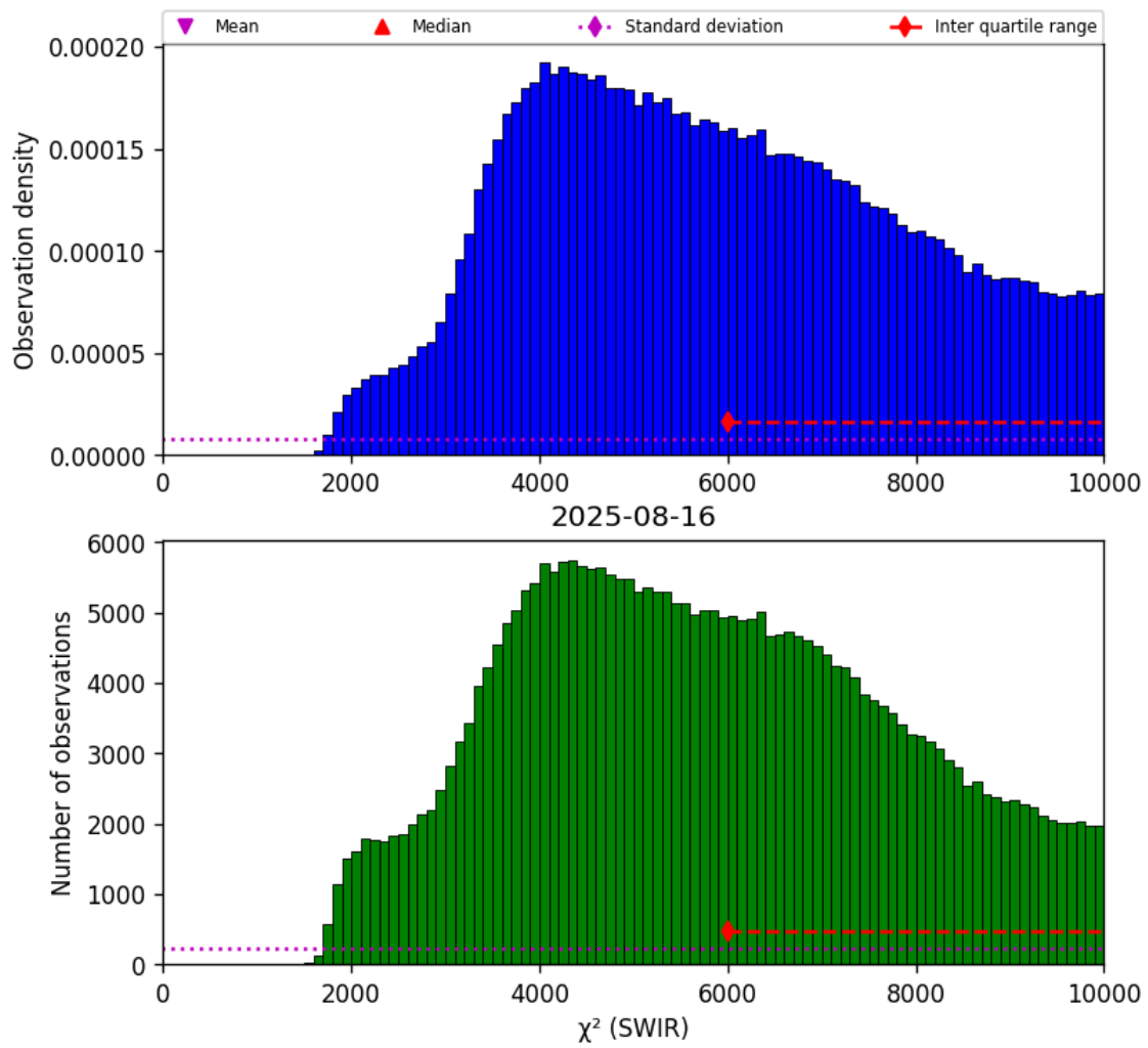
Figure 28: Histogram of “ \chi^2 (SWIR)” for 2025-08-15 to 2025-08-17
