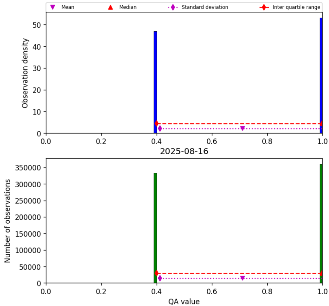
Figure 22: Histogram of “QA value” for 2025-08-15 to 2025-08-17
