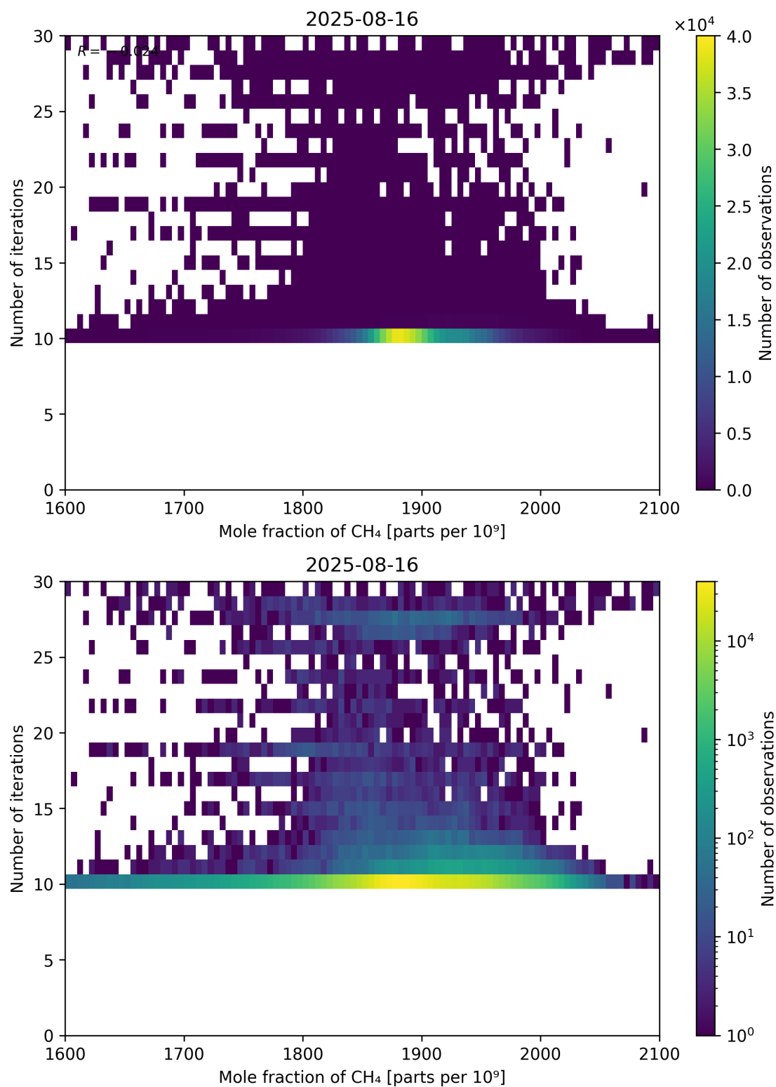
Figure 76: Scatter density plot of “Mole fraction of CH 4 ” against “Number of iterations” for 2025-08-15 to 2025-08-17.
