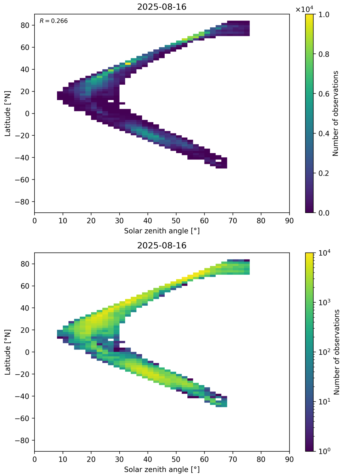
Figure 98: Scatter density plot of “Solar zenith angle” against “Latitude” for 2025-08-15 to 2025-08-17.
