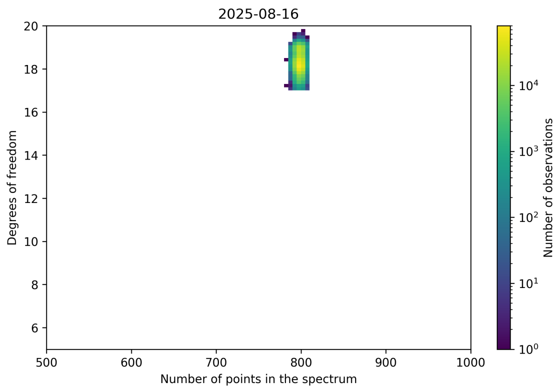
Figure 90: Scatter density plot of “Number of points in the spectrum” against “Degrees of freedom” for 2025-08-15 to 2025-08-17.
