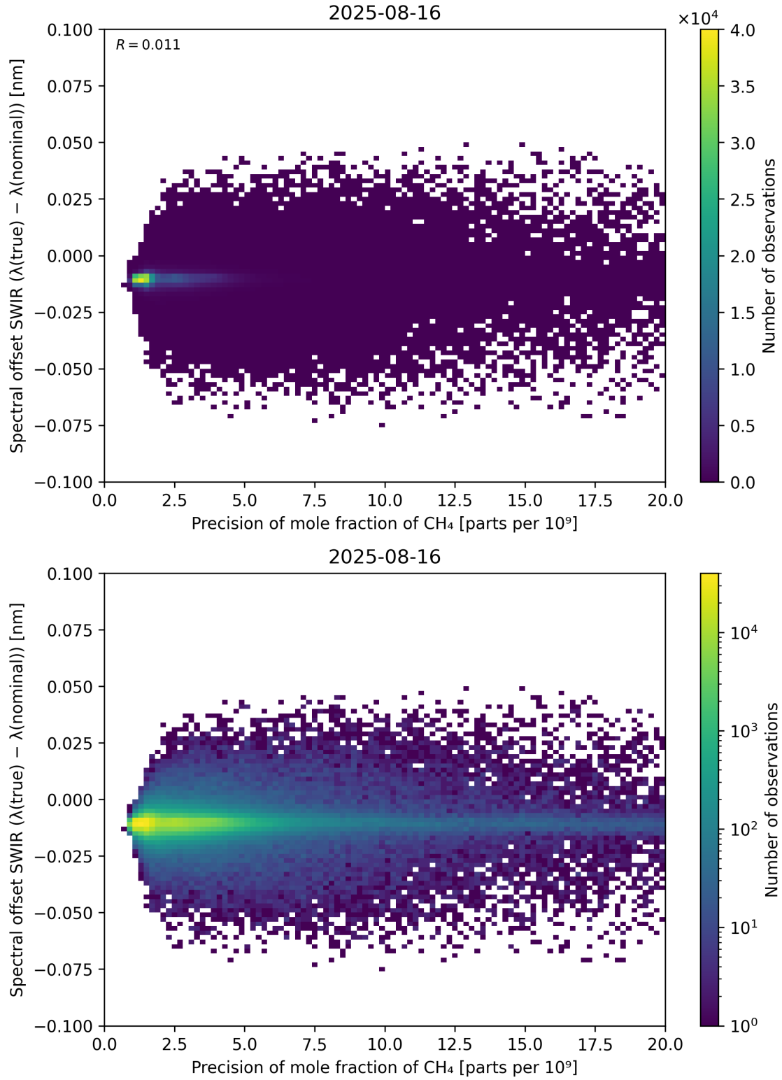
Figure 85: Scatter density plot of “Precision of mole fraction of CH 4 ” against “Spectral offset SWIR ( \lambda_{\text{true}} - \lambda_{\text{nominal}} )” for 2025-08-15 to 2025-08-17.
