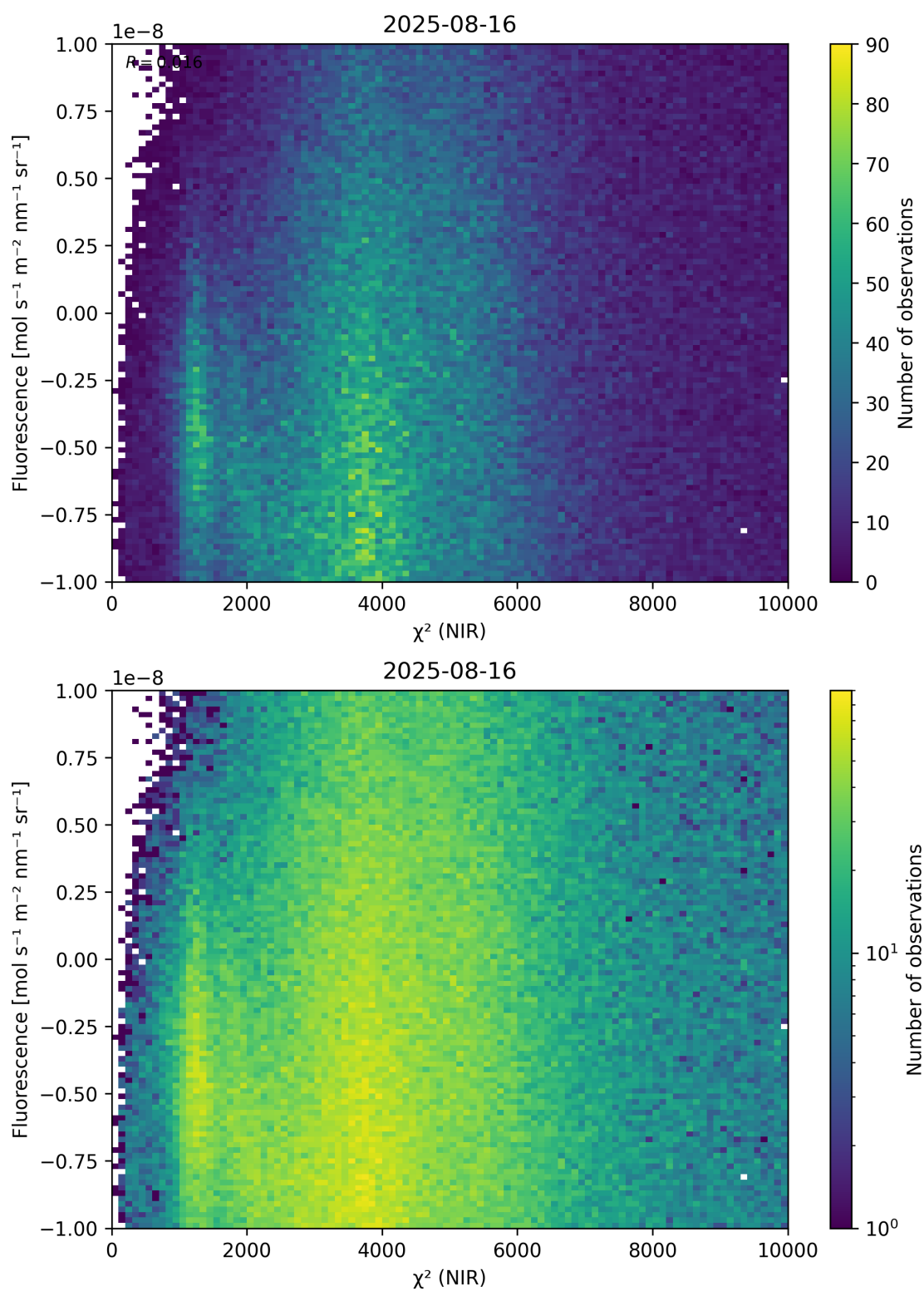
Figure 45: Scatter density plot of “ \chi^2 (NIR)” against “Fluorescence” for 2025-08-15 to 2025-08-17.
