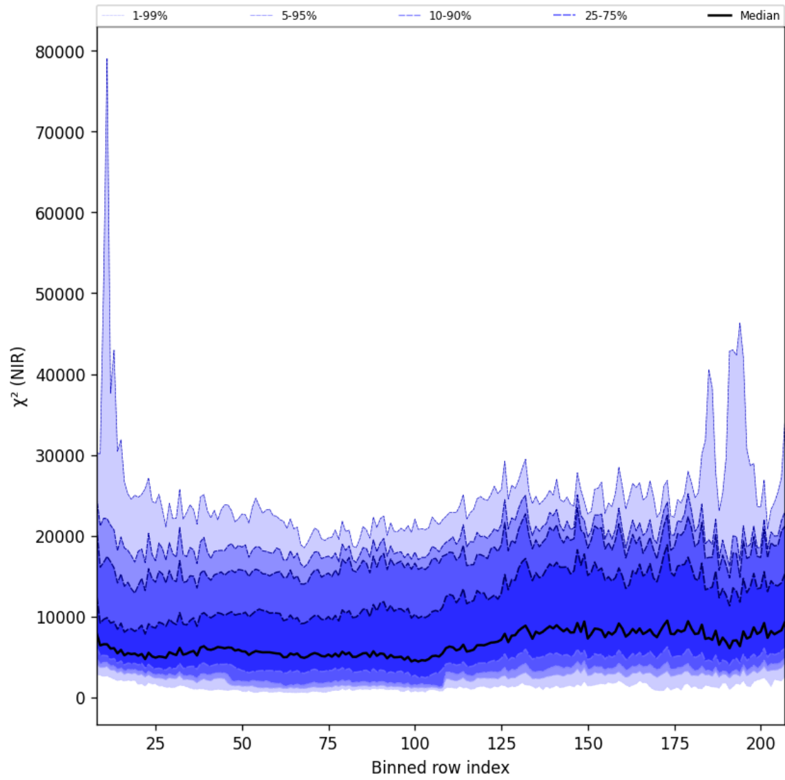
Figure 40: Along track statistics of “ \chi^2 (NIR)” for 2025-08-15 to 2025-08-17
