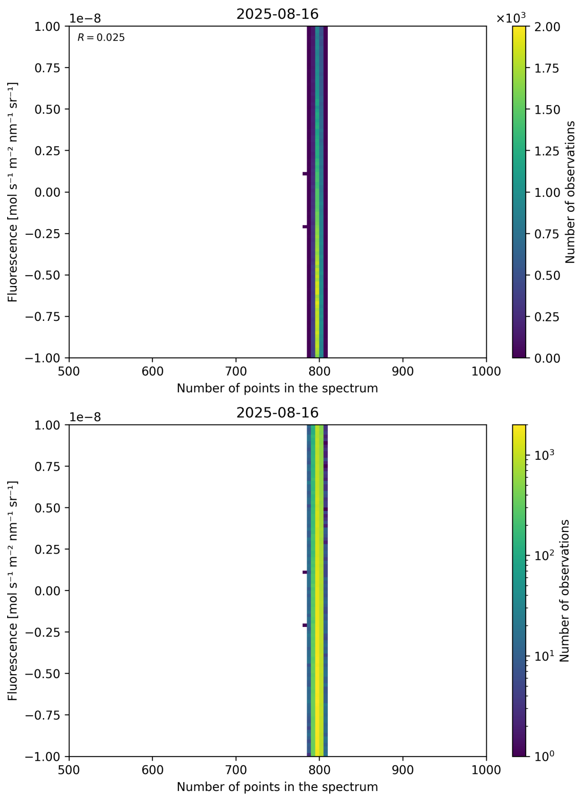
Figure 91: Scatter density plot of “Number of points in the spectrum” against “Fluorescence” for 2025-08-15 to 2025-08-17.
