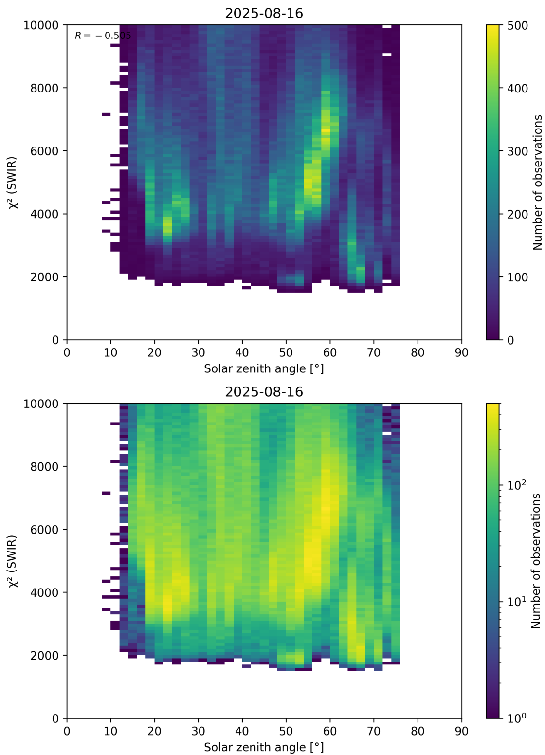
Figure 95: Scatter density plot of “Solar zenith angle” against “ \chi^2 (SWIR)” for 2025-08-15 to 2025-08-17.
