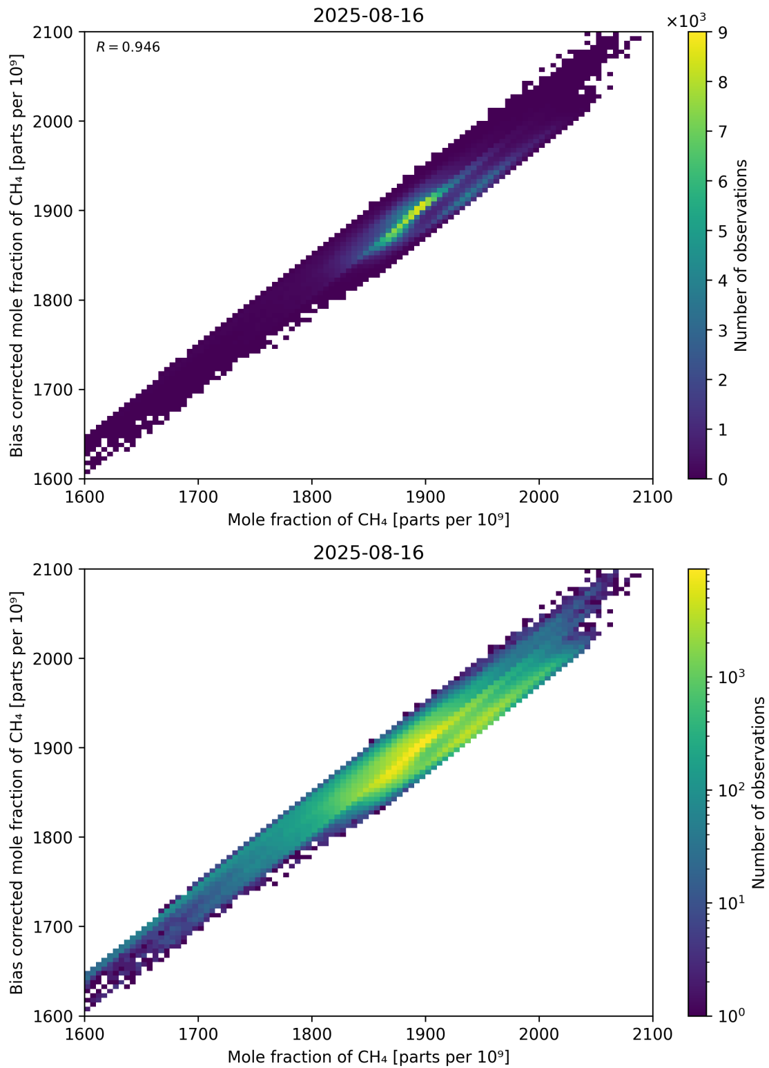
Figure 74: Scatter density plot of “Mole fraction of CH 4 ” against “Bias corrected mole fraction of CH 4 ” for 2025-08-15 to 2025-08-17.
