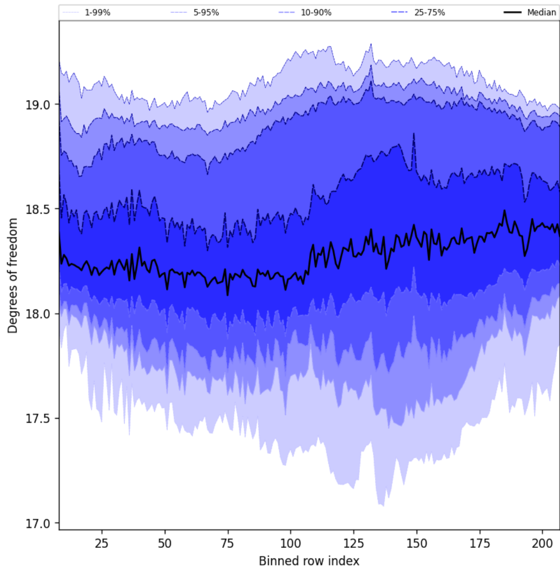
Figure 41: Along track statistics of “Degrees of freedom” for 2025-08-15 to 2025-08-17
