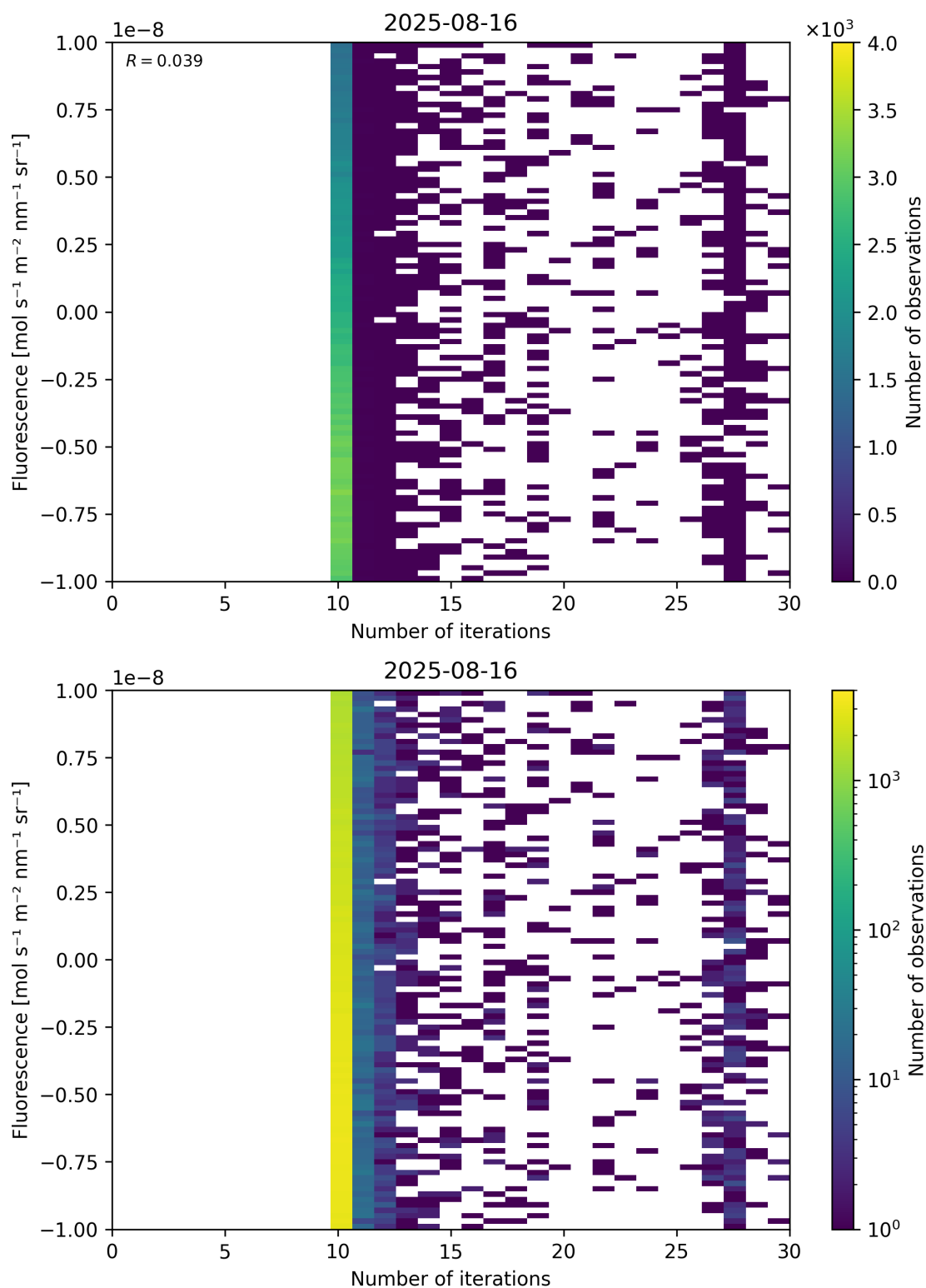
Figure 87: Scatter density plot of “Number of iterations” against “Fluorescence” for 2025-08-15 to 2025-08-17.
