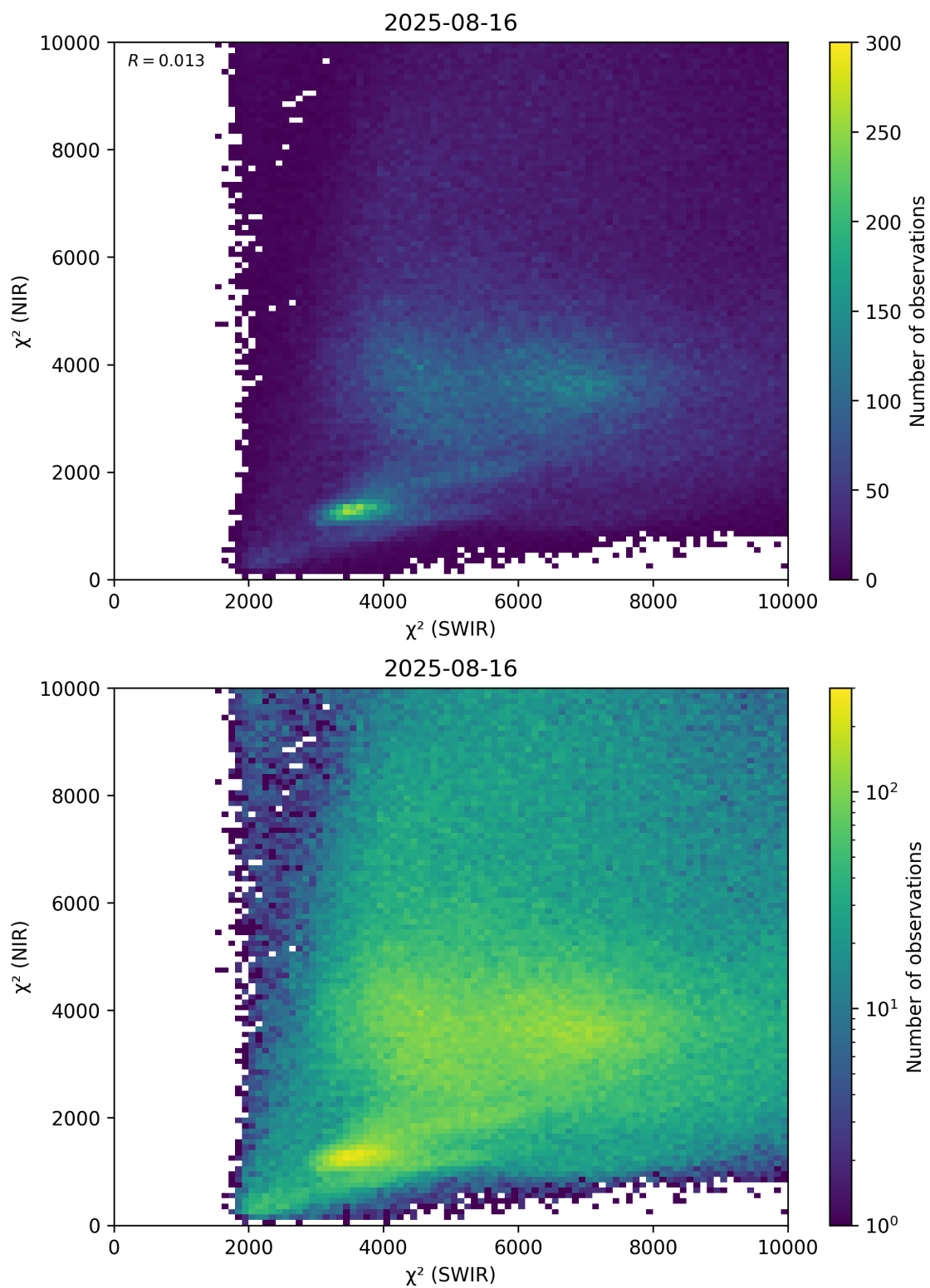
Figure 47: Scatter density plot of “ \chi^2 (SWIR)” against “ \chi^2 (NIR)” for 2025-08-15 to 2025-08-17.
