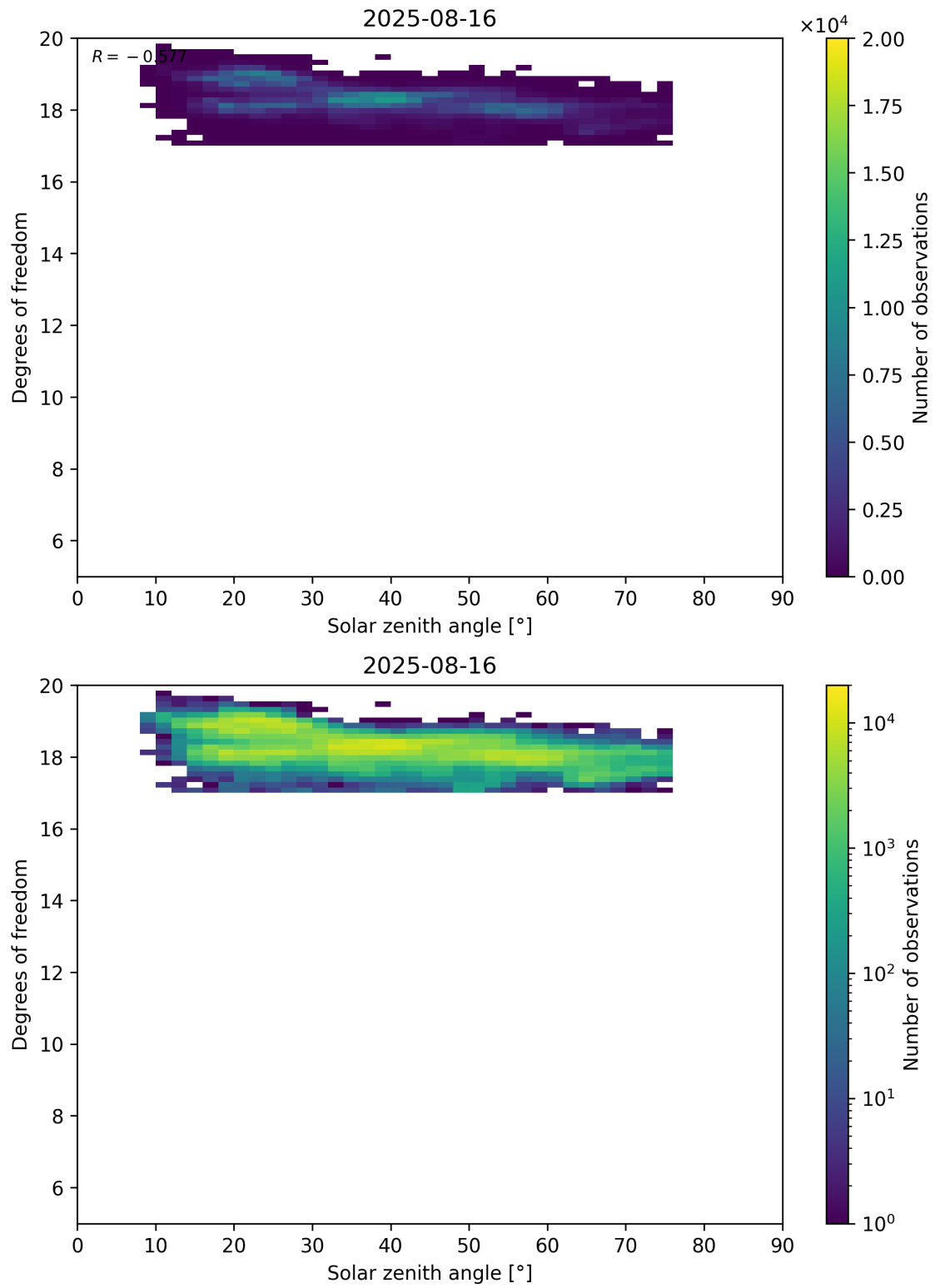
Figure 96: Scatter density plot of “Solar zenith angle” against “Degrees of freedom” for 2025-08-15 to 2025-08-17.
