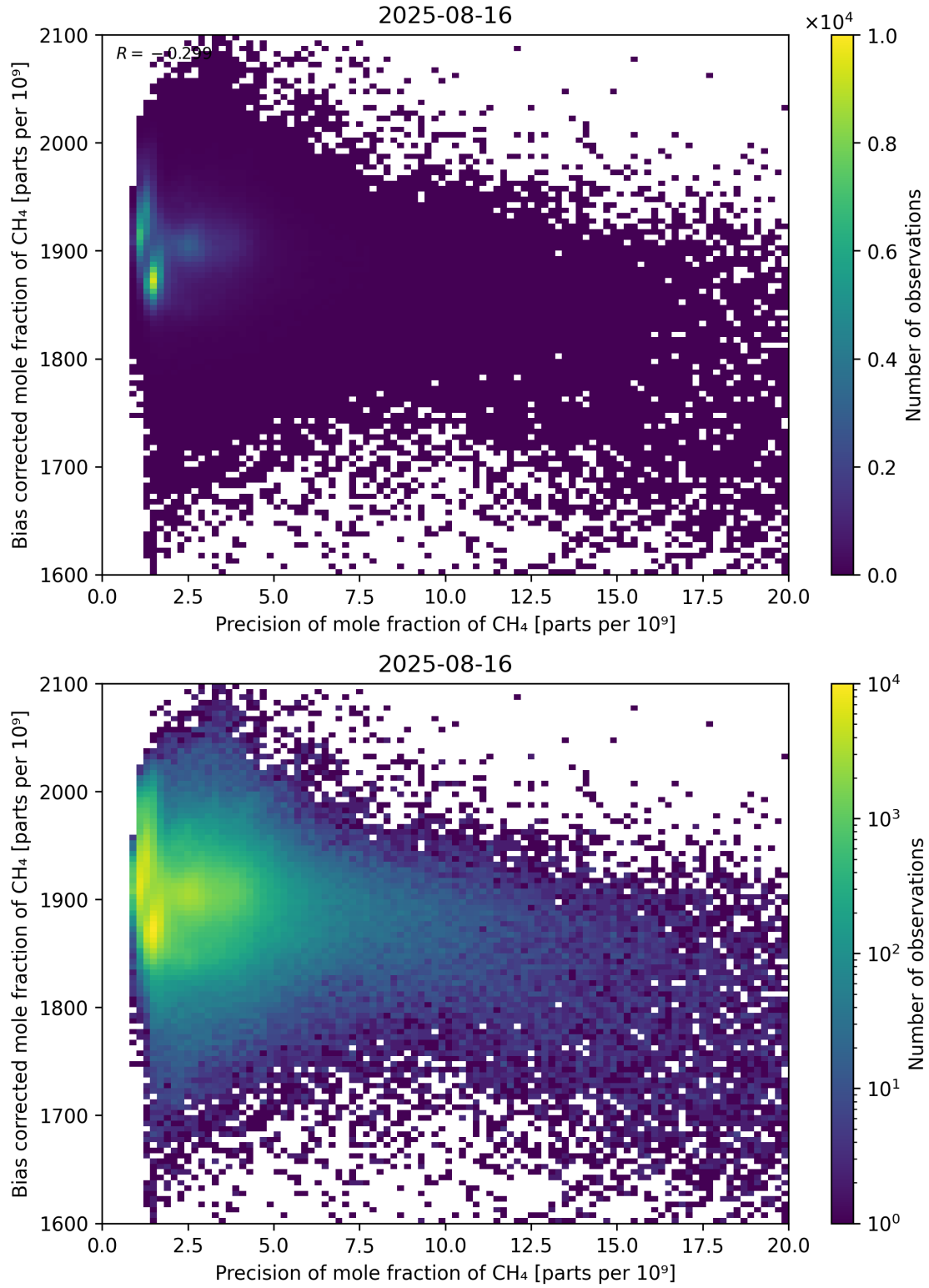
Figure 82: Scatter density plot of “Precision of mole fraction of CH 4 ” against “Bias corrected mole fraction of CH 4 ” for 2025-08-15 to 2025-08-17.
