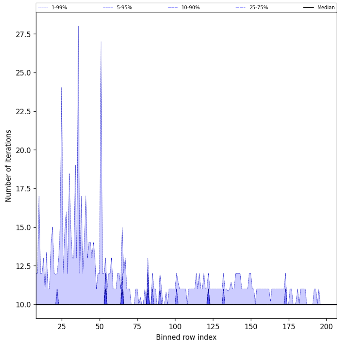
Figure 42: Along track statistics of “Number of iterations” for 2025-08-15 to 2025-08-17
