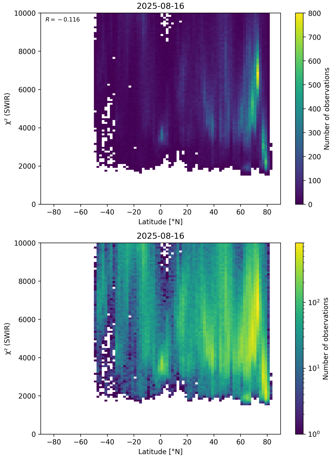
Figure 54: Scatter density plot of “Latitude” against “ \chi^2 (SWIR)” for 2025-08-15 to 2025-08-17.
