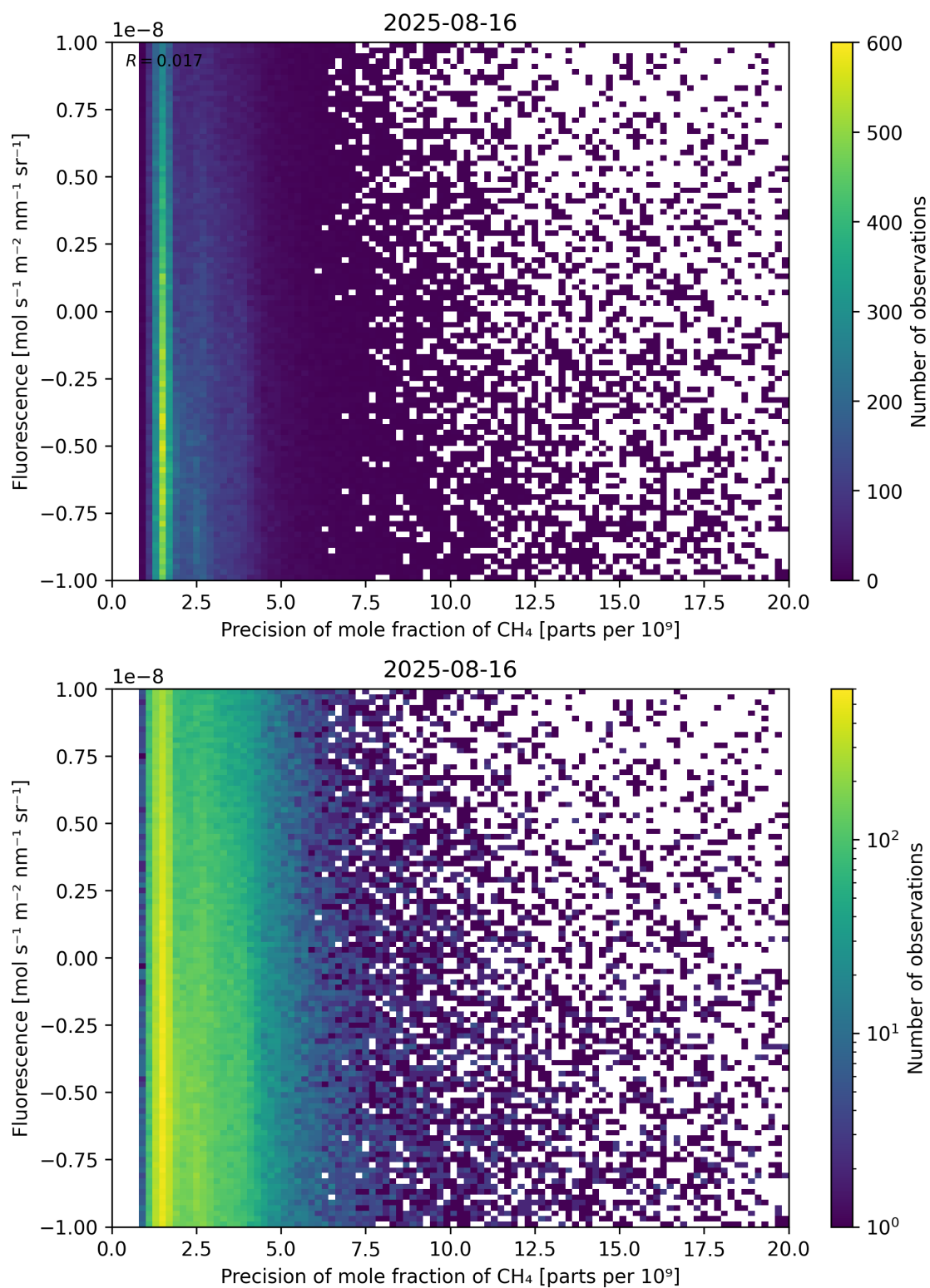
Figure 81: Scatter density plot of “Precision of mole fraction of \text{CH}_4 ” against “Fluorescence” for 2025-08-15 to 2025-08-17.
