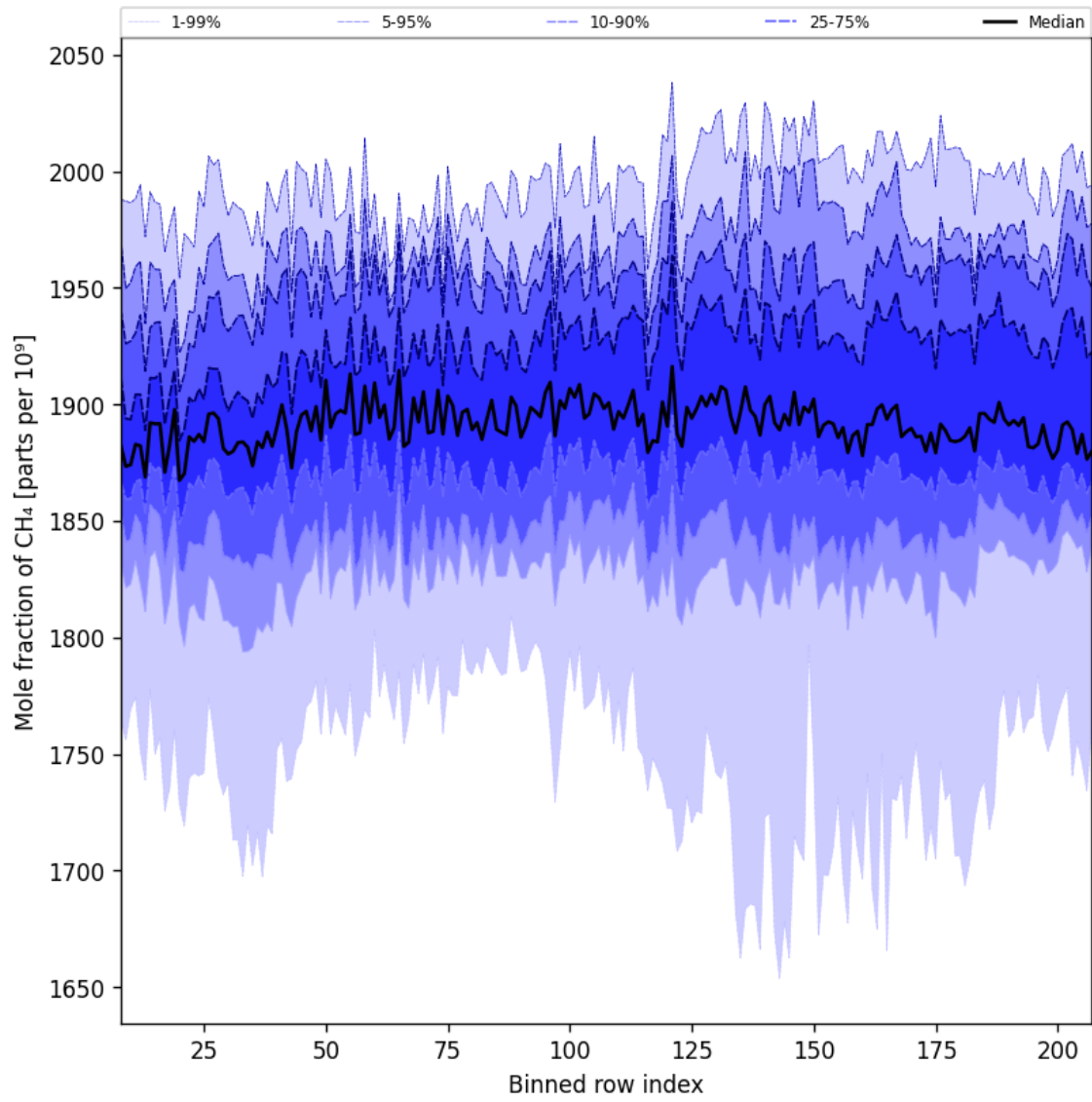
Figure 34: Along track statistics of “Mole fraction of CH 4 ” for 2025-08-15 to 2025-08-17
