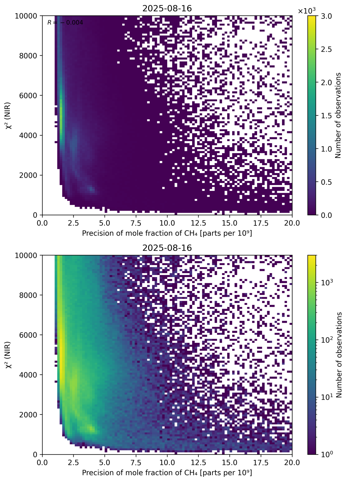
Figure 78: Scatter density plot of “Precision of mole fraction of CH 4 ” against “ \chi^2 (NIR)” for 2025-08-15 to 2025-08-17.
