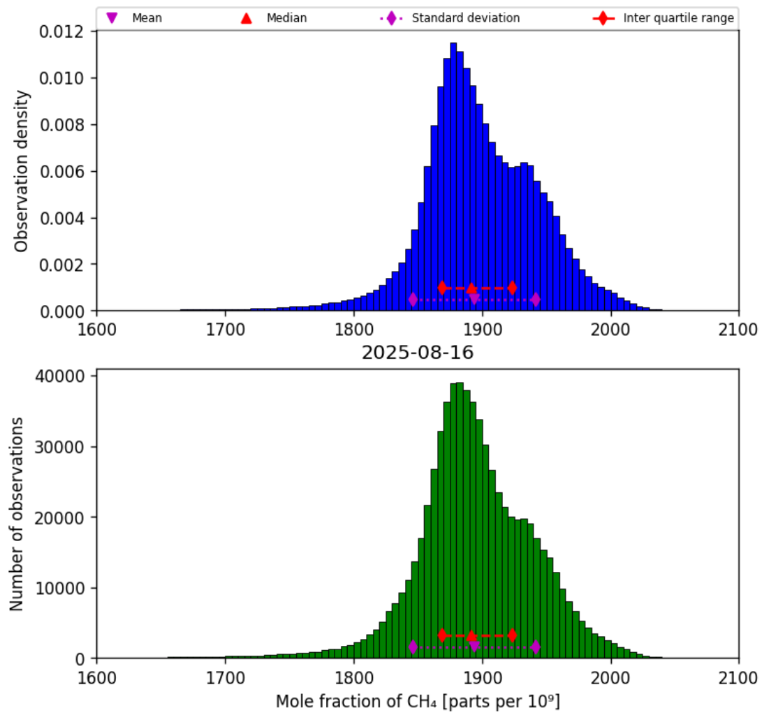
Figure 23: Histogram of “Mole fraction of CH 4 ” for 2025-08-15 to 2025-08-17
