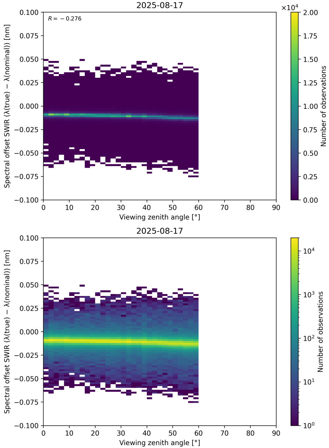
Figure 116: Scatter density plot of “Viewing zenith angle” against “Spectral offset SWIR ( \lambda_{\text{true}} - \lambda_{\text{nominal}} )” for 2025-08-16 to 2025-08-18.
