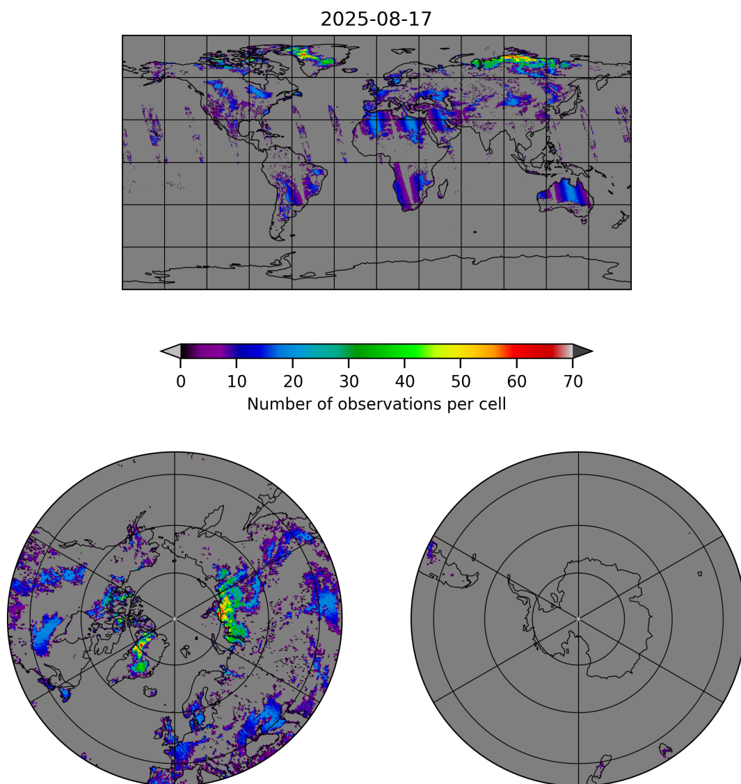
Figure 10: Map of the number of observations for 2025-08-16 to 2025-08-18
