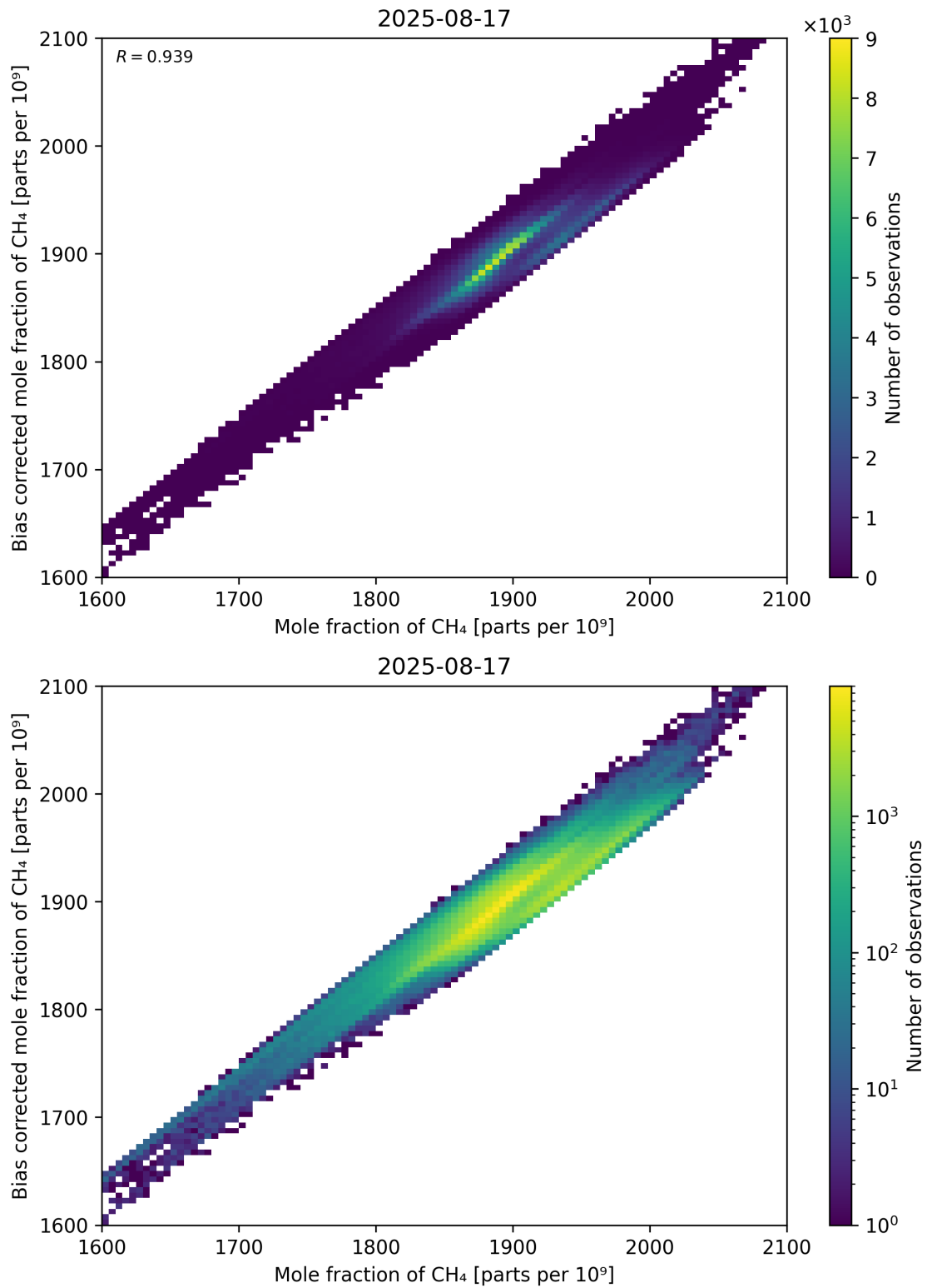
Figure 74: Scatter density plot of “Mole fraction of \text{CH}_4 ” against “Bias corrected mole fraction of \text{CH}_4 ” for 2025-08-16 to 2025-08-18.
