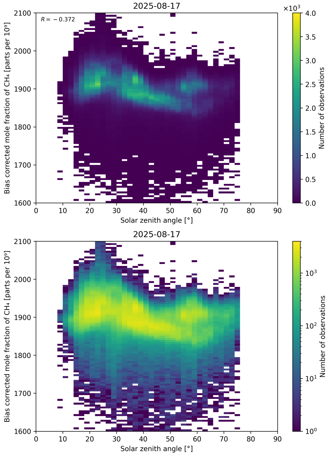
Figure 100: Scatter density plot of “Solar zenith angle” against “Bias corrected mole fraction of CH 4 ” for 2025-08-16 to 2025-08-18.
