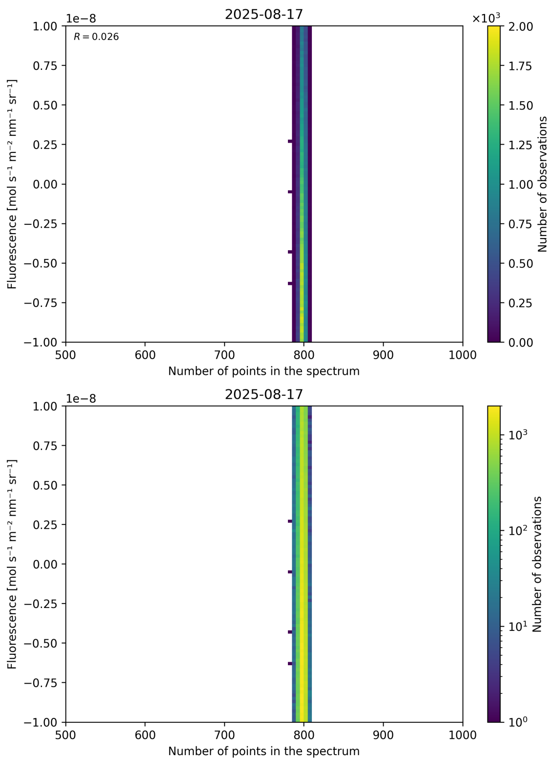
Figure 91: Scatter density plot of “Number of points in the spectrum” against “Fluorescence” for 2025-08-16 to 2025-08-18.
