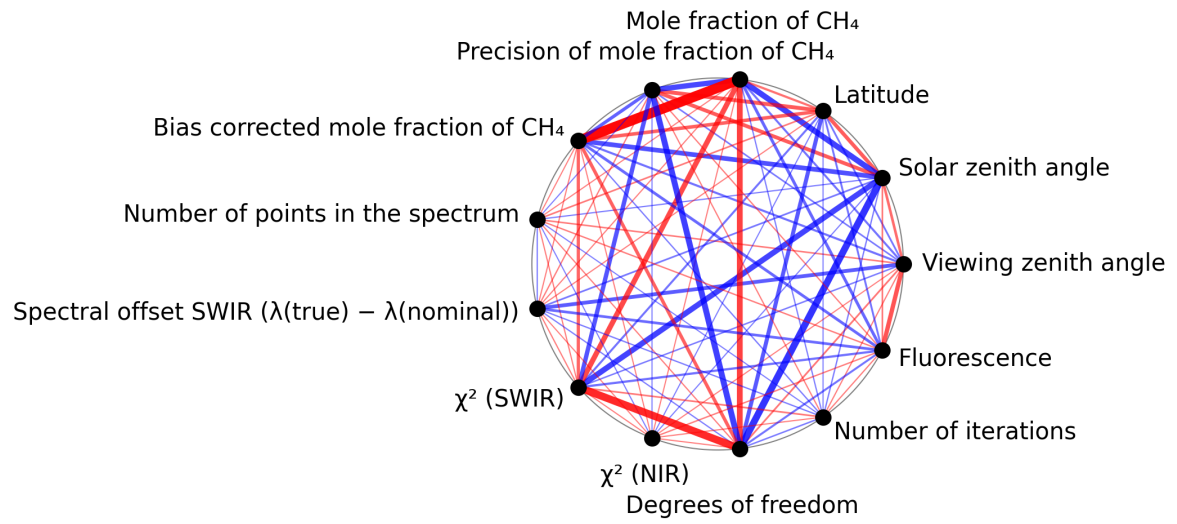
Figure 1: Map of correlation graph for 2025-08-16 to 2025-08-18.
