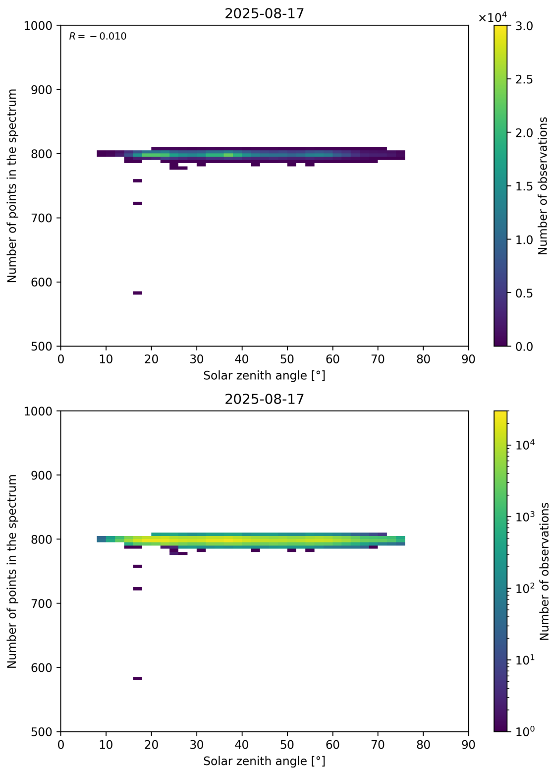
Figure 103: Scatter density plot of “Solar zenith angle” against “Number of points in the spectrum” for 2025-08-16 to 2025-08-18.
