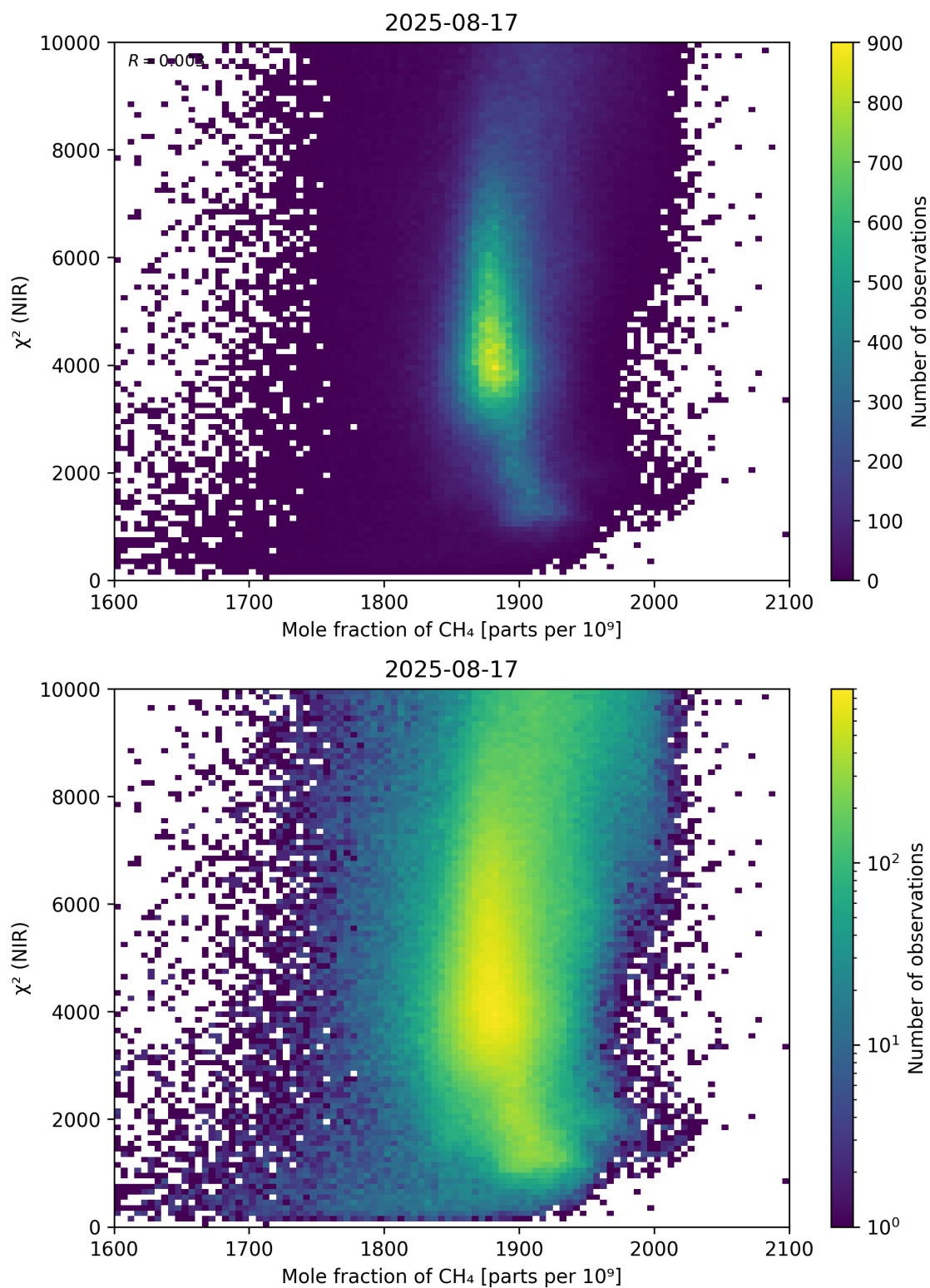
Figure 70: Scatter density plot of “Mole fraction of CH 4 ” against “ \chi^2 (NIR)” for 2025-08-16 to 2025-08-18.
