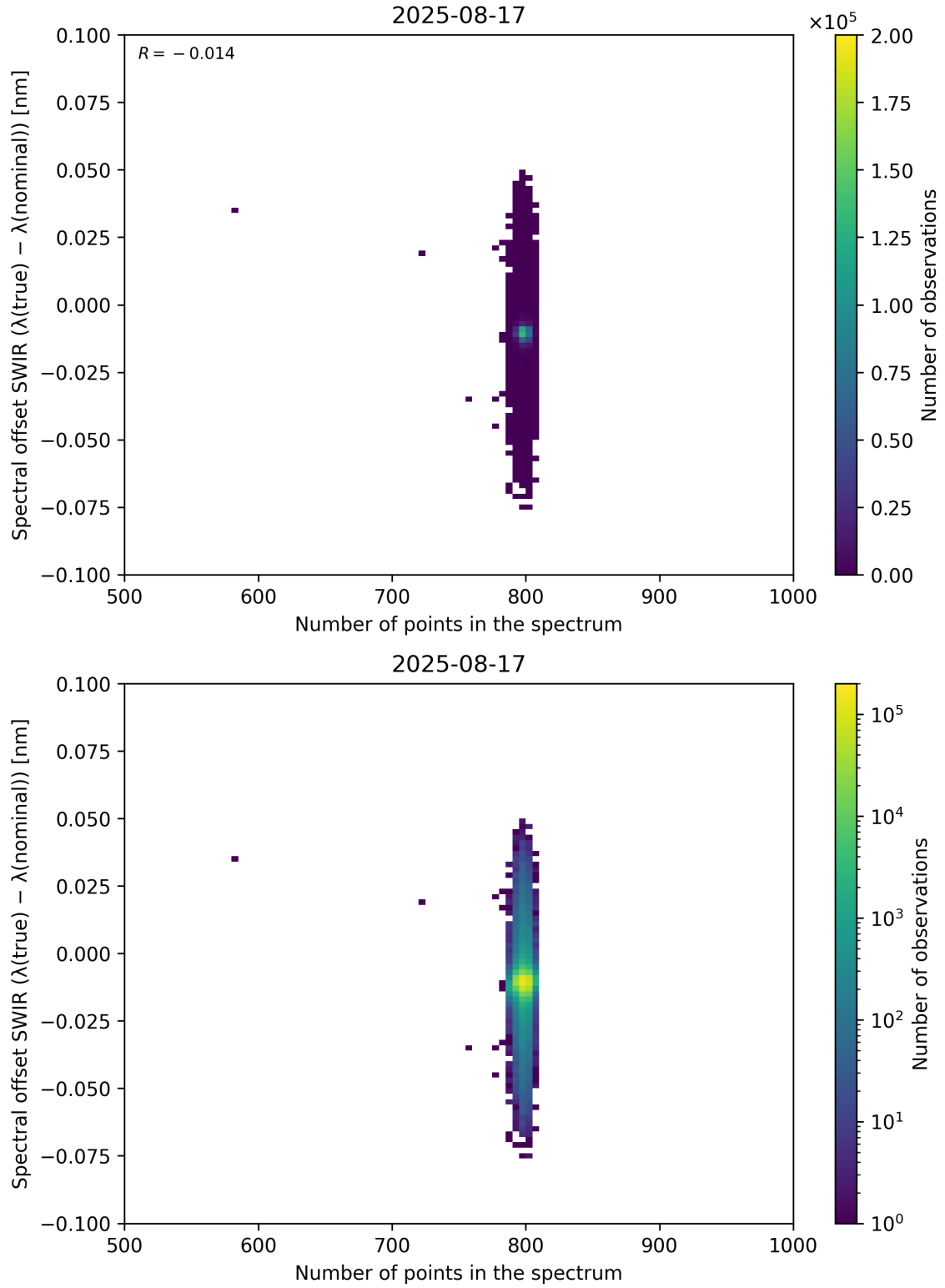
Figure 93: Scatter density plot of “Number of points in the spectrum” against “Spectral offset SWIR ( \lambda_{\text{true}} - \lambda_{\text{nominal}} )” for 2025-08-16 to 2025-08-18.
