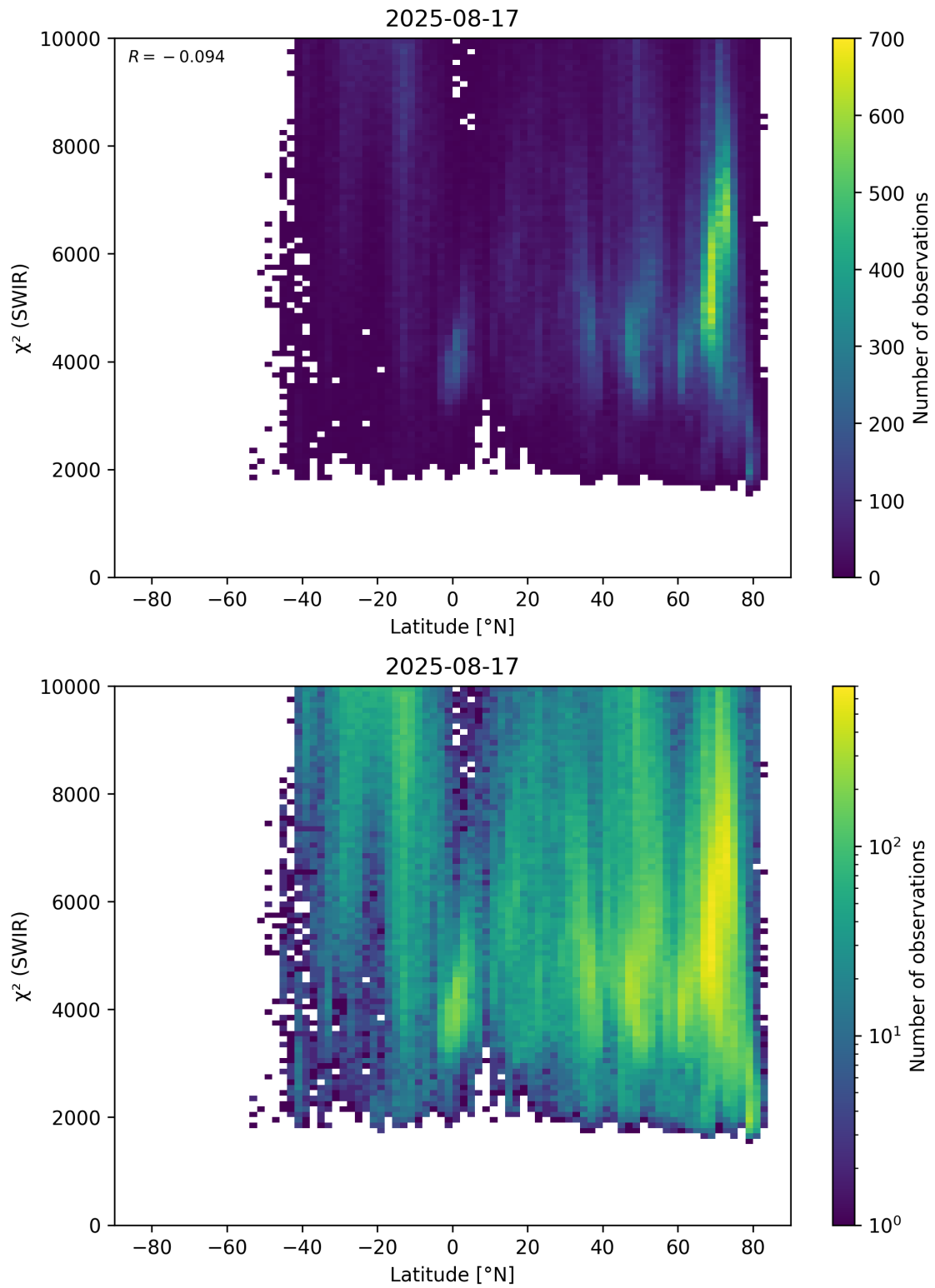
Figure 54: Scatter density plot of “Latitude” against “ \chi^2 (SWIR)” for 2025-08-16 to 2025-08-18.
