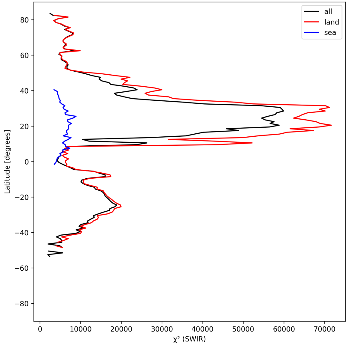
Figure 17: Zonal average of “ \chi^2 (SWIR)” for 2025-08-16 to 2025-08-18.
