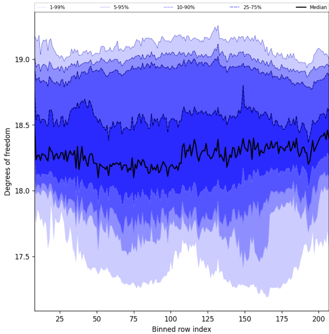
Figure 41: Along track statistics of “Degrees of freedom” for 2025-08-16 to 2025-08-18
