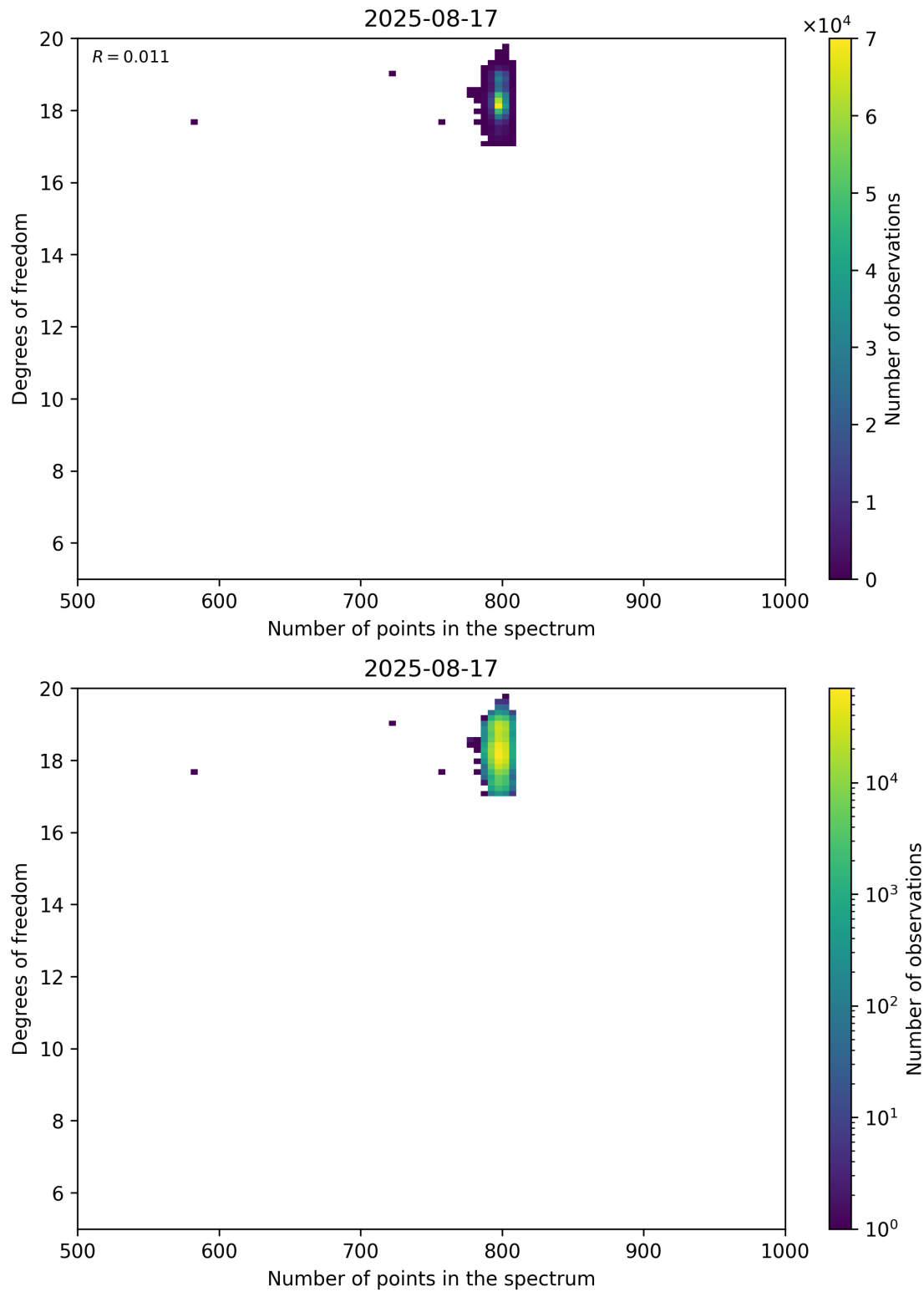
Figure 90: Scatter density plot of “Number of points in the spectrum” against “Degrees of freedom” for 2025-08-16 to 2025-08-18.
