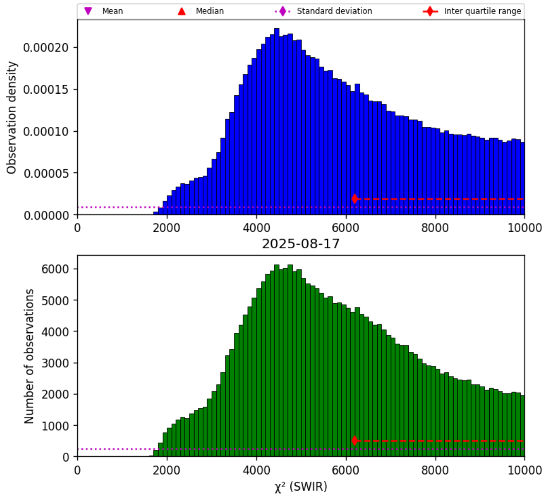
Figure 28: Histogram of " \chi^2 (SWIR)" for 2025-08-16 to 2025-08-18
