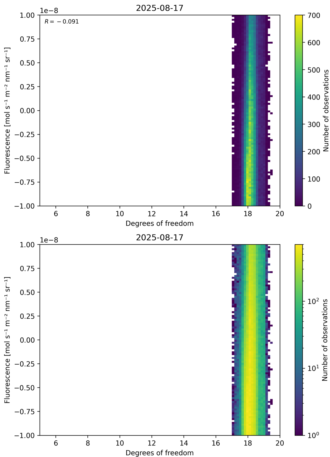
Figure 51: Scatter density plot of “Degrees of freedom” against “Fluorescence” for 2025-08-16 to 2025-08-18.
