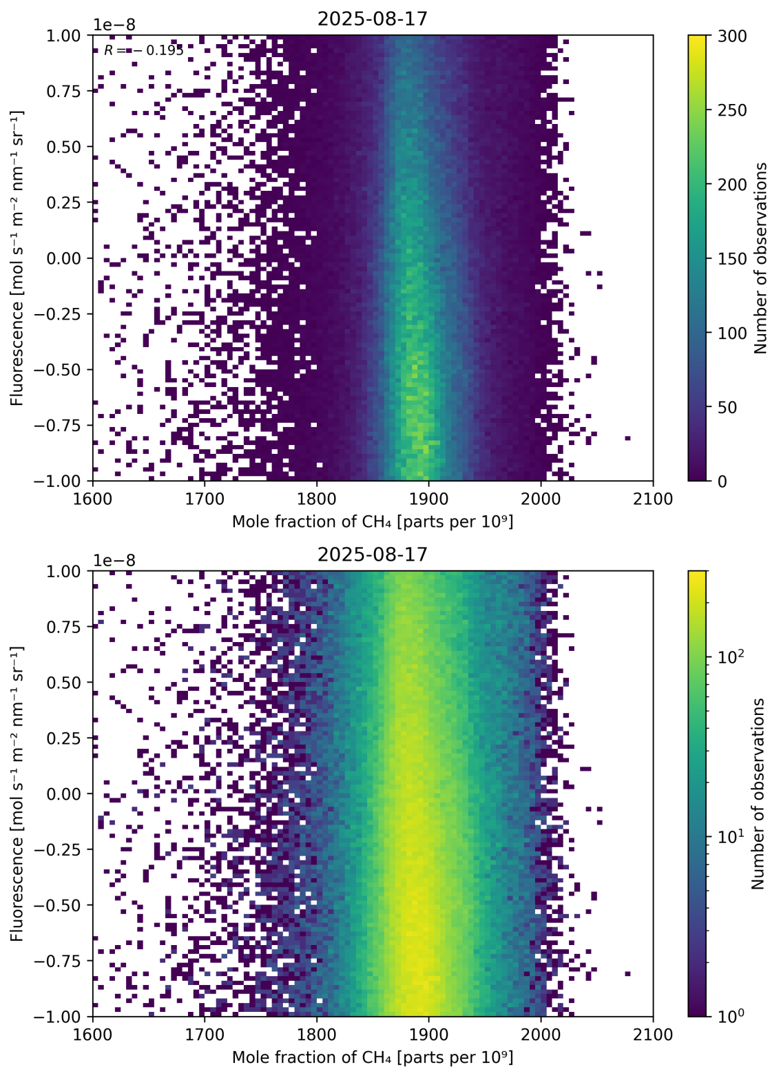
Figure 73: Scatter density plot of “Mole fraction of \text{CH}_4 ” against “Fluorescence” for 2025-08-16 to 2025-08-18.
