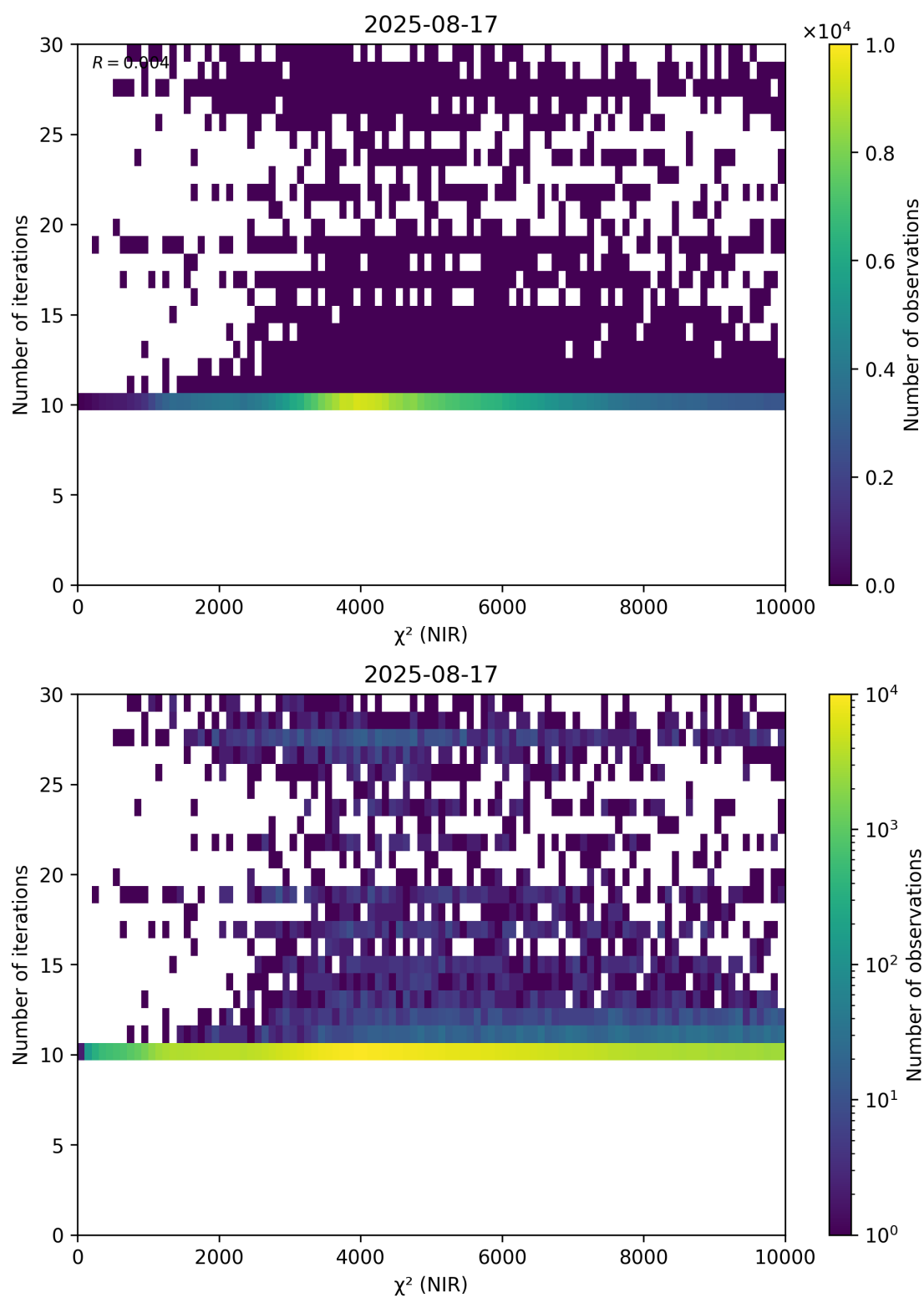
Figure 46: Scatter density plot of “ \chi^2 (NIR)” against “Number of iterations” for 2025-08-16 to 2025-08-18.
