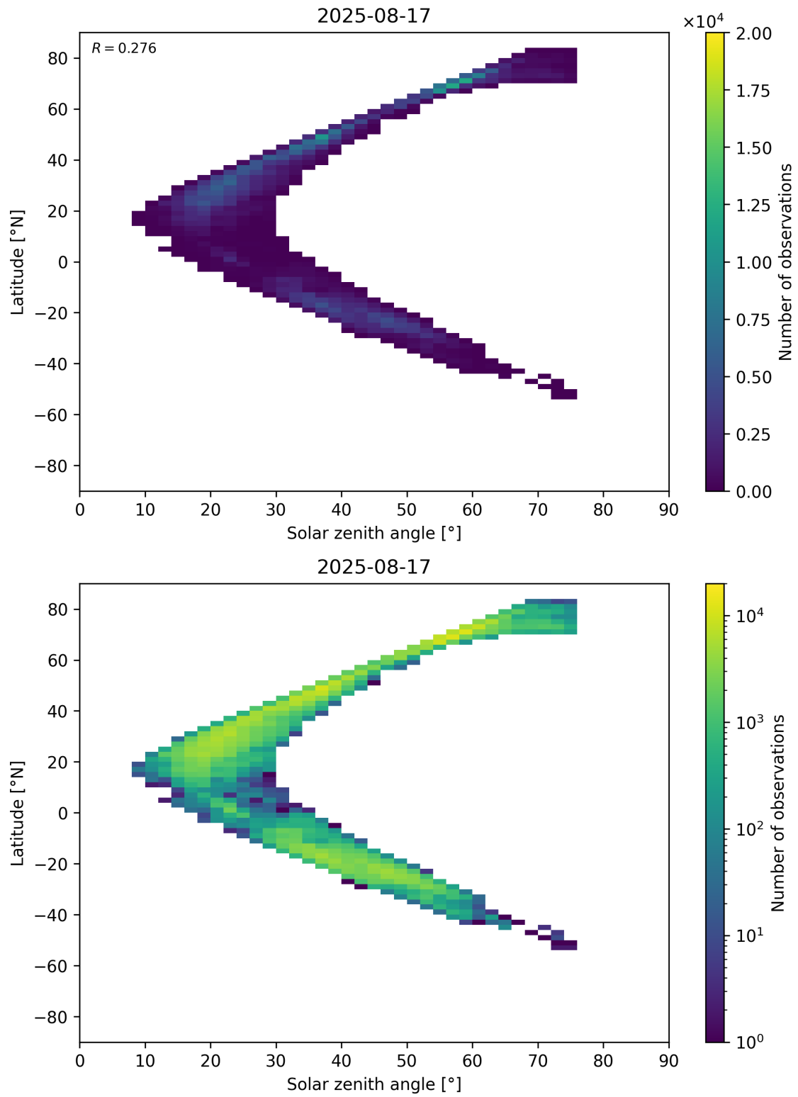
Figure 98: Scatter density plot of “Solar zenith angle” against “Latitude” for 2025-08-16 to 2025-08-18.
