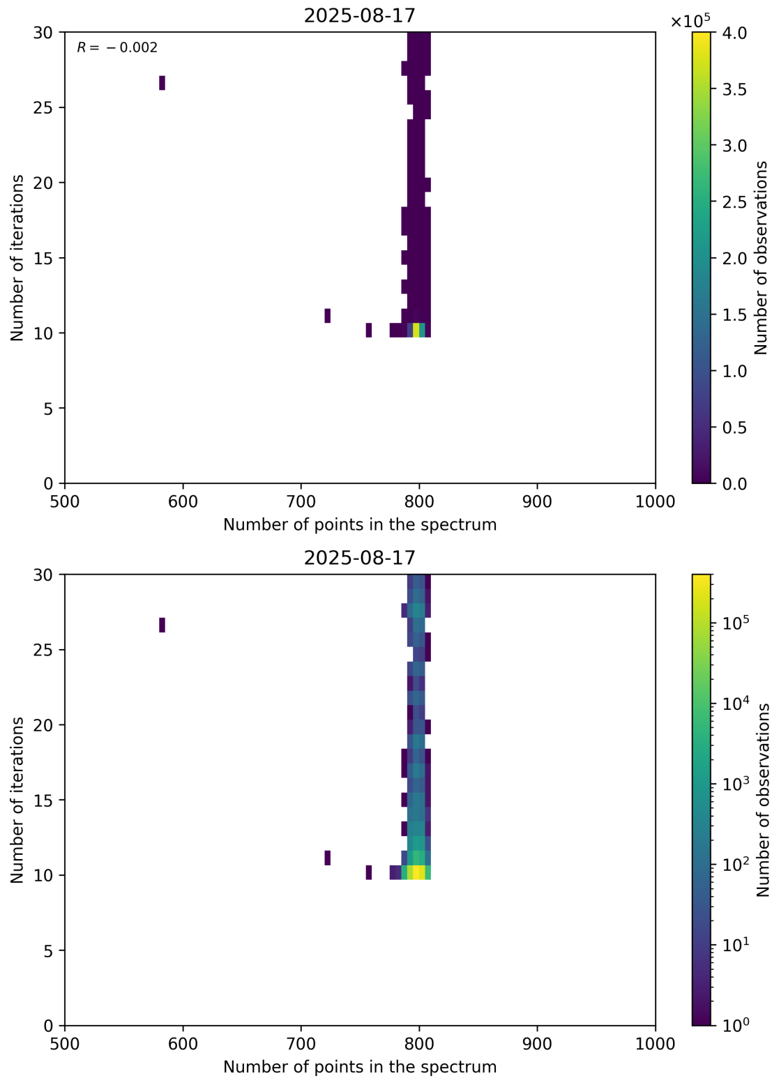
Figure 92: Scatter density plot of “Number of points in the spectrum” against “Number of iterations” for 2025-08-16 to 2025-08-18.
