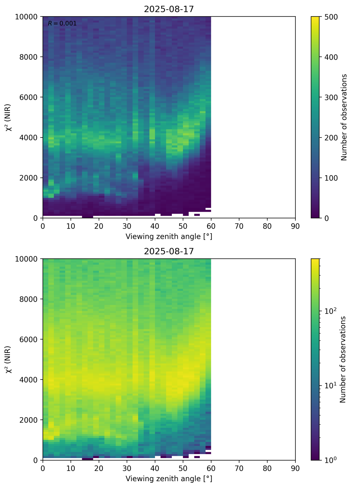
Figure 105: Scatter density plot of “Viewing zenith angle” against “ \chi^2 (NIR)” for 2025-08-16 to 2025-08-18.
