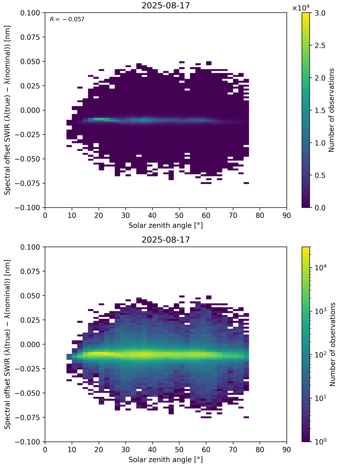
Figure 104: Scatter density plot of “Solar zenith angle” against “Spectral offset SWIR ( \lambda_{\text{true}} - \lambda_{\text{nominal}} )” for 2025-08-16 to 2025-08-18.
