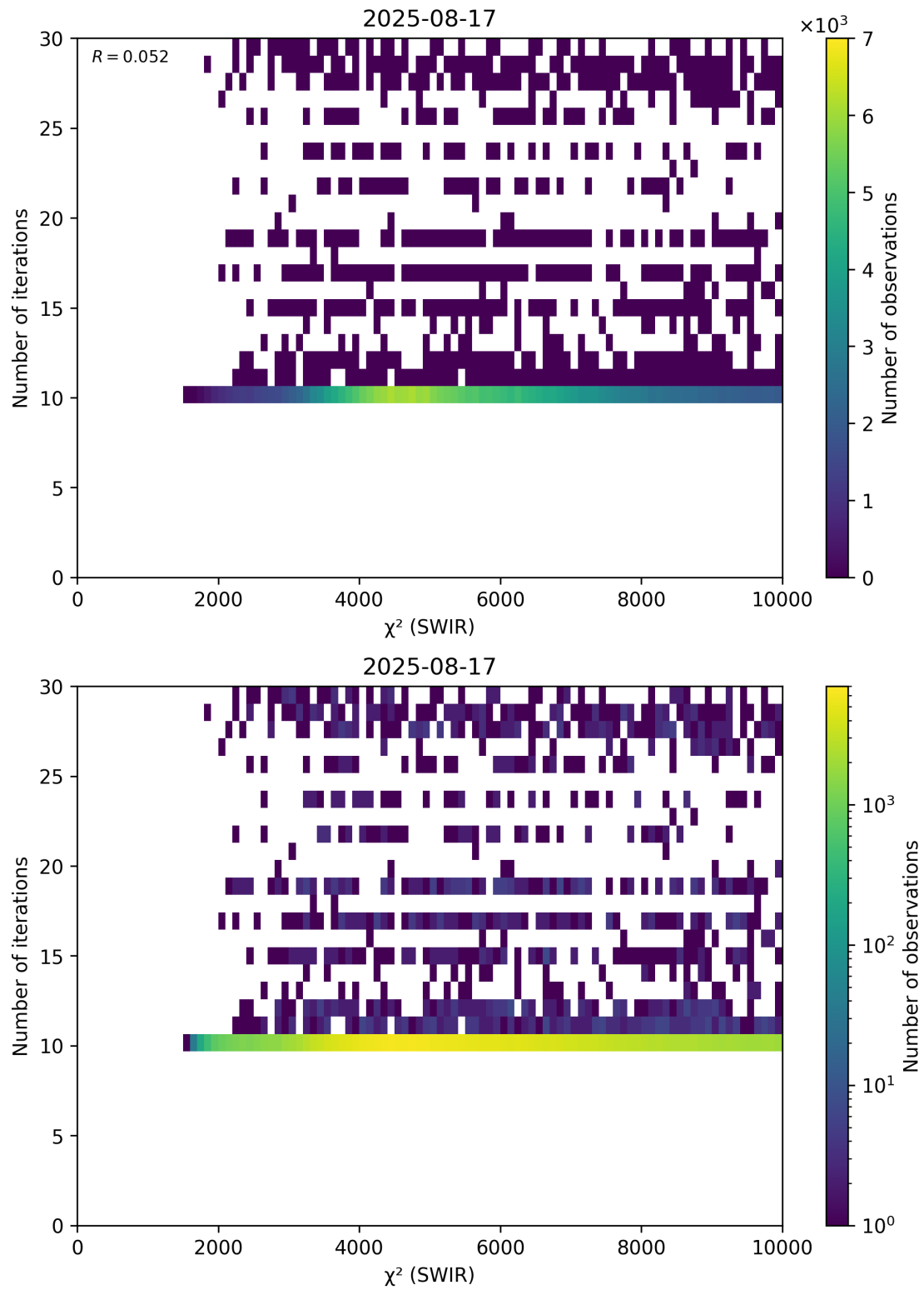
Figure 50: Scatter density plot of “ \chi^2 (SWIR)” against “Number of iterations” for 2025-08-16 to 2025-08-18.
