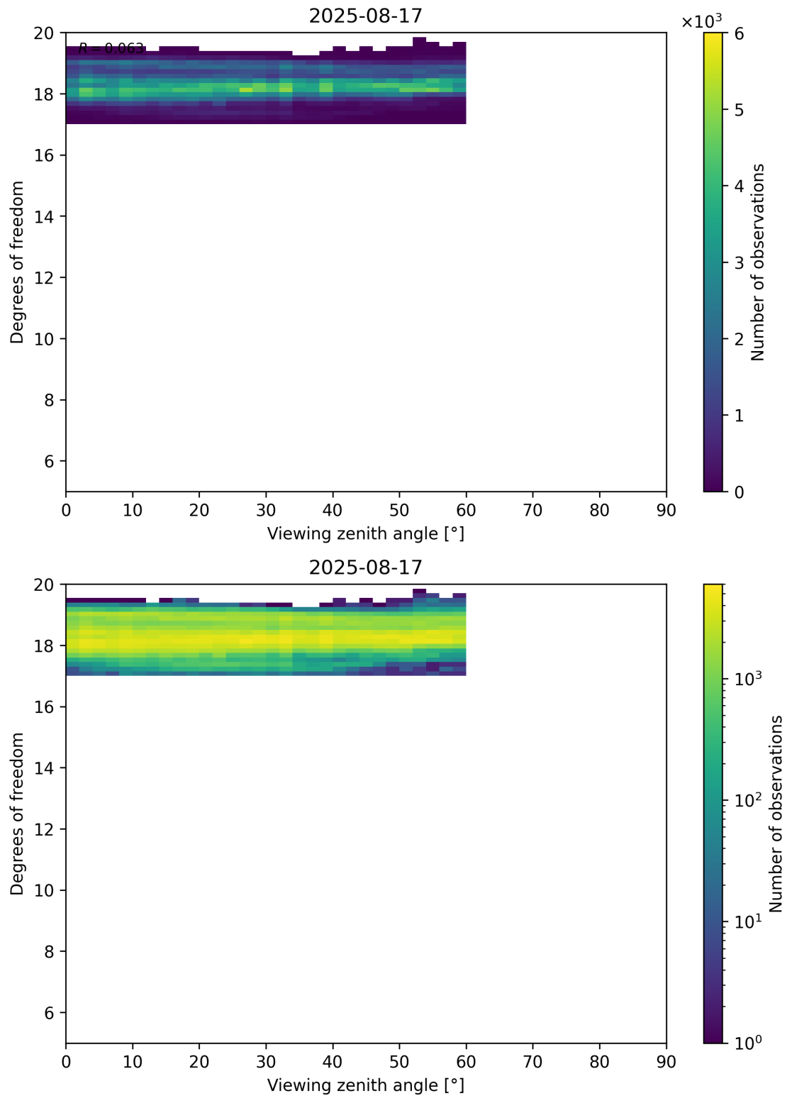
Figure 107: Scatter density plot of “Viewing zenith angle” against “Degrees of freedom” for 2025-08-16 to 2025-08-18.
