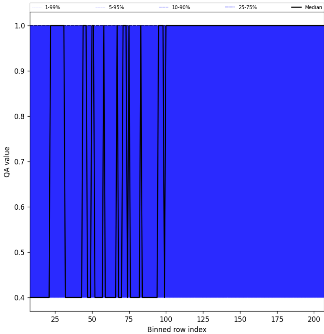
Figure 33: Along track statistics of “QA value” for 2025-08-16 to 2025-08-18
