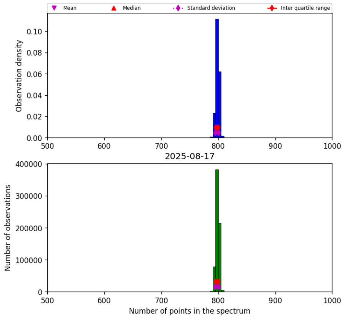
Figure 26: Histogram of “Number of points in the spectrum” for 2025-08-16 to 2025-08-18
