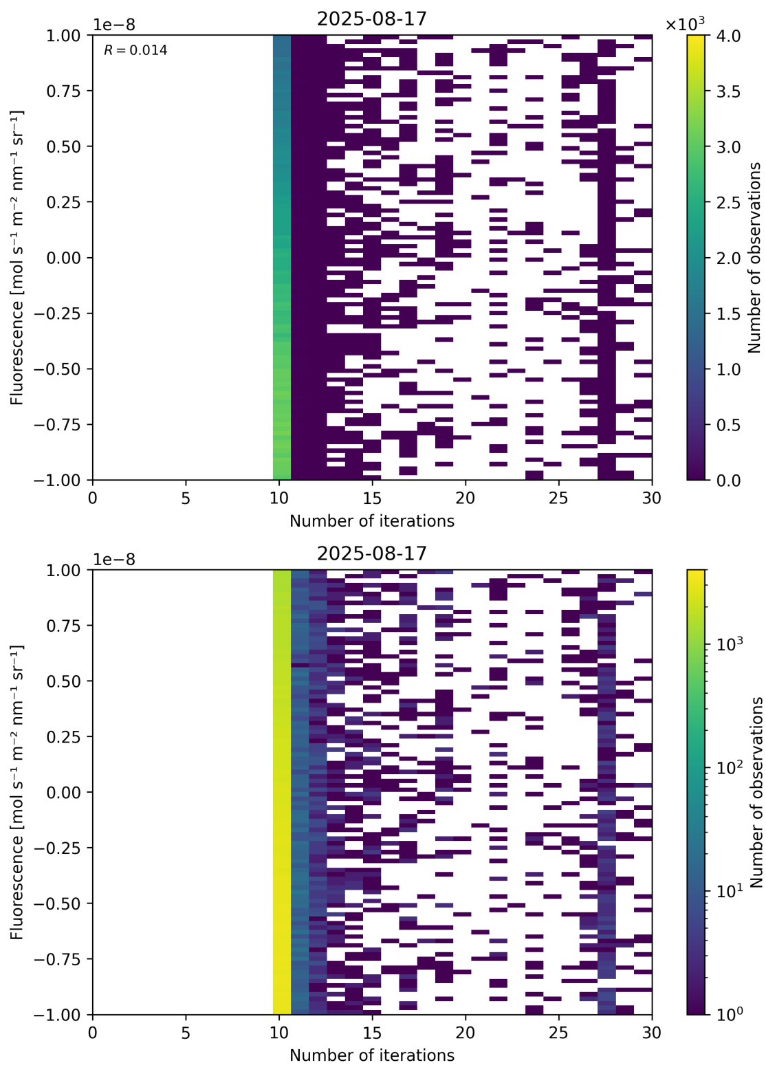
Figure 87: Scatter density plot of “Number of iterations” against “Fluorescence” for 2025-08-16 to 2025-08-18.
