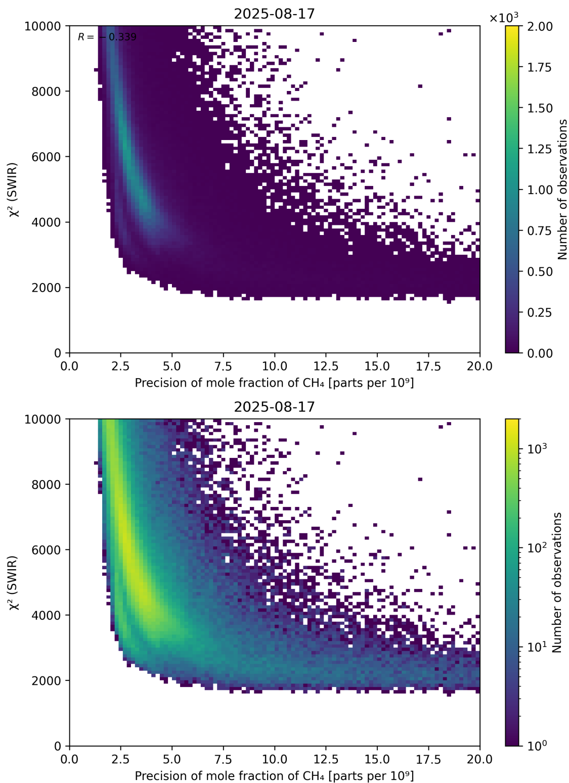
Figure 79: Scatter density plot of “Precision of mole fraction of \text{CH}_4 ” against “ \chi^2 (SWIR)” for 2025-08-16 to 2025-08-18.
