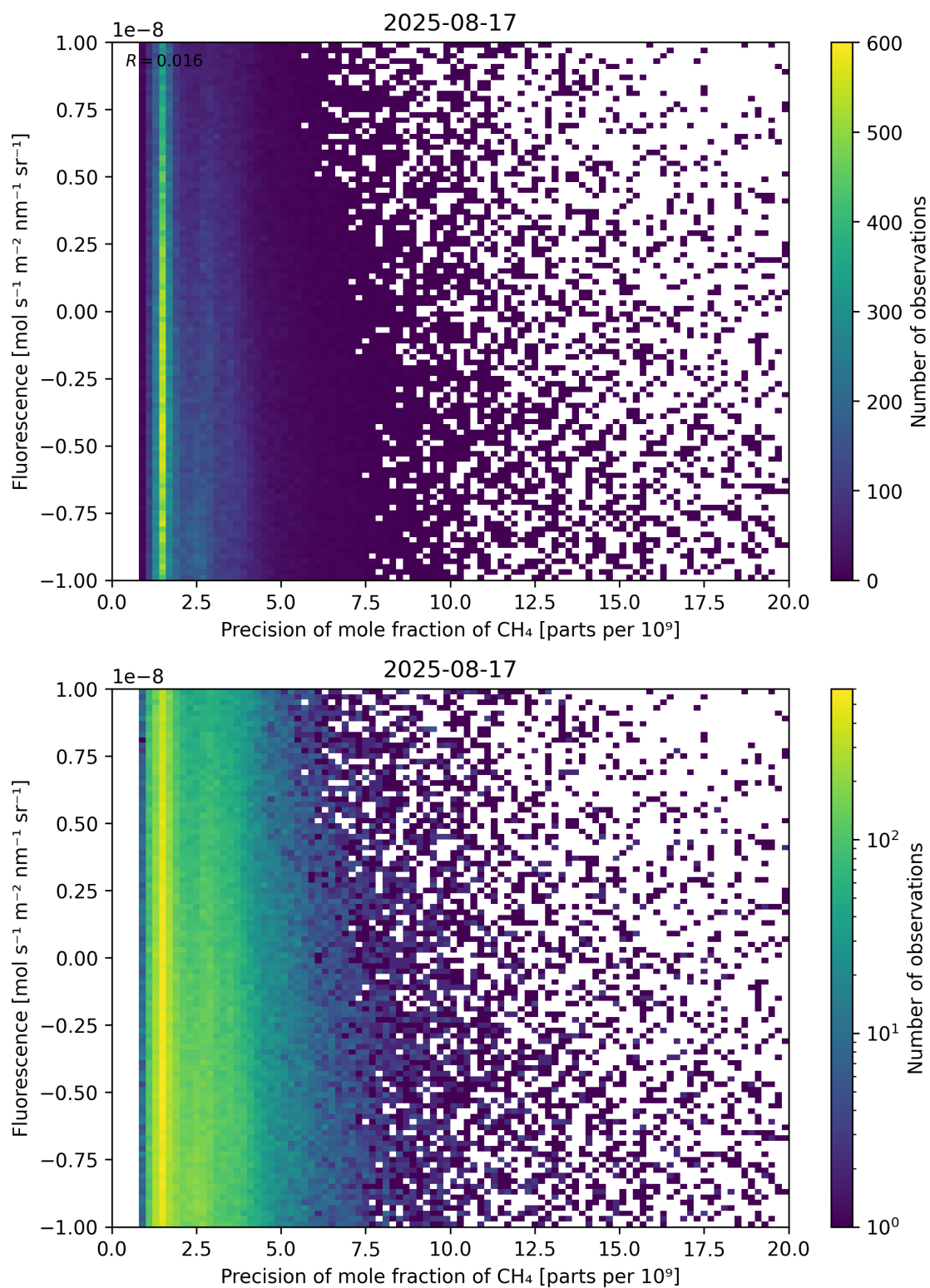
Figure 81: Scatter density plot of “Precision of mole fraction of \text{CH}_4 ” against “Fluorescence” for 2025-08-16 to 2025-08-18.
