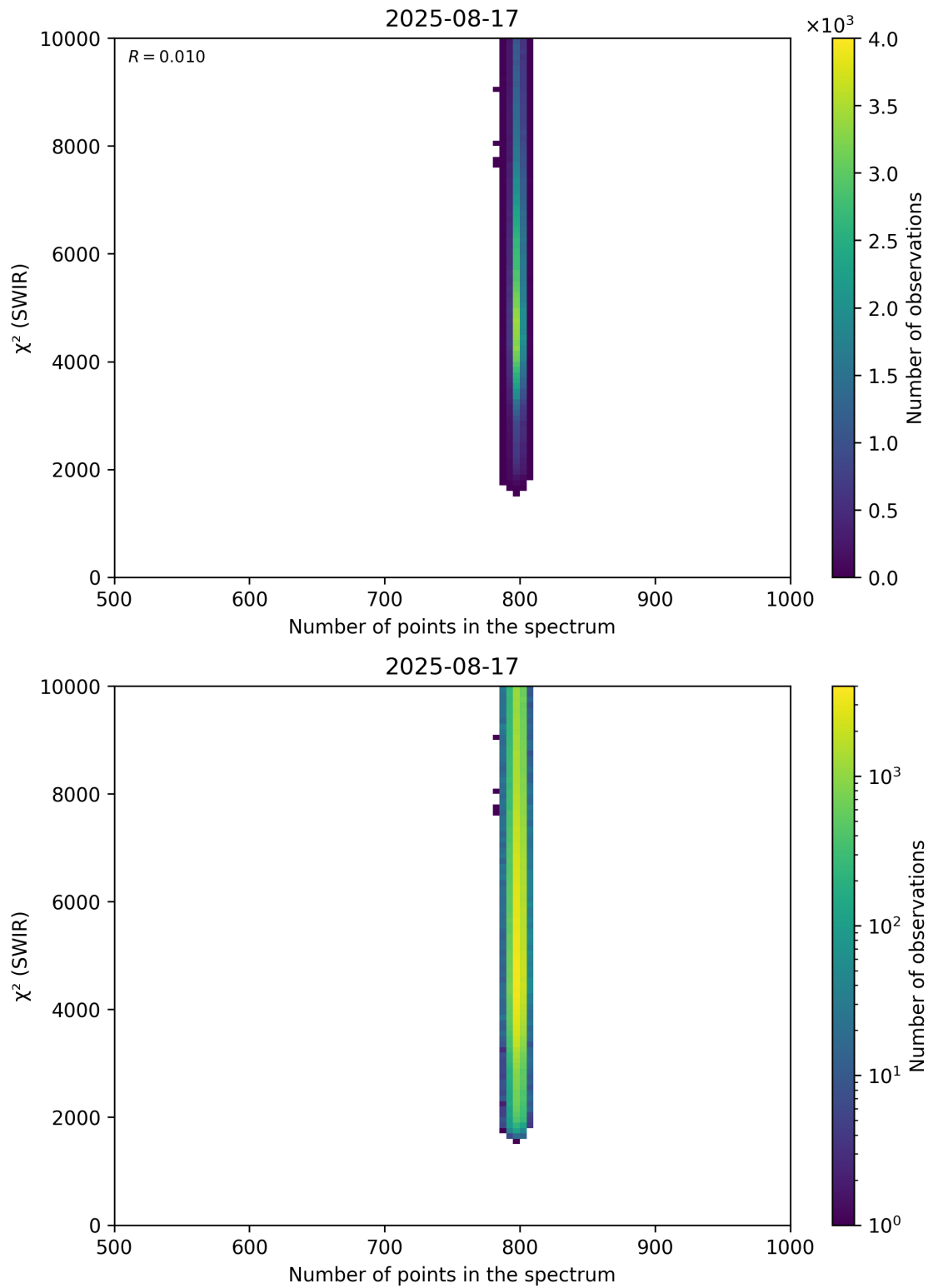
Figure 89: Scatter density plot of “Number of points in the spectrum” against “ \chi^2 (SWIR)” for 2025-08-16 to 2025-08-18.
