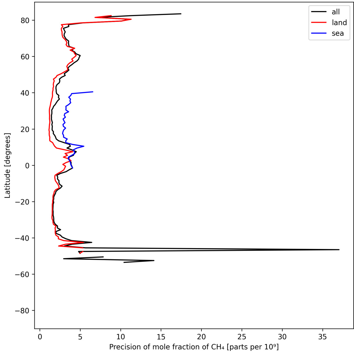
Figure 13: Zonal average of “Precision of mole fraction of CH 4 ” for 2025-08-16 to 2025-08-18.
