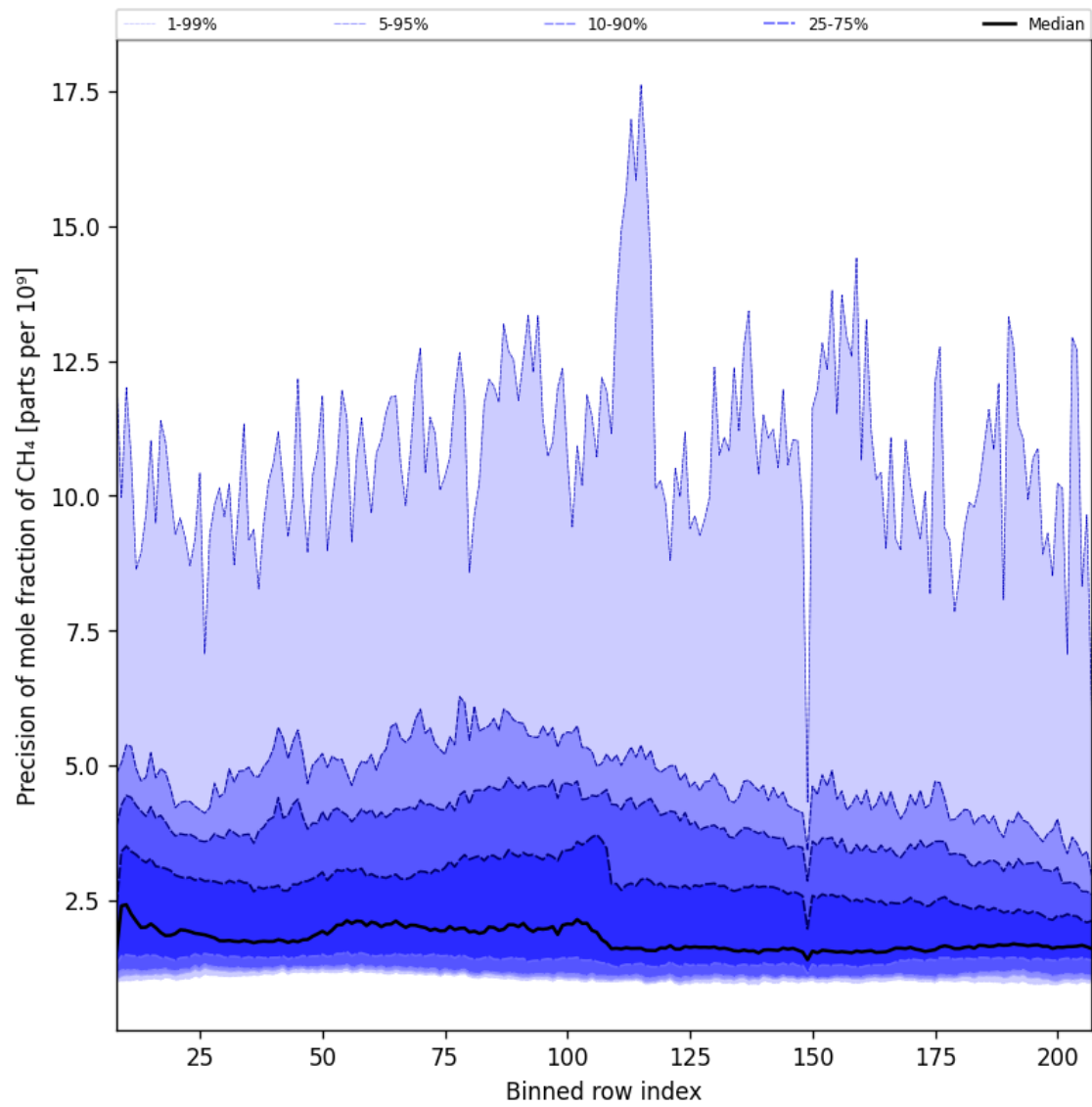
Figure 35: Along track statistics of “Precision of mole fraction of CH 4 ” for 2025-08-16 to 2025-08-18
