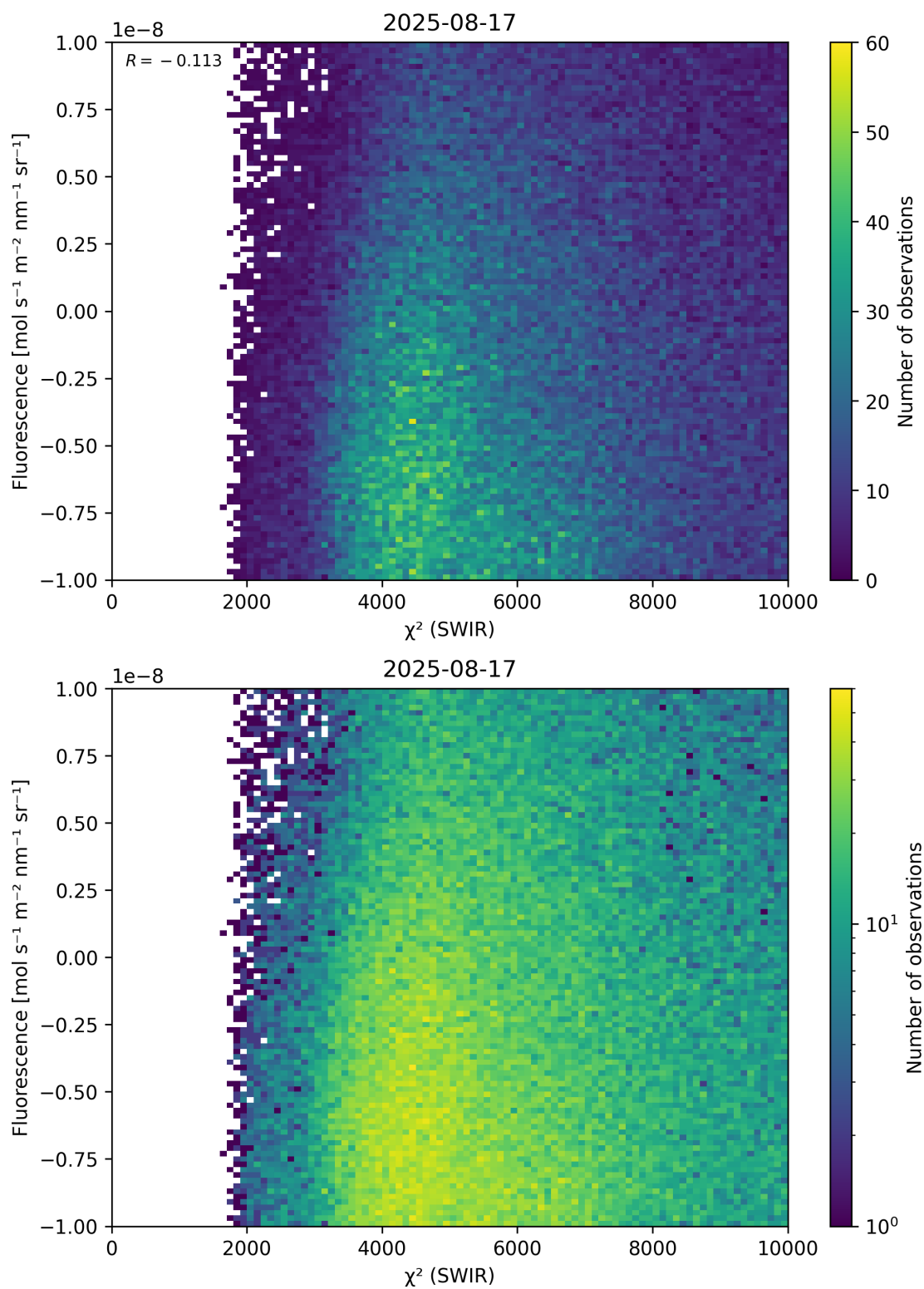
Figure 49: Scatter density plot of “ \chi^2 (SWIR)” against “Fluorescence” for 2025-08-16 to 2025-08-18.
