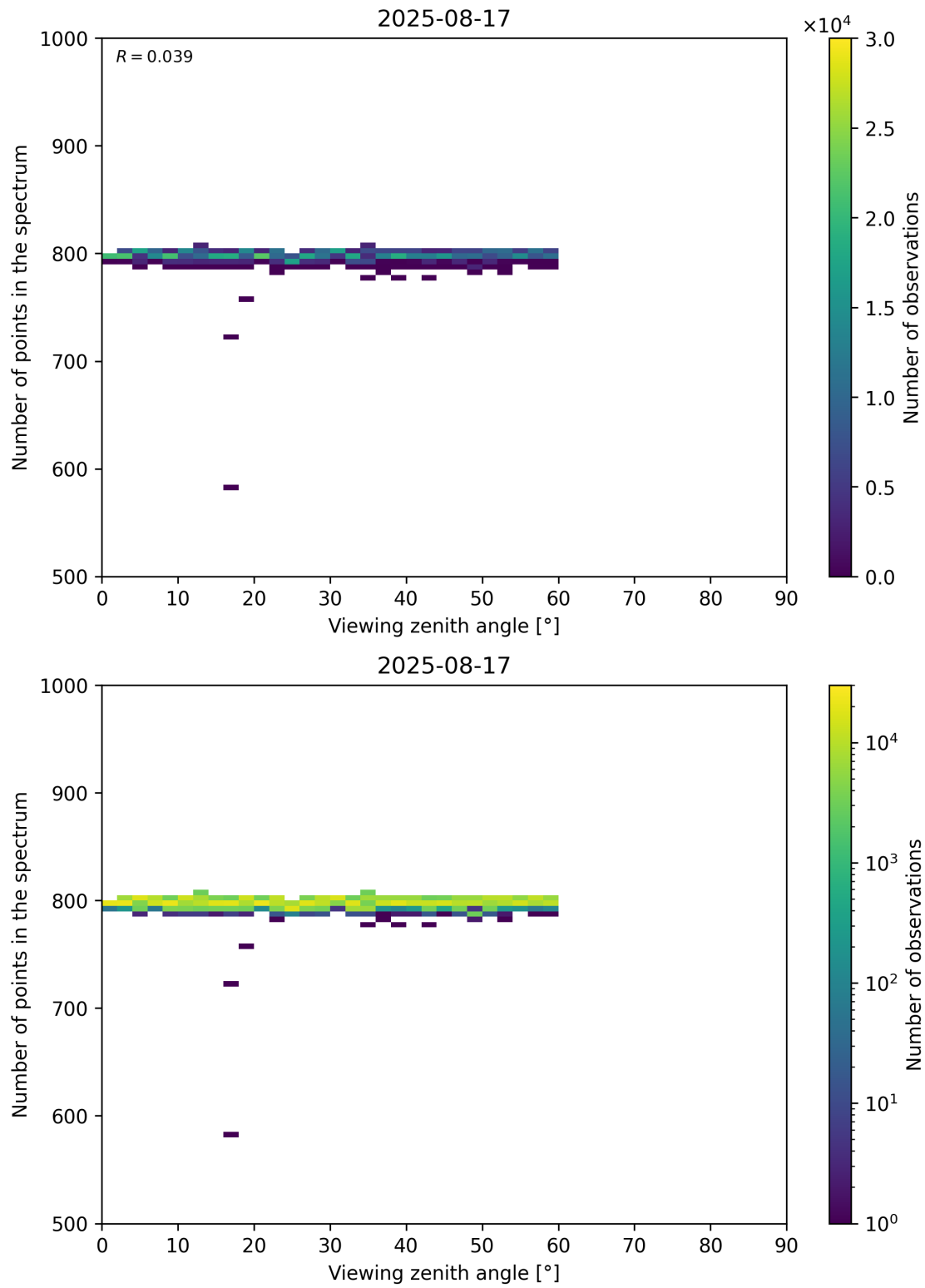
Figure 114: Scatter density plot of “Viewing zenith angle” against “Number of points in the spectrum” for 2025-08-16 to 2025-08-18.
