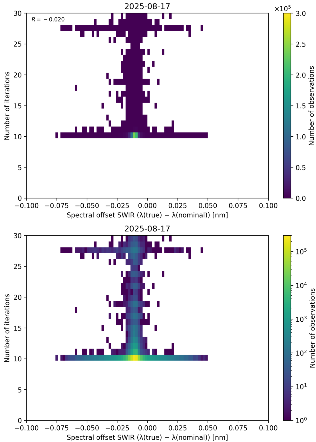
Figure 121: Scatter density plot of “Spectral offset SWIR ( \lambda_{\text{true}} - \lambda_{\text{nominal}} )” against “Number of iterations” for 2025-08-16 to 2025-08-18.
