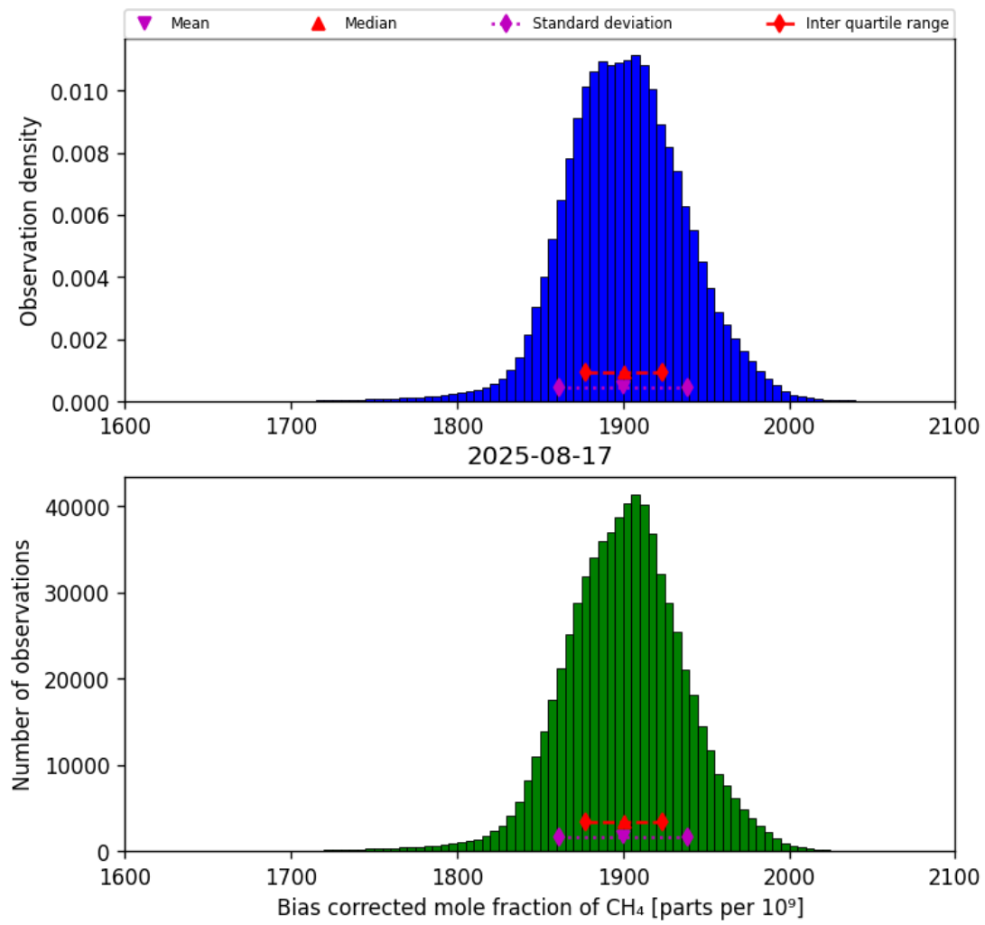
Figure 25: Histogram of “Bias corrected mole fraction of CH 4 ” for 2025-08-16 to 2025-08-18
