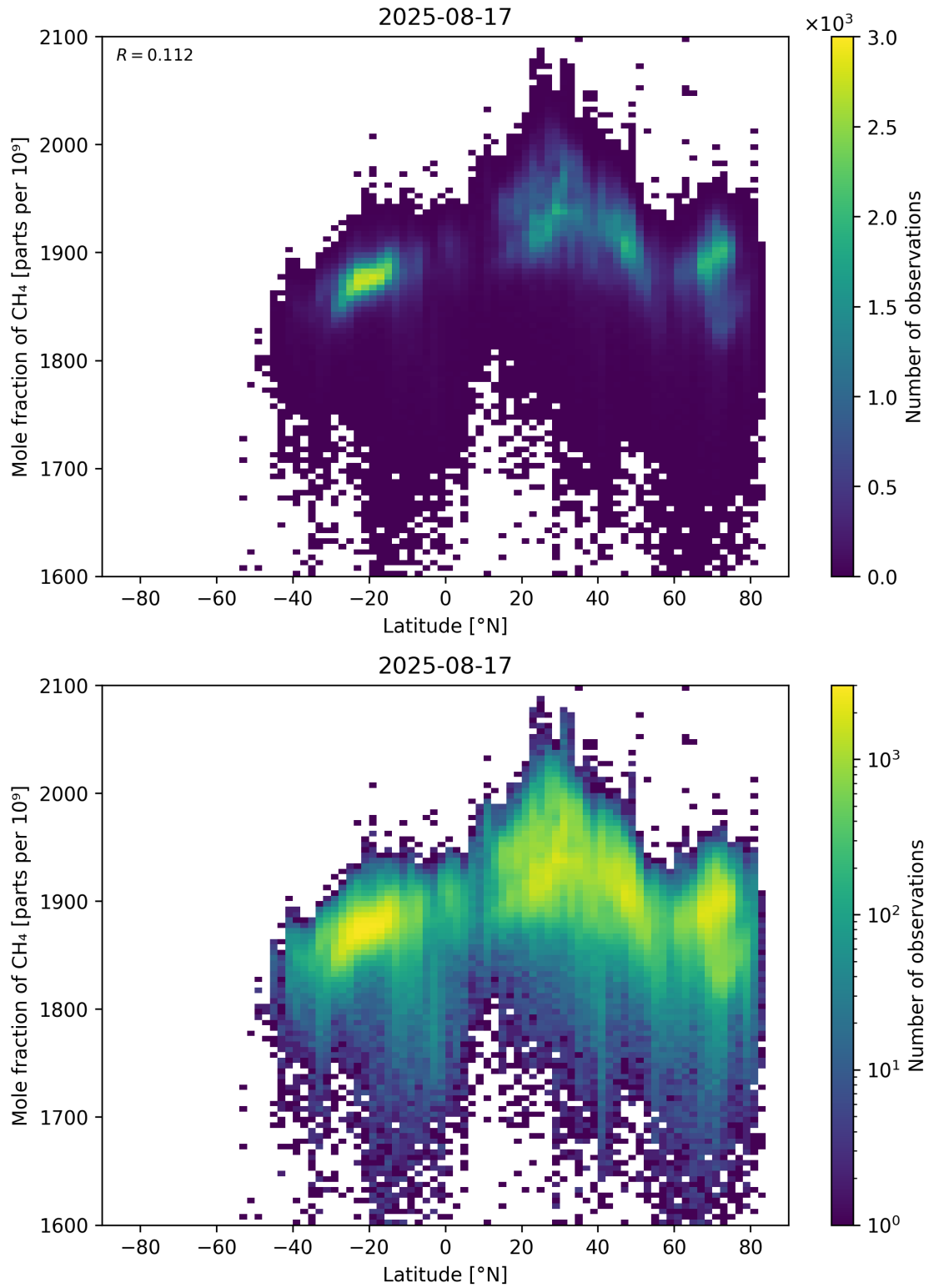
Figure 57: Scatter density plot of “Latitude” against “Mole fraction of \text{CH}_4 ” for 2025-08-16 to 2025-08-18.
