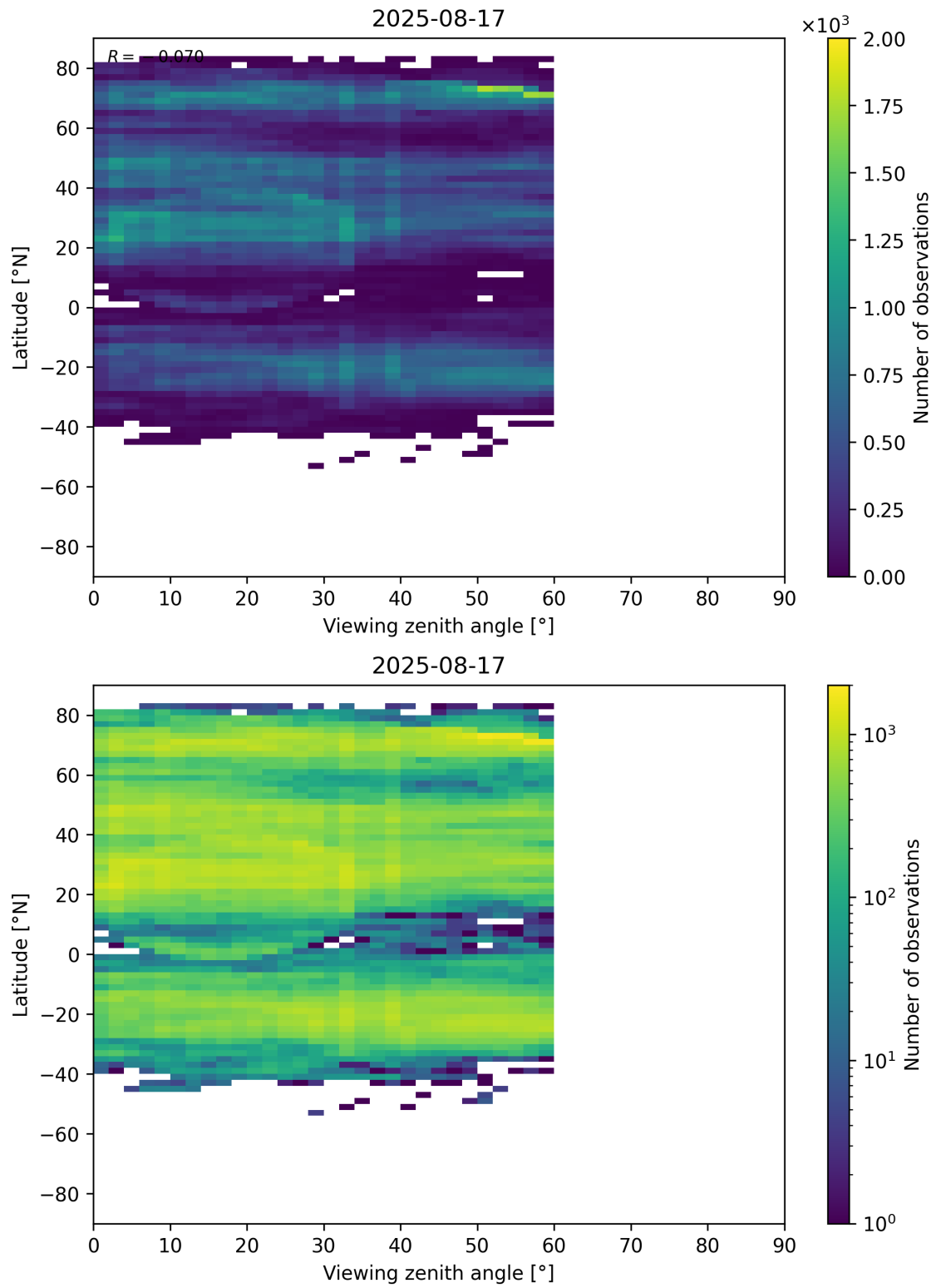
Figure 109: Scatter density plot of “Viewing zenith angle” against “Latitude” for 2025-08-16 to 2025-08-18.
