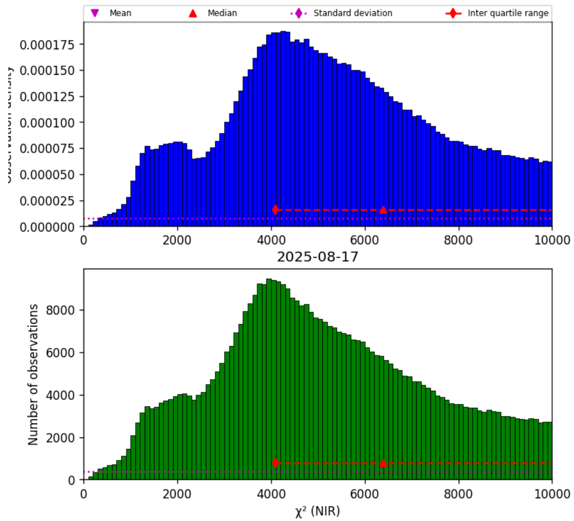
Figure 29: Histogram of “ \chi^2 (NIR)” for 2025-08-16 to 2025-08-18
