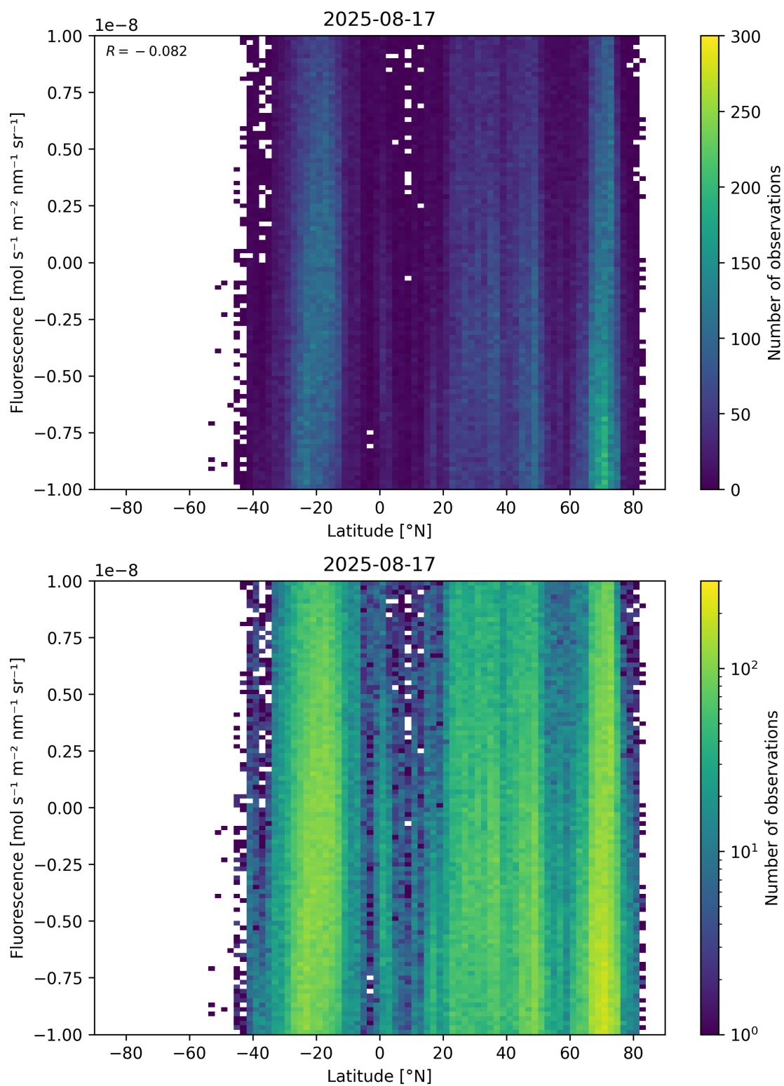
Figure 56: Scatter density plot of “Latitude” against “Fluorescence” for 2025-08-16 to 2025-08-18.
