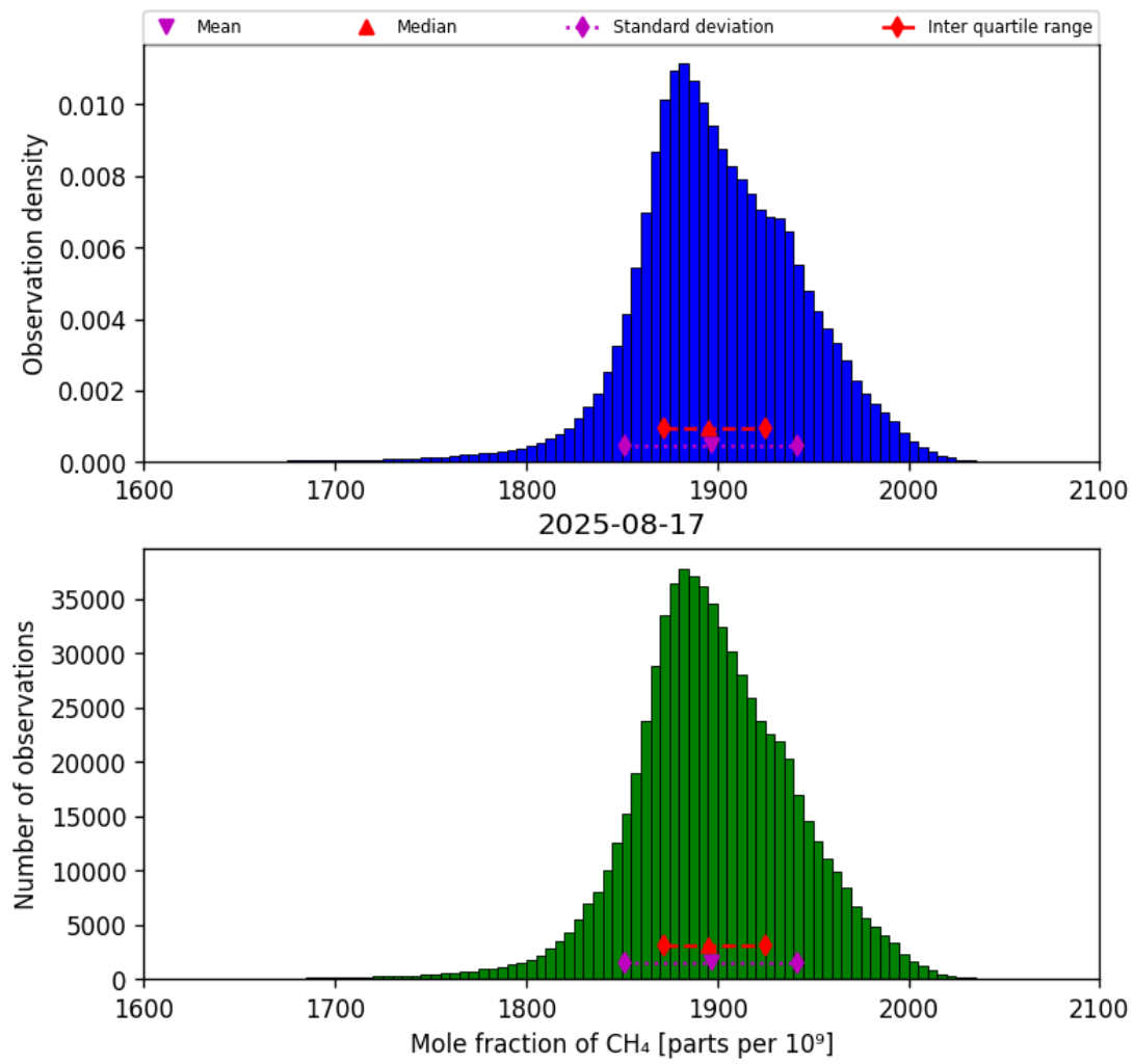
Figure 23: Histogram of “Mole fraction of CH 4 ” for 2025-08-16 to 2025-08-18
