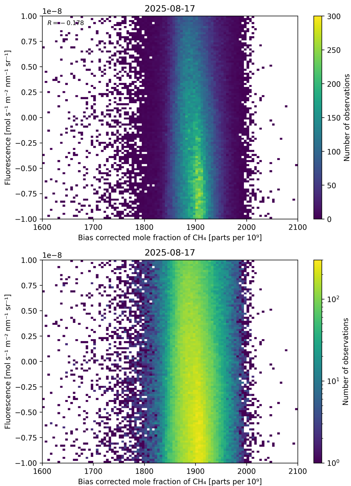
Figure 66: Scatter density plot of “Bias corrected mole fraction of \text{CH}_4 ” against “Fluorescence” for 2025-08-16 to 2025-08-18.
