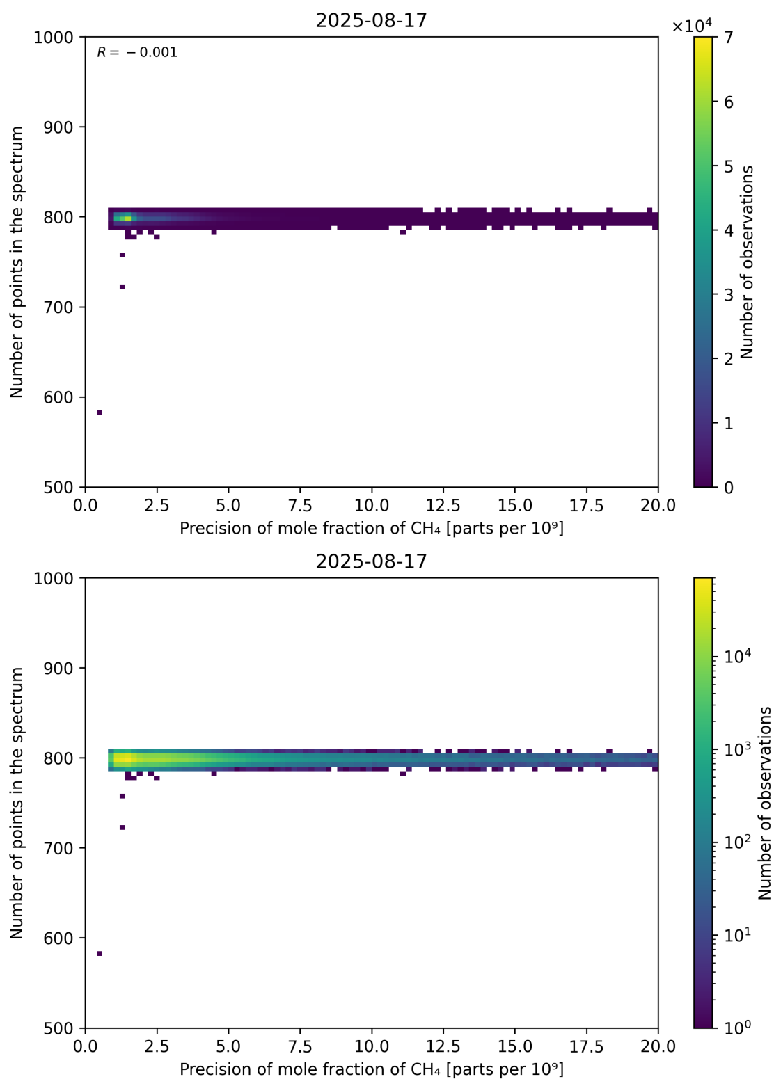
Figure 84: Scatter density plot of “Precision of mole fraction of CH 4 ” against “Number of points in the spectrum” for 2025-08-16 to 2025-08-18.
