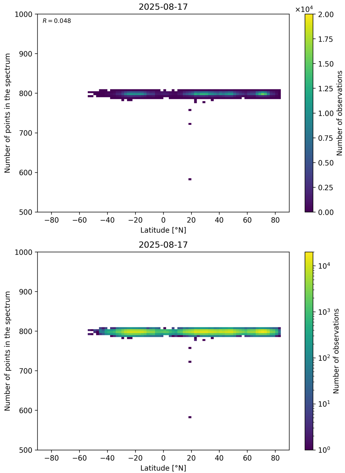
Figure 61: Scatter density plot of “Latitude” against “Number of points in the spectrum” for 2025-08-16 to 2025-08-18.
