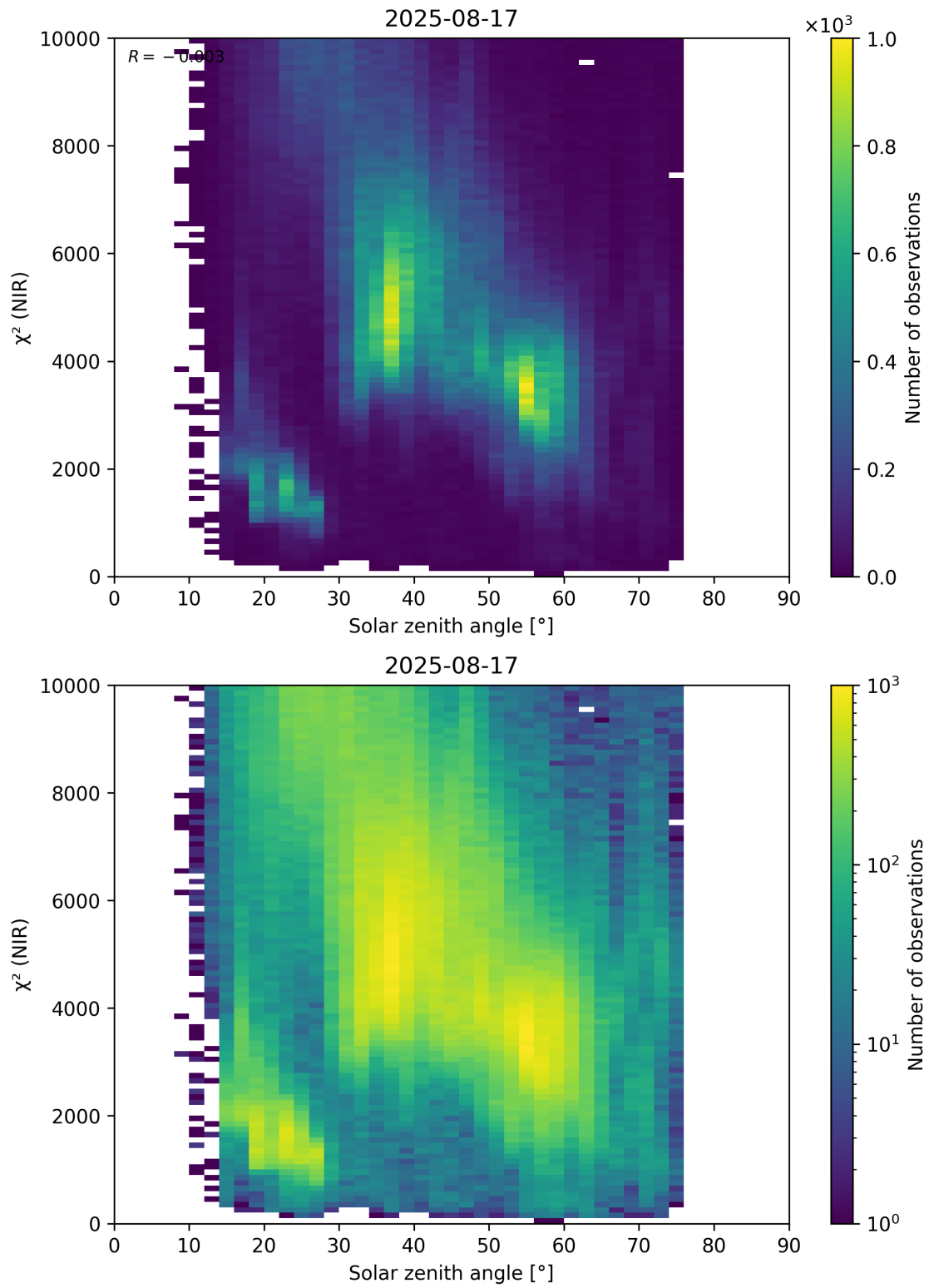
Figure 94: Scatter density plot of “Solar zenith angle” against “ \chi^2 (NIR)” for 2025-08-16 to 2025-08-18.
