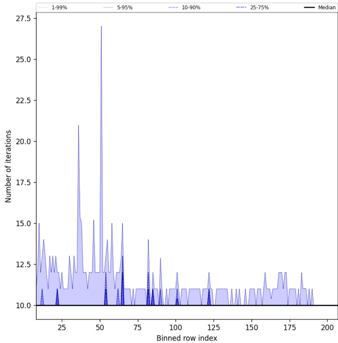
Figure 42: Along track statistics of “Number of iterations” for 2025-08-16 to 2025-08-18
