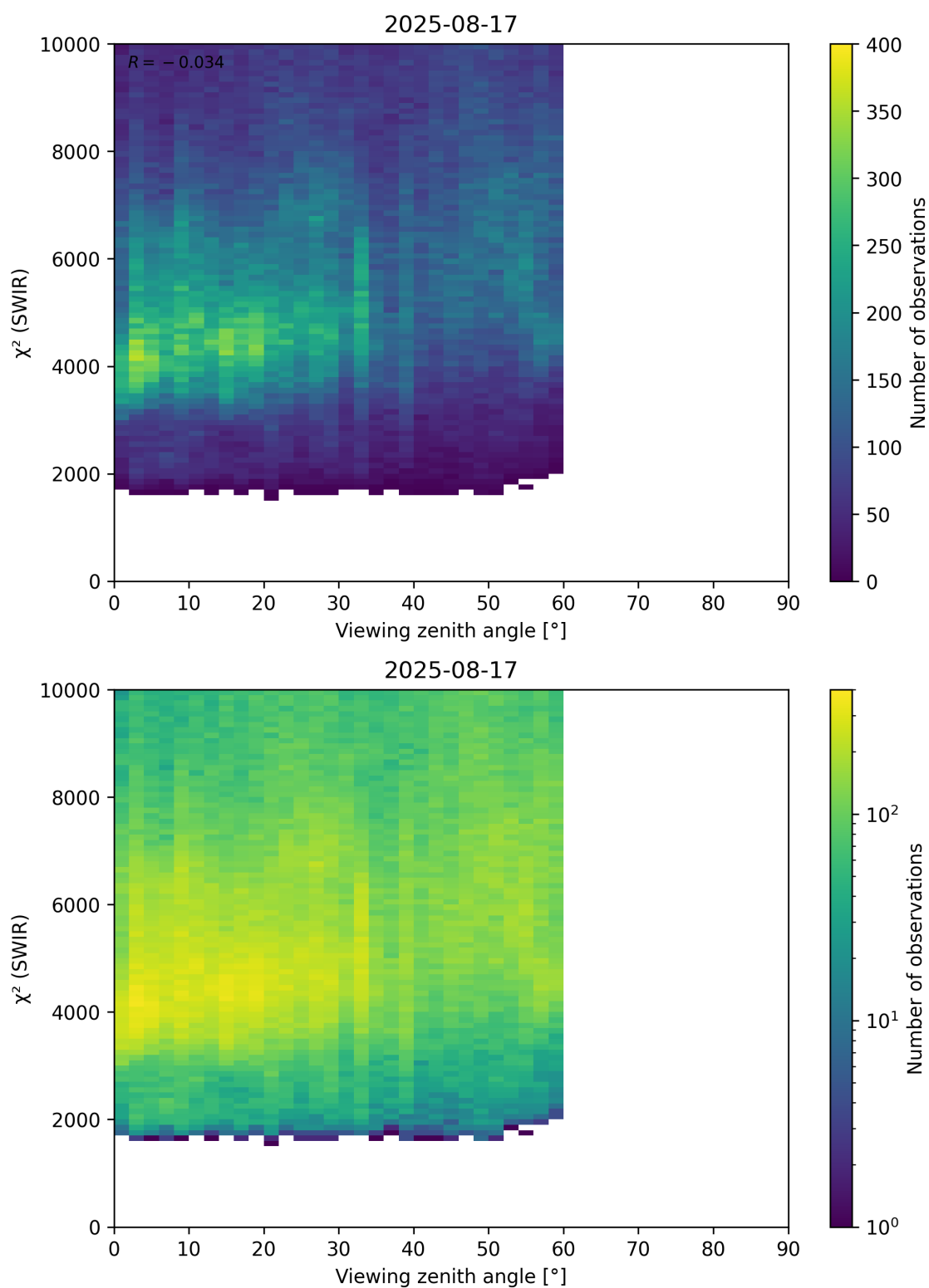
Figure 106: Scatter density plot of “Viewing zenith angle” against “ \chi^2 (SWIR)” for 2025-08-16 to 2025-08-18.
