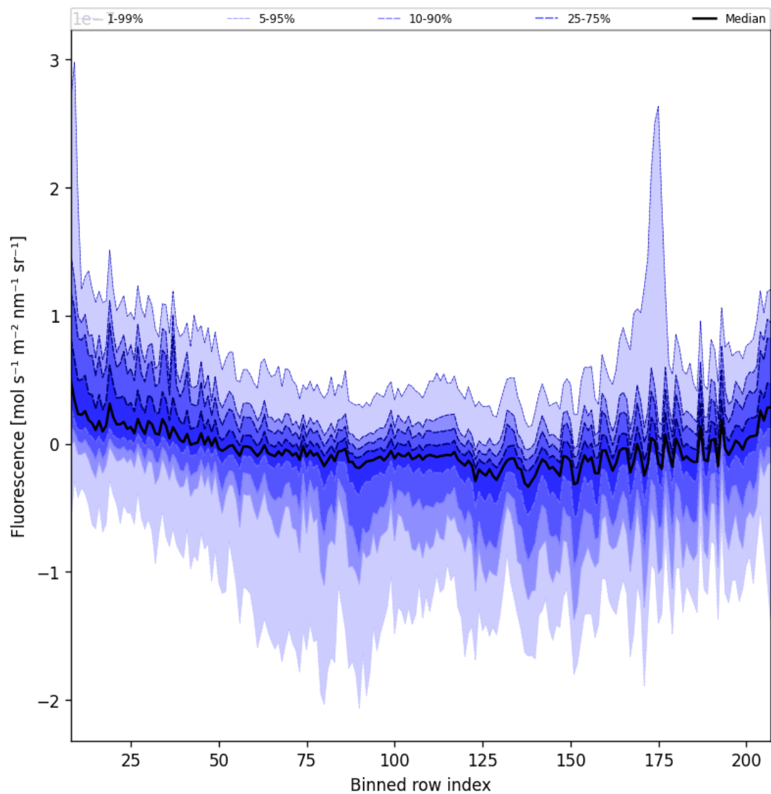
Figure 43: Along track statistics of “Fluorescence” for 2025-08-16 to 2025-08-18
