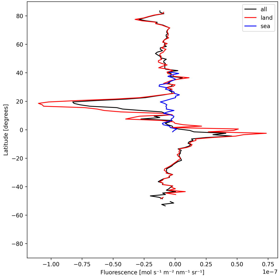
Figure 21: Zonal average of “Fluorescence” for 2025-08-16 to 2025-08-18.
