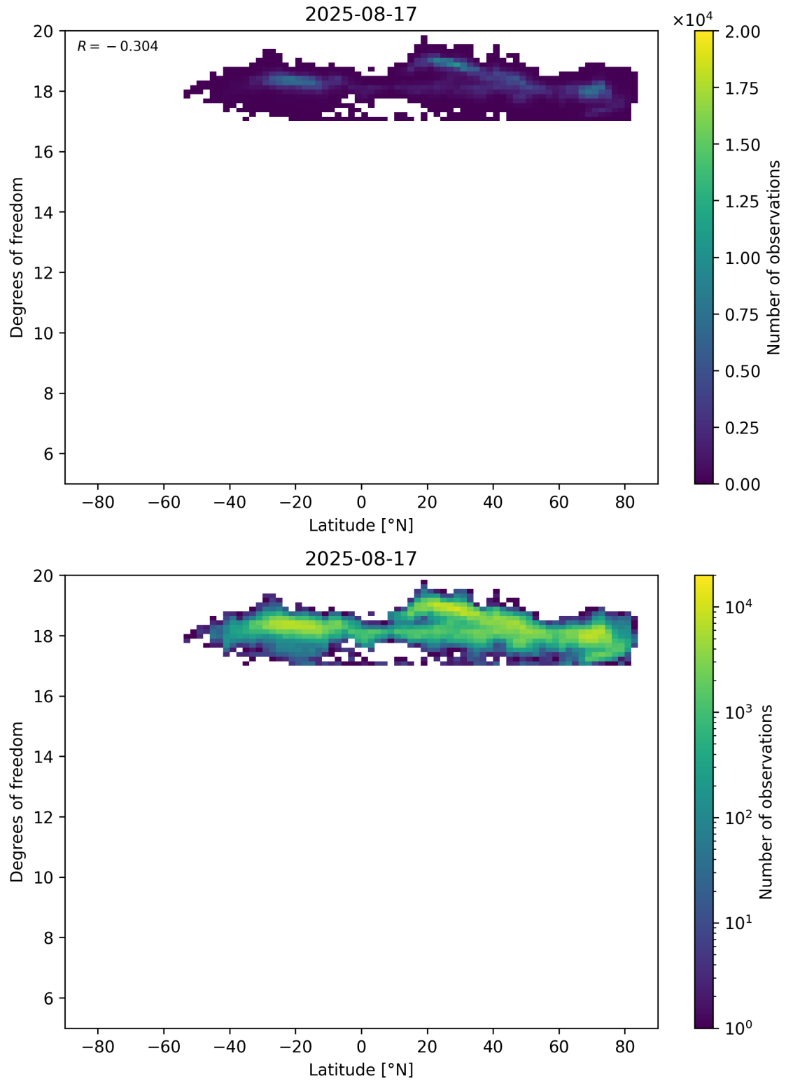
Figure 55: Scatter density plot of “Latitude” against “Degrees of freedom” for 2025-08-16 to 2025-08-18.
