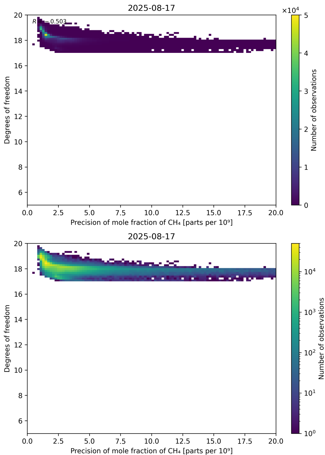
Figure 80: Scatter density plot of “Precision of mole fraction of CH 4 ” against “Degrees of freedom” for 2025-08-16 to 2025-08-18.
