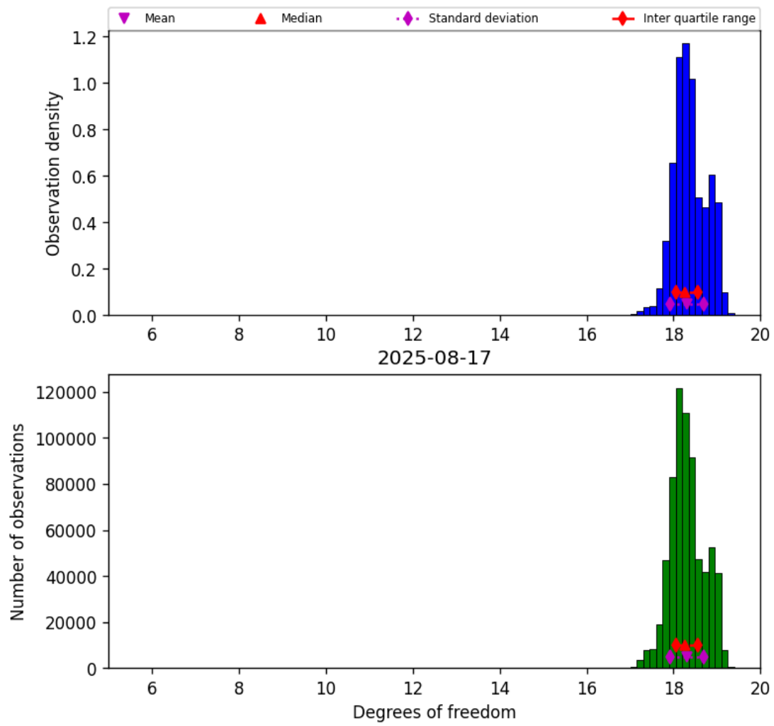
Figure 30: Histogram of “Degrees of freedom” for 2025-08-16 to 2025-08-18
