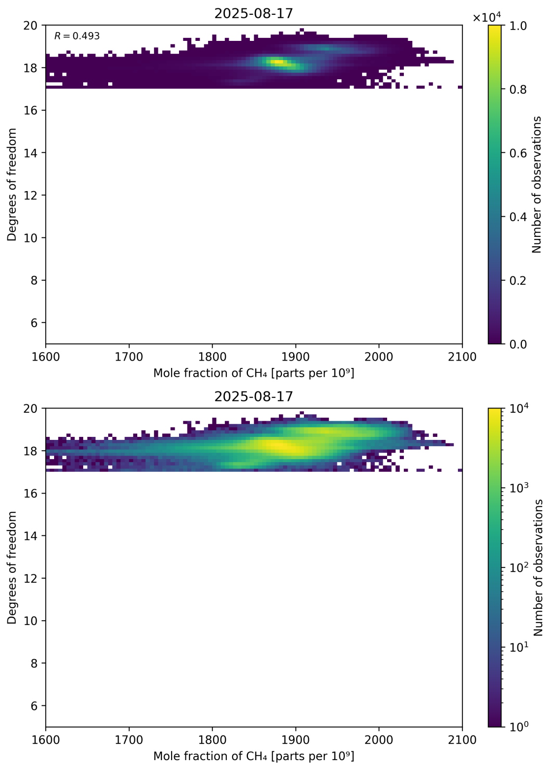
Figure 72: Scatter density plot of “Mole fraction of CH 4 ” against “Degrees of freedom” for 2025-08-16 to 2025-08-18.
