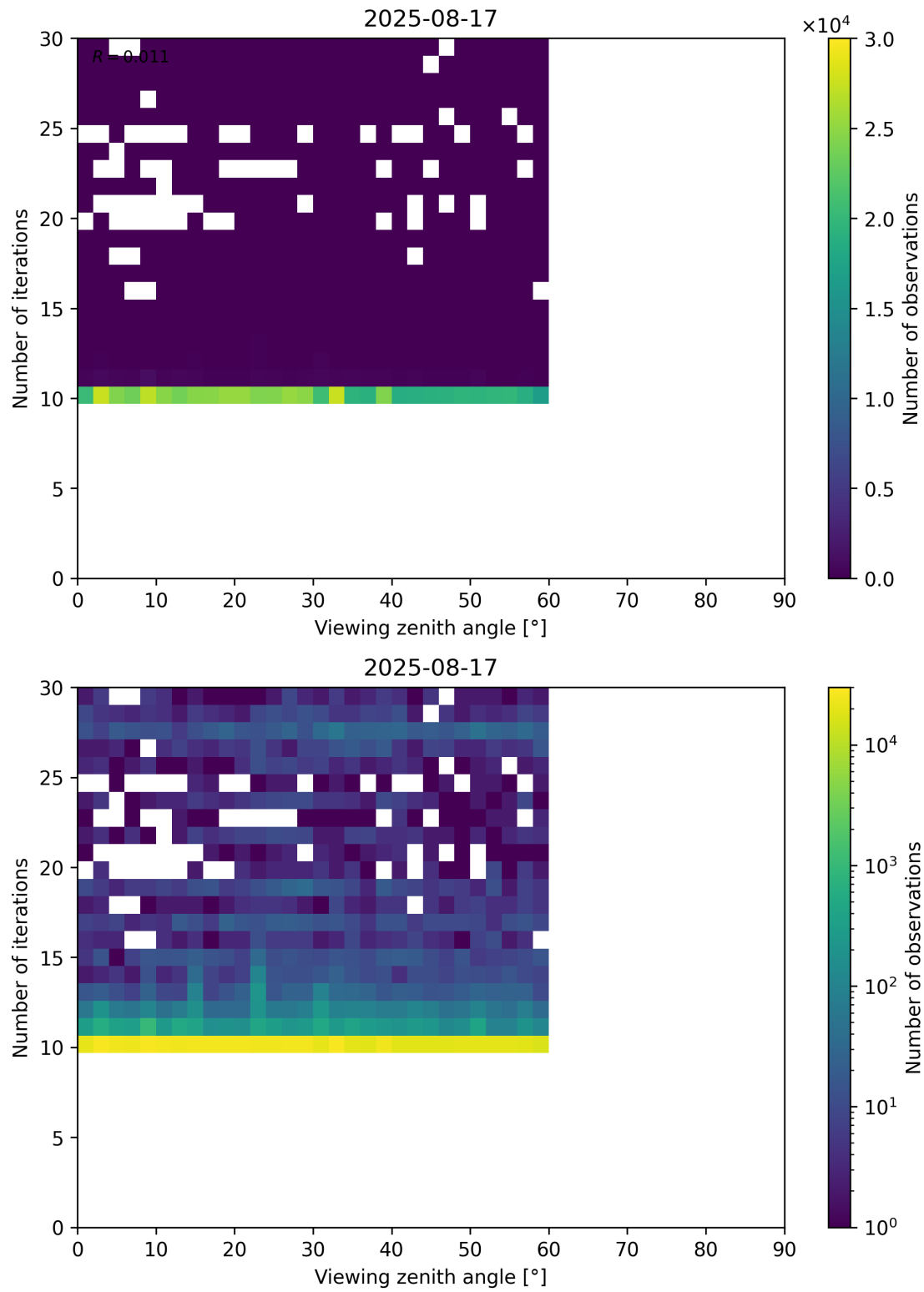
Figure 113: Scatter density plot of “Viewing zenith angle” against “Number of iterations” for 2025-08-16 to 2025-08-18.
