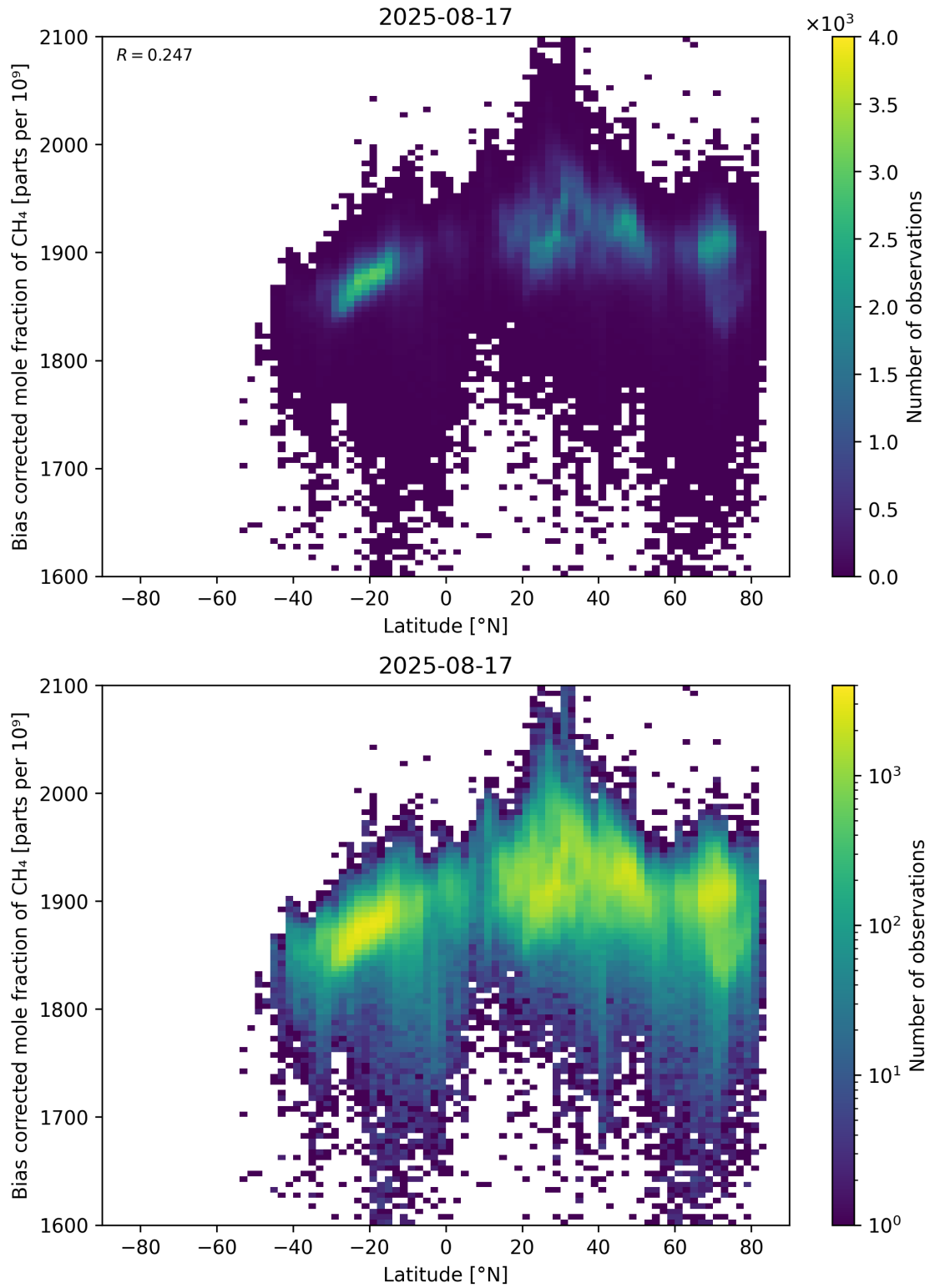
Figure 58: Scatter density plot of “Latitude” against “Bias corrected mole fraction of \text{CH}_4 ” for 2025-08-16 to 2025-08-18.
