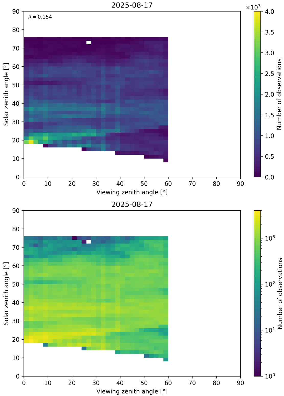
Figure 115: Scatter density plot of “Viewing zenith angle” against “Solar zenith angle” for 2025-08-16 to 2025-08-18.
