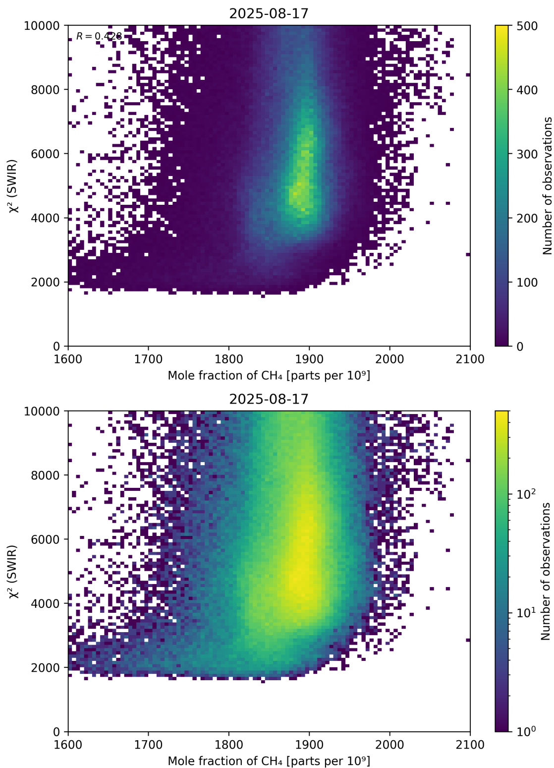
Figure 71: Scatter density plot of “Mole fraction of CH 4 ” against “ \chi^2 (SWIR)” for 2025-08-16 to 2025-08-18.
