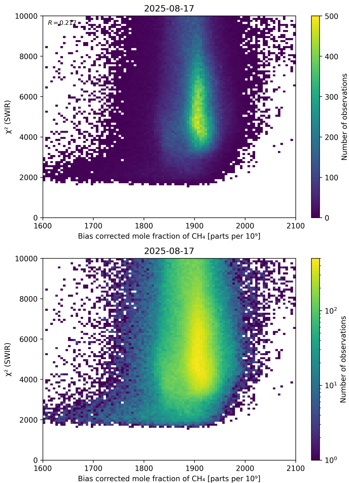
Figure 64: Scatter density plot of “Bias corrected mole fraction of \text{CH}_4 ” against “ \chi^2 (SWIR)” for 2025-08-16 to 2025-08-18.
