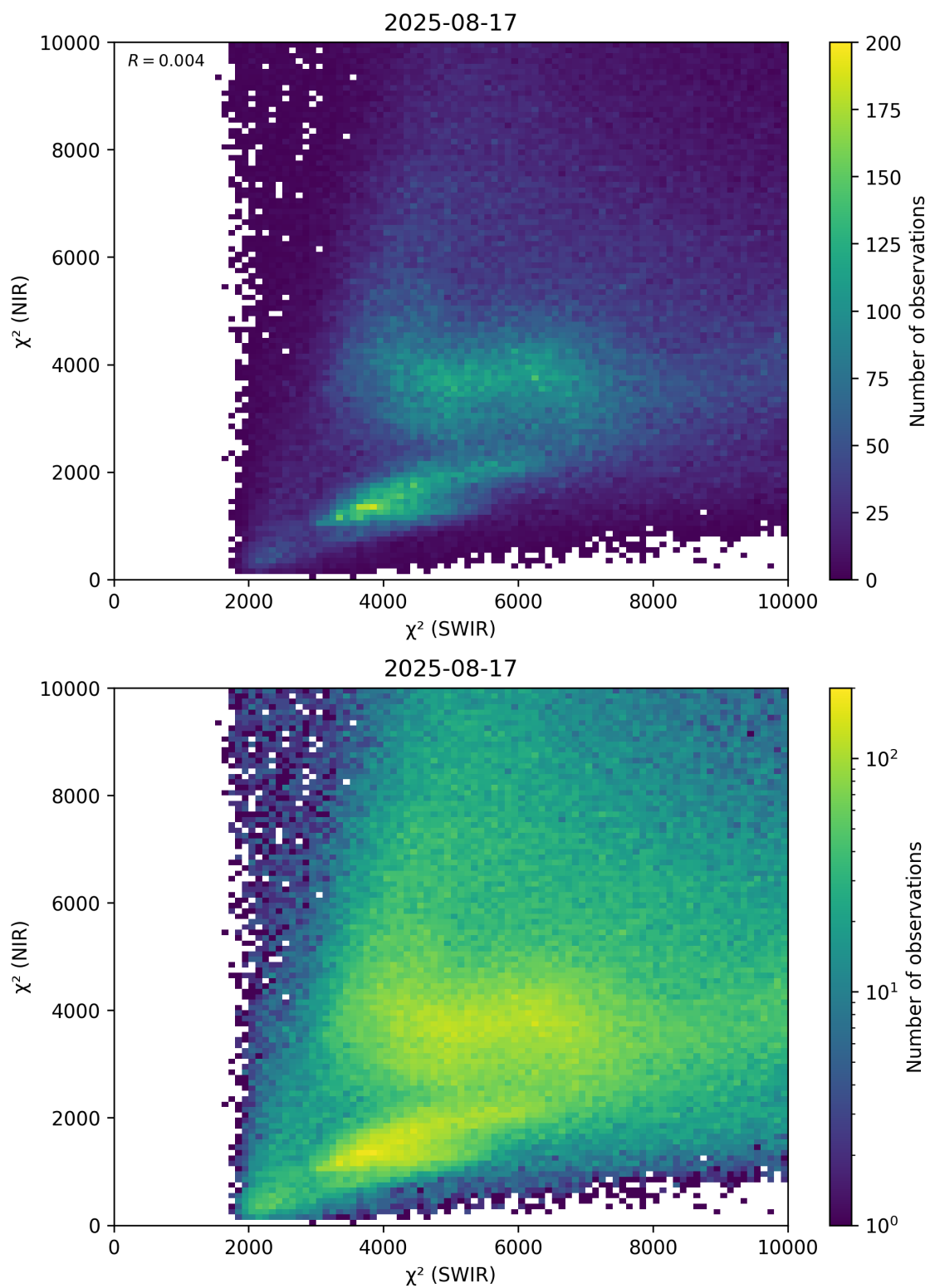
Figure 47: Scatter density plot of “ \chi^2 (SWIR)” against “ \chi^2 (NIR)” for 2025-08-16 to 2025-08-18.
