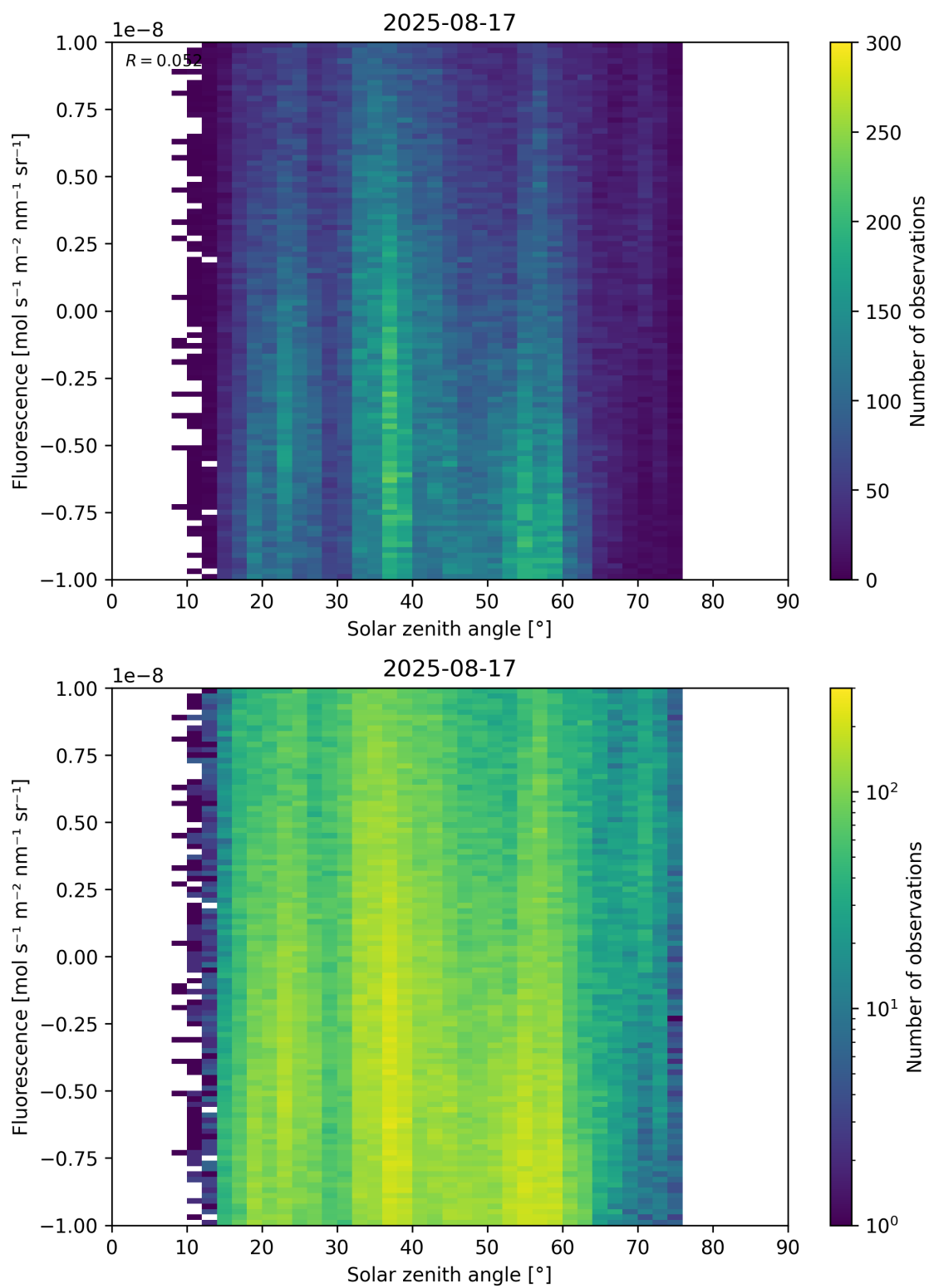
Figure 97: Scatter density plot of “Solar zenith angle” against “Fluorescence” for 2025-08-16 to 2025-08-18.
