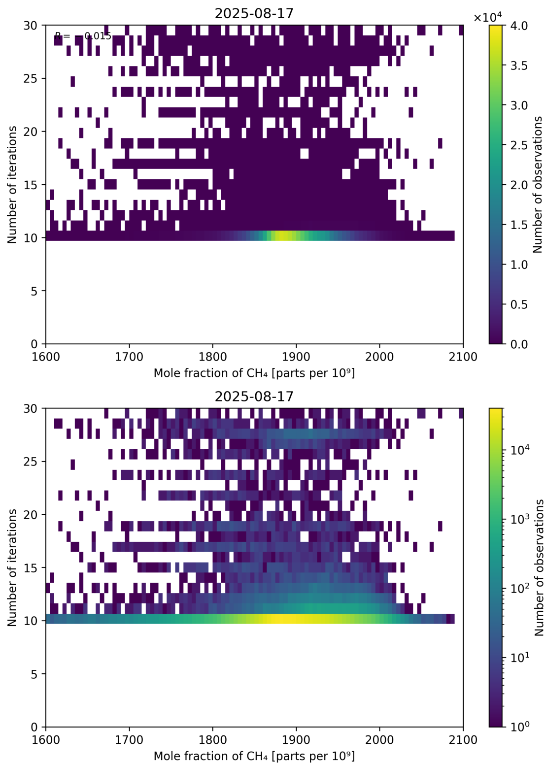
Figure 76: Scatter density plot of “Mole fraction of CH 4 ” against “Number of iterations” for 2025-08-16 to 2025-08-18.
