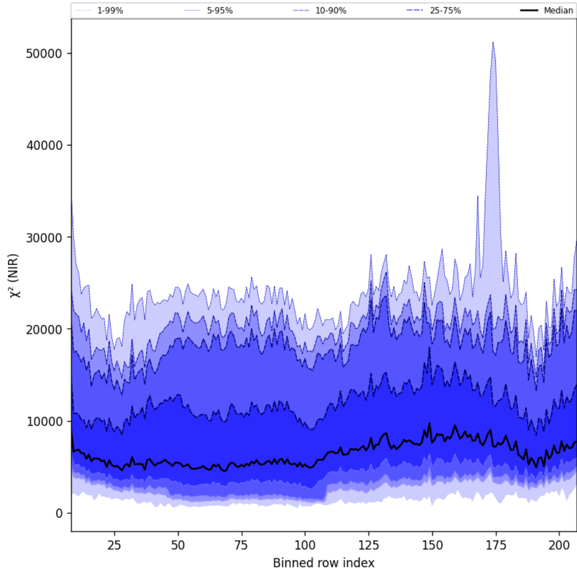
Figure 40: Along track statistics of “ \chi^2 (NIR)” for 2025-08-16 to 2025-08-18
