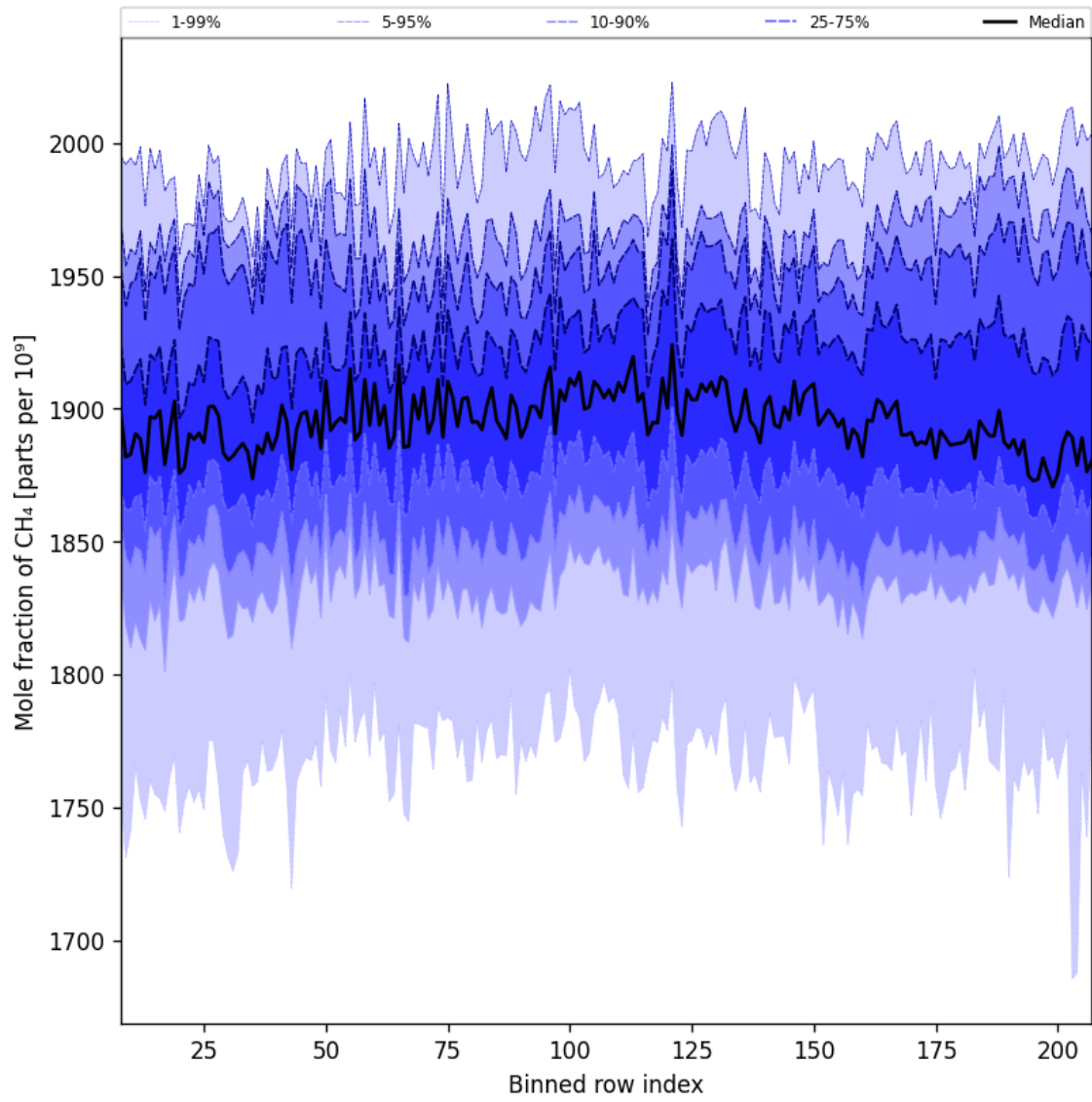
Figure 34: Along track statistics of “Mole fraction of CH 4 ” for 2025-08-16 to 2025-08-18
