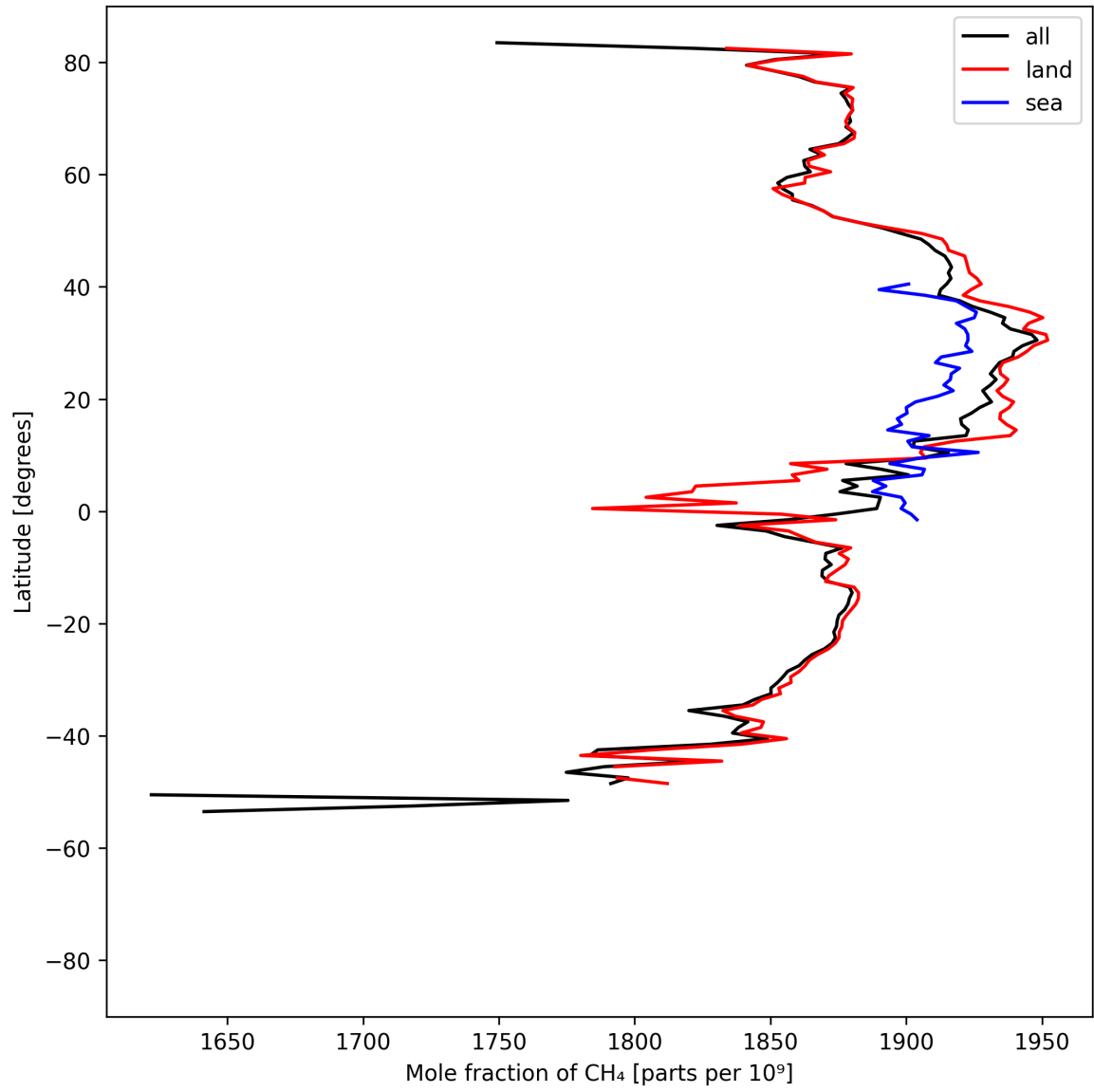
Figure 12: Zonal average of “Mole fraction of \text{CH}_4 ” for 2025-08-16 to 2025-08-18.
