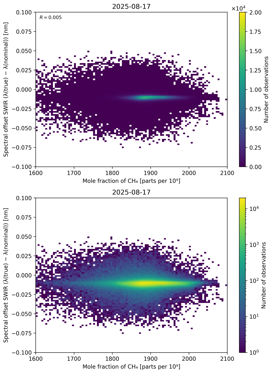
Figure 86: Scatter density plot of “Mole fraction of CH 4 ” against “Spectral offset SWIR ( \lambda_{\text{true}} - \lambda_{\text{nominal}} )” for 2025-08-16 to 2025-08-18.
