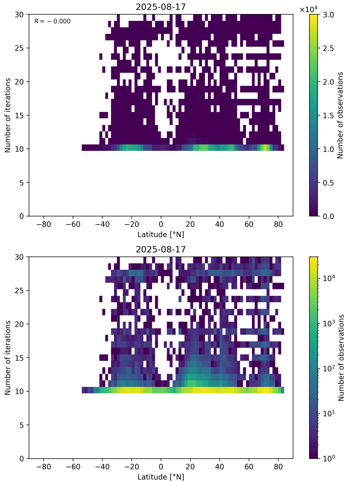
Figure 60: Scatter density plot of “Latitude” against “Number of iterations” for 2025-08-16 to 2025-08-18.
