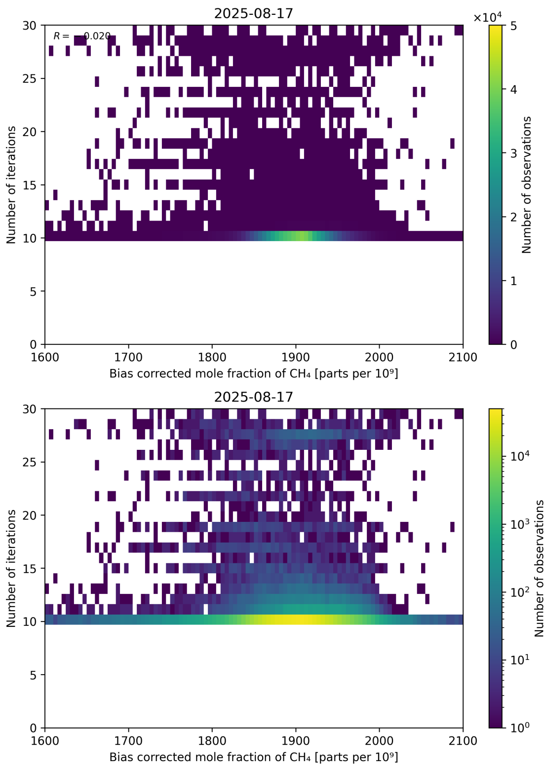
Figure 67: Scatter density plot of “Bias corrected mole fraction of CH 4 ” against “Number of iterations” for 2025-08-16 to 2025-08-18.
