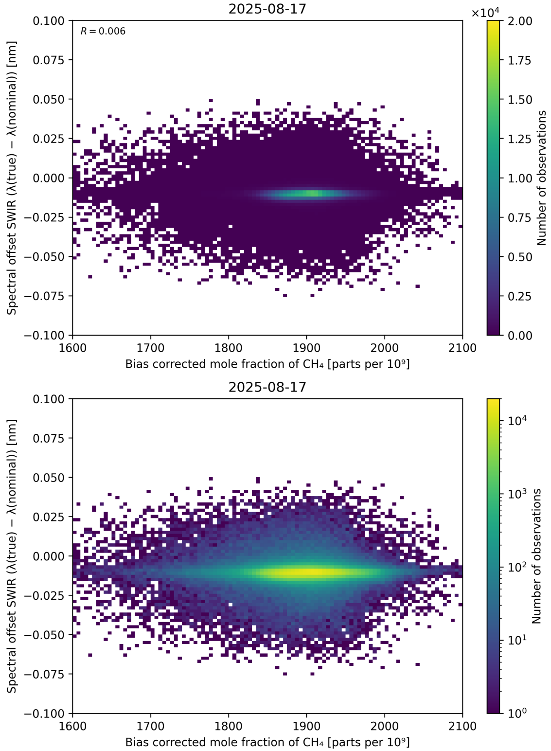
Figure 69: Scatter density plot of “Bias corrected mole fraction of CH 4 ” against “Spectral offset SWIR ( \lambda_{\text{true}} - \lambda_{\text{nominal}} )” for 2025-08-16 to 2025-08-18.
