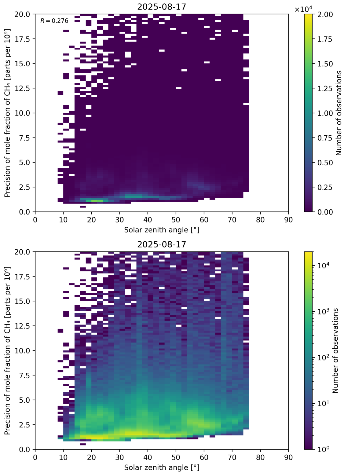
Figure 101: Scatter density plot of “Solar zenith angle” against “Precision of mole fraction of CH 4 ” for 2025-08-16 to 2025-08-18.
