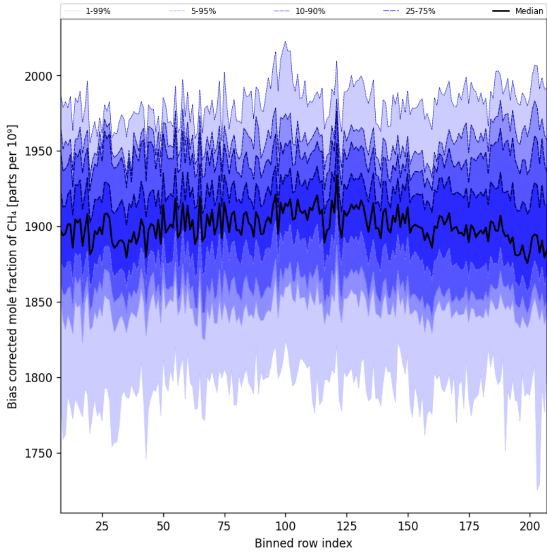
Figure 36: Along track statistics of “Bias corrected mole fraction of CH 4 ” for 2025-08-16 to 2025-08-18
