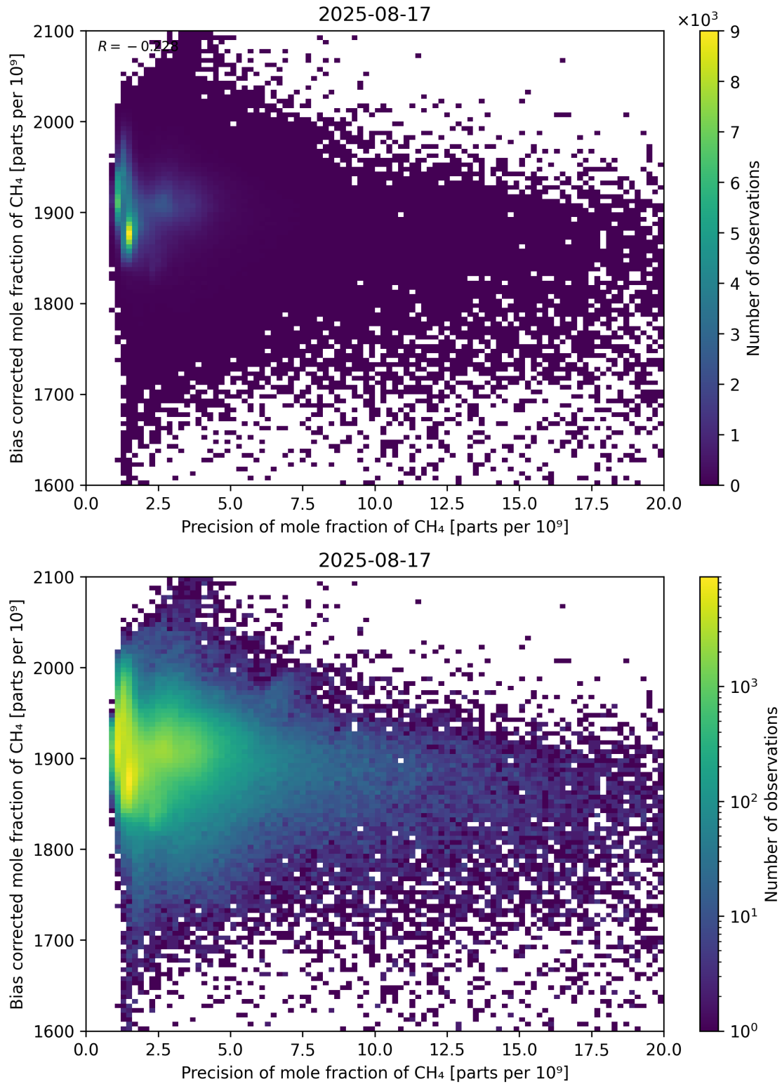
Figure 82: Scatter density plot of “Precision of mole fraction of CH 4 ” against “Bias corrected mole fraction of CH 4 ” for 2025-08-16 to 2025-08-18.
