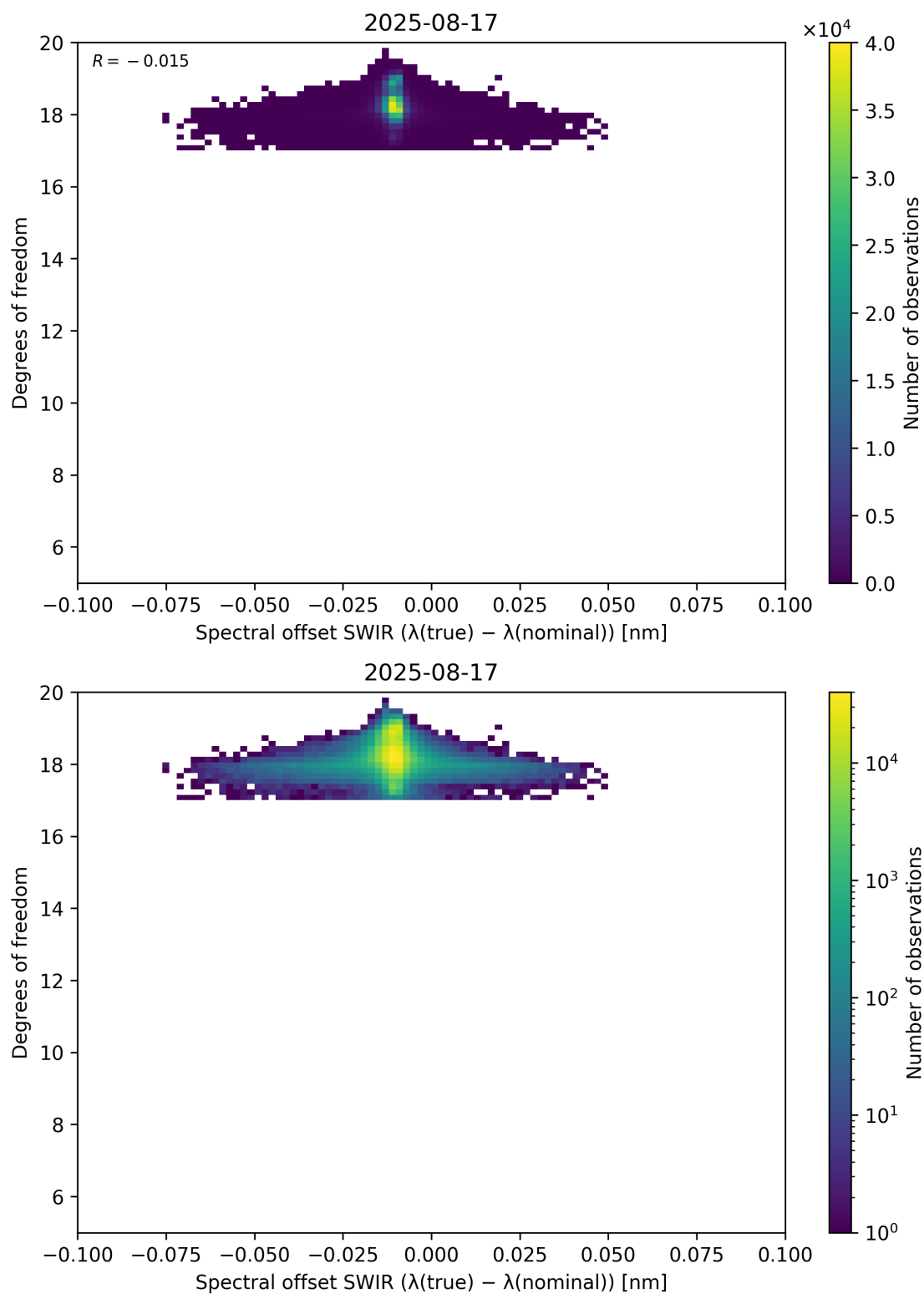
Figure 119: Scatter density plot of “Spectral offset SWIR ( \lambda_{\text{true}} - \lambda_{\text{nominal}} )” against “Degrees of freedom” for 2025-08-16 to 2025-08-18.
