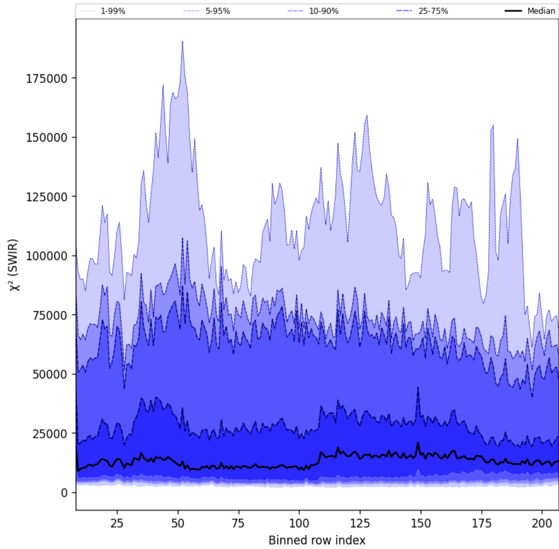
Figure 39: Along track statistics of " \chi^2 (SWIR)" for 2025-08-16 to 2025-08-18
