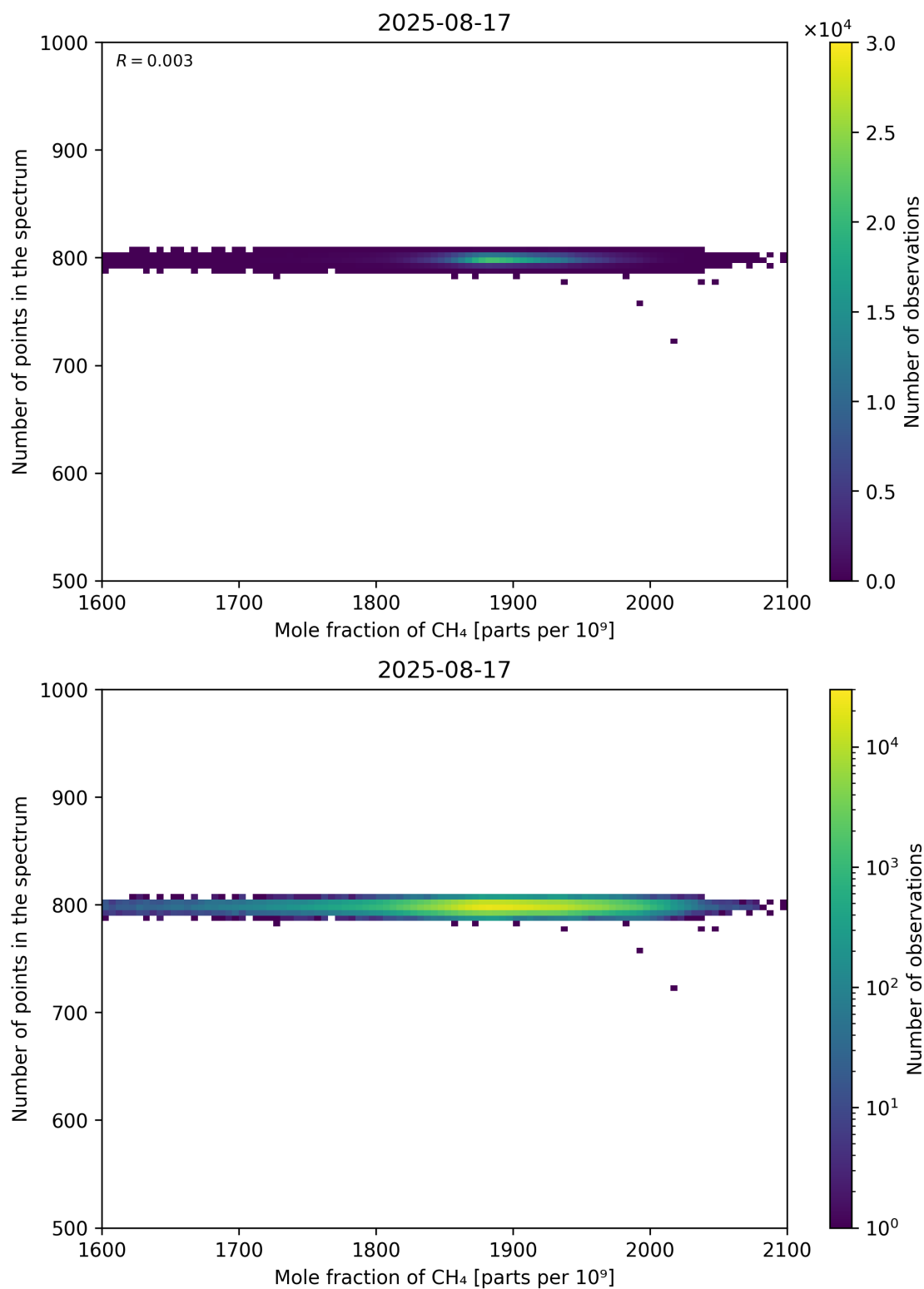
Figure 77: Scatter density plot of “Mole fraction of CH 4 ” against “Number of points in the spectrum” for 2025-08-16 to 2025-08-18.
