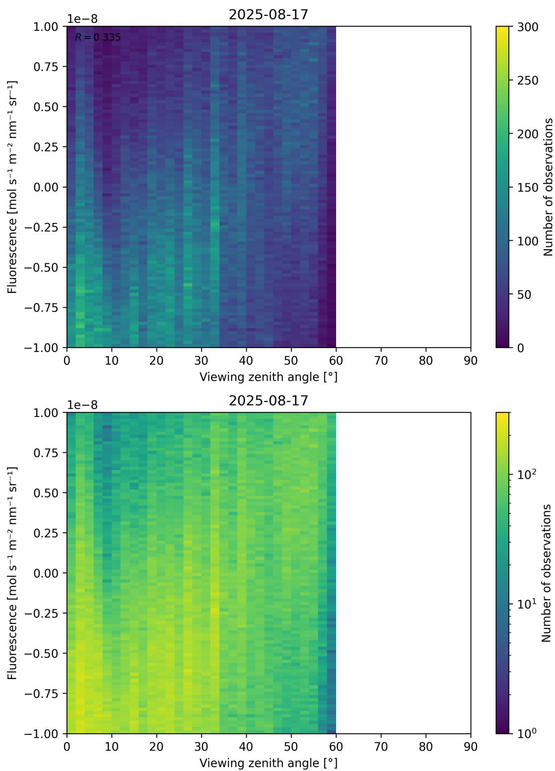
Figure 108: Scatter density plot of “Viewing zenith angle” against “Fluorescence” for 2025-08-16 to 2025-08-18.
