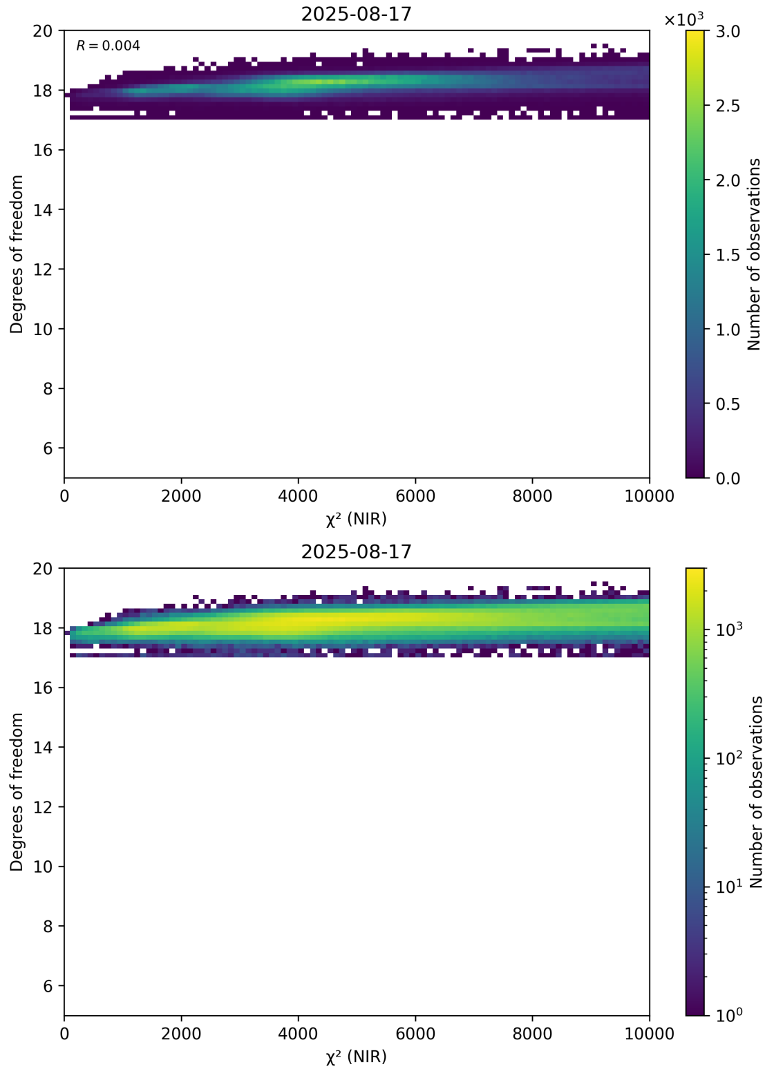
Figure 44: Scatter density plot of “ \chi^2 (NIR)” against “Degrees of freedom” for 2025-08-16 to 2025-08-18.
