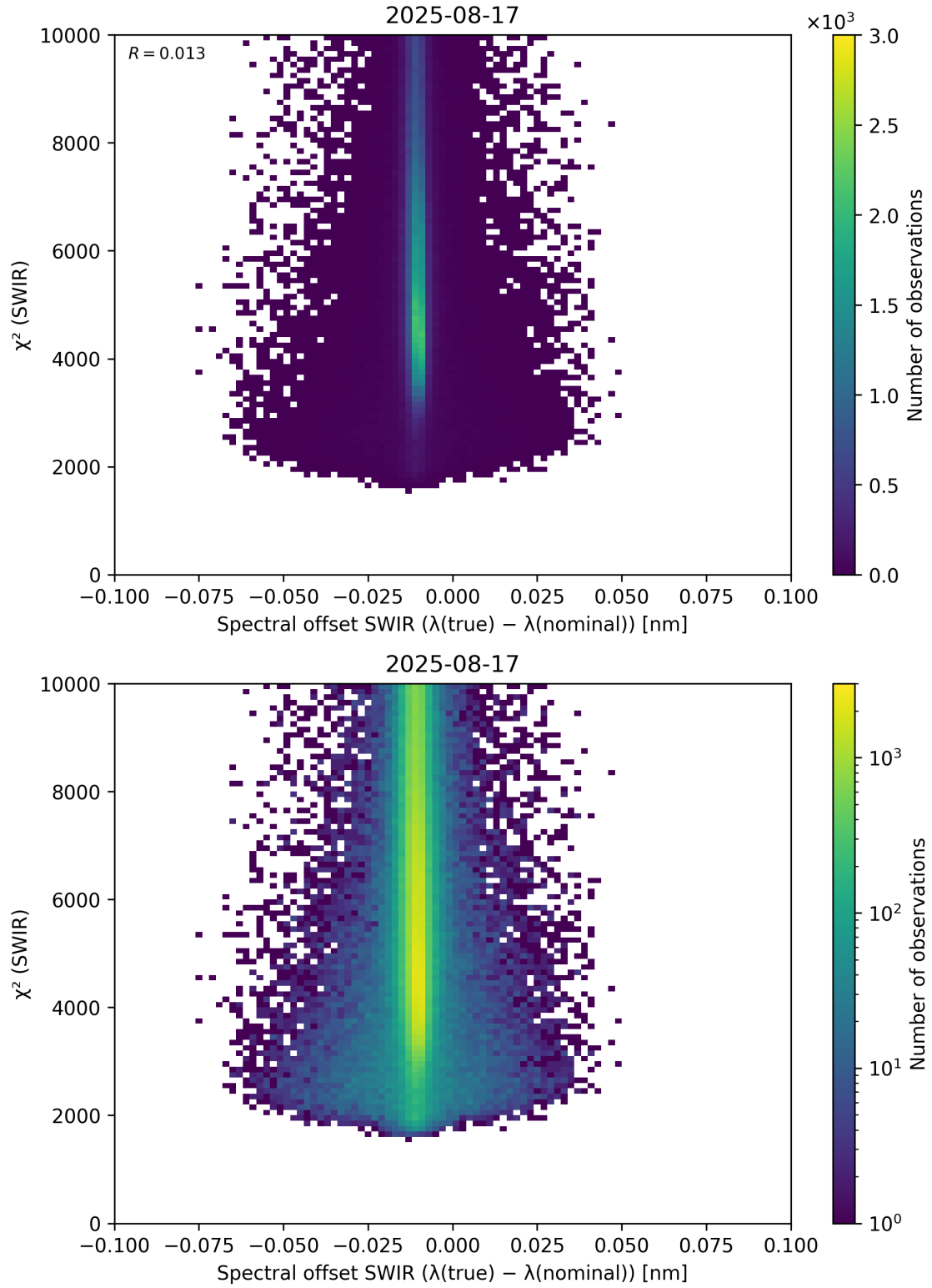
Figure 118: Scatter density plot of “Spectral offset SWIR ( \lambda_{\text{true}} - \lambda_{\text{nominal}} )” against “ \chi^2 (SWIR)” for 2025-08-16 to 2025-08-18.
