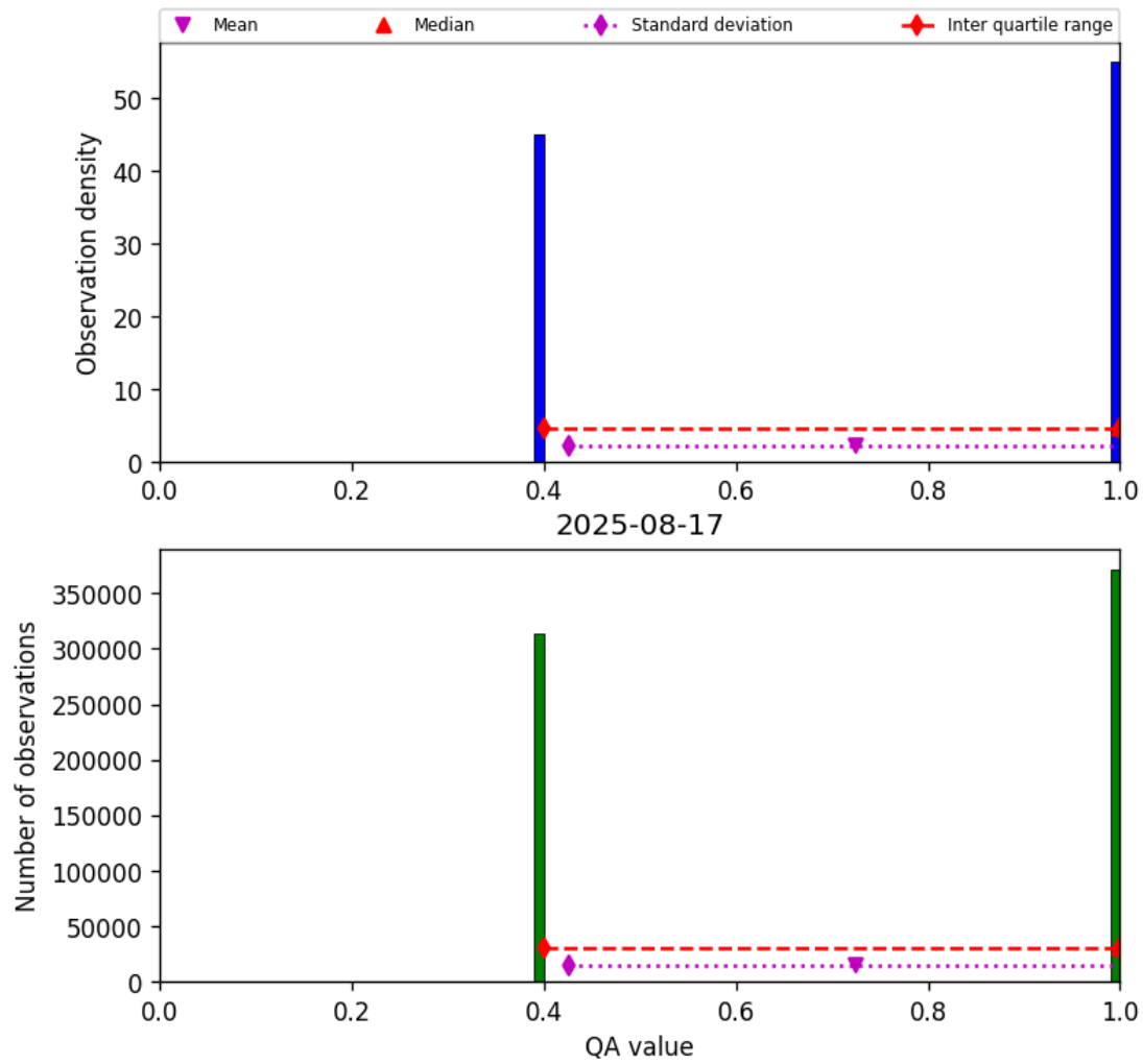
Figure 22: Histogram of “QA value” for 2025-08-16 to 2025-08-18
