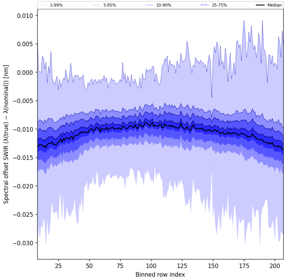
Figure 38: Along track statistics of “Spectral offset SWIR ( \lambda_{\text{true}} - \lambda_{\text{nominal}} )” for 2025-08-16 to 2025-08-18
