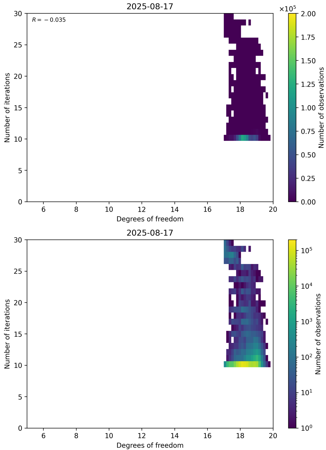
Figure 52: Scatter density plot of “Degrees of freedom” against “Number of iterations” for 2025-08-16 to 2025-08-18.
