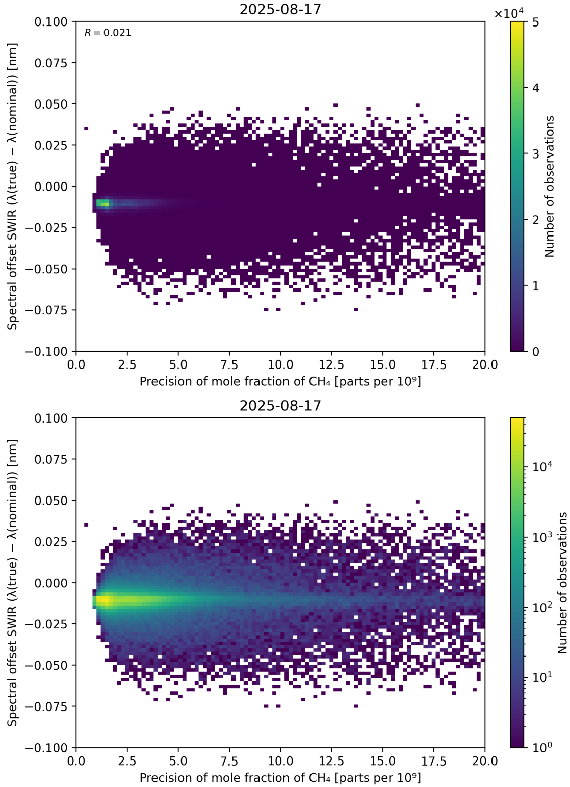
Figure 85: Scatter density plot of “Precision of mole fraction of CH 4 ” against “Spectral offset SWIR ( \lambda_{\text{true}} - \lambda_{\text{nominal}} )” for 2025-08-16 to 2025-08-18.
