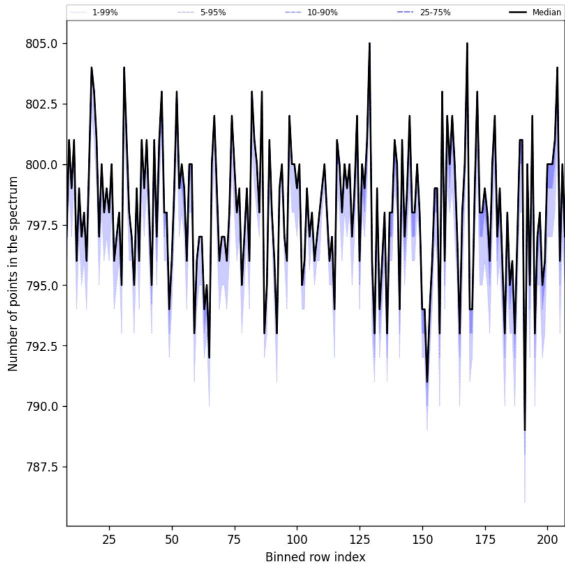
Figure 37: Along track statistics of “Number of points in the spectrum” for 2025-08-16 to 2025-08-18
