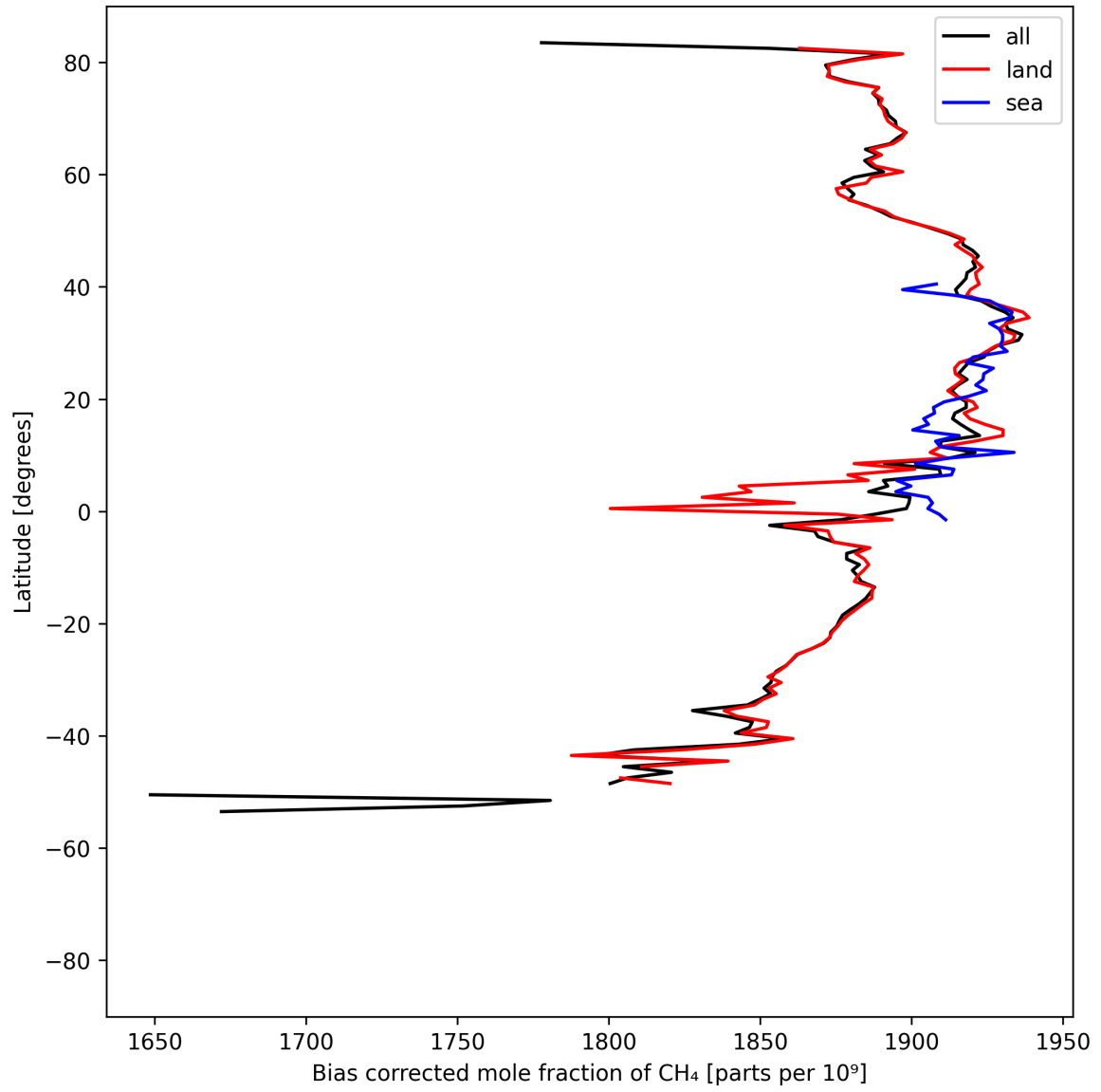
Figure 14: Zonal average of “Bias corrected mole fraction of CH 4 ” for 2025-08-16 to 2025-08-18.
