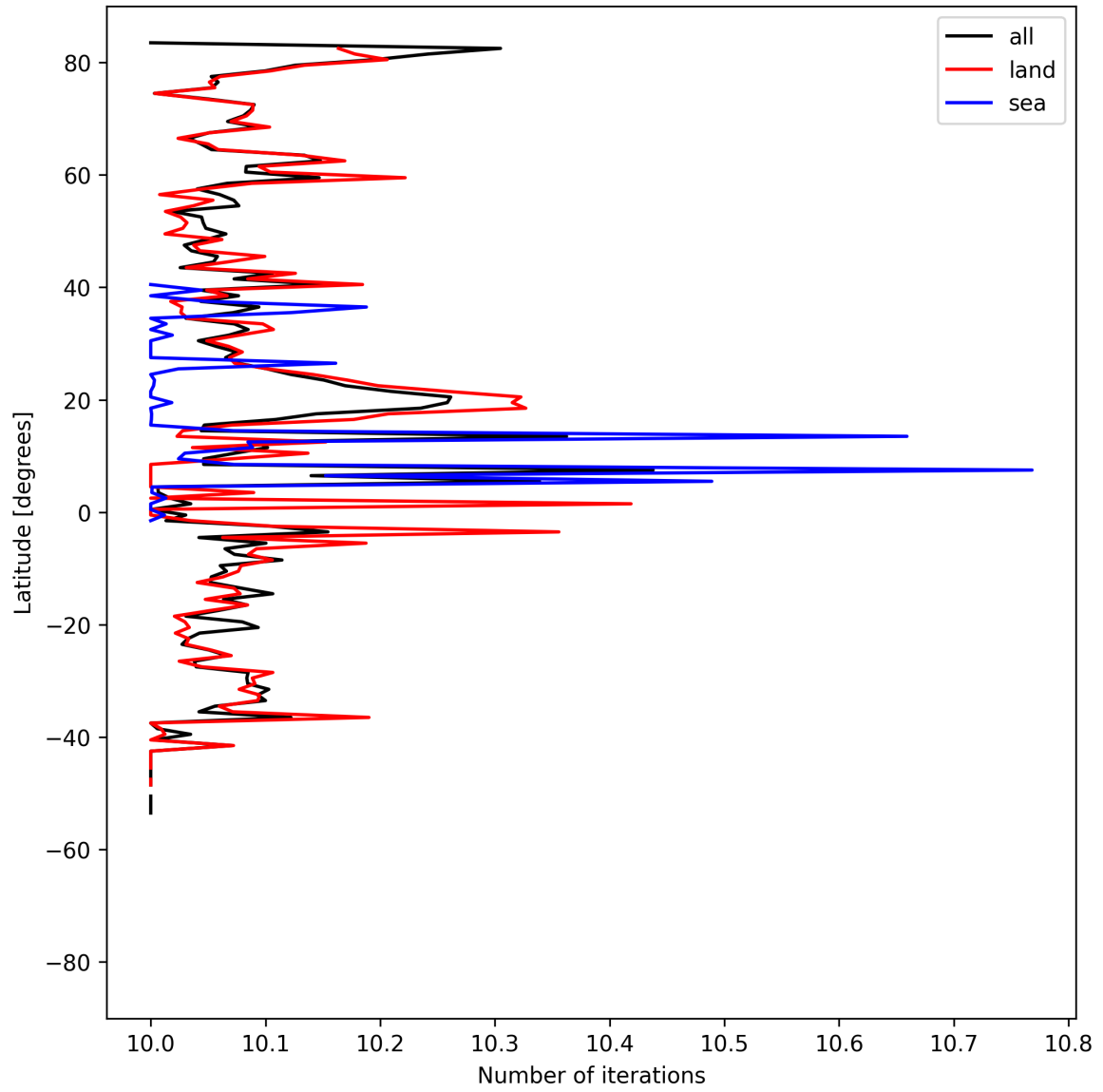
Figure 20: Zonal average of “Number of iterations” for 2025-08-16 to 2025-08-18.
