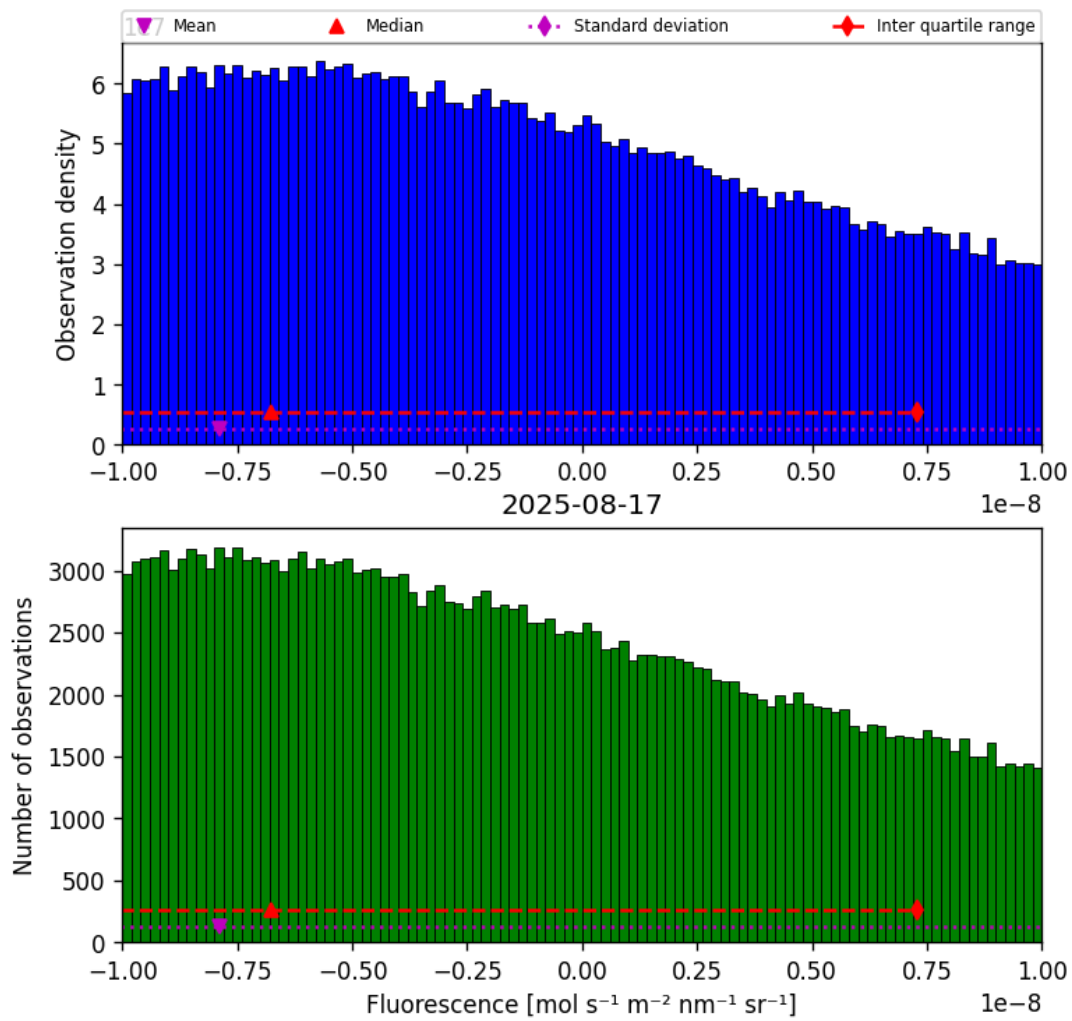
Figure 32: Histogram of “Fluorescence” for 2025-08-16 to 2025-08-18
