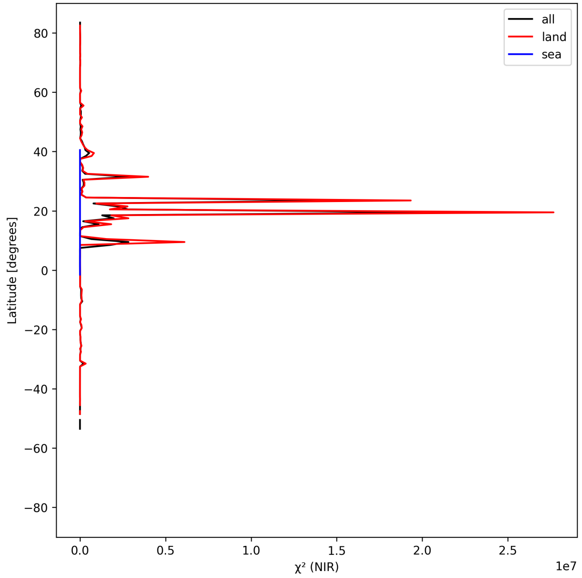
Figure 18: Zonal average of “ \chi^2 (NIR)” for 2025-08-16 to 2025-08-18.
