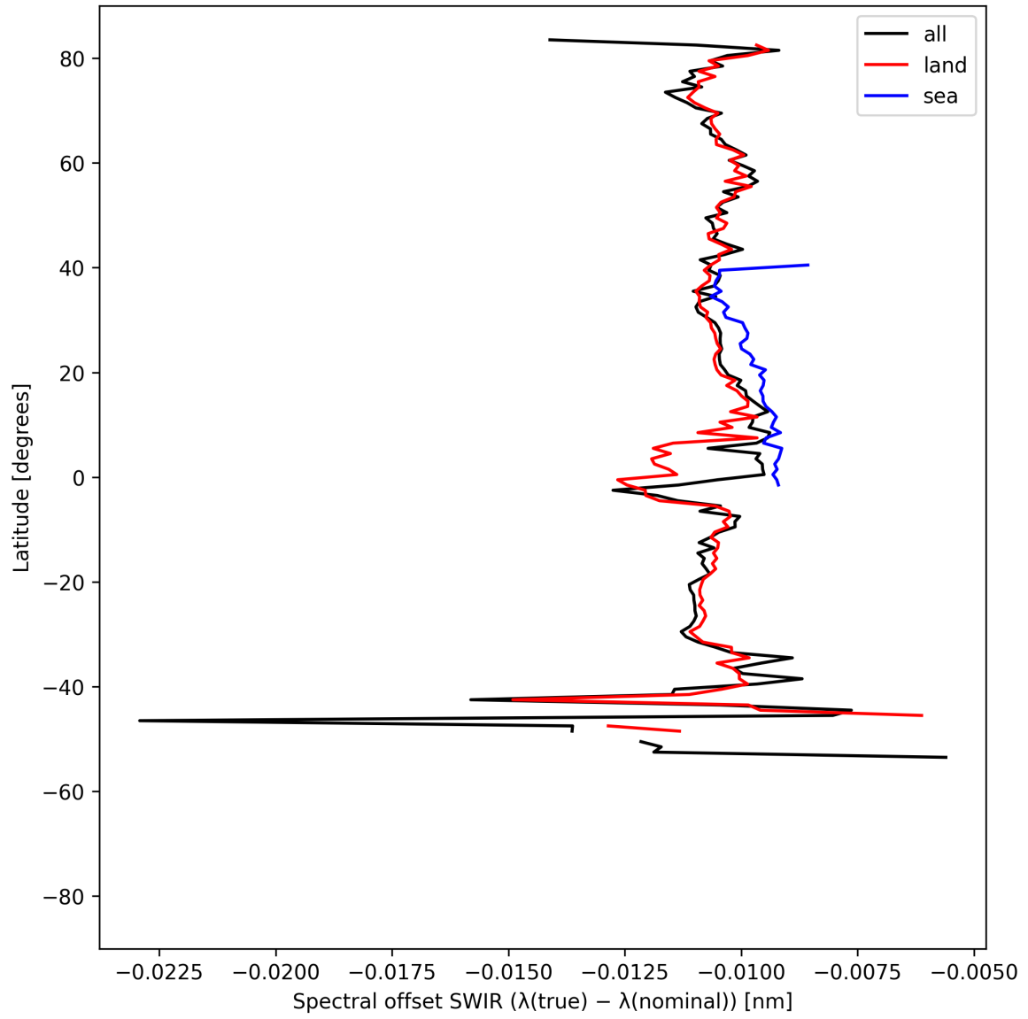
Figure 16: Zonal average of “Spectral offset SWIR ( \lambda_{\text{true}} - \lambda_{\text{nominal}} )” for 2025-08-16 to 2025-08-18.
