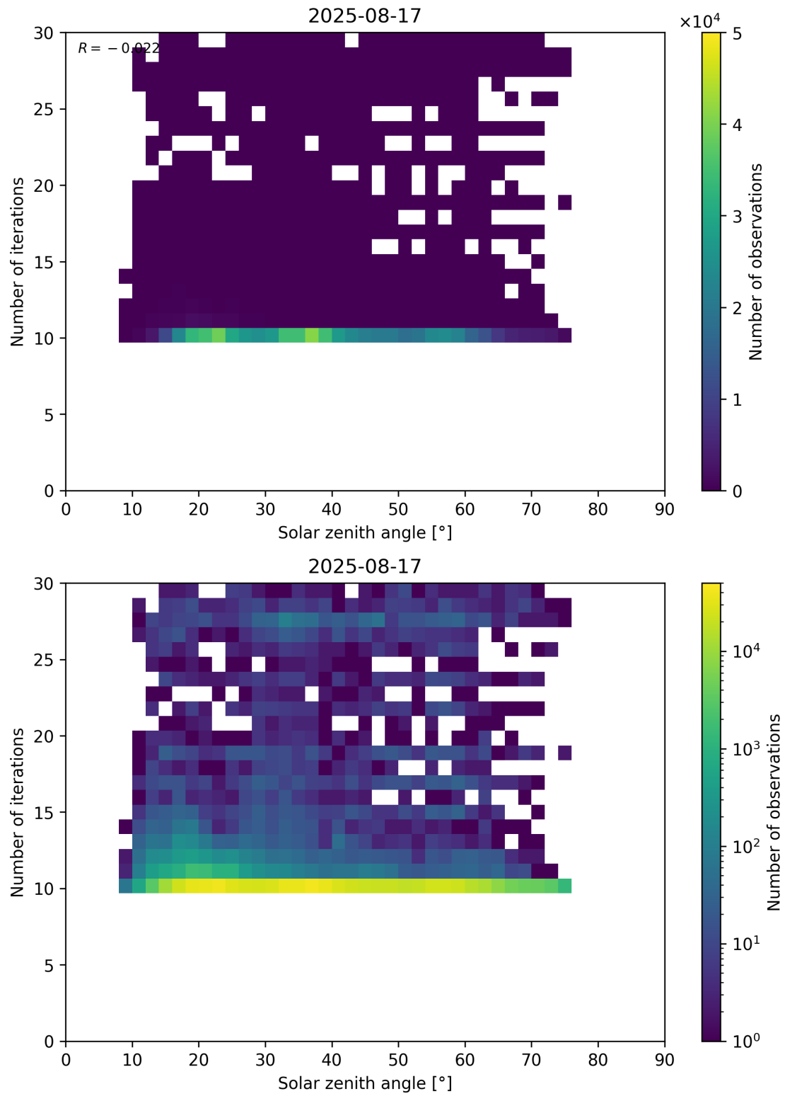
Figure 102: Scatter density plot of “Solar zenith angle” against “Number of iterations” for 2025-08-16 to 2025-08-18.
