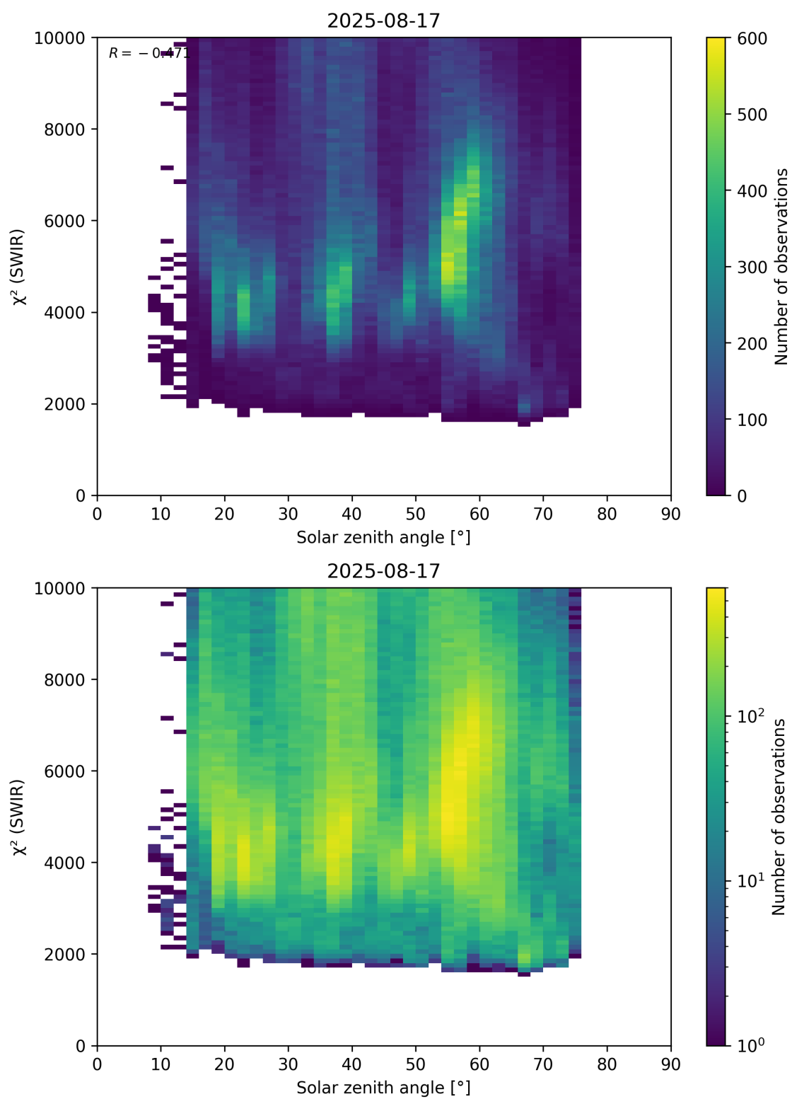
Figure 95: Scatter density plot of “Solar zenith angle” against “ \chi^2 (SWIR)” for 2025-08-16 to 2025-08-18.
