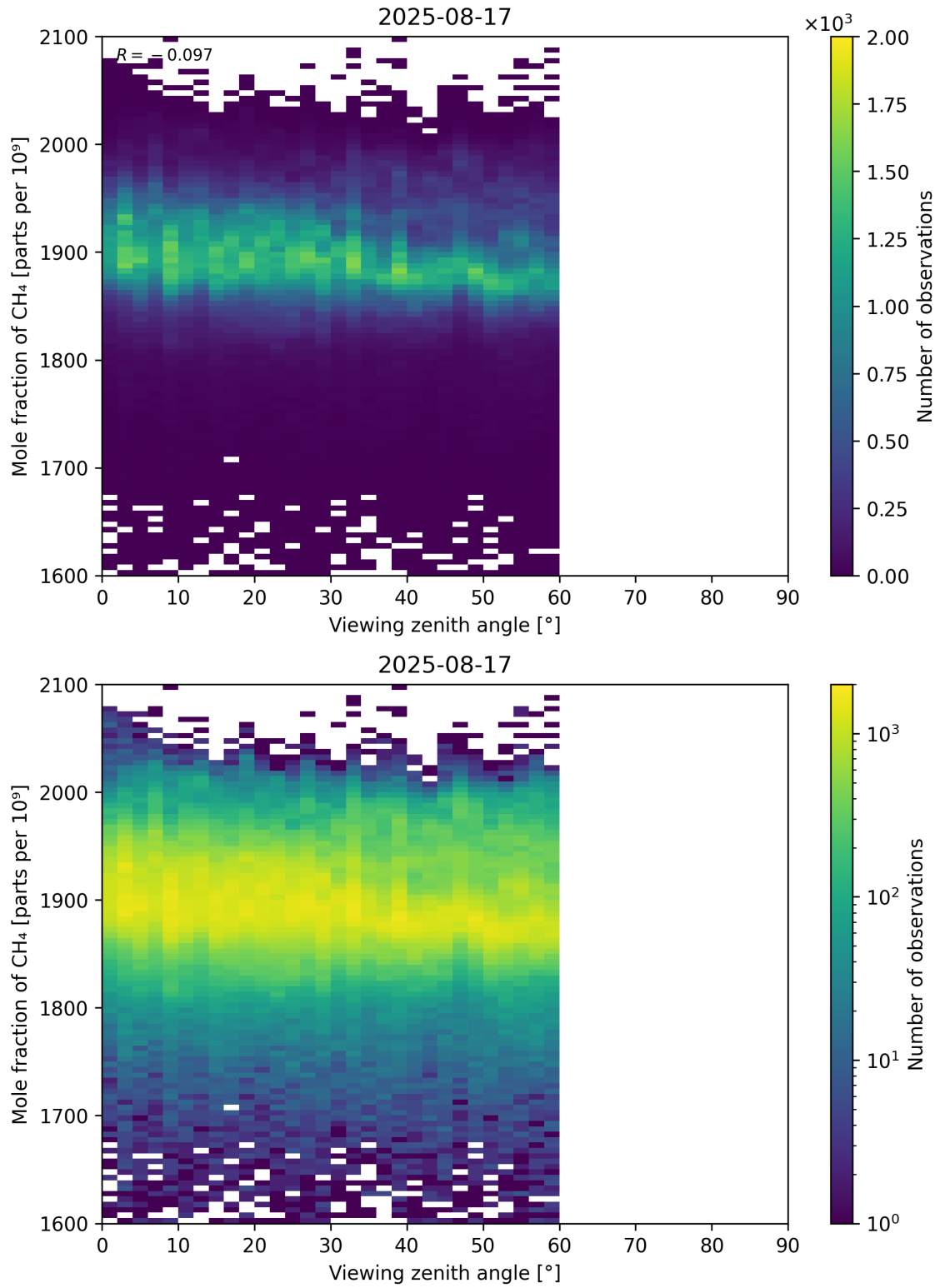
Figure 110: Scatter density plot of “Viewing zenith angle” against “Mole fraction of CH 4 ” for 2025-08-16 to 2025-08-18.
