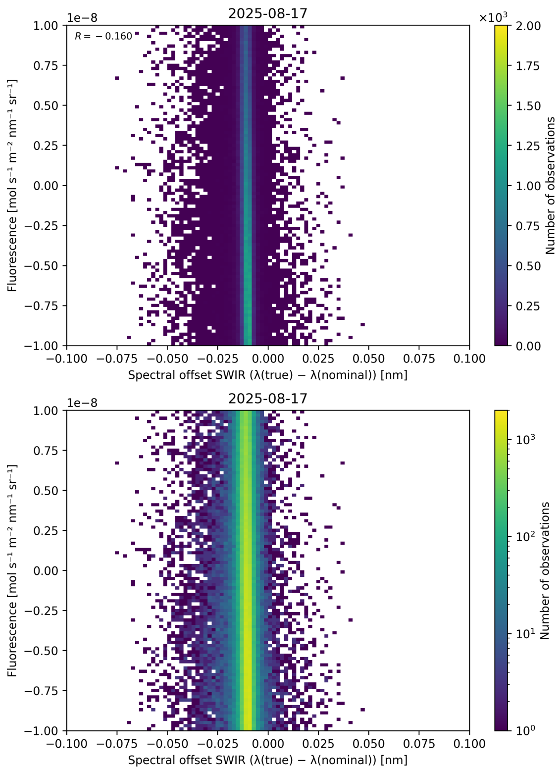
Figure 120: Scatter density plot of “Spectral offset SWIR ( \lambda_{\text{true}} - \lambda_{\text{nominal}} )” against “Fluorescence” for 2025-08-16 to 2025-08-18.
