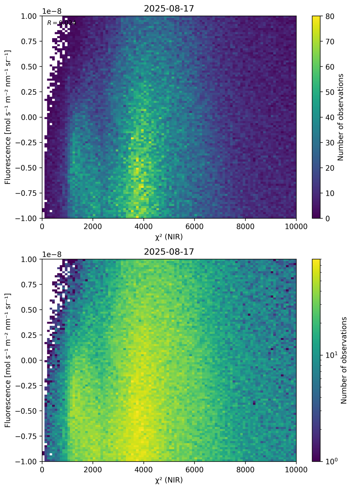
Figure 45: Scatter density plot of “ \chi^2 (NIR)” against “Fluorescence” for 2025-08-16 to 2025-08-18.
