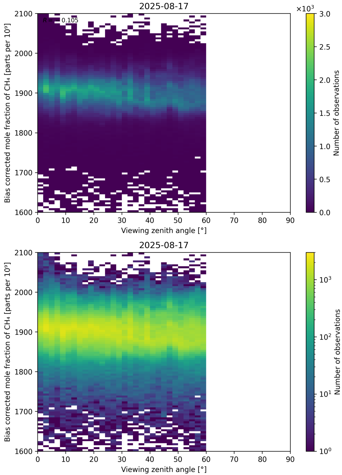
Figure 111: Scatter density plot of “Viewing zenith angle” against “Bias corrected mole fraction of CH 4 ” for 2025-08-16 to 2025-08-18.
