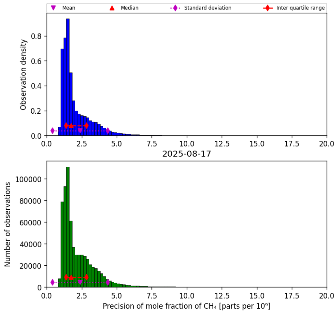
Figure 24: Histogram of “Precision of mole fraction of CH 4 ” for 2025-08-16 to 2025-08-18
