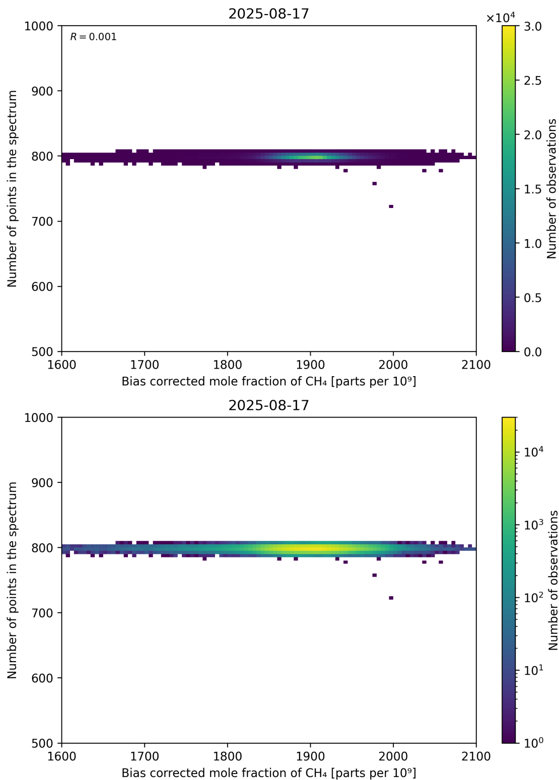
Figure 68: Scatter density plot of “Bias corrected mole fraction of CH 4 ” against “Number of points in the spectrum” for 2025-08-16 to 2025-08-18.
