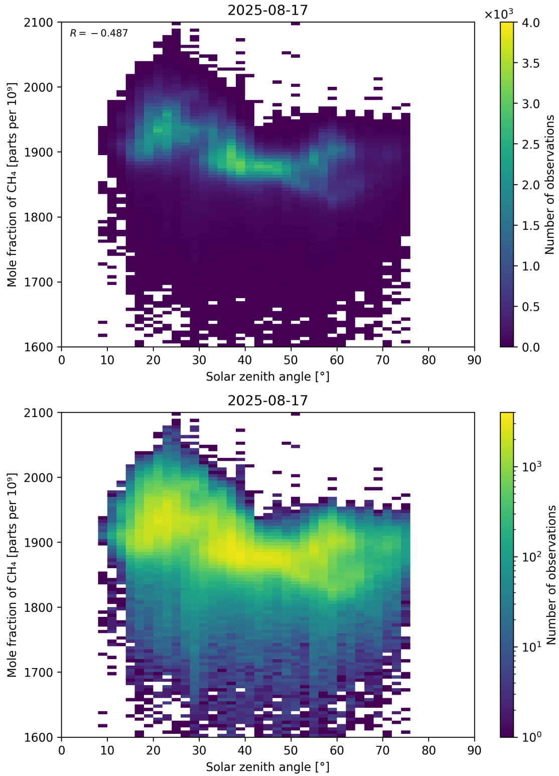
Figure 99: Scatter density plot of “Solar zenith angle” against “Mole fraction of CH 4 ” for 2025-08-16 to 2025-08-18.
