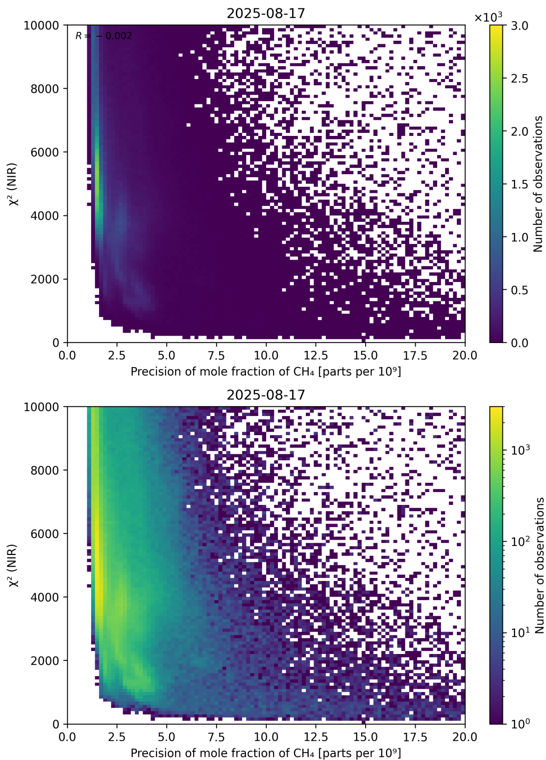
Figure 78: Scatter density plot of “Precision of mole fraction of CH 4 ” against “ \chi^2 (NIR)” for 2025-08-16 to 2025-08-18.
