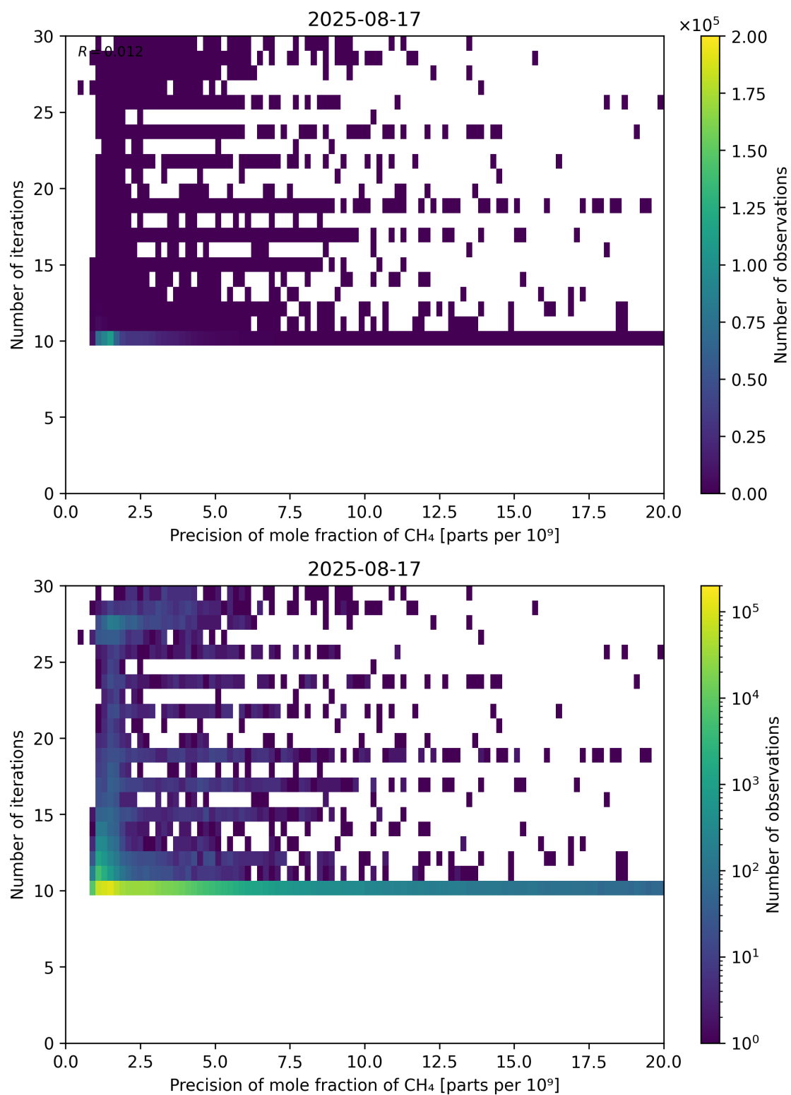
Figure 83: Scatter density plot of “Precision of mole fraction of CH 4 ” against “Number of iterations” for 2025-08-16 to 2025-08-18.
