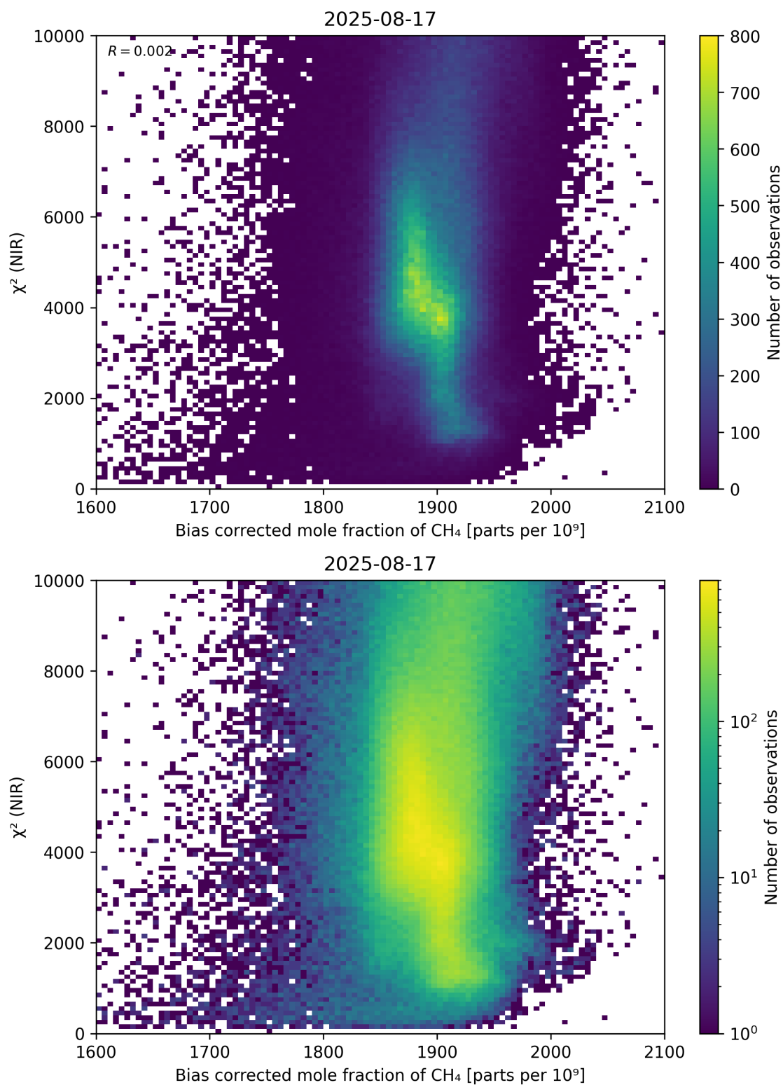
Figure 63: Scatter density plot of “Bias corrected mole fraction of \text{CH}_4 ” against “ \chi^2 (NIR)” for 2025-08-16 to 2025-08-18.
