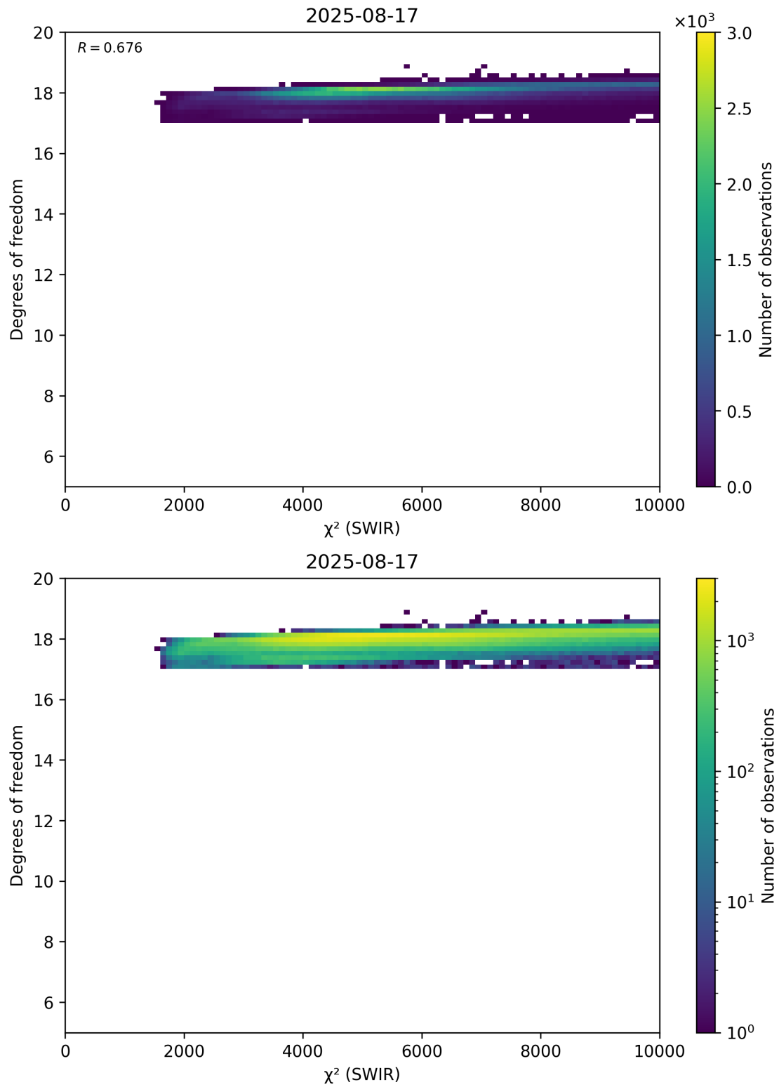
Figure 48: Scatter density plot of “ \chi^2 (SWIR)” against “Degrees of freedom” for 2025-08-16 to 2025-08-18.
