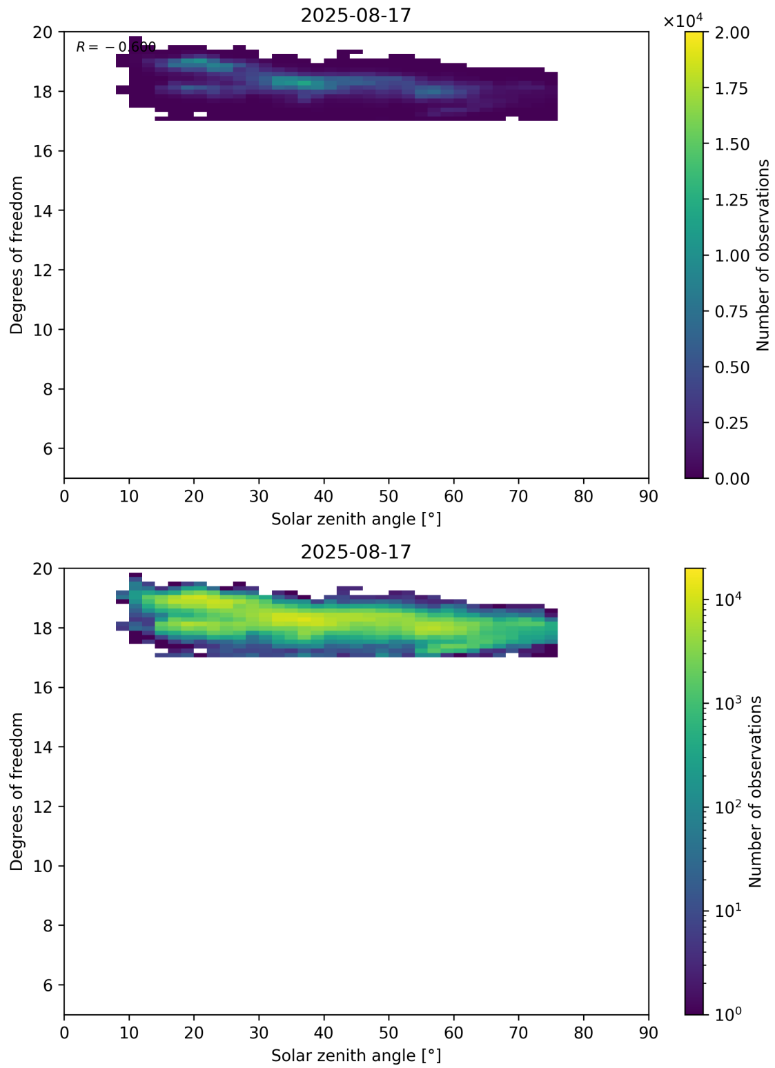
Figure 96: Scatter density plot of “Solar zenith angle” against “Degrees of freedom” for 2025-08-16 to 2025-08-18.
