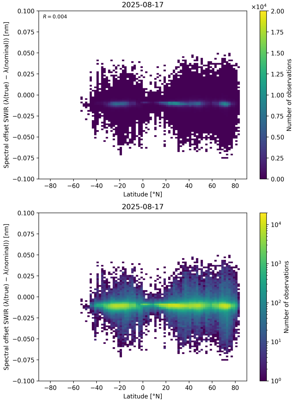
Figure 62: Scatter density plot of “Latitude” against “Spectral offset SWIR ( \lambda_{\text{true}} - \lambda_{\text{nominal}} )” for 2025-08-16 to 2025-08-18.
