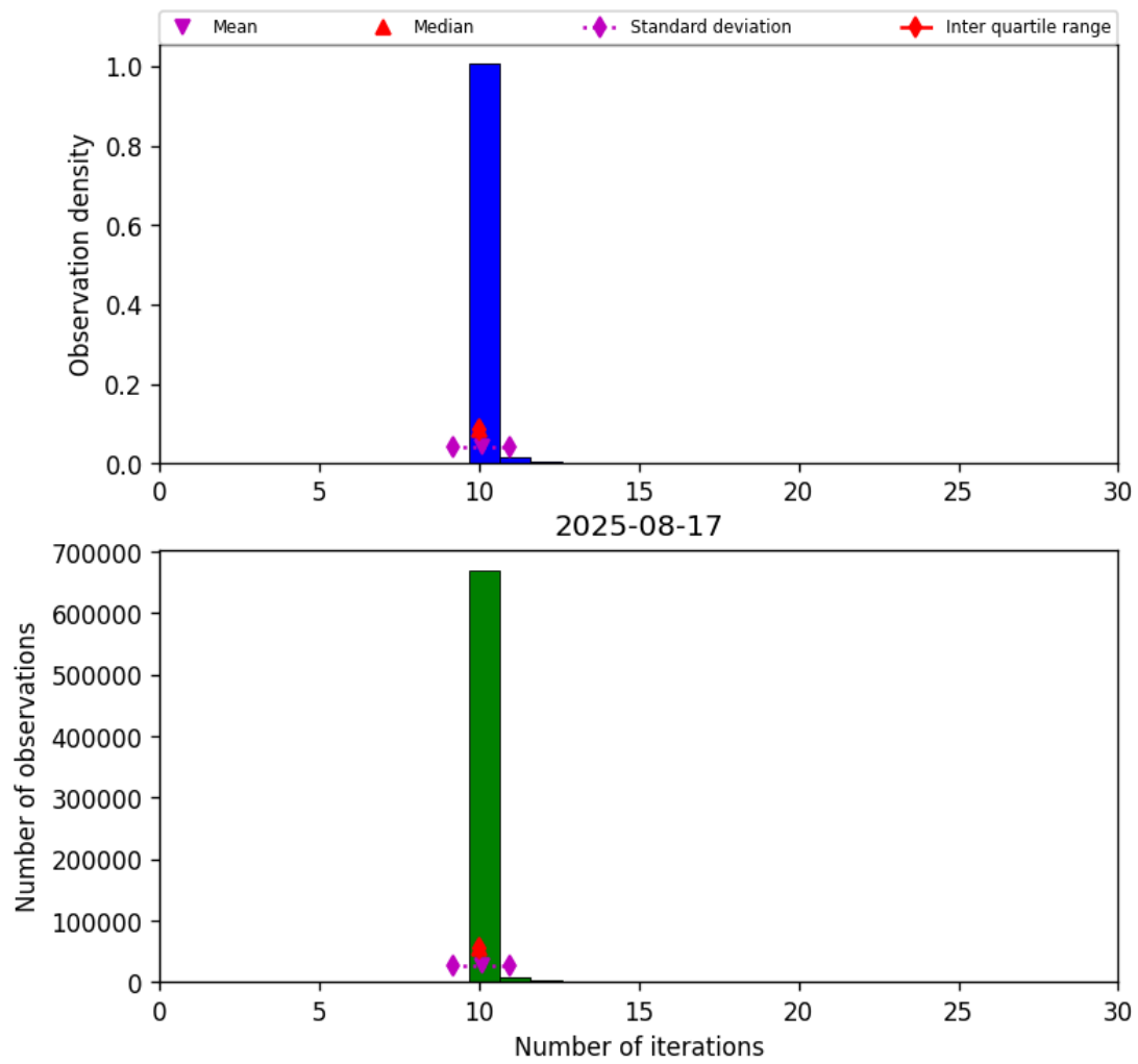
Figure 31: Histogram of “Number of iterations” for 2025-08-16 to 2025-08-18
