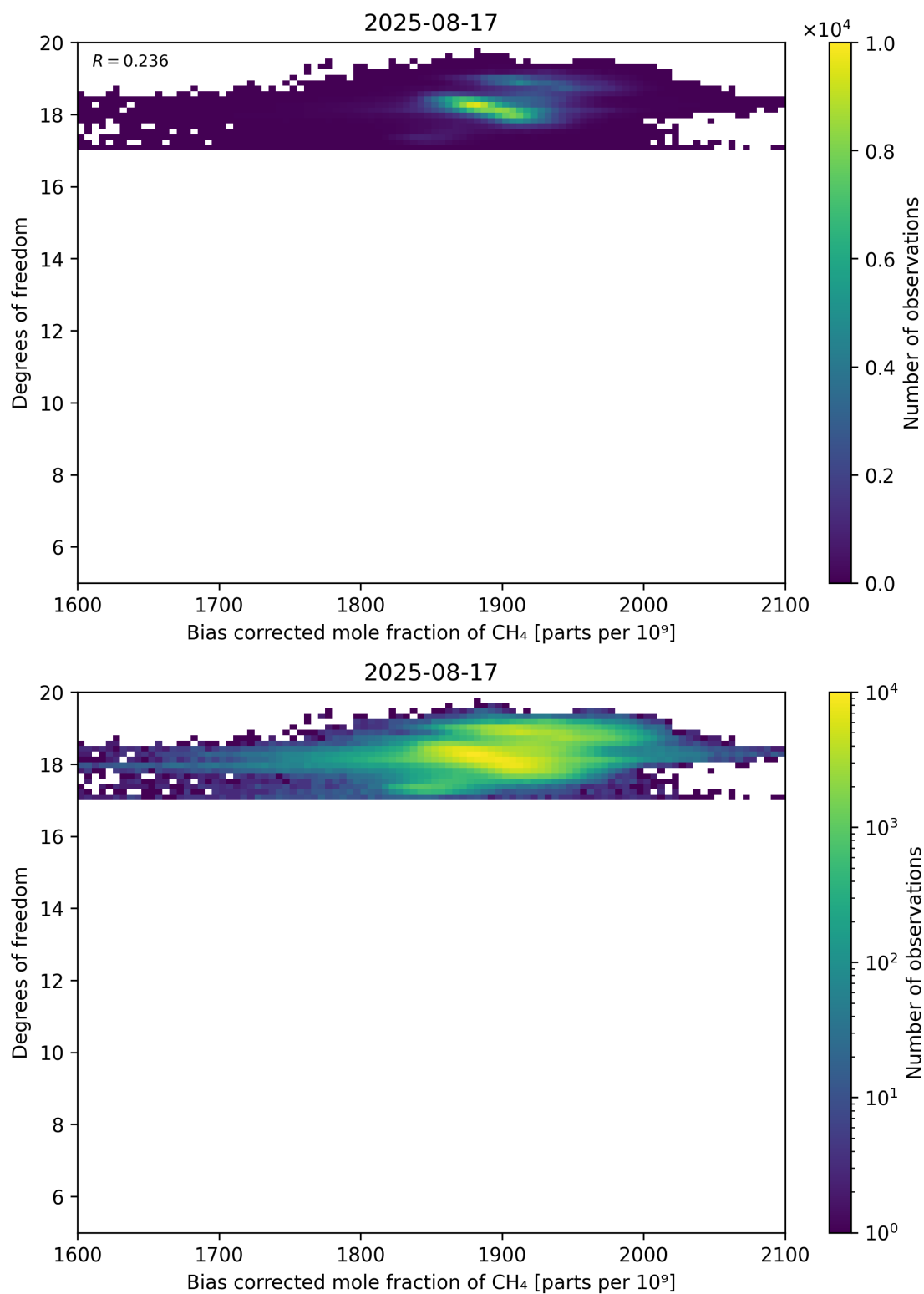
Figure 65: Scatter density plot of “Bias corrected mole fraction of CH 4 ” against “Degrees of freedom” for 2025-08-16 to 2025-08-18.
