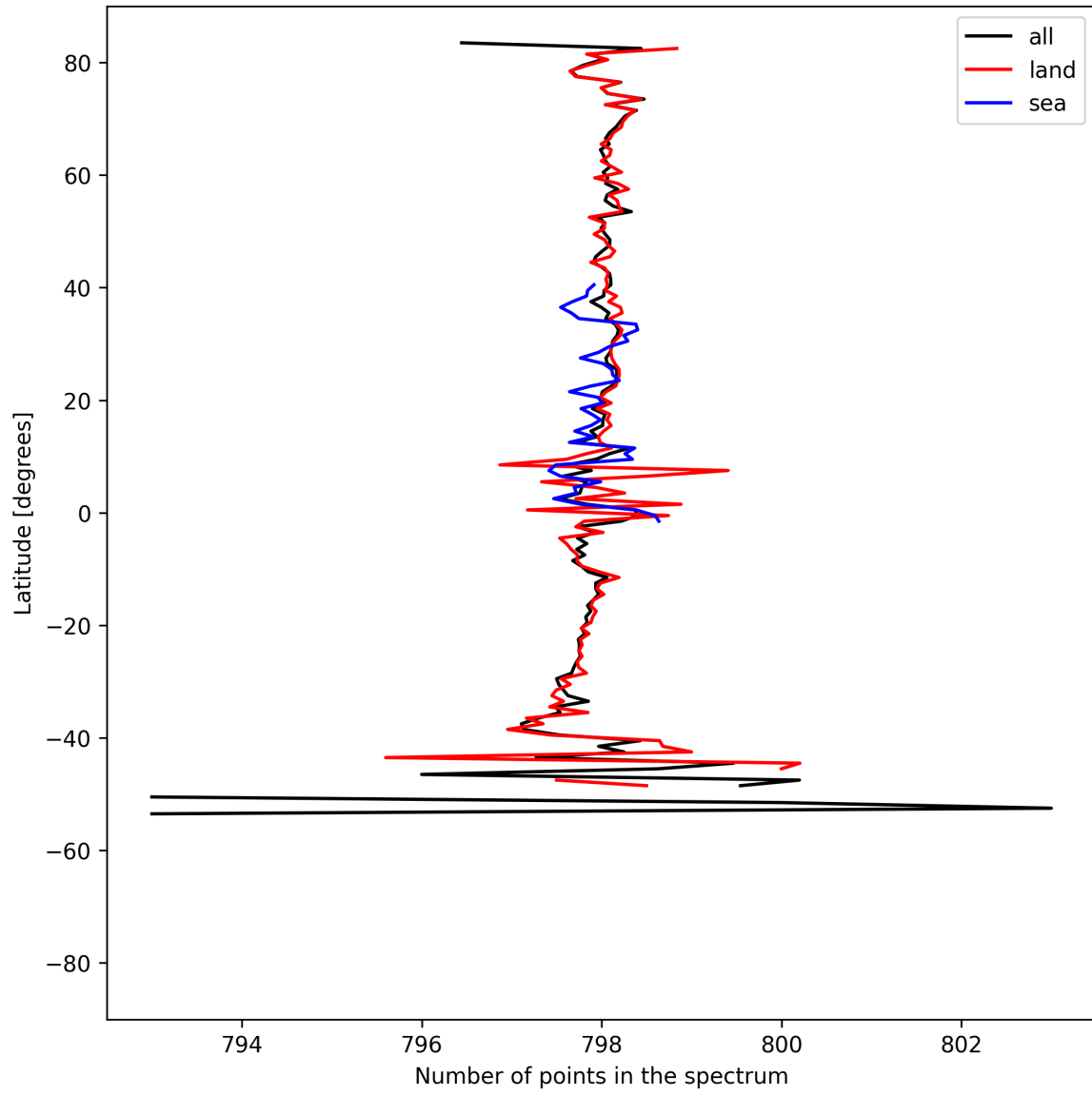
Figure 15: Zonal average of “Number of points in the spectrum” for 2025-08-16 to 2025-08-18.
