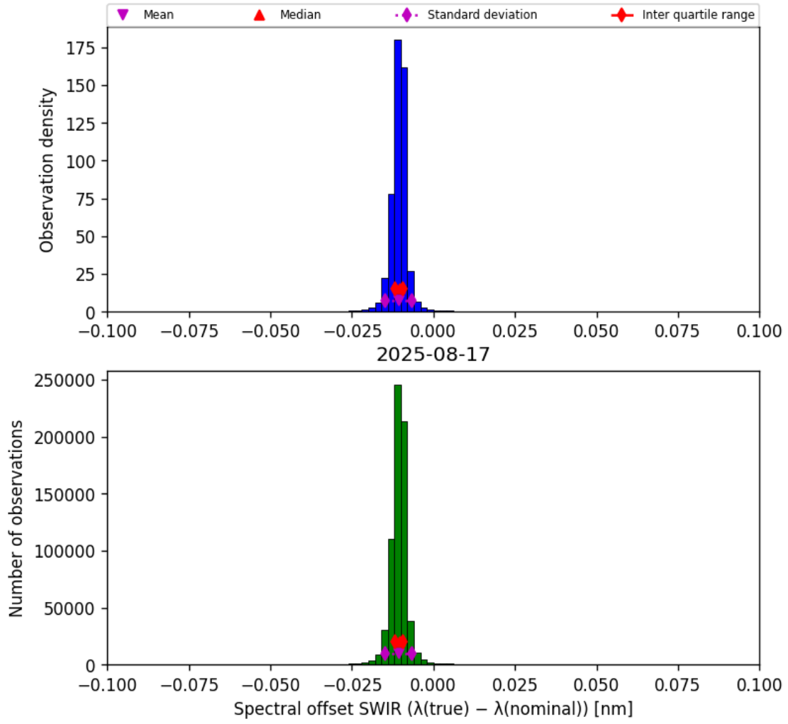
Figure 27: Histogram of “Spectral offset SWIR ( \lambda_{\text{true}} - \lambda_{\text{nominal}} )” for 2025-08-16 to 2025-08-18
