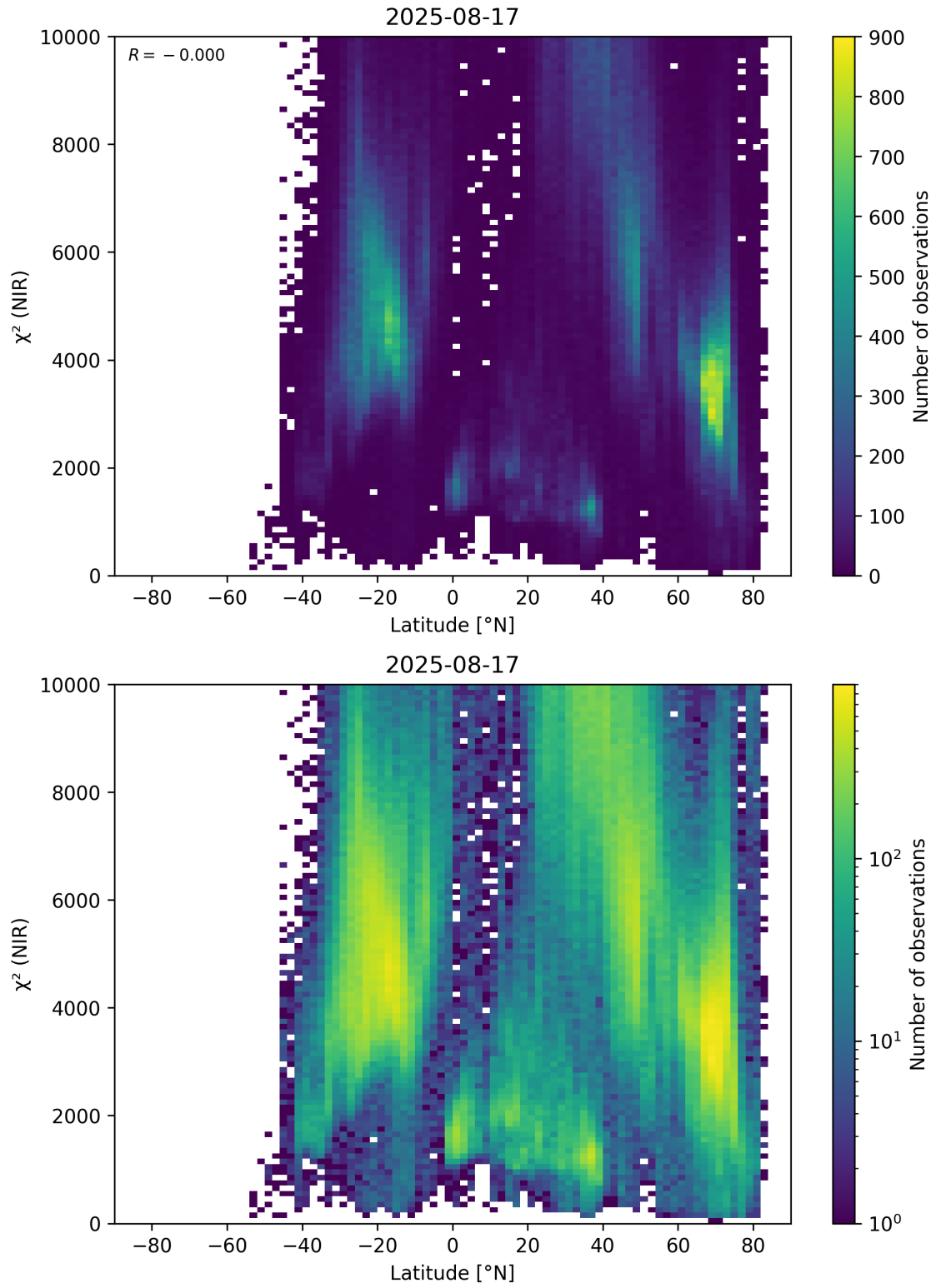
Figure 53: Scatter density plot of “Latitude” against “ \chi^2 (NIR)” for 2025-08-16 to 2025-08-18.
