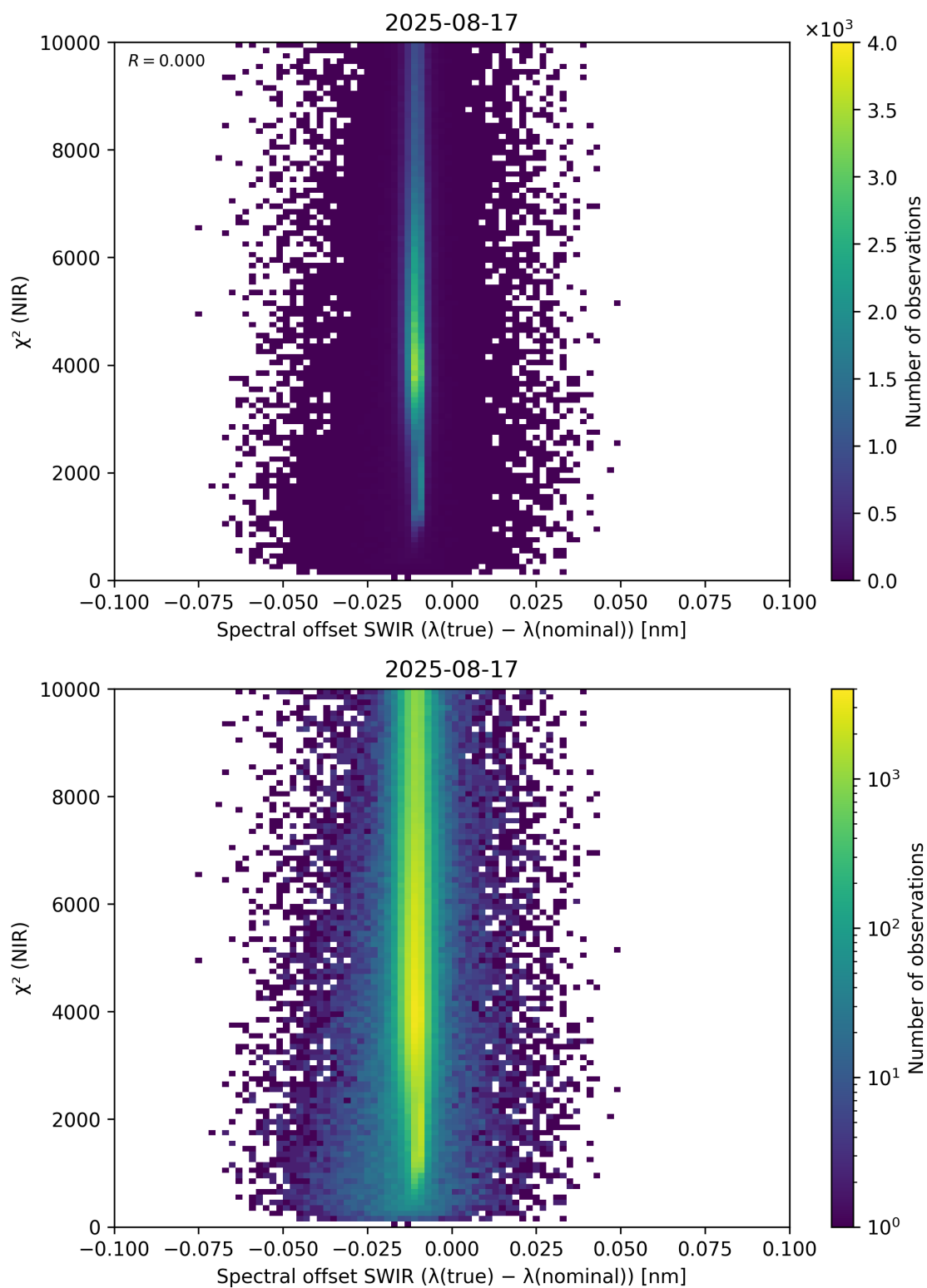
Figure 117: Scatter density plot of “Spectral offset SWIR ( \lambda_{\text{true}} - \lambda_{\text{nominal}} )” against “ \chi^2 (NIR)” for 2025-08-16 to 2025-08-18.
