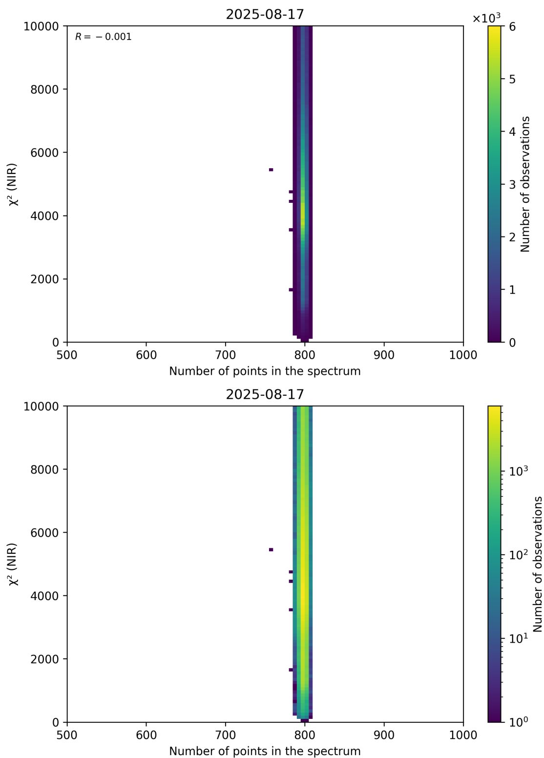
Figure 88: Scatter density plot of “Number of points in the spectrum” against “ \chi^2 (NIR)” for 2025-08-16 to 2025-08-18.
