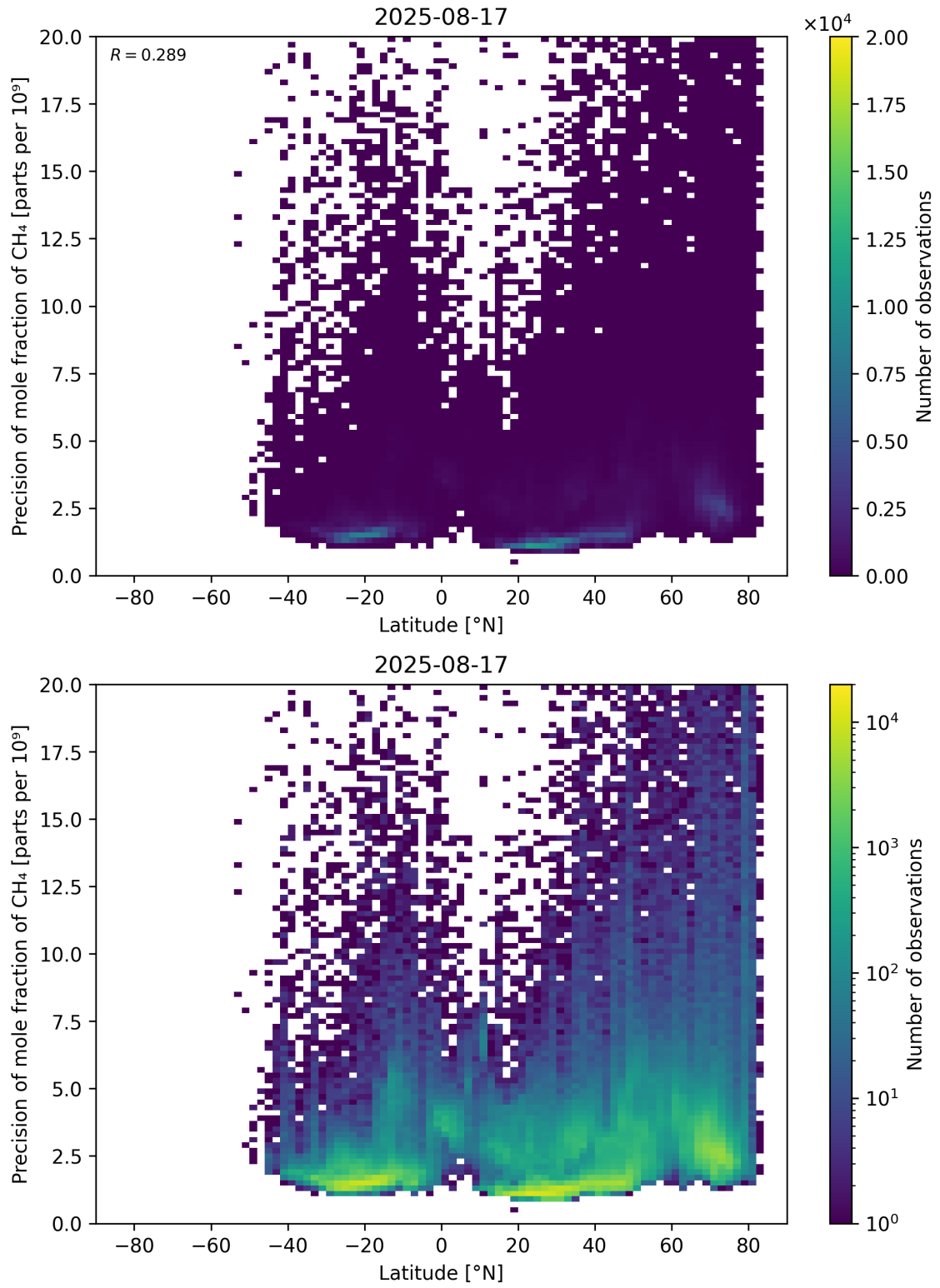
Figure 59: Scatter density plot of “Latitude” against “Precision of mole fraction of \text{CH}_4 ” for 2025-08-16 to 2025-08-18.
