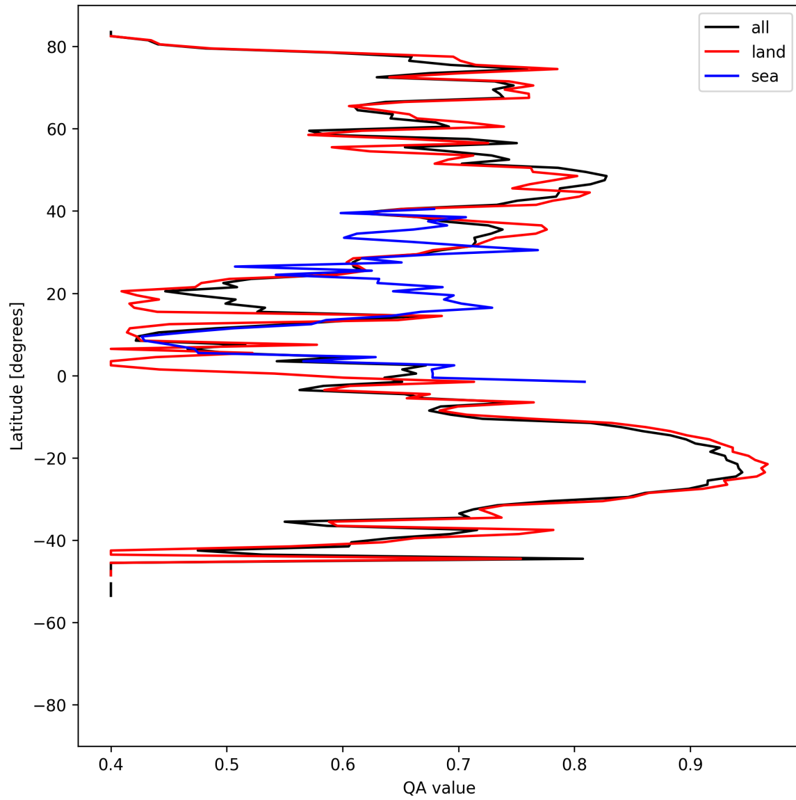
Figure 11: Zonal average of “QA value” for 2025-08-16 to 2025-08-18.
