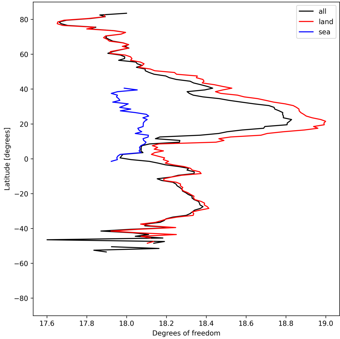
Figure 19: Zonal average of “Degrees of freedom” for 2025-08-16 to 2025-08-18.
