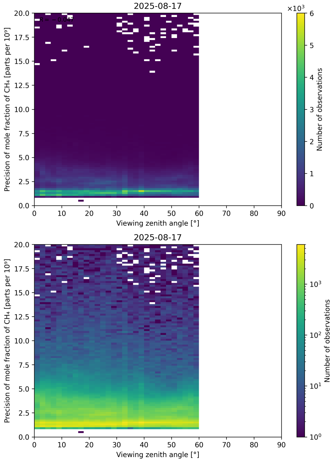
Figure 112: Scatter density plot of “Viewing zenith angle” against “Precision of mole fraction of CH 4 ” for 2025-08-16 to 2025-08-18.
