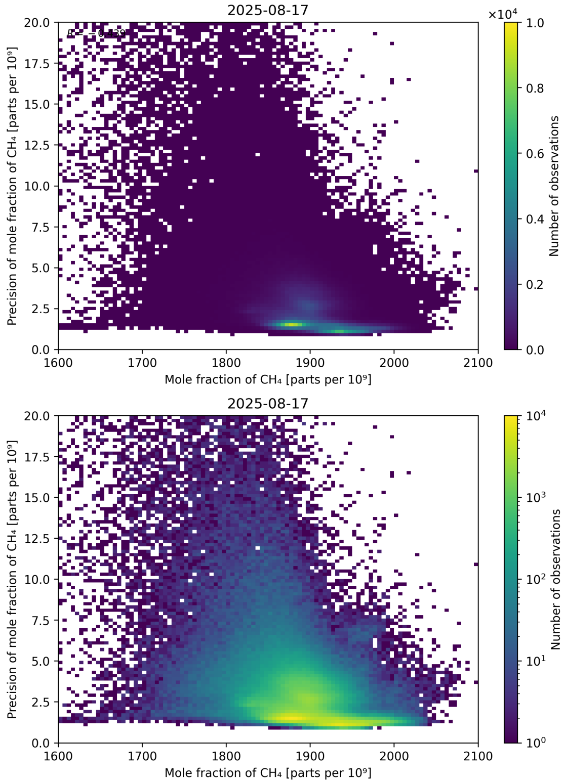
Figure 75: Scatter density plot of “Mole fraction of CH 4 ” against “Precision of mole fraction of CH 4 ” for 2025-08-16 to 2025-08-18.
