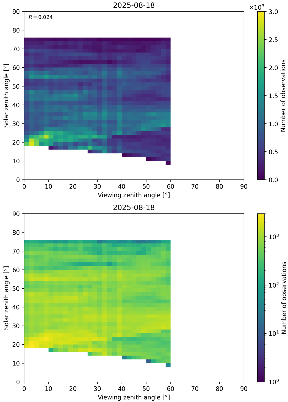
Figure 115: Scatter density plot of “Viewing zenith angle” against “Solar zenith angle” for 2025-08-17 to 2025-08-19.
