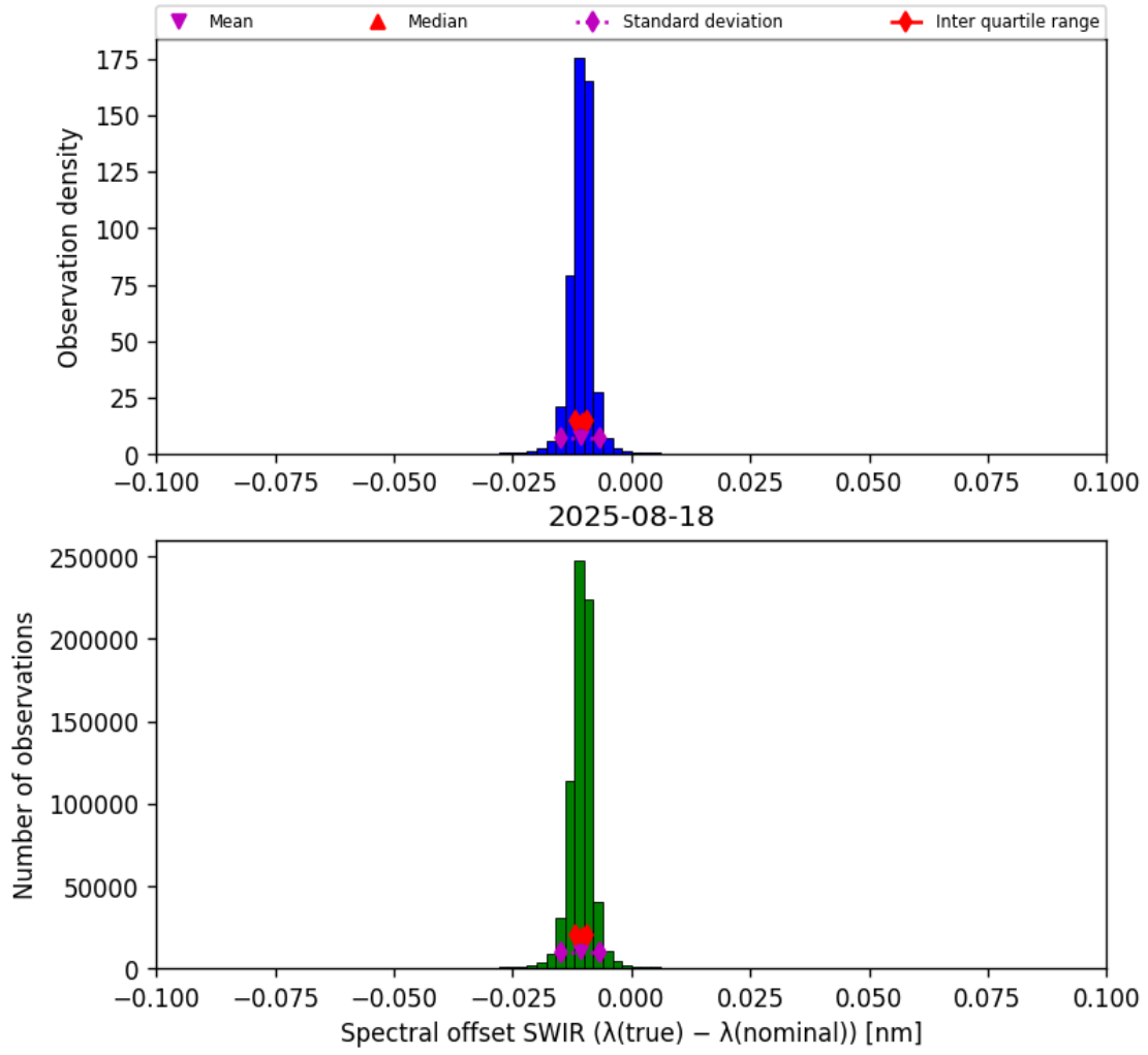
Figure 27: Histogram of “Spectral offset SWIR ( \lambda_{\text{true}} - \lambda_{\text{nominal}} )” for 2025-08-17 to 2025-08-19
