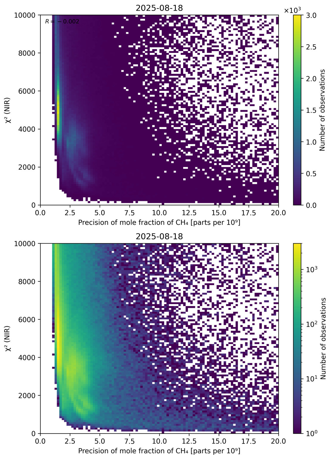
Figure 78: Scatter density plot of “Precision of mole fraction of CH 4 ” against “ \chi^2 (NIR)” for 2025-08-17 to 2025-08-19.
