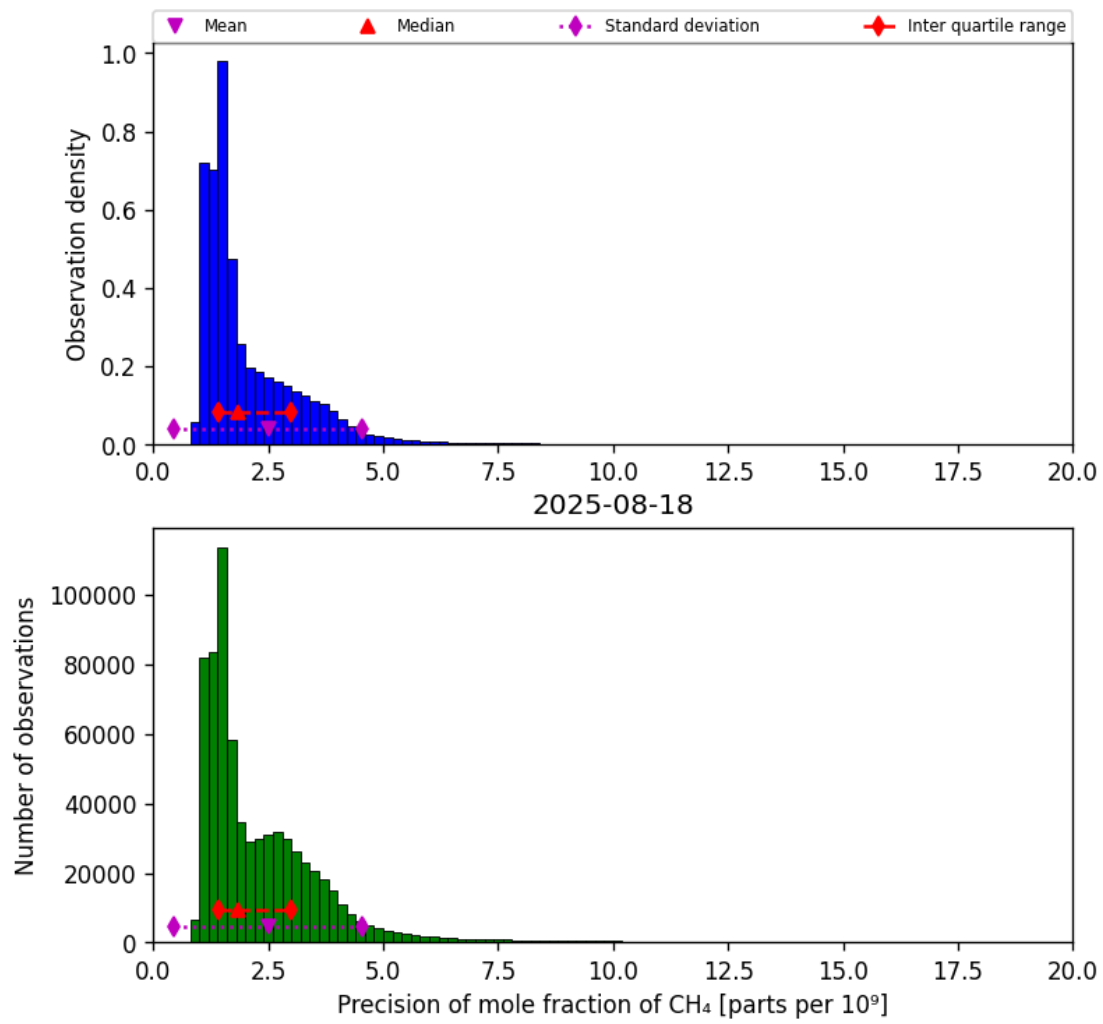
Figure 24: Histogram of “Precision of mole fraction of CH 4 ” for 2025-08-17 to 2025-08-19
