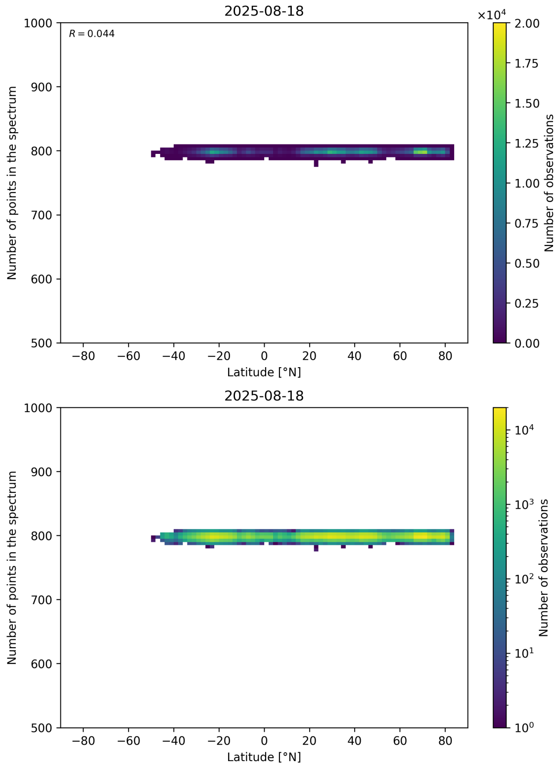
Figure 61: Scatter density plot of “Latitude” against “Number of points in the spectrum” for 2025-08-17 to 2025-08-19.
