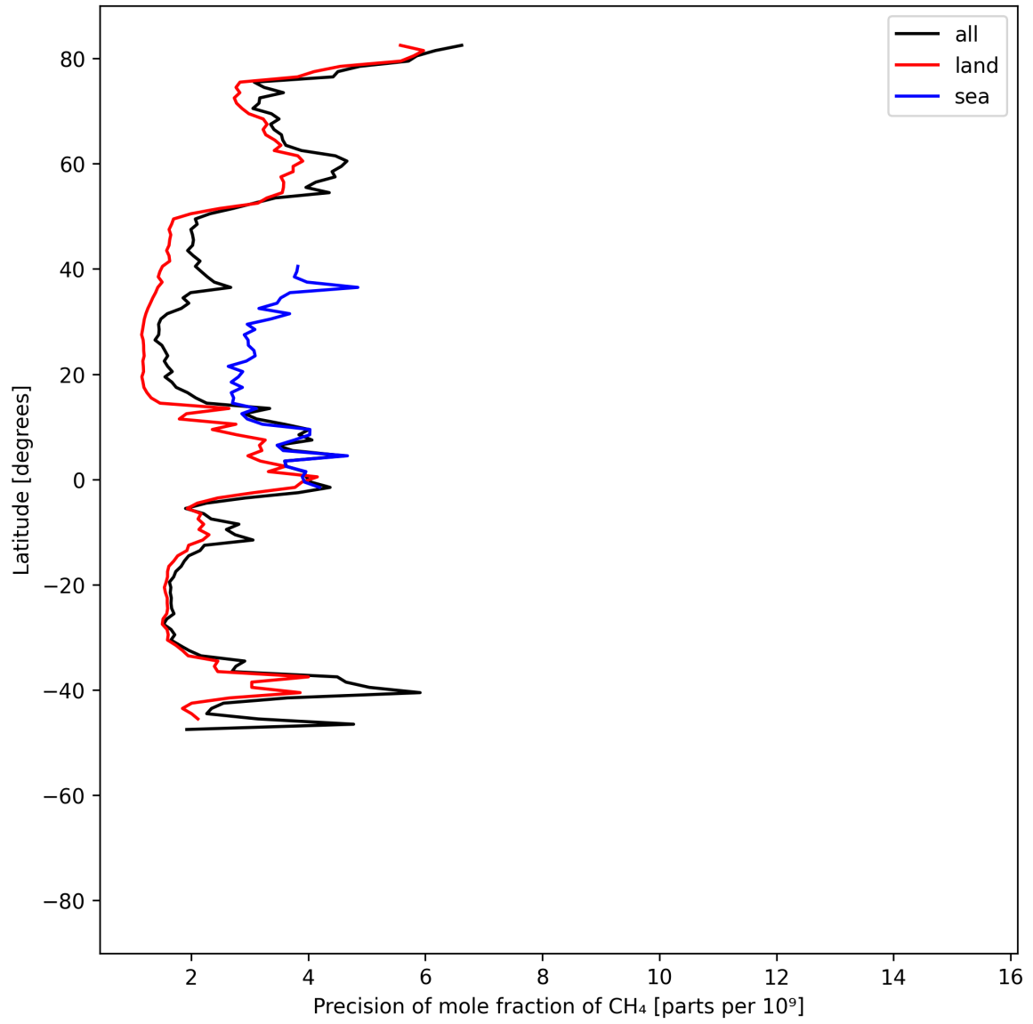
Figure 13: Zonal average of “Precision of mole fraction of CH 4 ” for 2025-08-17 to 2025-08-19.
