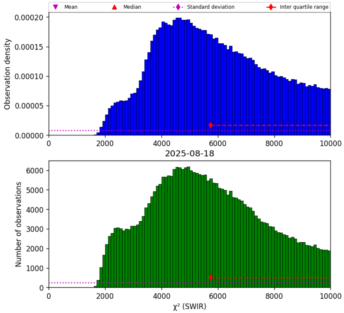
Figure 28: Histogram of “ \chi^2 (SWIR)” for 2025-08-17 to 2025-08-19
