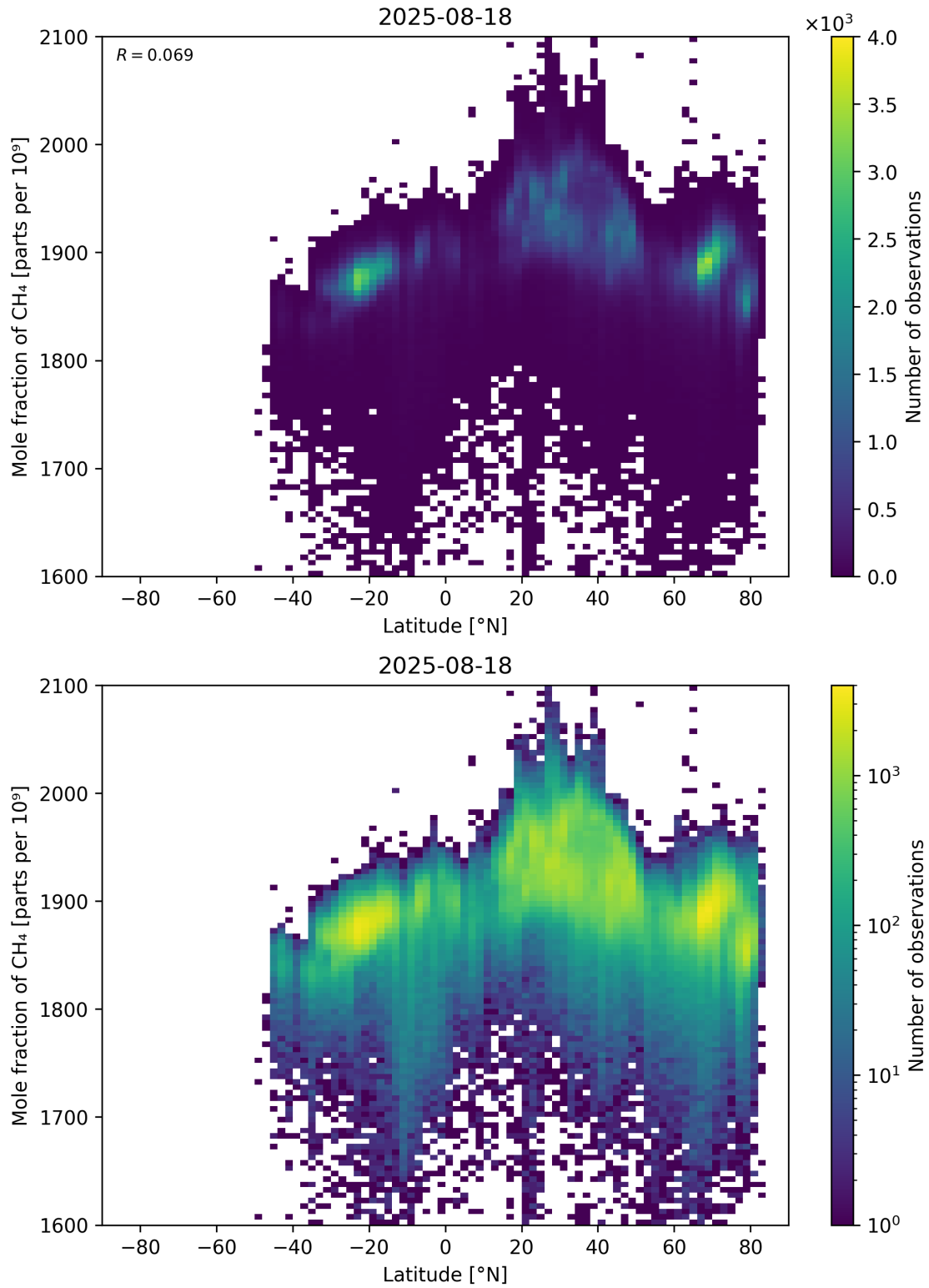
Figure 57: Scatter density plot of “Latitude” against “Mole fraction of CH 4 ” for 2025-08-17 to 2025-08-19.
