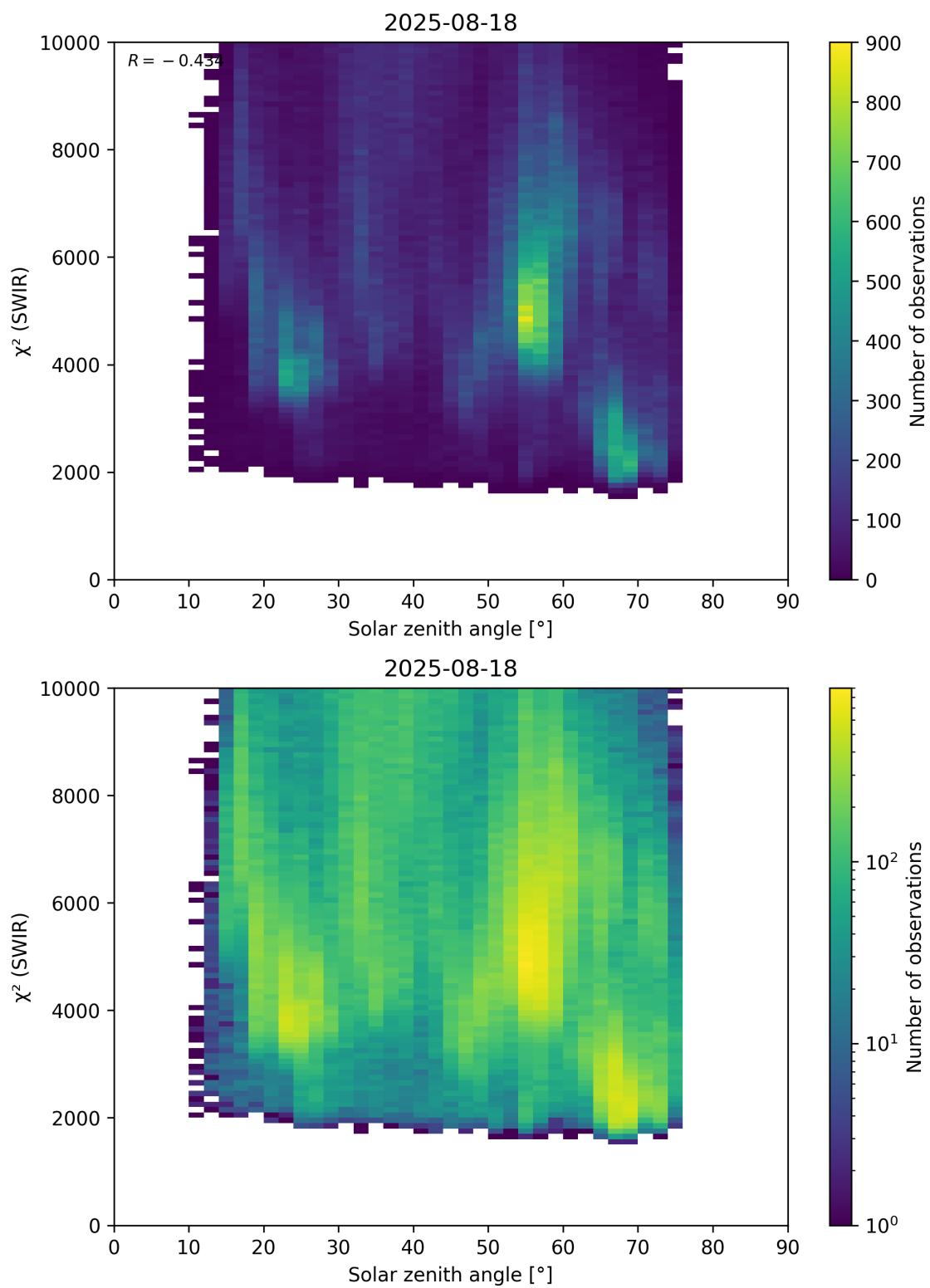
Figure 95: Scatter density plot of “Solar zenith angle” against “ \chi^2 (SWIR)” for 2025-08-17 to 2025-08-19.
