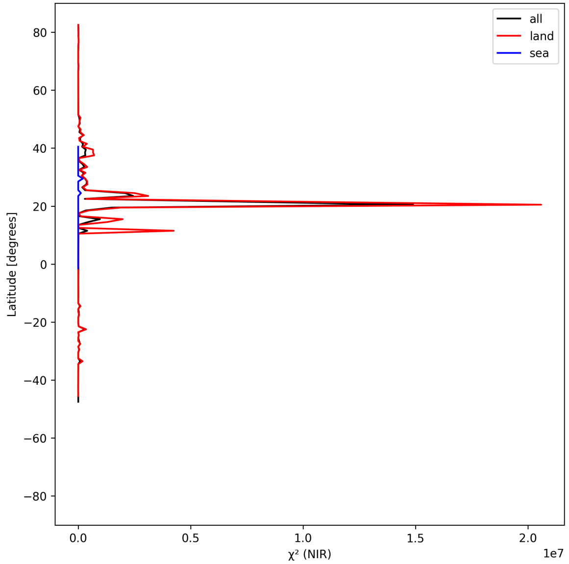
Figure 18: Zonal average of “ \chi^2 (NIR)” for 2025-08-17 to 2025-08-19.
