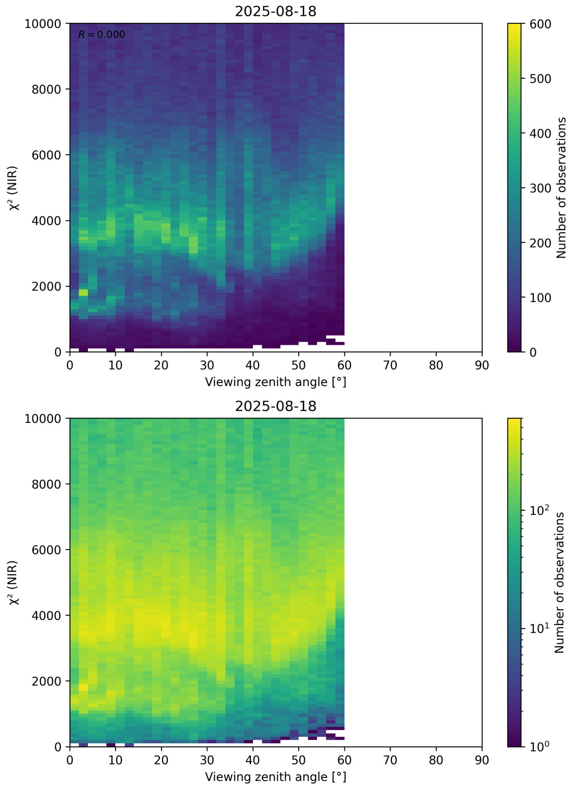
Figure 105: Scatter density plot of “Viewing zenith angle” against “ \chi^2 (NIR)” for 2025-08-17 to 2025-08-19.
