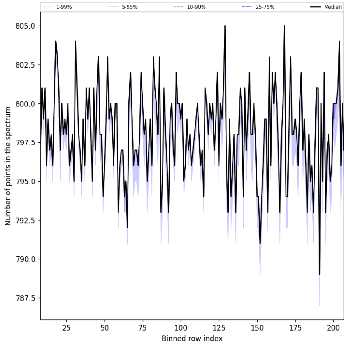
Figure 37: Along track statistics of “Number of points in the spectrum” for 2025-08-17 to 2025-08-19
