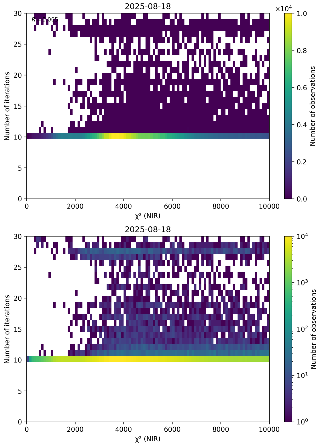
Figure 46: Scatter density plot of “ \chi^2 (NIR)” against “Number of iterations” for 2025-08-17 to 2025-08-19.
