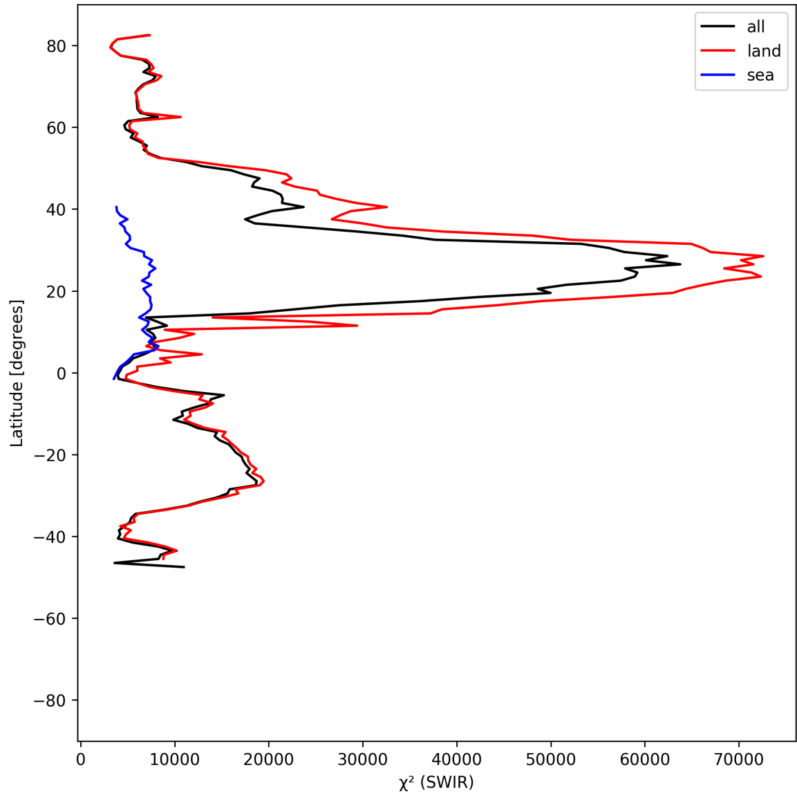
Figure 17: Zonal average of “ \chi^2 (SWIR)” for 2025-08-17 to 2025-08-19.
