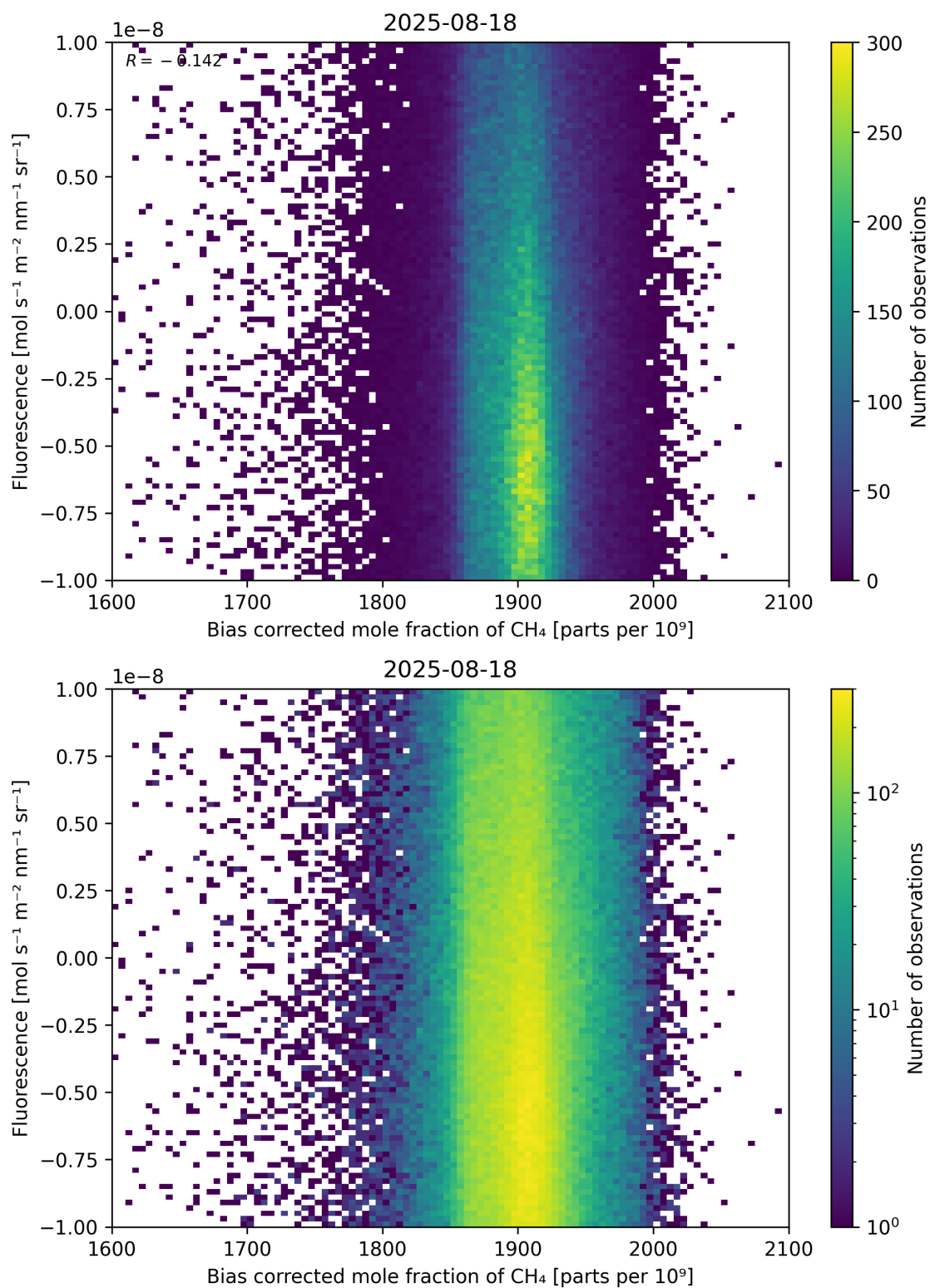
Figure 66: Scatter density plot of “Bias corrected mole fraction of \text{CH}_4 ” against “Fluorescence” for 2025-08-17 to 2025-08-19.
