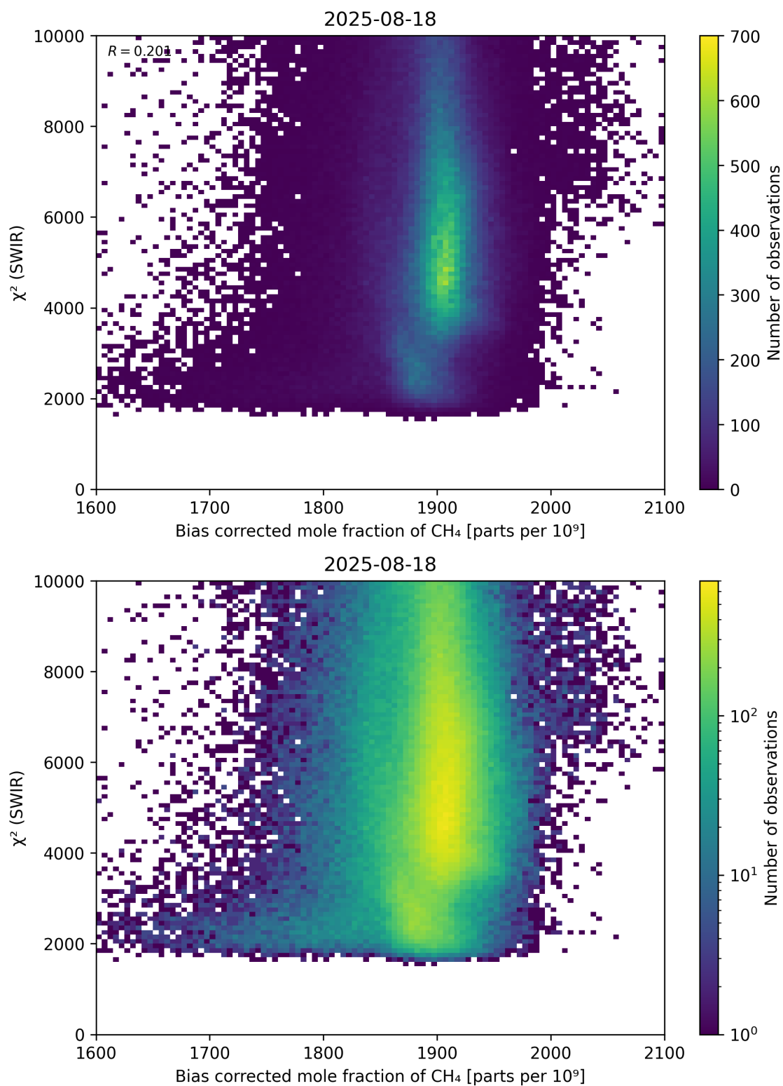
Figure 64: Scatter density plot of “Bias corrected mole fraction of \text{CH}_4 ” against “ \chi^2 (SWIR)” for 2025-08-17 to 2025-08-19.
