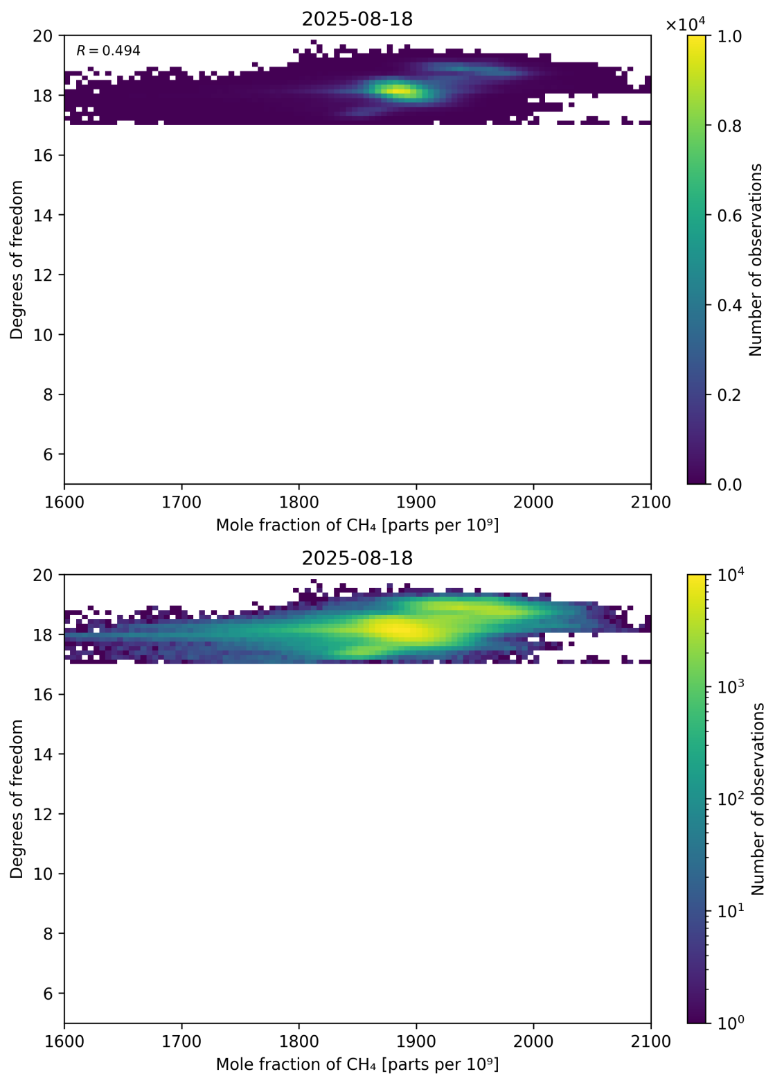
Figure 72: Scatter density plot of “Mole fraction of CH 4 ” against “Degrees of freedom” for 2025-08-17 to 2025-08-19.
