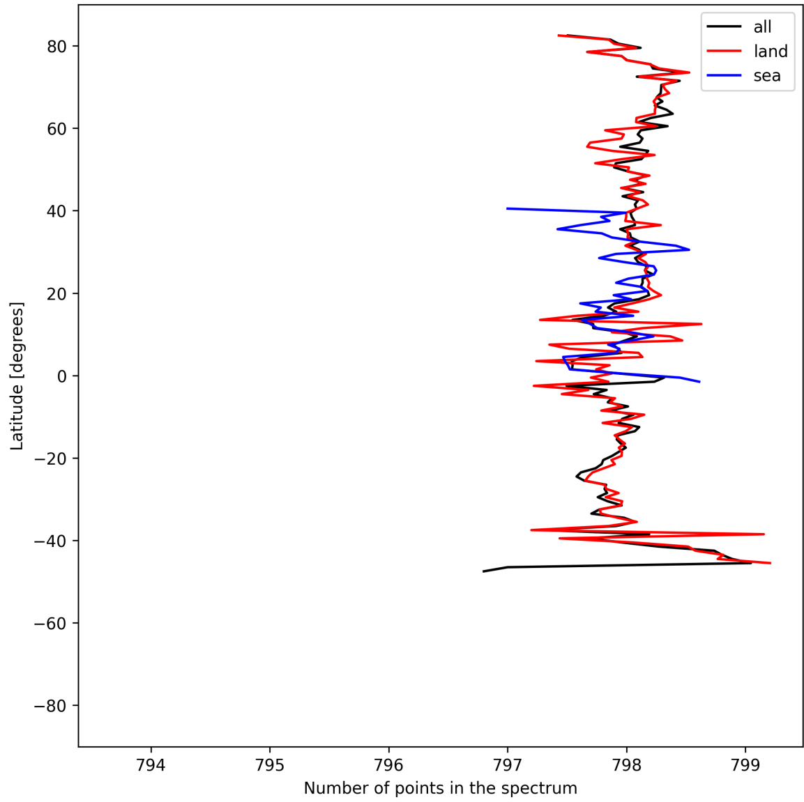
Figure 15: Zonal average of “Number of points in the spectrum” for 2025-08-17 to 2025-08-19.
