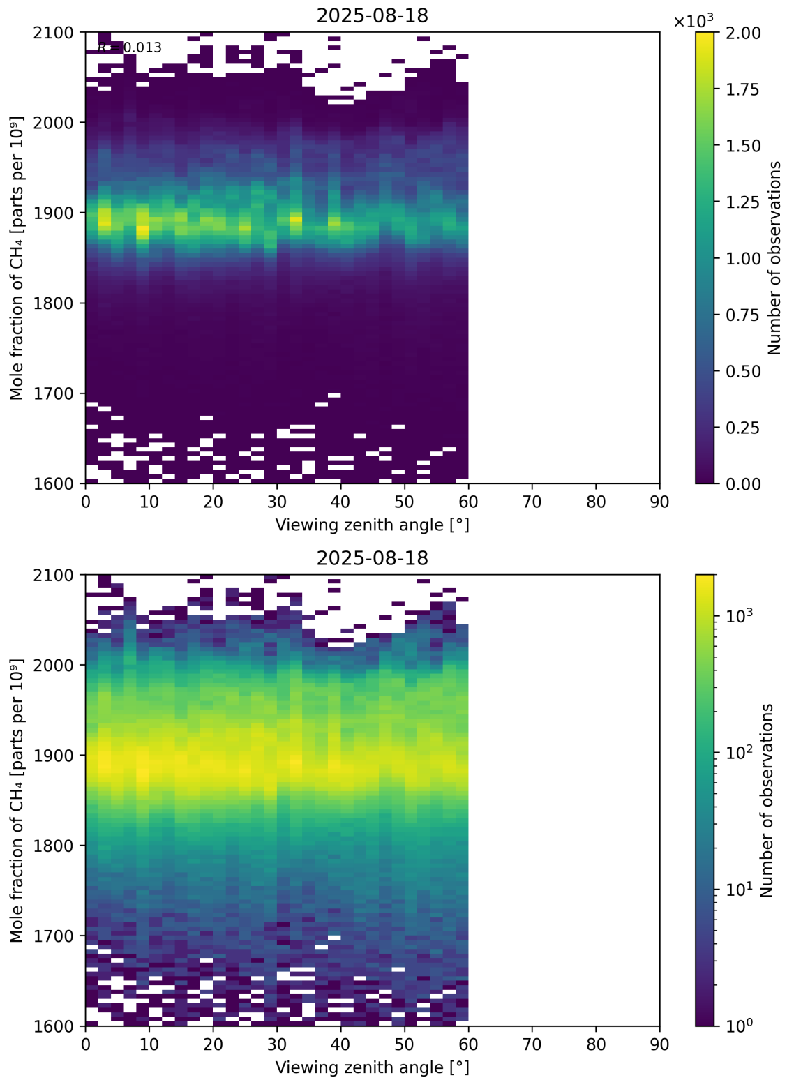
Figure 110: Scatter density plot of “Viewing zenith angle” against “Mole fraction of CH 4 ” for 2025-08-17 to 2025-08-19.
