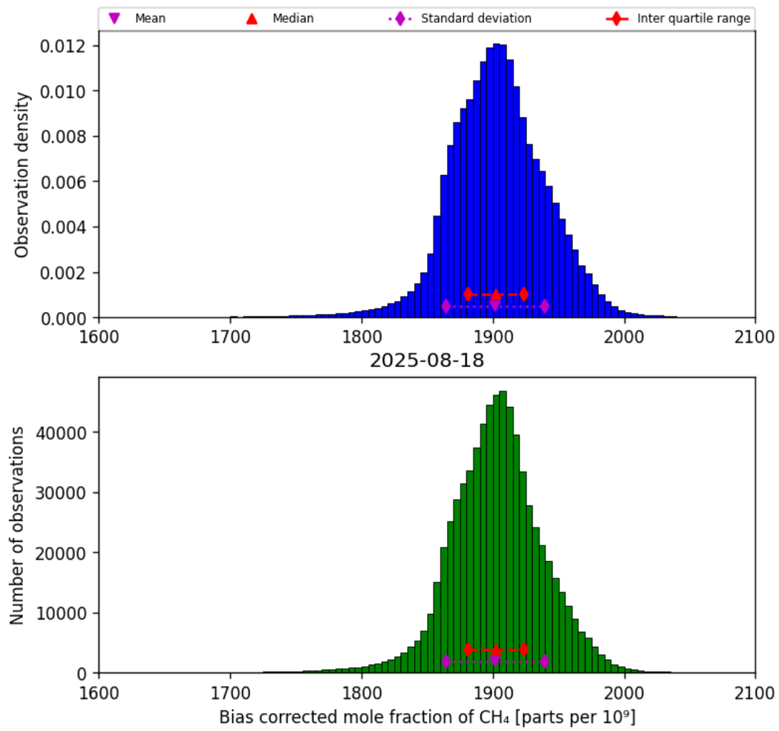
Figure 25: Histogram of “Bias corrected mole fraction of CH 4 ” for 2025-08-17 to 2025-08-19
