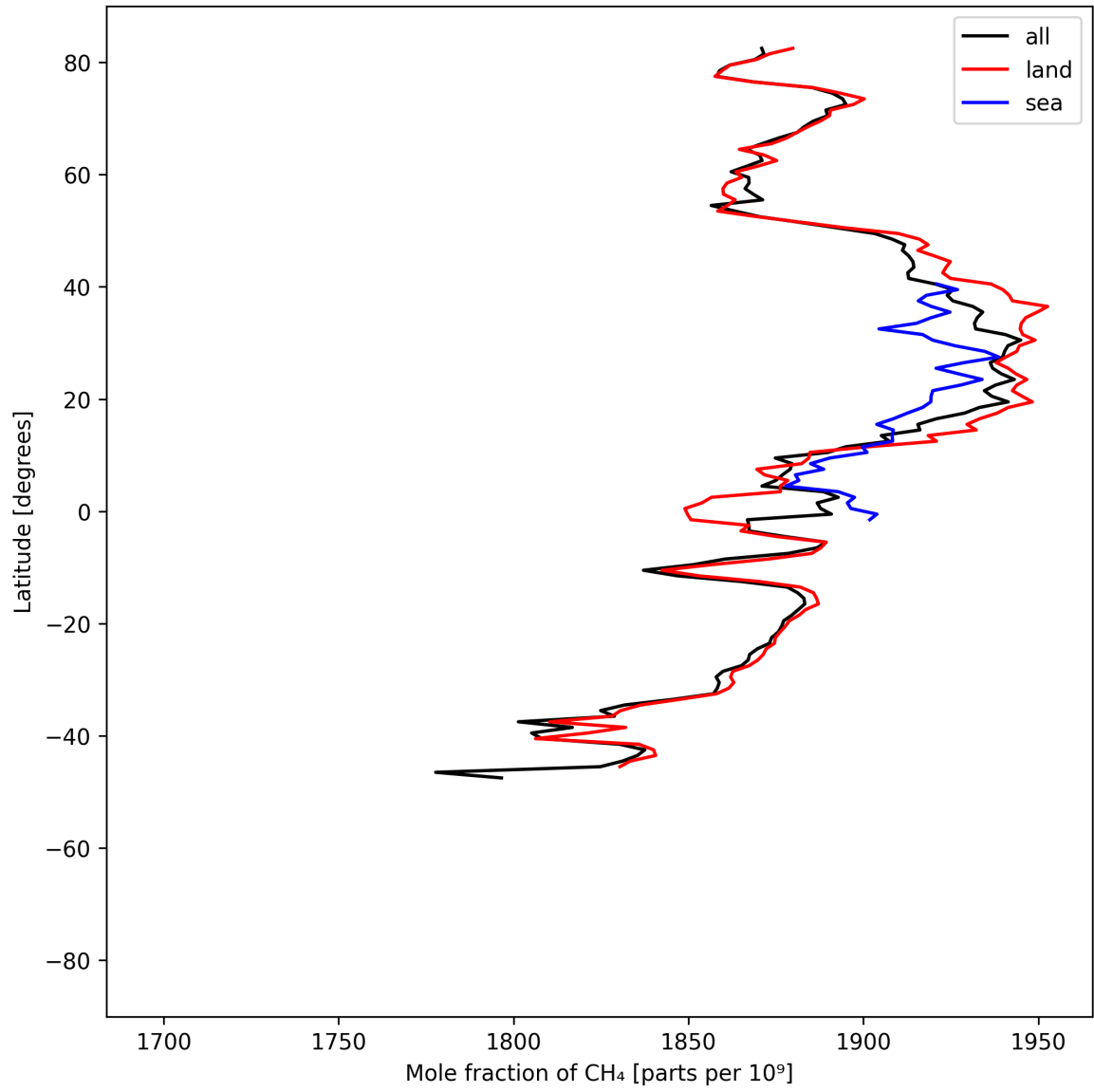
Figure 12: Zonal average of “Mole fraction of \text{CH}_4 ” for 2025-08-17 to 2025-08-19.
