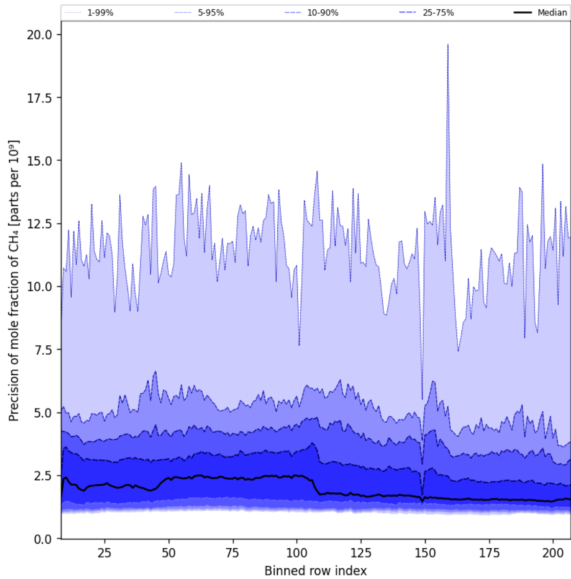
Figure 35: Along track statistics of “Precision of mole fraction of CH 4 ” for 2025-08-17 to 2025-08-19
