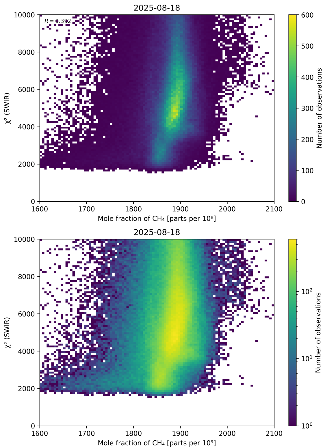
Figure 71: Scatter density plot of “Mole fraction of \text{CH}_4 ” against “ \chi^2 (SWIR)” for 2025-08-17 to 2025-08-19.
