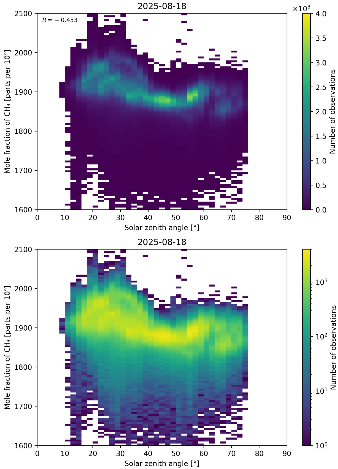
Figure 99: Scatter density plot of “Solar zenith angle” against “Mole fraction of \text{CH}_4 ” for 2025-08-17 to 2025-08-19.
