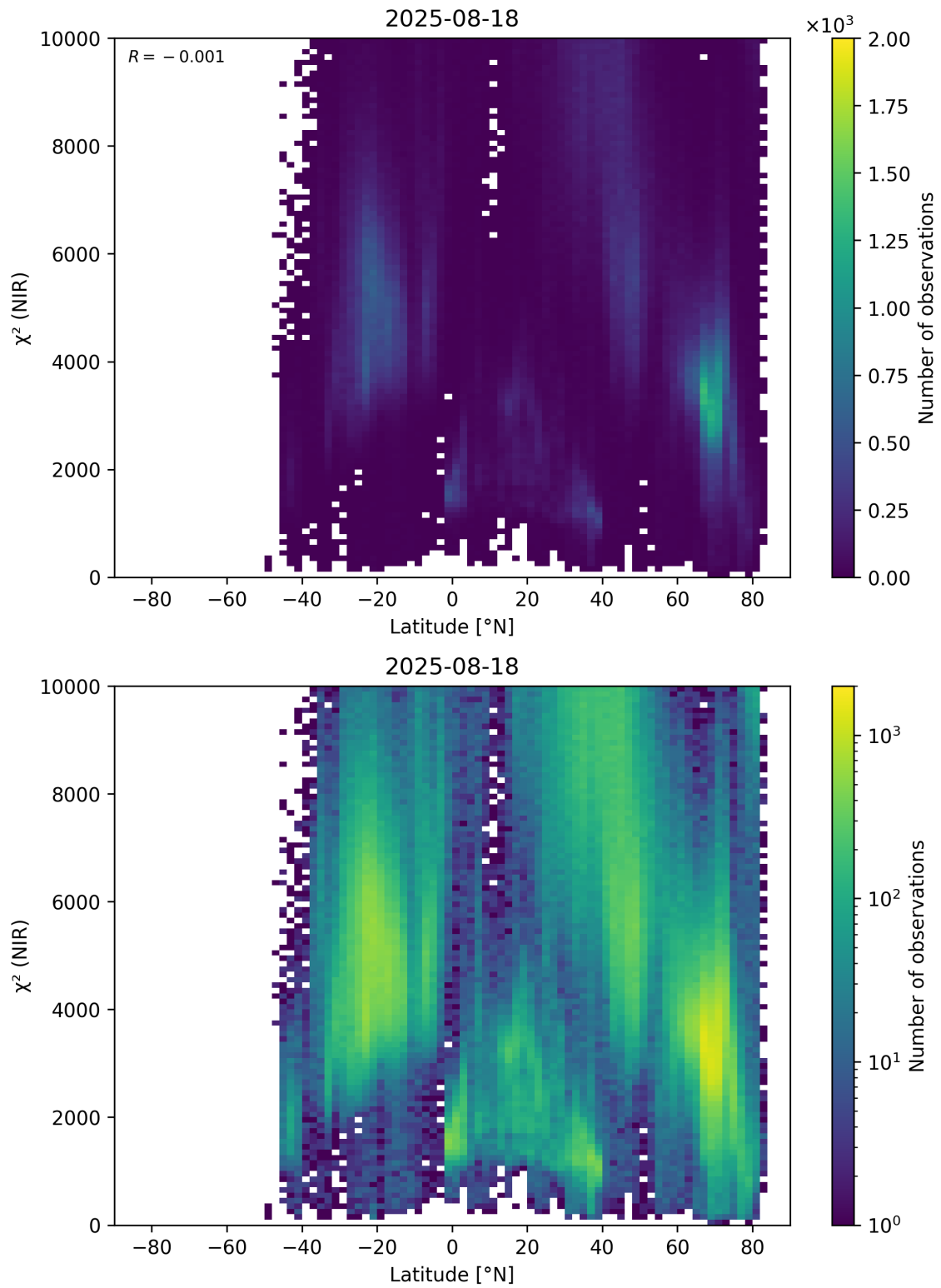
Figure 53: Scatter density plot of “Latitude” against “ \chi^2 (NIR)” for 2025-08-17 to 2025-08-19.
