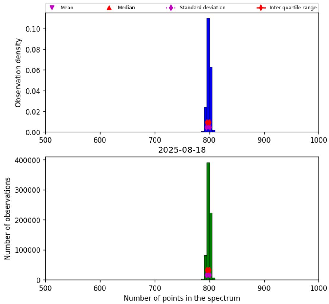
Figure 26: Histogram of “Number of points in the spectrum” for 2025-08-17 to 2025-08-19
