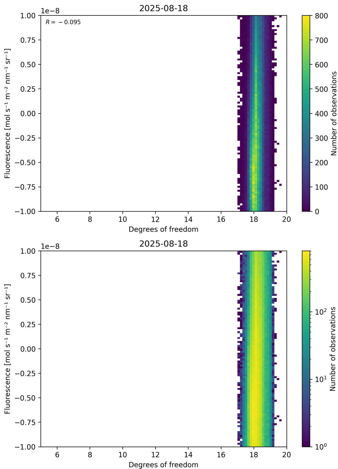
Figure 51: Scatter density plot of “Degrees of freedom” against “Fluorescence” for 2025-08-17 to 2025-08-19.
