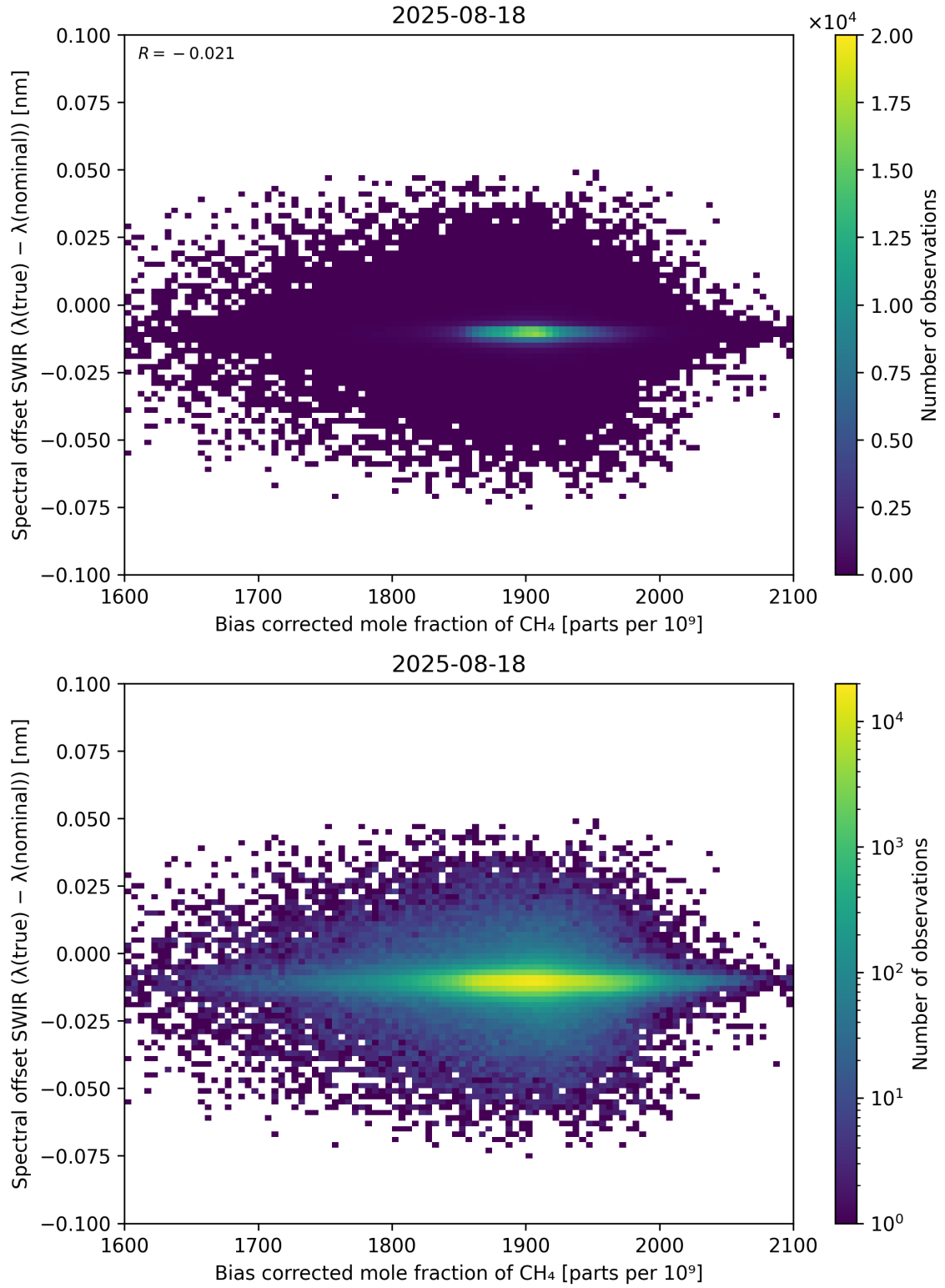
Figure 69: Scatter density plot of “Bias corrected mole fraction of \text{CH}_4 ” against “Spectral offset SWIR ( \lambda_{\text{true}} - \lambda_{\text{nominal}} )” for 2025-08-17 to 2025-08-19.
