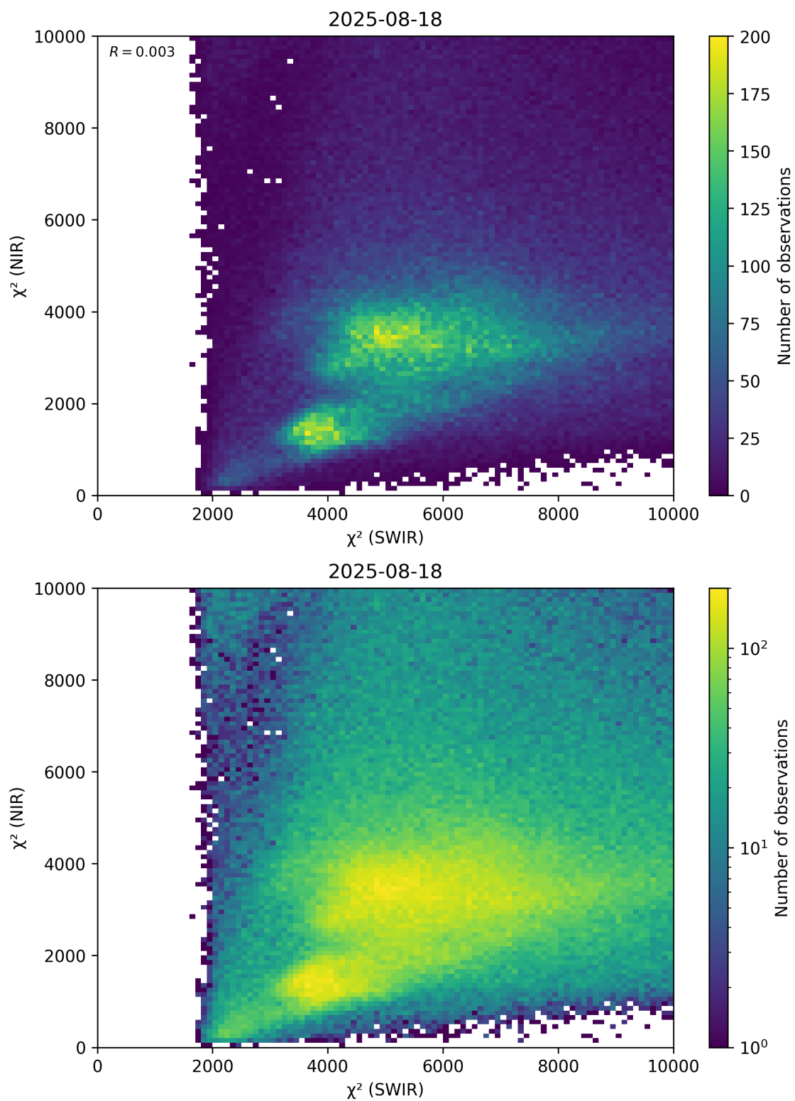
Figure 47: Scatter density plot of “ \chi^2 (SWIR)” against “ \chi^2 (NIR)” for 2025-08-17 to 2025-08-19.
