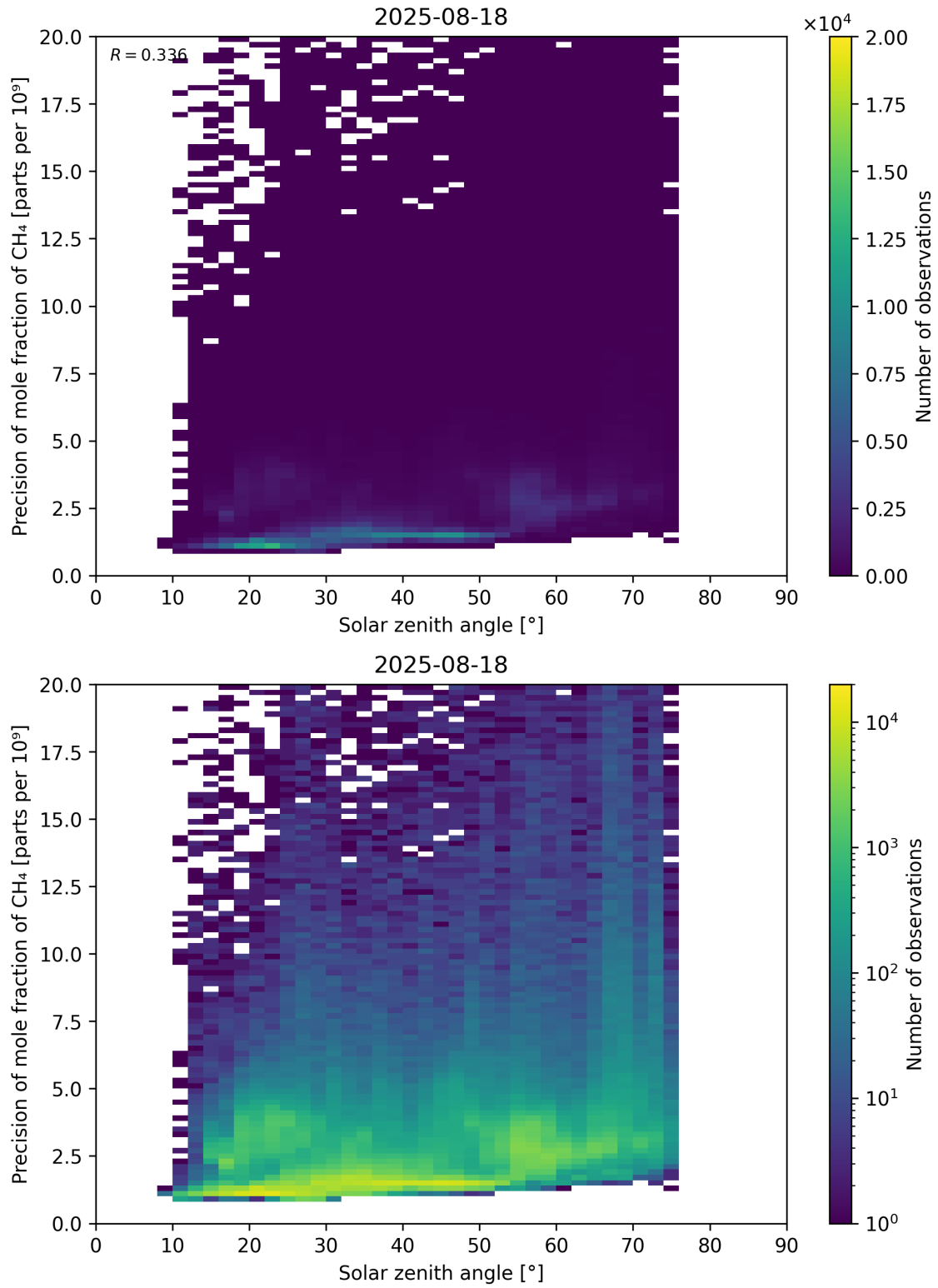
Figure 101: Scatter density plot of “Solar zenith angle” against “Precision of mole fraction of CH 4 ” for 2025-08-17 to 2025-08-19.
