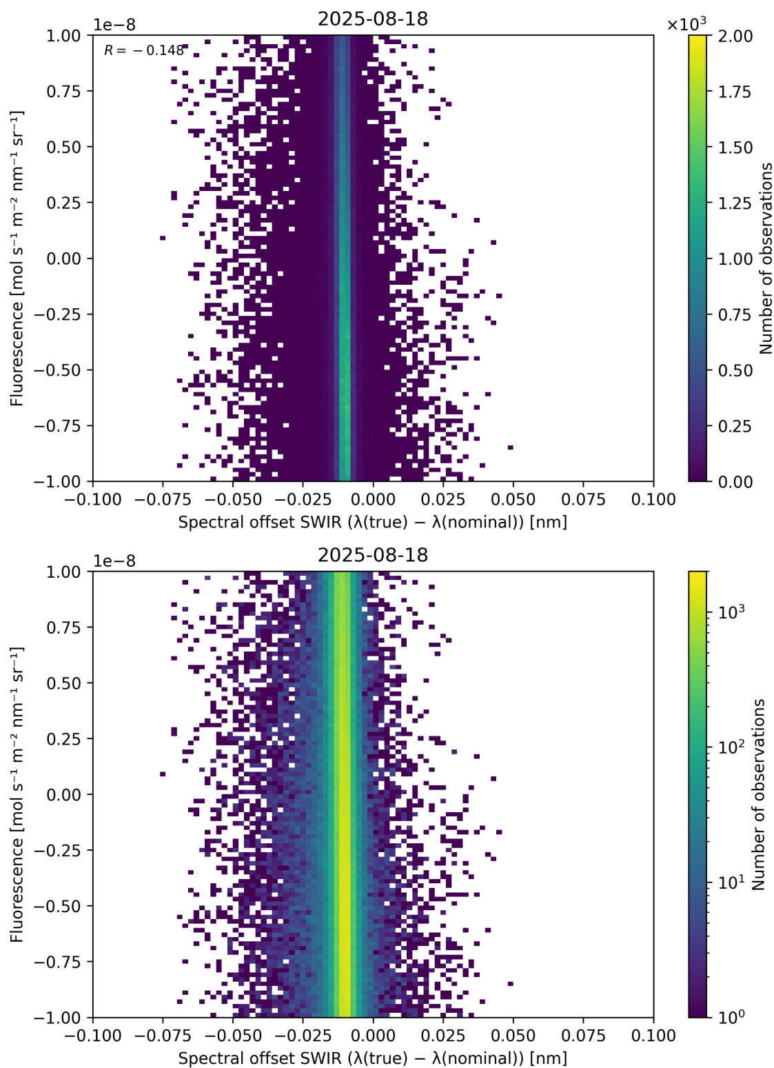
Figure 120: Scatter density plot of “Spectral offset SWIR ( \lambda_{\text{true}} - \lambda_{\text{nominal}} )” against “Fluorescence” for 2025-08-17 to 2025-08-19.
