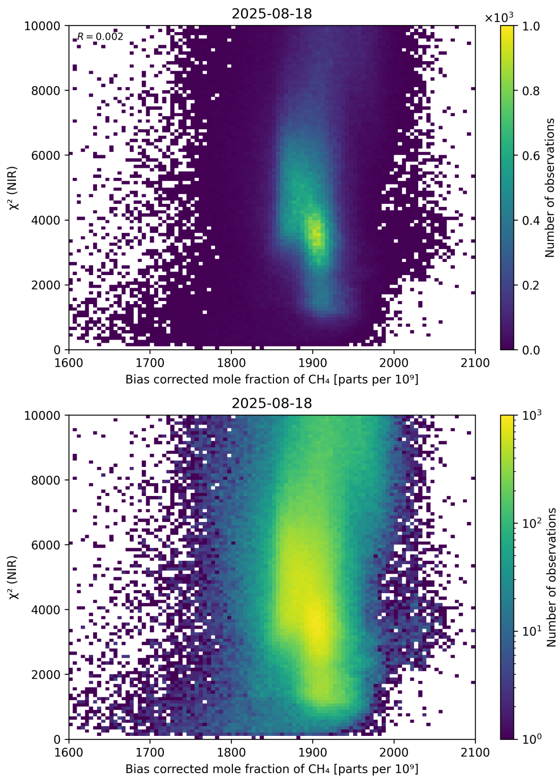
Figure 63: Scatter density plot of “Bias corrected mole fraction of \text{CH}_4 ” against “ \chi^2 (NIR)” for 2025-08-17 to 2025-08-19.
