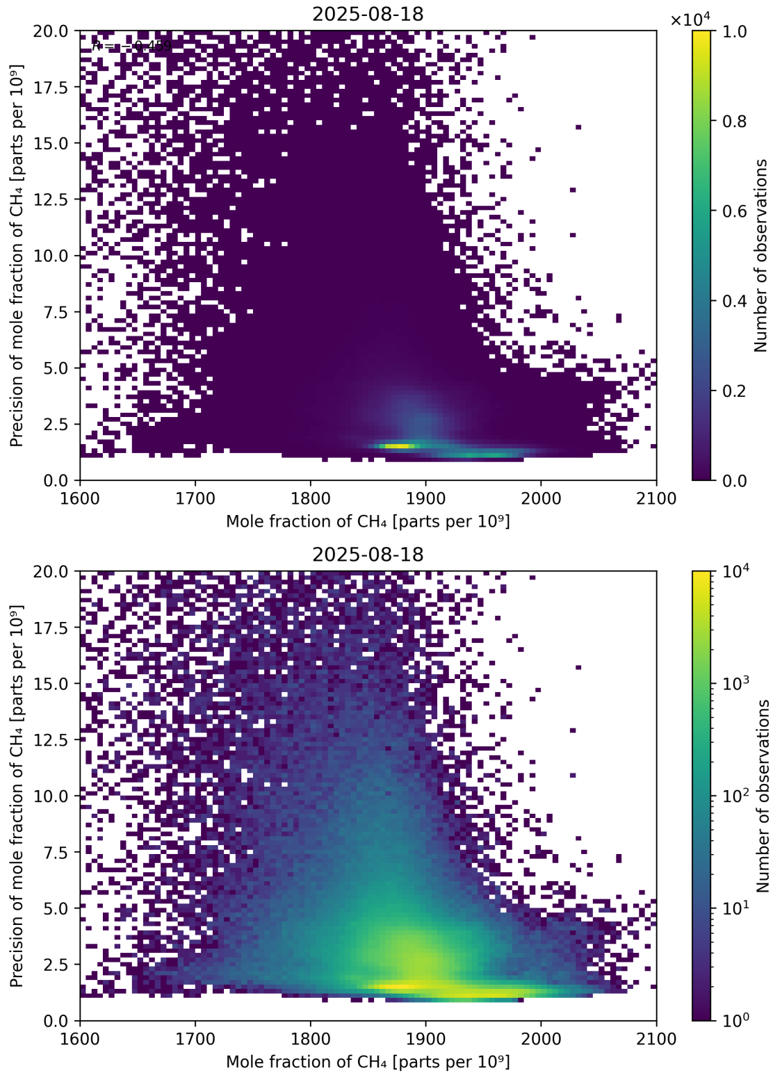
Figure 75: Scatter density plot of “Mole fraction of CH 4 ” against “Precision of mole fraction of CH 4 ” for 2025-08-17 to 2025-08-19.
