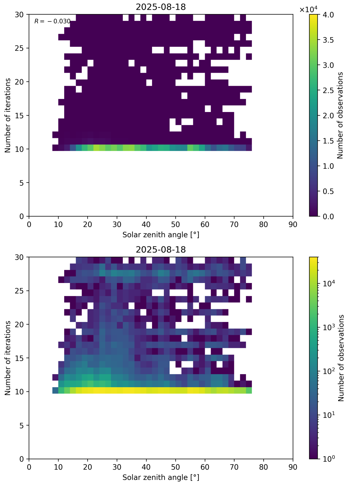
Figure 102: Scatter density plot of “Solar zenith angle” against “Number of iterations” for 2025-08-17 to 2025-08-19.
