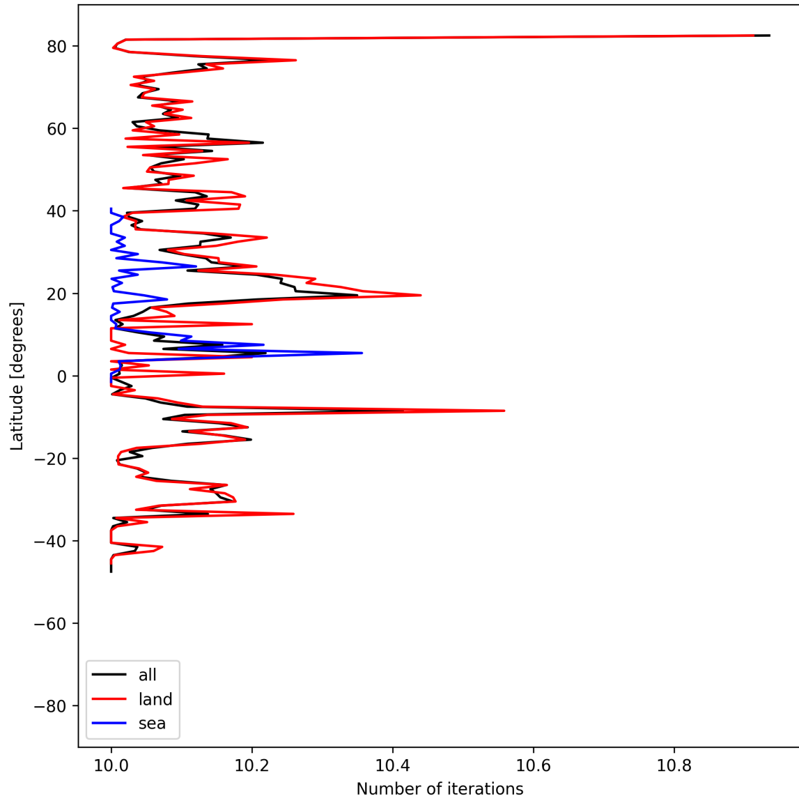
Figure 20: Zonal average of “Number of iterations” for 2025-08-17 to 2025-08-19.
