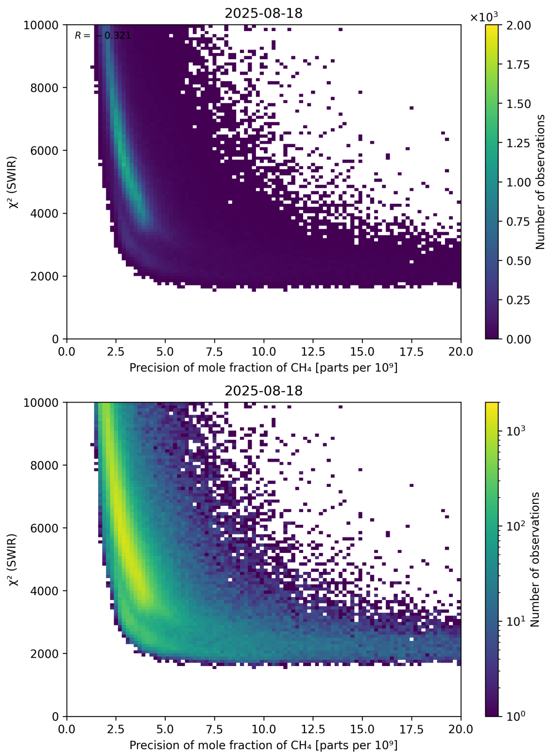
Figure 79: Scatter density plot of “Precision of mole fraction of CH 4 ” against “ \chi^2 (SWIR)” for 2025-08-17 to 2025-08-19.
