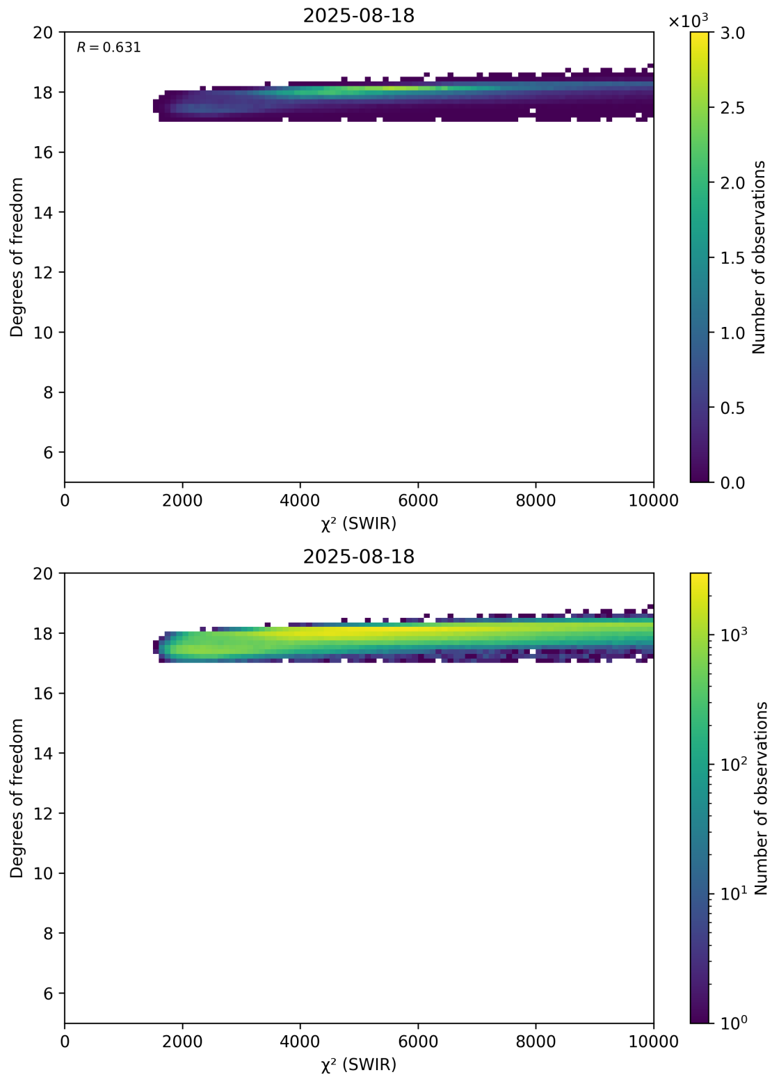
Figure 48: Scatter density plot of “ \chi^2 (SWIR)” against “Degrees of freedom” for 2025-08-17 to 2025-08-19.
