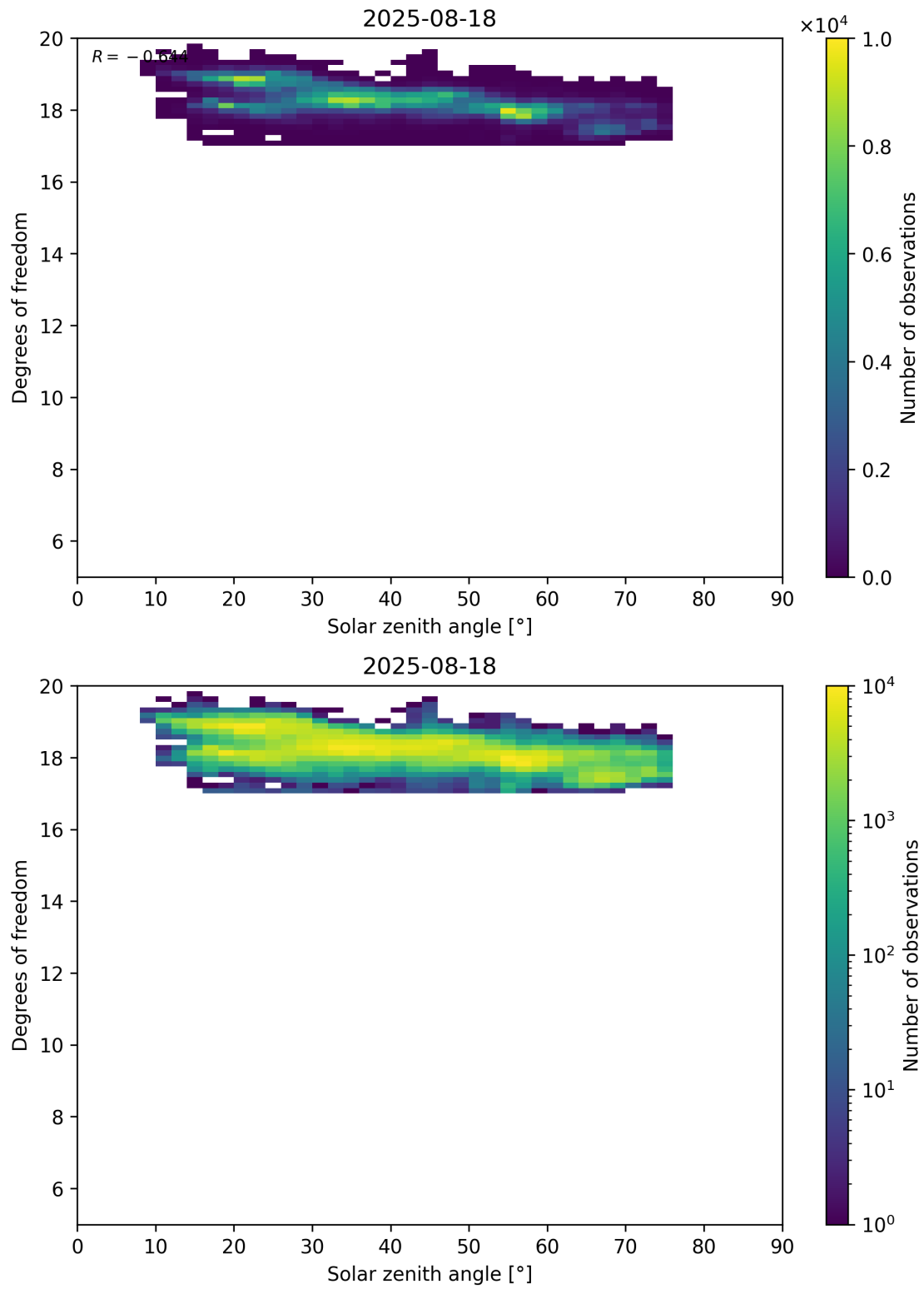
Figure 96: Scatter density plot of “Solar zenith angle” against “Degrees of freedom” for 2025-08-17 to 2025-08-19.
