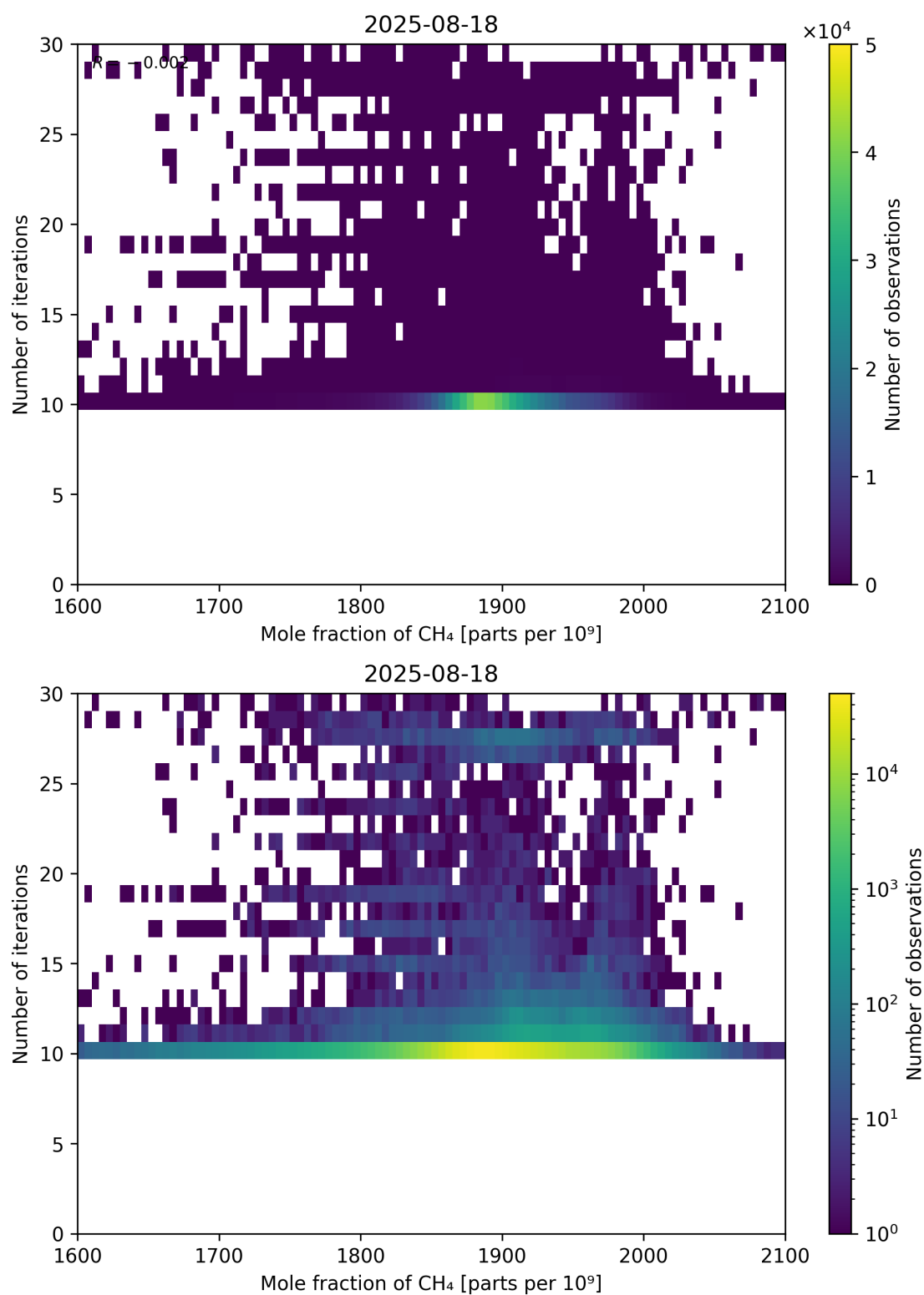
Figure 76: Scatter density plot of “Mole fraction of CH 4 ” against “Number of iterations” for 2025-08-17 to 2025-08-19.
