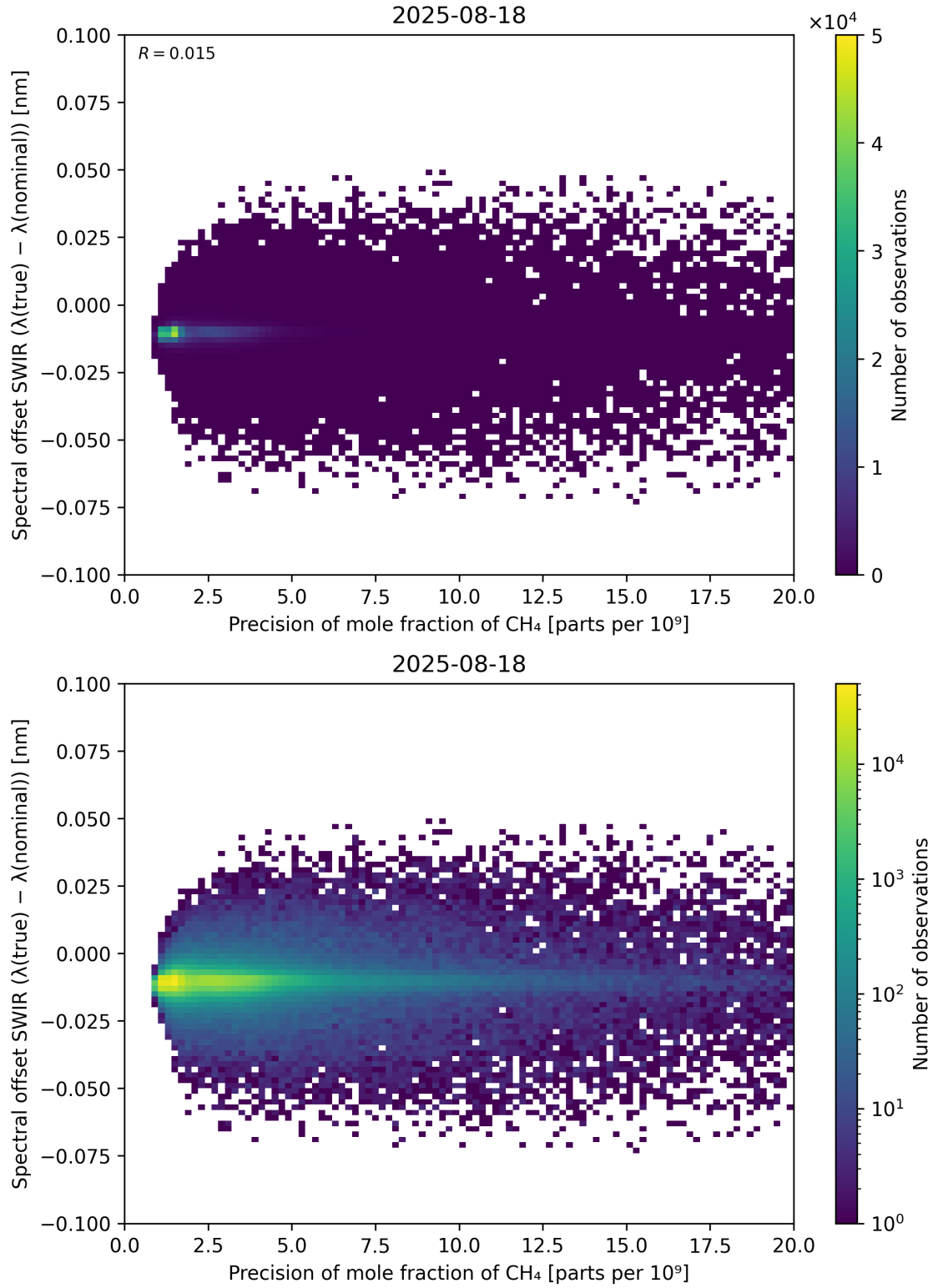
Figure 85: Scatter density plot of “Precision of mole fraction of CH 4 ” against “Spectral offset SWIR ( \lambda_{\text{true}} - \lambda_{\text{nominal}} )” for 2025-08-17 to 2025-08-19.
