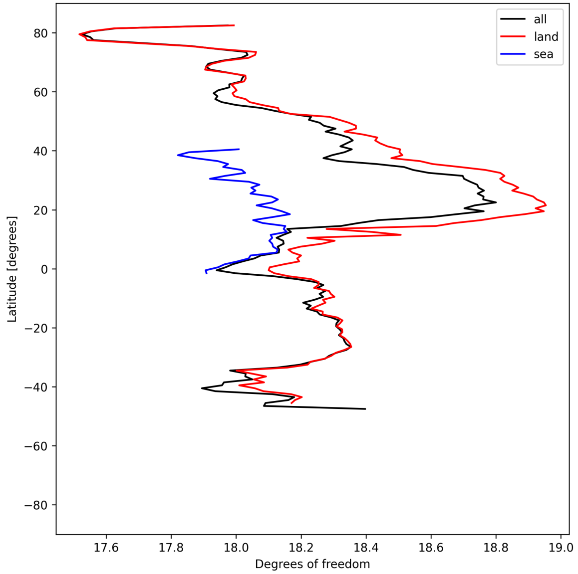
Figure 19: Zonal average of “Degrees of freedom” for 2025-08-17 to 2025-08-19.
