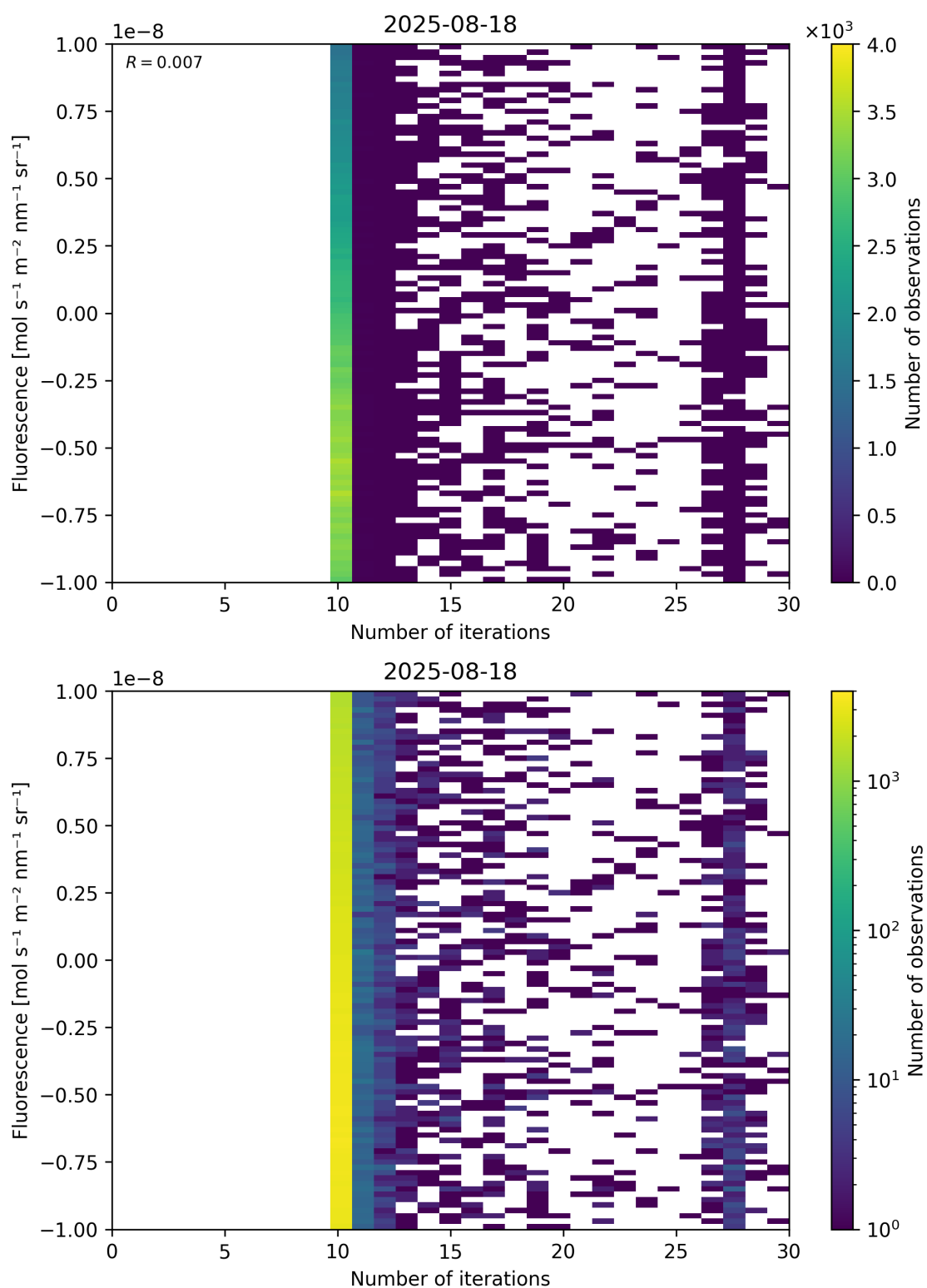
Figure 87: Scatter density plot of “Number of iterations” against “Fluorescence” for 2025-08-17 to 2025-08-19.
