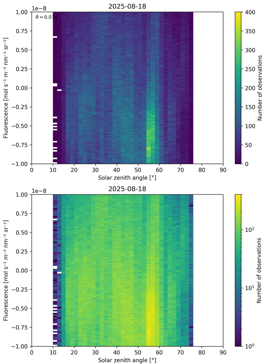
Figure 97: Scatter density plot of “Solar zenith angle” against “Fluorescence” for 2025-08-17 to 2025-08-19.
