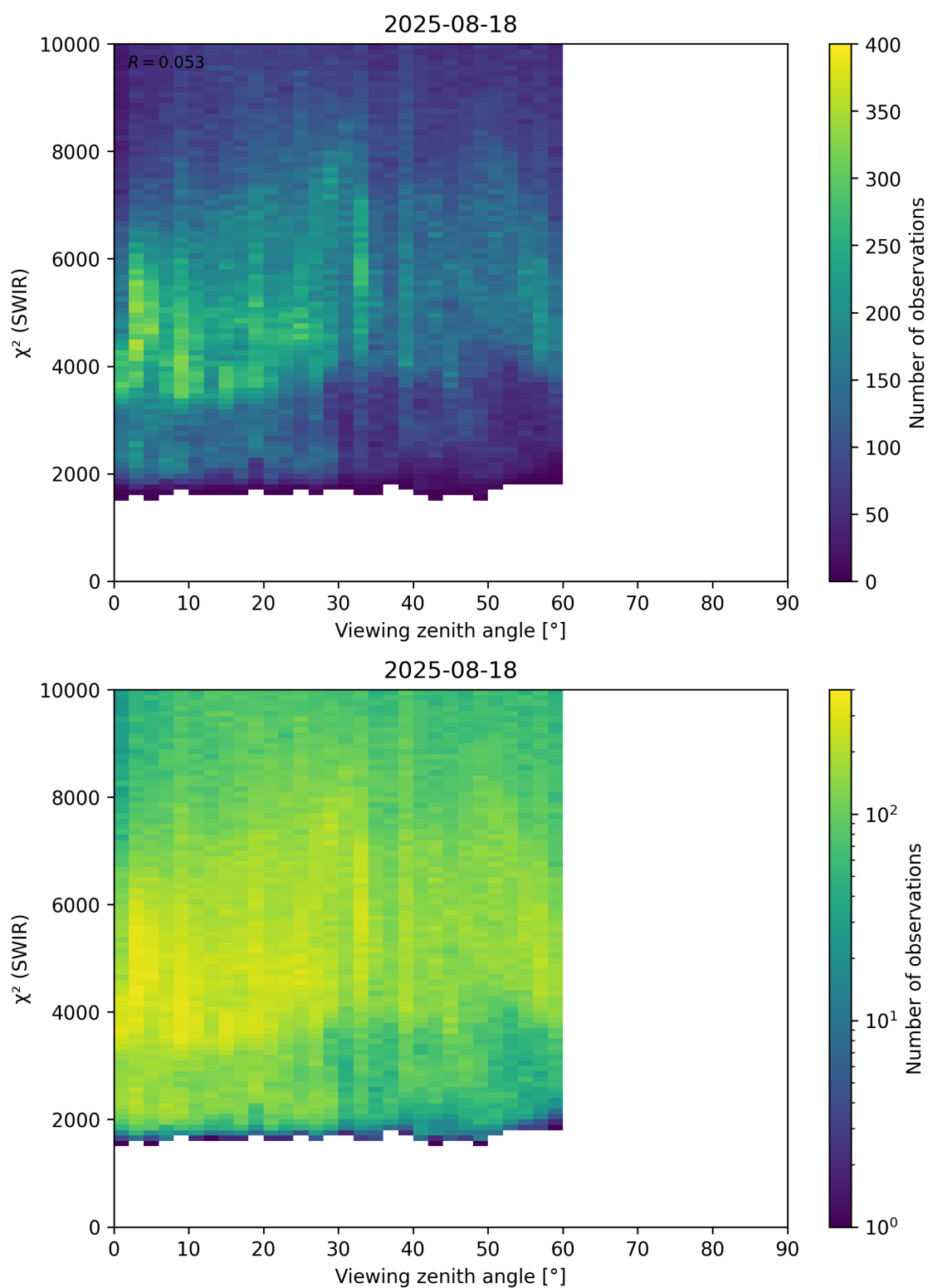
Figure 106: Scatter density plot of “Viewing zenith angle” against “ \chi^2 (SWIR)” for 2025-08-17 to 2025-08-19.
