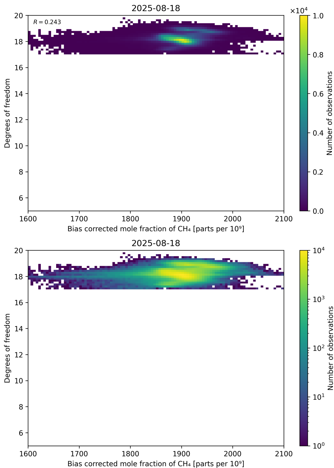
Figure 65: Scatter density plot of “Bias corrected mole fraction of \text{CH}_4 ” against “Degrees of freedom” for 2025-08-17 to 2025-08-19.
