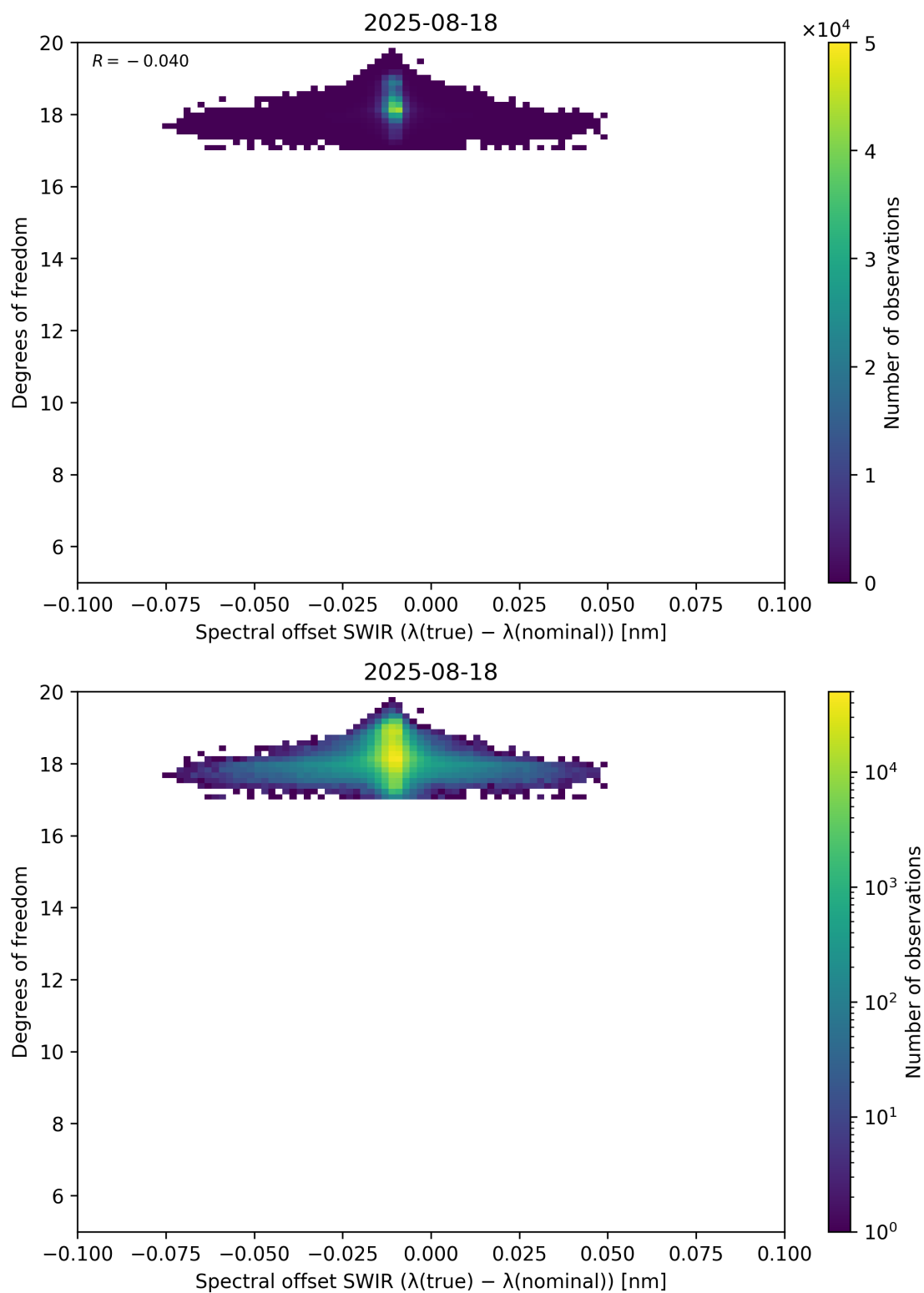
Figure 119: Scatter density plot of “Spectral offset SWIR ( \lambda_{\text{true}} - \lambda_{\text{nominal}} )” against “Degrees of freedom” for 2025-08-17 to 2025-08-19.
