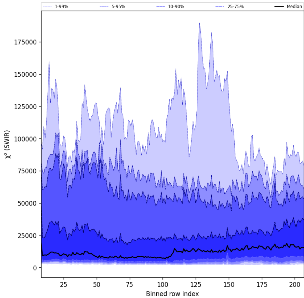
Figure 39: Along track statistics of “ \chi^2 (SWIR)” for 2025-08-17 to 2025-08-19
