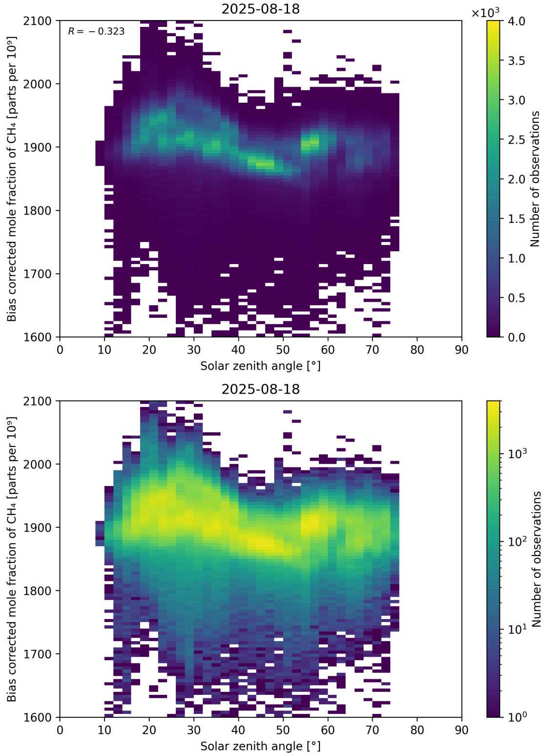
Figure 100: Scatter density plot of “Solar zenith angle” against “Bias corrected mole fraction of CH 4 ” for 2025-08-17 to 2025-08-19.
