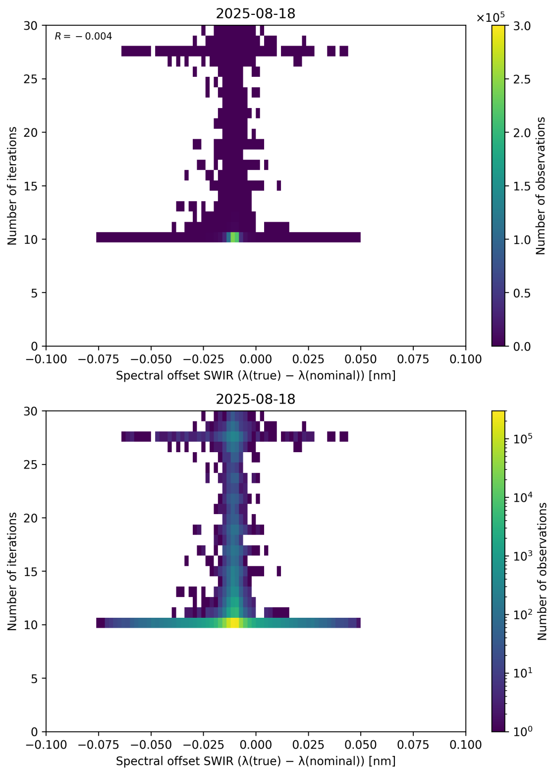
Figure 121: Scatter density plot of “Spectral offset SWIR ( \lambda_{\text{true}} - \lambda_{\text{nominal}} )” against “Number of iterations” for 2025-08-17 to 2025-08-19.
