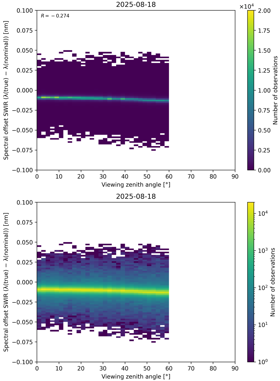
Figure 116: Scatter density plot of “Viewing zenith angle” against “Spectral offset SWIR ( \lambda_{\text{true}} - \lambda_{\text{nominal}} )” for 2025-08-17 to 2025-08-19.
