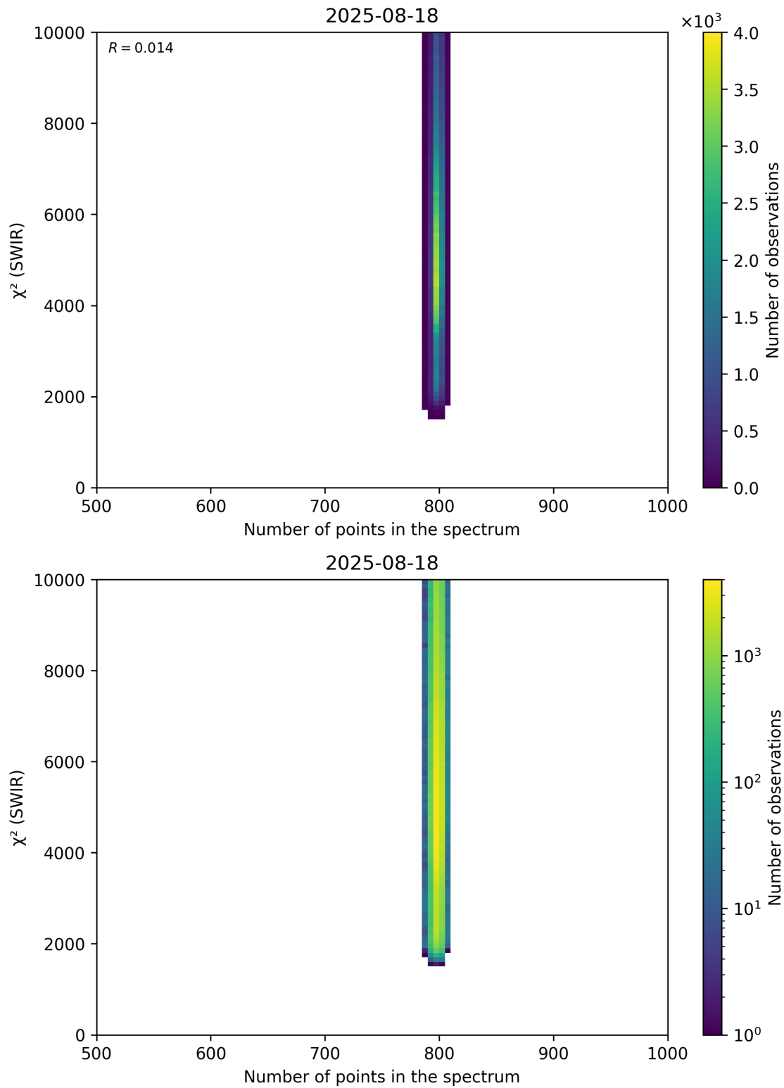
Figure 89: Scatter density plot of “Number of points in the spectrum” against “ \chi^2 (SWIR)” for 2025-08-17 to 2025-08-19.
