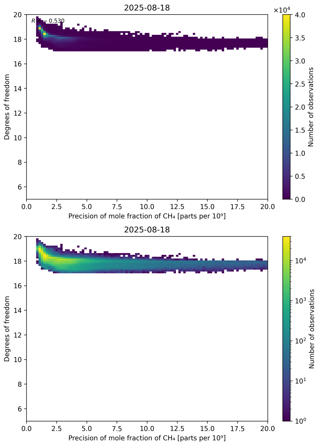
Figure 80: Scatter density plot of “Precision of mole fraction of CH 4 ” against “Degrees of freedom” for 2025-08-17 to 2025-08-19.
