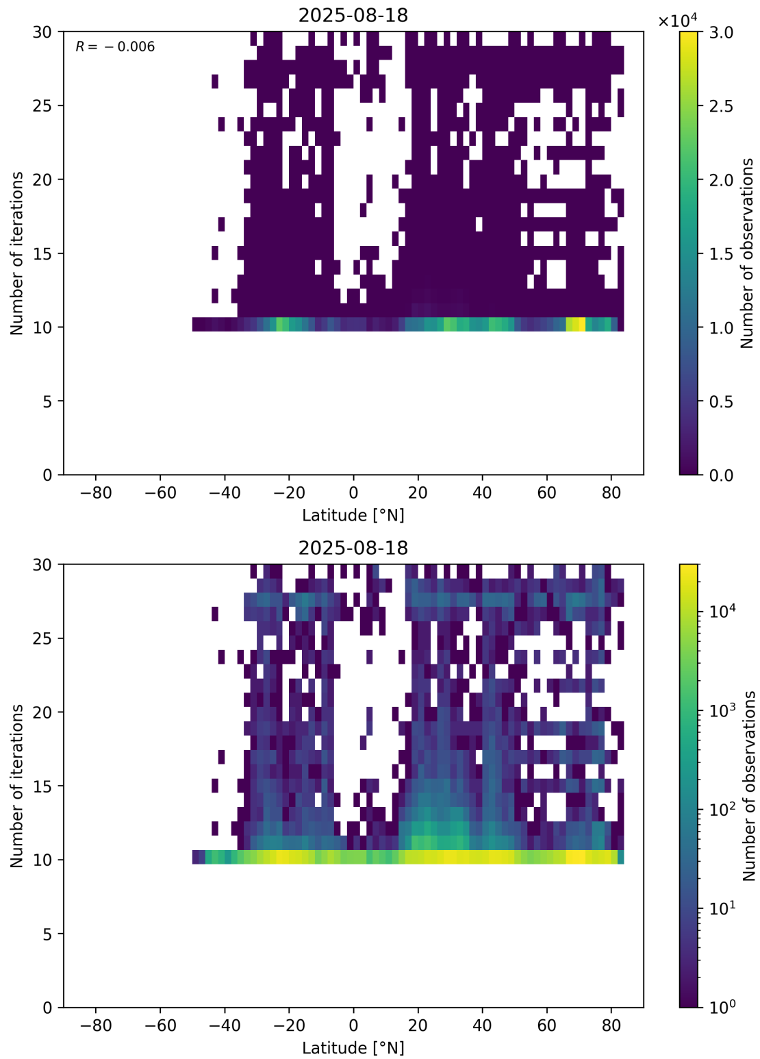
Figure 60: Scatter density plot of “Latitude” against “Number of iterations” for 2025-08-17 to 2025-08-19.
