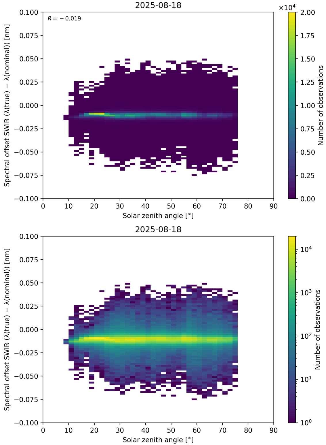
Figure 104: Scatter density plot of “Solar zenith angle” against “Spectral offset SWIR ( \lambda_{\text{true}} - \lambda_{\text{nominal}} )” for 2025-08-17 to 2025-08-19.
