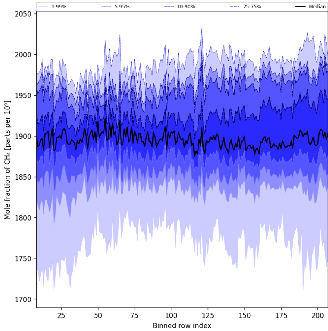
Figure 34: Along track statistics of “Mole fraction of CH 4 ” for 2025-08-17 to 2025-08-19
