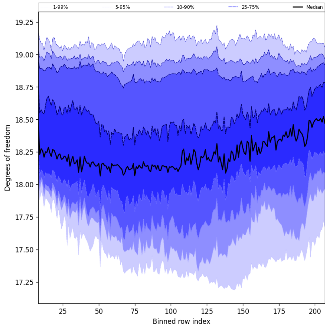
Figure 41: Along track statistics of “Degrees of freedom” for 2025-08-17 to 2025-08-19
