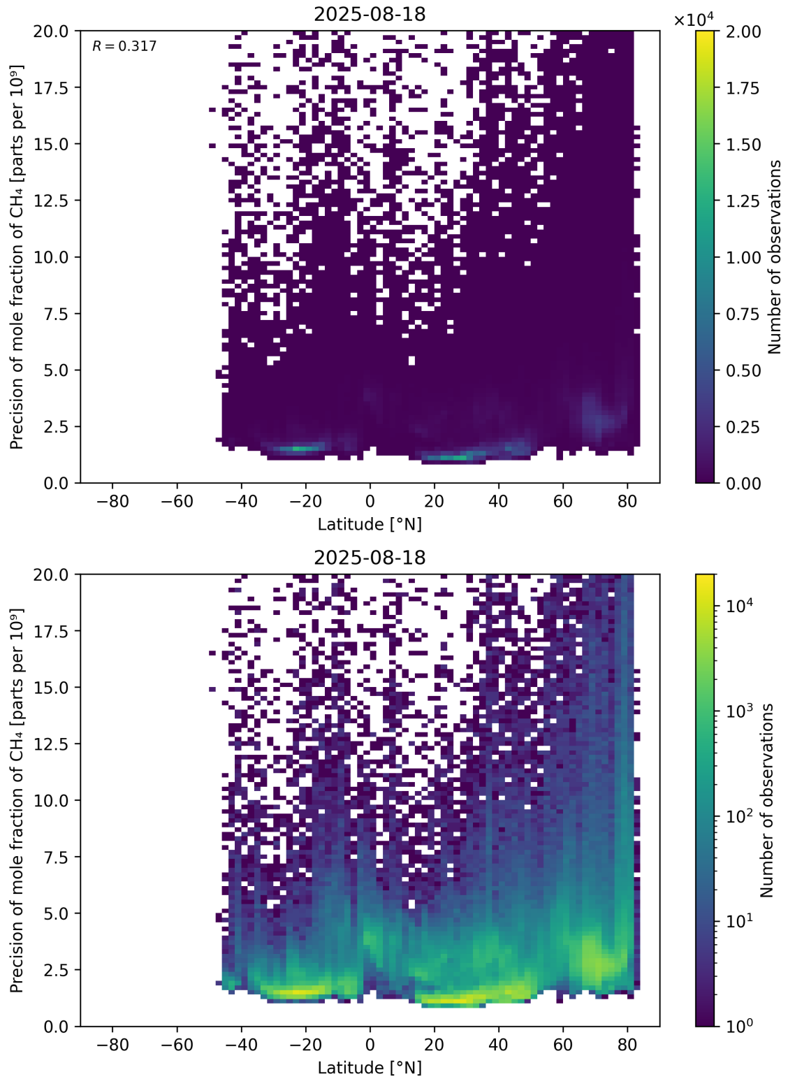
Figure 59: Scatter density plot of “Latitude” against “Precision of mole fraction of \text{CH}_4 ” for 2025-08-17 to 2025-08-19.
