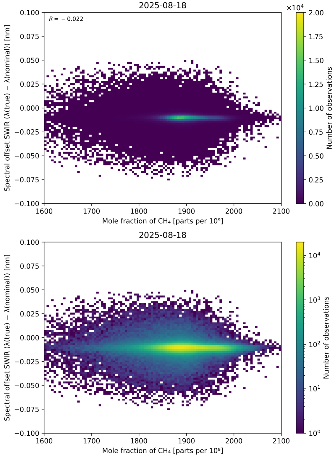
Figure 86: Scatter density plot of “Mole fraction of CH 4 ” against “Spectral offset SWIR ( \lambda_{\text{true}} - \lambda_{\text{nominal}} )” for 2025-08-17 to 2025-08-19.
