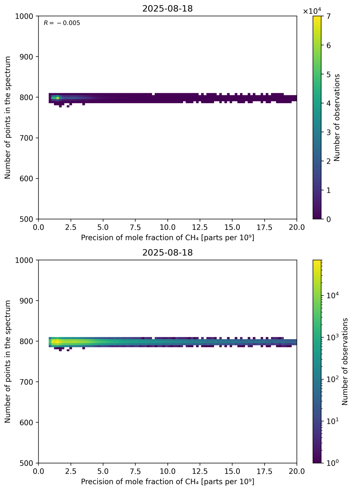
Figure 84: Scatter density plot of “Precision of mole fraction of CH 4 ” against “Number of points in the spectrum” for 2025-08-17 to 2025-08-19.
