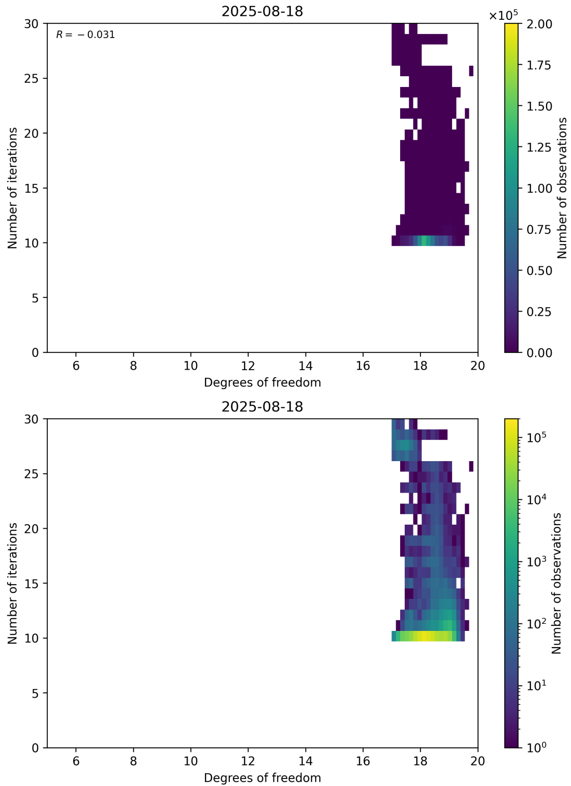
Figure 52: Scatter density plot of “Degrees of freedom” against “Number of iterations” for 2025-08-17 to 2025-08-19.
