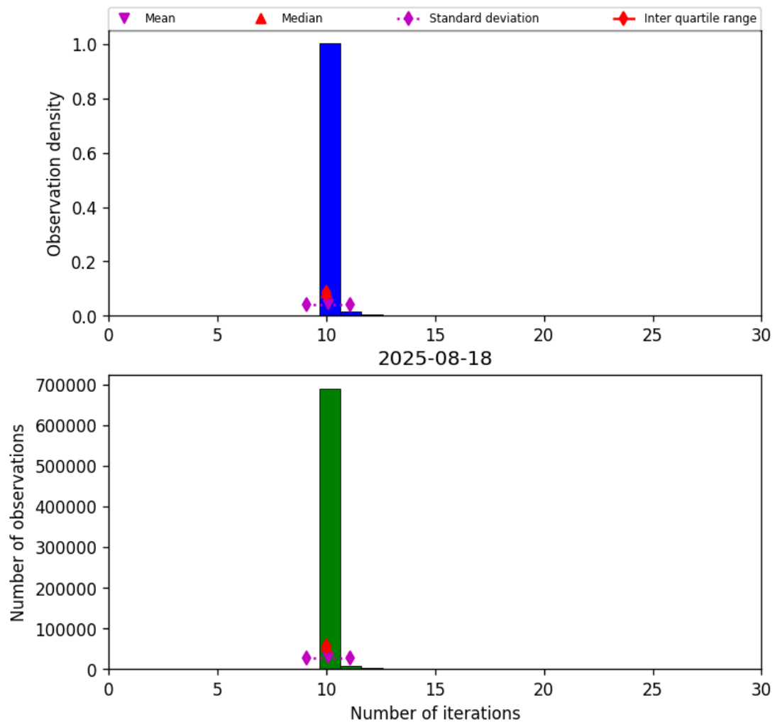
Figure 31: Histogram of “Number of iterations” for 2025-08-17 to 2025-08-19
