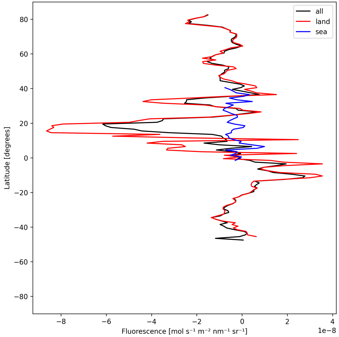
Figure 21: Zonal average of “Fluorescence” for 2025-08-17 to 2025-08-19.
