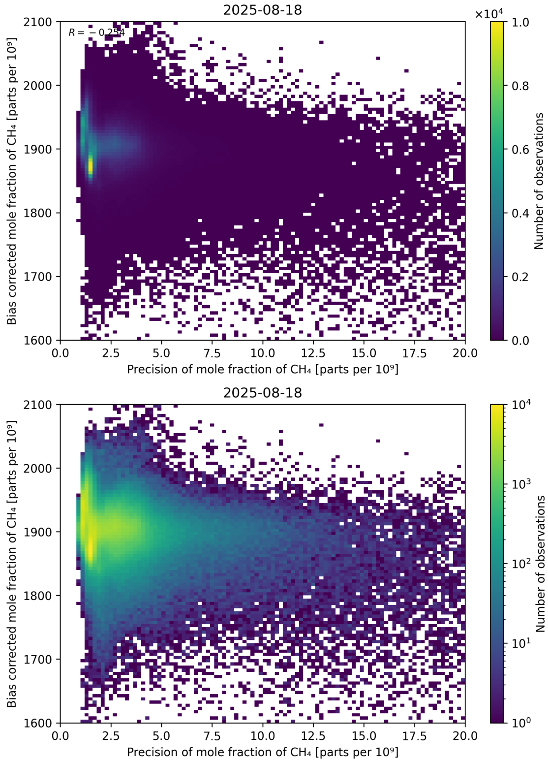
Figure 82: Scatter density plot of “Precision of mole fraction of CH 4 ” against “Bias corrected mole fraction of CH 4 ” for 2025-08-17 to 2025-08-19.
