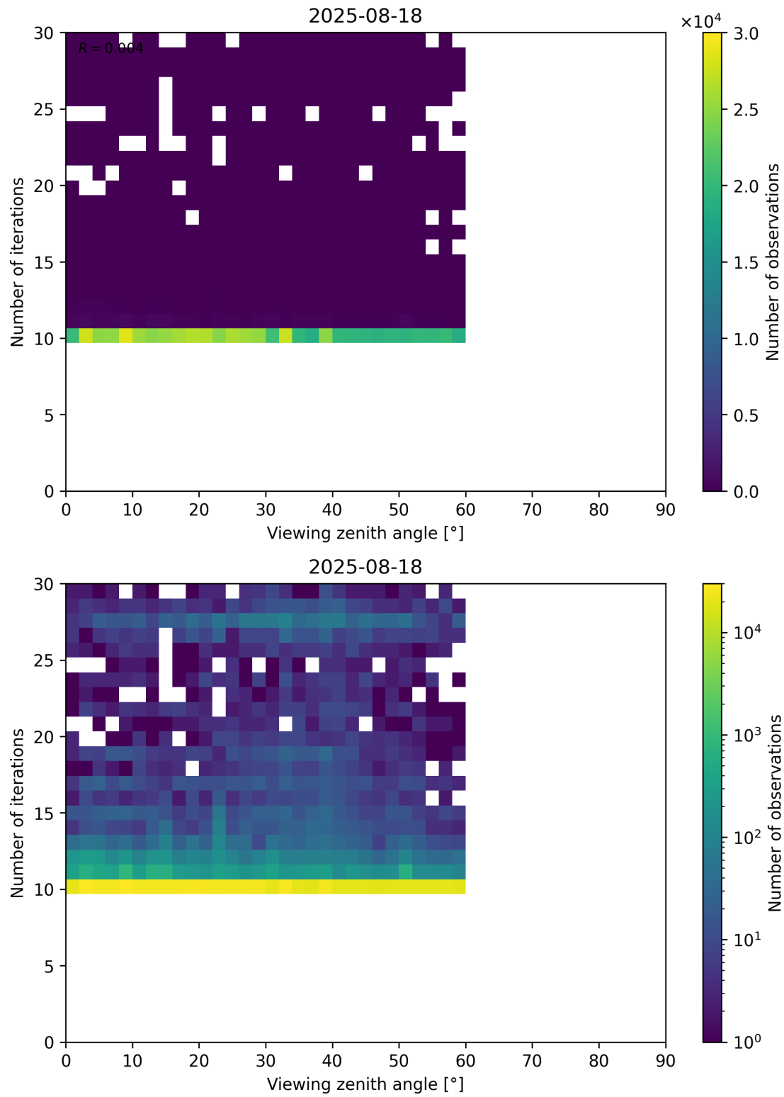
Figure 113: Scatter density plot of “Viewing zenith angle” against “Number of iterations” for 2025-08-17 to 2025-08-19.
