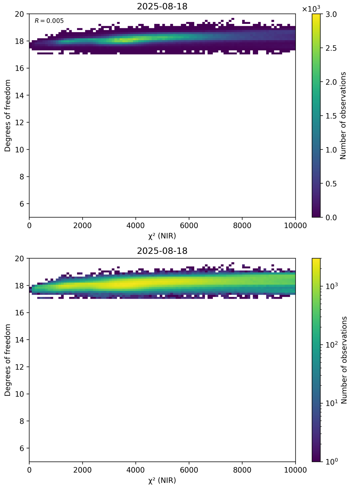
Figure 44: Scatter density plot of “ \chi^2 (NIR)” against “Degrees of freedom” for 2025-08-17 to 2025-08-19.
