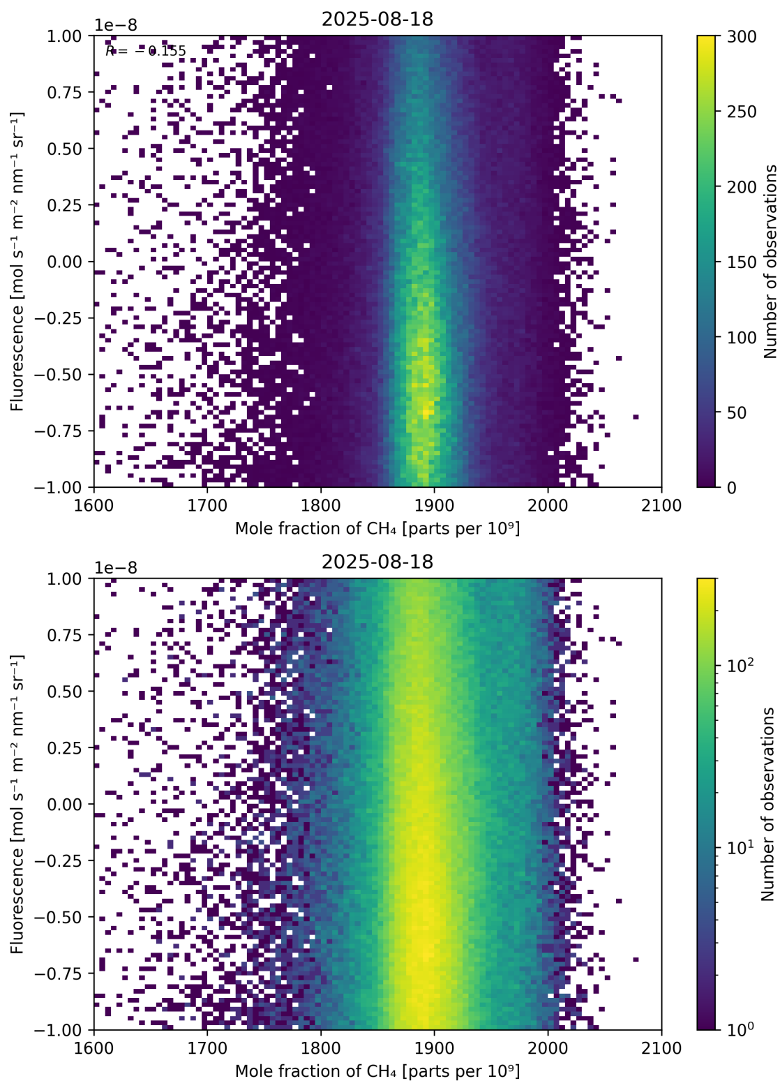
Figure 73: Scatter density plot of “Mole fraction of \text{CH}_4 ” against “Fluorescence” for 2025-08-17 to 2025-08-19.
