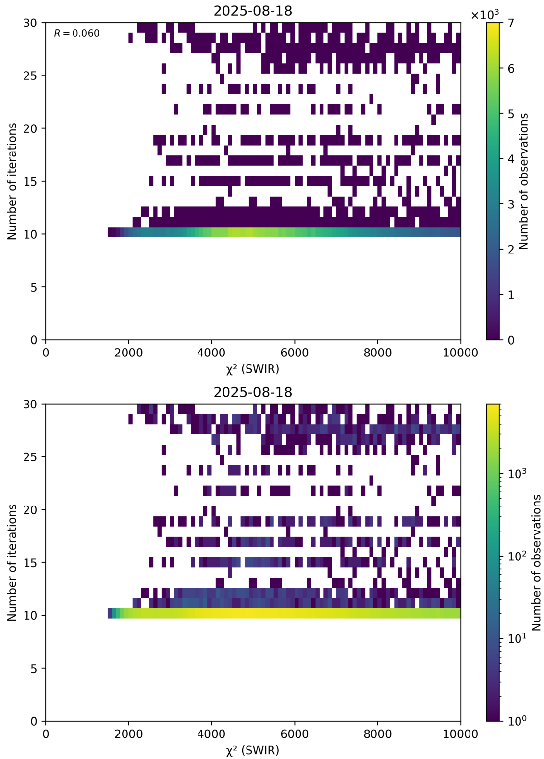
Figure 50: Scatter density plot of “ \chi^2 (SWIR)” against “Number of iterations” for 2025-08-17 to 2025-08-19.
