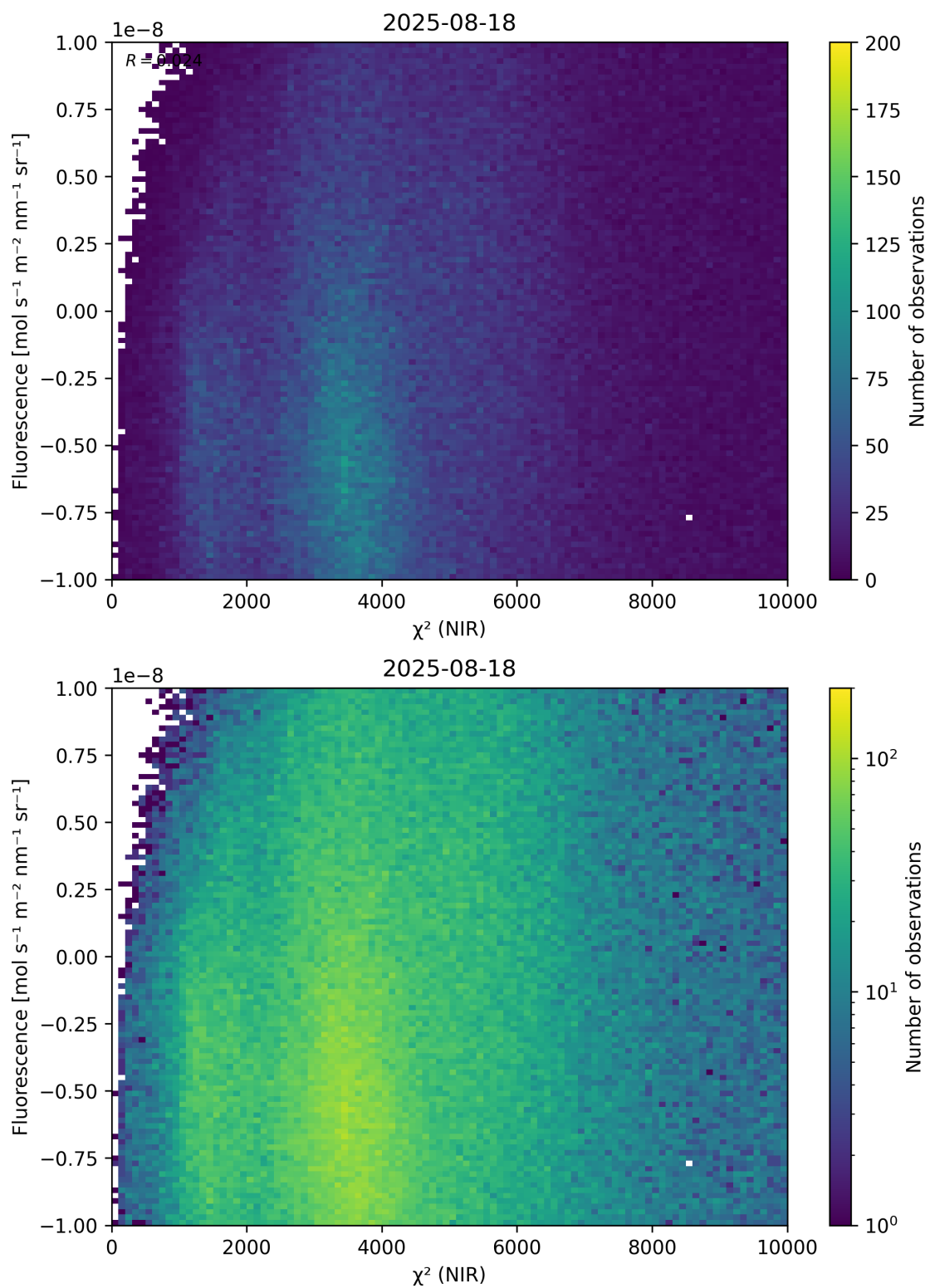
Figure 45: Scatter density plot of “ \chi^2 (NIR)” against “Fluorescence” for 2025-08-17 to 2025-08-19.
