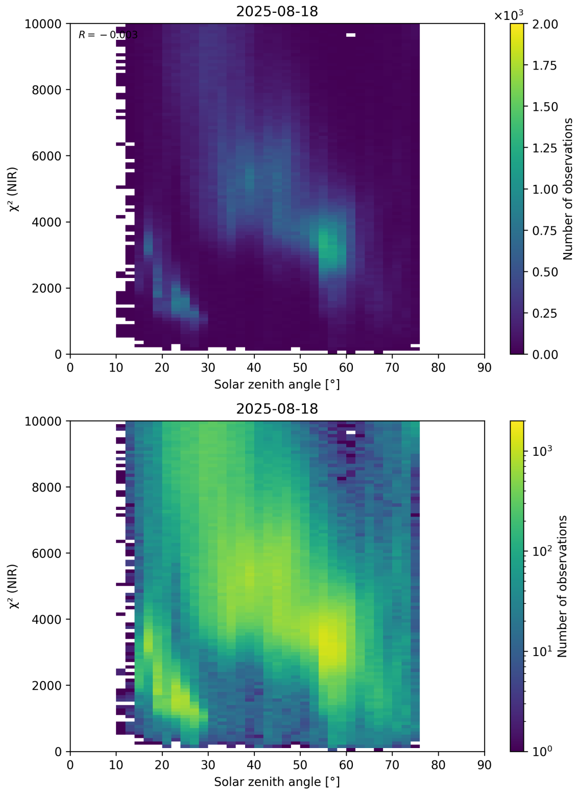
Figure 94: Scatter density plot of “Solar zenith angle” against “ \chi^2 (NIR)” for 2025-08-17 to 2025-08-19.
