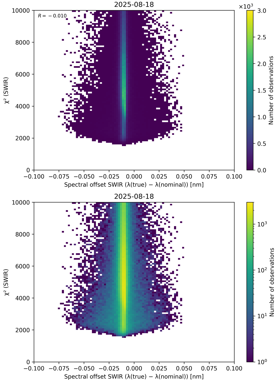
Figure 118: Scatter density plot of “Spectral offset SWIR ( \lambda_{\text{true}} - \lambda_{\text{nominal}} )” against “ \chi^2 (SWIR)” for 2025-08-17 to 2025-08-19.
