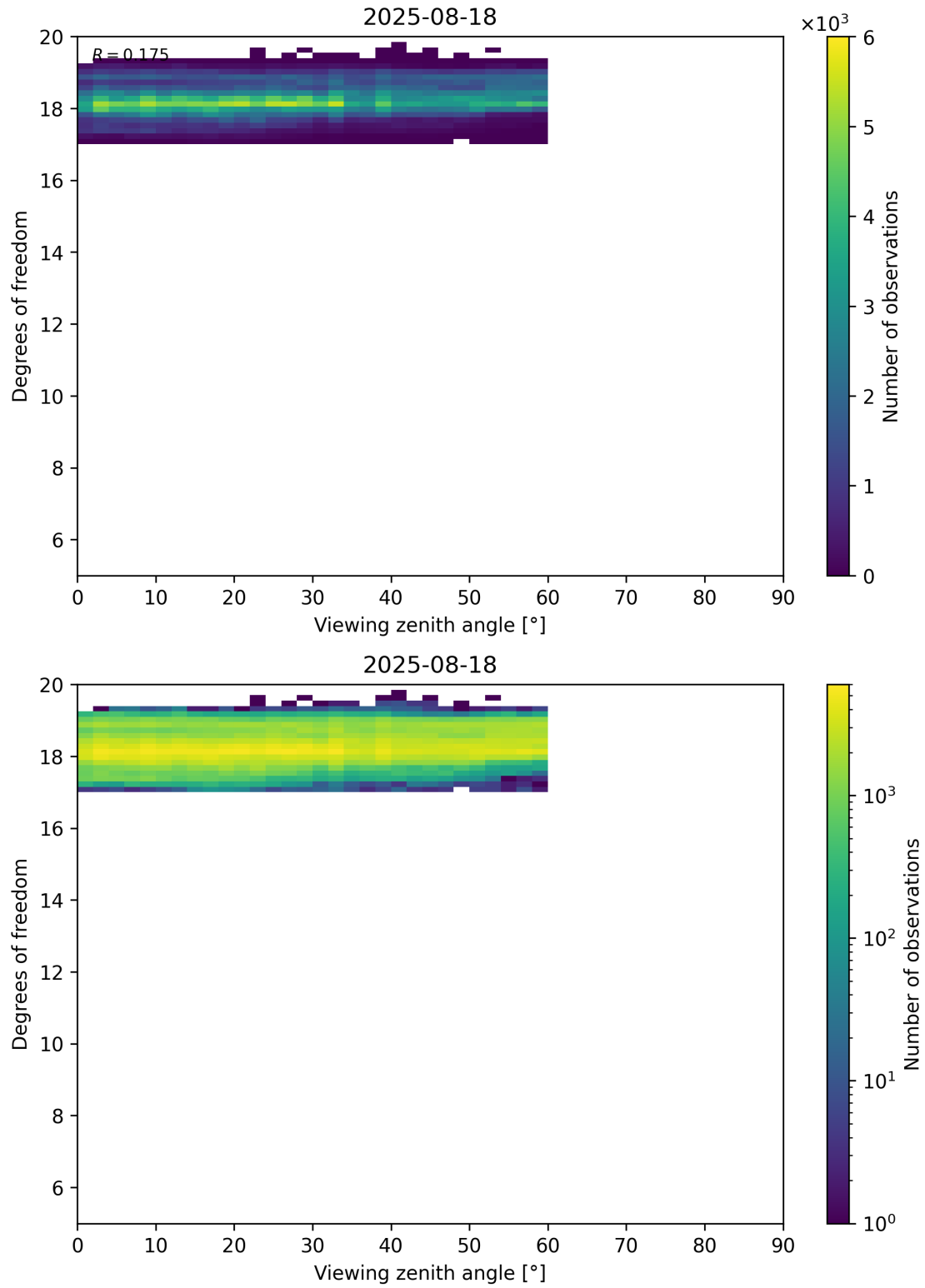
Figure 107: Scatter density plot of “Viewing zenith angle” against “Degrees of freedom” for 2025-08-17 to 2025-08-19.
