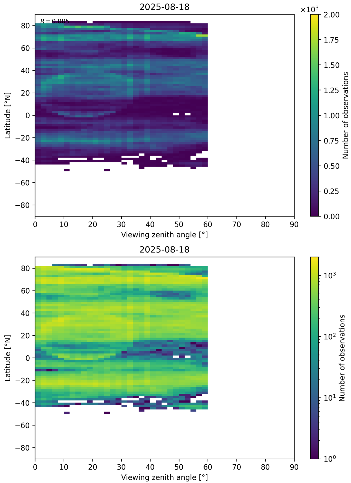
Figure 109: Scatter density plot of “Viewing zenith angle” against “Latitude” for 2025-08-17 to 2025-08-19.
