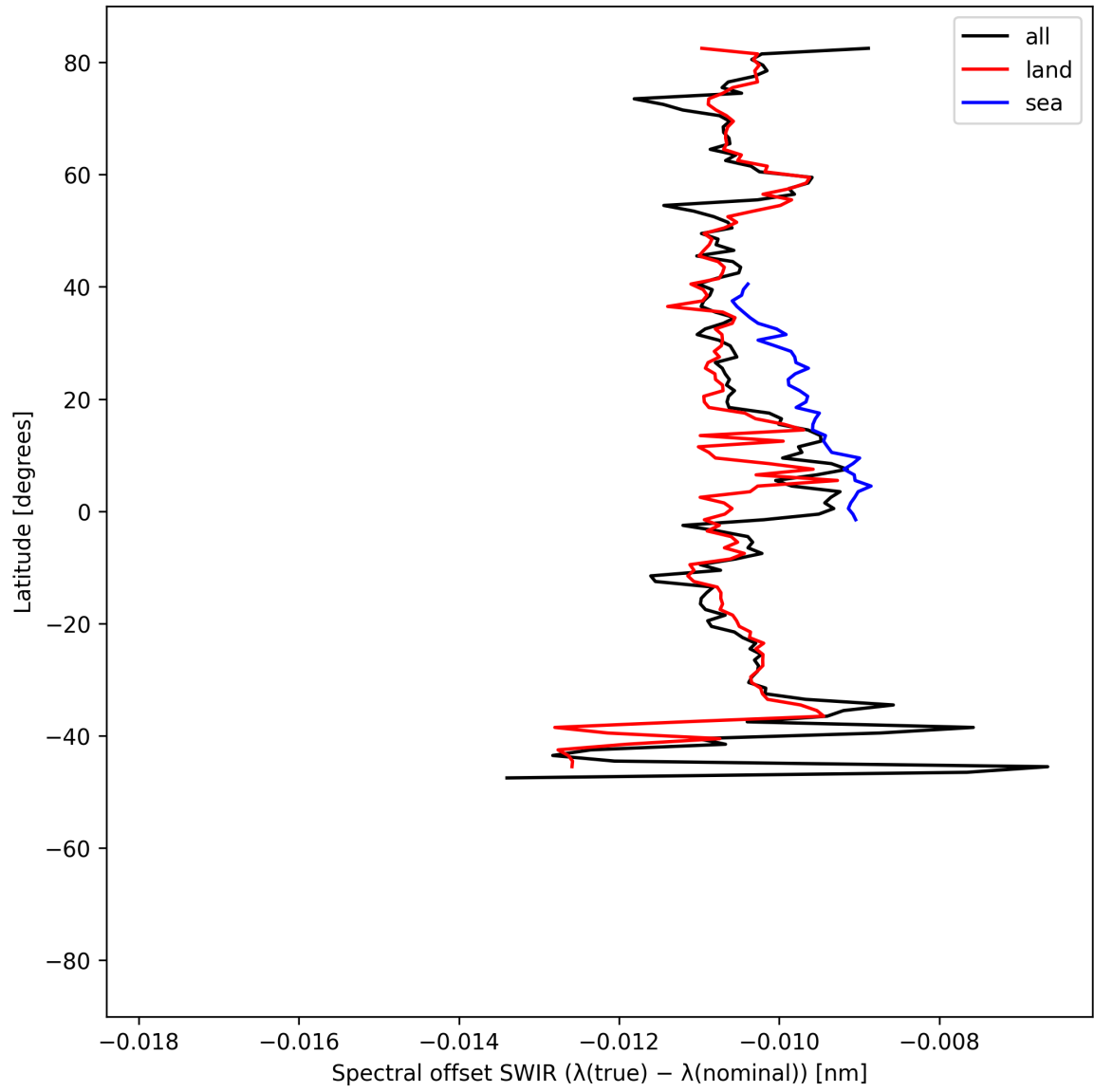
Figure 16: Zonal average of “Spectral offset SWIR ( \lambda_{\text{true}} - \lambda_{\text{nominal}} )” for 2025-08-17 to 2025-08-19.
