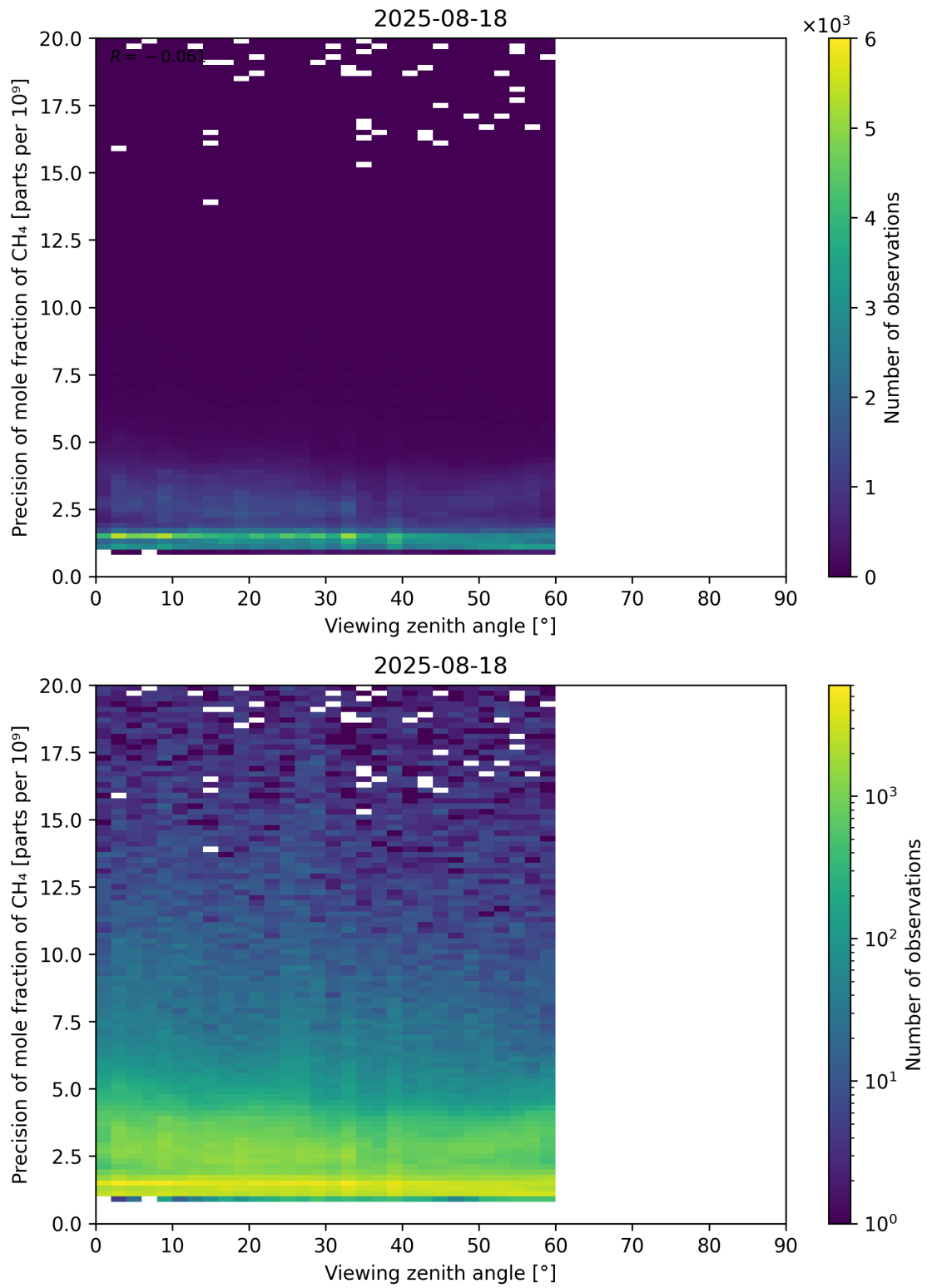
Figure 112: Scatter density plot of “Viewing zenith angle” against “Precision of mole fraction of CH 4 ” for 2025-08-17 to 2025-08-19.
