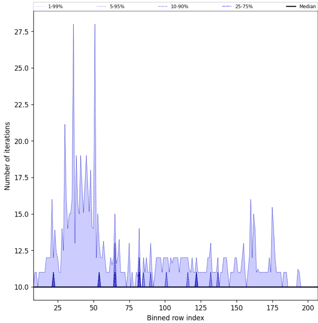
Figure 42: Along track statistics of “Number of iterations” for 2025-08-17 to 2025-08-19
