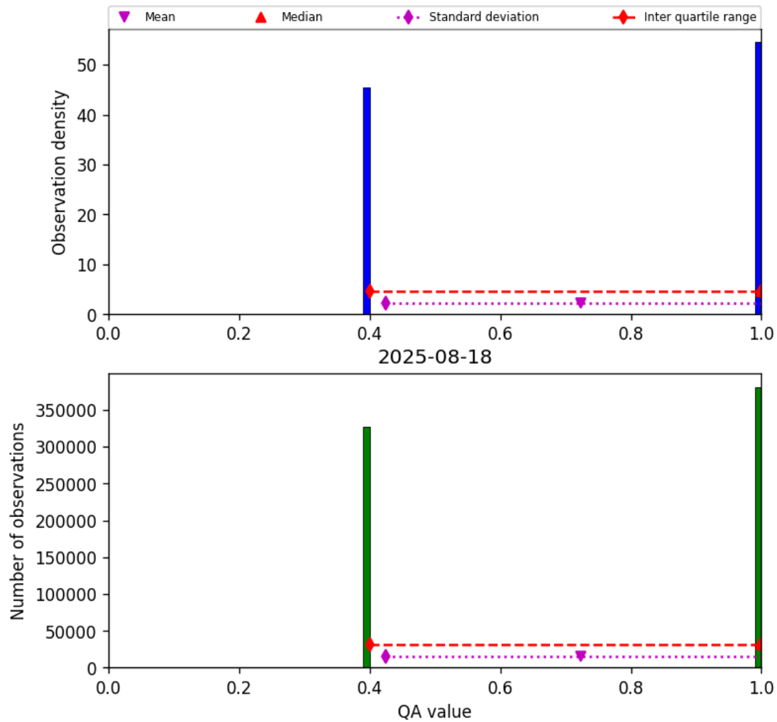
Figure 22: Histogram of “QA value” for 2025-08-17 to 2025-08-19
