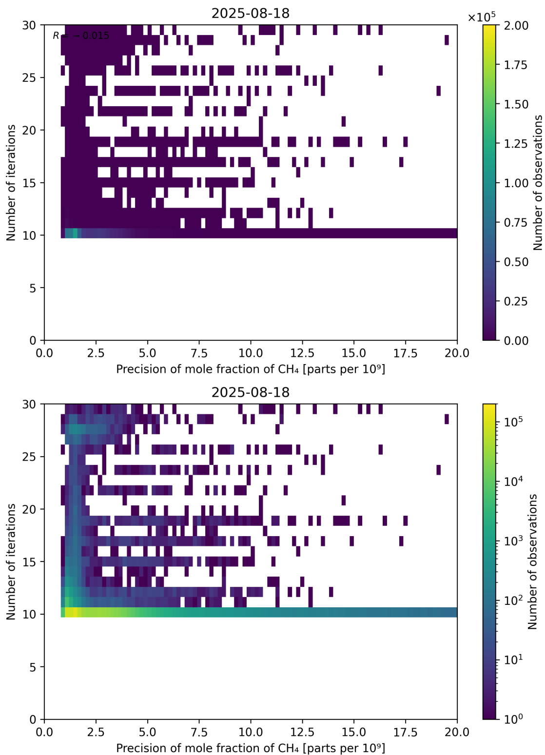
Figure 83: Scatter density plot of “Precision of mole fraction of CH 4 ” against “Number of iterations” for 2025-08-17 to 2025-08-19.
