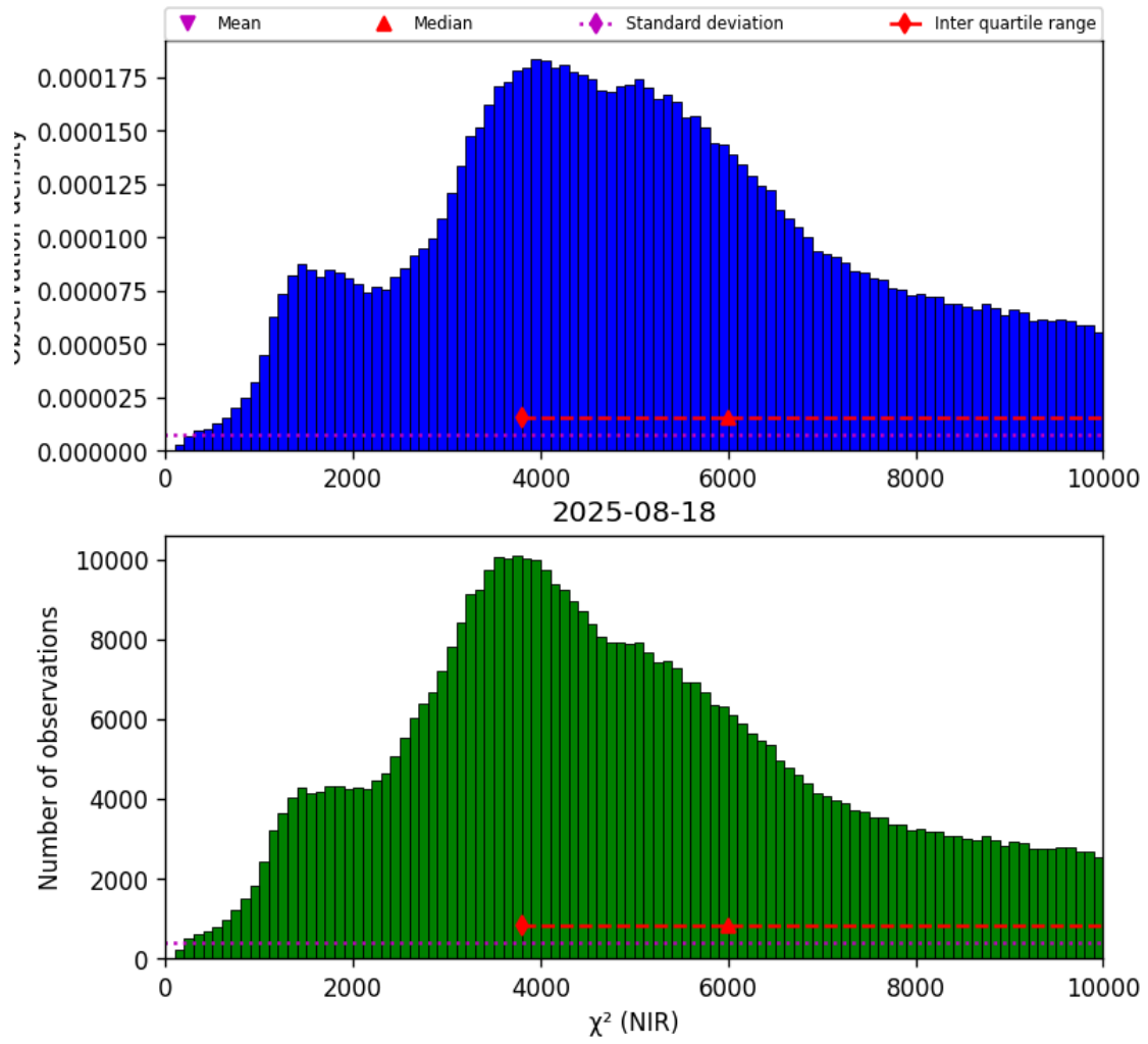
Figure 29: Histogram of “ \chi^2 (NIR)” for 2025-08-17 to 2025-08-19
