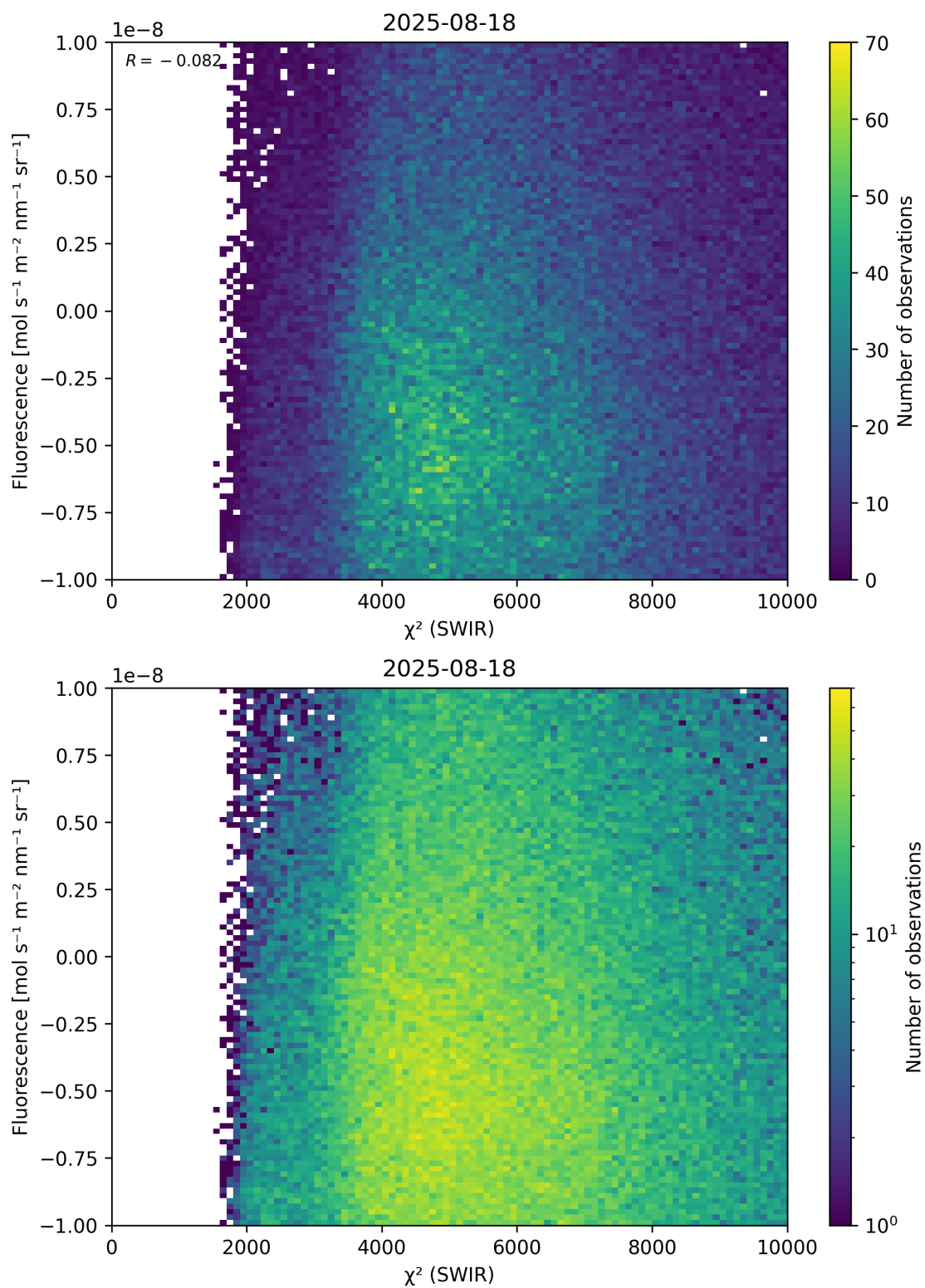
Figure 49: Scatter density plot of “ \chi^2 (SWIR)” against “Fluorescence” for 2025-08-17 to 2025-08-19.
