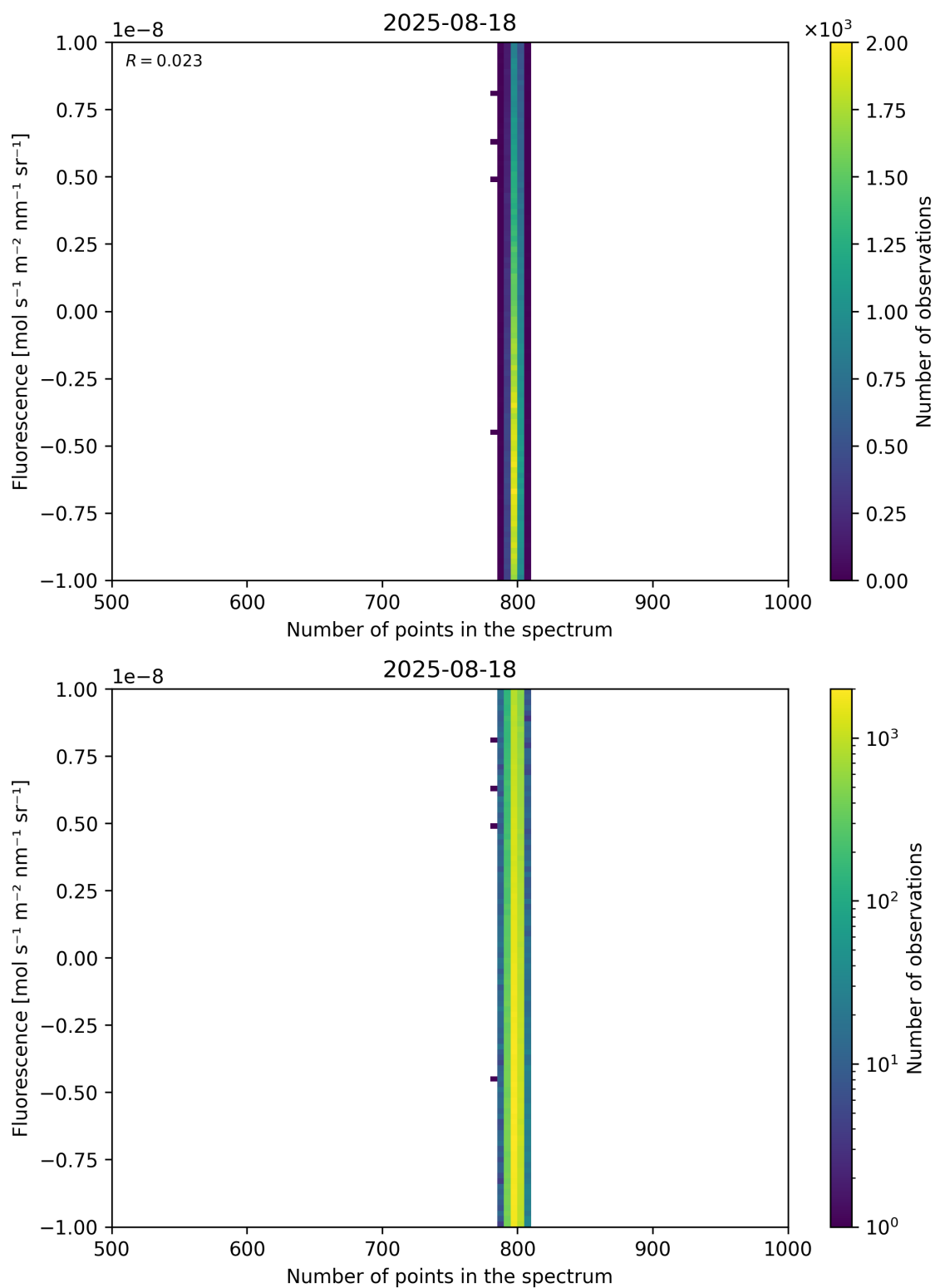
Figure 91: Scatter density plot of “Number of points in the spectrum” against “Fluorescence” for 2025-08-17 to 2025-08-19.
