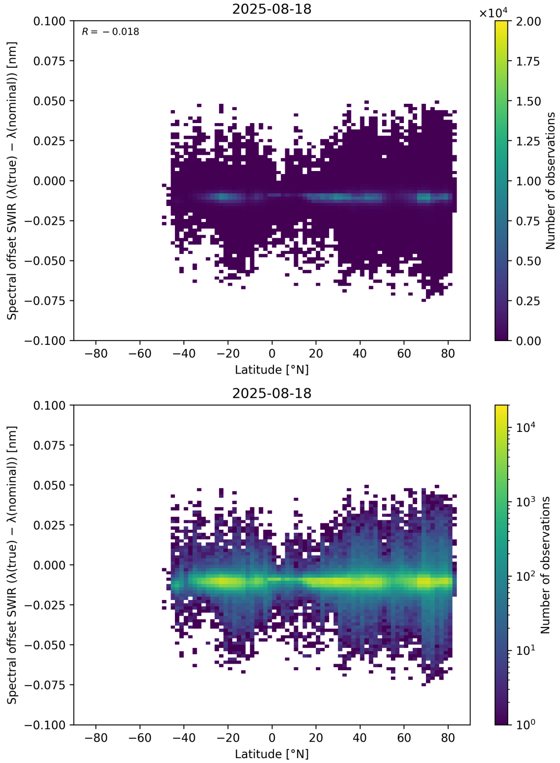
Figure 62: Scatter density plot of “Latitude” against “Spectral offset SWIR ( \lambda_{\text{true}} - \lambda_{\text{nominal}} )” for 2025-08-17 to 2025-08-19.
