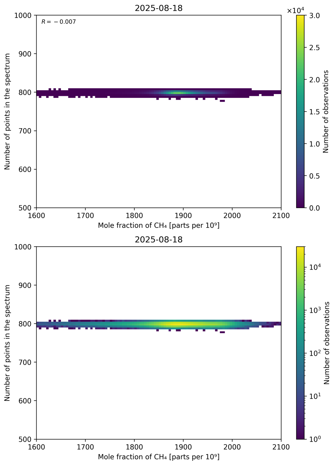
Figure 77: Scatter density plot of “Mole fraction of CH 4 ” against “Number of points in the spectrum” for 2025-08-17 to 2025-08-19.
