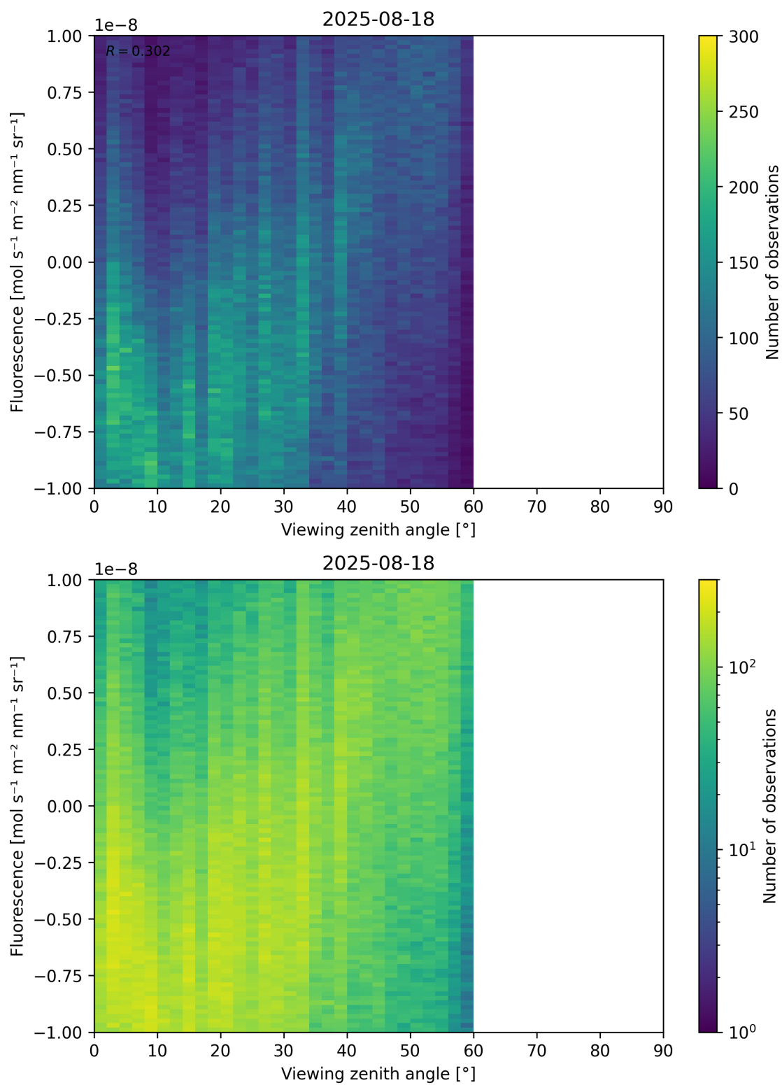
Figure 108: Scatter density plot of “Viewing zenith angle” against “Fluorescence” for 2025-08-17 to 2025-08-19.
