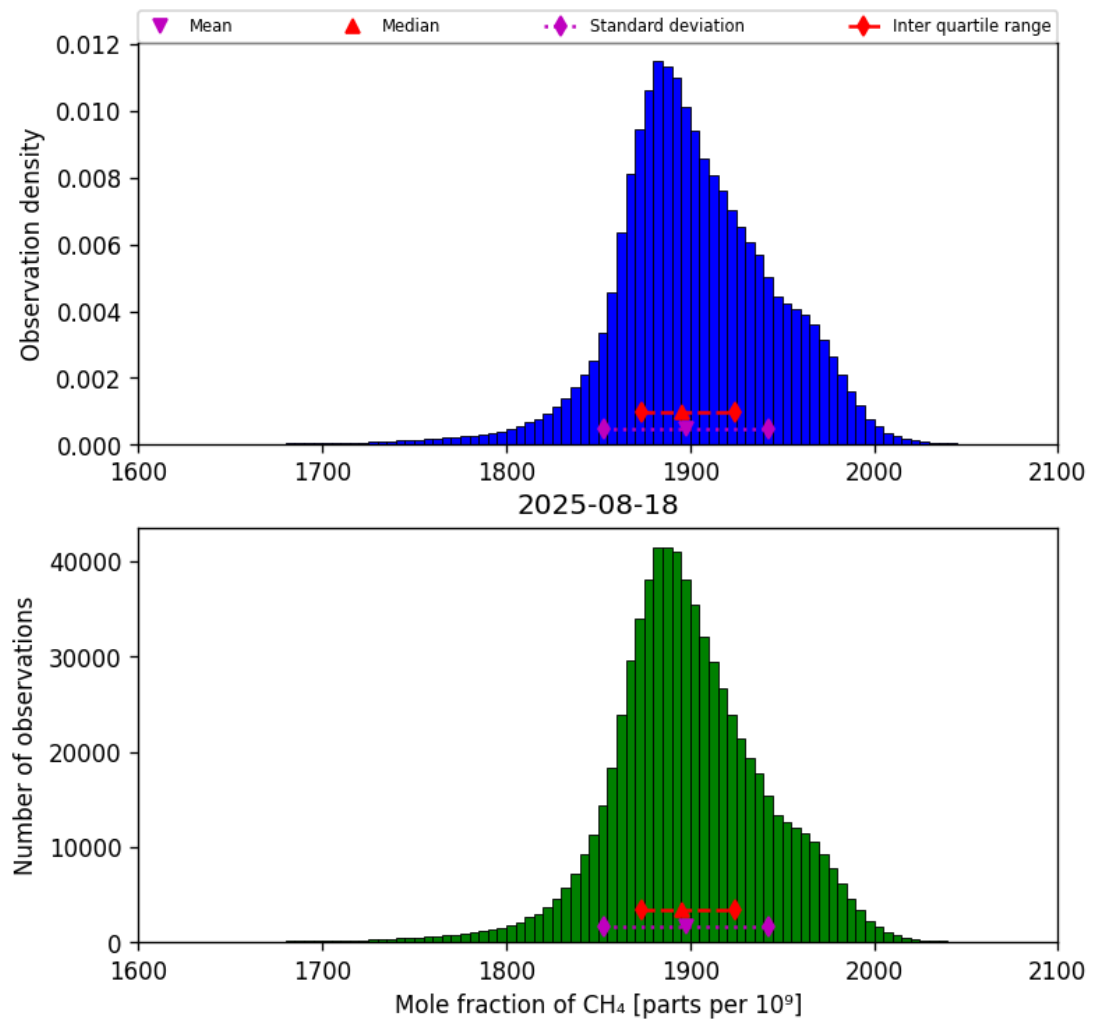
Figure 23: Histogram of “Mole fraction of CH 4 ” for 2025-08-17 to 2025-08-19
