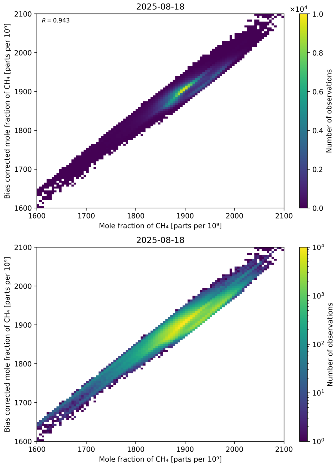
Figure 74: Scatter density plot of “Mole fraction of CH 4 ” against “Bias corrected mole fraction of CH 4 ” for 2025-08-17 to 2025-08-19.
