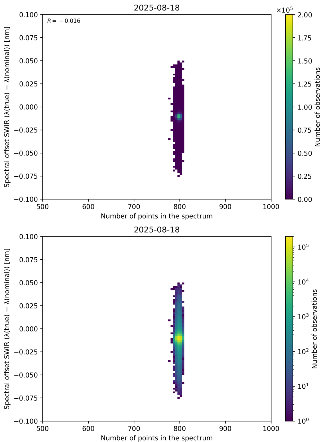
Figure 93: Scatter density plot of “Number of points in the spectrum” against “Spectral offset SWIR ( \lambda_{\text{true}} - \lambda_{\text{nominal}} )” for 2025-08-17 to 2025-08-19.
