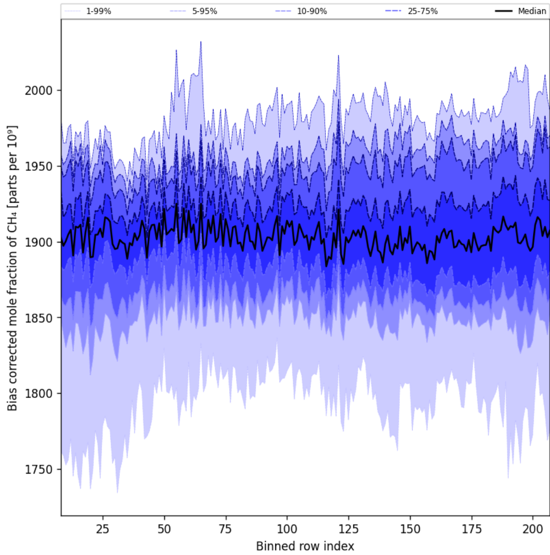
Figure 36: Along track statistics of “Bias corrected mole fraction of \text{CH}_4 ” for 2025-08-17 to 2025-08-19
