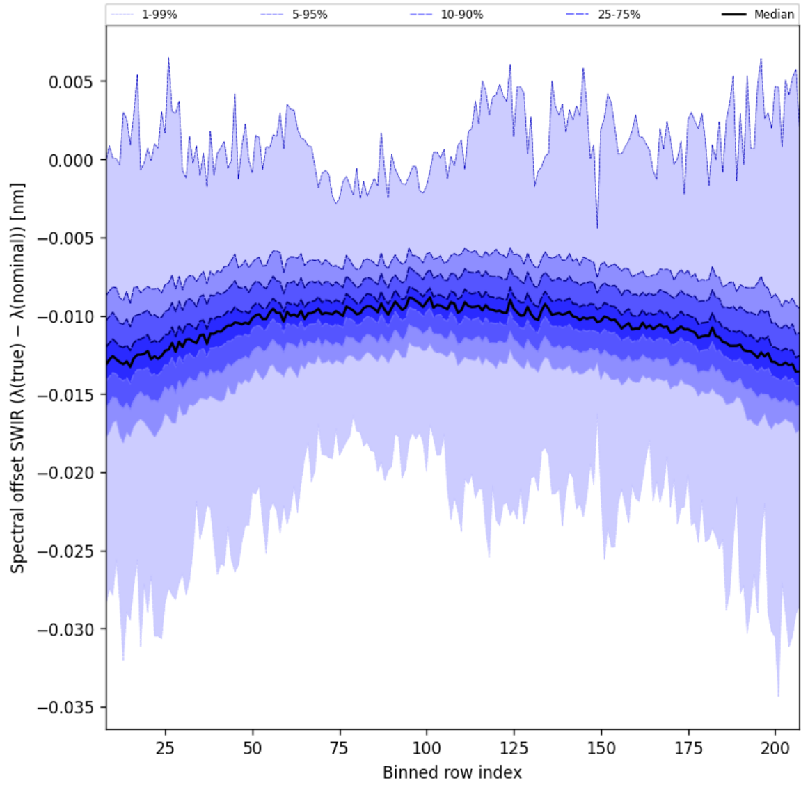
Figure 38: Along track statistics of “Spectral offset SWIR ( \lambda_{\text{true}} - \lambda_{\text{nominal}} )” for 2025-08-17 to 2025-08-19
