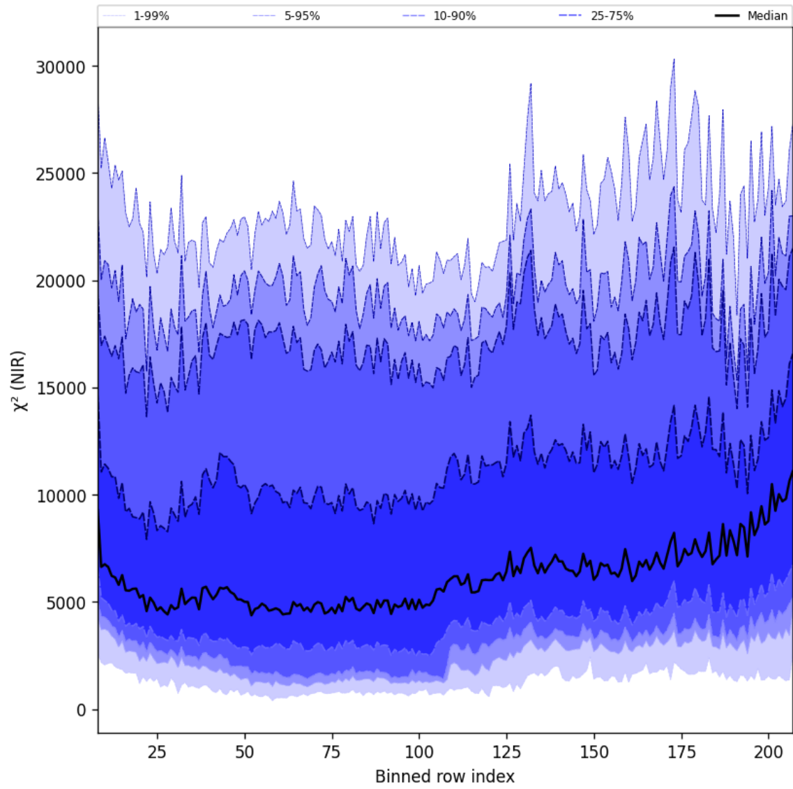
Figure 40: Along track statistics of “ \chi^2 (NIR)” for 2025-08-17 to 2025-08-19
