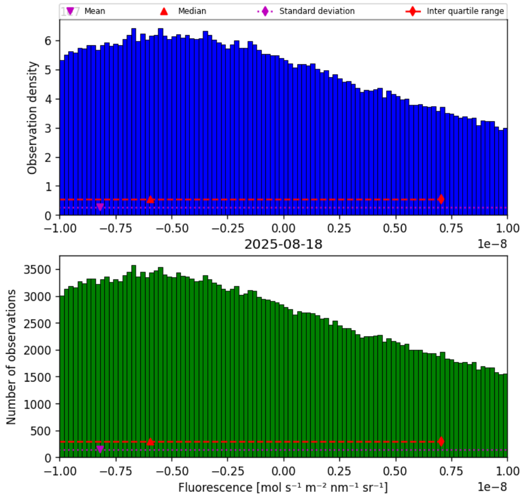
Figure 32: Histogram of “Fluorescence” for 2025-08-17 to 2025-08-19
