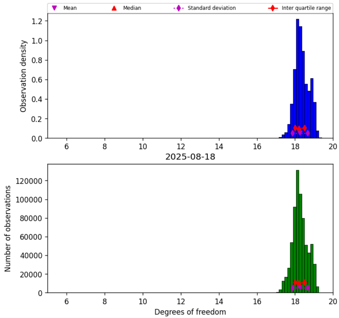
Figure 30: Histogram of “Degrees of freedom” for 2025-08-17 to 2025-08-19
