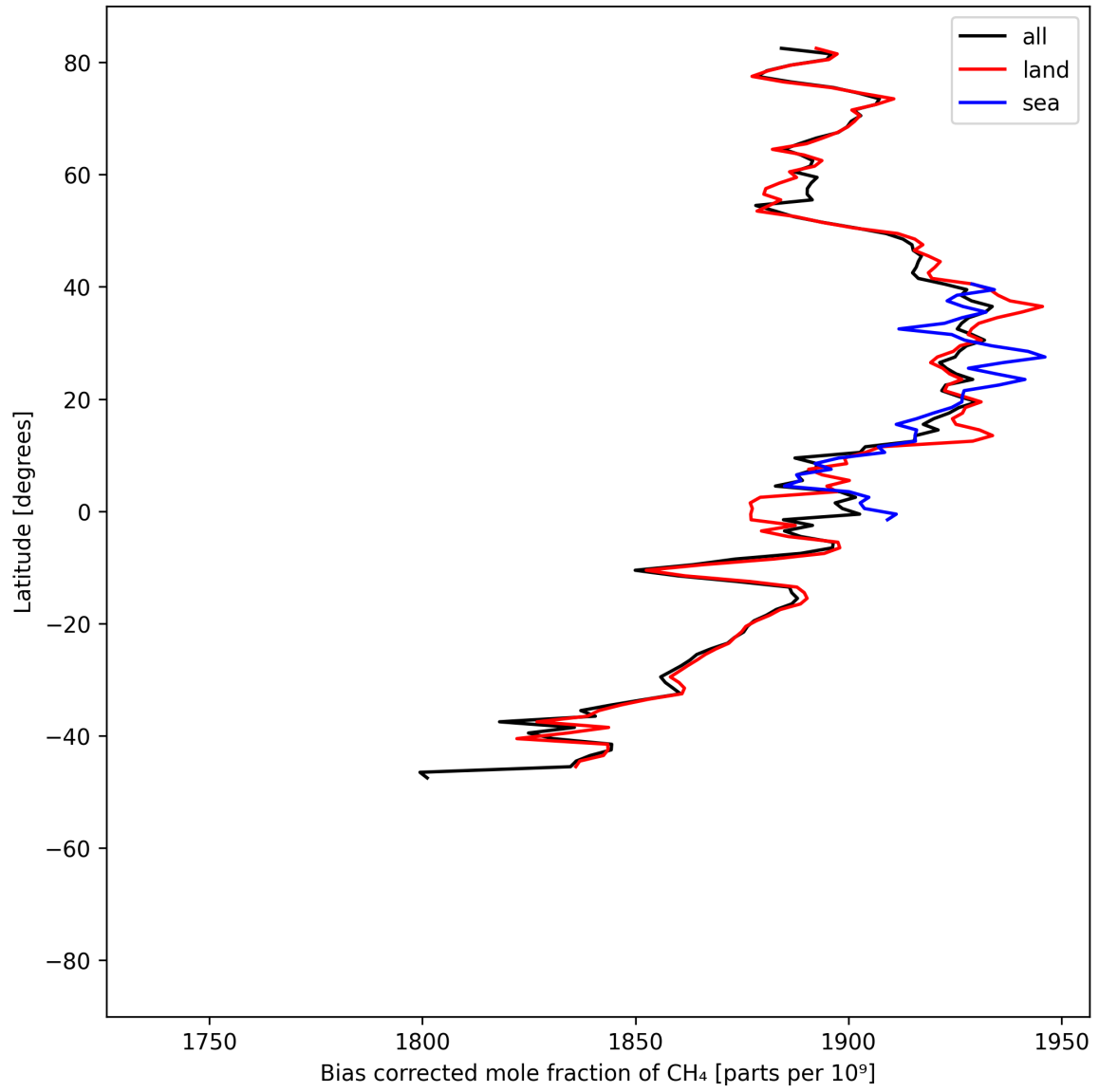
Figure 14: Zonal average of “Bias corrected mole fraction of CH 4 ” for 2025-08-17 to 2025-08-19.
