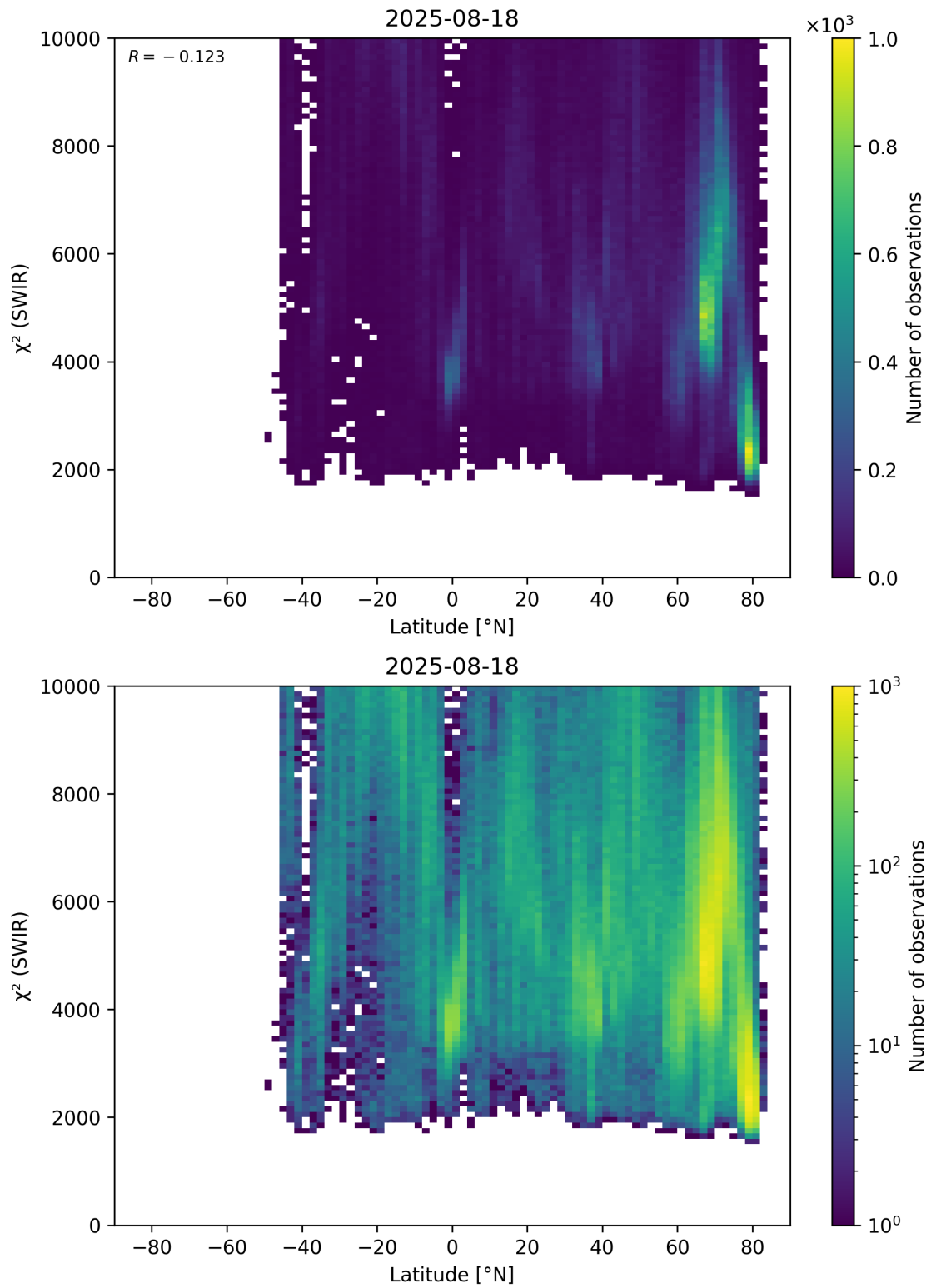
Figure 54: Scatter density plot of “Latitude” against “ \chi^2 (SWIR)” for 2025-08-17 to 2025-08-19.
