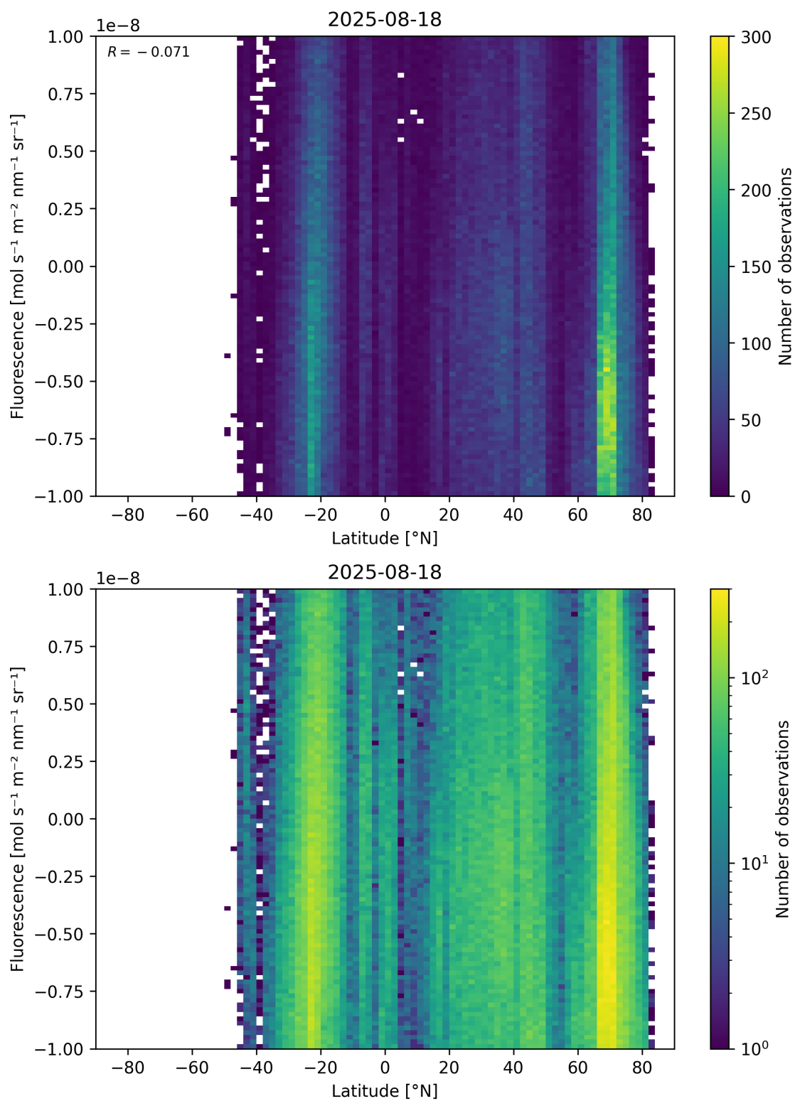
Figure 56: Scatter density plot of “Latitude” against “Fluorescence” for 2025-08-17 to 2025-08-19.
