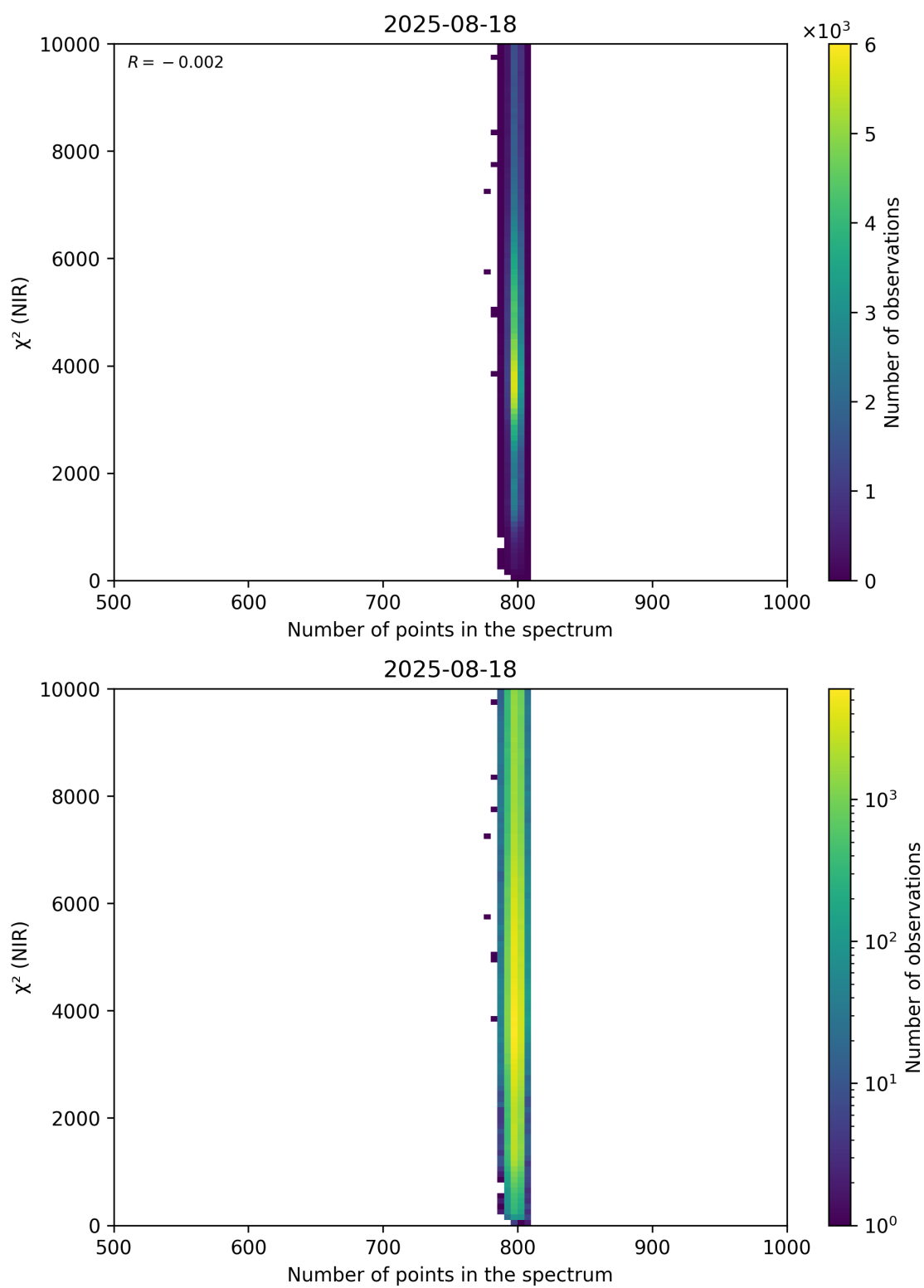
Figure 88: Scatter density plot of “Number of points in the spectrum” against “ \chi^2 (NIR)” for 2025-08-17 to 2025-08-19.
