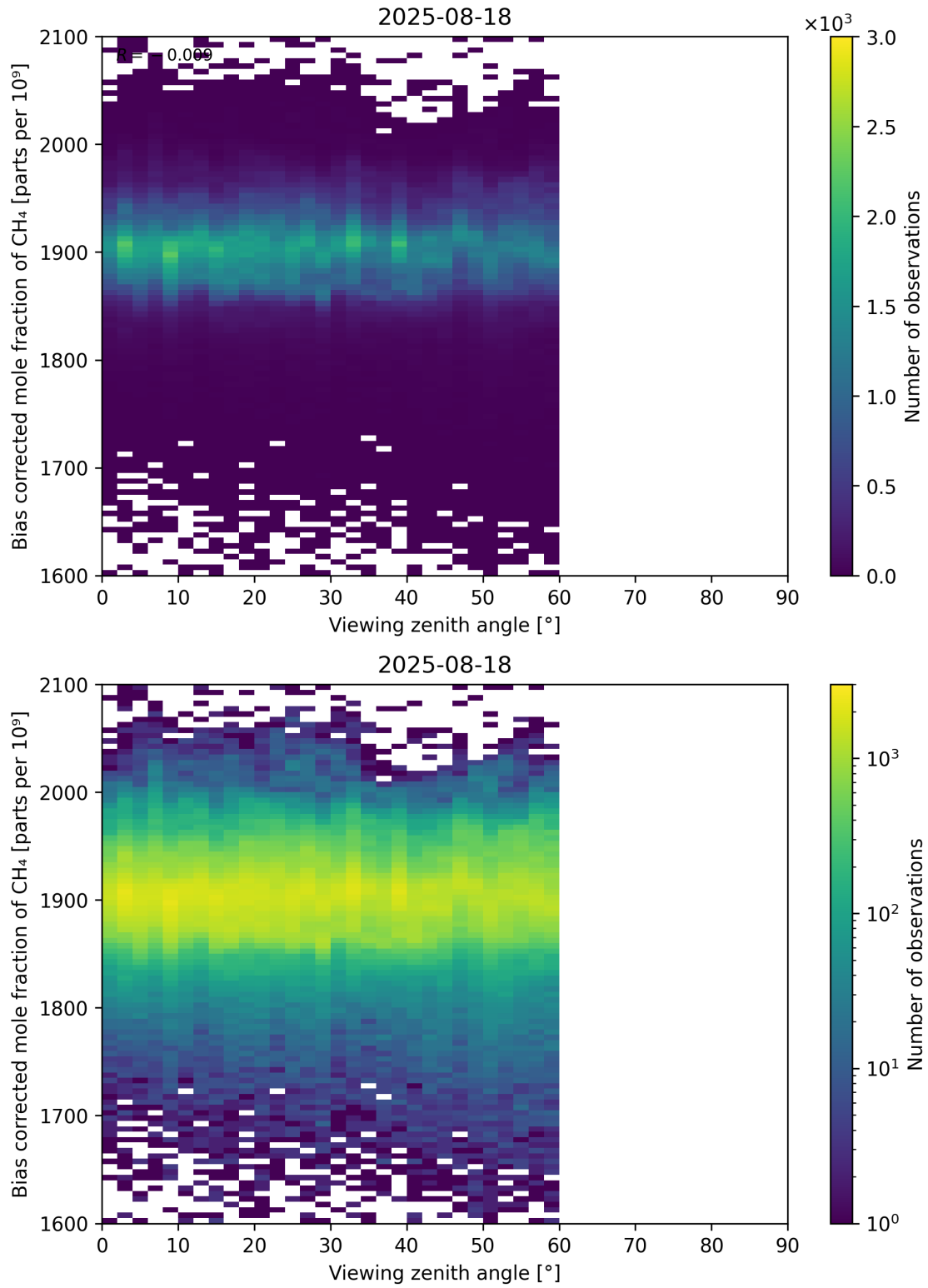
Figure 111: Scatter density plot of “Viewing zenith angle” against “Bias corrected mole fraction of CH 4 ” for 2025-08-17 to 2025-08-19.
