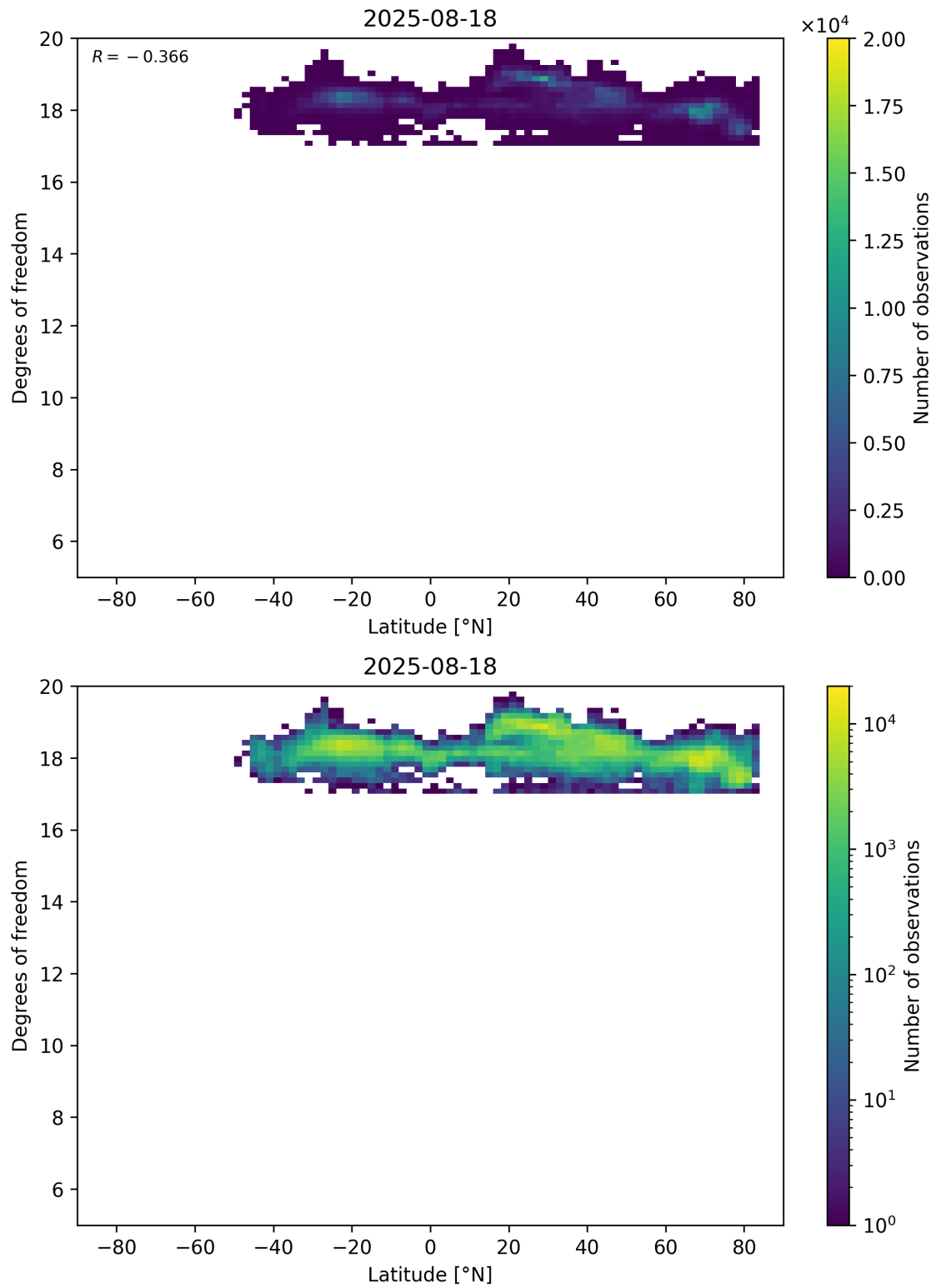
Figure 55: Scatter density plot of “Latitude” against “Degrees of freedom” for 2025-08-17 to 2025-08-19.
