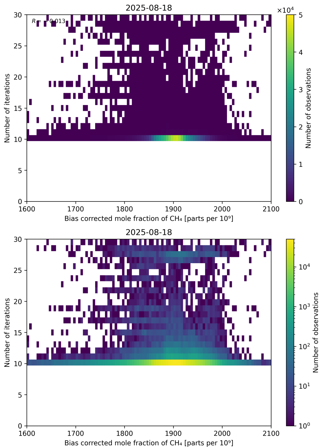
Figure 67: Scatter density plot of “Bias corrected mole fraction of CH 4 ” against “Number of iterations” for 2025-08-17 to 2025-08-19.
