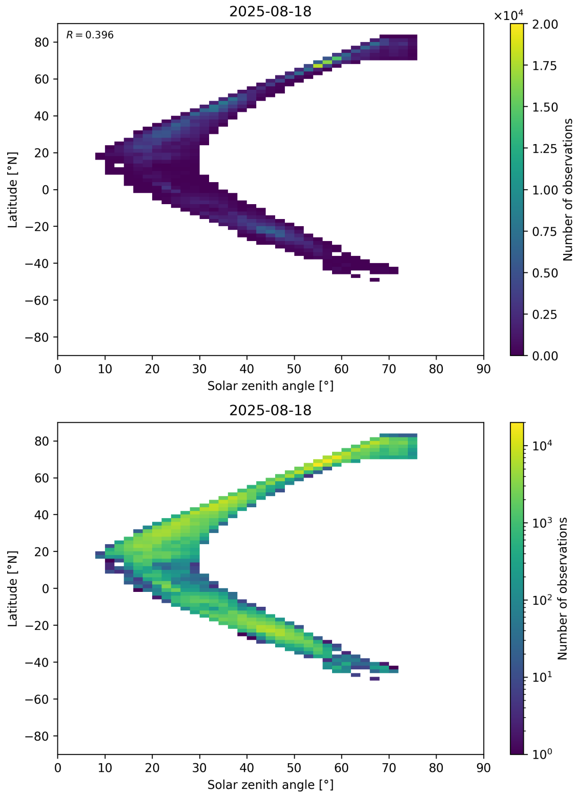
Figure 98: Scatter density plot of “Solar zenith angle” against “Latitude” for 2025-08-17 to 2025-08-19.
