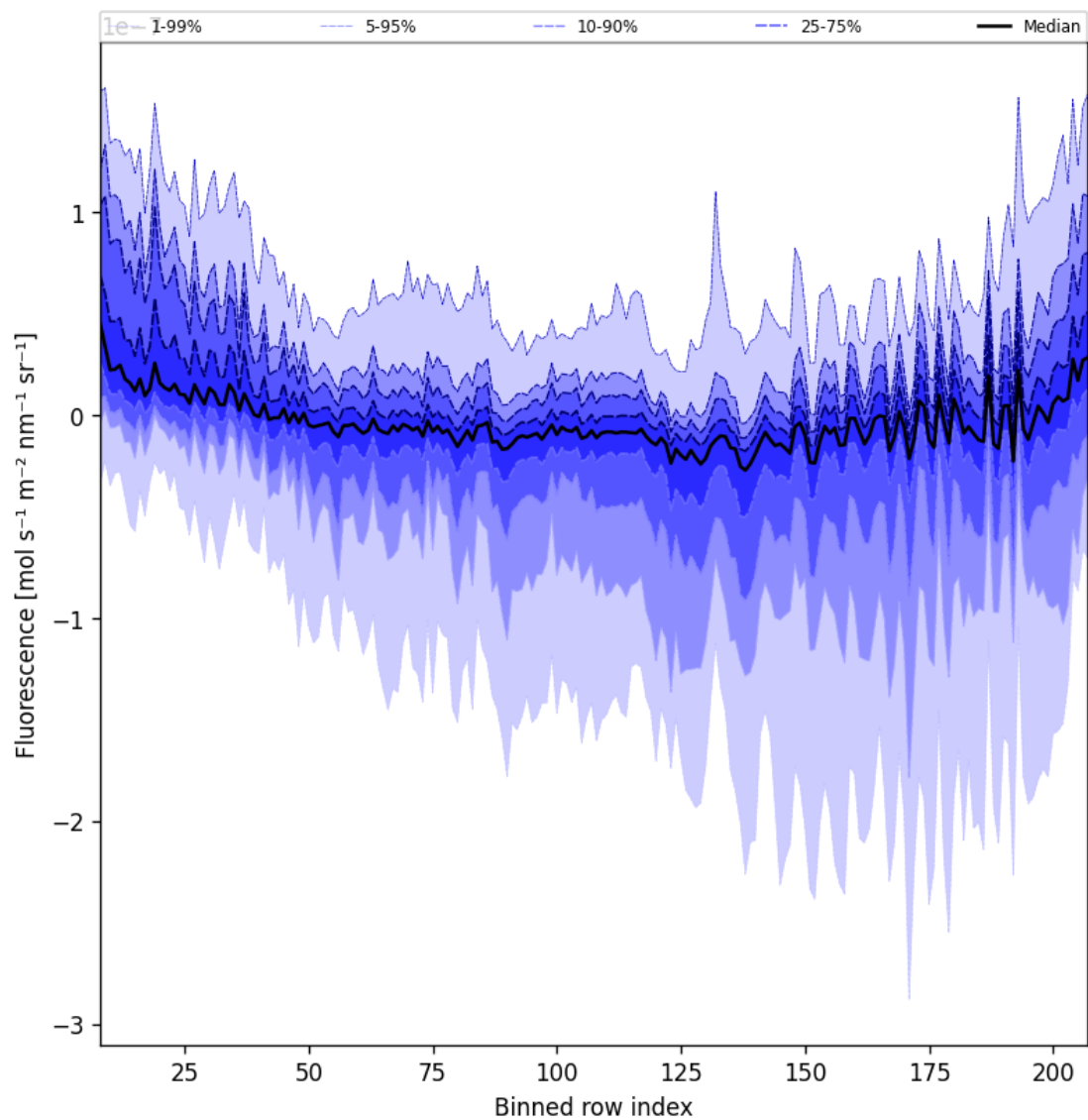
Figure 43: Along track statistics of “Fluorescence” for 2025-08-17 to 2025-08-19
