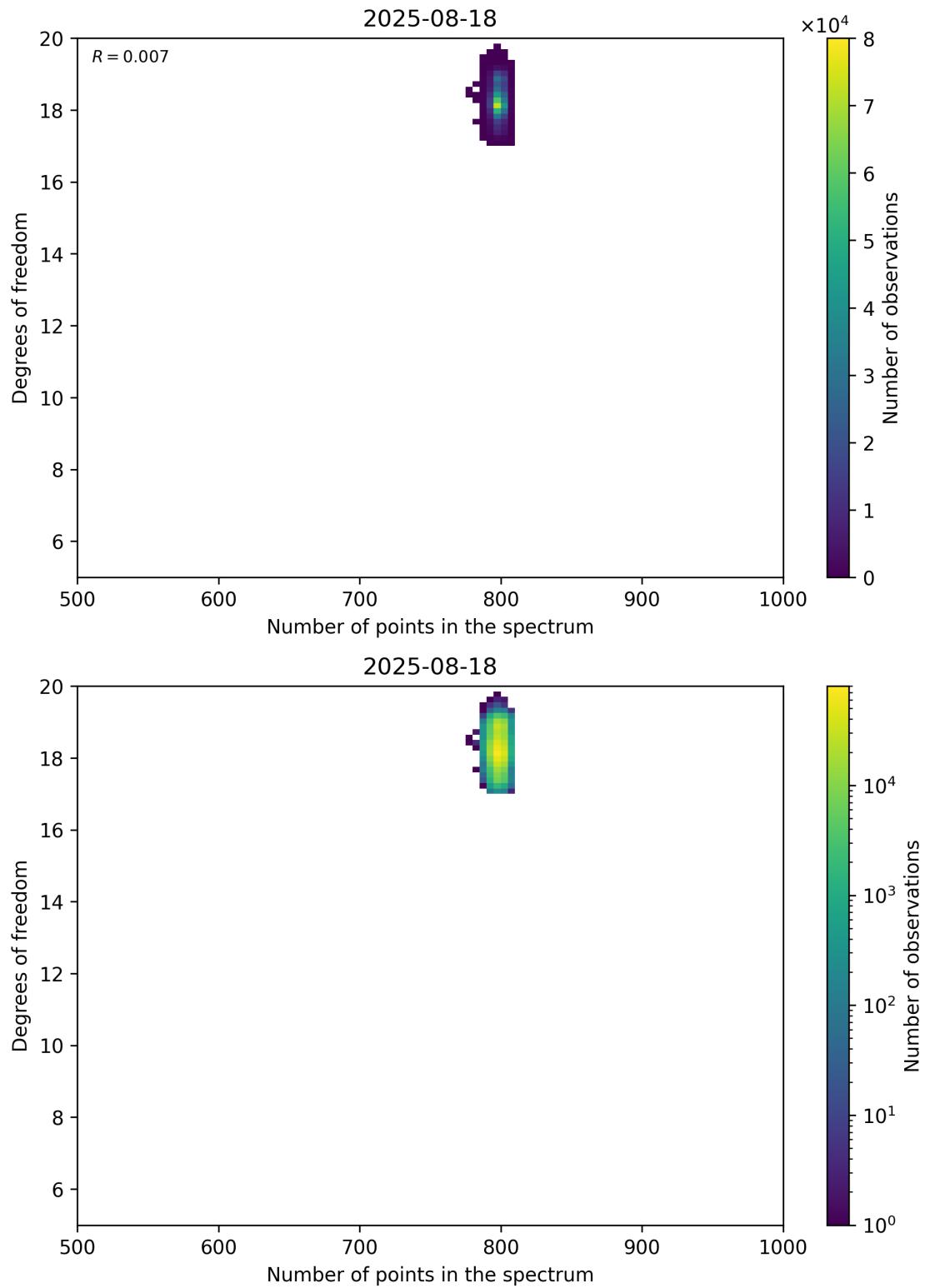
Figure 90: Scatter density plot of “Number of points in the spectrum” against “Degrees of freedom” for 2025-08-17 to 2025-08-19.
