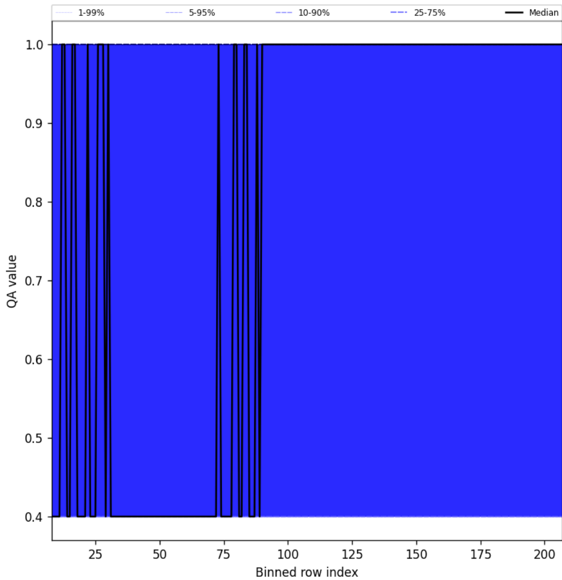
Figure 33: Along track statistics of “QA value” for 2025-08-17 to 2025-08-19
