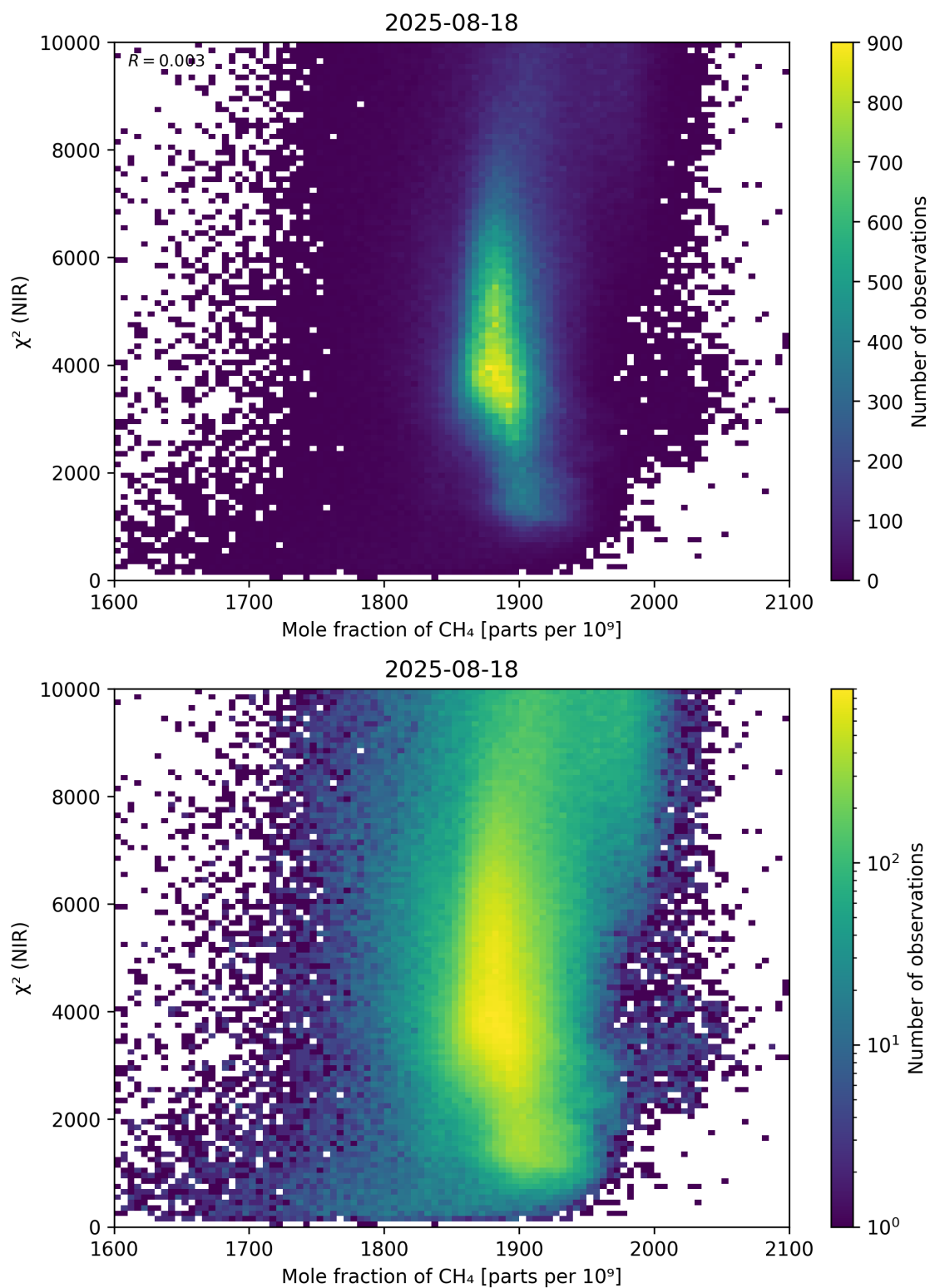
Figure 70: Scatter density plot of “Mole fraction of \text{CH}_4 ” against “ \chi^2 (NIR)” for 2025-08-17 to 2025-08-19.
