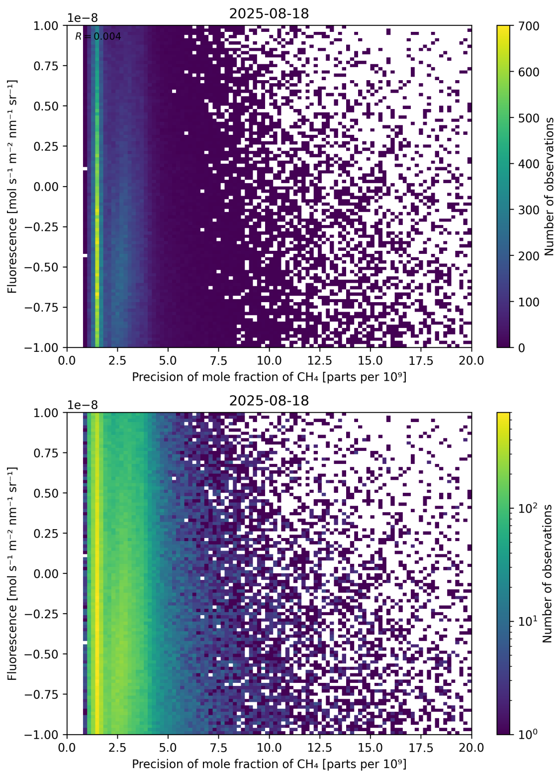
Figure 81: Scatter density plot of “Precision of mole fraction of \text{CH}_4 ” against “Fluorescence” for 2025-08-17 to 2025-08-19.
