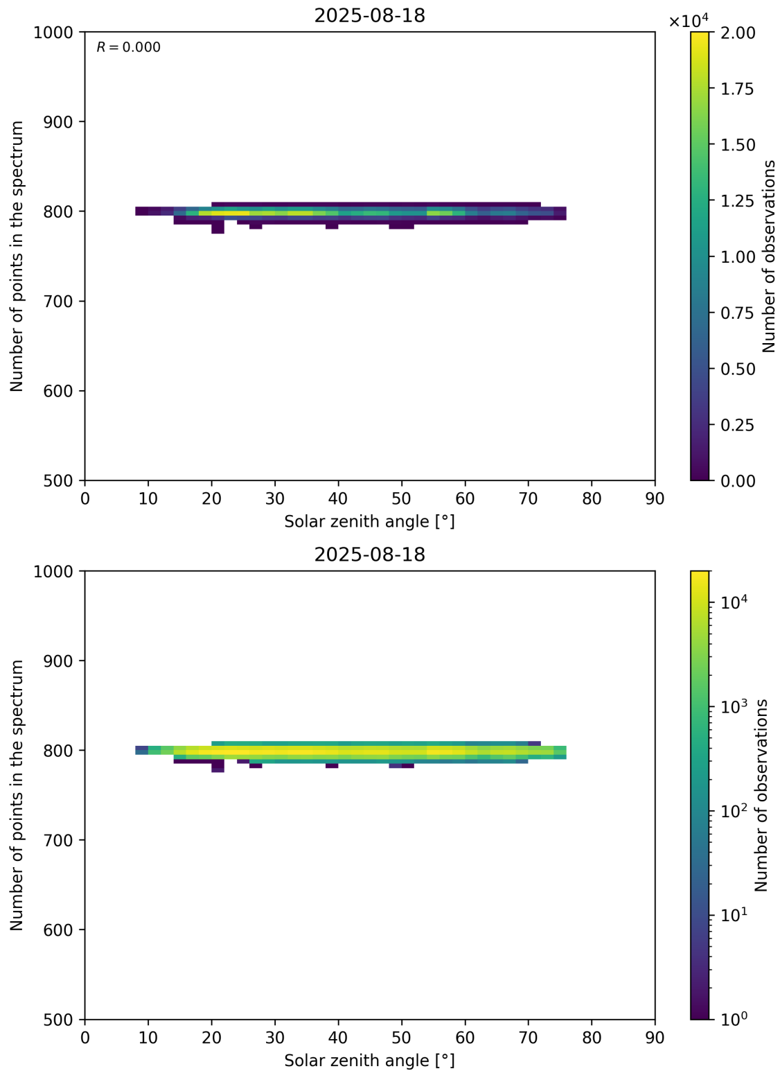
Figure 103: Scatter density plot of “Solar zenith angle” against “Number of points in the spectrum” for 2025-08-17 to 2025-08-19.
