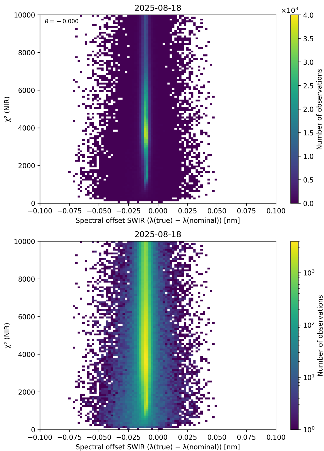
Figure 117: Scatter density plot of “Spectral offset SWIR ( \lambda_{\text{true}} - \lambda_{\text{nominal}} )” against “ \chi^2 (NIR)” for 2025-08-17 to 2025-08-19.
