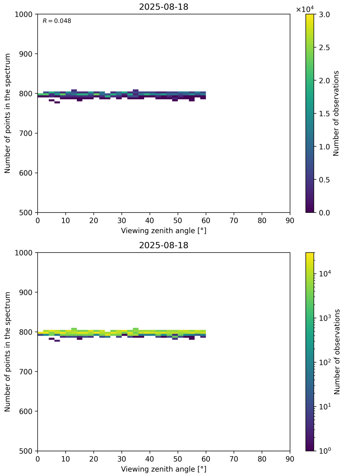
Figure 114: Scatter density plot of “Viewing zenith angle” against “Number of points in the spectrum” for 2025-08-17 to 2025-08-19.
