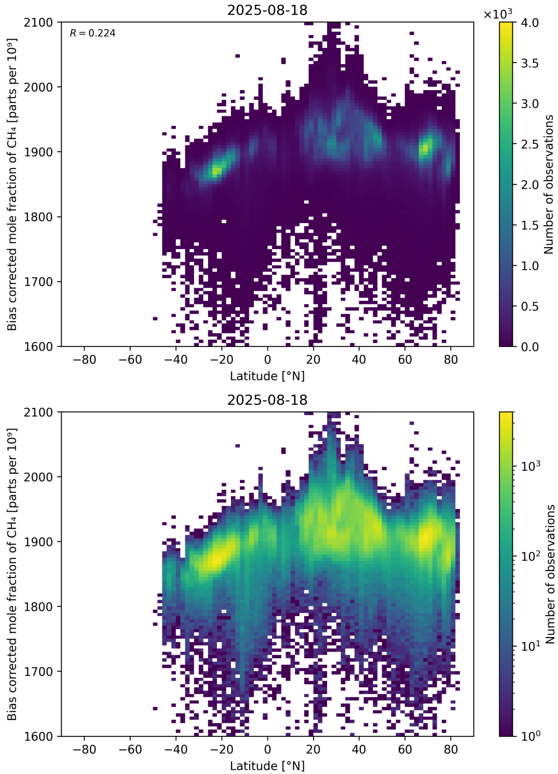
Figure 58: Scatter density plot of “Latitude” against “Bias corrected mole fraction of \text{CH}_4 ” for 2025-08-17 to 2025-08-19.
