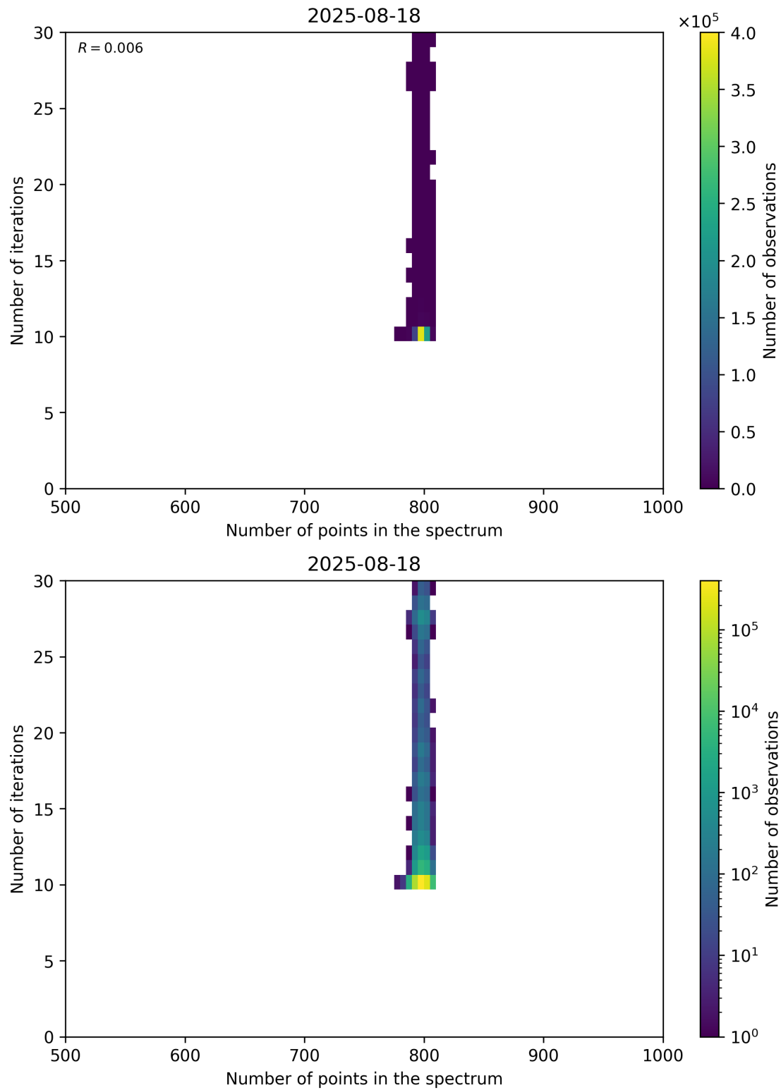
Figure 92: Scatter density plot of “Number of points in the spectrum” against “Number of iterations” for 2025-08-17 to 2025-08-19.
