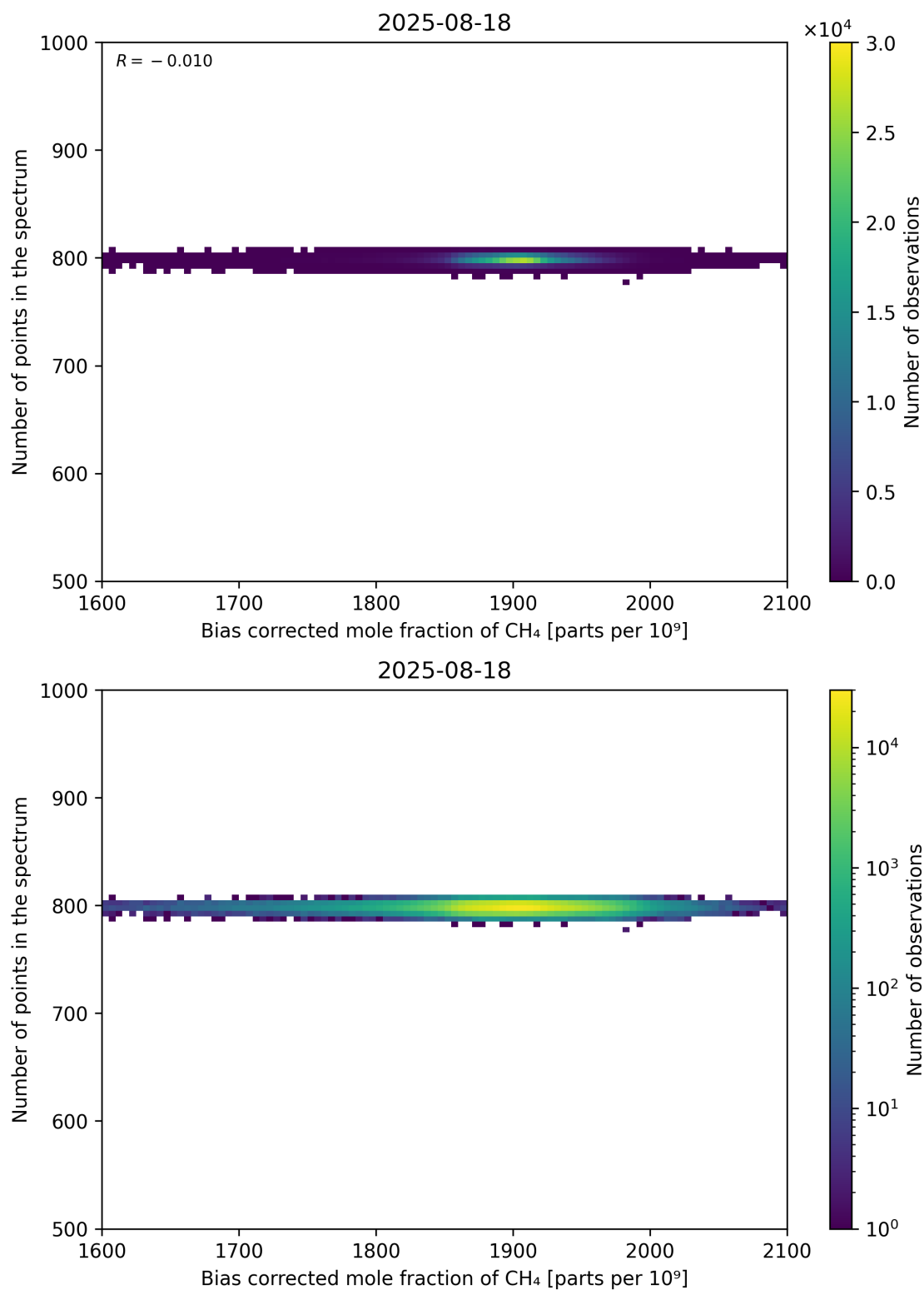
Figure 68: Scatter density plot of “Bias corrected mole fraction of CH 4 ” against “Number of points in the spectrum” for 2025-08-17 to 2025-08-19.
