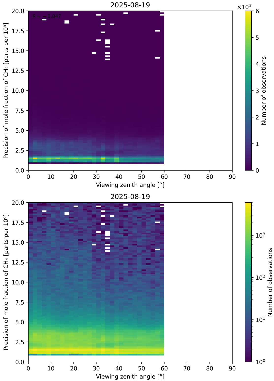
Figure 112: Scatter density plot of “Viewing zenith angle” against “Precision of mole fraction of CH 4 ” for 2025-08-19 to 2025-08-20.
