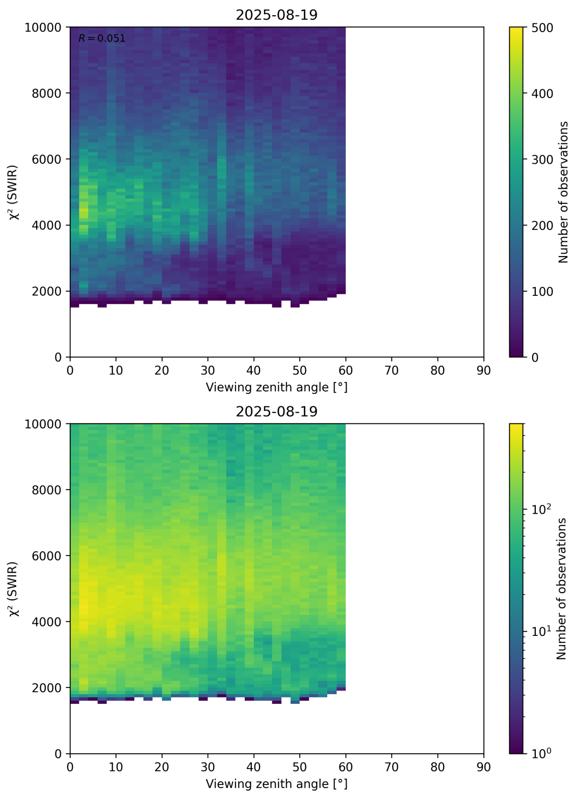
Figure 106: Scatter density plot of “Viewing zenith angle” against “ \chi^2 (SWIR)” for 2025-08-19 to 2025-08-20.
