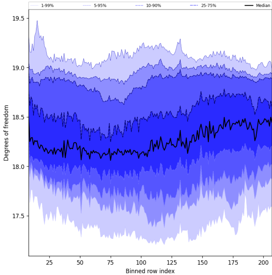
Figure 41: Along track statistics of “Degrees of freedom” for 2025-08-19 to 2025-08-20
