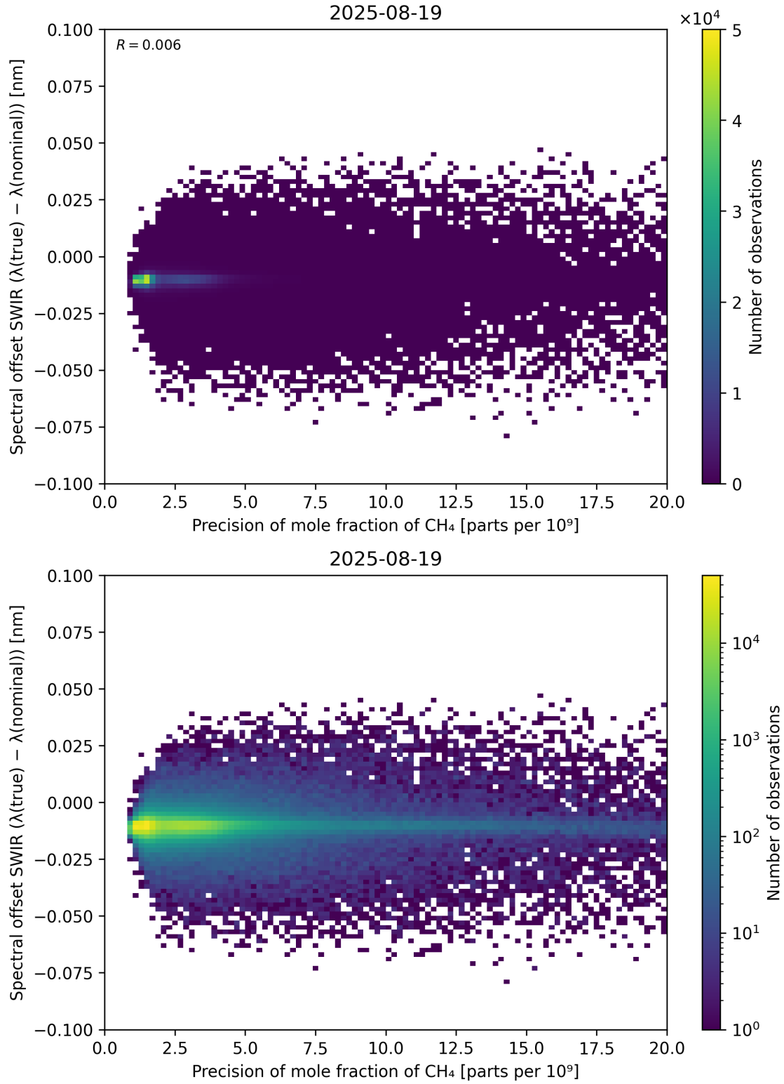
Figure 85: Scatter density plot of “Precision of mole fraction of CH 4 ” against “Spectral offset SWIR ( \lambda_{\text{true}} - \lambda_{\text{nominal}} )” for 2025-08-19 to 2025-08-20.
