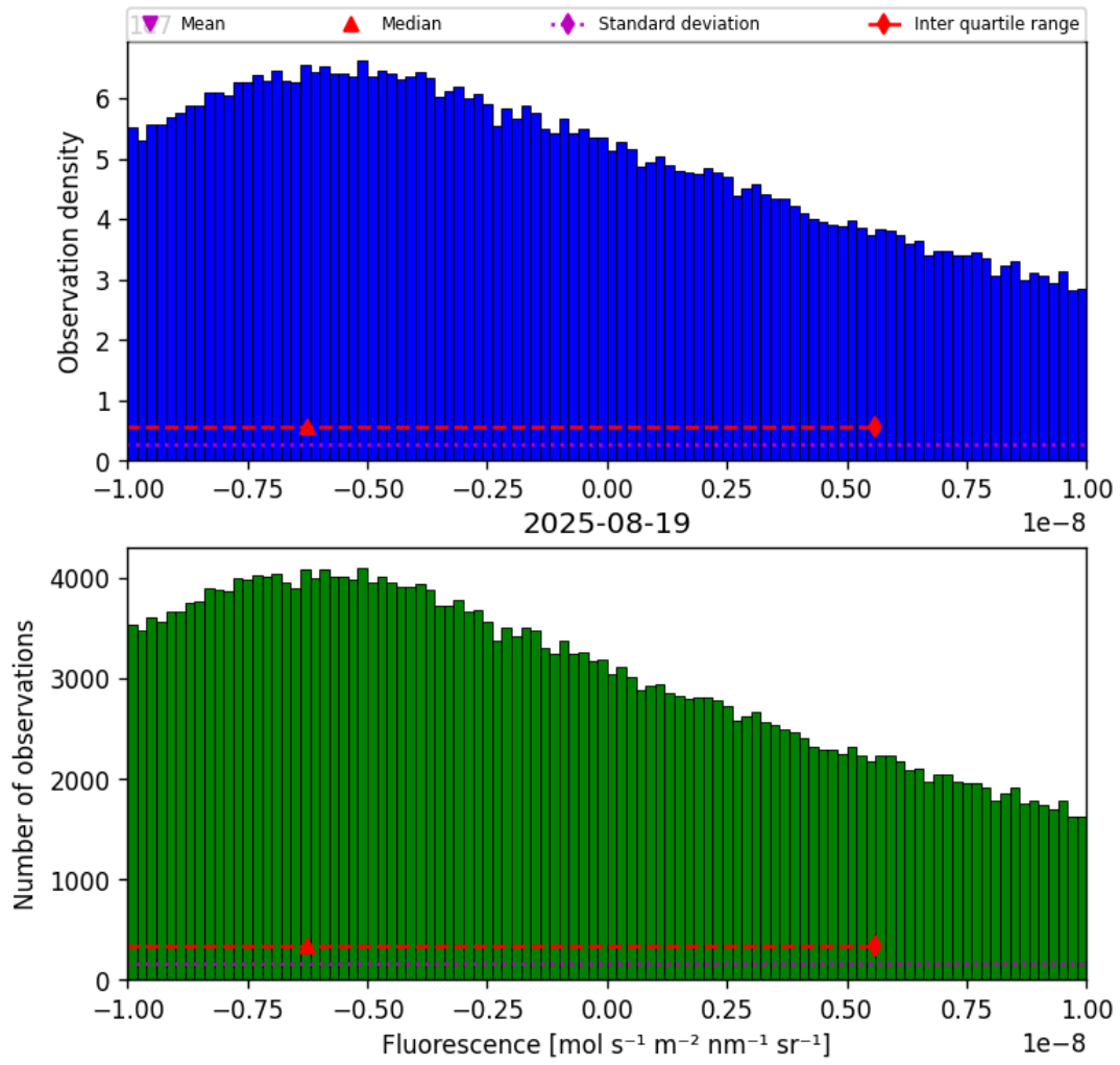
Figure 32: Histogram of “Fluorescence” for 2025-08-19 to 2025-08-20
