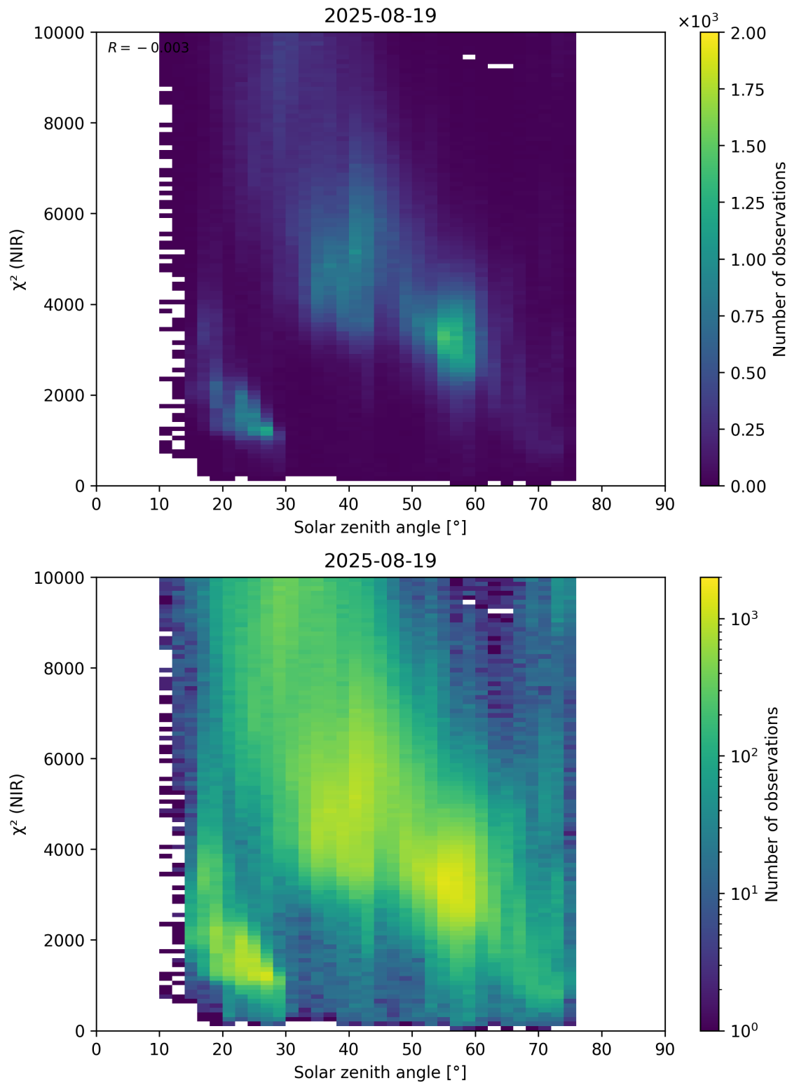
Figure 94: Scatter density plot of “Solar zenith angle” against “ \chi^2 (NIR)” for 2025-08-19 to 2025-08-20.
