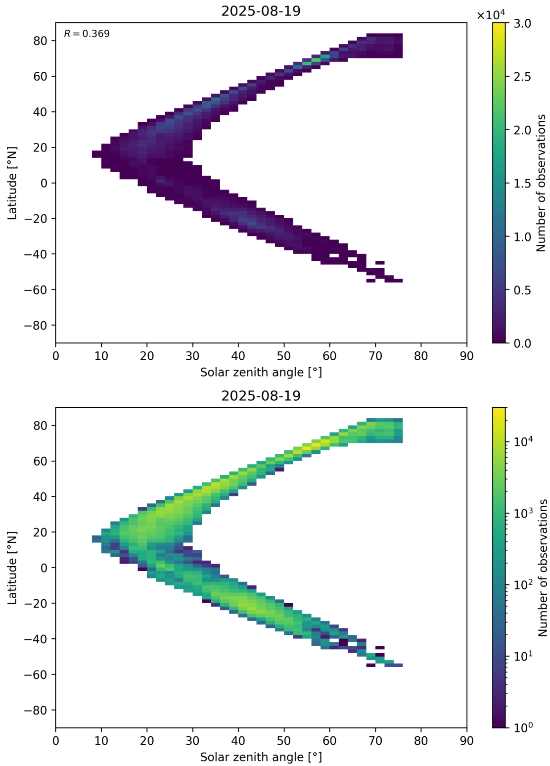
Figure 98: Scatter density plot of “Solar zenith angle” against “Latitude” for 2025-08-19 to 2025-08-20.
