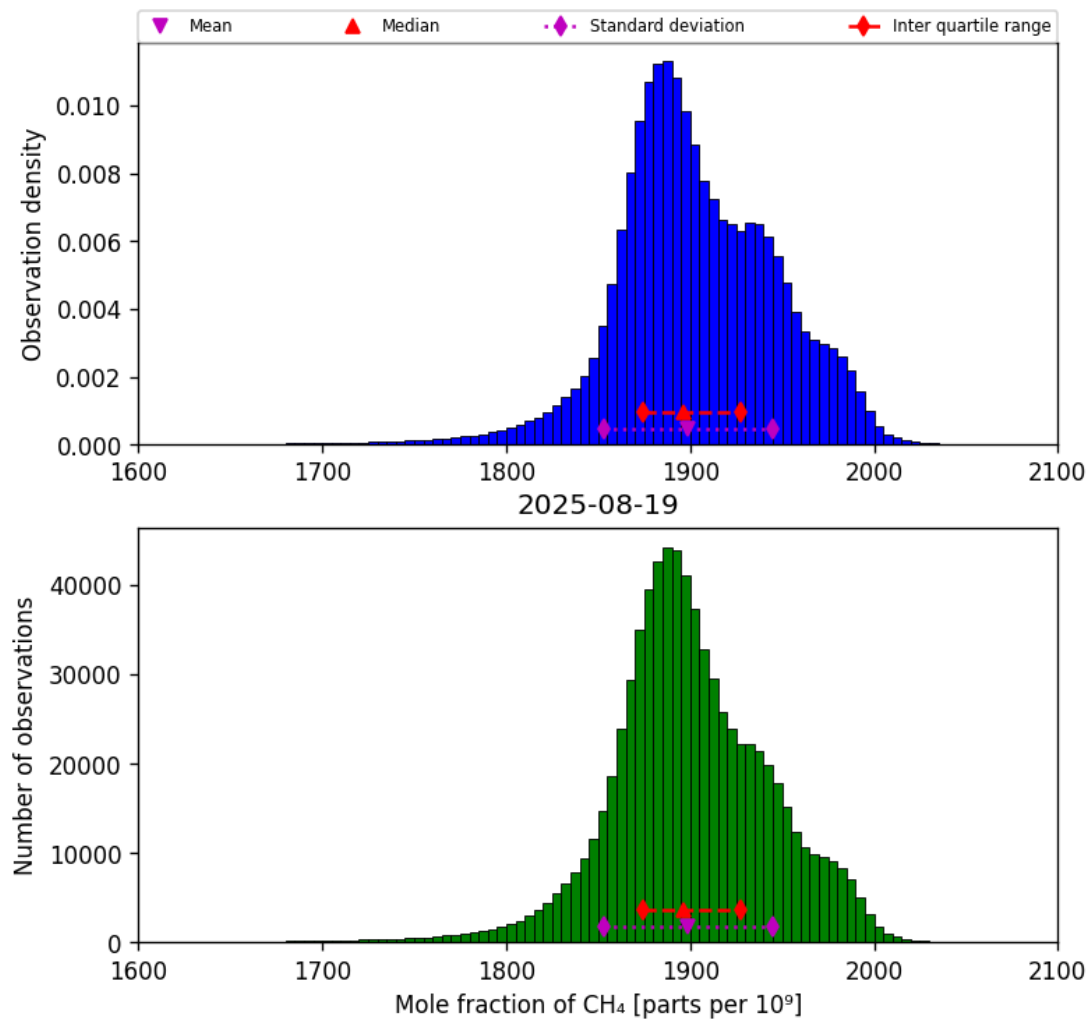
Figure 23: Histogram of “Mole fraction of CH 4 ” for 2025-08-19 to 2025-08-20
