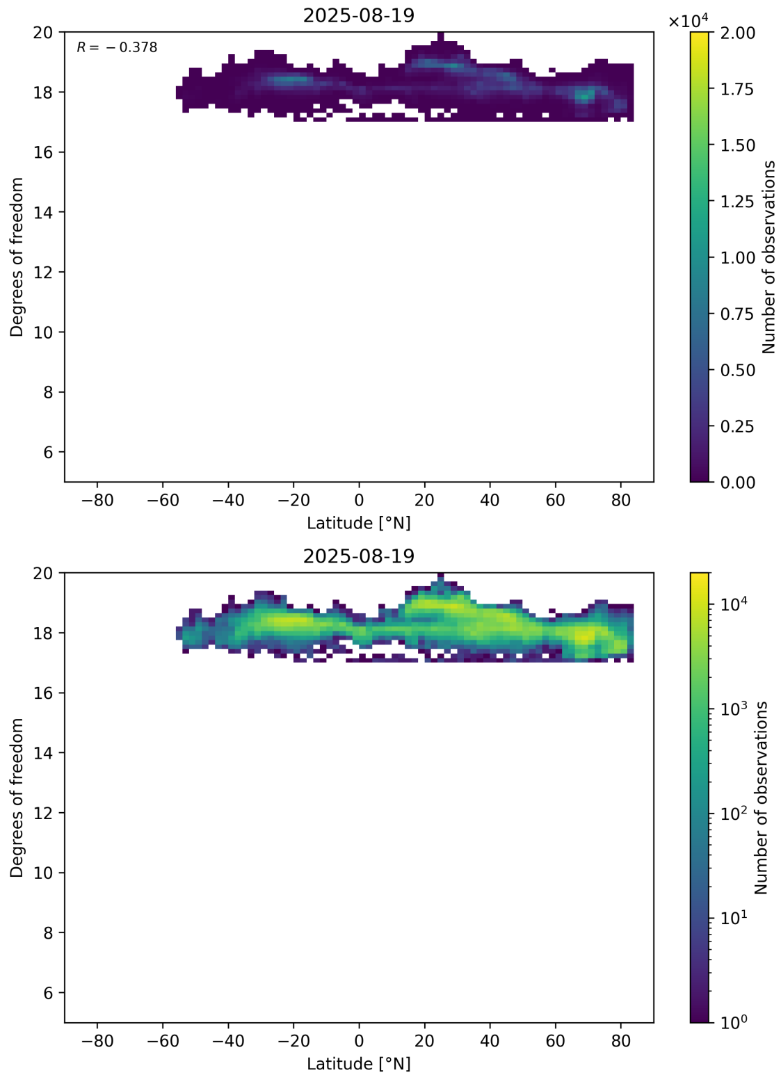
Figure 55: Scatter density plot of “Latitude” against “Degrees of freedom” for 2025-08-19 to 2025-08-20.
