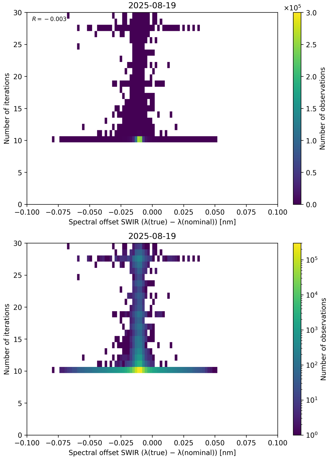
Figure 121: Scatter density plot of “Spectral offset SWIR ( \lambda_{\text{true}} - \lambda_{\text{nominal}} )” against “Number of iterations” for 2025-08-19 to 2025-08-20.
