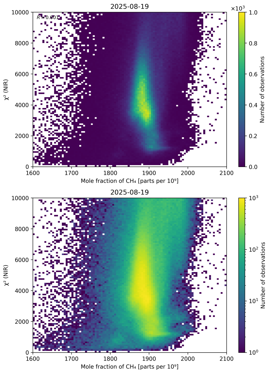
Figure 70: Scatter density plot of “Mole fraction of \text{CH}_4 ” against “ \chi^2 (NIR)” for 2025-08-19 to 2025-08-20.
