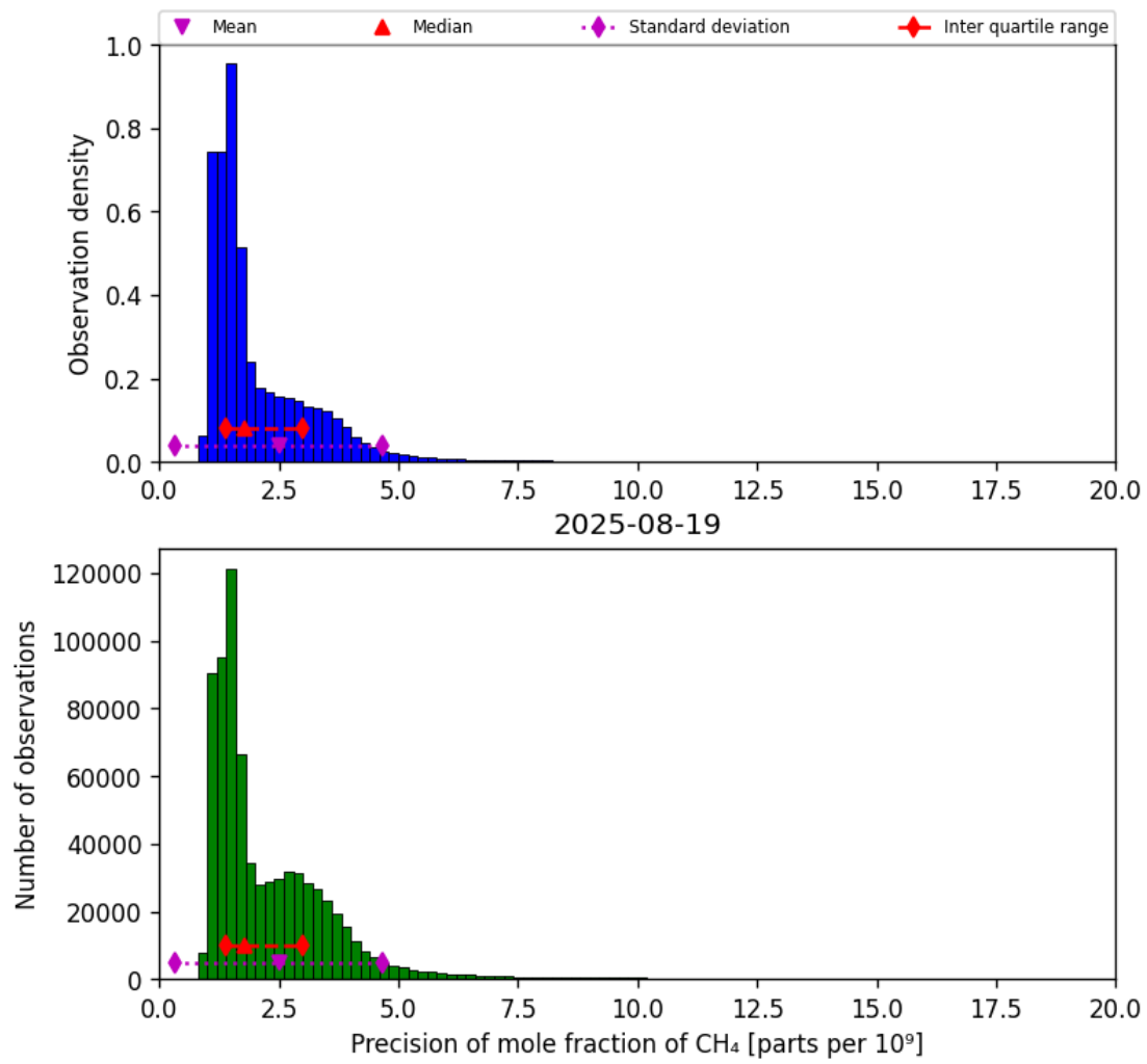
Figure 24: Histogram of “Precision of mole fraction of CH 4 ” for 2025-08-19 to 2025-08-20
