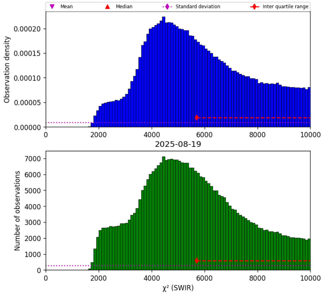
Figure 28: Histogram of “ \chi^2 (SWIR)” for 2025-08-19 to 2025-08-20
