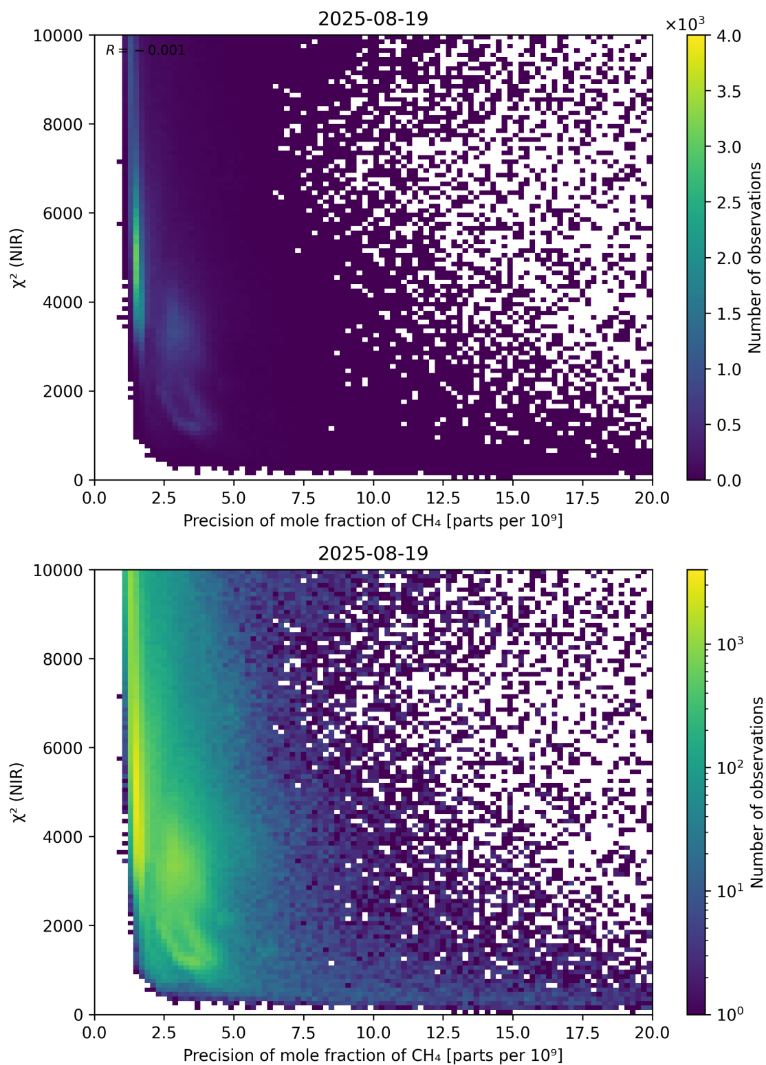
Figure 78: Scatter density plot of “Precision of mole fraction of CH 4 ” against “ \chi^2 (NIR)” for 2025-08-19 to 2025-08-20.
