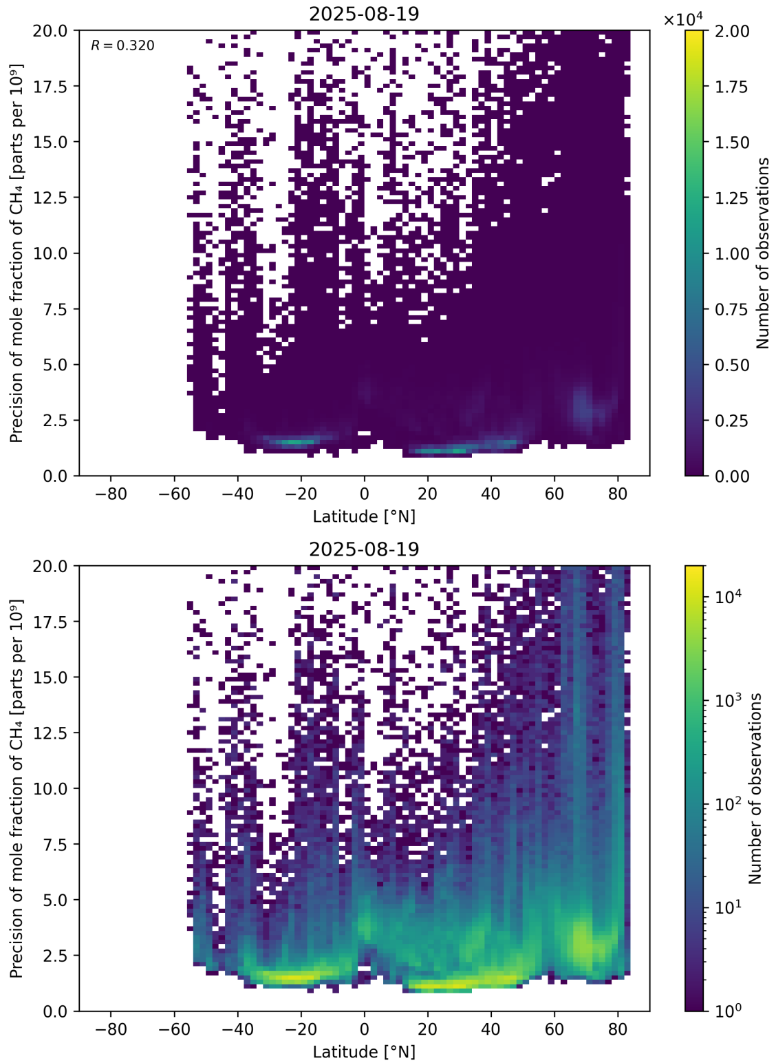
Figure 59: Scatter density plot of “Latitude” against “Precision of mole fraction of \text{CH}_4 ” for 2025-08-19 to 2025-08-20.
