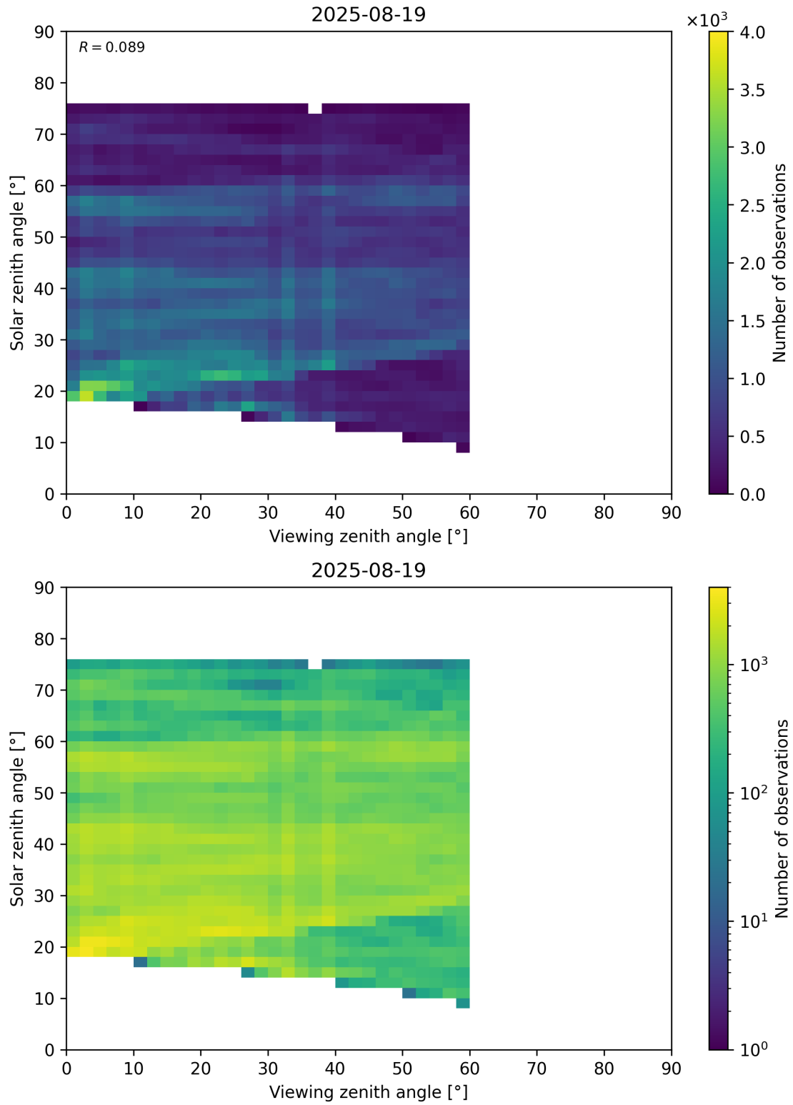
Figure 115: Scatter density plot of “Viewing zenith angle” against “Solar zenith angle” for 2025-08-19 to 2025-08-20.
