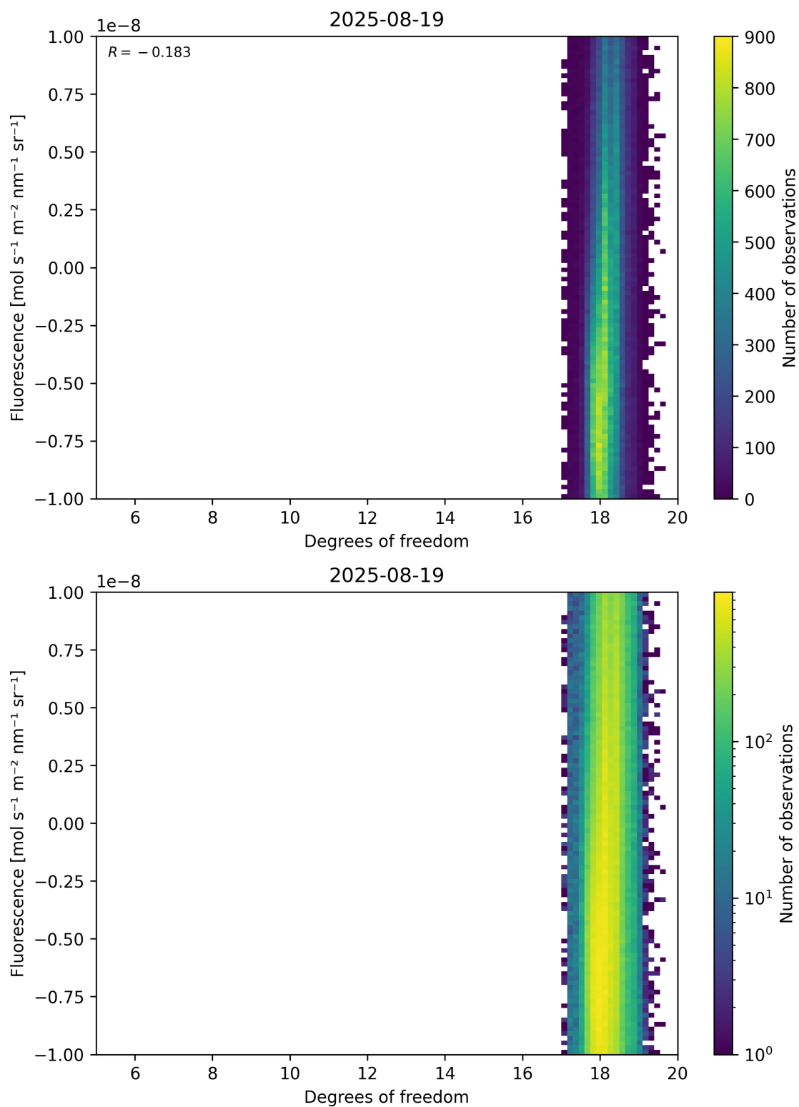
Figure 51: Scatter density plot of “Degrees of freedom” against “Fluorescence” for 2025-08-19 to 2025-08-20.
