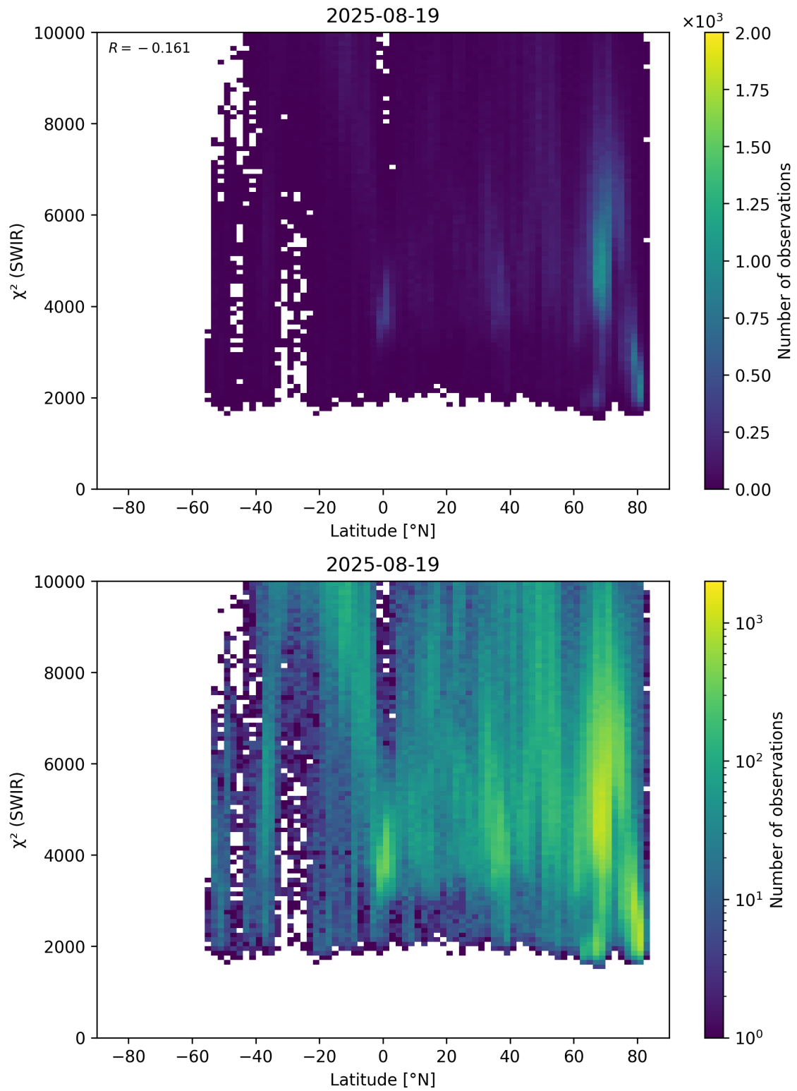
Figure 54: Scatter density plot of “Latitude” against “ \chi^2 (SWIR)” for 2025-08-19 to 2025-08-20.
