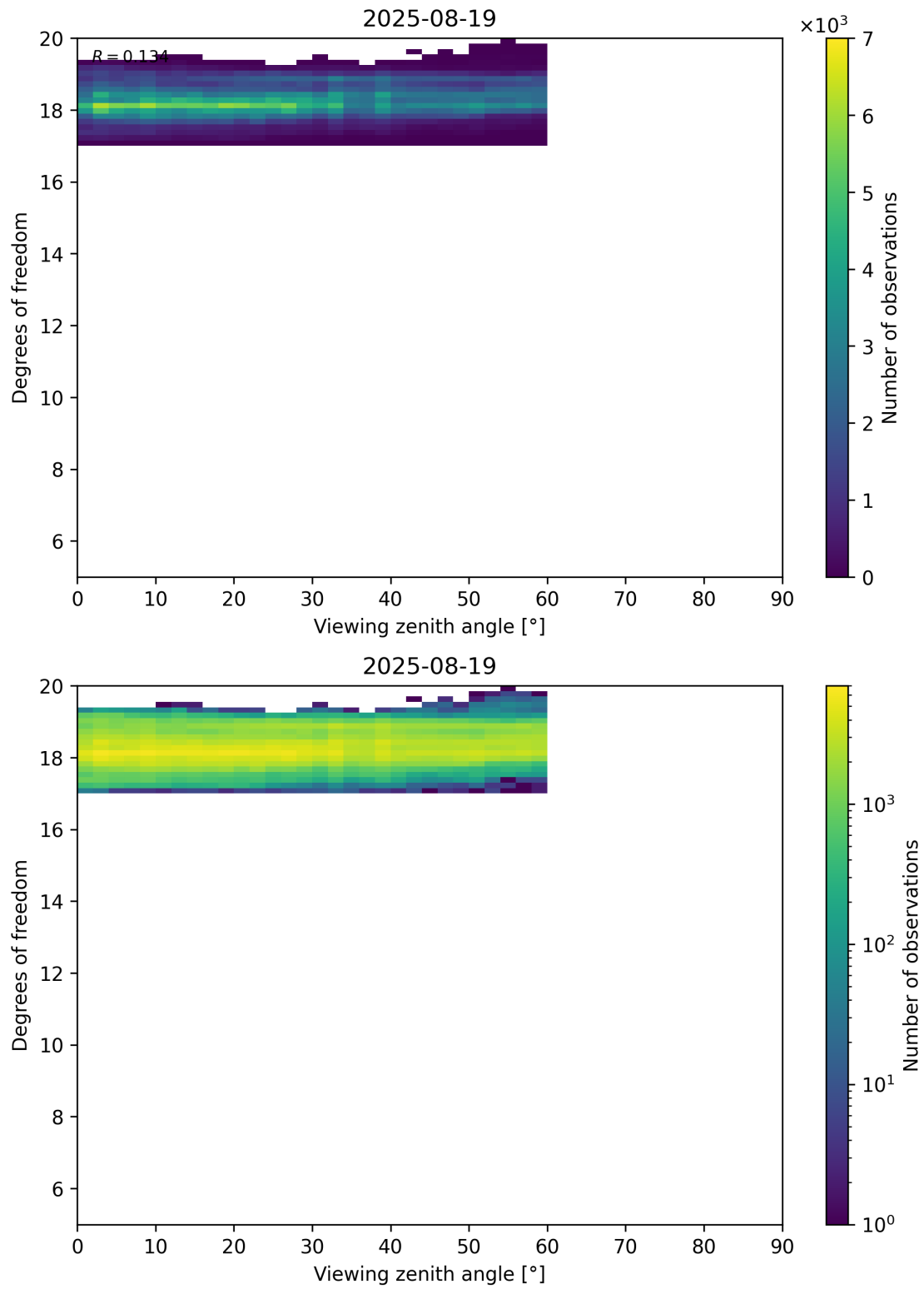
Figure 107: Scatter density plot of “Viewing zenith angle” against “Degrees of freedom” for 2025-08-19 to 2025-08-20.
