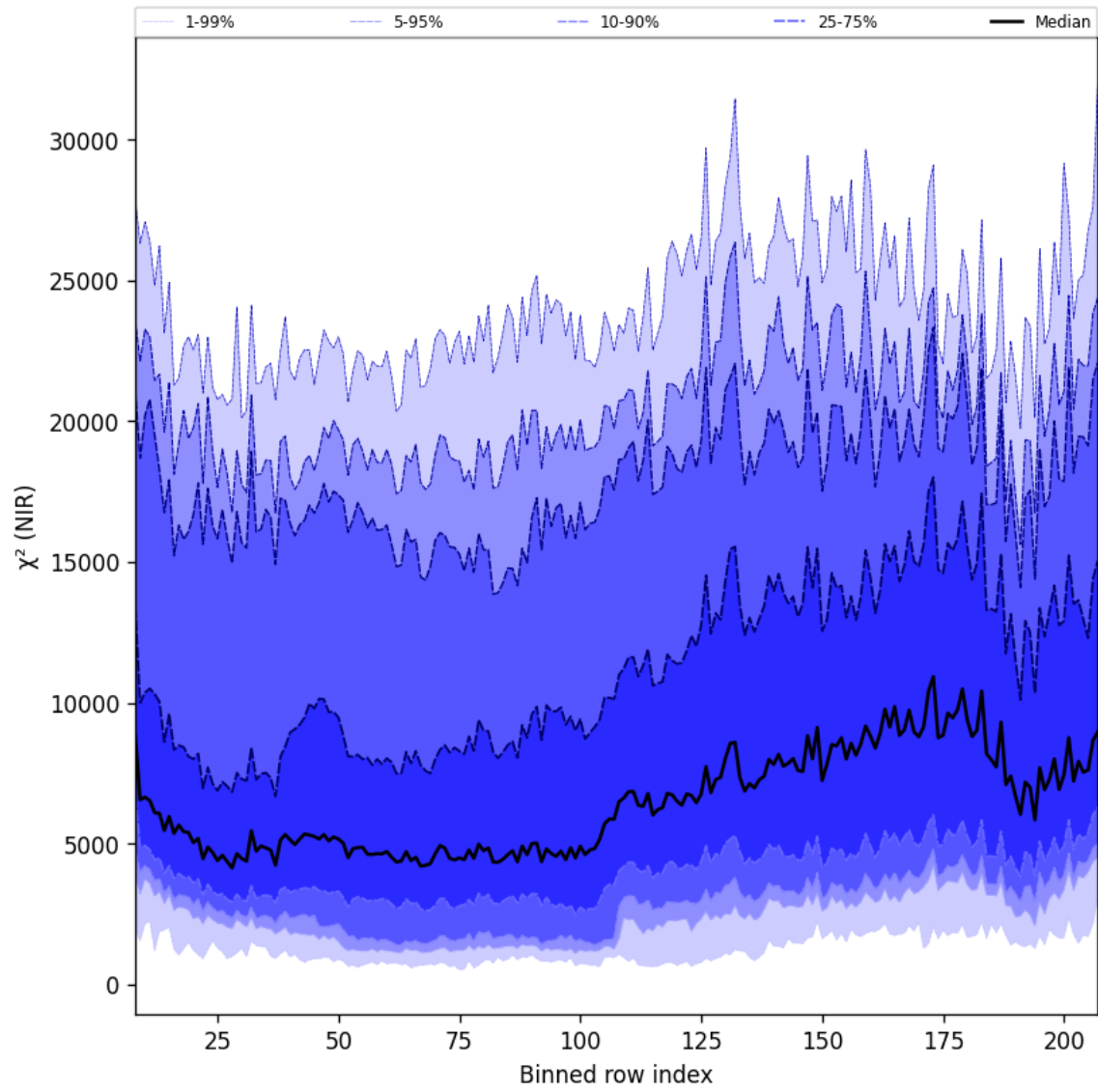
Figure 40: Along track statistics of “ \chi^2 (NIR)” for 2025-08-19 to 2025-08-20
