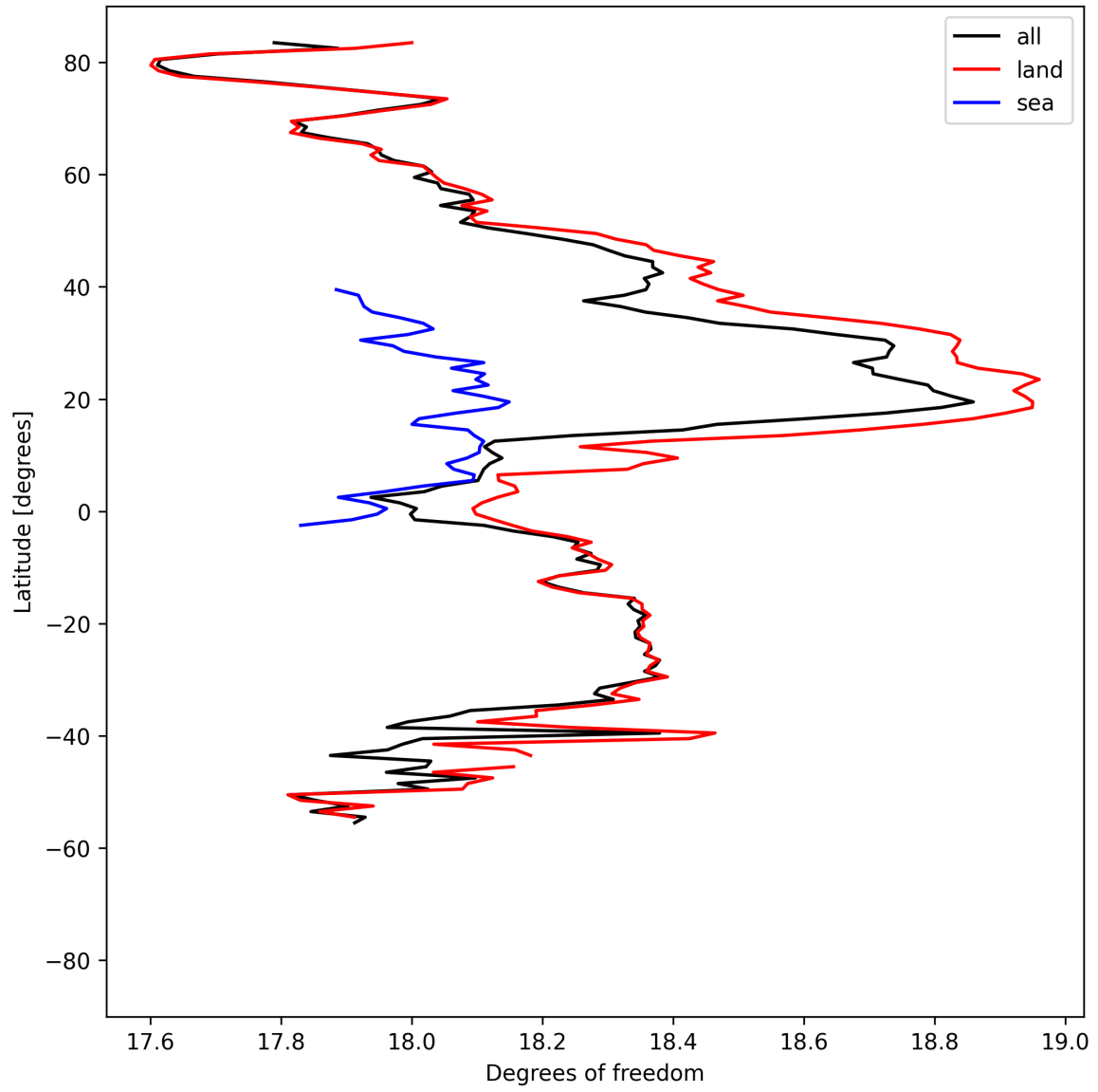
Figure 19: Zonal average of “Degrees of freedom” for 2025-08-19 to 2025-08-20.
