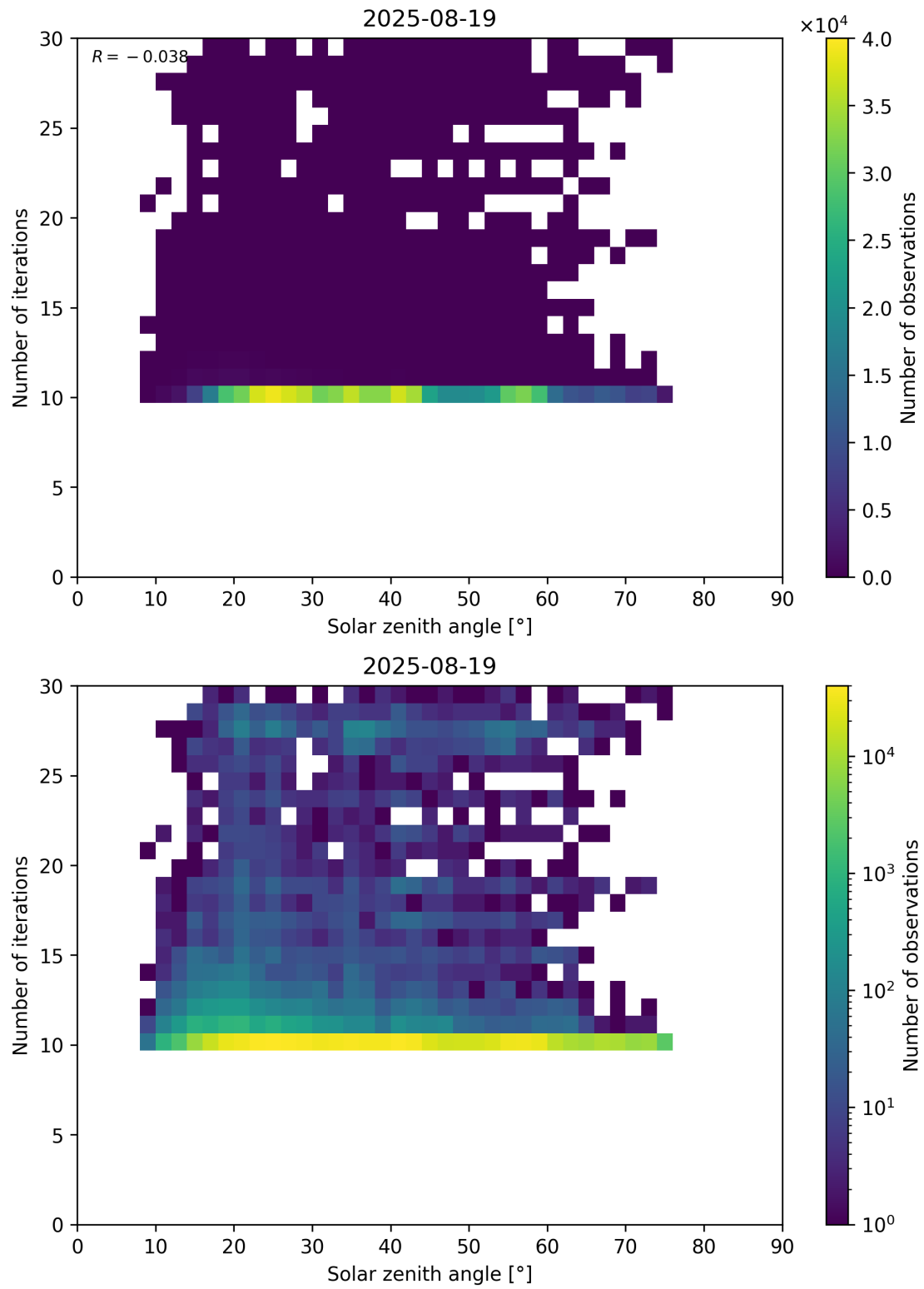
Figure 102: Scatter density plot of “Solar zenith angle” against “Number of iterations” for 2025-08-19 to 2025-08-20.
