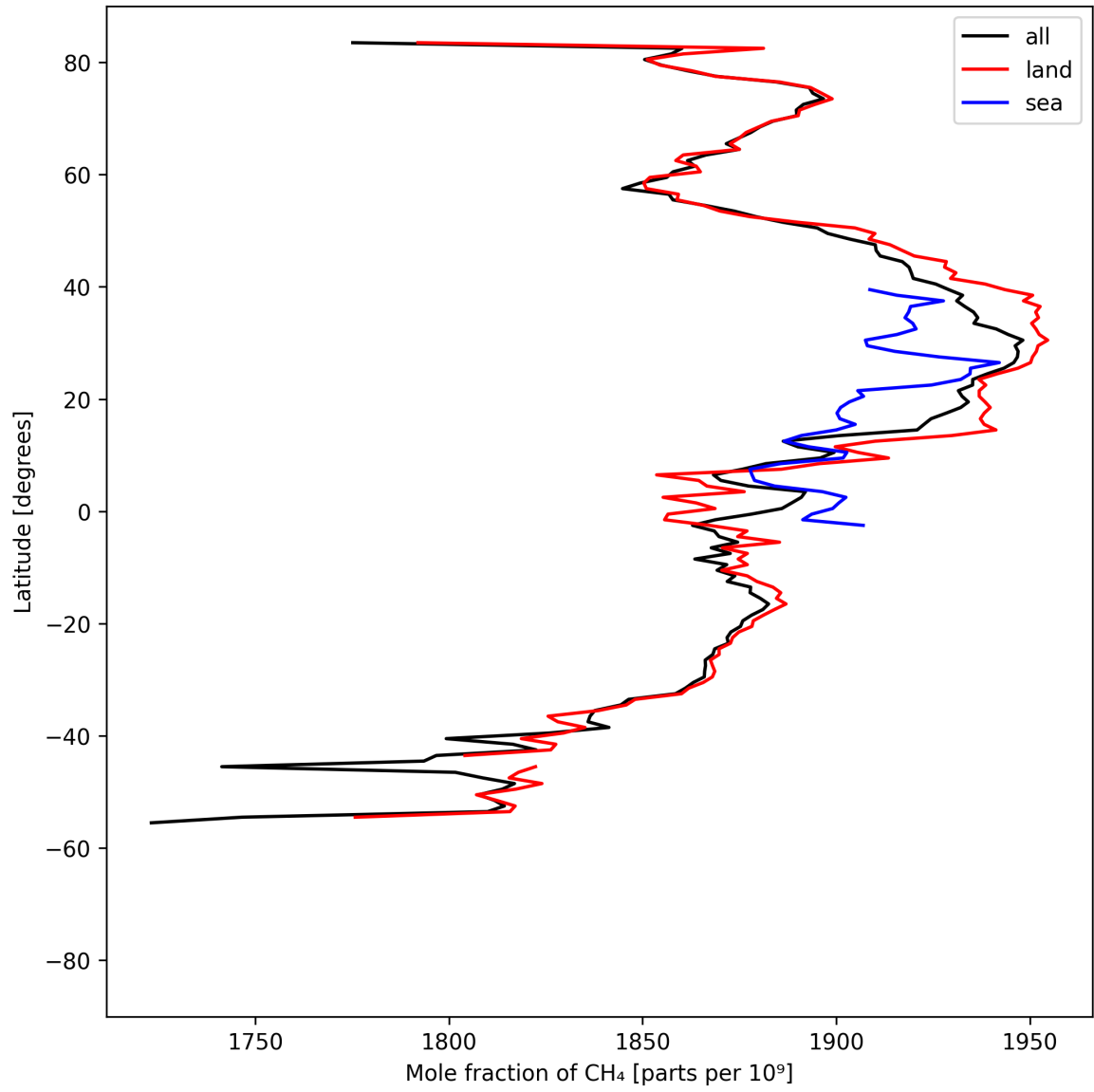
Figure 12: Zonal average of “Mole fraction of CH 4 ” for 2025-08-19 to 2025-08-20.
