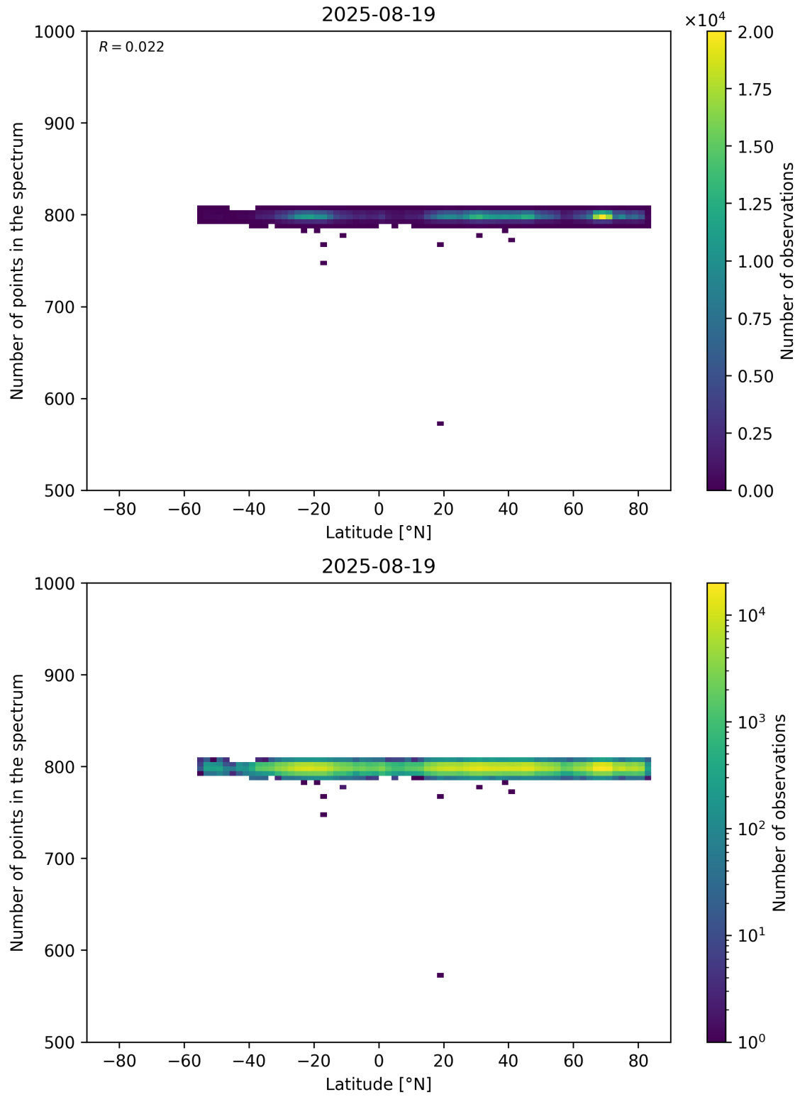
Figure 61: Scatter density plot of “Latitude” against “Number of points in the spectrum” for 2025-08-19 to 2025-08-20.
