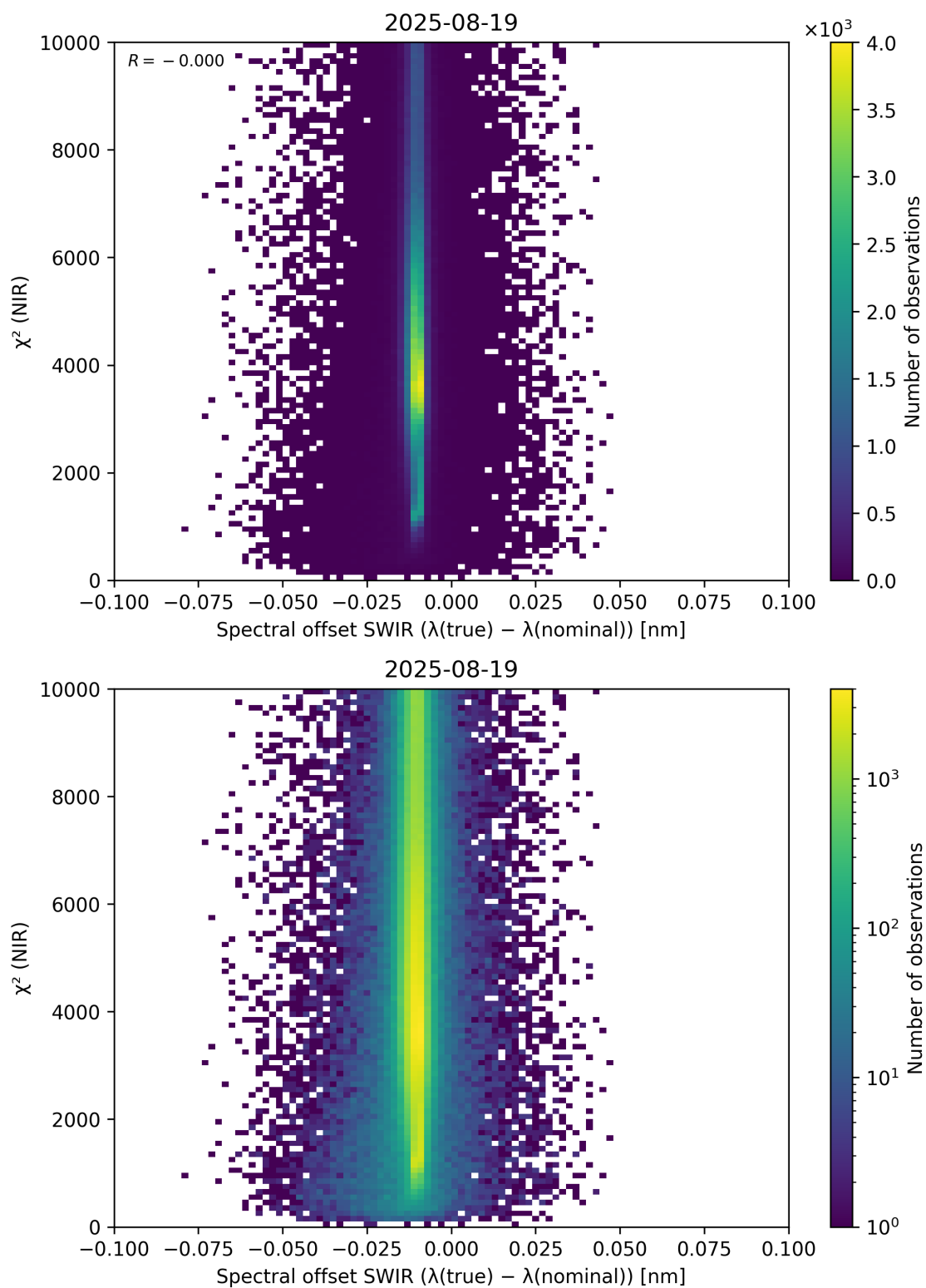
Figure 117: Scatter density plot of “Spectral offset SWIR ( \lambda_{\text{true}} - \lambda_{\text{nominal}} )” against “ \chi^2 (NIR)” for 2025-08-19 to 2025-08-20.
