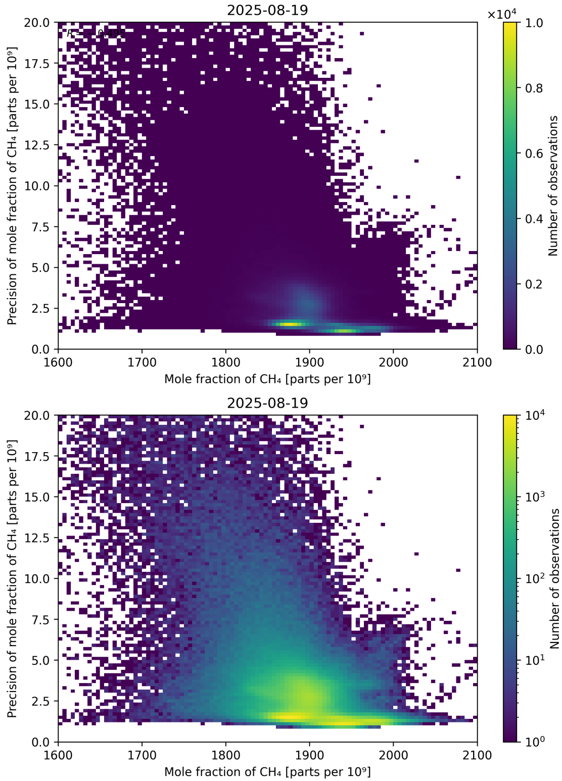
Figure 75: Scatter density plot of “Mole fraction of CH 4 ” against “Precision of mole fraction of CH 4 ” for 2025-08-19 to 2025-08-20.
