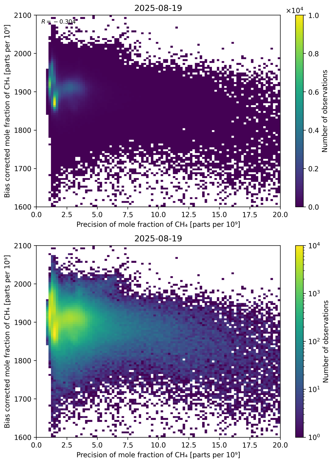
Figure 82: Scatter density plot of “Precision of mole fraction of CH 4 ” against “Bias corrected mole fraction of CH 4 ” for 2025-08-19 to 2025-08-20.
