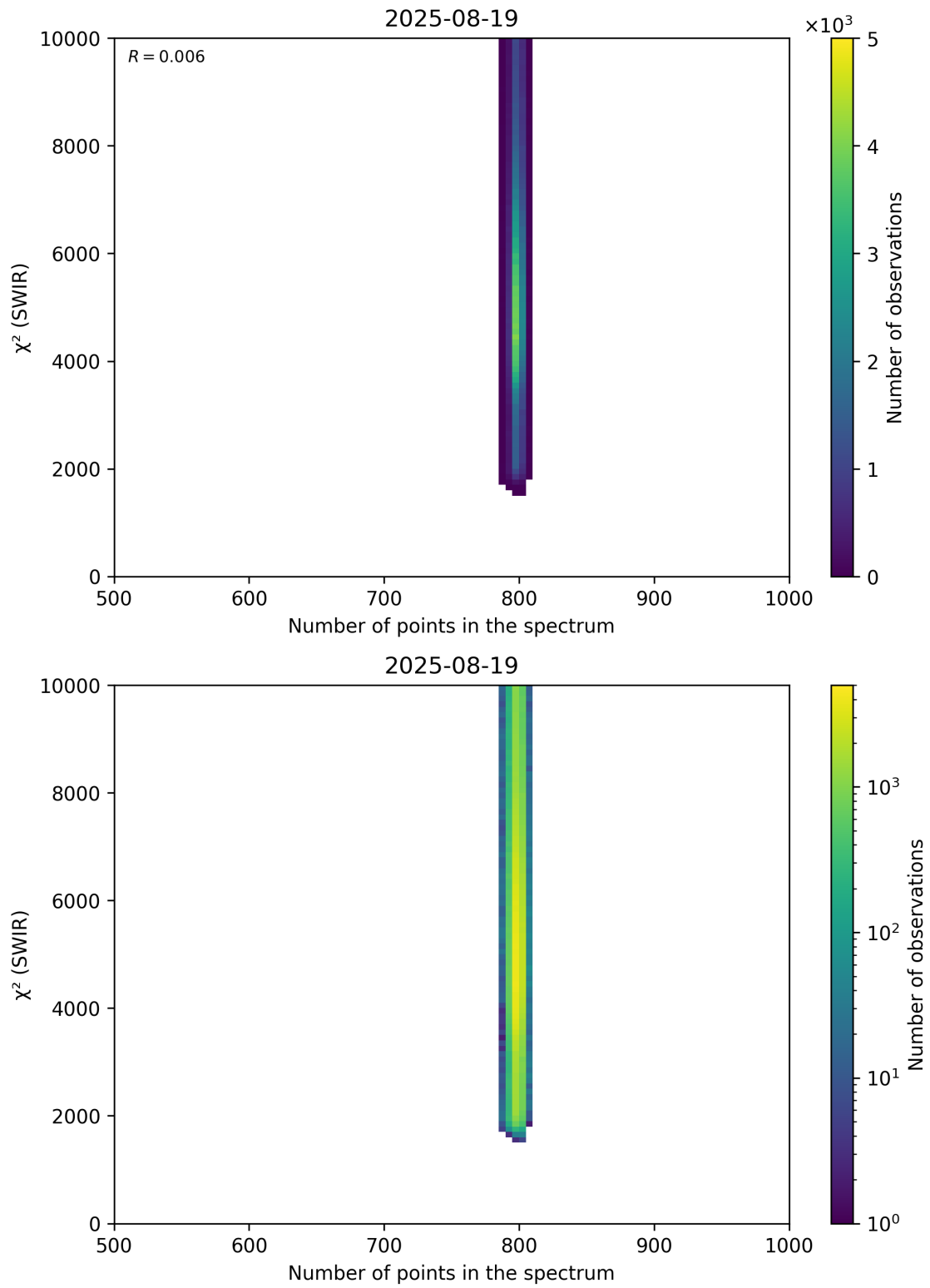
Figure 89: Scatter density plot of “Number of points in the spectrum” against “ \chi^2 (SWIR)” for 2025-08-19 to 2025-08-20.
