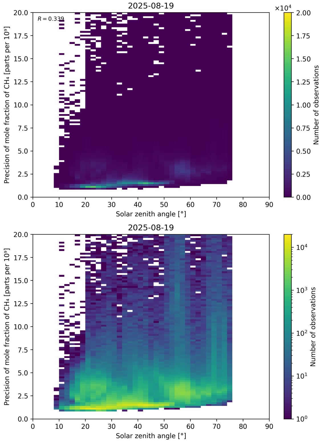
Figure 101: Scatter density plot of “Solar zenith angle” against “Precision of mole fraction of CH 4 ” for 2025-08-19 to 2025-08-20.
