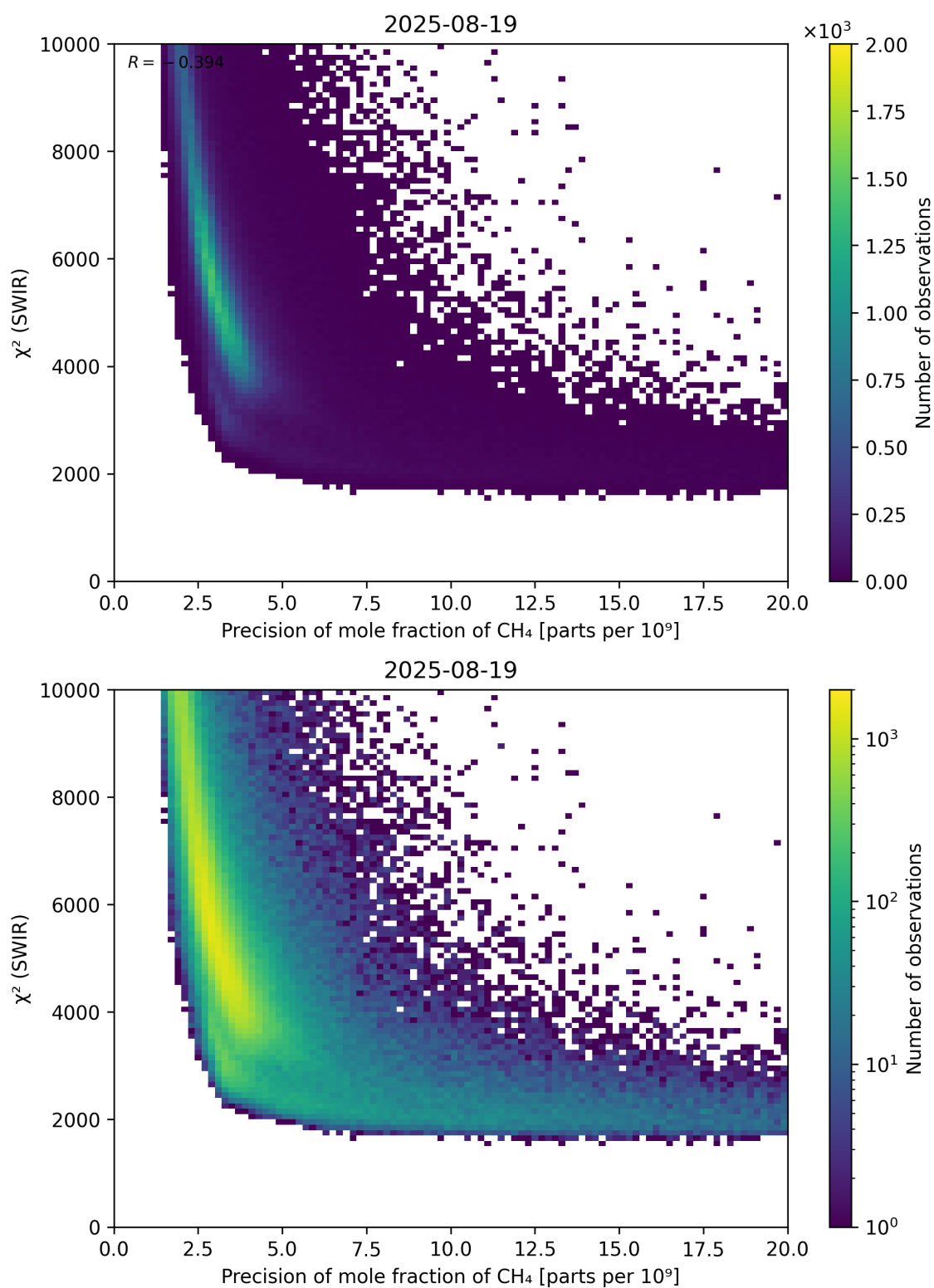
Figure 79: Scatter density plot of “Precision of mole fraction of \text{CH}_4 ” against “ \chi^2 (SWIR)” for 2025-08-19 to 2025-08-20.
