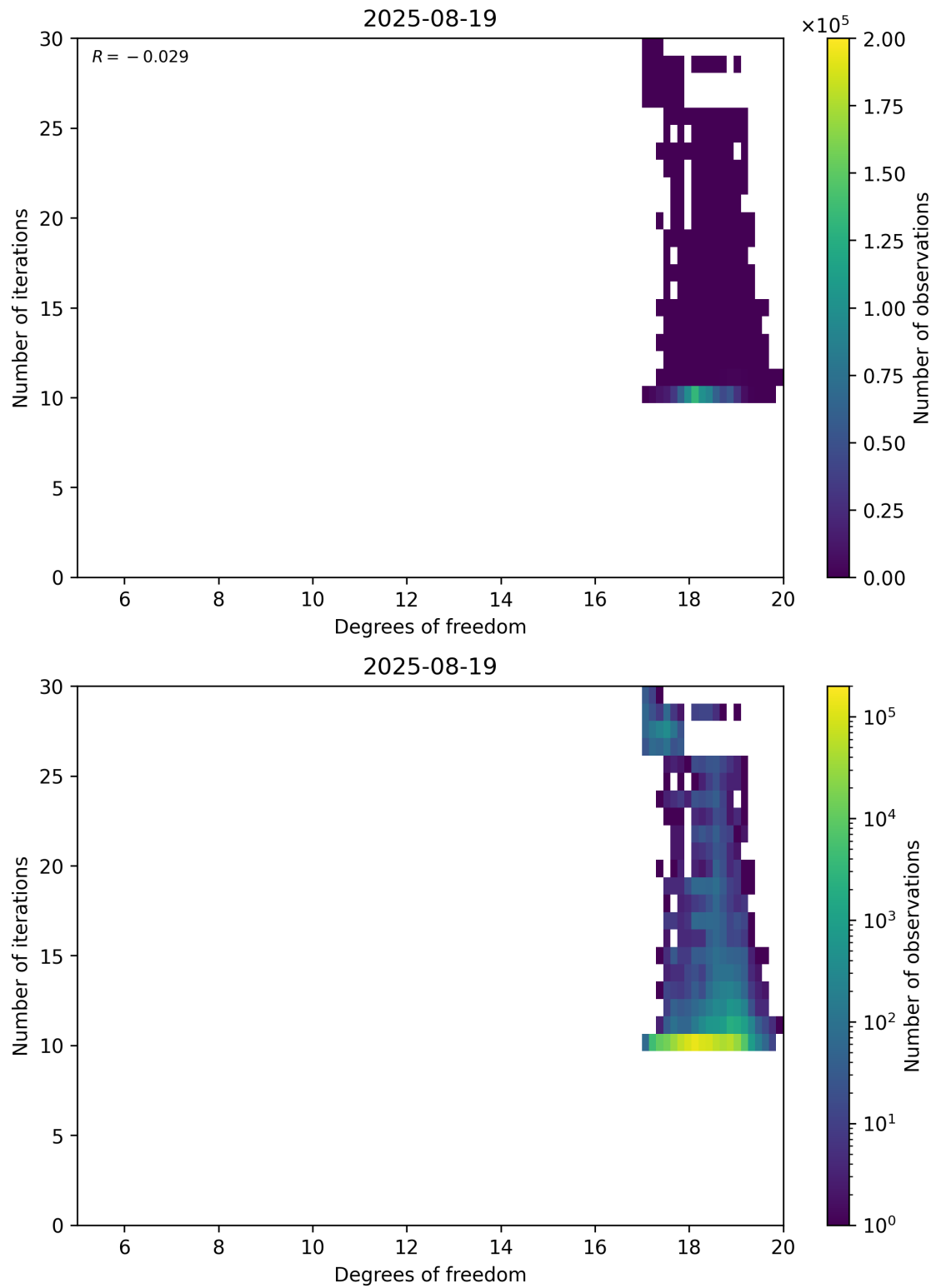
Figure 52: Scatter density plot of “Degrees of freedom” against “Number of iterations” for 2025-08-19 to 2025-08-20.
