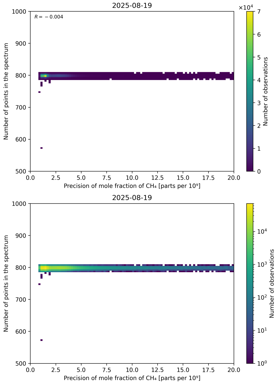
Figure 84: Scatter density plot of “Precision of mole fraction of CH 4 ” against “Number of points in the spectrum” for 2025-08-19 to 2025-08-20.
