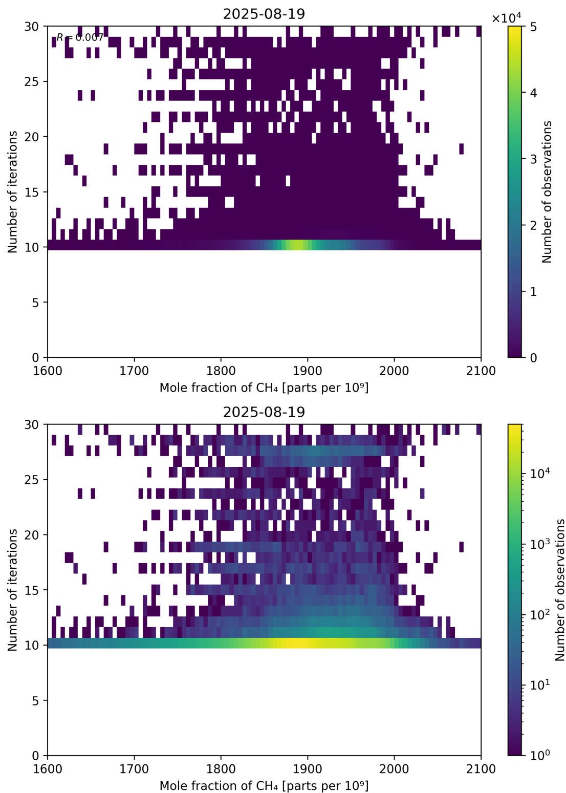
Figure 76: Scatter density plot of “Mole fraction of CH 4 ” against “Number of iterations” for 2025-08-19 to 2025-08-20.
