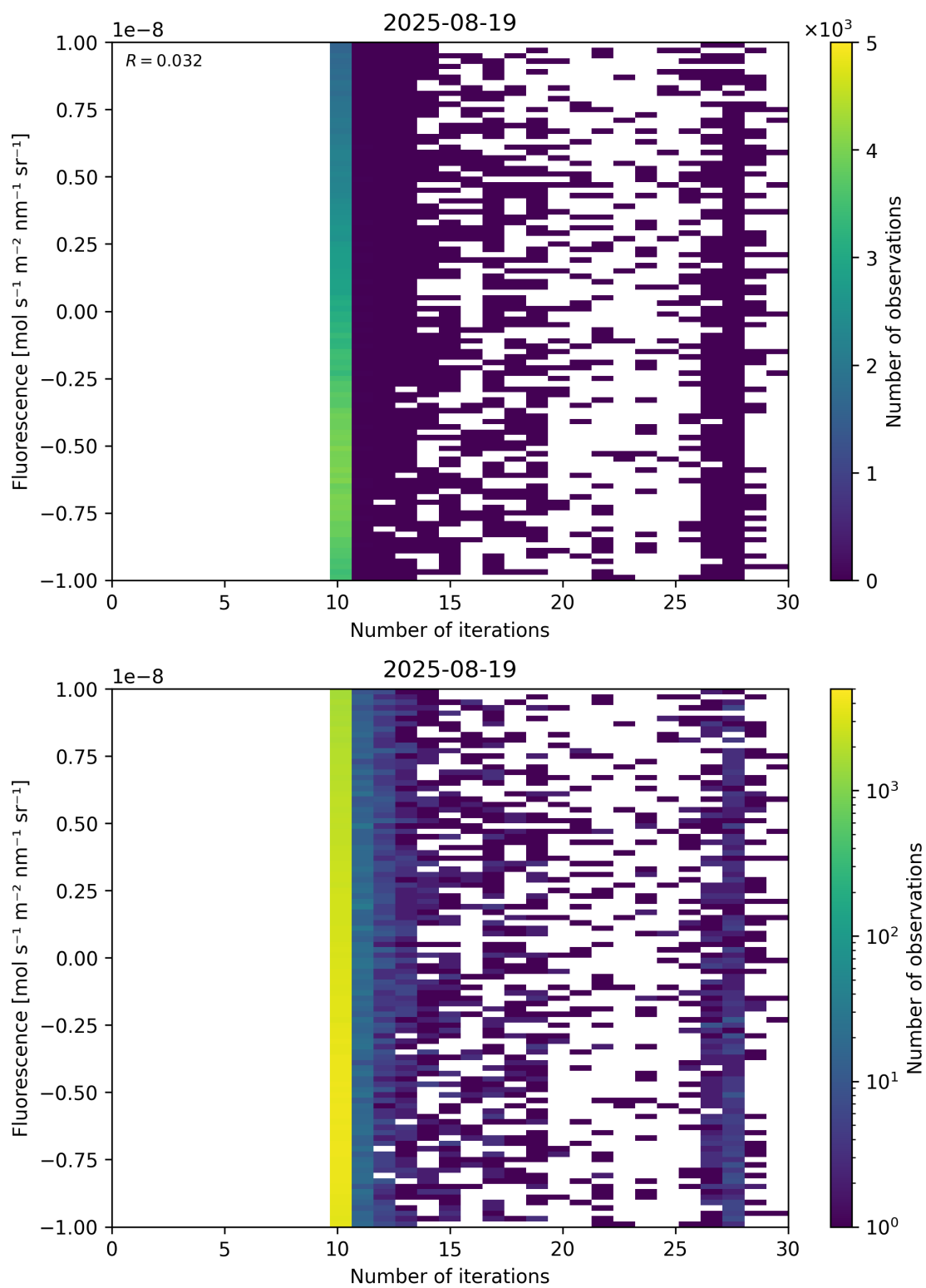
Figure 87: Scatter density plot of “Number of iterations” against “Fluorescence” for 2025-08-19 to 2025-08-20.
