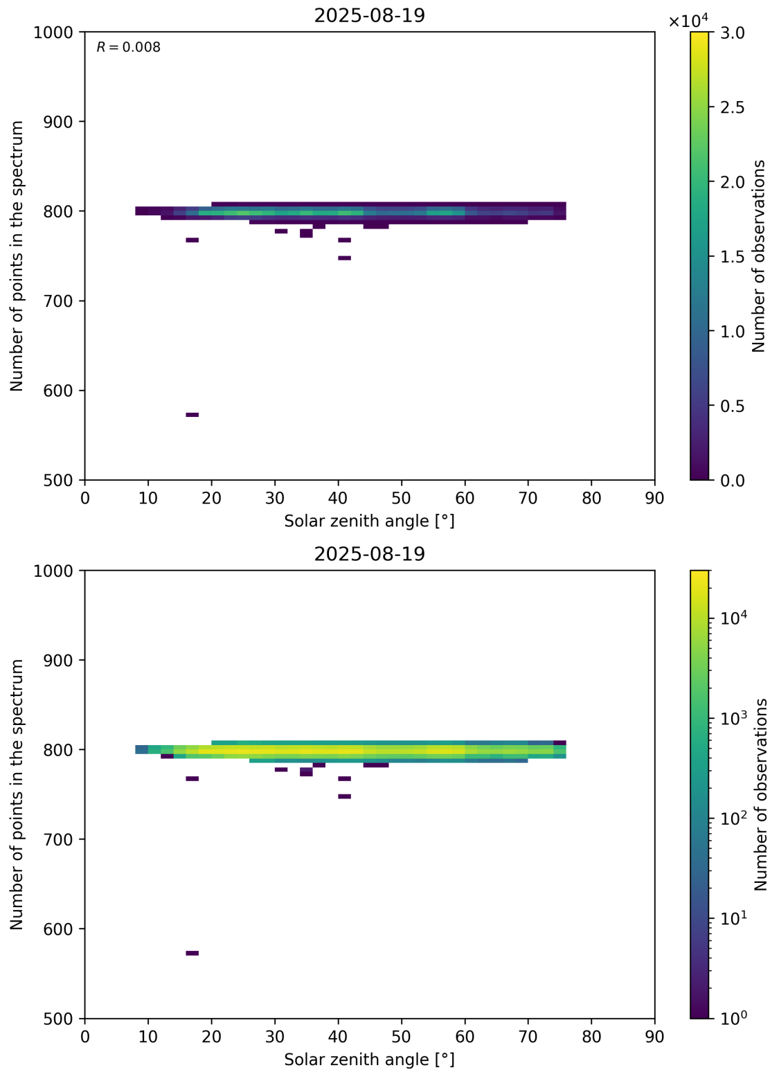
Figure 103: Scatter density plot of “Solar zenith angle” against “Number of points in the spectrum” for 2025-08-19 to 2025-08-20.
