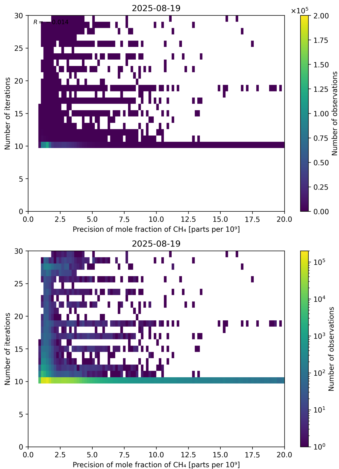
Figure 83: Scatter density plot of “Precision of mole fraction of CH 4 ” against “Number of iterations” for 2025-08-19 to 2025-08-20.
