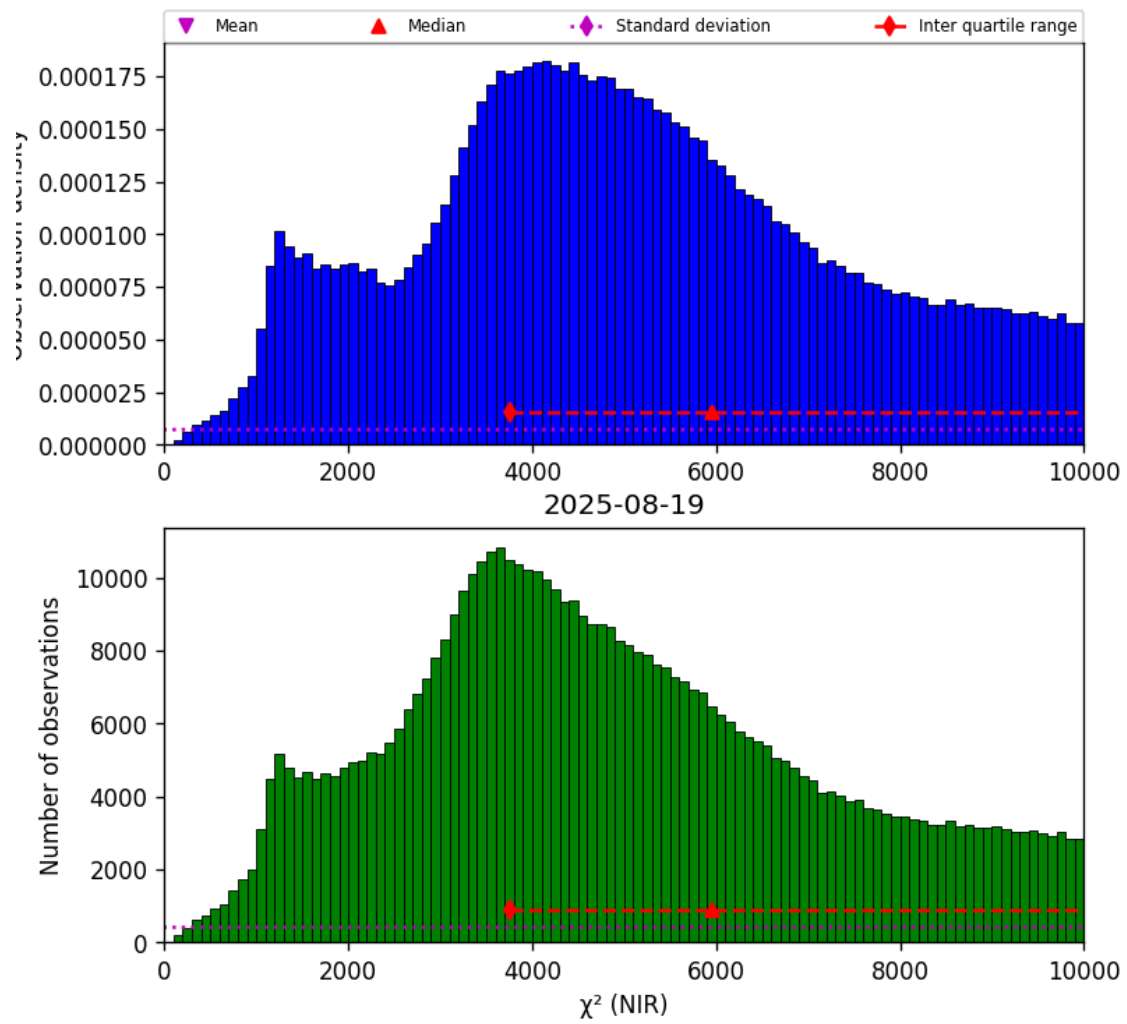
Figure 29: Histogram of “ \chi^2 (NIR)” for 2025-08-19 to 2025-08-20
