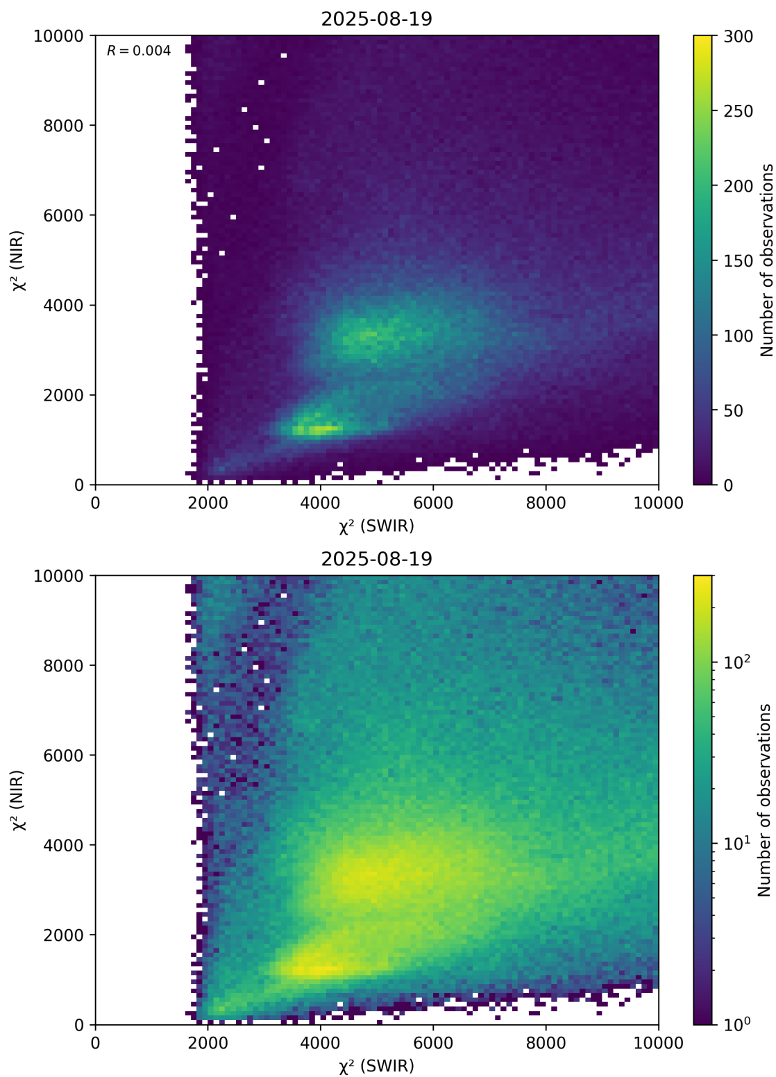
Figure 47: Scatter density plot of “ \chi^2 (SWIR)” against “ \chi^2 (NIR)” for 2025-08-19 to 2025-08-20.
