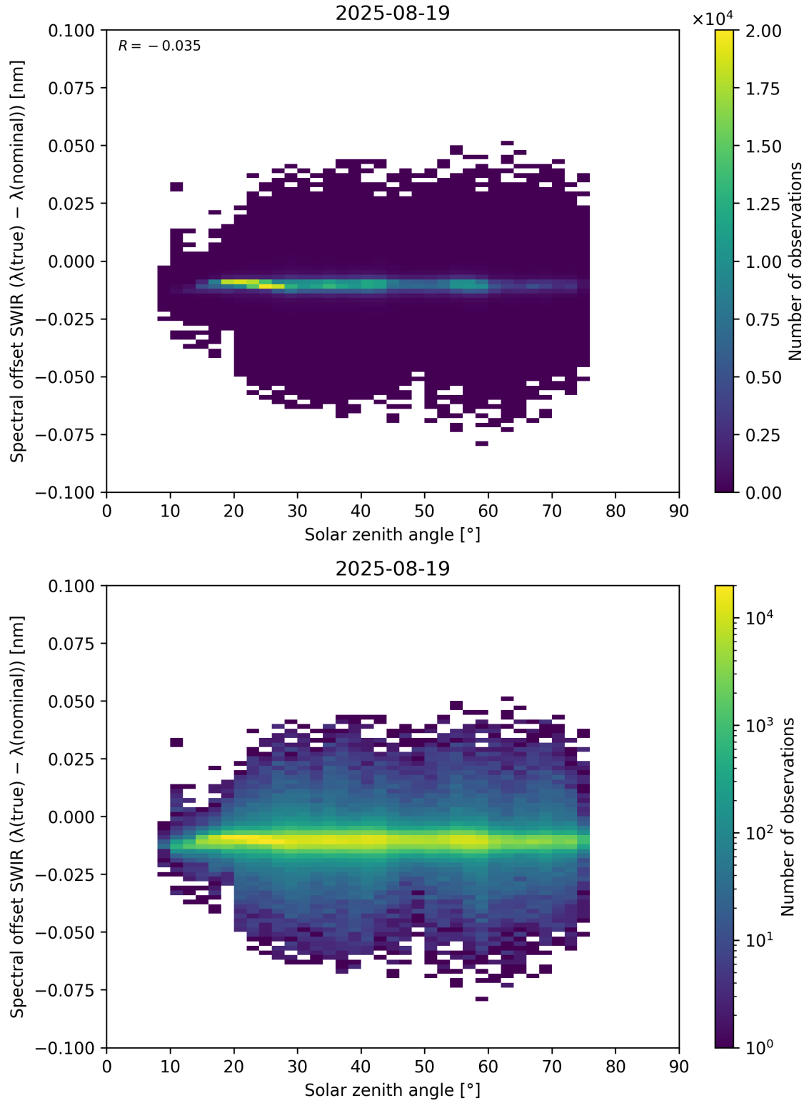
Figure 104: Scatter density plot of “Solar zenith angle” against “Spectral offset SWIR ( \lambda_{\text{true}} - \lambda_{\text{nominal}} )” for 2025-08-19 to 2025-08-20.
