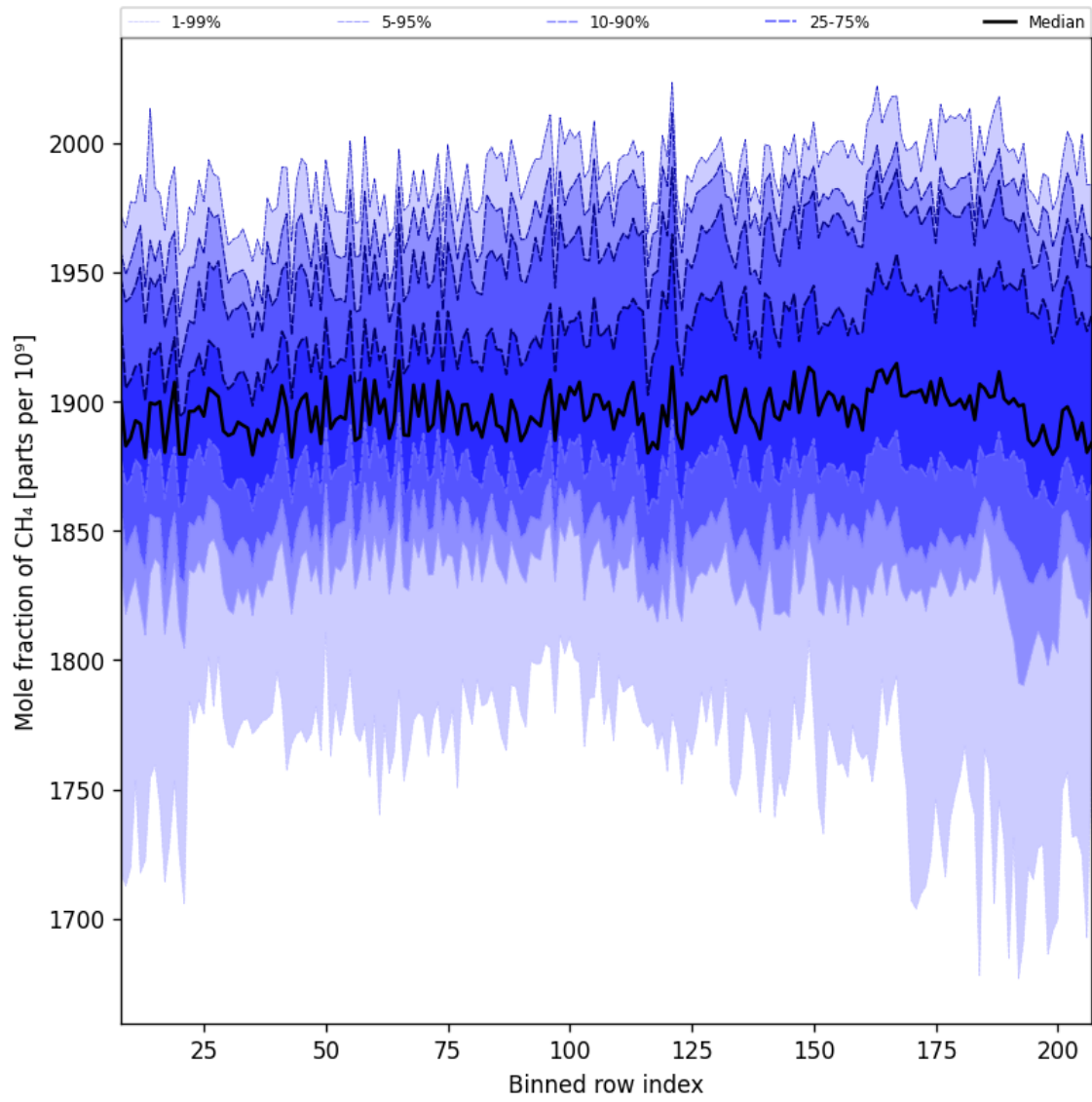
Figure 34: Along track statistics of “Mole fraction of CH 4 ” for 2025-08-19 to 2025-08-20
