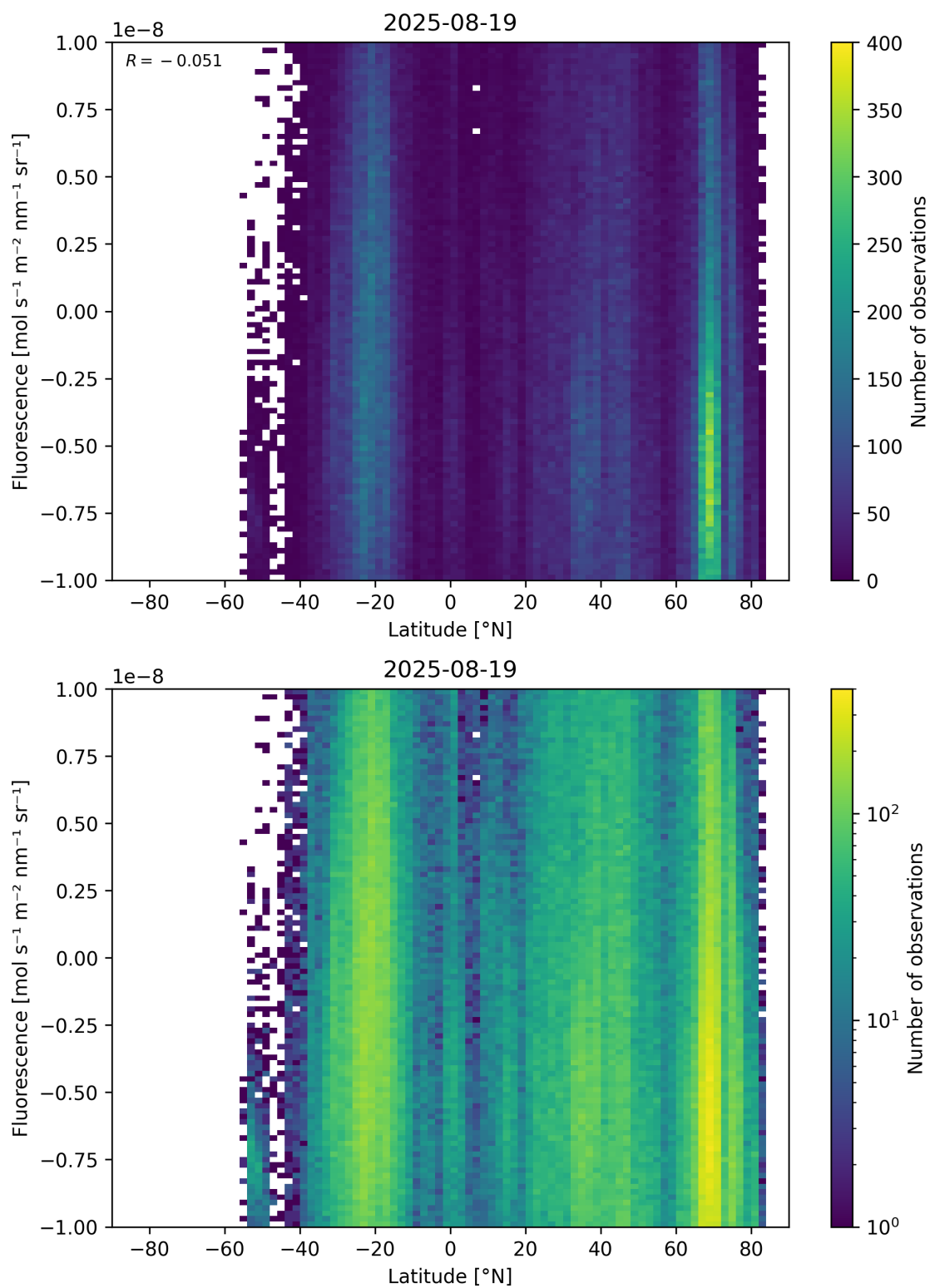
Figure 56: Scatter density plot of “Latitude” against “Fluorescence” for 2025-08-19 to 2025-08-20.
