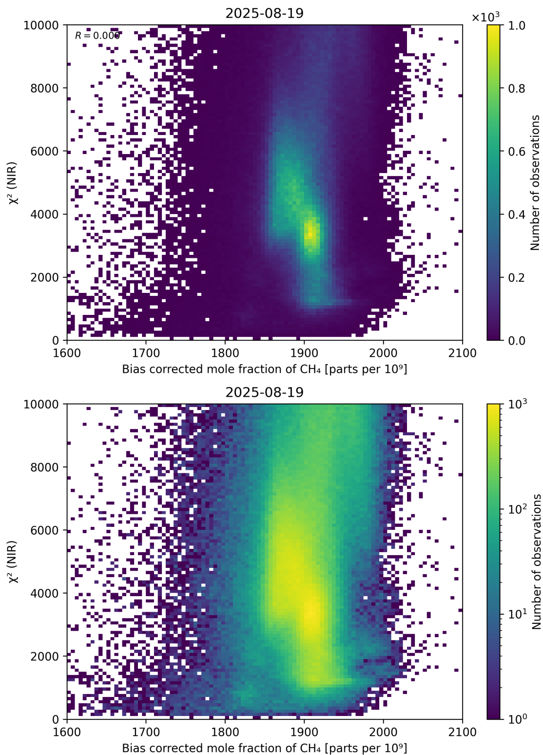
Figure 63: Scatter density plot of “Bias corrected mole fraction of \text{CH}_4 ” against “ \chi^2 (NIR)” for 2025-08-19 to 2025-08-20.
