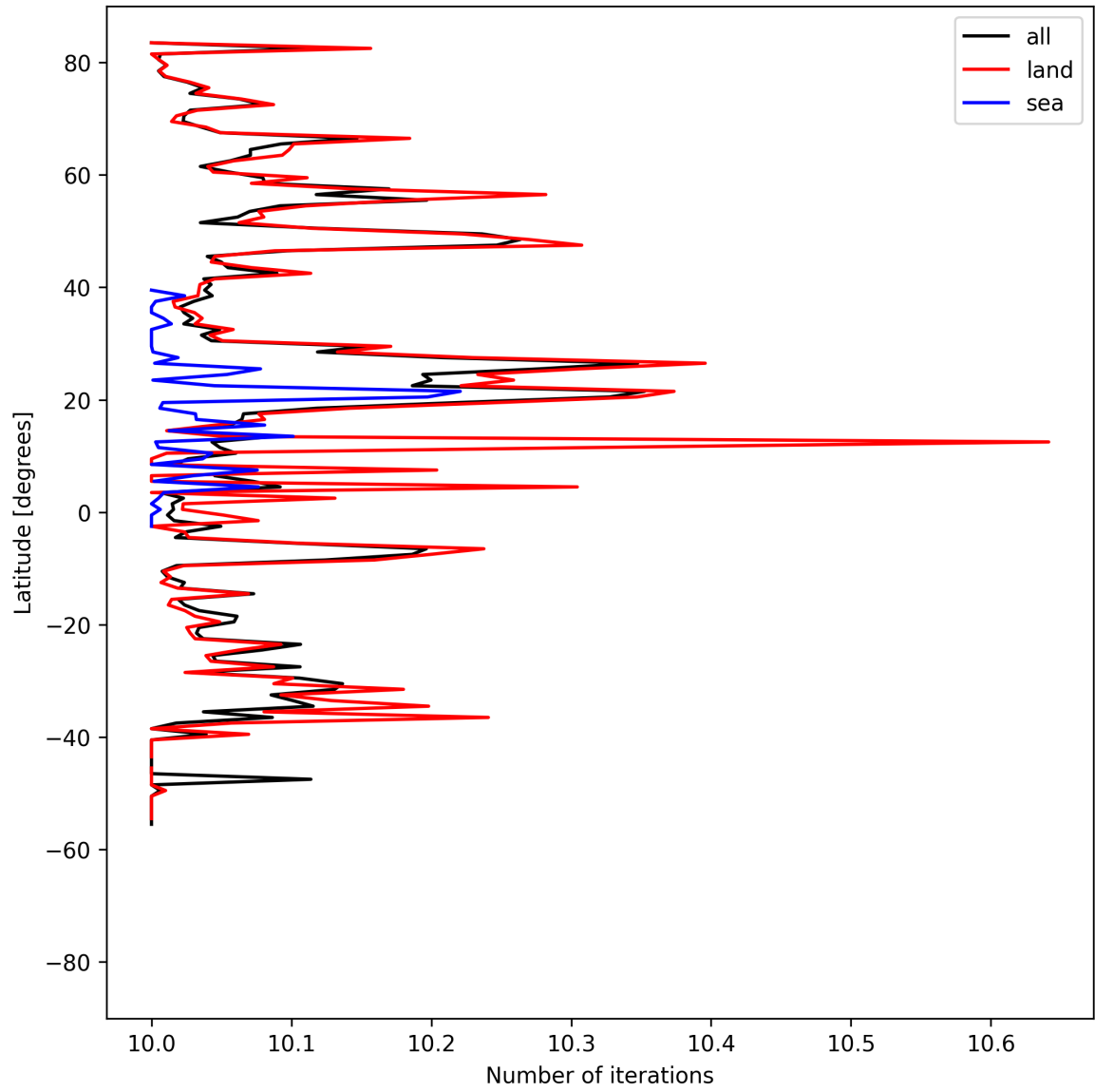
Figure 20: Zonal average of “Number of iterations” for 2025-08-19 to 2025-08-20.
