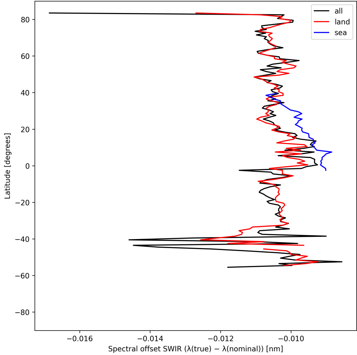
Figure 16: Zonal average of “Spectral offset SWIR ( \lambda_{\text{true}} - \lambda_{\text{nominal}} )” for 2025-08-19 to 2025-08-20.
