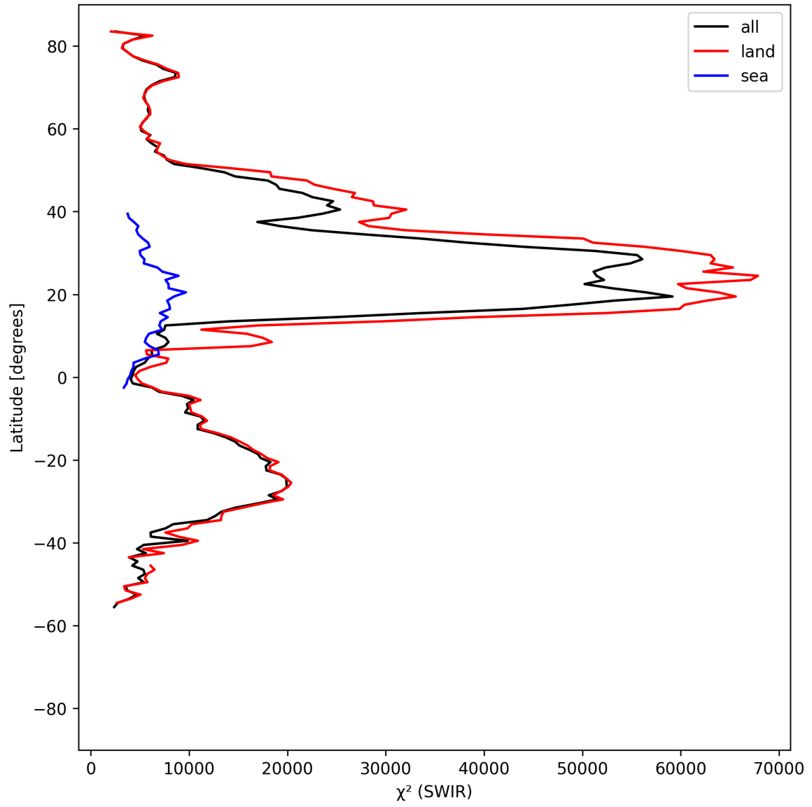
Figure 17: Zonal average of “ \chi^2 (SWIR)” for 2025-08-19 to 2025-08-20.
