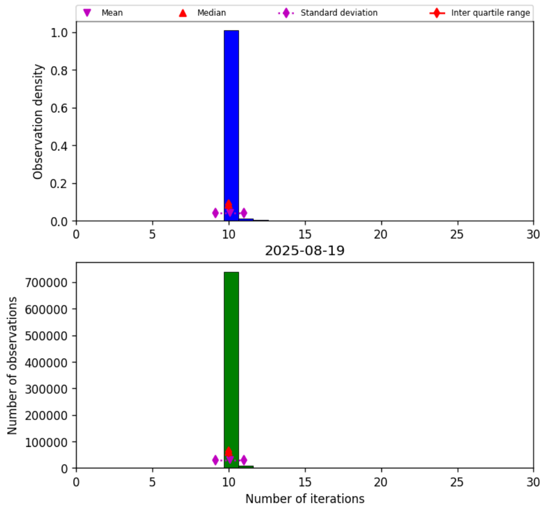
Figure 31: Histogram of “Number of iterations” for 2025-08-19 to 2025-08-20
