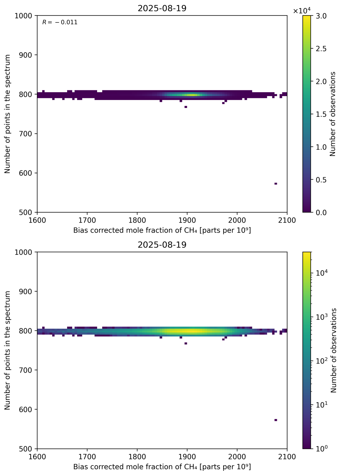
Figure 68: Scatter density plot of “Bias corrected mole fraction of CH 4 ” against “Number of points in the spectrum” for 2025-08-19 to 2025-08-20.
