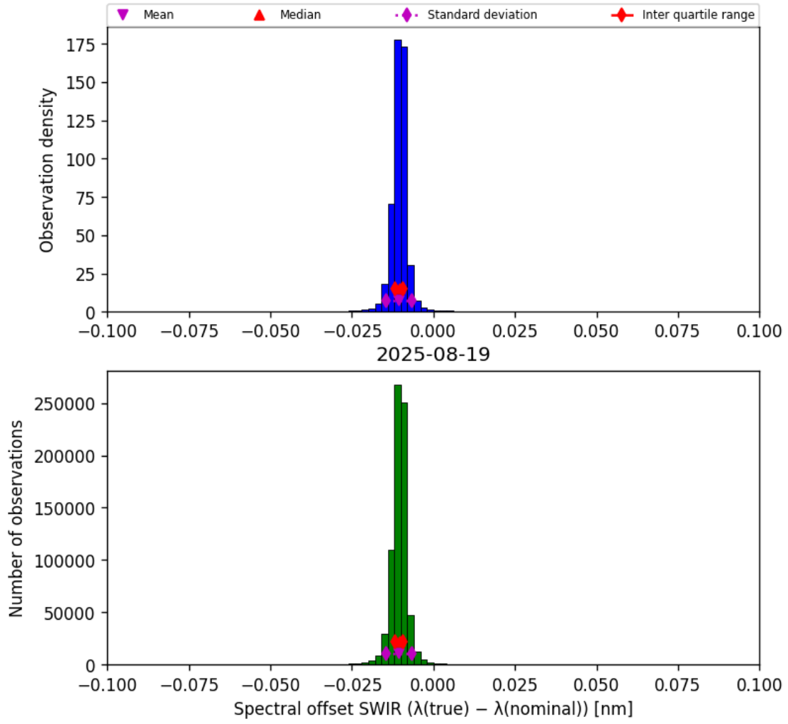
Figure 27: Histogram of “Spectral offset SWIR ( \lambda_{\text{true}} - \lambda_{\text{nominal}} )” for 2025-08-19 to 2025-08-20
