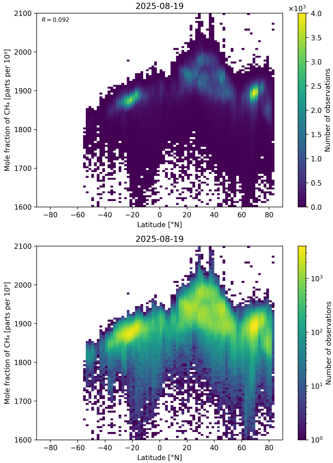
Figure 57: Scatter density plot of “Latitude” against “Mole fraction of CH 4 ” for 2025-08-19 to 2025-08-20.
