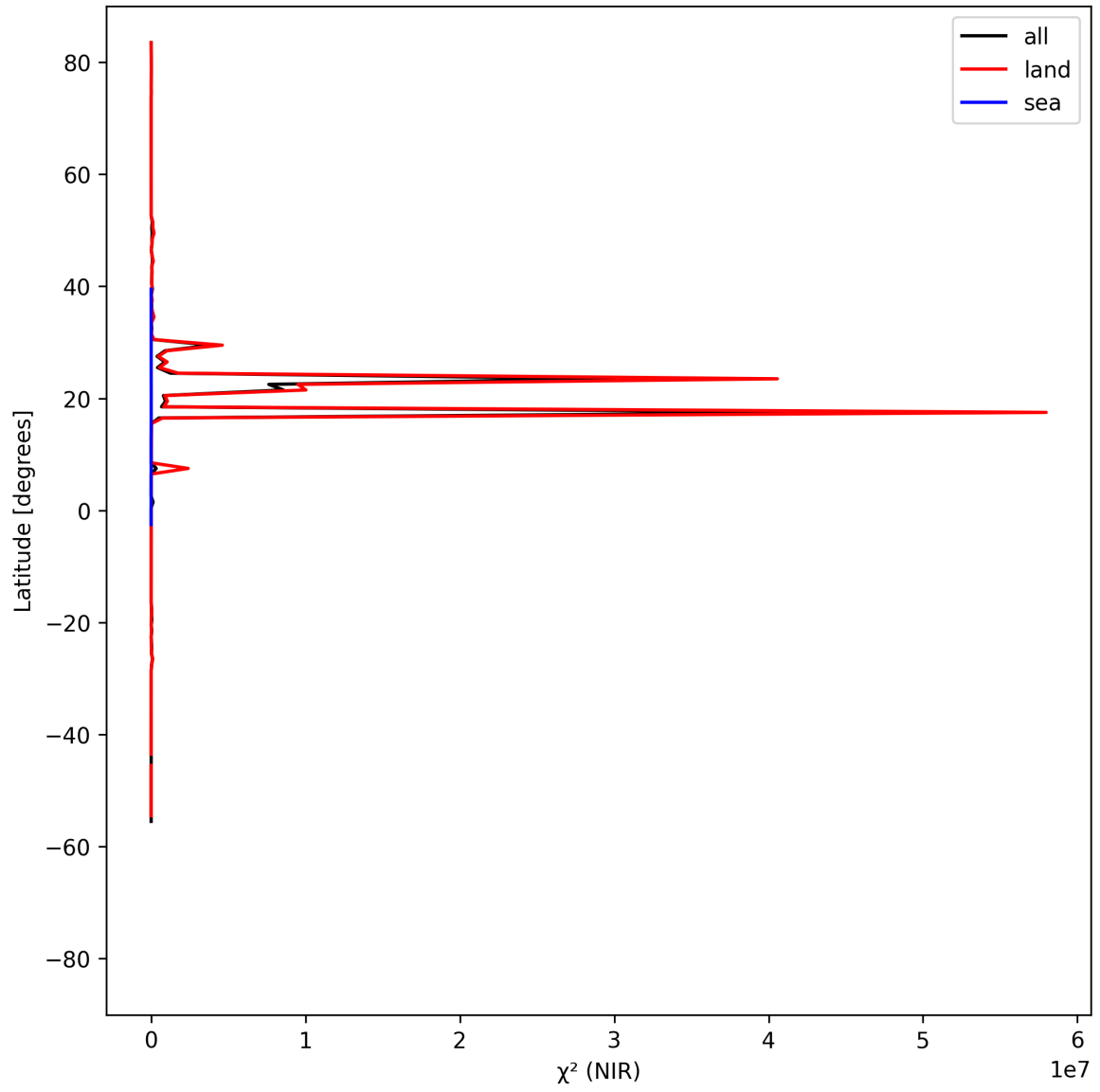
Figure 18: Zonal average of “ \chi^2 (NIR)” for 2025-08-19 to 2025-08-20.
