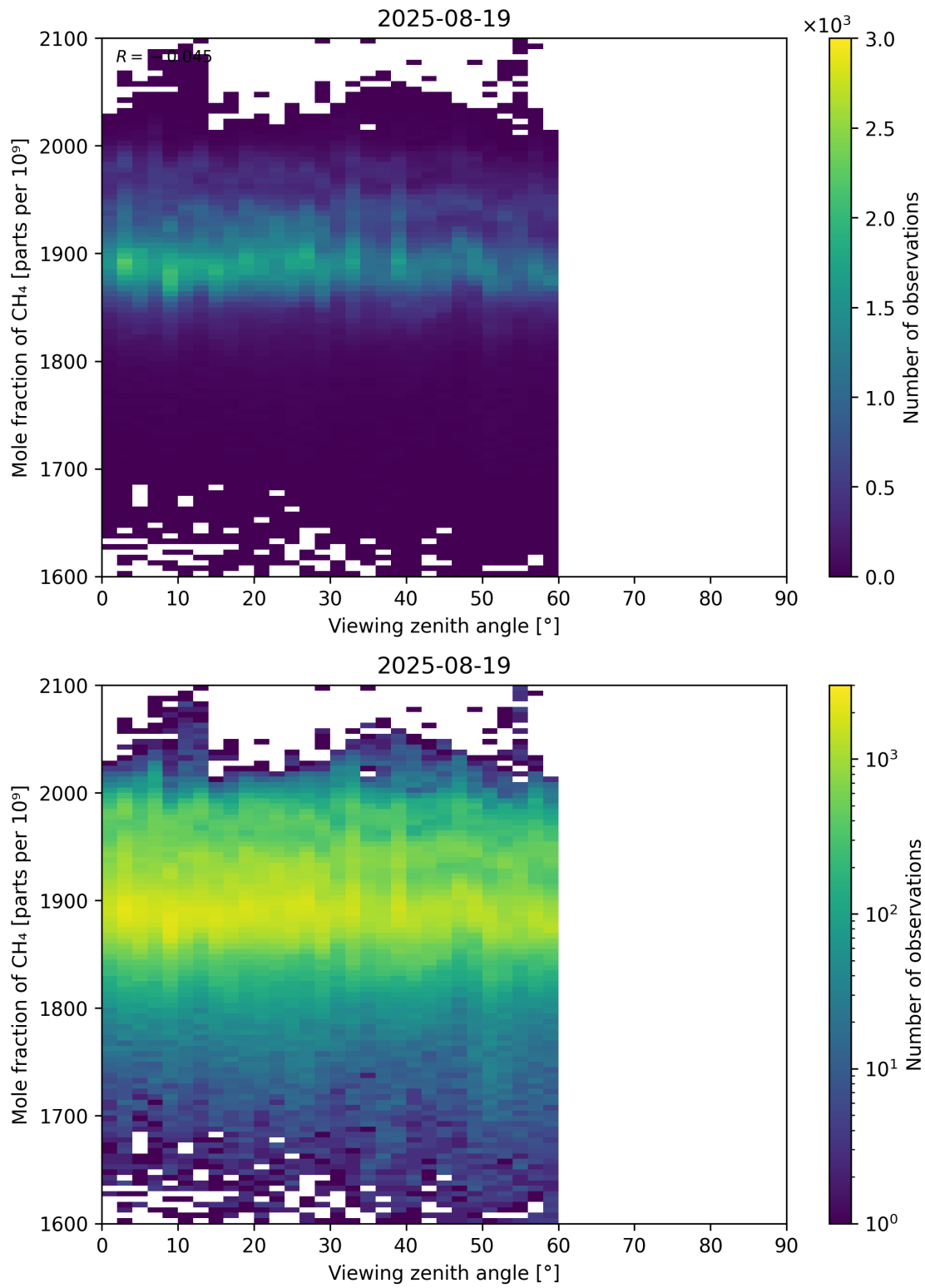
Figure 110: Scatter density plot of “Viewing zenith angle” against “Mole fraction of CH 4 ” for 2025-08-19 to 2025-08-20.
