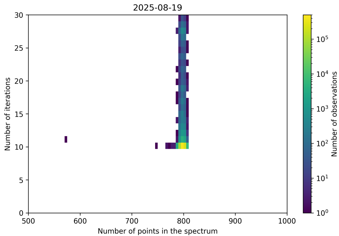
Figure 92: Scatter density plot of “Number of points in the spectrum” against “Number of iterations” for 2025-08-19 to 2025-08-20.
