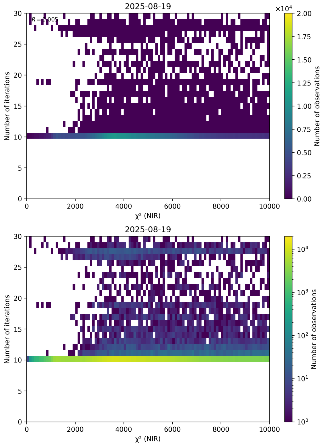
Figure 46: Scatter density plot of “ \chi^2 (NIR)” against “Number of iterations” for 2025-08-19 to 2025-08-20.
