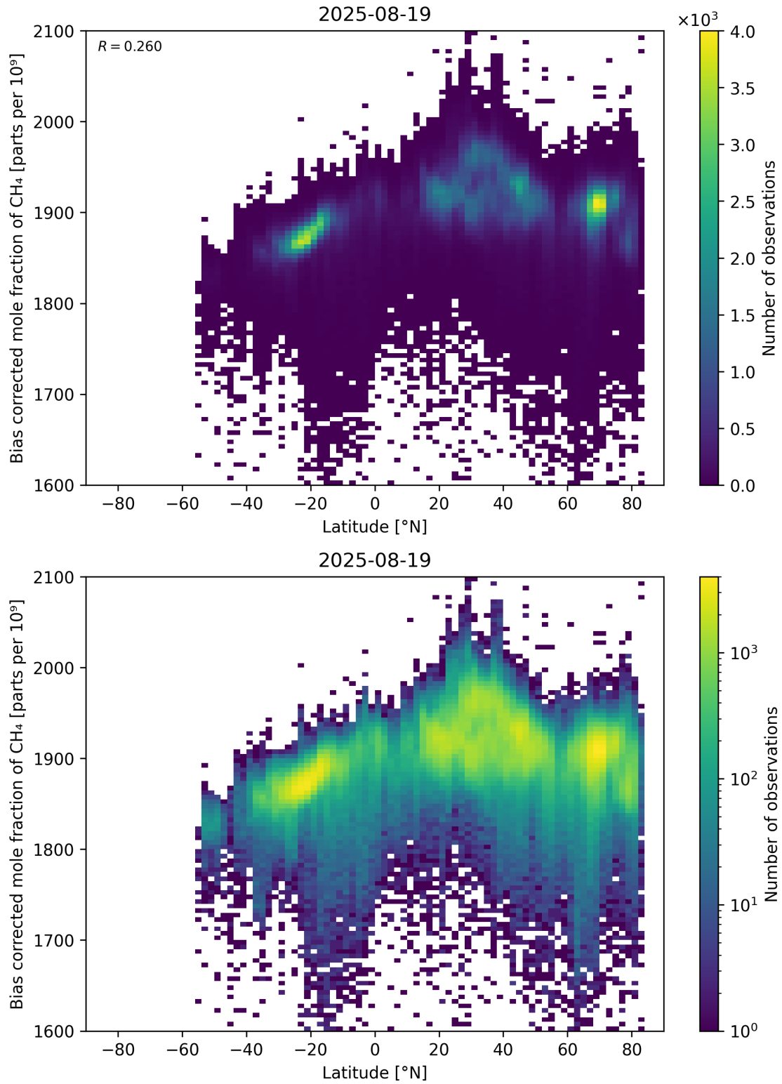
Figure 58: Scatter density plot of “Latitude” against “Bias corrected mole fraction of CH 4 ” for 2025-08-19 to 2025-08-20.
