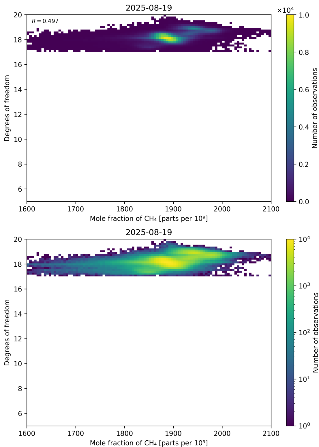
Figure 72: Scatter density plot of “Mole fraction of CH 4 ” against “Degrees of freedom” for 2025-08-19 to 2025-08-20.
