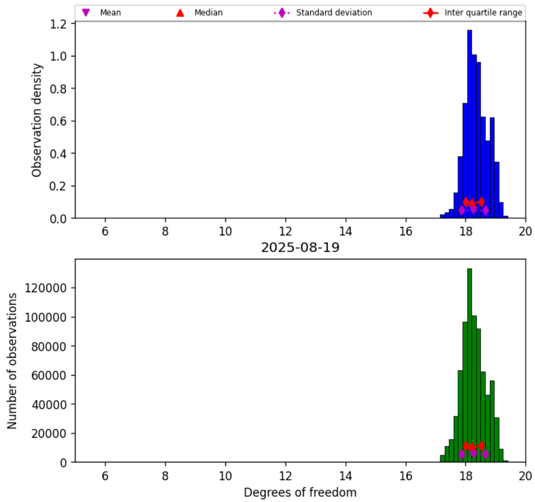
Figure 30: Histogram of “Degrees of freedom” for 2025-08-19 to 2025-08-20
