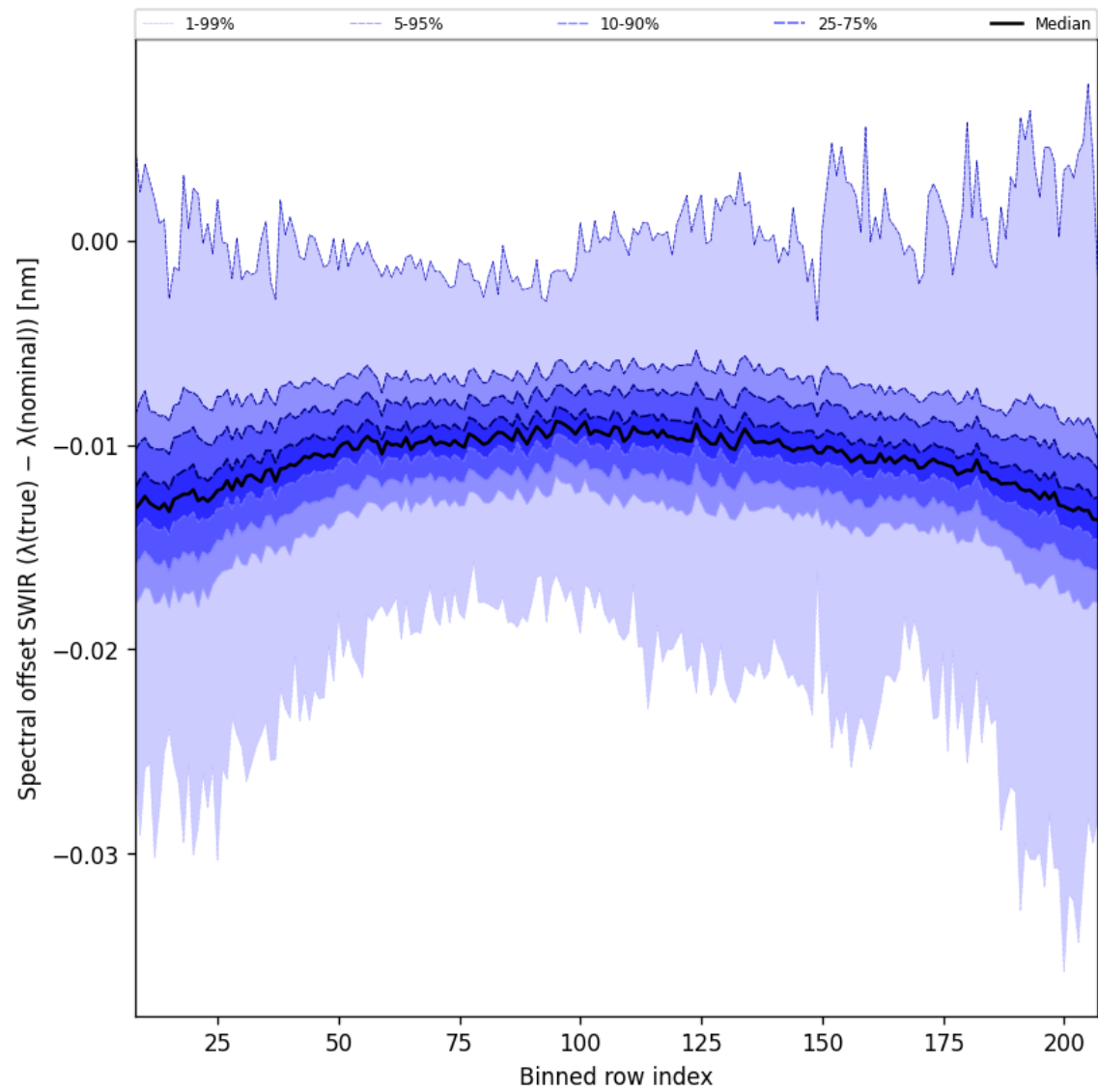
Figure 38: Along track statistics of “Spectral offset SWIR ( \lambda_{\text{true}} - \lambda_{\text{nominal}} )” for 2025-08-19 to 2025-08-20
