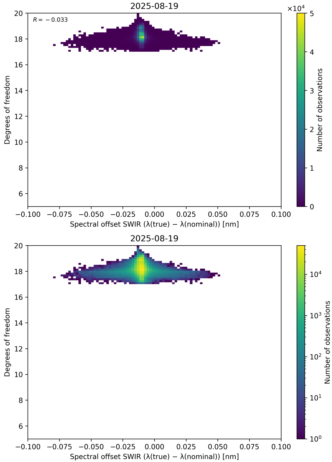
Figure 119: Scatter density plot of “Spectral offset SWIR ( \lambda_{\text{true}} - \lambda_{\text{nominal}} )” against “Degrees of freedom” for 2025-08-19 to 2025-08-20.
