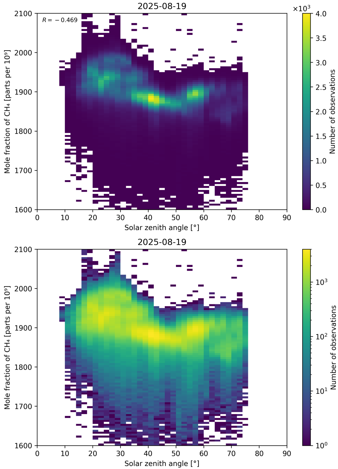
Figure 99: Scatter density plot of “Solar zenith angle” against “Mole fraction of CH 4 ” for 2025-08-19 to 2025-08-20.
