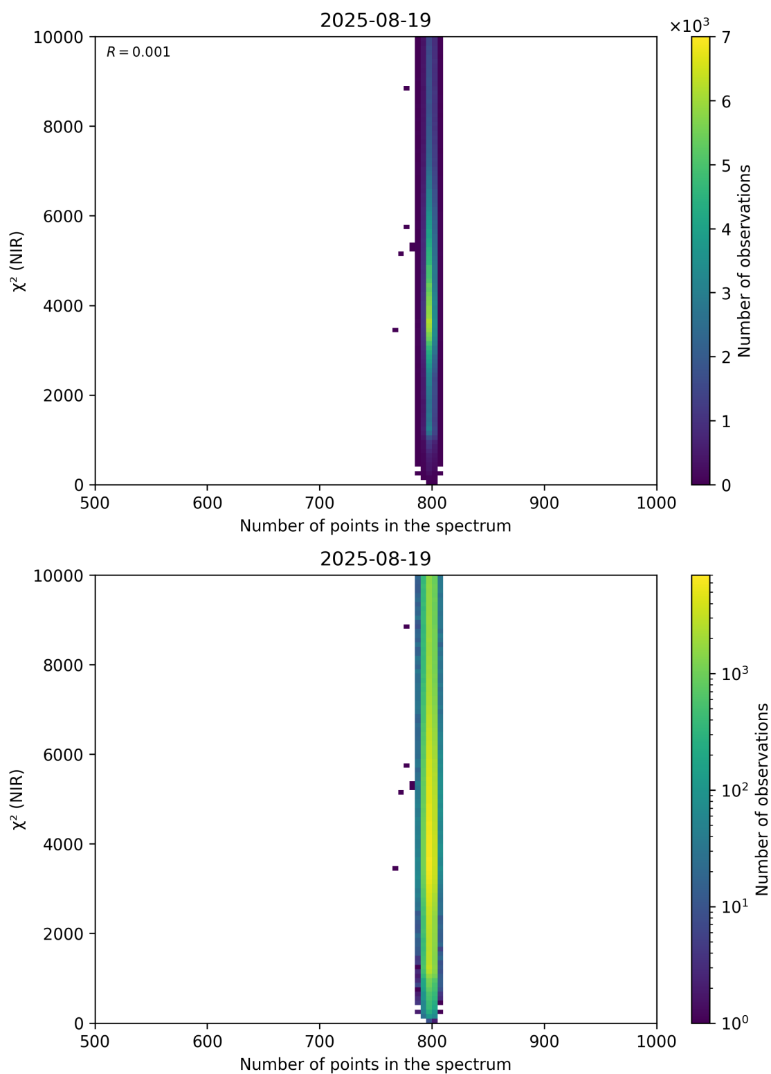
Figure 88: Scatter density plot of “Number of points in the spectrum” against “ \chi^2 (NIR)” for 2025-08-19 to 2025-08-20.
