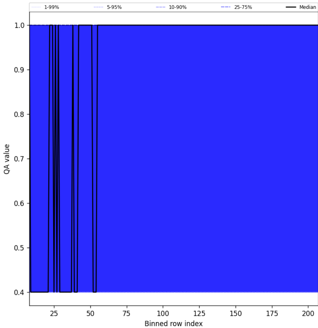
Figure 33: Along track statistics of “QA value” for 2025-08-19 to 2025-08-20
