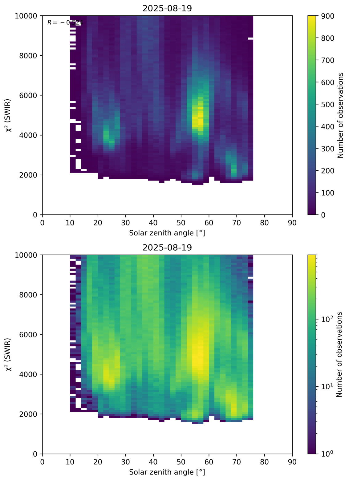
Figure 95: Scatter density plot of “Solar zenith angle” against “ \chi^2 (SWIR)” for 2025-08-19 to 2025-08-20.
