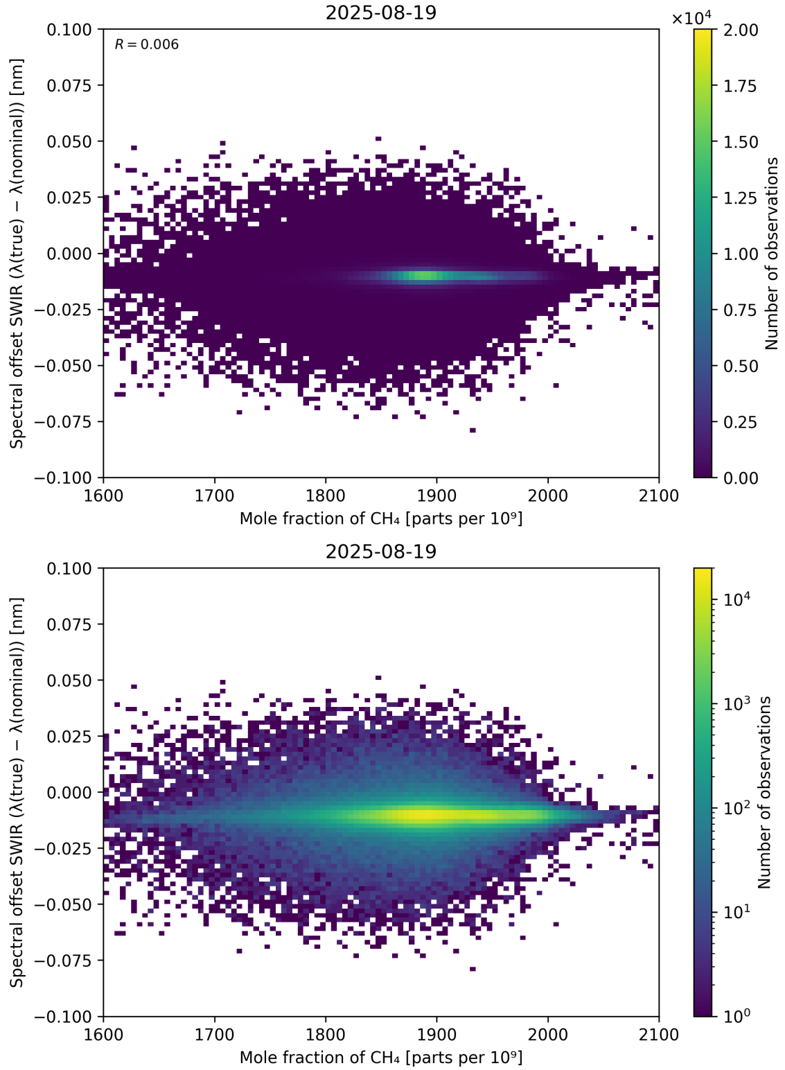
Figure 86: Scatter density plot of “Mole fraction of \text{CH}_4 ” against “Spectral offset SWIR ( \lambda_{\text{true}} - \lambda_{\text{nominal}} )” for 2025-08-19 to 2025-08-20.
