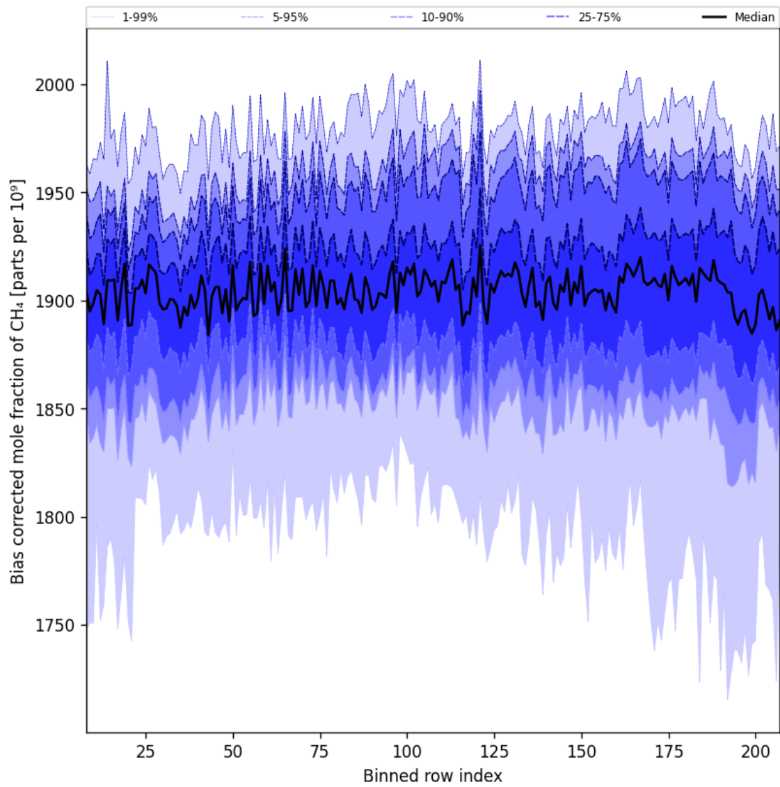
Figure 36: Along track statistics of “Bias corrected mole fraction of CH 4 ” for 2025-08-19 to 2025-08-20
