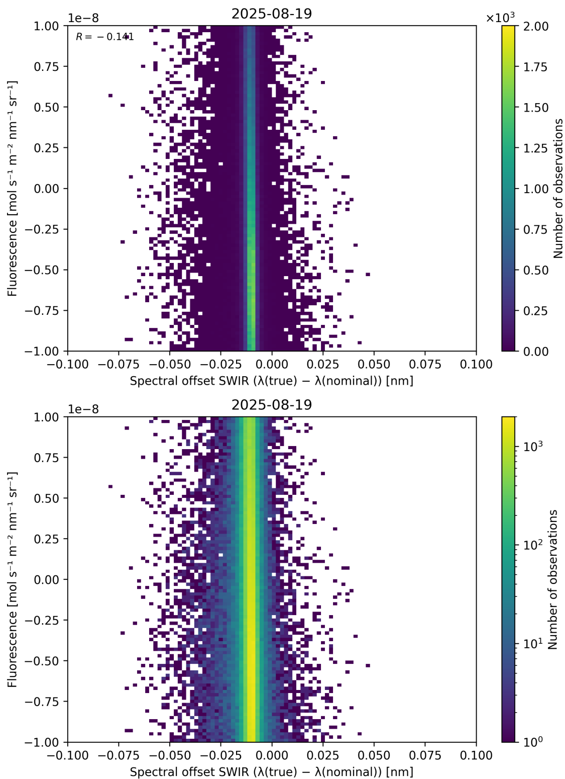
Figure 120: Scatter density plot of “Spectral offset SWIR ( \lambda_{\text{true}} - \lambda_{\text{nominal}} )” against “Fluorescence” for 2025-08-19 to 2025-08-20.
