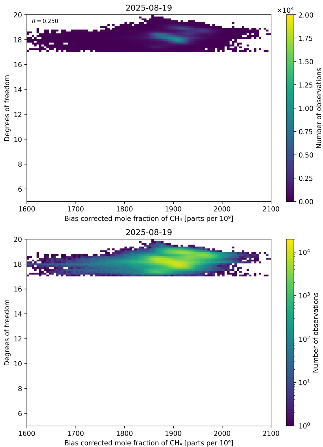
Figure 65: Scatter density plot of “Bias corrected mole fraction of CH 4 ” against “Degrees of freedom” for 2025-08-19 to 2025-08-20.
