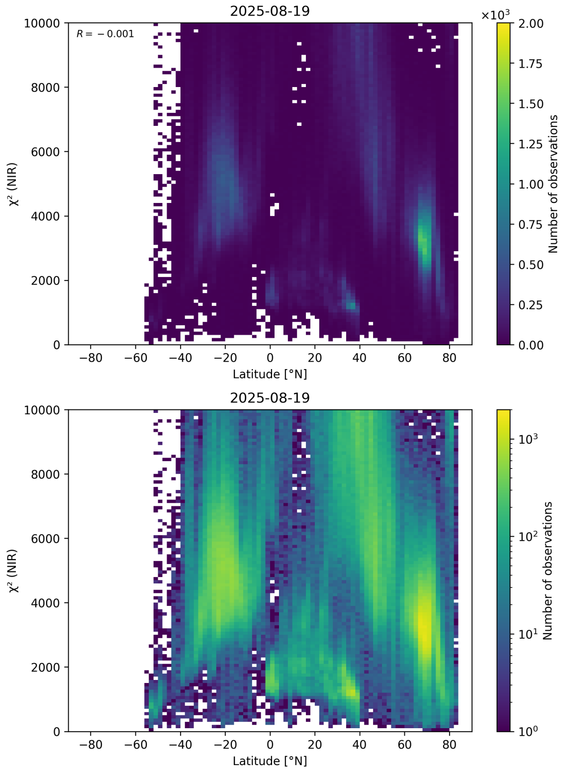
Figure 53: Scatter density plot of “Latitude” against “ \chi^2 (NIR)” for 2025-08-19 to 2025-08-20.
