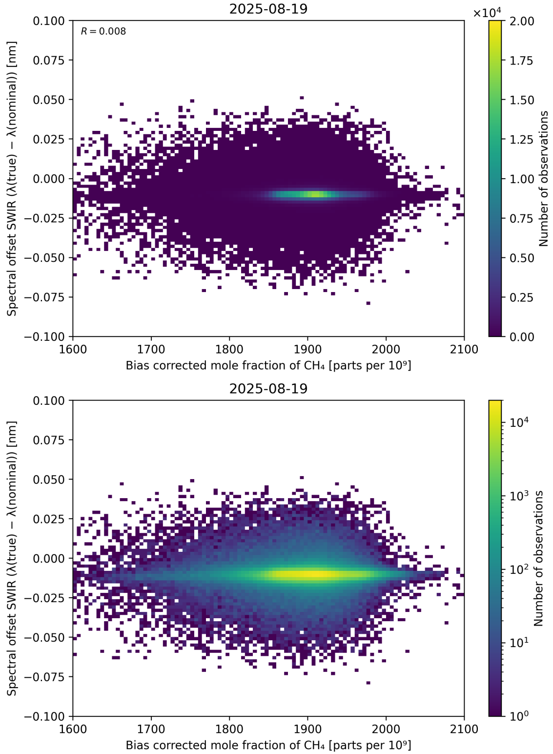
Figure 69: Scatter density plot of “Bias corrected mole fraction of CH 4 ” against “Spectral offset SWIR ( \lambda_{\text{true}} - \lambda_{\text{nominal}} )” for 2025-08-19 to 2025-08-20.
