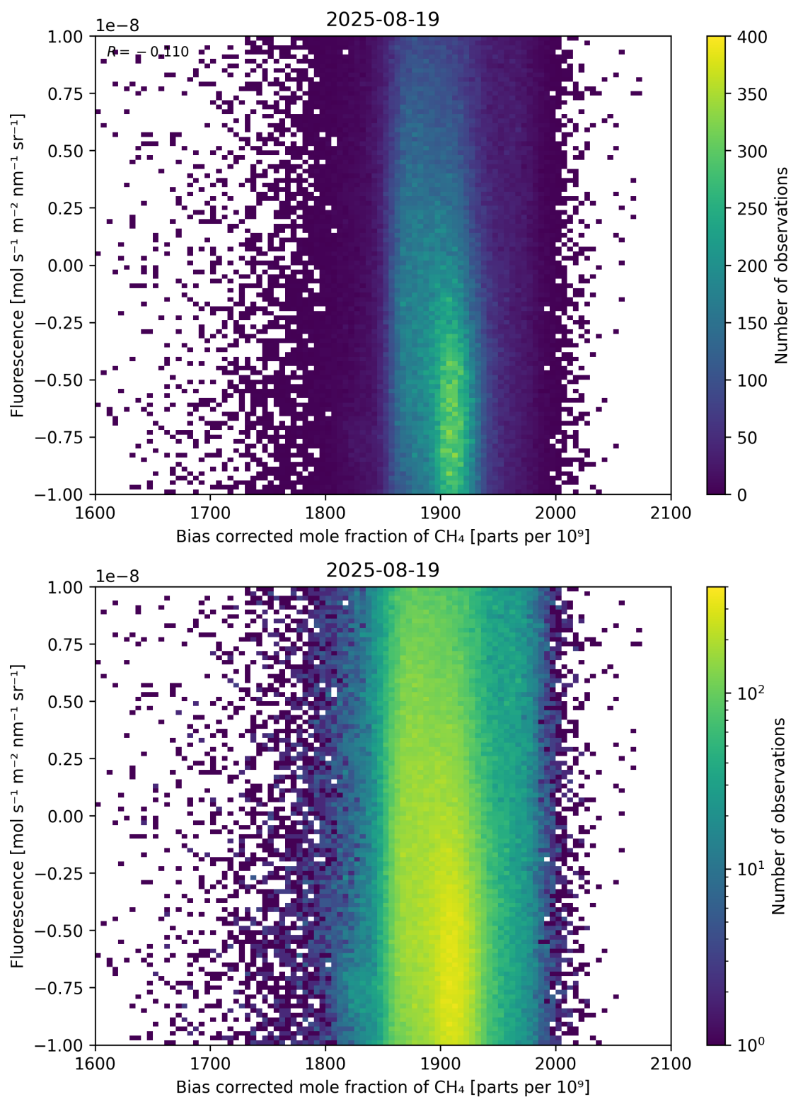
Figure 66: Scatter density plot of “Bias corrected mole fraction of \text{CH}_4 ” against “Fluorescence” for 2025-08-19 to 2025-08-20.
