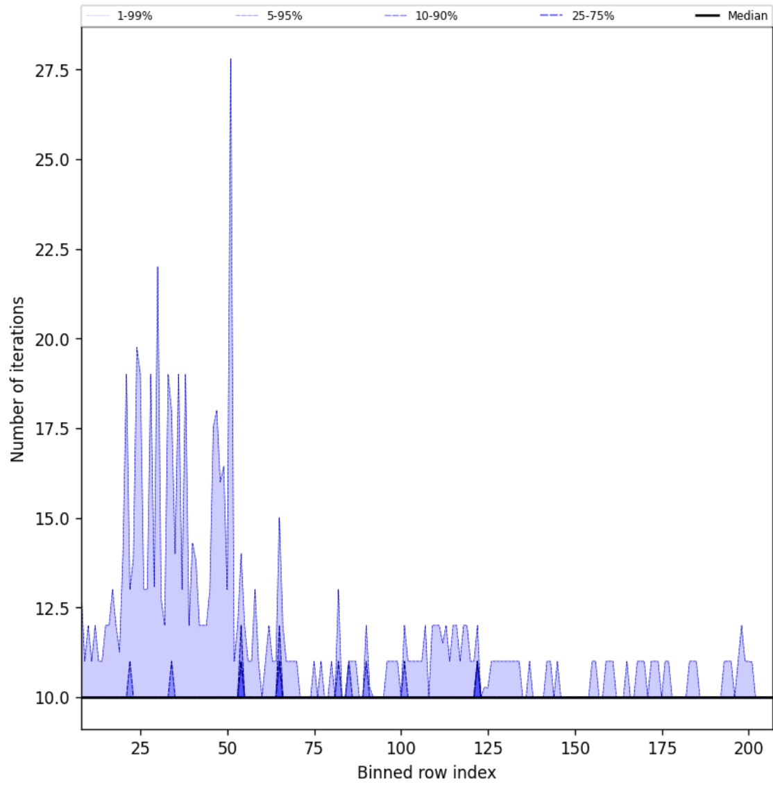
Figure 42: Along track statistics of “Number of iterations” for 2025-08-19 to 2025-08-20
