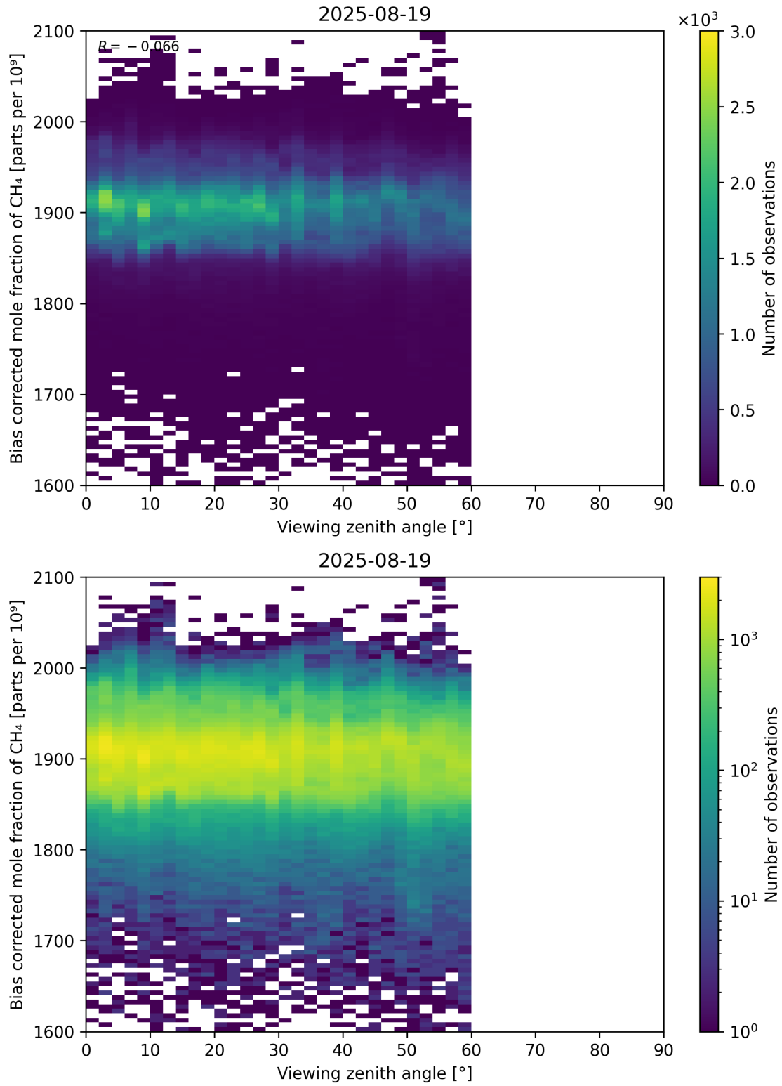
Figure 111: Scatter density plot of “Viewing zenith angle” against “Bias corrected mole fraction of CH 4 ” for 2025-08-19 to 2025-08-20.
