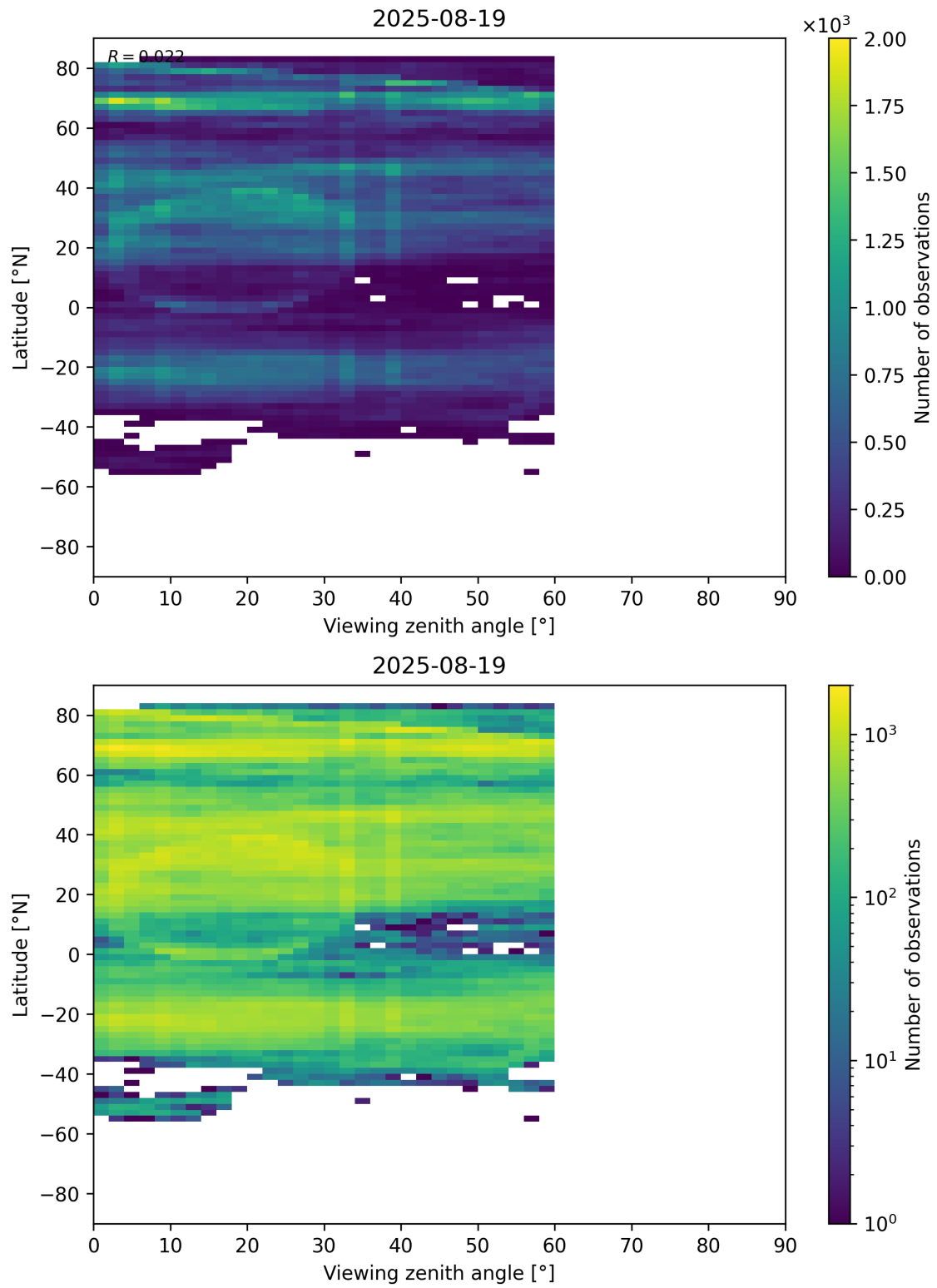
Figure 109: Scatter density plot of “Viewing zenith angle” against “Latitude” for 2025-08-19 to 2025-08-20.
