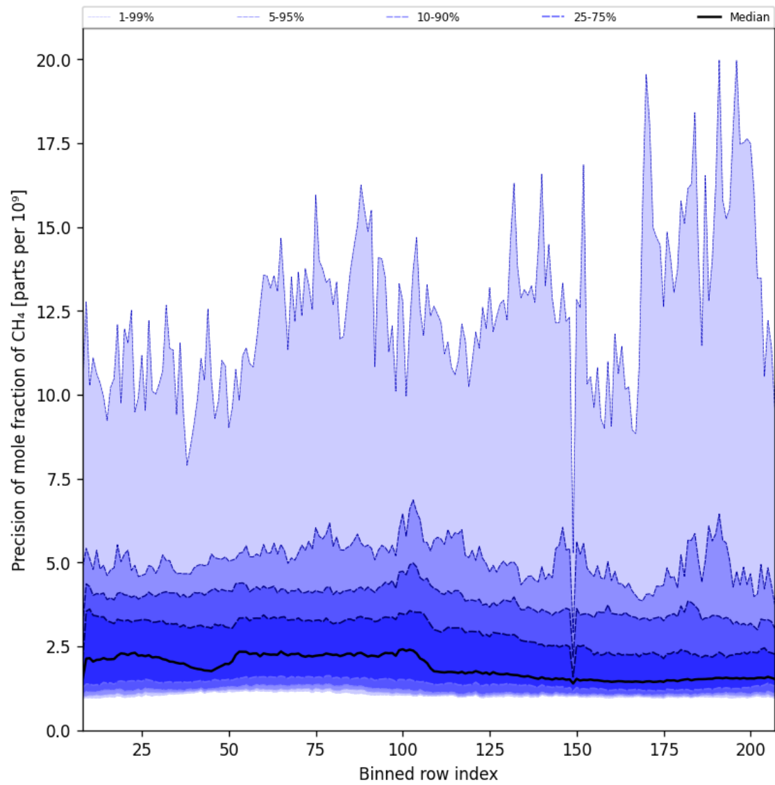
Figure 35: Along track statistics of “Precision of mole fraction of CH 4 ” for 2025-08-19 to 2025-08-20
