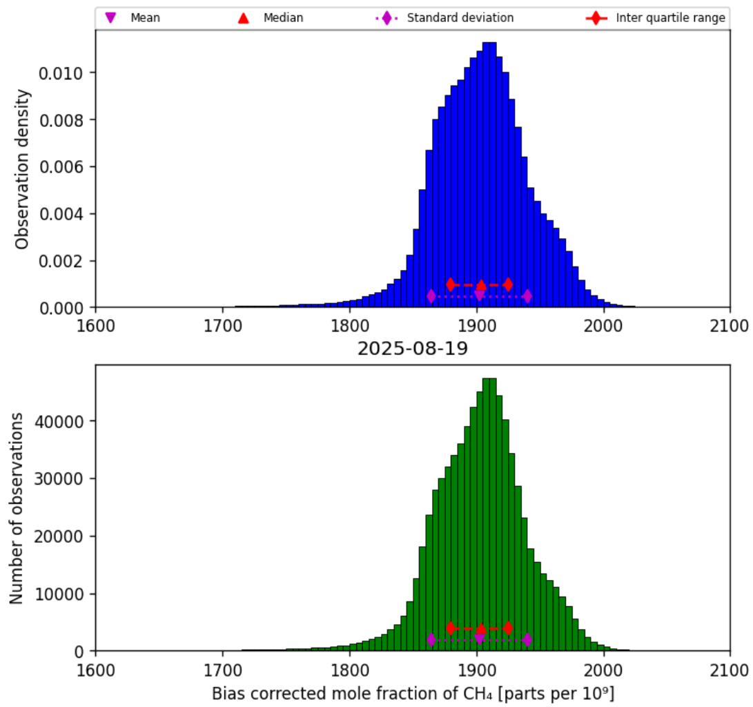
Figure 25: Histogram of “Bias corrected mole fraction of CH 4 ” for 2025-08-19 to 2025-08-20
