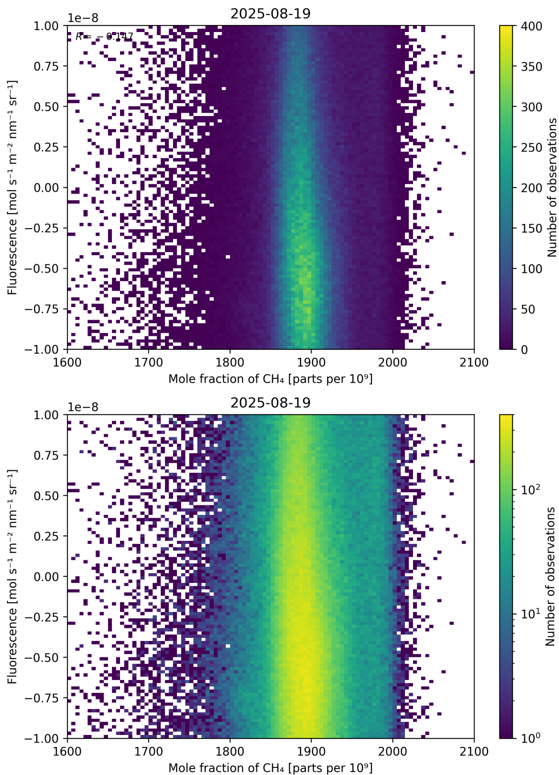
Figure 73: Scatter density plot of “Mole fraction of \text{CH}_4 ” against “Fluorescence” for 2025-08-19 to 2025-08-20.
