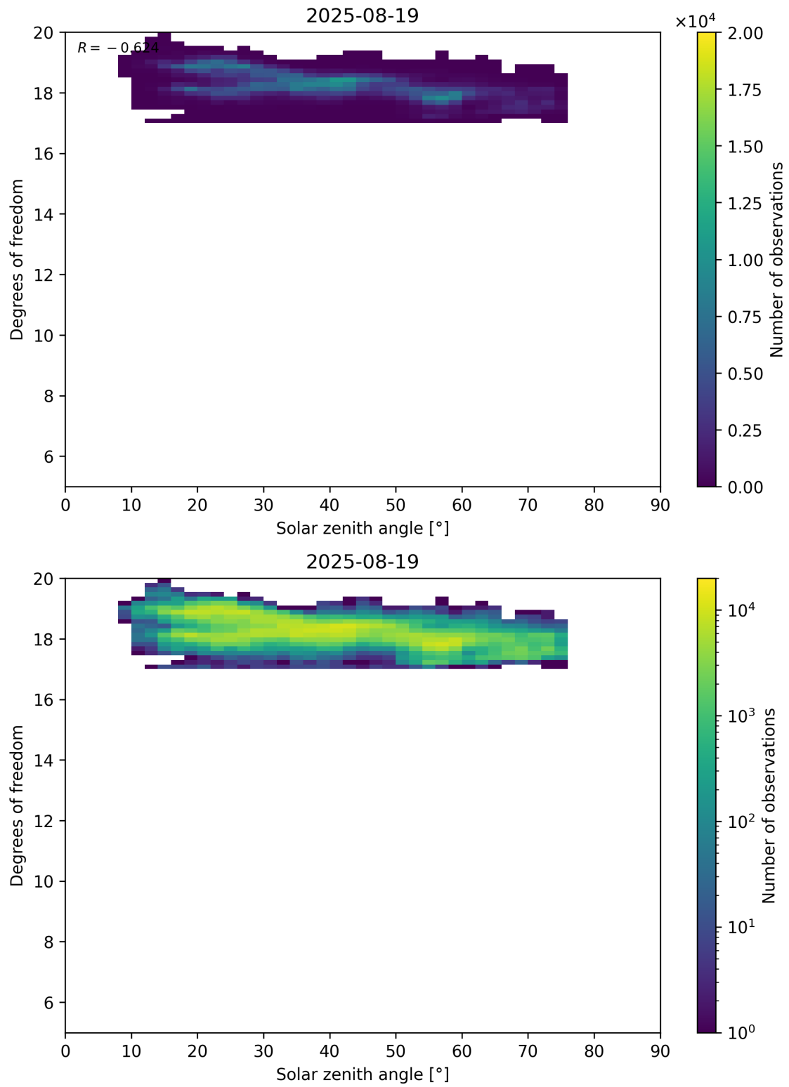
Figure 96: Scatter density plot of “Solar zenith angle” against “Degrees of freedom” for 2025-08-19 to 2025-08-20.
