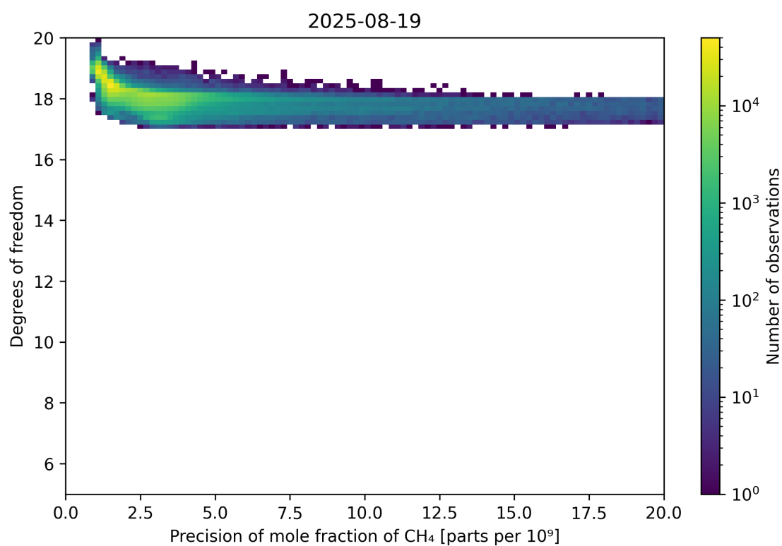
Figure 80: Scatter density plot of “Precision of mole fraction of CH 4 ” against “Degrees of freedom” for 2025-08-19 to 2025-08-20.
