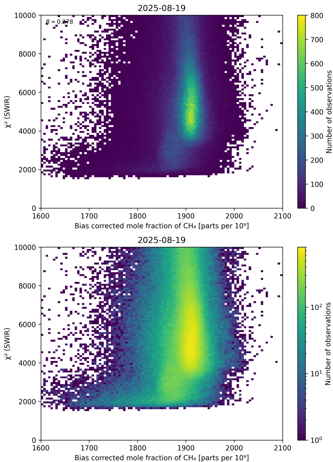
Figure 64: Scatter density plot of “Bias corrected mole fraction of \text{CH}_4 ” against “ \chi^2 (SWIR)” for 2025-08-19 to 2025-08-20.
