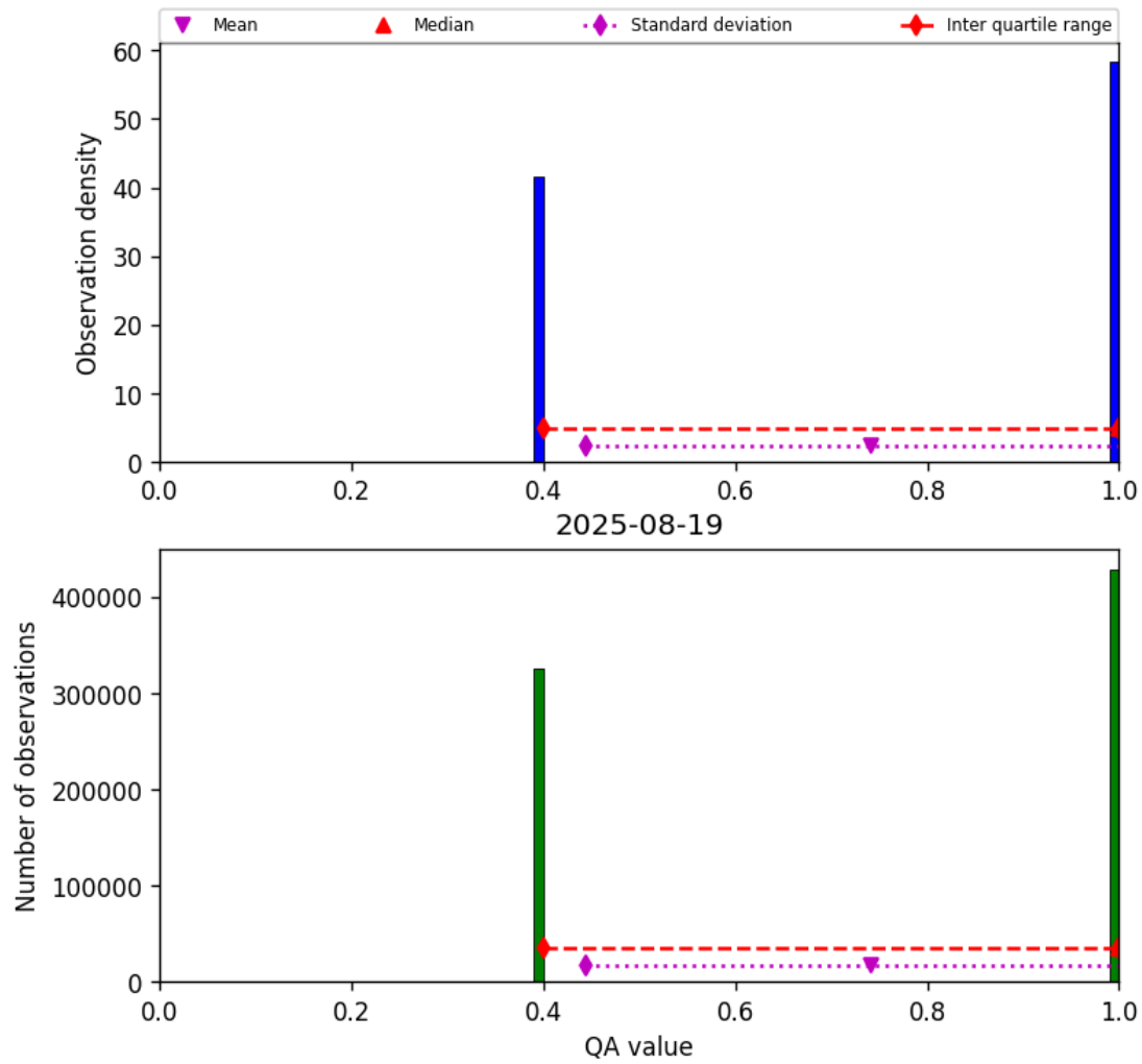
Figure 22: Histogram of “QA value” for 2025-08-19 to 2025-08-20
