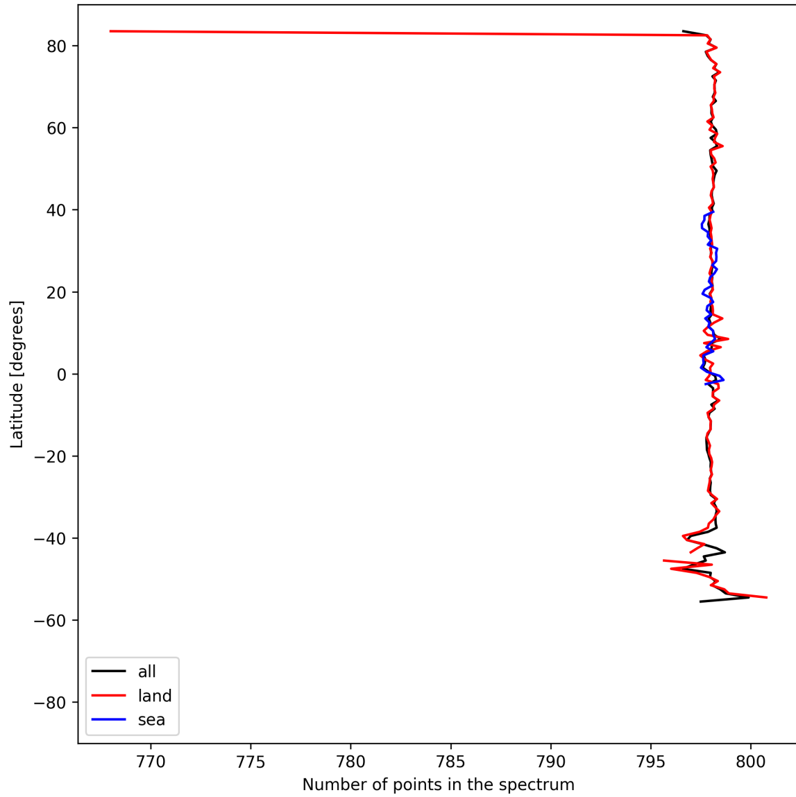
Figure 15: Zonal average of “Number of points in the spectrum” for 2025-08-19 to 2025-08-20.
