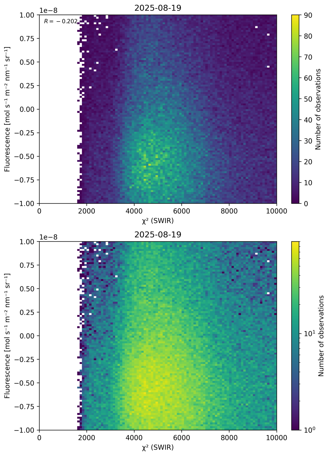
Figure 49: Scatter density plot of “ \chi^2 (SWIR)” against “Fluorescence” for 2025-08-19 to 2025-08-20.
