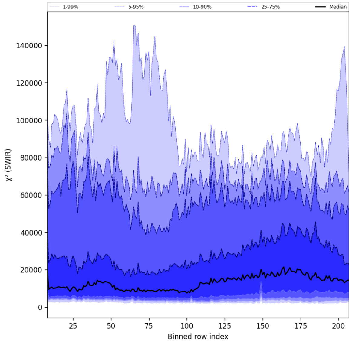
Figure 39: Along track statistics of “ \chi^2 (SWIR)” for 2025-08-19 to 2025-08-20
