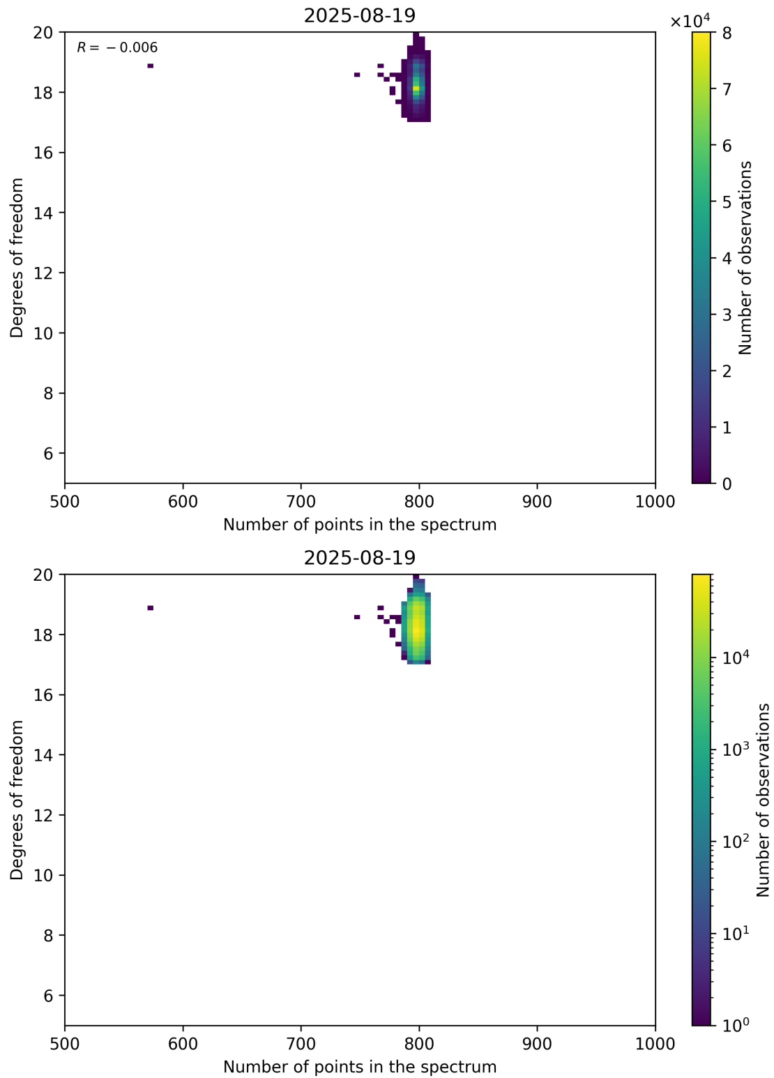
Figure 90: Scatter density plot of “Number of points in the spectrum” against “Degrees of freedom” for 2025-08-19 to 2025-08-20.
