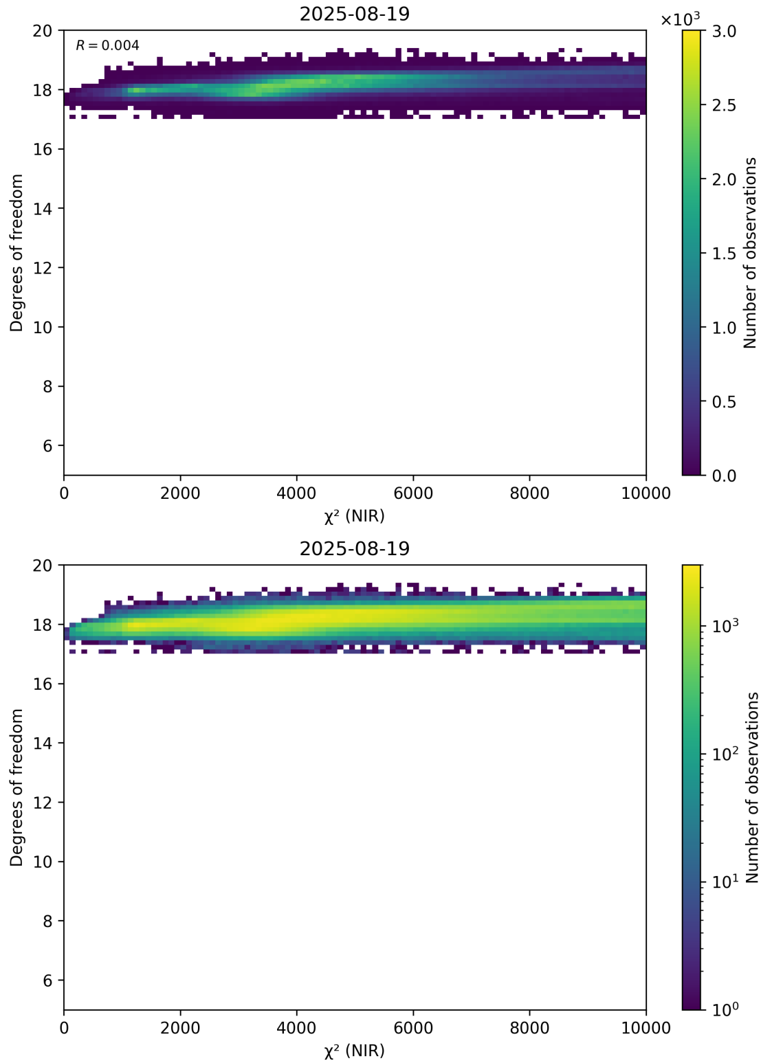
Figure 44: Scatter density plot of “ \chi^2 (NIR)” against “Degrees of freedom” for 2025-08-19 to 2025-08-20.
