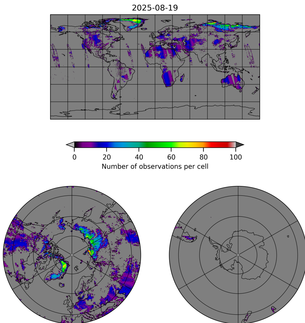
Figure 10: Map of the number of observations for 2025-08-19 to 2025-08-20
