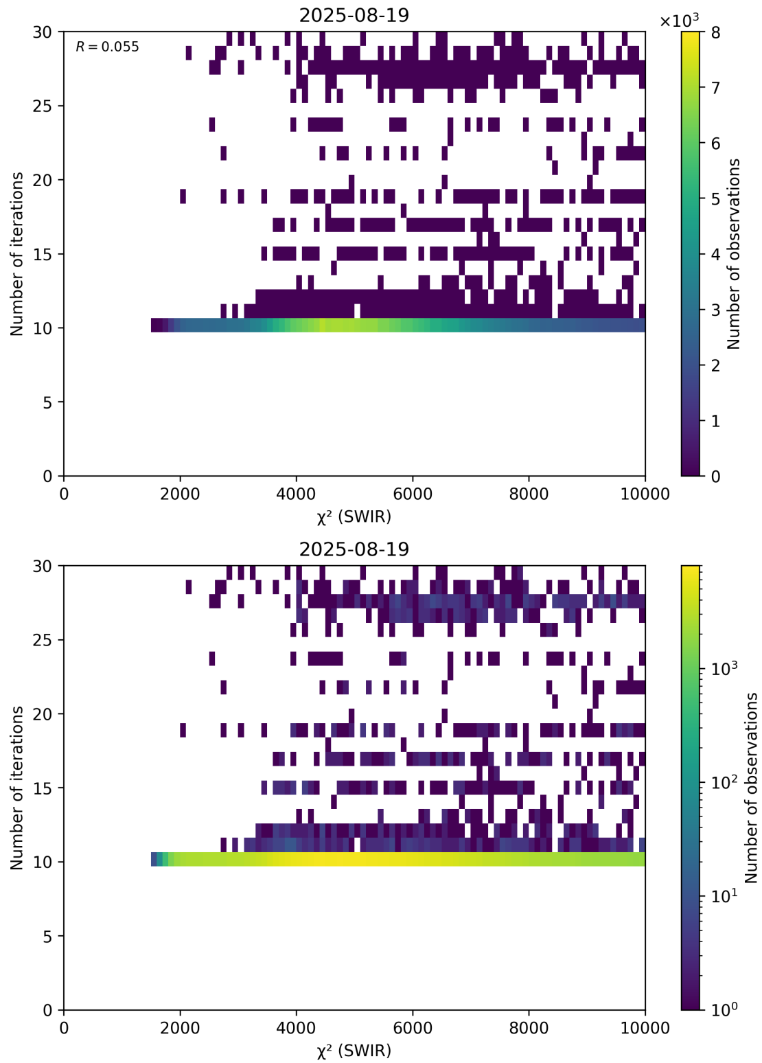
Figure 50: Scatter density plot of “ \chi^2 (SWIR)” against “Number of iterations” for 2025-08-19 to 2025-08-20.
