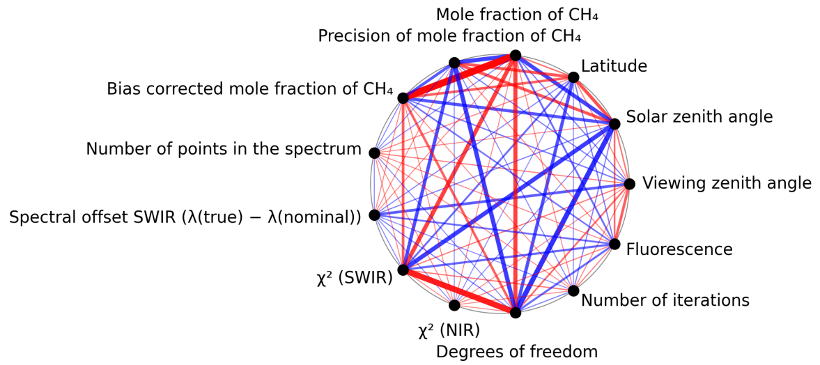
Figure 1: Map of correlation graph for 2025-08-19 to 2025-08-20.
