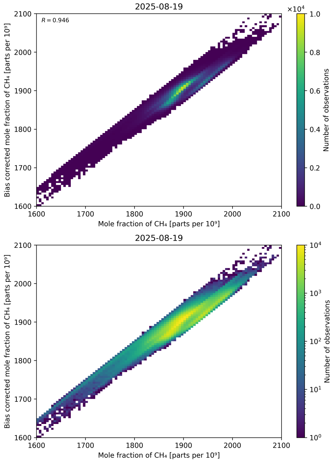
Figure 74: Scatter density plot of “Mole fraction of CH 4 ” against “Bias corrected mole fraction of CH 4 ” for 2025-08-19 to 2025-08-20.
