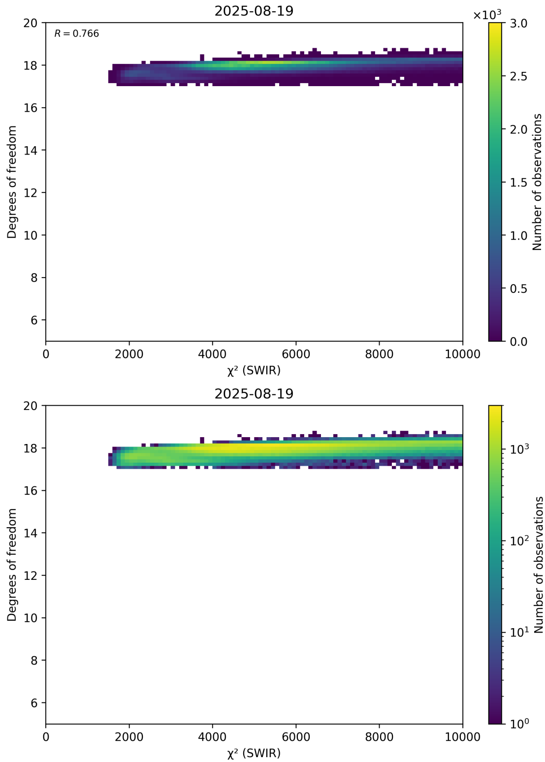
Figure 48: Scatter density plot of “ \chi^2 (SWIR)” against “Degrees of freedom” for 2025-08-19 to 2025-08-20.
