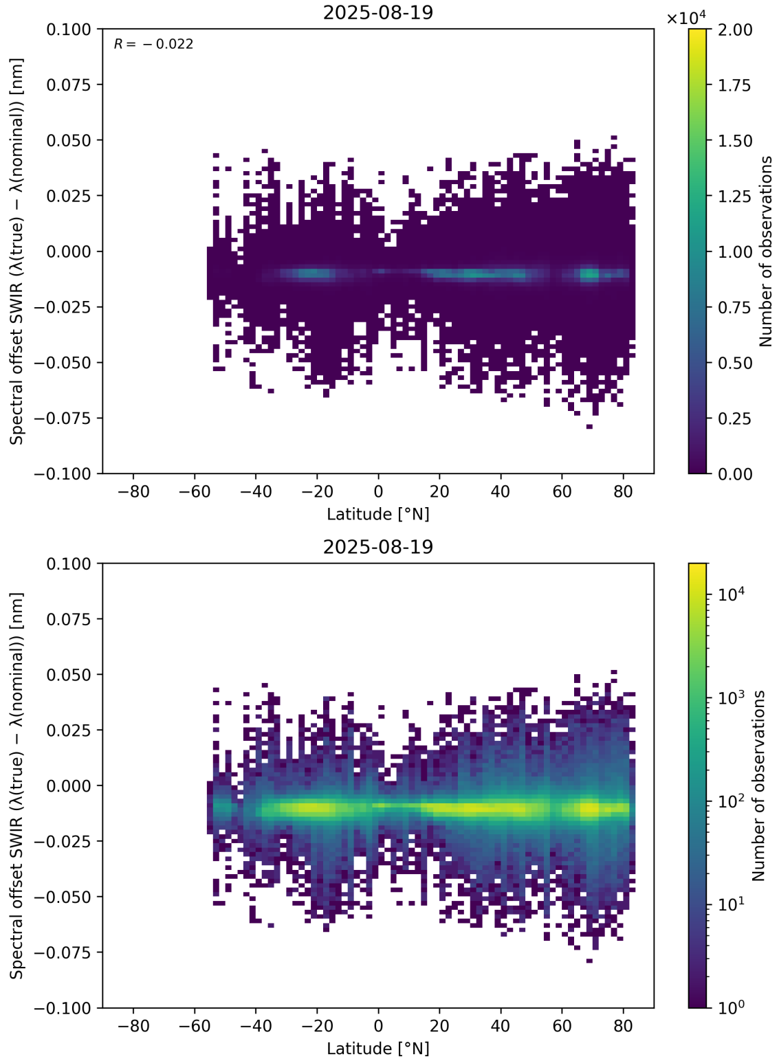
Figure 62: Scatter density plot of “Latitude” against “Spectral offset SWIR ( \lambda_{\text{true}} - \lambda_{\text{nominal}} )” for 2025-08-19 to 2025-08-20.
