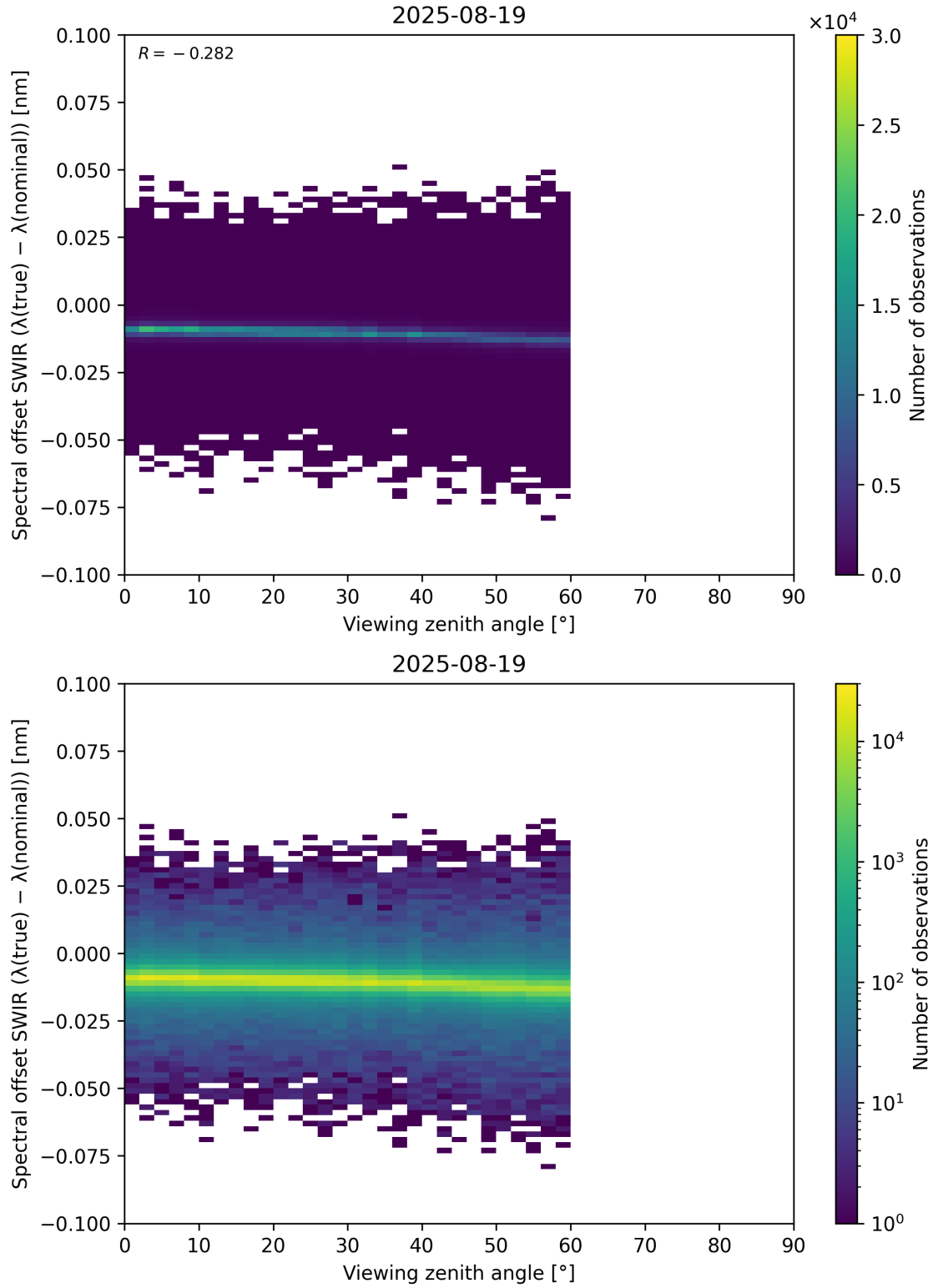
Figure 116: Scatter density plot of “Viewing zenith angle” against “Spectral offset SWIR ( \lambda_{\text{true}} - \lambda_{\text{nominal}} )” for 2025-08-19 to 2025-08-20.
