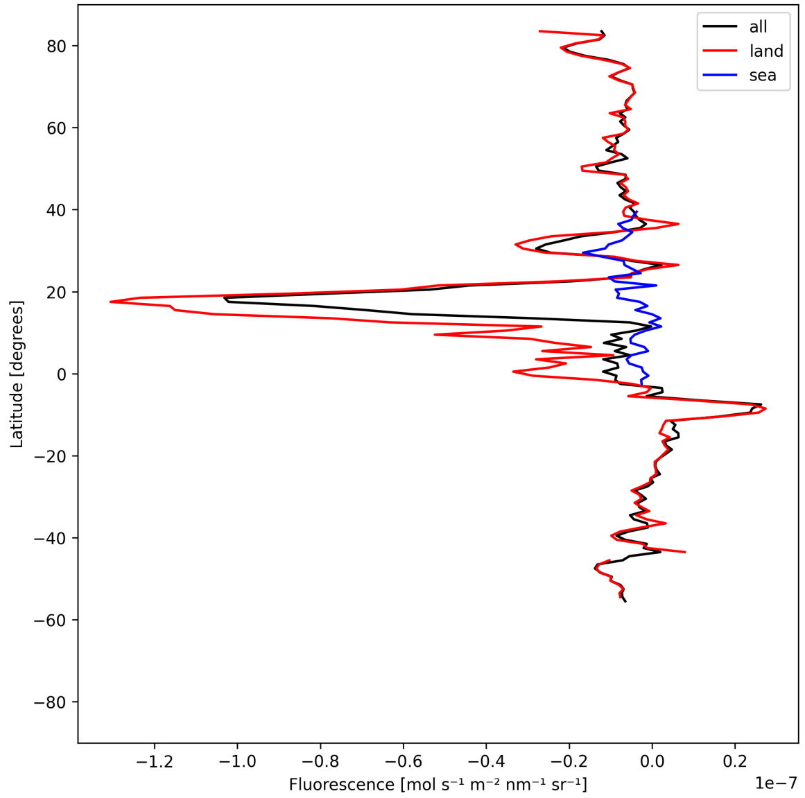
Figure 21: Zonal average of “Fluorescence” for 2025-08-19 to 2025-08-20.
