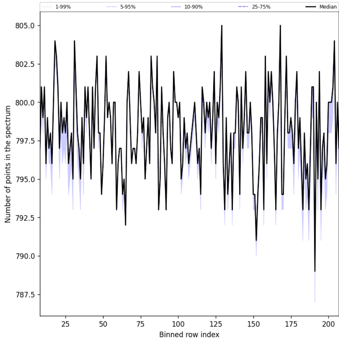
Figure 37: Along track statistics of “Number of points in the spectrum” for 2025-08-19 to 2025-08-20
