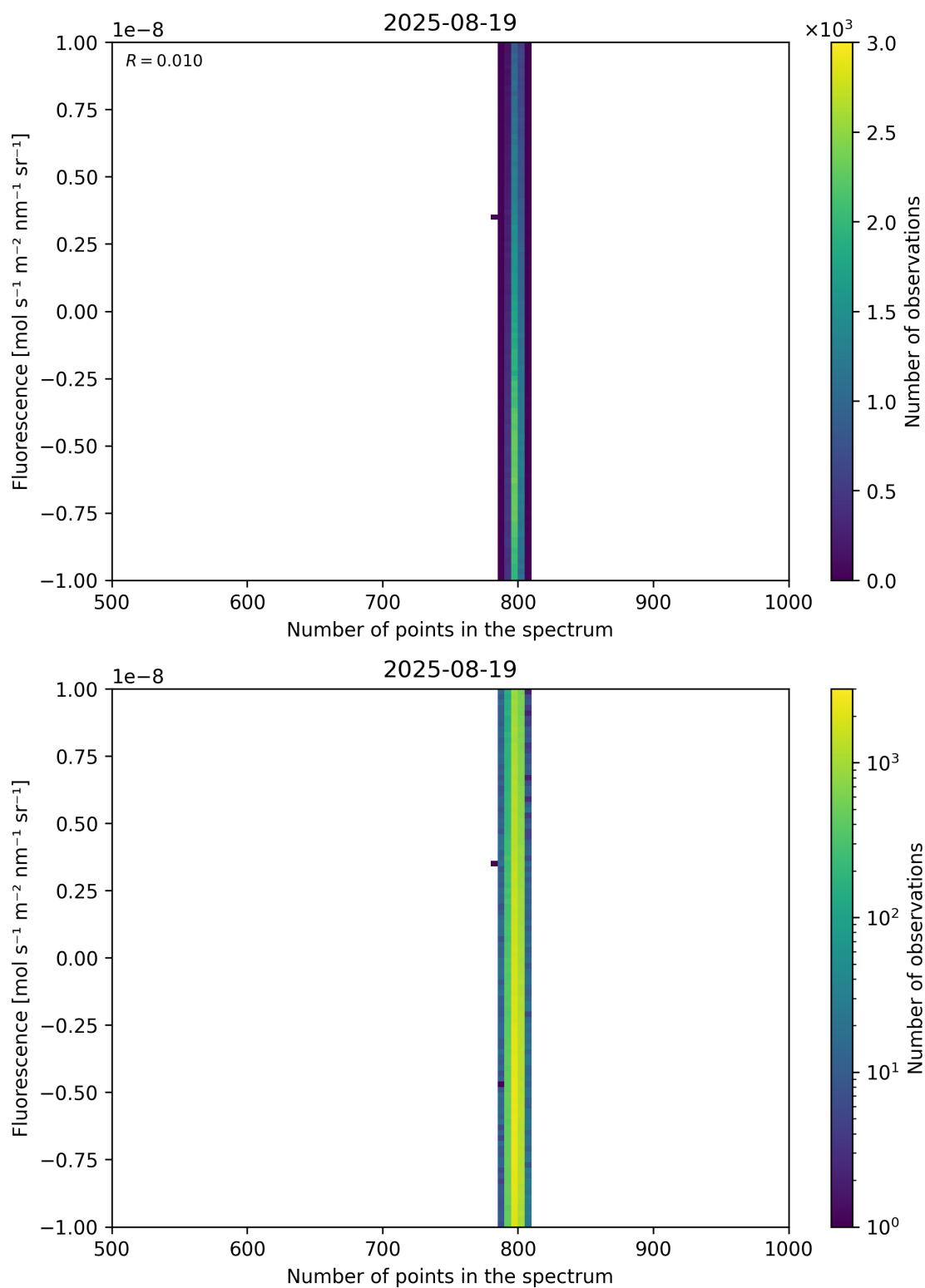
Figure 91: Scatter density plot of “Number of points in the spectrum” against “Fluorescence” for 2025-08-19 to 2025-08-20.
