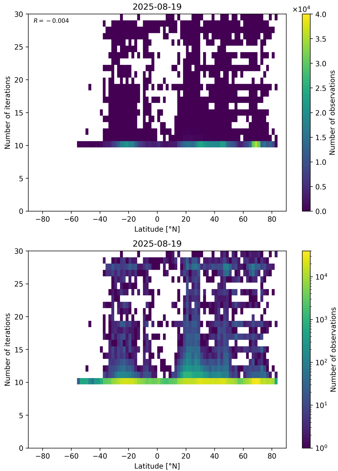
Figure 60: Scatter density plot of “Latitude” against “Number of iterations” for 2025-08-19 to 2025-08-20.
