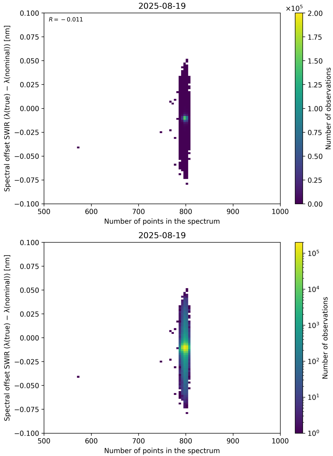
Figure 93: Scatter density plot of “Number of points in the spectrum” against “Spectral offset SWIR ( \lambda_{\text{true}} - \lambda_{\text{nominal}} )” for 2025-08-19 to 2025-08-20.
