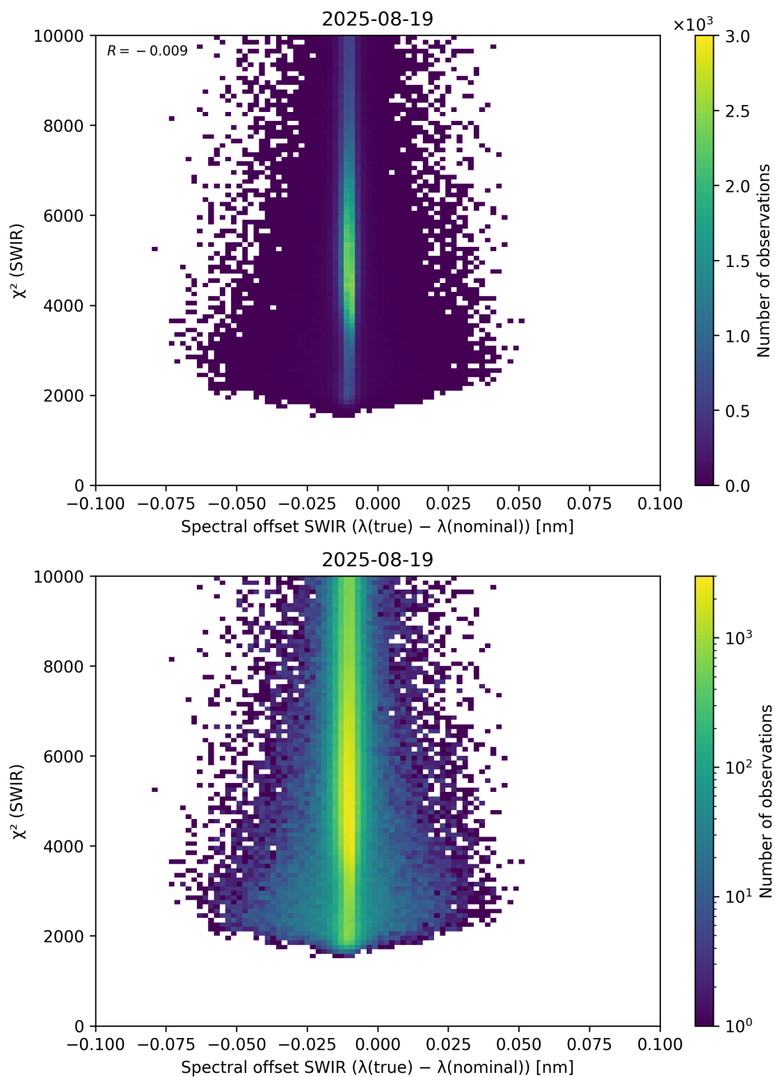
Figure 118: Scatter density plot of “Spectral offset SWIR ( \lambda_{\text{true}} - \lambda_{\text{nominal}} )” against “ \chi^2 (SWIR)” for 2025-08-19 to 2025-08-20.
