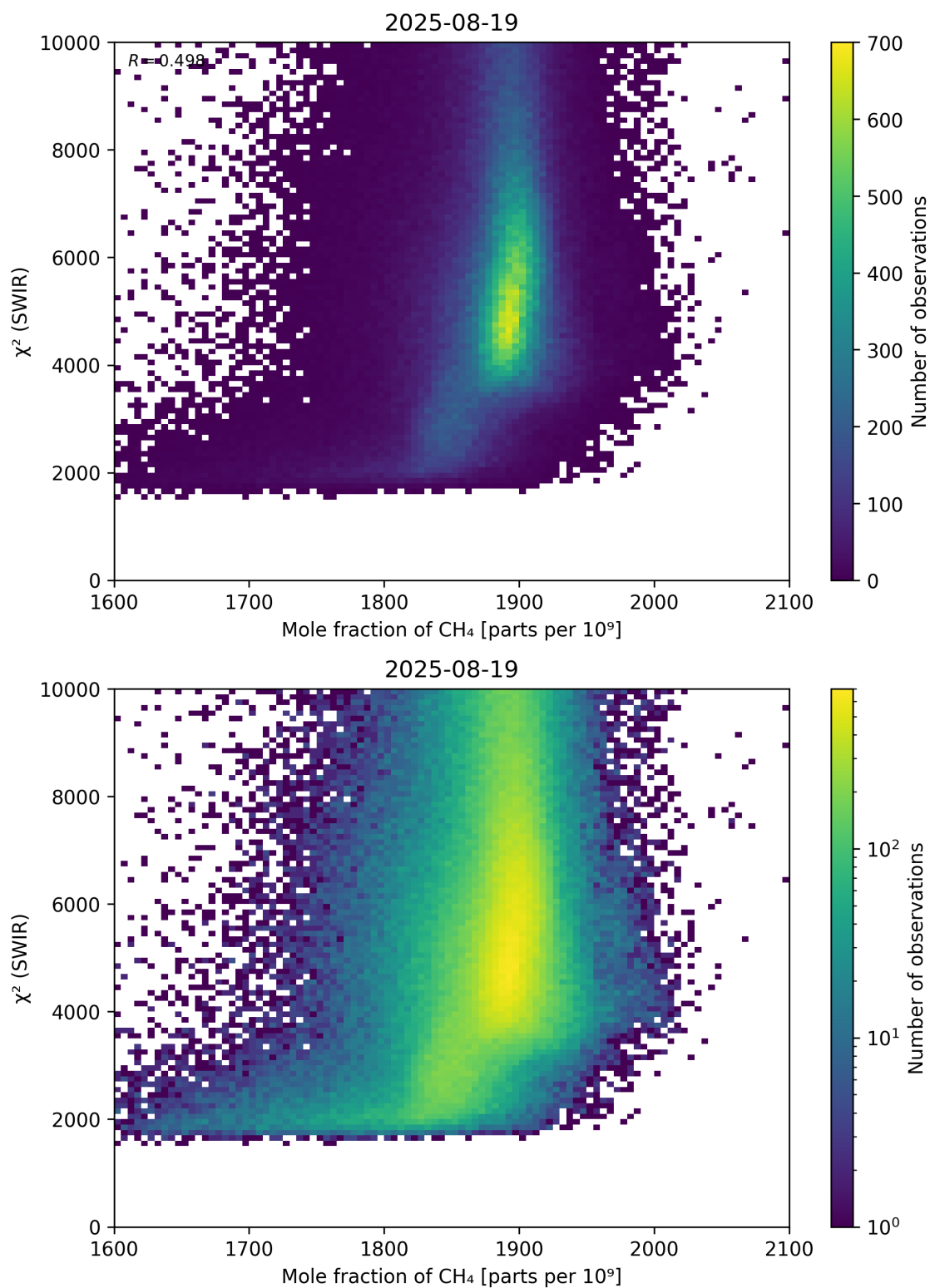
Figure 71: Scatter density plot of “Mole fraction of \text{CH}_4 ” against “ \chi^2 (SWIR)” for 2025-08-19 to 2025-08-20.
