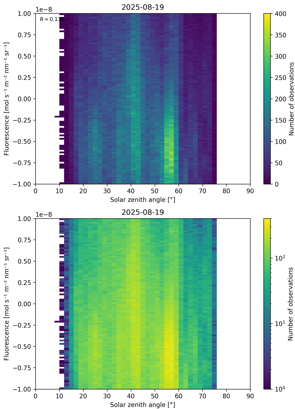
Figure 97: Scatter density plot of “Solar zenith angle” against “Fluorescence” for 2025-08-19 to 2025-08-20.
