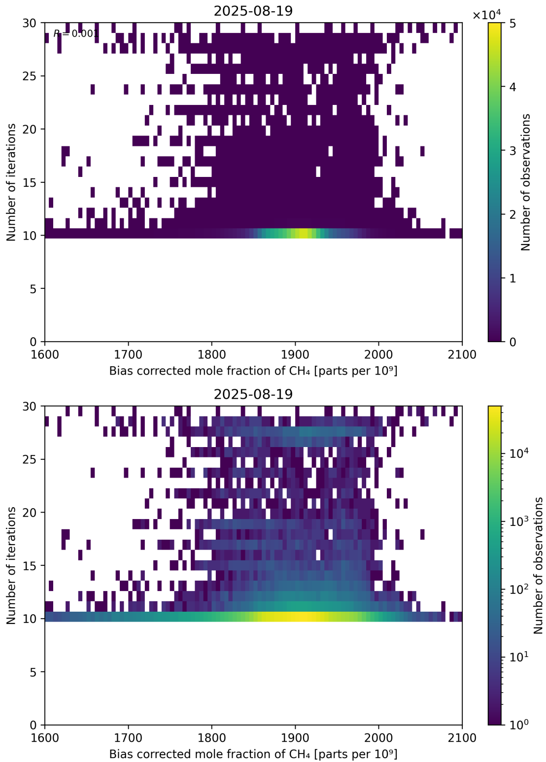
Figure 67: Scatter density plot of “Bias corrected mole fraction of CH 4 ” against “Number of iterations” for 2025-08-19 to 2025-08-20.
