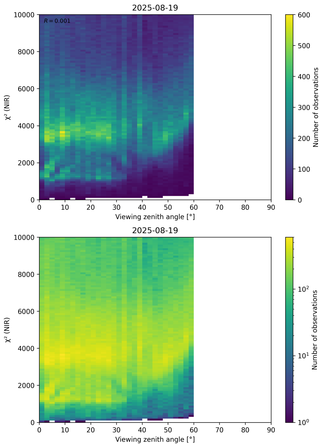
Figure 105: Scatter density plot of “Viewing zenith angle” against “ \chi^2 (NIR)” for 2025-08-19 to 2025-08-20.
