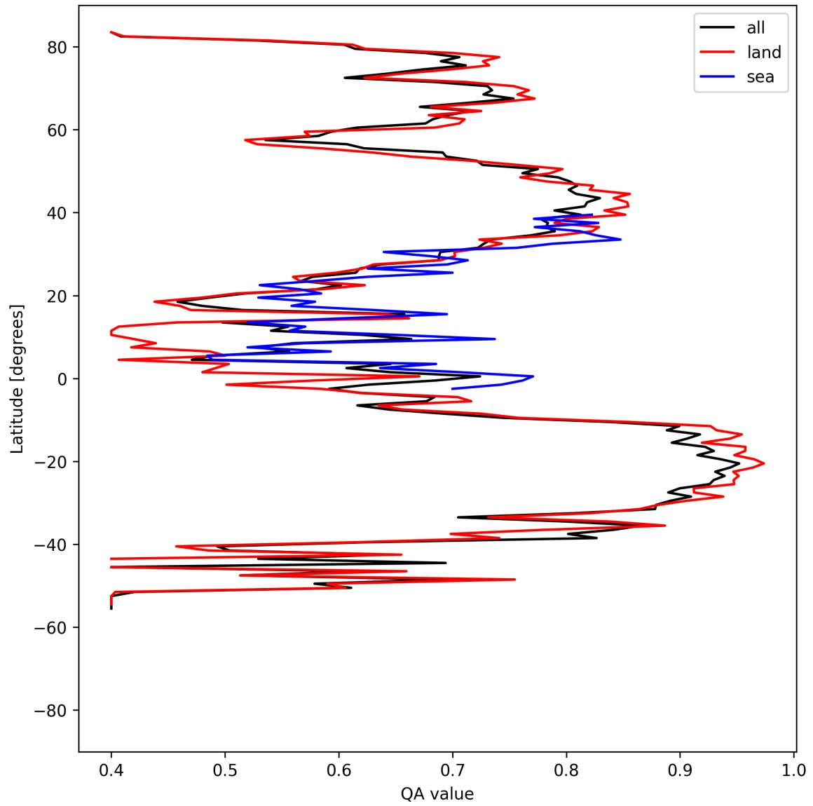
Figure 11: Zonal average of “QA value” for 2025-08-19 to 2025-08-20.
