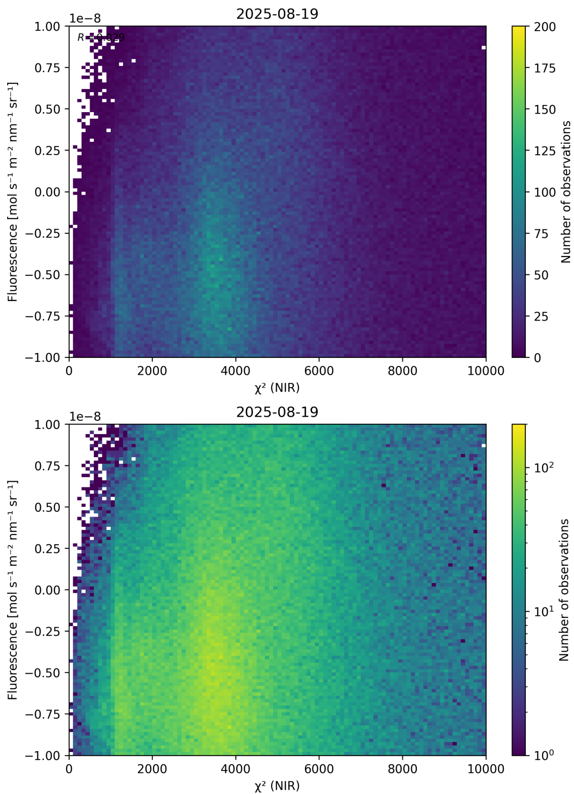
Figure 45: Scatter density plot of “ \chi^2 (NIR)” against “Fluorescence” for 2025-08-19 to 2025-08-20.
