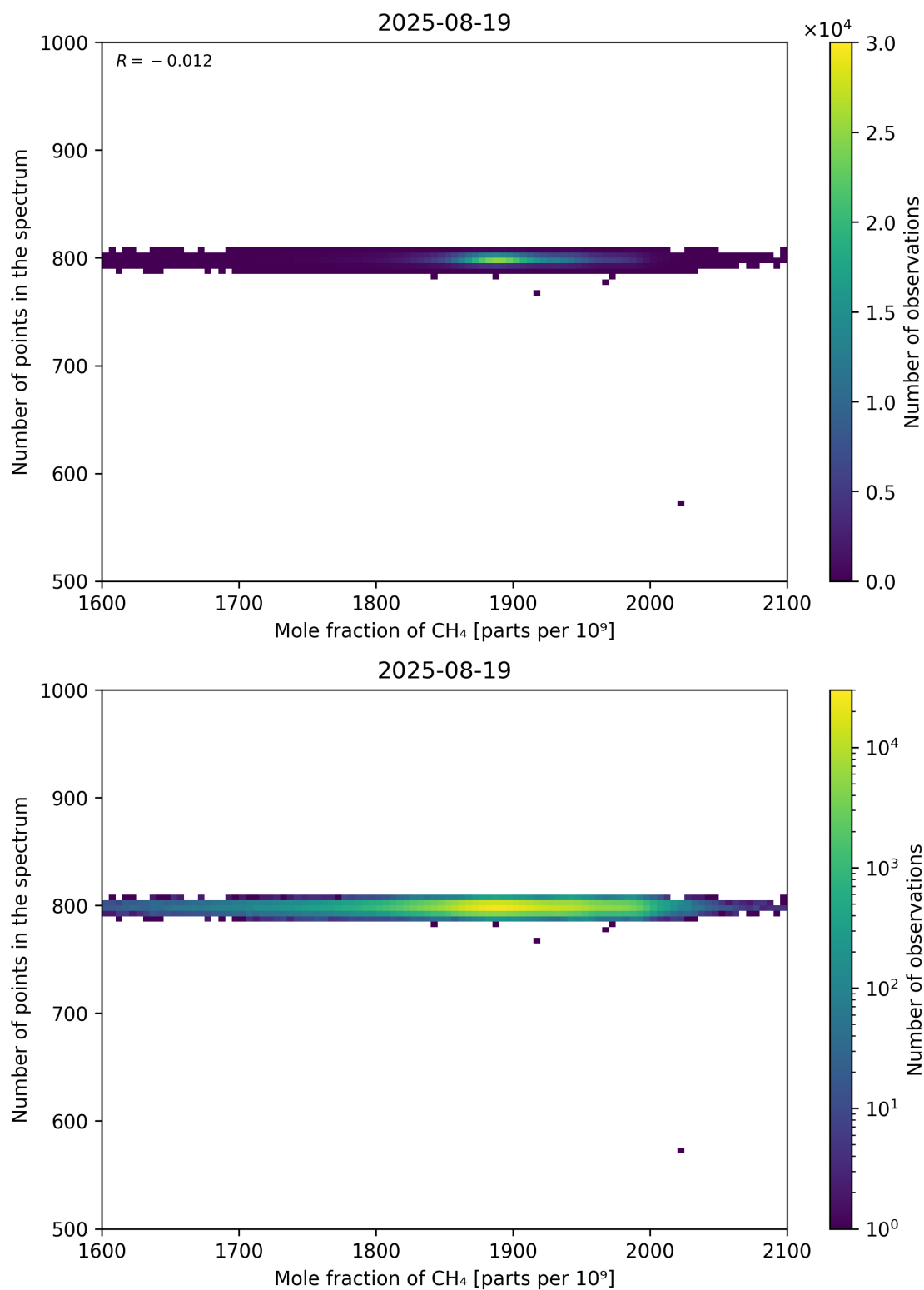
Figure 77: Scatter density plot of “Mole fraction of CH 4 ” against “Number of points in the spectrum” for 2025-08-19 to 2025-08-20.
