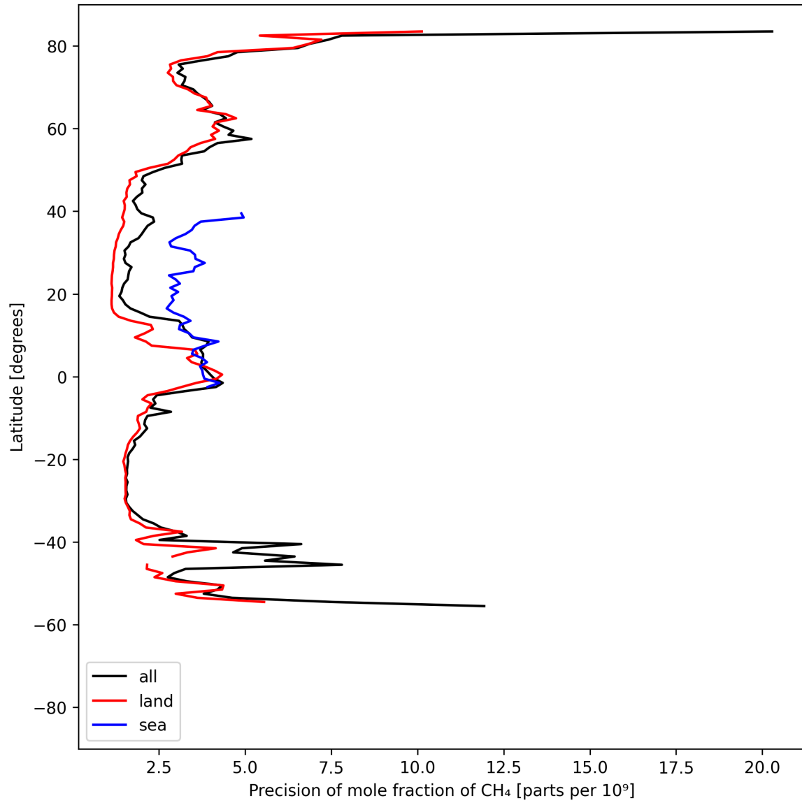
Figure 13: Zonal average of “Precision of mole fraction of CH 4 ” for 2025-08-19 to 2025-08-20.
