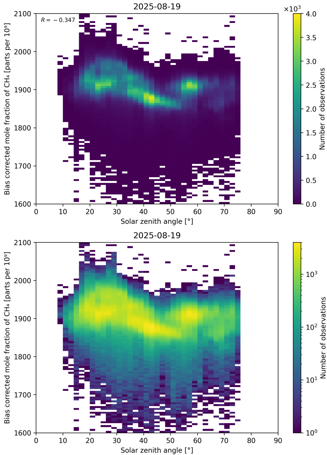
Figure 100: Scatter density plot of “Solar zenith angle” against “Bias corrected mole fraction of CH 4 ” for 2025-08-19 to 2025-08-20.
