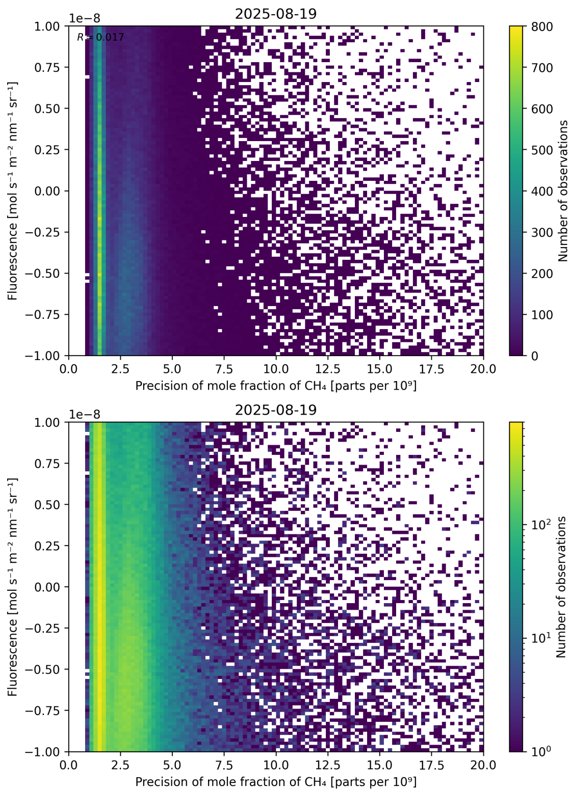
Figure 81: Scatter density plot of “Precision of mole fraction of \text{CH}_4 ” against “Fluorescence” for 2025-08-19 to 2025-08-20.
