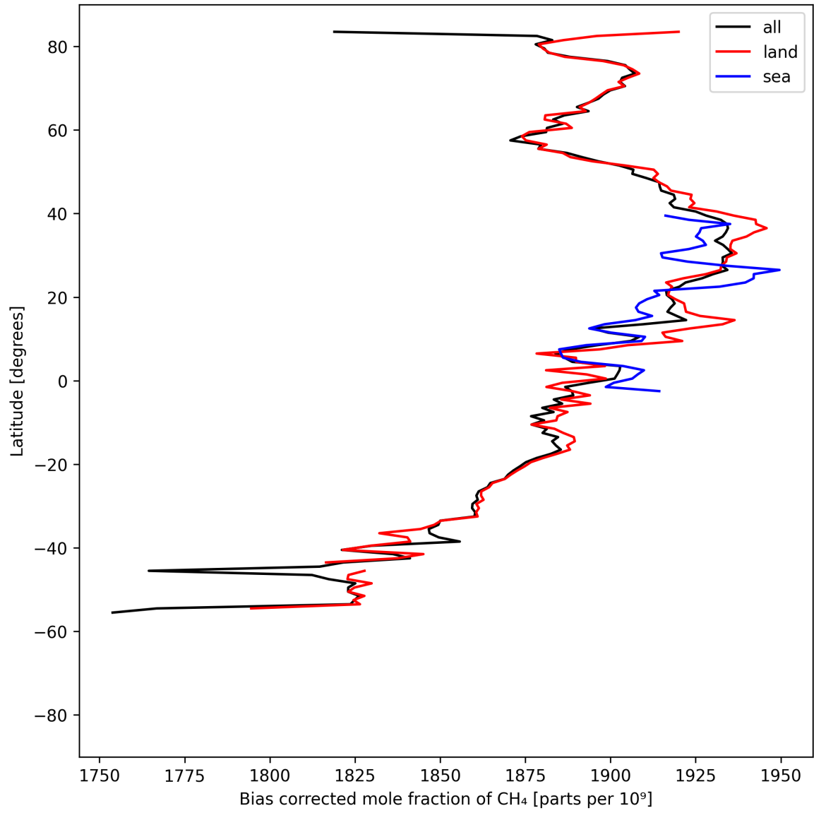
Figure 14: Zonal average of “Bias corrected mole fraction of CH 4 ” for 2025-08-19 to 2025-08-20.
