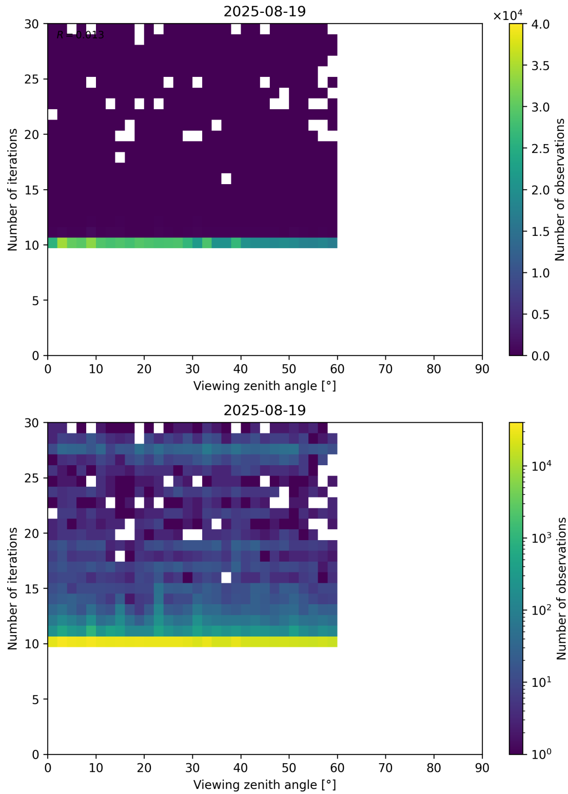
Figure 113: Scatter density plot of “Viewing zenith angle” against “Number of iterations” for 2025-08-19 to 2025-08-20.
