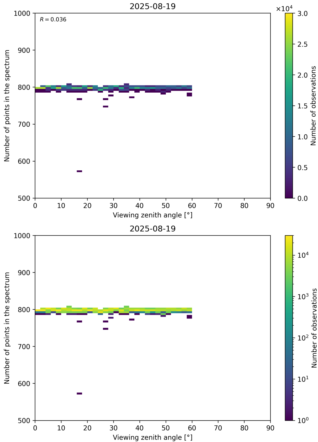
Figure 114: Scatter density plot of “Viewing zenith angle” against “Number of points in the spectrum” for 2025-08-19 to 2025-08-20.
