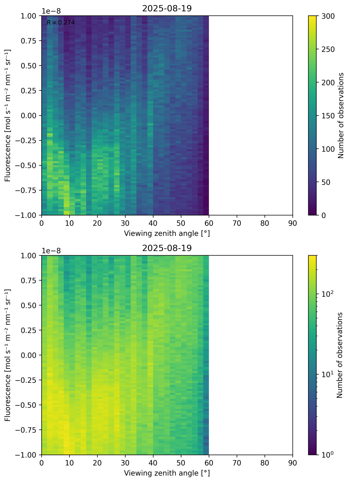
Figure 108: Scatter density plot of “Viewing zenith angle” against “Fluorescence” for 2025-08-19 to 2025-08-20.
