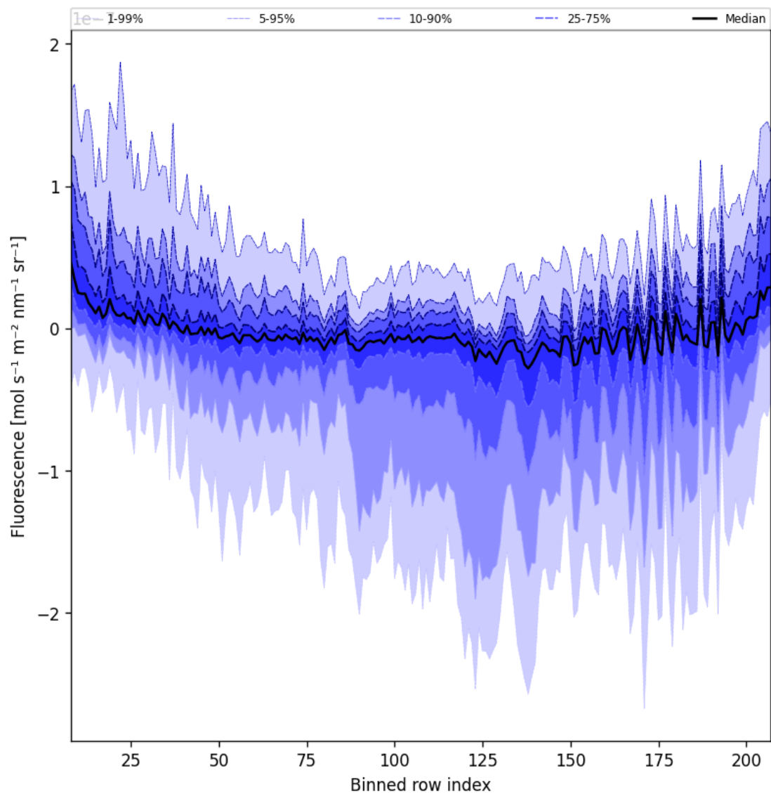
Figure 43: Along track statistics of “Fluorescence” for 2025-08-19 to 2025-08-20
