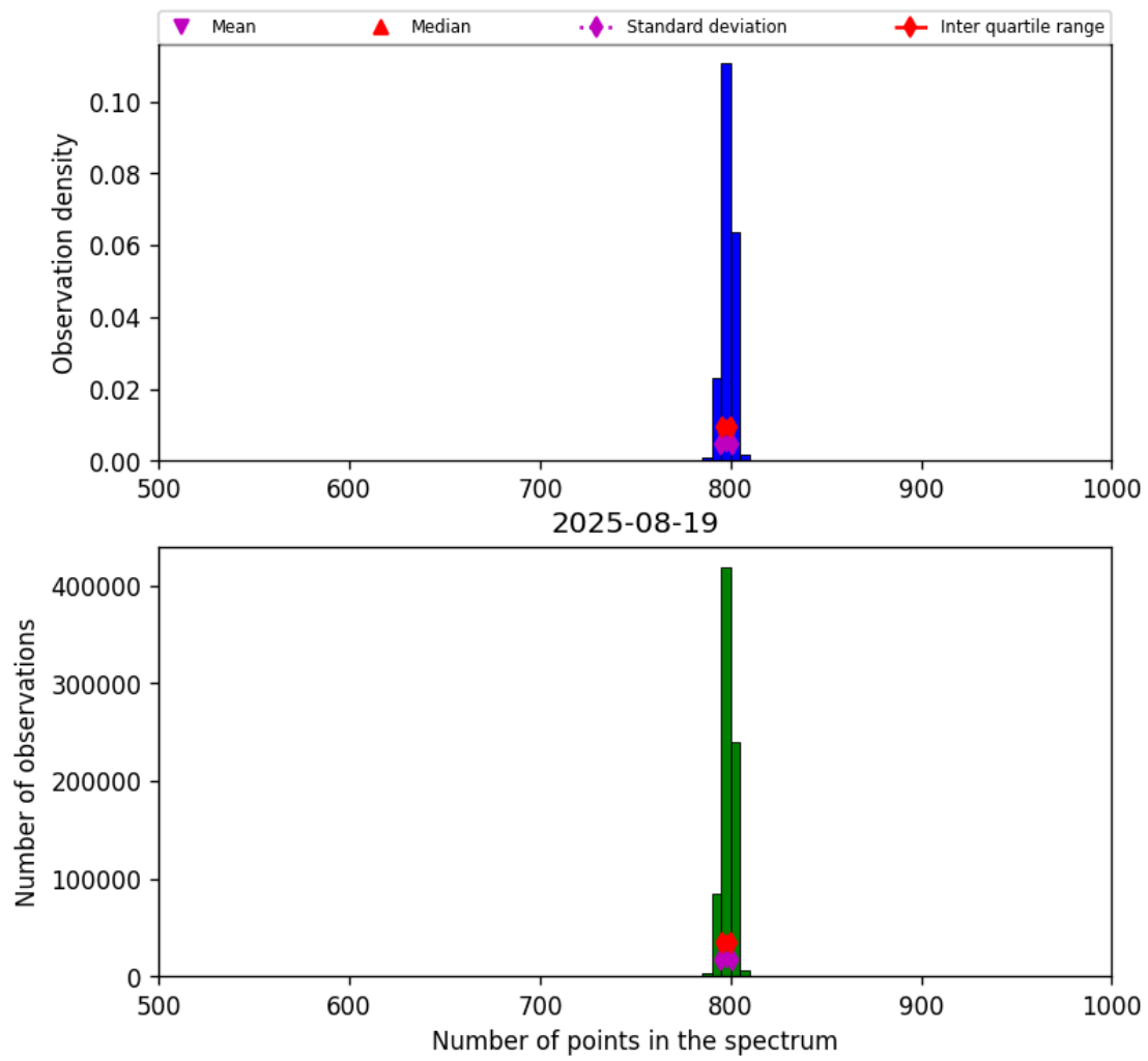
Figure 26: Histogram of “Number of points in the spectrum” for 2025-08-19 to 2025-08-20
