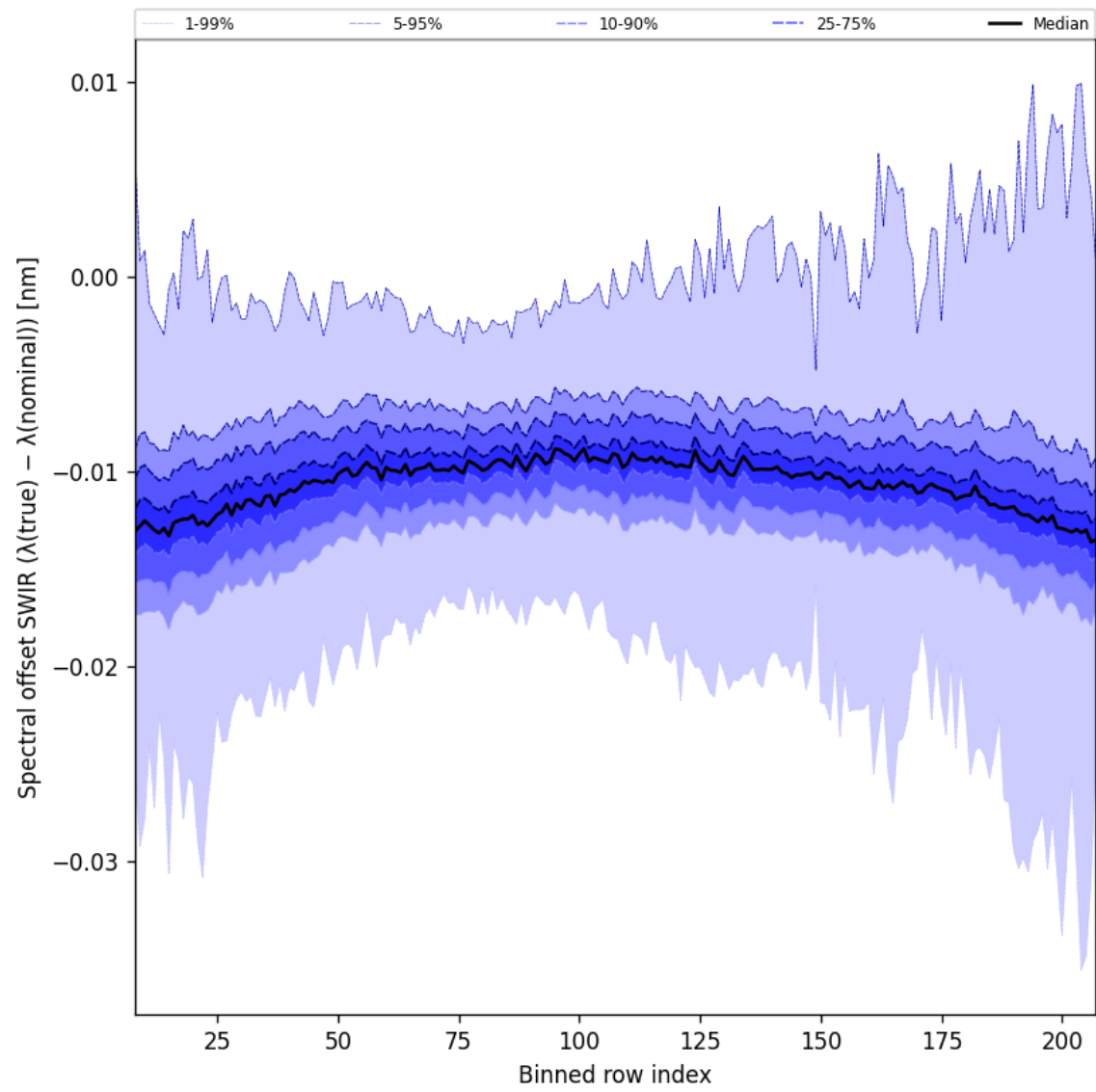
Figure 38: Along track statistics of “Spectral offset SWIR ( \lambda_{\text{true}} - \lambda_{\text{nominal}} )” for 2025-08-20 to 2025-08-22
