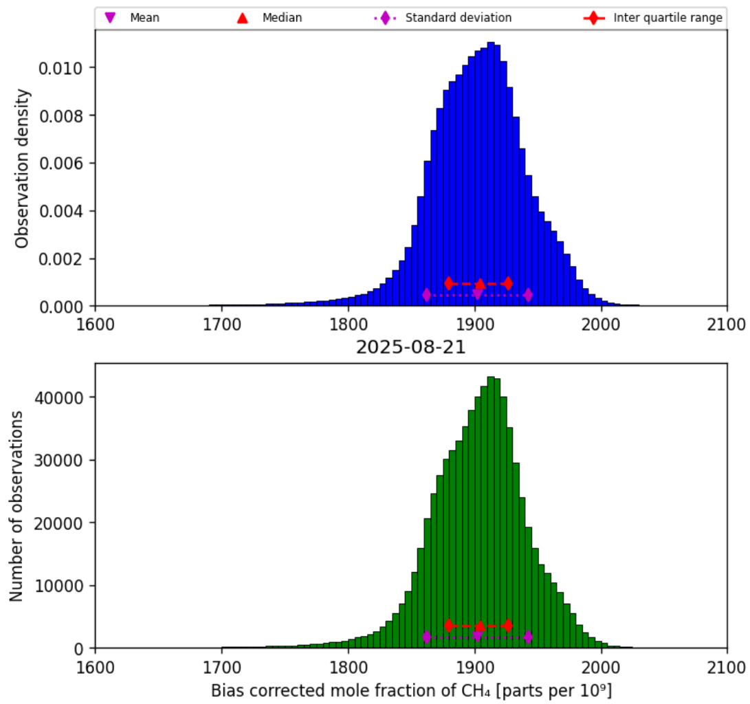
Figure 25: Histogram of “Bias corrected mole fraction of CH 4 ” for 2025-08-20 to 2025-08-22
