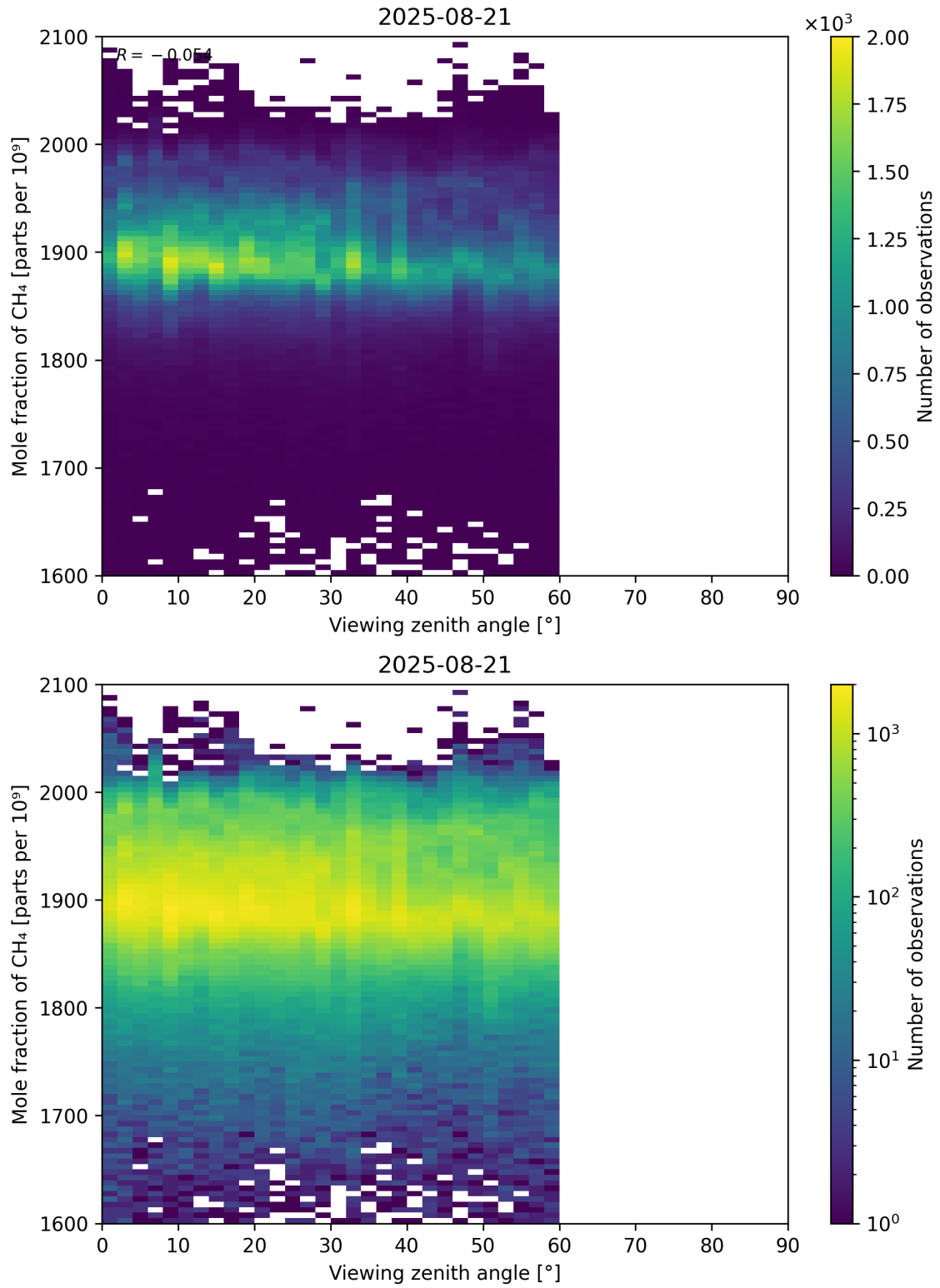
Figure 110: Scatter density plot of “Viewing zenith angle” against “Mole fraction of CH 4 ” for 2025-08-20 to 2025-08-22.
