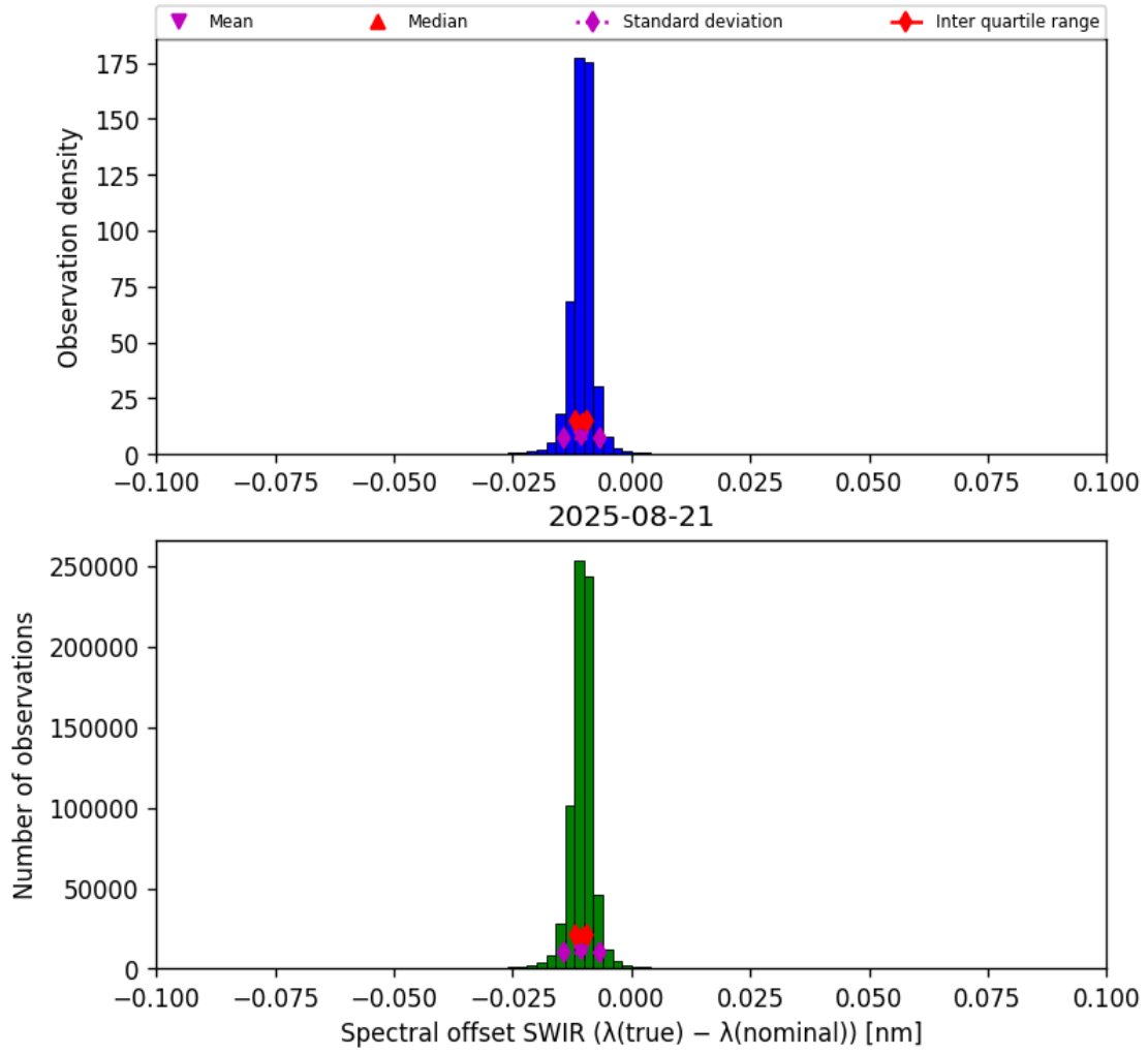
Figure 27: Histogram of “Spectral offset SWIR ( \lambda_{\text{true}} - \lambda_{\text{nominal}} )” for 2025-08-20 to 2025-08-22
