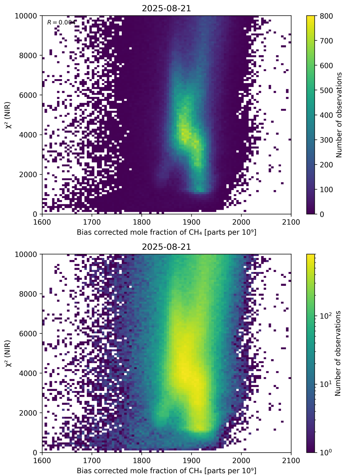
Figure 63: Scatter density plot of “Bias corrected mole fraction of \text{CH}_4 ” against “ \chi^2 (NIR)” for 2025-08-20 to 2025-08-22.
