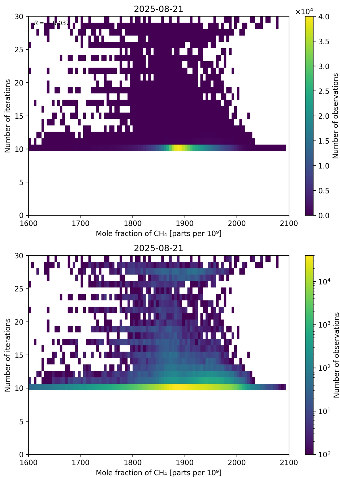
Figure 76: Scatter density plot of “Mole fraction of CH 4 ” against “Number of iterations” for 2025-08-20 to 2025-08-22.
