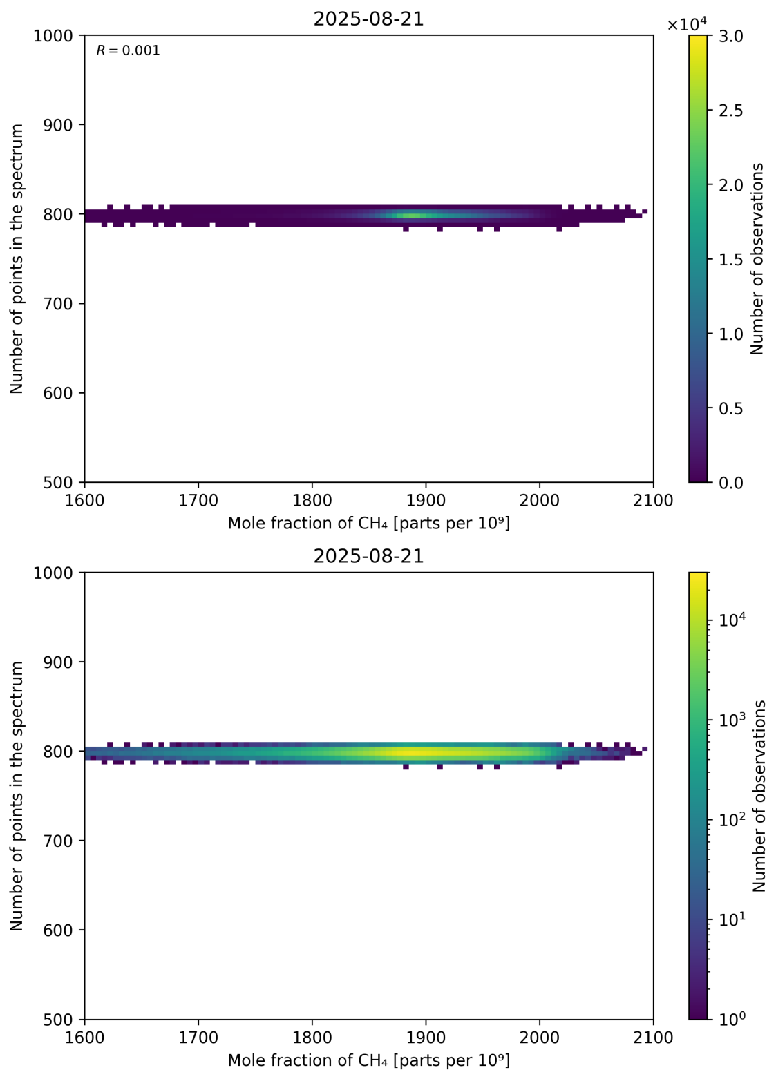
Figure 77: Scatter density plot of “Mole fraction of CH 4 ” against “Number of points in the spectrum” for 2025-08-20 to 2025-08-22.
