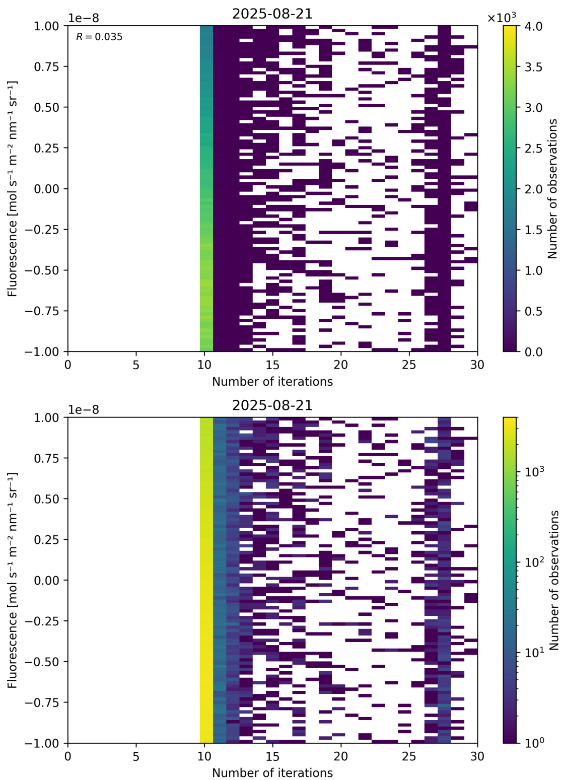
Figure 87: Scatter density plot of “Number of iterations” against “Fluorescence” for 2025-08-20 to 2025-08-22.
