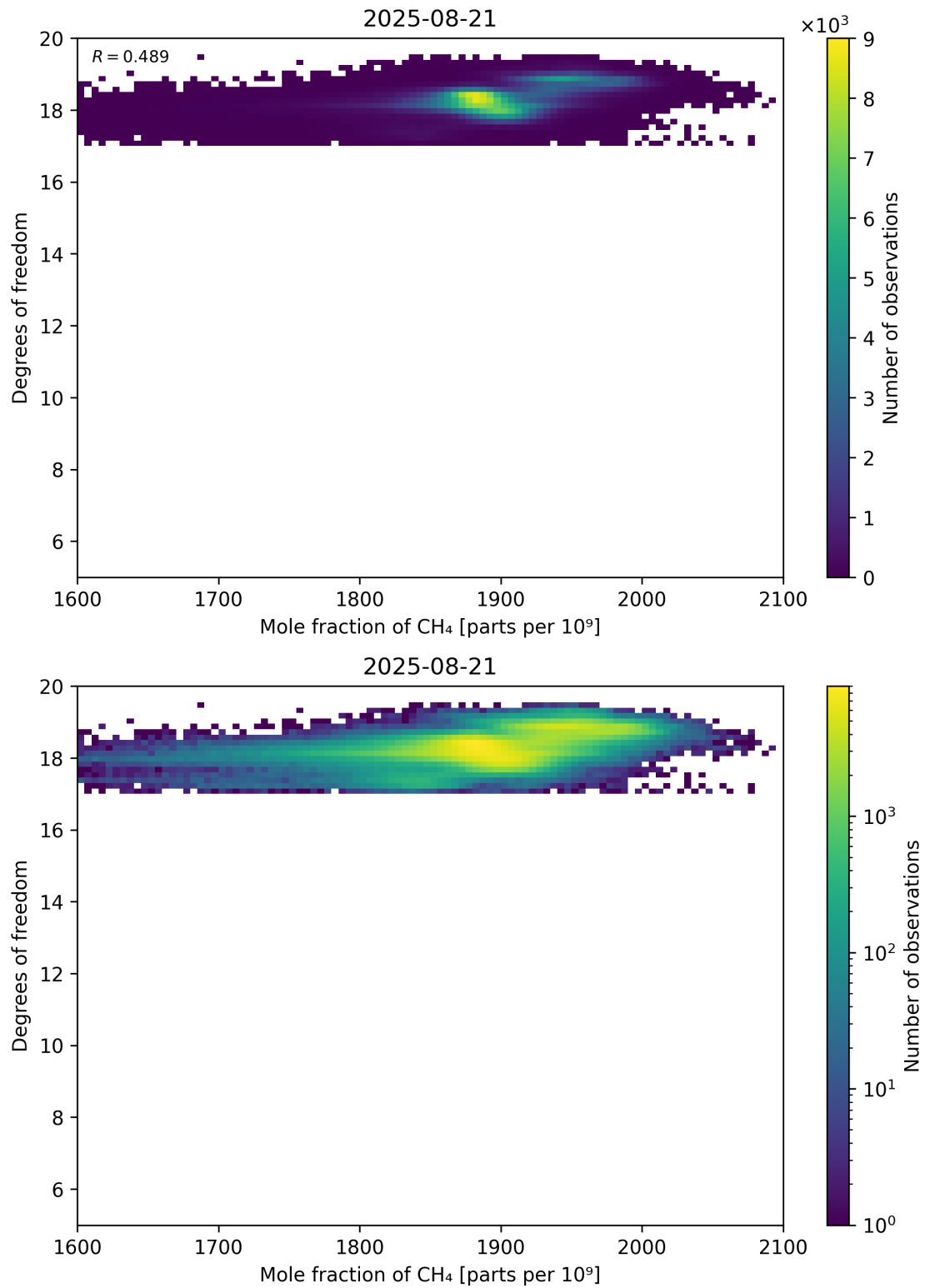
Figure 72: Scatter density plot of “Mole fraction of CH 4 ” against “Degrees of freedom” for 2025-08-20 to 2025-08-22.
