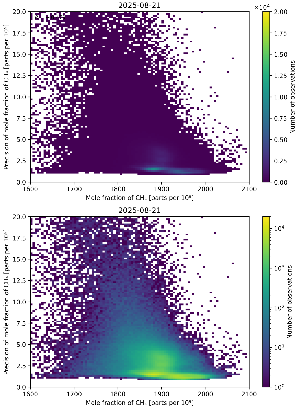
Figure 75: Scatter density plot of “Mole fraction of CH 4 ” against “Precision of mole fraction of CH 4 ” for 2025-08-20 to 2025-08-22.
