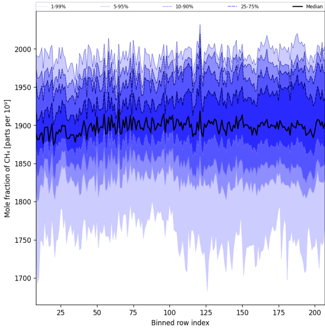
Figure 34: Along track statistics of “Mole fraction of CH 4 ” for 2025-08-20 to 2025-08-22
