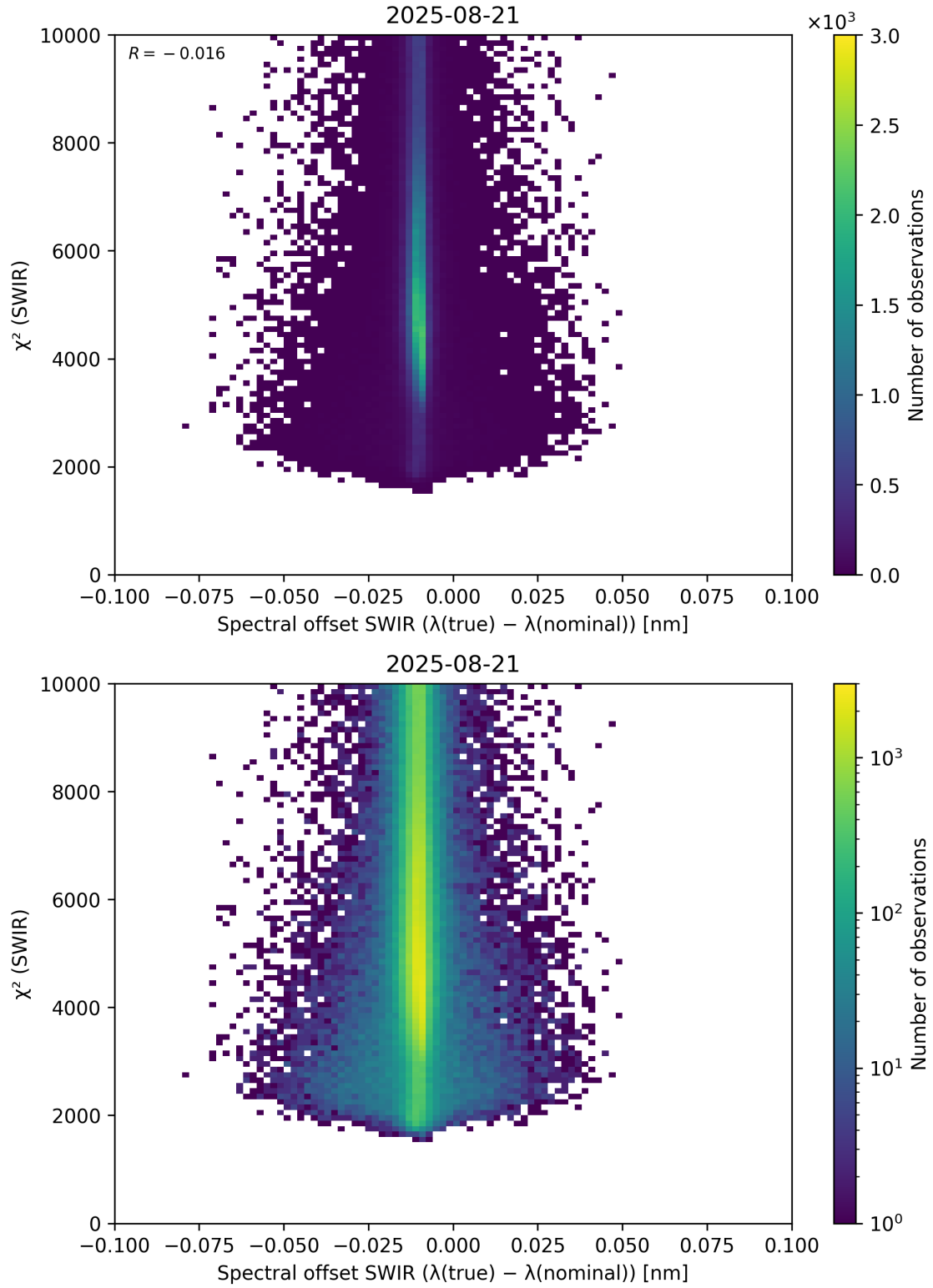
Figure 118: Scatter density plot of “Spectral offset SWIR ( \lambda_{\text{true}} - \lambda_{\text{nominal}} )” against “ \chi^2 (SWIR)” for 2025-08-20 to 2025-08-22.
