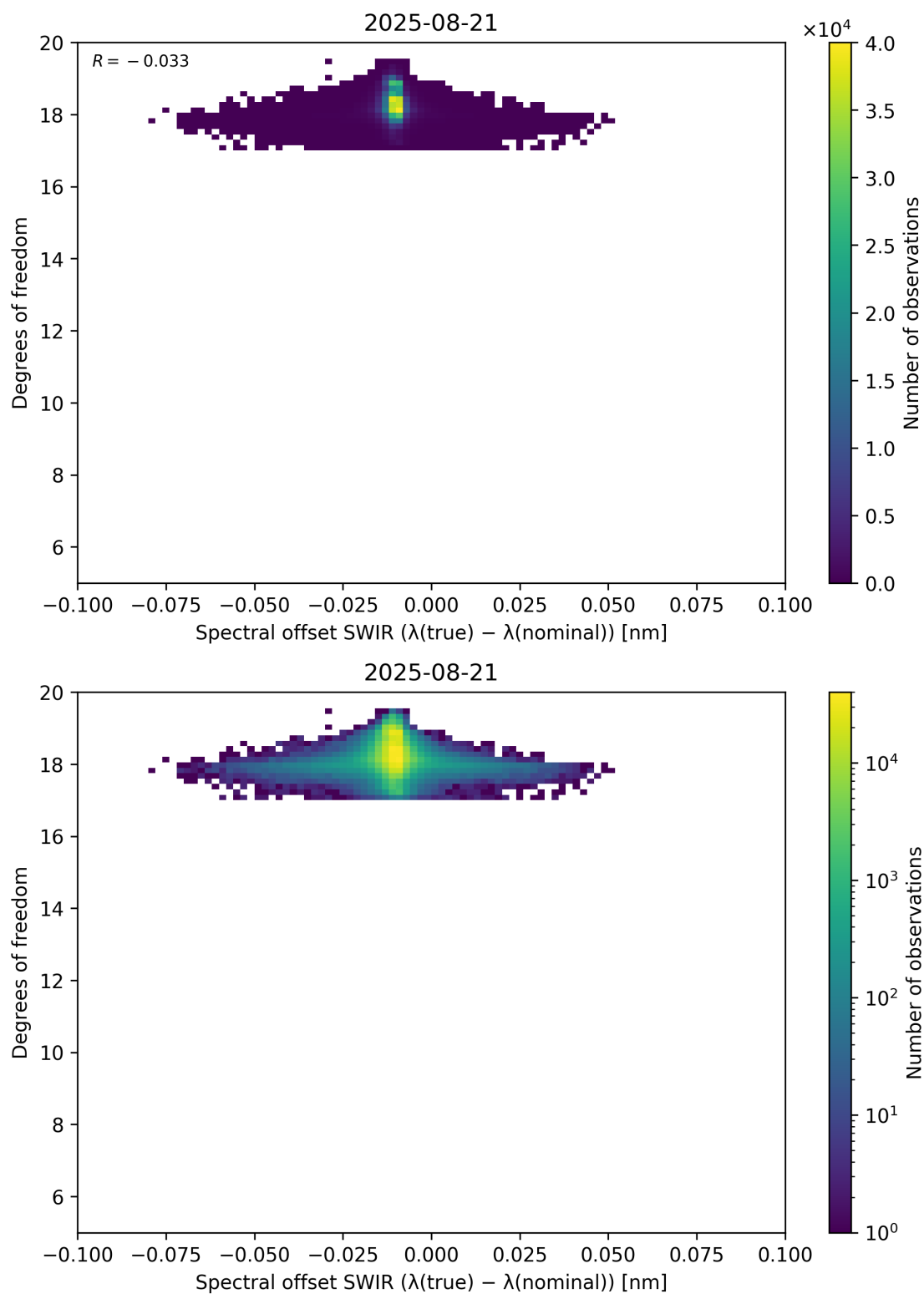
Figure 119: Scatter density plot of “Spectral offset SWIR ( \lambda_{\text{true}} - \lambda_{\text{nominal}} )” against “Degrees of freedom” for 2025-08-20 to 2025-08-22.
