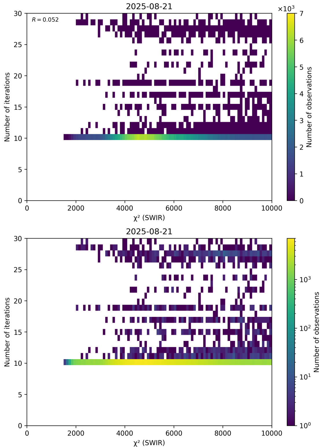
Figure 50: Scatter density plot of “ \chi^2 (SWIR)” against “Number of iterations” for 2025-08-20 to 2025-08-22.
