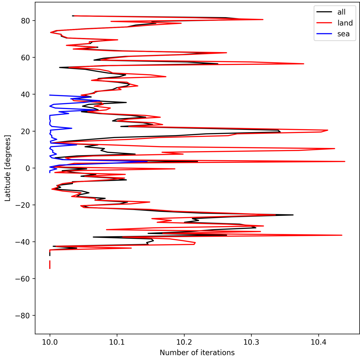
Figure 20: Zonal average of “Number of iterations” for 2025-08-20 to 2025-08-22.
