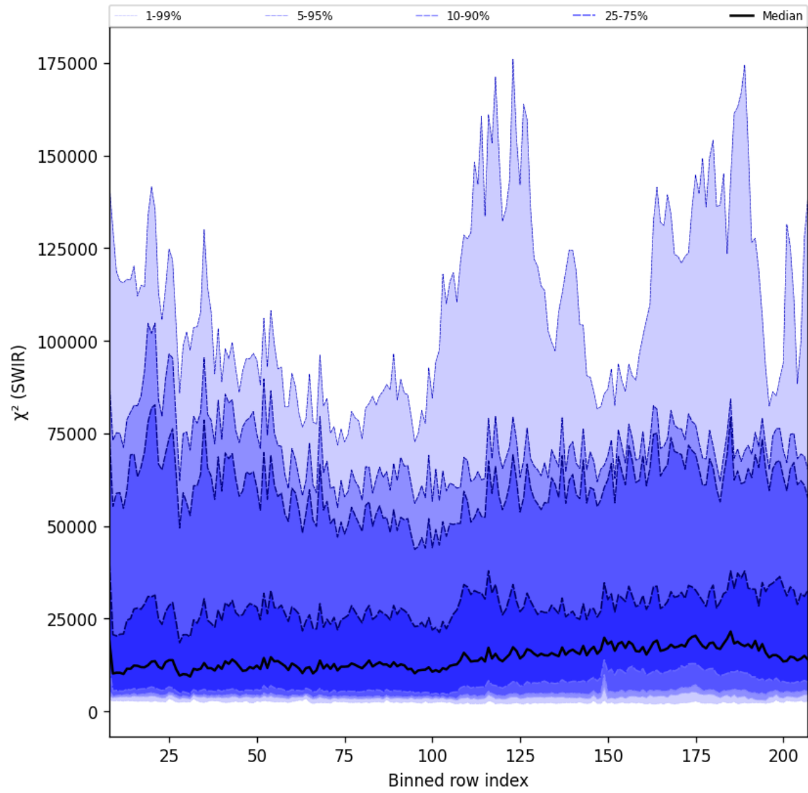
Figure 39: Along track statistics of “ \chi^2 (SWIR)” for 2025-08-20 to 2025-08-22
