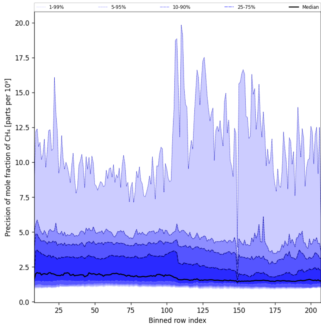
Figure 35: Along track statistics of “Precision of mole fraction of CH 4 ” for 2025-08-20 to 2025-08-22
