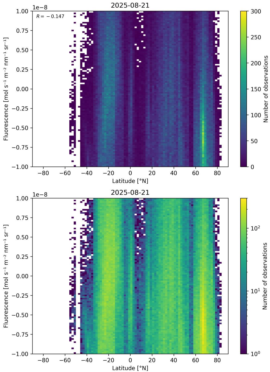
Figure 56: Scatter density plot of “Latitude” against “Fluorescence” for 2025-08-20 to 2025-08-22.
