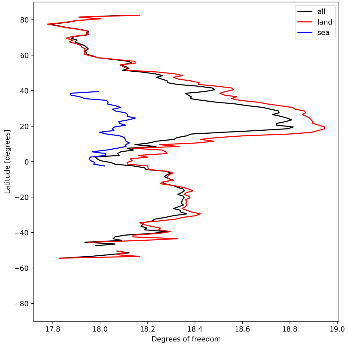
Figure 19: Zonal average of “Degrees of freedom” for 2025-08-20 to 2025-08-22.
