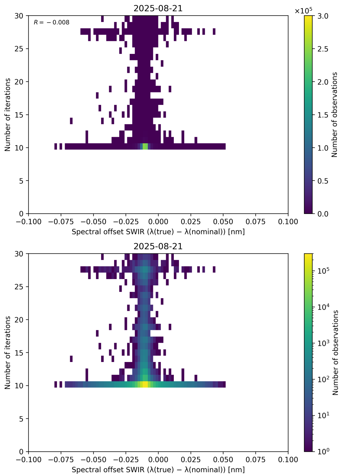
Figure 121: Scatter density plot of “Spectral offset SWIR ( \lambda_{\text{true}} - \lambda_{\text{nominal}} )” against “Number of iterations” for 2025-08-20 to 2025-08-22.
