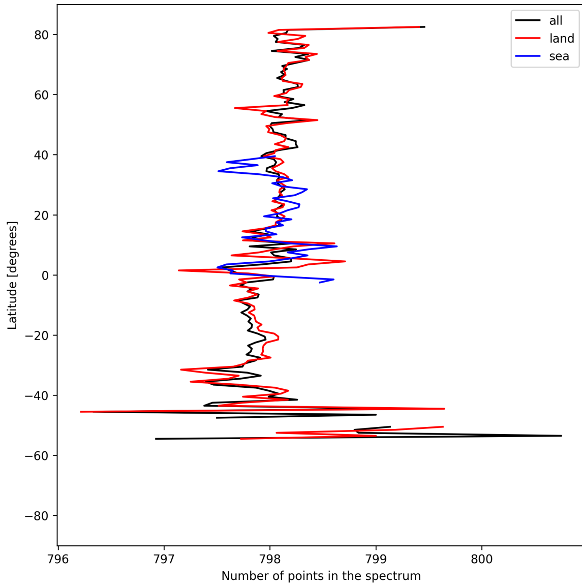
Figure 15: Zonal average of “Number of points in the spectrum” for 2025-08-20 to 2025-08-22.
