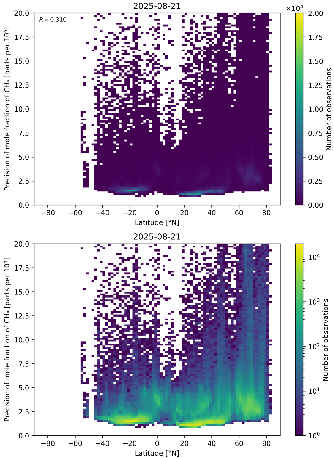
Figure 59: Scatter density plot of “Latitude” against “Precision of mole fraction of \text{CH}_4 ” for 2025-08-20 to 2025-08-22.
