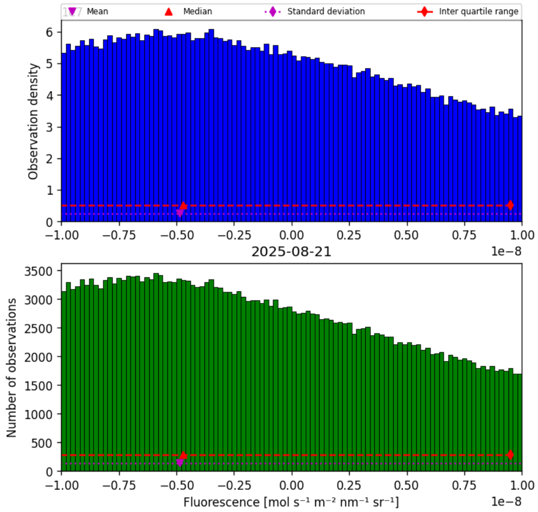
Figure 32: Histogram of “Fluorescence” for 2025-08-20 to 2025-08-22
