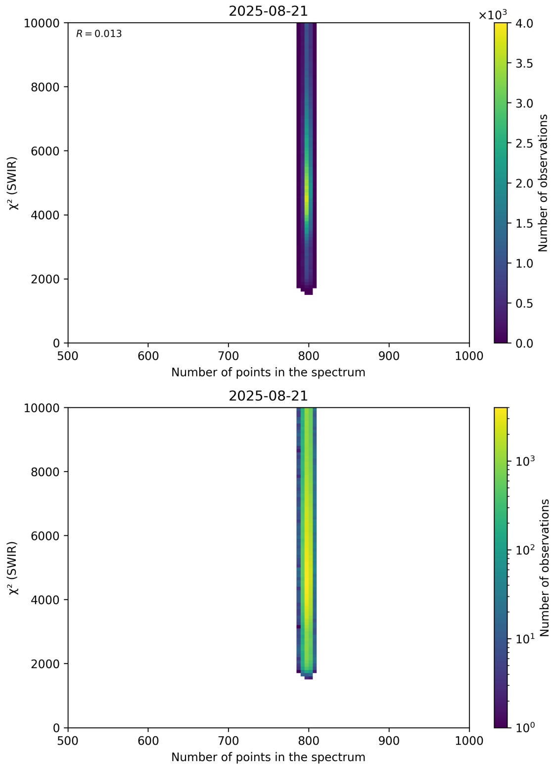
Figure 89: Scatter density plot of “Number of points in the spectrum” against “ \chi^2 (SWIR)” for 2025-08-20 to 2025-08-22.
