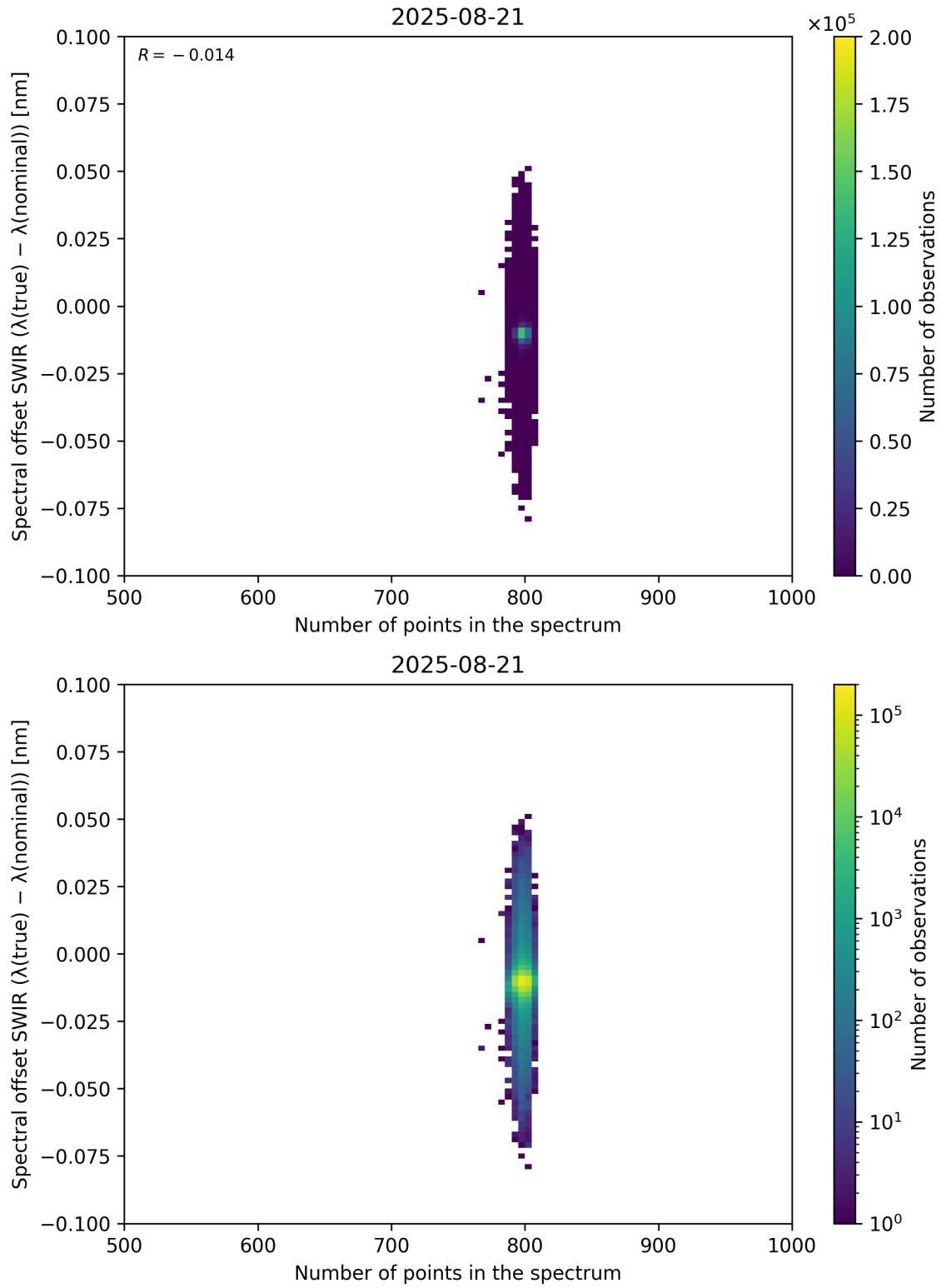
Figure 93: Scatter density plot of “Number of points in the spectrum” against “Spectral offset SWIR ( \lambda_{\text{true}} - \lambda_{\text{nominal}} )” for 2025-08-20 to 2025-08-22.
