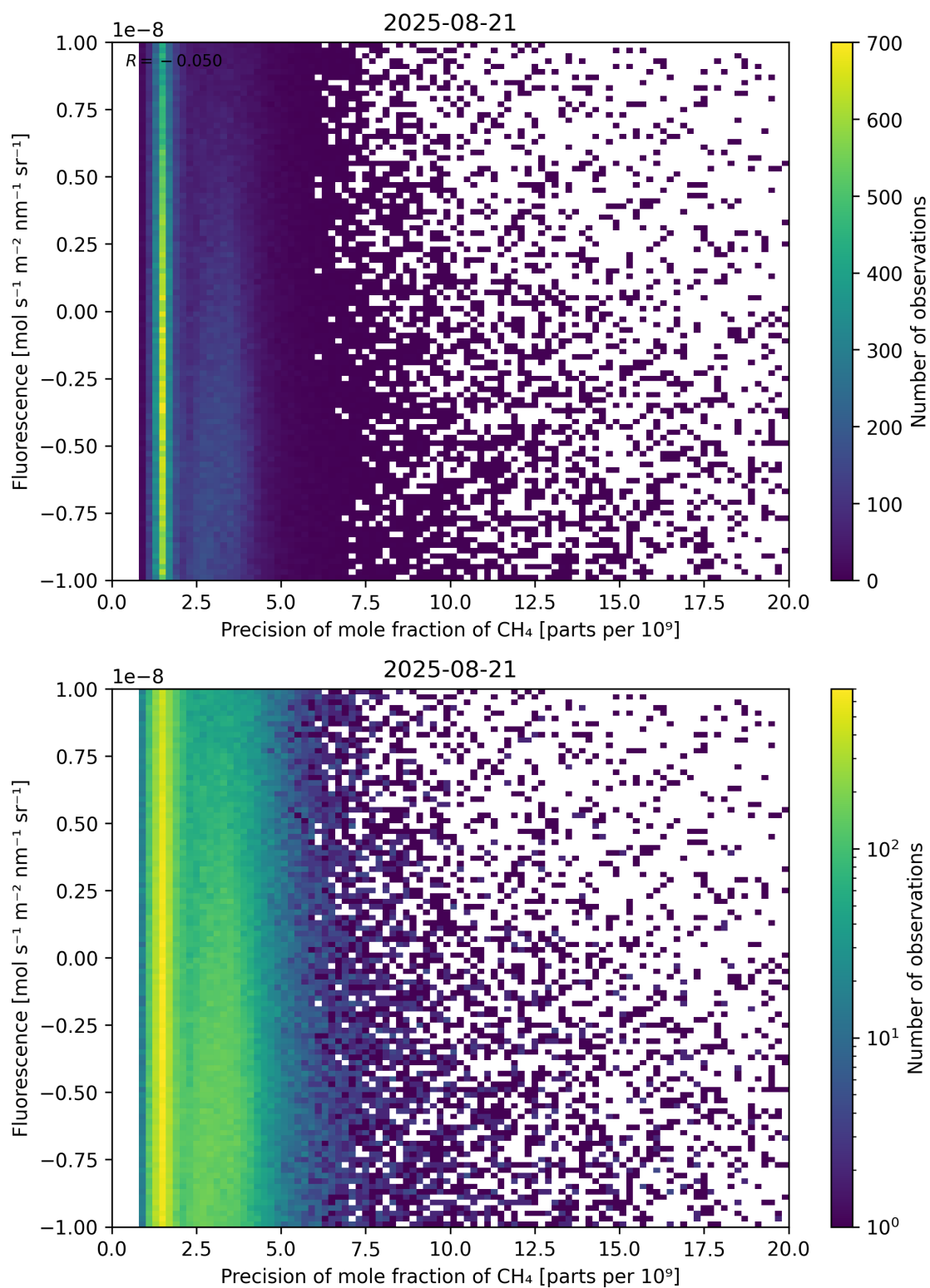
Figure 81: Scatter density plot of “Precision of mole fraction of \text{CH}_4 ” against “Fluorescence” for 2025-08-20 to 2025-08-22.
