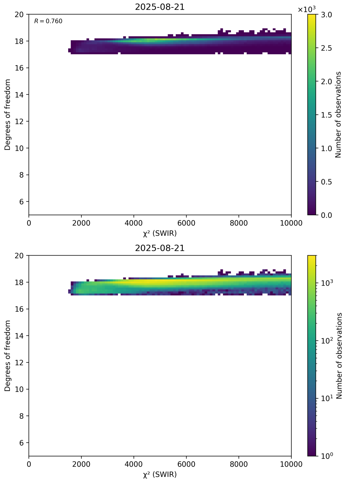
Figure 48: Scatter density plot of “ \chi^2 (SWIR)” against “Degrees of freedom” for 2025-08-20 to 2025-08-22.
