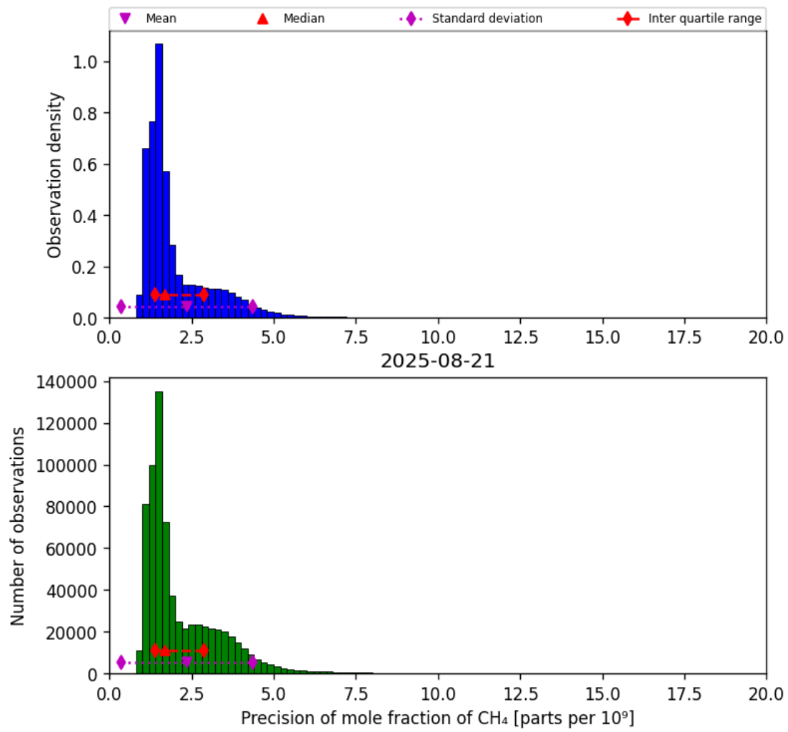
Figure 24: Histogram of “Precision of mole fraction of CH 4 ” for 2025-08-20 to 2025-08-22
