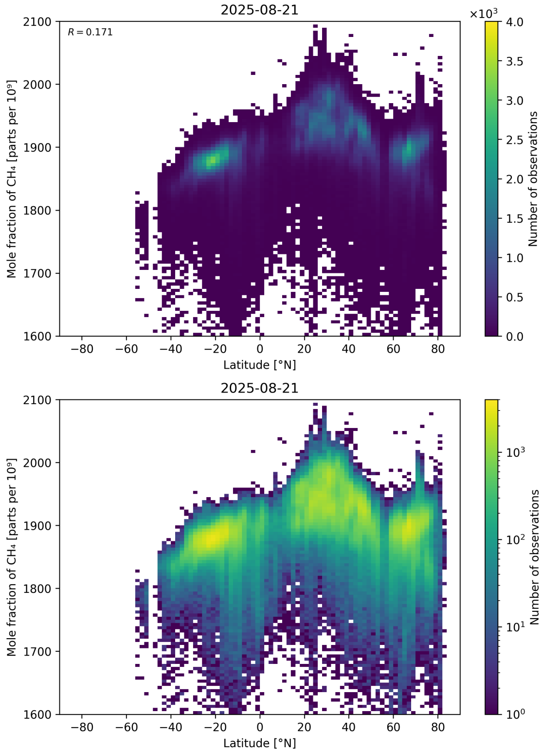
Figure 57: Scatter density plot of “Latitude” against “Mole fraction of \text{CH}_4 ” for 2025-08-20 to 2025-08-22.
