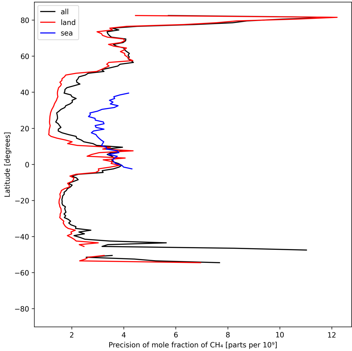
Figure 13: Zonal average of “Precision of mole fraction of CH 4 ” for 2025-08-20 to 2025-08-22.
