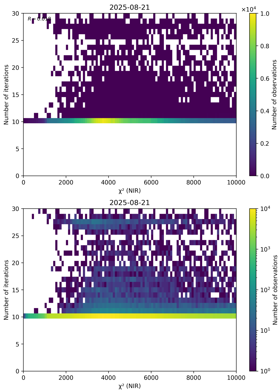
Figure 46: Scatter density plot of “ \chi^2 (NIR)” against “Number of iterations” for 2025-08-20 to 2025-08-22.
