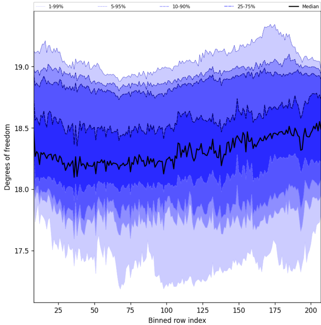
Figure 41: Along track statistics of “Degrees of freedom” for 2025-08-20 to 2025-08-22
