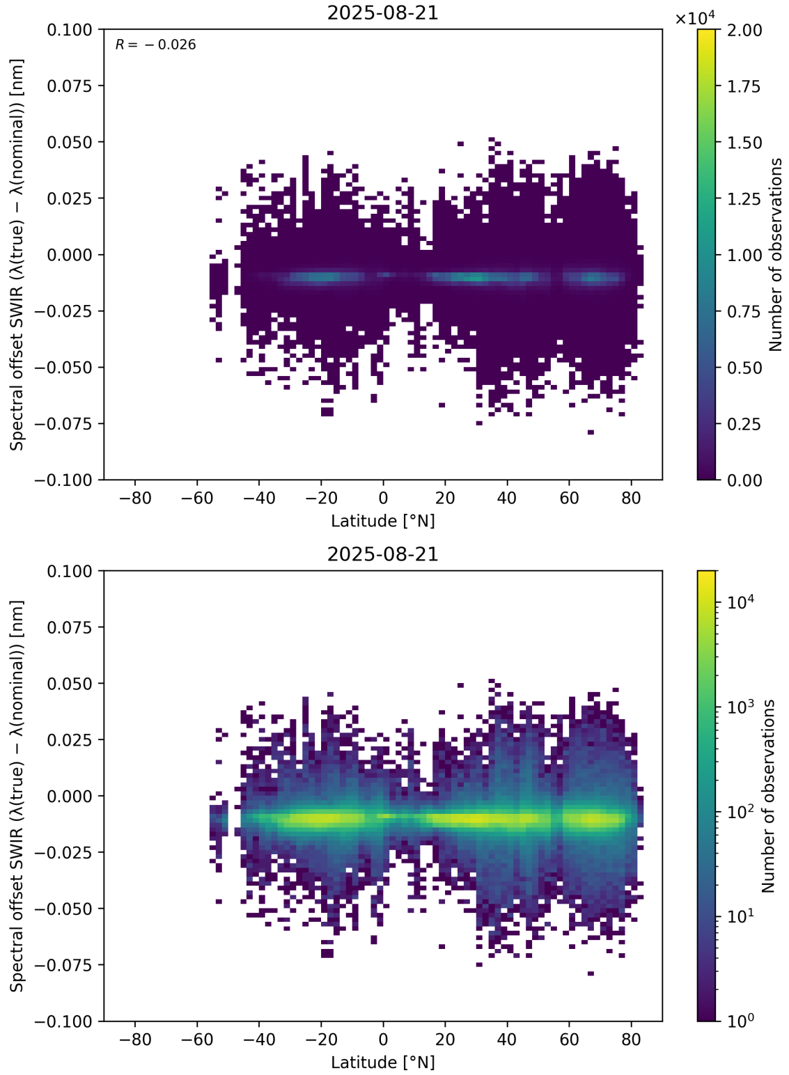
Figure 62: Scatter density plot of “Latitude” against “Spectral offset SWIR ( \lambda_{\text{true}} - \lambda_{\text{nominal}} )” for 2025-08-20 to 2025-08-22.
