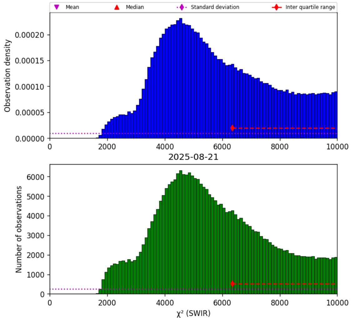
Figure 28: Histogram of “ \chi^2 (SWIR)” for 2025-08-20 to 2025-08-22
