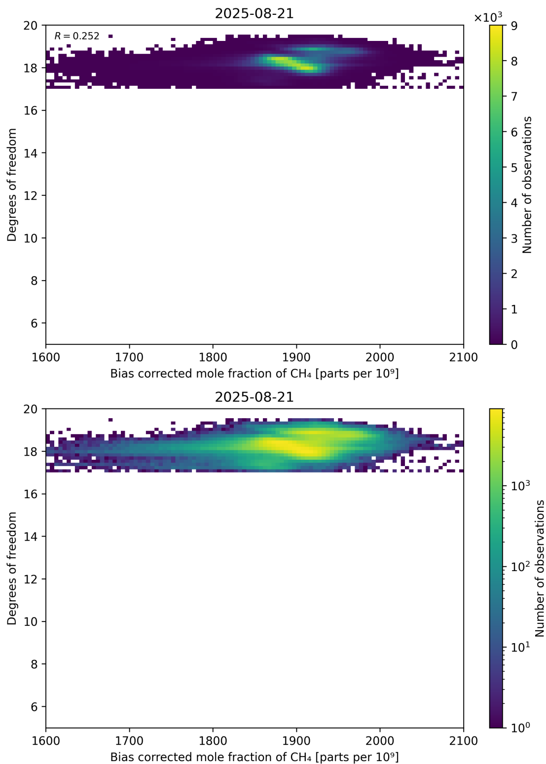
Figure 65: Scatter density plot of “Bias corrected mole fraction of CH 4 ” against “Degrees of freedom” for 2025-08-20 to 2025-08-22.
