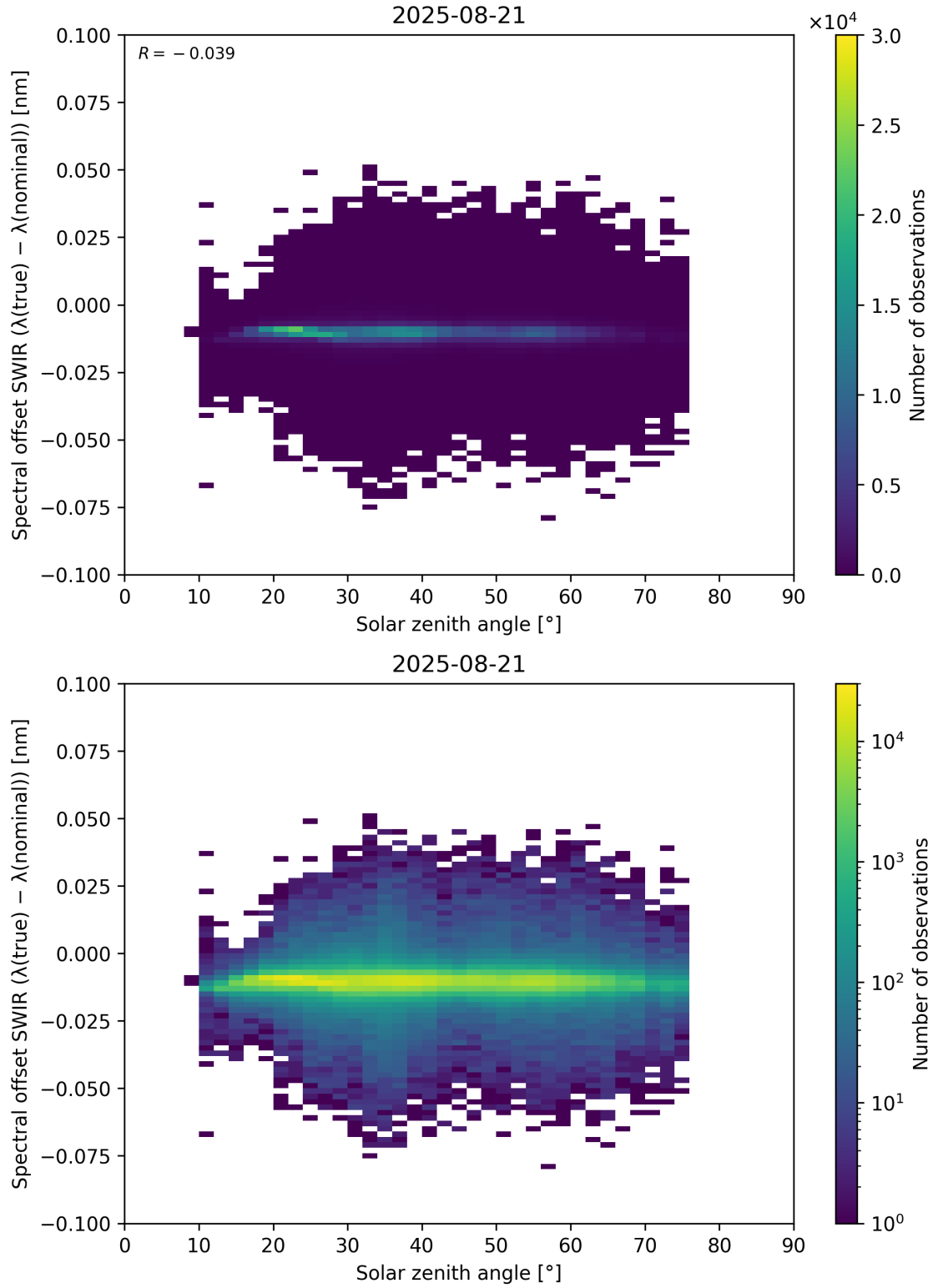
Figure 104: Scatter density plot of “Solar zenith angle” against “Spectral offset SWIR ( \lambda_{\text{true}} - \lambda_{\text{nominal}} )” for 2025-08-20 to 2025-08-22.
