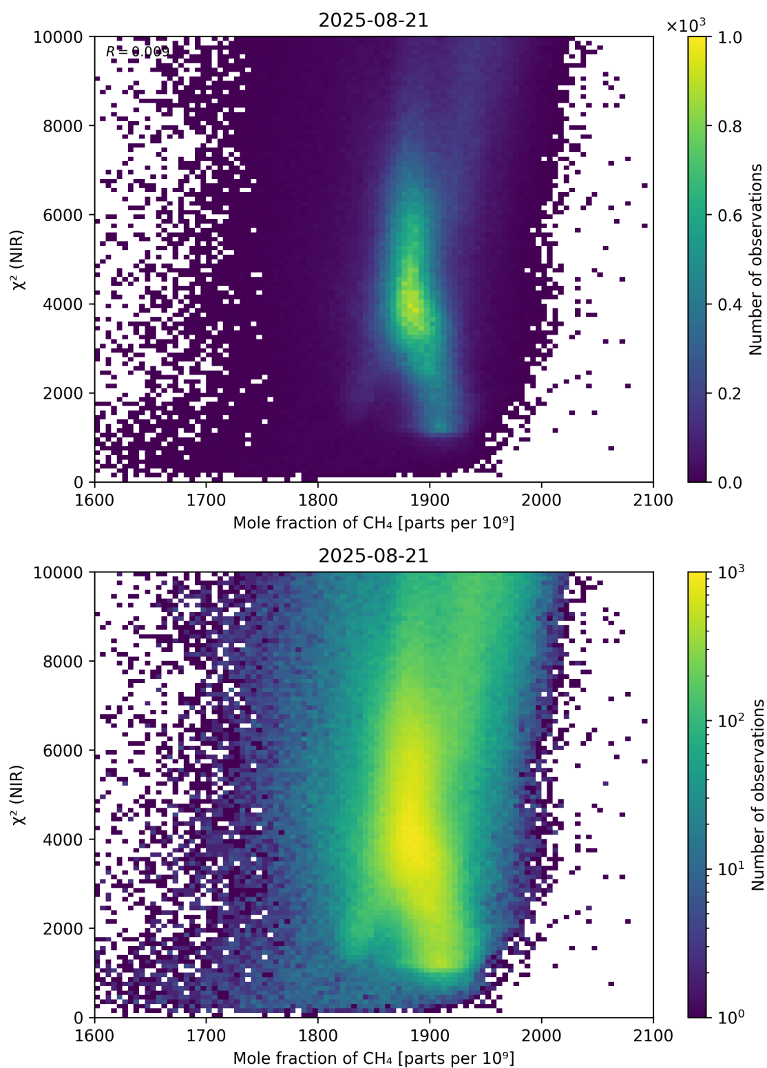
Figure 70: Scatter density plot of “Mole fraction of \text{CH}_4 ” against “ \chi^2 (NIR)” for 2025-08-20 to 2025-08-22.
