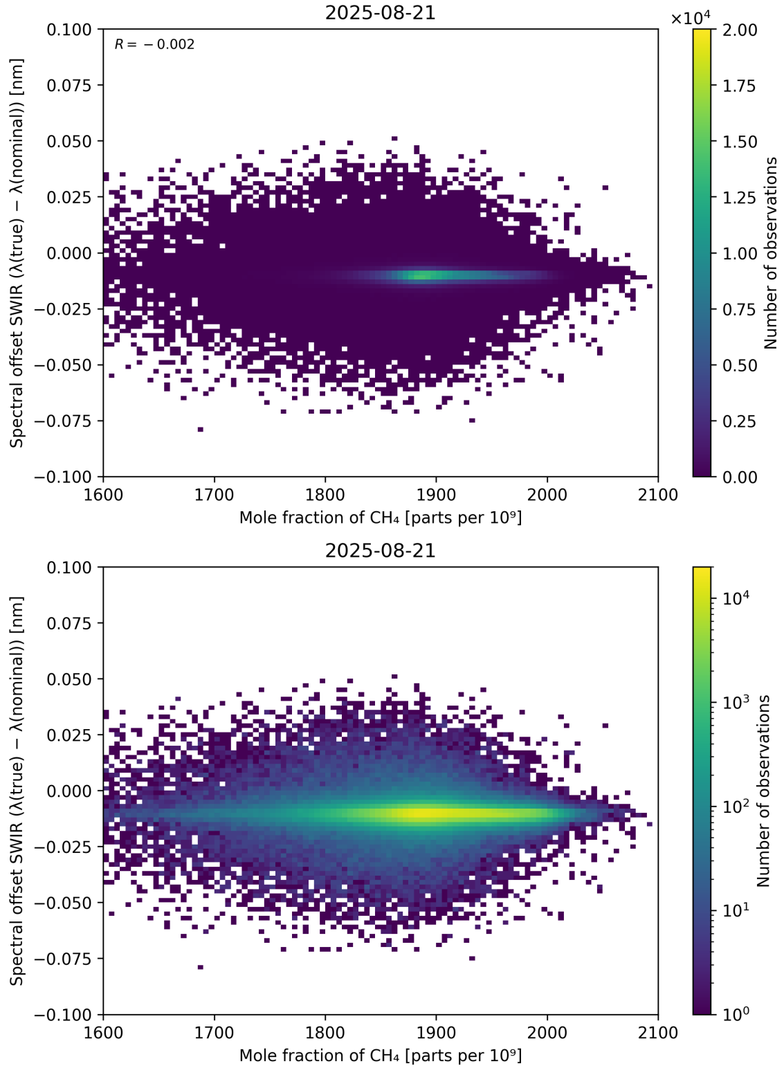
Figure 86: Scatter density plot of “Mole fraction of CH 4 ” against “Spectral offset SWIR ( \lambda_{\text{true}} - \lambda_{\text{nominal}} )” for 2025-08-20 to 2025-08-22.
