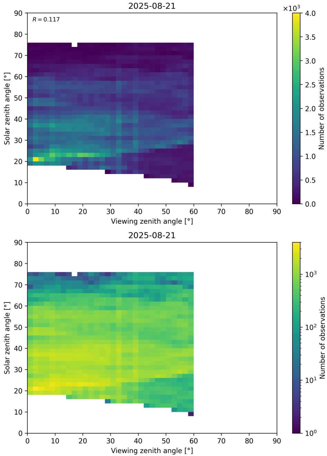
Figure 115: Scatter density plot of “Viewing zenith angle” against “Solar zenith angle” for 2025-08-20 to 2025-08-22.
