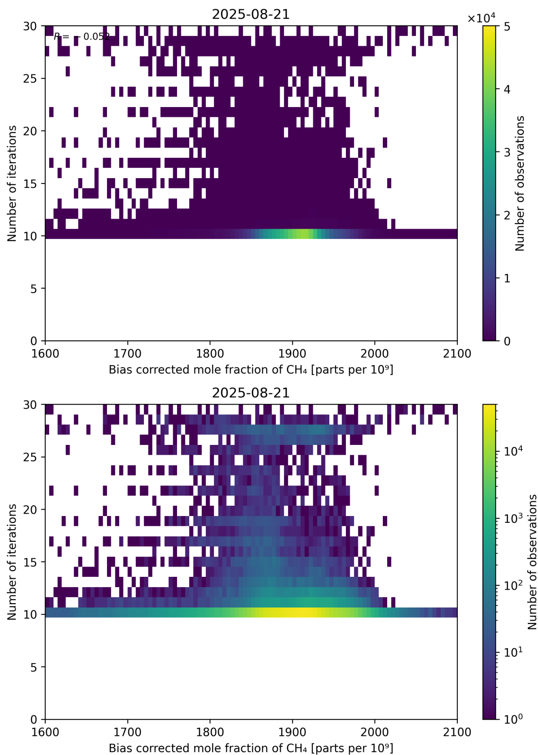
Figure 67: Scatter density plot of “Bias corrected mole fraction of CH 4 ” against “Number of iterations” for 2025-08-20 to 2025-08-22.
