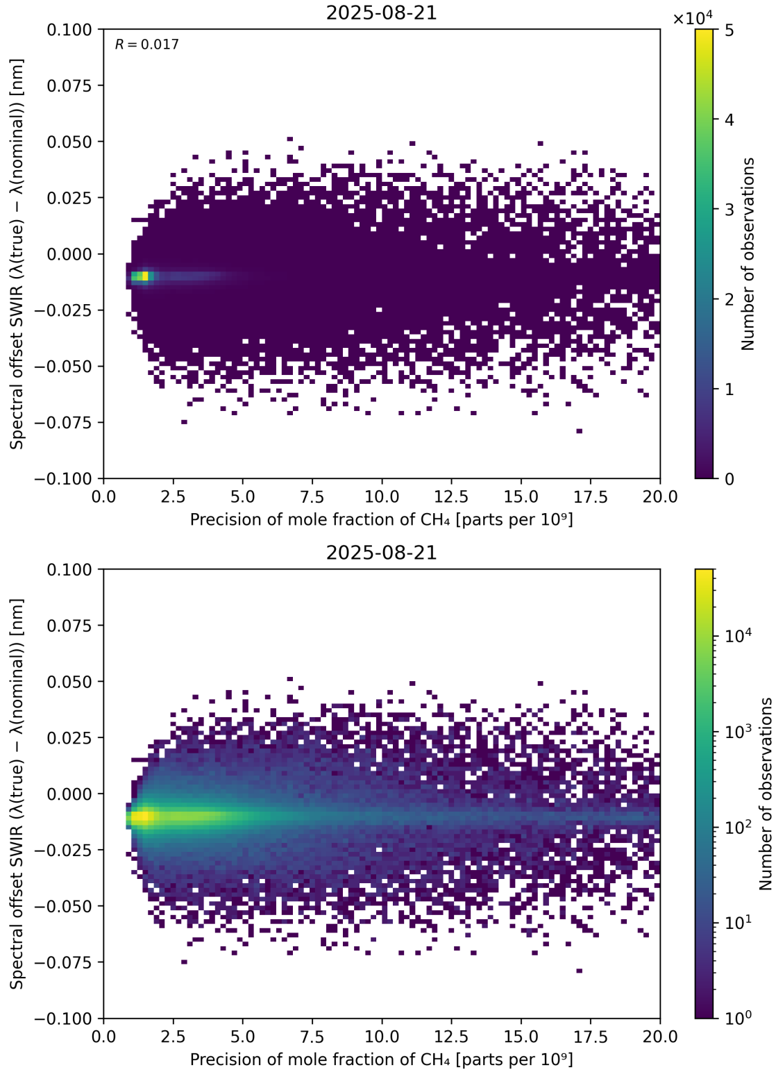
Figure 85: Scatter density plot of “Precision of mole fraction of CH 4 ” against “Spectral offset SWIR ( \lambda_{\text{true}} - \lambda_{\text{nominal}} )” for 2025-08-20 to 2025-08-22.
