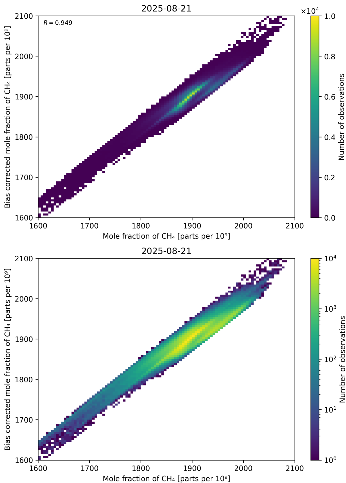
Figure 74: Scatter density plot of “Mole fraction of \text{CH}_4 ” against “Bias corrected mole fraction of \text{CH}_4 ” for 2025-08-20 to 2025-08-22.
