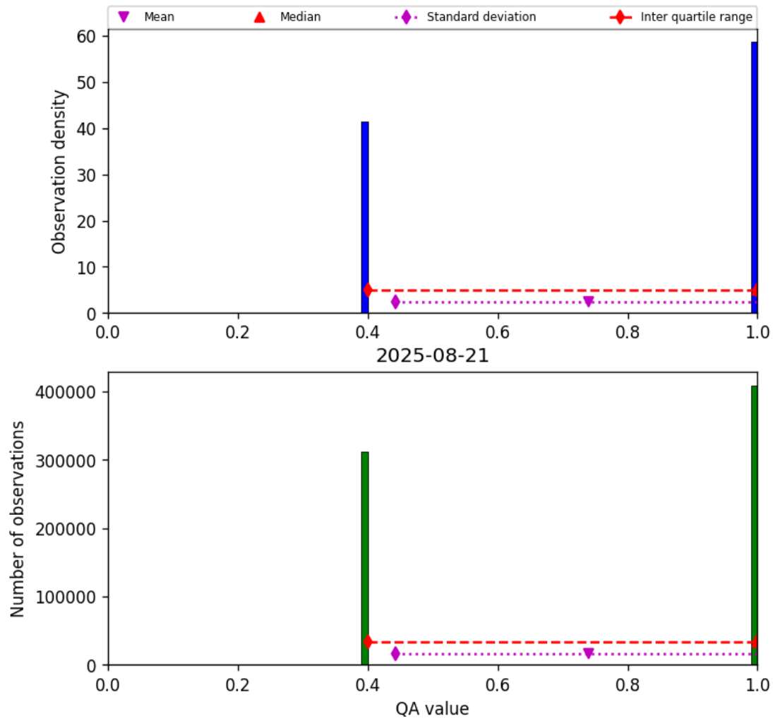
Figure 22: Histogram of “QA value” for 2025-08-20 to 2025-08-22
