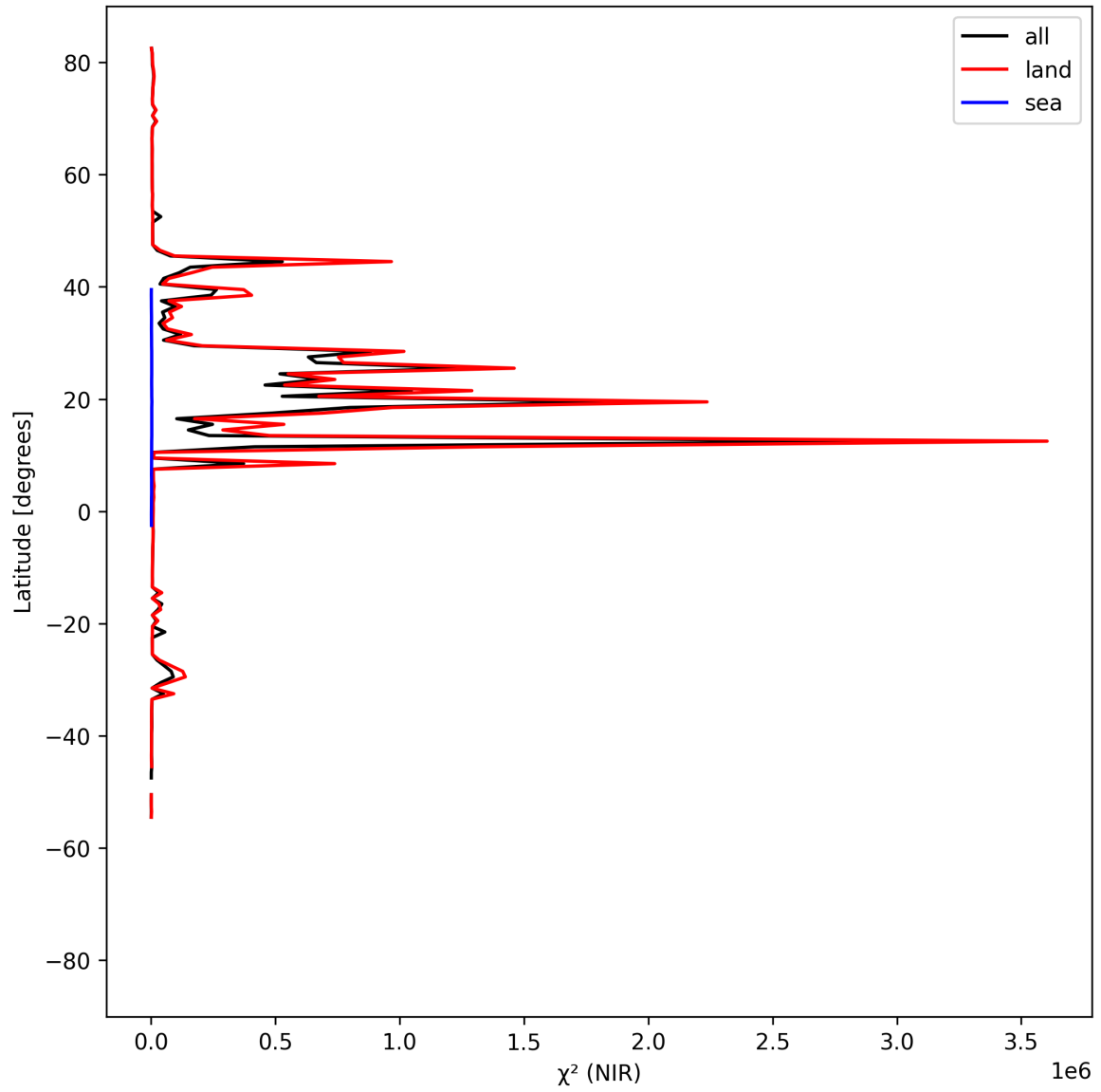
Figure 18: Zonal average of “ \chi^2 (NIR)” for 2025-08-20 to 2025-08-22.
