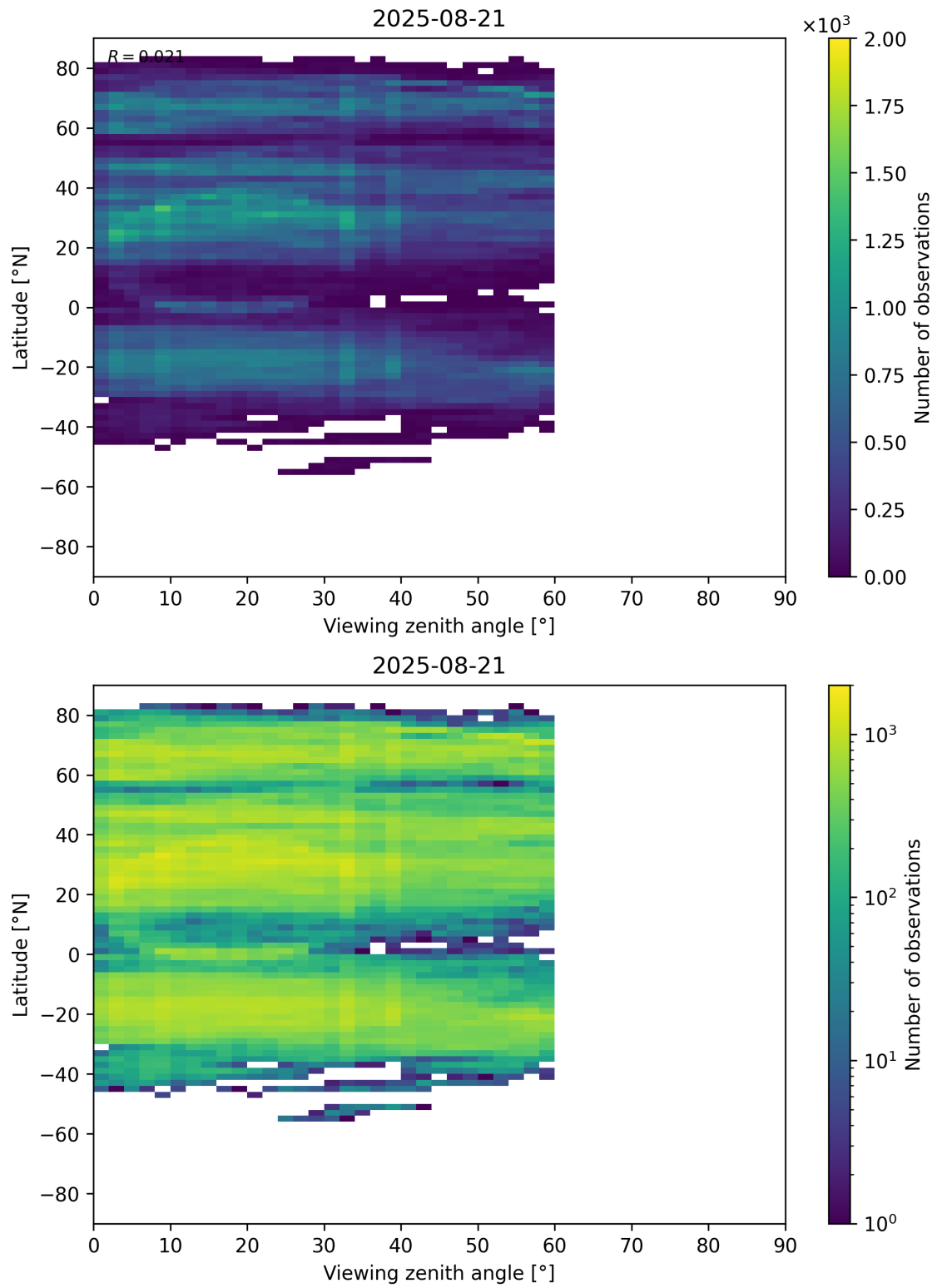
Figure 109: Scatter density plot of “Viewing zenith angle” against “Latitude” for 2025-08-20 to 2025-08-22.
