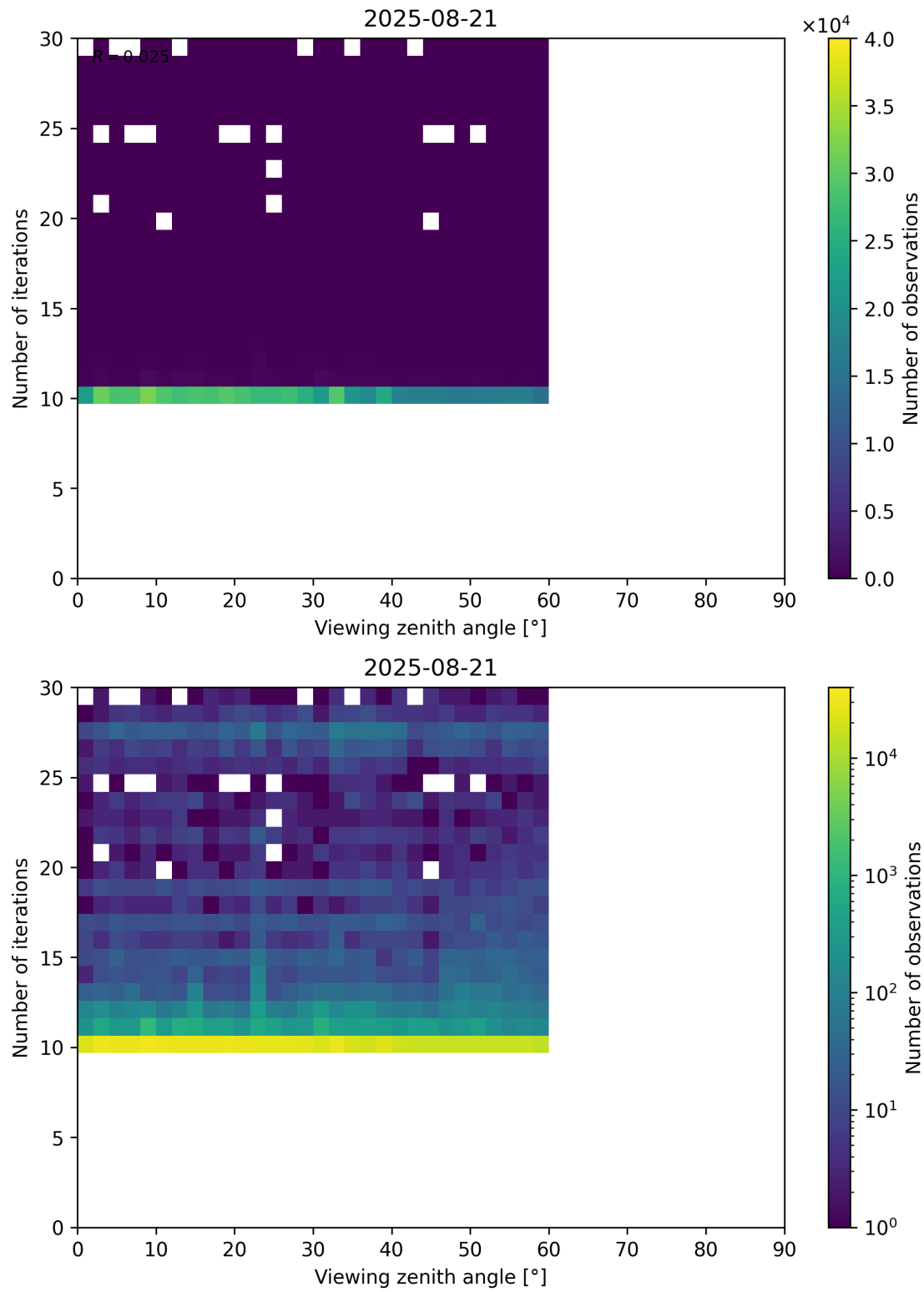
Figure 113: Scatter density plot of “Viewing zenith angle” against “Number of iterations” for 2025-08-20 to 2025-08-22.
