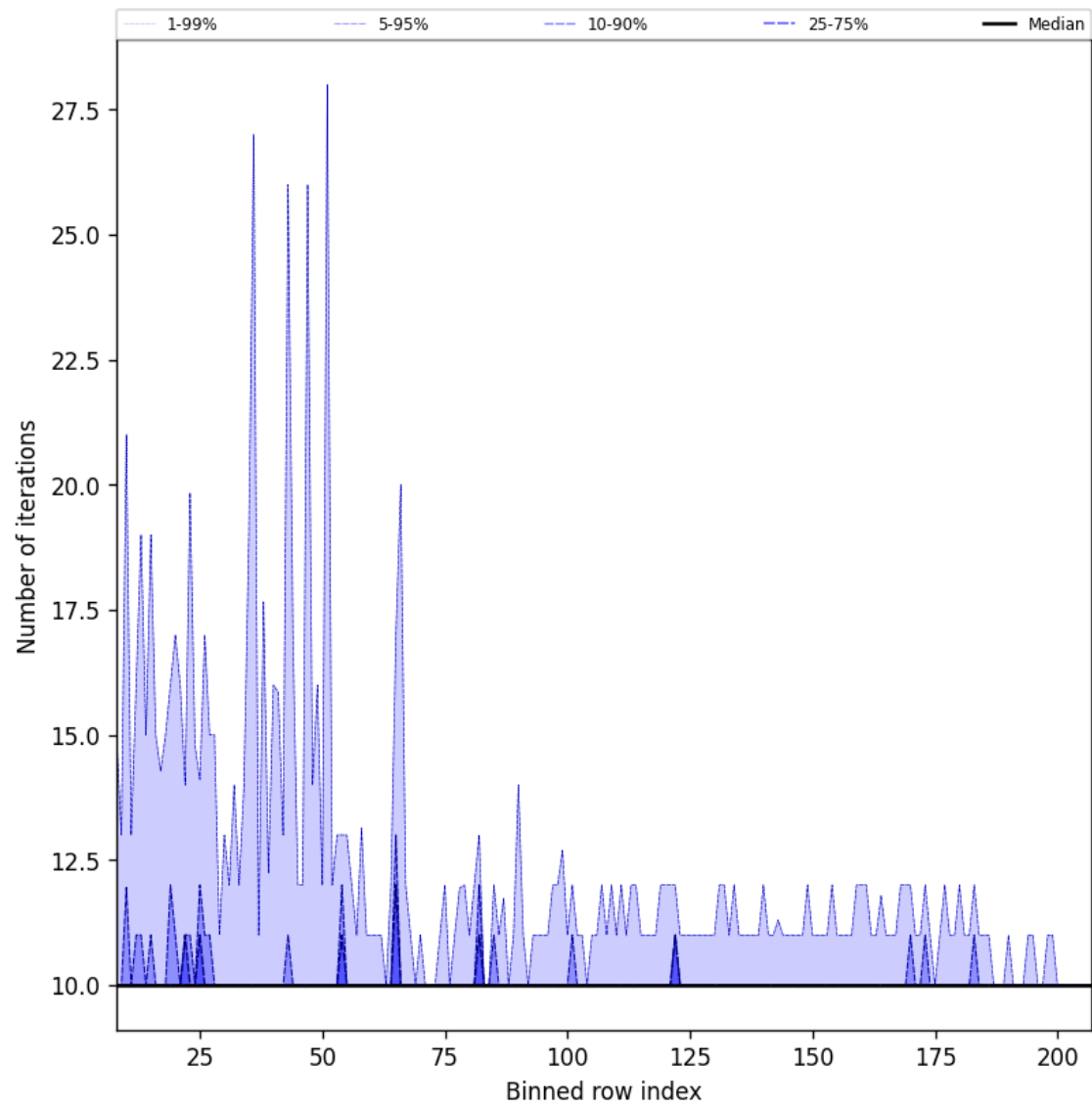
Figure 42: Along track statistics of “Number of iterations” for 2025-08-20 to 2025-08-22
