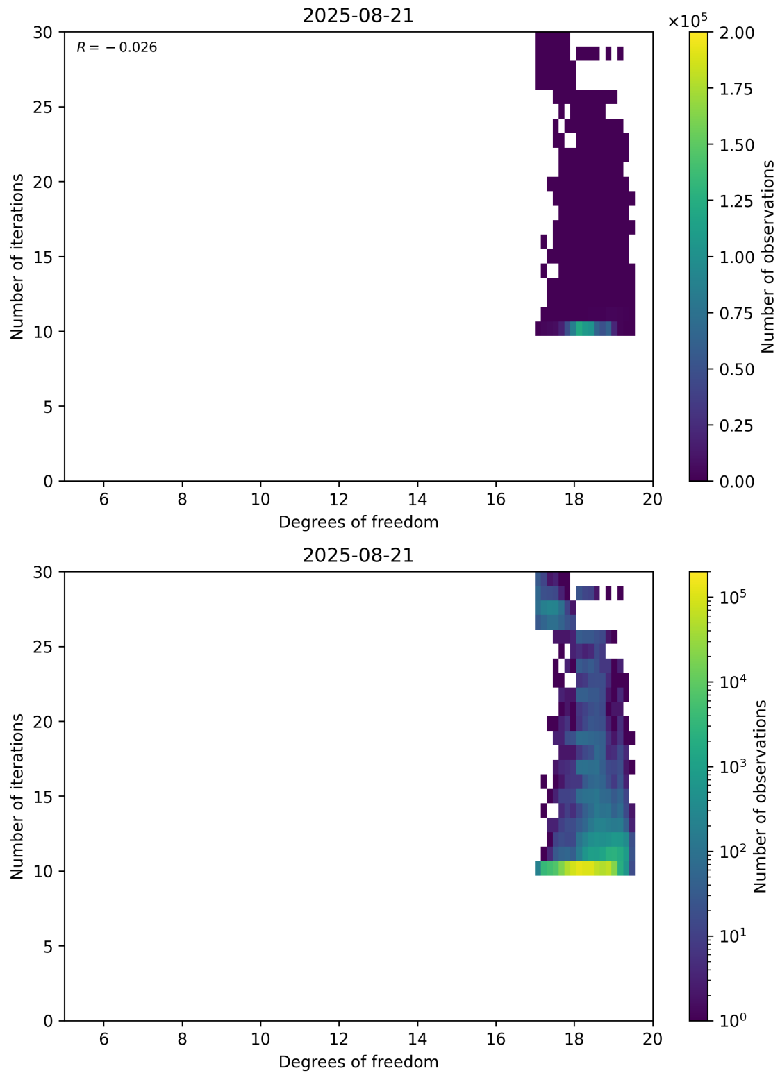
Figure 52: Scatter density plot of “Degrees of freedom” against “Number of iterations” for 2025-08-20 to 2025-08-22.
