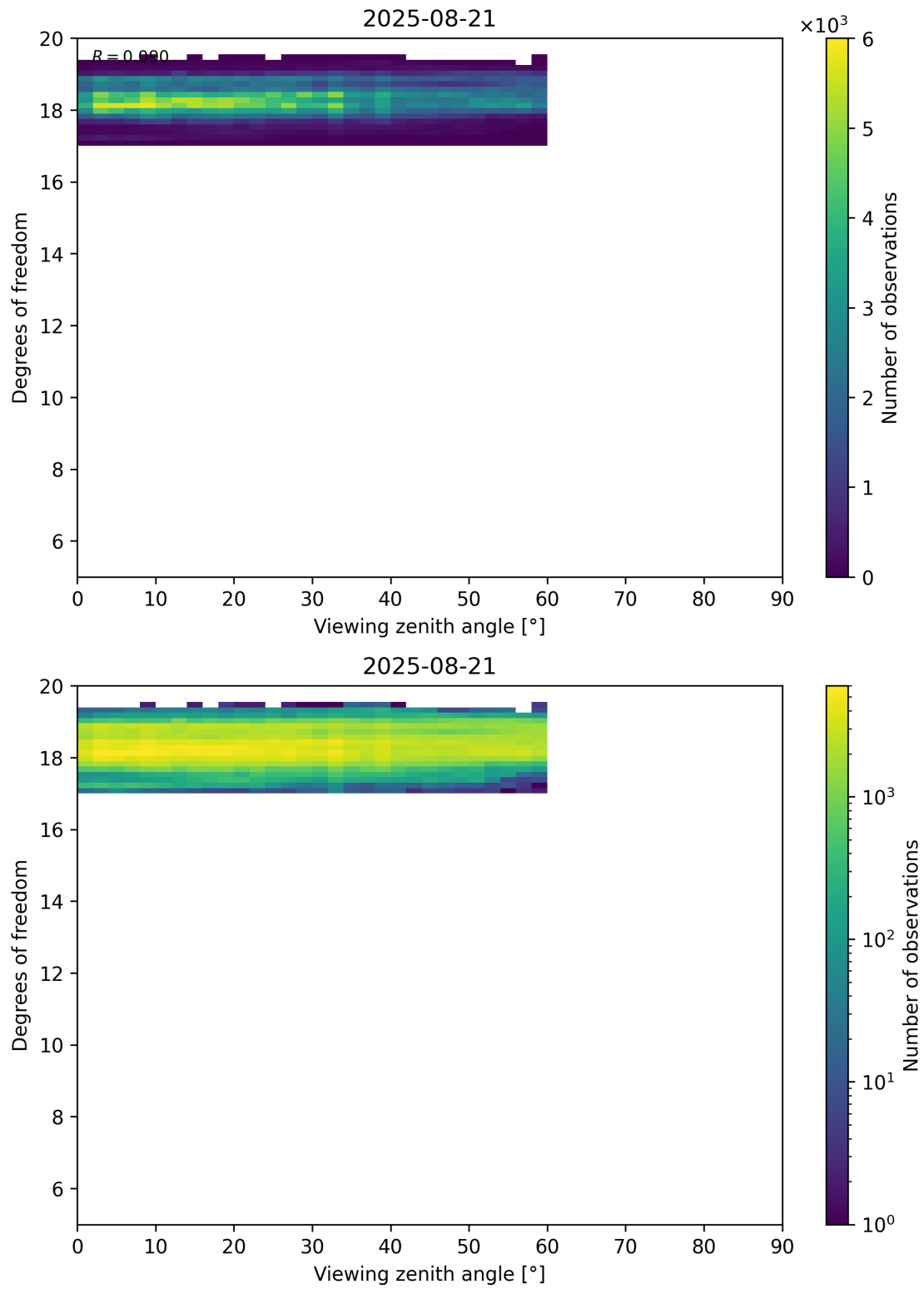
Figure 107: Scatter density plot of “Viewing zenith angle” against “Degrees of freedom” for 2025-08-20 to 2025-08-22.
