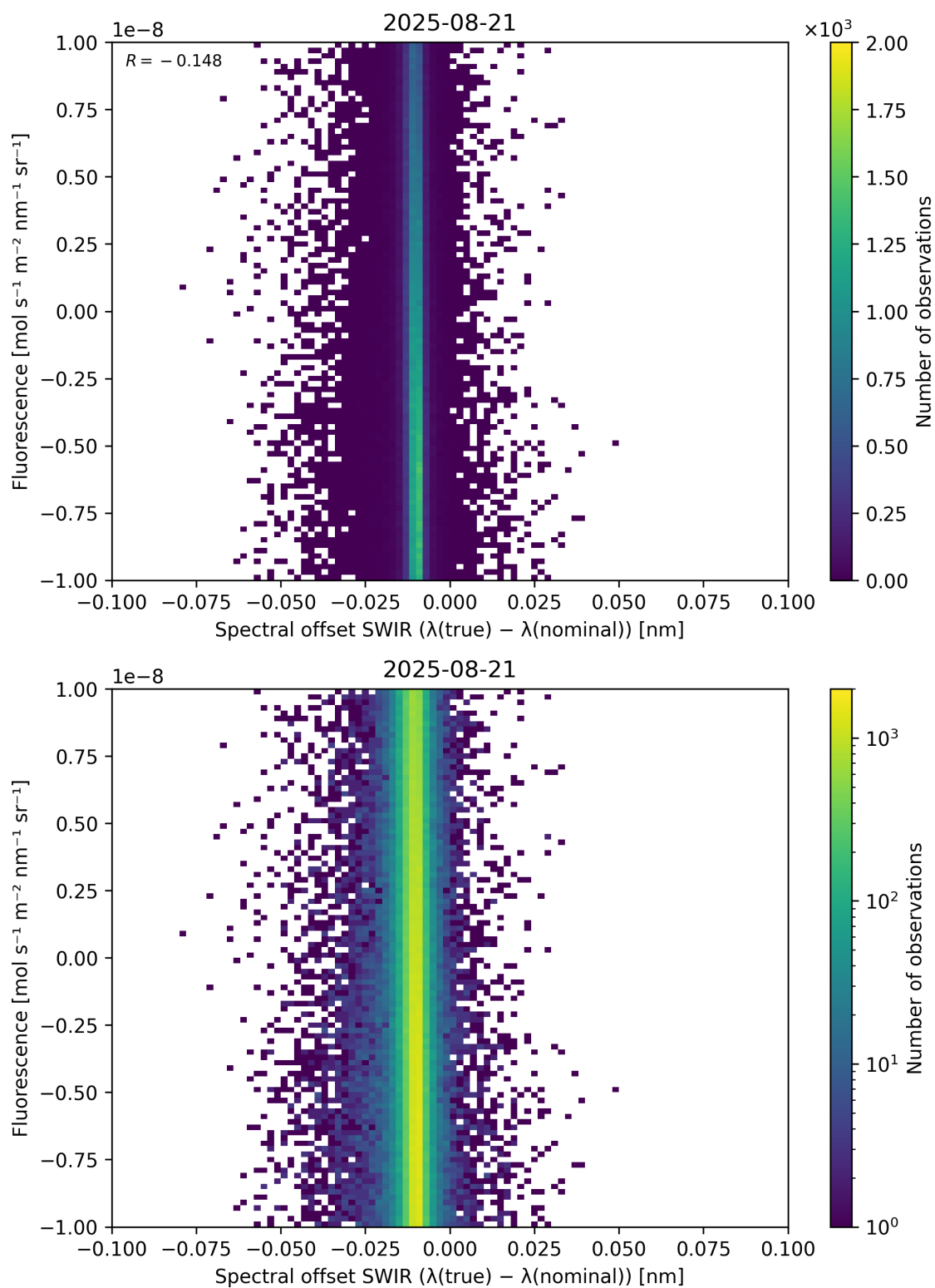
Figure 120: Scatter density plot of “Spectral offset SWIR ( \lambda_{\text{true}} - \lambda_{\text{nominal}} )” against “Fluorescence” for 2025-08-20 to 2025-08-22.
