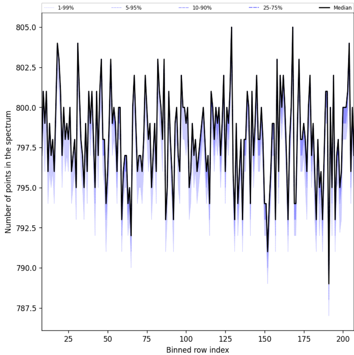
Figure 37: Along track statistics of “Number of points in the spectrum” for 2025-08-20 to 2025-08-22
