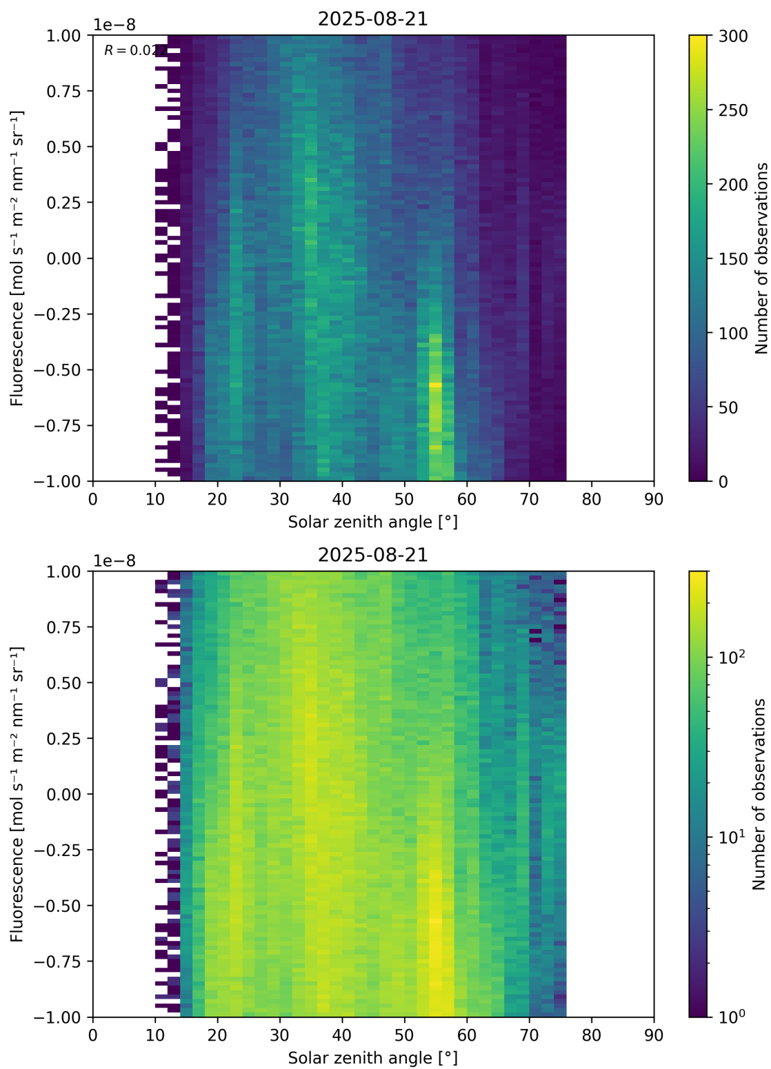
Figure 97: Scatter density plot of “Solar zenith angle” against “Fluorescence” for 2025-08-20 to 2025-08-22.
