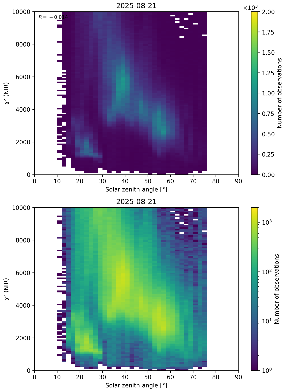
Figure 94: Scatter density plot of “Solar zenith angle” against “ \chi^2 (NIR)” for 2025-08-20 to 2025-08-22.
