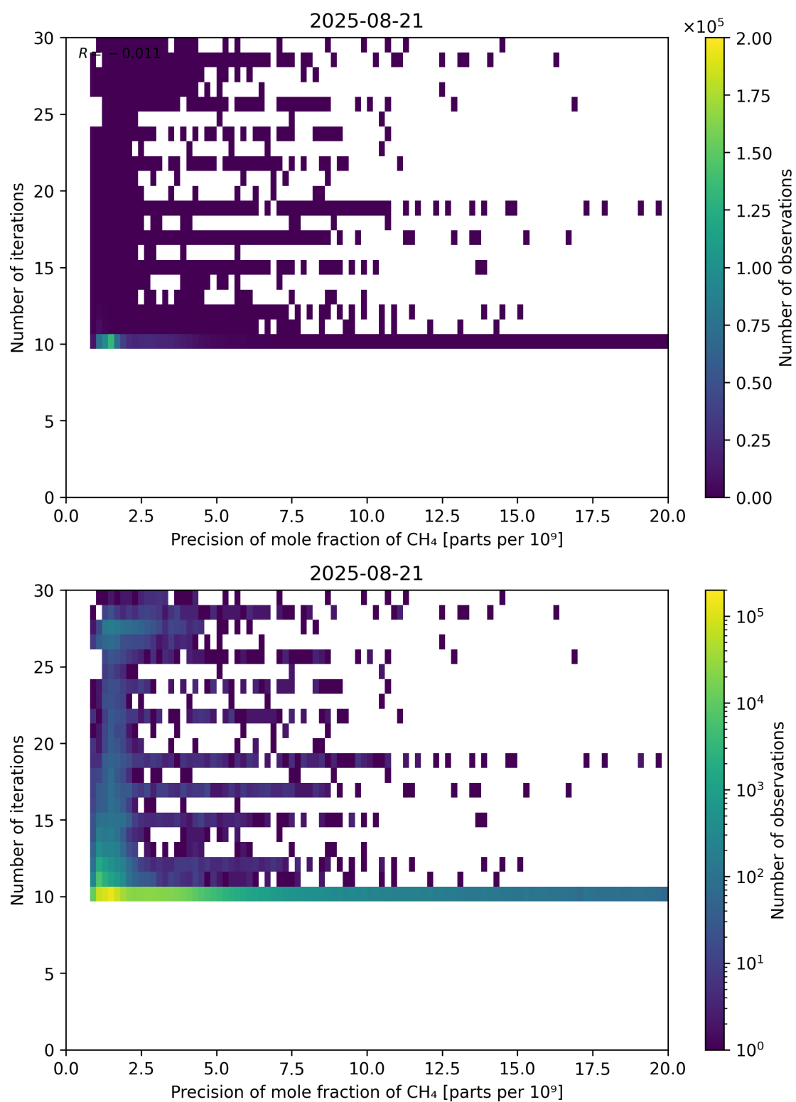
Figure 83: Scatter density plot of “Precision of mole fraction of CH 4 ” against “Number of iterations” for 2025-08-20 to 2025-08-22.
