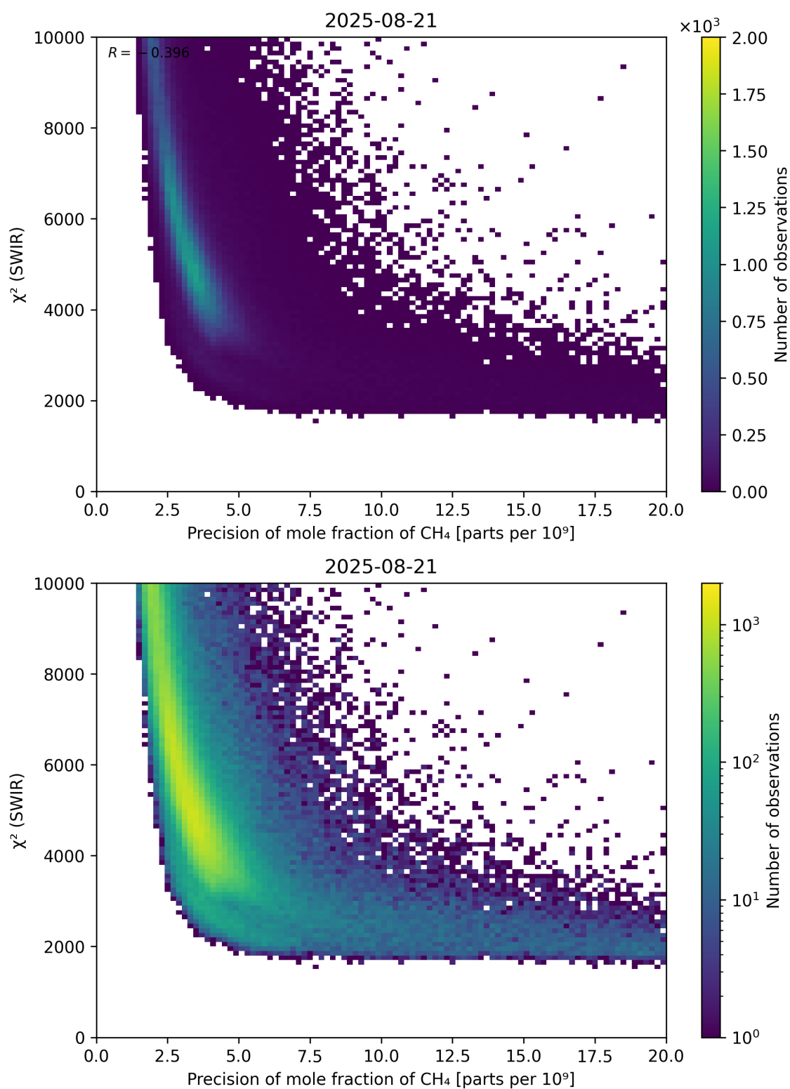
Figure 79: Scatter density plot of “Precision of mole fraction of \text{CH}_4 ” against “ \chi^2 (SWIR)” for 2025-08-20 to 2025-08-22.
