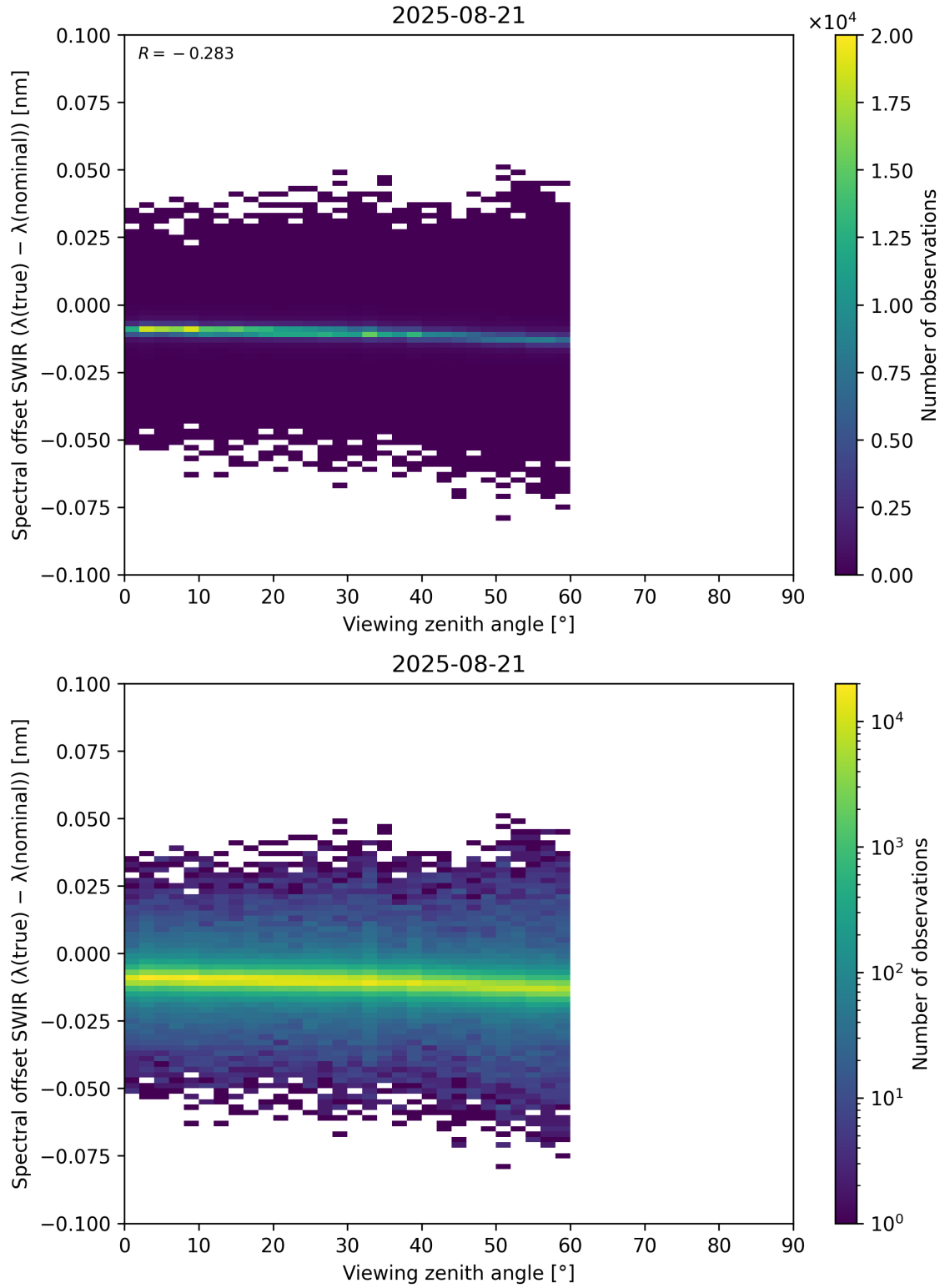
Figure 116: Scatter density plot of “Viewing zenith angle” against “Spectral offset SWIR ( \lambda_{\text{true}} - \lambda_{\text{nominal}} )” for 2025-08-20 to 2025-08-22.
