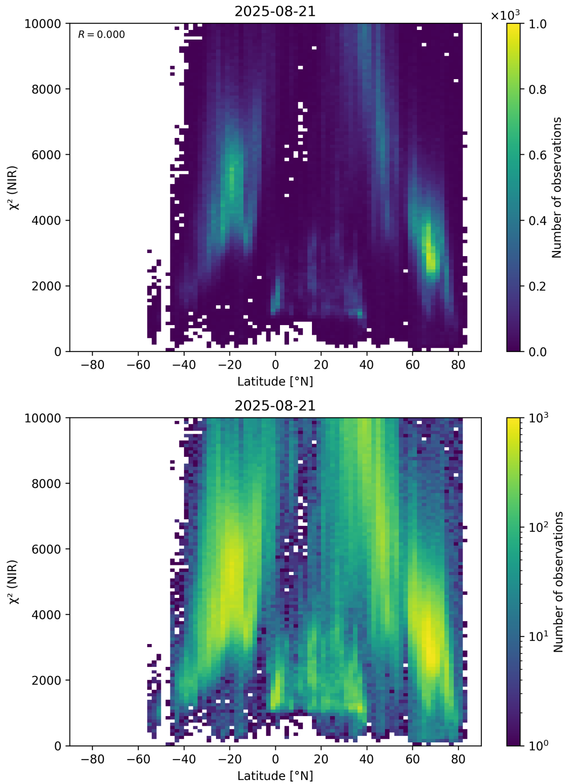
Figure 53: Scatter density plot of “Latitude” against “ \chi^2 (NIR)” for 2025-08-20 to 2025-08-22.
