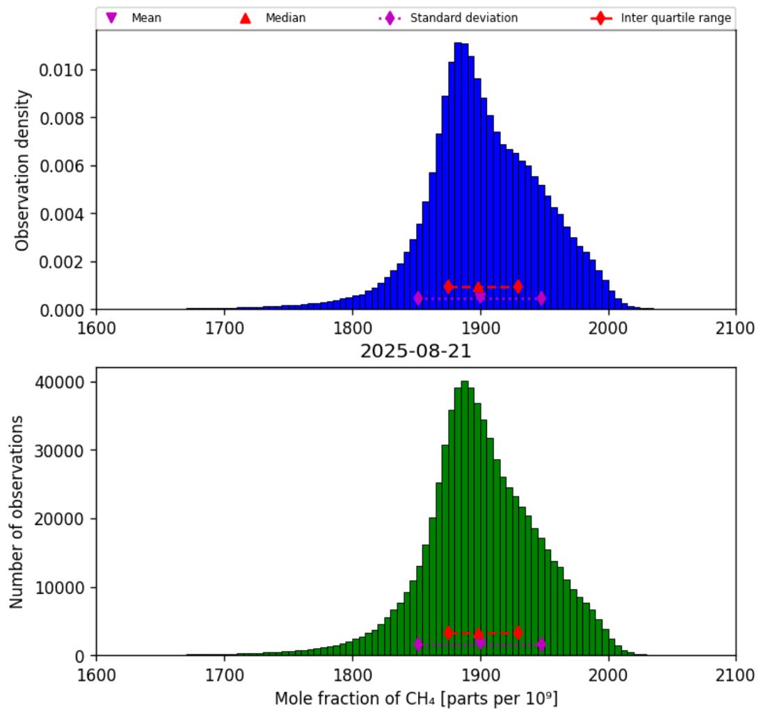
Figure 23: Histogram of “Mole fraction of CH 4 ” for 2025-08-20 to 2025-08-22
