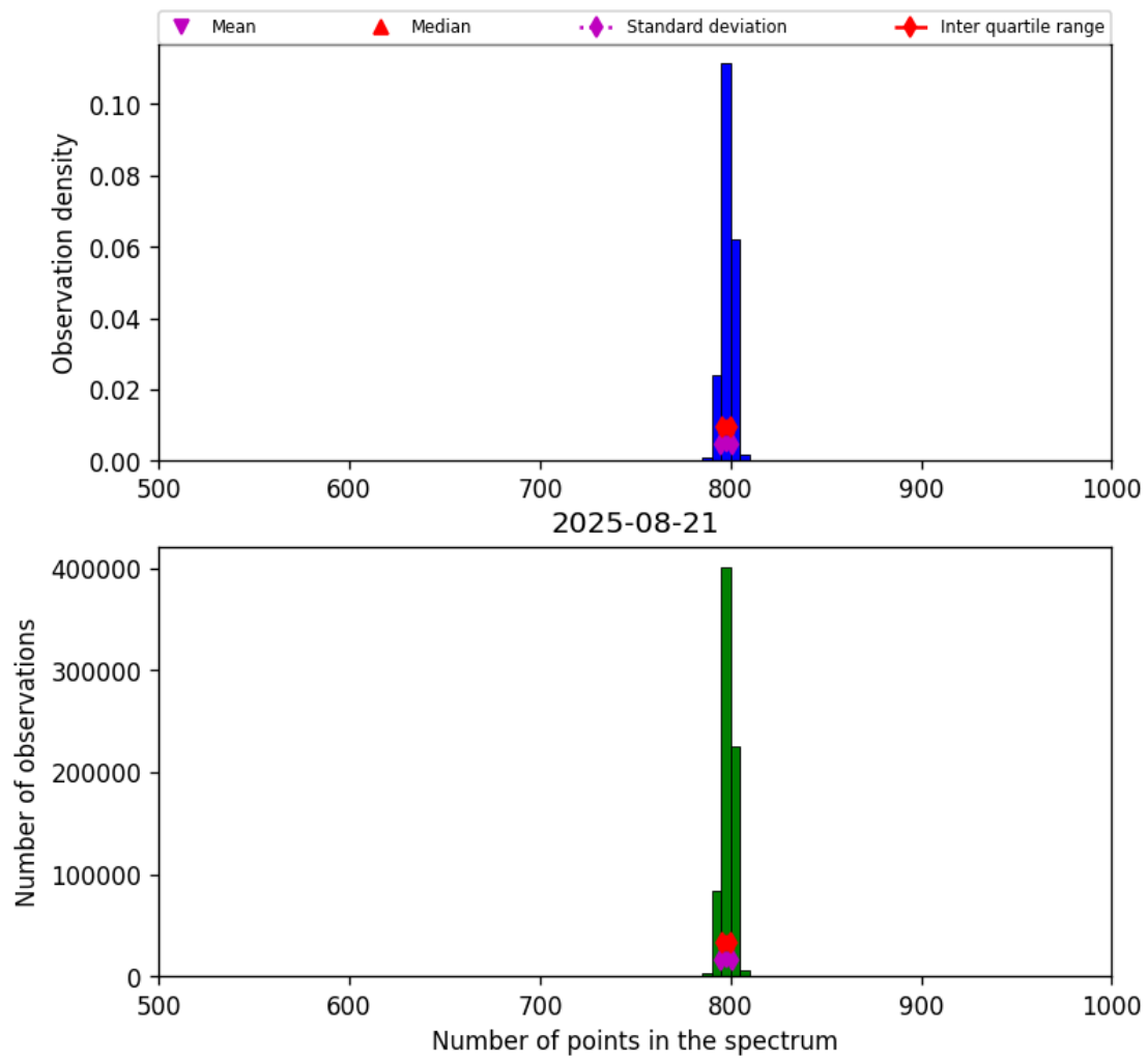
Figure 26: Histogram of “Number of points in the spectrum” for 2025-08-20 to 2025-08-22
