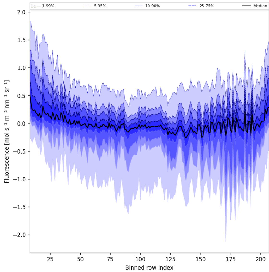
Figure 43: Along track statistics of “Fluorescence” for 2025-08-20 to 2025-08-22
