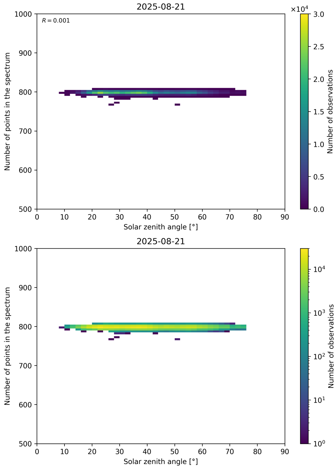
Figure 103: Scatter density plot of “Solar zenith angle” against “Number of points in the spectrum” for 2025-08-20 to 2025-08-22.
