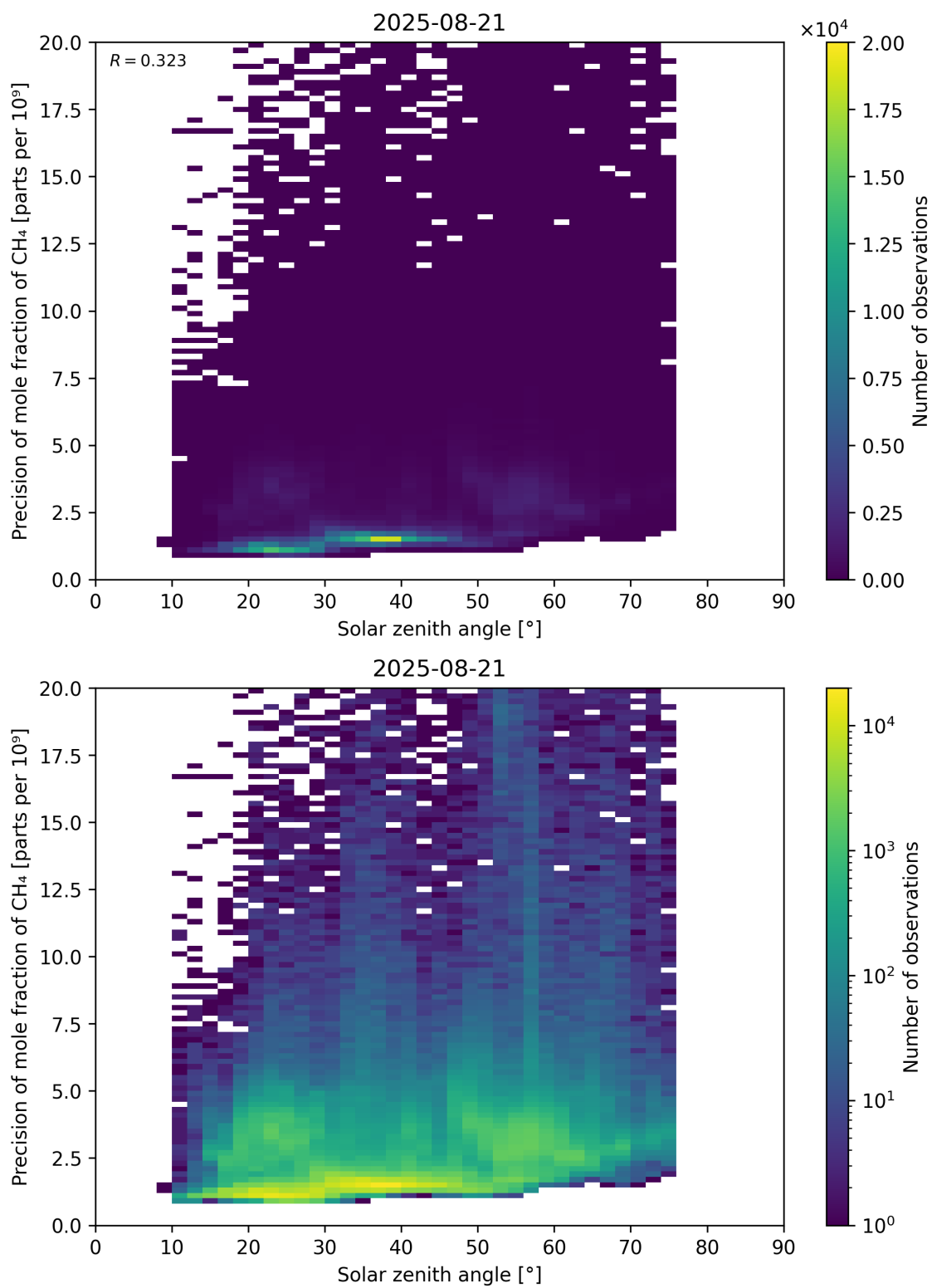
Figure 101: Scatter density plot of “Solar zenith angle” against “Precision of mole fraction of \text{CH}_4 ” for 2025-08-20 to 2025-08-22.
