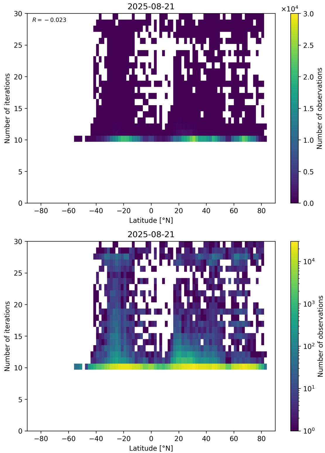
Figure 60: Scatter density plot of “Latitude” against “Number of iterations” for 2025-08-20 to 2025-08-22.
