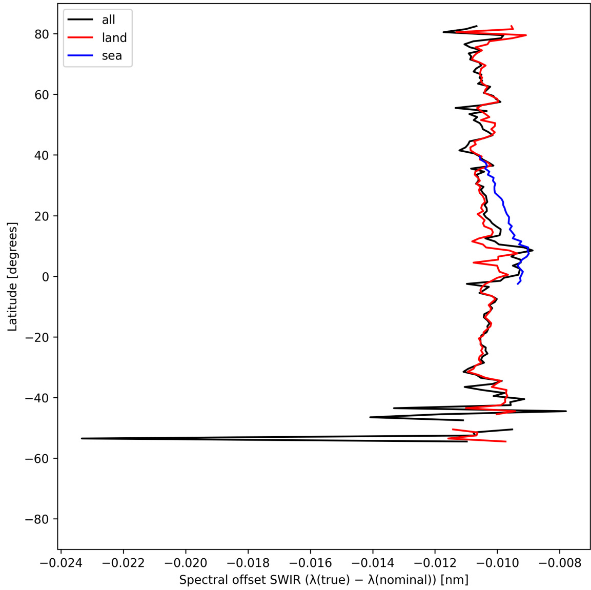
Figure 16: Zonal average of “Spectral offset SWIR ( \lambda_{\text{true}} - \lambda_{\text{nominal}} )” for 2025-08-20 to 2025-08-22.
