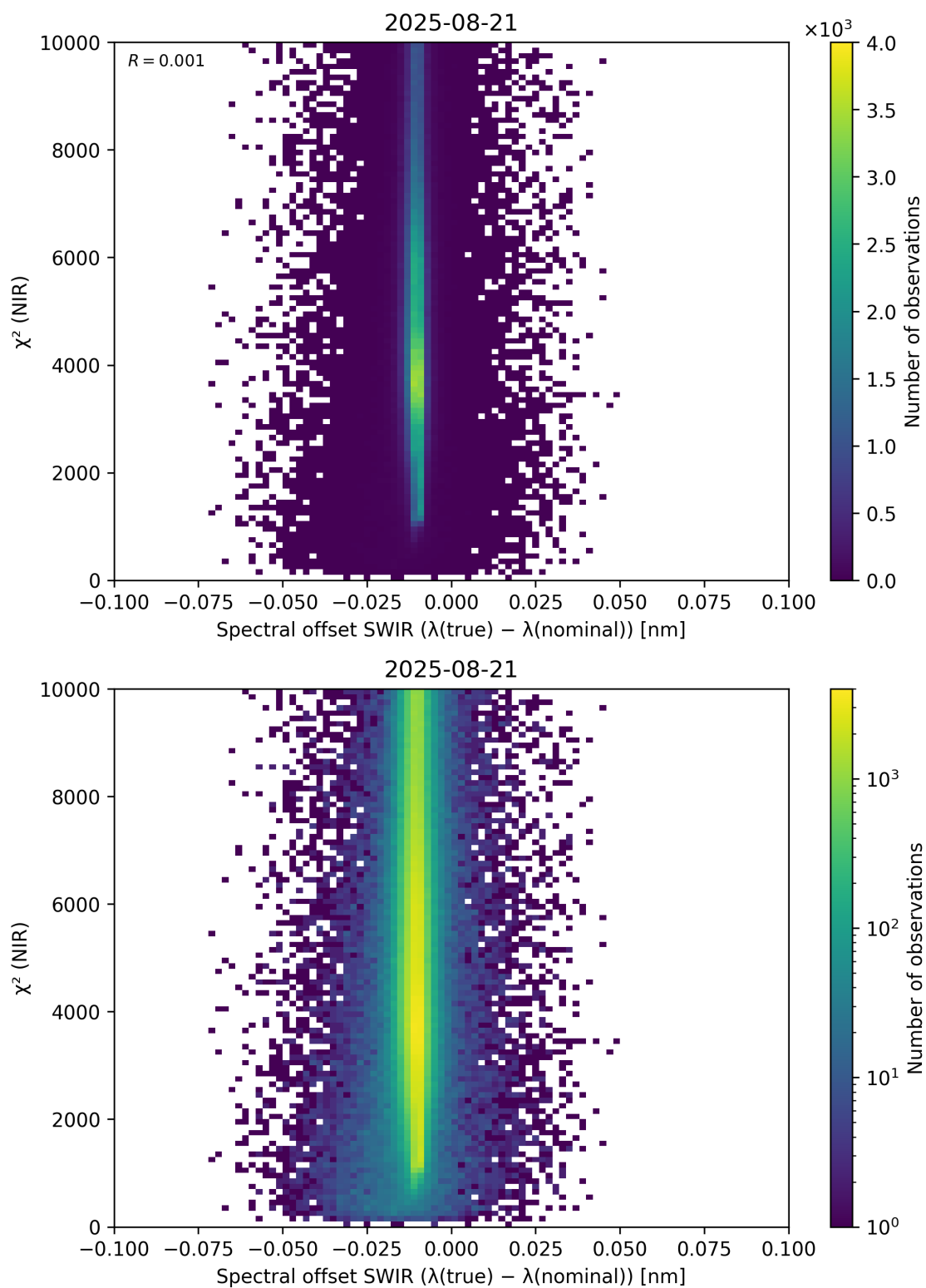
Figure 117: Scatter density plot of “Spectral offset SWIR ( \lambda_{\text{true}} - \lambda_{\text{nominal}} )” against “ \chi^2 (NIR)” for 2025-08-20 to 2025-08-22.
