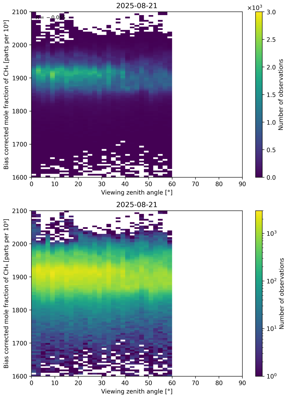
Figure 111: Scatter density plot of “Viewing zenith angle” against “Bias corrected mole fraction of CH 4 ” for 2025-08-20 to 2025-08-22.
