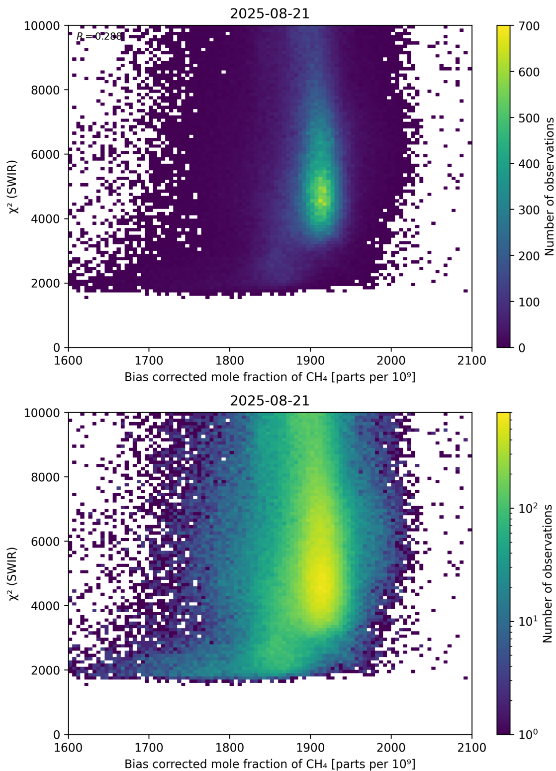
Figure 64: Scatter density plot of “Bias corrected mole fraction of \text{CH}_4 ” against “ \chi^2 (SWIR)” for 2025-08-20 to 2025-08-22.
