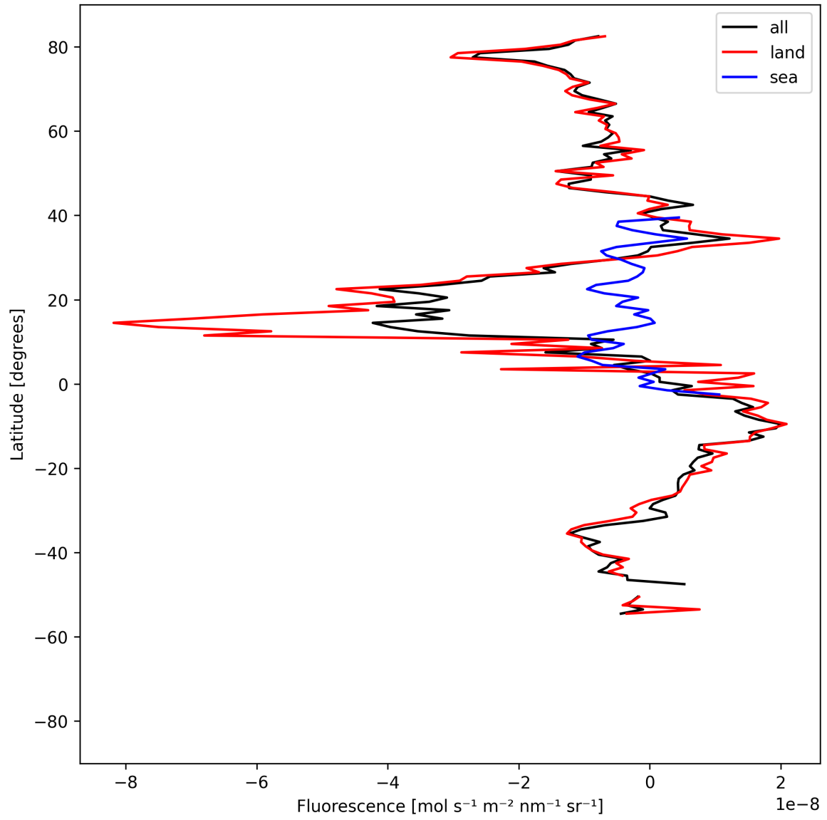
Figure 21: Zonal average of “Fluorescence” for 2025-08-20 to 2025-08-22.
