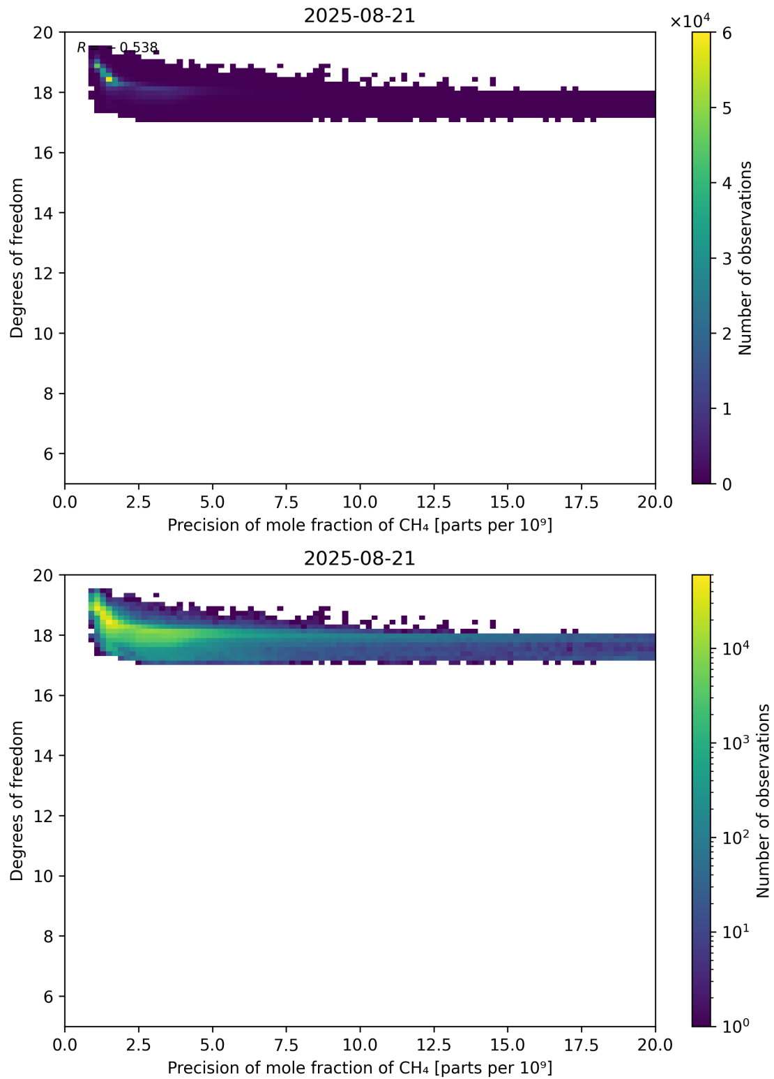
Figure 80: Scatter density plot of “Precision of mole fraction of CH 4 ” against “Degrees of freedom” for 2025-08-20 to 2025-08-22.
