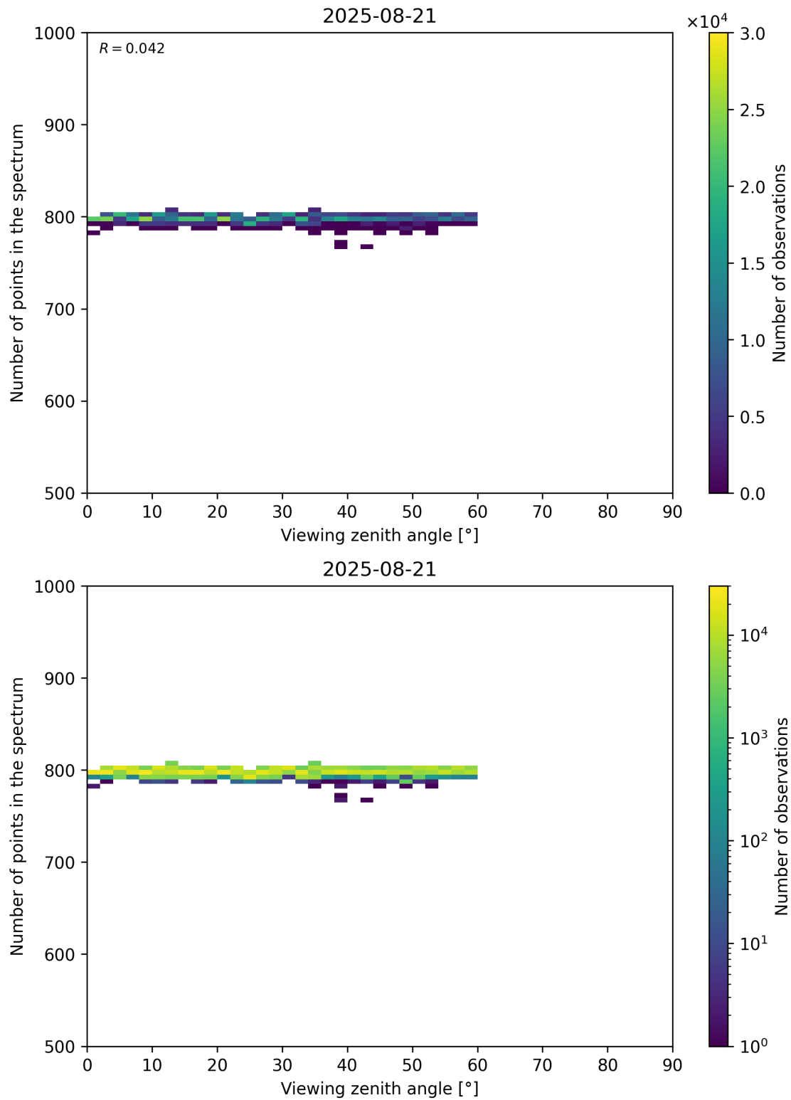
Figure 114: Scatter density plot of “Viewing zenith angle” against “Number of points in the spectrum” for 2025-08-20 to 2025-08-22.
