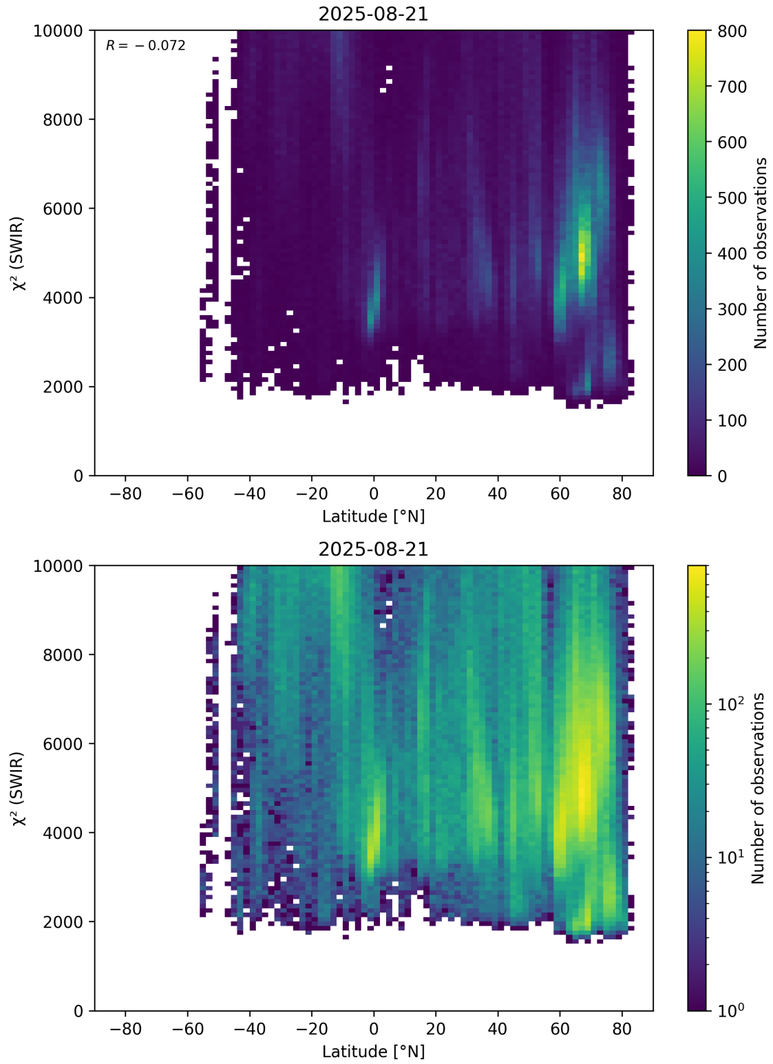
Figure 54: Scatter density plot of “Latitude” against “ \chi^2 (SWIR)” for 2025-08-20 to 2025-08-22.
