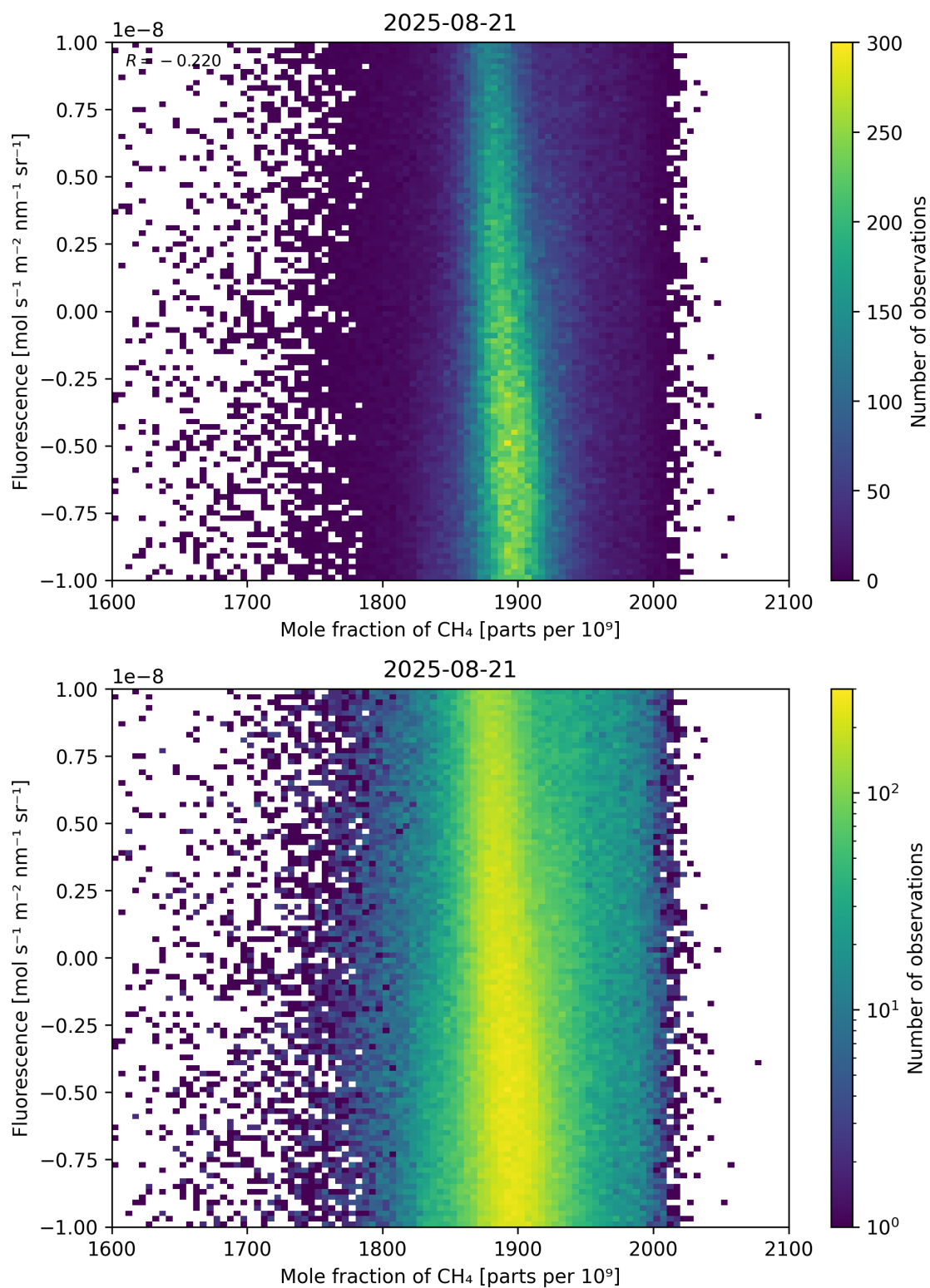
Figure 73: Scatter density plot of “Mole fraction of \text{CH}_4 ” against “Fluorescence” for 2025-08-20 to 2025-08-22.
