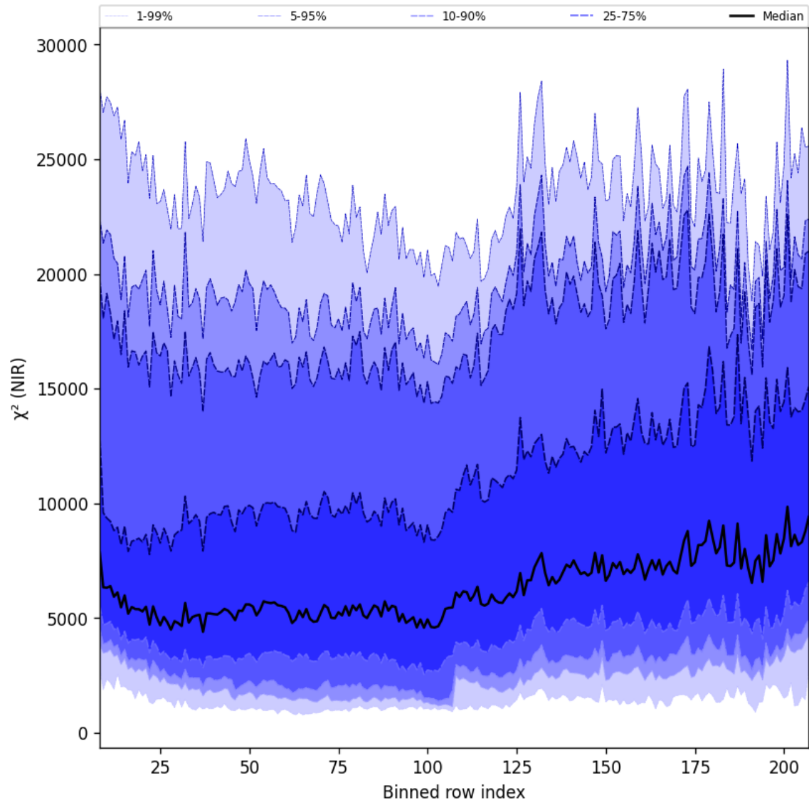
Figure 40: Along track statistics of “ \chi^2 (NIR)” for 2025-08-20 to 2025-08-22
