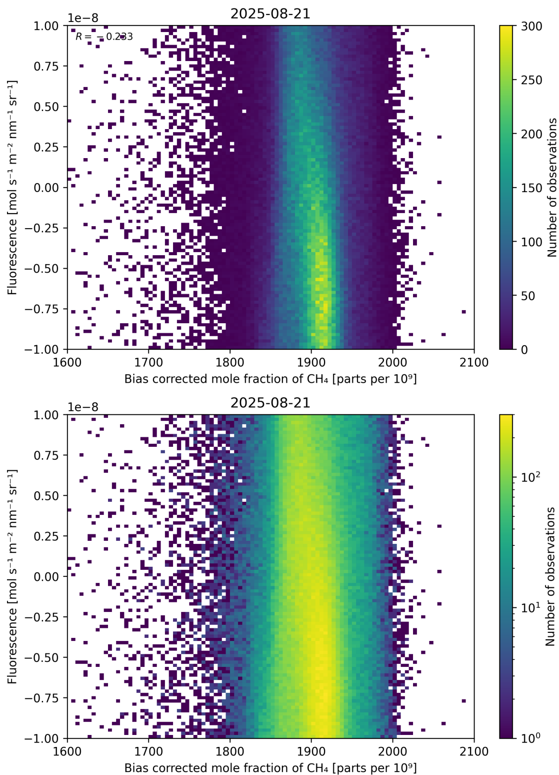
Figure 66: Scatter density plot of “Bias corrected mole fraction of \text{CH}_4 ” against “Fluorescence” for 2025-08-20 to 2025-08-22.
