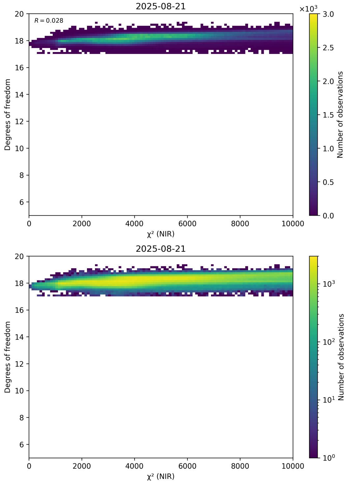
Figure 44: Scatter density plot of “ \chi^2 (NIR)” against “Degrees of freedom” for 2025-08-20 to 2025-08-22.
