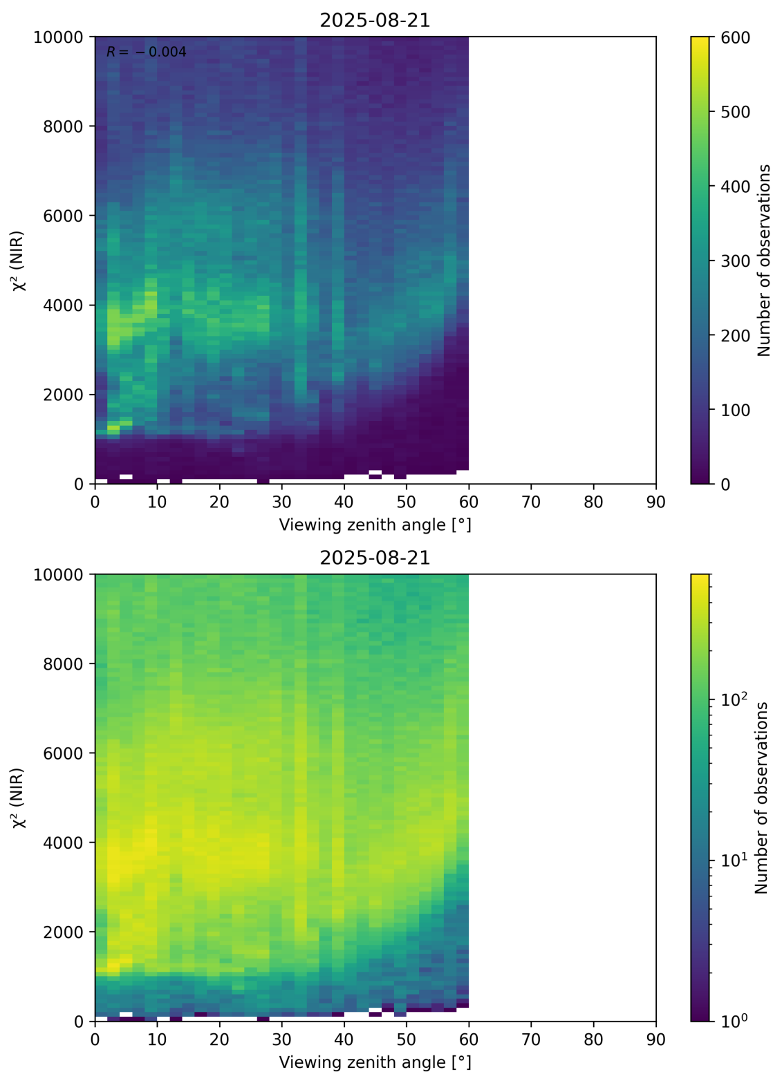
Figure 105: Scatter density plot of “Viewing zenith angle” against “ \chi^2 (NIR)” for 2025-08-20 to 2025-08-22.
