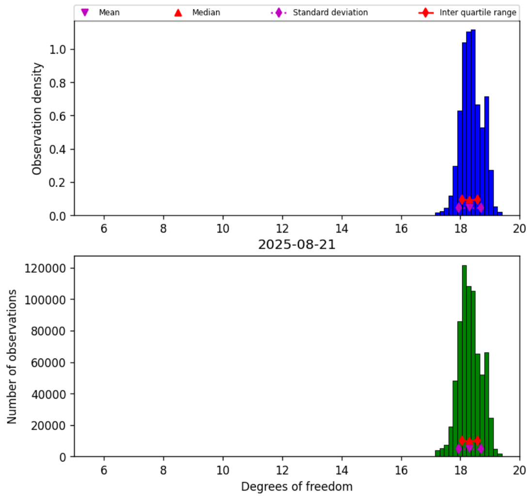
Figure 30: Histogram of “Degrees of freedom” for 2025-08-20 to 2025-08-22
