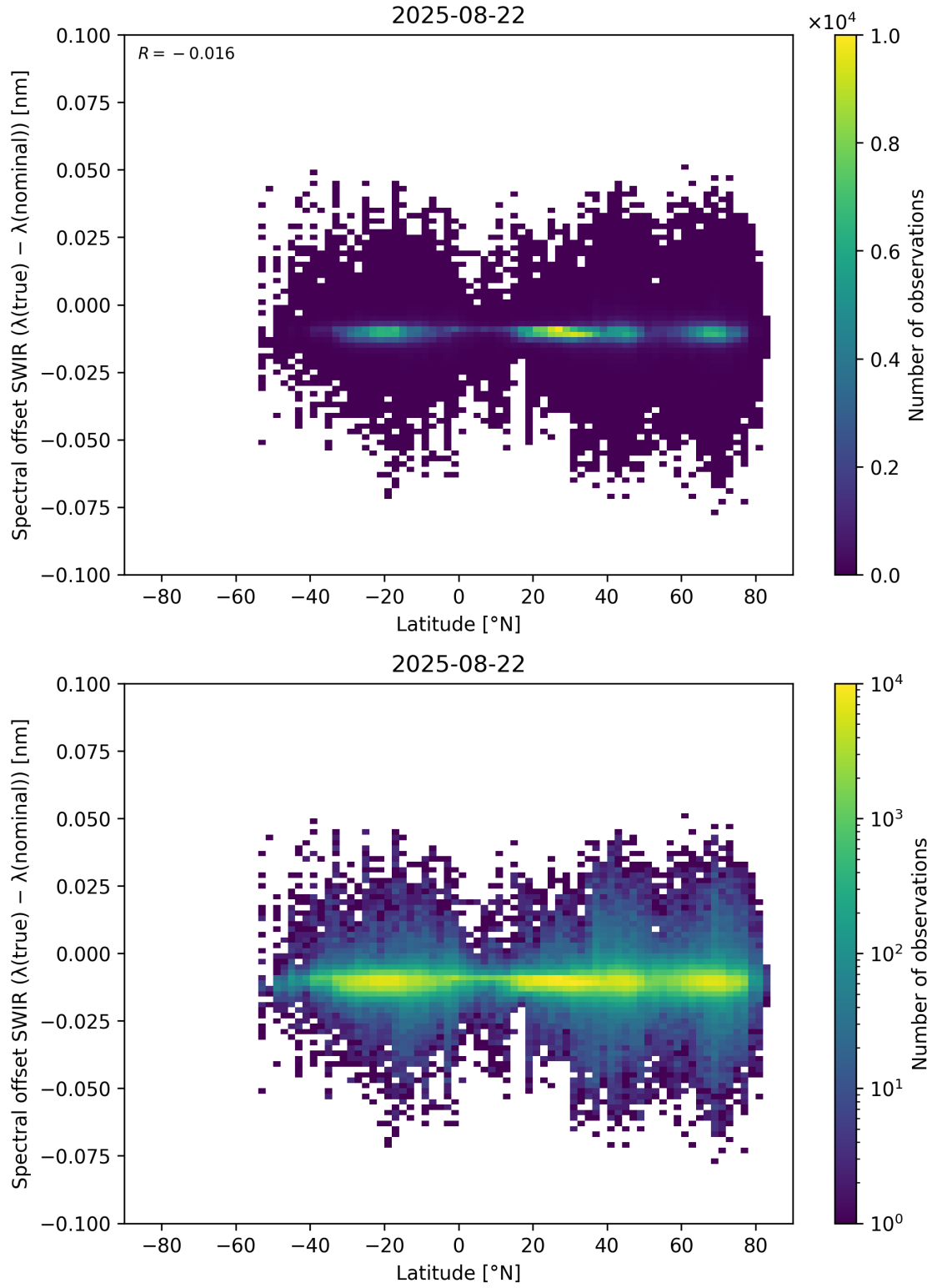
Figure 62: Scatter density plot of “Latitude” against “Spectral offset SWIR ( \lambda_{\text{true}} - \lambda_{\text{nominal}} )” for 2025-08-21 to 2025-08-23.
