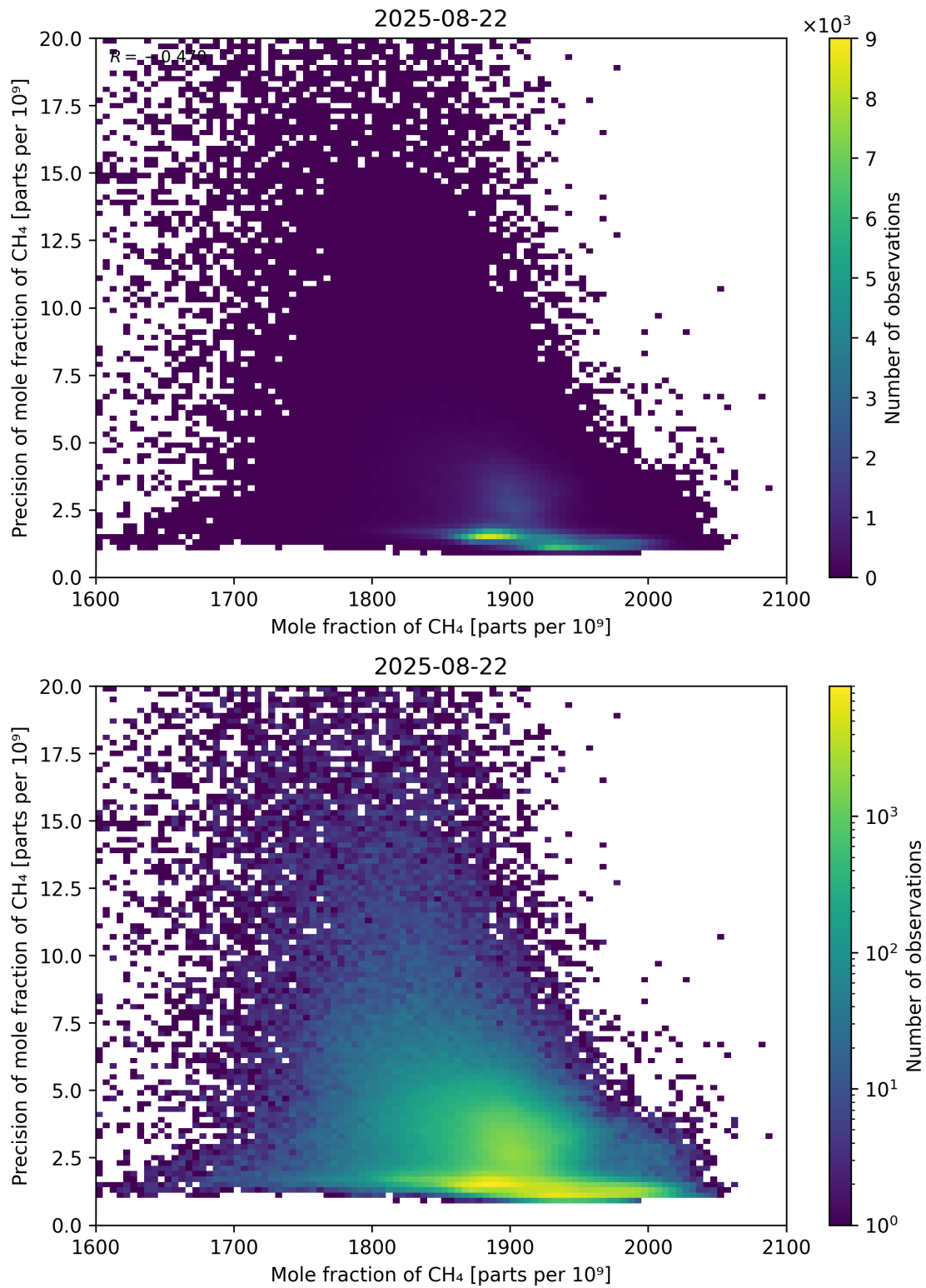
Figure 75: Scatter density plot of “Mole fraction of CH 4 ” against “Precision of mole fraction of CH 4 ” for 2025-08-21 to 2025-08-23.
