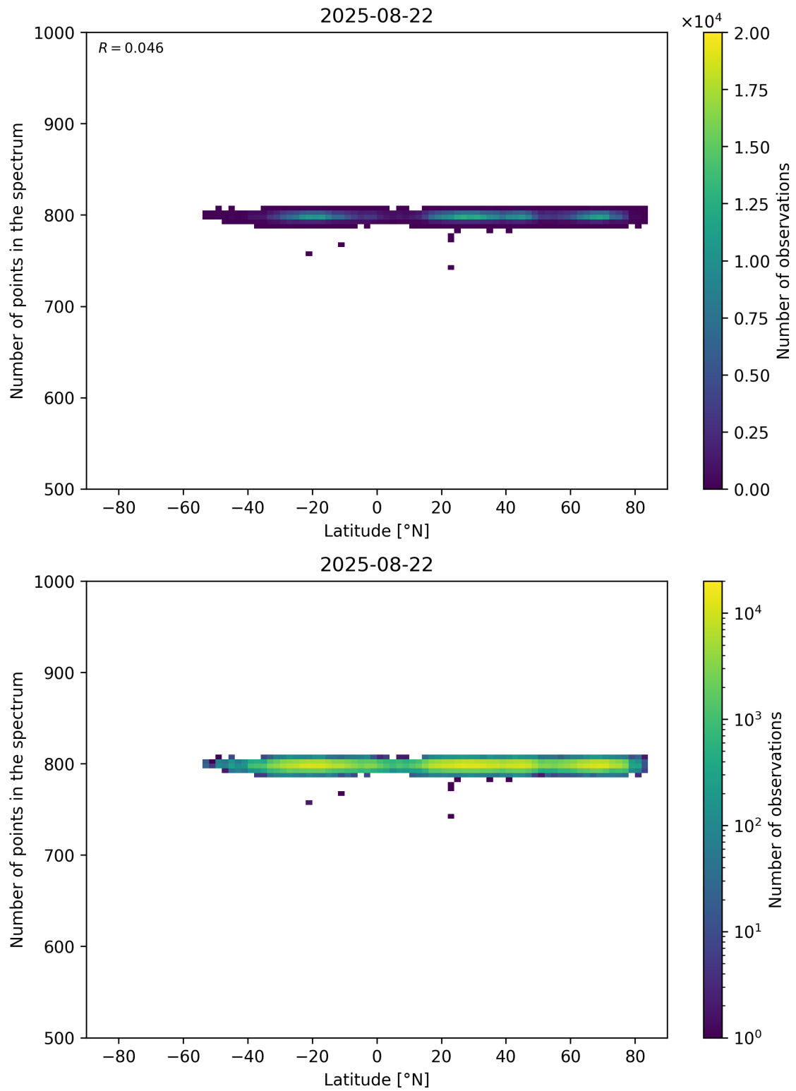
Figure 61: Scatter density plot of “Latitude” against “Number of points in the spectrum” for 2025-08-21 to 2025-08-23.
