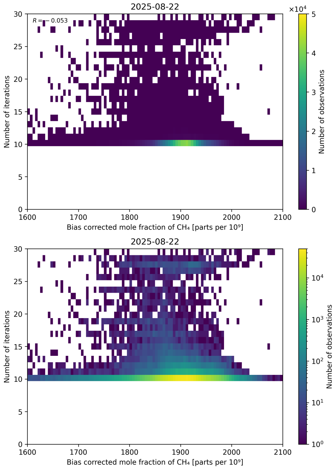
Figure 67: Scatter density plot of “Bias corrected mole fraction of CH 4 ” against “Number of iterations” for 2025-08-21 to 2025-08-23.
