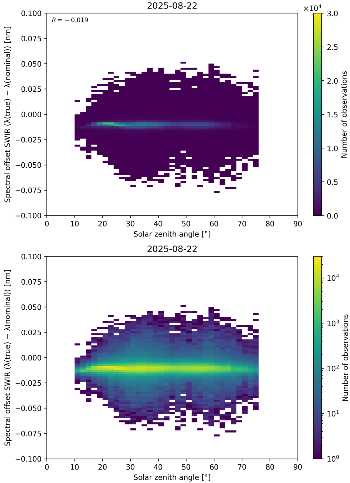
Figure 104: Scatter density plot of “Solar zenith angle” against “Spectral offset SWIR ( \lambda_{\text{true}} - \lambda_{\text{nominal}} )” for 2025-08-21 to 2025-08-23.
