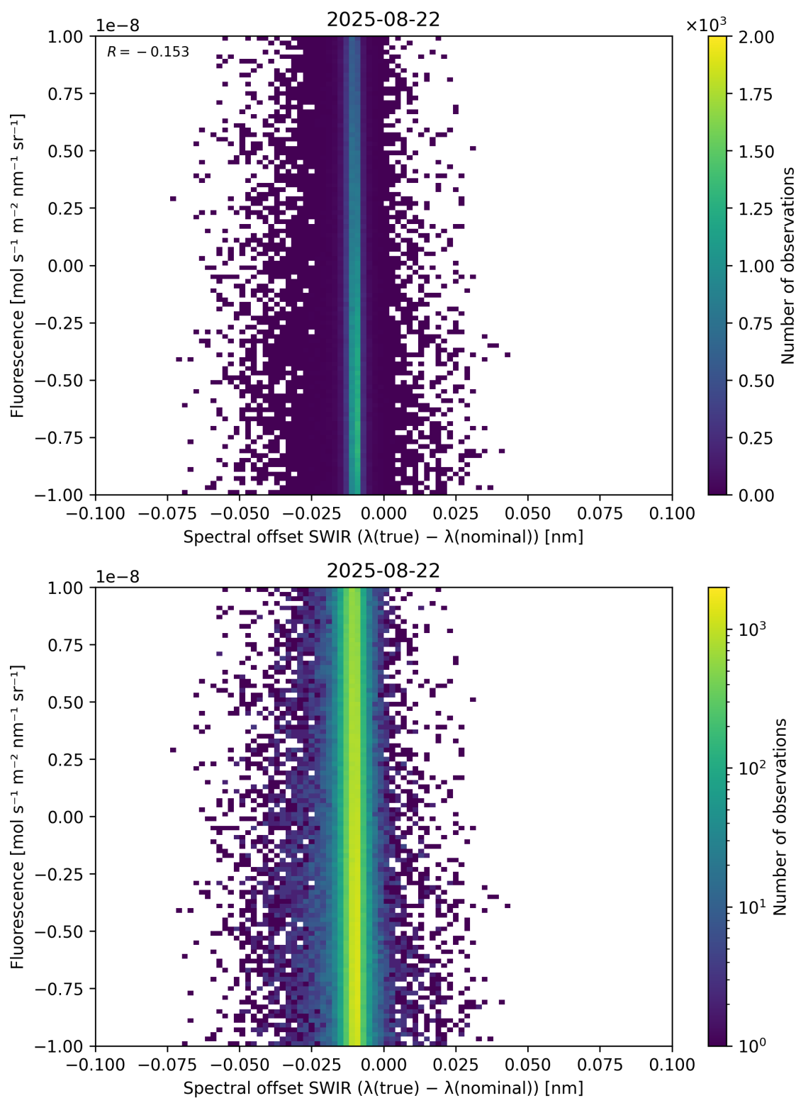
Figure 120: Scatter density plot of “Spectral offset SWIR ( \lambda_{\text{true}} - \lambda_{\text{nominal}} )” against “Fluorescence” for 2025-08-21 to 2025-08-23.
