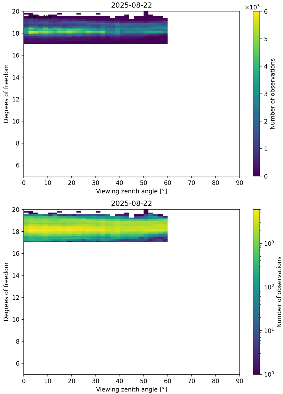
Figure 107: Scatter density plot of “Viewing zenith angle” against “Degrees of freedom” for 2025-08-21 to 2025-08-23.
