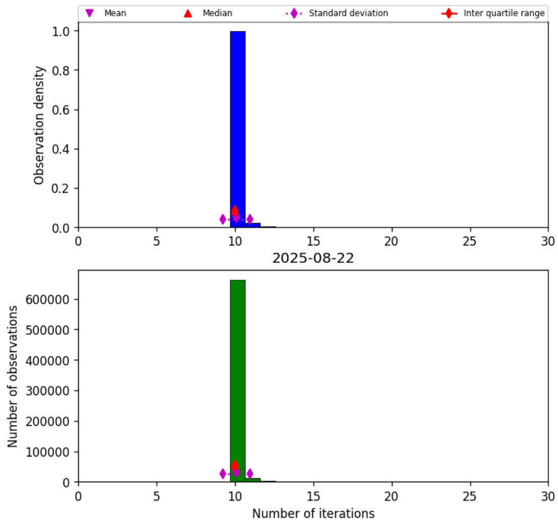
Figure 31: Histogram of “Number of iterations” for 2025-08-21 to 2025-08-23
