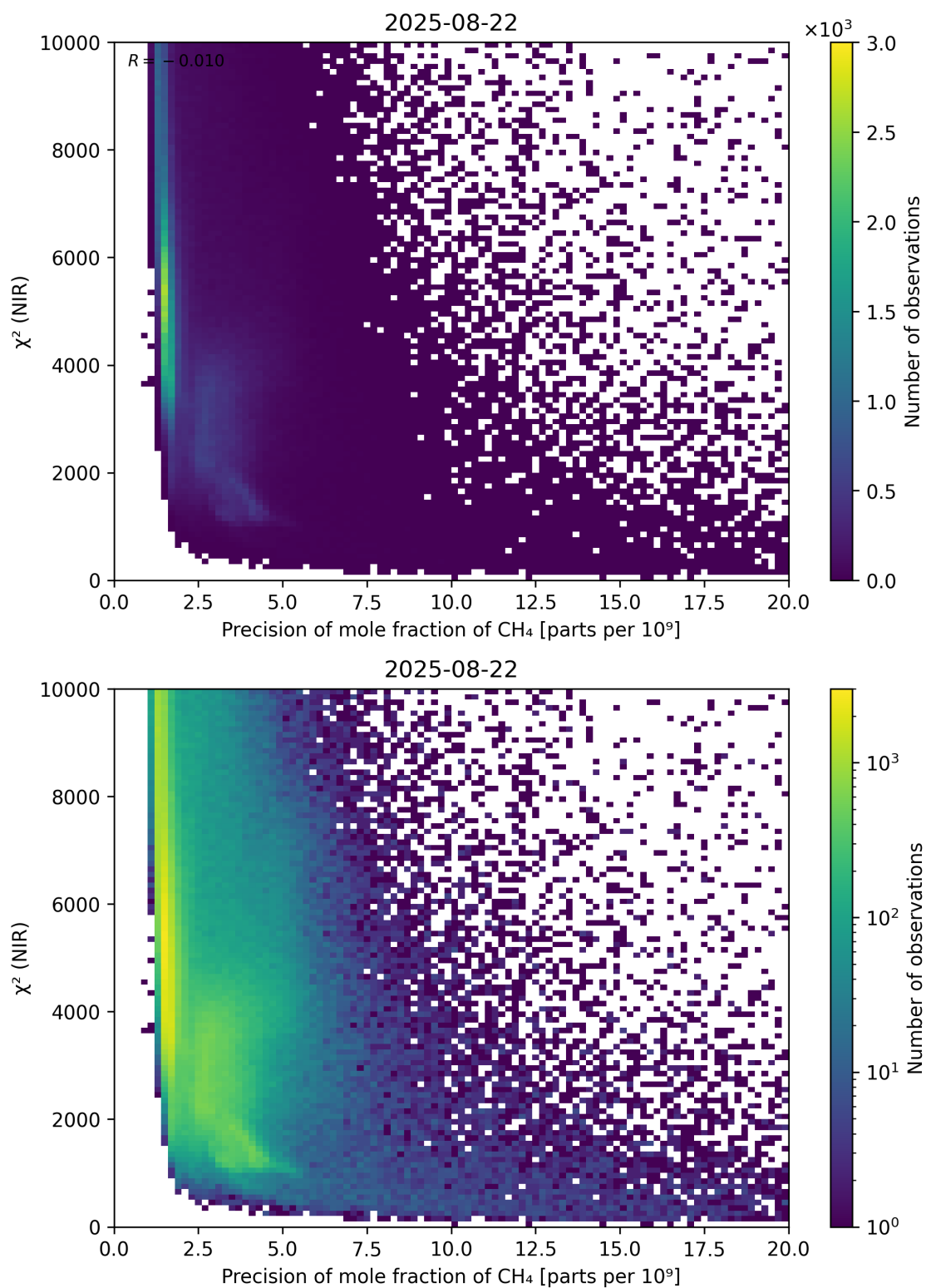
Figure 78: Scatter density plot of “Precision of mole fraction of CH 4 ” against “ \chi^2 (NIR)” for 2025-08-21 to 2025-08-23.
