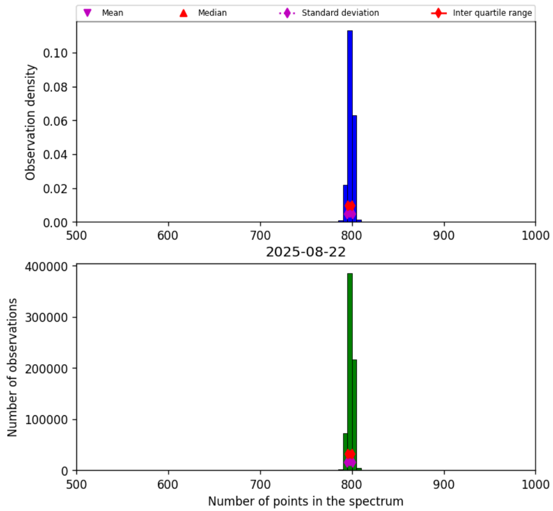
Figure 26: Histogram of “Number of points in the spectrum” for 2025-08-21 to 2025-08-23
