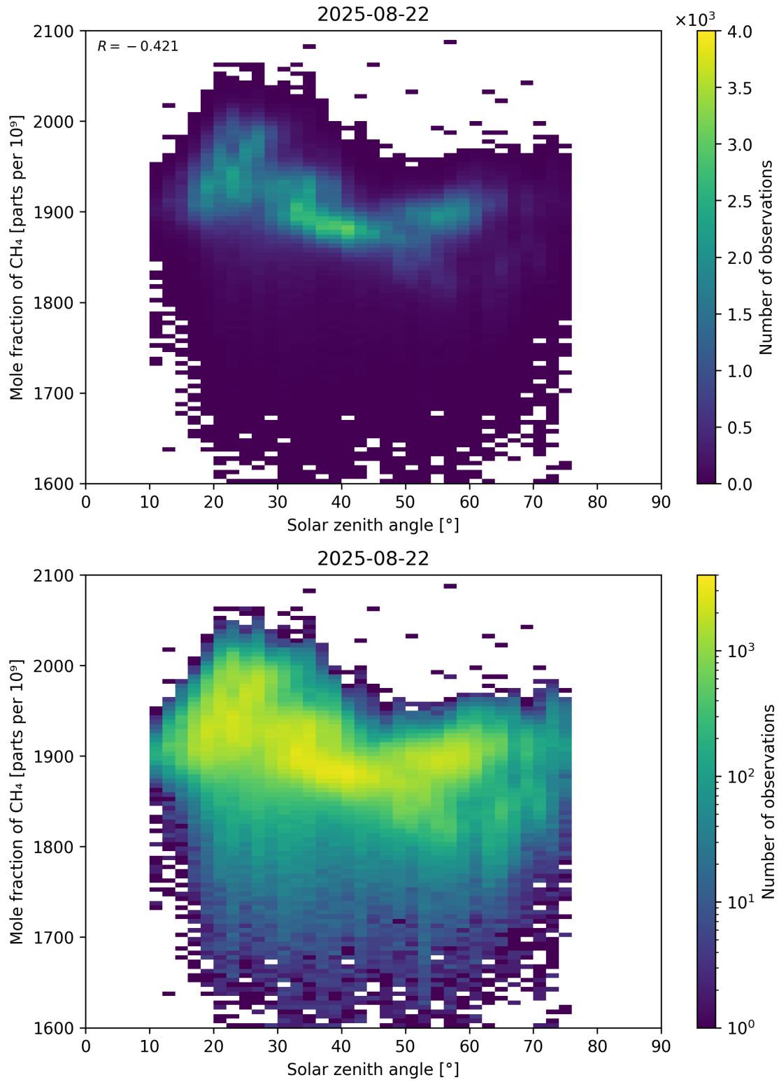
Figure 99: Scatter density plot of “Solar zenith angle” against “Mole fraction of CH 4 ” for 2025-08-21 to 2025-08-23.
