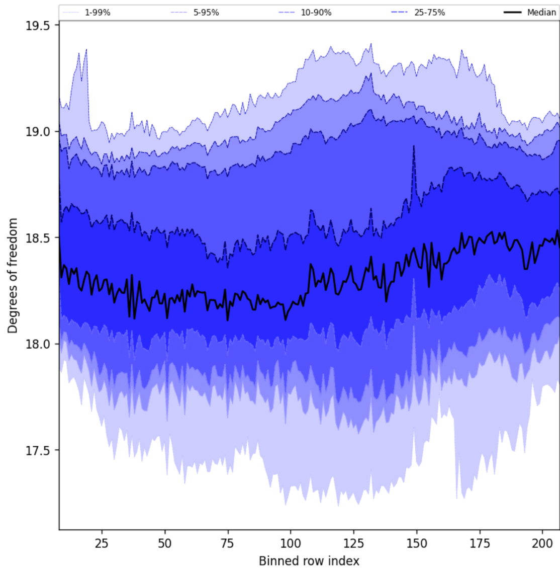
Figure 41: Along track statistics of “Degrees of freedom” for 2025-08-21 to 2025-08-23
