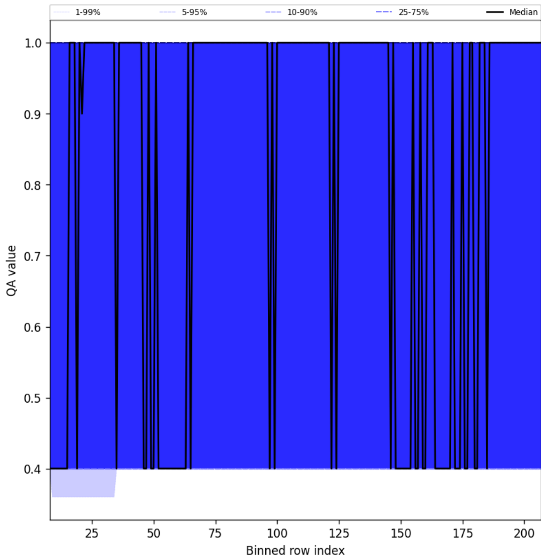
Figure 33: Along track statistics of “QA value” for 2025-08-21 to 2025-08-23
