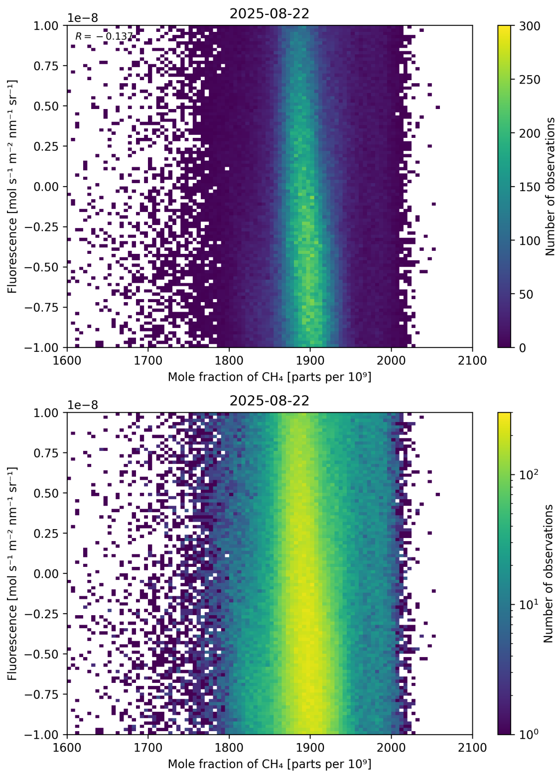
Figure 73: Scatter density plot of “Mole fraction of CH 4 ” against “Fluorescence” for 2025-08-21 to 2025-08-23.
