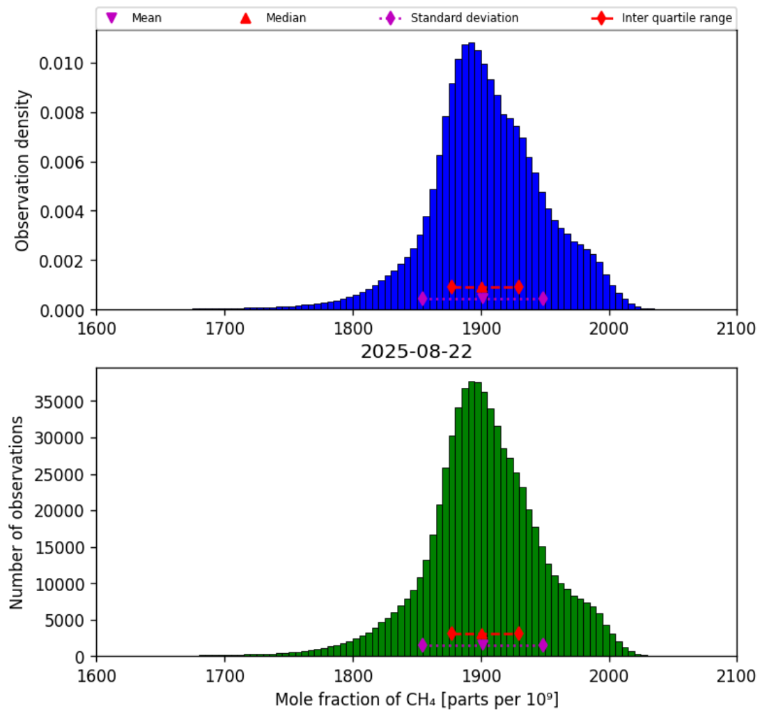
Figure 23: Histogram of “Mole fraction of CH 4 ” for 2025-08-21 to 2025-08-23
