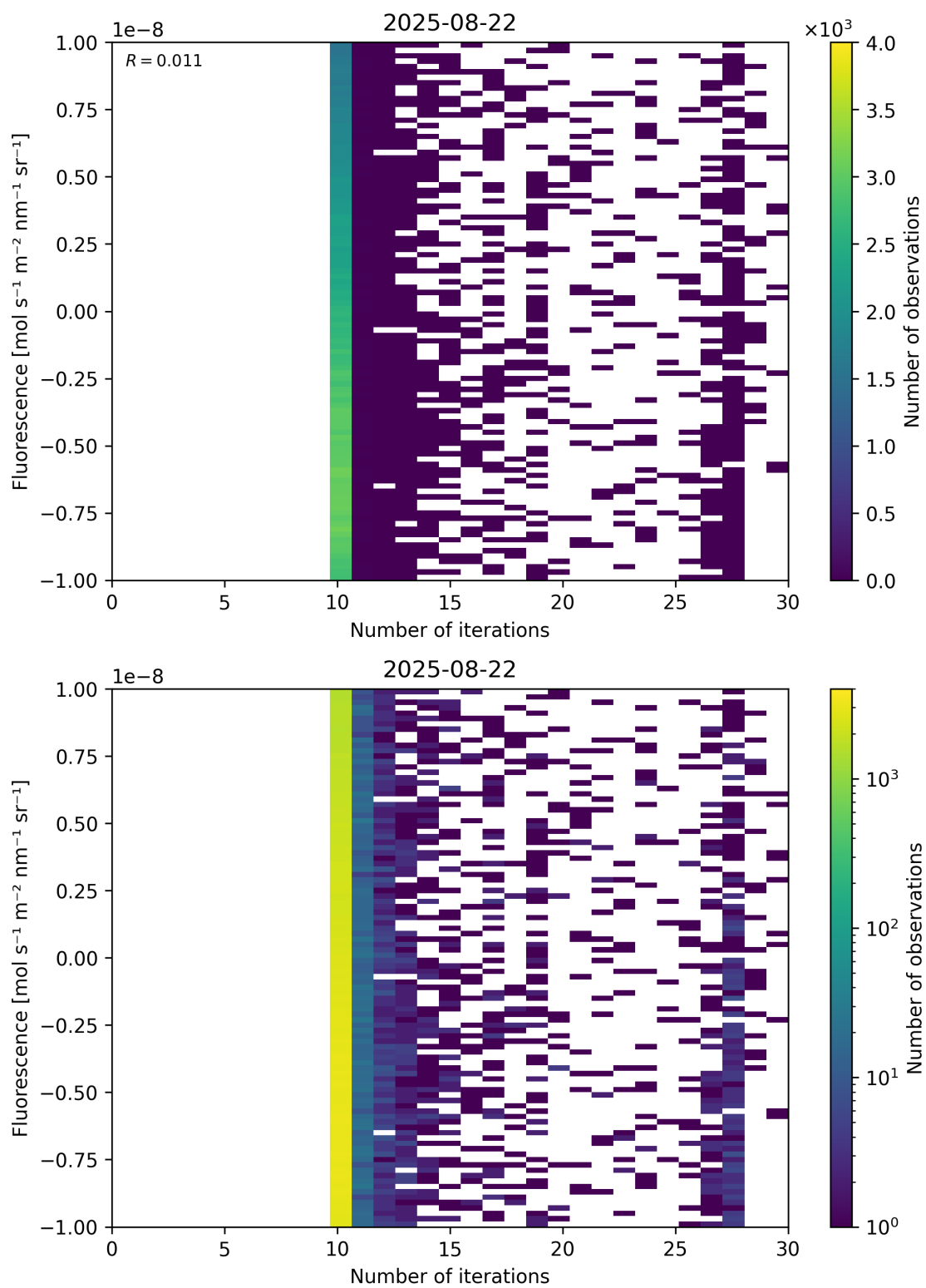
Figure 87: Scatter density plot of “Number of iterations” against “Fluorescence” for 2025-08-21 to 2025-08-23.
