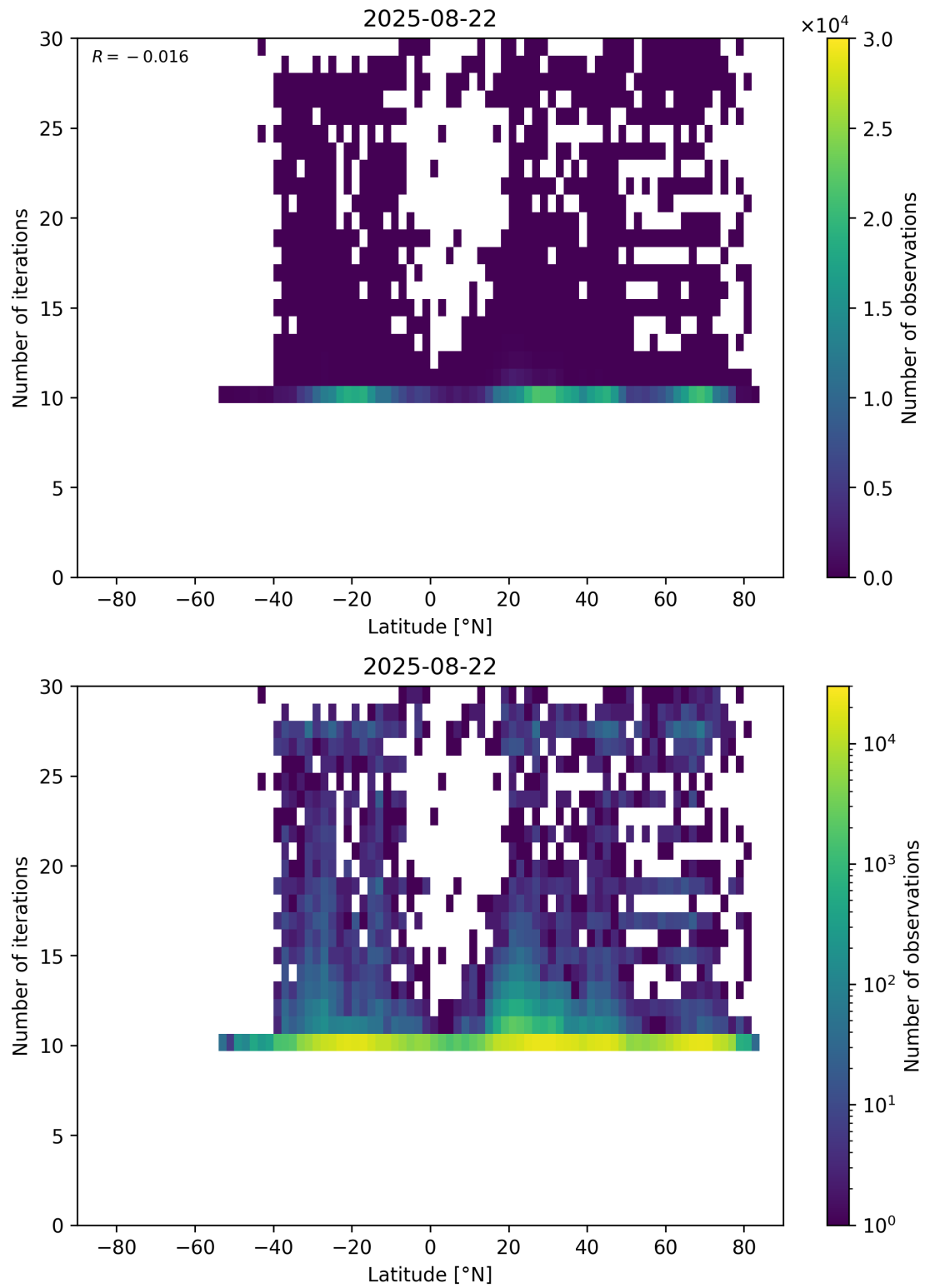
Figure 60: Scatter density plot of “Latitude” against “Number of iterations” for 2025-08-21 to 2025-08-23.
