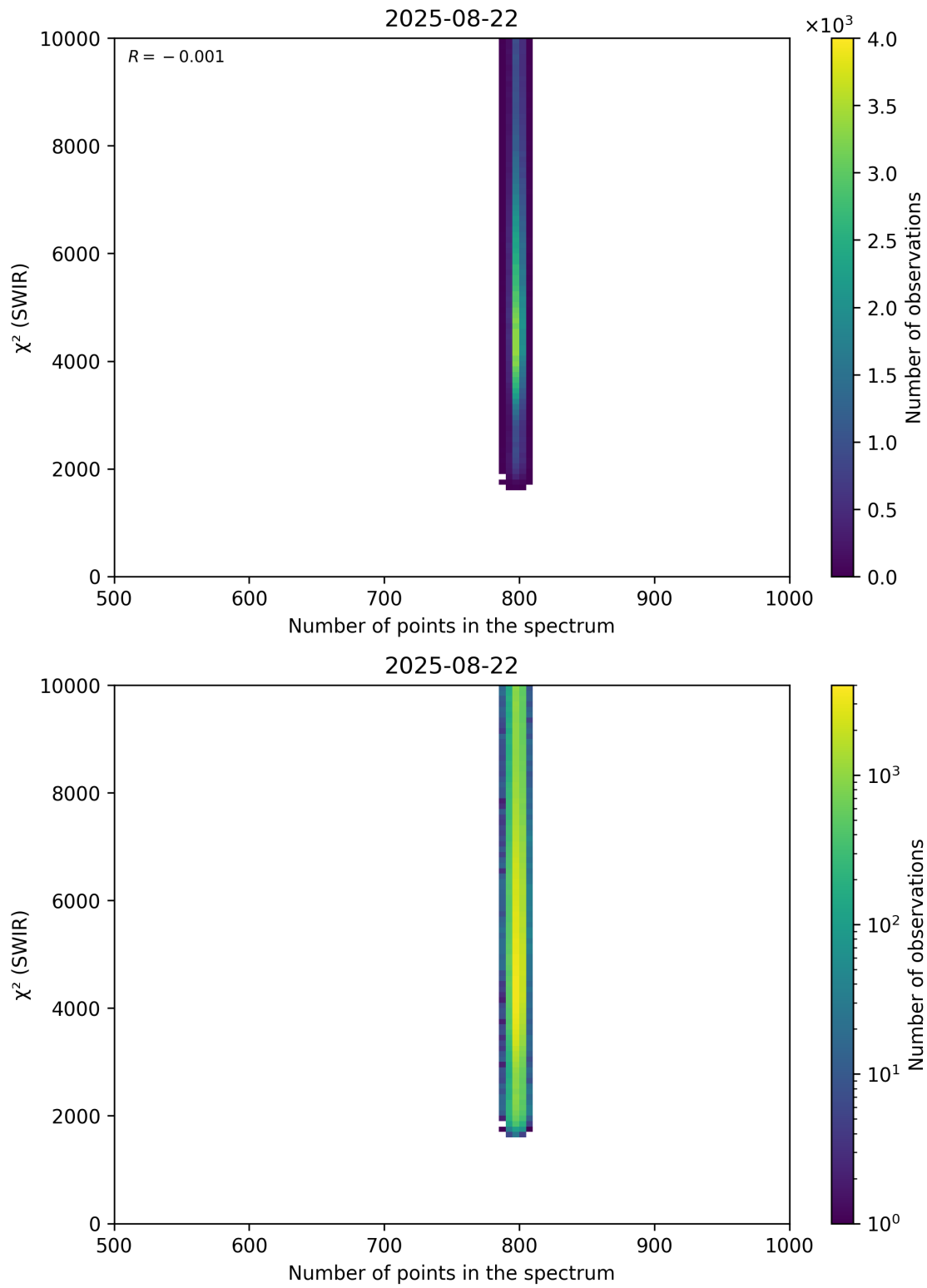
Figure 89: Scatter density plot of “Number of points in the spectrum” against “ \chi^2 (SWIR)” for 2025-08-21 to 2025-08-23.
