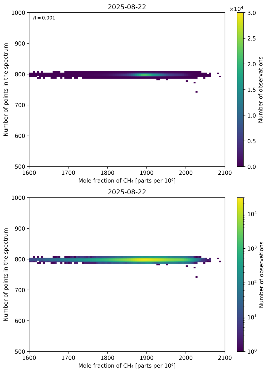
Figure 77: Scatter density plot of “Mole fraction of CH 4 ” against “Number of points in the spectrum” for 2025-08-21 to 2025-08-23.
