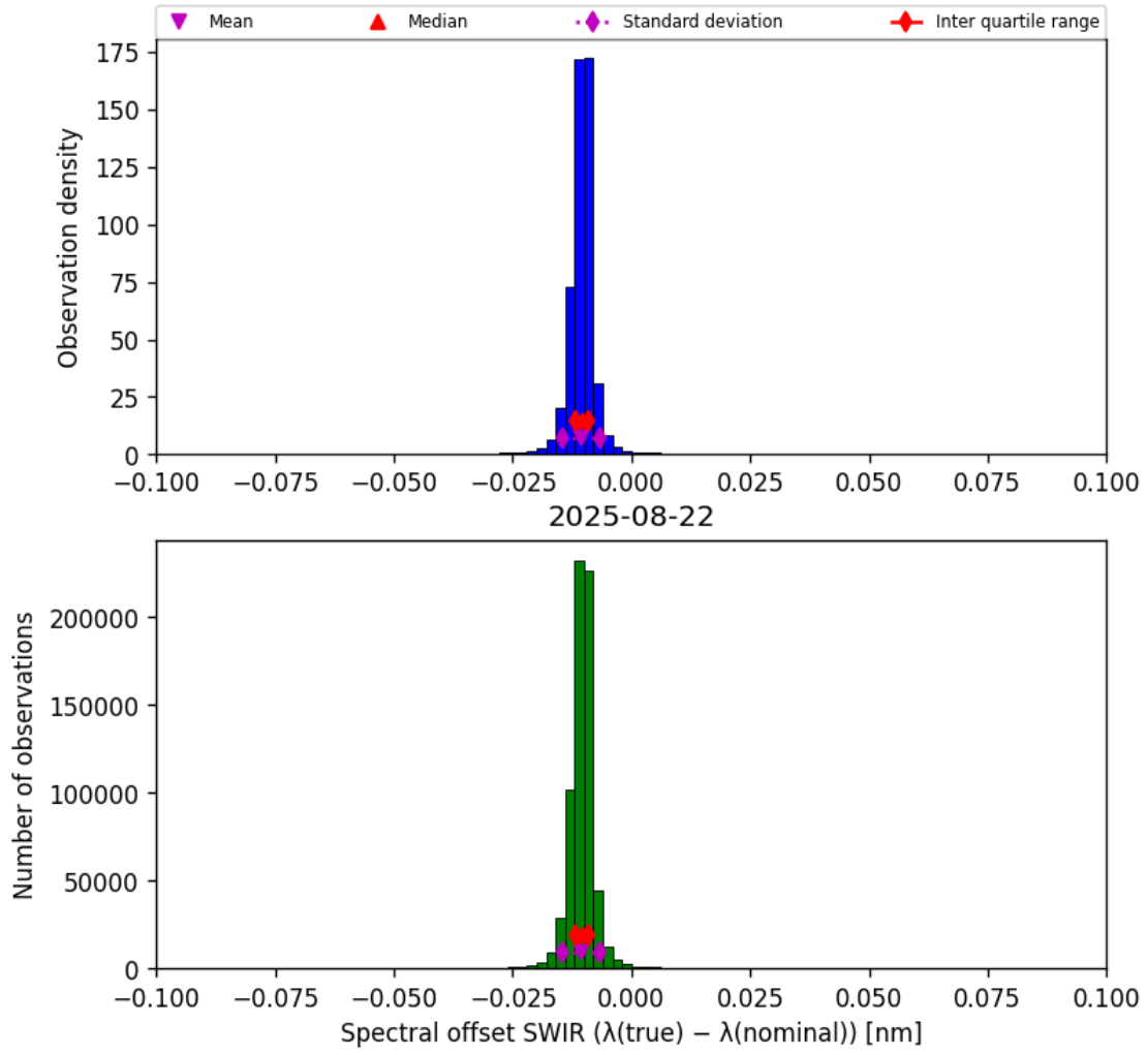
Figure 27: Histogram of “Spectral offset SWIR ( \lambda_{\text{true}} - \lambda_{\text{nominal}} )” for 2025-08-21 to 2025-08-23
