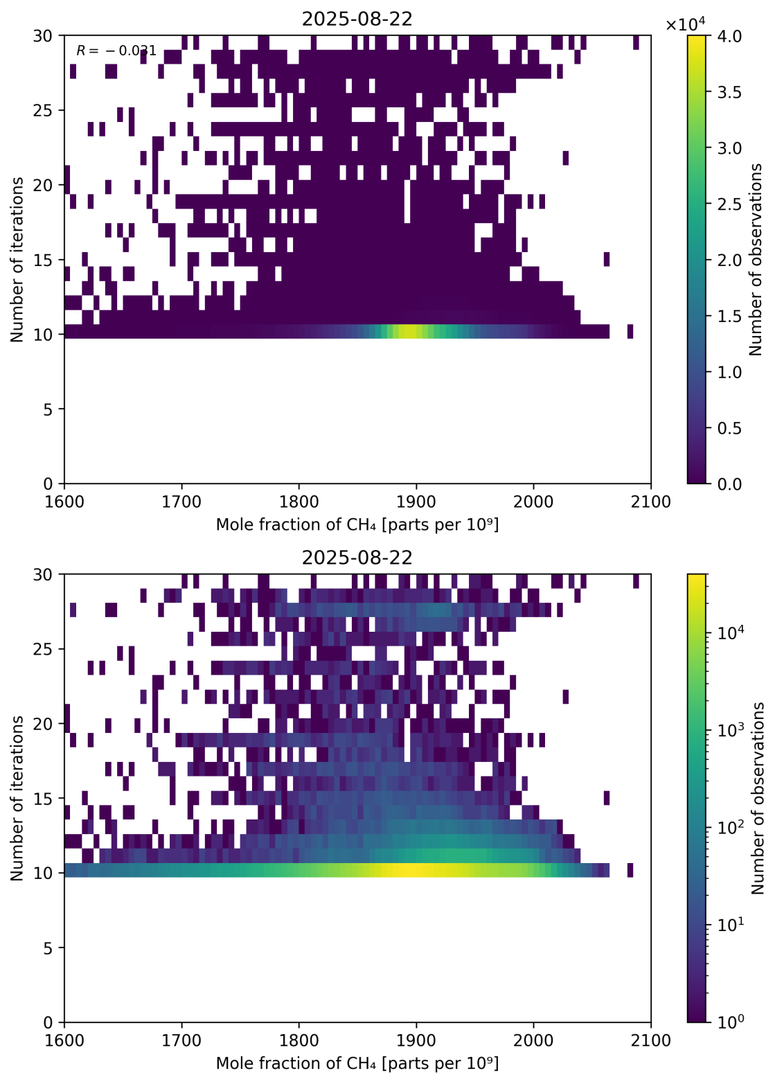
Figure 76: Scatter density plot of “Mole fraction of CH 4 ” against “Number of iterations” for 2025-08-21 to 2025-08-23.
