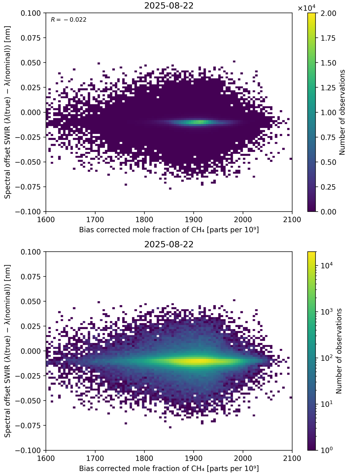
Figure 69: Scatter density plot of “Bias corrected mole fraction of \text{CH}_4 ” against “Spectral offset SWIR ( \lambda_{\text{true}} - \lambda_{\text{nominal}} )” for 2025-08-21 to 2025-08-23.
