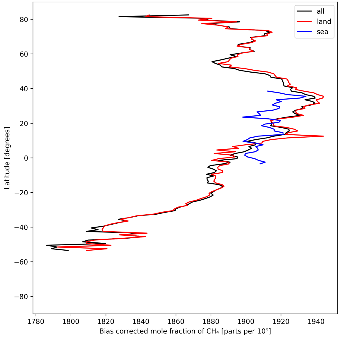
Figure 14: Zonal average of “Bias corrected mole fraction of \text{CH}_4 ” for 2025-08-21 to 2025-08-23.
