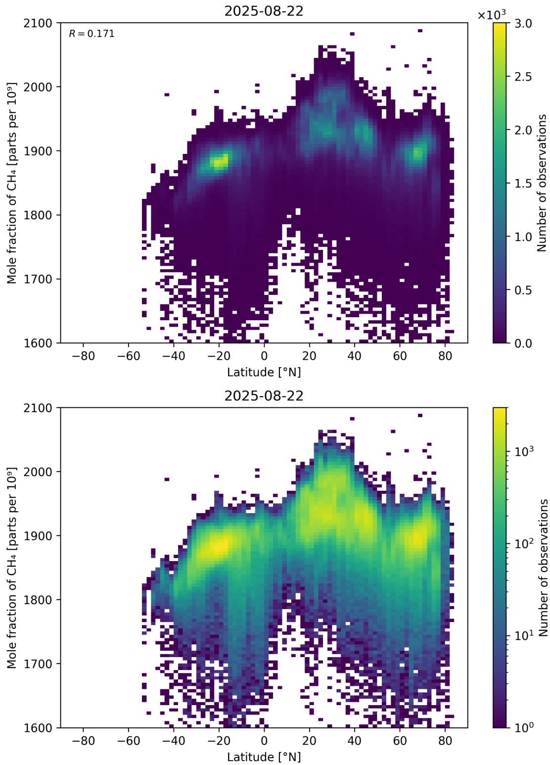
Figure 57: Scatter density plot of “Latitude” against “Mole fraction of \text{CH}_4 ” for 2025-08-21 to 2025-08-23.
