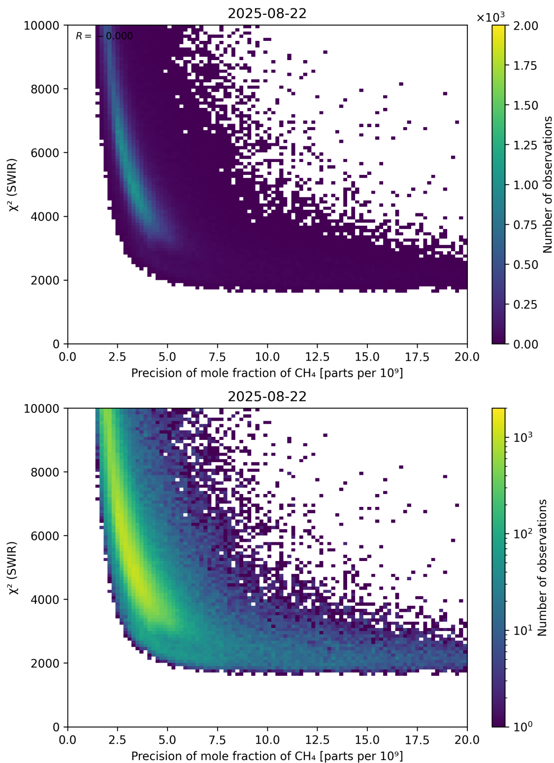
Figure 79: Scatter density plot of “Precision of mole fraction of \text{CH}_4 ” against “ \chi^2 (SWIR)” for 2025-08-21 to 2025-08-23.
