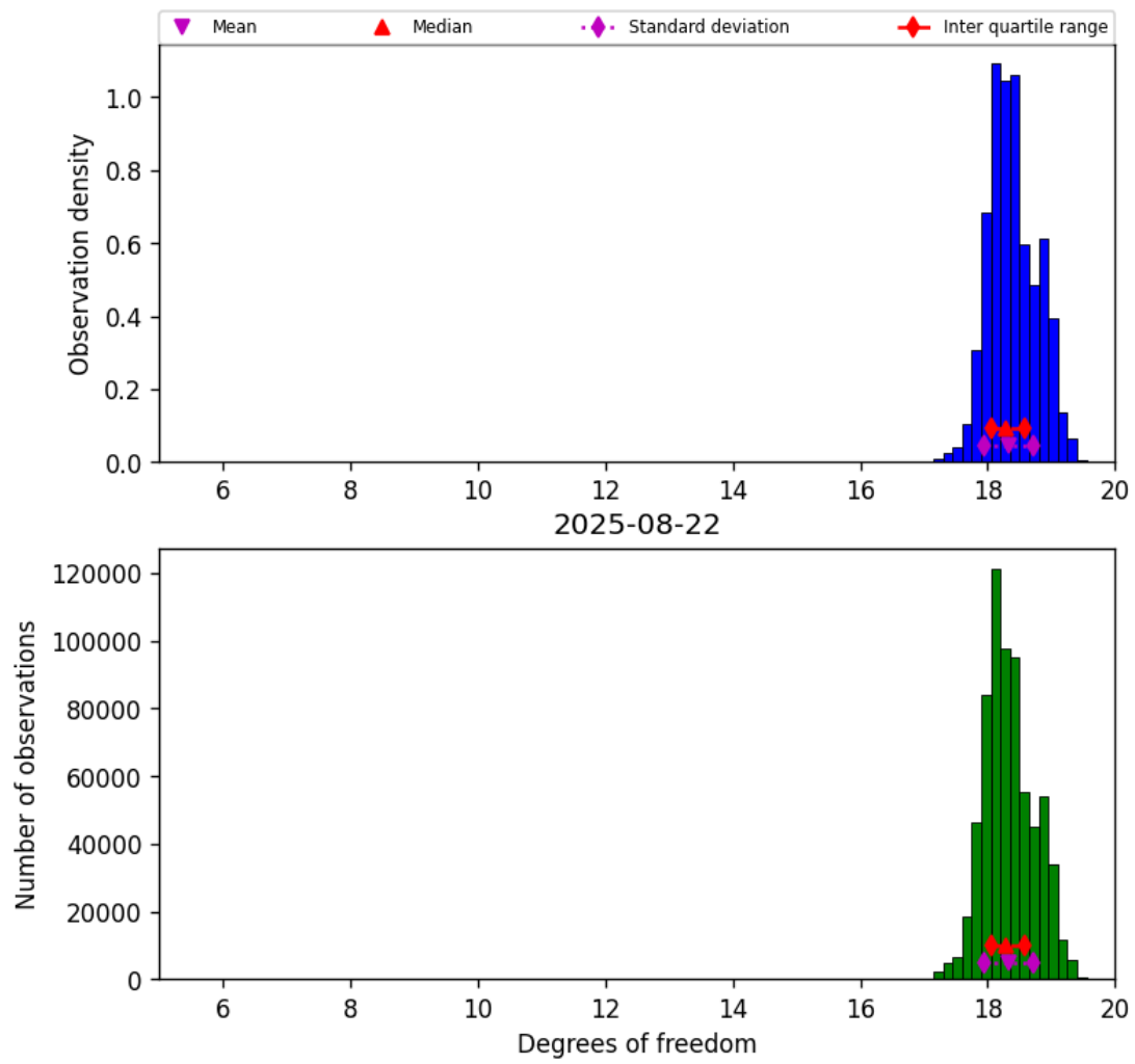
Figure 30: Histogram of “Degrees of freedom” for 2025-08-21 to 2025-08-23
