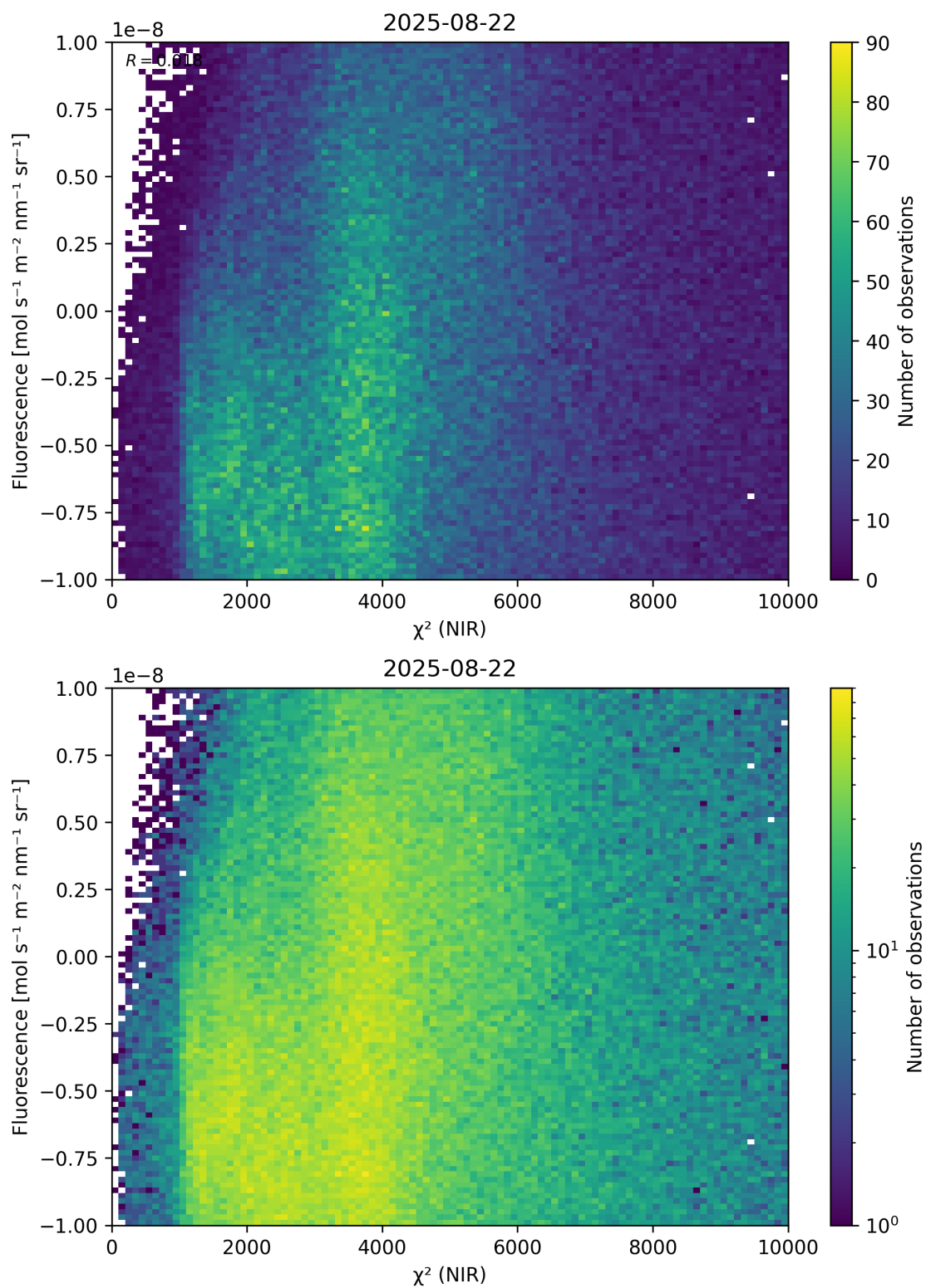
Figure 45: Scatter density plot of “ \chi^2 (NIR)” against “Fluorescence” for 2025-08-21 to 2025-08-23.
