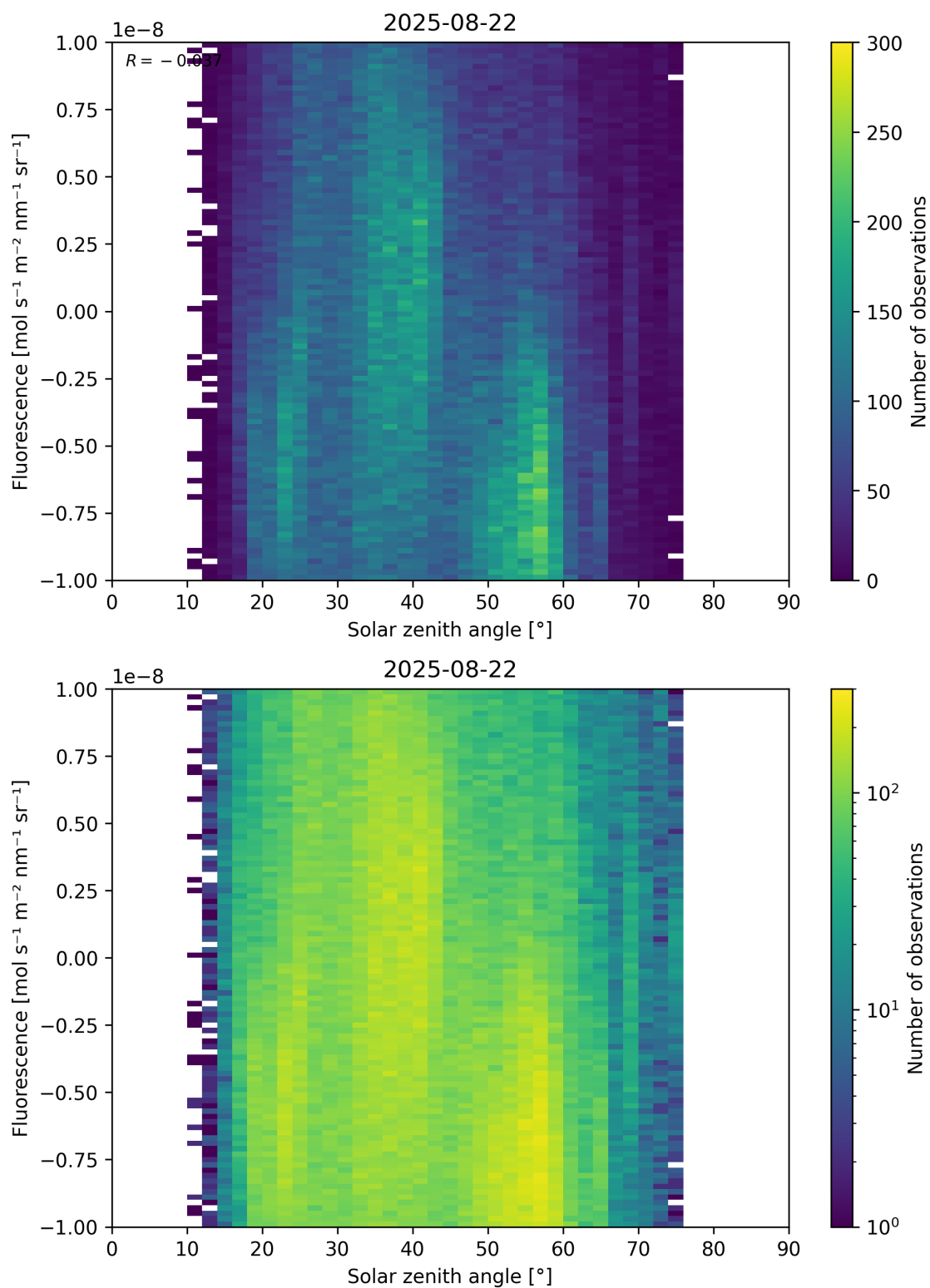
Figure 97: Scatter density plot of “Solar zenith angle” against “Fluorescence” for 2025-08-21 to 2025-08-23.
