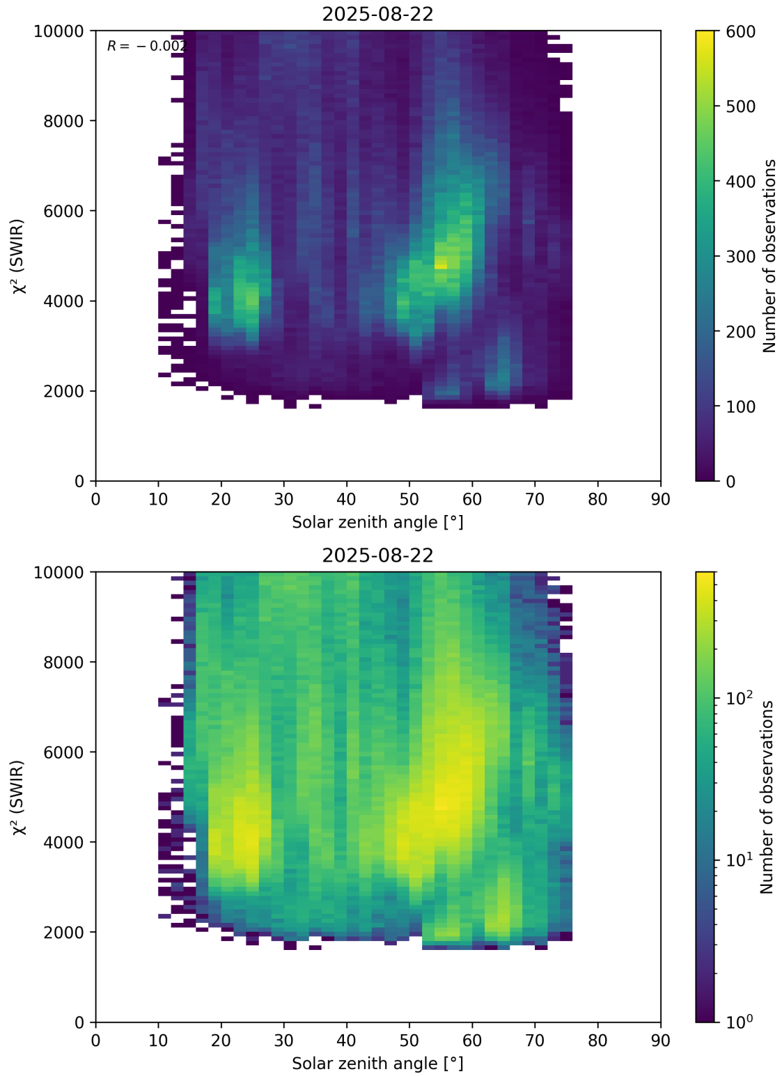
Figure 95: Scatter density plot of “Solar zenith angle” against “ \chi^2 (SWIR)” for 2025-08-21 to 2025-08-23.
