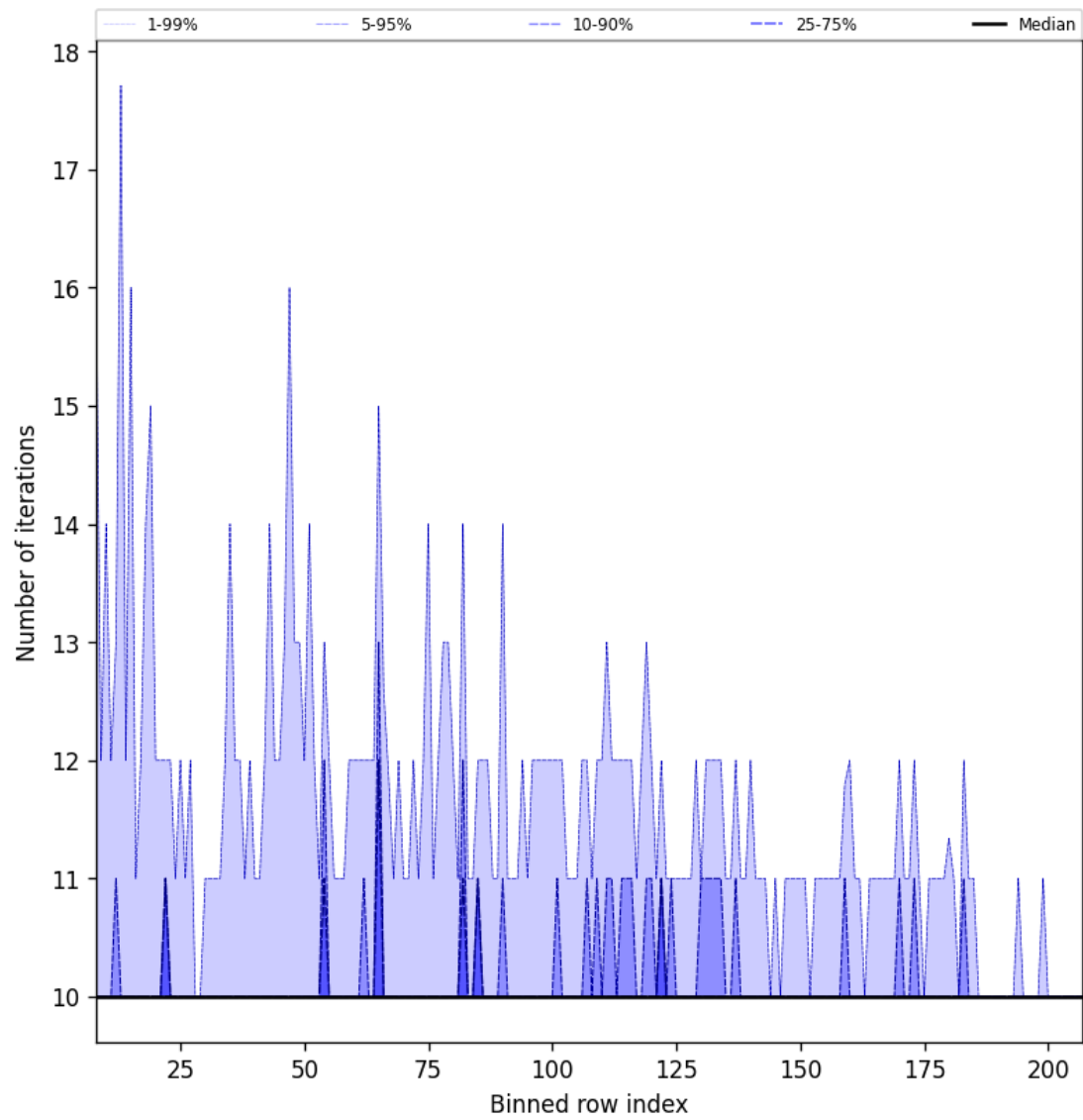
Figure 42: Along track statistics of “Number of iterations” for 2025-08-21 to 2025-08-23
