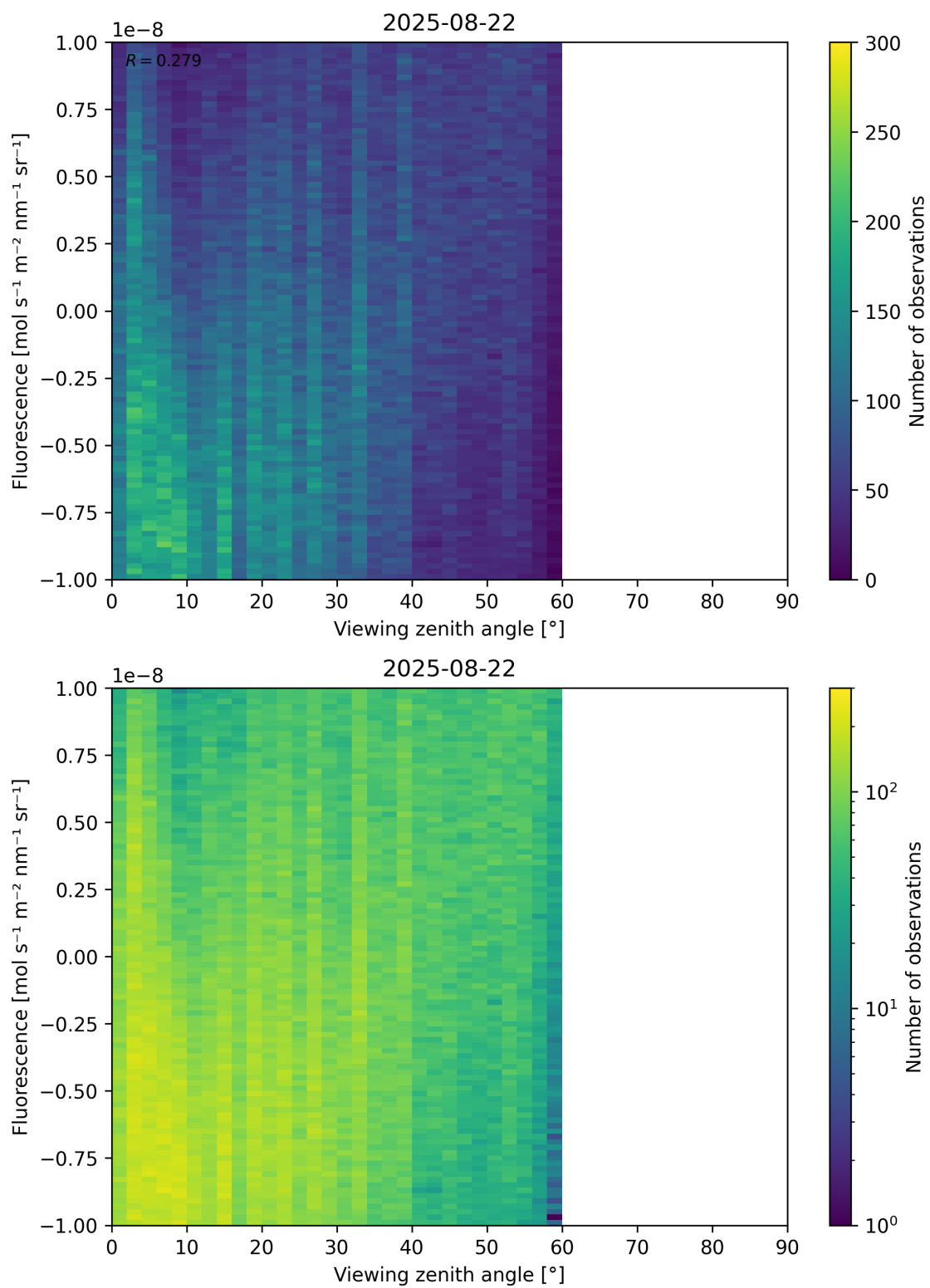
Figure 108: Scatter density plot of “Viewing zenith angle” against “Fluorescence” for 2025-08-21 to 2025-08-23.
