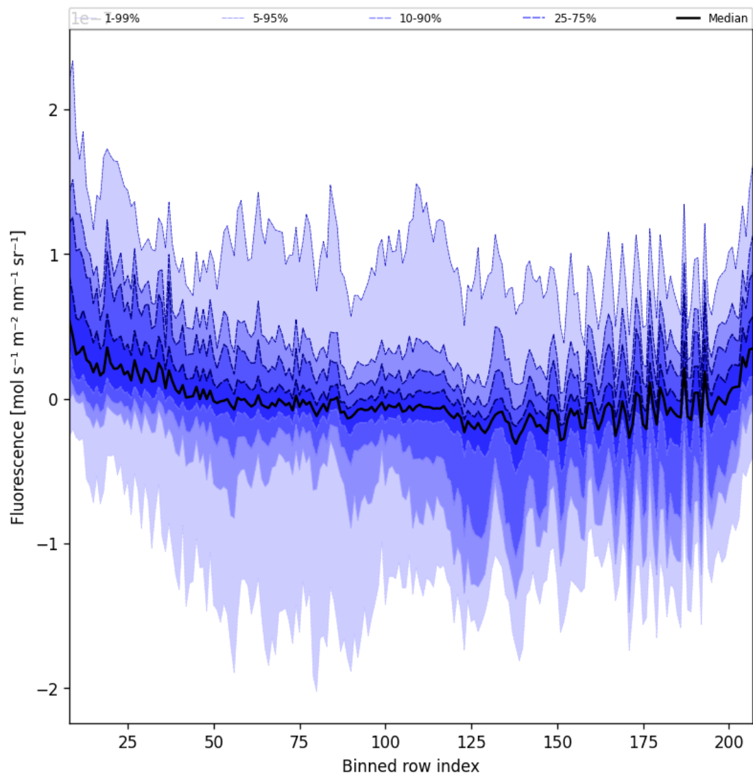
Figure 43: Along track statistics of “Fluorescence” for 2025-08-21 to 2025-08-23
