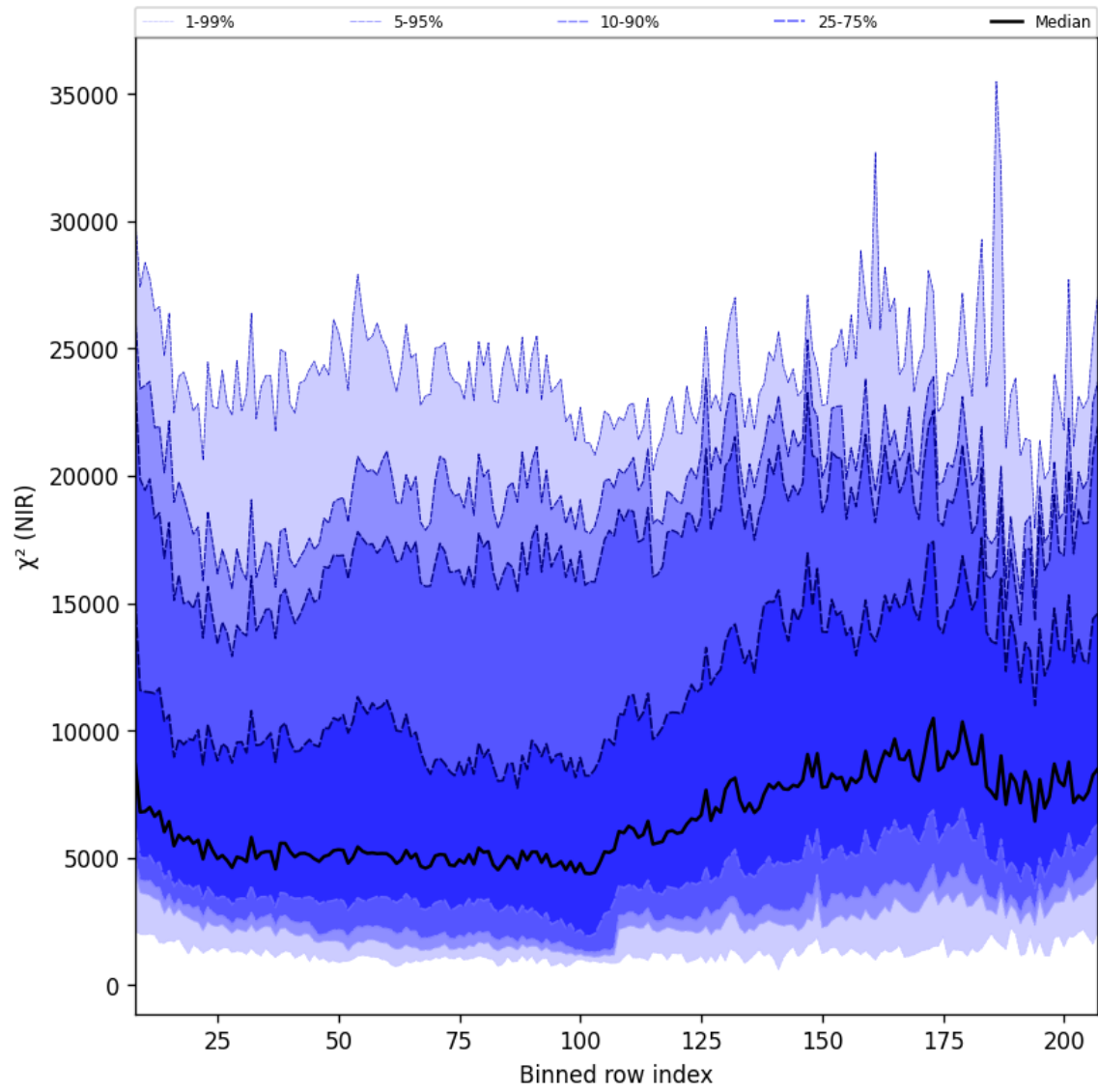
Figure 40: Along track statistics of “ \chi^2 (NIR)” for 2025-08-21 to 2025-08-23
