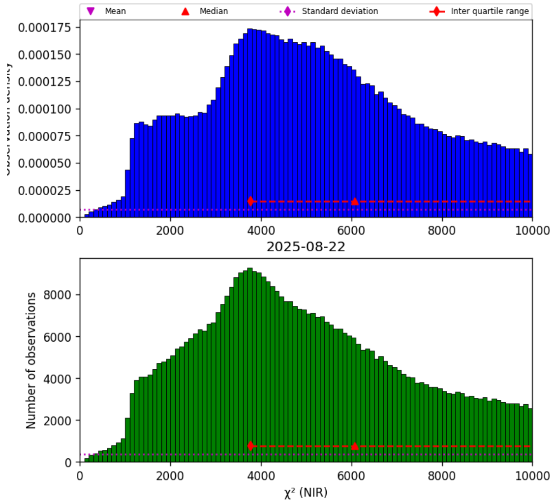
Figure 29: Histogram of “ \chi^2 (NIR)” for 2025-08-21 to 2025-08-23
