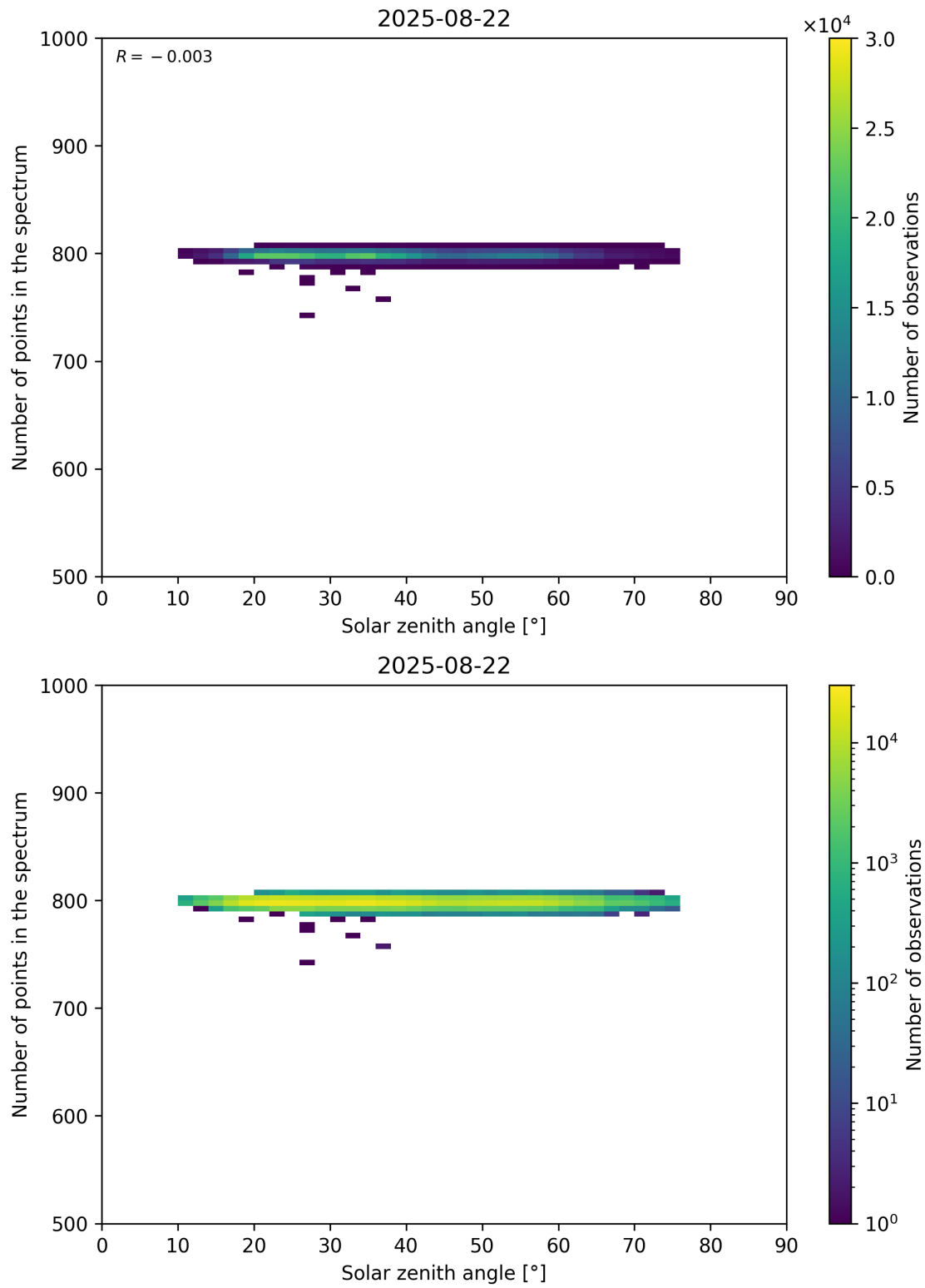
Figure 103: Scatter density plot of “Solar zenith angle” against “Number of points in the spectrum” for 2025-08-21 to 2025-08-23.
