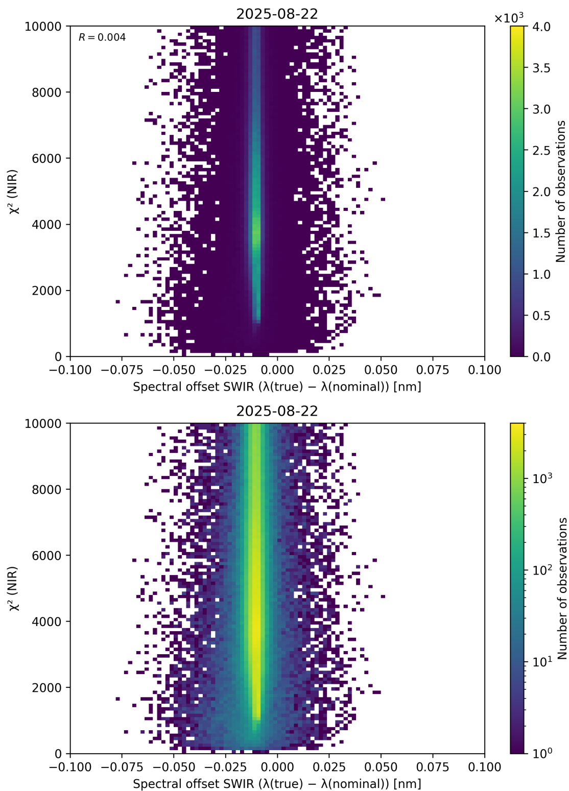
Figure 117: Scatter density plot of “Spectral offset SWIR ( \lambda_{\text{true}} - \lambda_{\text{nominal}} )” against “ \chi^2 (NIR)” for 2025-08-21 to 2025-08-23.
