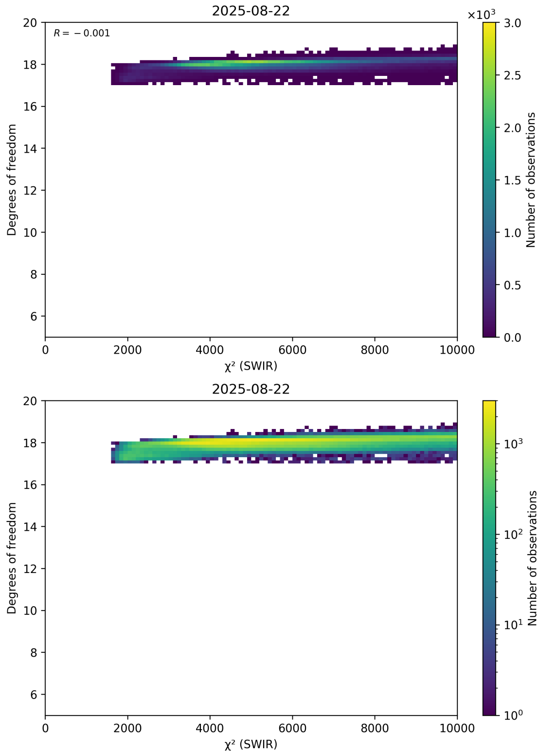
Figure 48: Scatter density plot of “ \chi^2 (SWIR)” against “Degrees of freedom” for 2025-08-21 to 2025-08-23.
