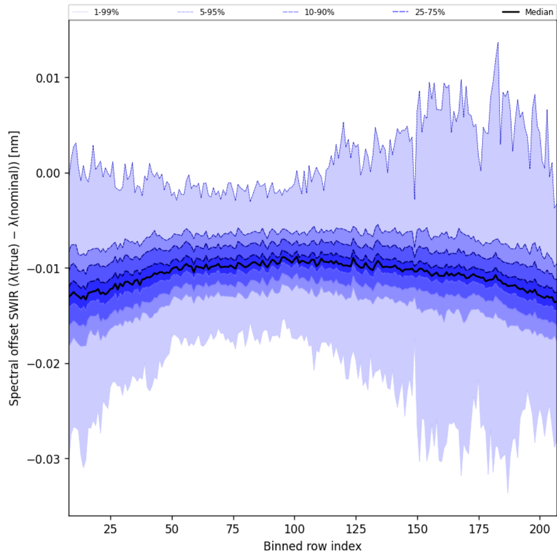
Figure 38: Along track statistics of “Spectral offset SWIR ( \lambda_{\text{true}} - \lambda_{\text{nominal}} )” for 2025-08-21 to 2025-08-23
