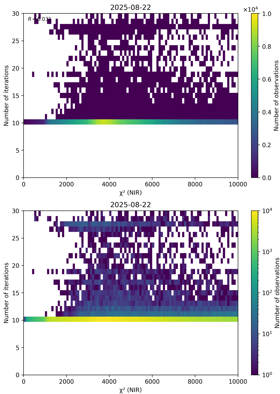
Figure 46: Scatter density plot of “ \chi^2 (NIR)” against “Number of iterations” for 2025-08-21 to 2025-08-23.
