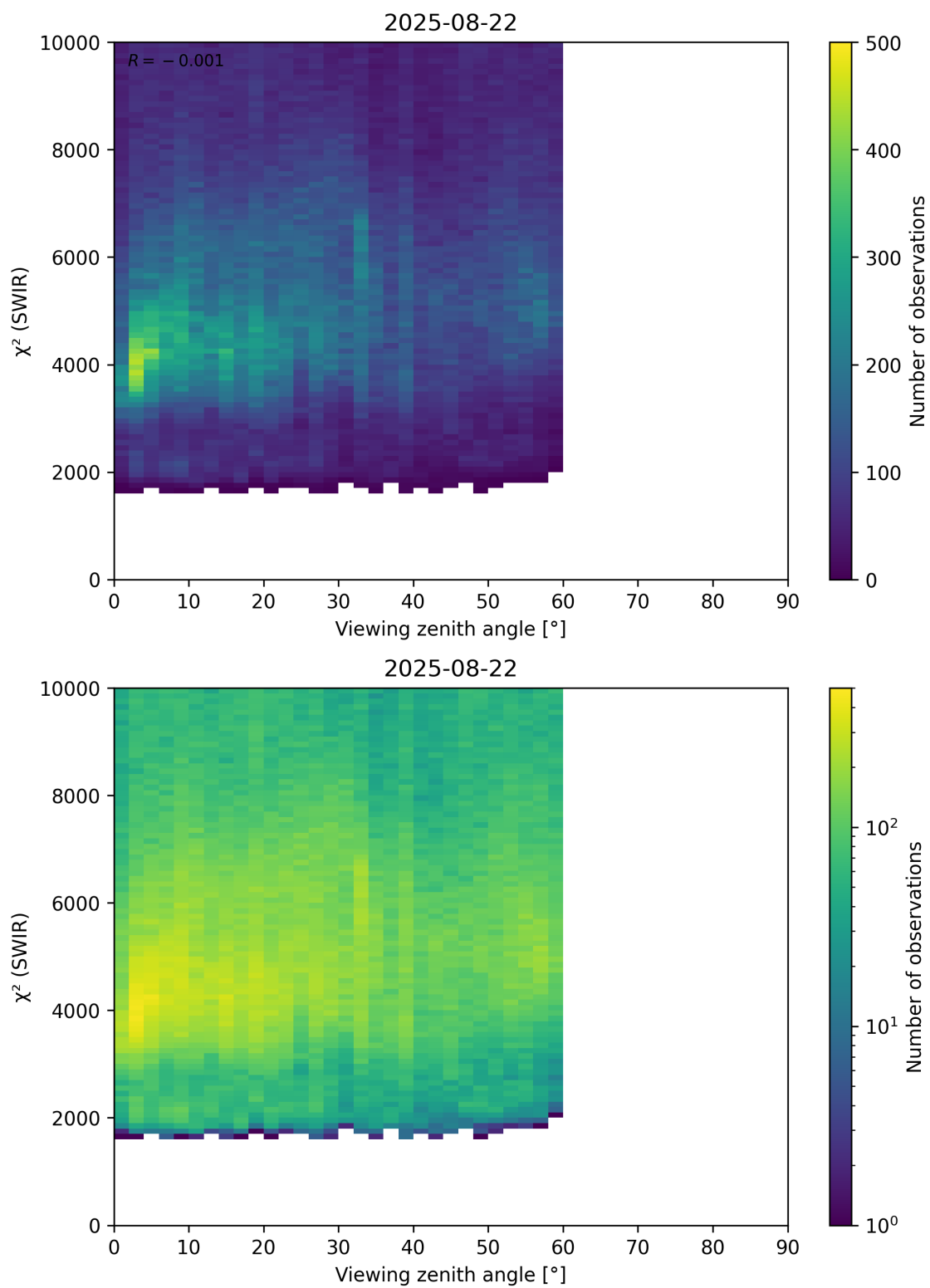
Figure 106: Scatter density plot of “Viewing zenith angle” against “ \chi^2 (SWIR)” for 2025-08-21 to 2025-08-23.
