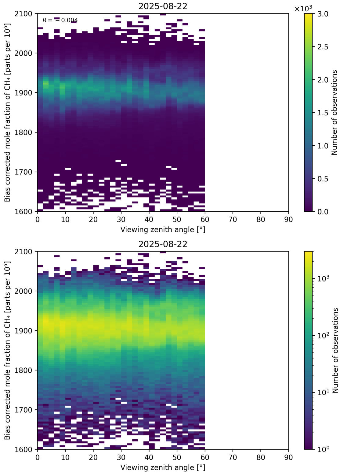
Figure 111: Scatter density plot of “Viewing zenith angle” against “Bias corrected mole fraction of CH 4 ” for 2025-08-21 to 2025-08-23.
