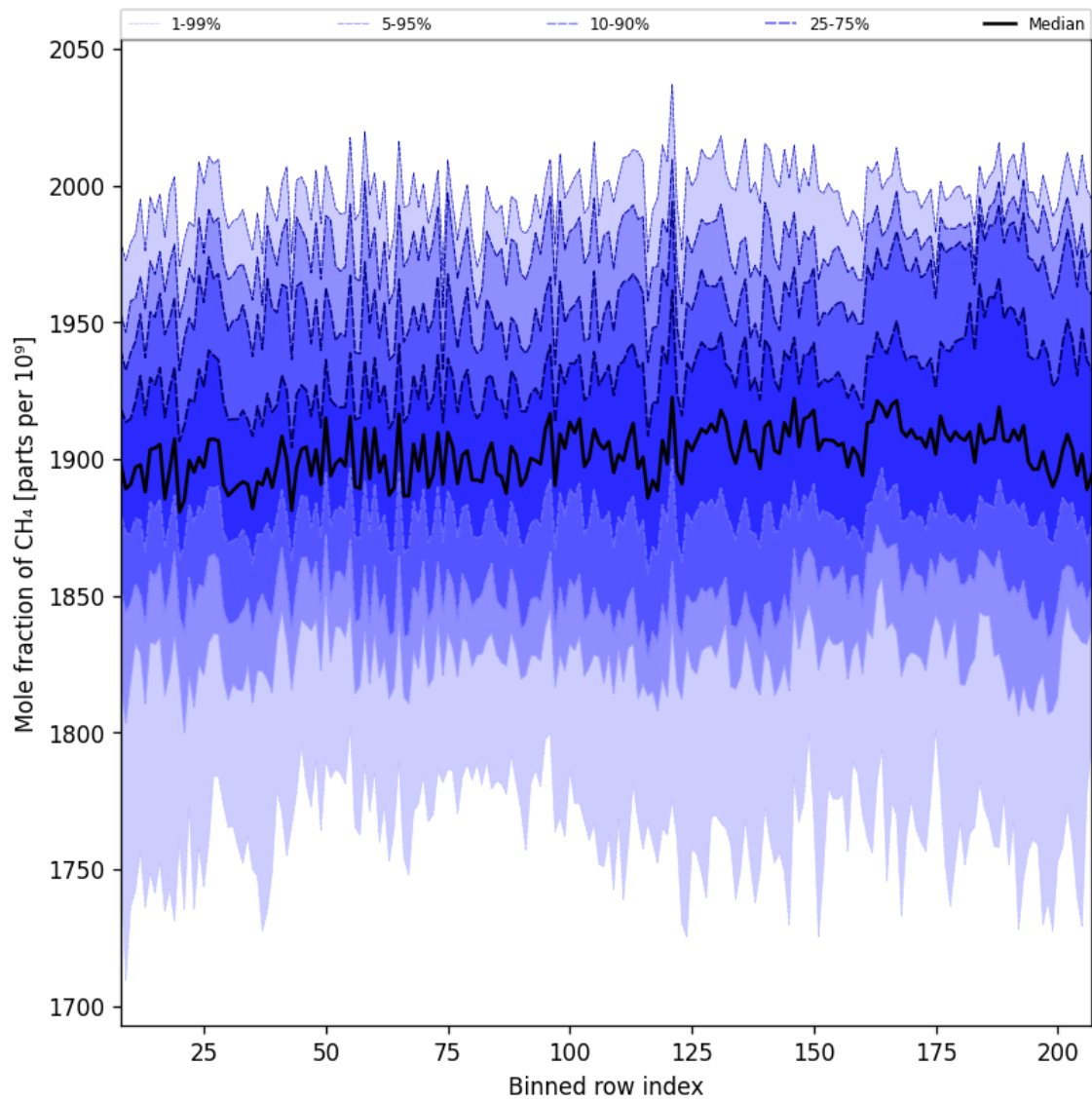
Figure 34: Along track statistics of “Mole fraction of CH 4 ” for 2025-08-21 to 2025-08-23
