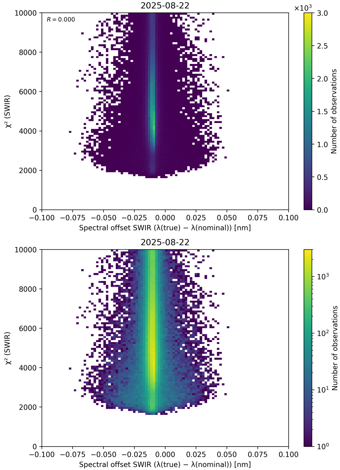
Figure 118: Scatter density plot of “Spectral offset SWIR ( \lambda_{\text{true}} - \lambda_{\text{nominal}} )” against “ \chi^2 (SWIR)” for 2025-08-21 to 2025-08-23.
