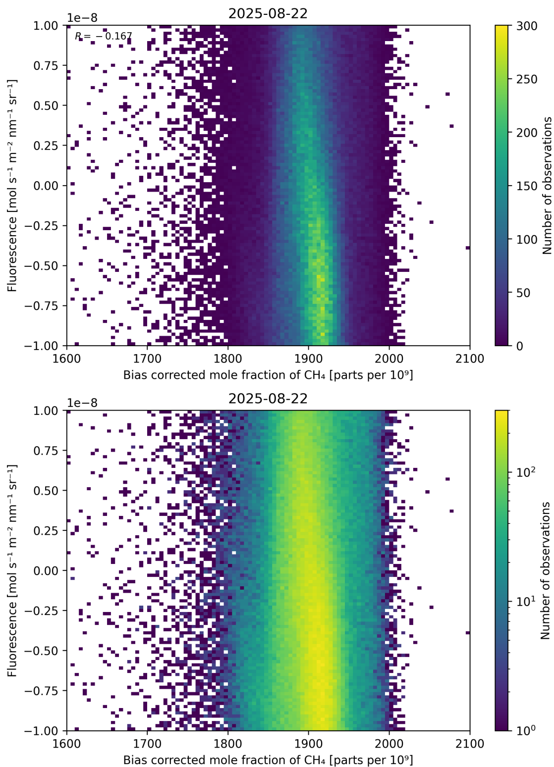
Figure 66: Scatter density plot of “Bias corrected mole fraction of \text{CH}_4 ” against “Fluorescence” for 2025-08-21 to 2025-08-23.
