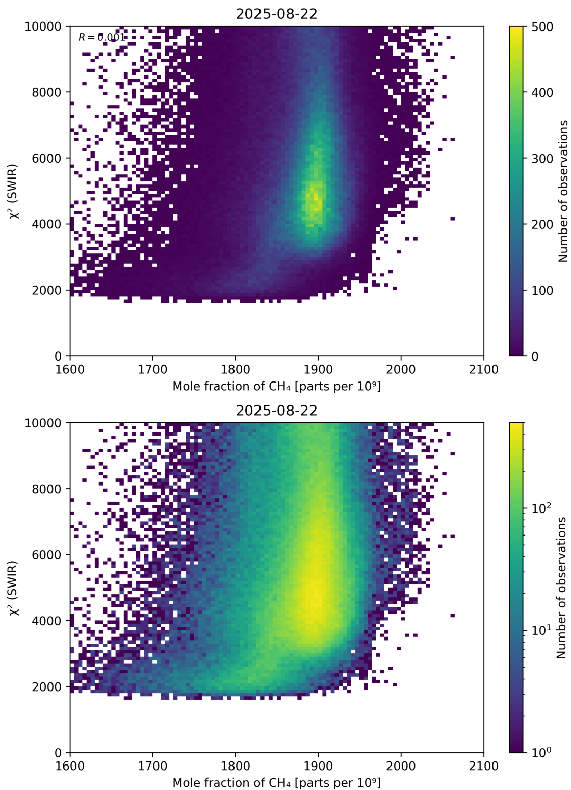
Figure 71: Scatter density plot of “Mole fraction of CH 4 ” against “ \chi^2 (SWIR)” for 2025-08-21 to 2025-08-23.
