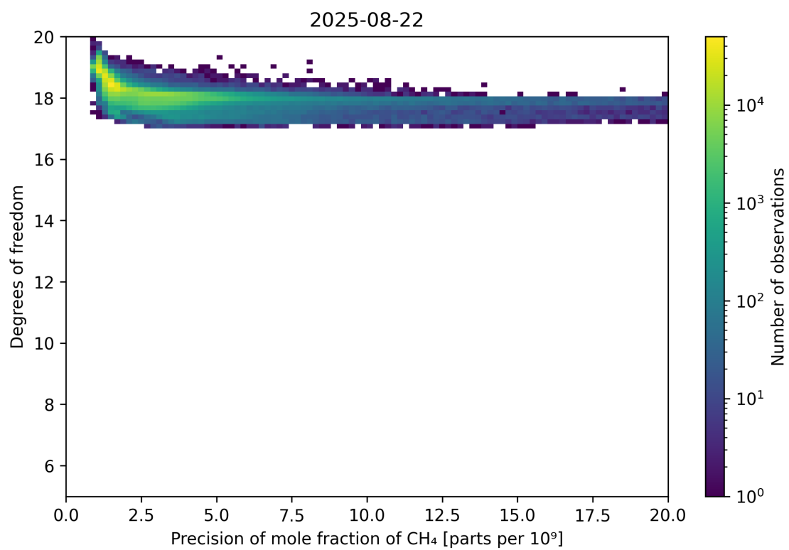
Figure 80: Scatter density plot of “Precision of mole fraction of CH 4 ” against “Degrees of freedom” for 2025-08-21 to 2025-08-23.
