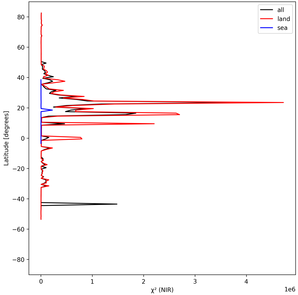
Figure 18: Zonal average of “ \chi^2 (NIR)” for 2025-08-21 to 2025-08-23.
