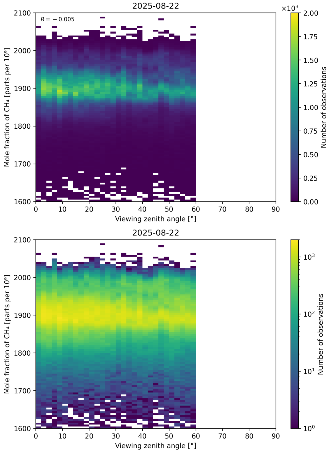
Figure 110: Scatter density plot of “Viewing zenith angle” against “Mole fraction of CH 4 ” for 2025-08-21 to 2025-08-23.
