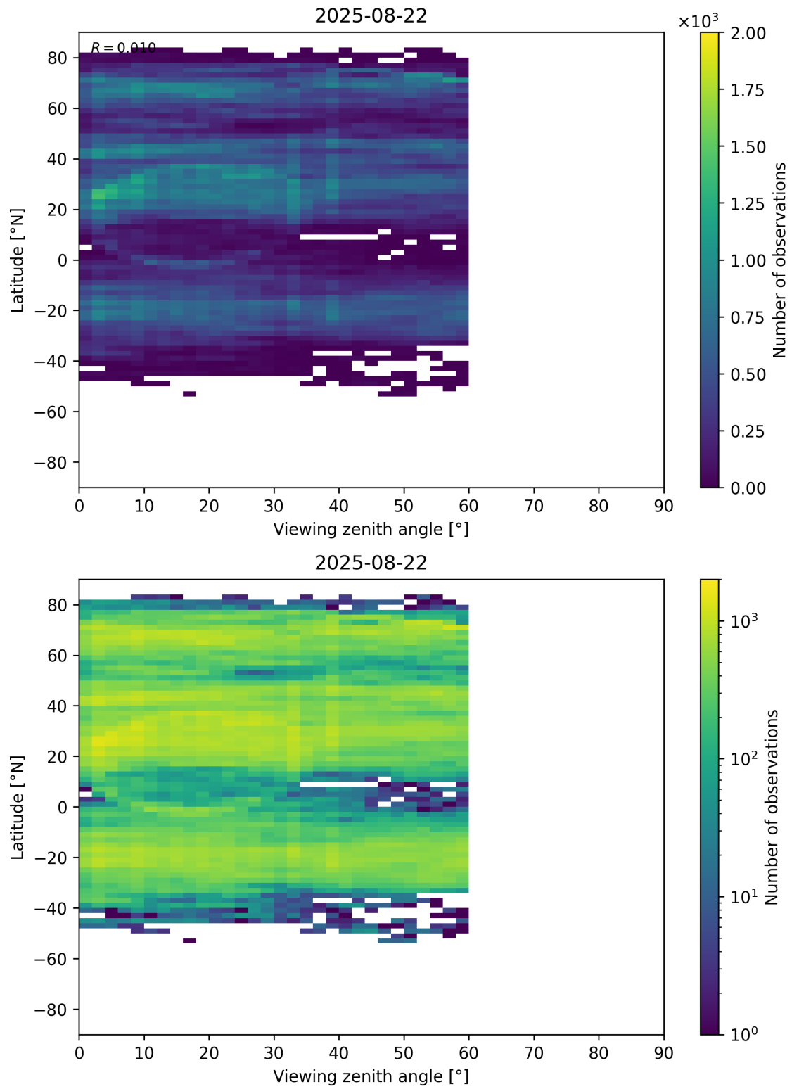
Figure 109: Scatter density plot of “Viewing zenith angle” against “Latitude” for 2025-08-21 to 2025-08-23.
