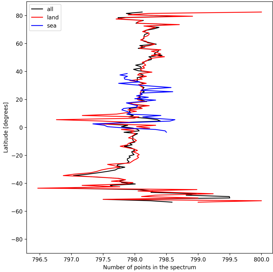
Figure 15: Zonal average of “Number of points in the spectrum” for 2025-08-21 to 2025-08-23.
