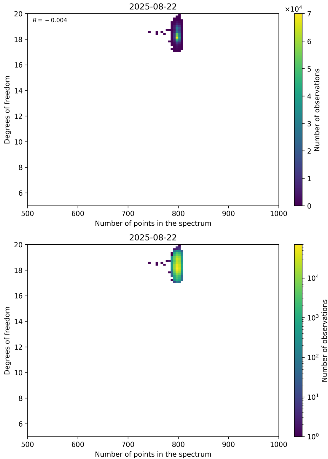
Figure 90: Scatter density plot of “Number of points in the spectrum” against “Degrees of freedom” for 2025-08-21 to 2025-08-23.
