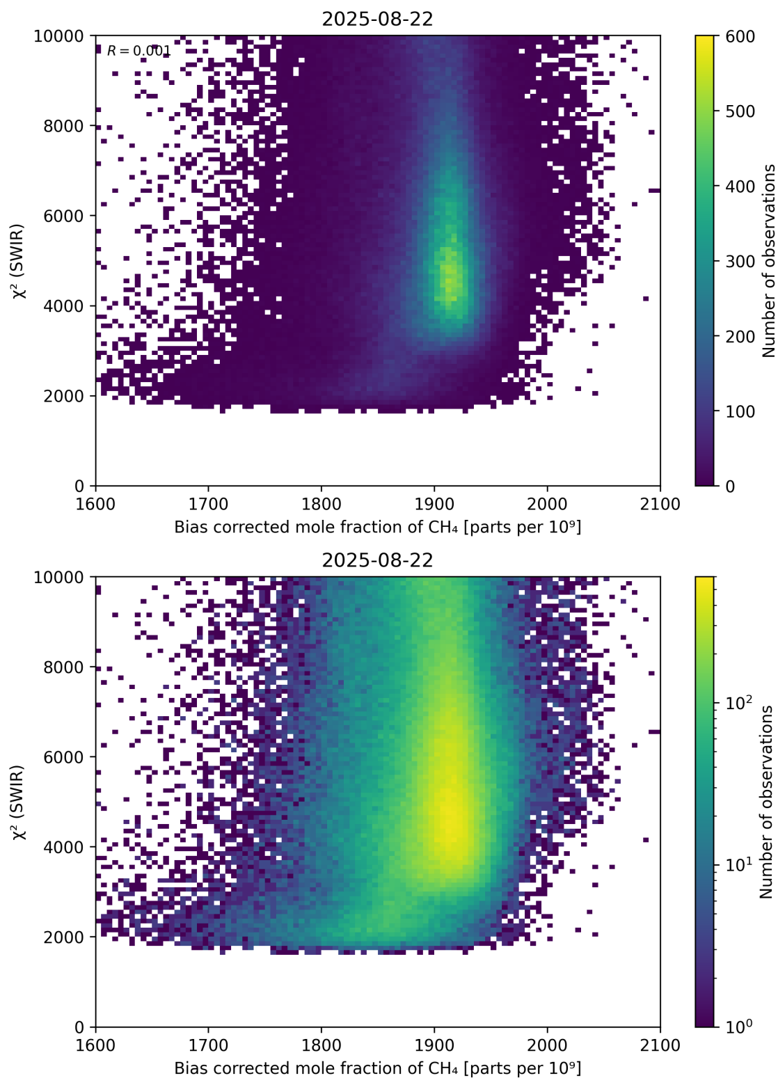
Figure 64: Scatter density plot of “Bias corrected mole fraction of \text{CH}_4 ” against “ \chi^2 (SWIR)” for 2025-08-21 to 2025-08-23.
