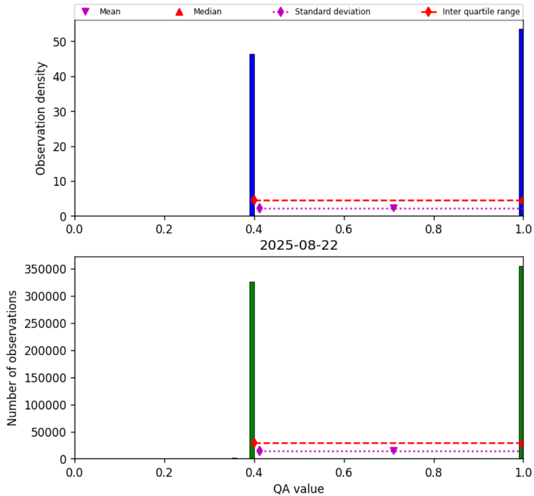
Figure 22: Histogram of “QA value” for 2025-08-21 to 2025-08-23
