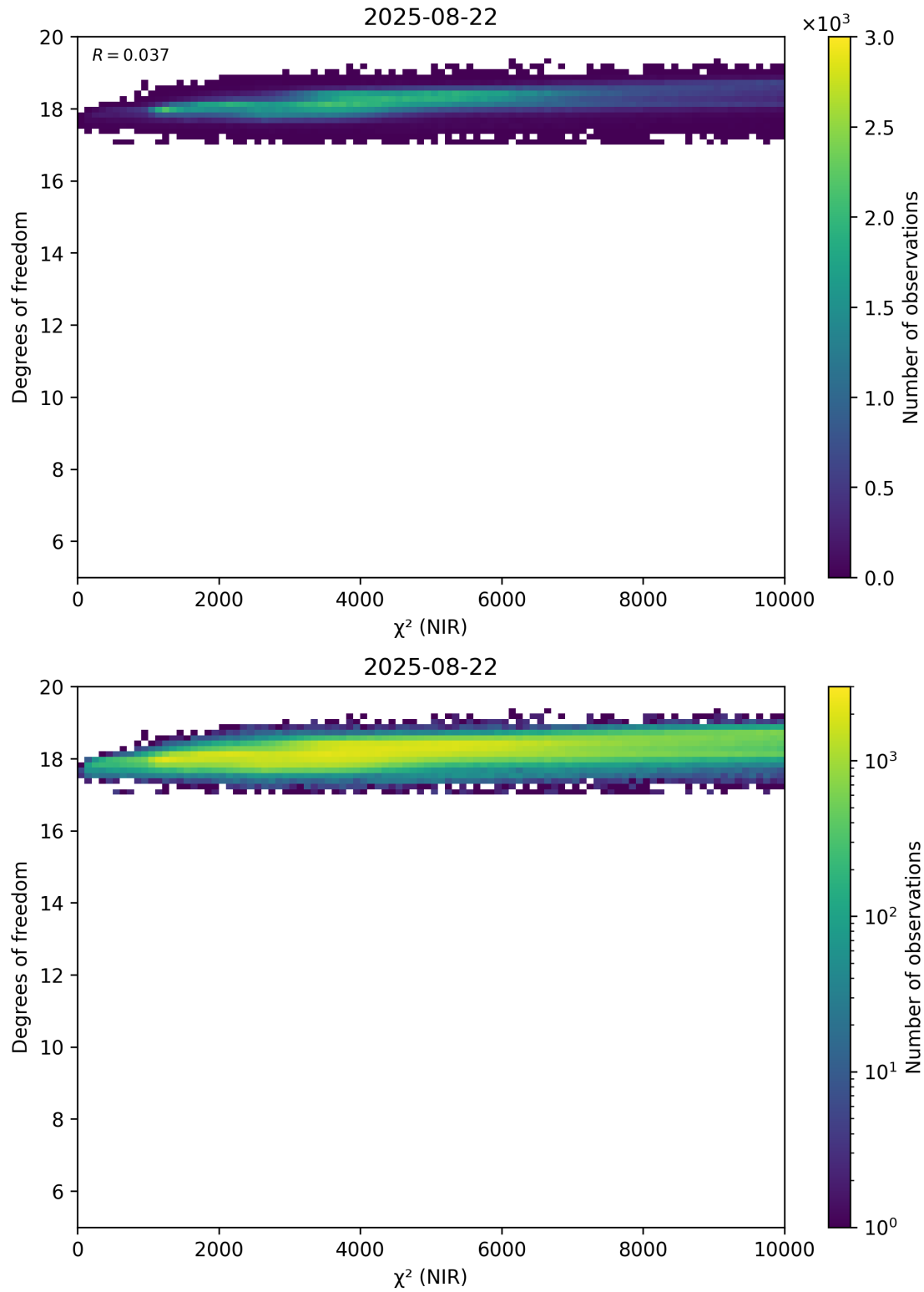
Figure 44: Scatter density plot of “ \chi^2 (NIR)” against “Degrees of freedom” for 2025-08-21 to 2025-08-23.
