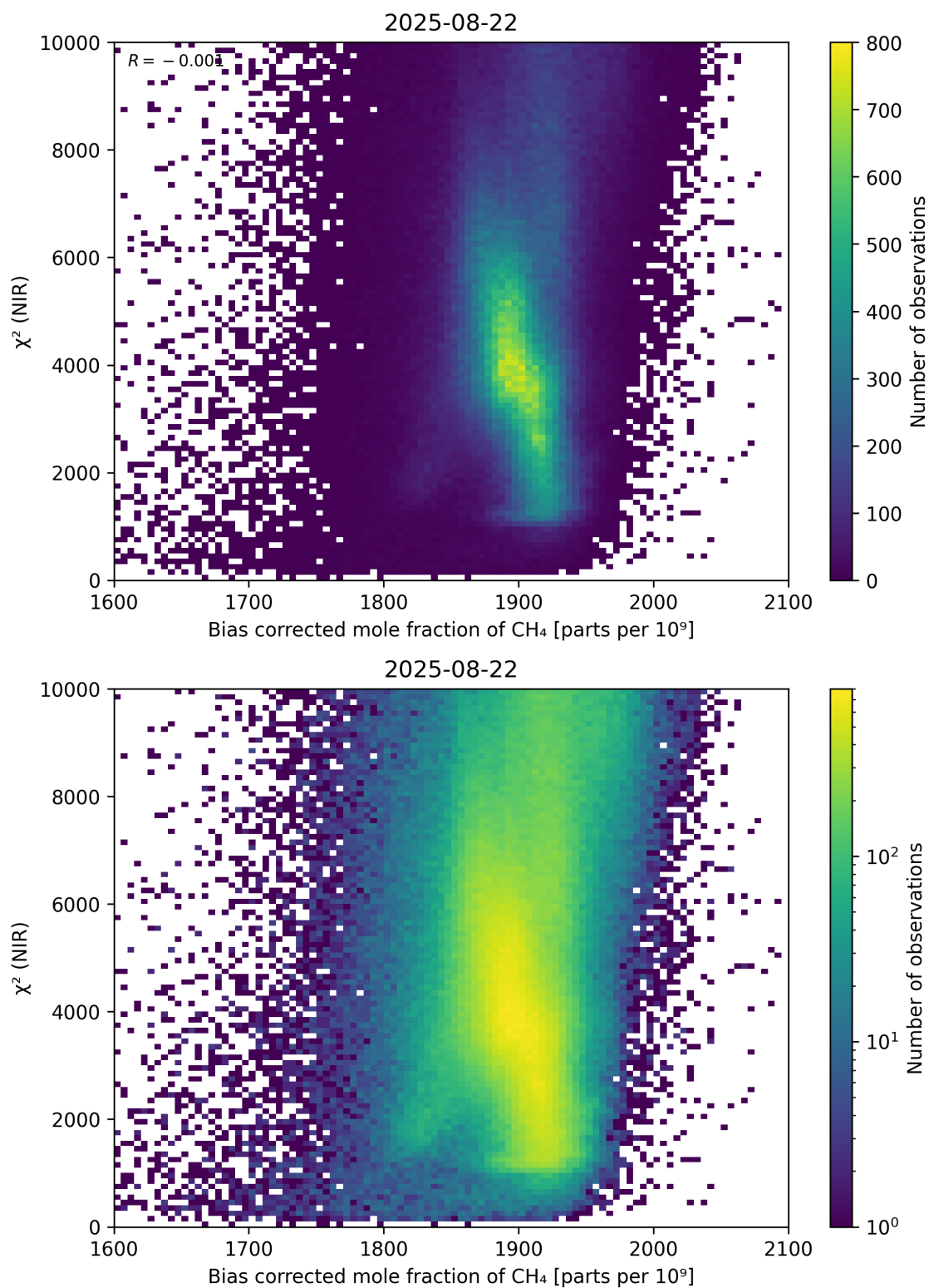
Figure 63: Scatter density plot of “Bias corrected mole fraction of \text{CH}_4 ” against “ \chi^2 (NIR)” for 2025-08-21 to 2025-08-23.
