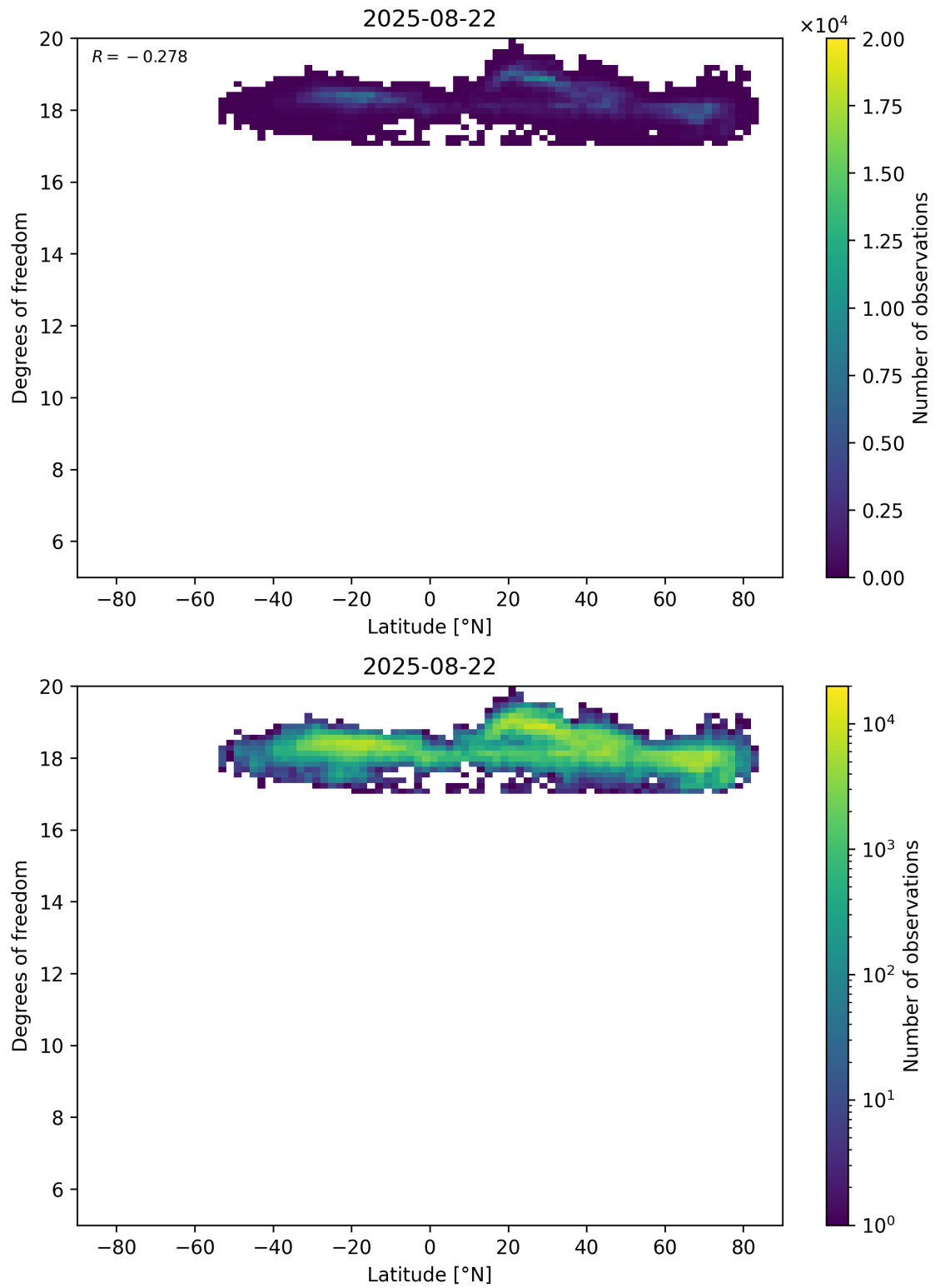
Figure 55: Scatter density plot of “Latitude” against “Degrees of freedom” for 2025-08-21 to 2025-08-23.
