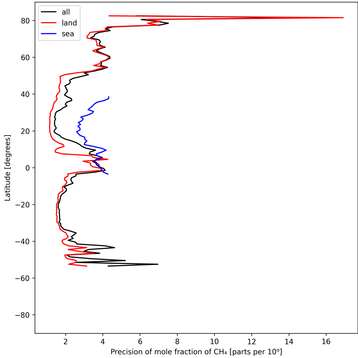
Figure 13: Zonal average of “Precision of mole fraction of CH 4 ” for 2025-08-21 to 2025-08-23.
