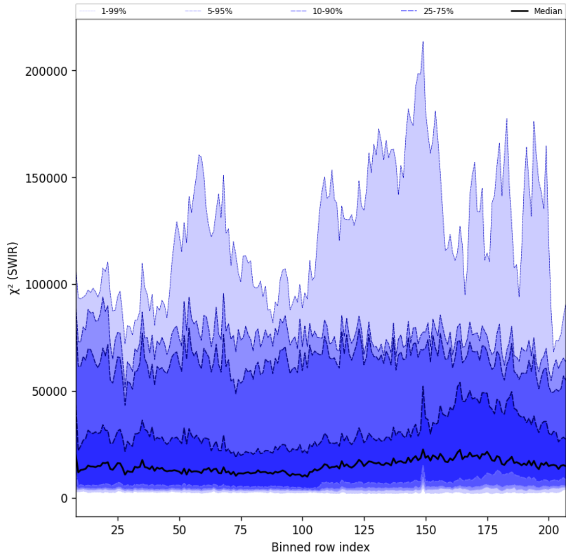
Figure 39: Along track statistics of " \chi^2 (SWIR)" for 2025-08-21 to 2025-08-23
