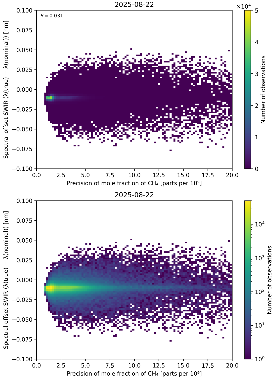
Figure 85: Scatter density plot of “Precision of mole fraction of CH 4 ” against “Spectral offset SWIR ( \lambda_{\text{true}} - \lambda_{\text{nominal}} )” for 2025-08-21 to 2025-08-23.
