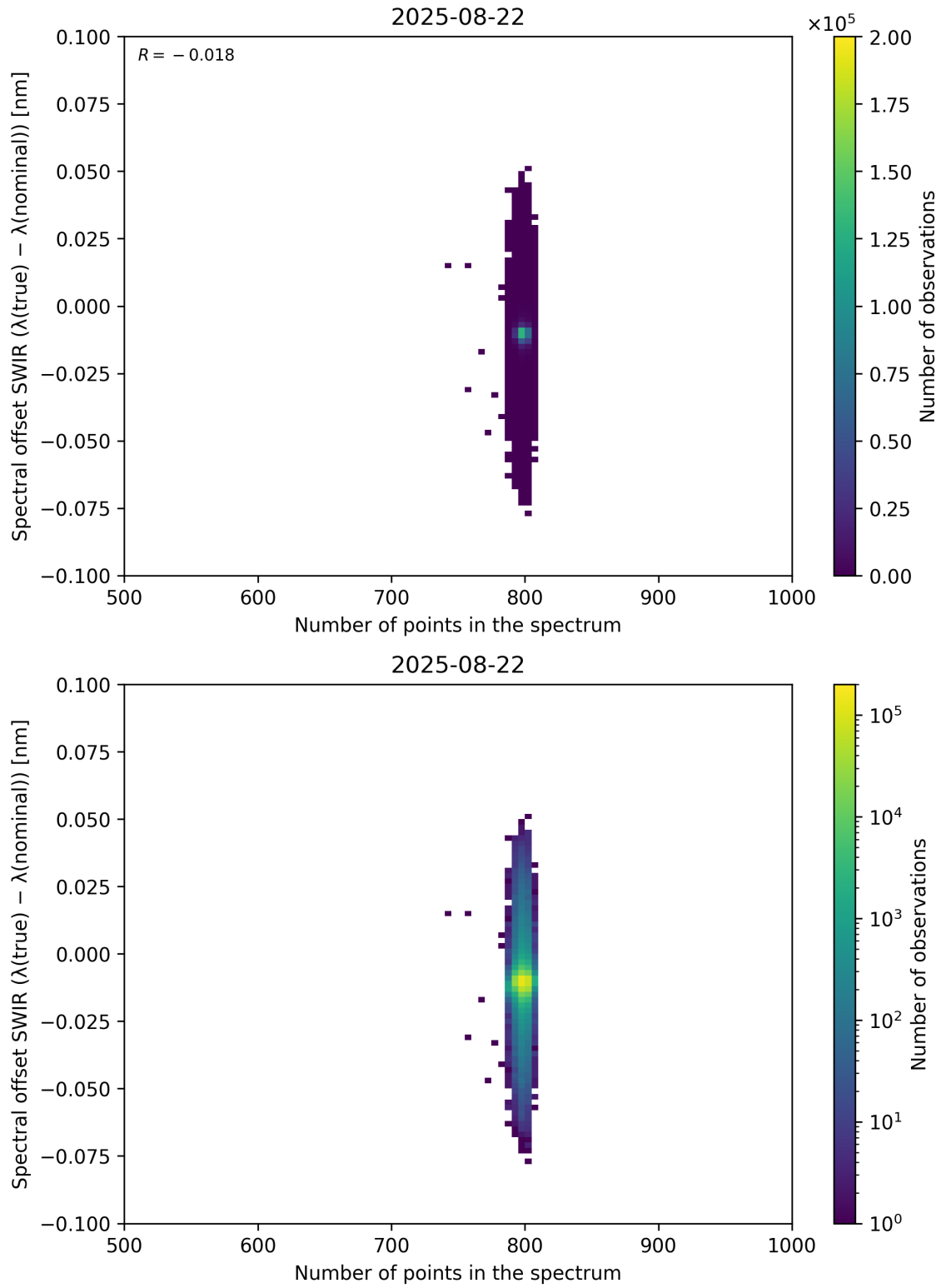
Figure 93: Scatter density plot of “Number of points in the spectrum” against “Spectral offset SWIR ( \lambda_{\text{true}} - \lambda_{\text{nominal}} )” for 2025-08-21 to 2025-08-23.
