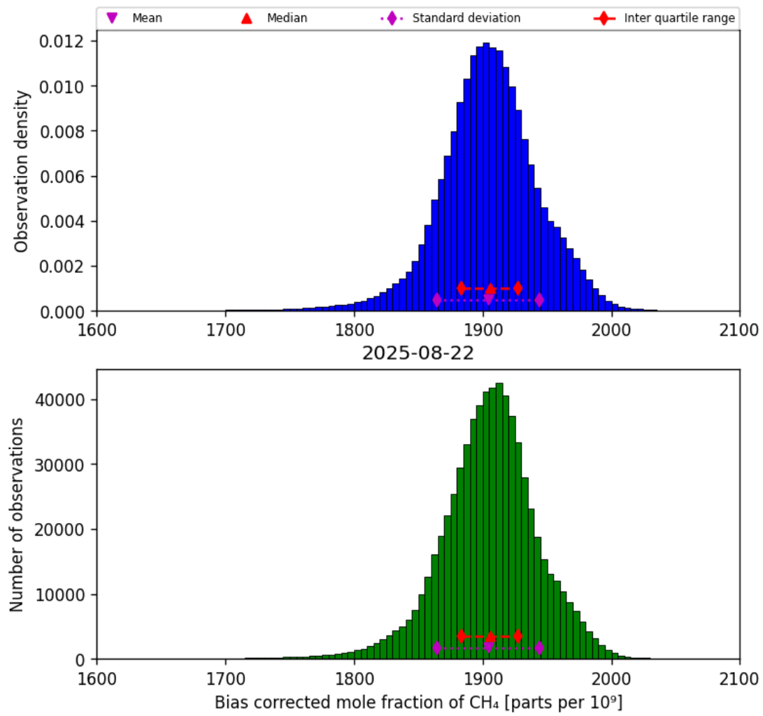
Figure 25: Histogram of “Bias corrected mole fraction of CH 4 ” for 2025-08-21 to 2025-08-23
