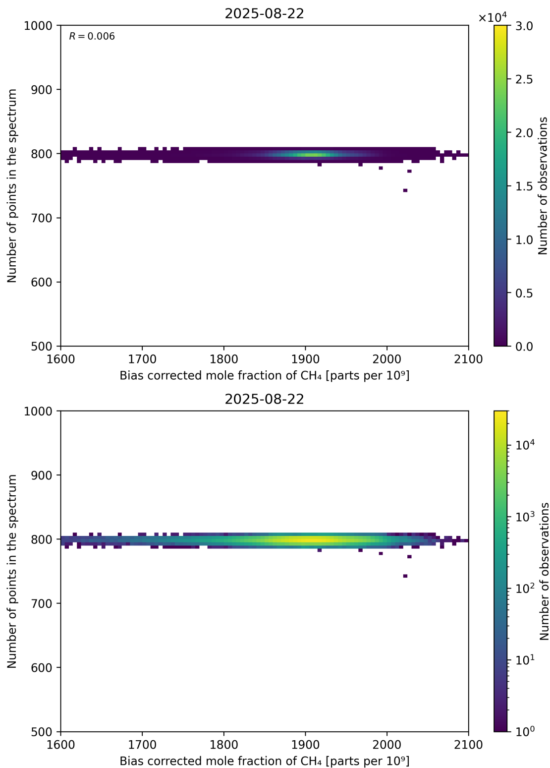
Figure 68: Scatter density plot of “Bias corrected mole fraction of CH 4 ” against “Number of points in the spectrum” for 2025-08-21 to 2025-08-23.
