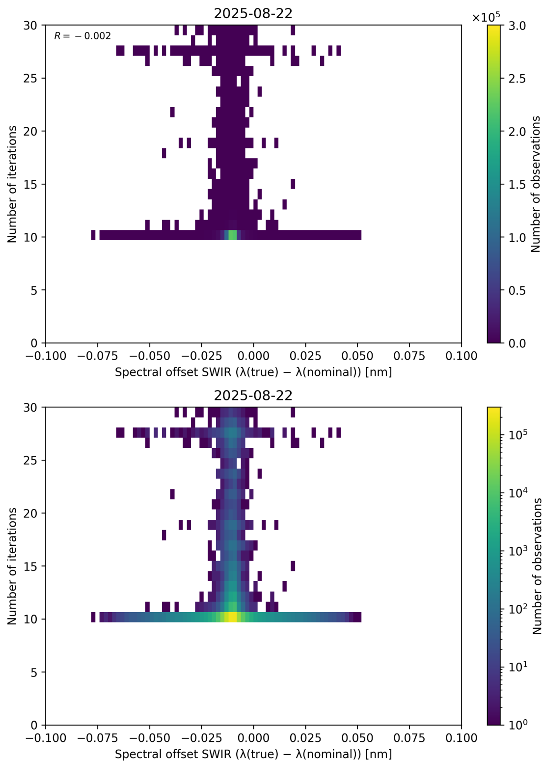
Figure 121: Scatter density plot of “Spectral offset SWIR ( \lambda_{\text{true}} - \lambda_{\text{nominal}} )” against “Number of iterations” for 2025-08-21 to 2025-08-23.
