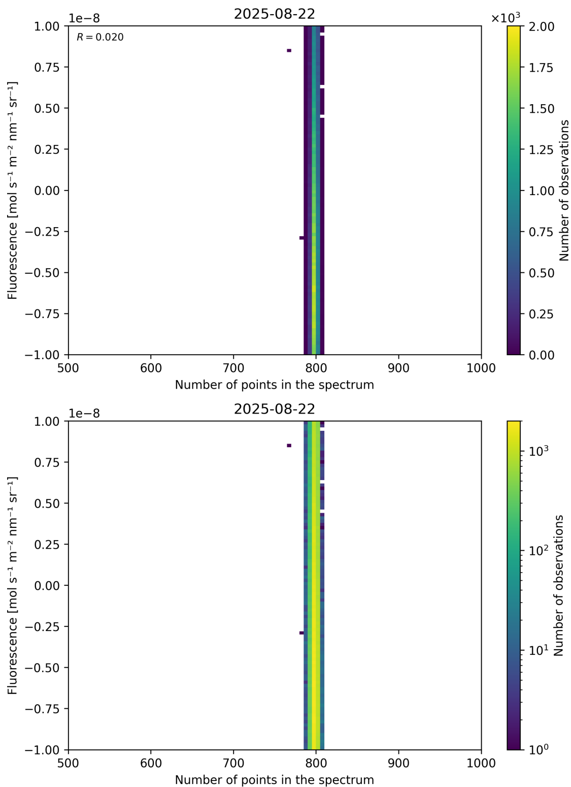
Figure 91: Scatter density plot of “Number of points in the spectrum” against “Fluorescence” for 2025-08-21 to 2025-08-23.
