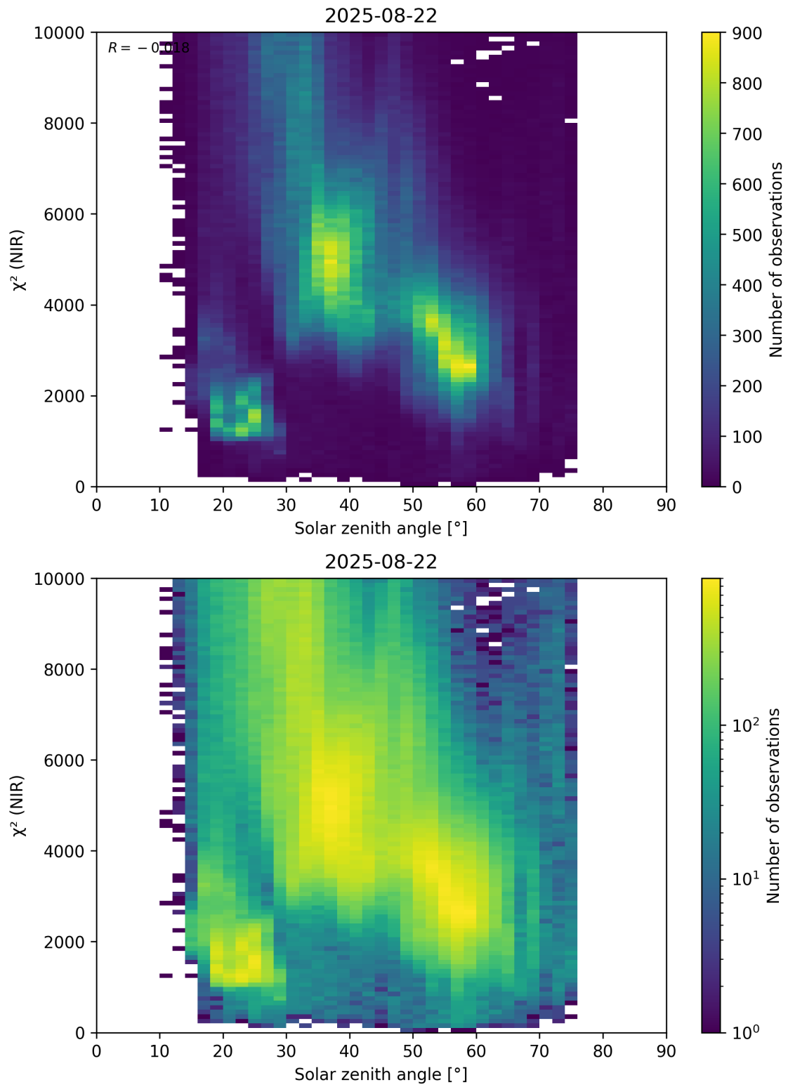
Figure 94: Scatter density plot of “Solar zenith angle” against “ \chi^2 (NIR)” for 2025-08-21 to 2025-08-23.
