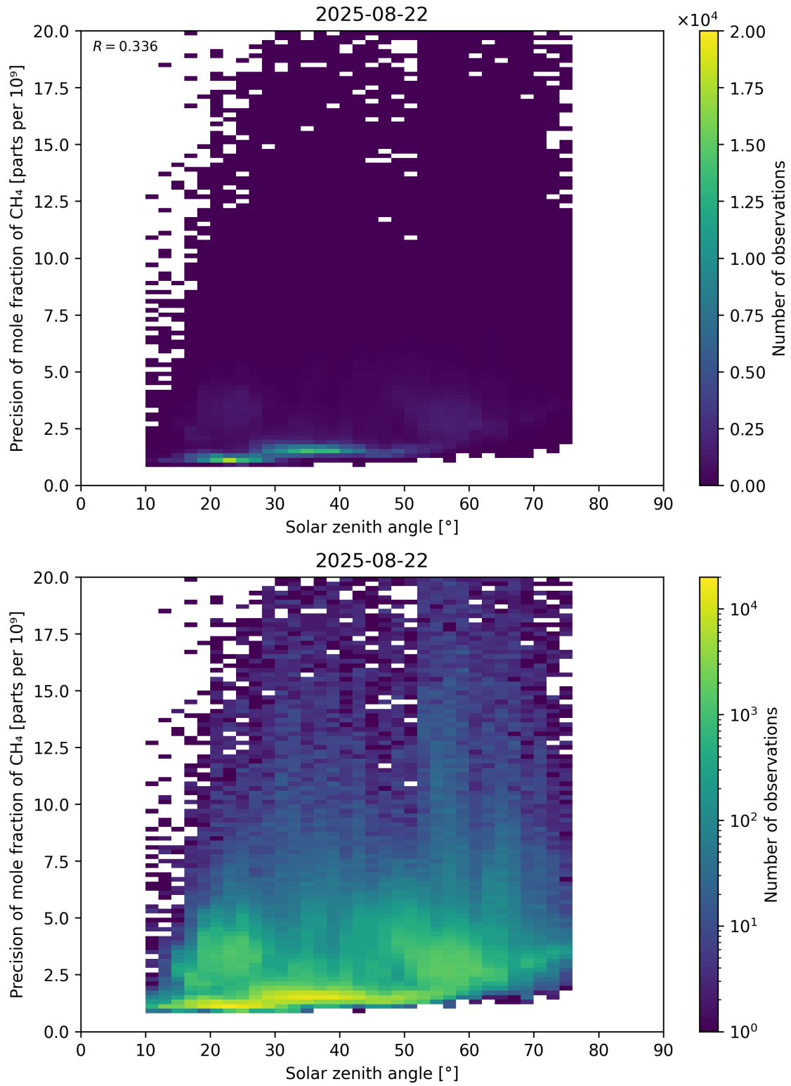
Figure 101: Scatter density plot of “Solar zenith angle” against “Precision of mole fraction of CH 4 ” for 2025-08-21 to 2025-08-23.
