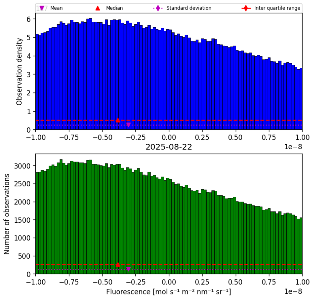
Figure 32: Histogram of “Fluorescence” for 2025-08-21 to 2025-08-23
