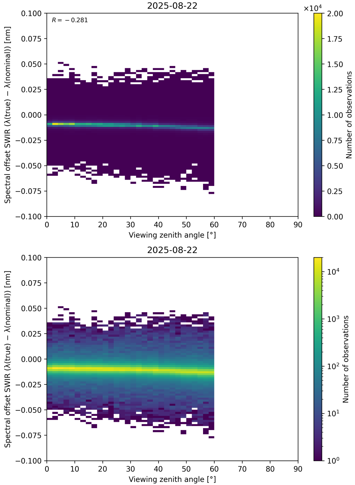
Figure 116: Scatter density plot of “Viewing zenith angle” against “Spectral offset SWIR ( \lambda_{\text{true}} - \lambda_{\text{nominal}} )” for 2025-08-21 to 2025-08-23.
