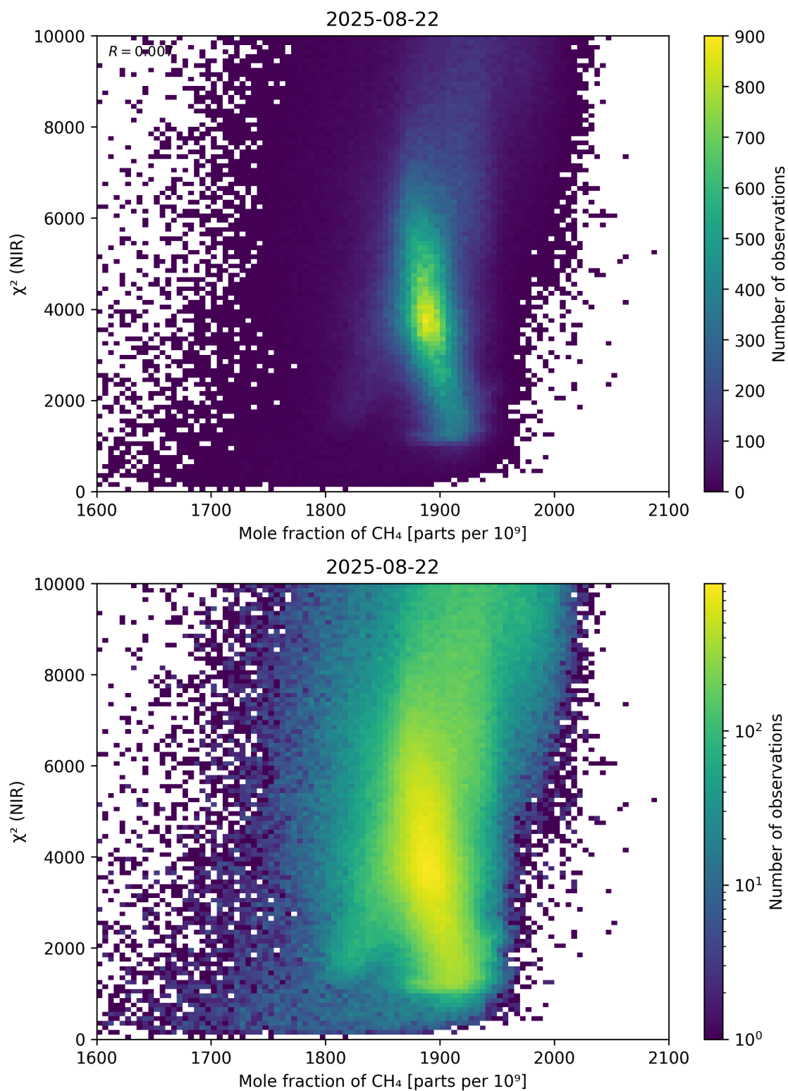
Figure 70: Scatter density plot of “Mole fraction of CH 4 ” against “ \chi^2 (NIR)” for 2025-08-21 to 2025-08-23.
