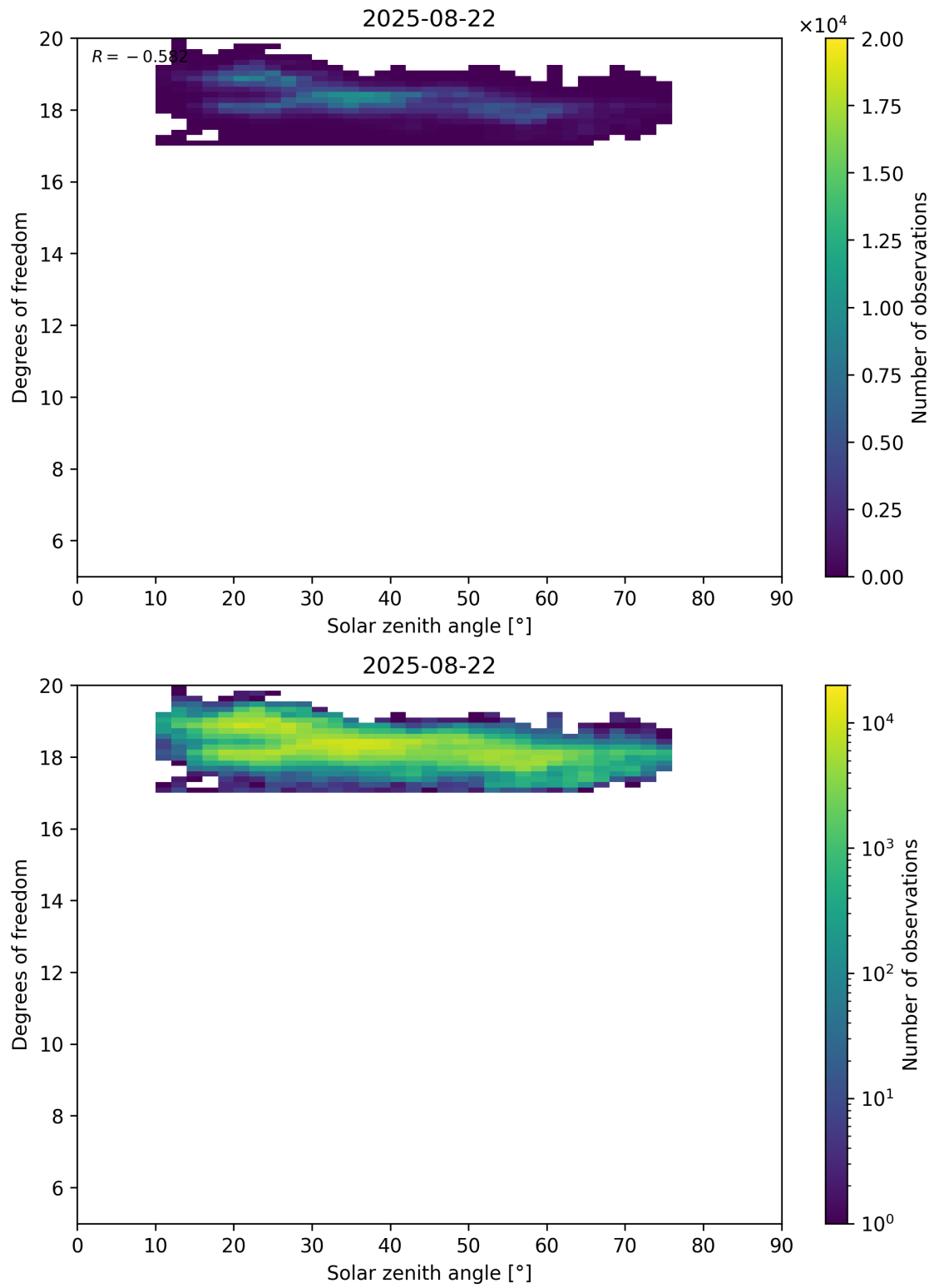
Figure 96: Scatter density plot of “Solar zenith angle” against “Degrees of freedom” for 2025-08-21 to 2025-08-23.
