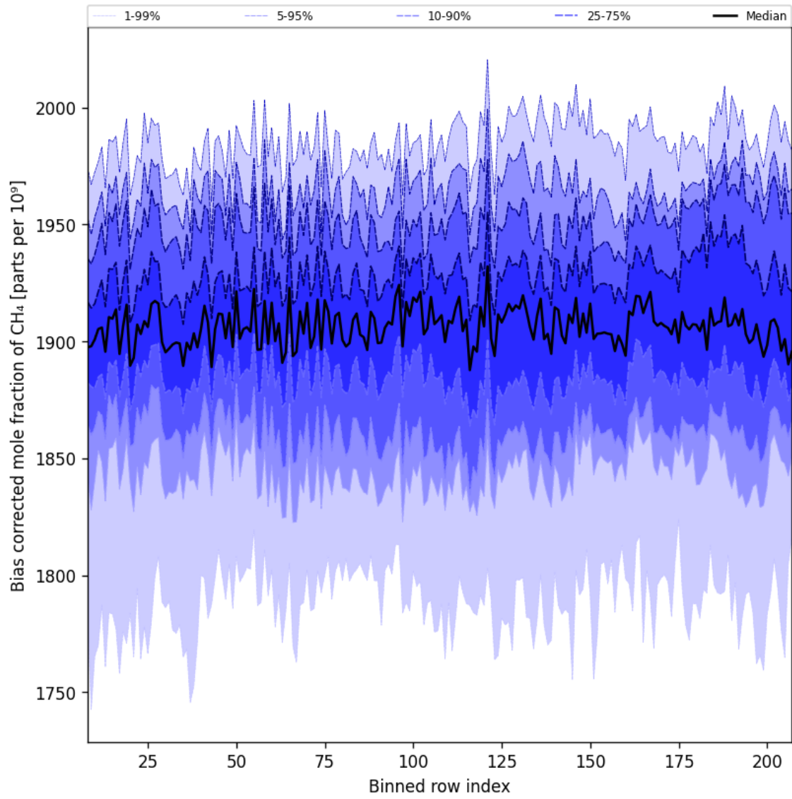
Figure 36: Along track statistics of “Bias corrected mole fraction of CH 4 ” for 2025-08-21 to 2025-08-23
