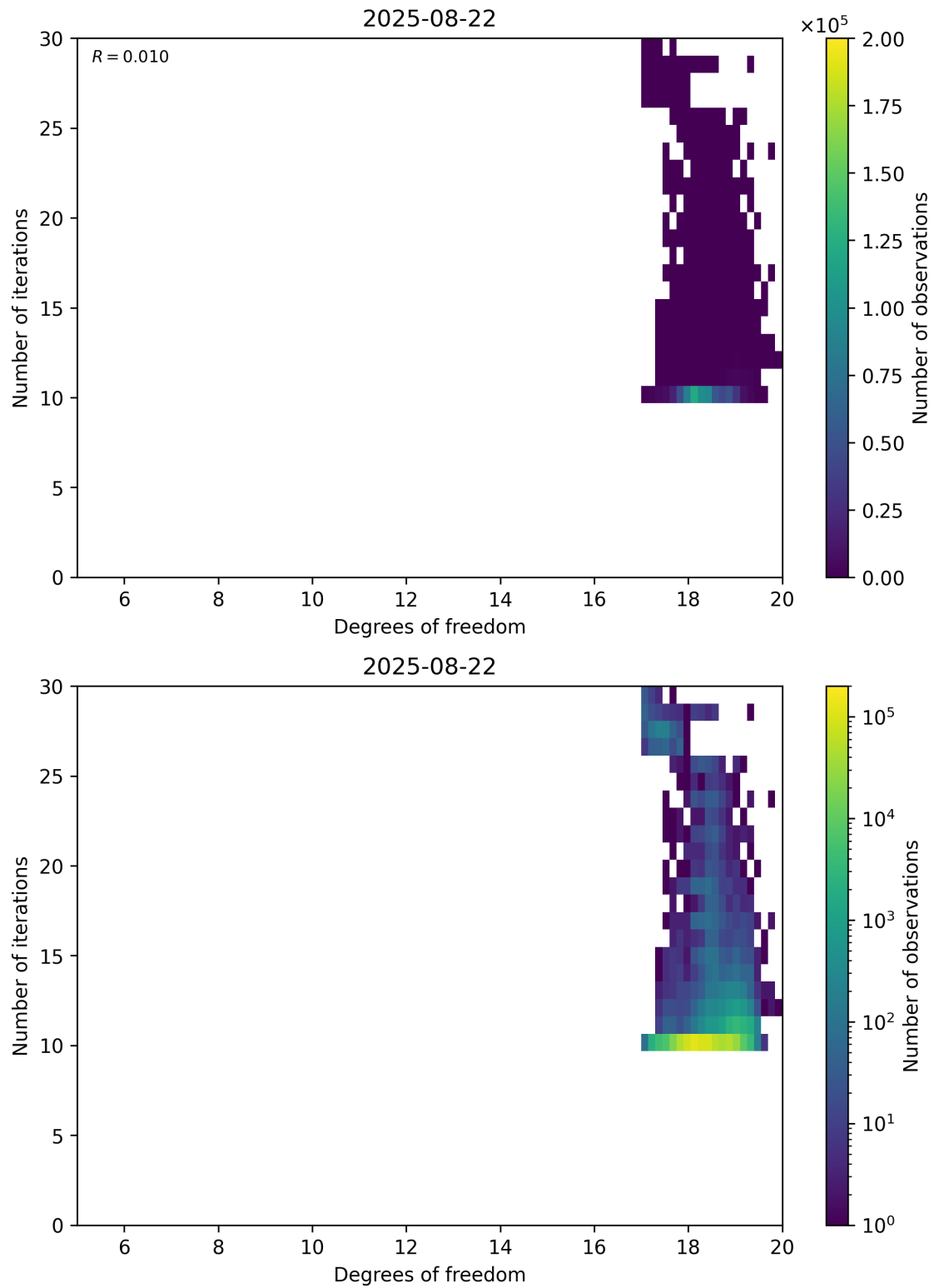
Figure 52: Scatter density plot of “Degrees of freedom” against “Number of iterations” for 2025-08-21 to 2025-08-23.
