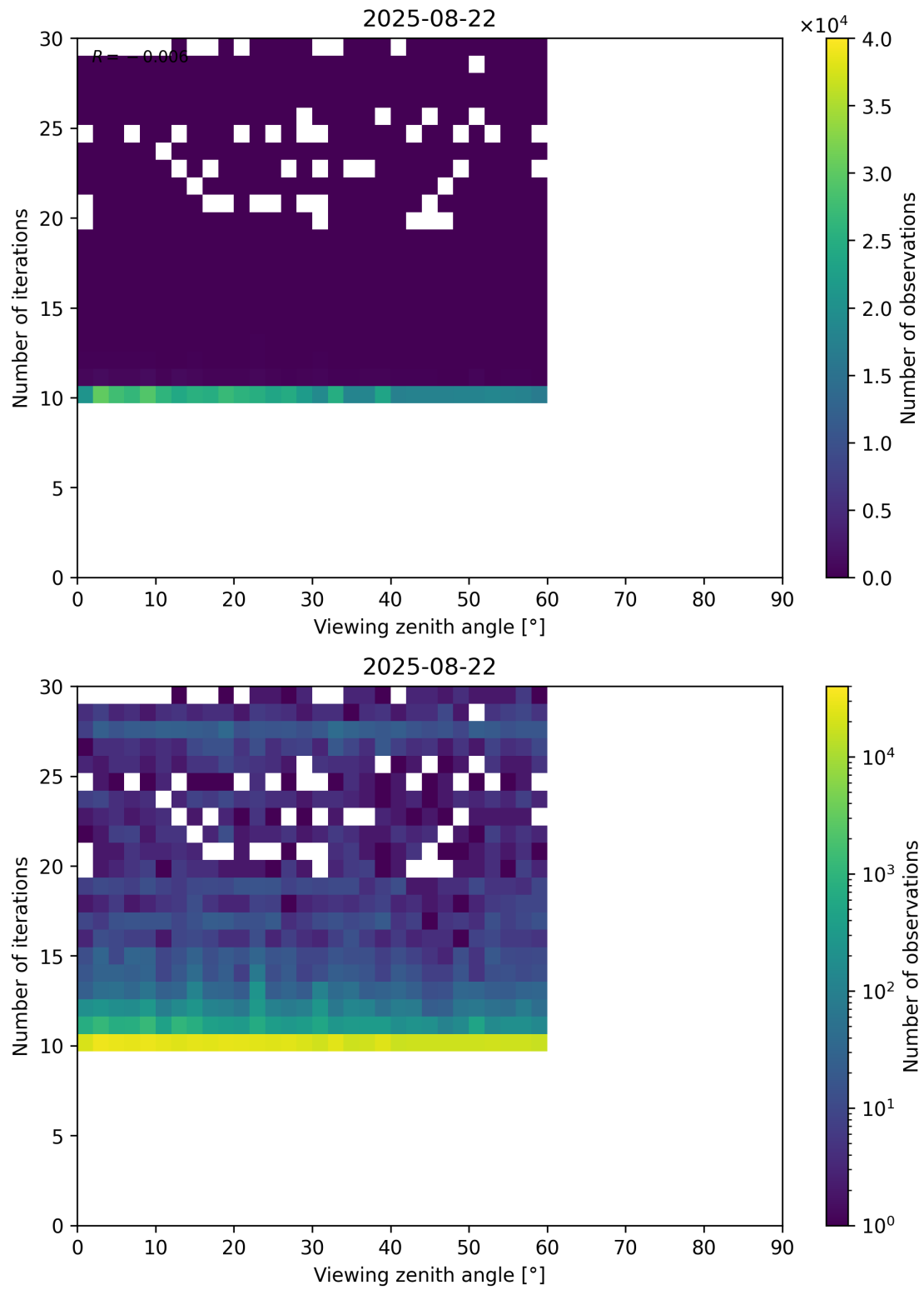
Figure 113: Scatter density plot of “Viewing zenith angle” against “Number of iterations” for 2025-08-21 to 2025-08-23.
