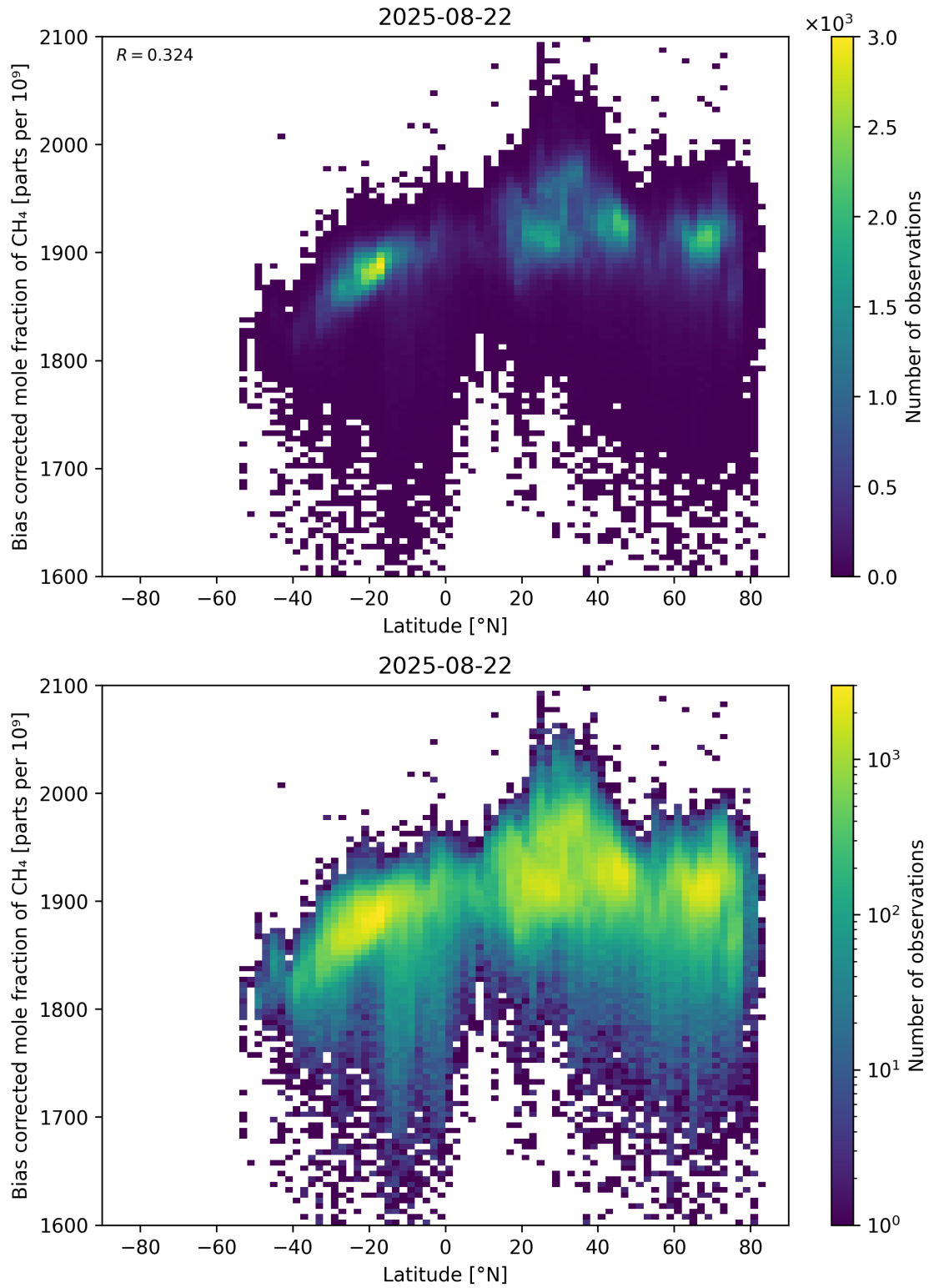
Figure 58: Scatter density plot of “Latitude” against “Bias corrected mole fraction of CH 4 ” for 2025-08-21 to 2025-08-23.
