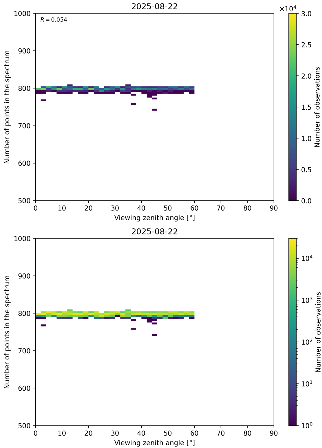
Figure 114: Scatter density plot of “Viewing zenith angle” against “Number of points in the spectrum” for 2025-08-21 to 2025-08-23.
