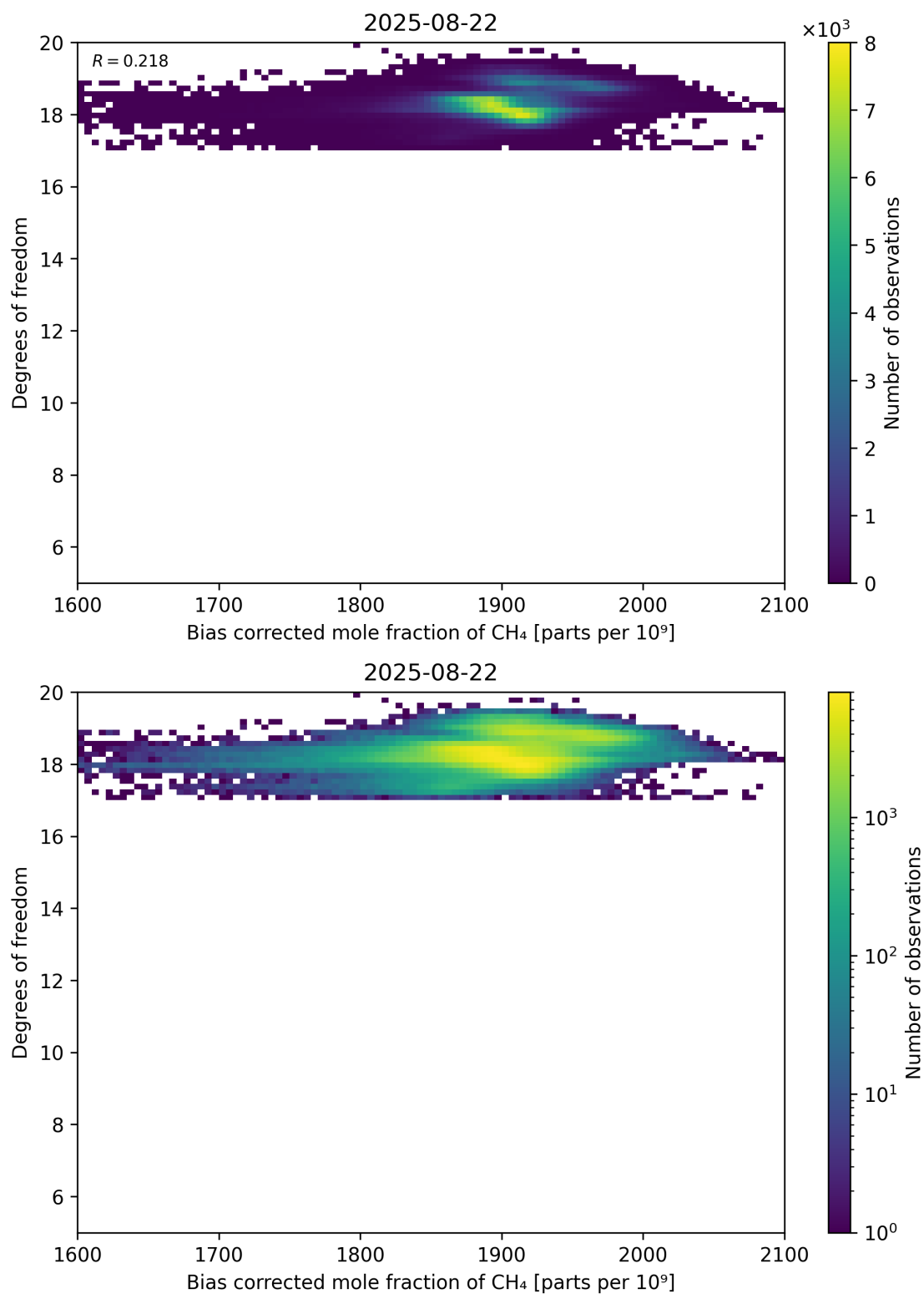
Figure 65: Scatter density plot of “Bias corrected mole fraction of CH 4 ” against “Degrees of freedom” for 2025-08-21 to 2025-08-23.
