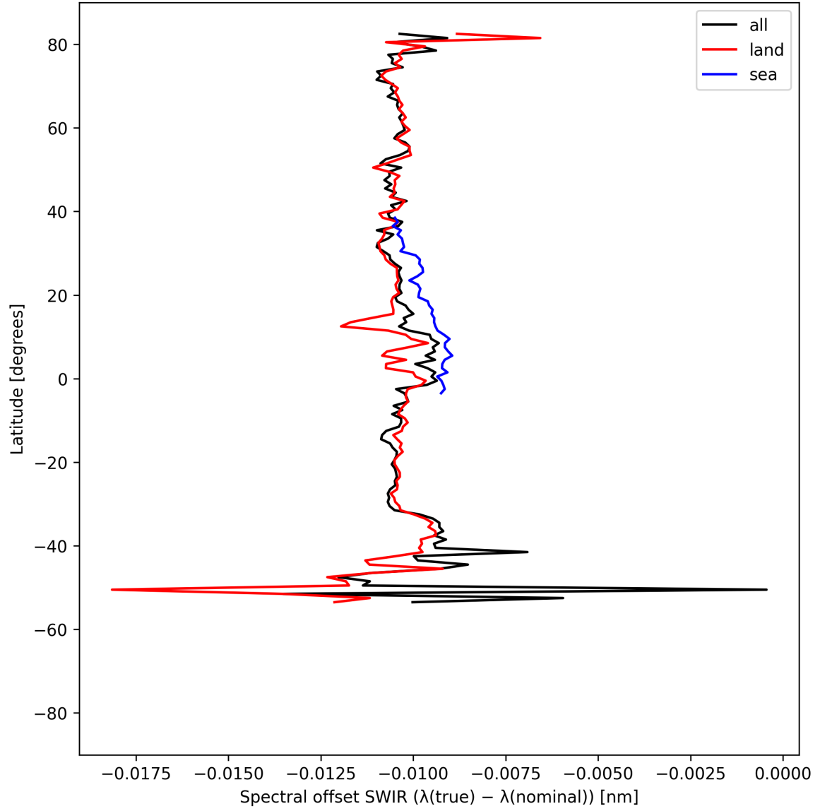
Figure 16: Zonal average of “Spectral offset SWIR ( \lambda_{\text{true}} - \lambda_{\text{nominal}} )” for 2025-08-21 to 2025-08-23.
