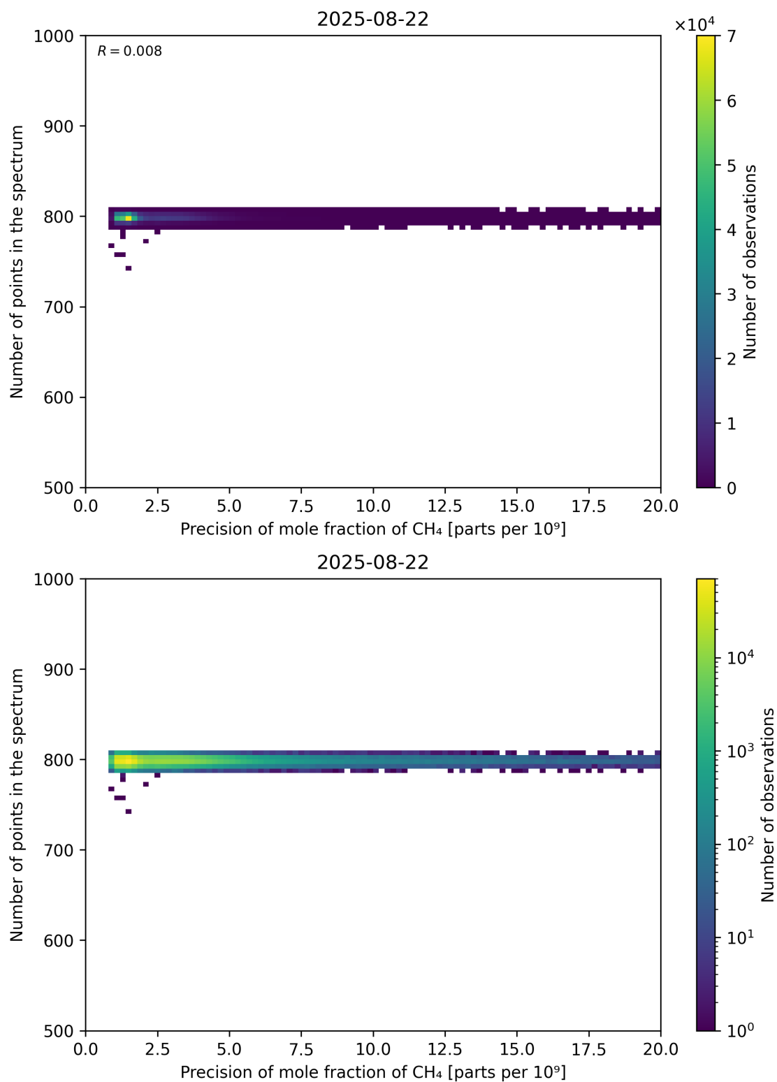
Figure 84: Scatter density plot of “Precision of mole fraction of CH 4 ” against “Number of points in the spectrum” for 2025-08-21 to 2025-08-23.
