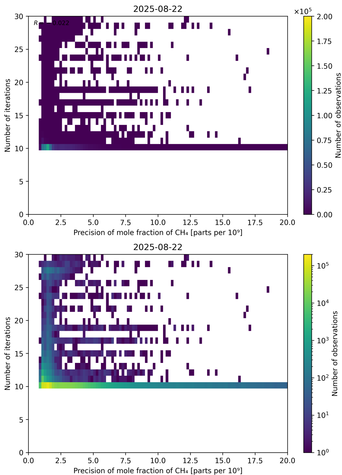
Figure 83: Scatter density plot of “Precision of mole fraction of CH 4 ” against “Number of iterations” for 2025-08-21 to 2025-08-23.
