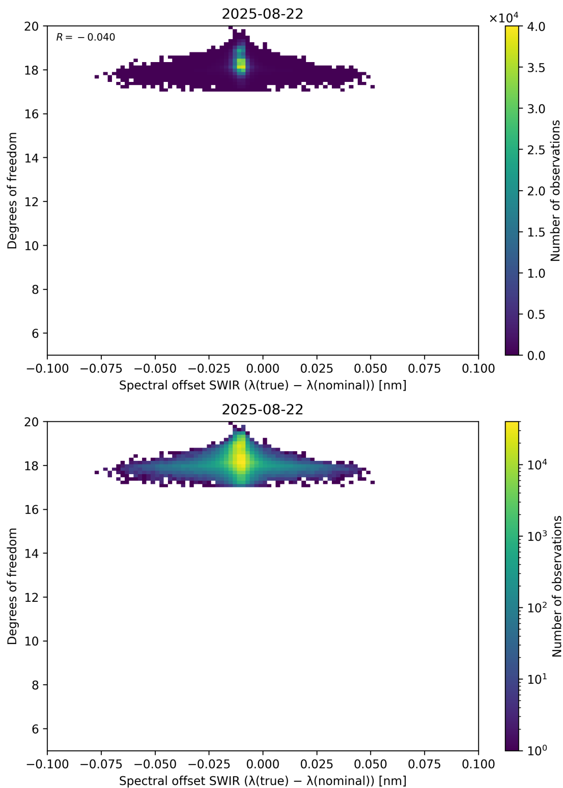
Figure 119: Scatter density plot of “Spectral offset SWIR ( \lambda_{\text{true}} - \lambda_{\text{nominal}} )” against “Degrees of freedom” for 2025-08-21 to 2025-08-23.
