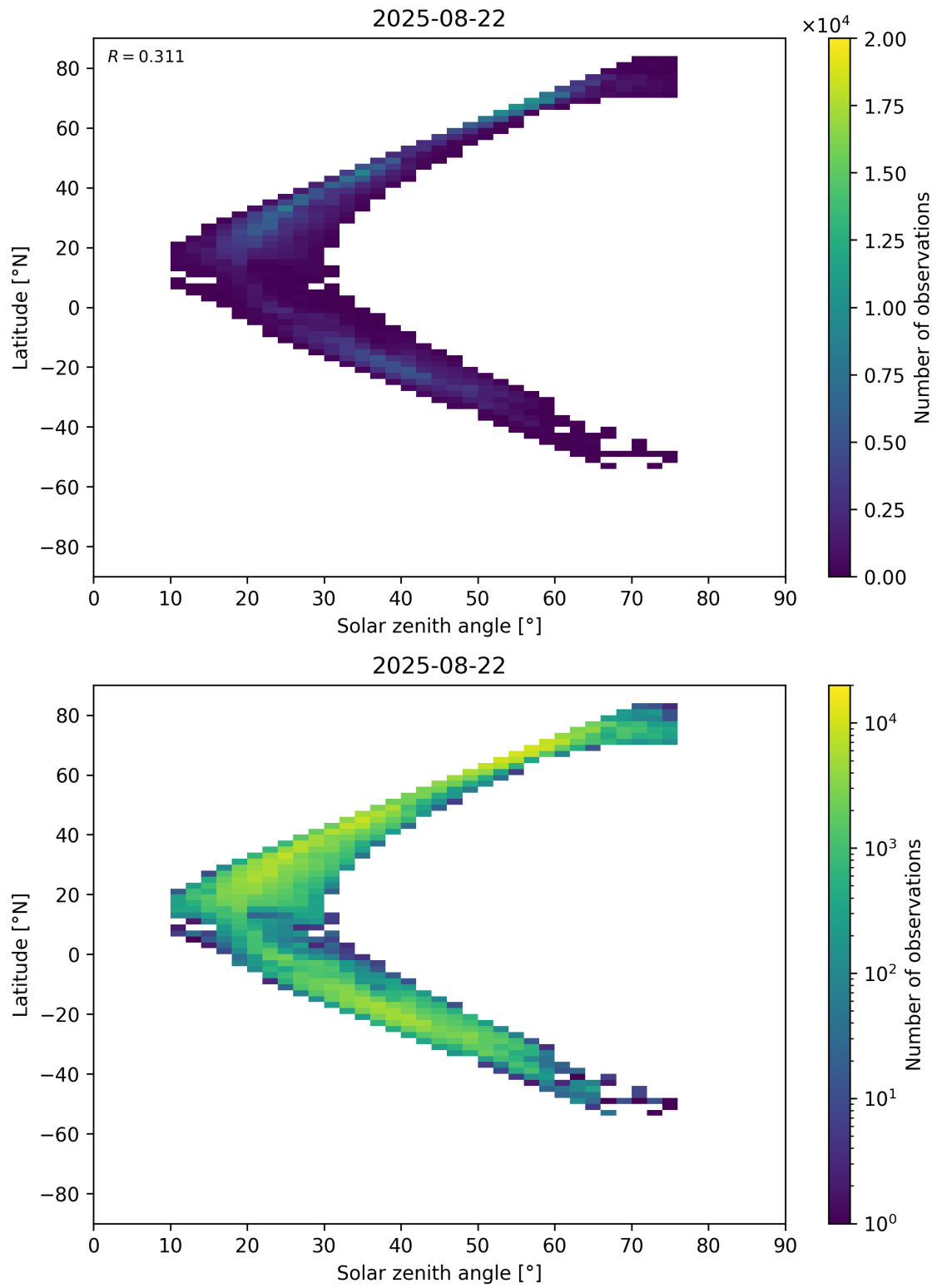
Figure 98: Scatter density plot of “Solar zenith angle” against “Latitude” for 2025-08-21 to 2025-08-23.
