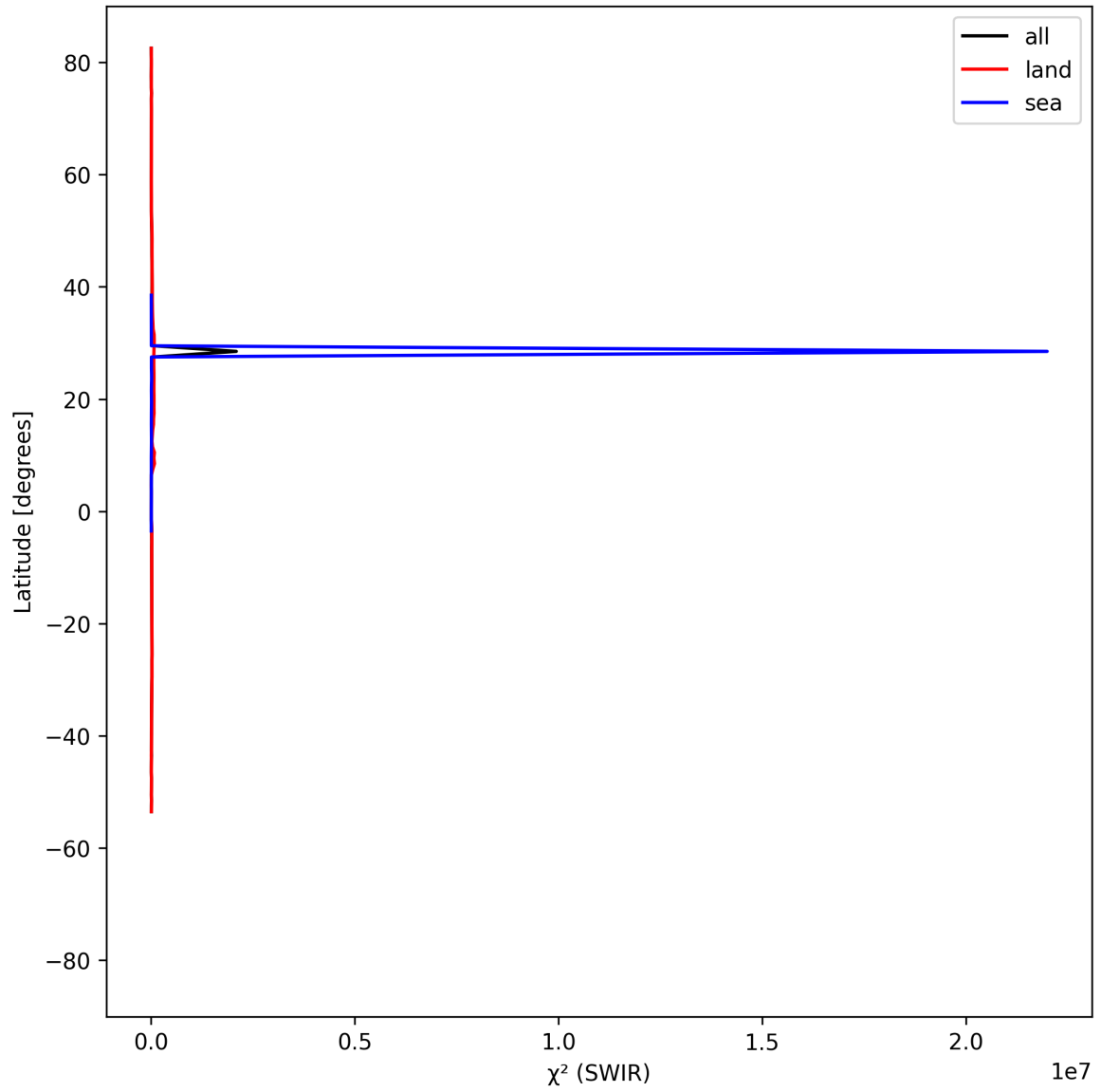
Figure 17: Zonal average of “ \chi^2 (SWIR)” for 2025-08-21 to 2025-08-23.
