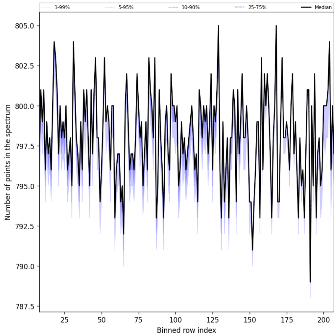
Figure 37: Along track statistics of “Number of points in the spectrum” for 2025-08-21 to 2025-08-23
