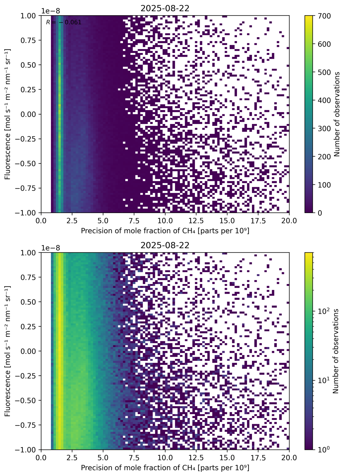
Figure 81: Scatter density plot of “Precision of mole fraction of \text{CH}_4 ” against “Fluorescence” for 2025-08-21 to 2025-08-23.
