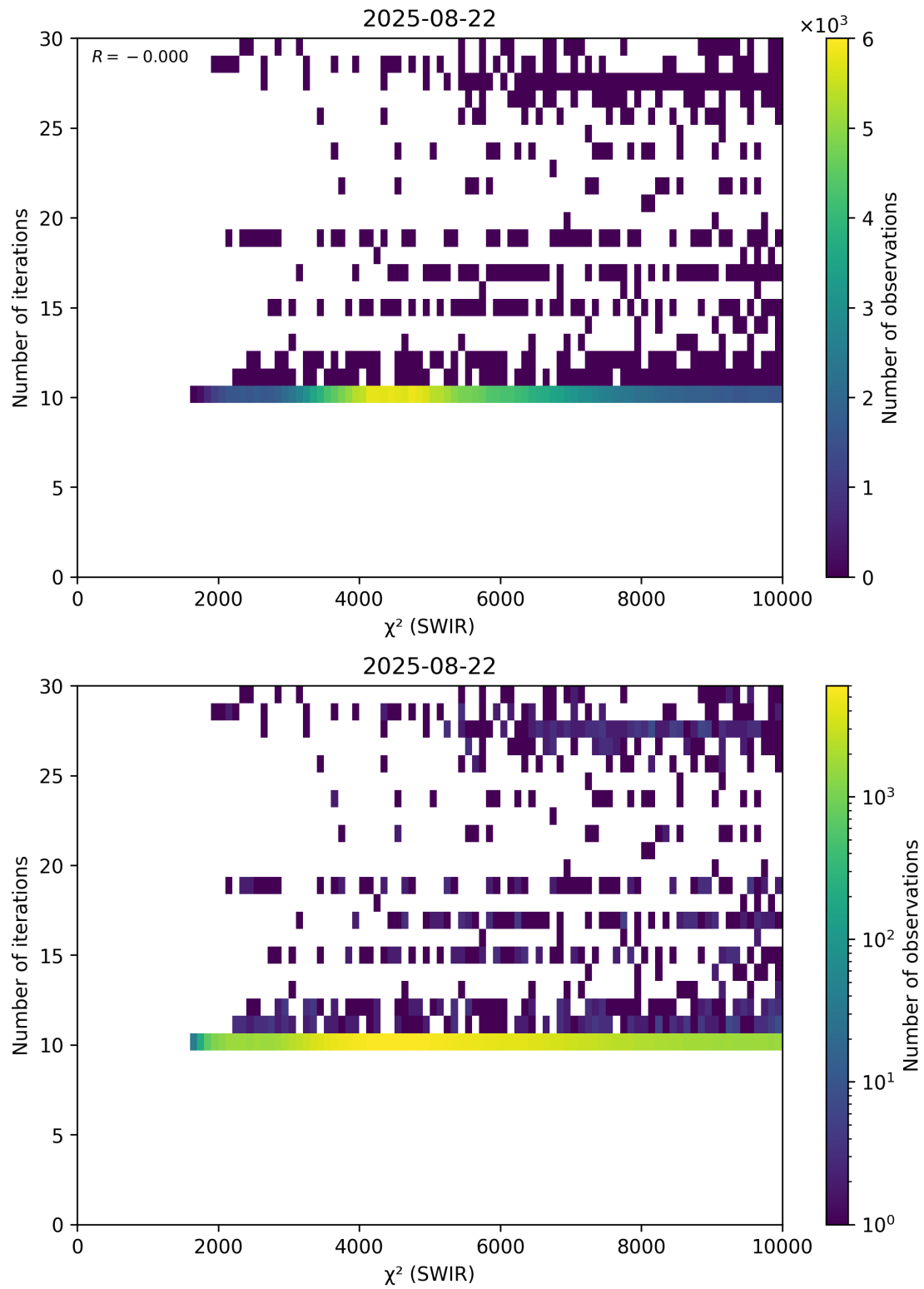
Figure 50: Scatter density plot of “ \chi^2 (SWIR)” against “Number of iterations” for 2025-08-21 to 2025-08-23.
