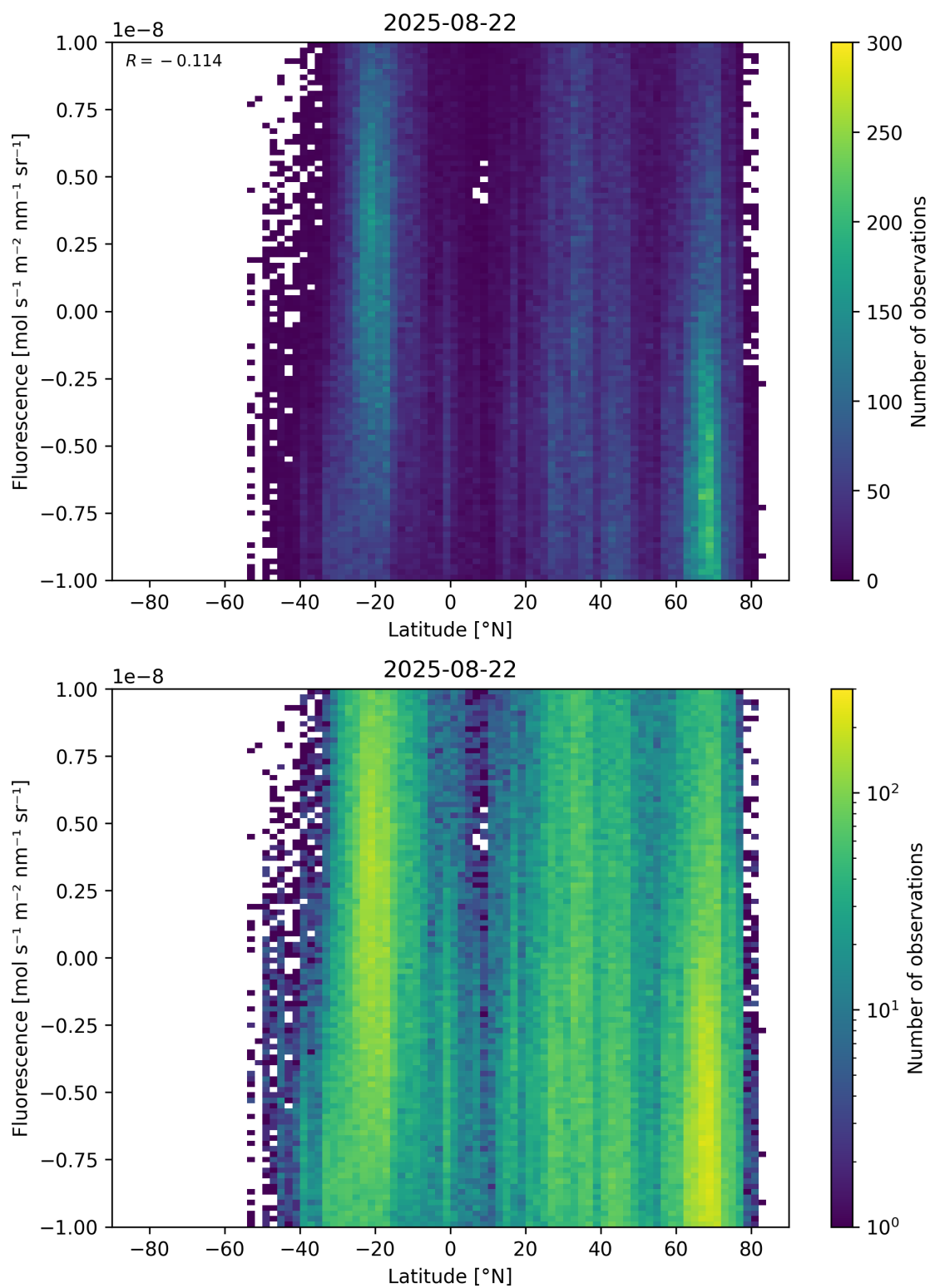
Figure 56: Scatter density plot of “Latitude” against “Fluorescence” for 2025-08-21 to 2025-08-23.
