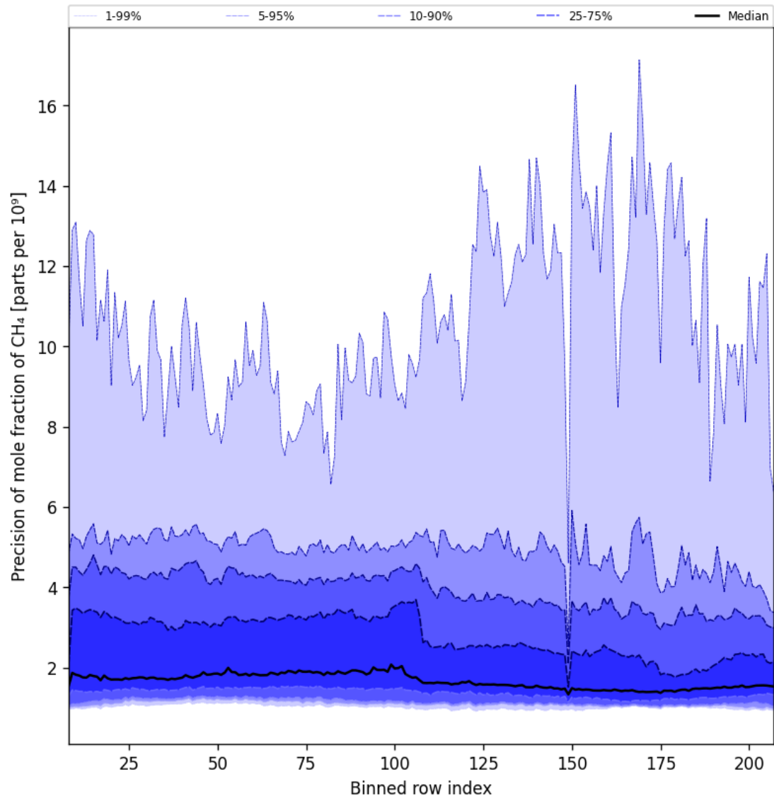
Figure 35: Along track statistics of “Precision of mole fraction of CH 4 ” for 2025-08-21 to 2025-08-23
