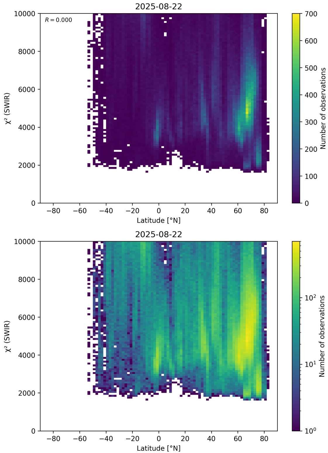
Figure 54: Scatter density plot of “Latitude” against “ \chi^2 (SWIR)” for 2025-08-21 to 2025-08-23.
