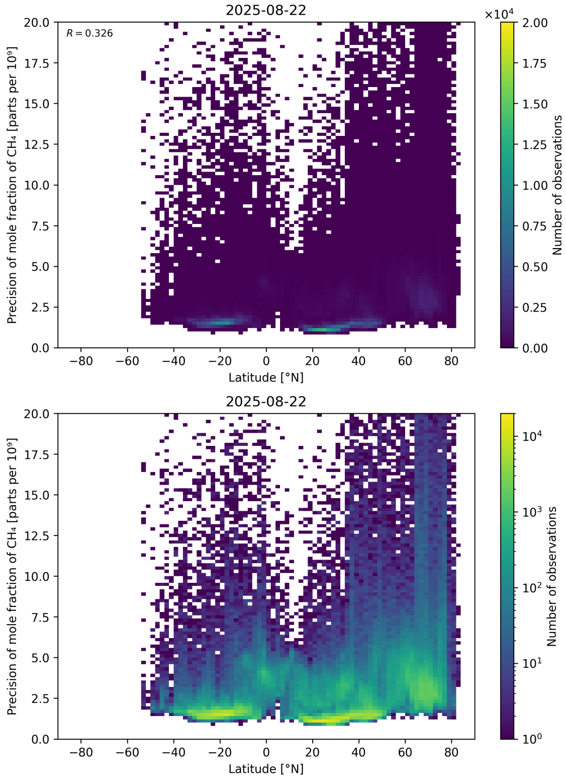
Figure 59: Scatter density plot of “Latitude” against “Precision of mole fraction of \text{CH}_4 ” for 2025-08-21 to 2025-08-23.
