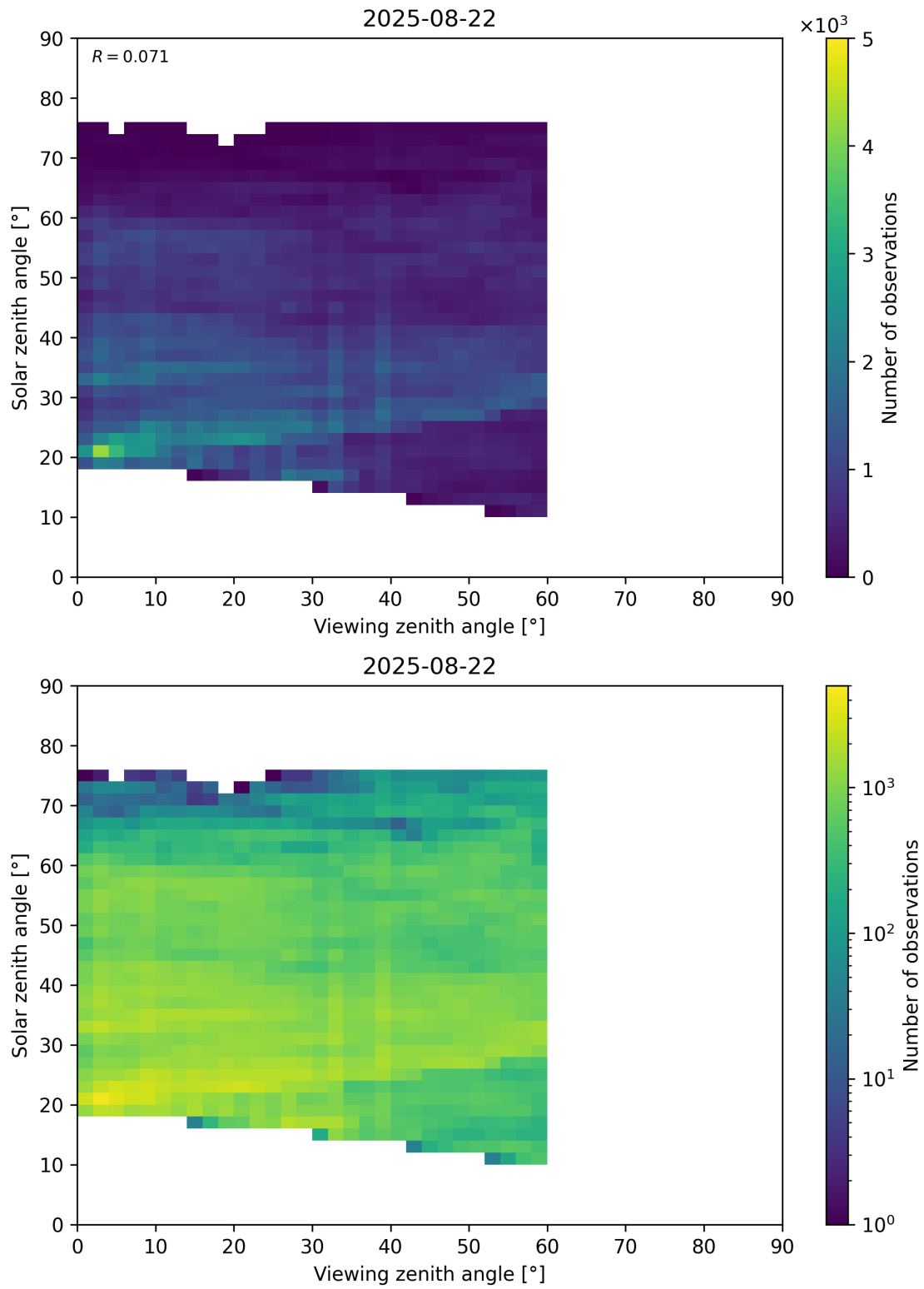
Figure 115: Scatter density plot of “Viewing zenith angle” against “Solar zenith angle” for 2025-08-21 to 2025-08-23.
