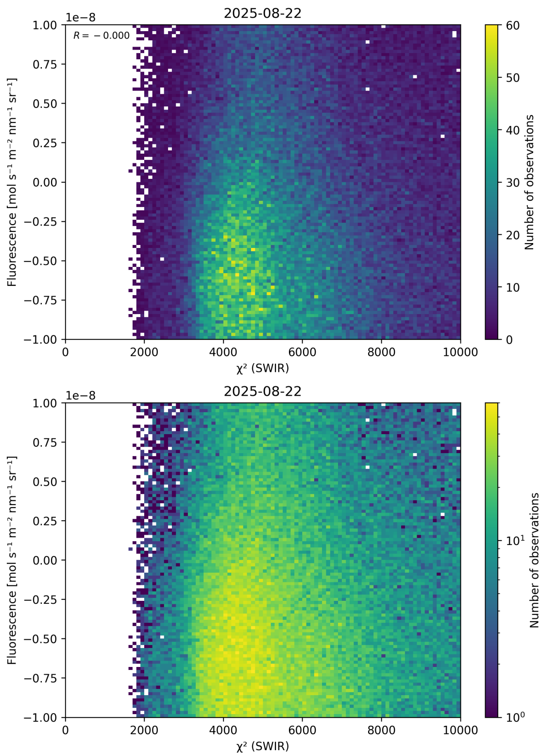
Figure 49: Scatter density plot of “ \chi^2 (SWIR)” against “Fluorescence” for 2025-08-21 to 2025-08-23.
