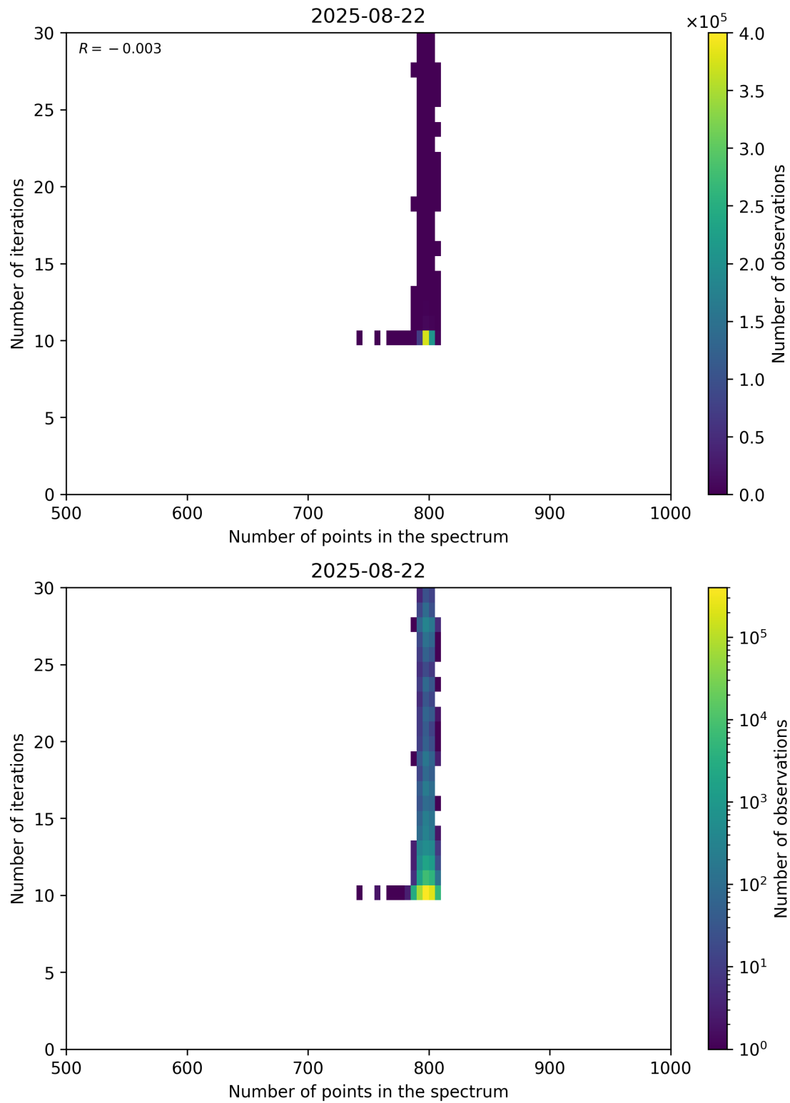
Figure 92: Scatter density plot of “Number of points in the spectrum” against “Number of iterations” for 2025-08-21 to 2025-08-23.
