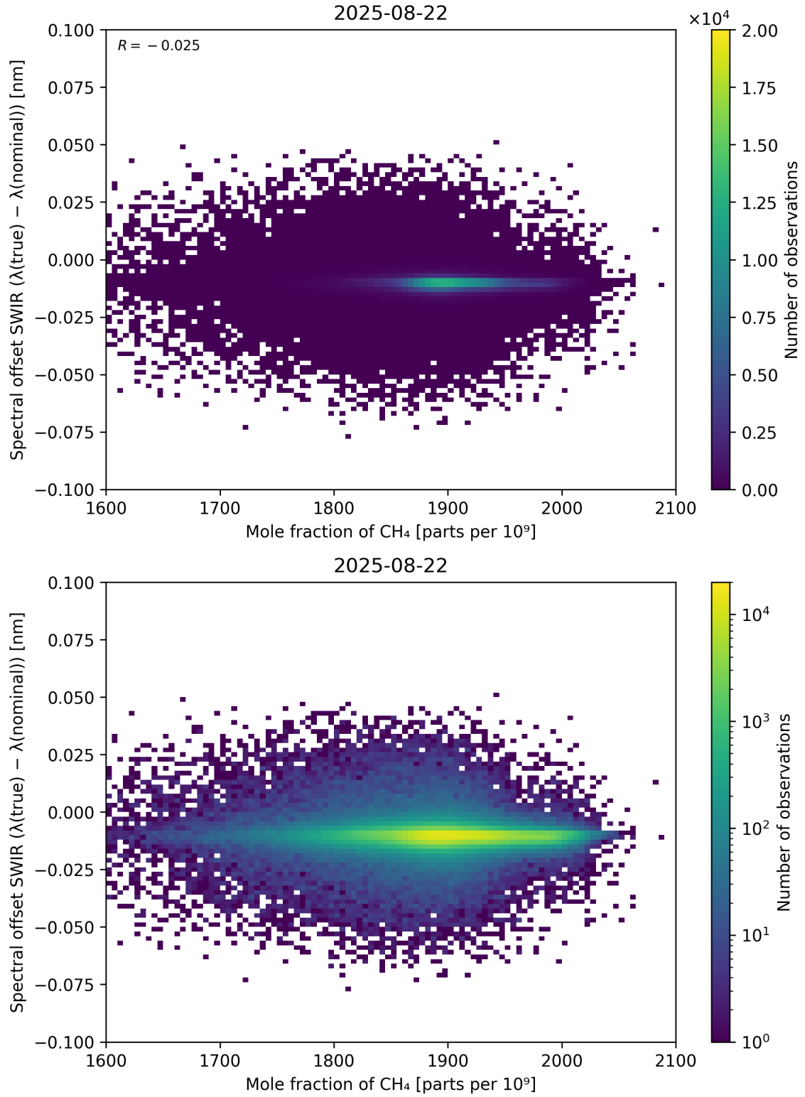
Figure 86: Scatter density plot of “Mole fraction of \text{CH}_4 ” against “Spectral offset SWIR ( \lambda_{\text{true}} - \lambda_{\text{nominal}} )” for 2025-08-21 to 2025-08-23.
