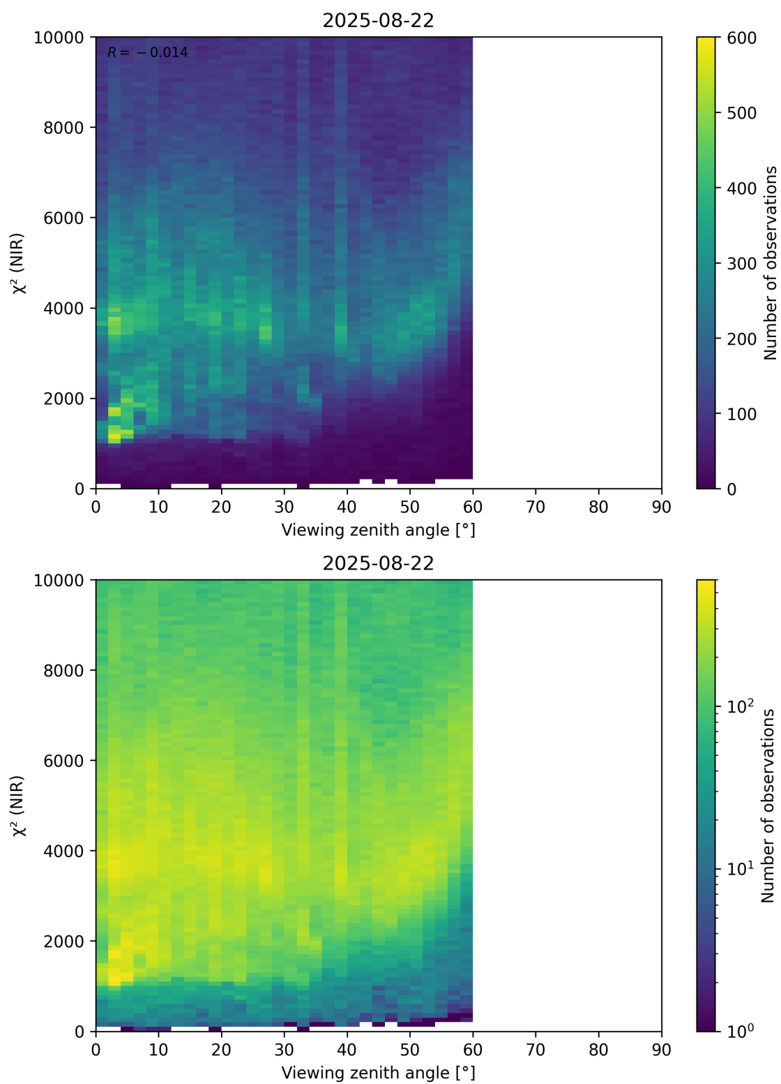
Figure 105: Scatter density plot of “Viewing zenith angle” against “ \chi^2 (NIR)” for 2025-08-21 to 2025-08-23.
