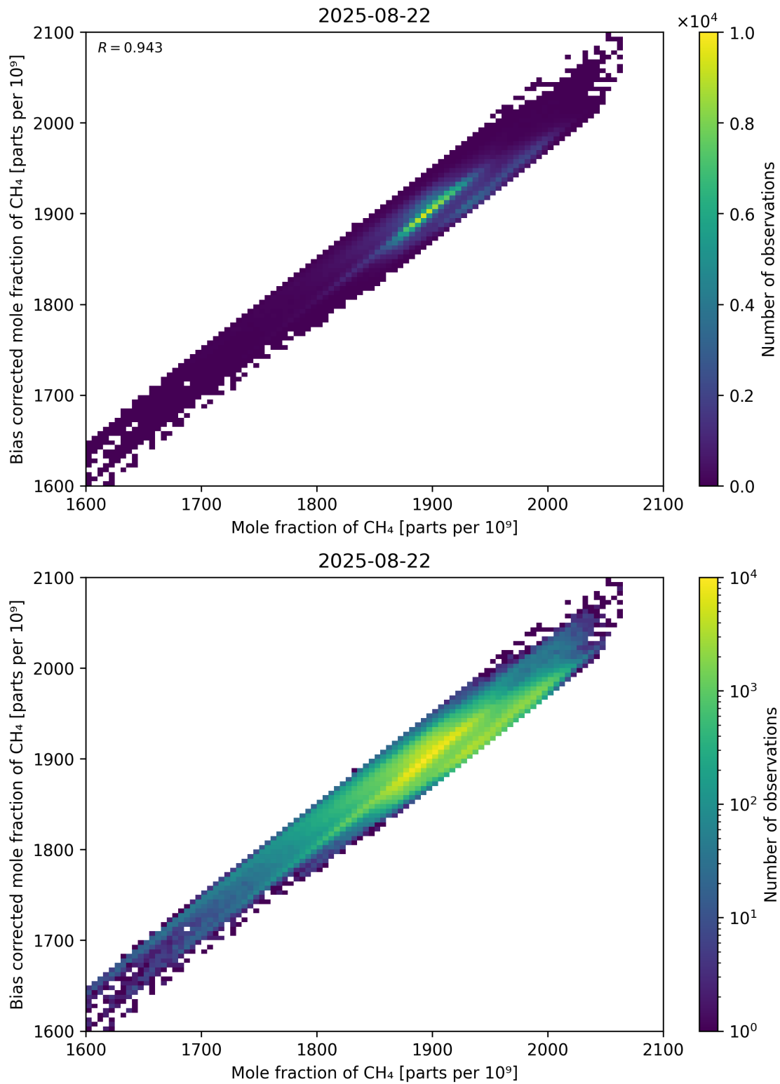
Figure 74: Scatter density plot of “Mole fraction of CH 4 ” against “Bias corrected mole fraction of CH 4 ” for 2025-08-21 to 2025-08-23.
