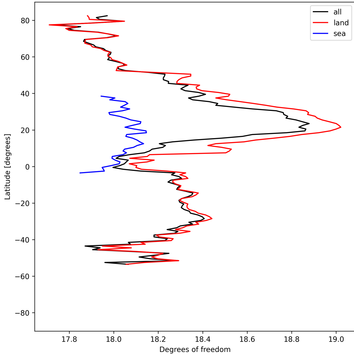
Figure 19: Zonal average of “Degrees of freedom” for 2025-08-21 to 2025-08-23.
