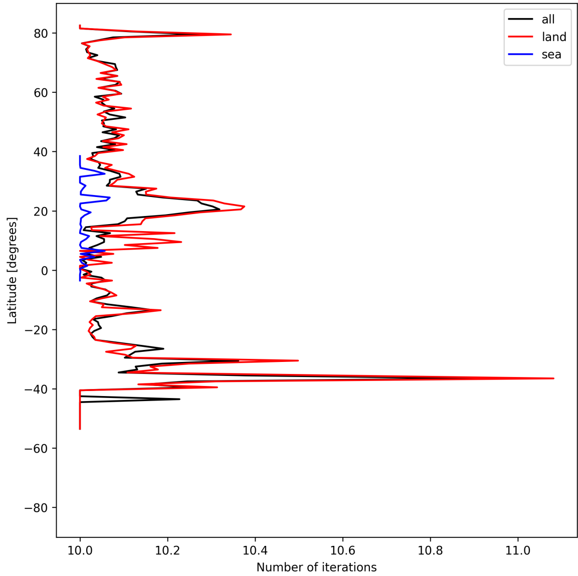
Figure 20: Zonal average of “Number of iterations” for 2025-08-21 to 2025-08-23.
