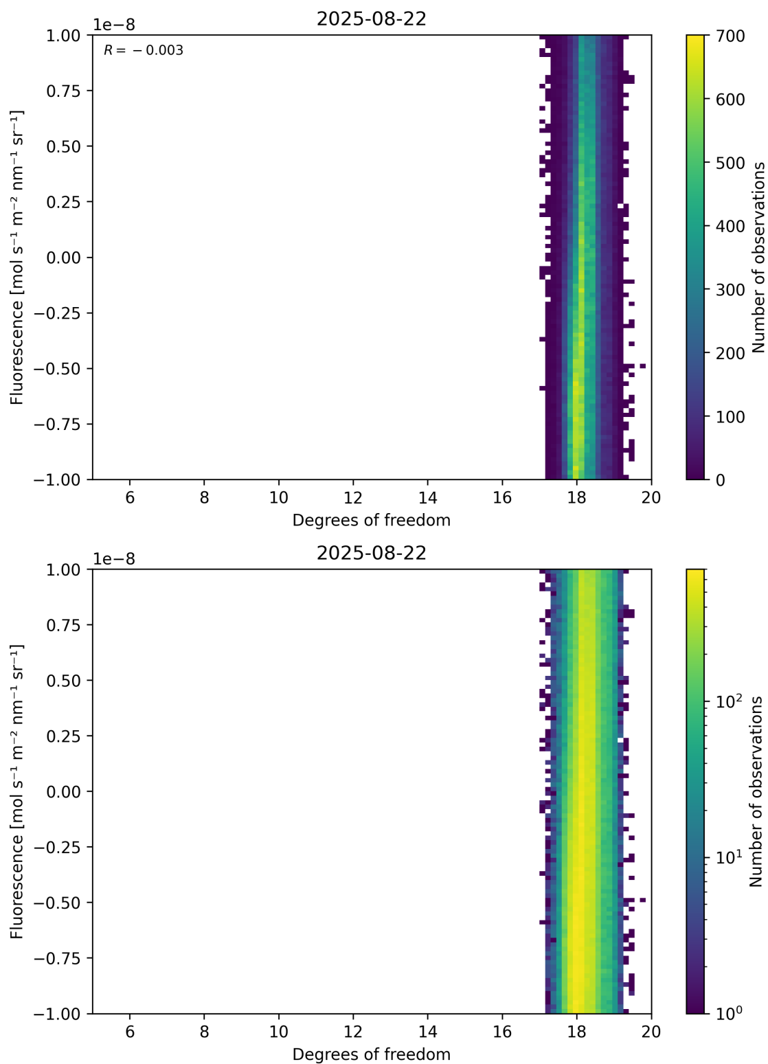
Figure 51: Scatter density plot of “Degrees of freedom” against “Fluorescence” for 2025-08-21 to 2025-08-23.
