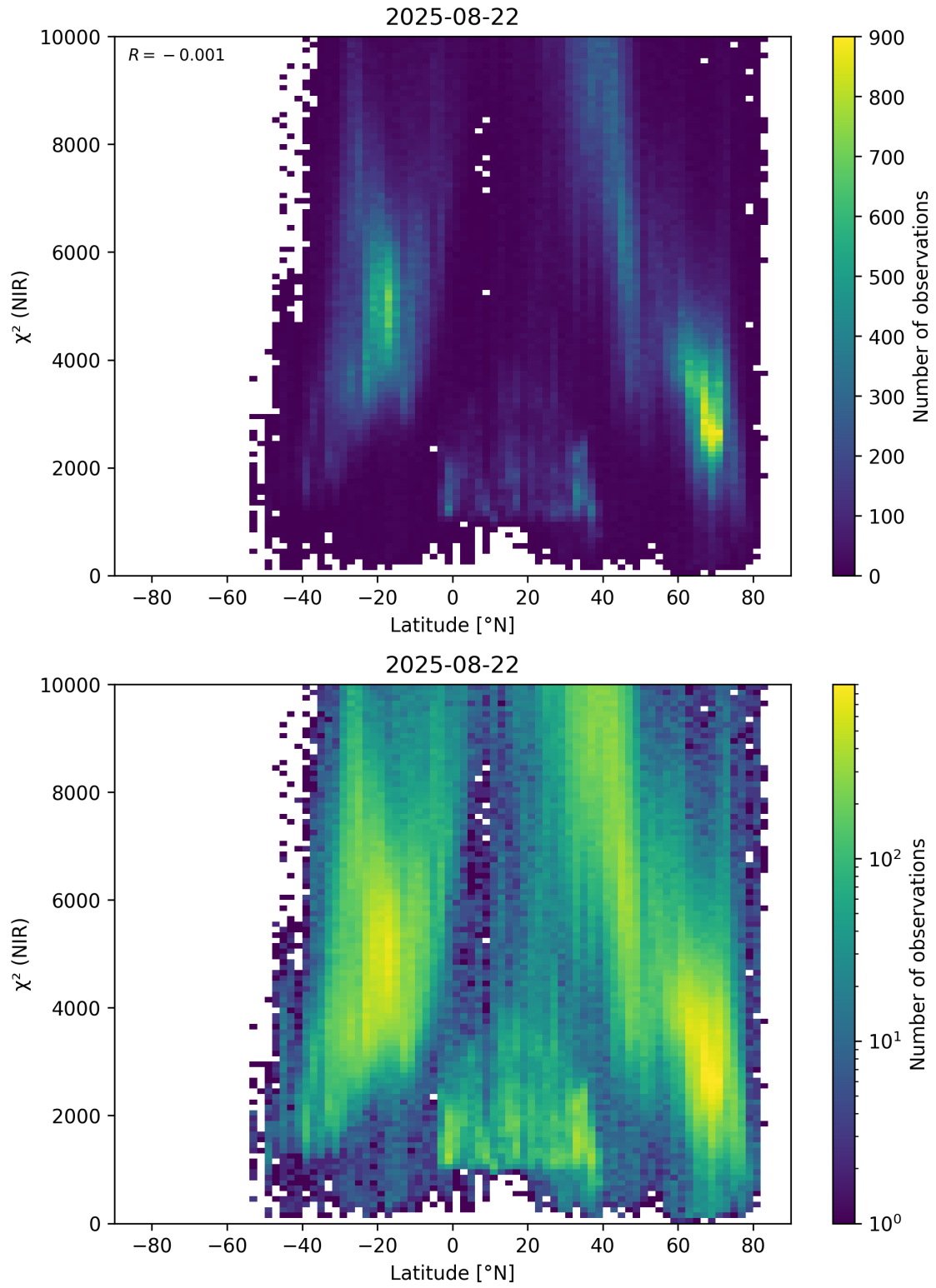
Figure 53: Scatter density plot of “Latitude” against “ \chi^2 (NIR)” for 2025-08-21 to 2025-08-23.
