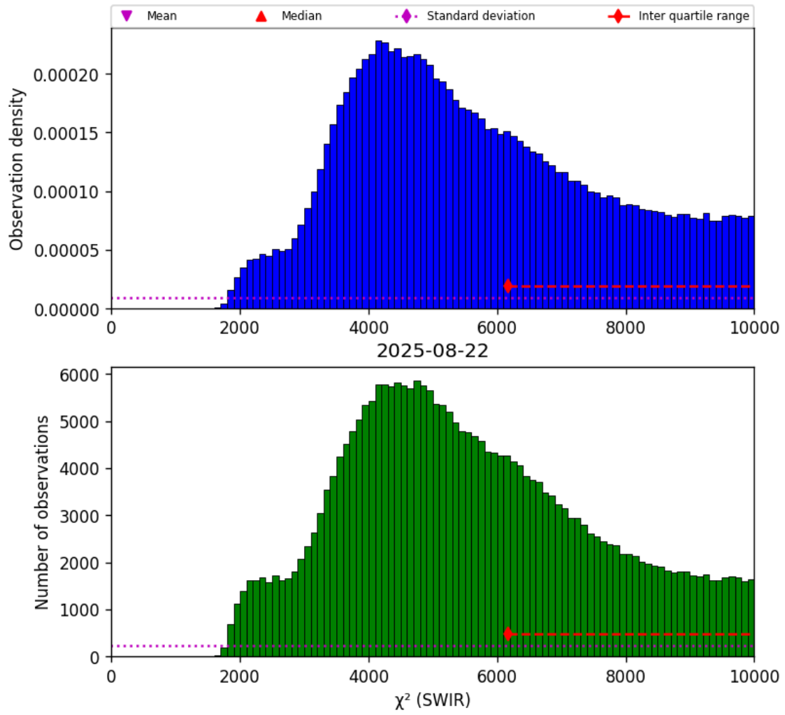
Figure 28: Histogram of “ \chi^2 (SWIR)” for 2025-08-21 to 2025-08-23
