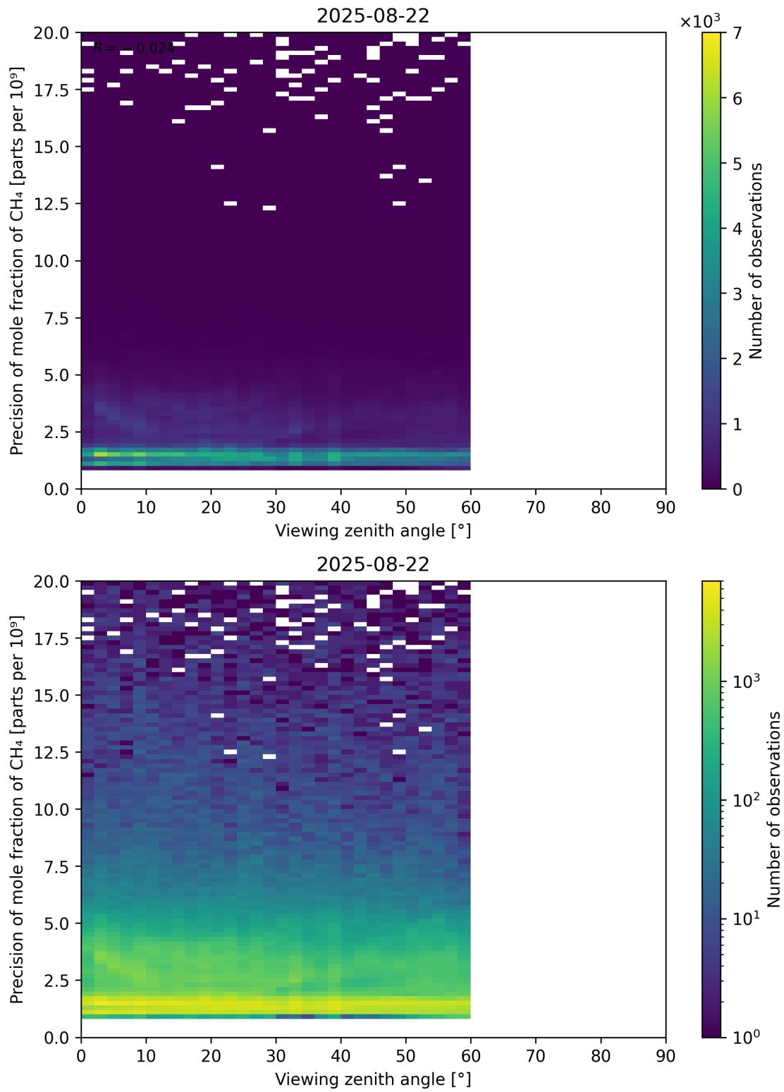
Figure 112: Scatter density plot of “Viewing zenith angle” against “Precision of mole fraction of CH 4 ” for 2025-08-21 to 2025-08-23.
