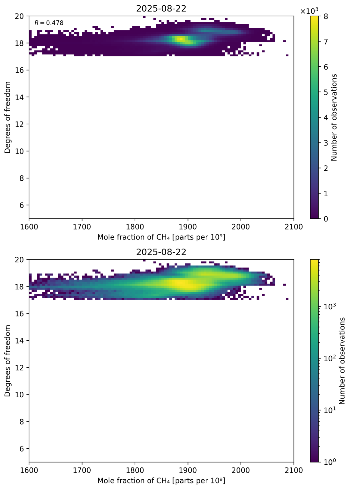
Figure 72: Scatter density plot of “Mole fraction of CH 4 ” against “Degrees of freedom” for 2025-08-21 to 2025-08-23.
