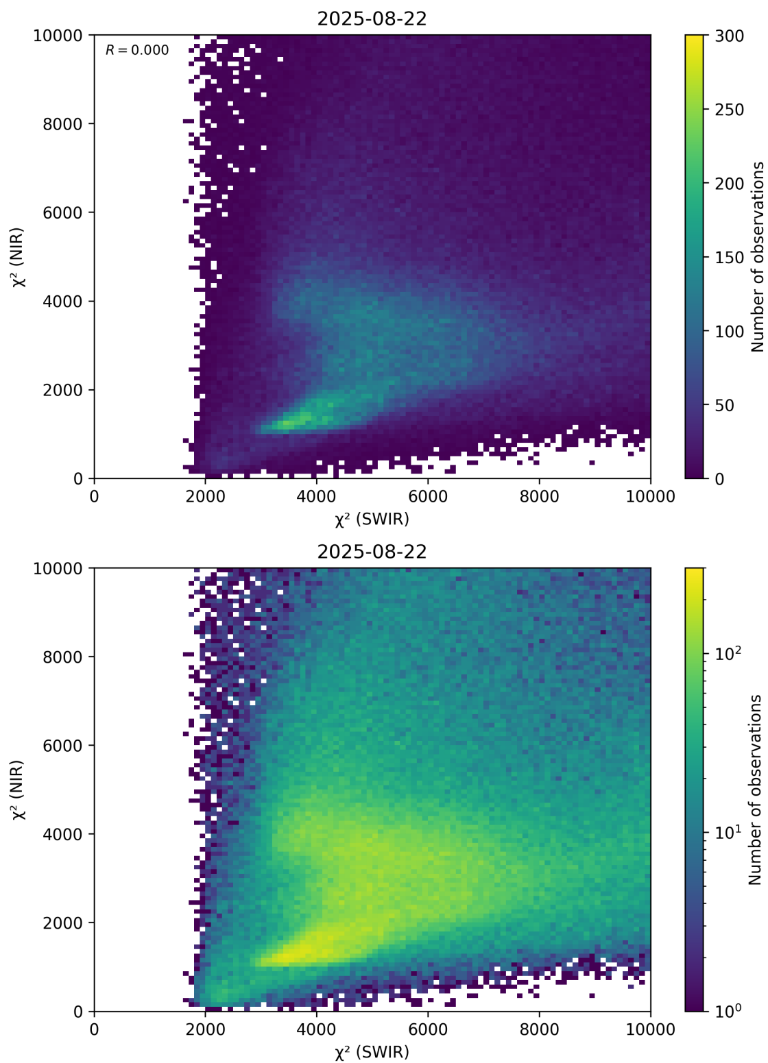
Figure 47: Scatter density plot of “ \chi^2 (SWIR)” against “ \chi^2 (NIR)” for 2025-08-21 to 2025-08-23.
