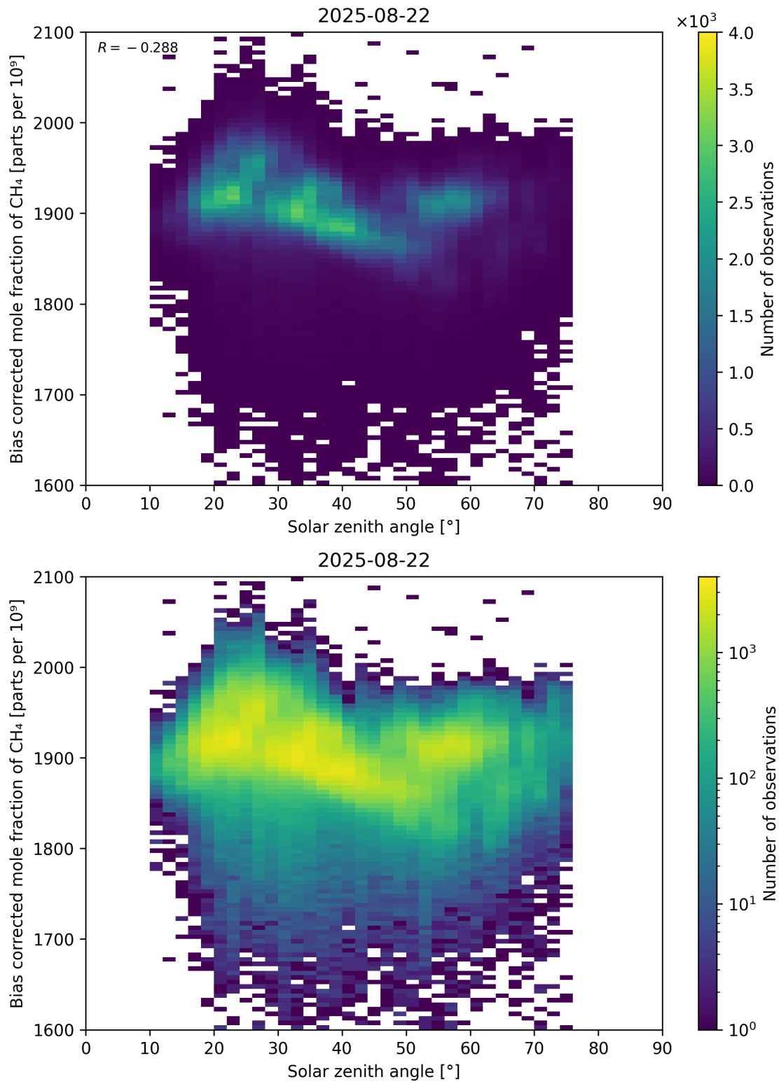
Figure 100: Scatter density plot of “Solar zenith angle” against “Bias corrected mole fraction of \text{CH}_4 ” for 2025-08-21 to 2025-08-23.
