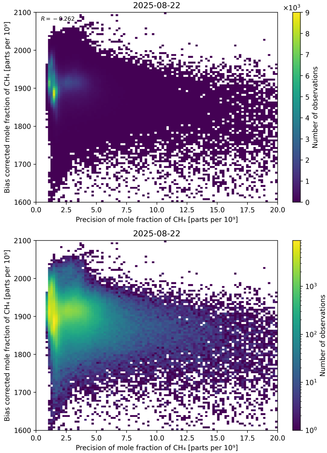
Figure 82: Scatter density plot of “Precision of mole fraction of CH 4 ” against “Bias corrected mole fraction of CH 4 ” for 2025-08-21 to 2025-08-23.
