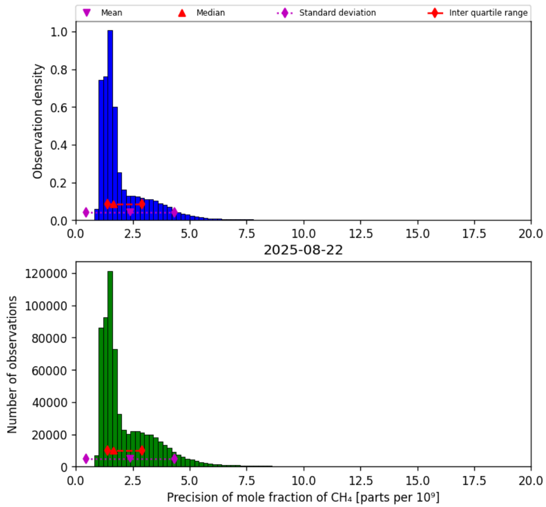
Figure 24: Histogram of “Precision of mole fraction of CH 4 ” for 2025-08-21 to 2025-08-23
