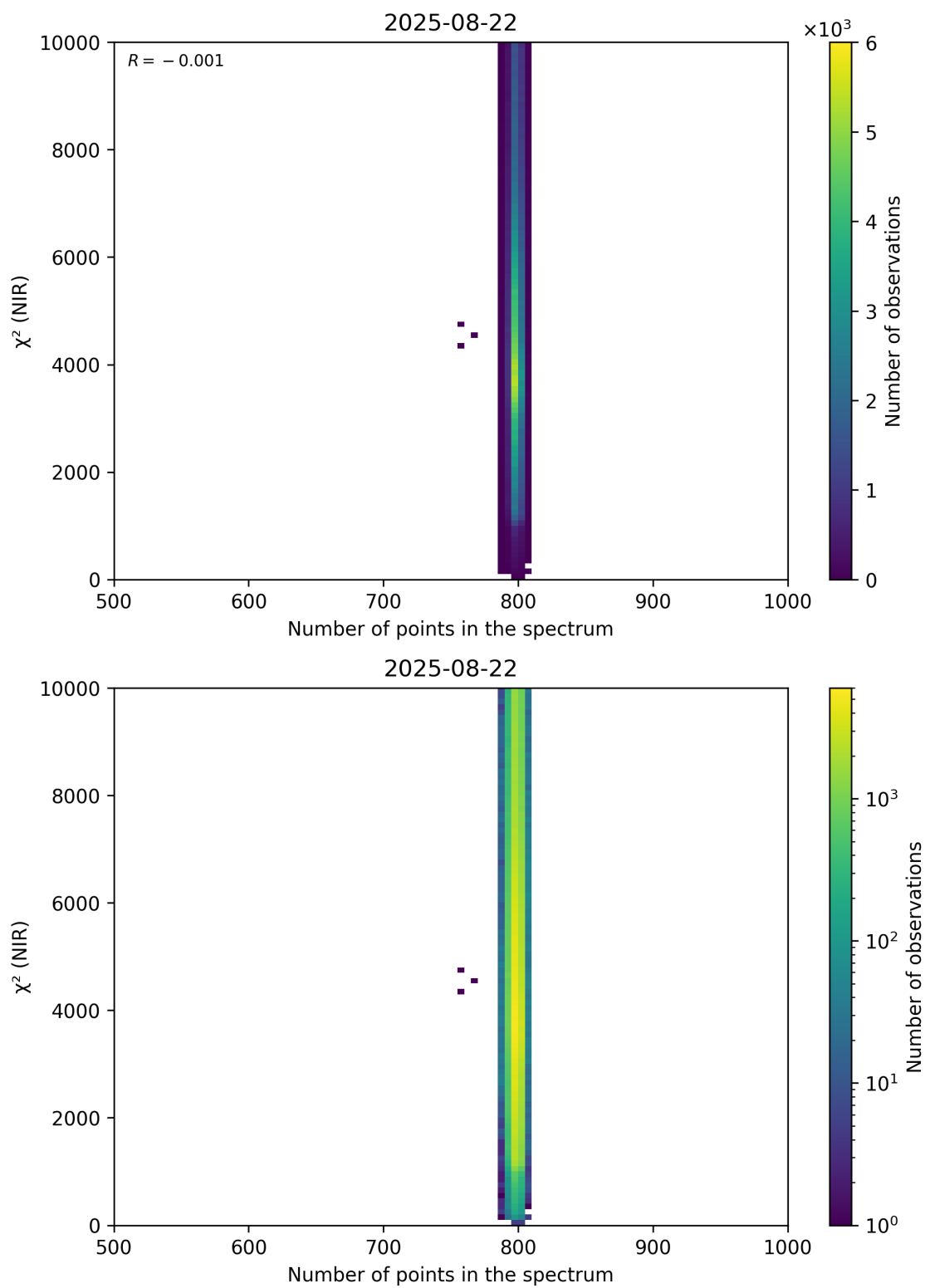
Figure 88: Scatter density plot of “Number of points in the spectrum” against “ \chi^2 (NIR)” for 2025-08-21 to 2025-08-23.
