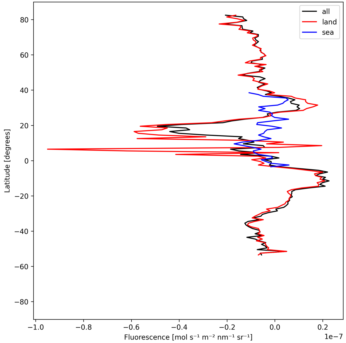
Figure 21: Zonal average of “Fluorescence” for 2025-08-21 to 2025-08-23.
