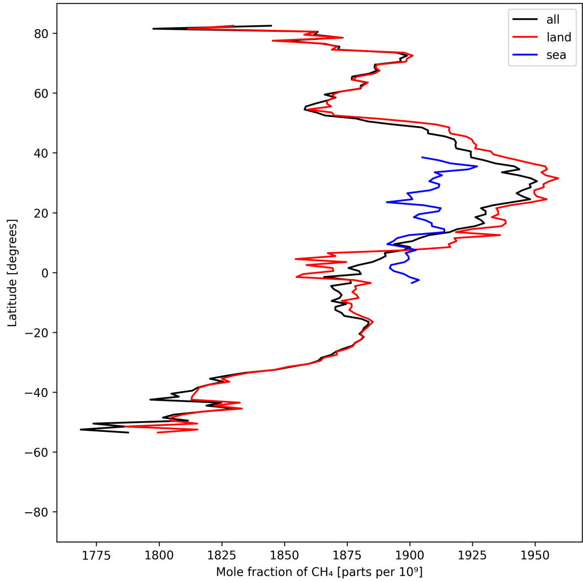
Figure 12: Zonal average of “Mole fraction of \text{CH}_4 ” for 2025-08-21 to 2025-08-23.
