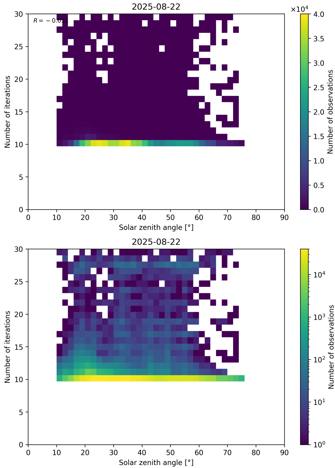
Figure 102: Scatter density plot of “Solar zenith angle” against “Number of iterations” for 2025-08-21 to 2025-08-23.
