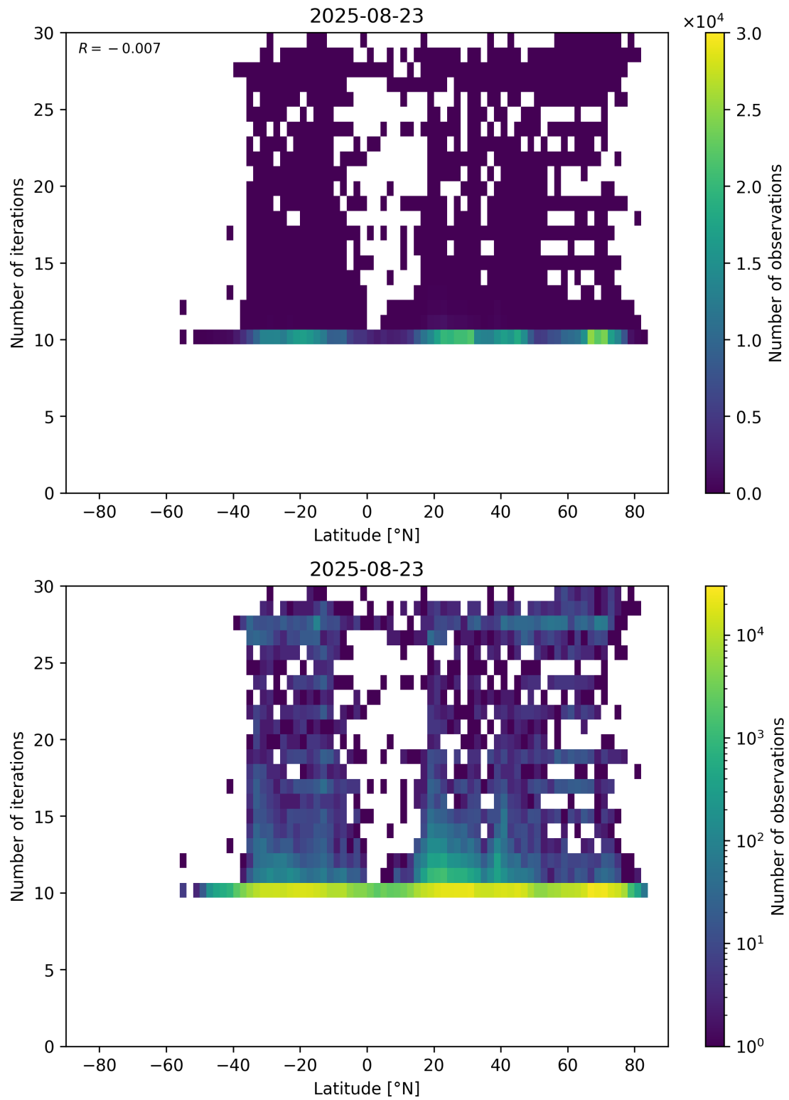
Figure 60: Scatter density plot of “Latitude” against “Number of iterations” for 2025-08-22 to 2025-08-24.
