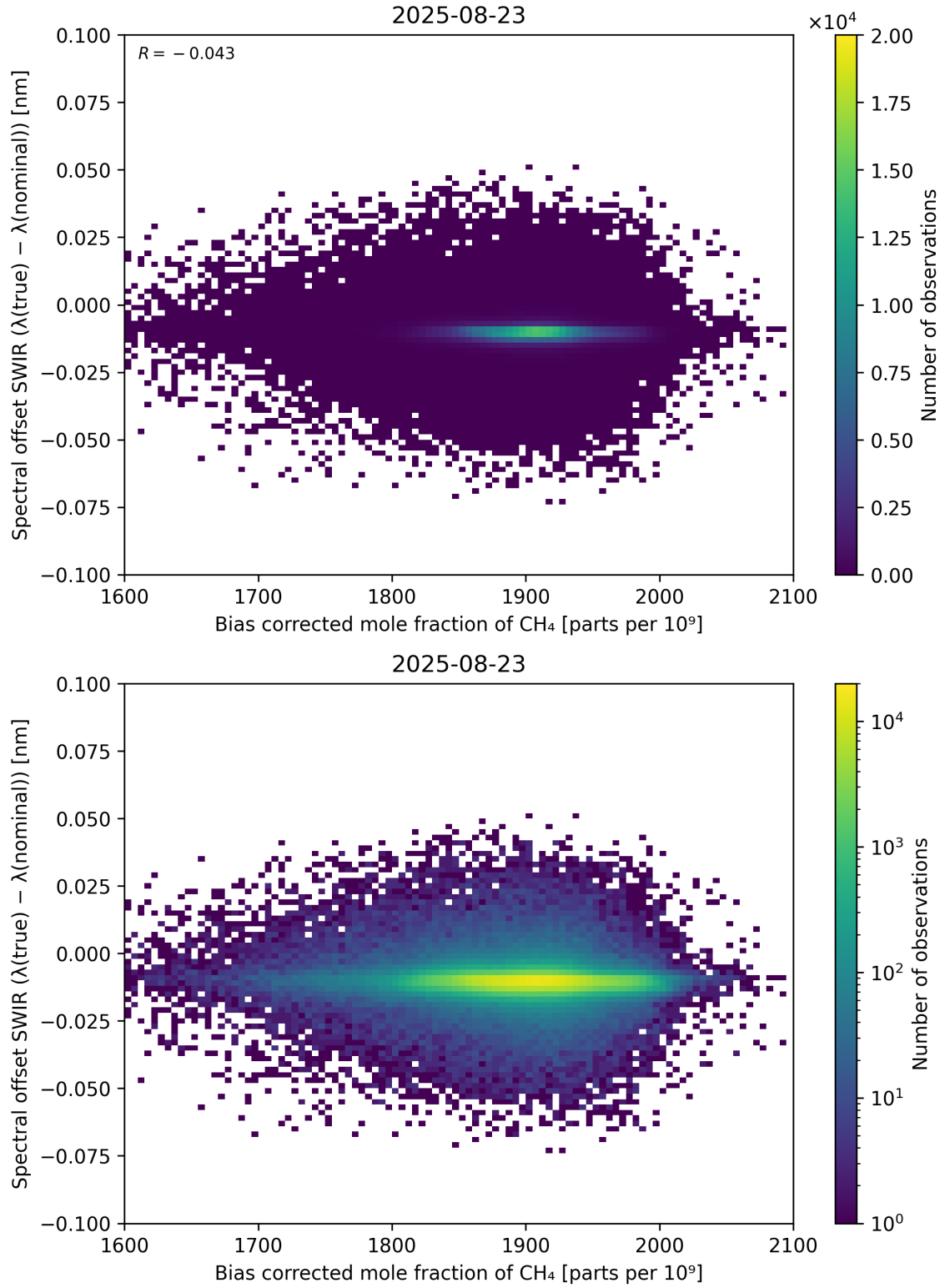
Figure 69: Scatter density plot of “Bias corrected mole fraction of \text{CH}_4 ” against “Spectral offset SWIR ( \lambda_{\text{true}} - \lambda_{\text{nominal}} )” for 2025-08-22 to 2025-08-24.
