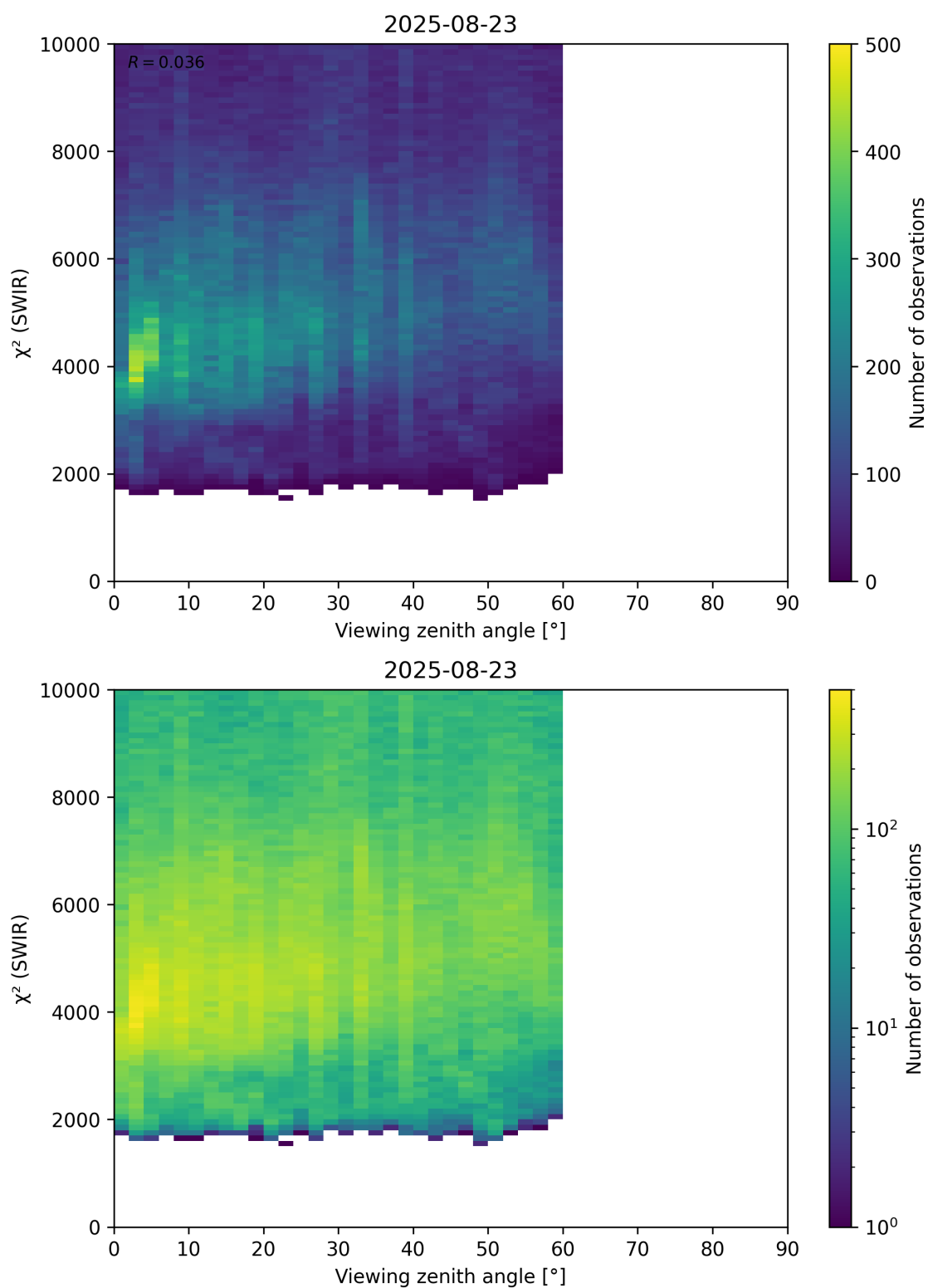
Figure 106: Scatter density plot of “Viewing zenith angle” against “ \chi^2 (SWIR)” for 2025-08-22 to 2025-08-24.
