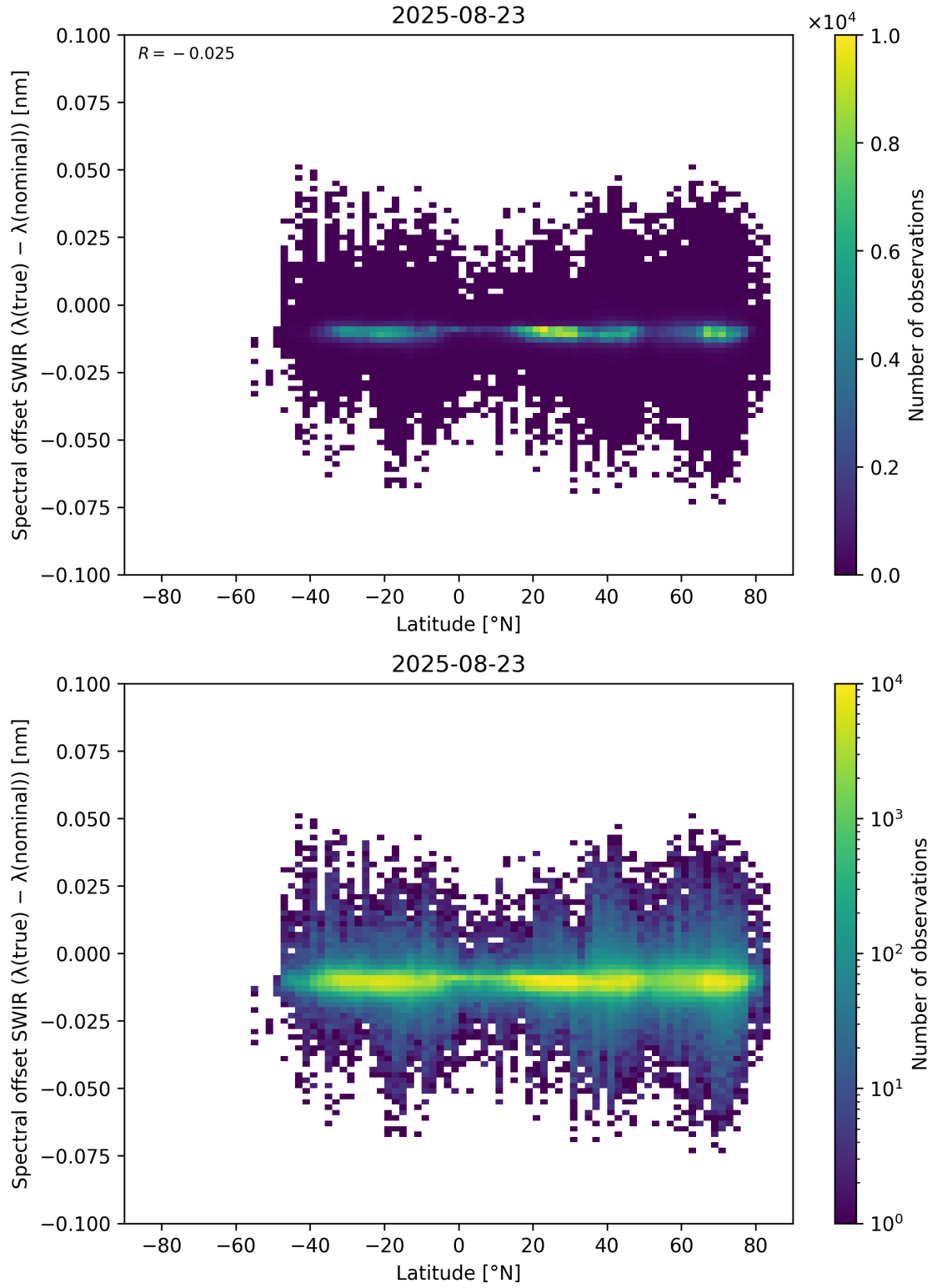
Figure 62: Scatter density plot of “Latitude” against “Spectral offset SWIR ( \lambda_{\text{true}} - \lambda_{\text{nominal}} )” for 2025-08-22 to 2025-08-24.
