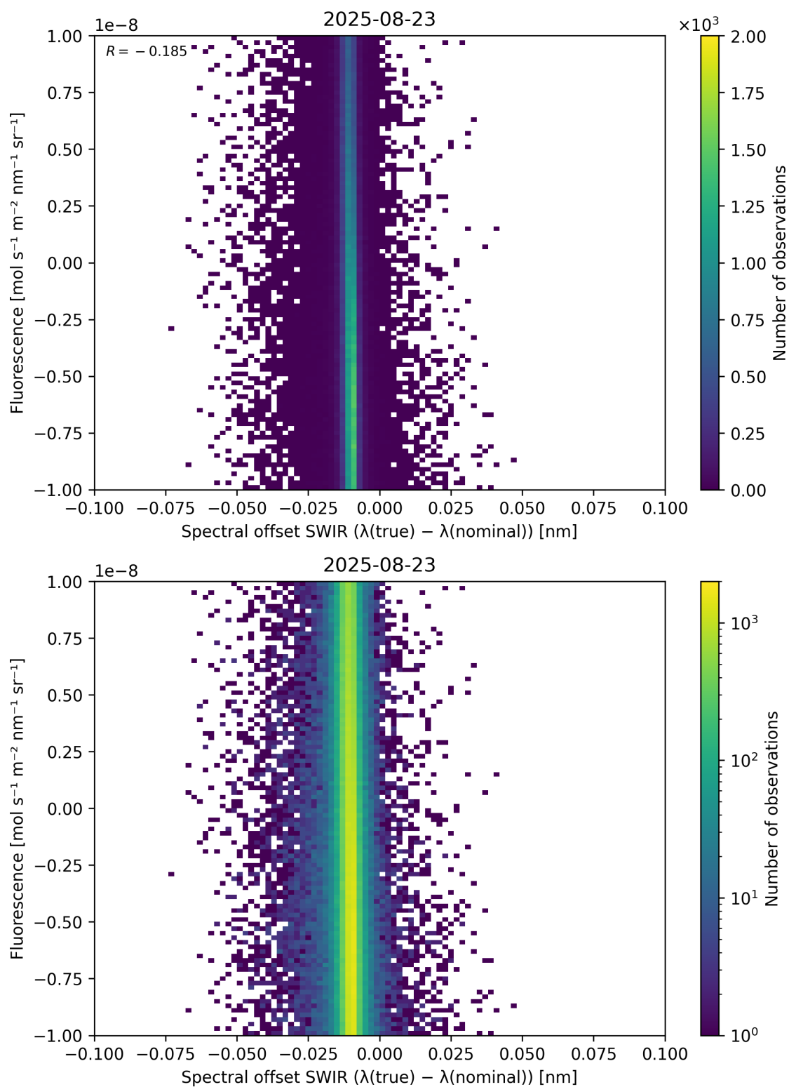
Figure 120: Scatter density plot of “Spectral offset SWIR ( \lambda_{\text{true}} - \lambda_{\text{nominal}} )” against “Fluorescence” for 2025-08-22 to 2025-08-24.
