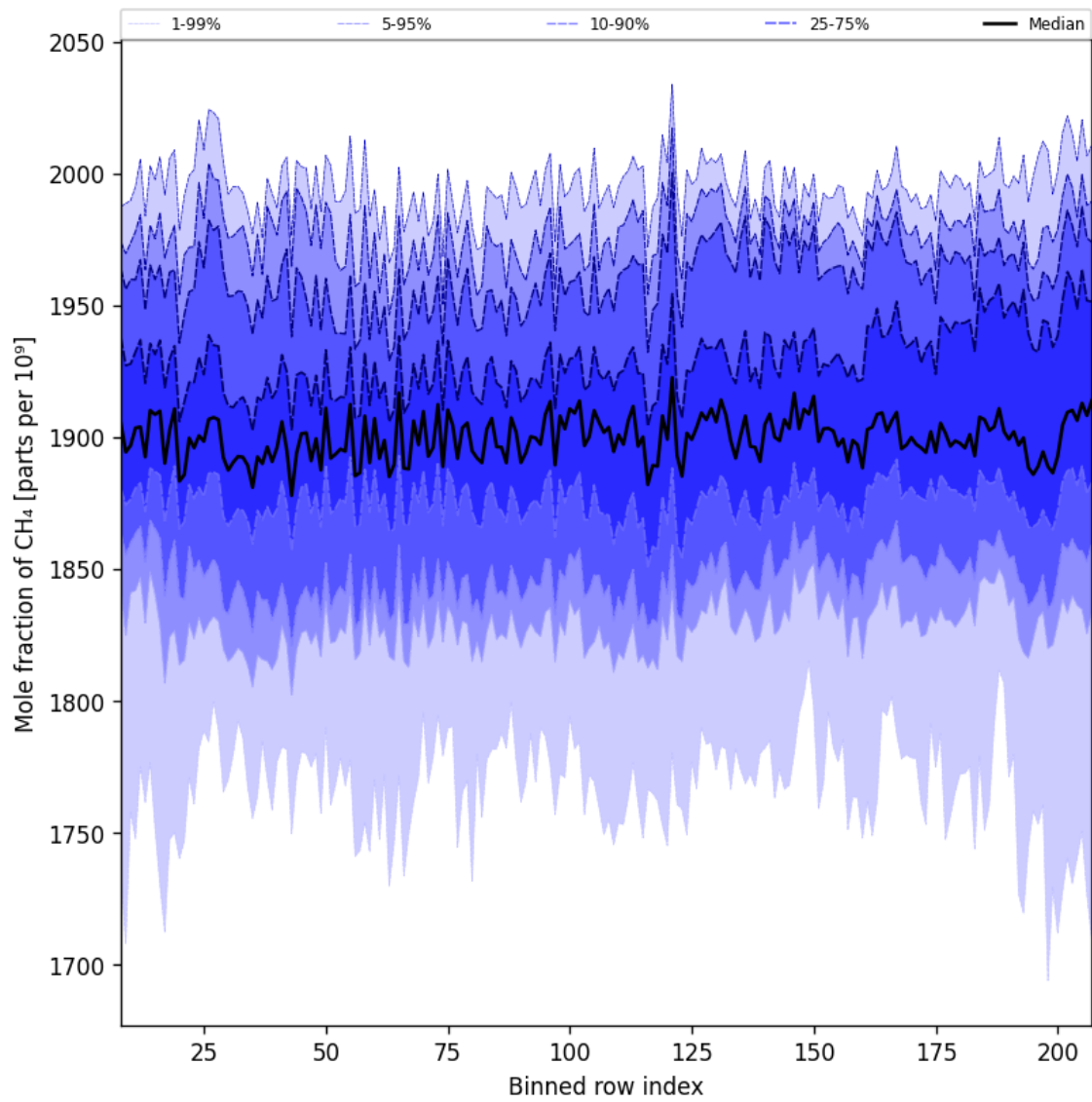
Figure 34: Along track statistics of “Mole fraction of CH 4 ” for 2025-08-22 to 2025-08-24
