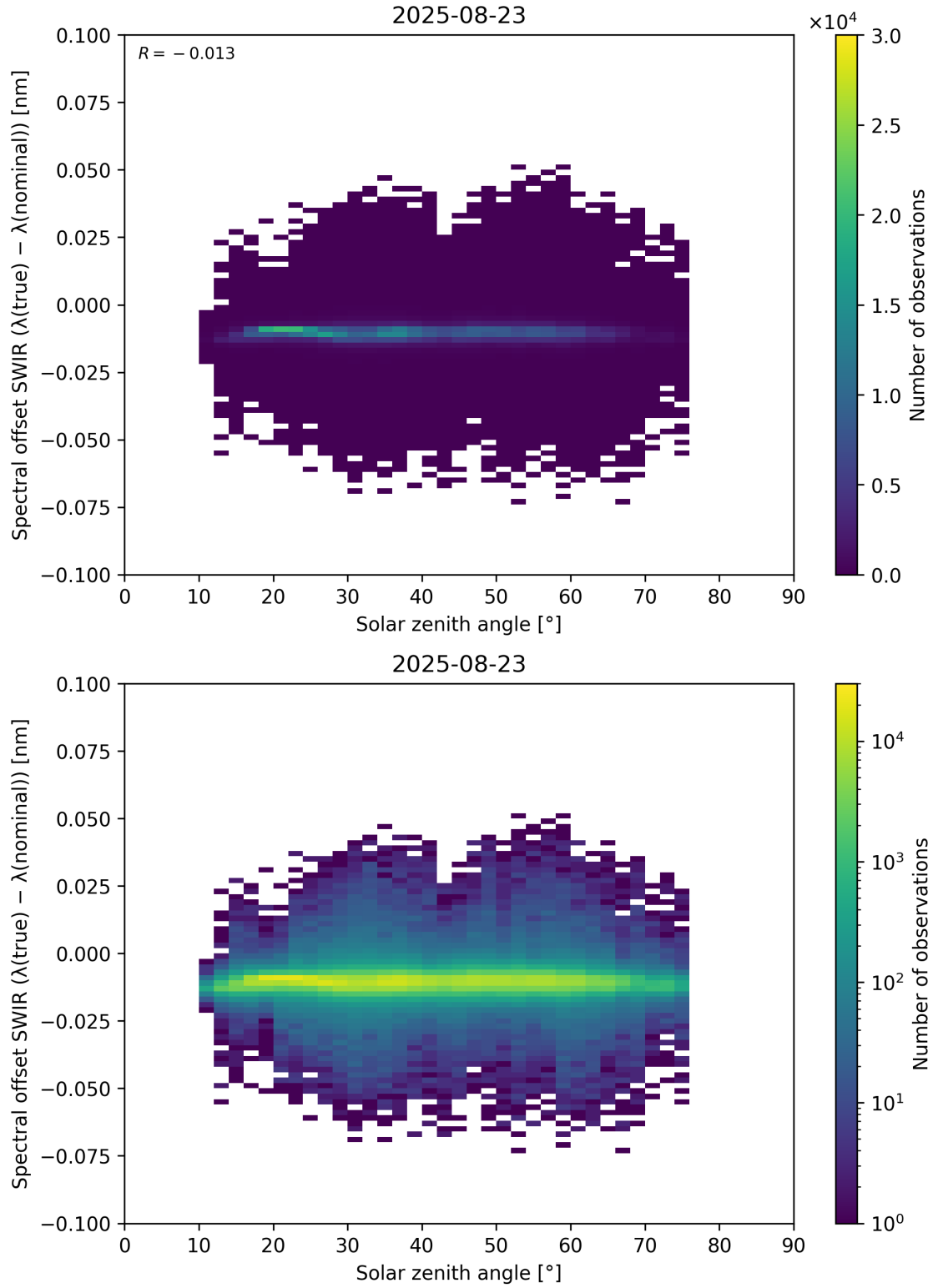
Figure 104: Scatter density plot of “Solar zenith angle” against “Spectral offset SWIR ( \lambda_{\text{true}} - \lambda_{\text{nominal}} )” for 2025-08-22 to 2025-08-24.
