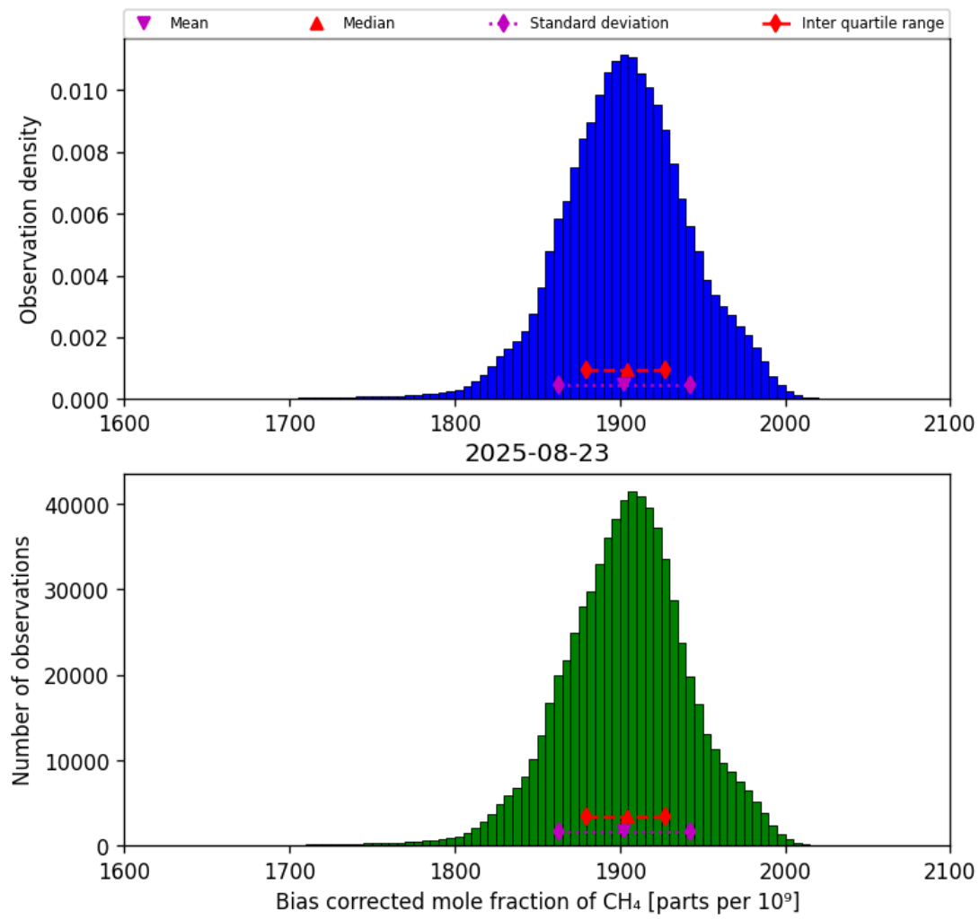
Figure 25: Histogram of “Bias corrected mole fraction of CH 4 ” for 2025-08-22 to 2025-08-24
