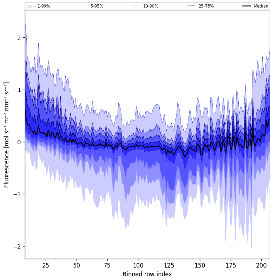
Figure 43: Along track statistics of “Fluorescence” for 2025-08-22 to 2025-08-24
