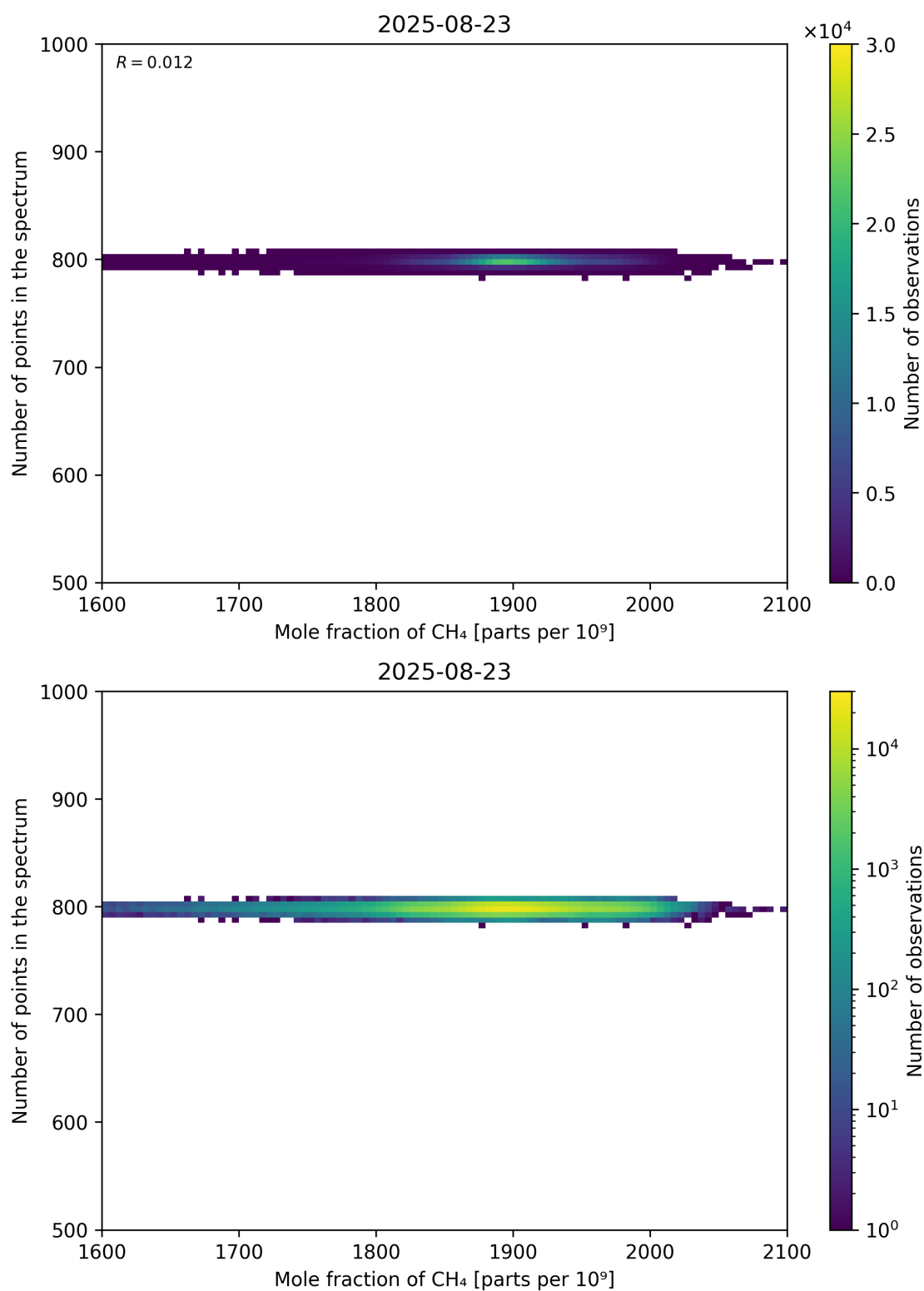
Figure 77: Scatter density plot of “Mole fraction of CH 4 ” against “Number of points in the spectrum” for 2025-08-22 to 2025-08-24.
