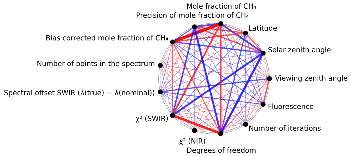
Figure 1: Map of correlation graph for 2025-08-22 to 2025-08-24.
