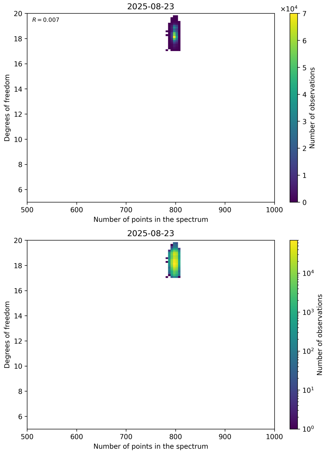
Figure 90: Scatter density plot of “Number of points in the spectrum” against “Degrees of freedom” for 2025-08-22 to 2025-08-24.
