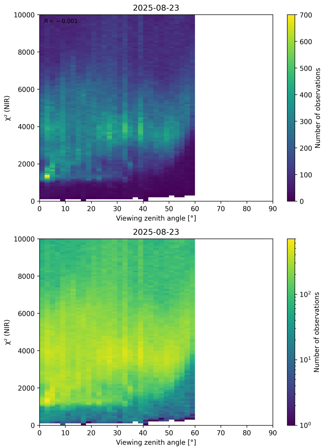
Figure 105: Scatter density plot of “Viewing zenith angle” against “ \chi^2 (NIR)” for 2025-08-22 to 2025-08-24.
