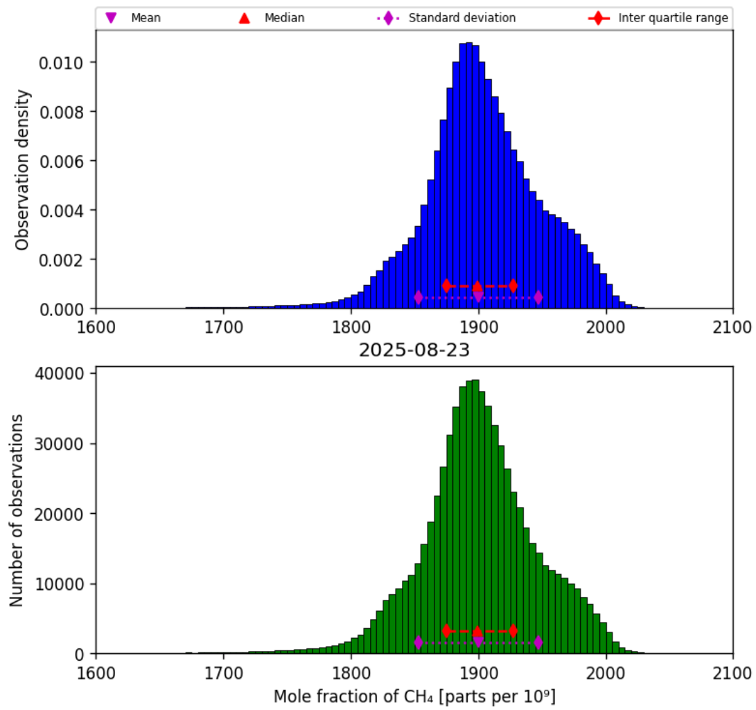
Figure 23: Histogram of “Mole fraction of CH 4 ” for 2025-08-22 to 2025-08-24
