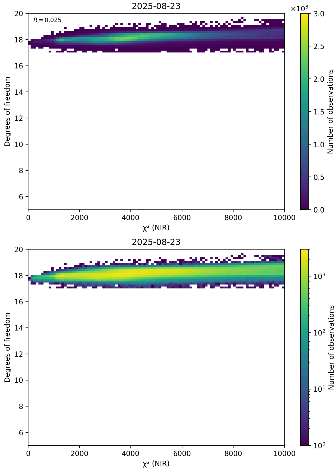
Figure 44: Scatter density plot of “ \chi^2 (NIR)” against “Degrees of freedom” for 2025-08-22 to 2025-08-24.
