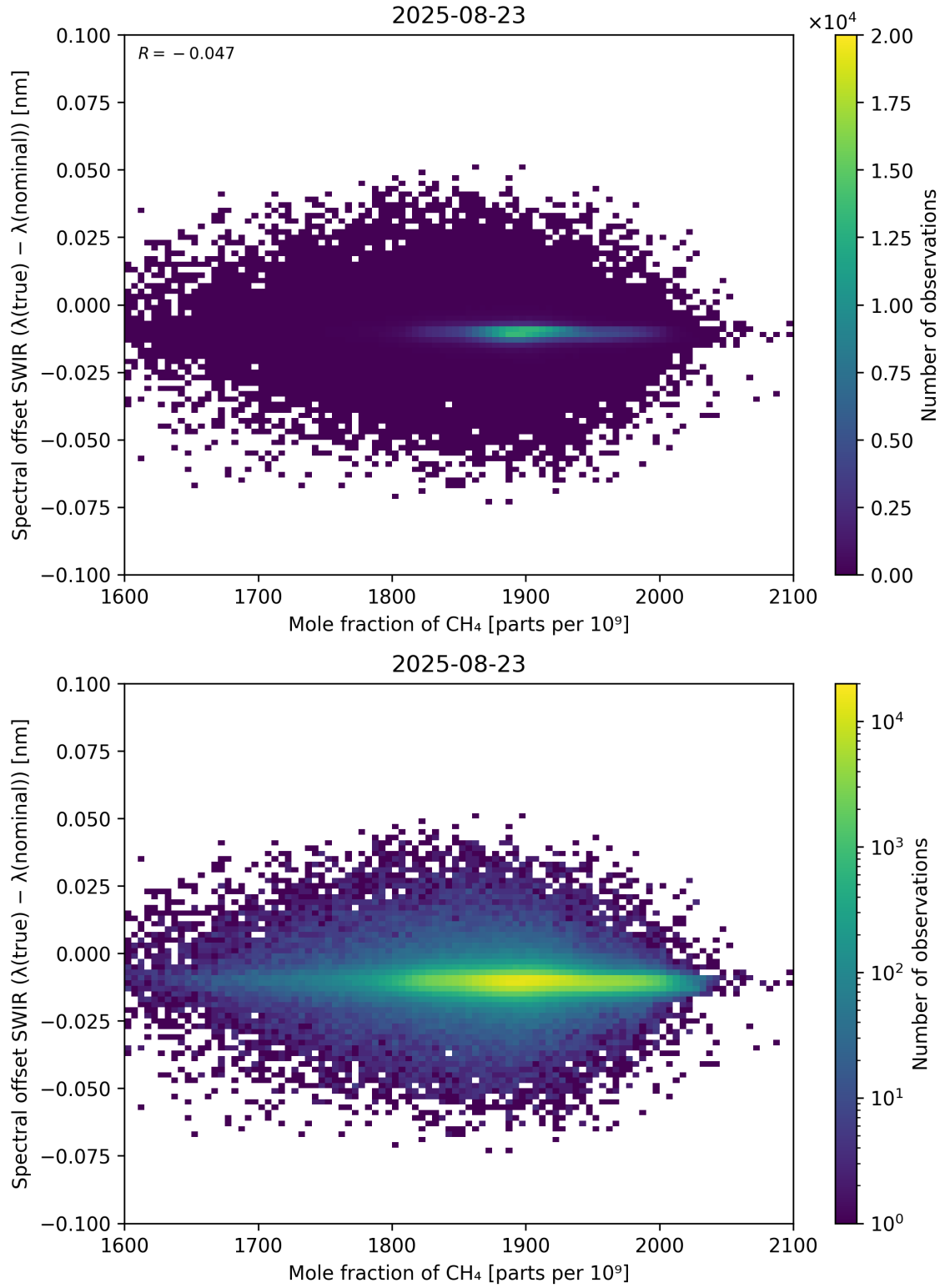
Figure 86: Scatter density plot of “Mole fraction of CH 4 ” against “Spectral offset SWIR ( \lambda_{\text{true}} - \lambda_{\text{nominal}} )” for 2025-08-22 to 2025-08-24.
