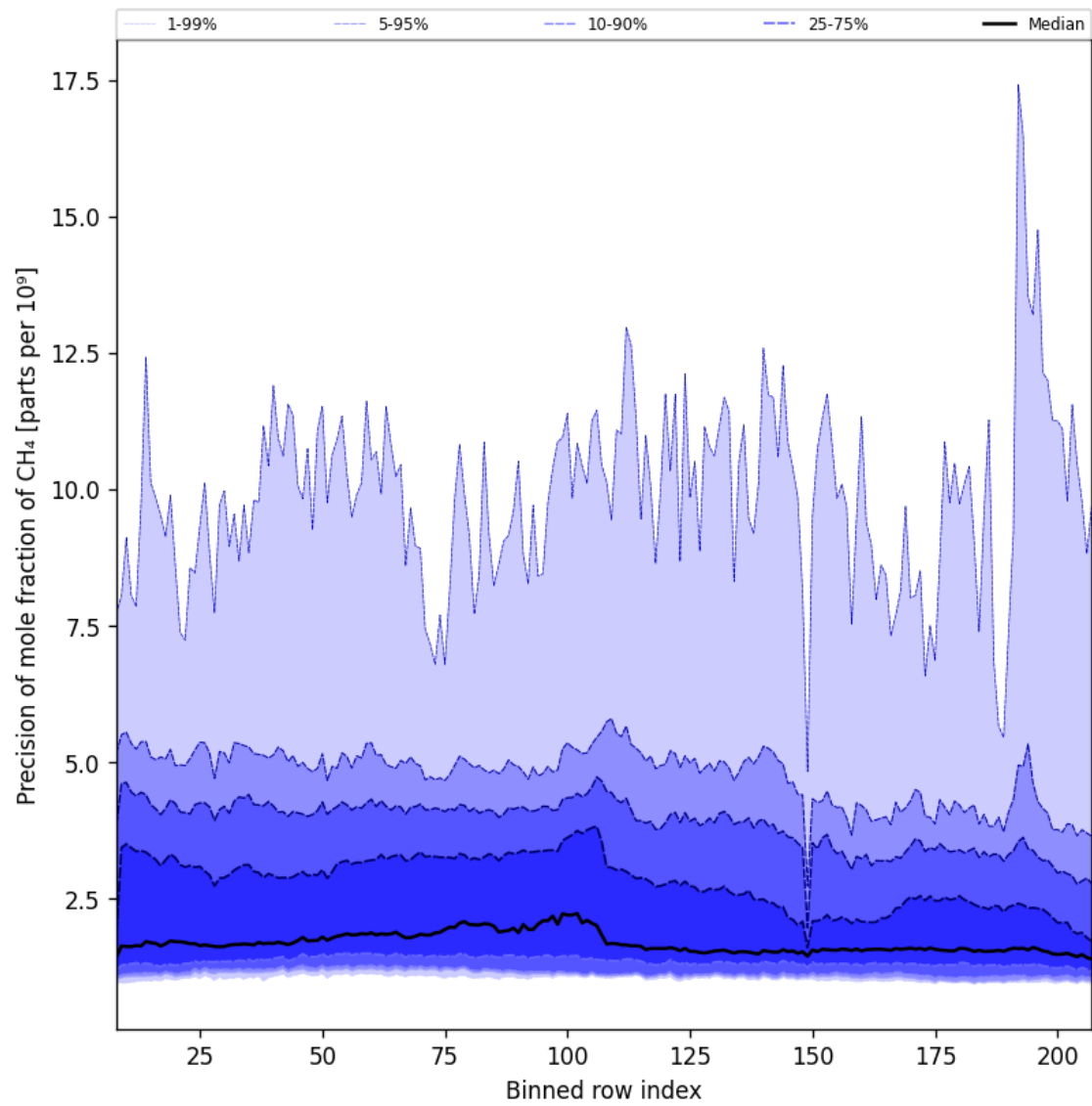
Figure 35: Along track statistics of “Precision of mole fraction of CH 4 ” for 2025-08-22 to 2025-08-24
