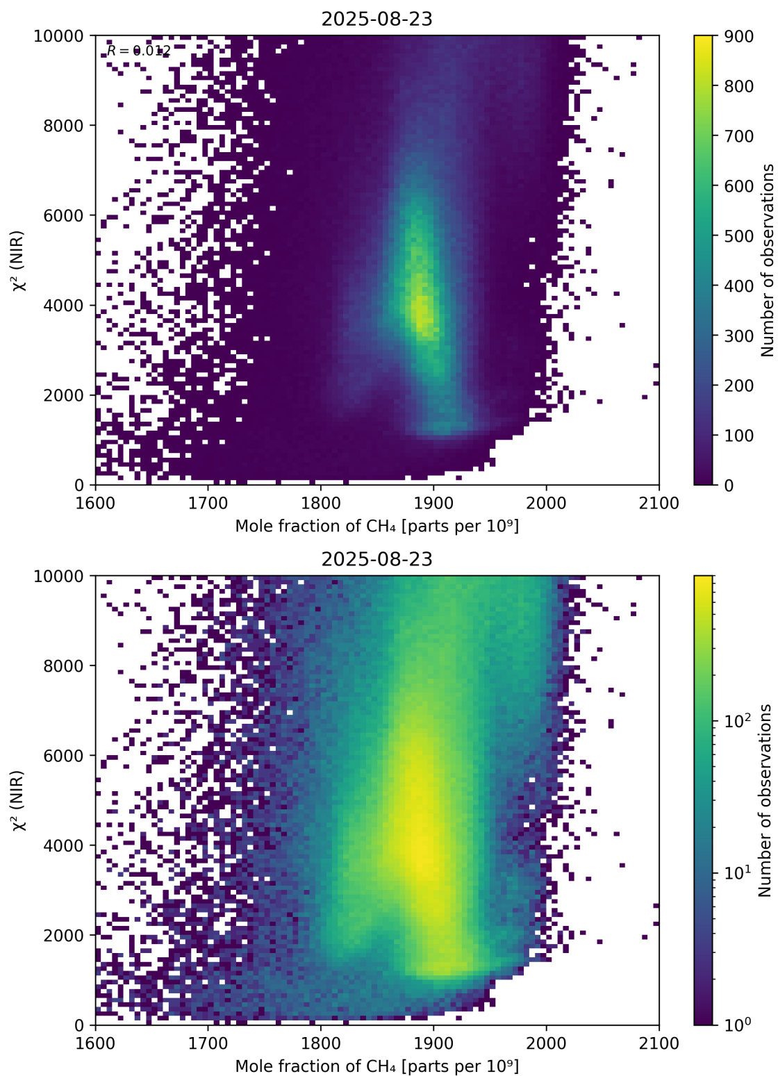
Figure 70: Scatter density plot of “Mole fraction of \text{CH}_4 ” against “ \chi^2 (NIR)” for 2025-08-22 to 2025-08-24.
