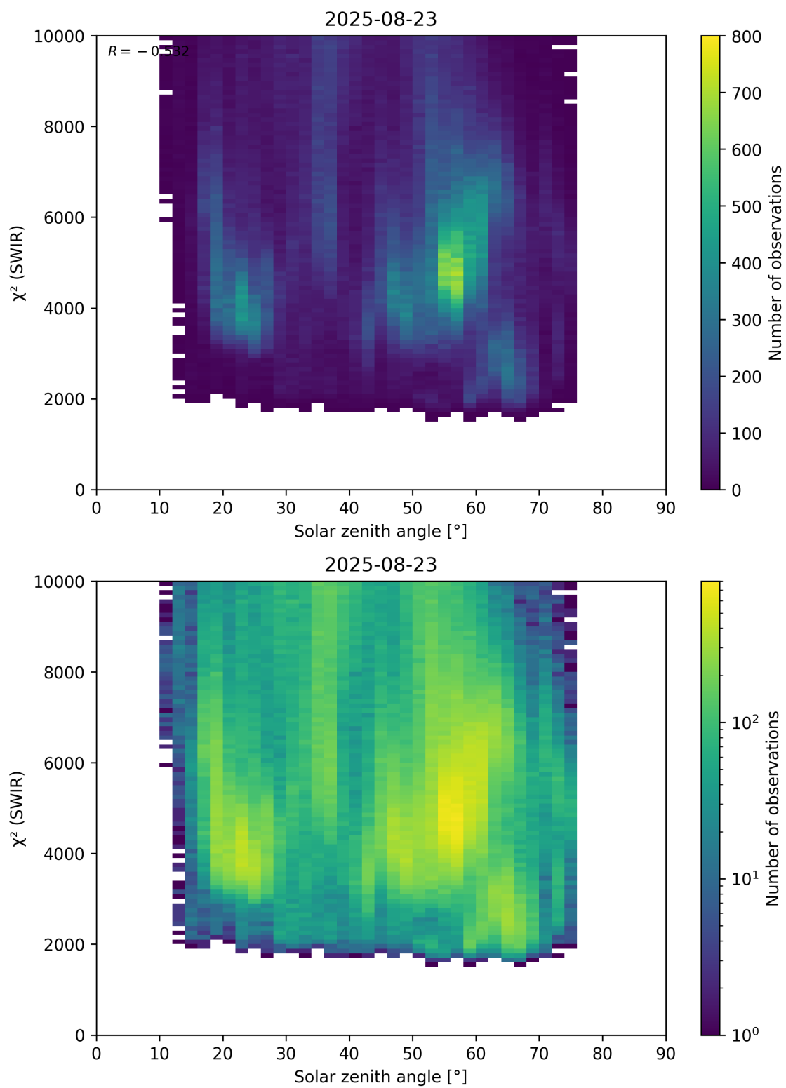
Figure 95: Scatter density plot of “Solar zenith angle” against “ \chi^2 (SWIR)” for 2025-08-22 to 2025-08-24.
