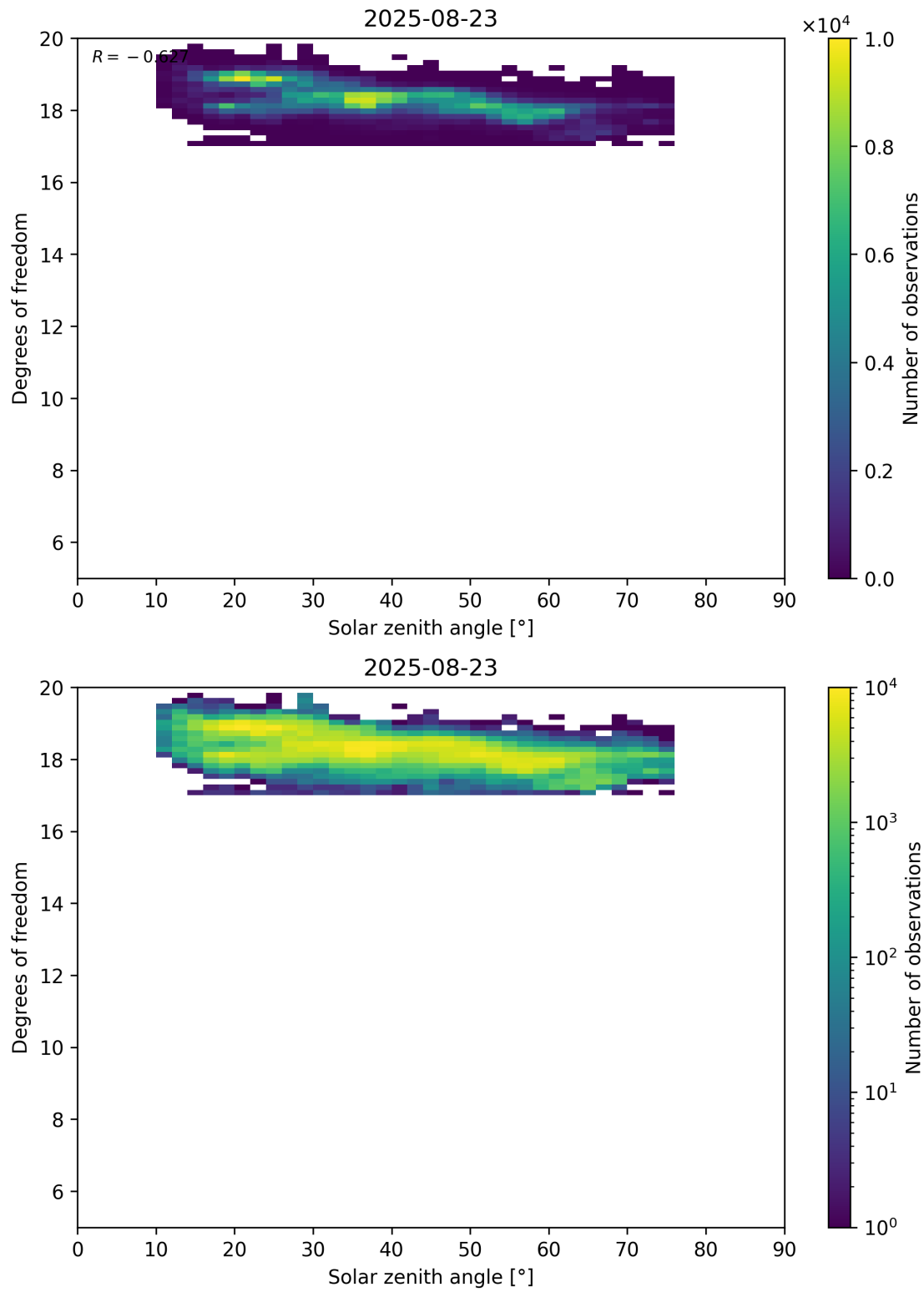
Figure 96: Scatter density plot of “Solar zenith angle” against “Degrees of freedom” for 2025-08-22 to 2025-08-24.
