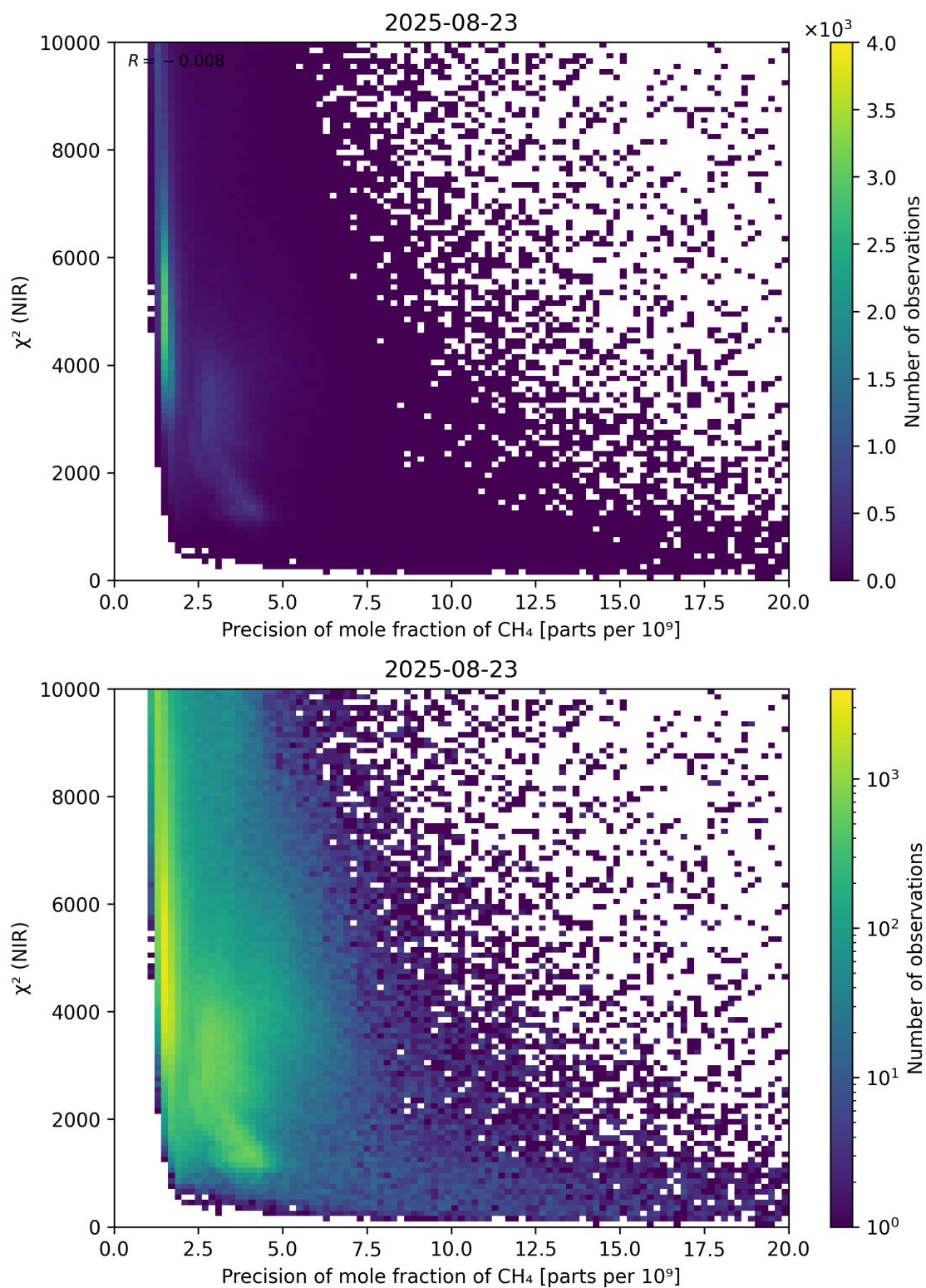
Figure 78: Scatter density plot of “Precision of mole fraction of CH 4 ” against “ \chi^2 (NIR)” for 2025-08-22 to 2025-08-24.
