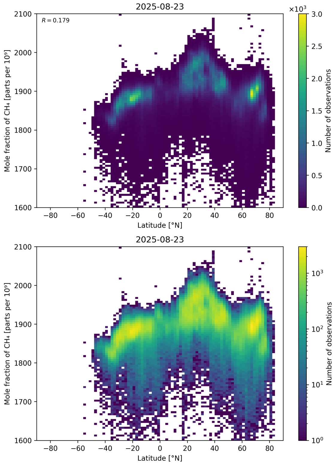
Figure 57: Scatter density plot of “Latitude” against “Mole fraction of CH 4 ” for 2025-08-22 to 2025-08-24.
