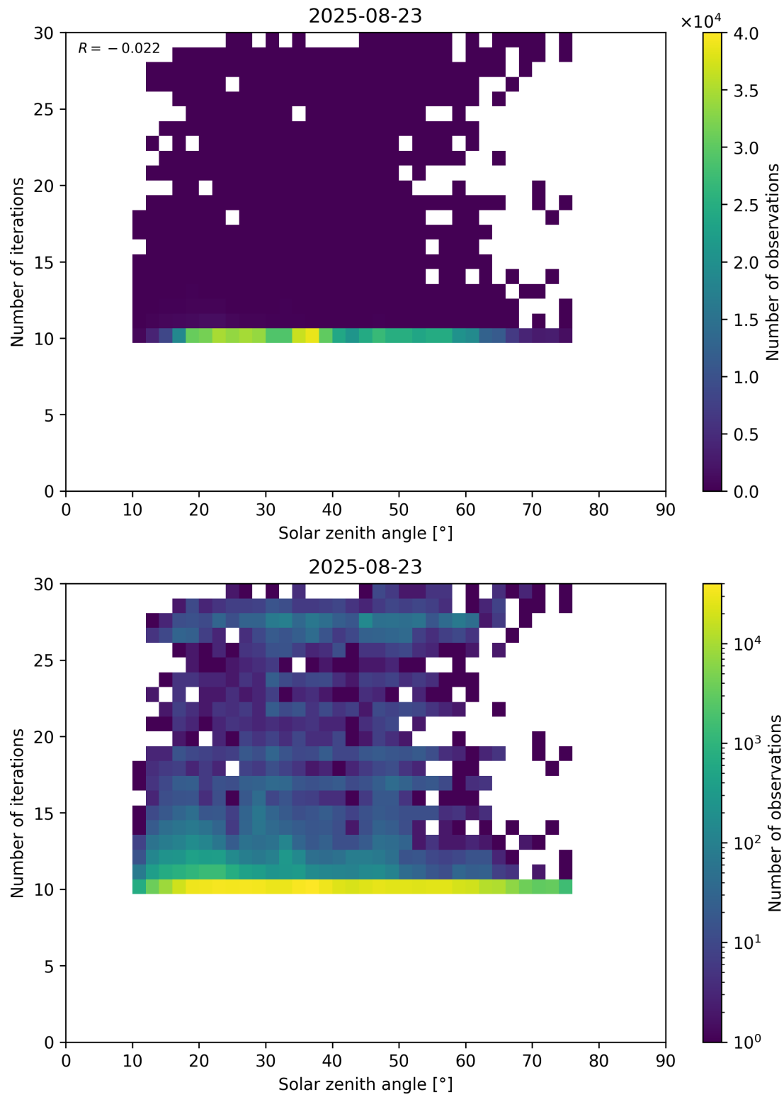
Figure 102: Scatter density plot of “Solar zenith angle” against “Number of iterations” for 2025-08-22 to 2025-08-24.
