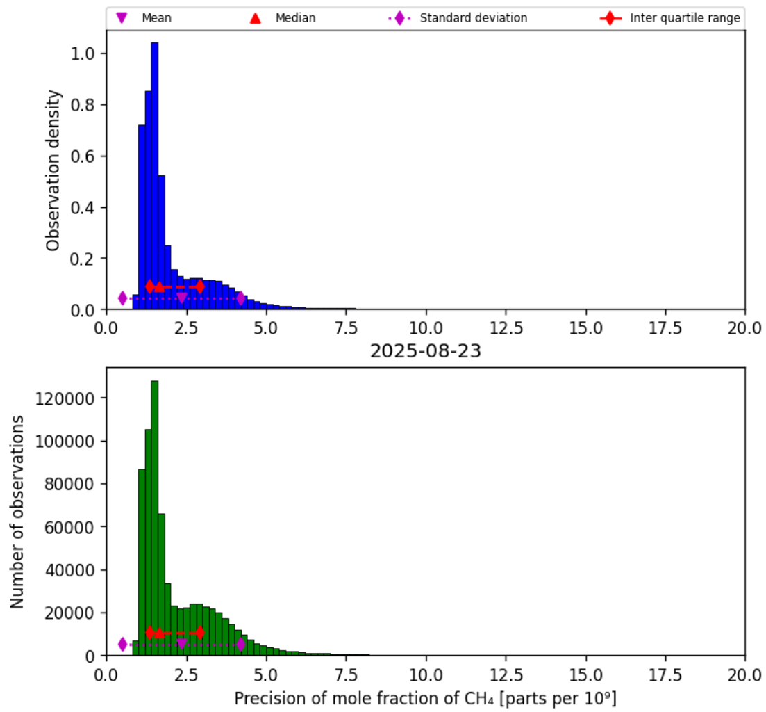
Figure 24: Histogram of “Precision of mole fraction of CH 4 ” for 2025-08-22 to 2025-08-24
