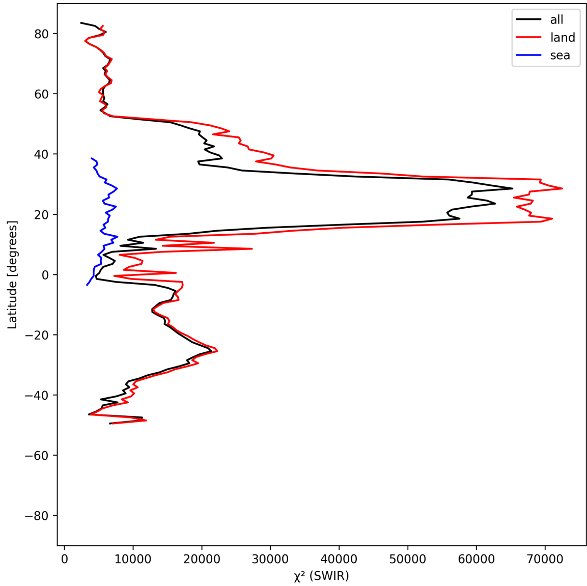
Figure 17: Zonal average of “ \chi^2 (SWIR)” for 2025-08-22 to 2025-08-24.
