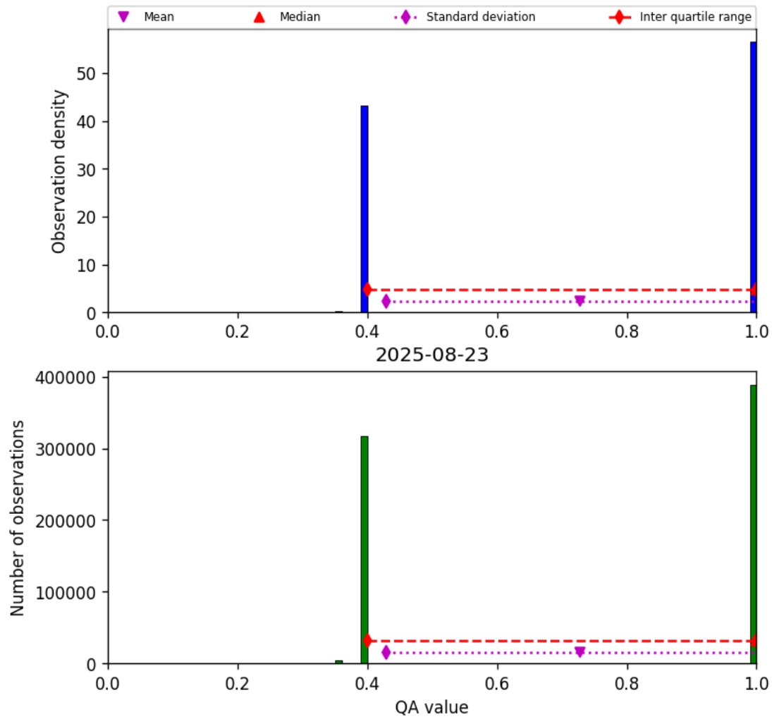
Figure 22: Histogram of “QA value” for 2025-08-22 to 2025-08-24
