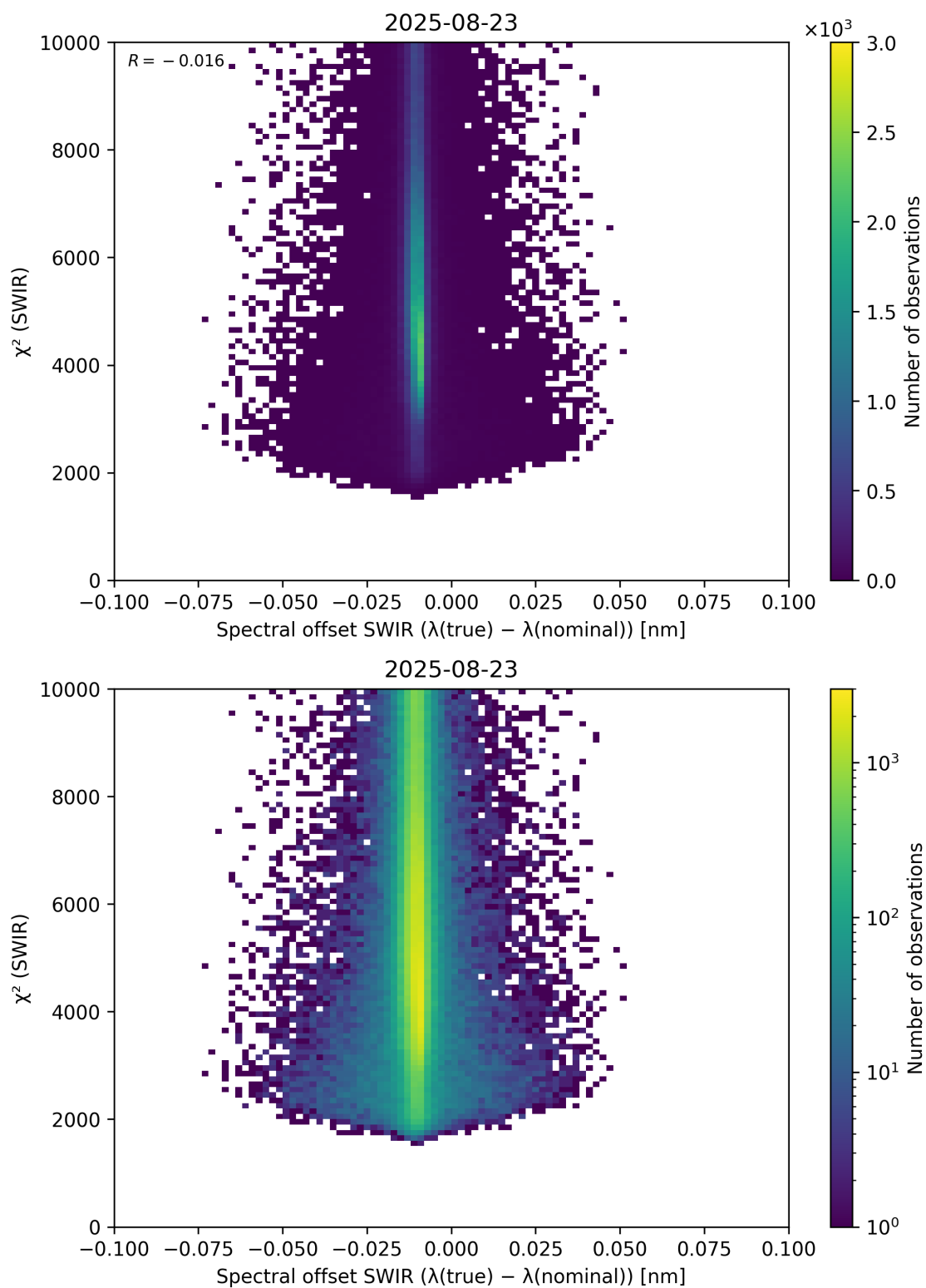
Figure 118: Scatter density plot of “Spectral offset SWIR ( \lambda_{\text{true}} - \lambda_{\text{nominal}} )” against “ \chi^2 (SWIR)” for 2025-08-22 to 2025-08-24.
