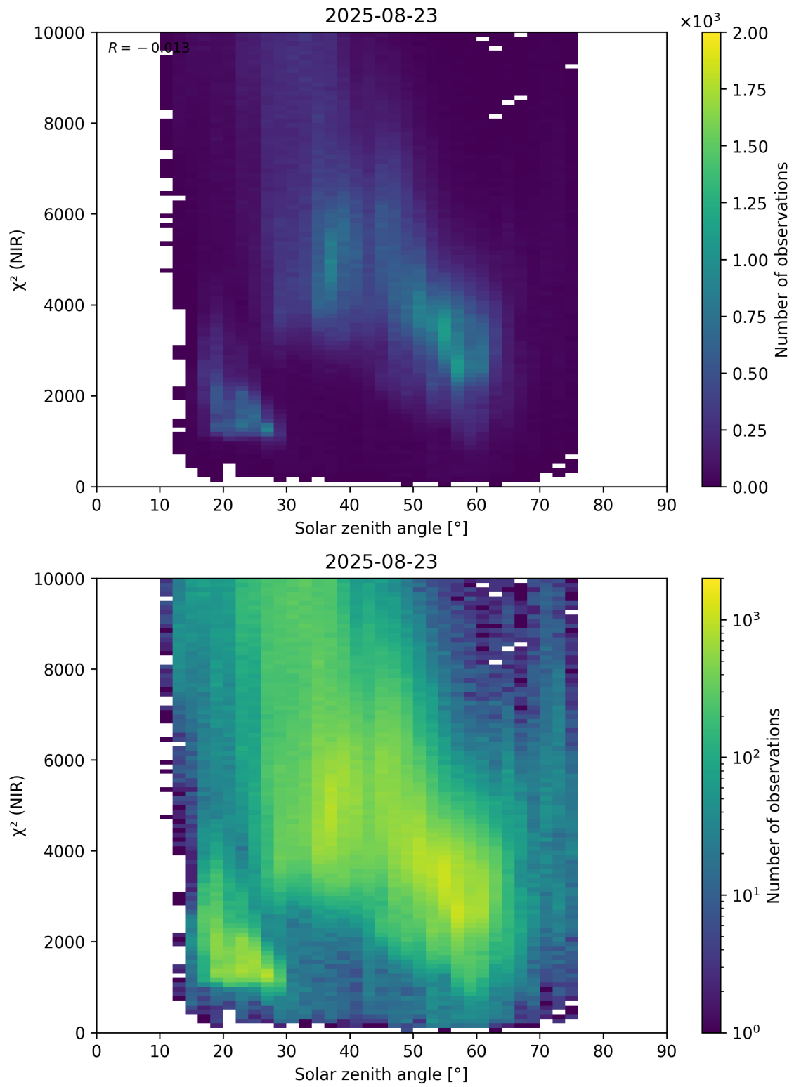
Figure 94: Scatter density plot of “Solar zenith angle” against “ \chi^2 (NIR)” for 2025-08-22 to 2025-08-24.
