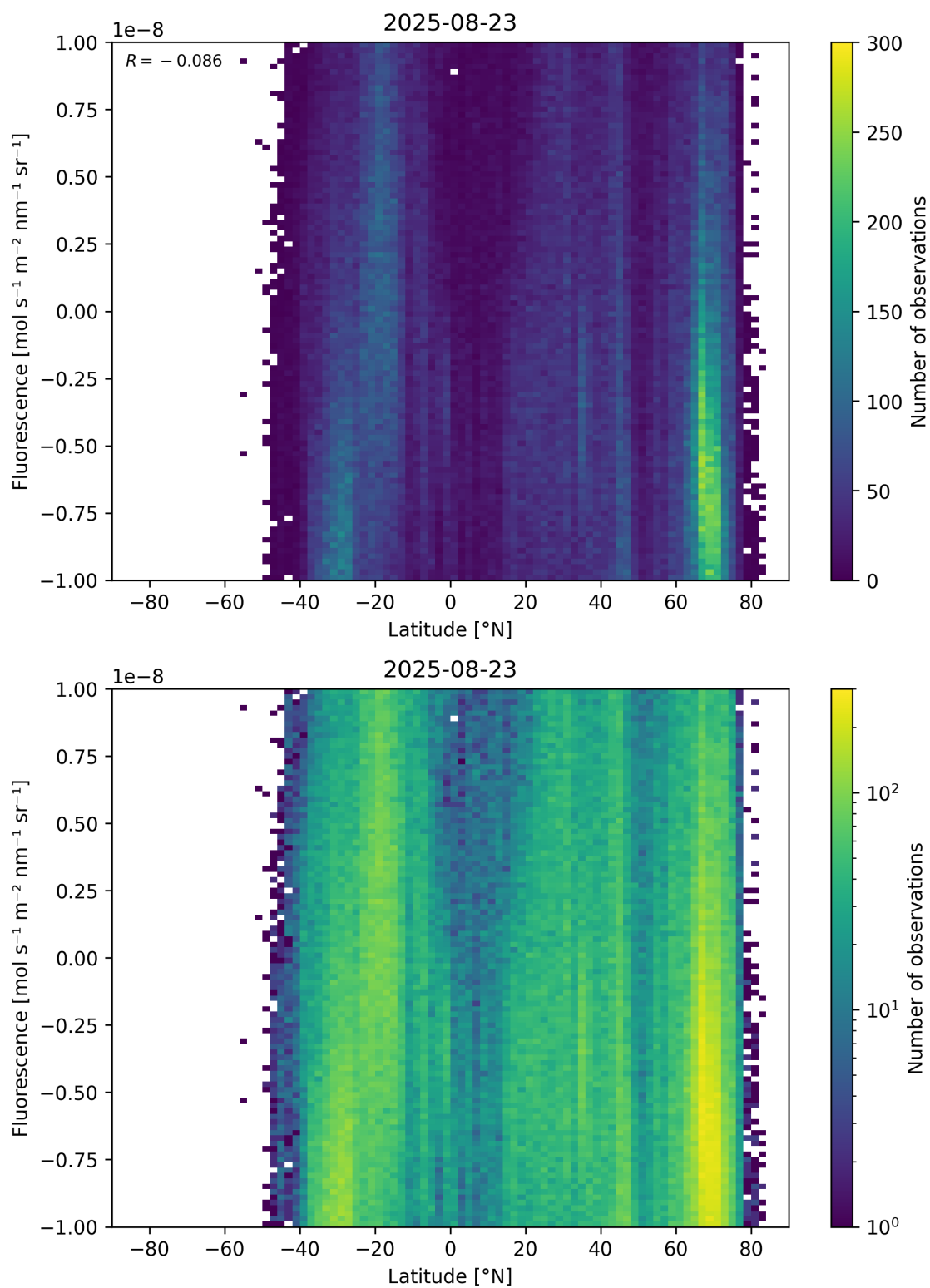
Figure 56: Scatter density plot of “Latitude” against “Fluorescence” for 2025-08-22 to 2025-08-24.
