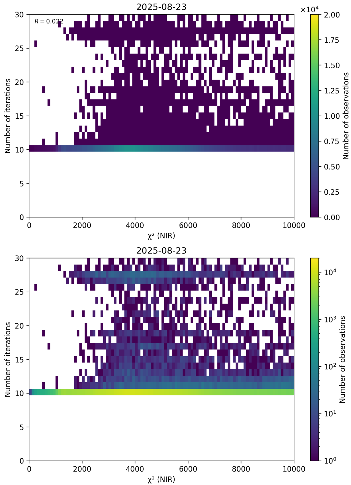
Figure 46: Scatter density plot of “ \chi^2 (NIR)” against “Number of iterations” for 2025-08-22 to 2025-08-24.
