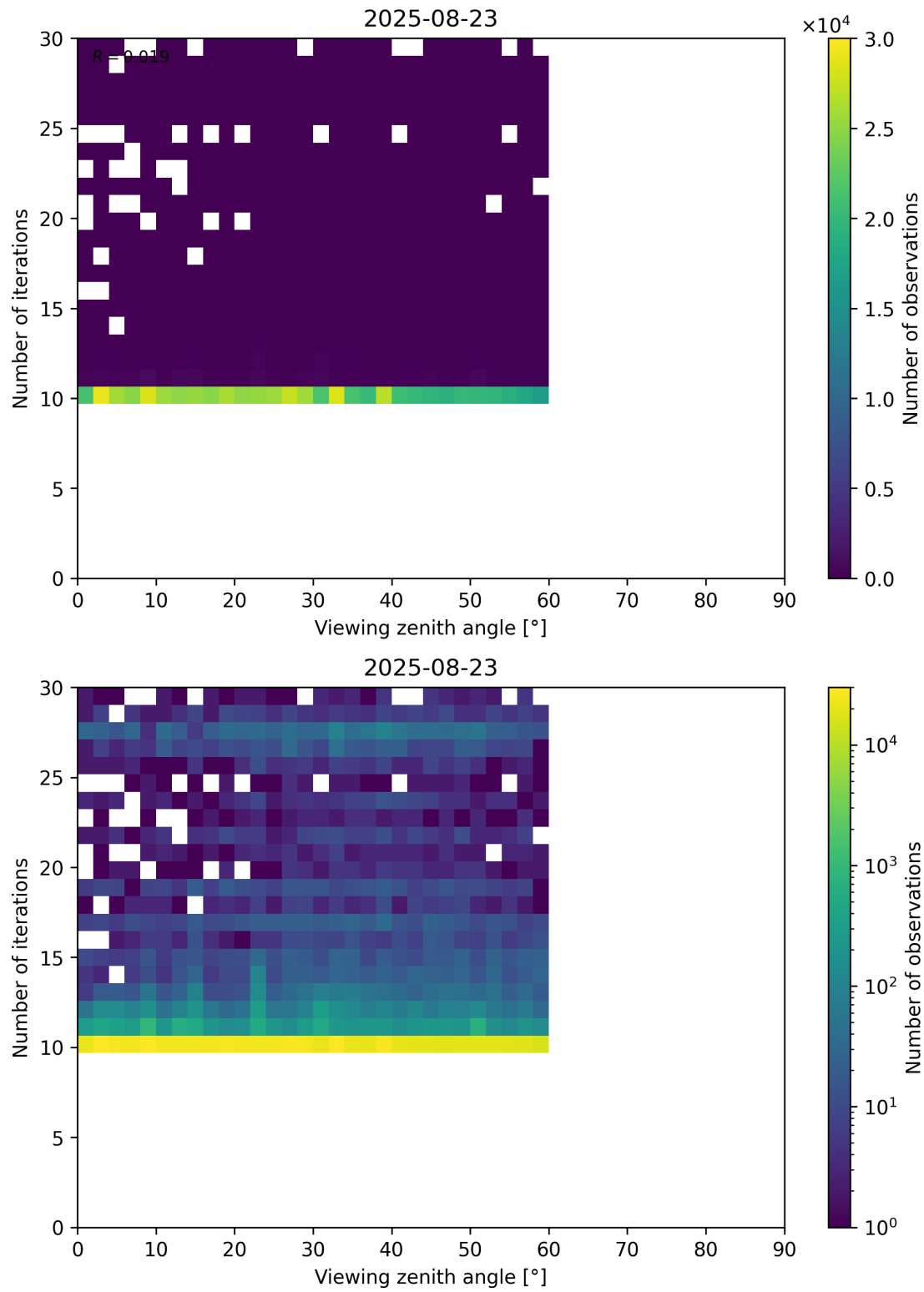
Figure 113: Scatter density plot of “Viewing zenith angle” against “Number of iterations” for 2025-08-22 to 2025-08-24.
