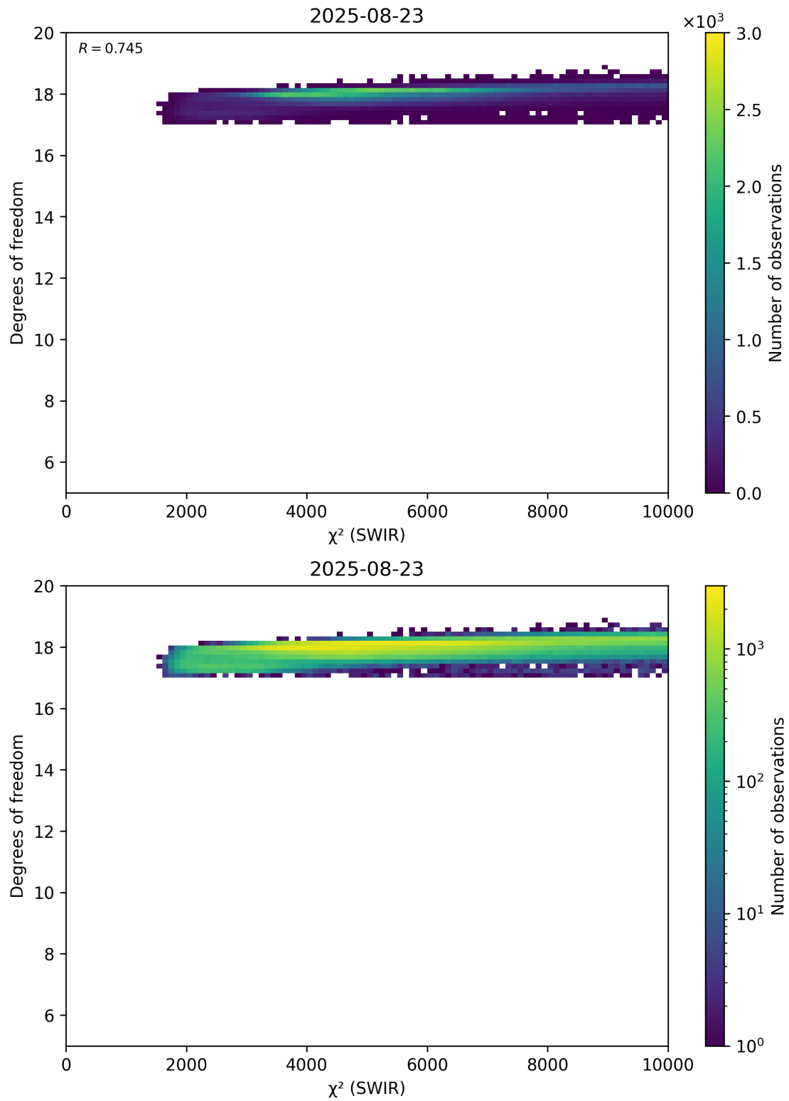
Figure 48: Scatter density plot of “ \chi^2 (SWIR)” against “Degrees of freedom” for 2025-08-22 to 2025-08-24.
