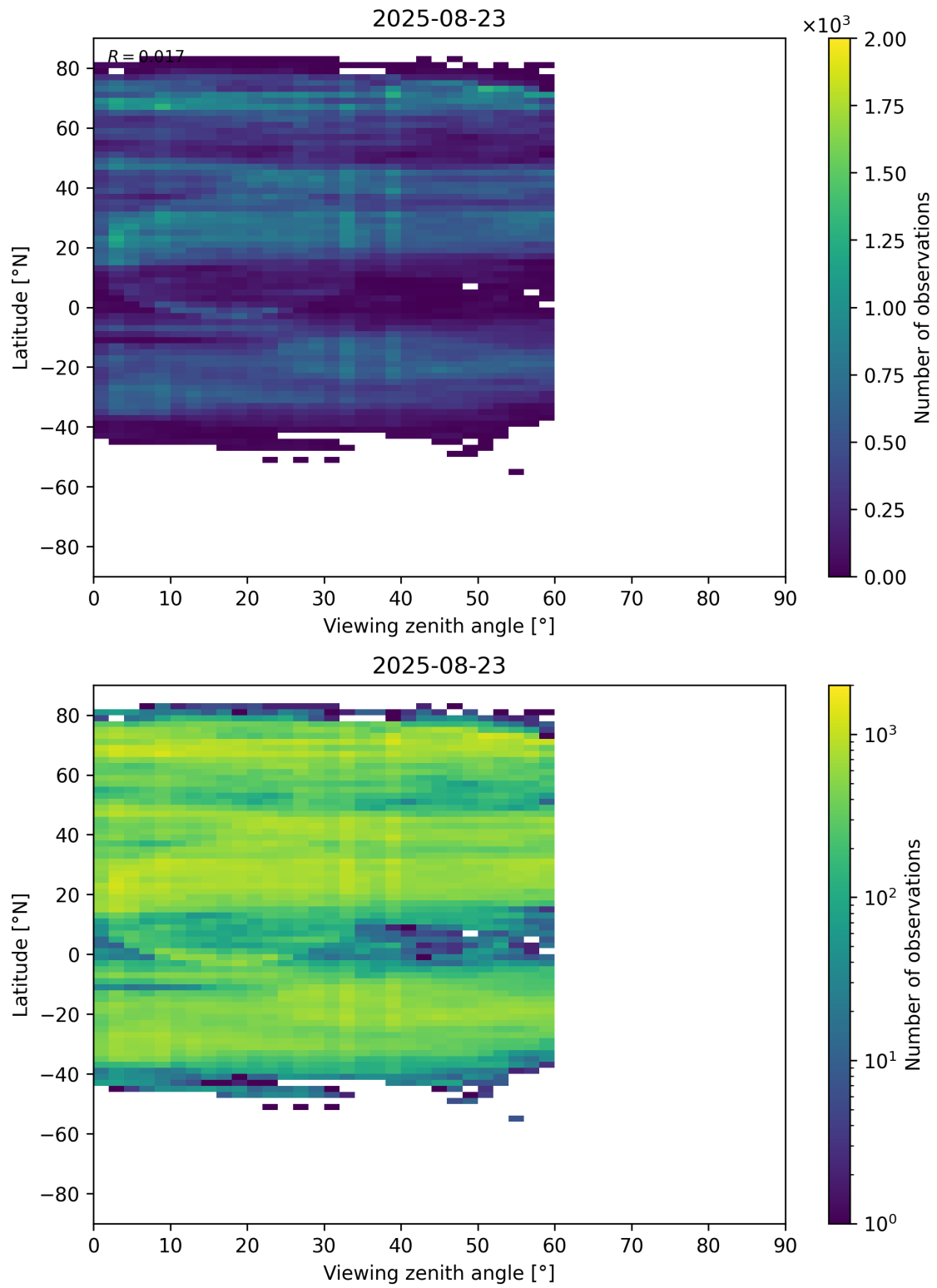
Figure 109: Scatter density plot of “Viewing zenith angle” against “Latitude” for 2025-08-22 to 2025-08-24.
