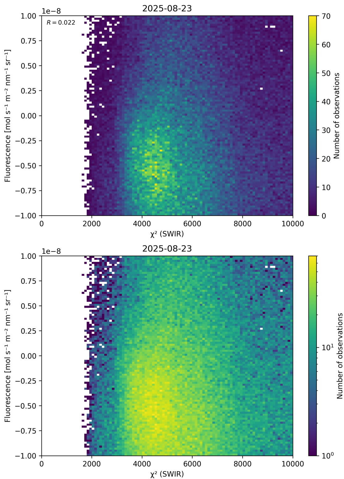
Figure 49: Scatter density plot of “ \chi^2 (SWIR)” against “Fluorescence” for 2025-08-22 to 2025-08-24.
