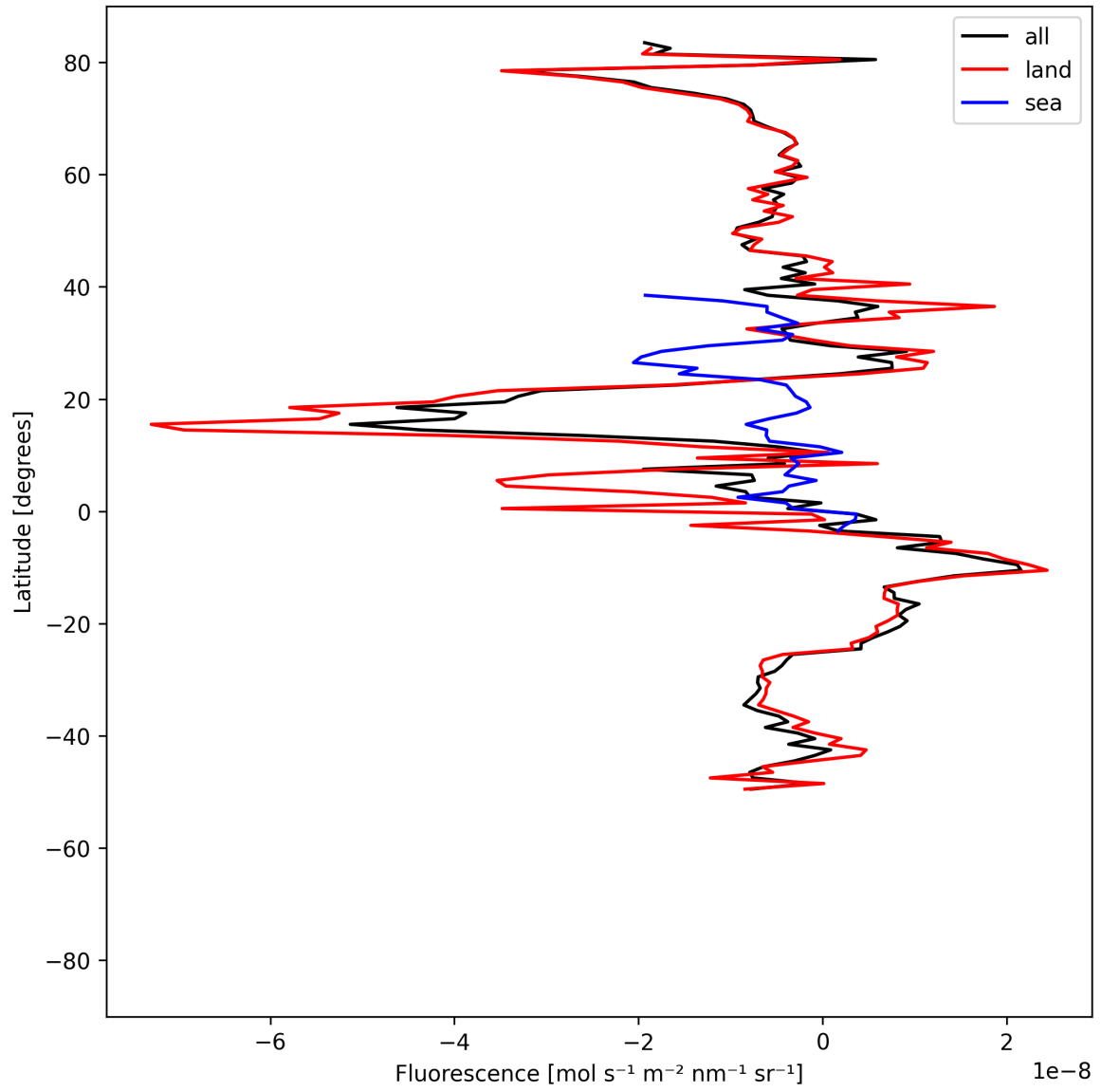
Figure 21: Zonal average of “Fluorescence” for 2025-08-22 to 2025-08-24.
