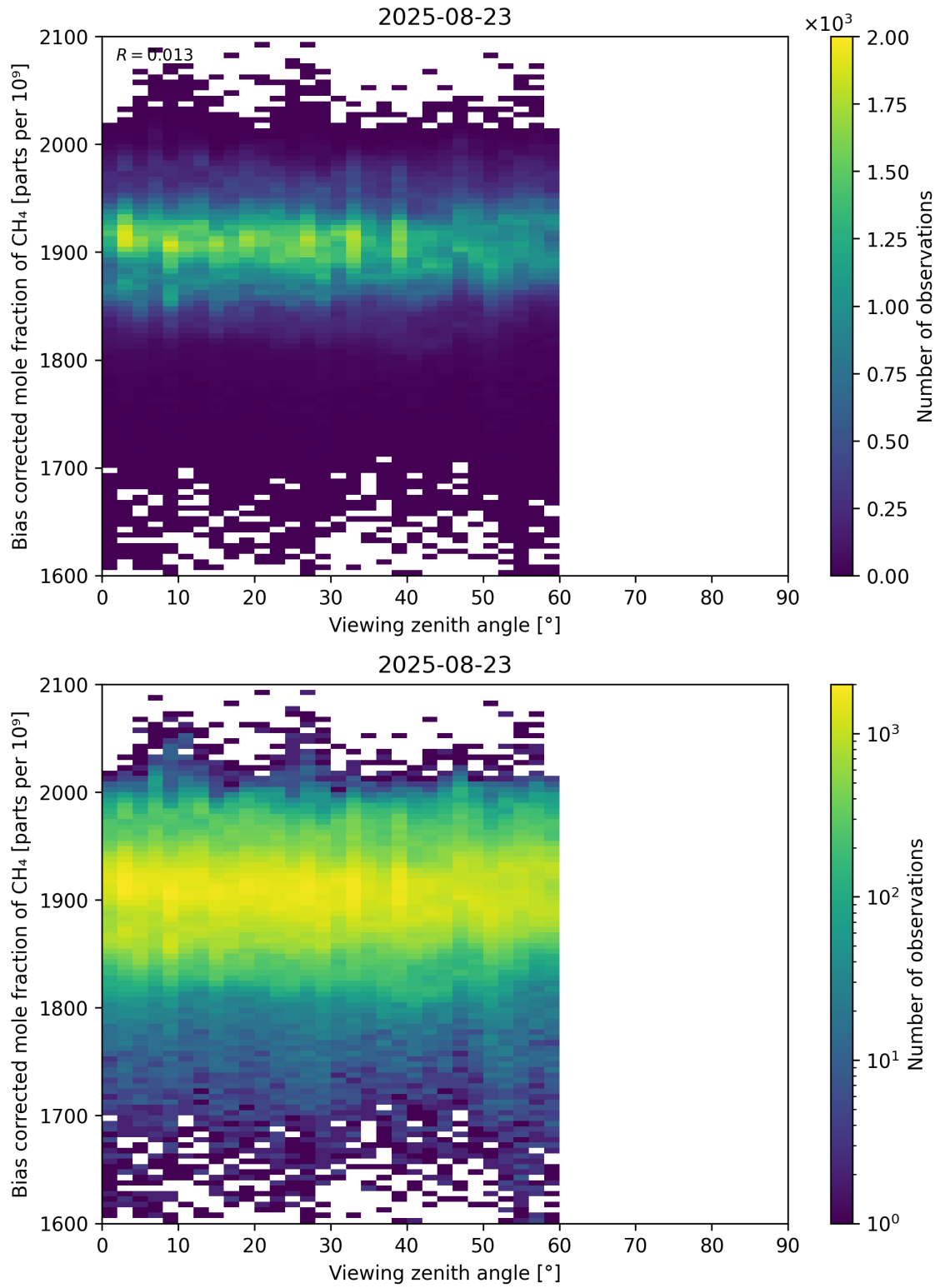
Figure 111: Scatter density plot of “Viewing zenith angle” against “Bias corrected mole fraction of CH 4 ” for 2025-08-22 to 2025-08-24.
