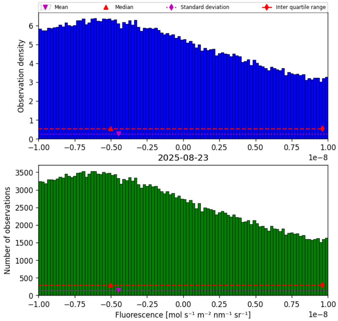
Figure 32: Histogram of “Fluorescence” for 2025-08-22 to 2025-08-24
