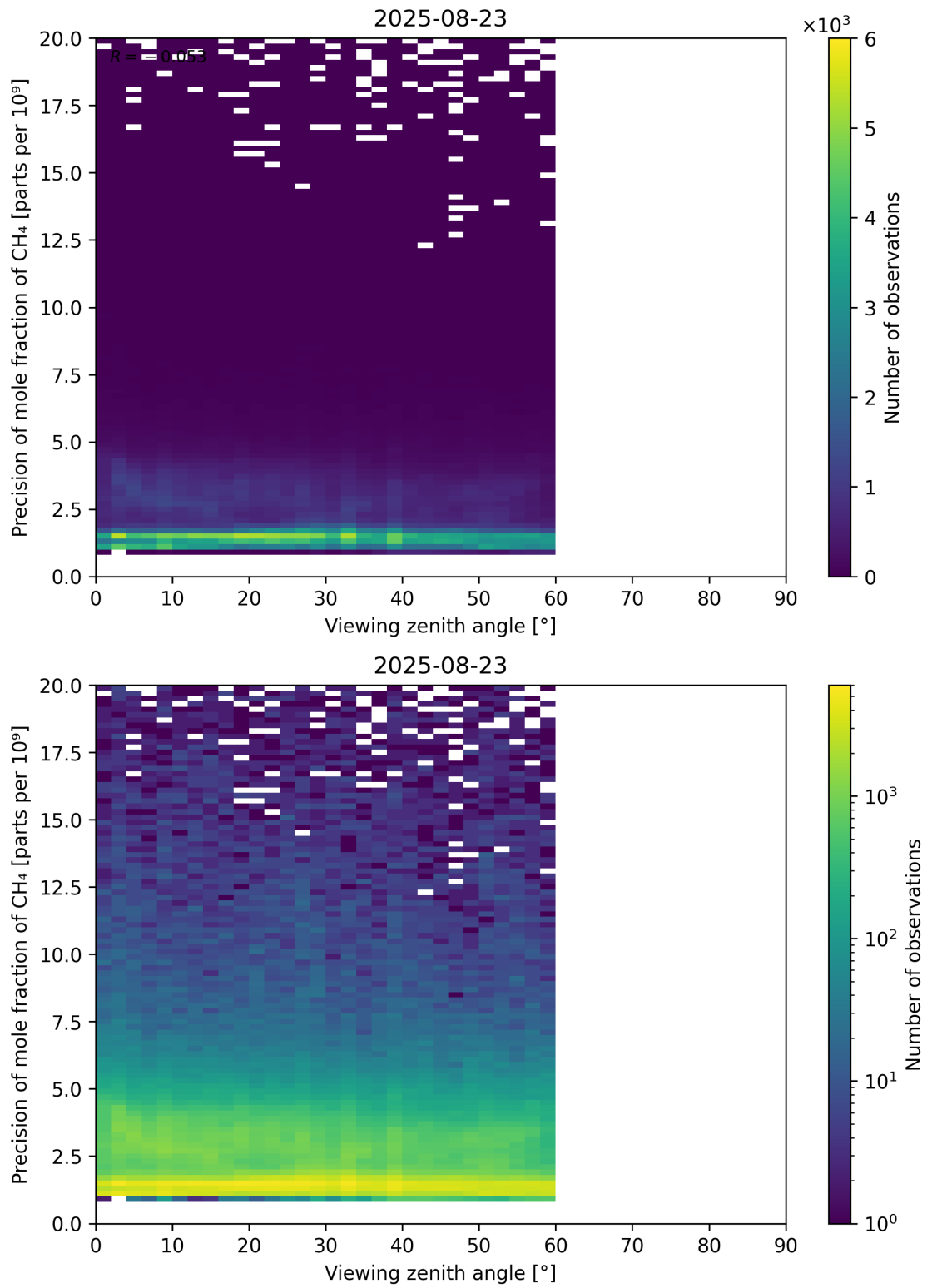
Figure 112: Scatter density plot of “Viewing zenith angle” against “Precision of mole fraction of CH 4 ” for 2025-08-22 to 2025-08-24.
