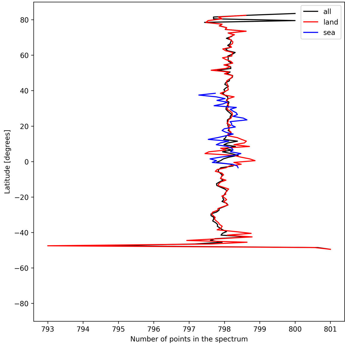
Figure 15: Zonal average of “Number of points in the spectrum” for 2025-08-22 to 2025-08-24.
