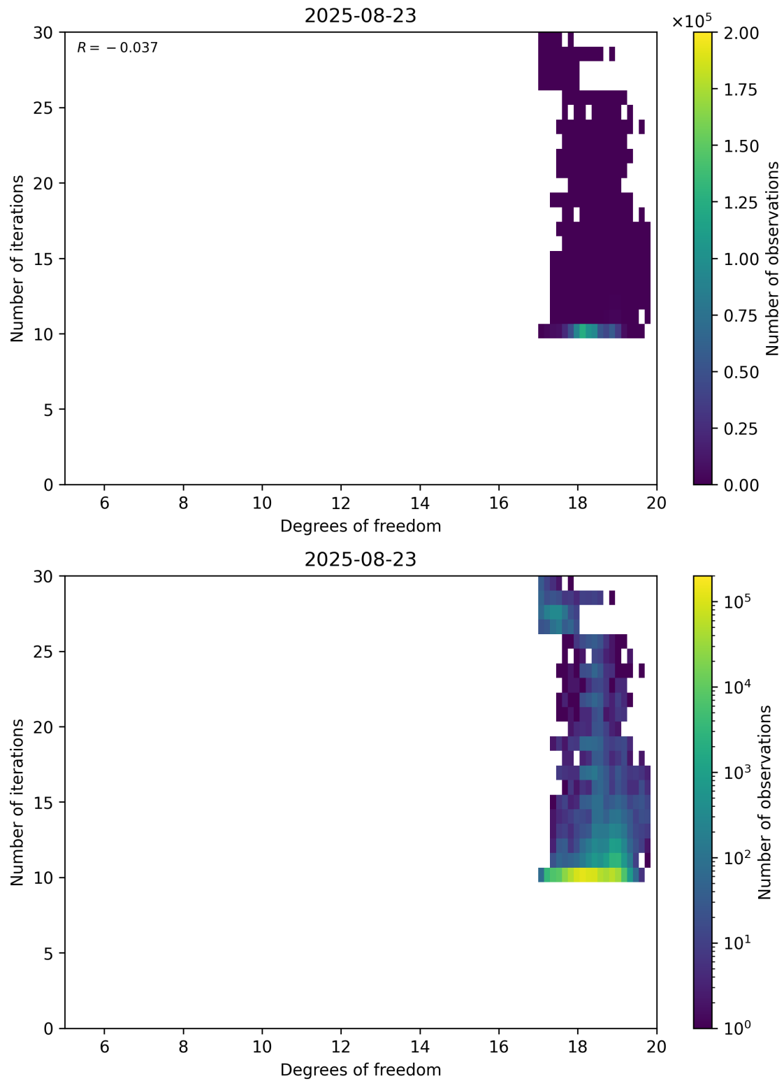
Figure 52: Scatter density plot of “Degrees of freedom” against “Number of iterations” for 2025-08-22 to 2025-08-24.
