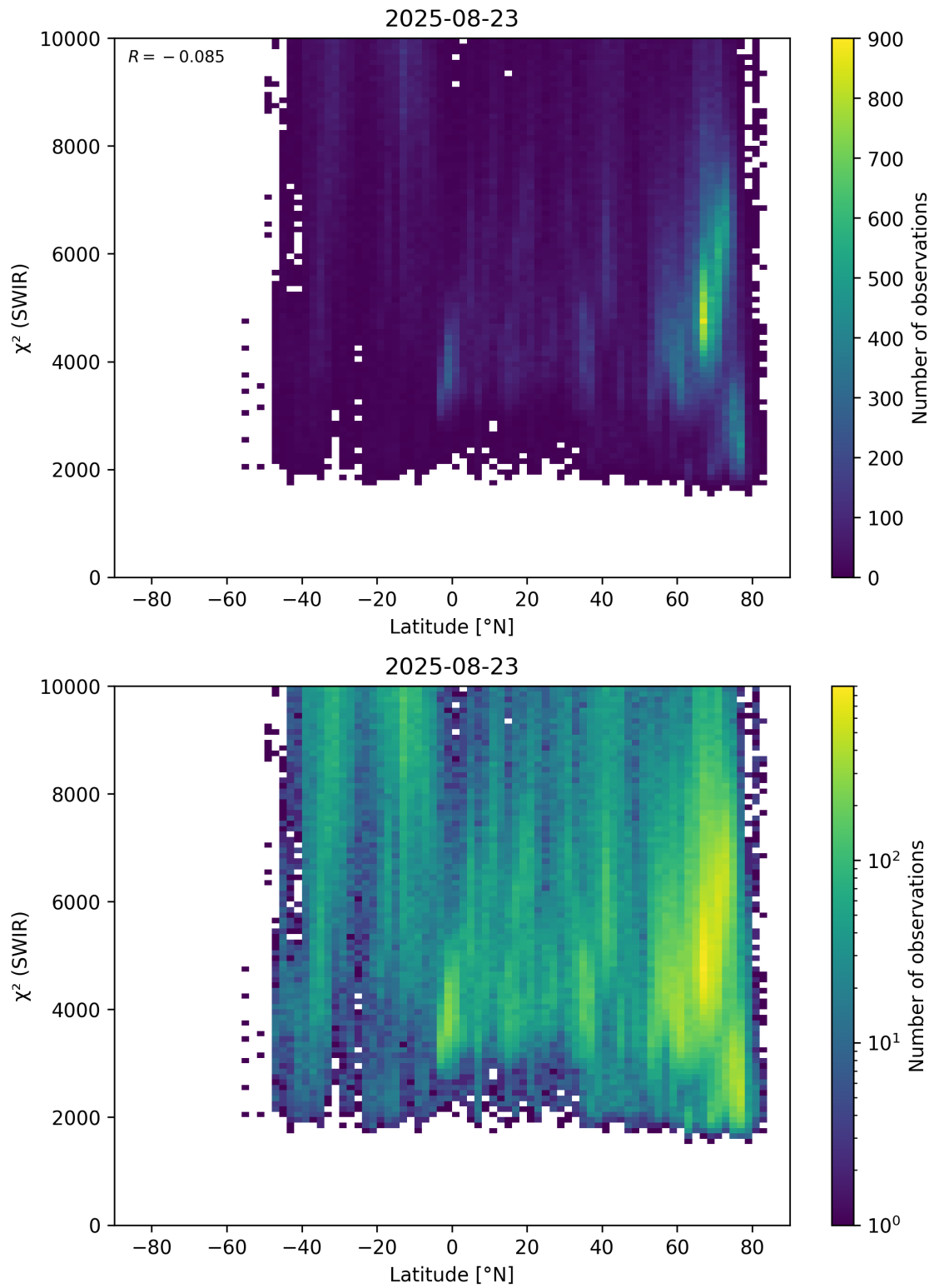
Figure 54: Scatter density plot of “Latitude” against “ \chi^2 (SWIR)” for 2025-08-22 to 2025-08-24.
