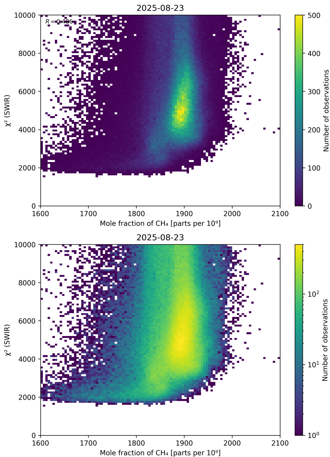
Figure 71: Scatter density plot of “Mole fraction of \text{CH}_4 ” against “ \chi^2 (SWIR)” for 2025-08-22 to 2025-08-24.
