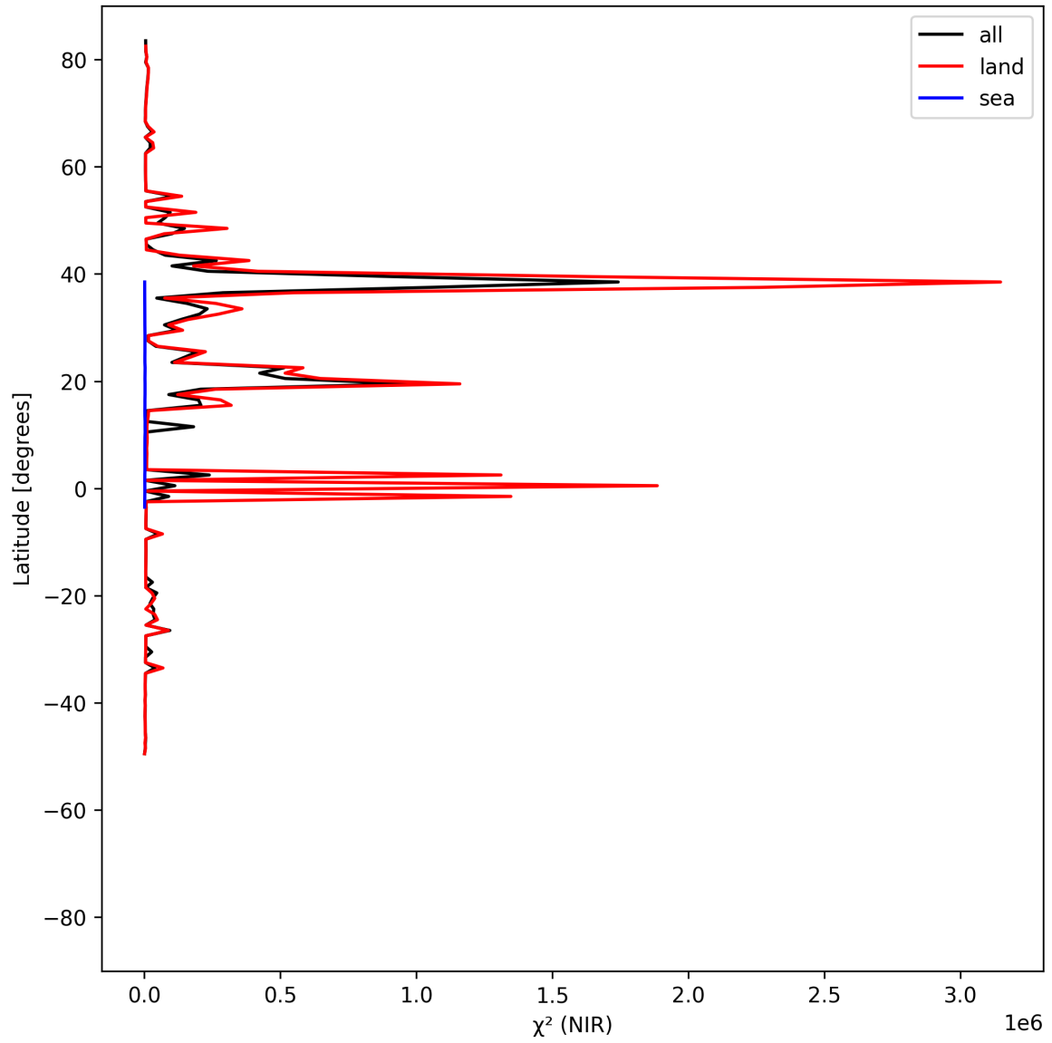
Figure 18: Zonal average of “ \chi^2 (NIR)” for 2025-08-22 to 2025-08-24.
