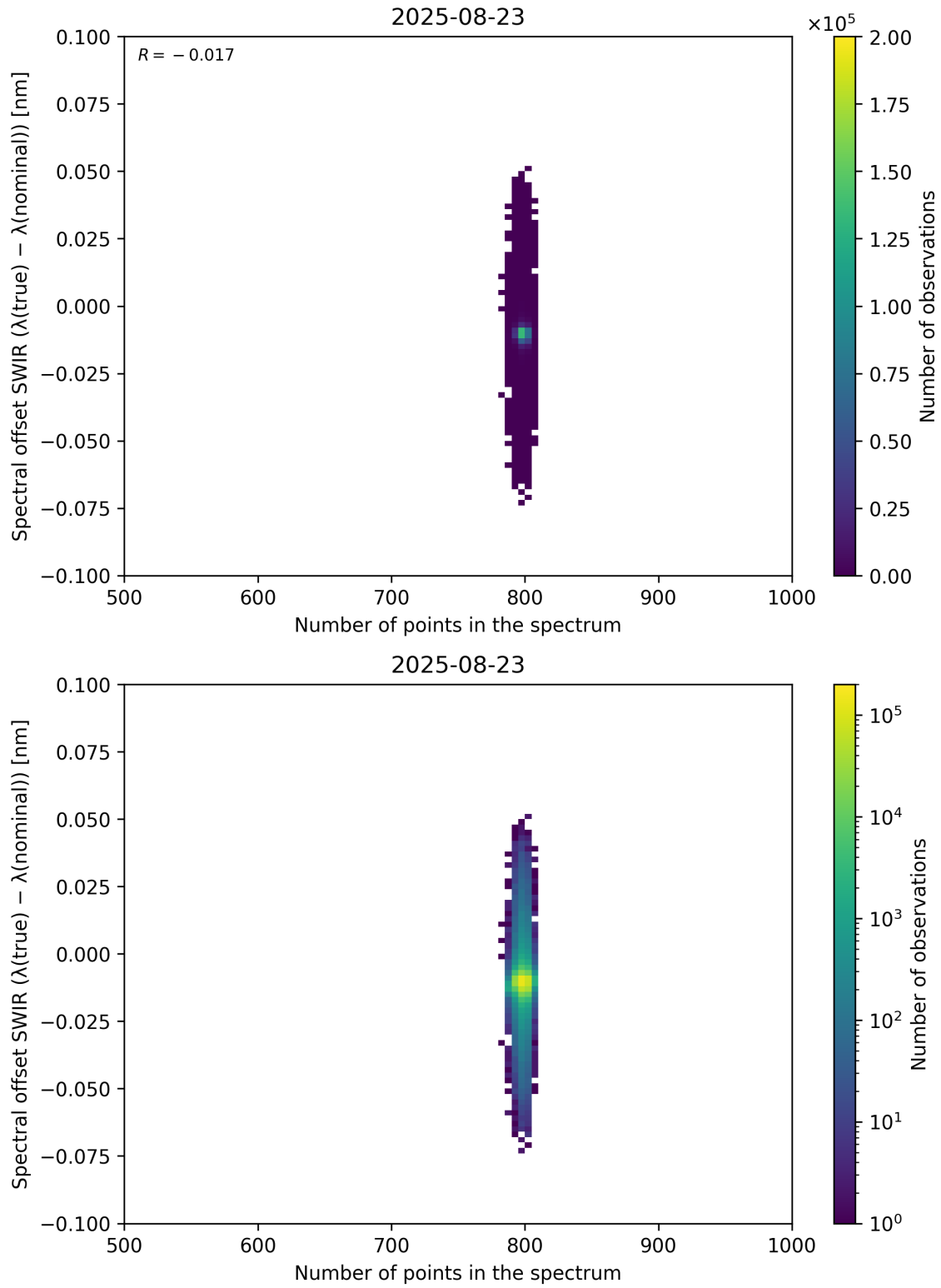
Figure 93: Scatter density plot of “Number of points in the spectrum” against “Spectral offset SWIR ( \lambda_{\text{true}} - \lambda_{\text{nominal}} )” for 2025-08-22 to 2025-08-24.
