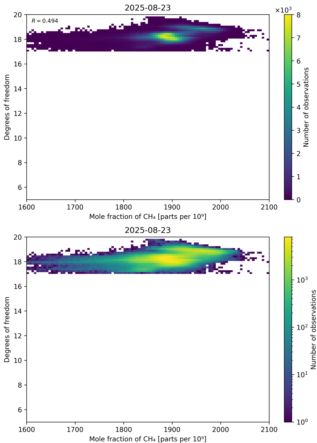
Figure 72: Scatter density plot of “Mole fraction of CH 4 ” against “Degrees of freedom” for 2025-08-22 to 2025-08-24.
