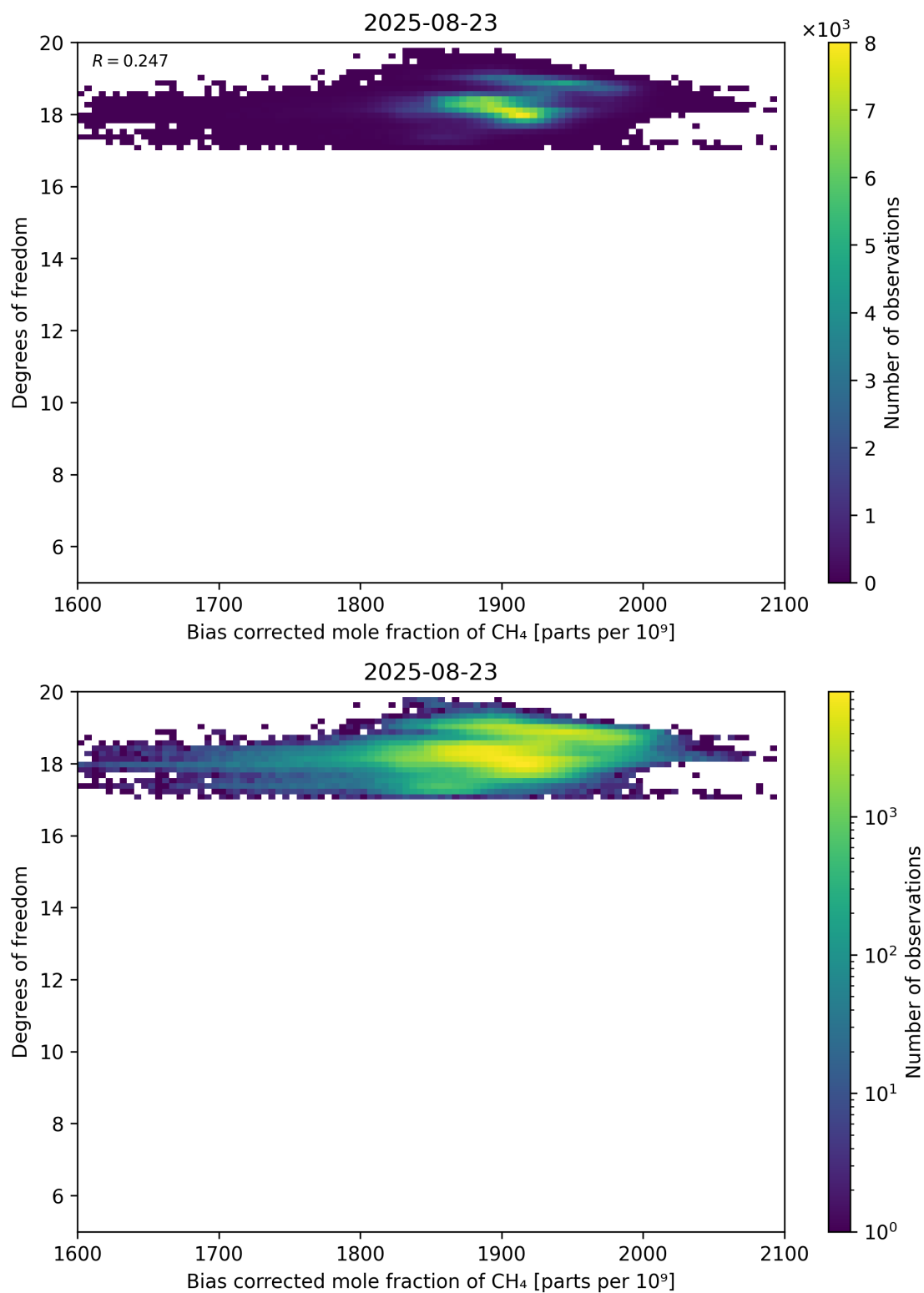
Figure 65: Scatter density plot of “Bias corrected mole fraction of CH 4 ” against “Degrees of freedom” for 2025-08-22 to 2025-08-24.
