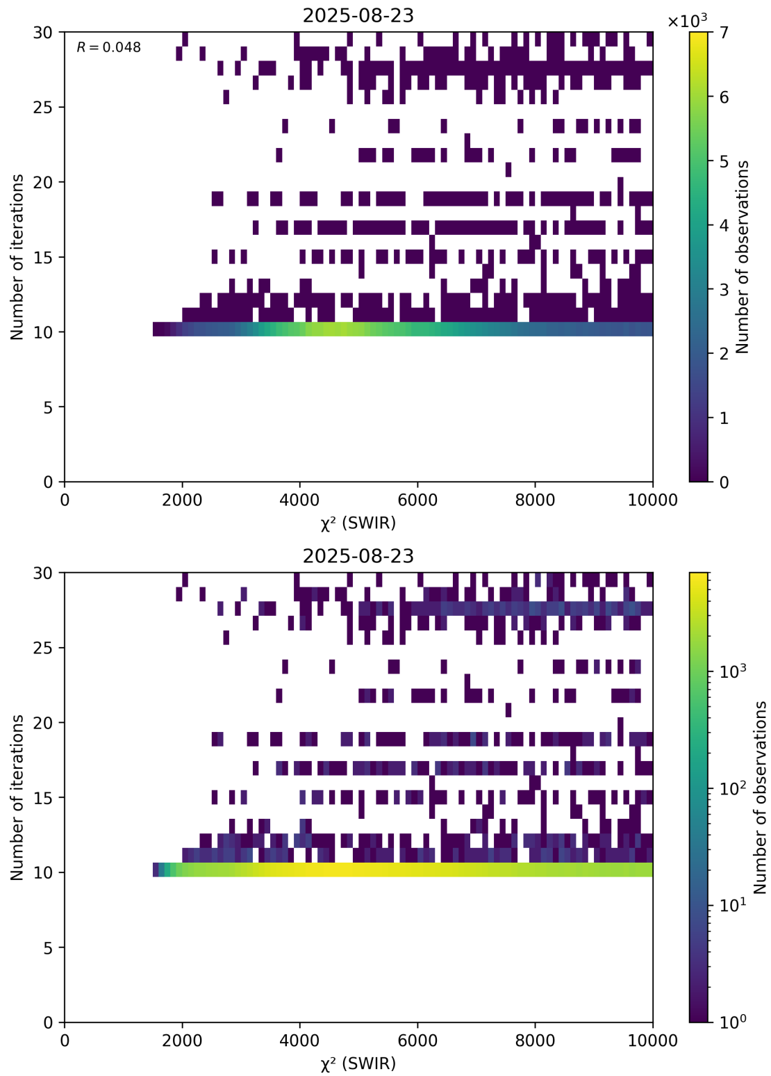
Figure 50: Scatter density plot of “ \chi^2 (SWIR)” against “Number of iterations” for 2025-08-22 to 2025-08-24.
