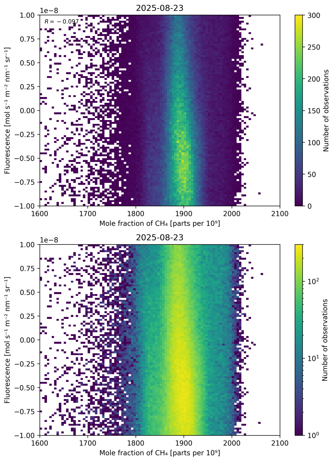
Figure 73: Scatter density plot of “Mole fraction of \text{CH}_4 ” against “Fluorescence” for 2025-08-22 to 2025-08-24.
