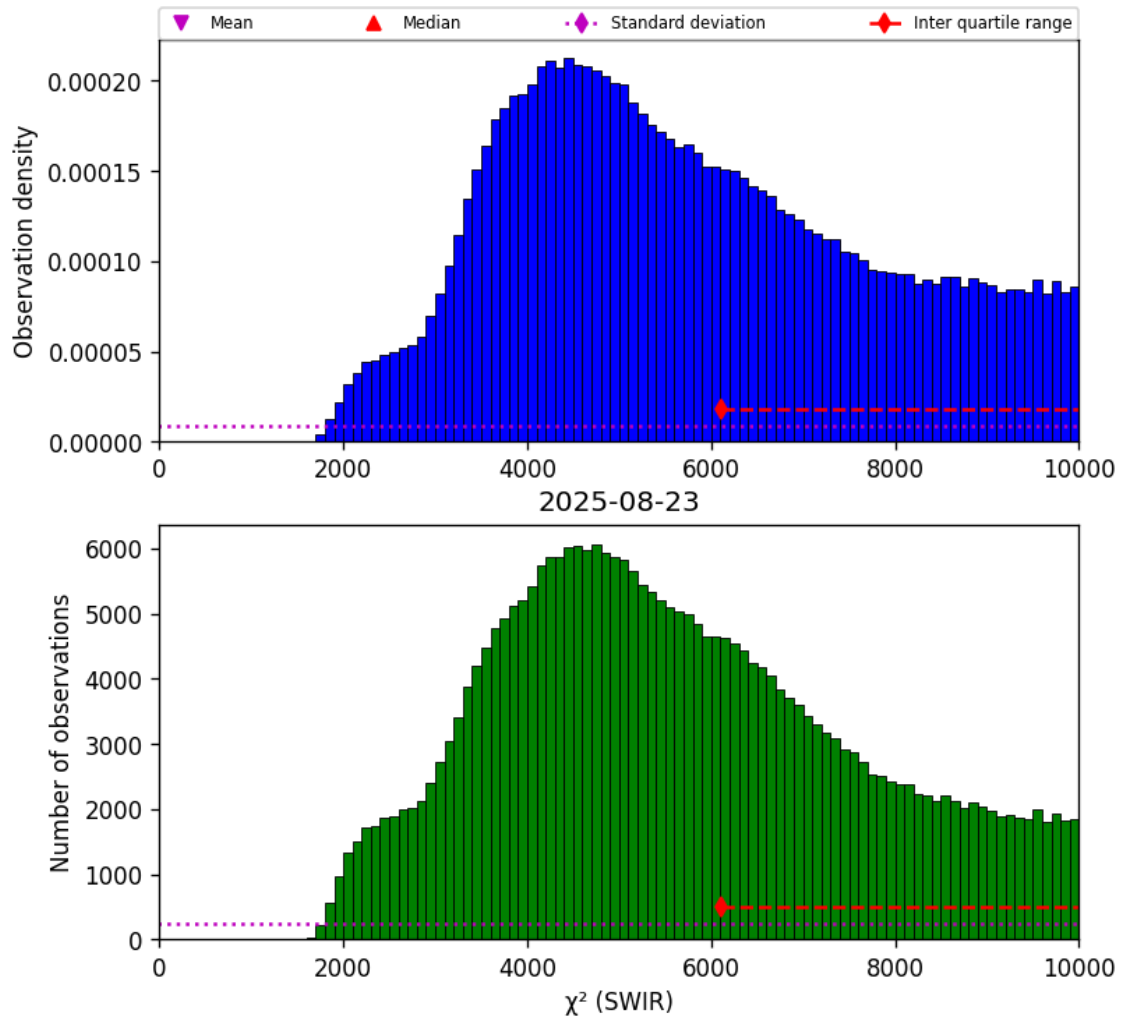
Figure 28: Histogram of " \chi^2 (SWIR)" for 2025-08-22 to 2025-08-24
