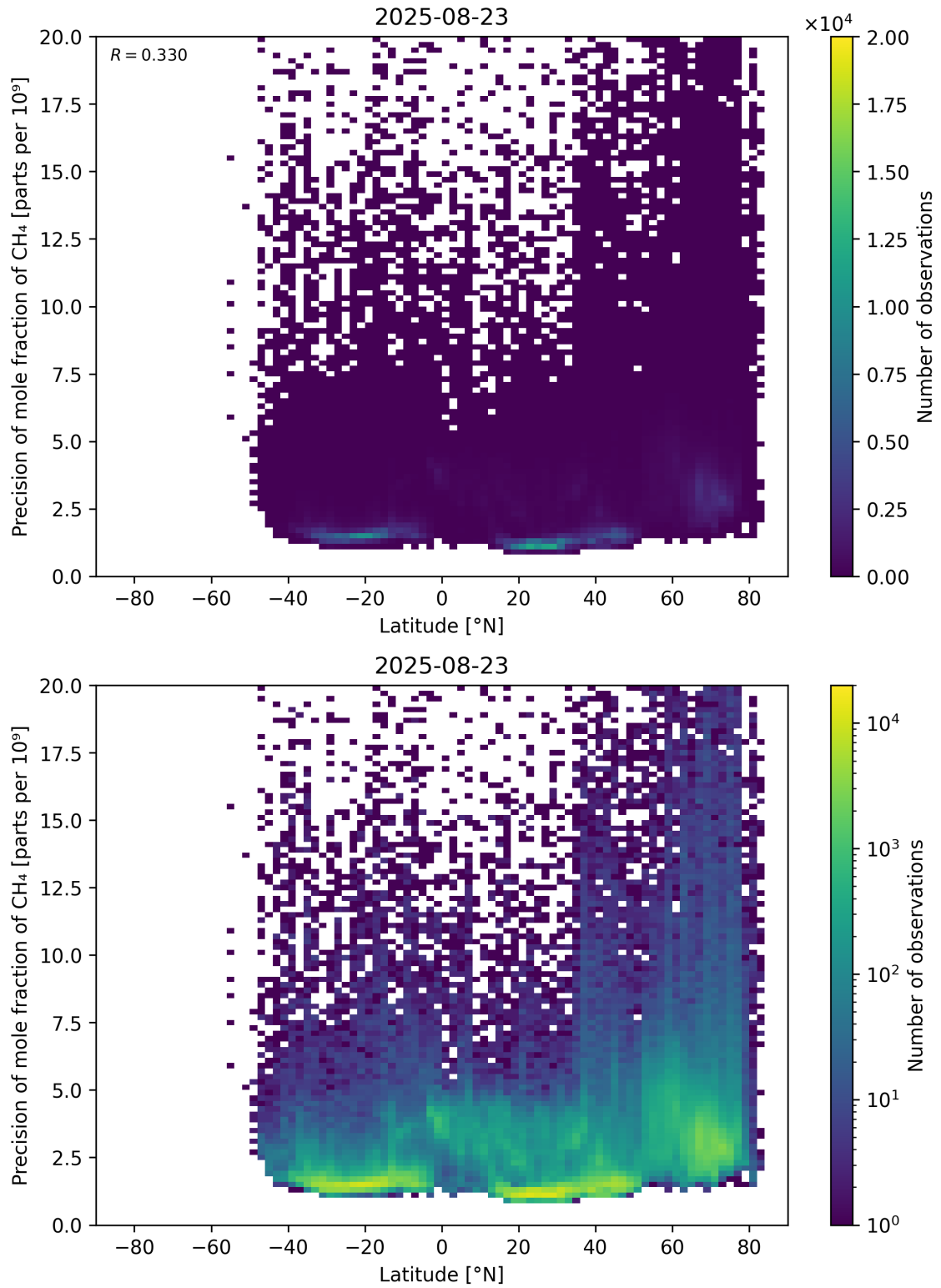
Figure 59: Scatter density plot of “Latitude” against “Precision of mole fraction of \text{CH}_4 ” for 2025-08-22 to 2025-08-24.
