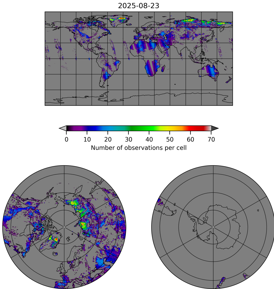
Figure 10: Map of the number of observations for 2025-08-22 to 2025-08-24
