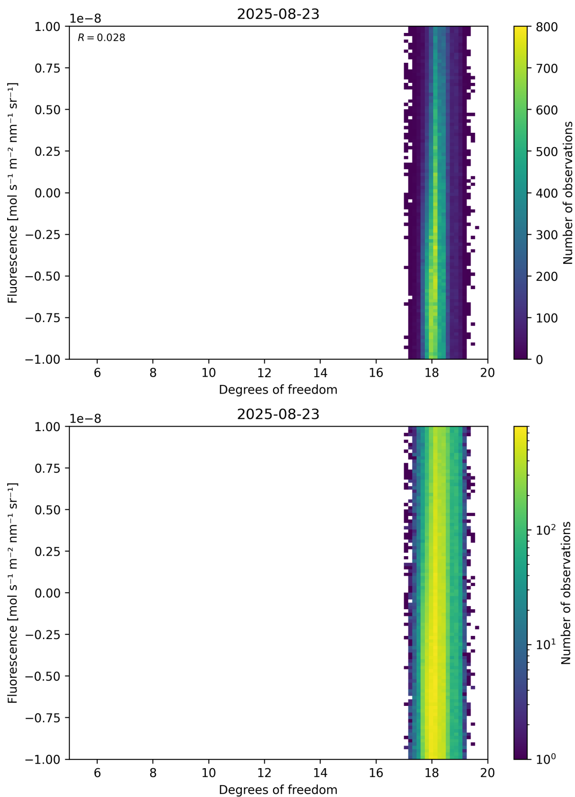
Figure 51: Scatter density plot of “Degrees of freedom” against “Fluorescence” for 2025-08-22 to 2025-08-24.
