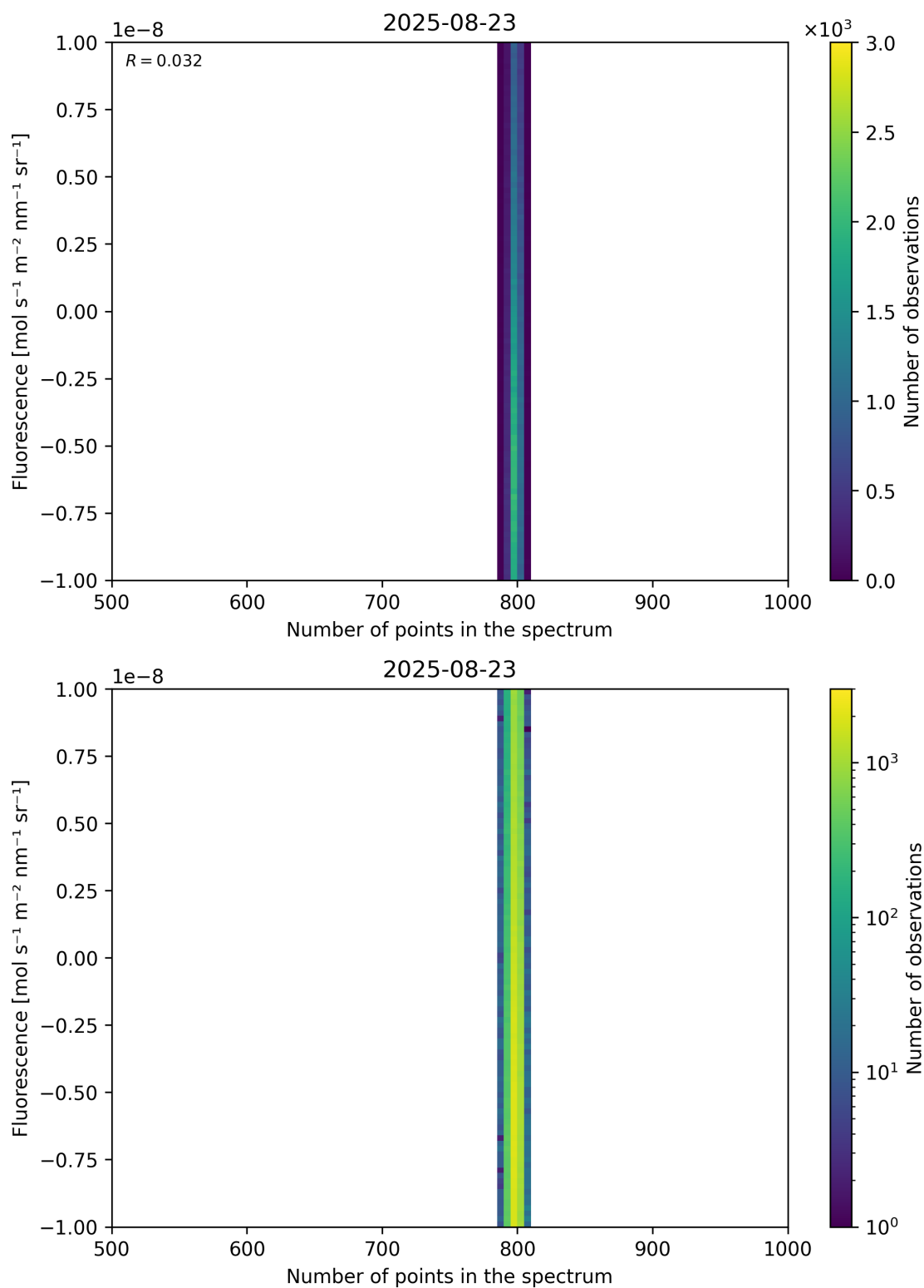
Figure 91: Scatter density plot of “Number of points in the spectrum” against “Fluorescence” for 2025-08-22 to 2025-08-24.
