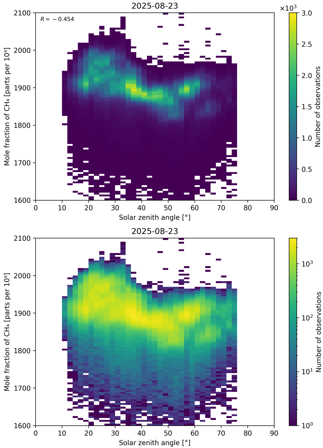
Figure 99: Scatter density plot of “Solar zenith angle” against “Mole fraction of CH 4 ” for 2025-08-22 to 2025-08-24.
