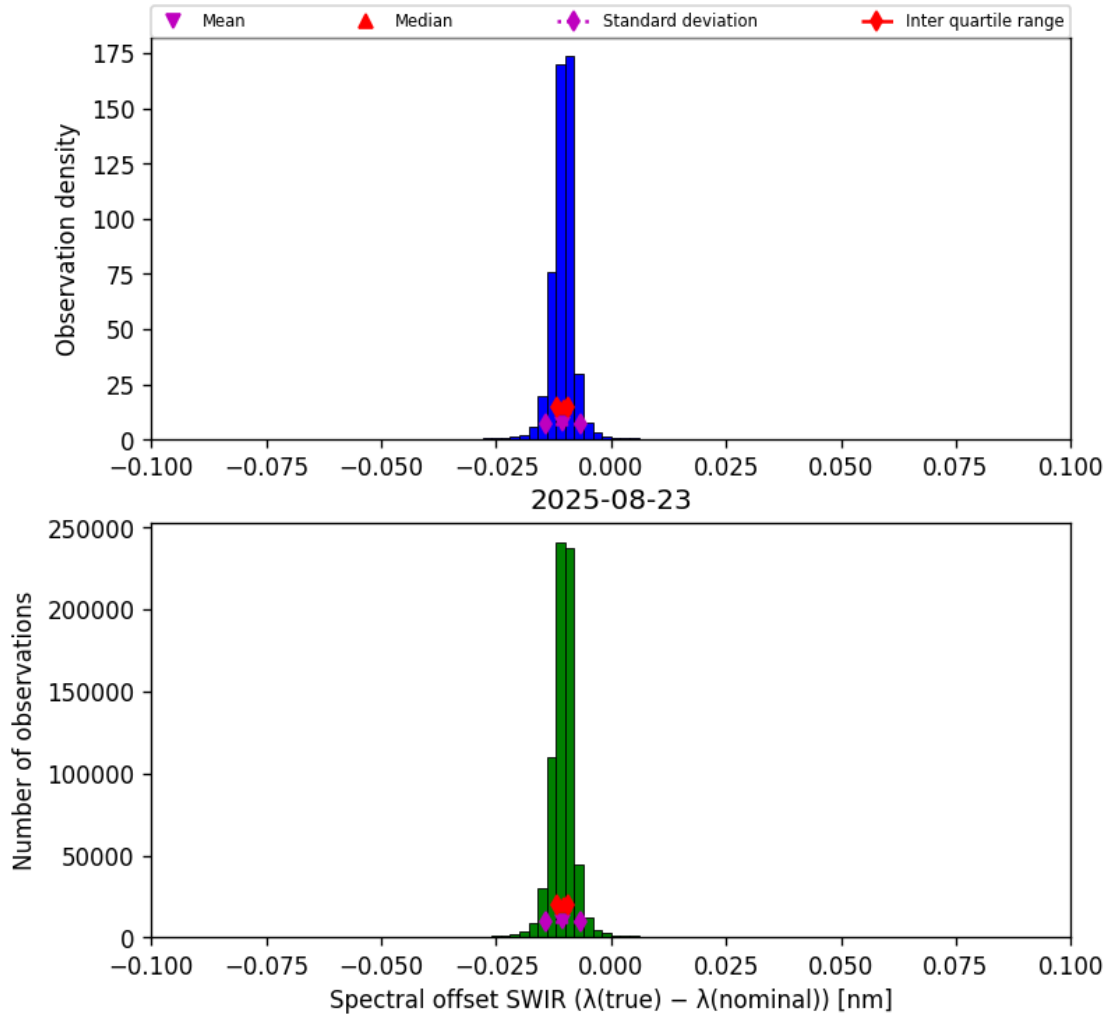
Figure 27: Histogram of “Spectral offset SWIR ( \lambda_{\text{true}} - \lambda_{\text{nominal}} )” for 2025-08-22 to 2025-08-24
