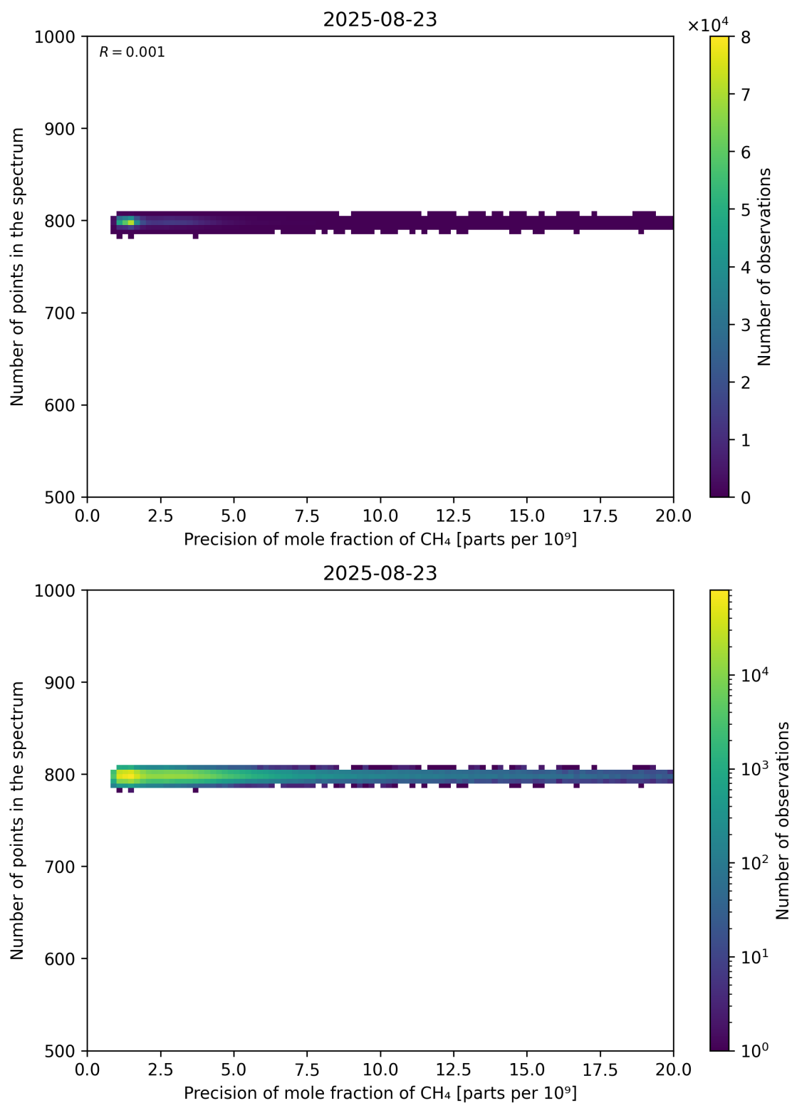
Figure 84: Scatter density plot of “Precision of mole fraction of CH 4 ” against “Number of points in the spectrum” for 2025-08-22 to 2025-08-24.
