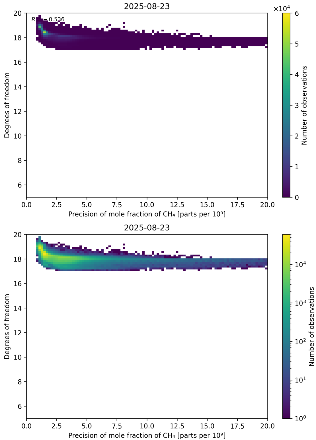
Figure 80: Scatter density plot of “Precision of mole fraction of CH 4 ” against “Degrees of freedom” for 2025-08-22 to 2025-08-24.
