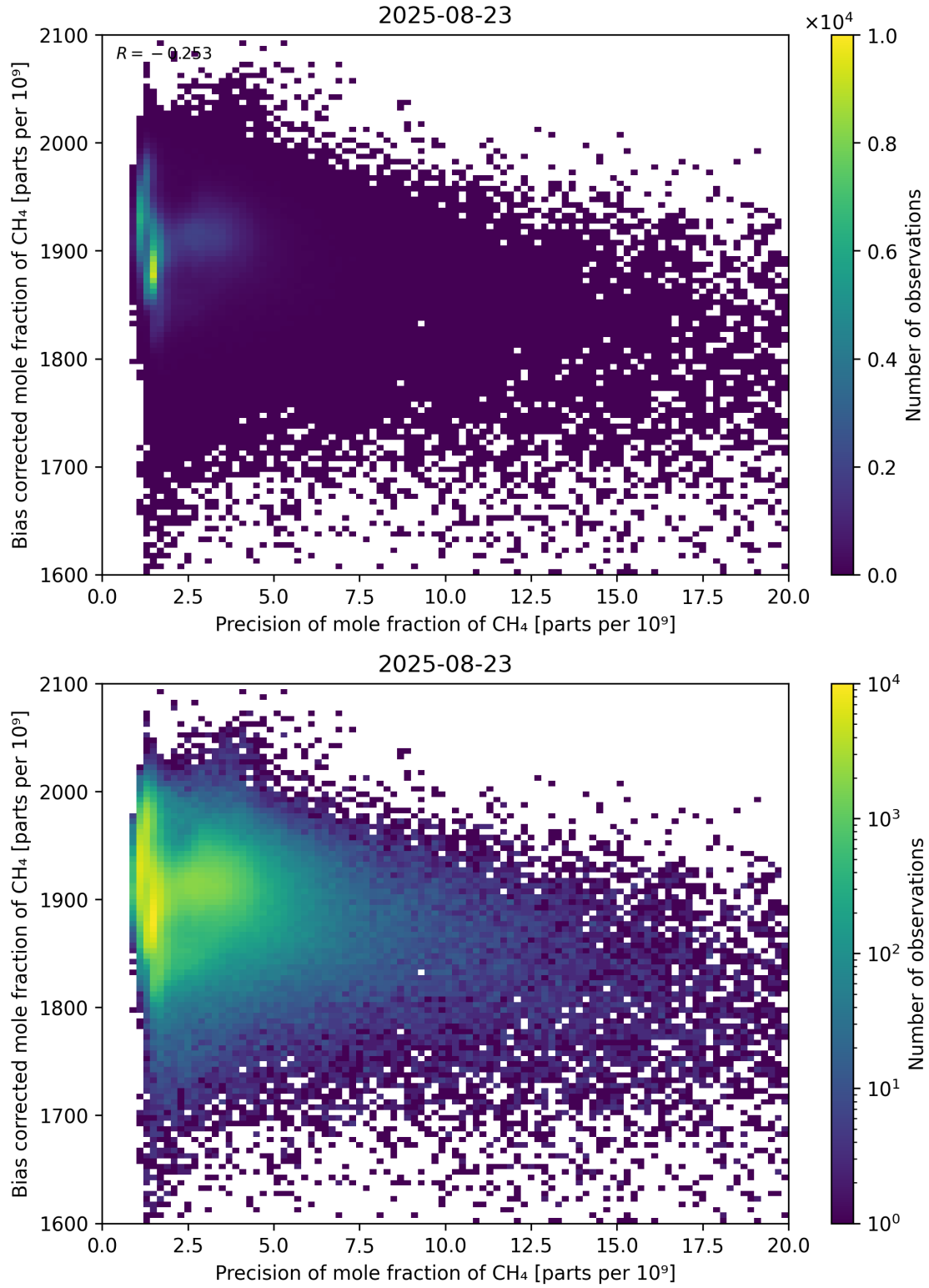
Figure 82: Scatter density plot of “Precision of mole fraction of CH 4 ” against “Bias corrected mole fraction of CH 4 ” for 2025-08-22 to 2025-08-24.
