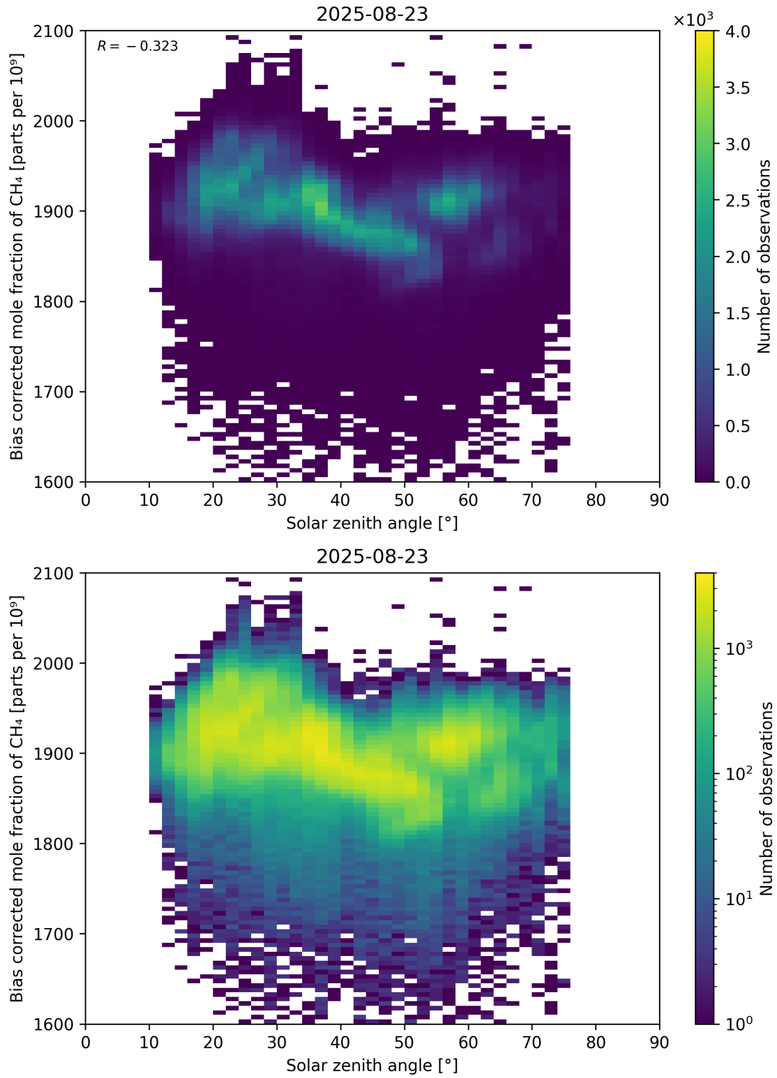
Figure 100: Scatter density plot of “Solar zenith angle” against “Bias corrected mole fraction of \text{CH}_4 ” for 2025-08-22 to 2025-08-24.
