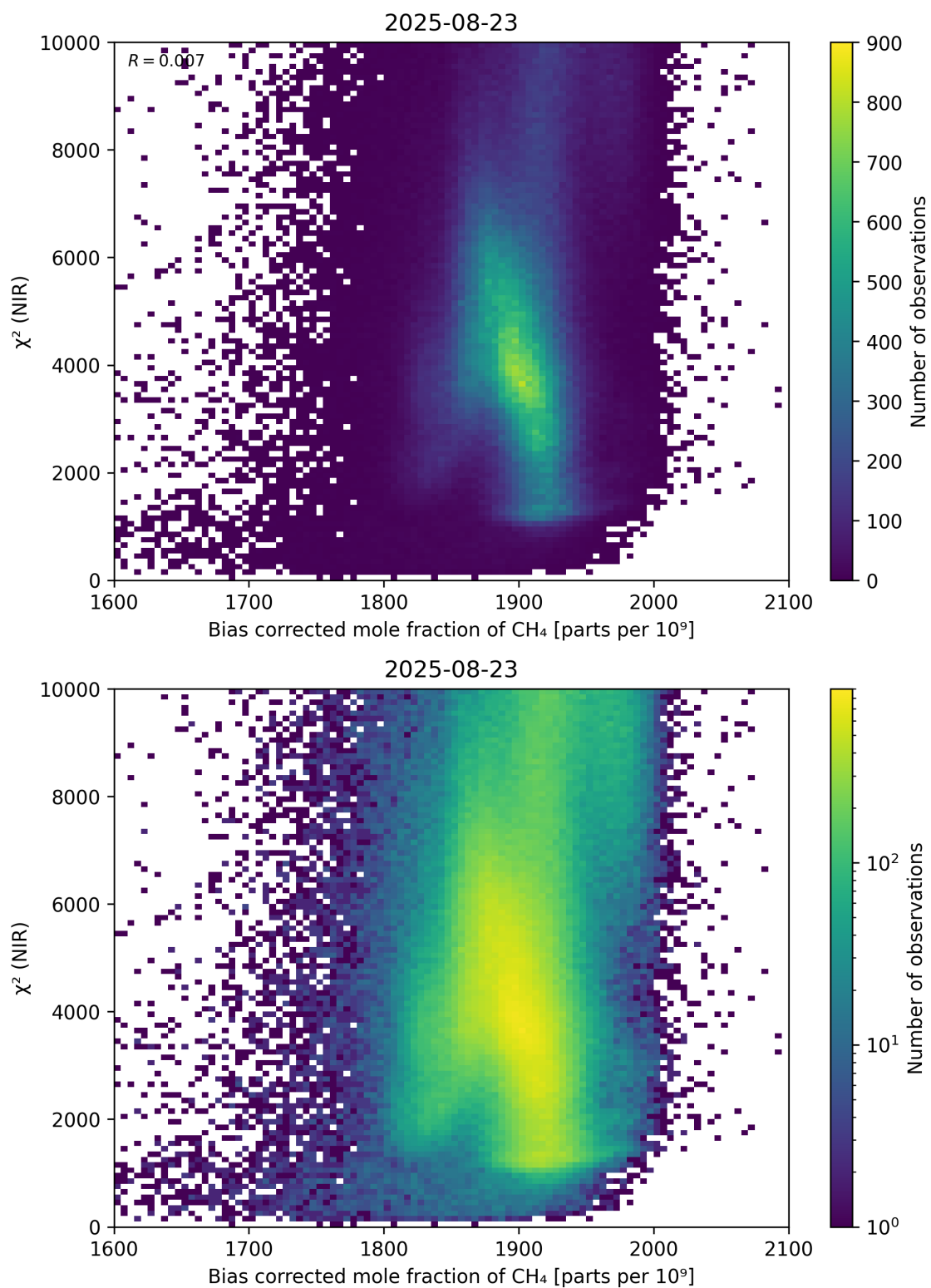
Figure 63: Scatter density plot of “Bias corrected mole fraction of CH 4 ” against “ \chi^2 (NIR)” for 2025-08-22 to 2025-08-24.
