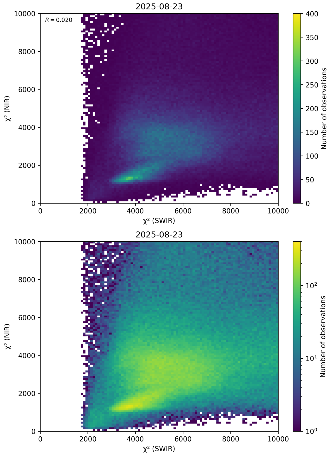
Figure 47: Scatter density plot of “ \chi^2 (SWIR)” against “ \chi^2 (NIR)” for 2025-08-22 to 2025-08-24.
