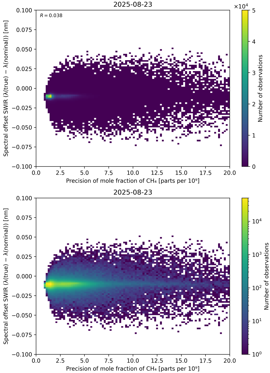
Figure 85: Scatter density plot of “Precision of mole fraction of CH 4 ” against “Spectral offset SWIR ( \lambda_{\text{true}} - \lambda_{\text{nominal}} )” for 2025-08-22 to 2025-08-24.
