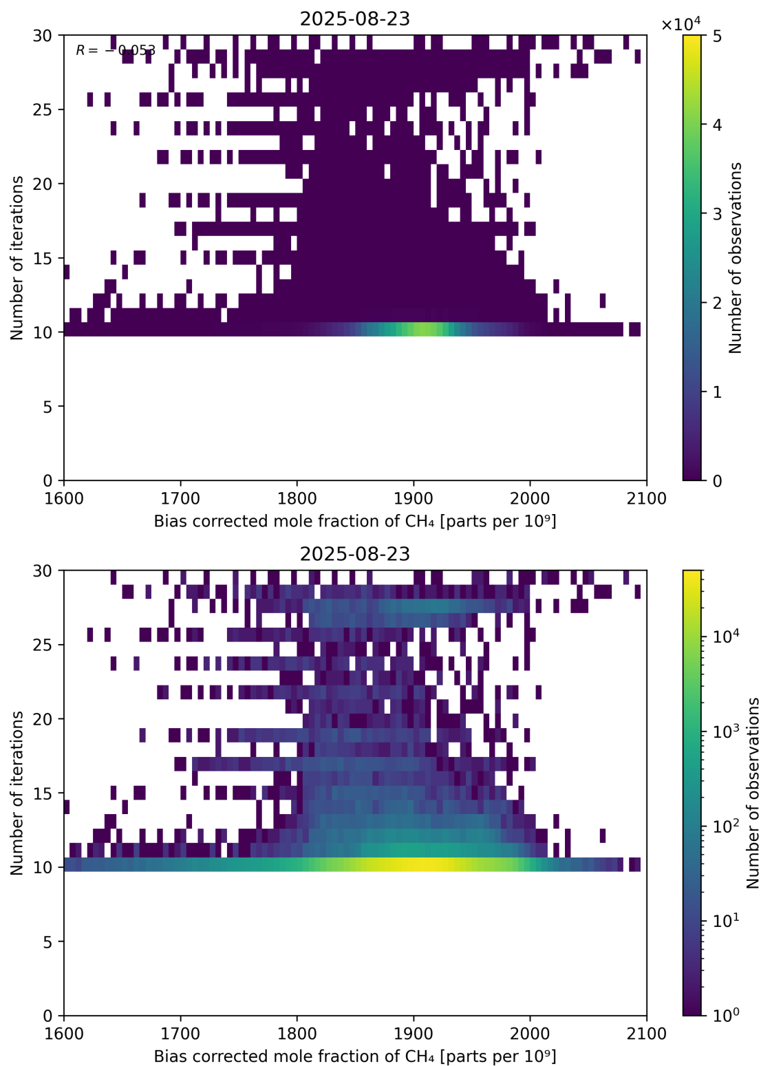
Figure 67: Scatter density plot of “Bias corrected mole fraction of CH 4 ” against “Number of iterations” for 2025-08-22 to 2025-08-24.
