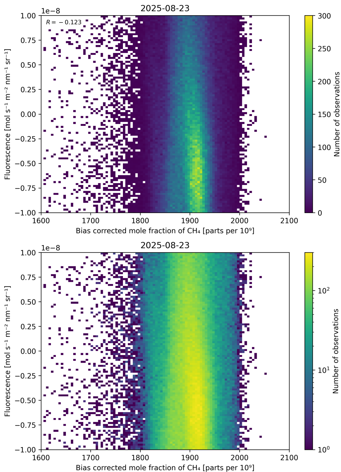
Figure 66: Scatter density plot of “Bias corrected mole fraction of \text{CH}_4 ” against “Fluorescence” for 2025-08-22 to 2025-08-24.
