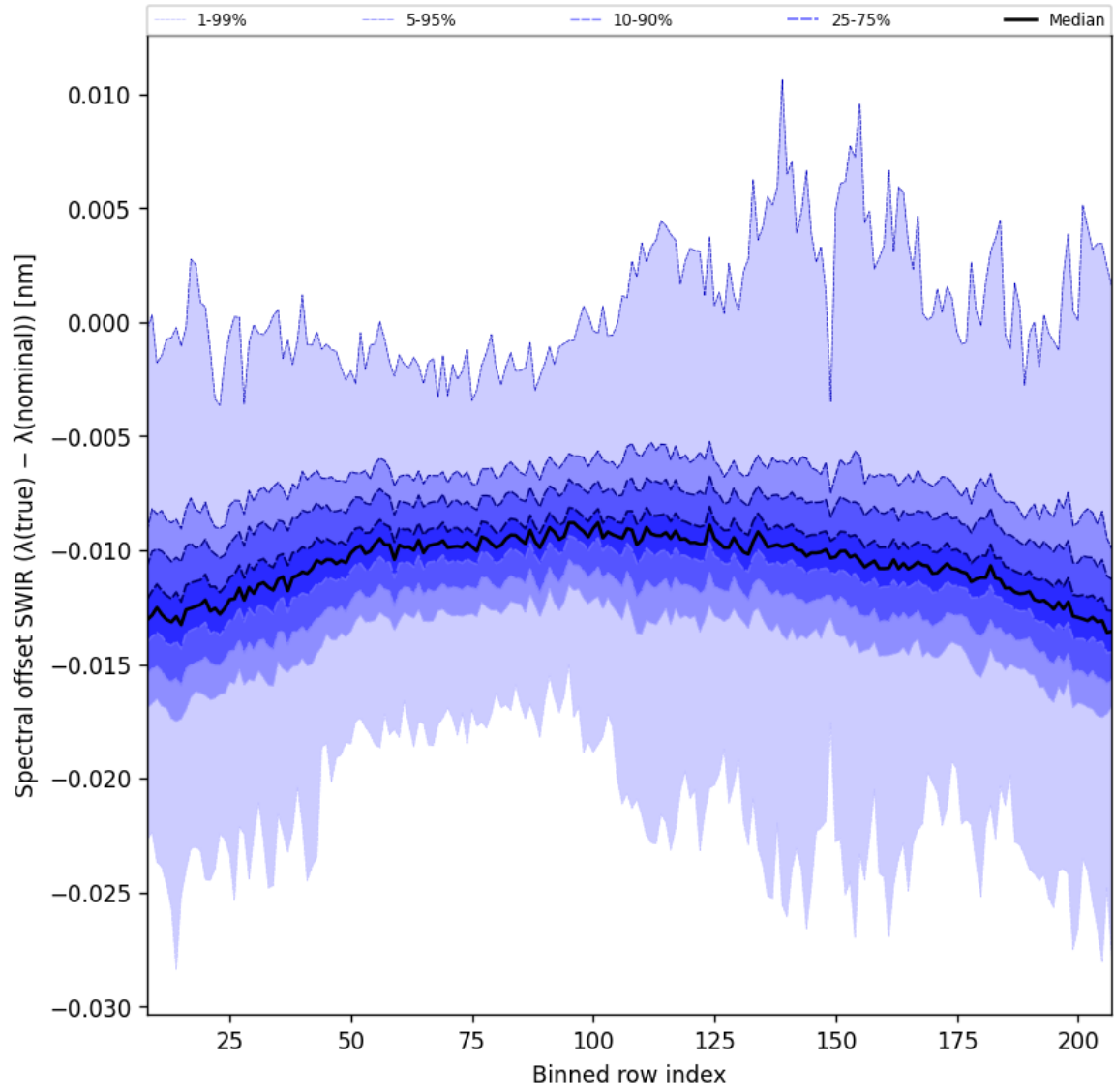
Figure 38: Along track statistics of “Spectral offset SWIR ( \lambda_{\text{true}} - \lambda_{\text{nominal}} )” for 2025-08-22 to 2025-08-24
