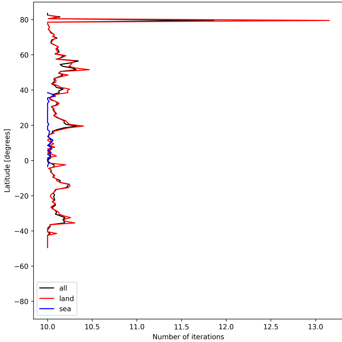
Figure 20: Zonal average of “Number of iterations” for 2025-08-22 to 2025-08-24.
