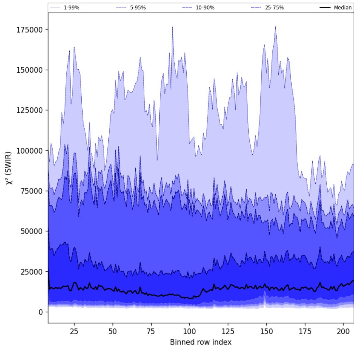
Figure 39: Along track statistics of “ \chi^2 (SWIR)” for 2025-08-22 to 2025-08-24
