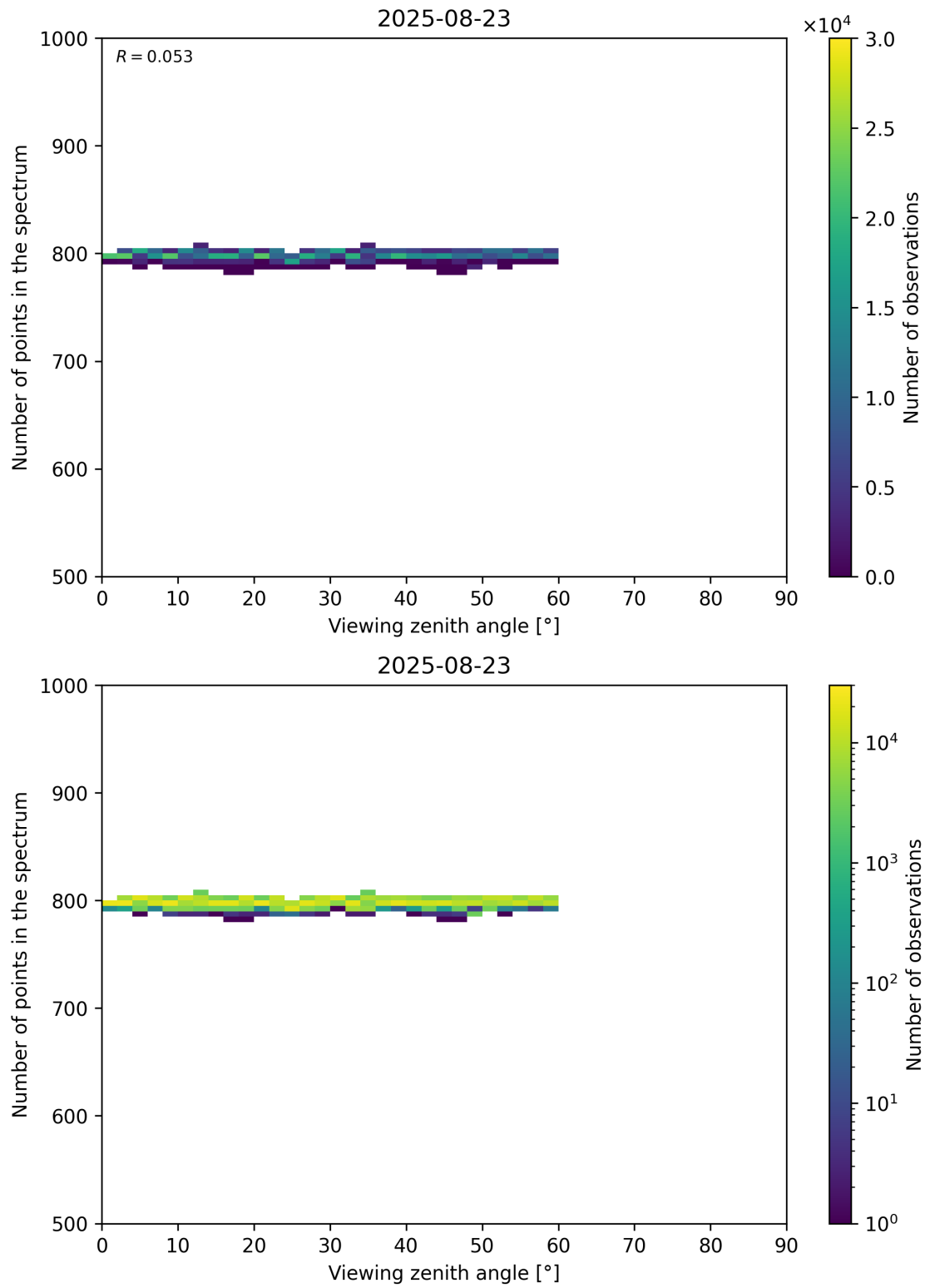
Figure 114: Scatter density plot of “Viewing zenith angle” against “Number of points in the spectrum” for 2025-08-22 to 2025-08-24.
