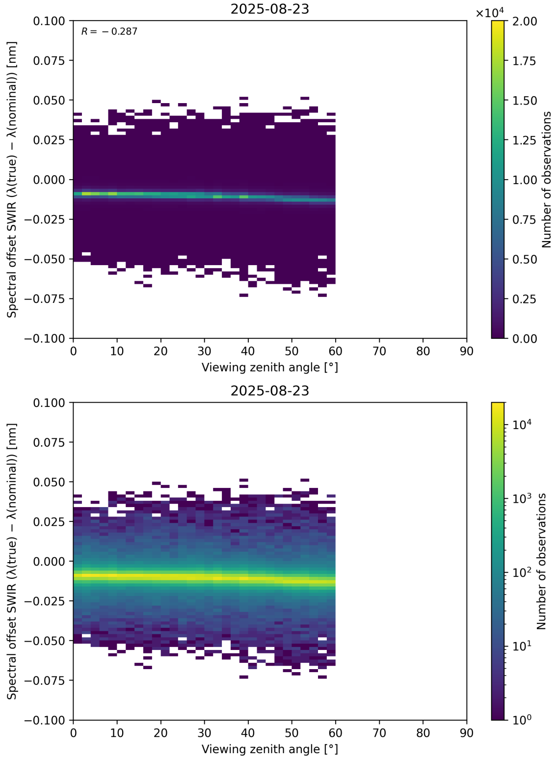
Figure 116: Scatter density plot of “Viewing zenith angle” against “Spectral offset SWIR ( \lambda_{\text{true}} - \lambda_{\text{nominal}} )” for 2025-08-22 to 2025-08-24.
