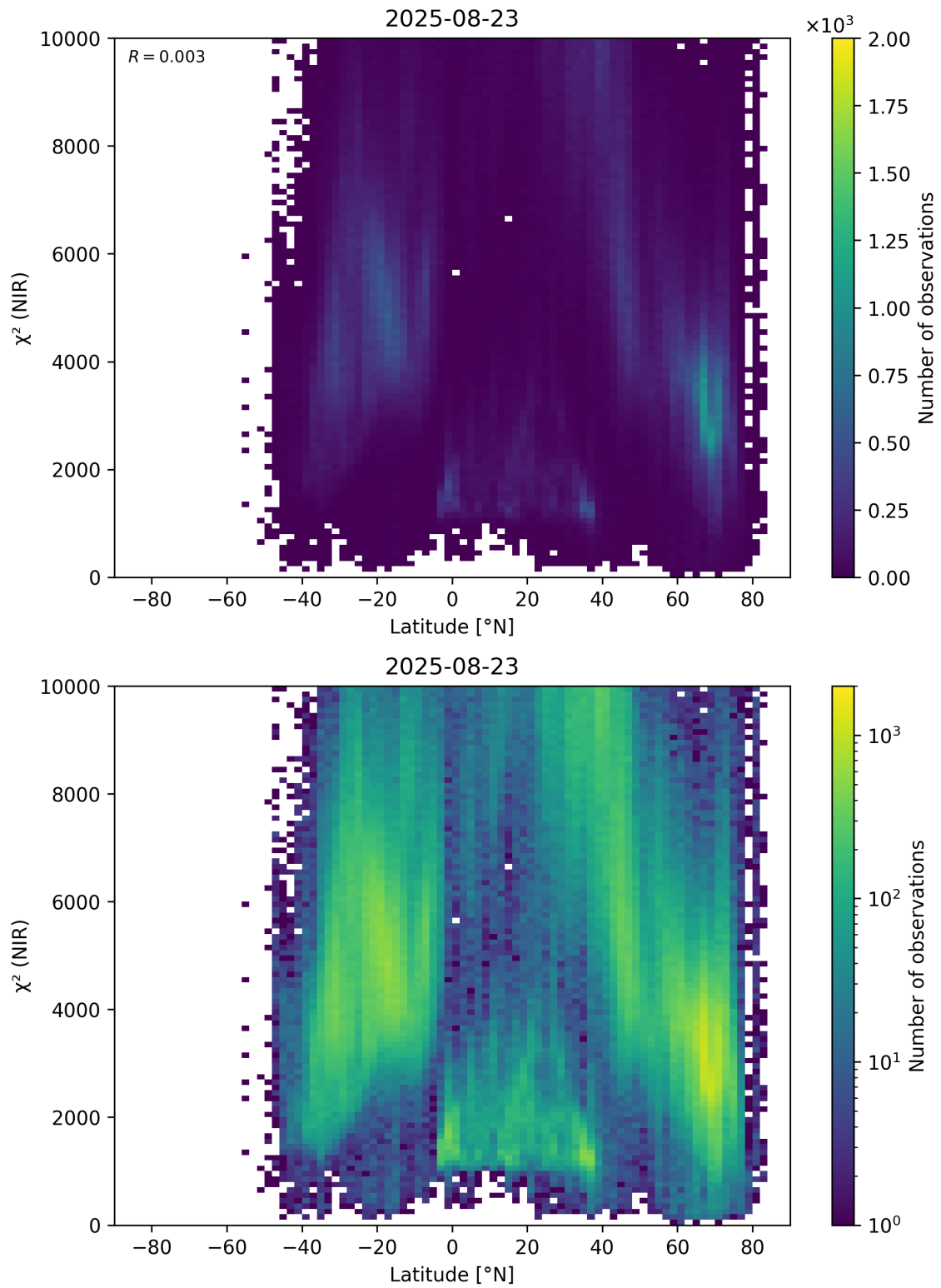
Figure 53: Scatter density plot of “Latitude” against “ \chi^2 (NIR)” for 2025-08-22 to 2025-08-24.
