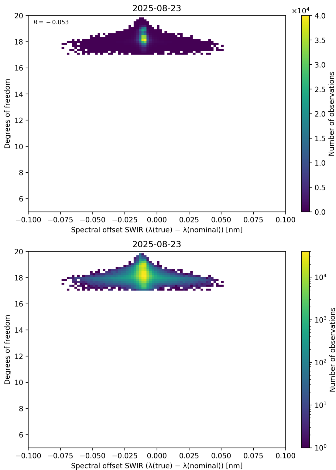
Figure 119: Scatter density plot of “Spectral offset SWIR ( \lambda_{\text{true}} - \lambda_{\text{nominal}} )” against “Degrees of freedom” for 2025-08-22 to 2025-08-24.
