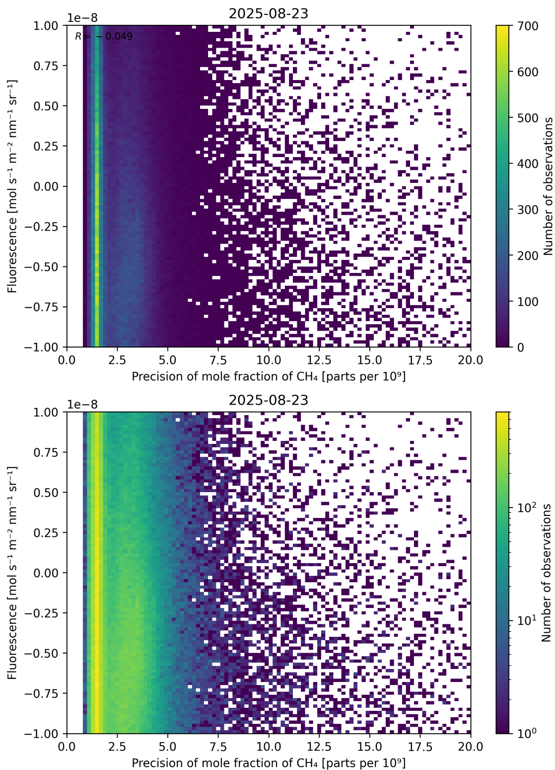
Figure 81: Scatter density plot of “Precision of mole fraction of \text{CH}_4 ” against “Fluorescence” for 2025-08-22 to 2025-08-24.
