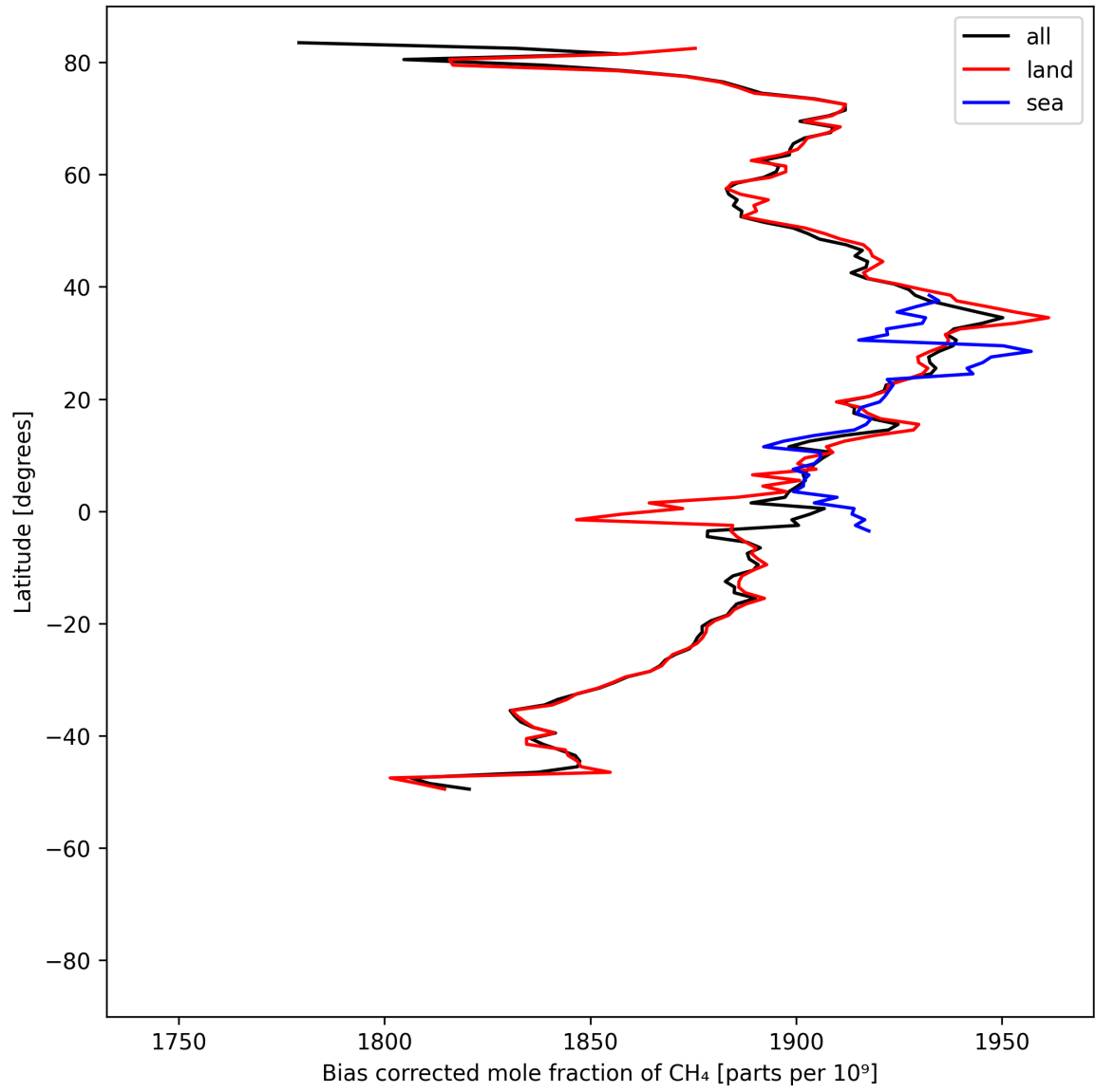
Figure 14: Zonal average of “Bias corrected mole fraction of CH 4 ” for 2025-08-22 to 2025-08-24.
