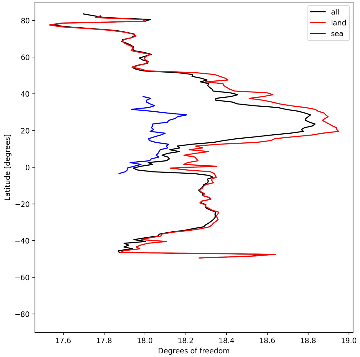
Figure 19: Zonal average of “Degrees of freedom” for 2025-08-22 to 2025-08-24.
