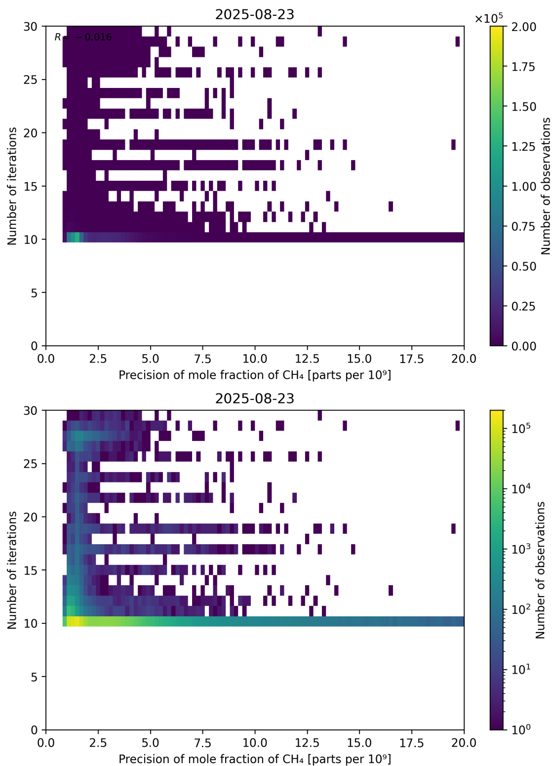
Figure 83: Scatter density plot of “Precision of mole fraction of CH 4 ” against “Number of iterations” for 2025-08-22 to 2025-08-24.
