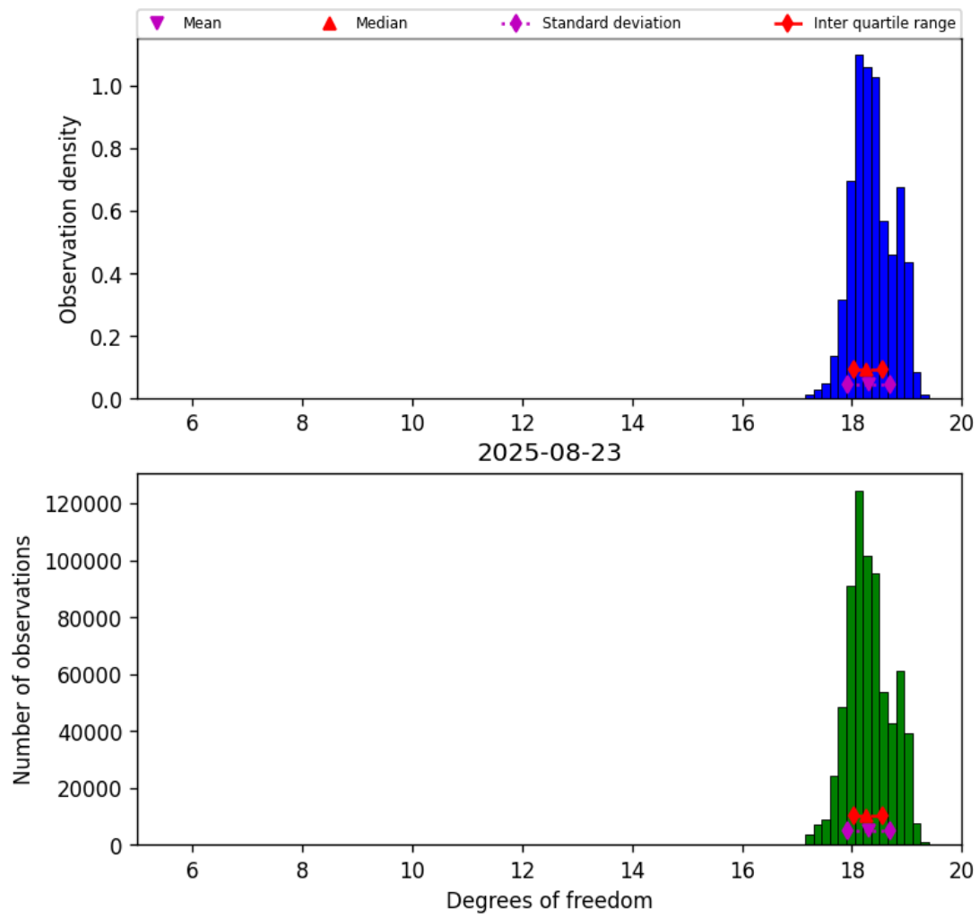
Figure 30: Histogram of “Degrees of freedom” for 2025-08-22 to 2025-08-24
