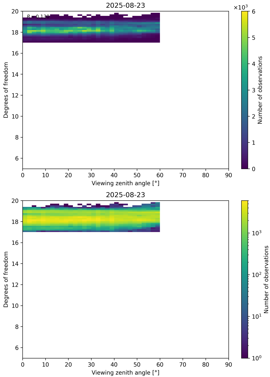
Figure 107: Scatter density plot of “Viewing zenith angle” against “Degrees of freedom” for 2025-08-22 to 2025-08-24.
