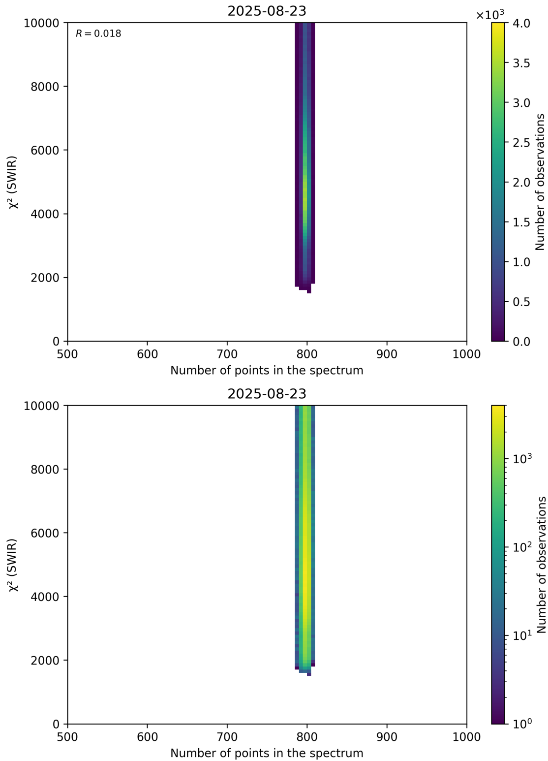
Figure 89: Scatter density plot of “Number of points in the spectrum” against “ \chi^2 (SWIR)” for 2025-08-22 to 2025-08-24.
