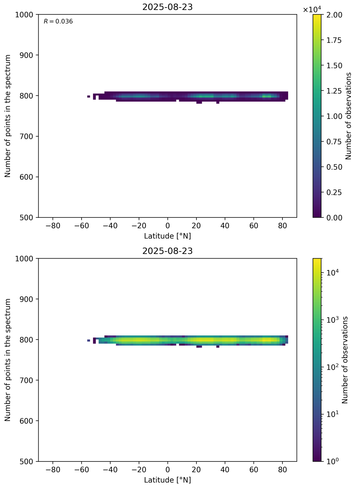
Figure 61: Scatter density plot of “Latitude” against “Number of points in the spectrum” for 2025-08-22 to 2025-08-24.
