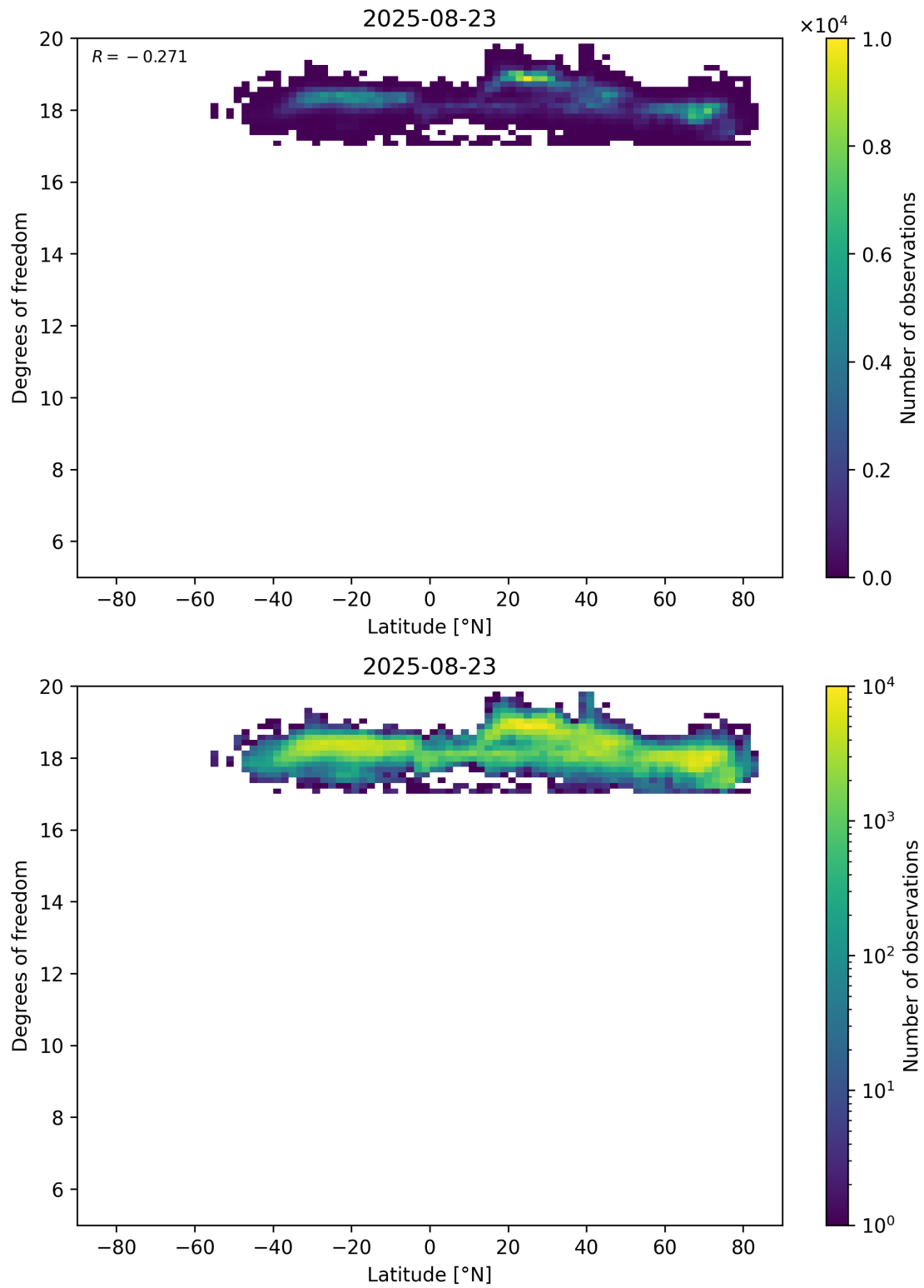
Figure 55: Scatter density plot of “Latitude” against “Degrees of freedom” for 2025-08-22 to 2025-08-24.
