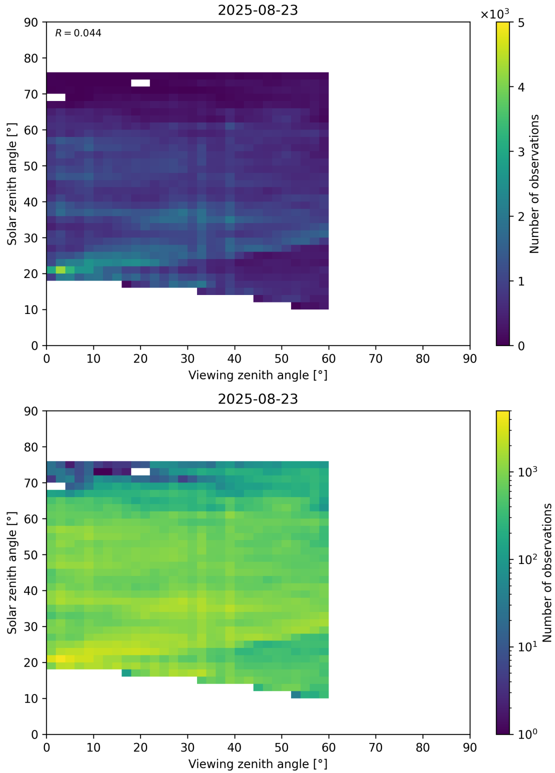
Figure 115: Scatter density plot of “Viewing zenith angle” against “Solar zenith angle” for 2025-08-22 to 2025-08-24.
