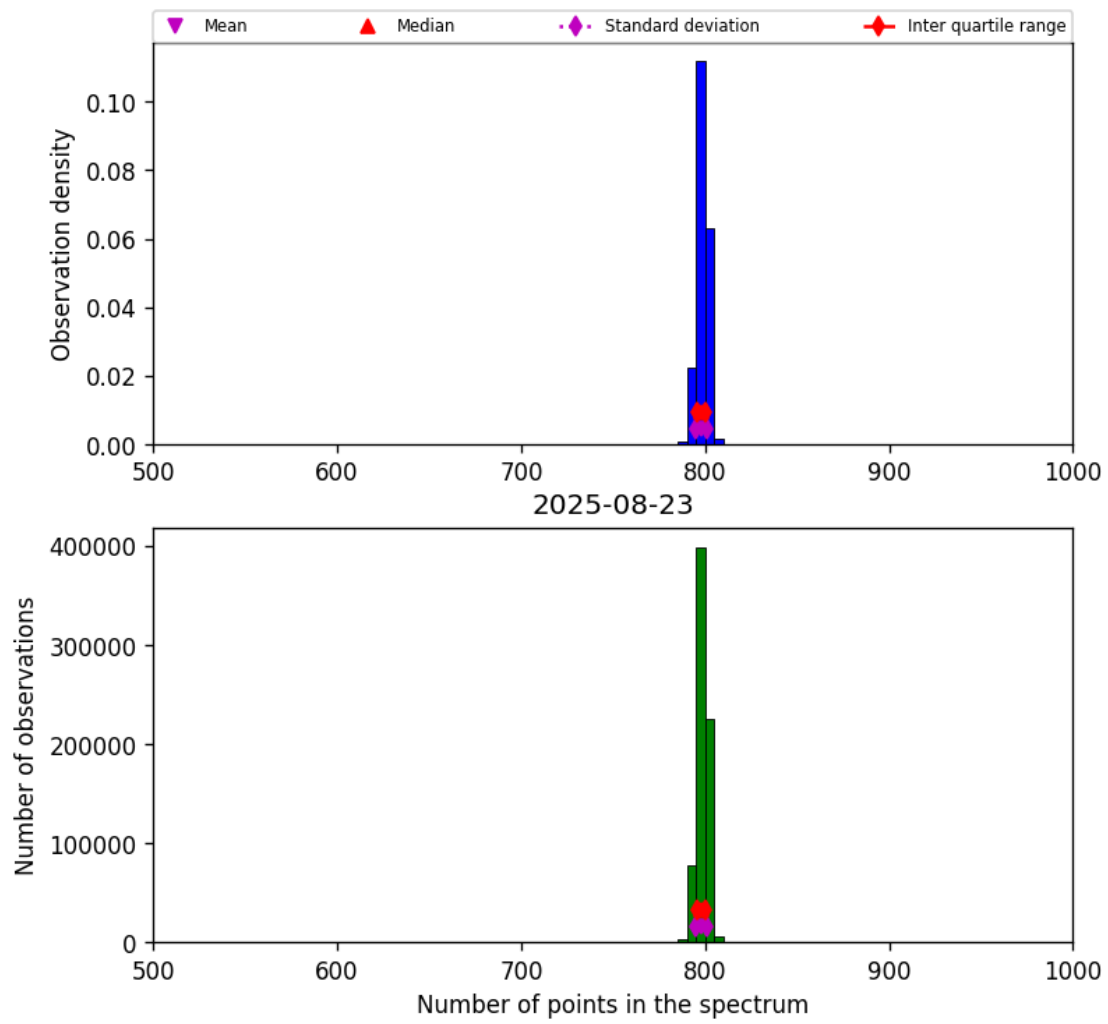
Figure 26: Histogram of “Number of points in the spectrum” for 2025-08-22 to 2025-08-24
