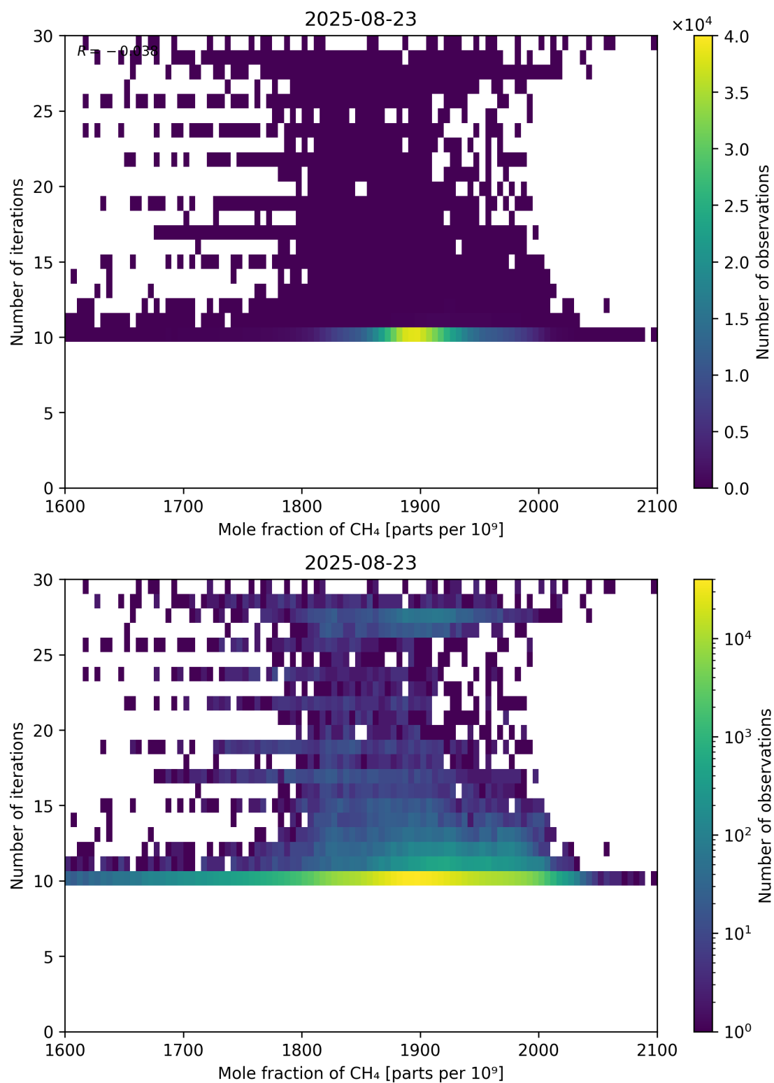
Figure 76: Scatter density plot of “Mole fraction of CH 4 ” against “Number of iterations” for 2025-08-22 to 2025-08-24.
