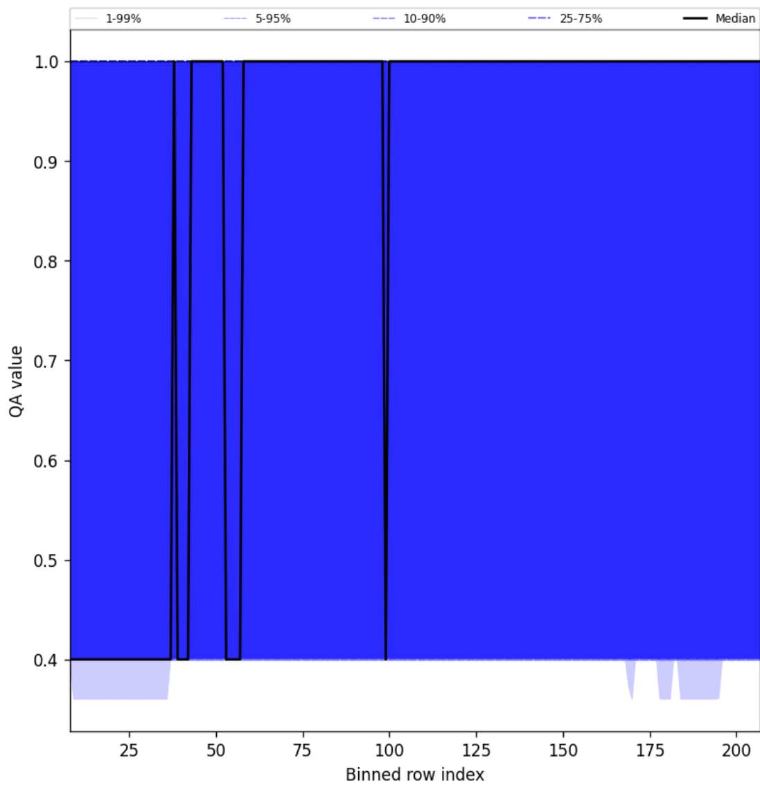
Figure 33: Along track statistics of “QA value” for 2025-08-22 to 2025-08-24
