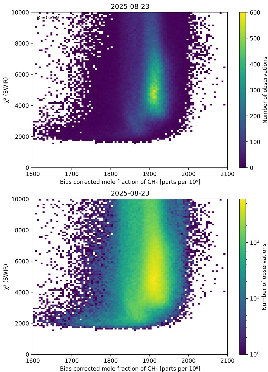
Figure 64: Scatter density plot of “Bias corrected mole fraction of \text{CH}_4 ” against “ \chi^2 (SWIR)” for 2025-08-22 to 2025-08-24.
