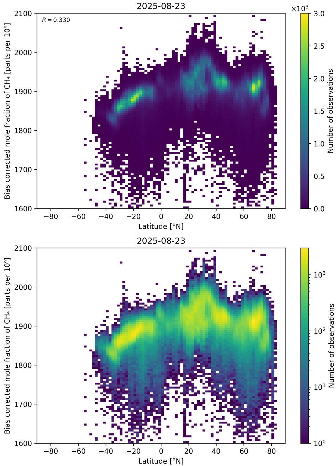
Figure 58: Scatter density plot of “Latitude” against “Bias corrected mole fraction of CH 4 ” for 2025-08-22 to 2025-08-24.
