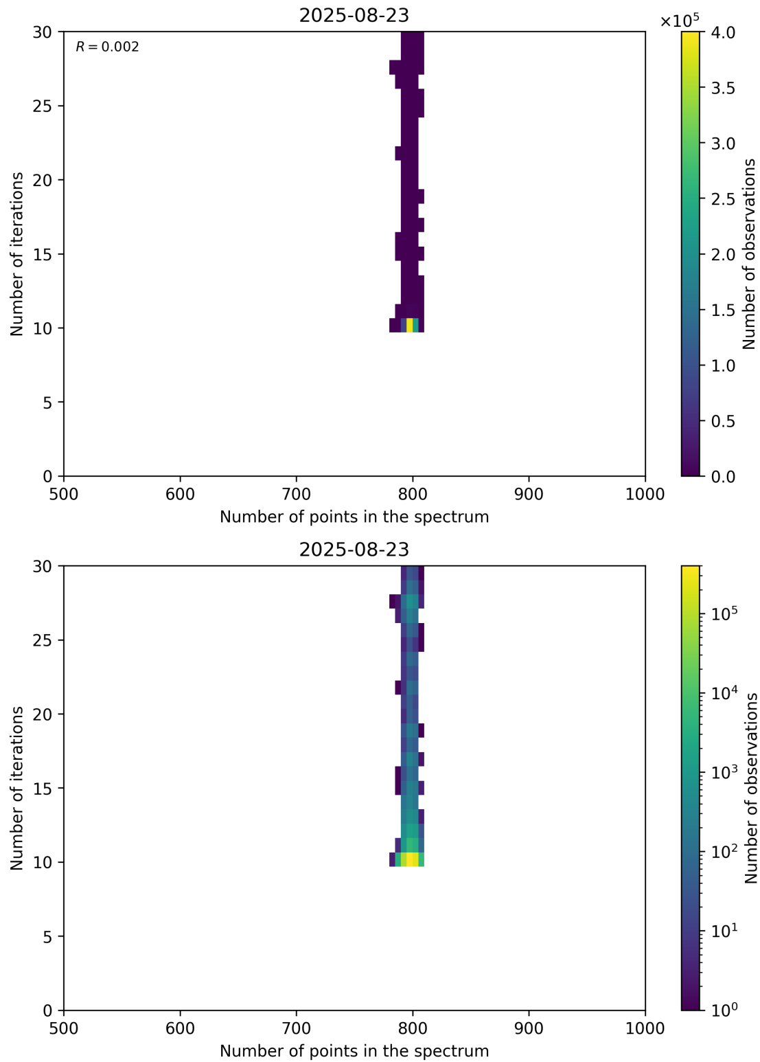
Figure 92: Scatter density plot of “Number of points in the spectrum” against “Number of iterations” for 2025-08-22 to 2025-08-24.
