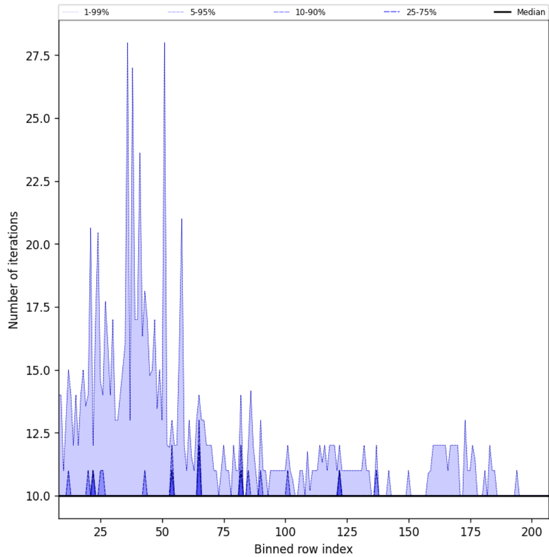
Figure 42: Along track statistics of “Number of iterations” for 2025-08-22 to 2025-08-24
