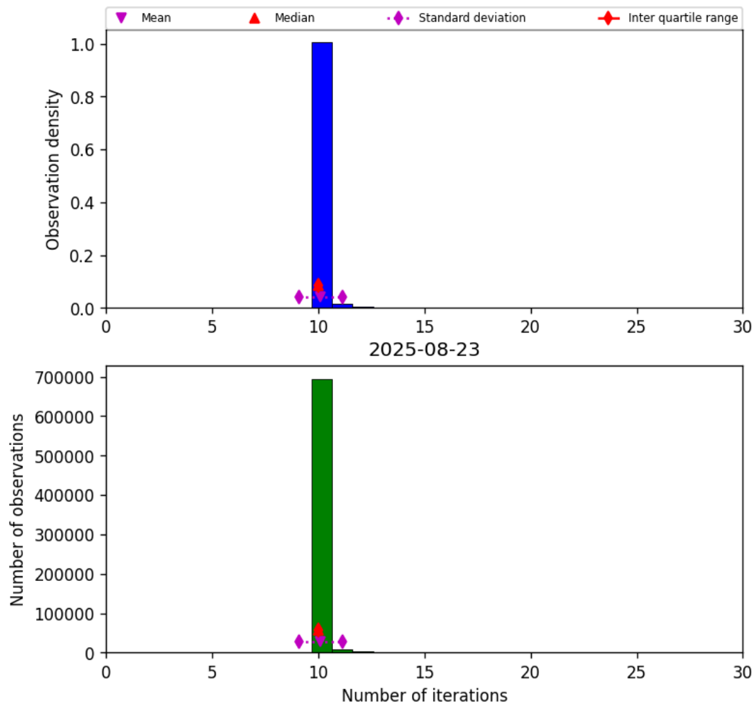
Figure 31: Histogram of “Number of iterations” for 2025-08-22 to 2025-08-24
