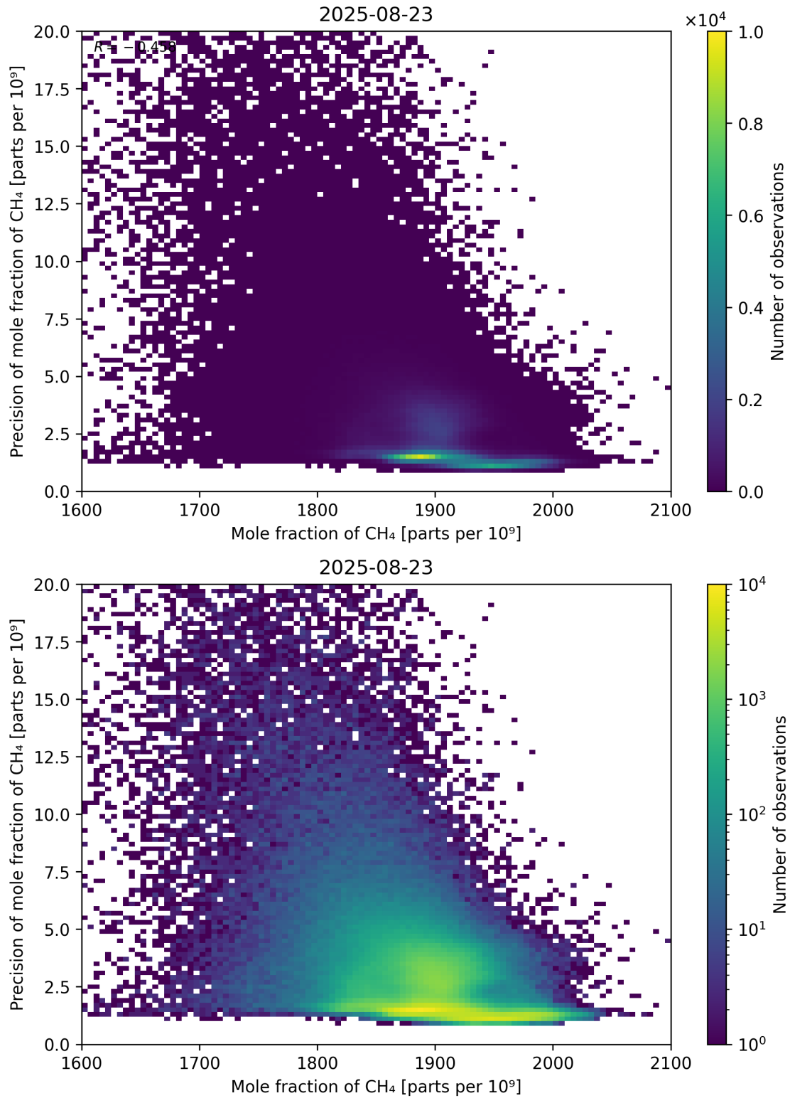
Figure 75: Scatter density plot of “Mole fraction of CH 4 ” against “Precision of mole fraction of CH 4 ” for 2025-08-22 to 2025-08-24.
