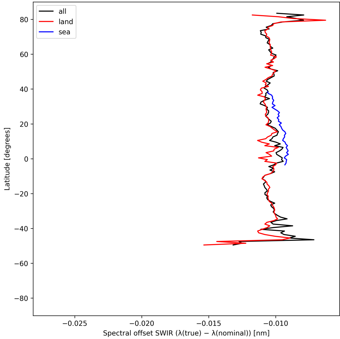
Figure 16: Zonal average of “Spectral offset SWIR ( \lambda_{\text{true}} - \lambda_{\text{nominal}} )” for 2025-08-22 to 2025-08-24.
