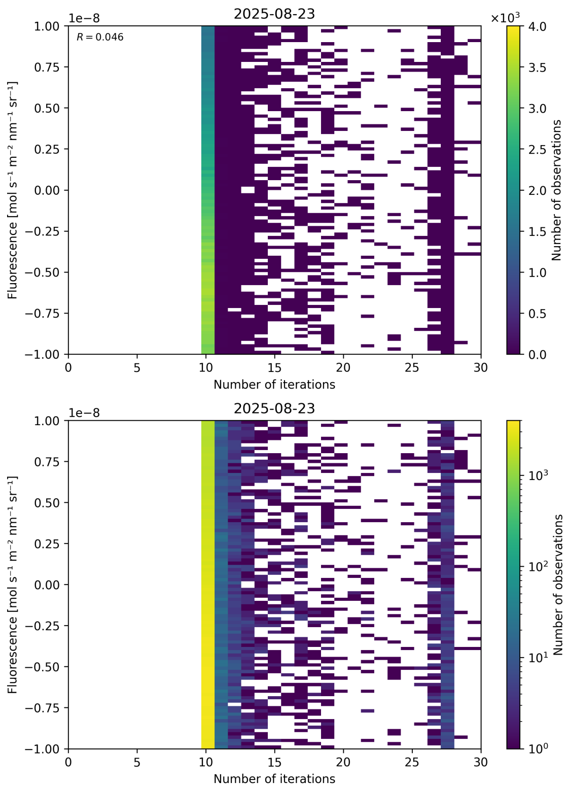
Figure 87: Scatter density plot of “Number of iterations” against “Fluorescence” for 2025-08-22 to 2025-08-24.
