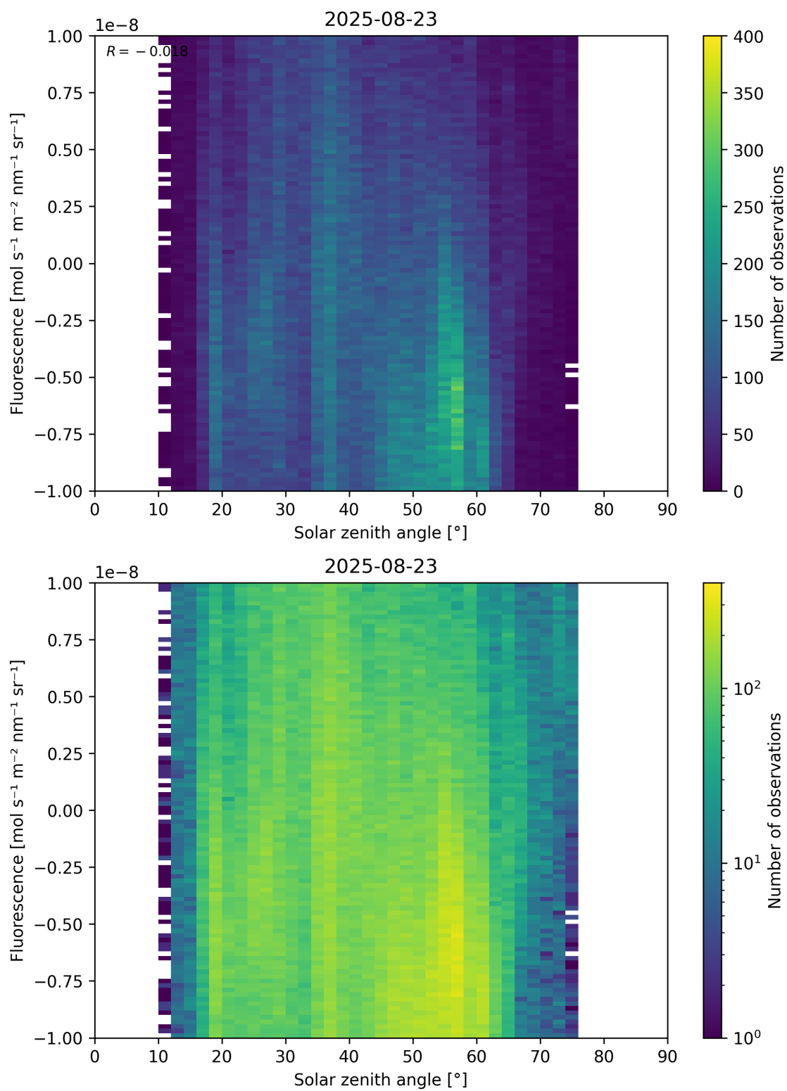
Figure 97: Scatter density plot of “Solar zenith angle” against “Fluorescence” for 2025-08-22 to 2025-08-24.
