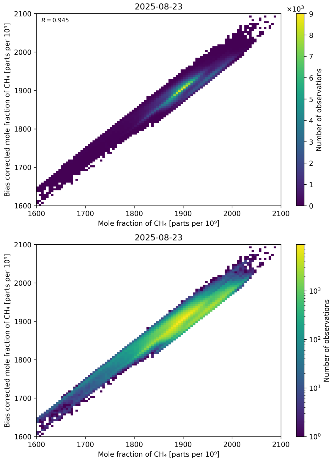
Figure 74: Scatter density plot of “Mole fraction of CH 4 ” against “Bias corrected mole fraction of CH 4 ” for 2025-08-22 to 2025-08-24.
