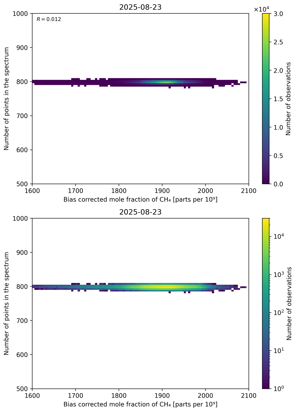
Figure 68: Scatter density plot of “Bias corrected mole fraction of CH 4 ” against “Number of points in the spectrum” for 2025-08-22 to 2025-08-24.
