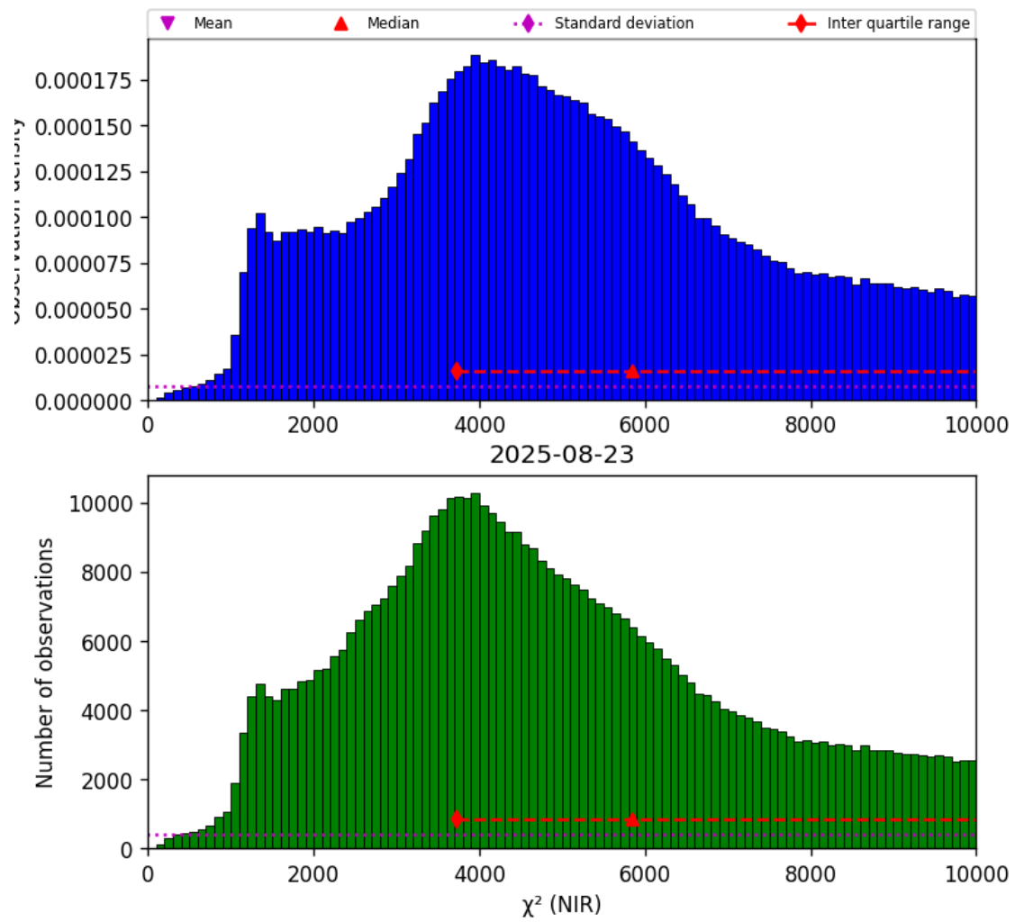
Figure 29: Histogram of “ \chi^2 (NIR)” for 2025-08-22 to 2025-08-24
