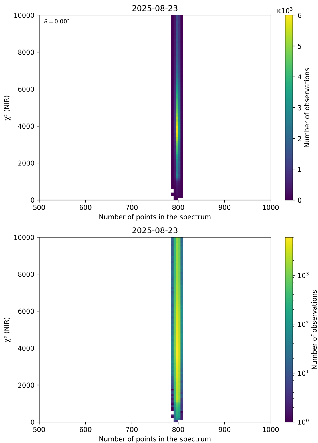
Figure 88: Scatter density plot of “Number of points in the spectrum” against “ \chi^2 (NIR)” for 2025-08-22 to 2025-08-24.
