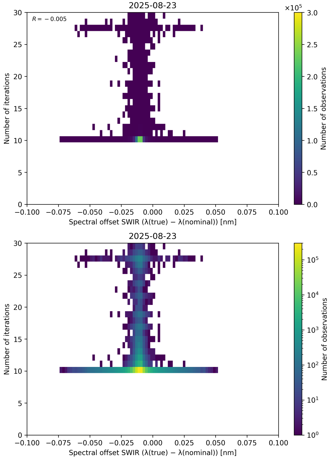
Figure 121: Scatter density plot of “Spectral offset SWIR ( \lambda_{\text{true}} - \lambda_{\text{nominal}} )” against “Number of iterations” for 2025-08-22 to 2025-08-24.
