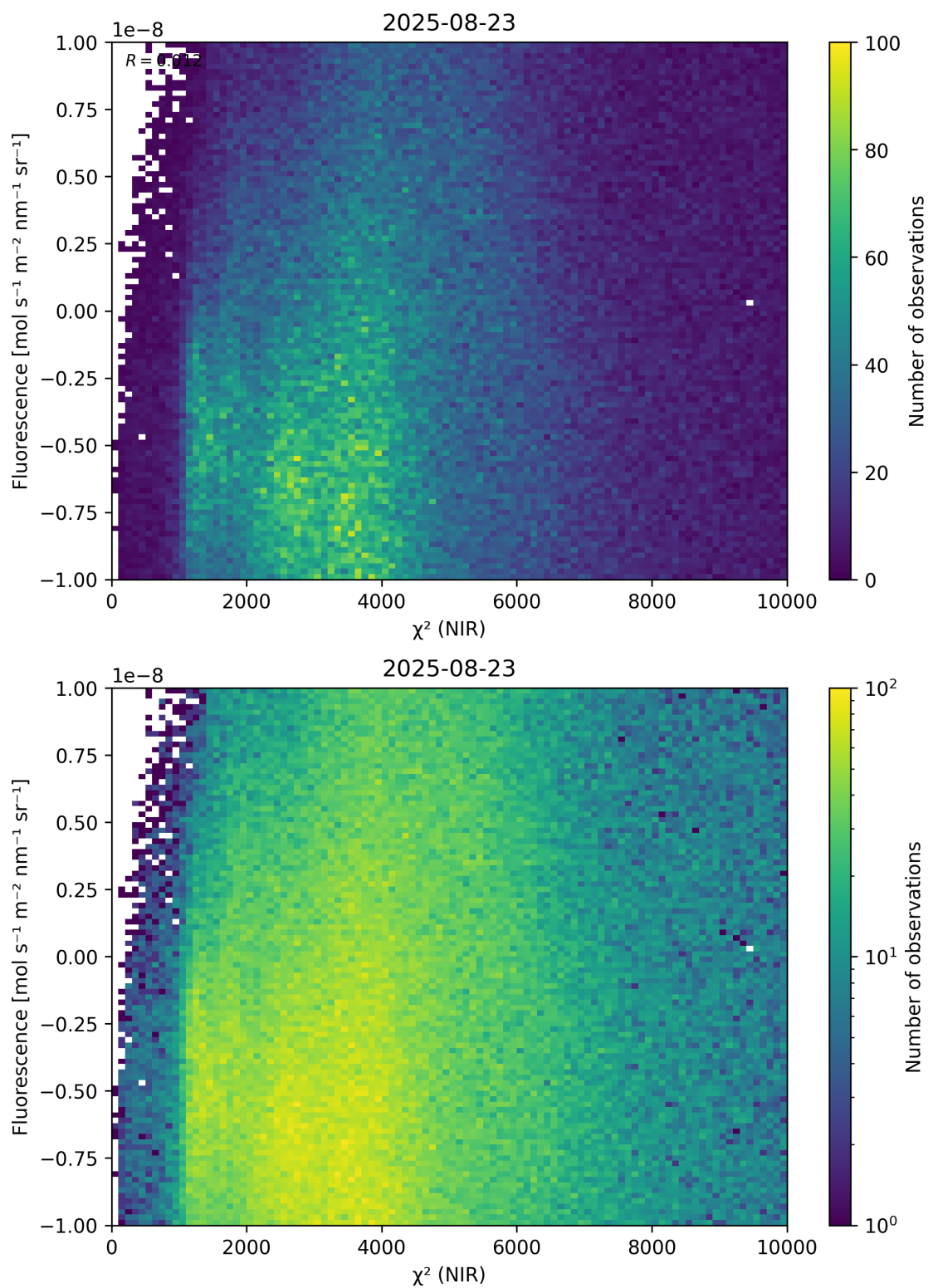
Figure 45: Scatter density plot of “ \chi^2 (NIR)” against “Fluorescence” for 2025-08-22 to 2025-08-24.
