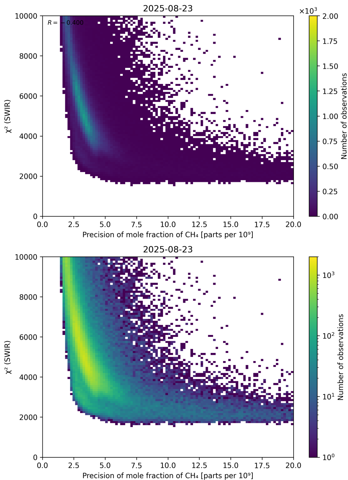
Figure 79: Scatter density plot of “Precision of mole fraction of \text{CH}_4 ” against “ \chi^2 (SWIR)” for 2025-08-22 to 2025-08-24.
