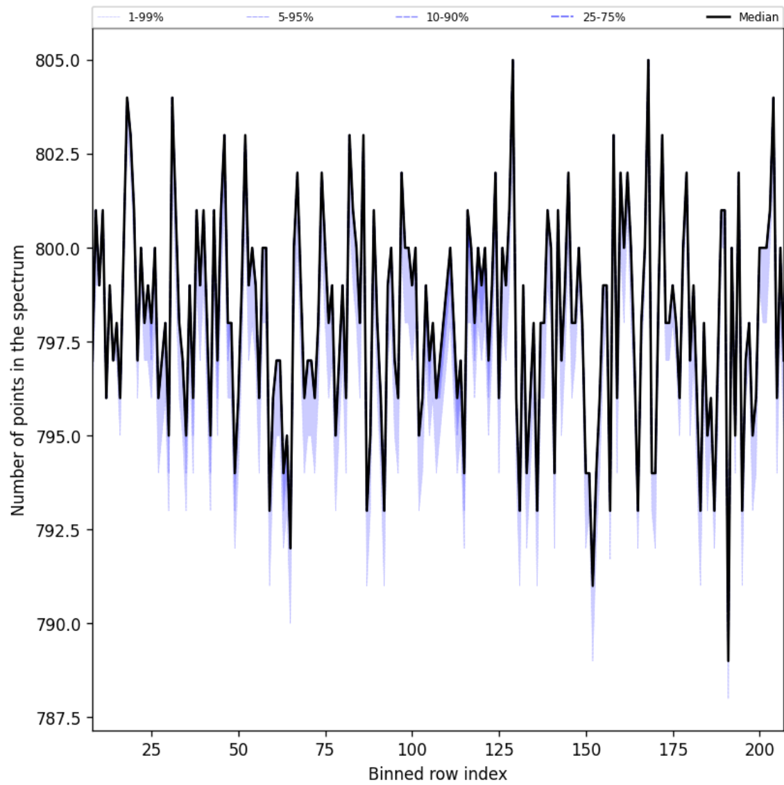
Figure 37: Along track statistics of “Number of points in the spectrum” for 2025-08-22 to 2025-08-24
