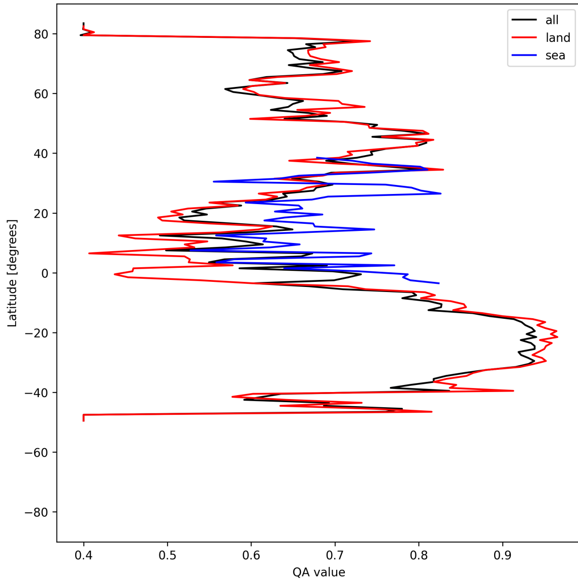
Figure 11: Zonal average of “QA value” for 2025-08-22 to 2025-08-24.
