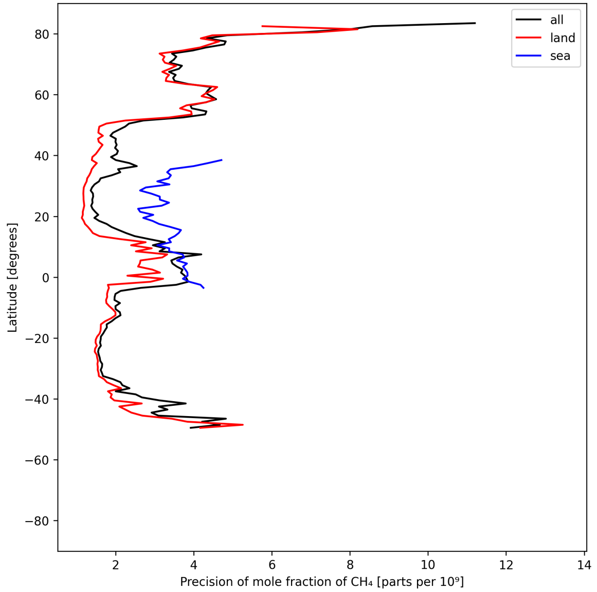
Figure 13: Zonal average of “Precision of mole fraction of CH 4 ” for 2025-08-22 to 2025-08-24.
