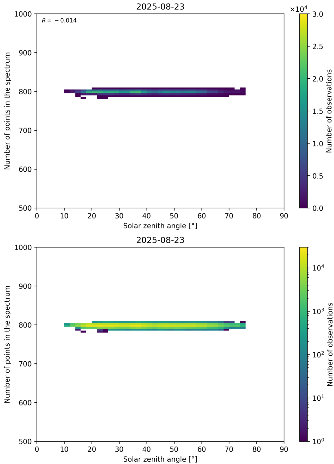
Figure 103: Scatter density plot of “Solar zenith angle” against “Number of points in the spectrum” for 2025-08-22 to 2025-08-24.
