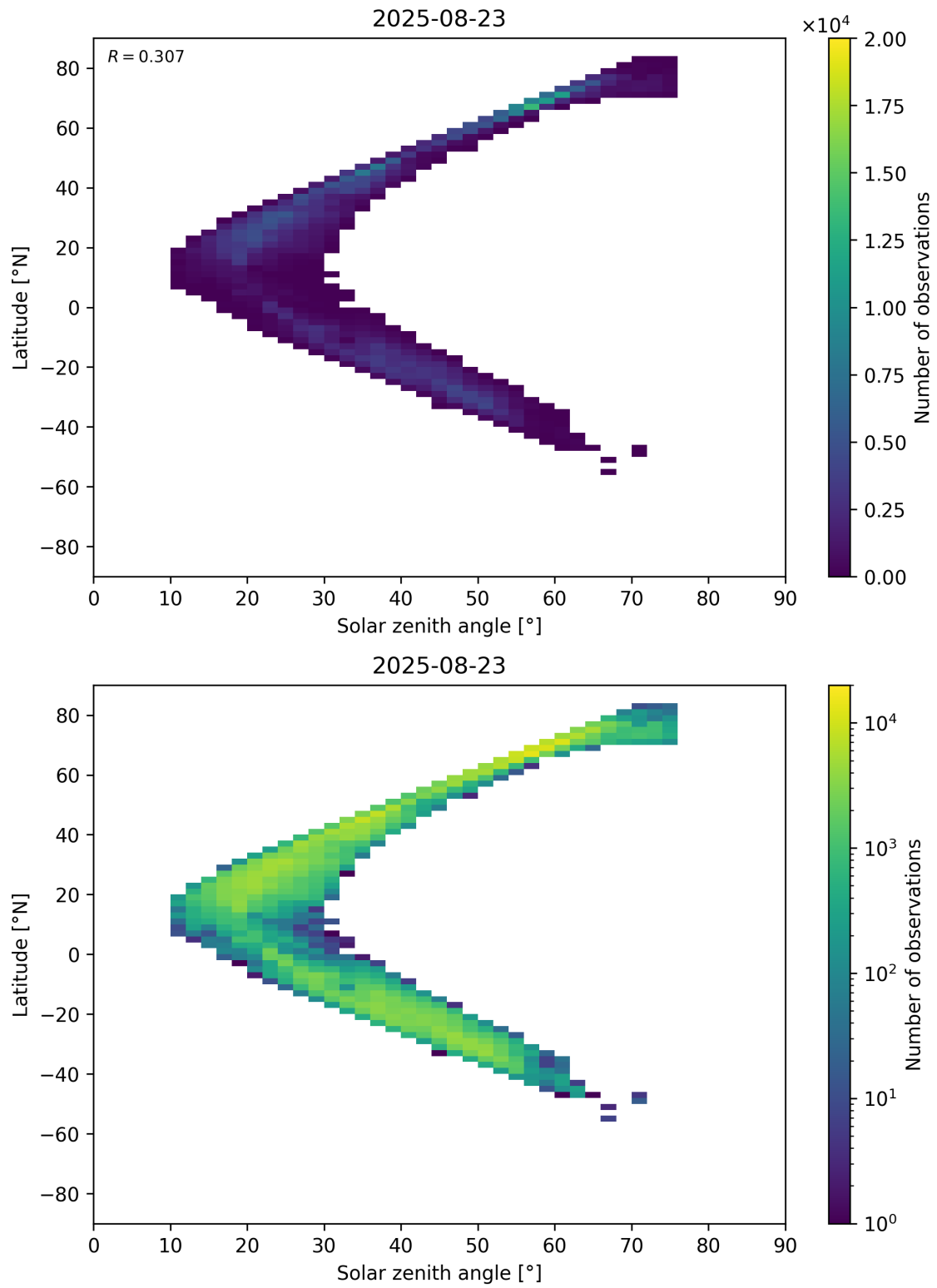
Figure 98: Scatter density plot of “Solar zenith angle” against “Latitude” for 2025-08-22 to 2025-08-24.
