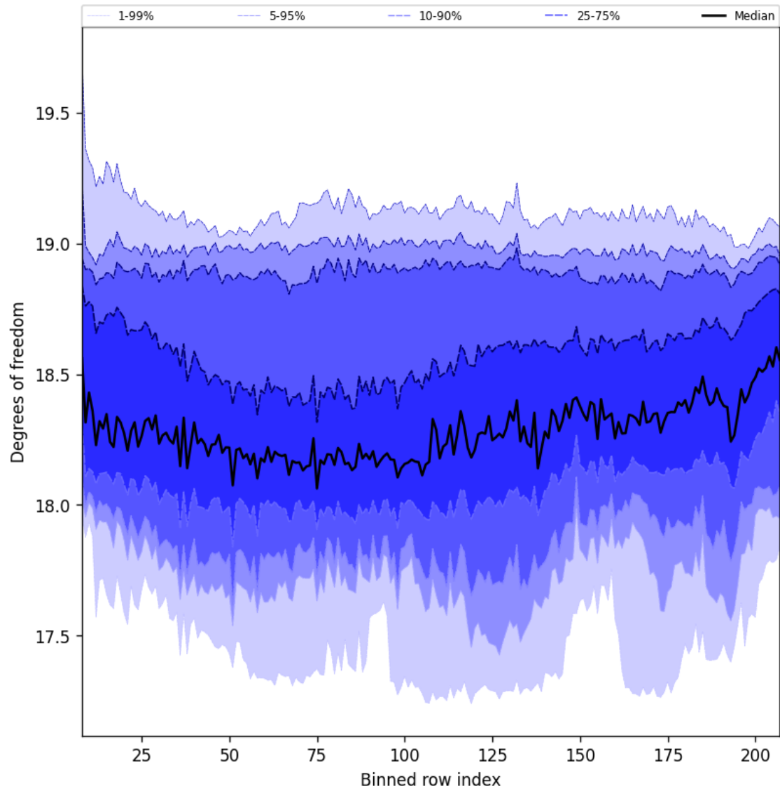
Figure 41: Along track statistics of “Degrees of freedom” for 2025-08-22 to 2025-08-24
