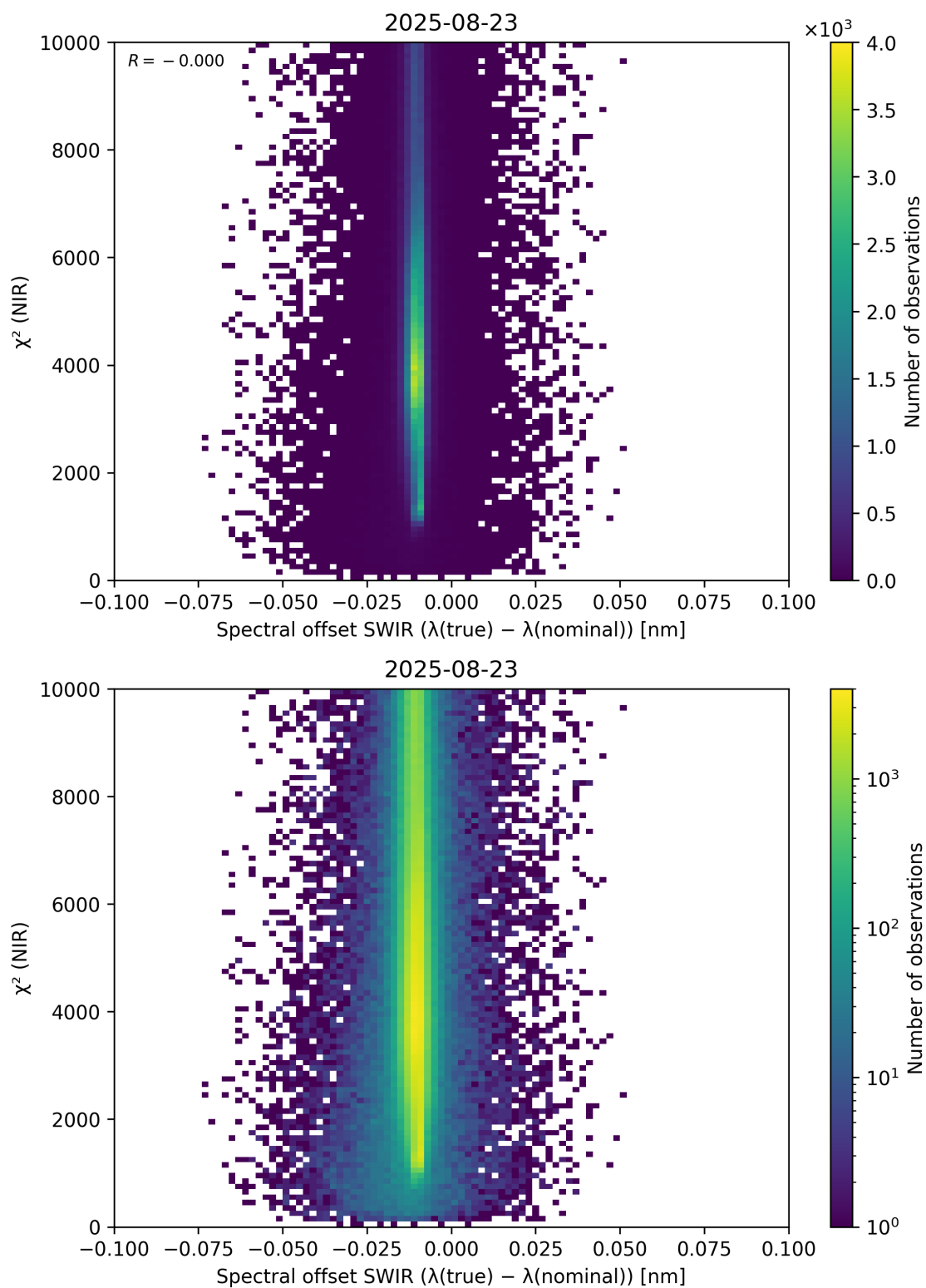
Figure 117: Scatter density plot of “Spectral offset SWIR ( \lambda_{\text{true}} - \lambda_{\text{nominal}} )” against “ \chi^2 (NIR)” for 2025-08-22 to 2025-08-24.
