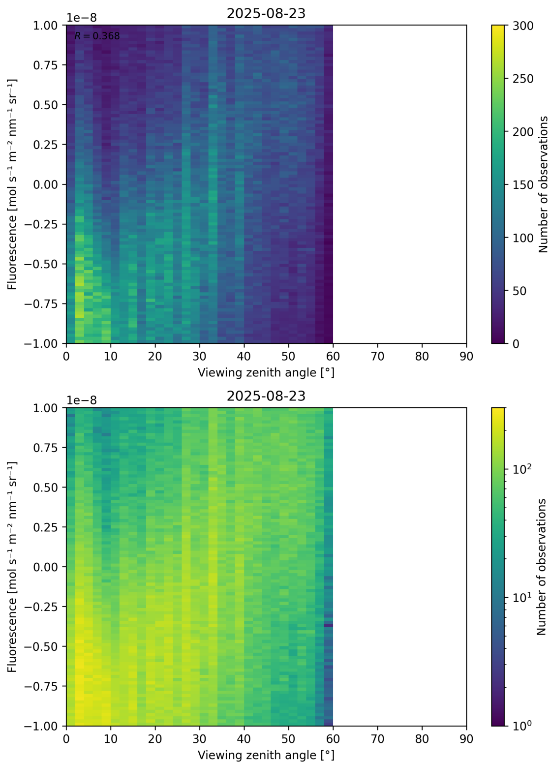
Figure 108: Scatter density plot of “Viewing zenith angle” against “Fluorescence” for 2025-08-22 to 2025-08-24.
