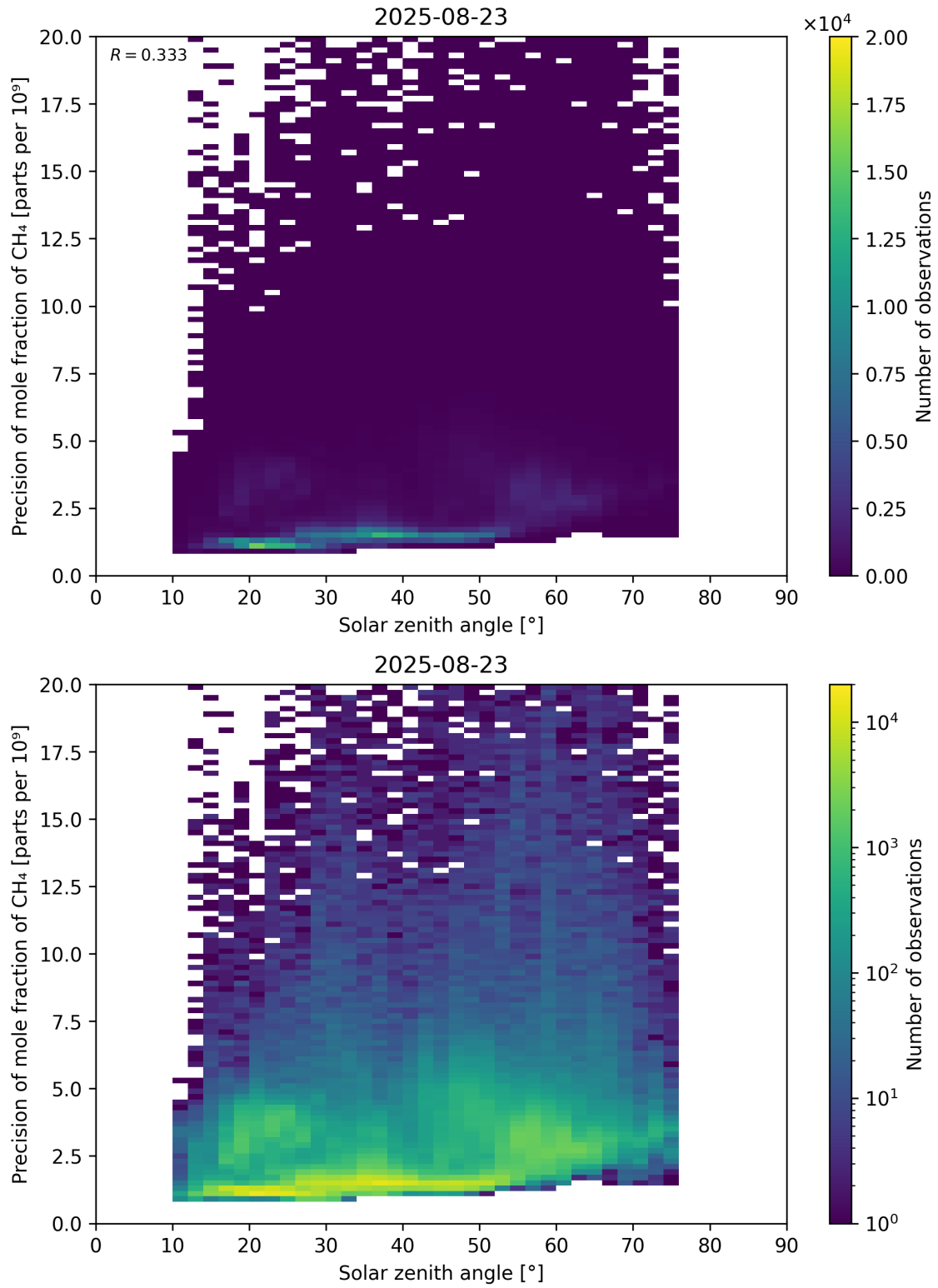
Figure 101: Scatter density plot of “Solar zenith angle” against “Precision of mole fraction of CH 4 ” for 2025-08-22 to 2025-08-24.
