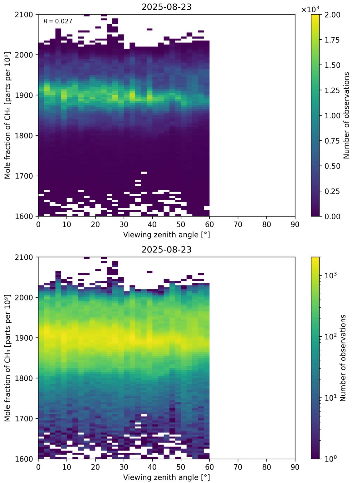
Figure 110: Scatter density plot of “Viewing zenith angle” against “Mole fraction of CH 4 ” for 2025-08-22 to 2025-08-24.
