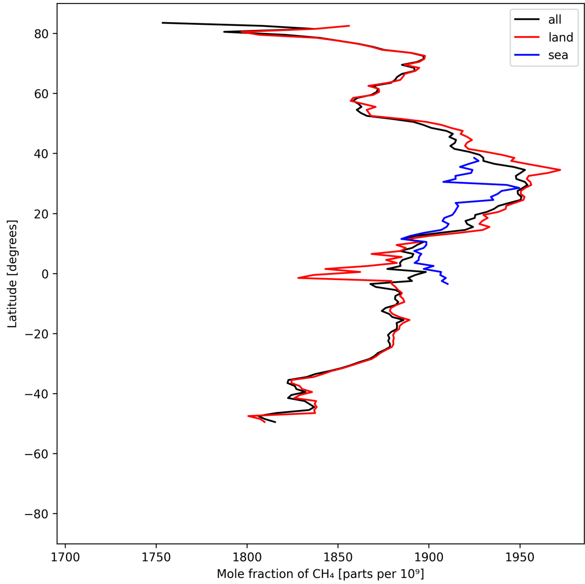
Figure 12: Zonal average of “Mole fraction of \text{CH}_4 ” for 2025-08-22 to 2025-08-24.
