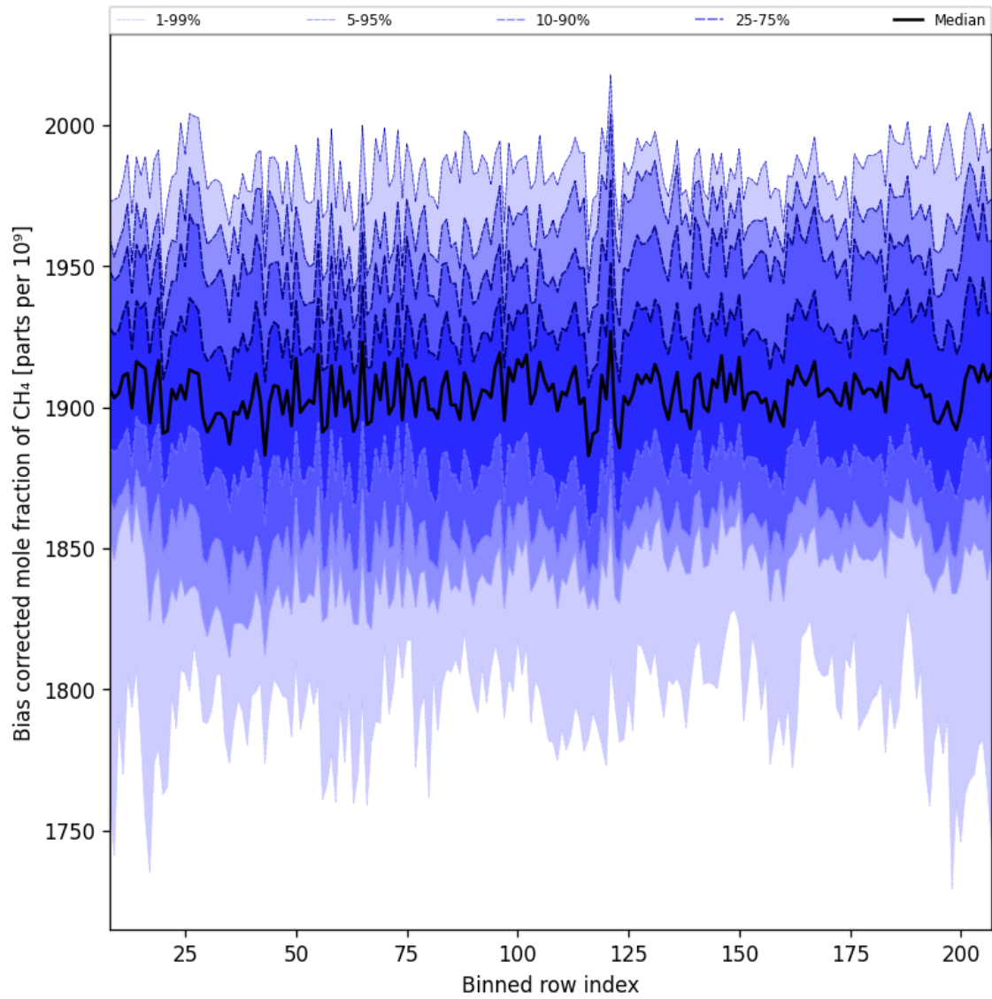
Figure 36: Along track statistics of “Bias corrected mole fraction of \text{CH}_4 ” for 2025-08-22 to 2025-08-24
