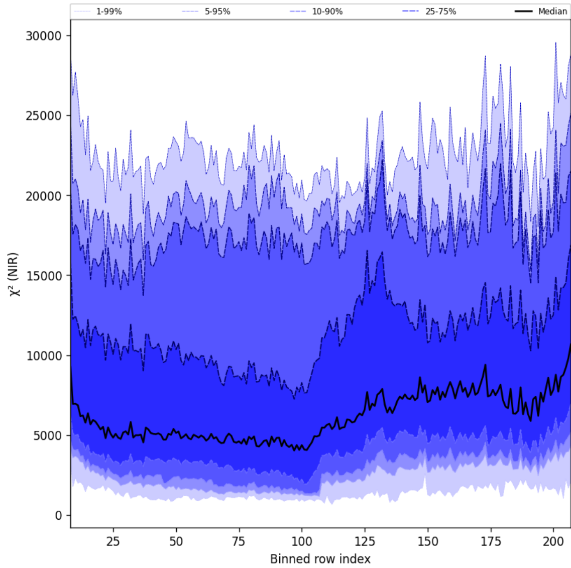
Figure 40: Along track statistics of “ \chi^2 (NIR)” for 2025-08-22 to 2025-08-24
