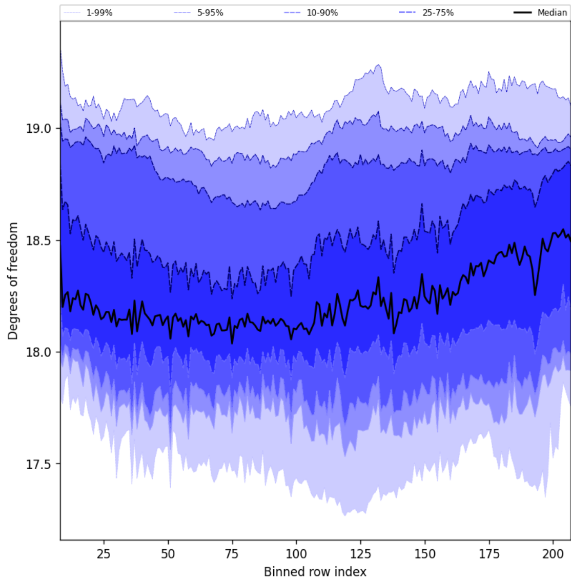
Figure 41: Along track statistics of “Degrees of freedom” for 2025-08-23 to 2025-08-25
