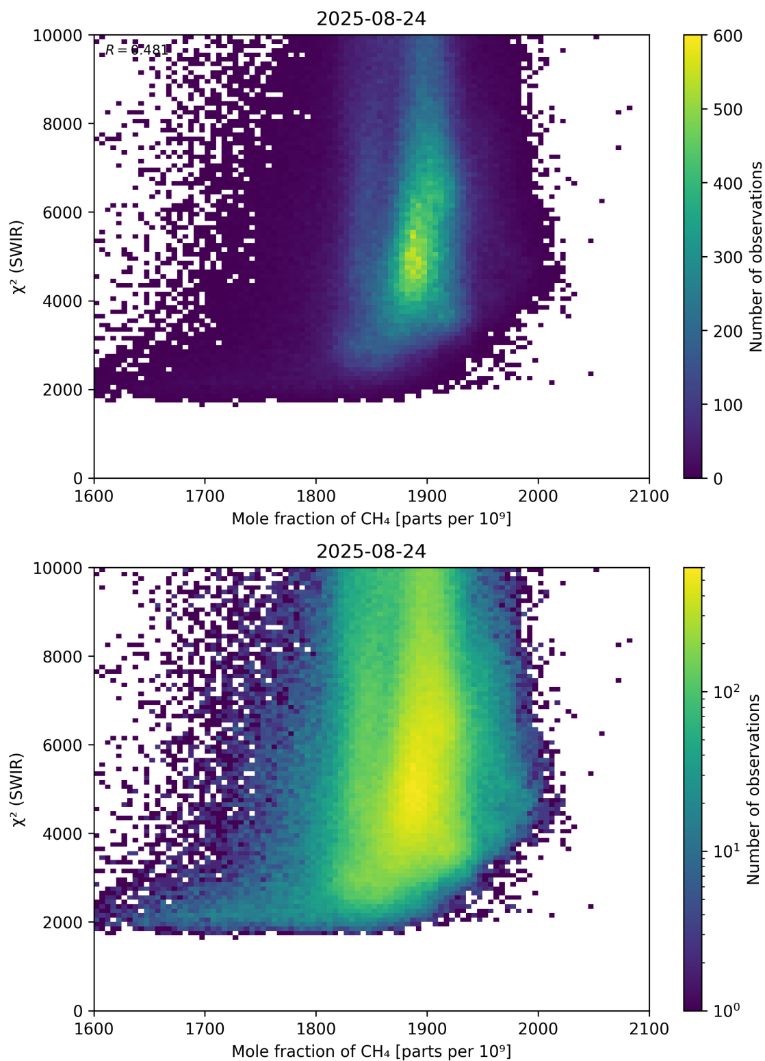
Figure 71: Scatter density plot of “Mole fraction of \text{CH}_4 ” against “ \chi^2 (SWIR)” for 2025-08-23 to 2025-08-25.
