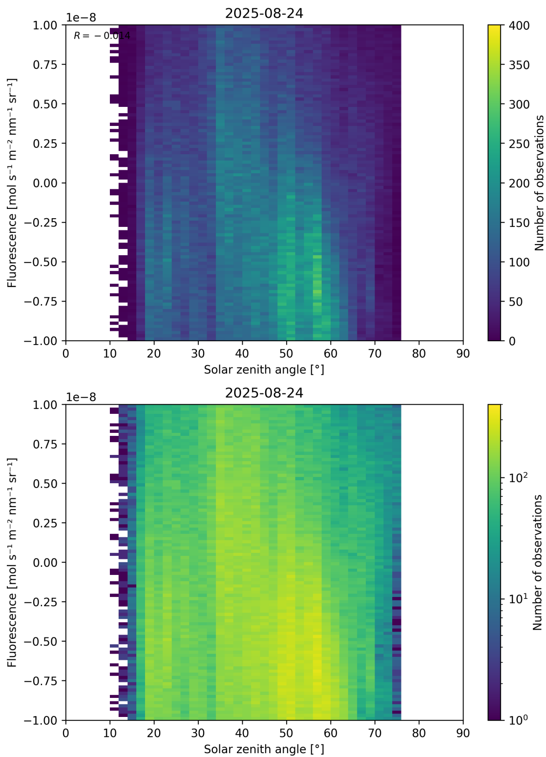
Figure 97: Scatter density plot of “Solar zenith angle” against “Fluorescence” for 2025-08-23 to 2025-08-25.
