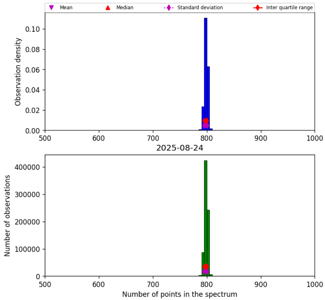
Figure 26: Histogram of “Number of points in the spectrum” for 2025-08-23 to 2025-08-25
