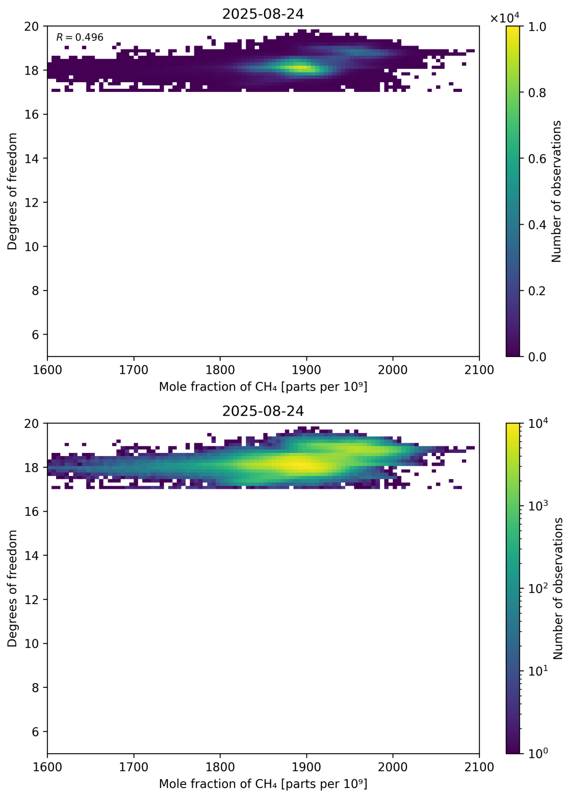
Figure 72: Scatter density plot of “Mole fraction of CH 4 ” against “Degrees of freedom” for 2025-08-23 to 2025-08-25.
