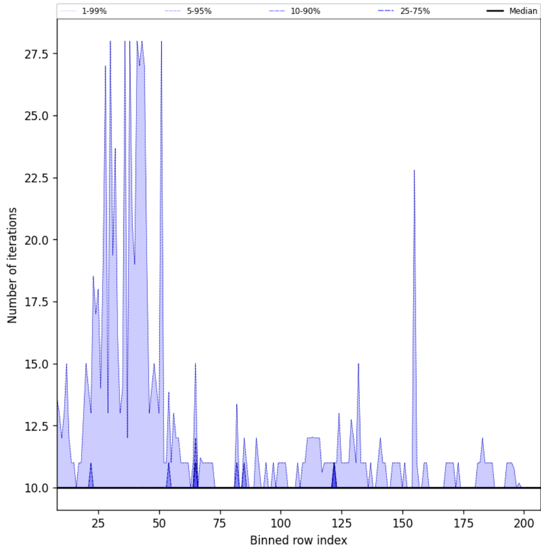
Figure 42: Along track statistics of “Number of iterations” for 2025-08-23 to 2025-08-25
