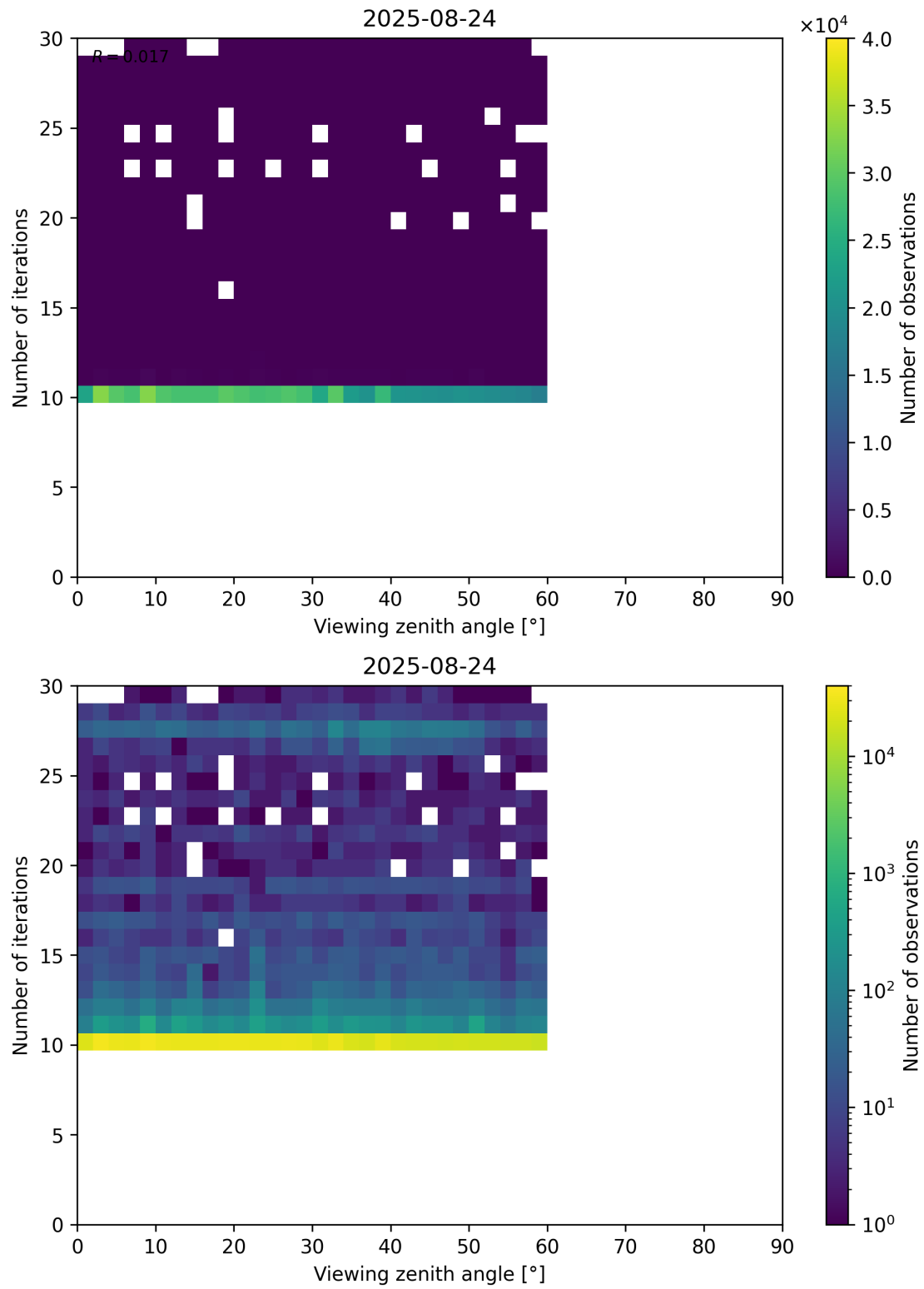
Figure 113: Scatter density plot of “Viewing zenith angle” against “Number of iterations” for 2025-08-23 to 2025-08-25.
