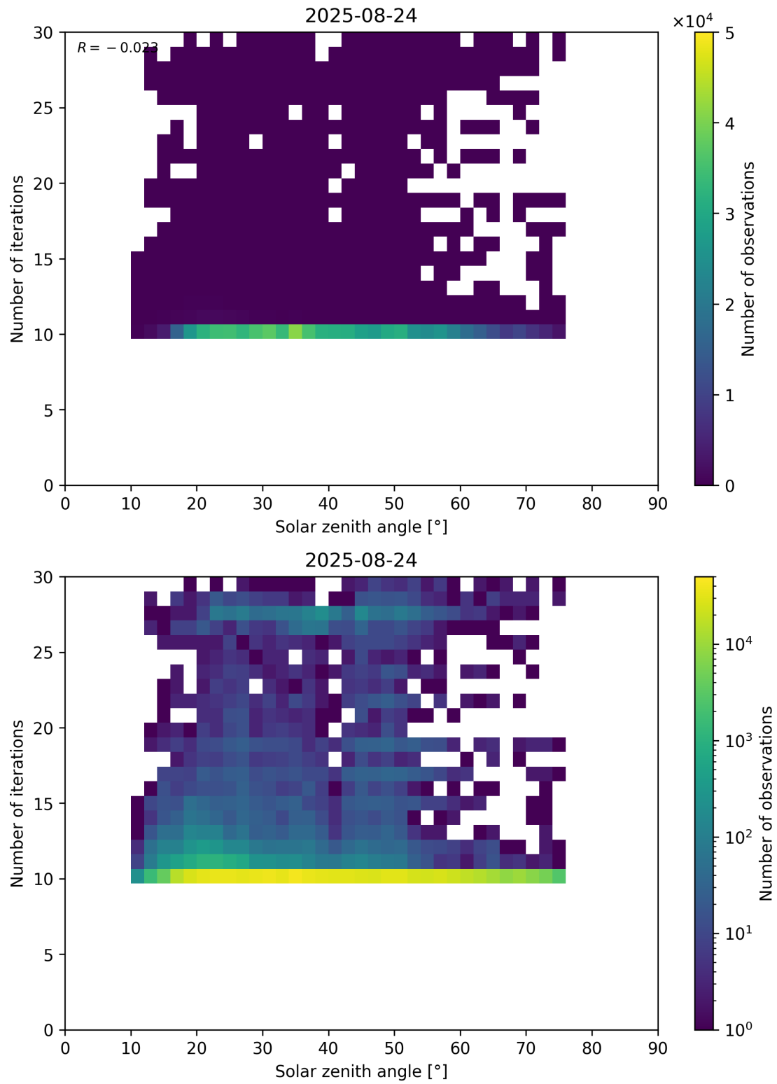
Figure 102: Scatter density plot of “Solar zenith angle” against “Number of iterations” for 2025-08-23 to 2025-08-25.
