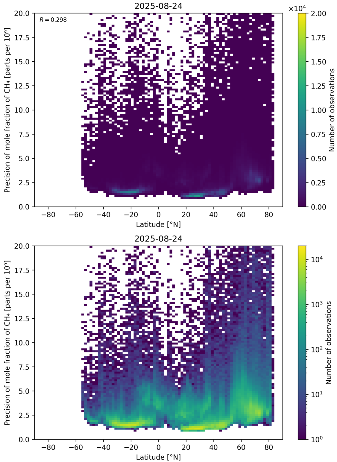
Figure 59: Scatter density plot of “Latitude” against “Precision of mole fraction of \text{CH}_4 ” for 2025-08-23 to 2025-08-25.
