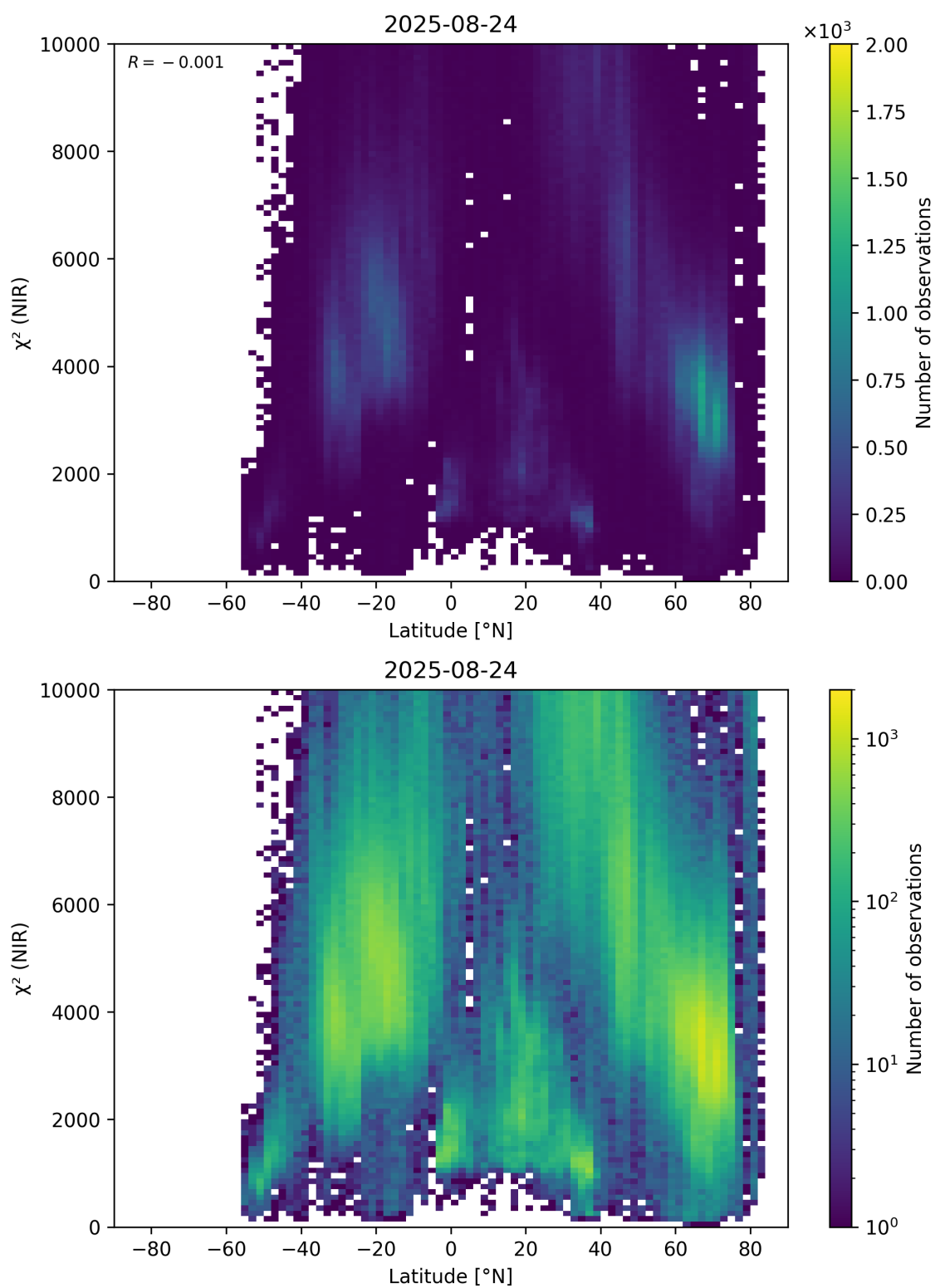
Figure 53: Scatter density plot of “Latitude” against “ \chi^2 (NIR)” for 2025-08-23 to 2025-08-25.
