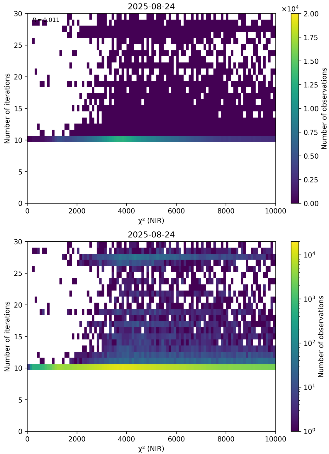
Figure 46: Scatter density plot of “ \chi^2 (NIR)” against “Number of iterations” for 2025-08-23 to 2025-08-25.
