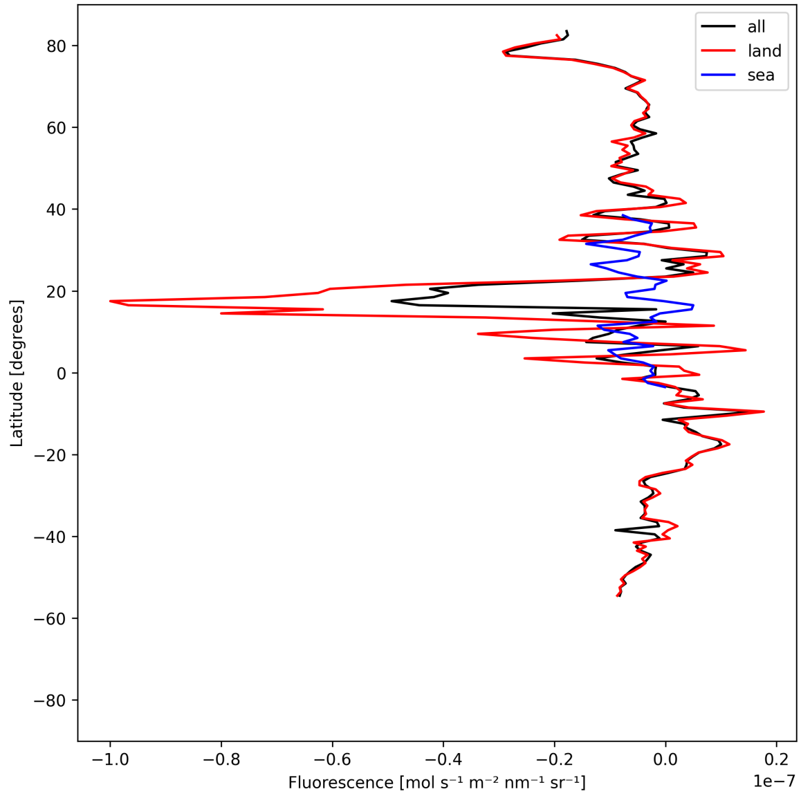
Figure 21: Zonal average of “Fluorescence” for 2025-08-23 to 2025-08-25.
