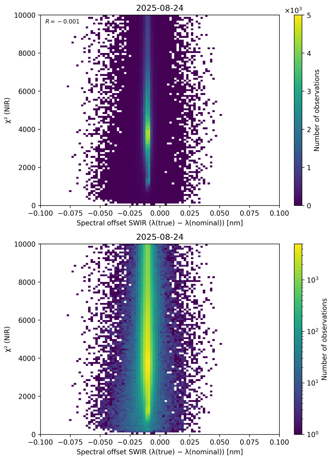
Figure 117: Scatter density plot of “Spectral offset SWIR ( \lambda_{\text{true}} - \lambda_{\text{nominal}} )” against “ \chi^2 (NIR)” for 2025-08-23 to 2025-08-25.
