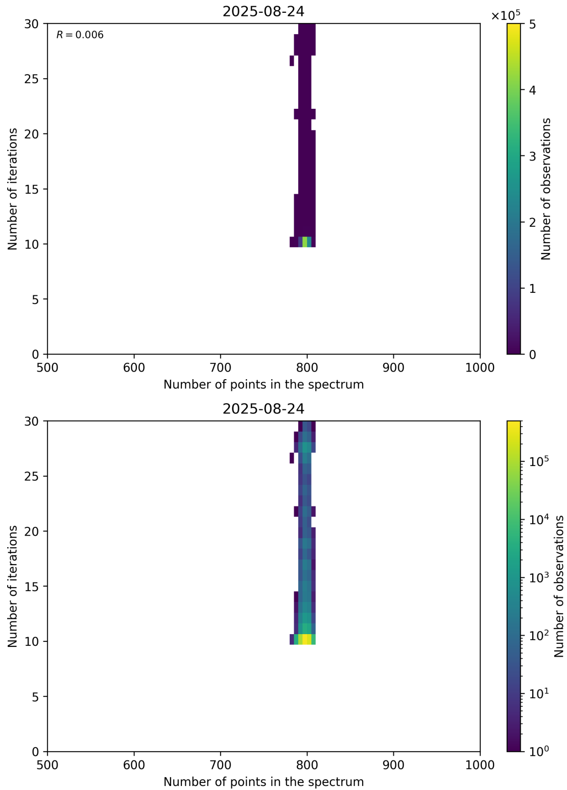
Figure 92: Scatter density plot of “Number of points in the spectrum” against “Number of iterations” for 2025-08-23 to 2025-08-25.
