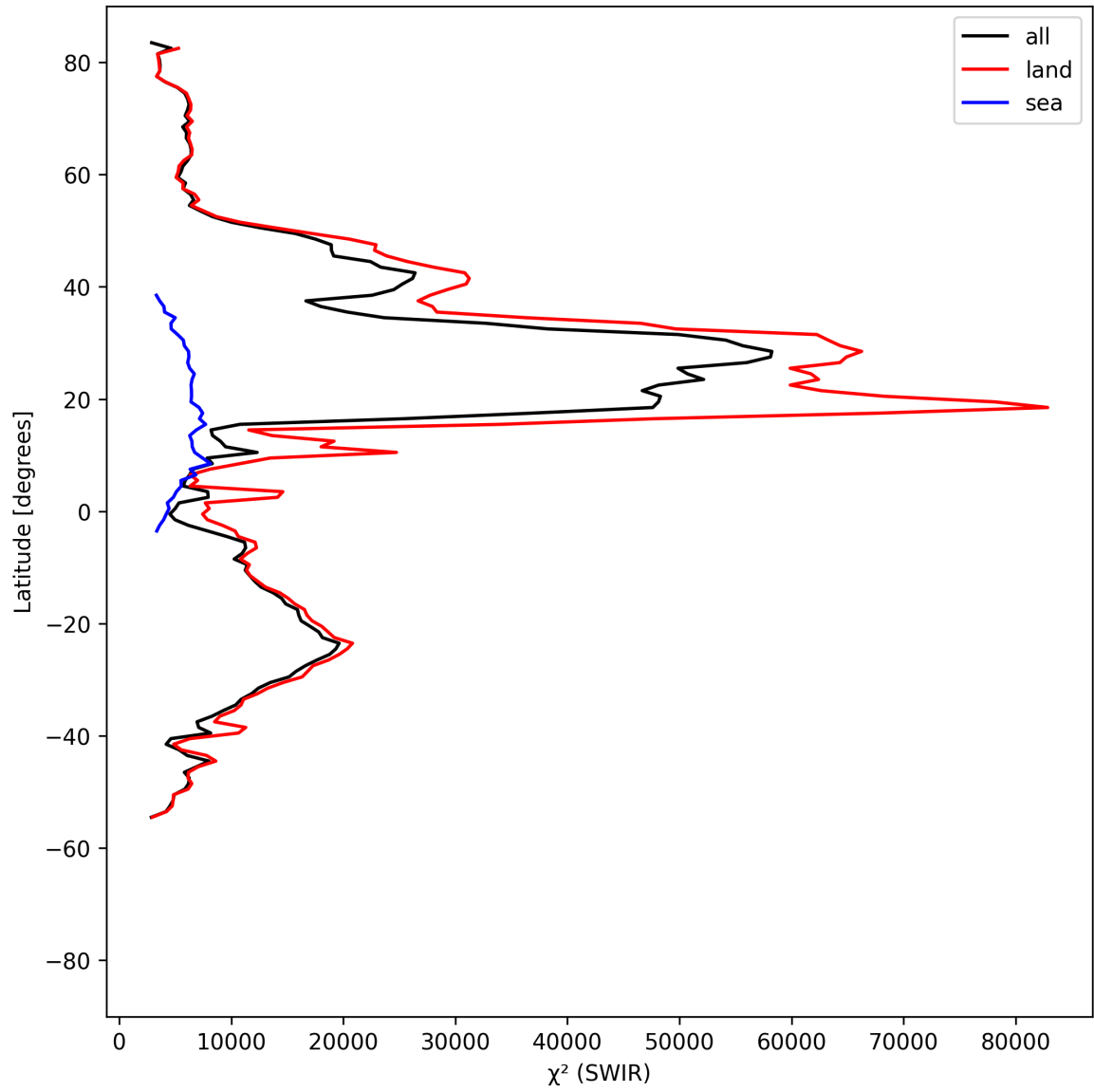
Figure 17: Zonal average of “ \chi^2 (SWIR)” for 2025-08-23 to 2025-08-25.
