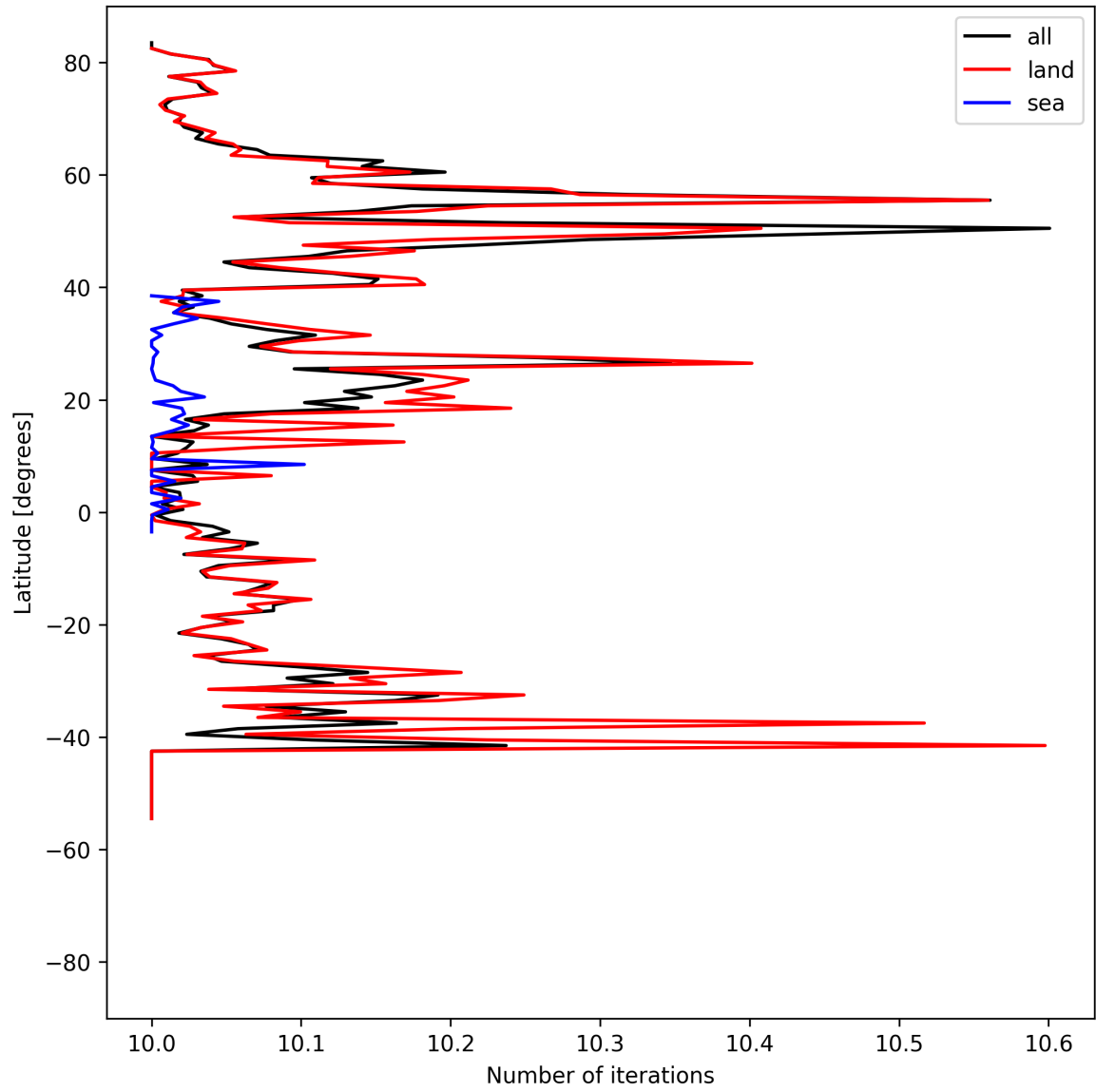
Figure 20: Zonal average of “Number of iterations” for 2025-08-23 to 2025-08-25.
