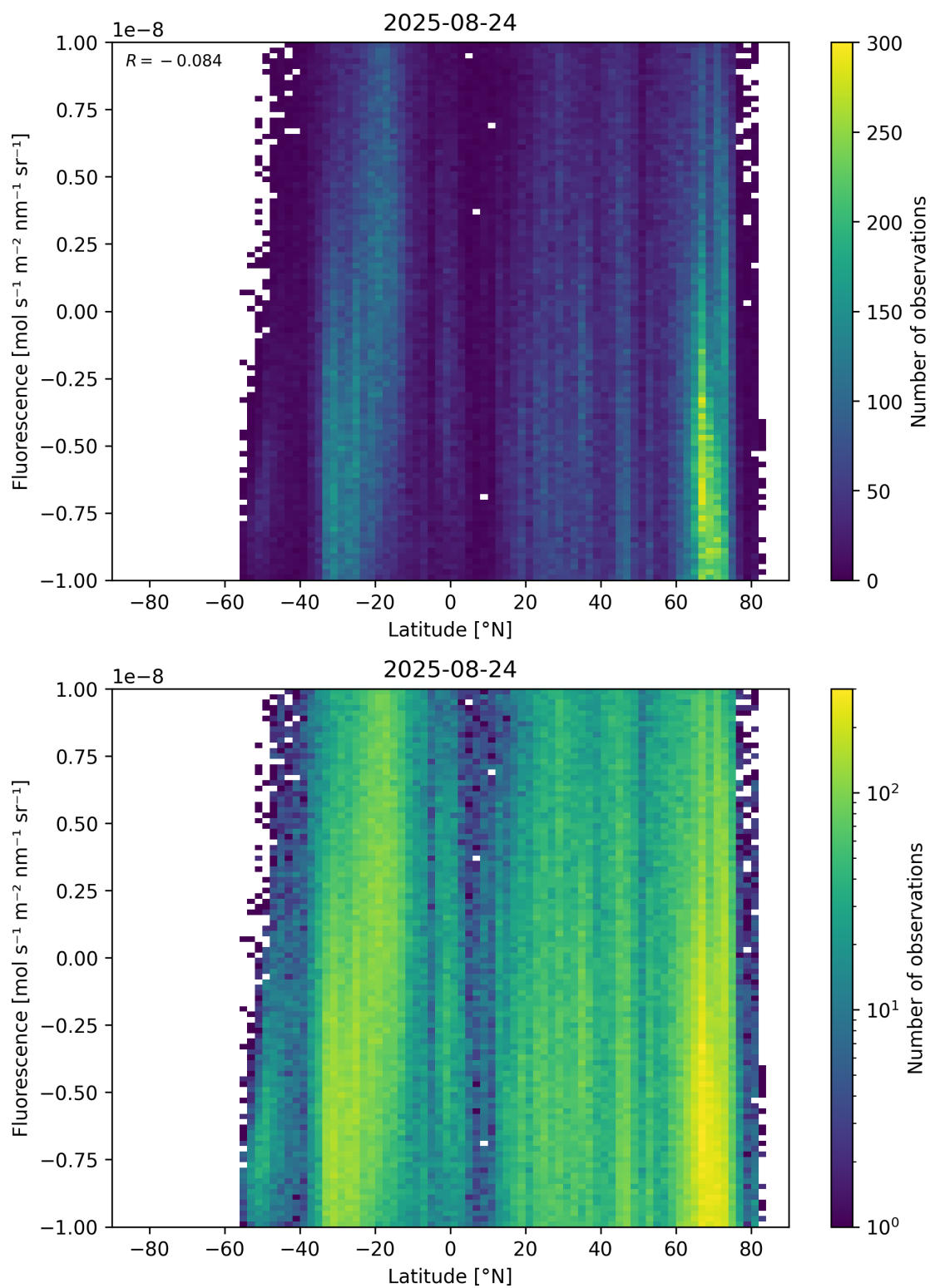
Figure 56: Scatter density plot of “Latitude” against “Fluorescence” for 2025-08-23 to 2025-08-25.
