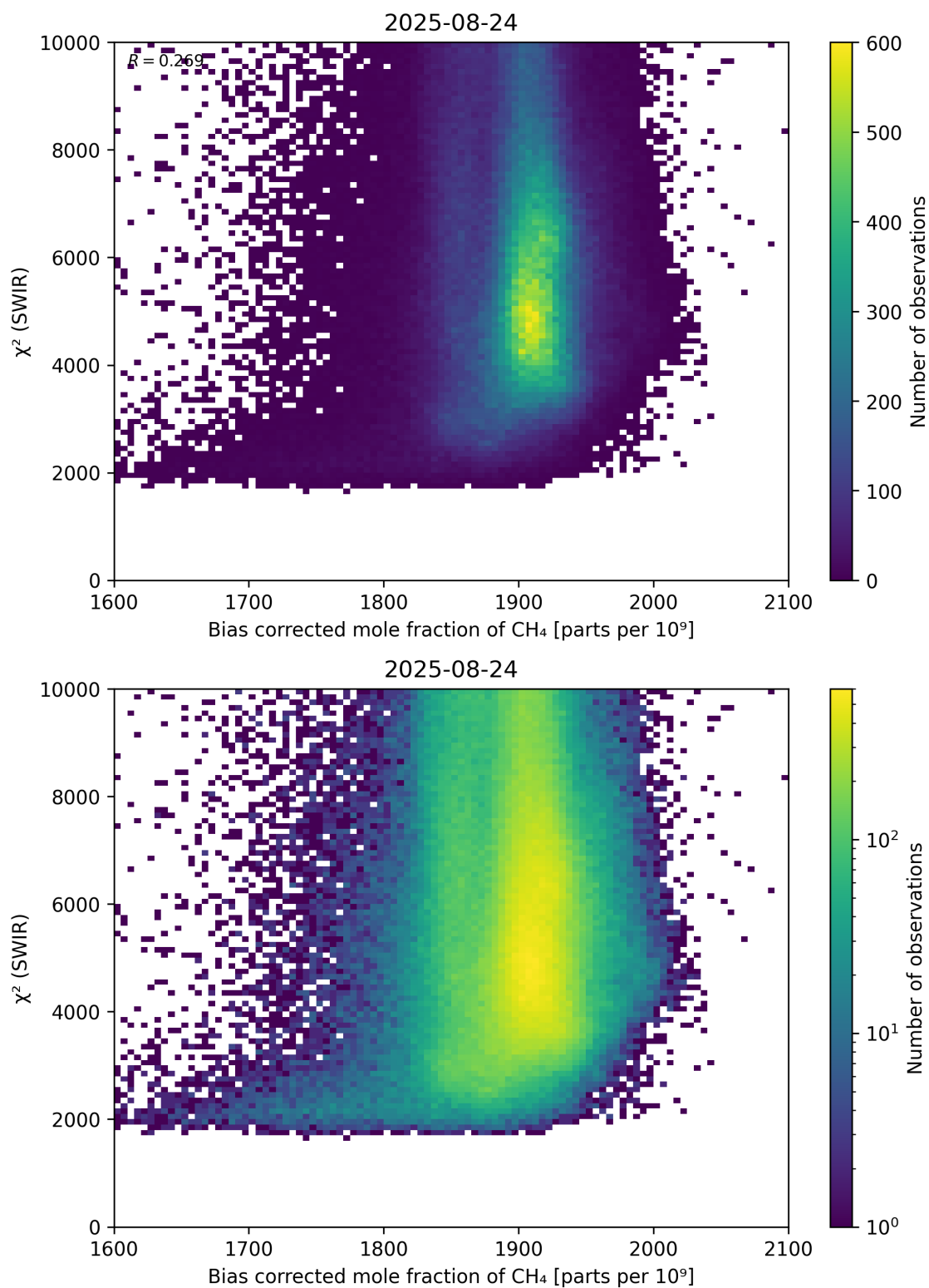
Figure 64: Scatter density plot of “Bias corrected mole fraction of CH 4 ” against “ \chi^2 (SWIR)” for 2025-08-23 to 2025-08-25.
