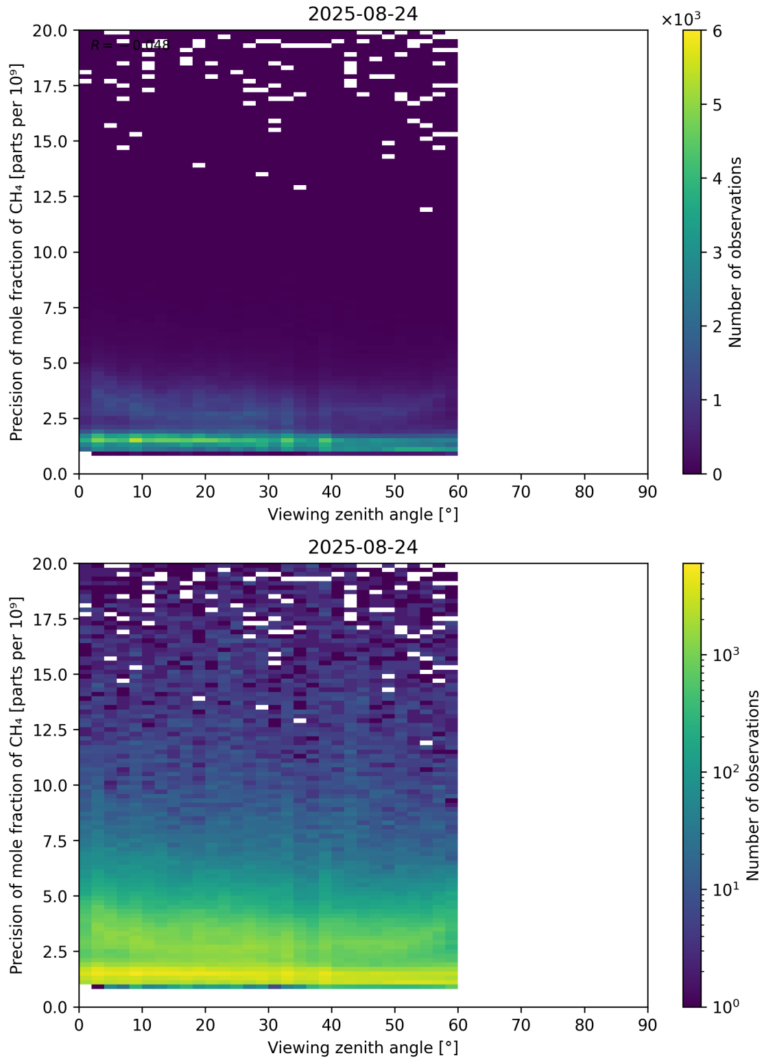
Figure 112: Scatter density plot of “Viewing zenith angle” against “Precision of mole fraction of CH 4 ” for 2025-08-23 to 2025-08-25.
