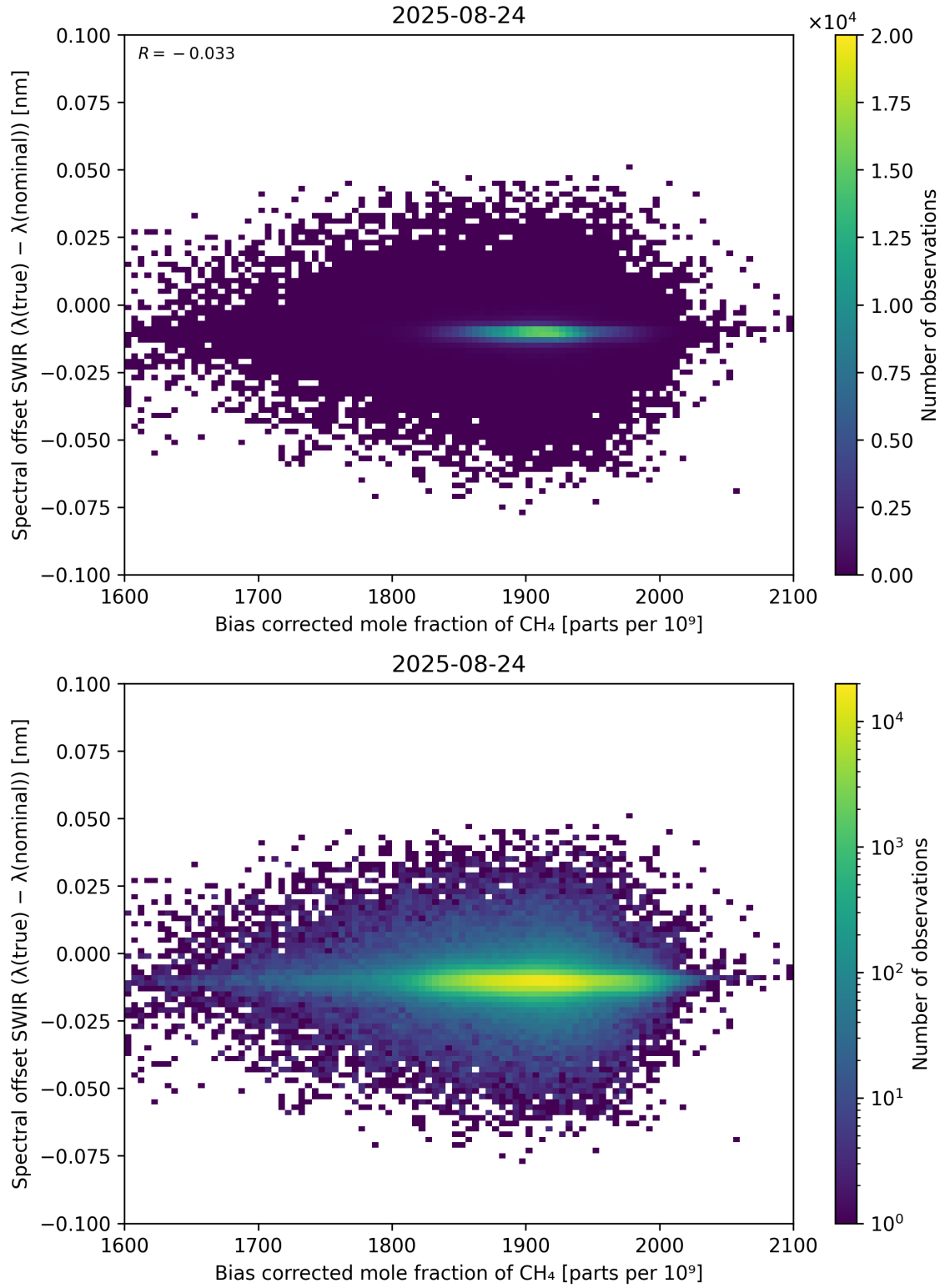
Figure 69: Scatter density plot of “Bias corrected mole fraction of \text{CH}_4 ” against “Spectral offset SWIR ( \lambda_{\text{true}} - \lambda_{\text{nominal}} )” for 2025-08-23 to 2025-08-25.
