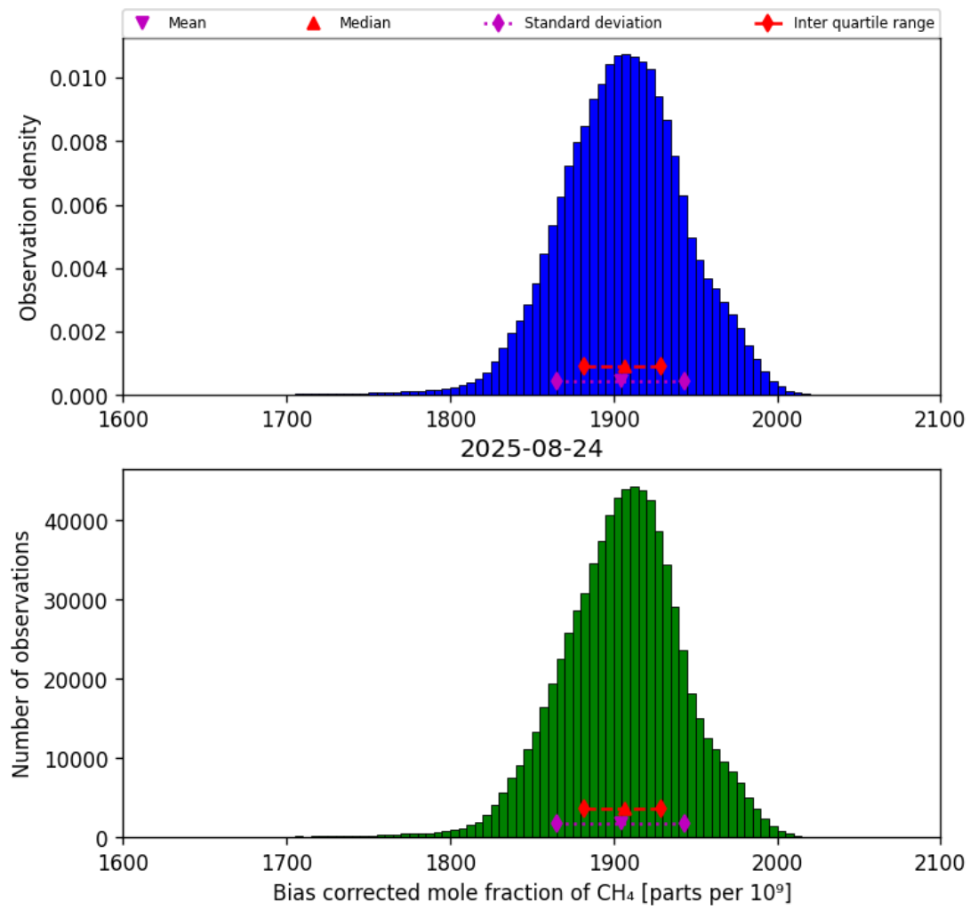
Figure 25: Histogram of “Bias corrected mole fraction of CH 4 ” for 2025-08-23 to 2025-08-25
