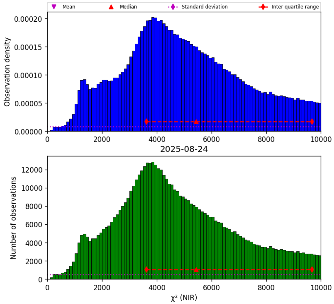
Figure 29: Histogram of " \chi^2 (NIR)" for 2025-08-23 to 2025-08-25
