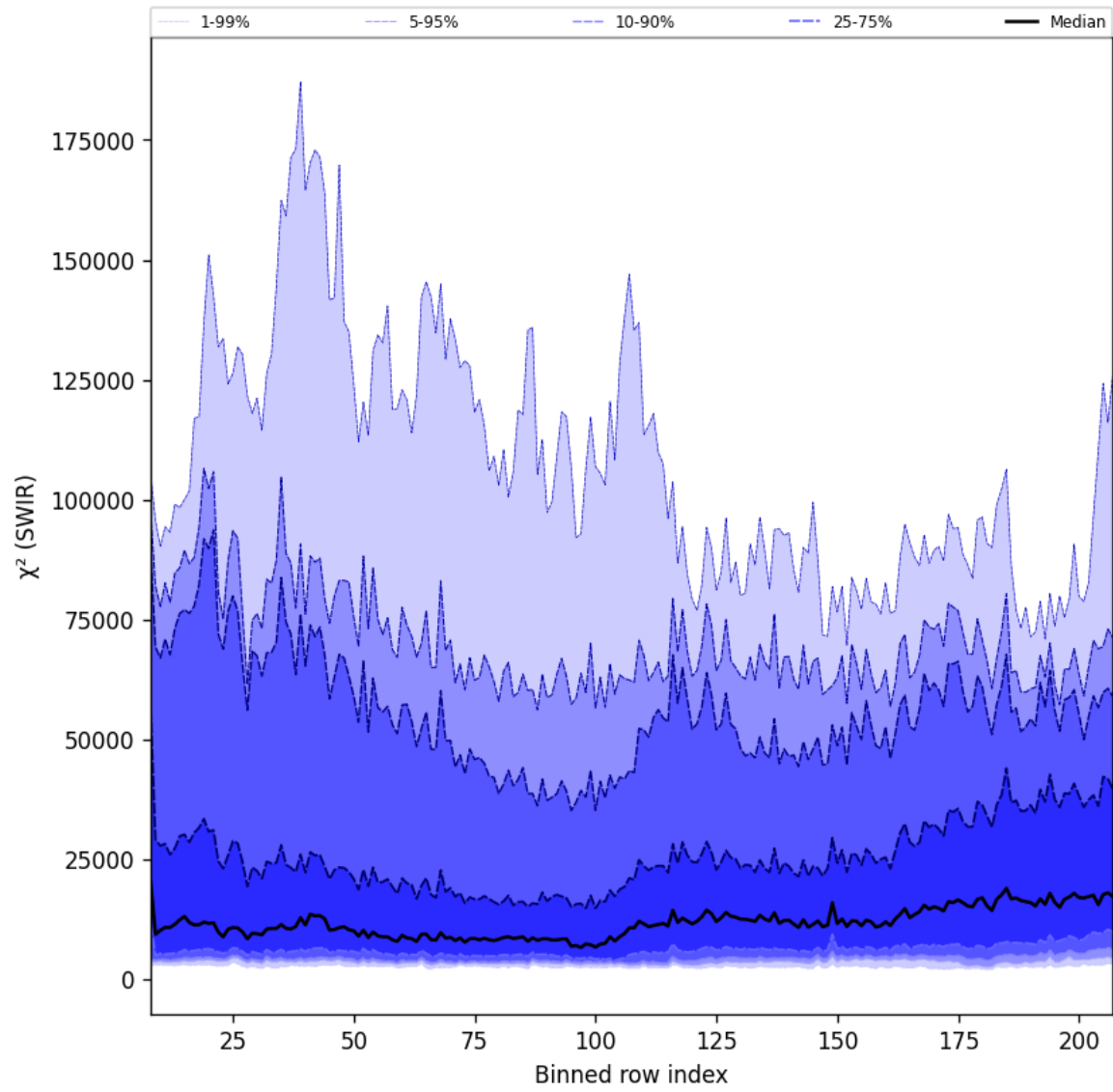
Figure 39: Along track statistics of “ \chi^2 (SWIR)” for 2025-08-23 to 2025-08-25
