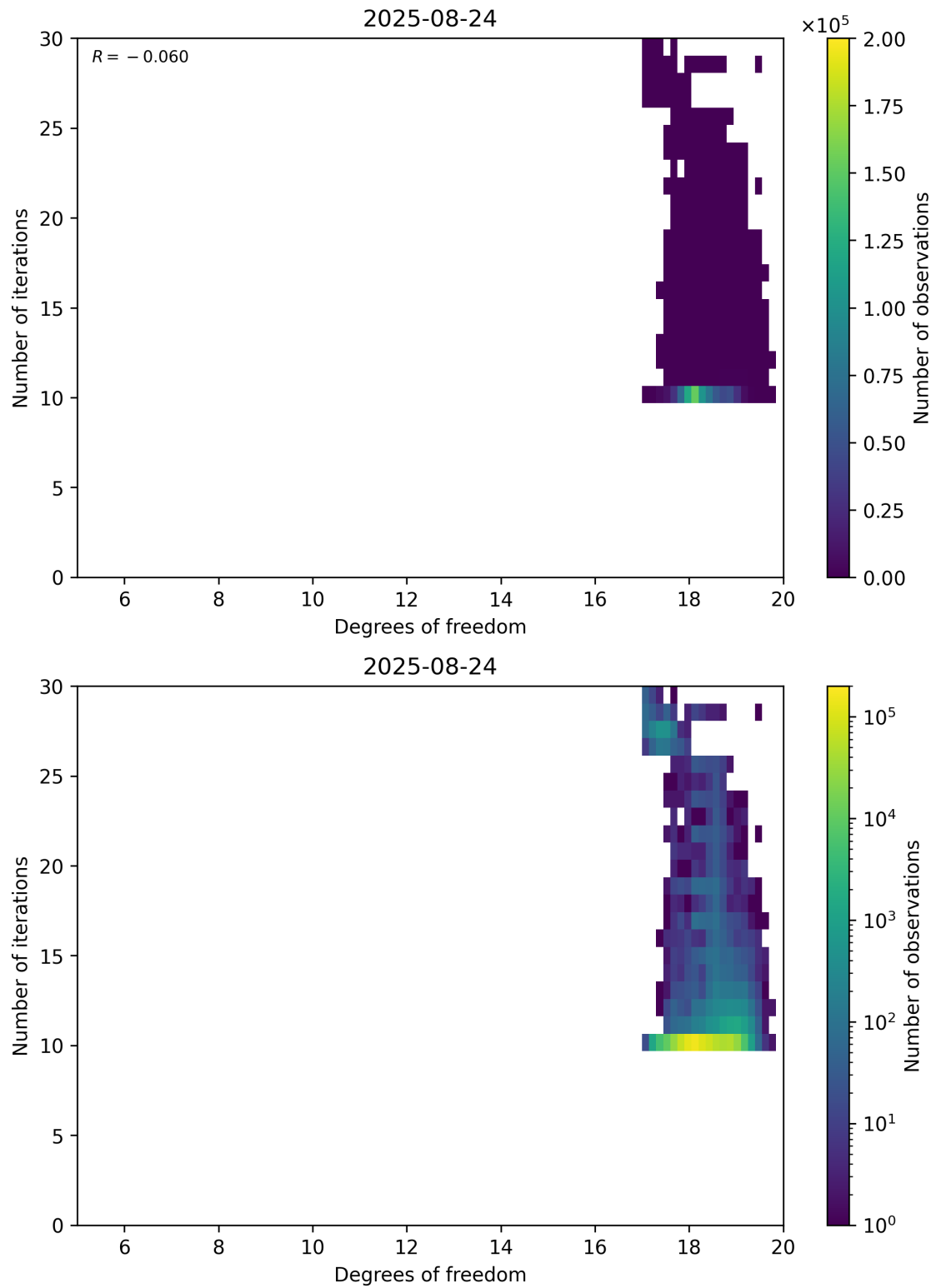
Figure 52: Scatter density plot of “Degrees of freedom” against “Number of iterations” for 2025-08-23 to 2025-08-25.
