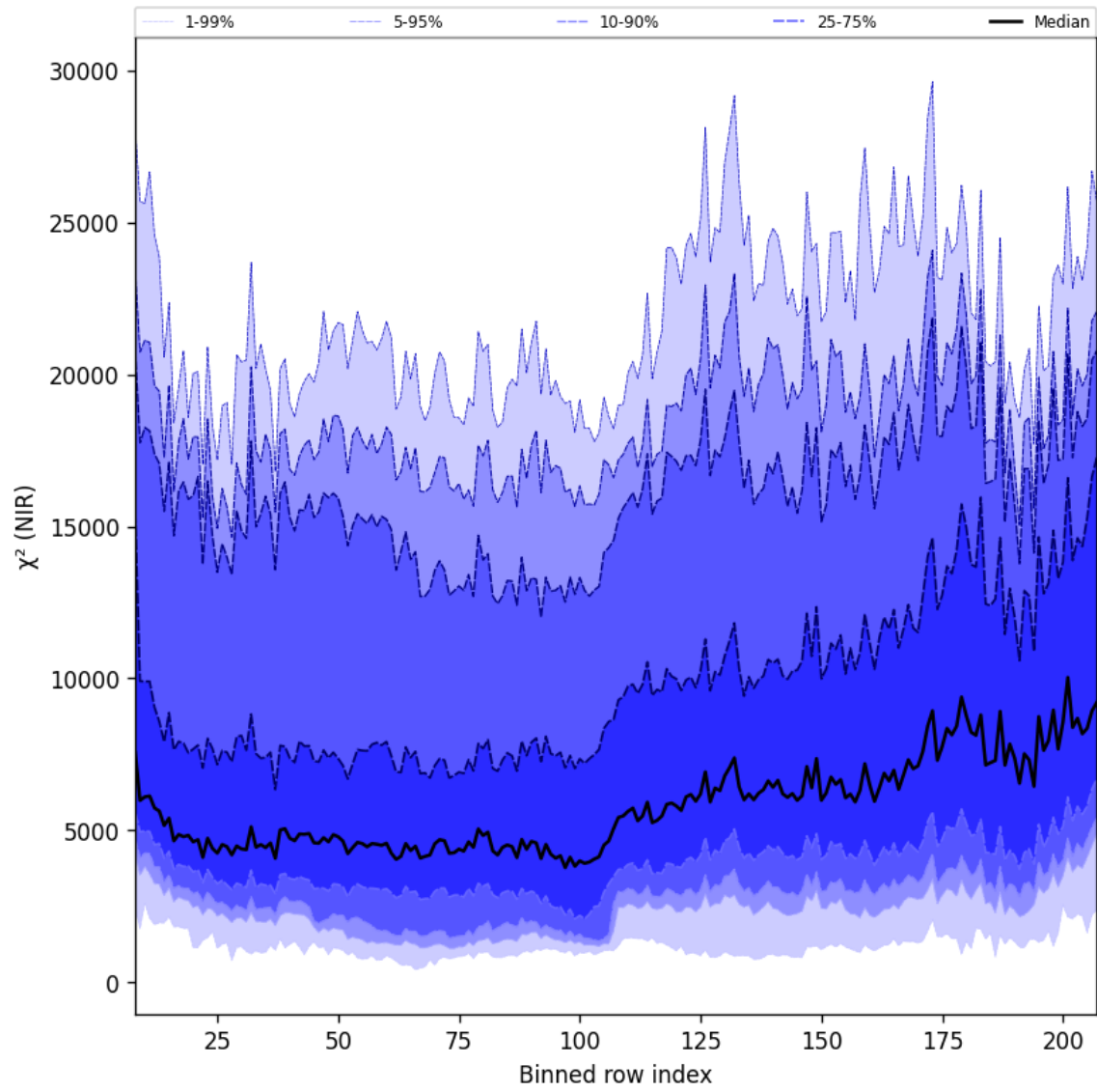
Figure 40: Along track statistics of “ \chi^2 (NIR)” for 2025-08-23 to 2025-08-25
