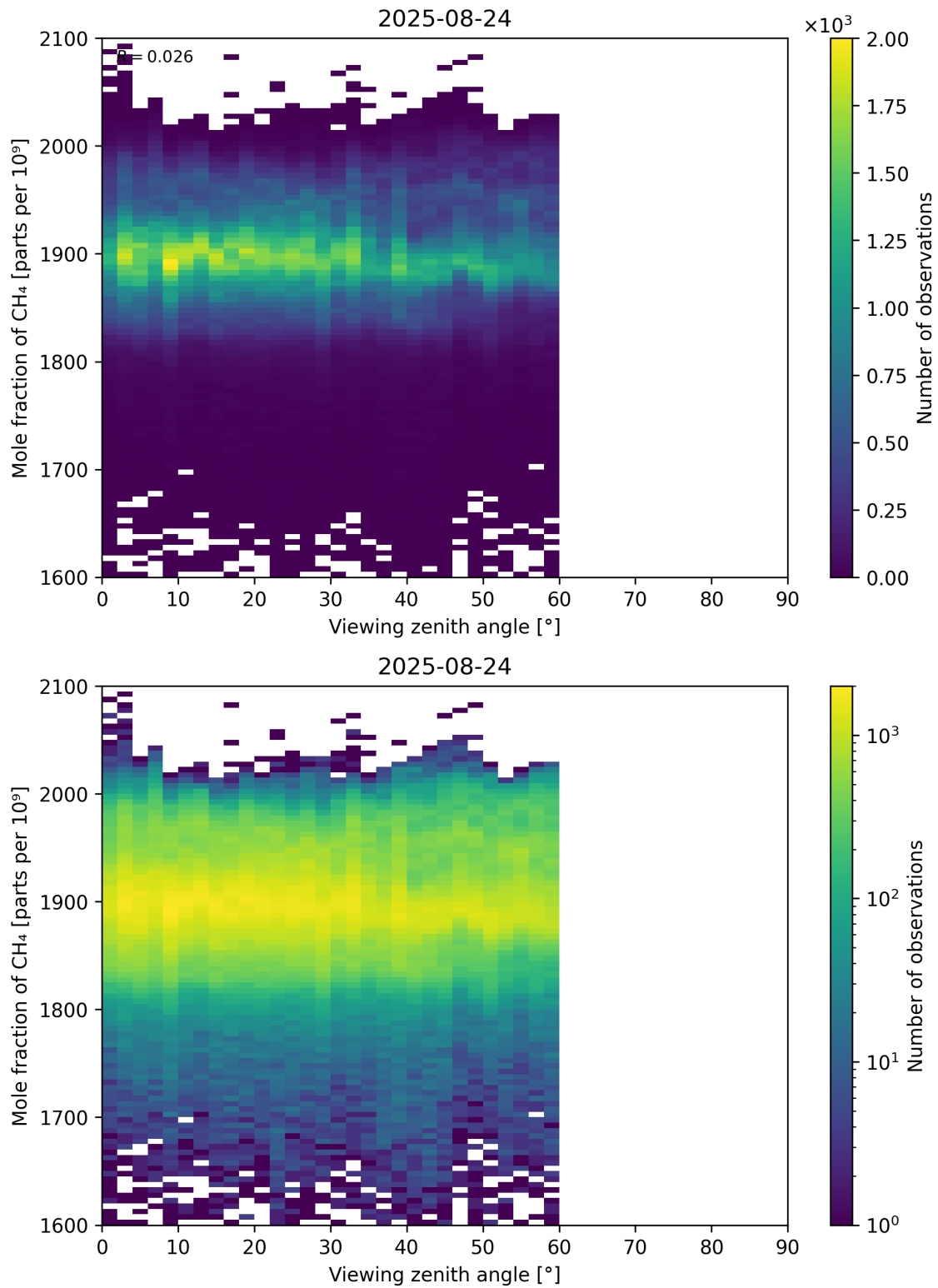
Figure 110: Scatter density plot of “Viewing zenith angle” against “Mole fraction of CH 4 ” for 2025-08-23 to 2025-08-25.
