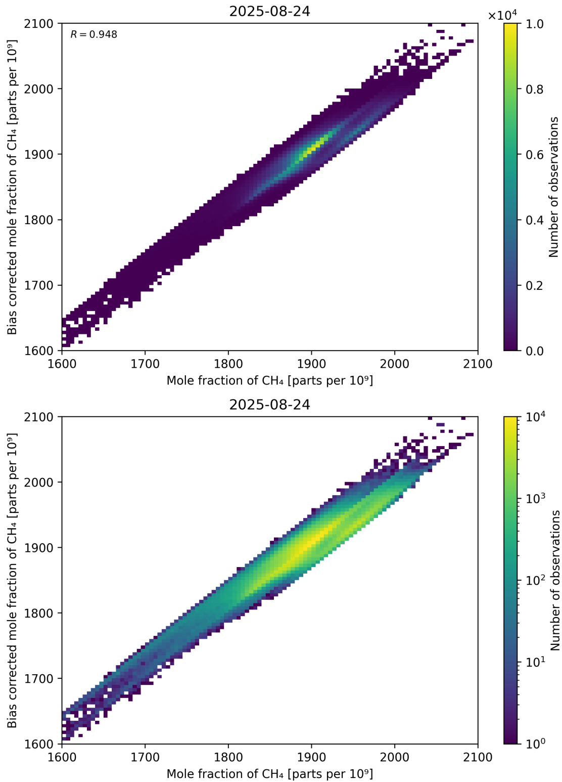
Figure 74: Scatter density plot of “Mole fraction of CH 4 ” against “Bias corrected mole fraction of CH 4 ” for 2025-08-23 to 2025-08-25.
