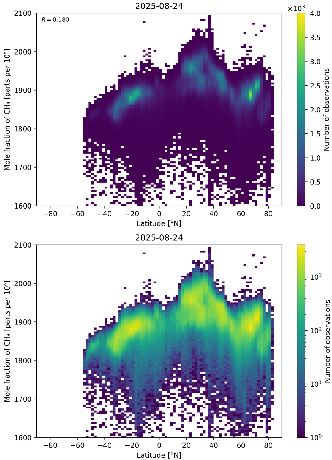
Figure 57: Scatter density plot of “Latitude” against “Mole fraction of \text{CH}_4 ” for 2025-08-23 to 2025-08-25.
