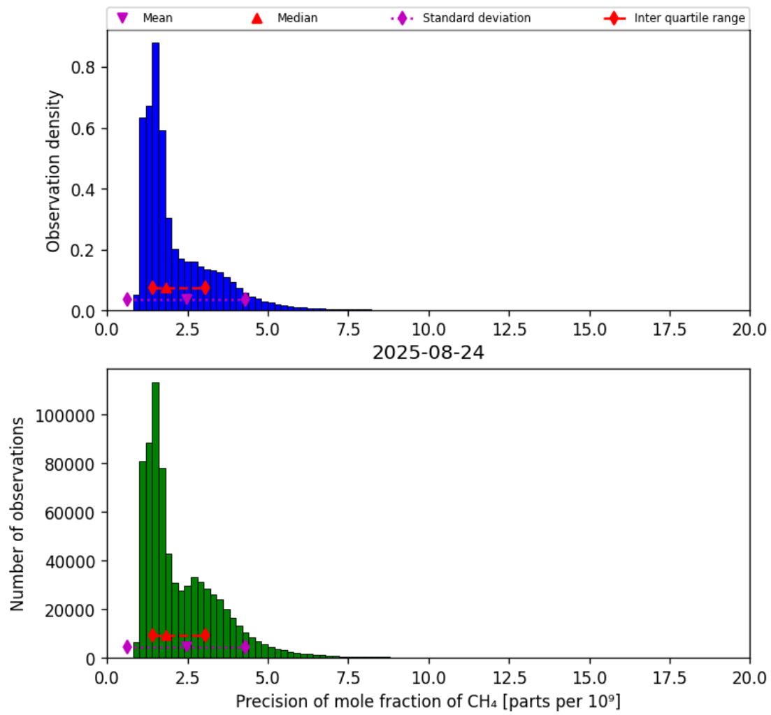
Figure 24: Histogram of “Precision of mole fraction of CH 4 ” for 2025-08-23 to 2025-08-25
