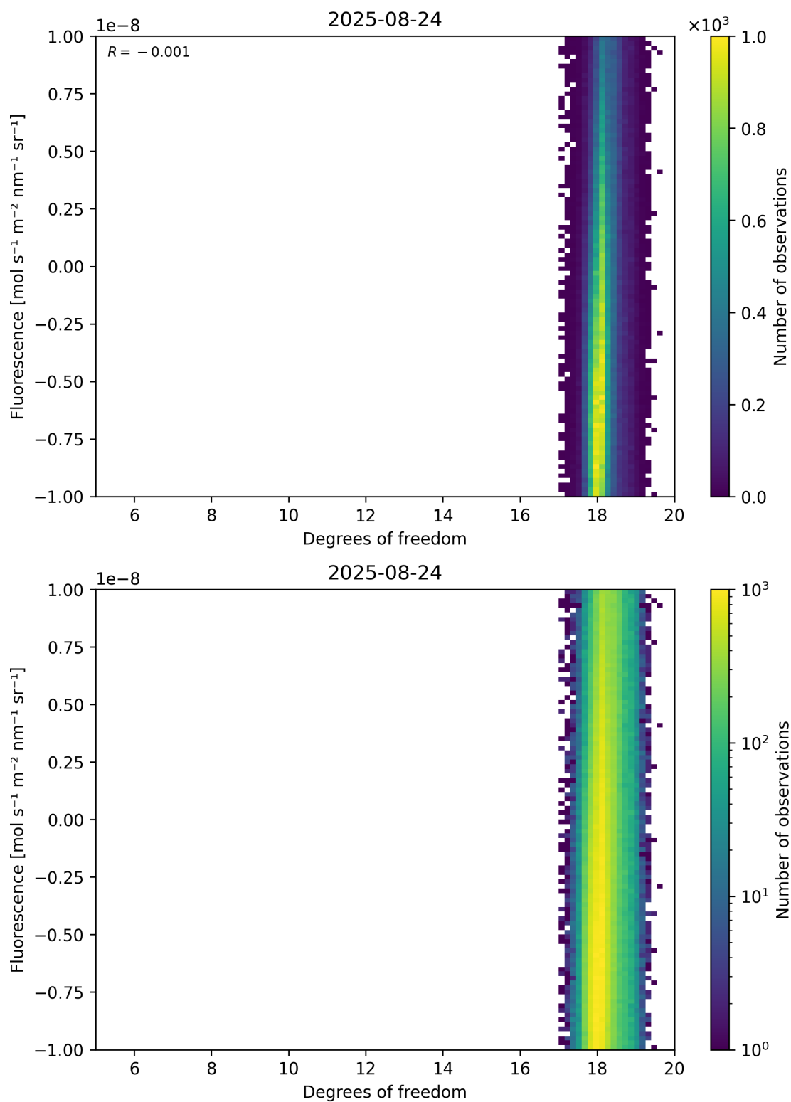
Figure 51: Scatter density plot of “Degrees of freedom” against “Fluorescence” for 2025-08-23 to 2025-08-25.
