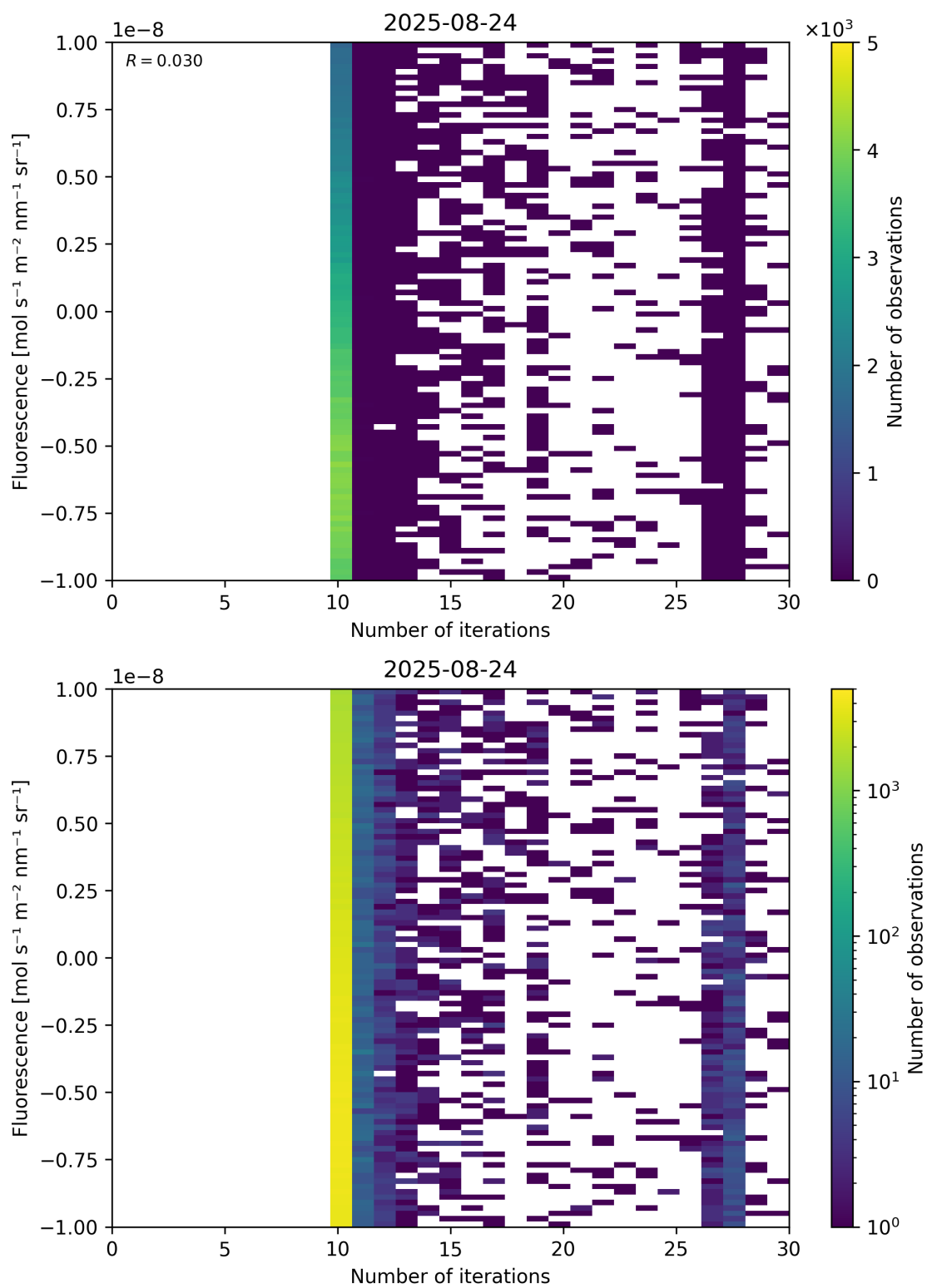
Figure 87: Scatter density plot of “Number of iterations” against “Fluorescence” for 2025-08-23 to 2025-08-25.
