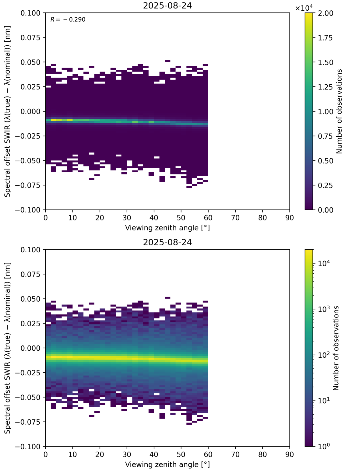
Figure 116: Scatter density plot of “Viewing zenith angle” against “Spectral offset SWIR ( \lambda_{\text{true}} - \lambda_{\text{nominal}} )” for 2025-08-23 to 2025-08-25.
