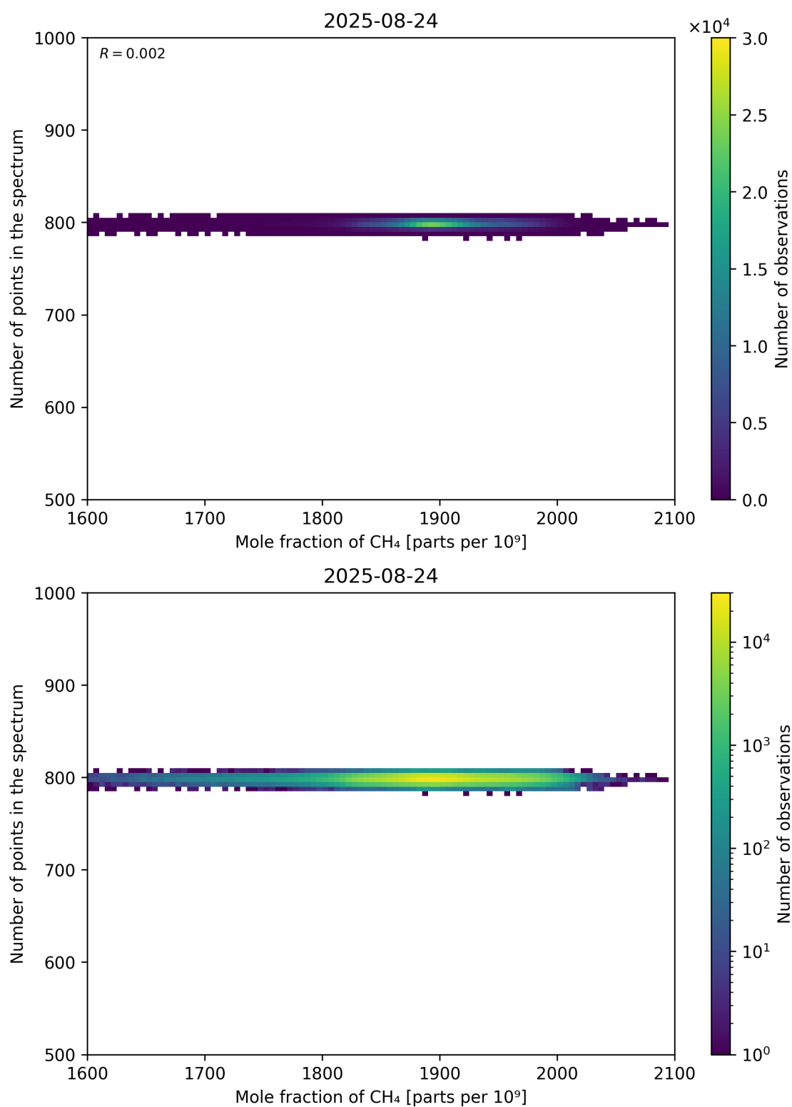
Figure 77: Scatter density plot of “Mole fraction of CH 4 ” against “Number of points in the spectrum” for 2025-08-23 to 2025-08-25.
