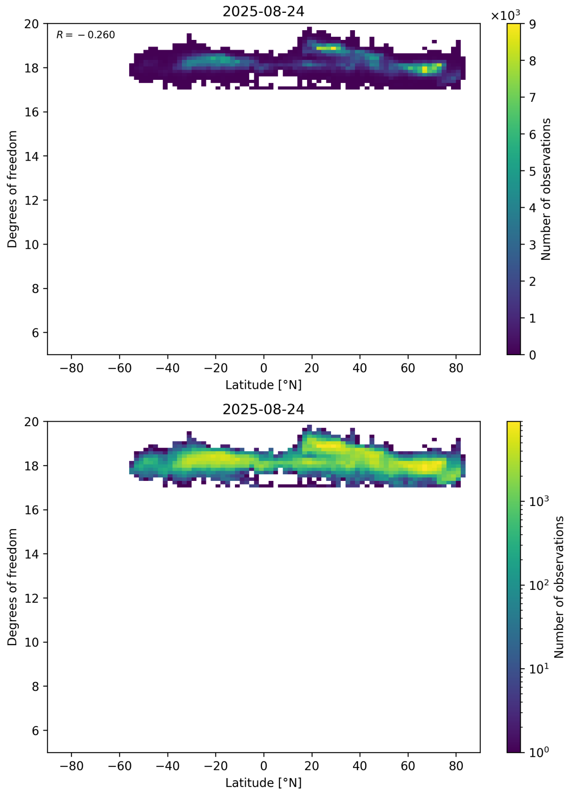
Figure 55: Scatter density plot of “Latitude” against “Degrees of freedom” for 2025-08-23 to 2025-08-25.
