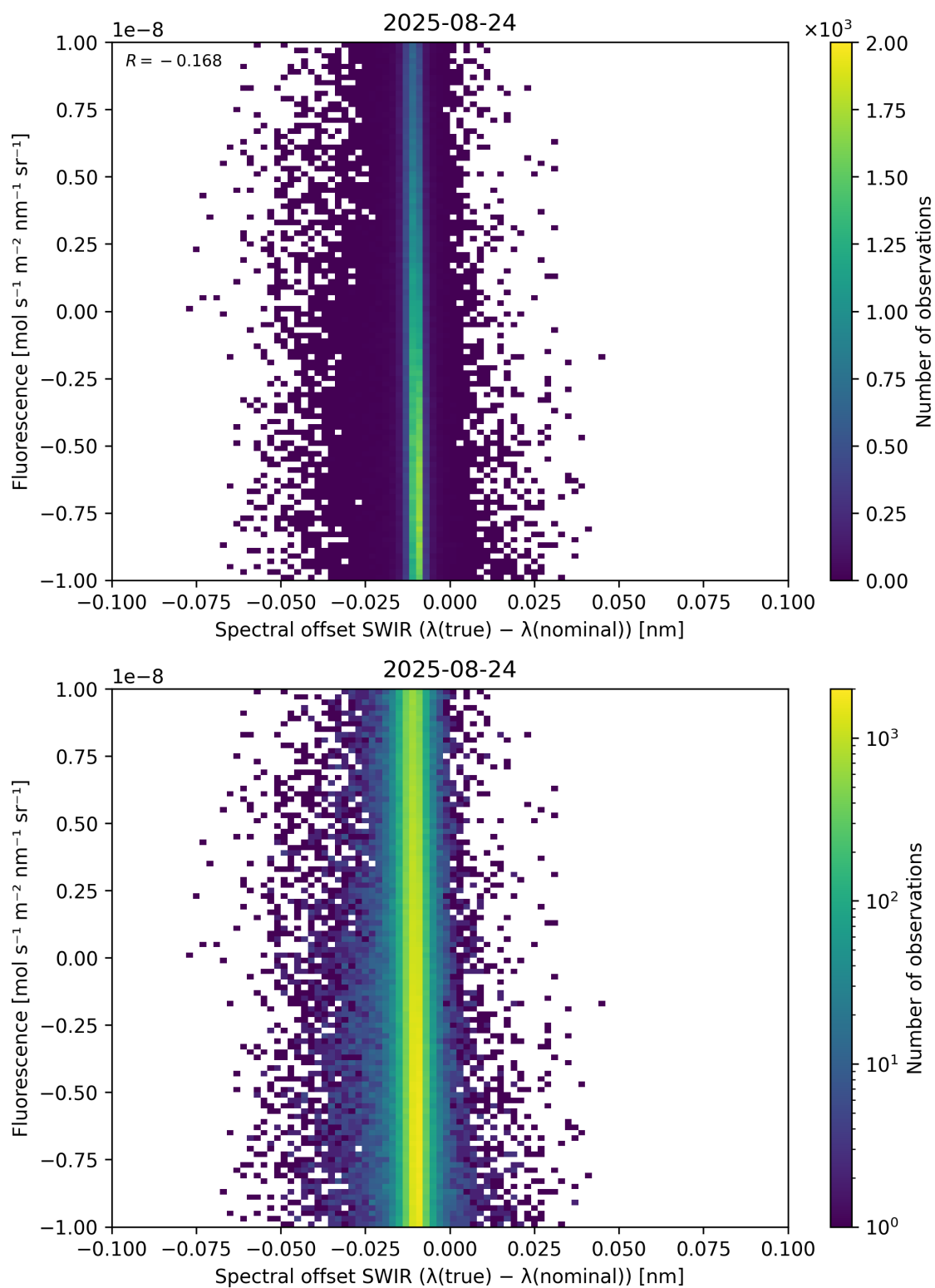
Figure 120: Scatter density plot of “Spectral offset SWIR ( \lambda_{\text{true}} - \lambda_{\text{nominal}} )” against “Fluorescence” for 2025-08-23 to 2025-08-25.
