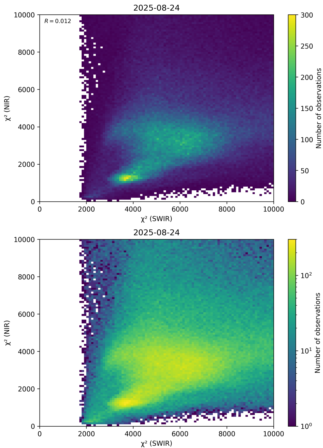
Figure 47: Scatter density plot of “ \chi^2 (SWIR)” against “ \chi^2 (NIR)” for 2025-08-23 to 2025-08-25.
