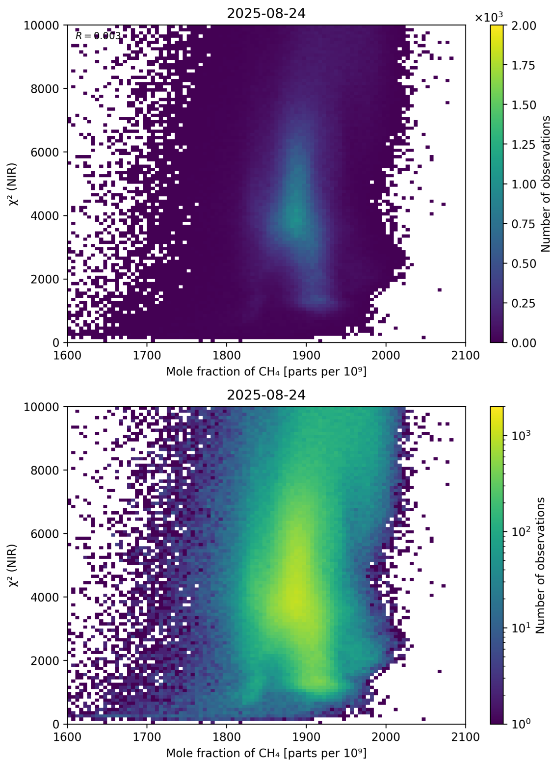
Figure 70: Scatter density plot of “Mole fraction of \text{CH}_4 ” against “ \chi^2 (NIR)” for 2025-08-23 to 2025-08-25.
