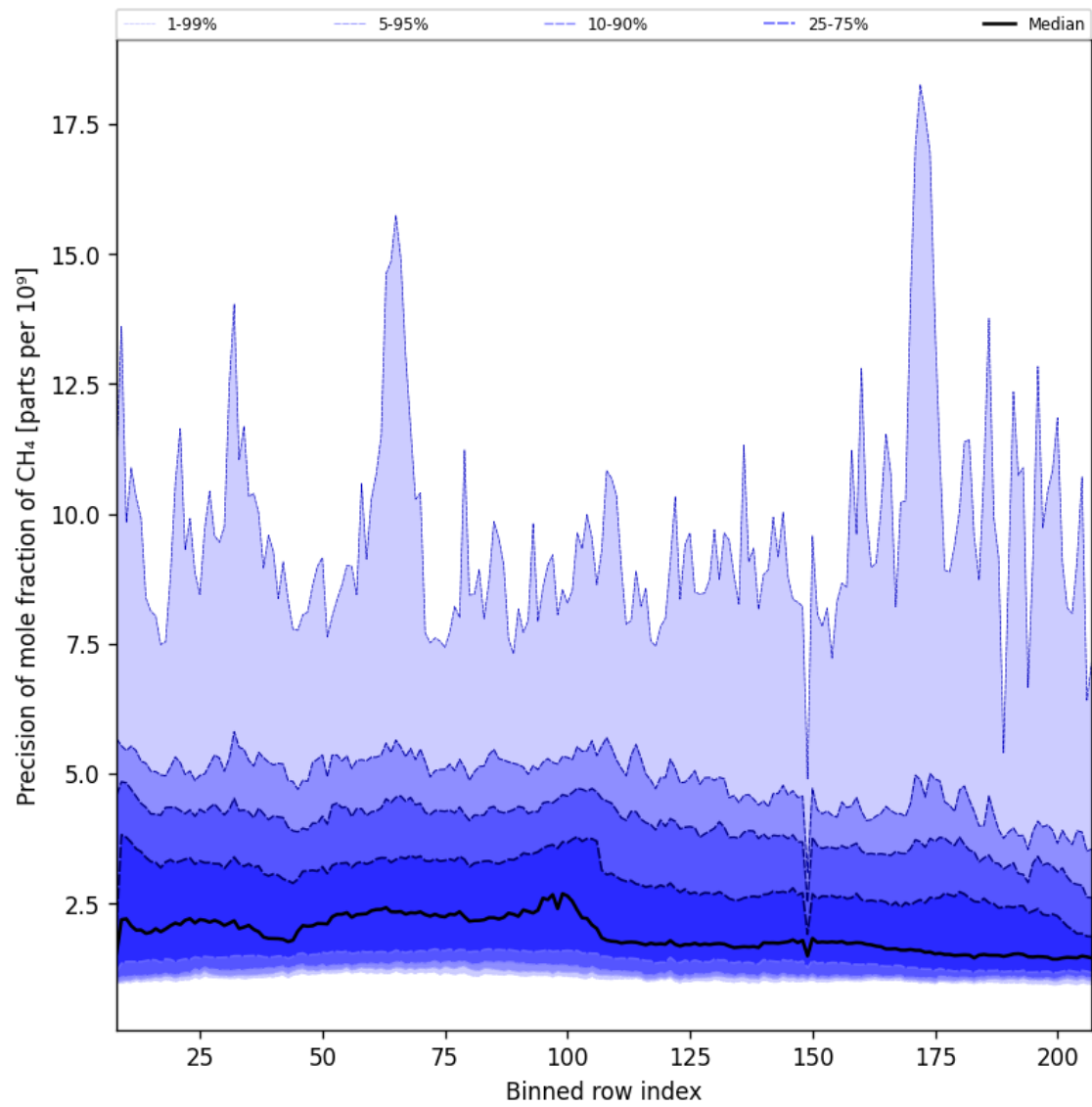
Figure 35: Along track statistics of “Precision of mole fraction of CH 4 ” for 2025-08-23 to 2025-08-25
