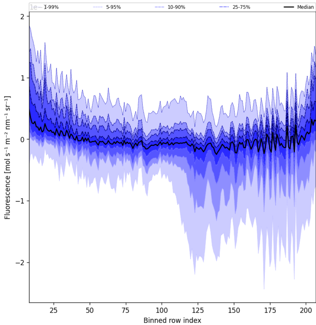
Figure 43: Along track statistics of “Fluorescence” for 2025-08-23 to 2025-08-25
