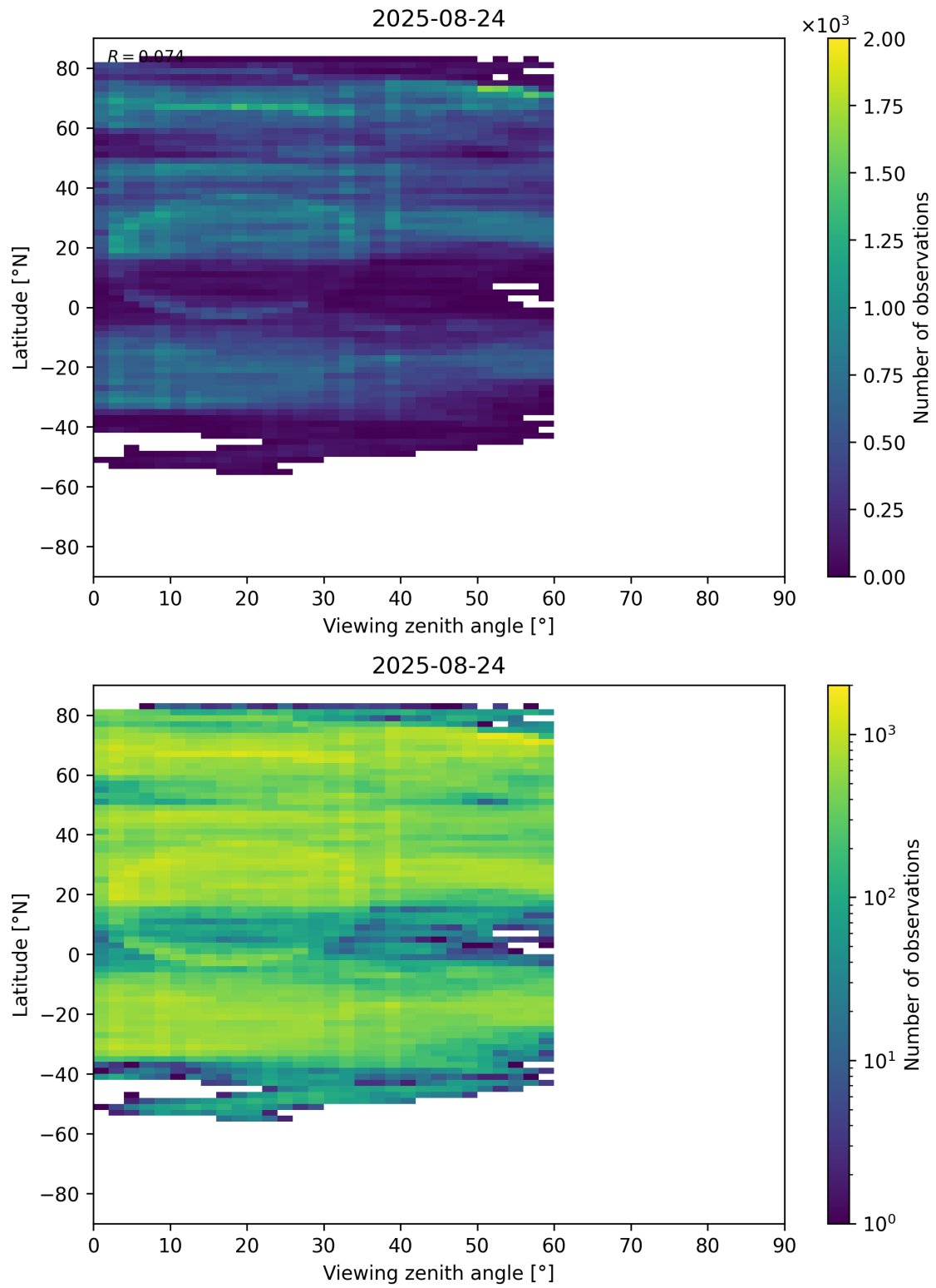
Figure 109: Scatter density plot of “Viewing zenith angle” against “Latitude” for 2025-08-23 to 2025-08-25.
