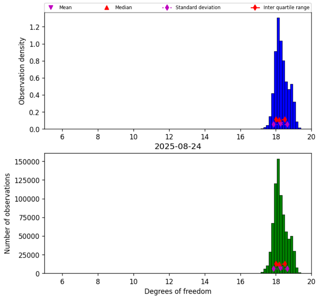
Figure 30: Histogram of “Degrees of freedom” for 2025-08-23 to 2025-08-25
