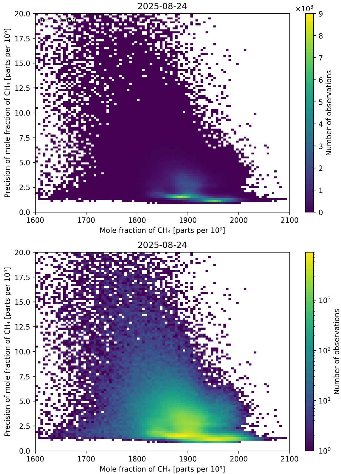
Figure 75: Scatter density plot of “Mole fraction of CH 4 ” against “Precision of mole fraction of CH 4 ” for 2025-08-23 to 2025-08-25.
