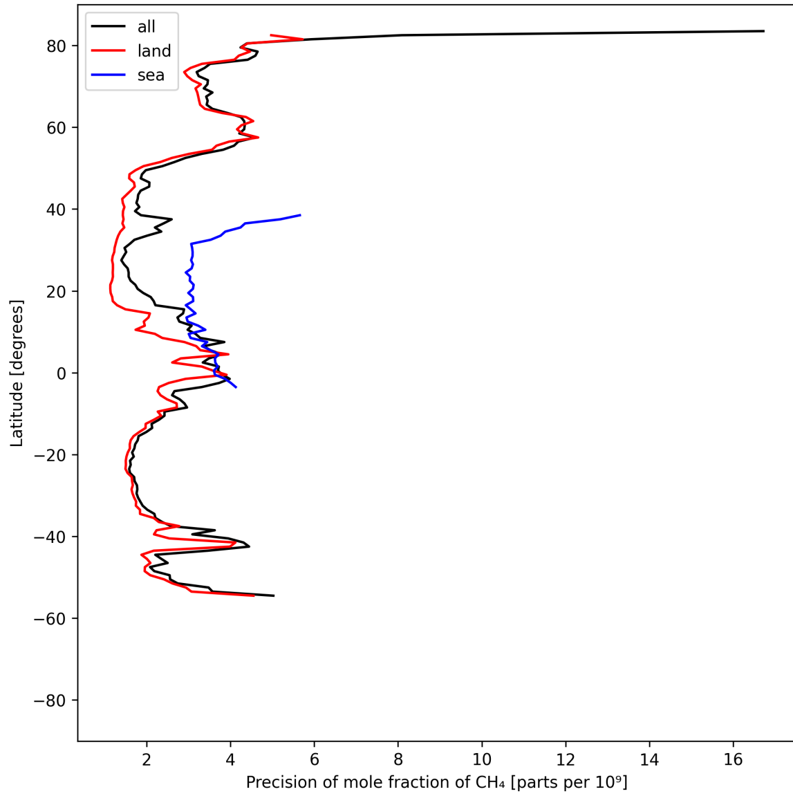
Figure 13: Zonal average of “Precision of mole fraction of CH 4 ” for 2025-08-23 to 2025-08-25.
