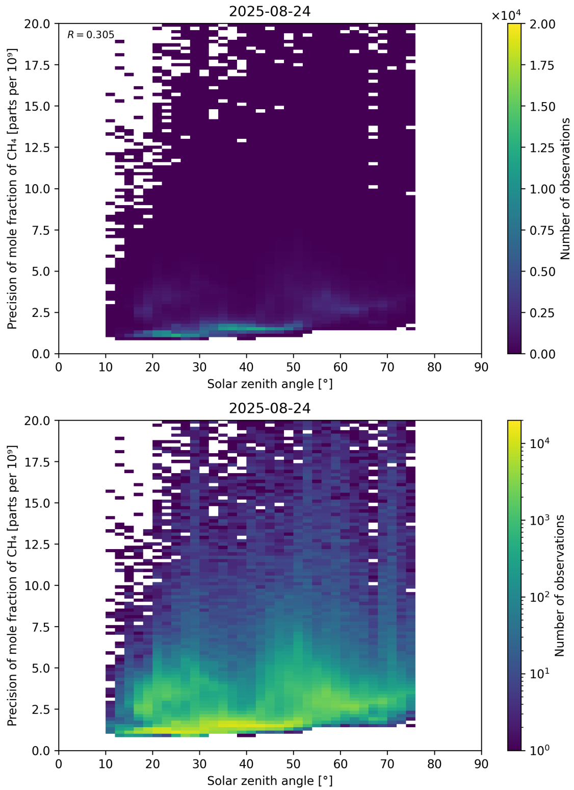
Figure 101: Scatter density plot of “Solar zenith angle” against “Precision of mole fraction of CH 4 ” for 2025-08-23 to 2025-08-25.
