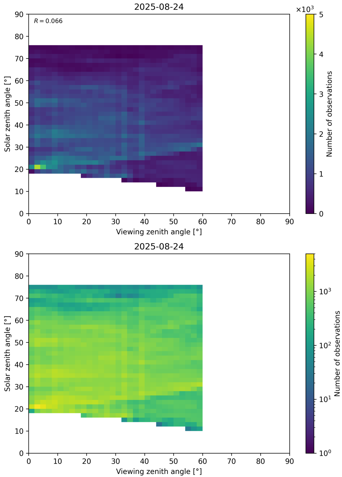
Figure 115: Scatter density plot of “Viewing zenith angle” against “Solar zenith angle” for 2025-08-23 to 2025-08-25.
