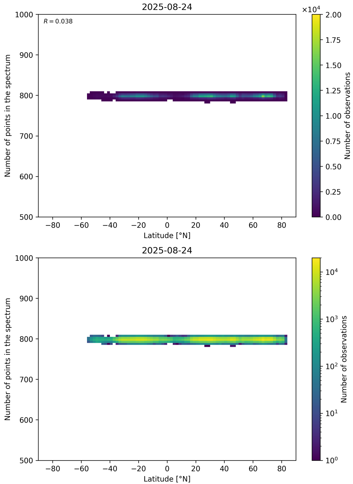
Figure 61: Scatter density plot of “Latitude” against “Number of points in the spectrum” for 2025-08-23 to 2025-08-25.
