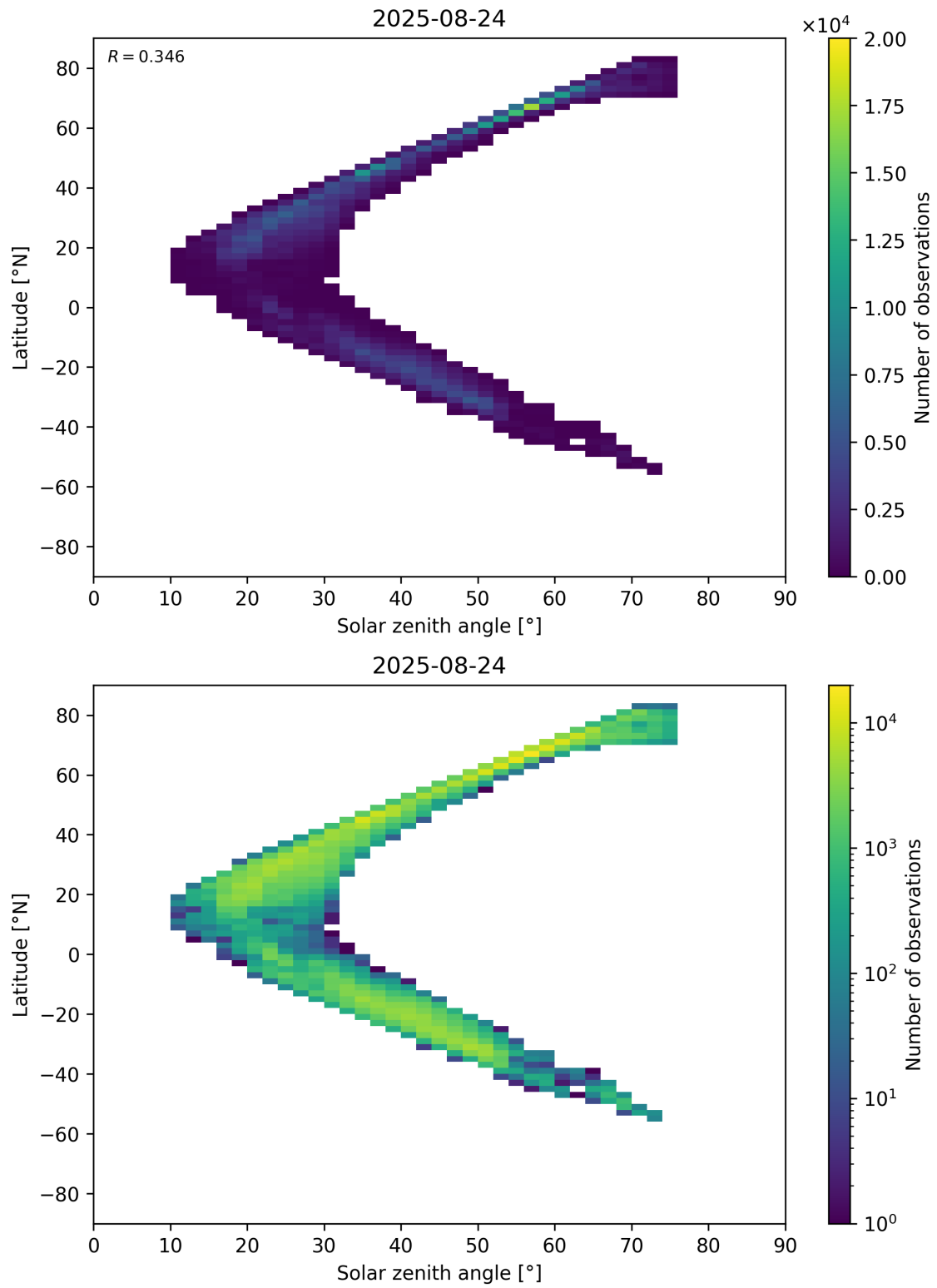
Figure 98: Scatter density plot of “Solar zenith angle” against “Latitude” for 2025-08-23 to 2025-08-25.
