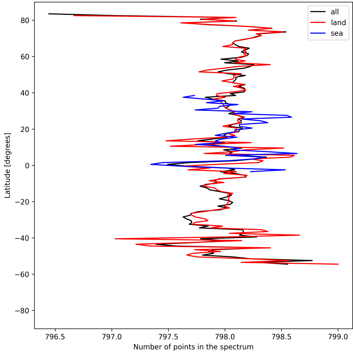
Figure 15: Zonal average of “Number of points in the spectrum” for 2025-08-23 to 2025-08-25.
