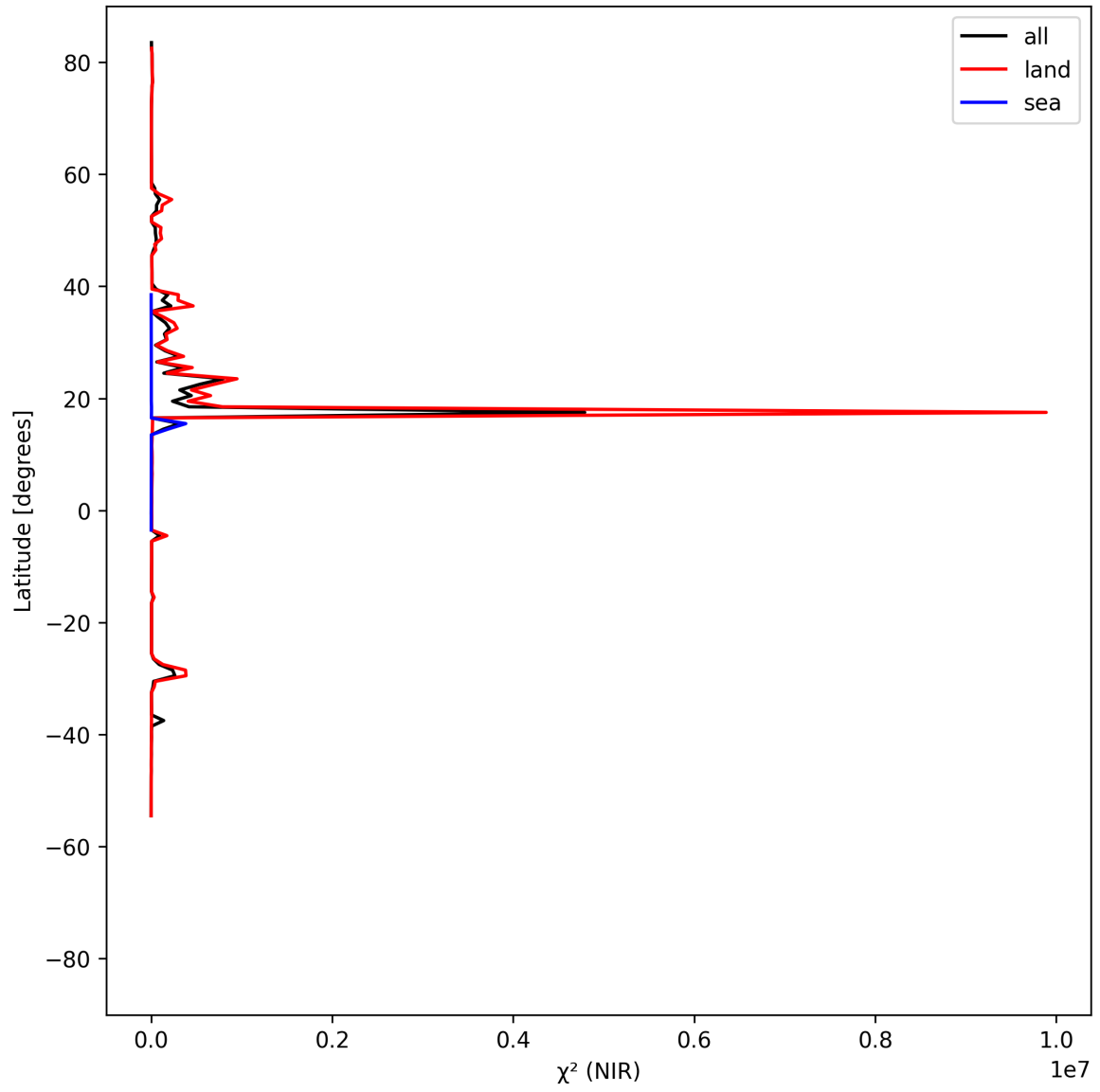
Figure 18: Zonal average of “ \chi^2 (NIR)” for 2025-08-23 to 2025-08-25.
