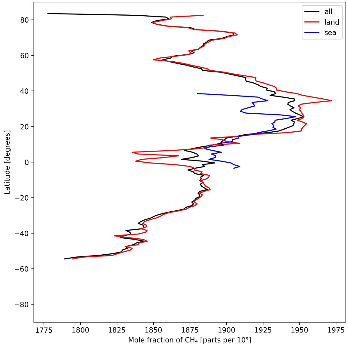
Figure 12: Zonal average of “Mole fraction of \text{CH}_4 ” for 2025-08-23 to 2025-08-25.
