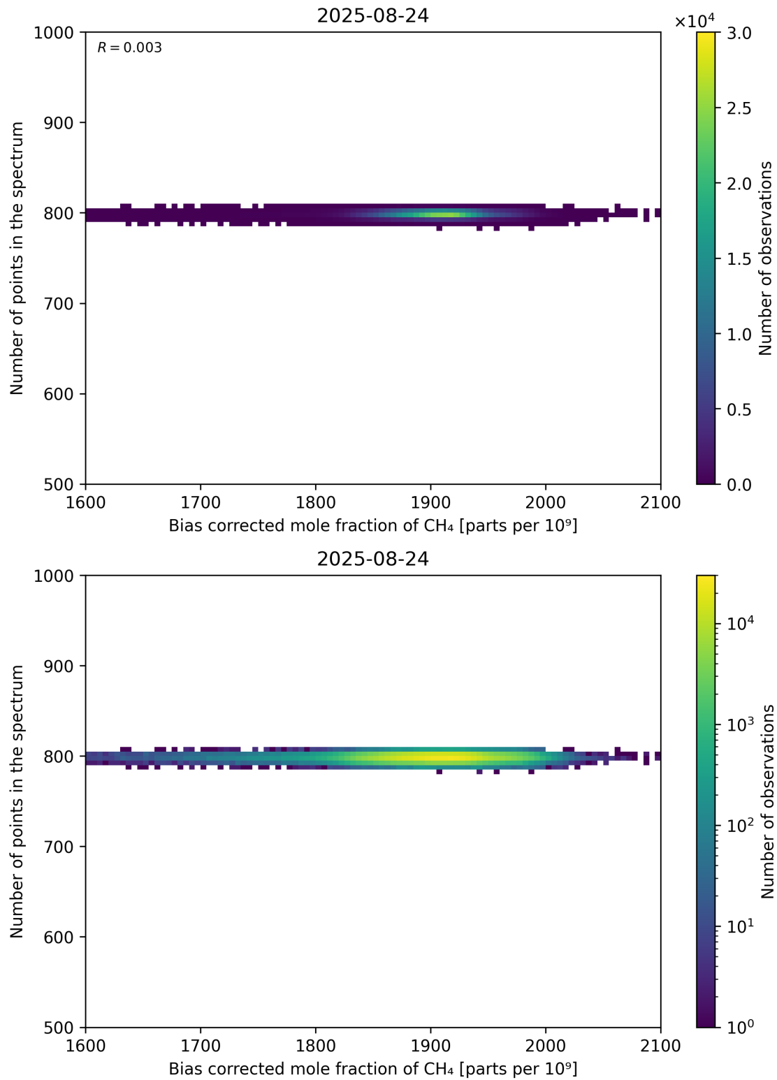
Figure 68: Scatter density plot of “Bias corrected mole fraction of CH 4 ” against “Number of points in the spectrum” for 2025-08-23 to 2025-08-25.
