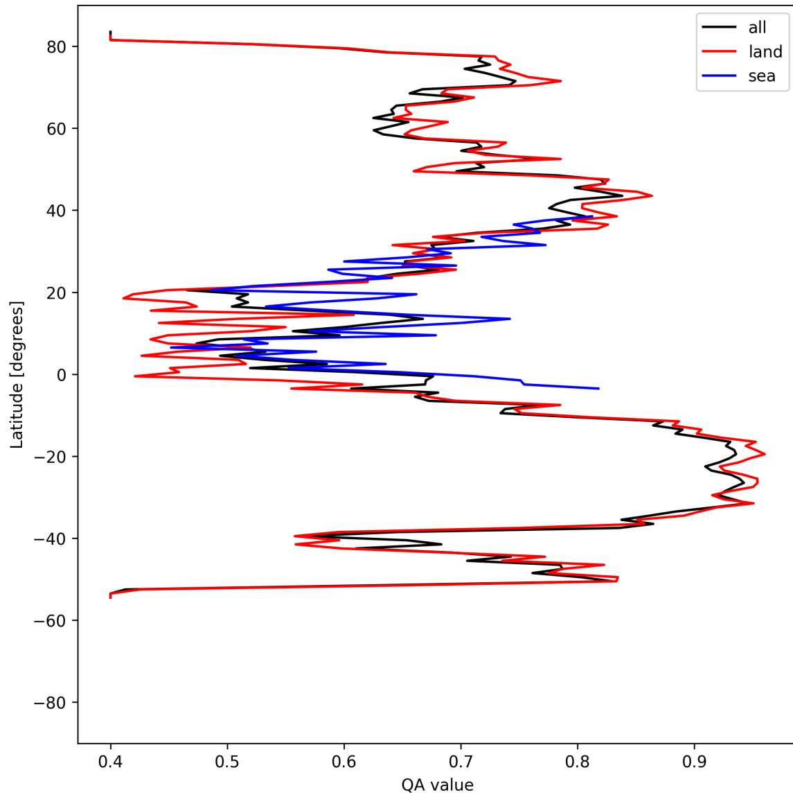
Figure 11: Zonal average of “QA value” for 2025-08-23 to 2025-08-25.
