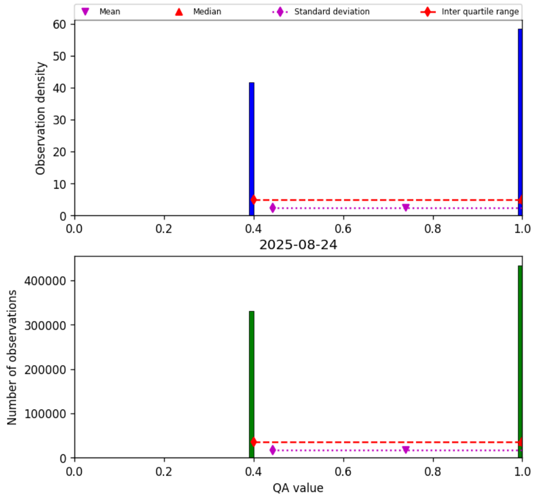
Figure 22: Histogram of “QA value” for 2025-08-23 to 2025-08-25
