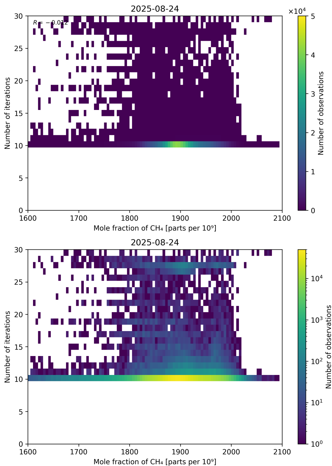
Figure 76: Scatter density plot of “Mole fraction of CH 4 ” against “Number of iterations” for 2025-08-23 to 2025-08-25.
