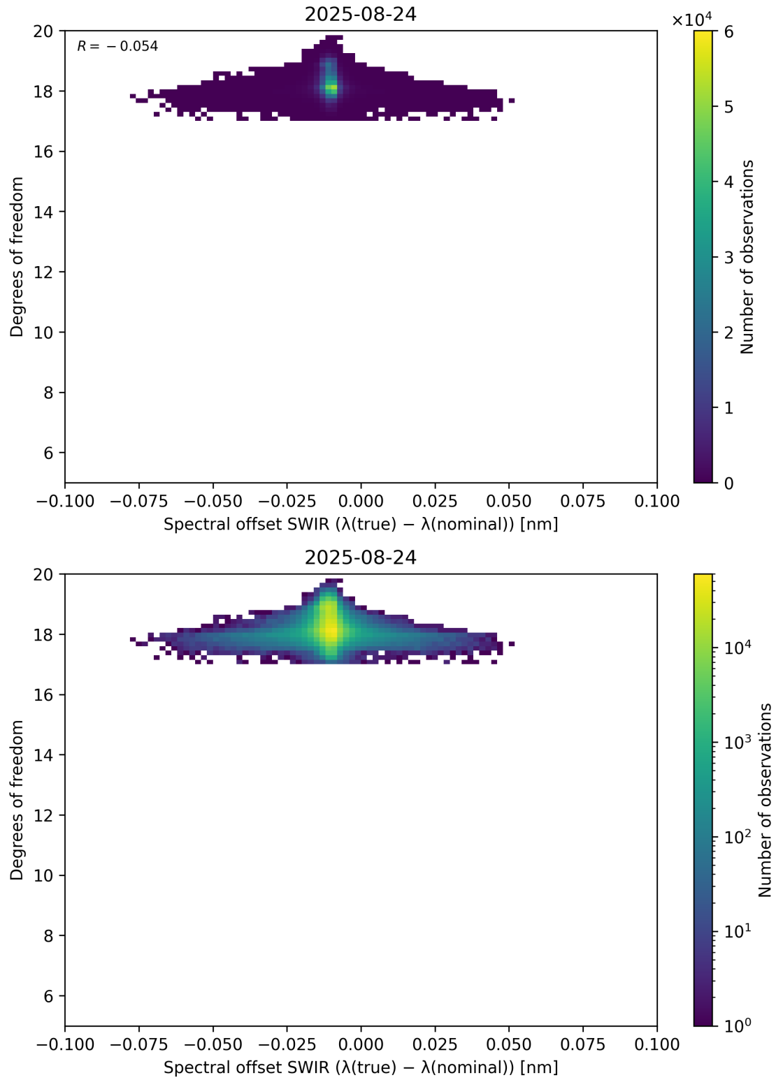
Figure 119: Scatter density plot of “Spectral offset SWIR ( \lambda_{\text{true}} - \lambda_{\text{nominal}} )” against “Degrees of freedom” for 2025-08-23 to 2025-08-25.
