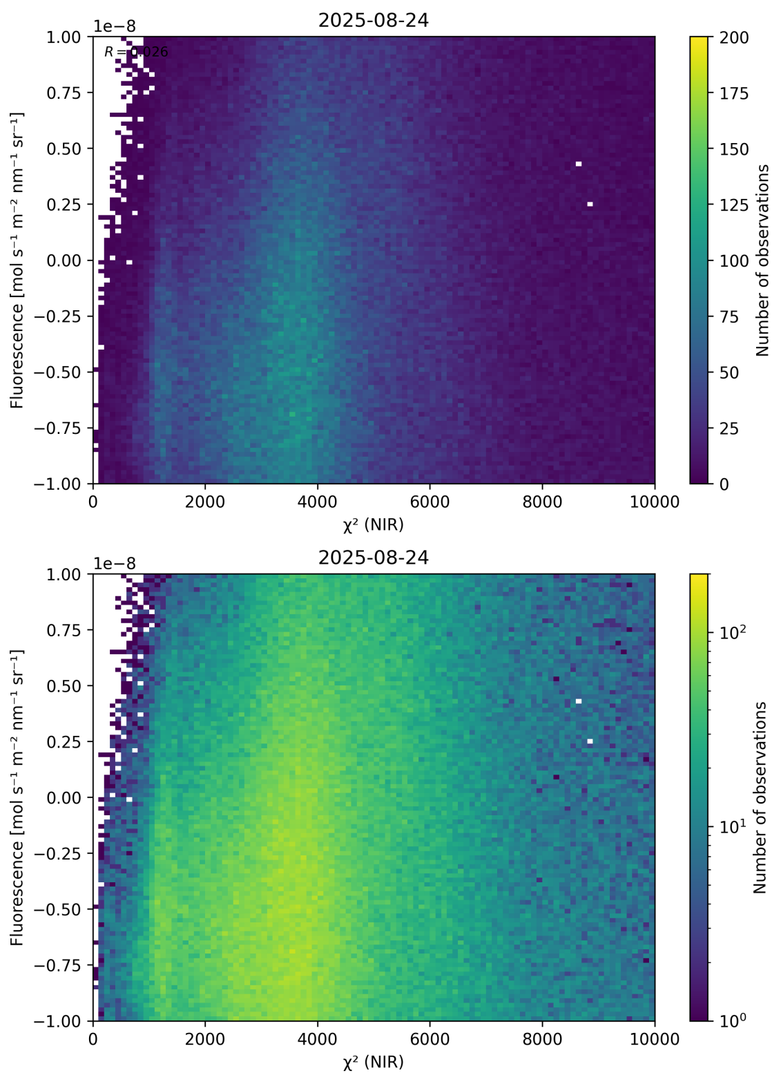
Figure 45: Scatter density plot of “ \chi^2 (NIR)” against “Fluorescence” for 2025-08-23 to 2025-08-25.
