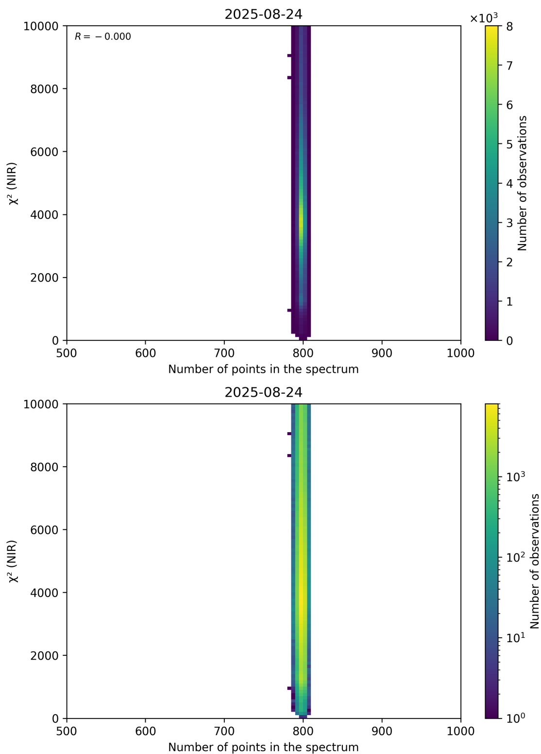
Figure 88: Scatter density plot of “Number of points in the spectrum” against “ \chi^2 (NIR)” for 2025-08-23 to 2025-08-25.
