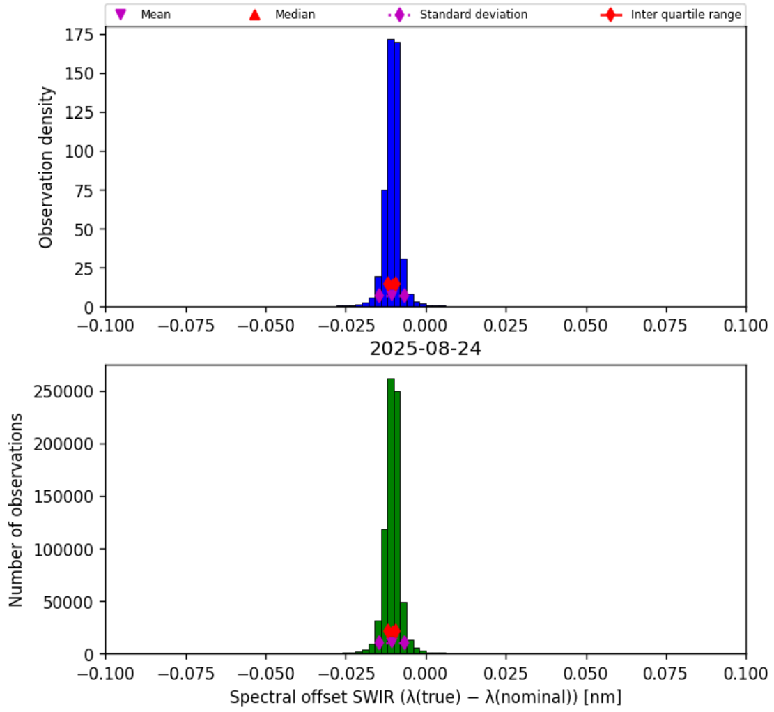
Figure 27: Histogram of “Spectral offset SWIR ( \lambda_{\text{true}} - \lambda_{\text{nominal}} )” for 2025-08-23 to 2025-08-25
