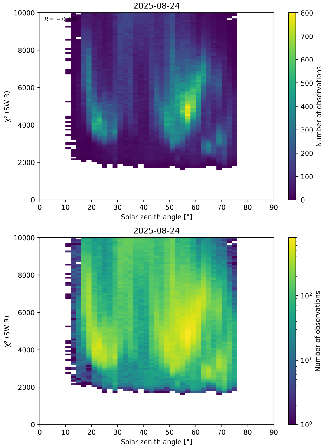
Figure 95: Scatter density plot of “Solar zenith angle” against “ \chi^2 (SWIR)” for 2025-08-23 to 2025-08-25.
