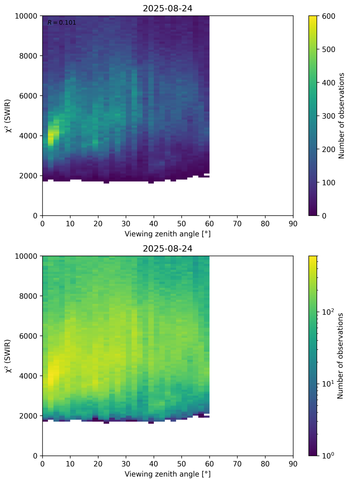
Figure 106: Scatter density plot of “Viewing zenith angle” against “ \chi^2 (SWIR)” for 2025-08-23 to 2025-08-25.
