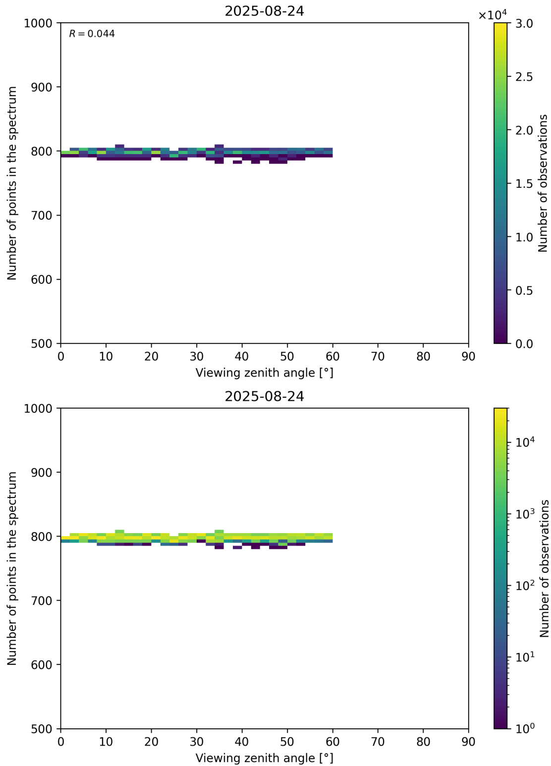
Figure 114: Scatter density plot of “Viewing zenith angle” against “Number of points in the spectrum” for 2025-08-23 to 2025-08-25.
