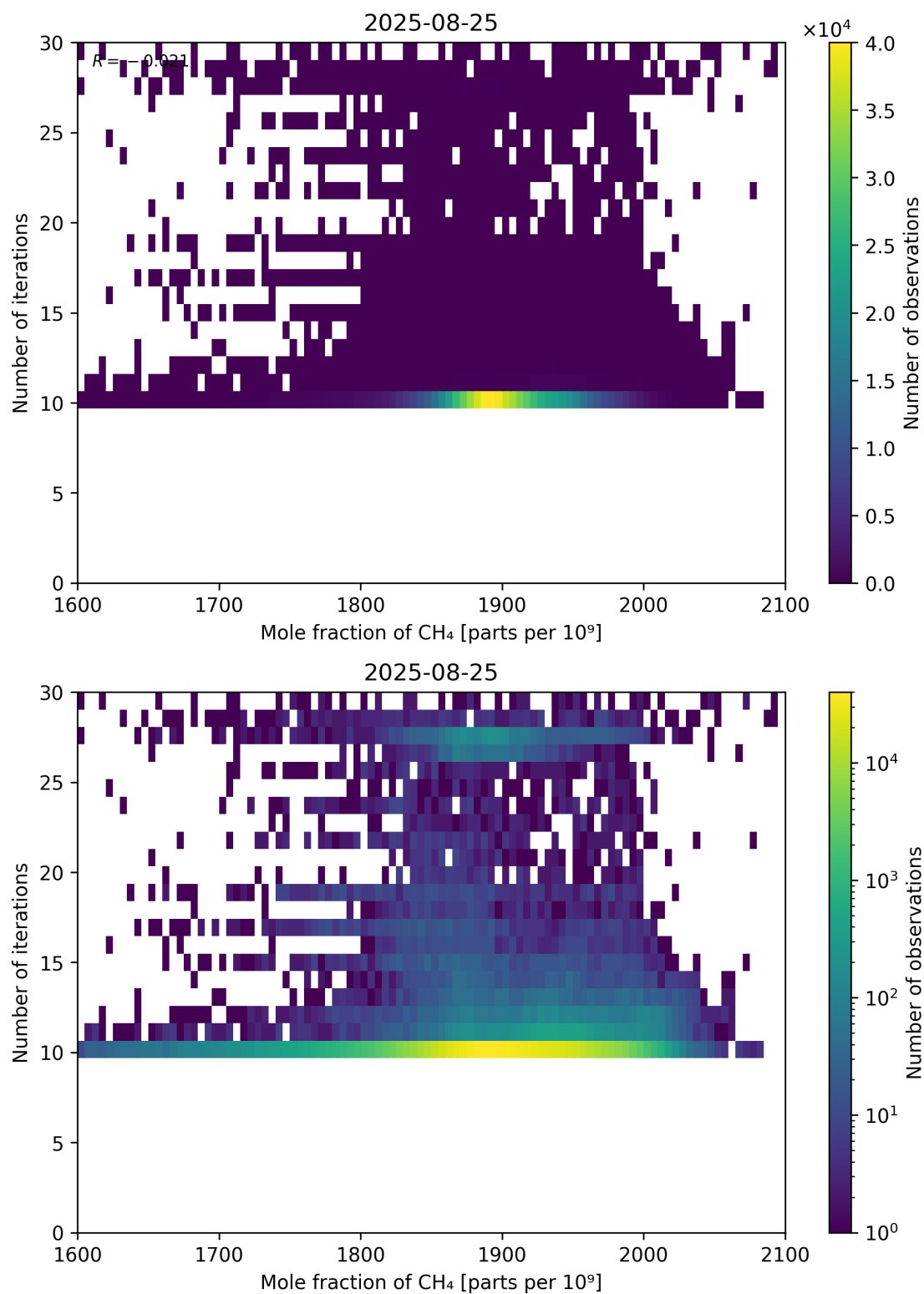
Figure 76: Scatter density plot of “Mole fraction of CH 4 ” against “Number of iterations” for 2025-08-25 to 2025-08-26.
