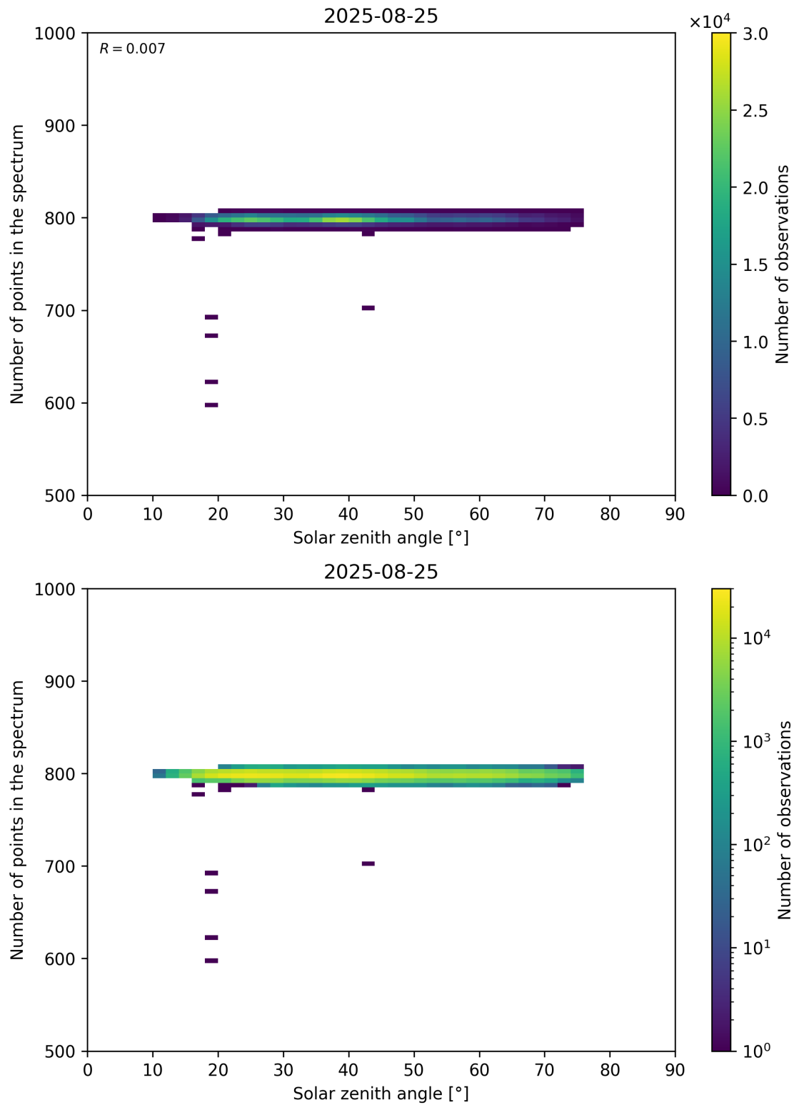
Figure 103: Scatter density plot of “Solar zenith angle” against “Number of points in the spectrum” for 2025-08-25 to 2025-08-26.
