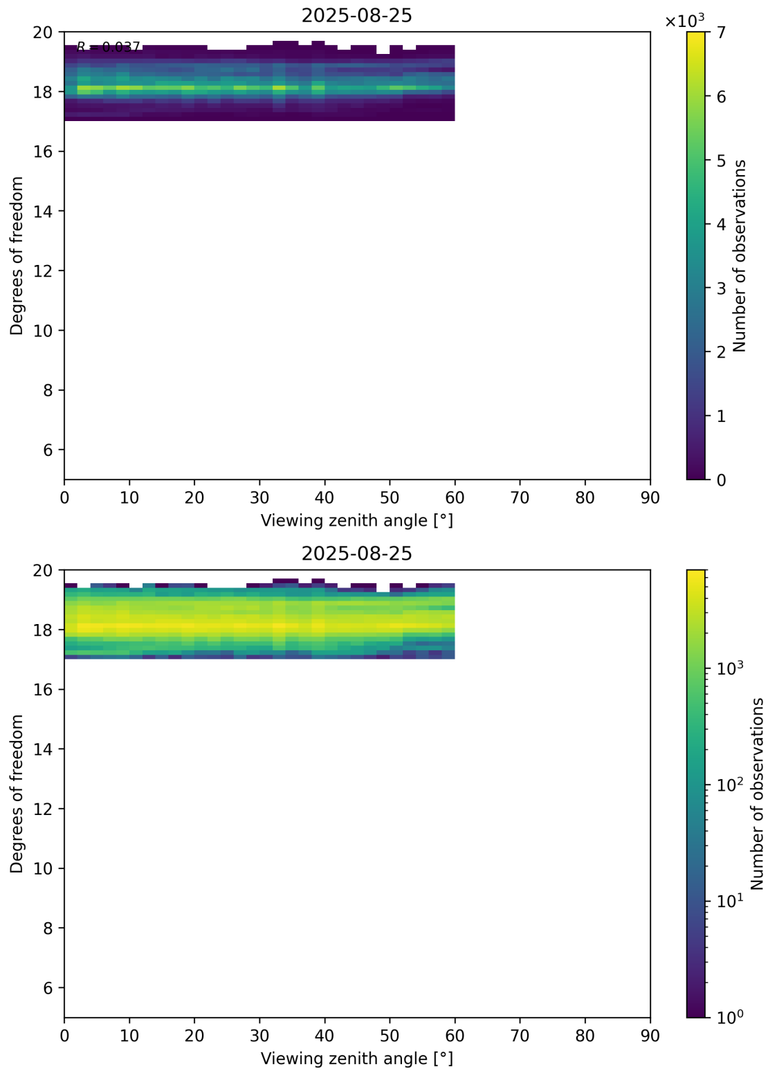
Figure 107: Scatter density plot of “Viewing zenith angle” against “Degrees of freedom” for 2025-08-25 to 2025-08-26.
