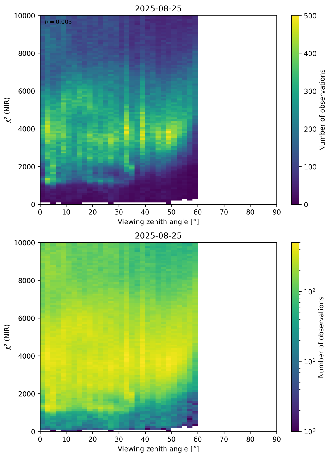
Figure 105: Scatter density plot of “Viewing zenith angle” against “ \chi^2 (NIR)” for 2025-08-25 to 2025-08-26.
