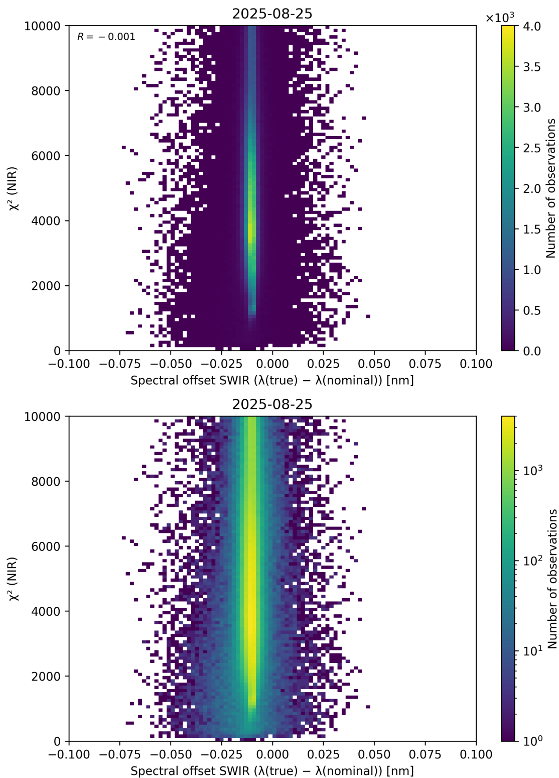
Figure 117: Scatter density plot of “Spectral offset SWIR ( \lambda_{\text{true}} - \lambda_{\text{nominal}} )” against “ \chi^2 (NIR)” for 2025-08-25 to 2025-08-26.
