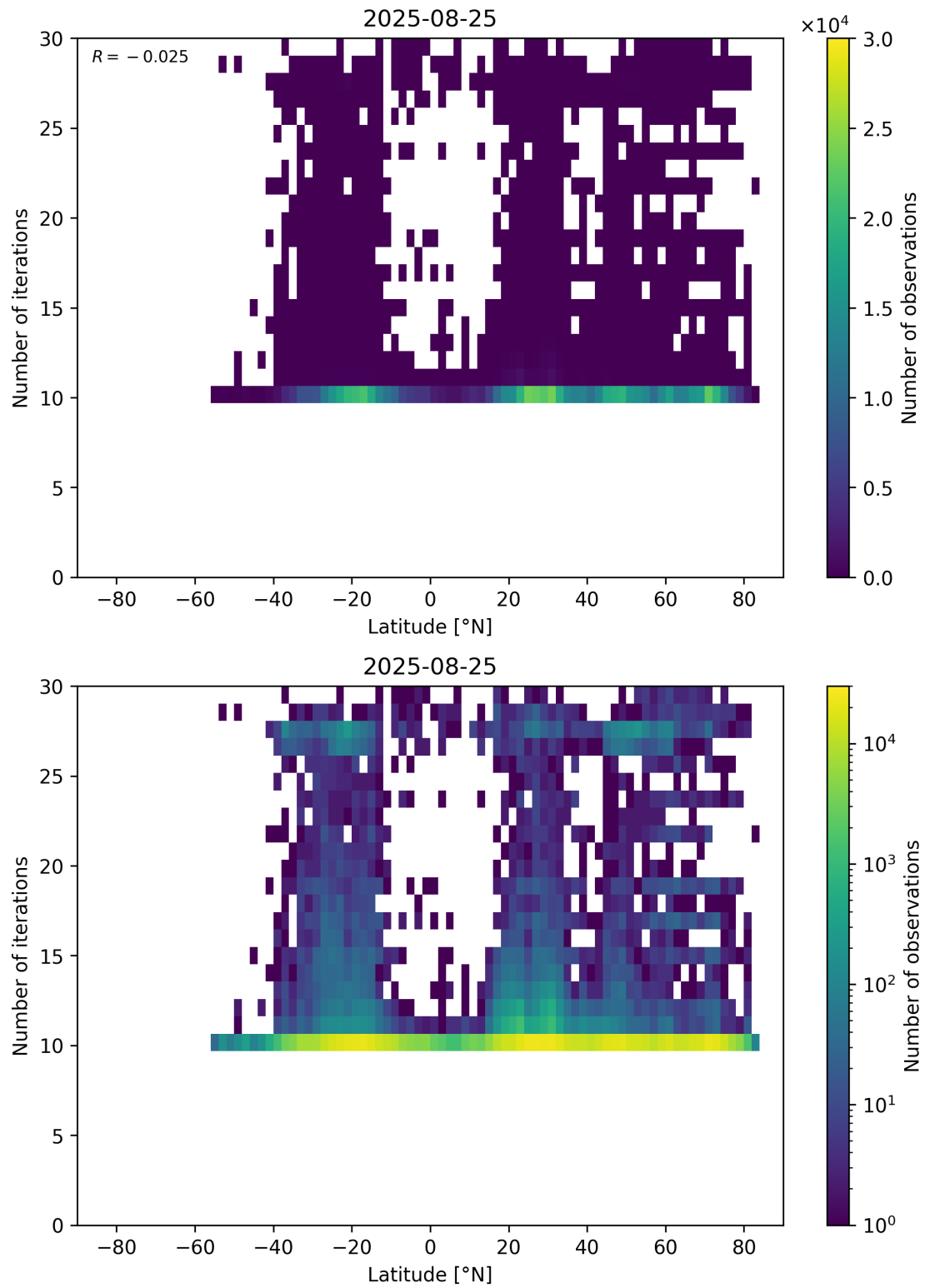
Figure 60: Scatter density plot of “Latitude” against “Number of iterations” for 2025-08-25 to 2025-08-26.
