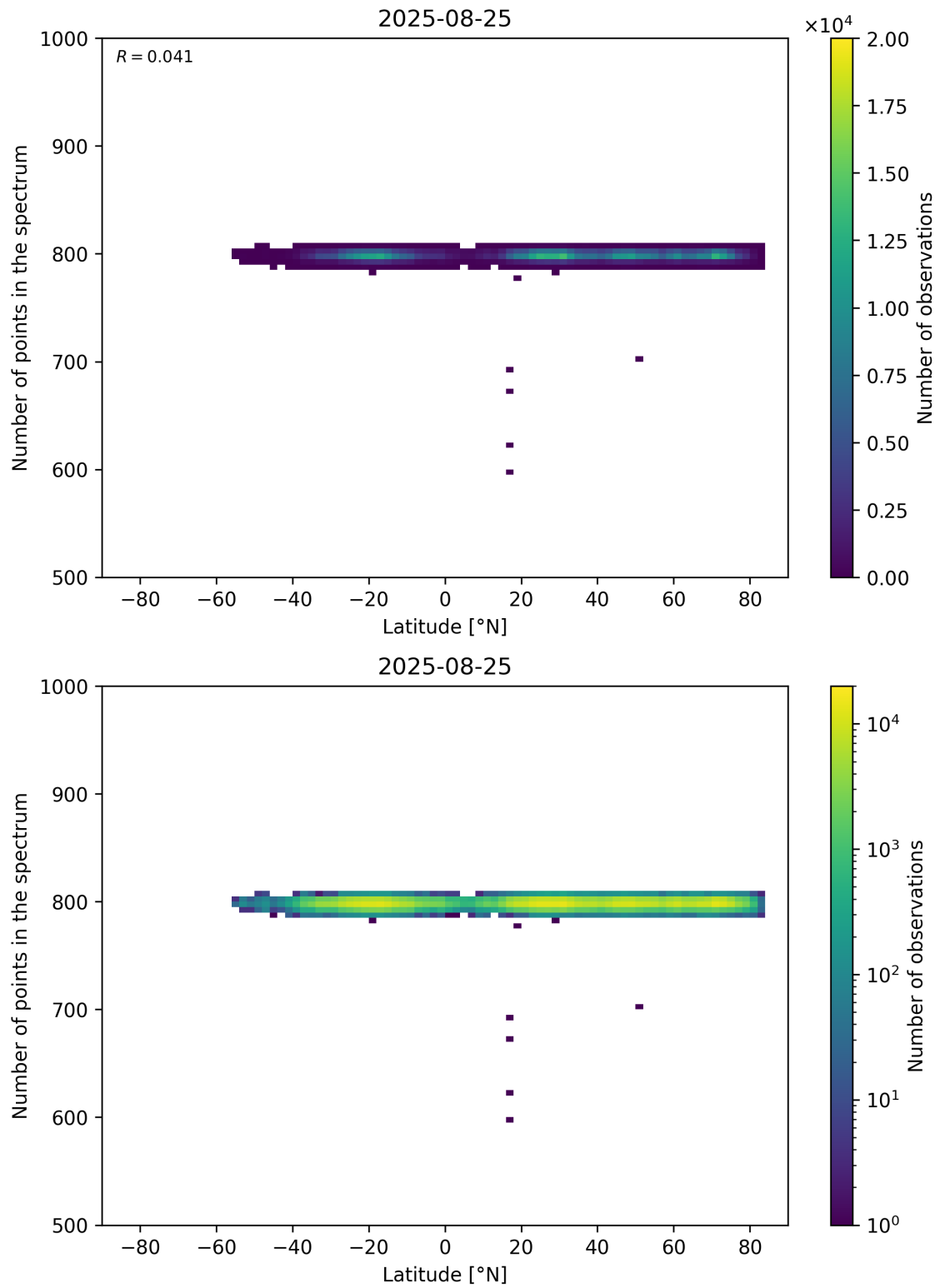
Figure 61: Scatter density plot of “Latitude” against “Number of points in the spectrum” for 2025-08-25 to 2025-08-26.
