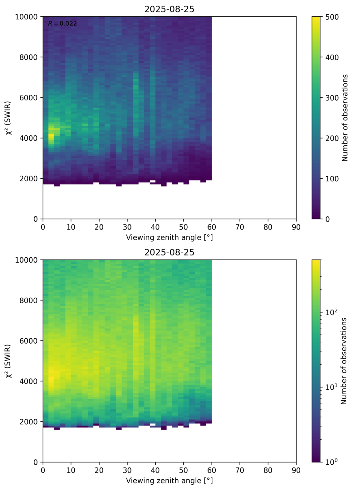
Figure 106: Scatter density plot of “Viewing zenith angle” against “ \chi^2 (SWIR)” for 2025-08-25 to 2025-08-26.
