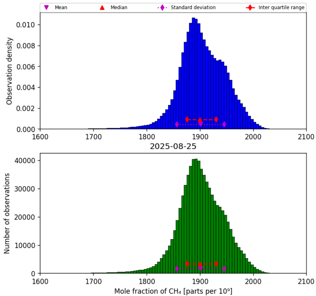
Figure 23: Histogram of “Mole fraction of CH 4 ” for 2025-08-25 to 2025-08-26
