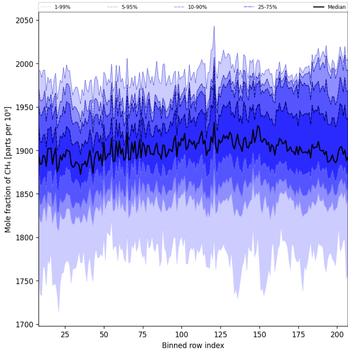
Figure 34: Along track statistics of “Mole fraction of CH 4 ” for 2025-08-25 to 2025-08-26
