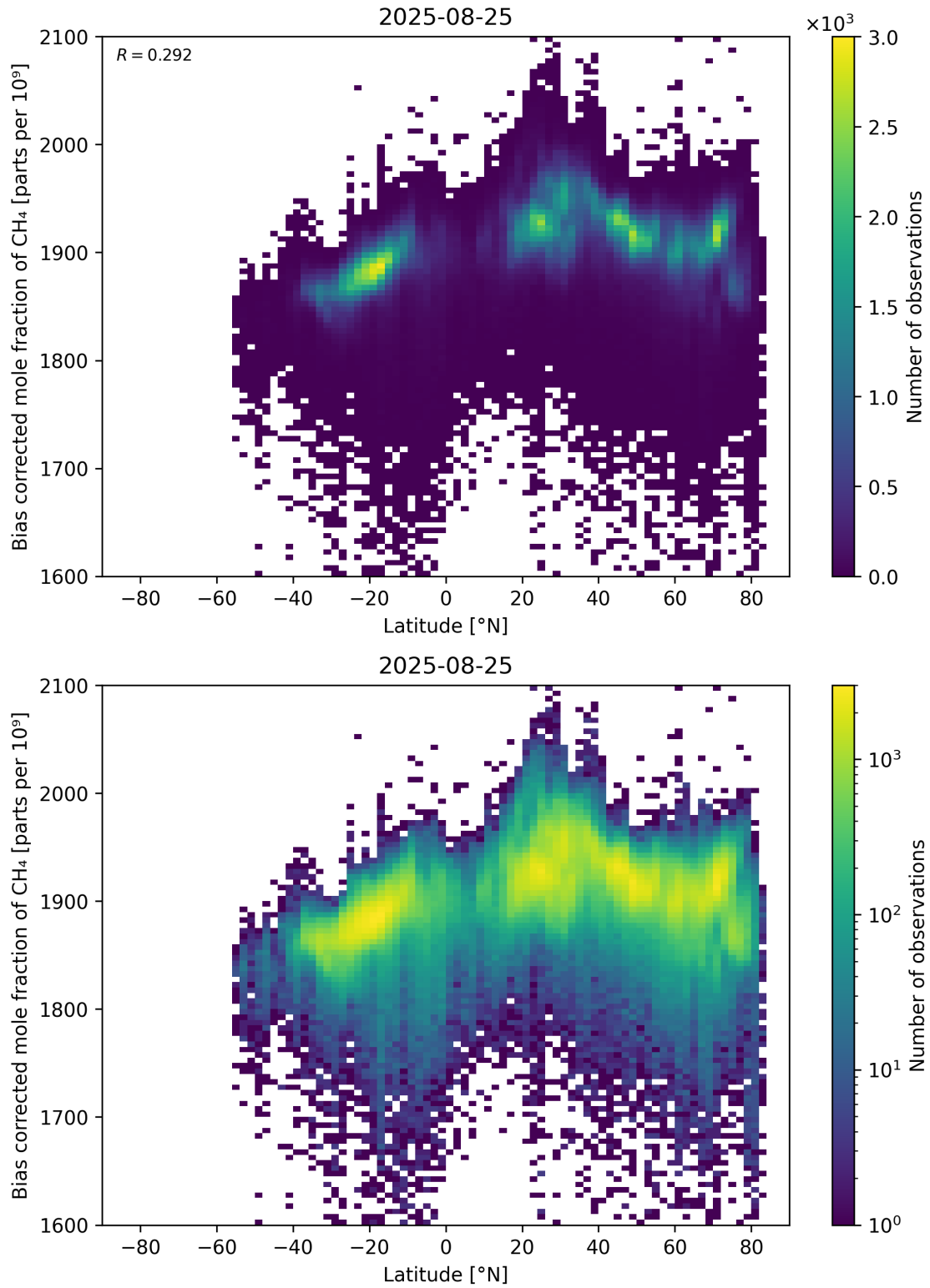
Figure 58: Scatter density plot of “Latitude” against “Bias corrected mole fraction of CH 4 ” for 2025-08-25 to 2025-08-26.
