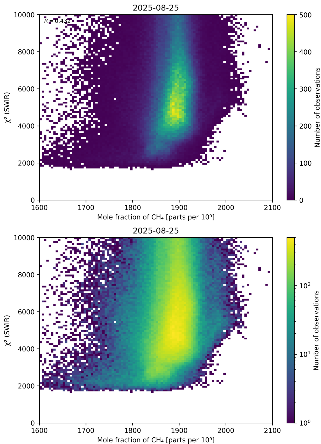
Figure 71: Scatter density plot of “Mole fraction of \text{CH}_4 ” against “ \chi^2 (SWIR)” for 2025-08-25 to 2025-08-26.
