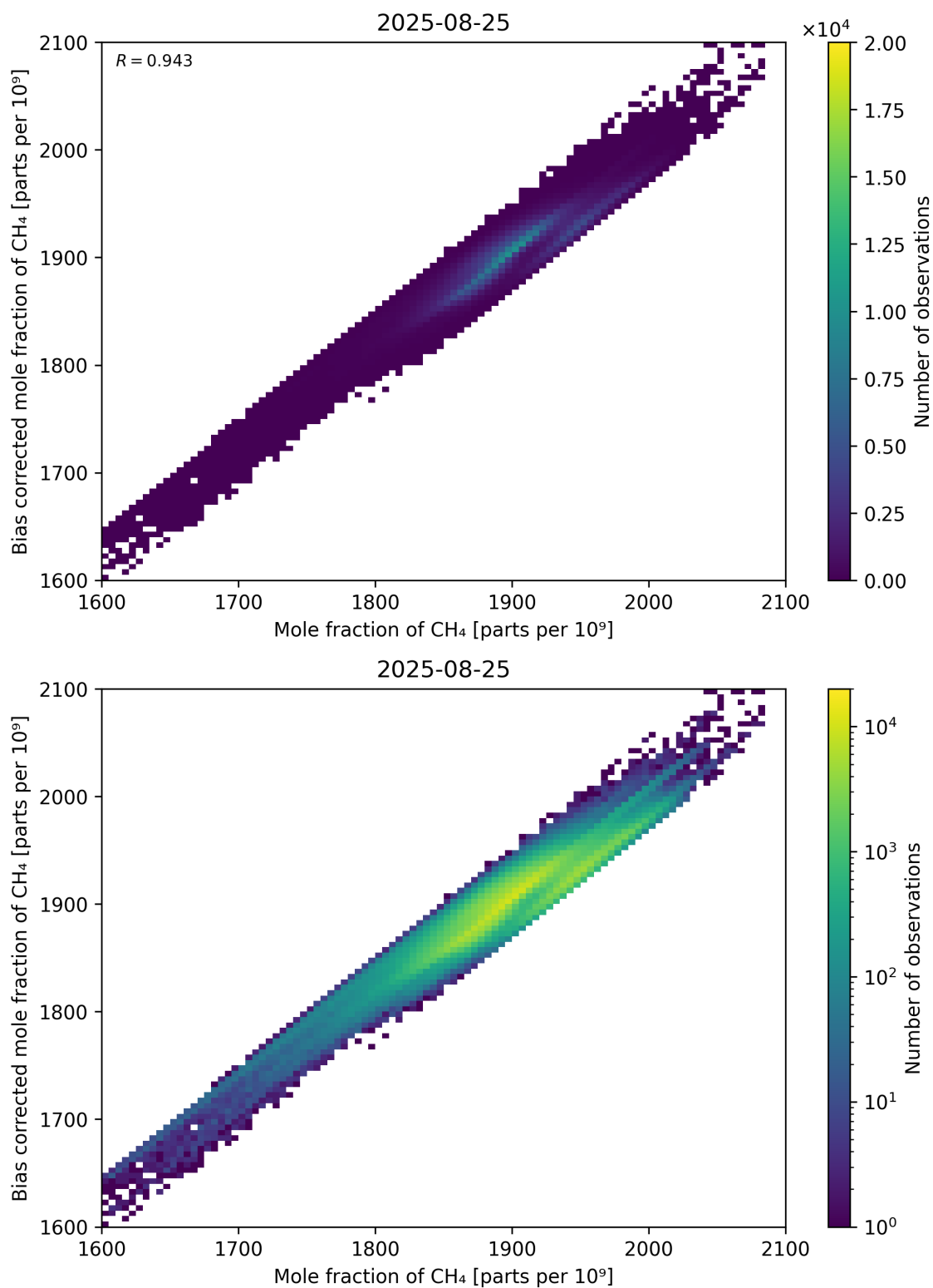
Figure 74: Scatter density plot of “Mole fraction of CH 4 ” against “Bias corrected mole fraction of CH 4 ” for 2025-08-25 to 2025-08-26.
