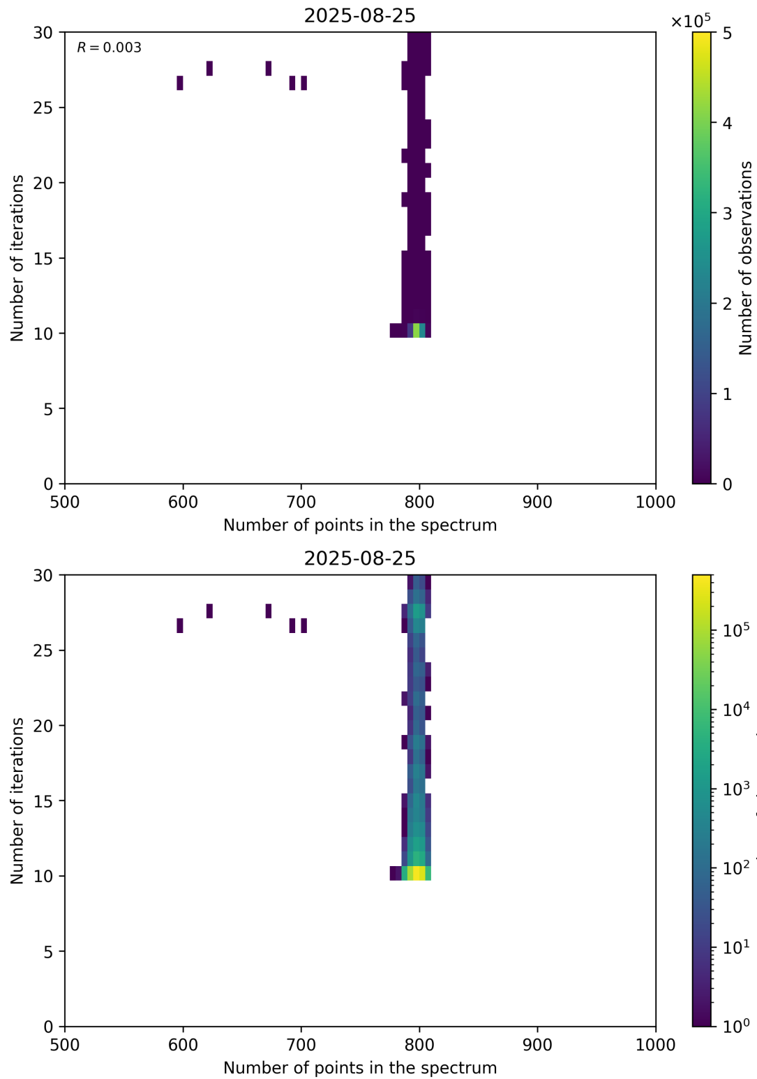
Figure 92: Scatter density plot of “Number of points in the spectrum” against “Number of iterations” for 2025-08-25 to 2025-08-26.
