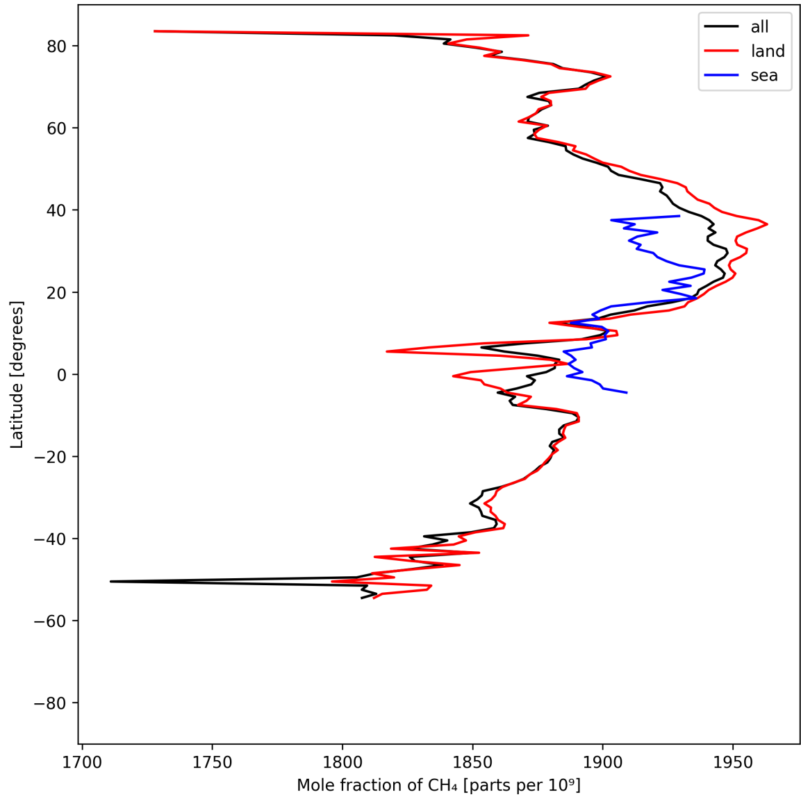
Figure 12: Zonal average of “Mole fraction of \text{CH}_4 ” for 2025-08-25 to 2025-08-26.
