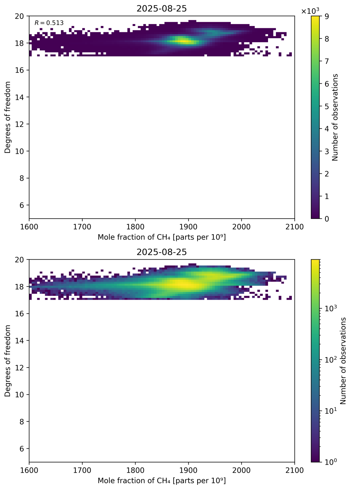
Figure 72: Scatter density plot of “Mole fraction of CH 4 ” against “Degrees of freedom” for 2025-08-25 to 2025-08-26.
