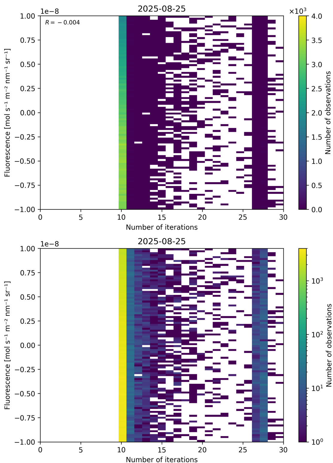
Figure 87: Scatter density plot of “Number of iterations” against “Fluorescence” for 2025-08-25 to 2025-08-26.
