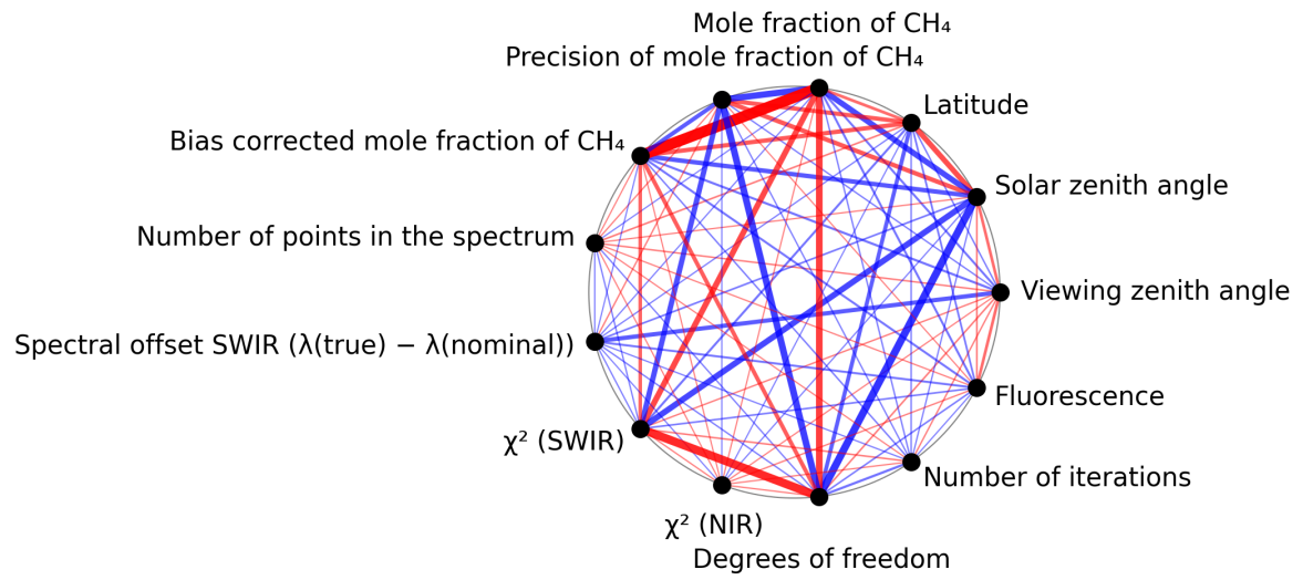
Figure 1: Map of correlation graph for 2025-08-25 to 2025-08-26.
