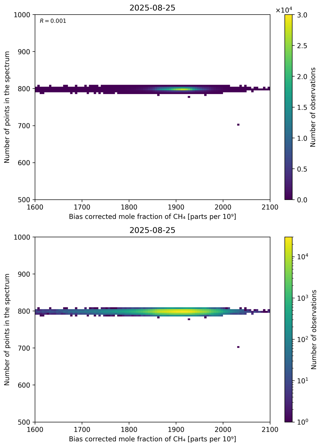
Figure 68: Scatter density plot of “Bias corrected mole fraction of CH 4 ” against “Number of points in the spectrum” for 2025-08-25 to 2025-08-26.
