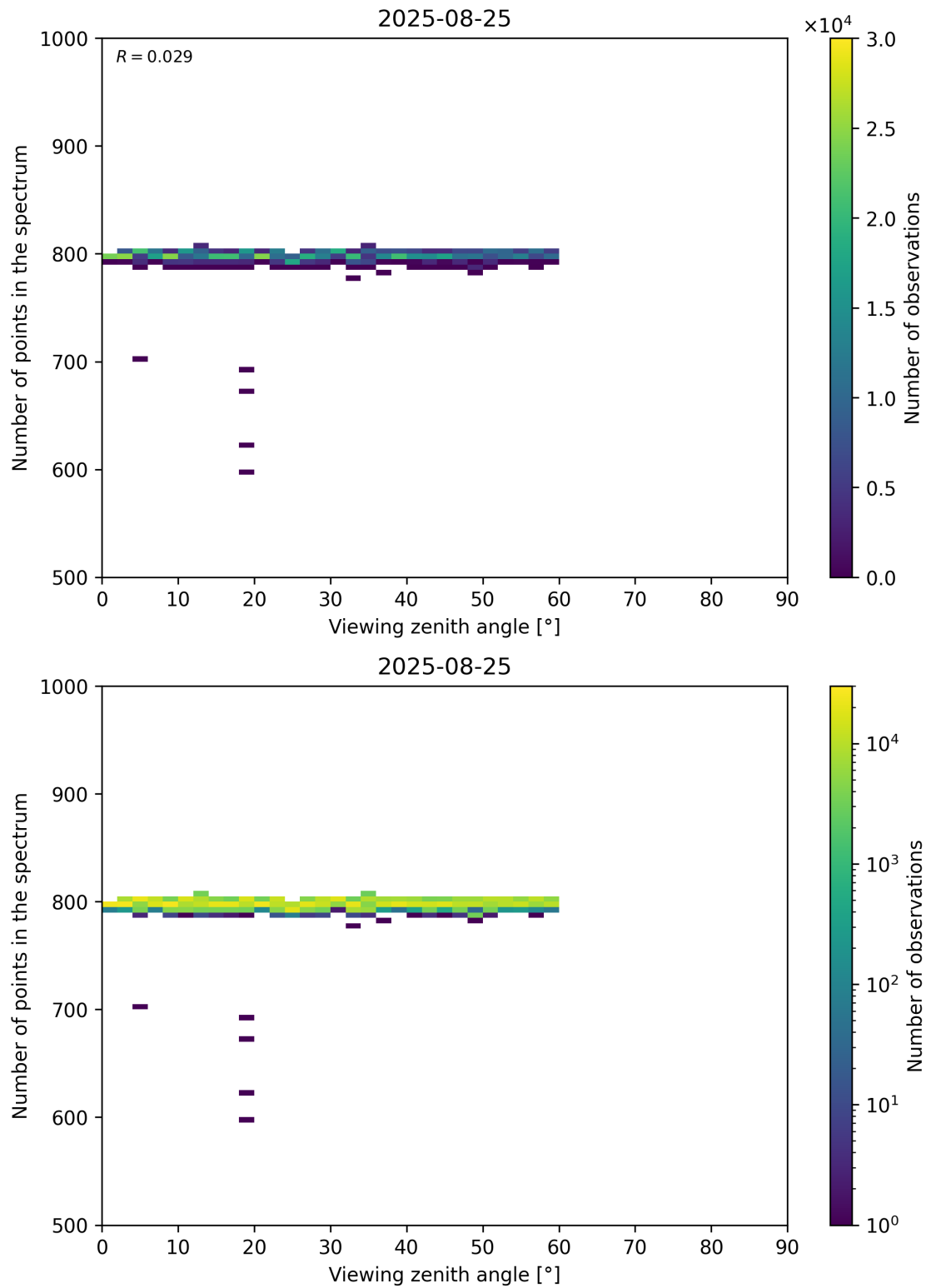
Figure 114: Scatter density plot of “Viewing zenith angle” against “Number of points in the spectrum” for 2025-08-25 to 2025-08-26.
