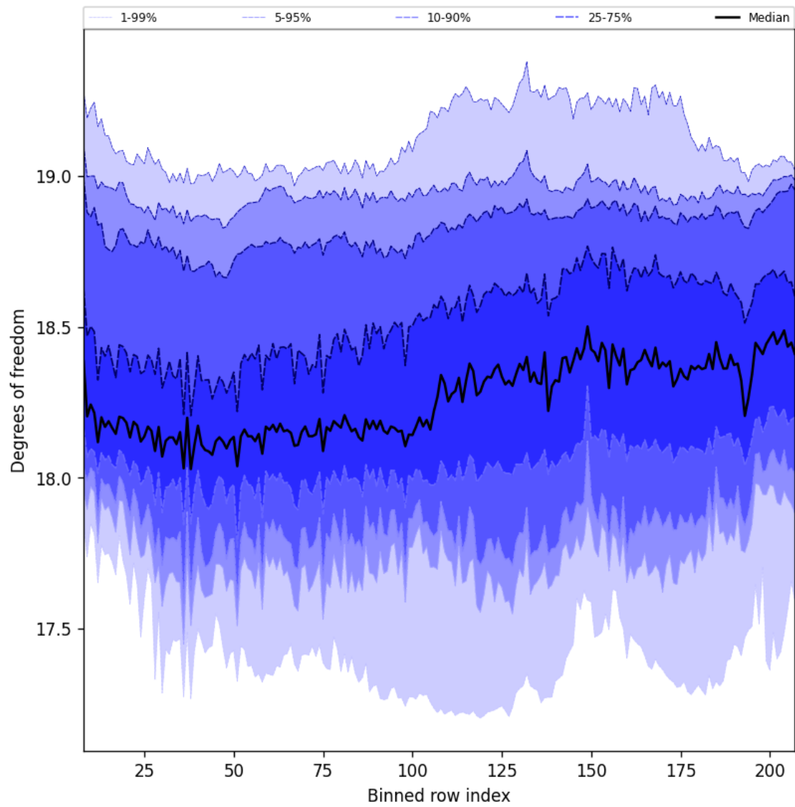
Figure 41: Along track statistics of “Degrees of freedom” for 2025-08-25 to 2025-08-26
