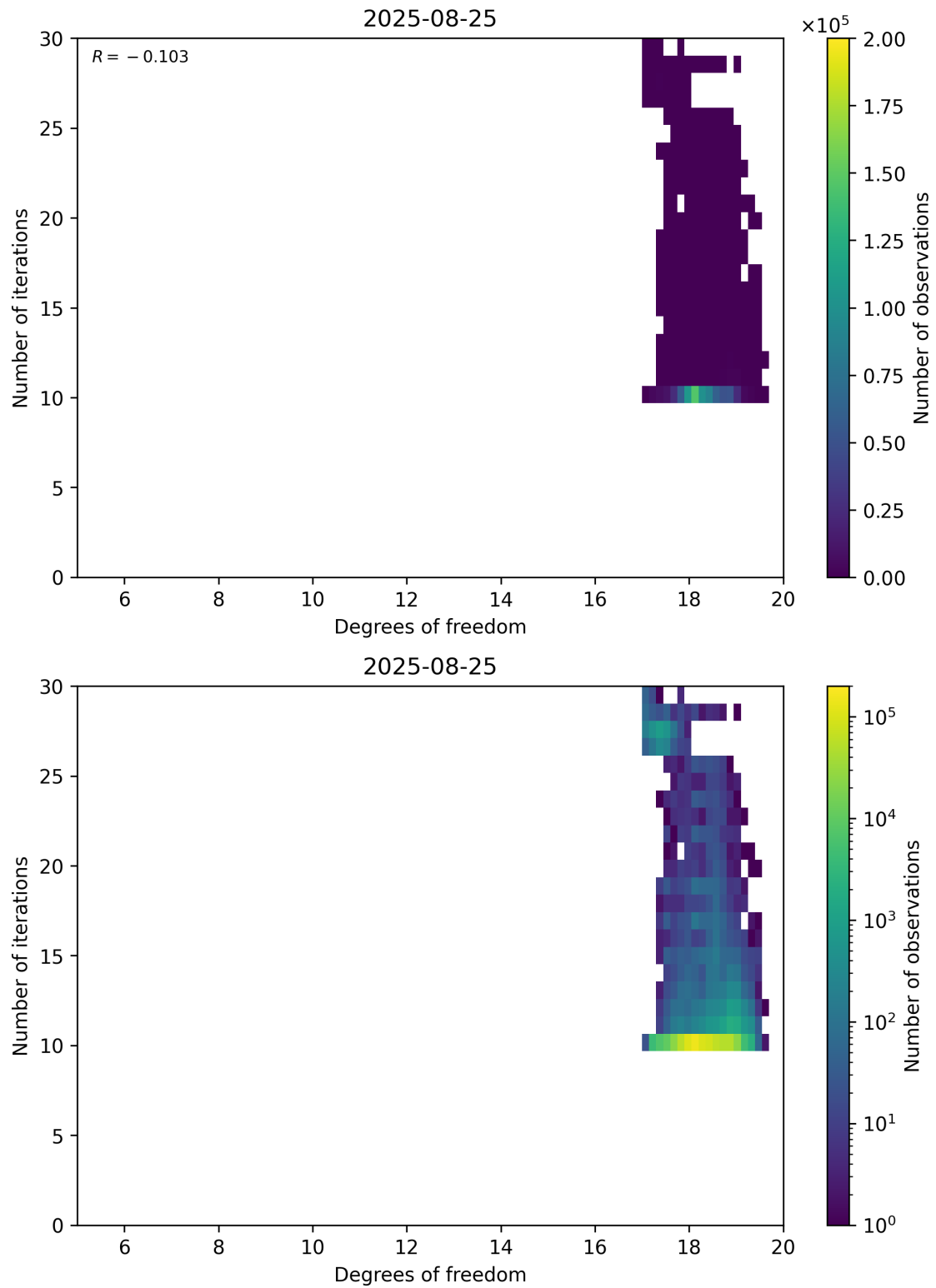
Figure 52: Scatter density plot of “Degrees of freedom” against “Number of iterations” for 2025-08-25 to 2025-08-26.
