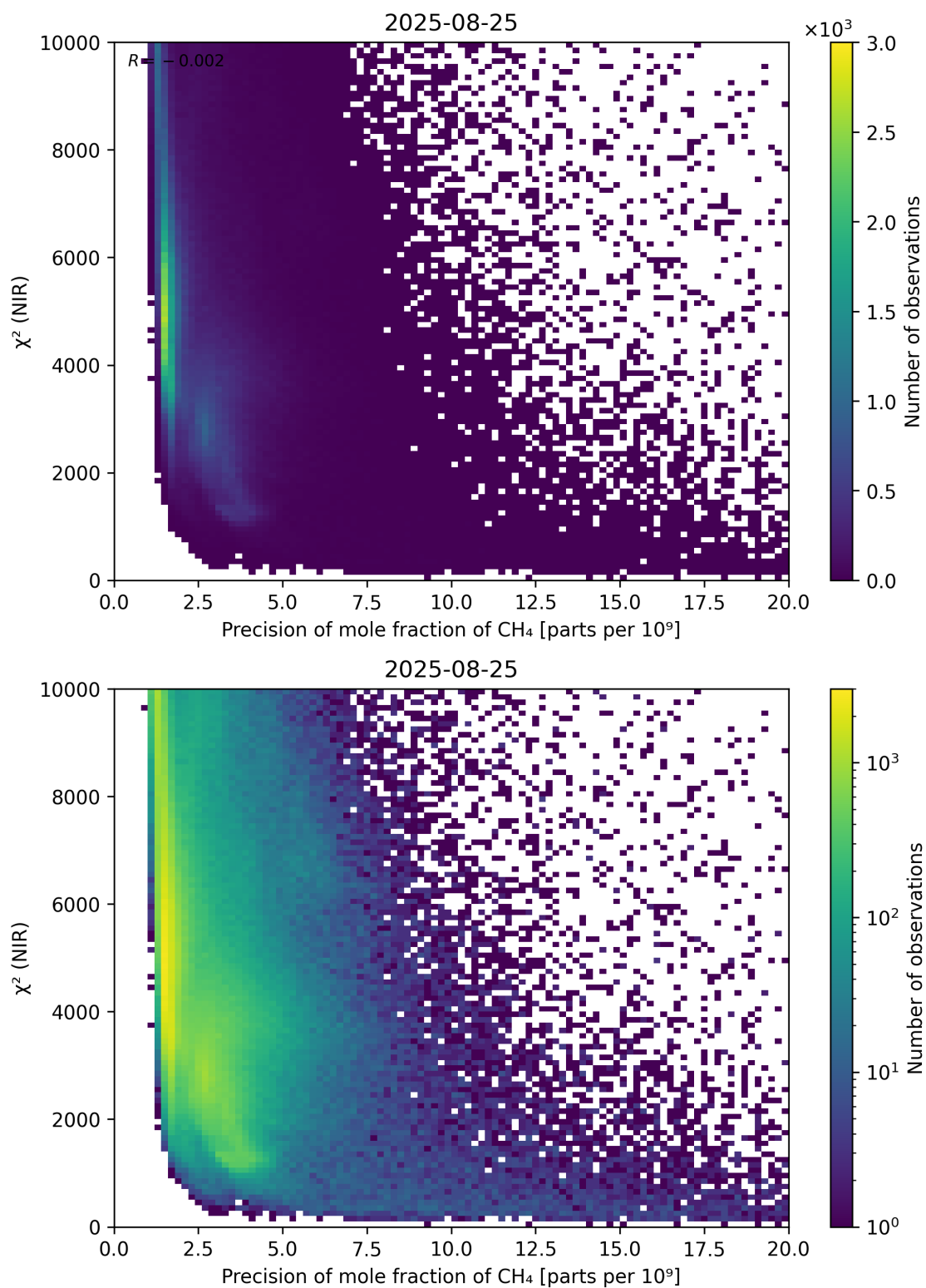
Figure 78: Scatter density plot of “Precision of mole fraction of CH 4 ” against “ \chi^2 (NIR)” for 2025-08-25 to 2025-08-26.
