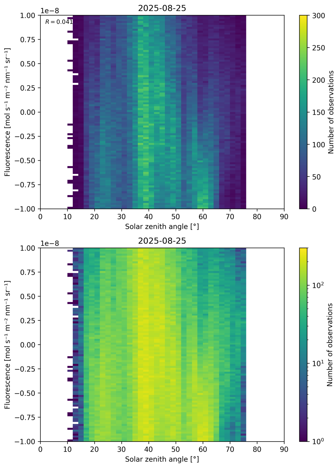
Figure 97: Scatter density plot of “Solar zenith angle” against “Fluorescence” for 2025-08-25 to 2025-08-26.
