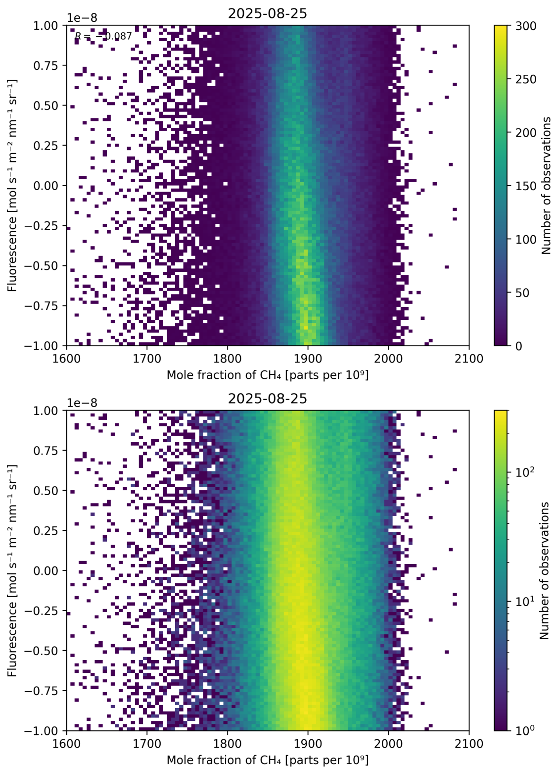
Figure 73: Scatter density plot of “Mole fraction of \text{CH}_4 ” against “Fluorescence” for 2025-08-25 to 2025-08-26.
