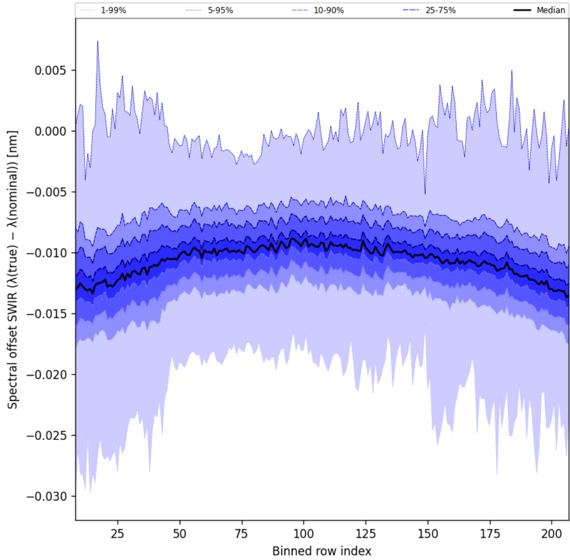
Figure 38: Along track statistics of “Spectral offset SWIR ( \lambda_{\text{true}} - \lambda_{\text{nominal}} )” for 2025-08-25 to 2025-08-26
