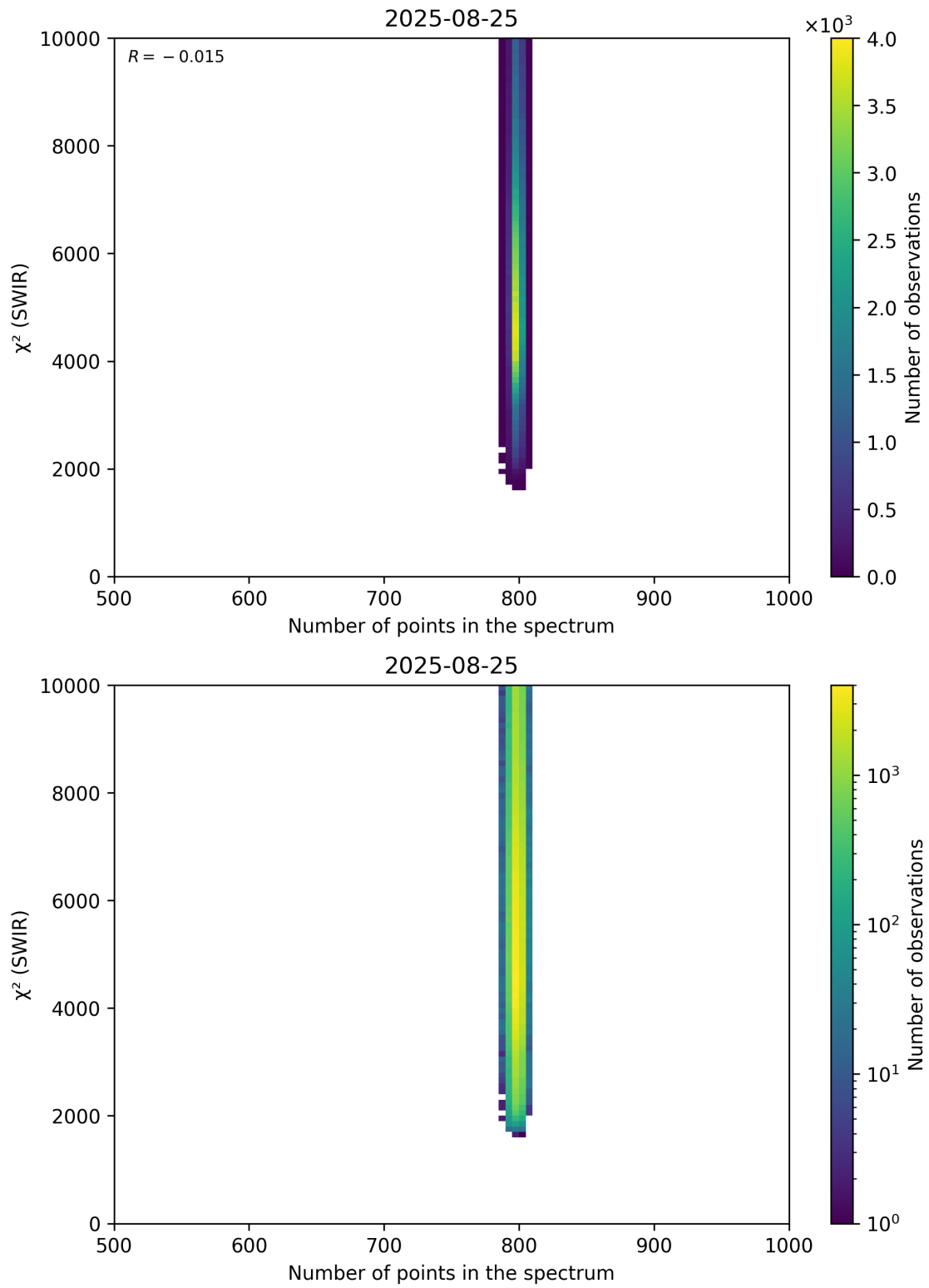
Figure 89: Scatter density plot of “Number of points in the spectrum” against “ \chi^2 (SWIR)” for 2025-08-25 to 2025-08-26.
