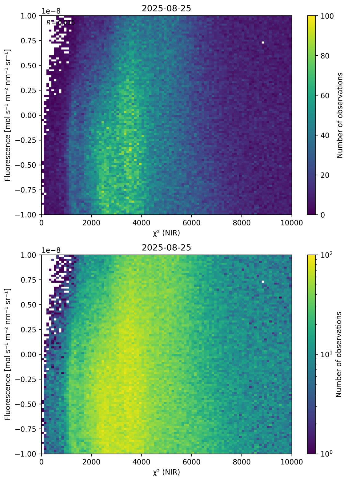
Figure 45: Scatter density plot of “ \chi^2 (NIR)” against “Fluorescence” for 2025-08-25 to 2025-08-26.
