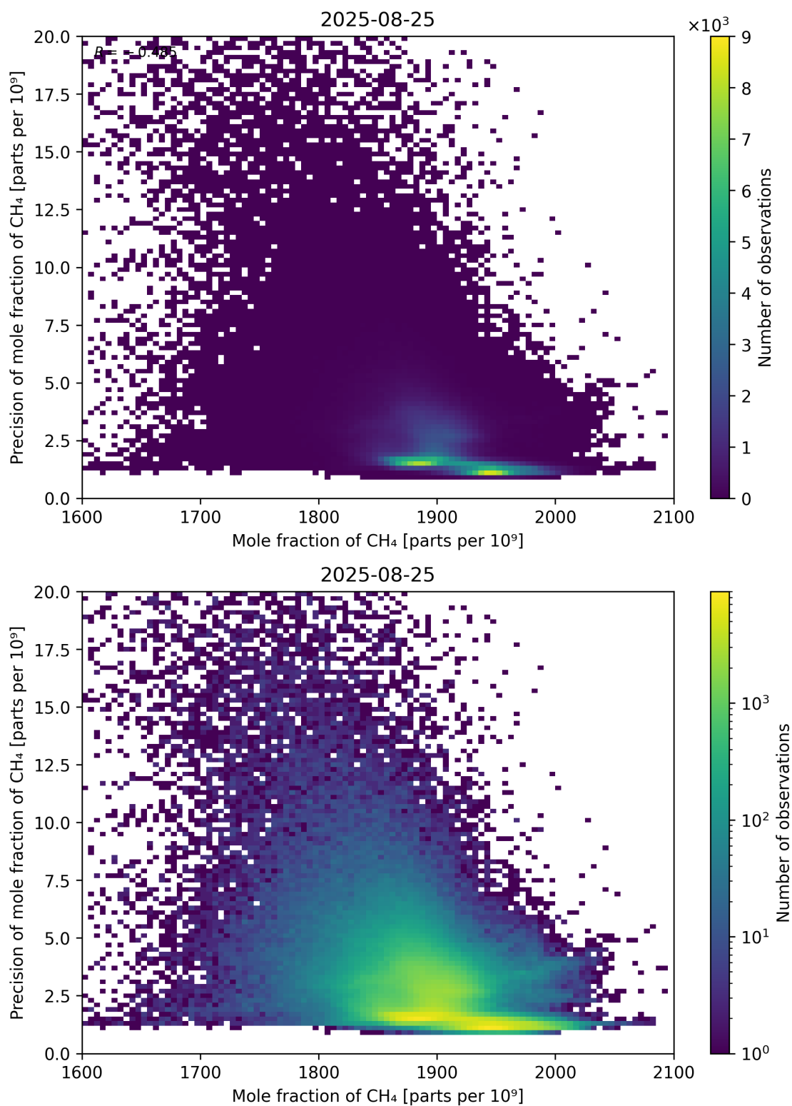
Figure 75: Scatter density plot of “Mole fraction of CH 4 ” against “Precision of mole fraction of CH 4 ” for 2025-08-25 to 2025-08-26.
