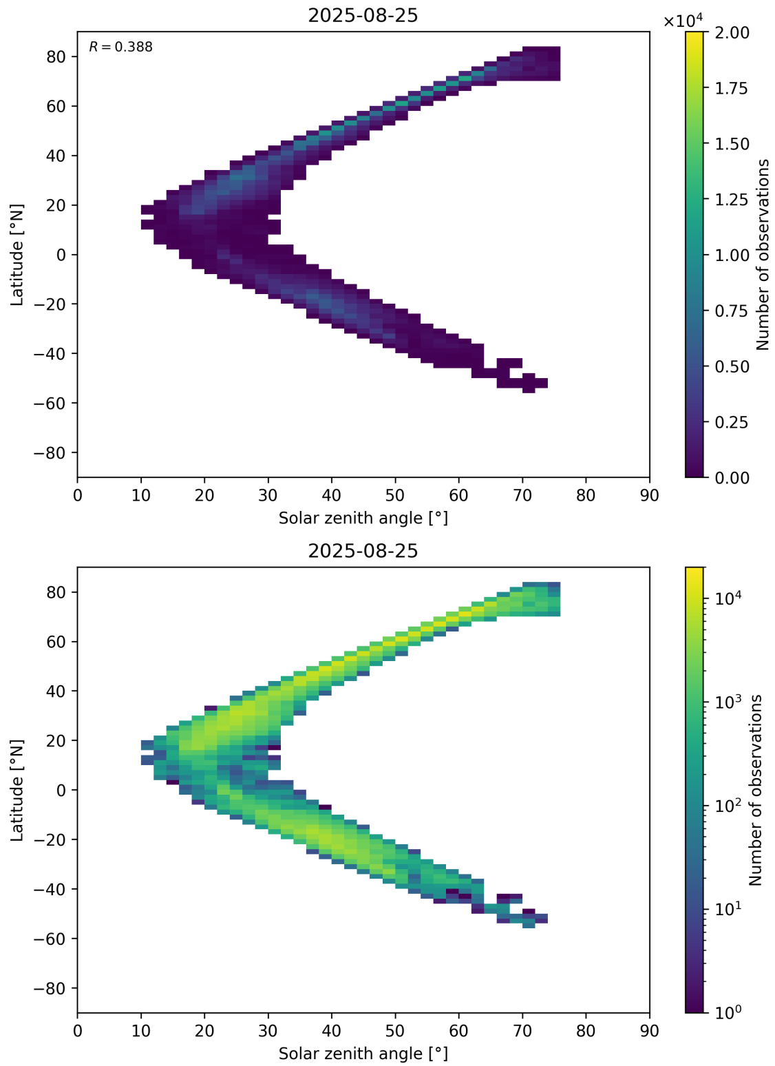
Figure 98: Scatter density plot of “Solar zenith angle” against “Latitude” for 2025-08-25 to 2025-08-26.
