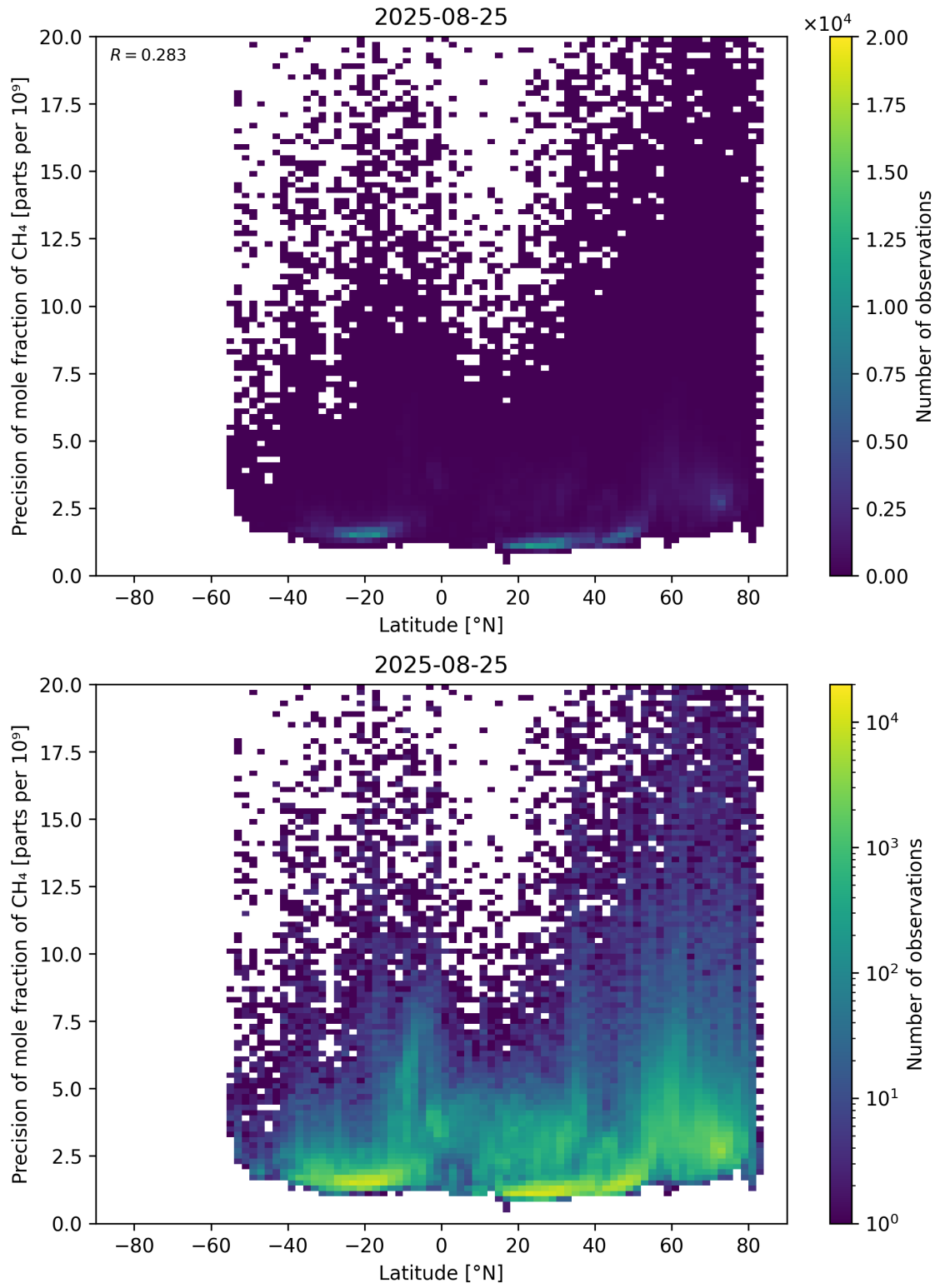
Figure 59: Scatter density plot of “Latitude” against “Precision of mole fraction of \text{CH}_4 ” for 2025-08-25 to 2025-08-26.
