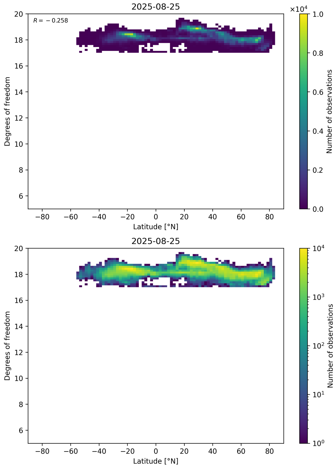
Figure 55: Scatter density plot of “Latitude” against “Degrees of freedom” for 2025-08-25 to 2025-08-26.
