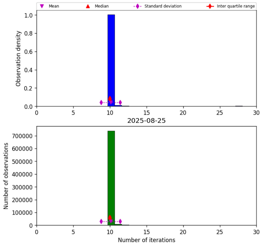
Figure 31: Histogram of “Number of iterations” for 2025-08-25 to 2025-08-26
