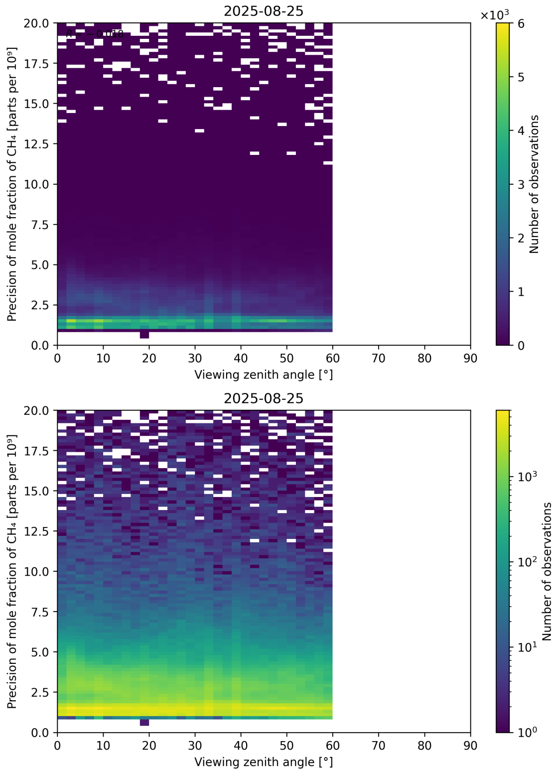
Figure 112: Scatter density plot of “Viewing zenith angle” against “Precision of mole fraction of CH 4 ” for 2025-08-25 to 2025-08-26.
