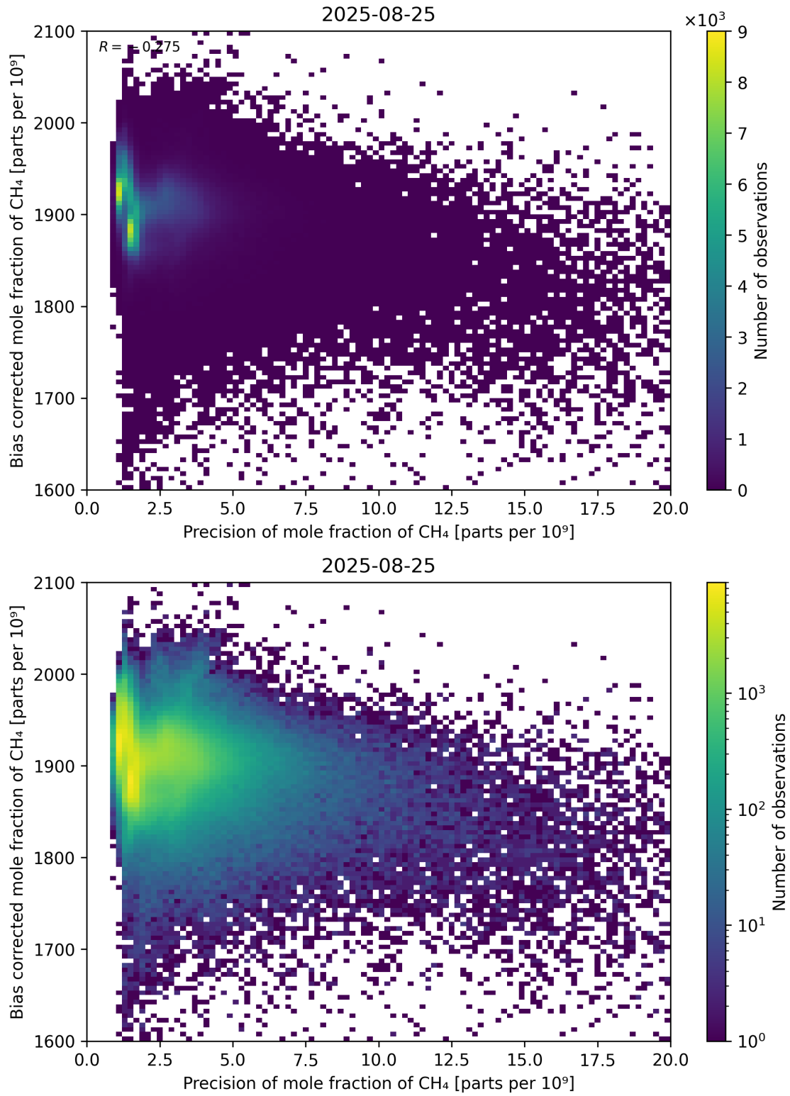
Figure 82: Scatter density plot of “Precision of mole fraction of CH 4 ” against “Bias corrected mole fraction of CH 4 ” for 2025-08-25 to 2025-08-26.
