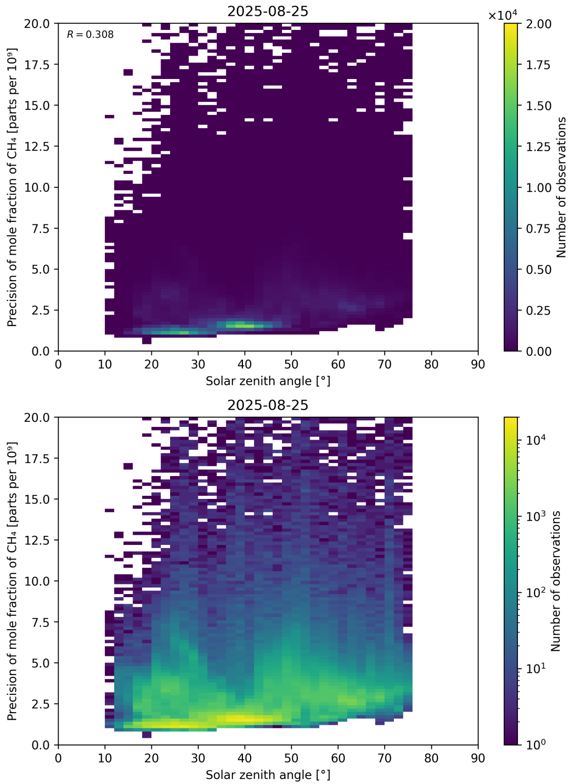
Figure 101: Scatter density plot of “Solar zenith angle” against “Precision of mole fraction of CH 4 ” for 2025-08-25 to 2025-08-26.
