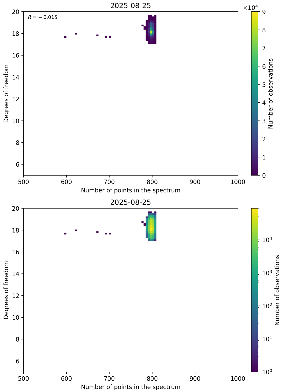
Figure 90: Scatter density plot of “Number of points in the spectrum” against “Degrees of freedom” for 2025-08-25 to 2025-08-26.
