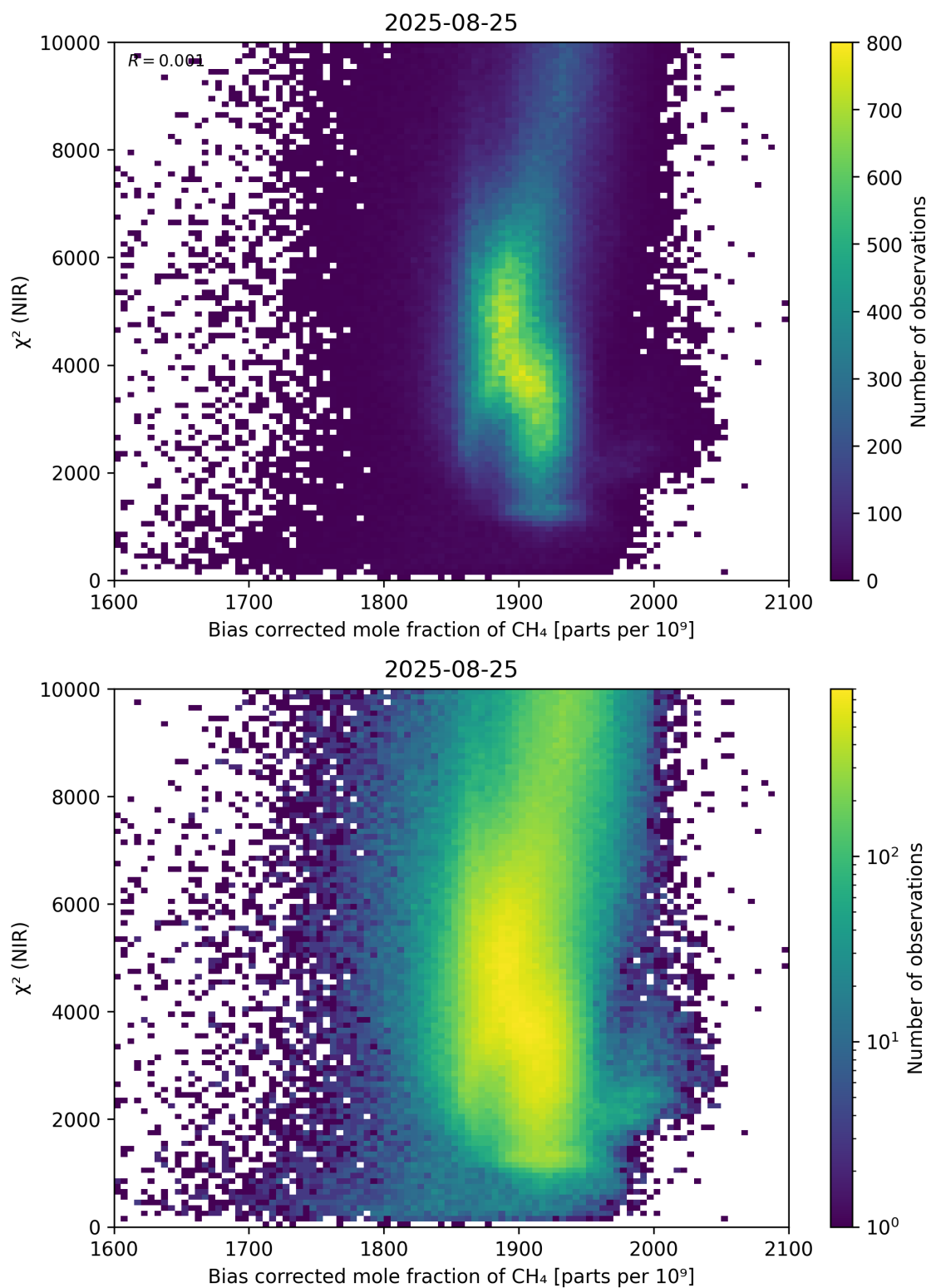
Figure 63: Scatter density plot of “Bias corrected mole fraction of \text{CH}_4 ” against “ \chi^2 (NIR)” for 2025-08-25 to 2025-08-26.
