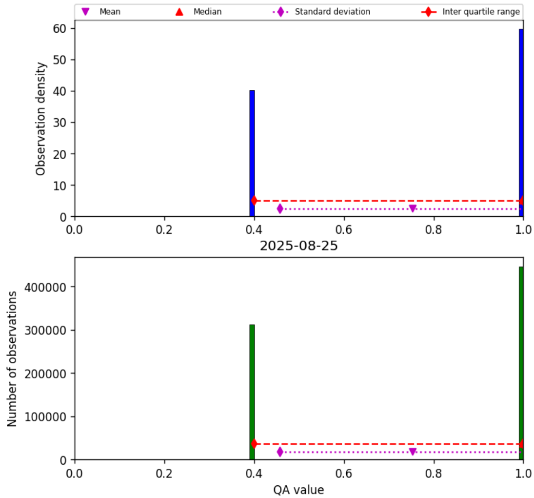
Figure 22: Histogram of “QA value” for 2025-08-25 to 2025-08-26
