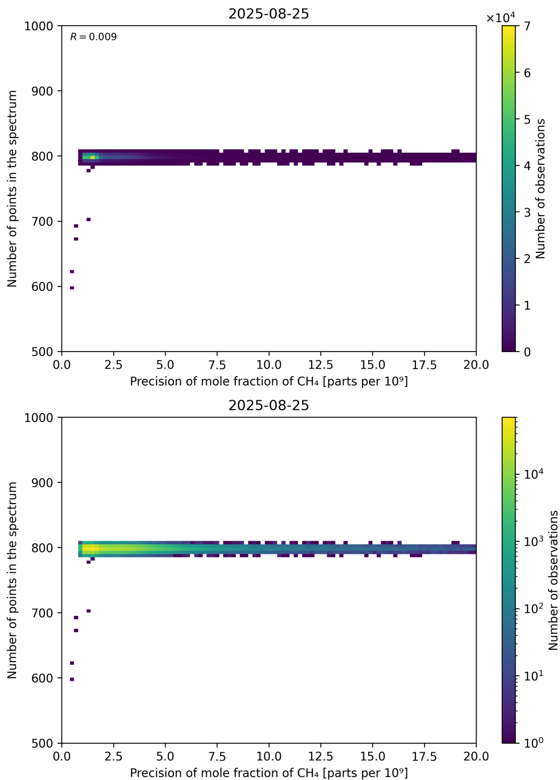
Figure 84: Scatter density plot of “Precision of mole fraction of CH 4 ” against “Number of points in the spectrum” for 2025-08-25 to 2025-08-26.
