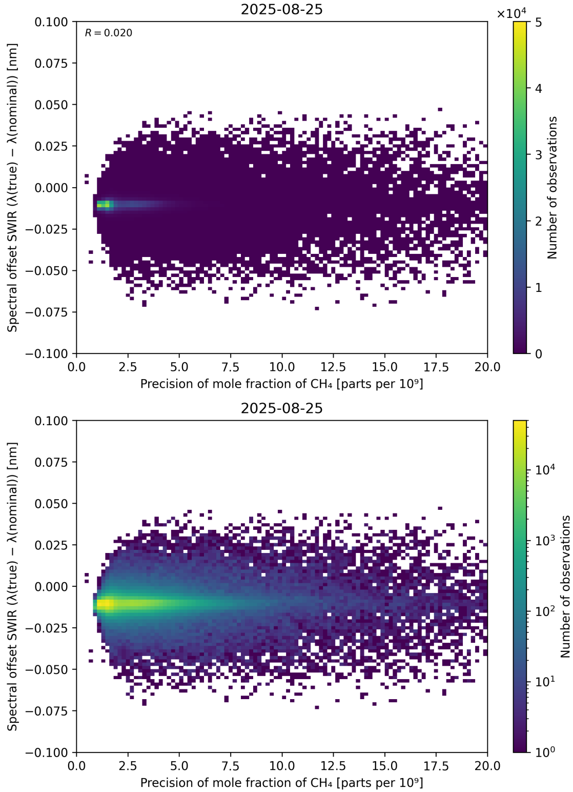
Figure 85: Scatter density plot of “Precision of mole fraction of CH 4 ” against “Spectral offset SWIR ( \lambda_{\text{true}} - \lambda_{\text{nominal}} )” for 2025-08-25 to 2025-08-26.
