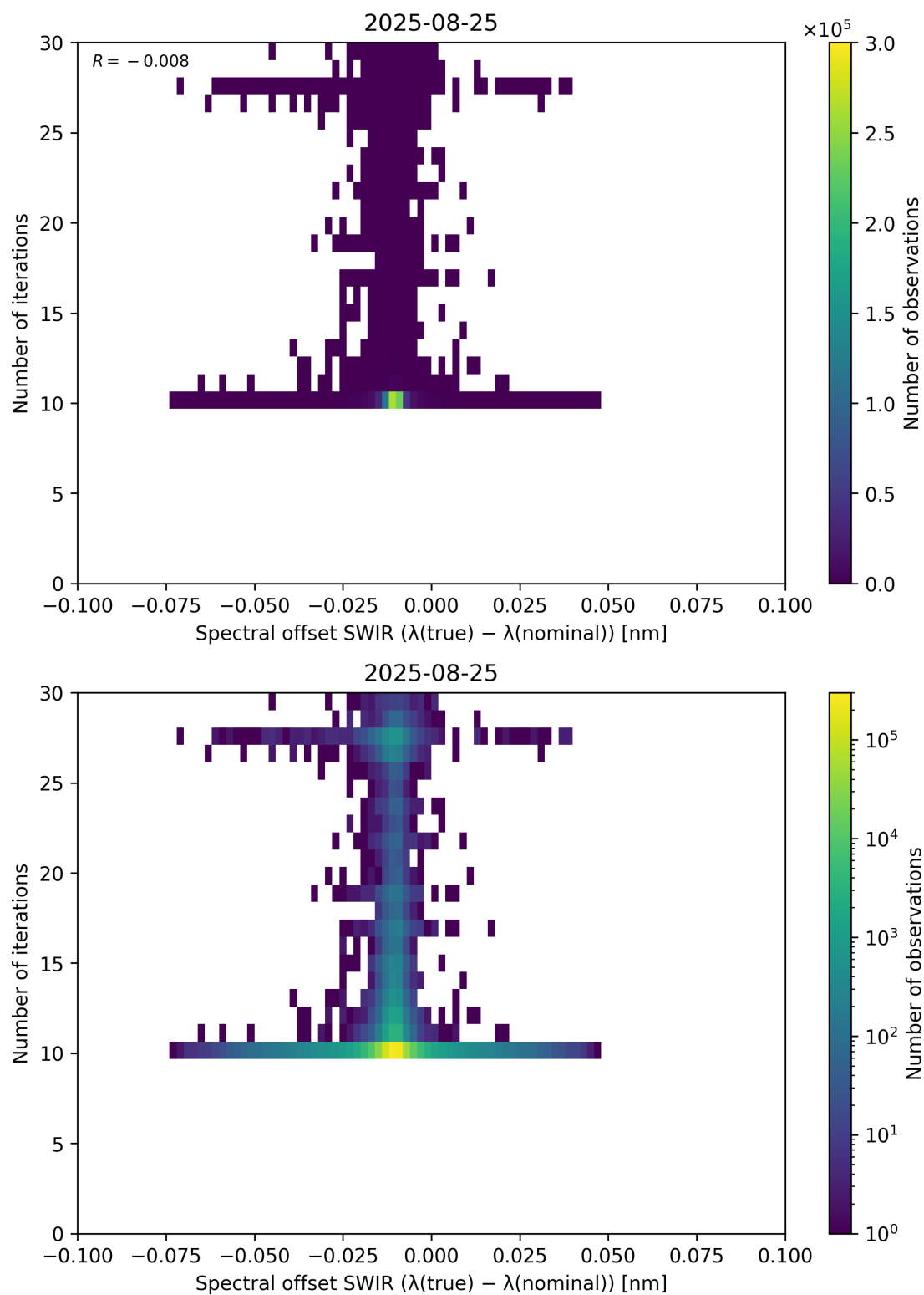
Figure 121: Scatter density plot of “Spectral offset SWIR ( \lambda_{\text{true}} - \lambda_{\text{nominal}} )” against “Number of iterations” for 2025-08-25 to 2025-08-26.
