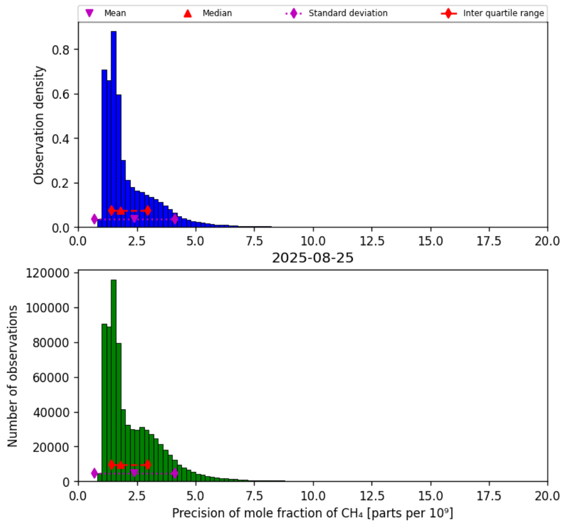
Figure 24: Histogram of “Precision of mole fraction of CH 4 ” for 2025-08-25 to 2025-08-26
