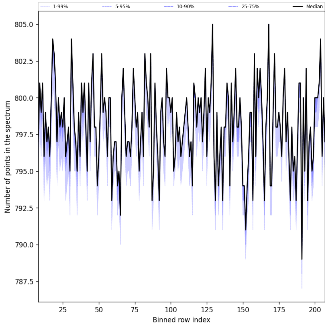
Figure 37: Along track statistics of “Number of points in the spectrum” for 2025-08-25 to 2025-08-26
