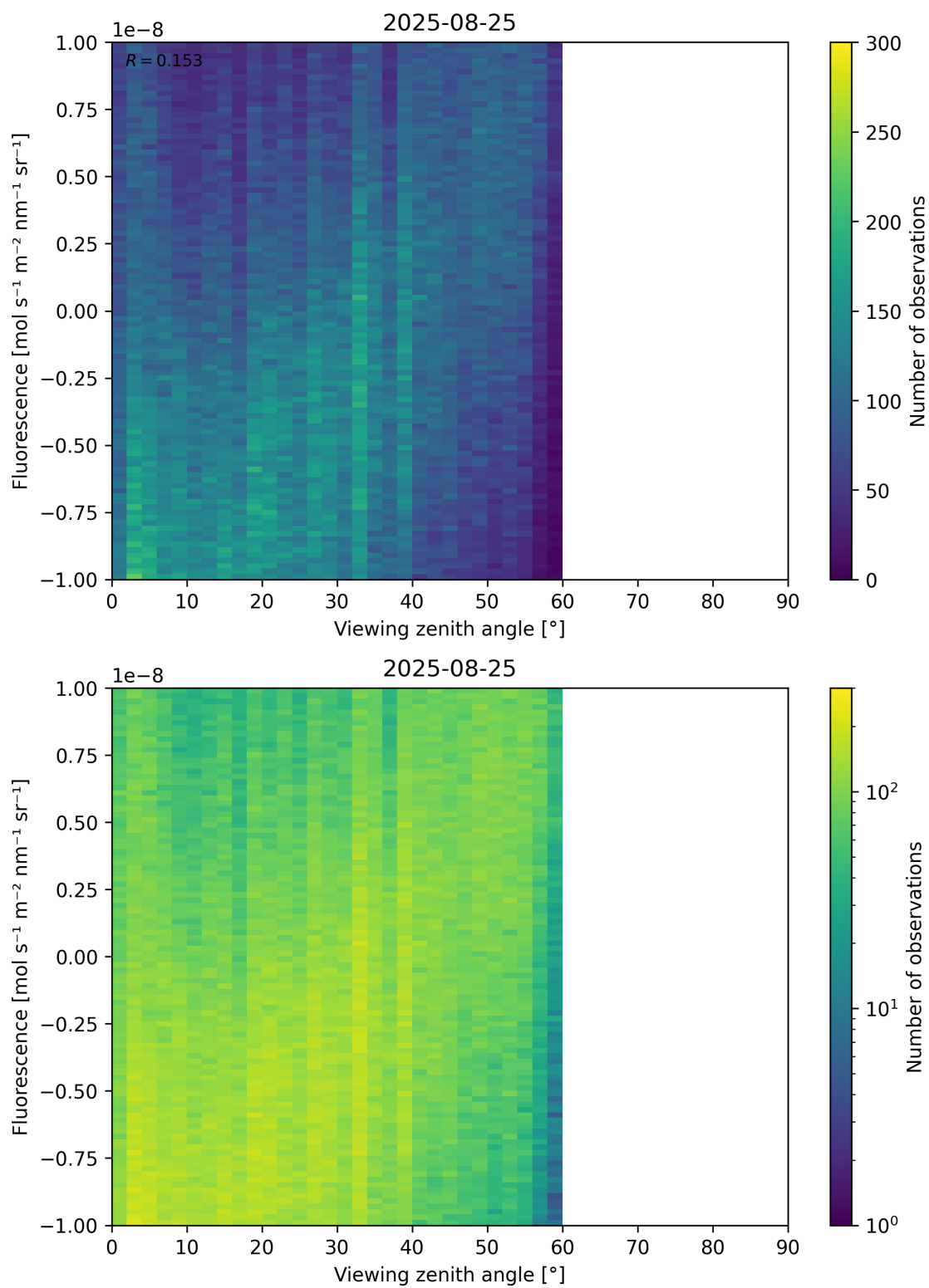
Figure 108: Scatter density plot of “Viewing zenith angle” against “Fluorescence” for 2025-08-25 to 2025-08-26.
