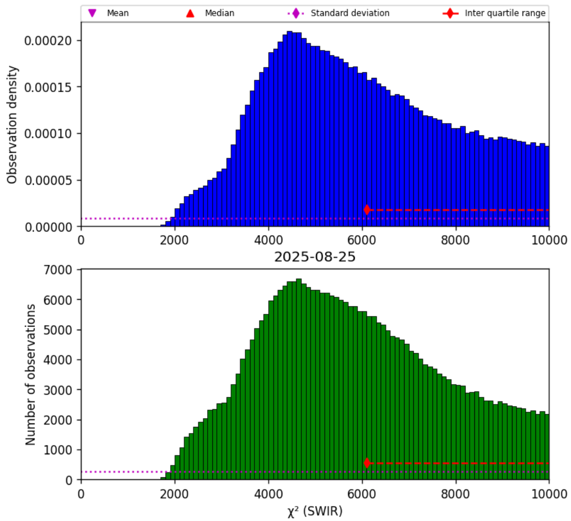
Figure 28: Histogram of “ \chi^2 (SWIR)” for 2025-08-25 to 2025-08-26
