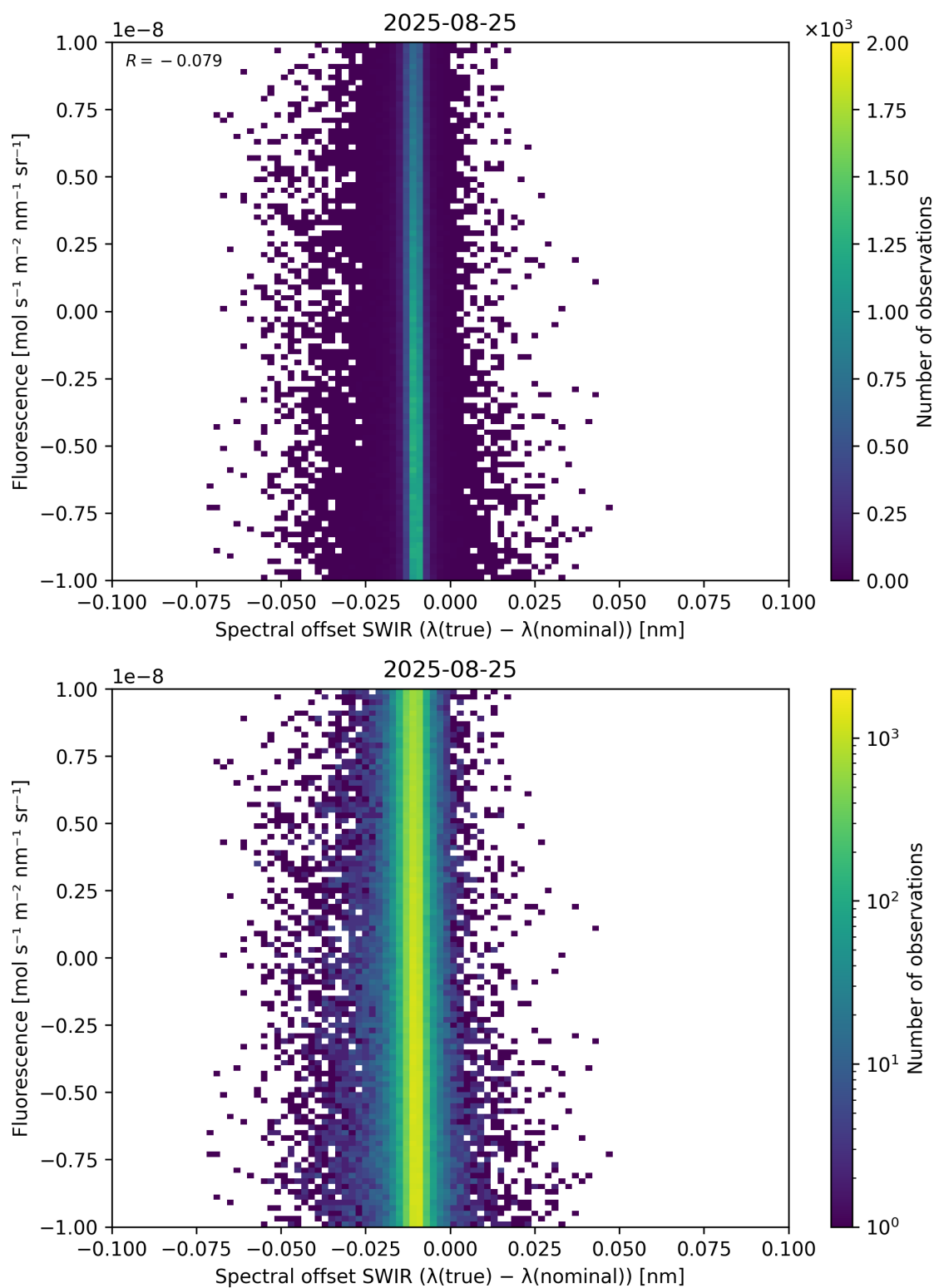
Figure 120: Scatter density plot of “Spectral offset SWIR ( \lambda_{\text{true}} - \lambda_{\text{nominal}} )” against “Fluorescence” for 2025-08-25 to 2025-08-26.
