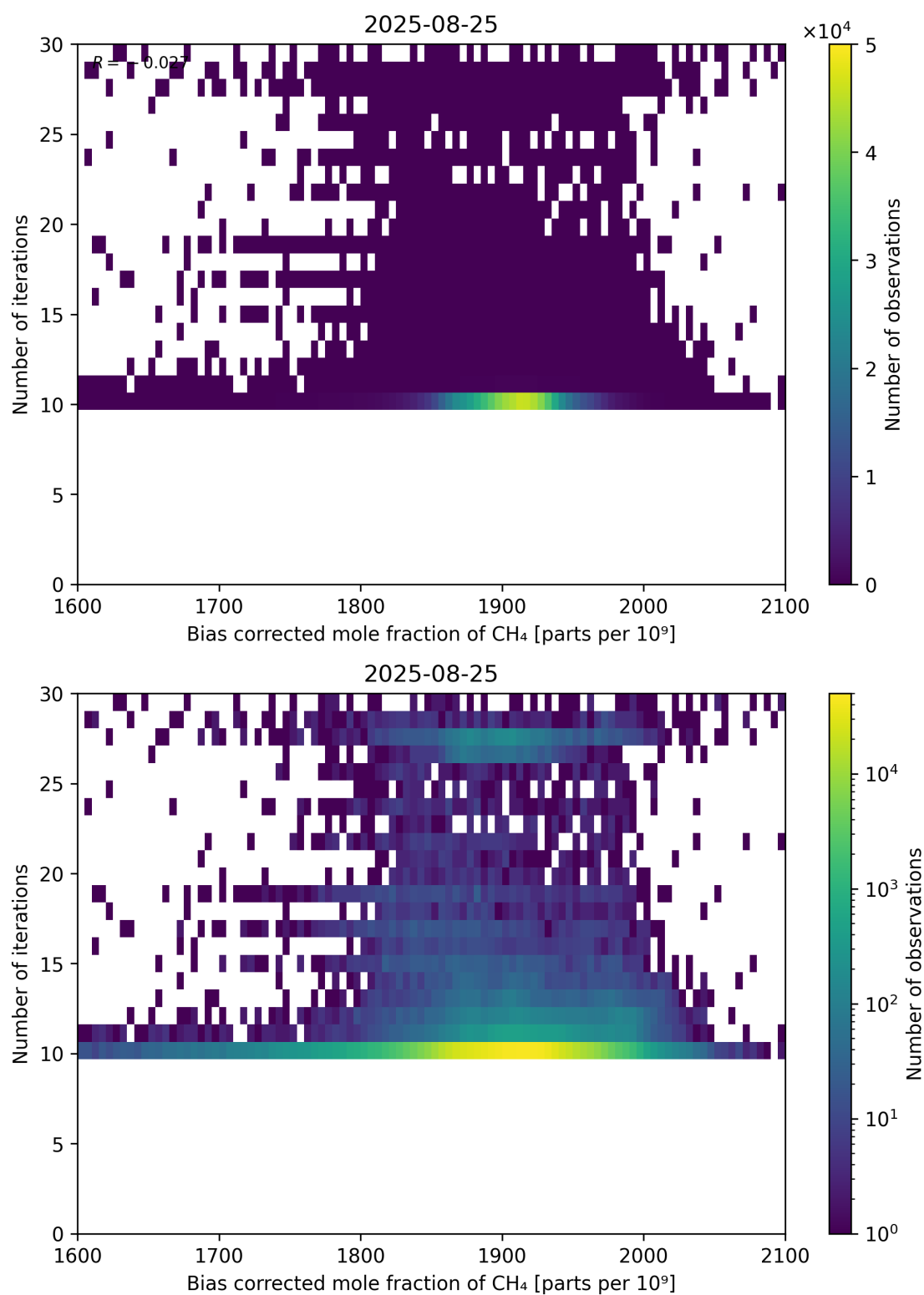
Figure 67: Scatter density plot of “Bias corrected mole fraction of CH 4 ” against “Number of iterations” for 2025-08-25 to 2025-08-26.
