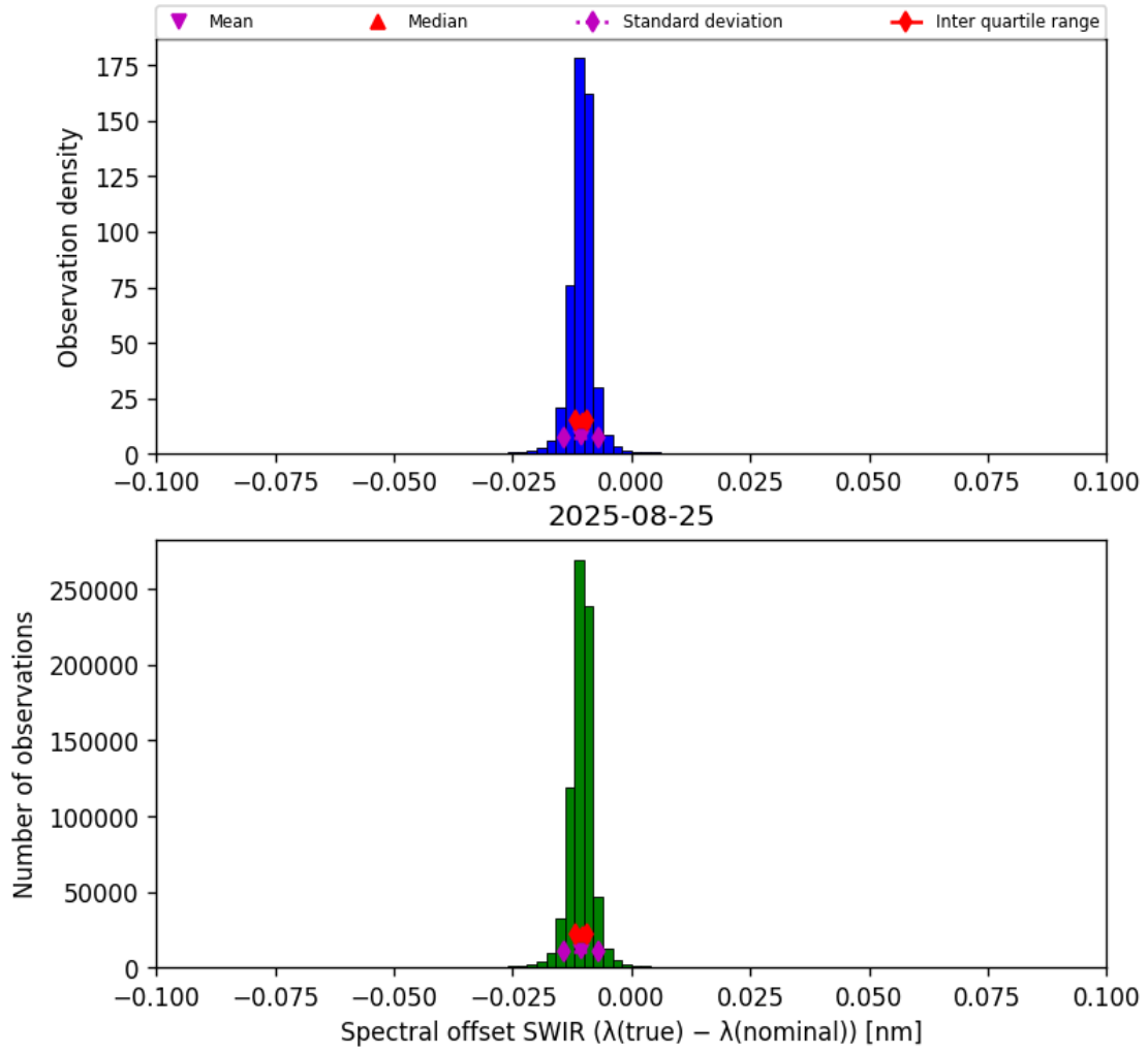
Figure 27: Histogram of “Spectral offset SWIR ( \lambda_{\text{true}} - \lambda_{\text{nominal}} )” for 2025-08-25 to 2025-08-26
