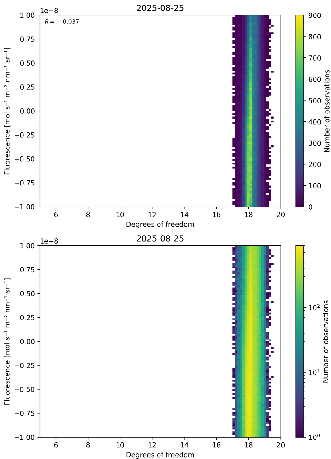
Figure 51: Scatter density plot of “Degrees of freedom” against “Fluorescence” for 2025-08-25 to 2025-08-26.
