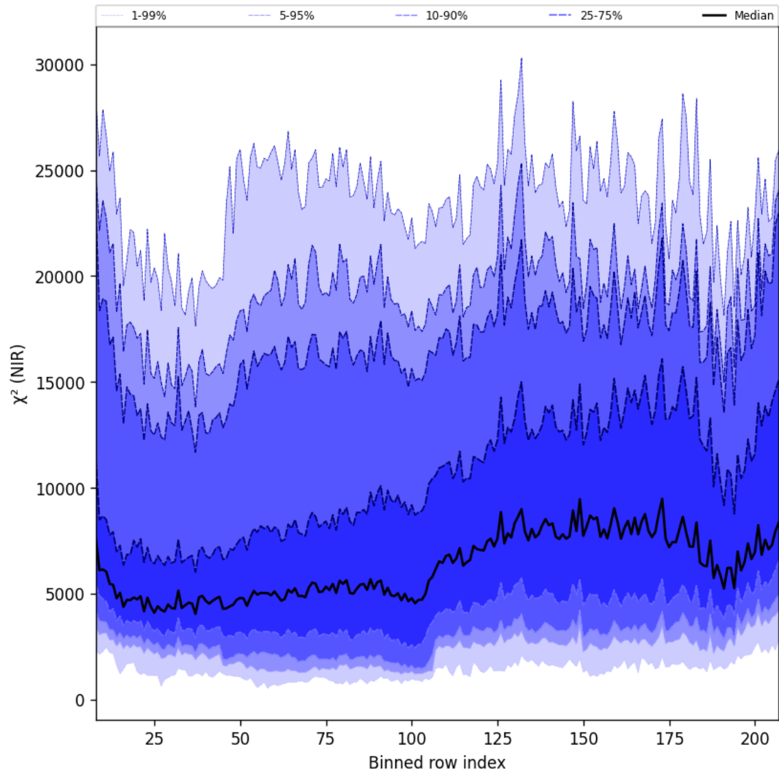
Figure 40: Along track statistics of “ \chi^2 (NIR)” for 2025-08-25 to 2025-08-26
