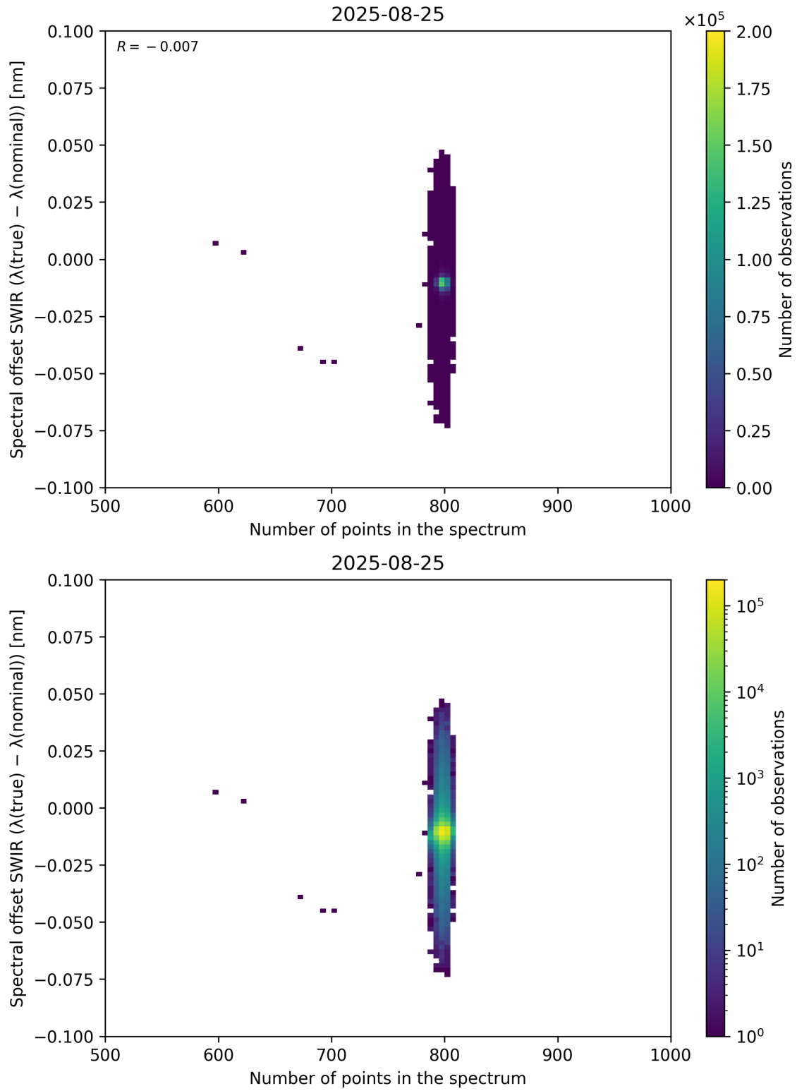
Figure 93: Scatter density plot of “Number of points in the spectrum” against “Spectral offset SWIR ( \lambda_{\text{true}} - \lambda_{\text{nominal}} )” for 2025-08-25 to 2025-08-26.
