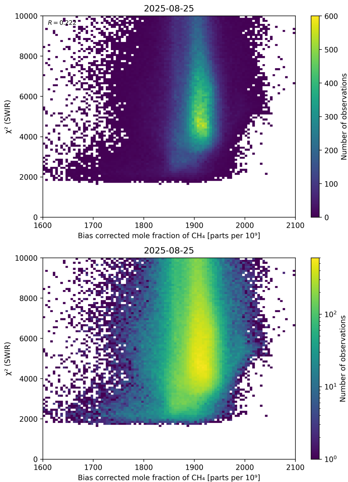
Figure 64: Scatter density plot of “Bias corrected mole fraction of \text{CH}_4 ” against “ \chi^2 (SWIR)” for 2025-08-25 to 2025-08-26.
