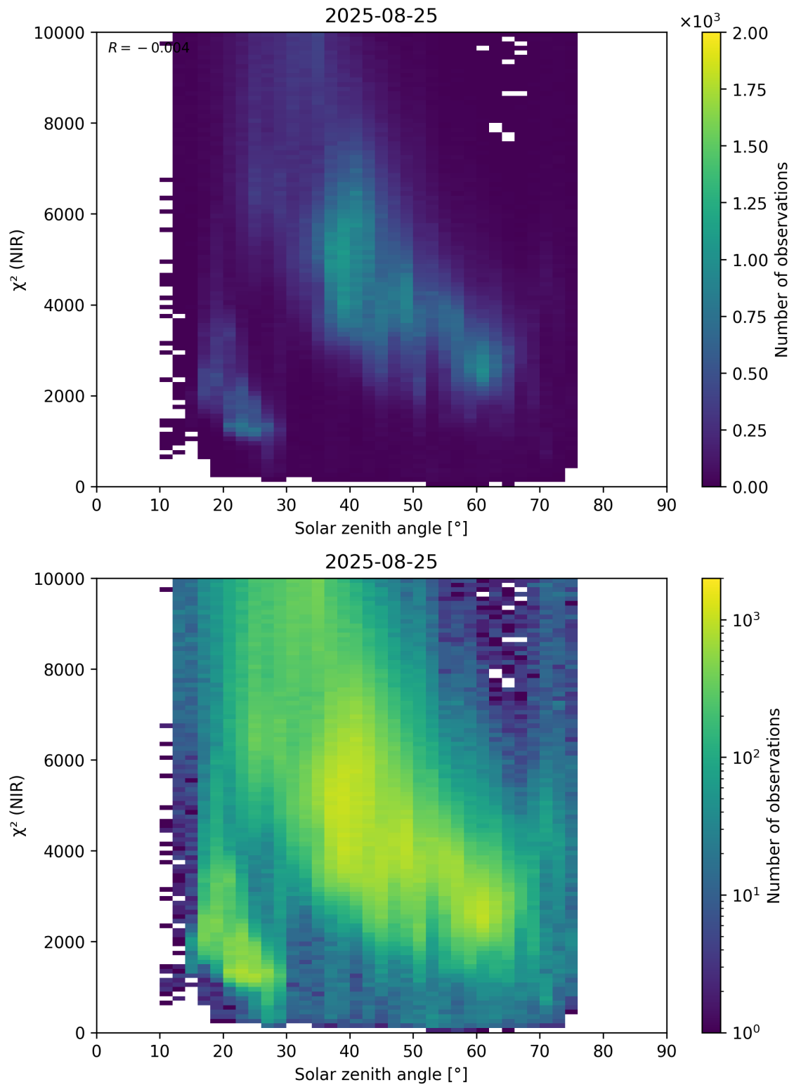
Figure 94: Scatter density plot of “Solar zenith angle” against “ \chi^2 (NIR)” for 2025-08-25 to 2025-08-26.
