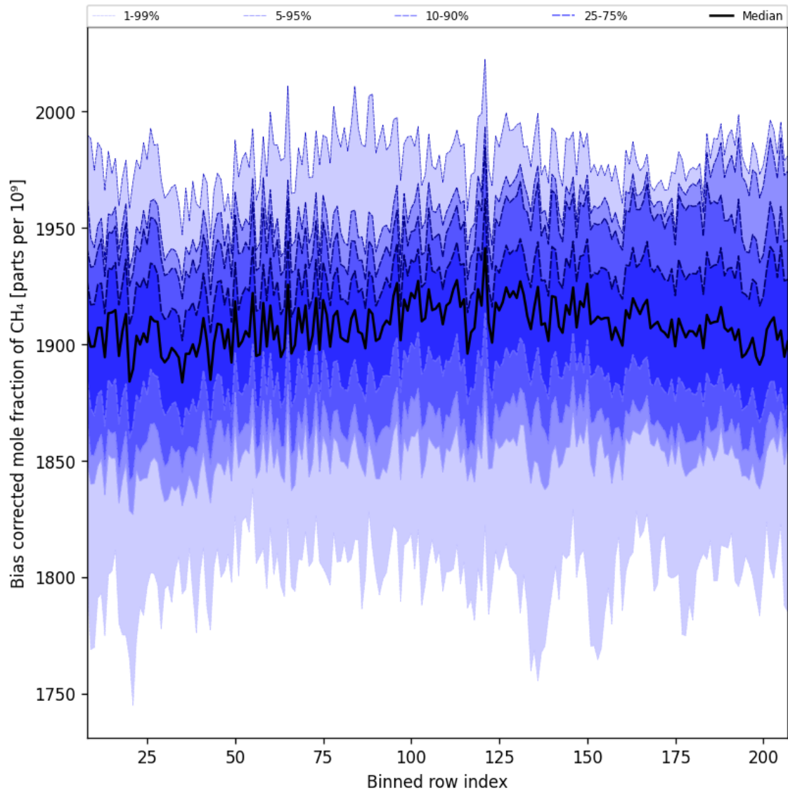
Figure 36: Along track statistics of “Bias corrected mole fraction of CH 4 ” for 2025-08-25 to 2025-08-26
