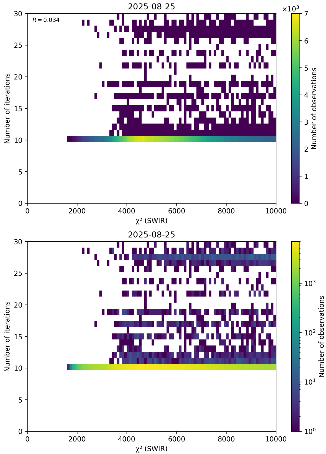
Figure 50: Scatter density plot of “ \chi^2 (SWIR)” against “Number of iterations” for 2025-08-25 to 2025-08-26.
