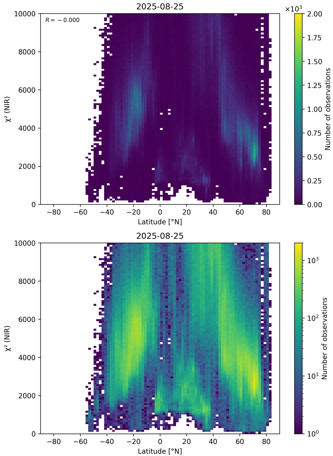
Figure 53: Scatter density plot of “Latitude” against “ \chi^2 (NIR)” for 2025-08-25 to 2025-08-26.
