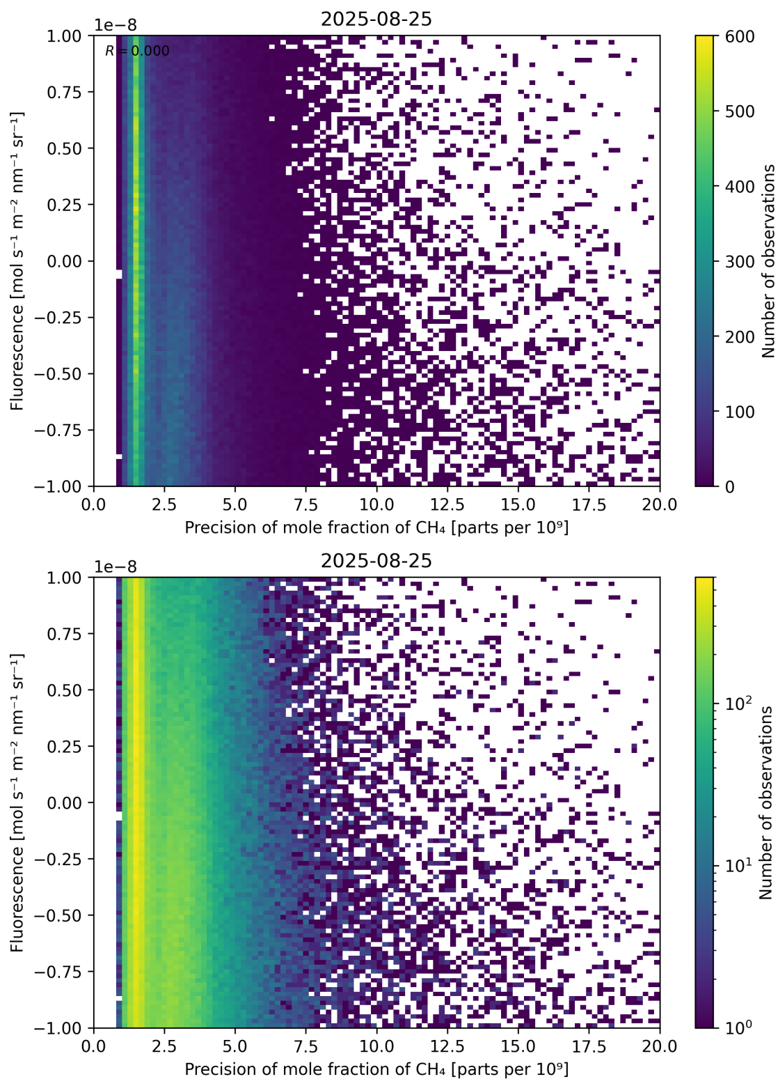
Figure 81: Scatter density plot of “Precision of mole fraction of CH 4 ” against “Fluorescence” for 2025-08-25 to 2025-08-26.
