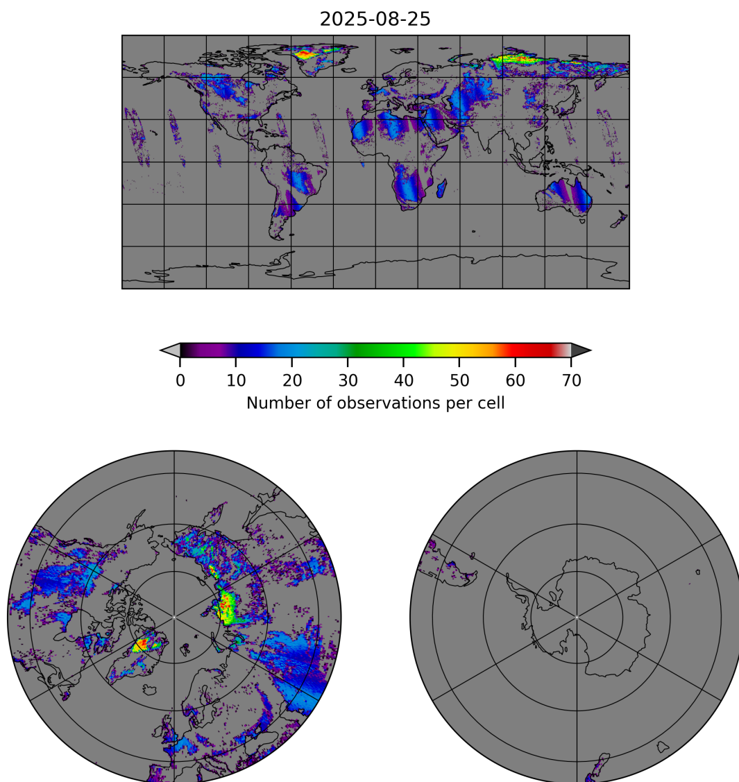
Figure 10: Map of the number of observations for 2025-08-25 to 2025-08-26
