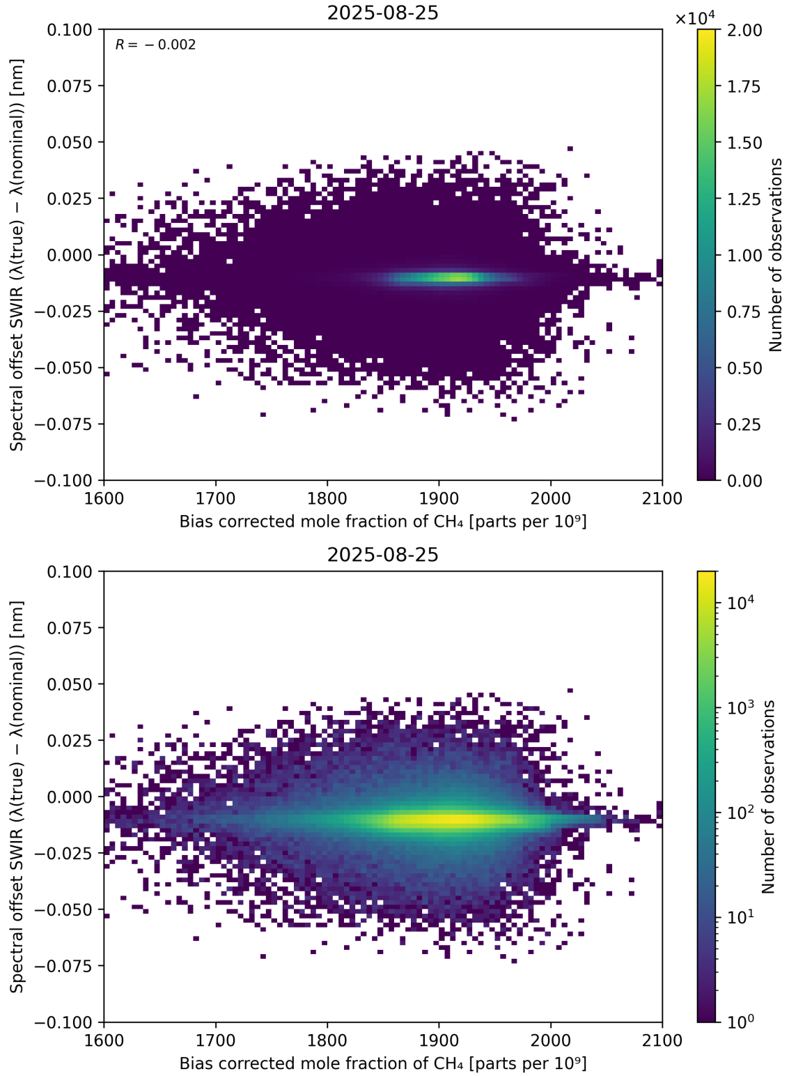
Figure 69: Scatter density plot of “Bias corrected mole fraction of \text{CH}_4 ” against “Spectral offset SWIR ( \lambda_{\text{true}} - \lambda_{\text{nominal}} )” for 2025-08-25 to 2025-08-26.
