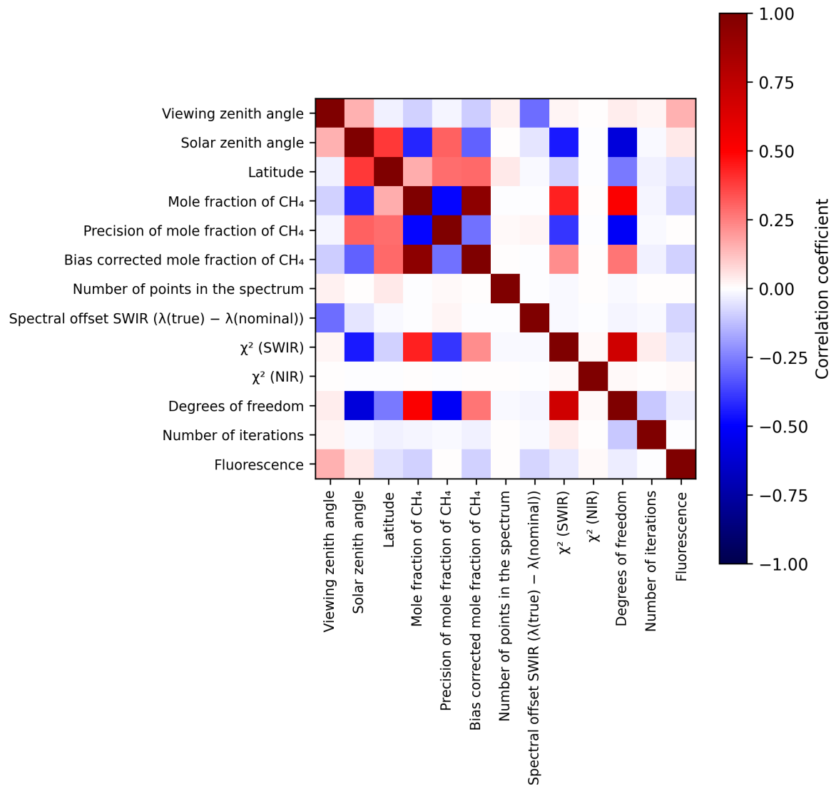
Figure 2: Map of correlation matrix for 2025-08-25 to 2025-08-26.
