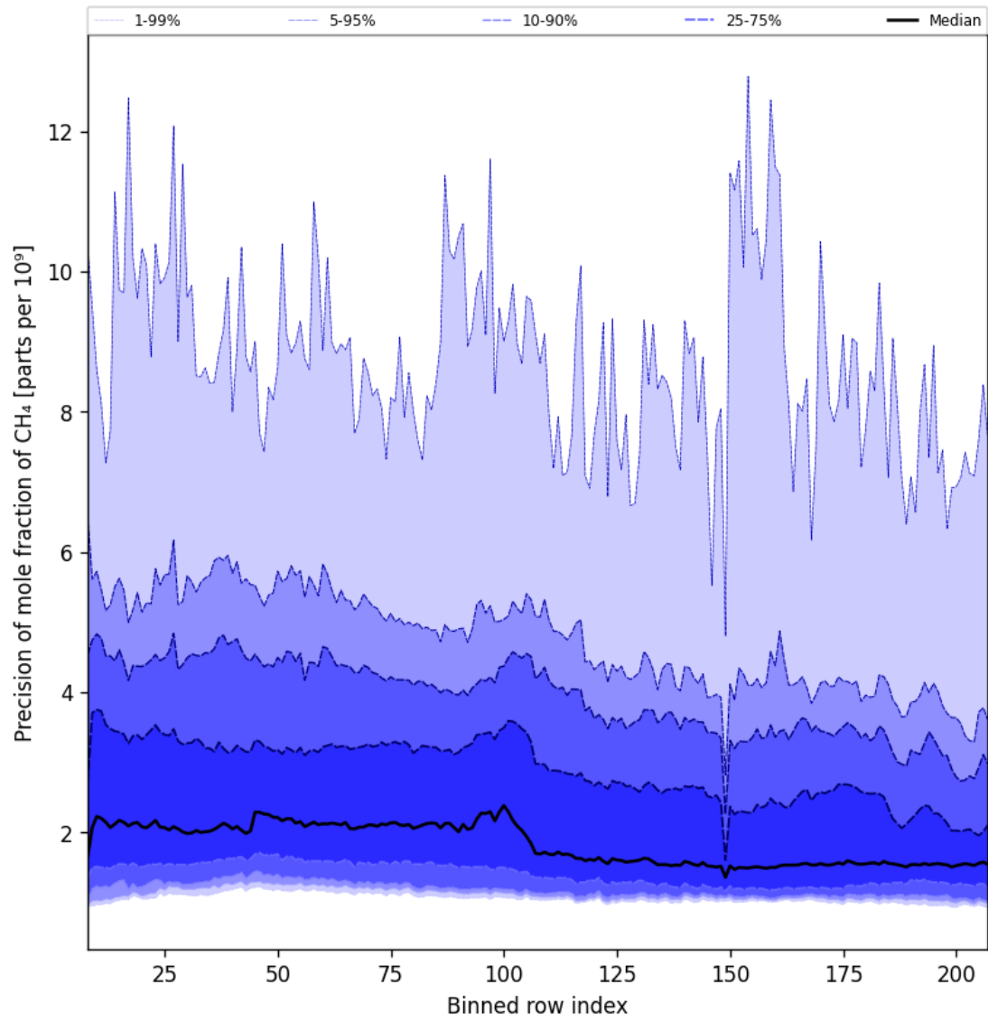
Figure 35: Along track statistics of “Precision of mole fraction of CH 4 ” for 2025-08-25 to 2025-08-26
