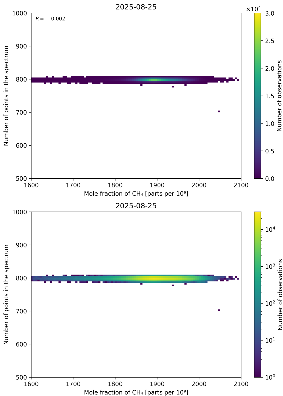
Figure 77: Scatter density plot of “Mole fraction of CH 4 ” against “Number of points in the spectrum” for 2025-08-25 to 2025-08-26.
