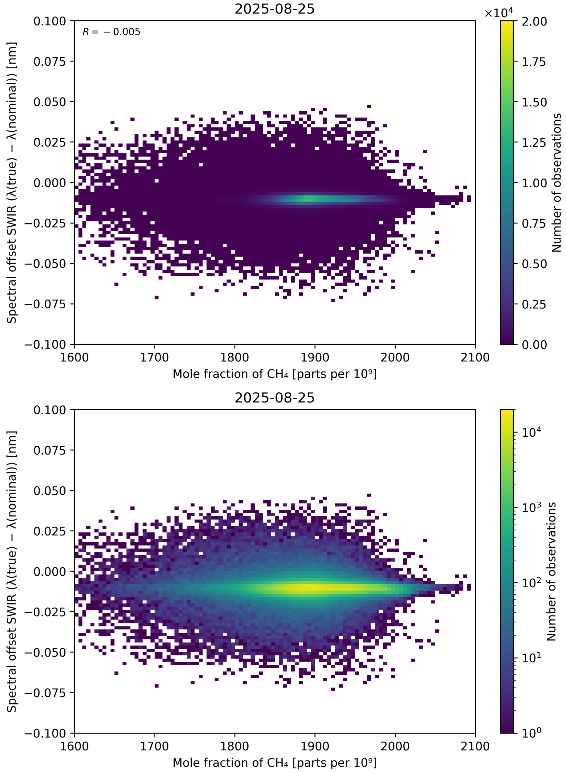
Figure 86: Scatter density plot of “Mole fraction of CH 4 ” against “Spectral offset SWIR ( \lambda_{\text{true}} - \lambda_{\text{nominal}} )” for 2025-08-25 to 2025-08-26.
