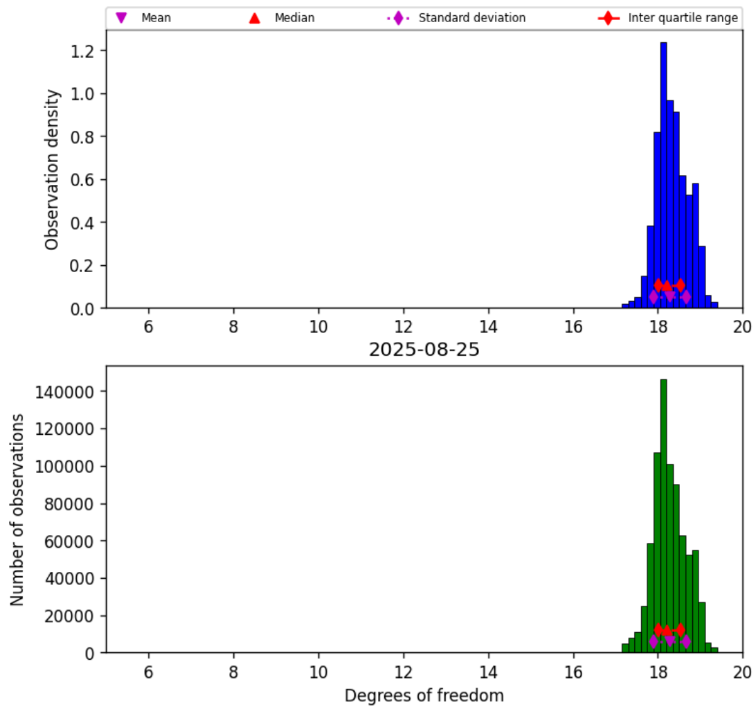
Figure 30: Histogram of “Degrees of freedom” for 2025-08-25 to 2025-08-26
