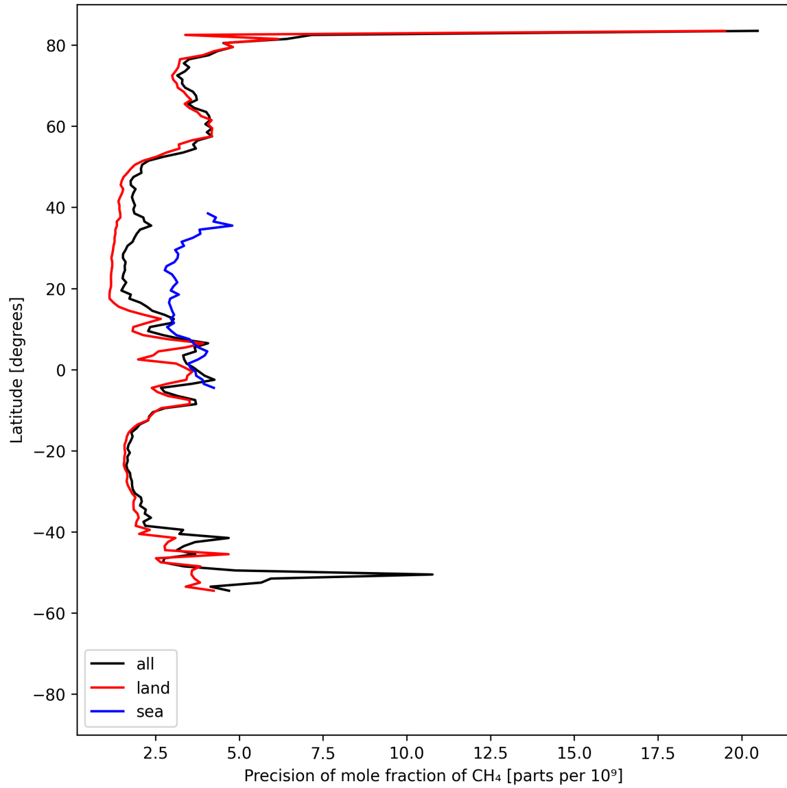
Figure 13: Zonal average of “Precision of mole fraction of CH 4 ” for 2025-08-25 to 2025-08-26.
