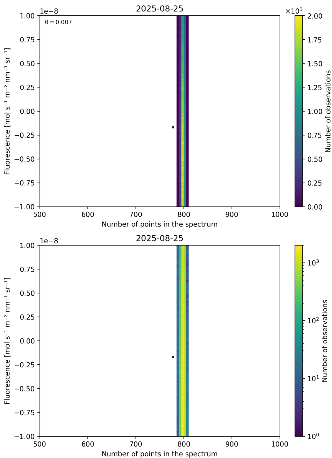
Figure 91: Scatter density plot of “Number of points in the spectrum” against “Fluorescence” for 2025-08-25 to 2025-08-26.
