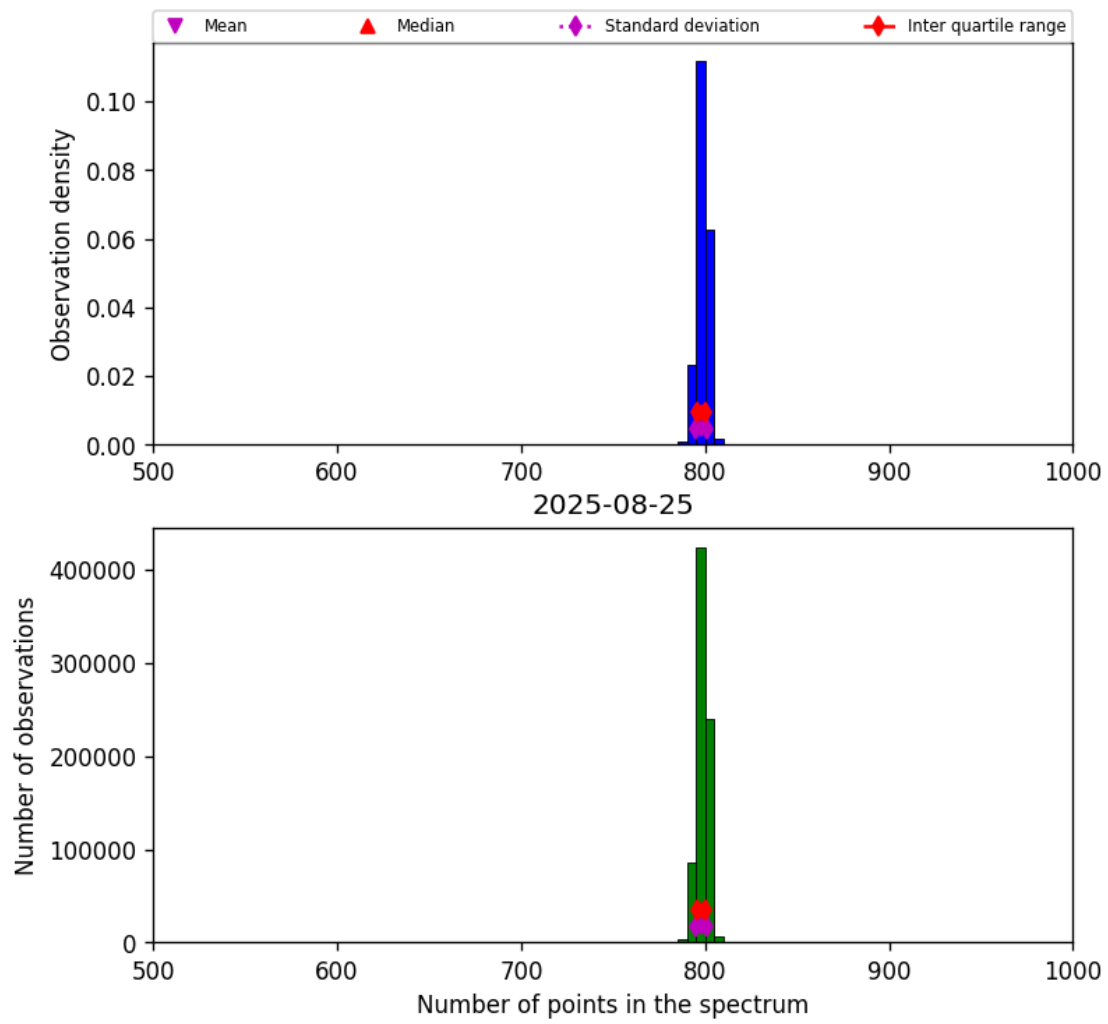
Figure 26: Histogram of “Number of points in the spectrum” for 2025-08-25 to 2025-08-26
