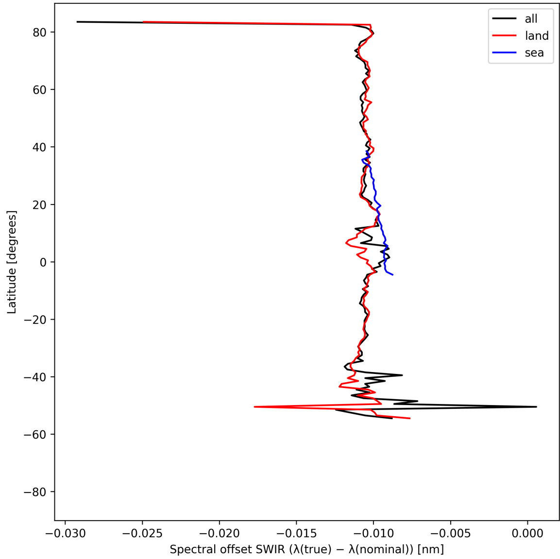
Figure 16: Zonal average of “Spectral offset SWIR ( \lambda_{\text{true}} - \lambda_{\text{nominal}} )” for 2025-08-25 to 2025-08-26.
