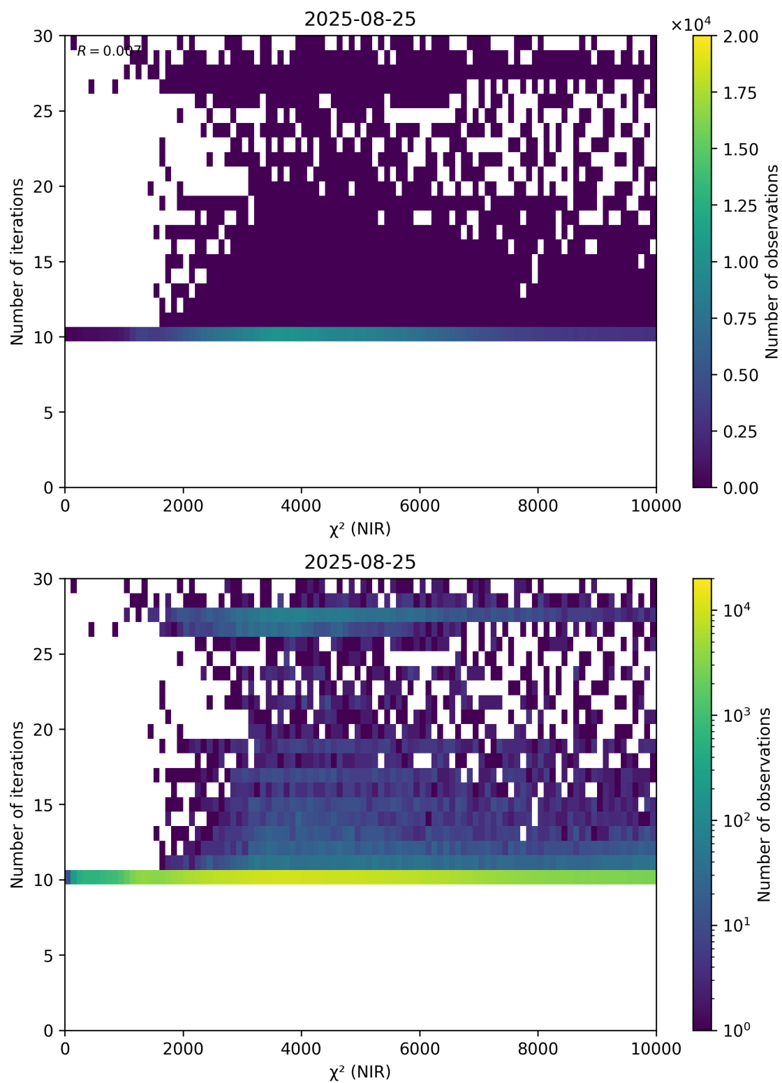
Figure 46: Scatter density plot of “ \chi^2 (NIR)” against “Number of iterations” for 2025-08-25 to 2025-08-26.
