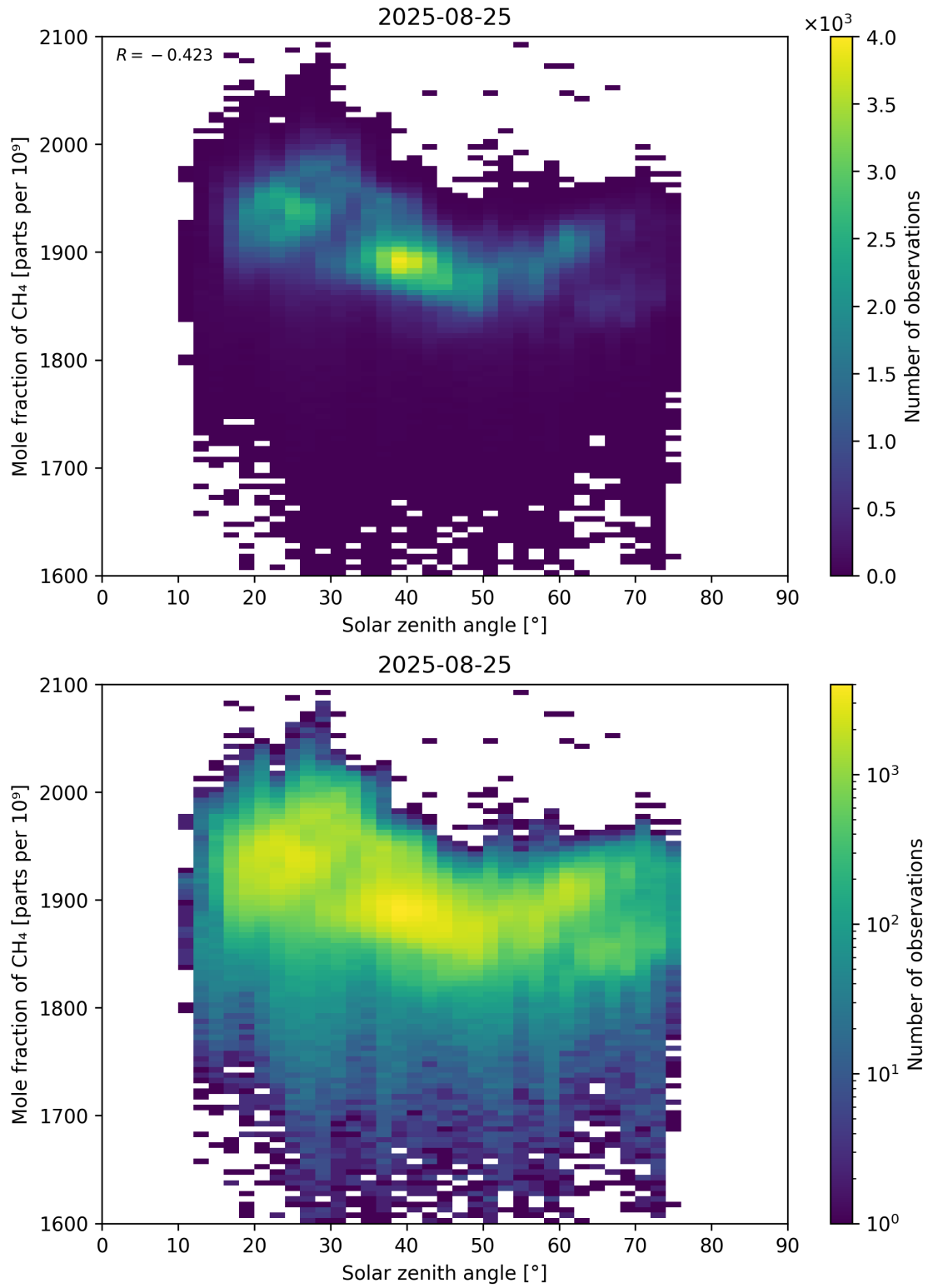
Figure 99: Scatter density plot of “Solar zenith angle” against “Mole fraction of CH 4 ” for 2025-08-25 to 2025-08-26.
