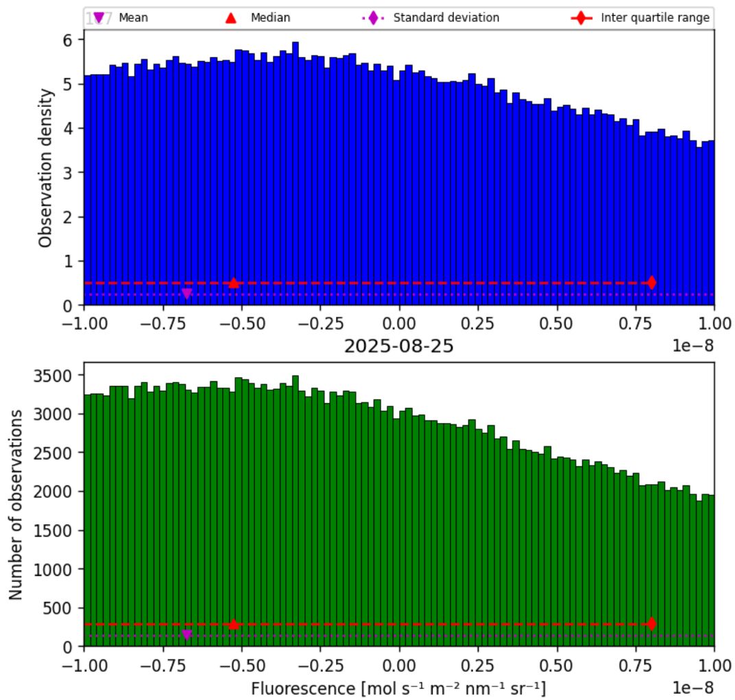
Figure 32: Histogram of “Fluorescence” for 2025-08-25 to 2025-08-26
