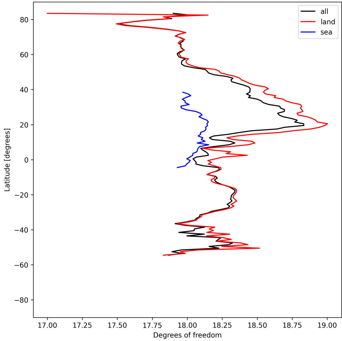
Figure 19: Zonal average of “Degrees of freedom” for 2025-08-25 to 2025-08-26.
