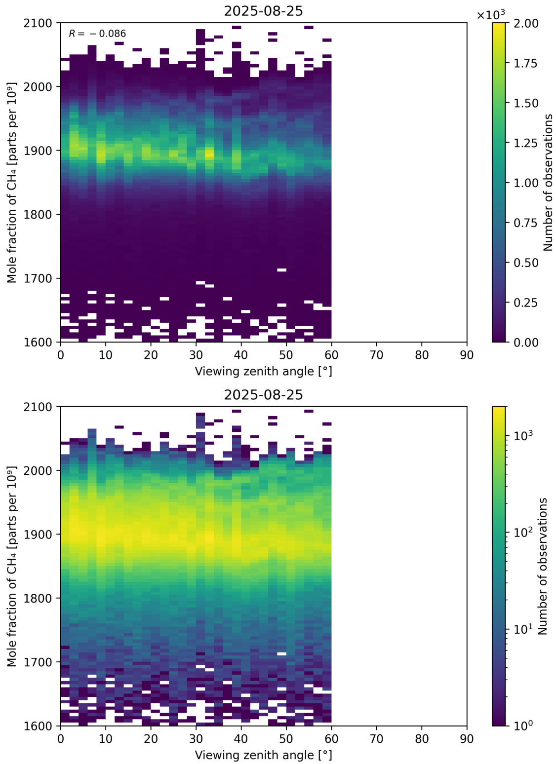
Figure 110: Scatter density plot of “Viewing zenith angle” against “Mole fraction of CH 4 ” for 2025-08-25 to 2025-08-26.
