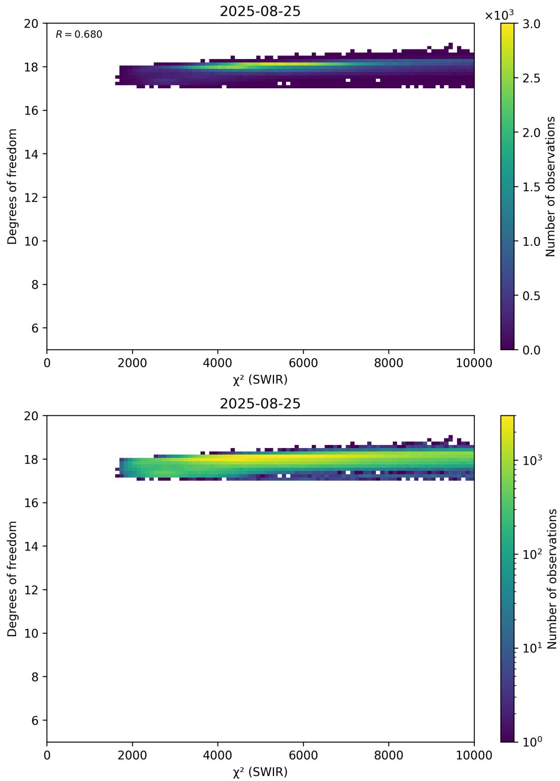
Figure 48: Scatter density plot of “ \chi^2 (SWIR)” against “Degrees of freedom” for 2025-08-25 to 2025-08-26.
