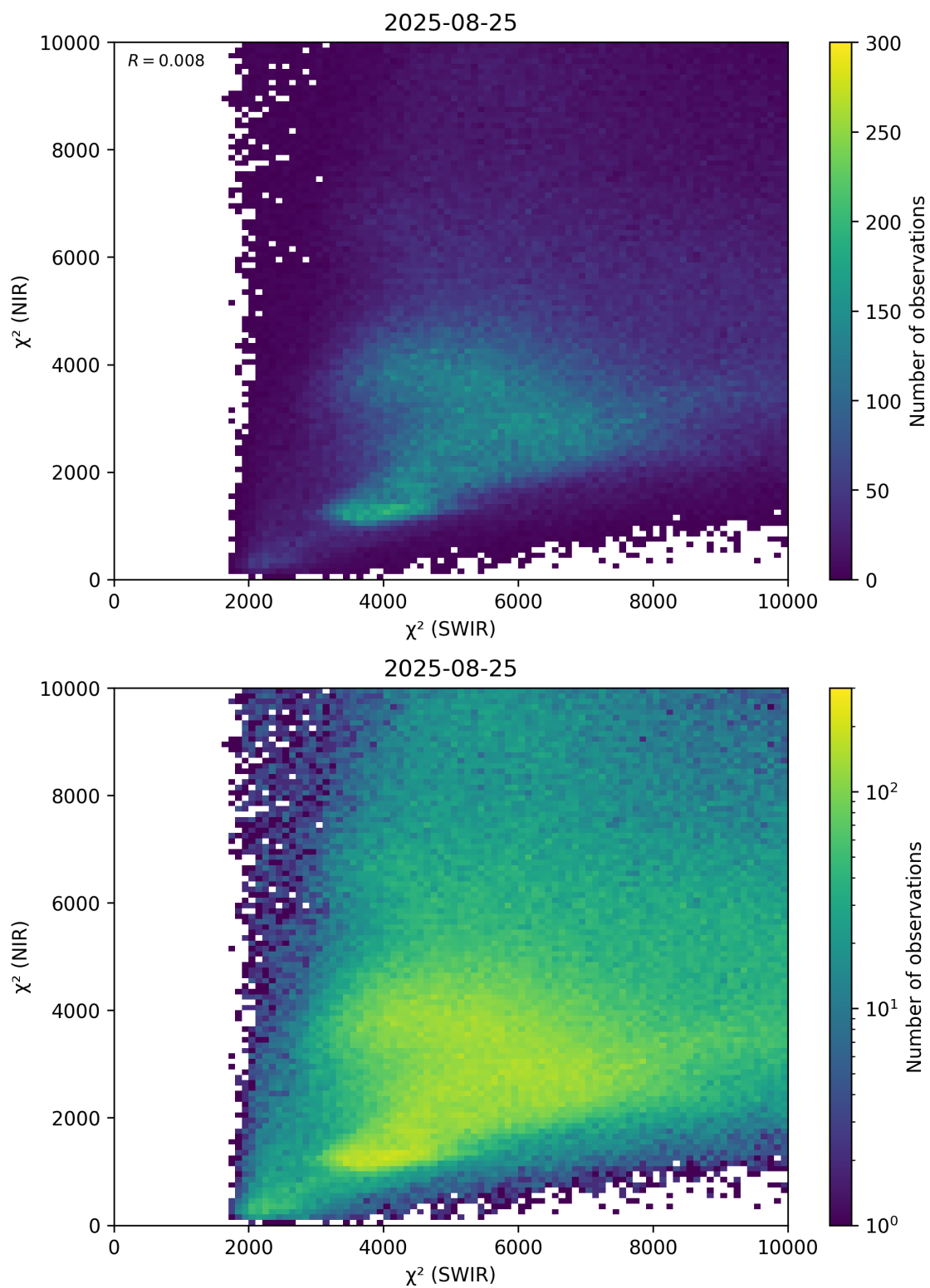
Figure 47: Scatter density plot of “ \chi^2 (SWIR)” against “ \chi^2 (NIR)” for 2025-08-25 to 2025-08-26.
