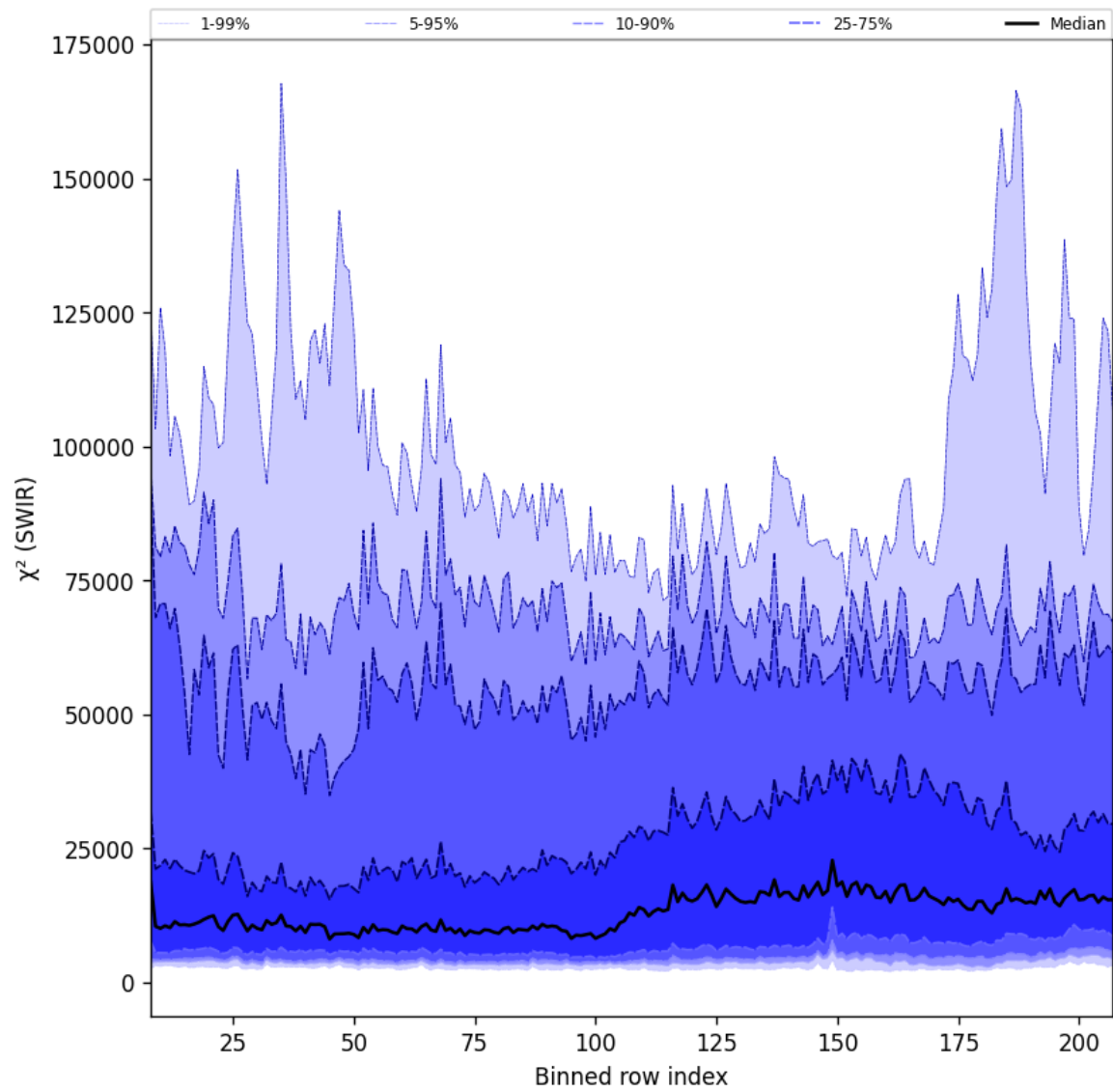
Figure 39: Along track statistics of " \chi^2 (SWIR)" for 2025-08-25 to 2025-08-26
