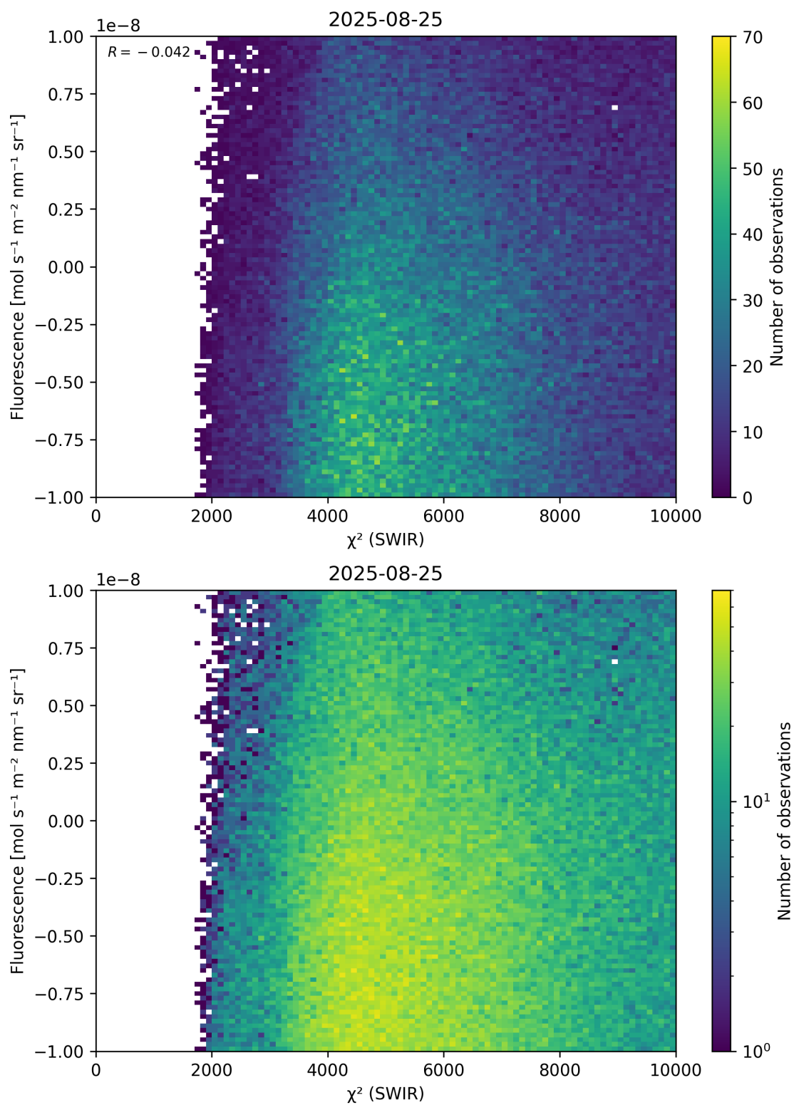
Figure 49: Scatter density plot of “ \chi^2 (SWIR)” against “Fluorescence” for 2025-08-25 to 2025-08-26.
