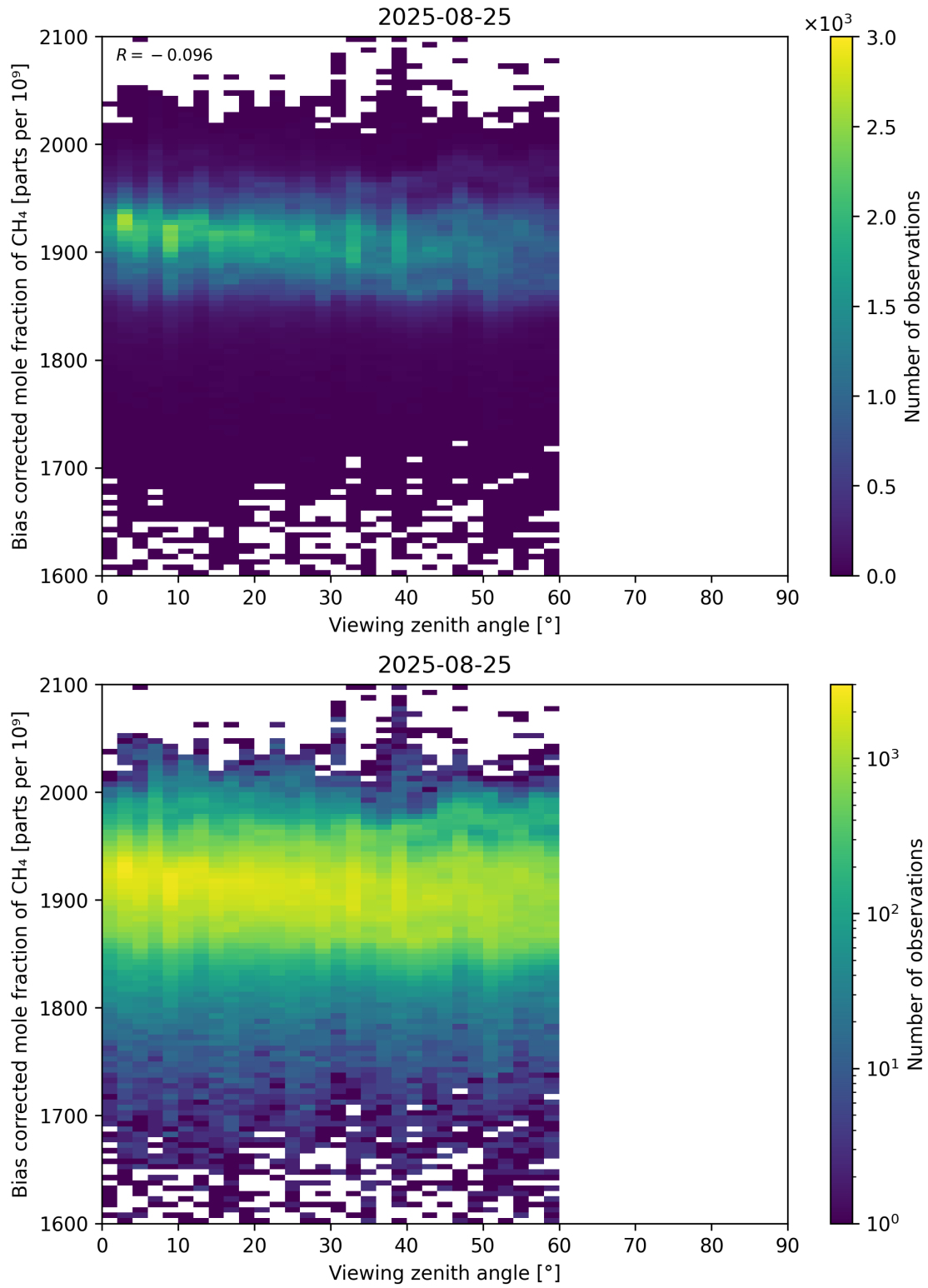
Figure 111: Scatter density plot of “Viewing zenith angle” against “Bias corrected mole fraction of CH 4 ” for 2025-08-25 to 2025-08-26.
