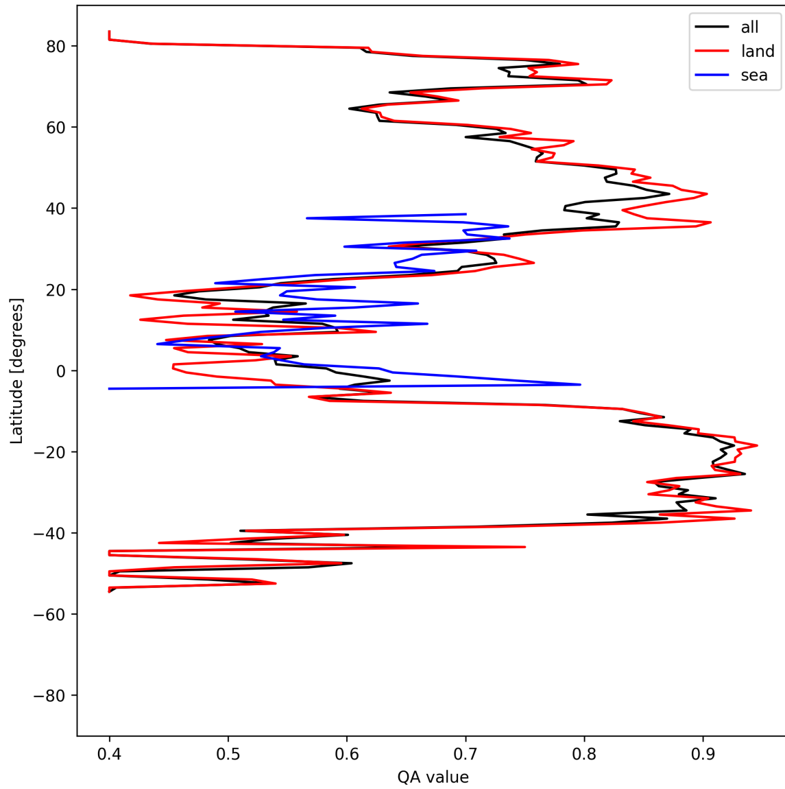
Figure 11: Zonal average of “QA value” for 2025-08-25 to 2025-08-26.
