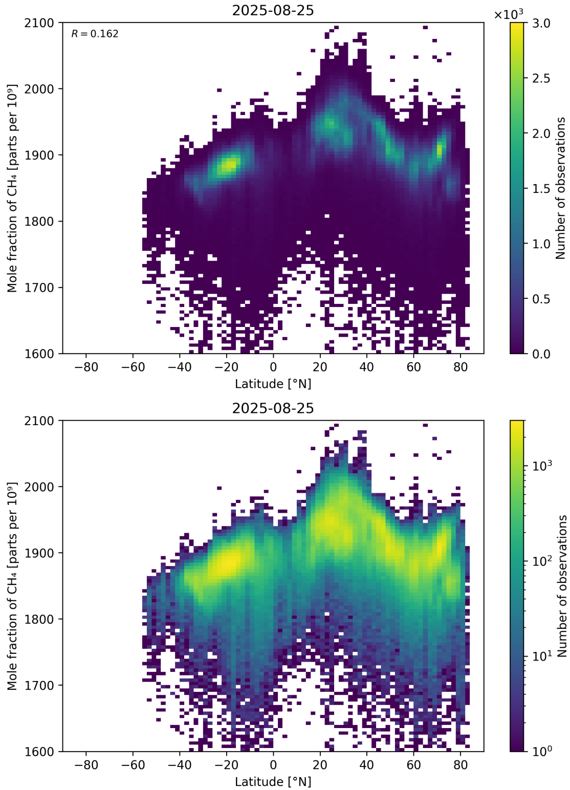
Figure 57: Scatter density plot of “Latitude” against “Mole fraction of \text{CH}_4 ” for 2025-08-25 to 2025-08-26.
