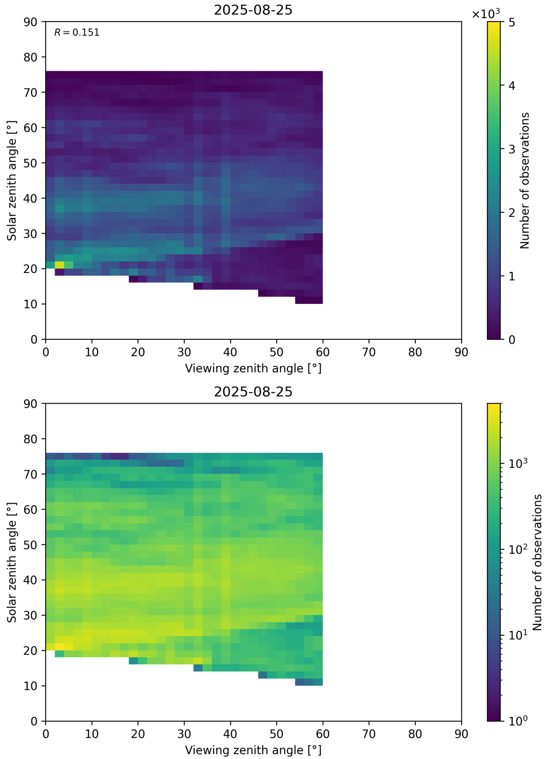
Figure 115: Scatter density plot of “Viewing zenith angle” against “Solar zenith angle” for 2025-08-25 to 2025-08-26.
