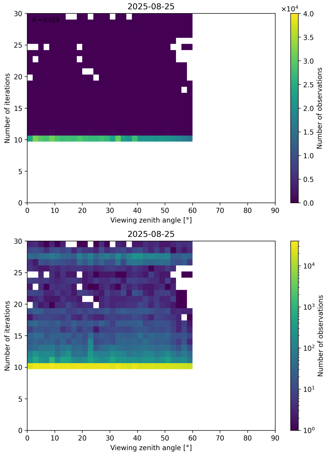
Figure 113: Scatter density plot of “Viewing zenith angle” against “Number of iterations” for 2025-08-25 to 2025-08-26.
