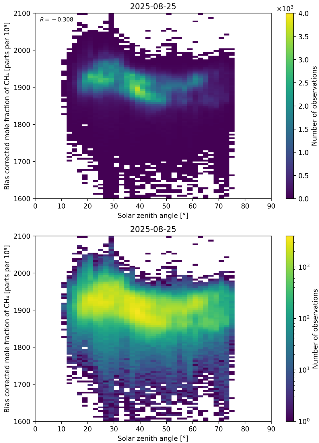
Figure 100: Scatter density plot of “Solar zenith angle” against “Bias corrected mole fraction of CH 4 ” for 2025-08-25 to 2025-08-26.
