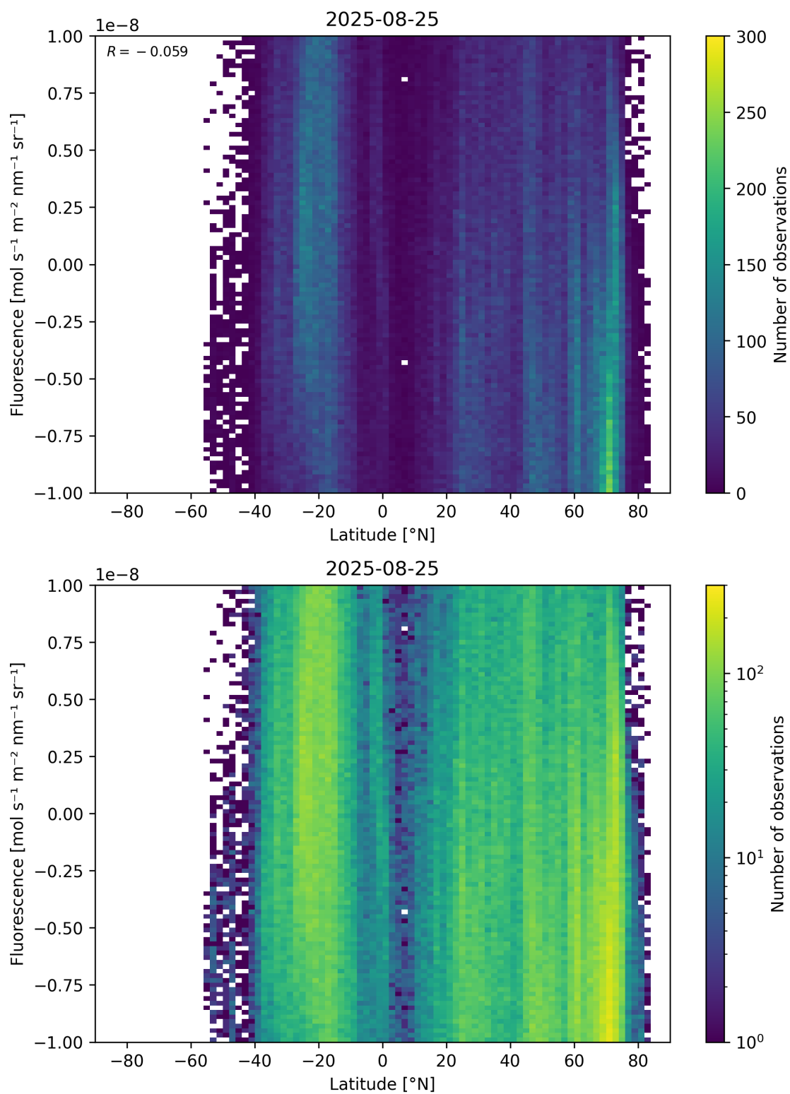
Figure 56: Scatter density plot of “Latitude” against “Fluorescence” for 2025-08-25 to 2025-08-26.
