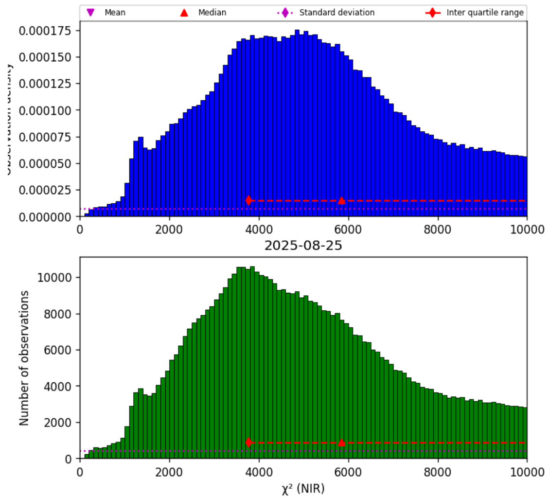
Figure 29: Histogram of “ \chi^2 (NIR)” for 2025-08-25 to 2025-08-26
