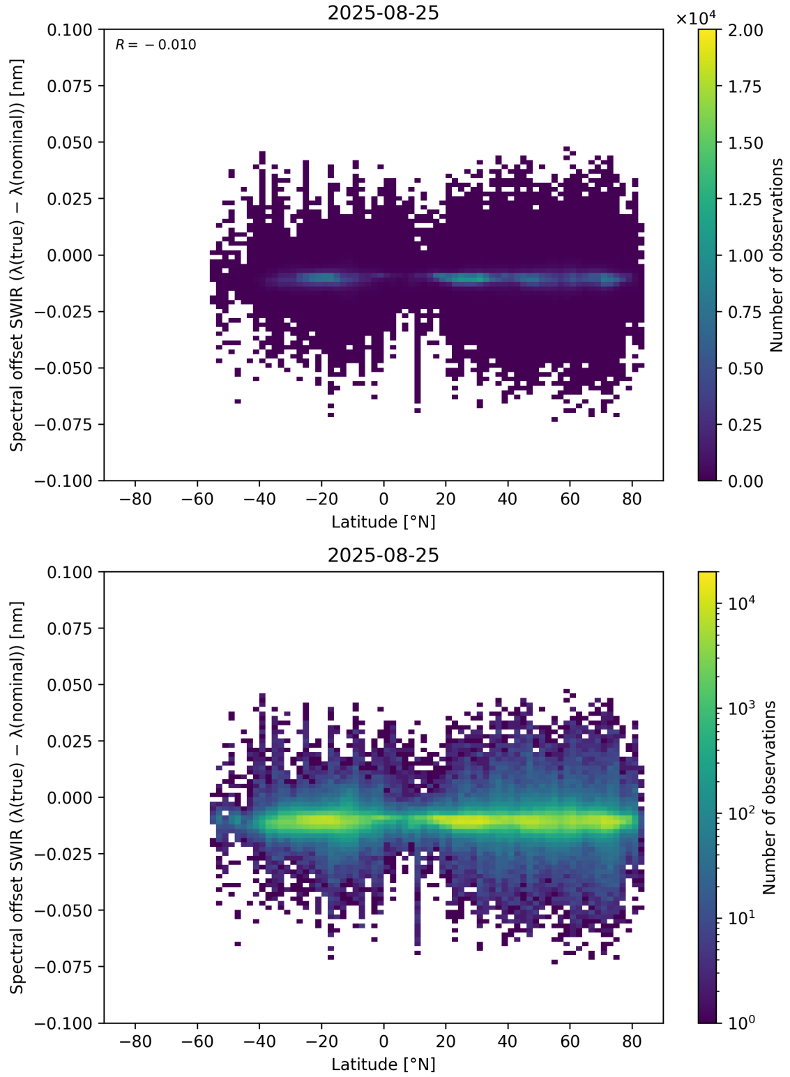
Figure 62: Scatter density plot of “Latitude” against “Spectral offset SWIR ( \lambda_{\text{true}} - \lambda_{\text{nominal}} )” for 2025-08-25 to 2025-08-26.
