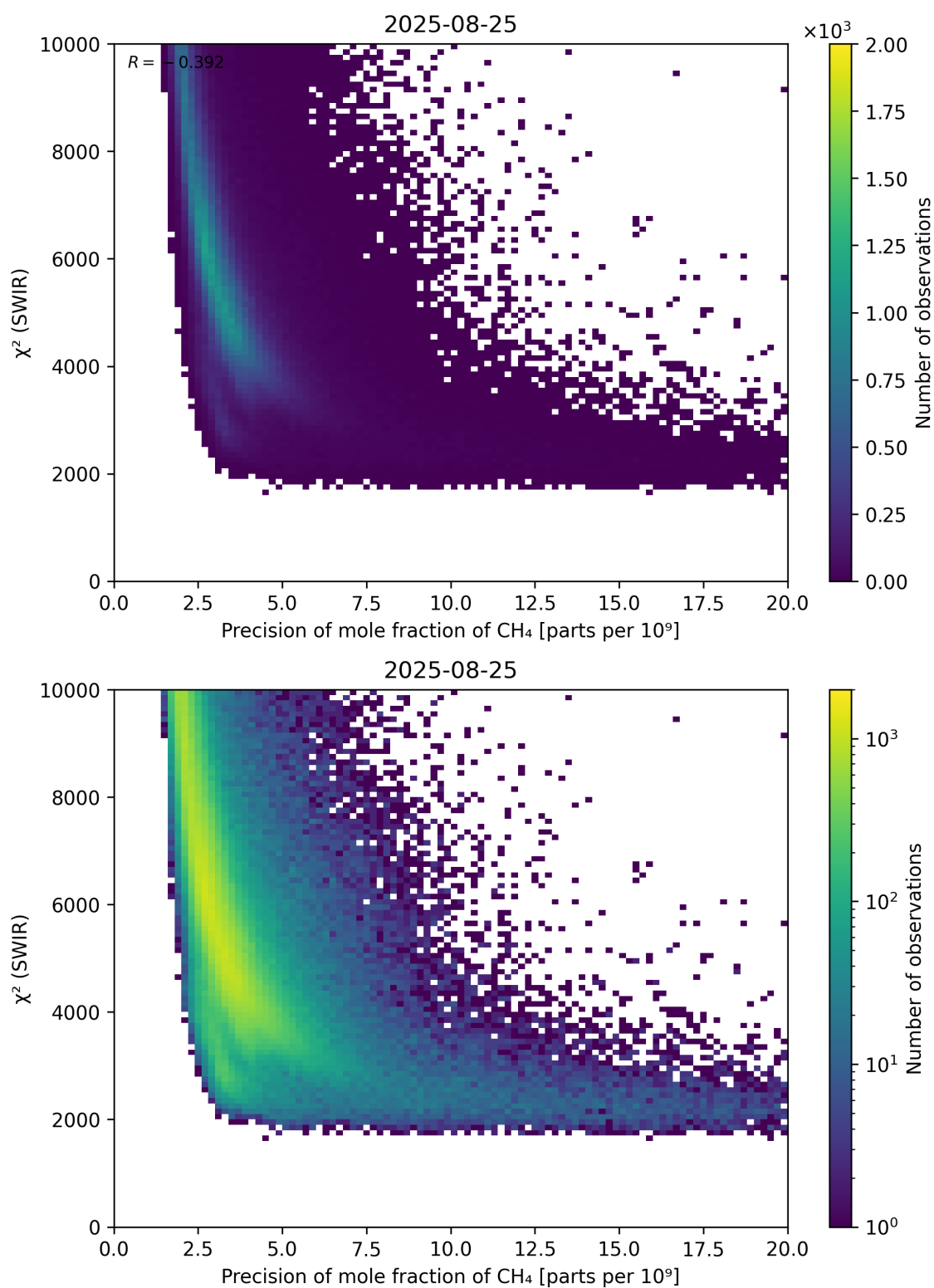
Figure 79: Scatter density plot of “Precision of mole fraction of \text{CH}_4 ” against “ \chi^2 (SWIR)” for 2025-08-25 to 2025-08-26.
