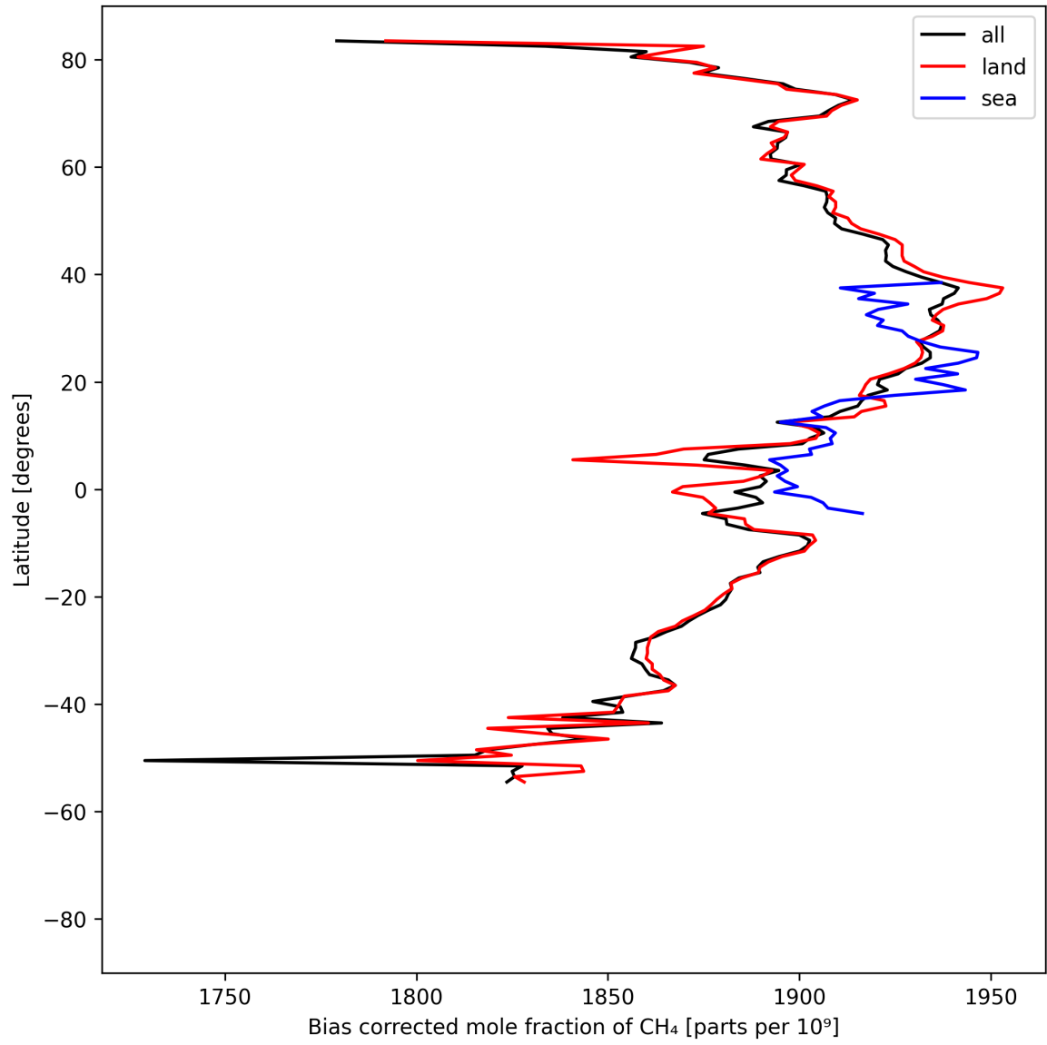
Figure 14: Zonal average of “Bias corrected mole fraction of \text{CH}_4 ” for 2025-08-25 to 2025-08-26.
