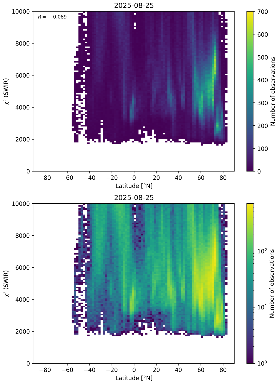
Figure 54: Scatter density plot of “Latitude” against “ \chi^2 (SWIR)” for 2025-08-25 to 2025-08-26.
