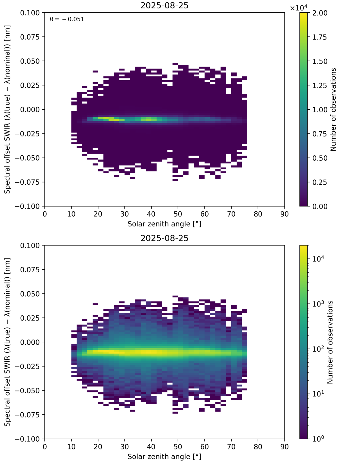
Figure 104: Scatter density plot of “Solar zenith angle” against “Spectral offset SWIR ( \lambda_{\text{true}} - \lambda_{\text{nominal}} )” for 2025-08-25 to 2025-08-26.
