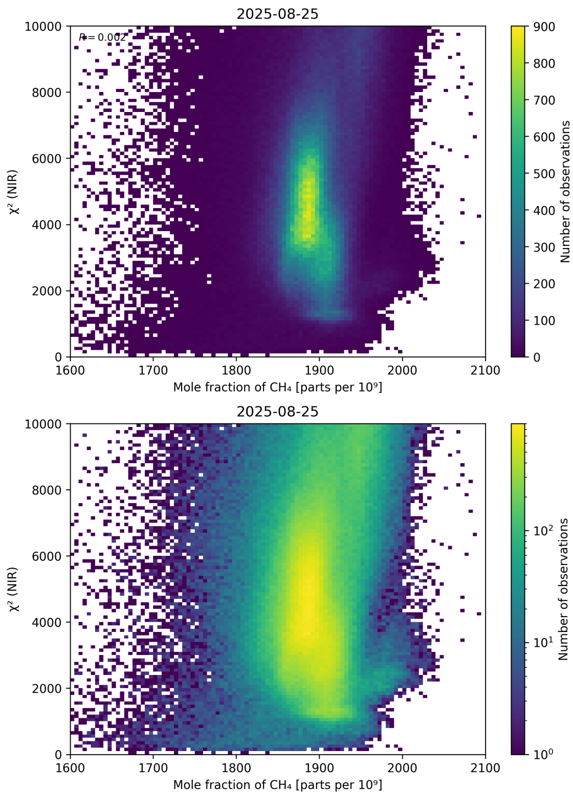
Figure 70: Scatter density plot of “Mole fraction of CH 4 ” against “ \chi^2 (NIR)” for 2025-08-25 to 2025-08-26.
