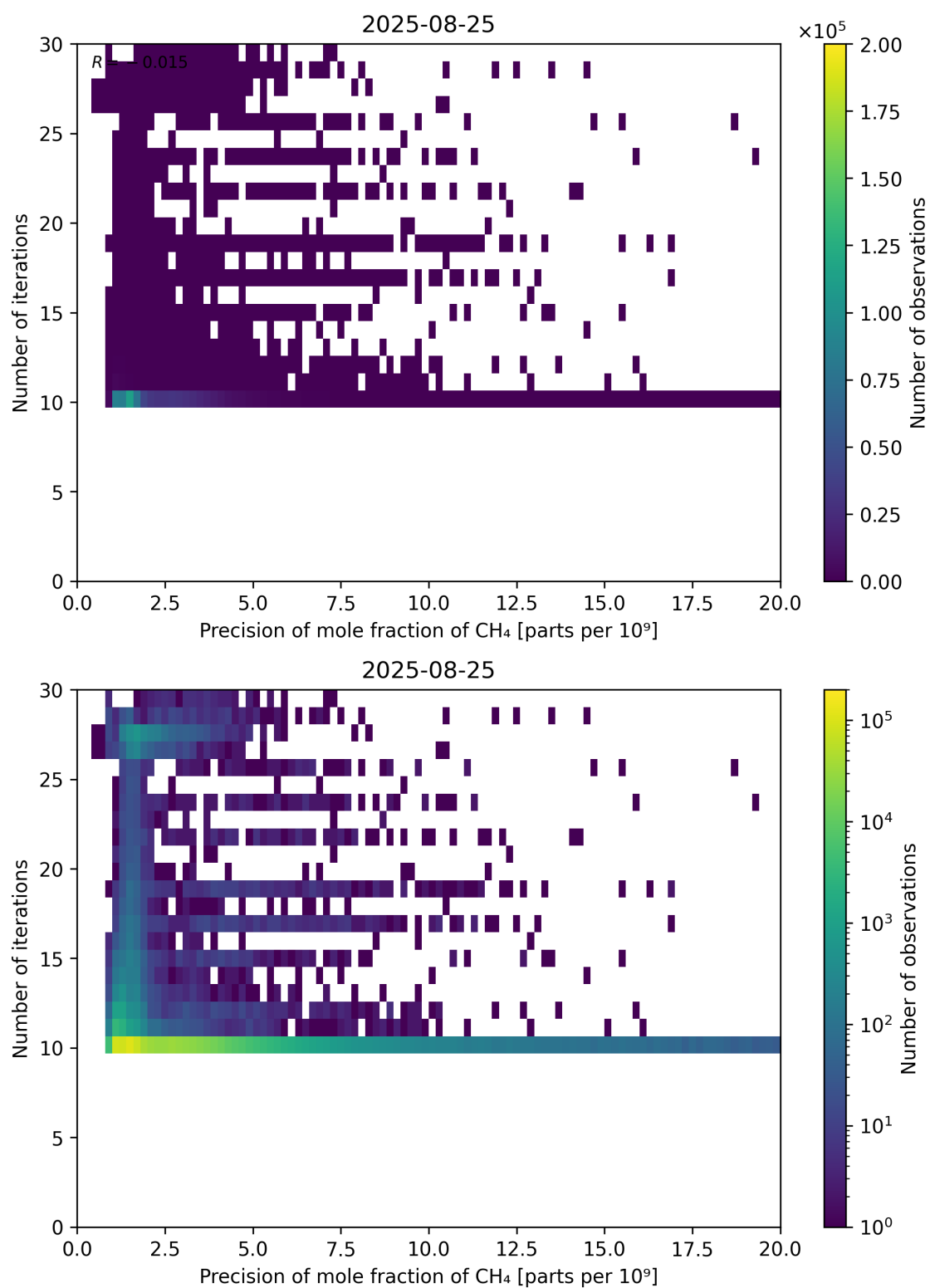
Figure 83: Scatter density plot of “Precision of mole fraction of CH 4 ” against “Number of iterations” for 2025-08-25 to 2025-08-26.
