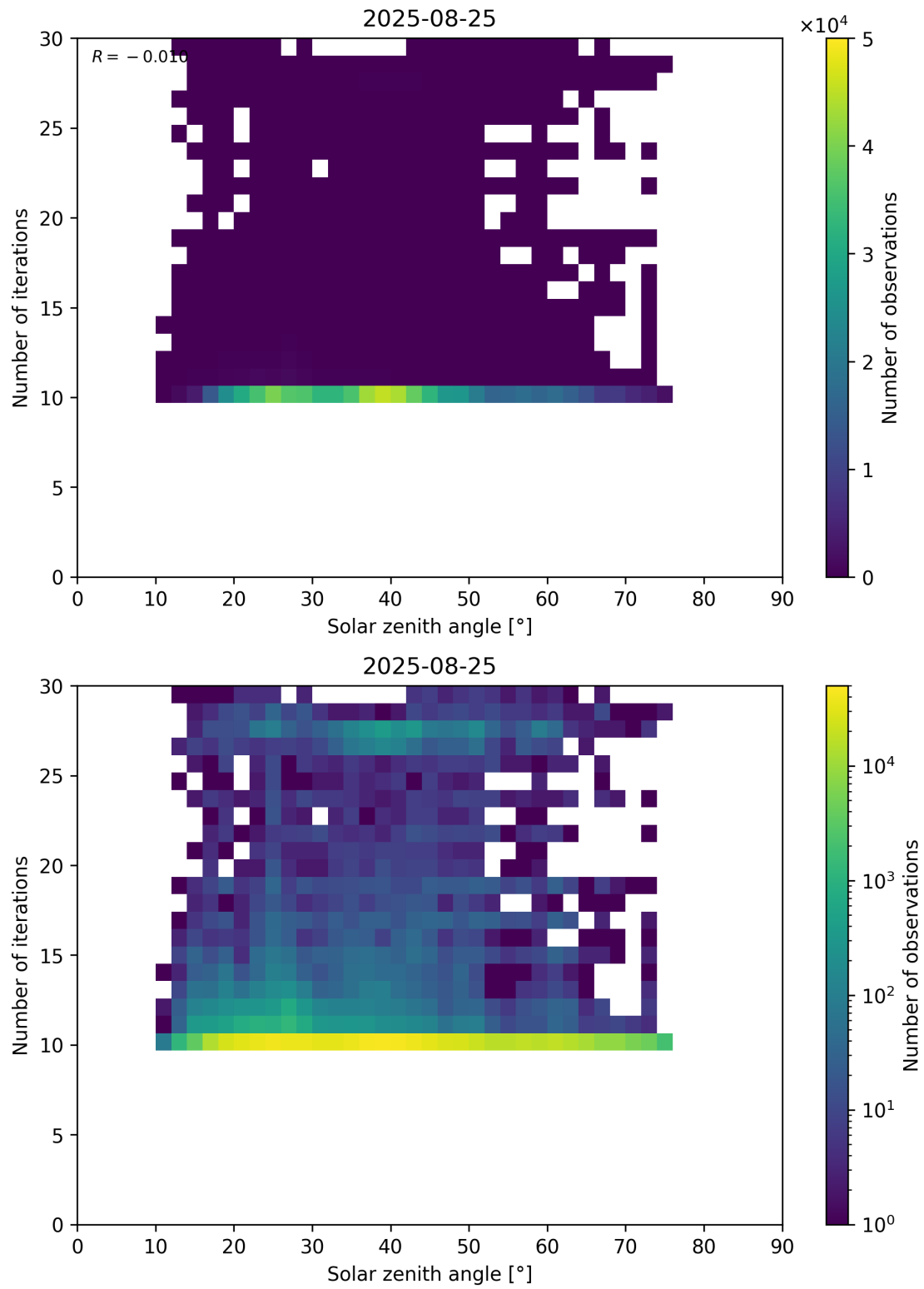
Figure 102: Scatter density plot of “Solar zenith angle” against “Number of iterations” for 2025-08-25 to 2025-08-26.
