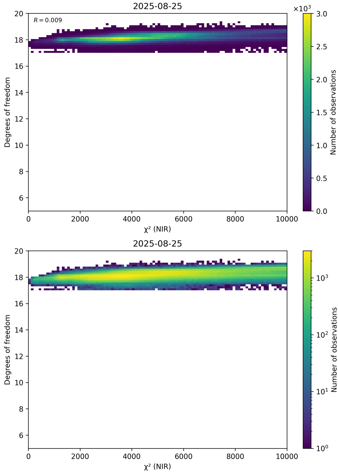
Figure 44: Scatter density plot of “ \chi^2 (NIR)” against “Degrees of freedom” for 2025-08-25 to 2025-08-26.
