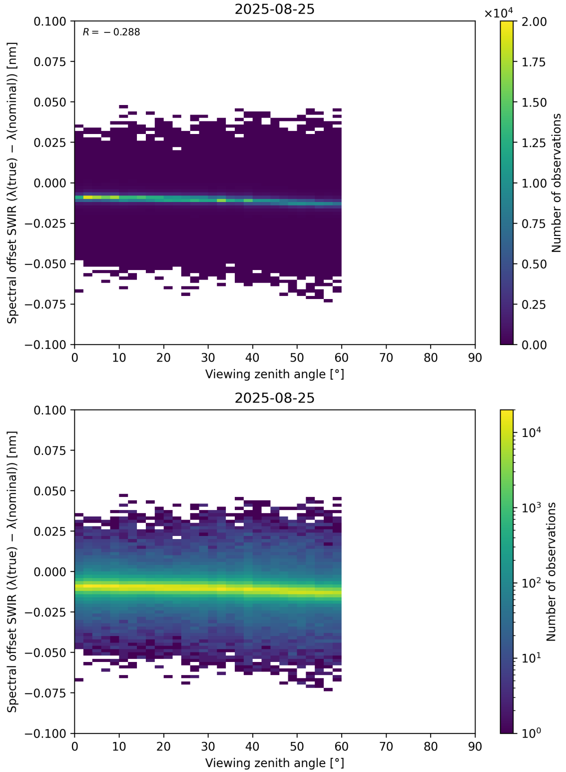
Figure 116: Scatter density plot of “Viewing zenith angle” against “Spectral offset SWIR ( \lambda_{\text{true}} - \lambda_{\text{nominal}} )” for 2025-08-25 to 2025-08-26.
