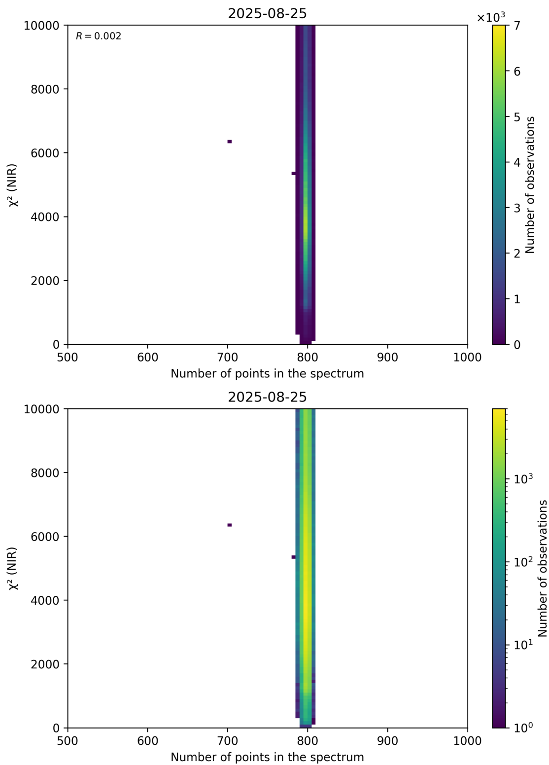
Figure 88: Scatter density plot of “Number of points in the spectrum” against “ \chi^2 (NIR)” for 2025-08-25 to 2025-08-26.
