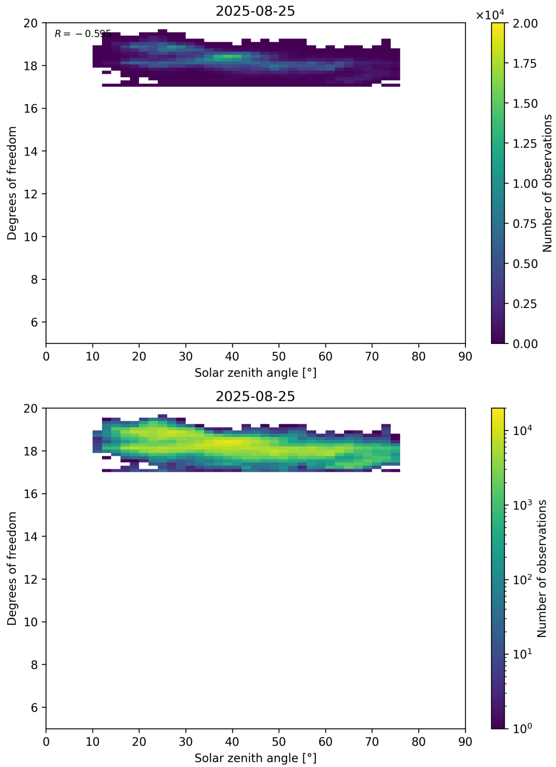
Figure 96: Scatter density plot of “Solar zenith angle” against “Degrees of freedom” for 2025-08-25 to 2025-08-26.
