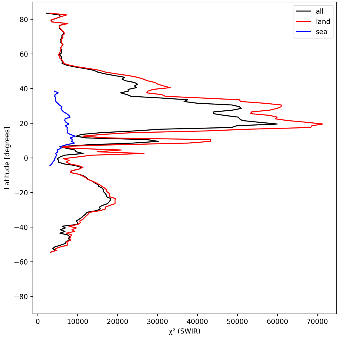
Figure 17: Zonal average of “ \chi^2 (SWIR)” for 2025-08-25 to 2025-08-26.
