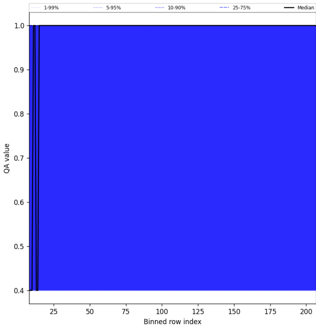
Figure 33: Along track statistics of “QA value” for 2025-08-25 to 2025-08-26
