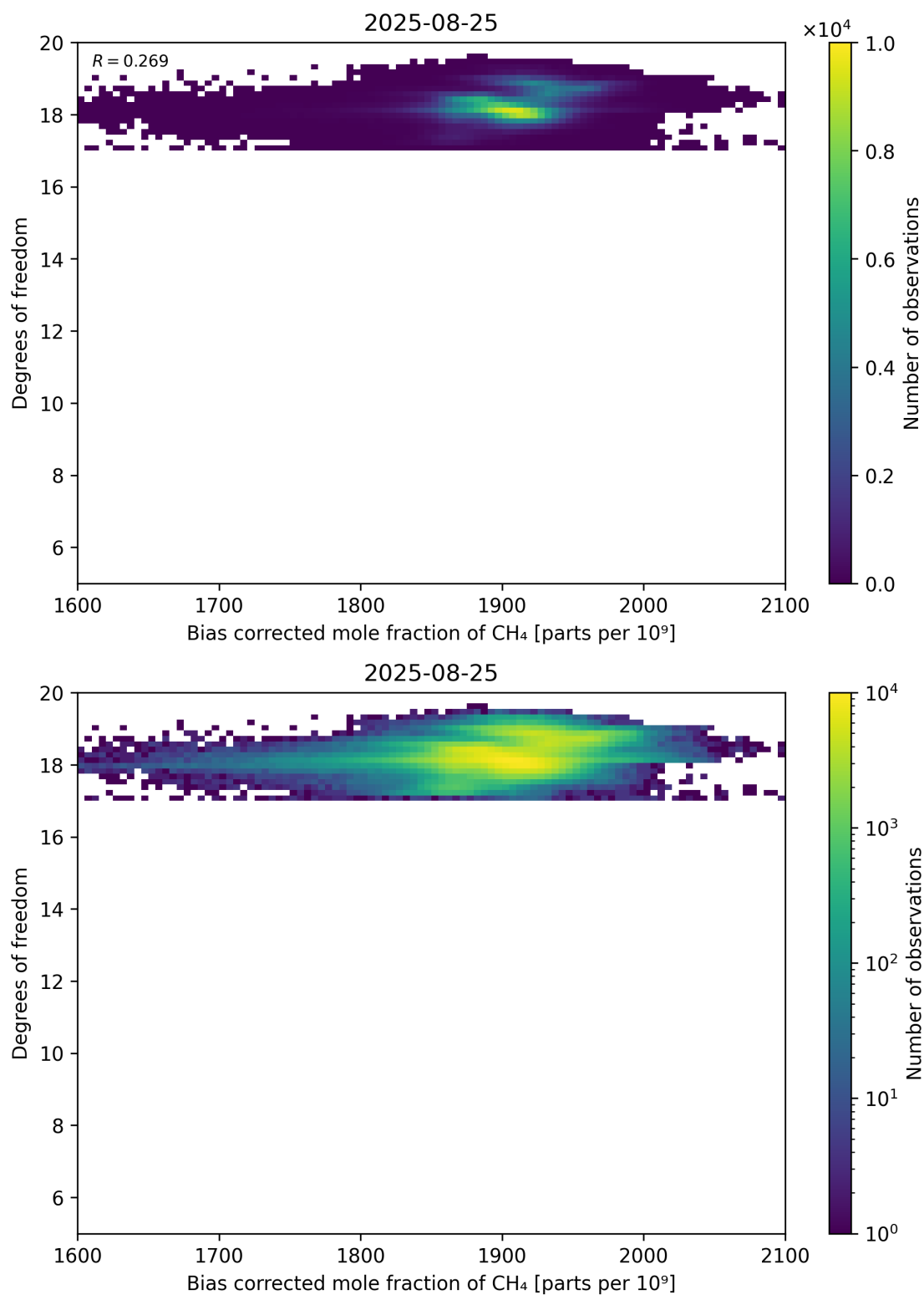
Figure 65: Scatter density plot of “Bias corrected mole fraction of CH 4 ” against “Degrees of freedom” for 2025-08-25 to 2025-08-26.
