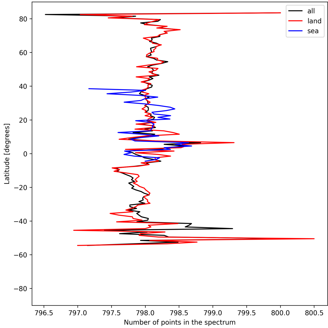
Figure 15: Zonal average of “Number of points in the spectrum” for 2025-08-25 to 2025-08-26.
