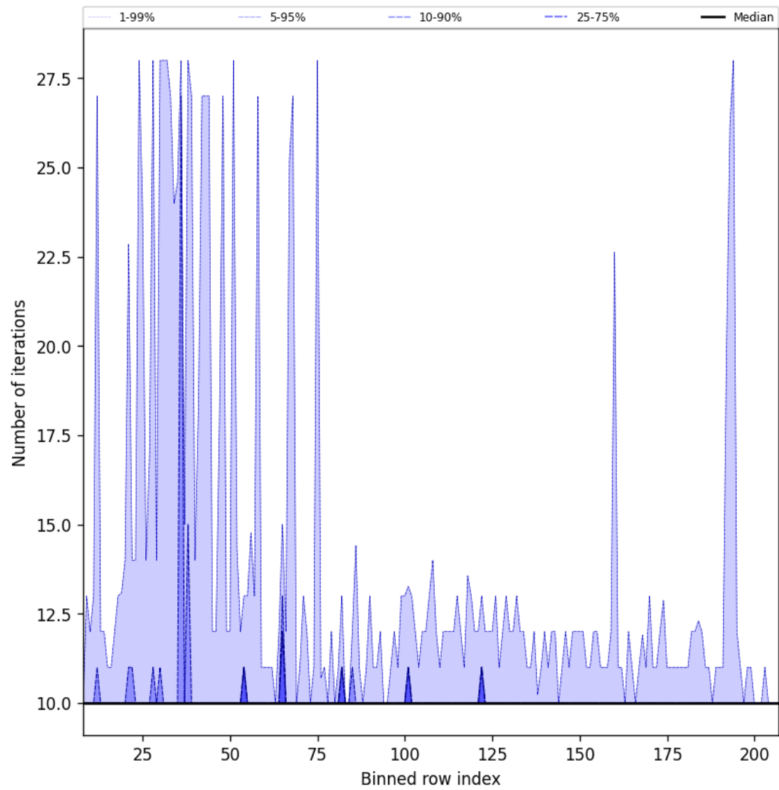
Figure 42: Along track statistics of “Number of iterations” for 2025-08-25 to 2025-08-26
