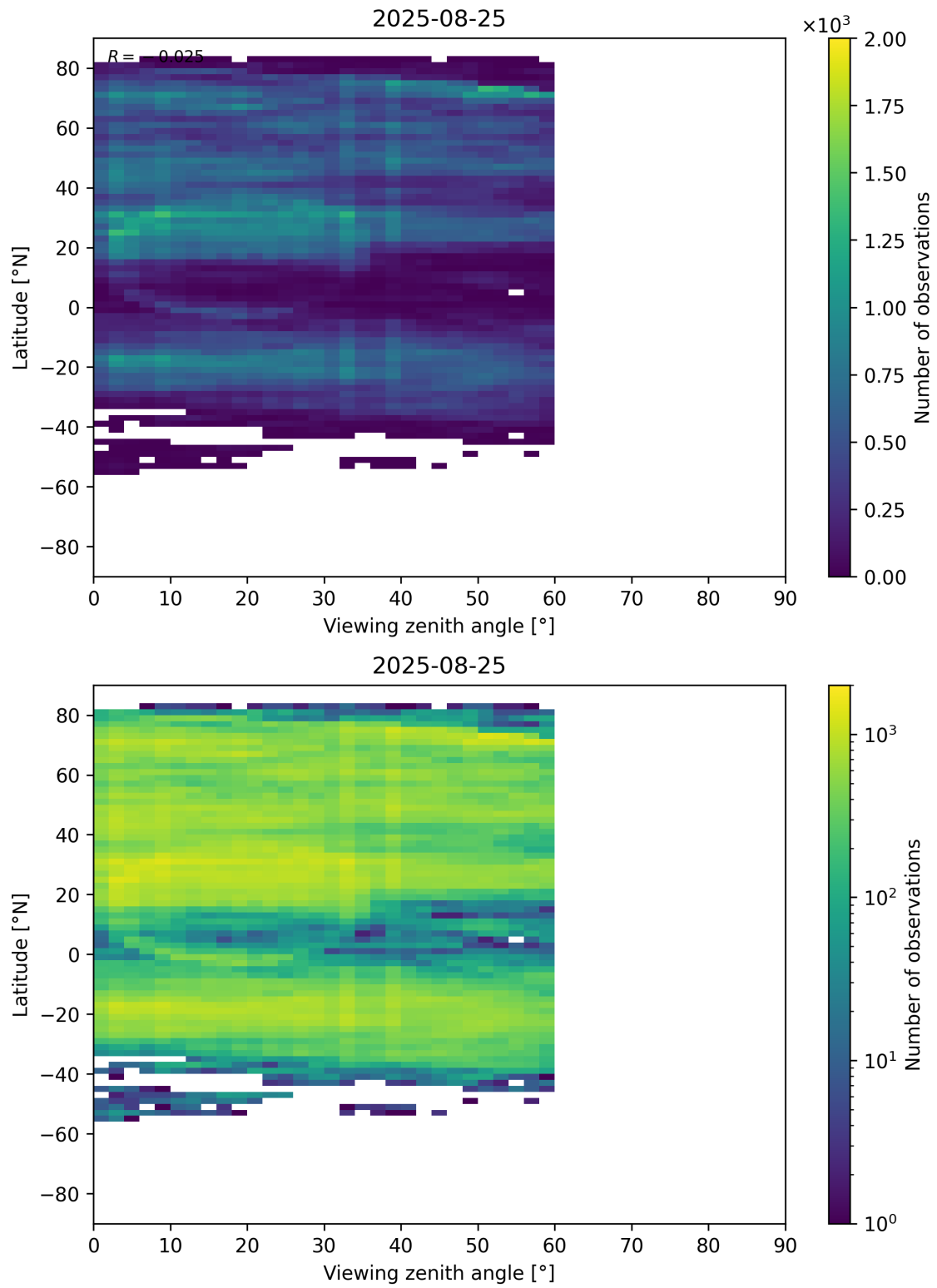
Figure 109: Scatter density plot of “Viewing zenith angle” against “Latitude” for 2025-08-25 to 2025-08-26.
