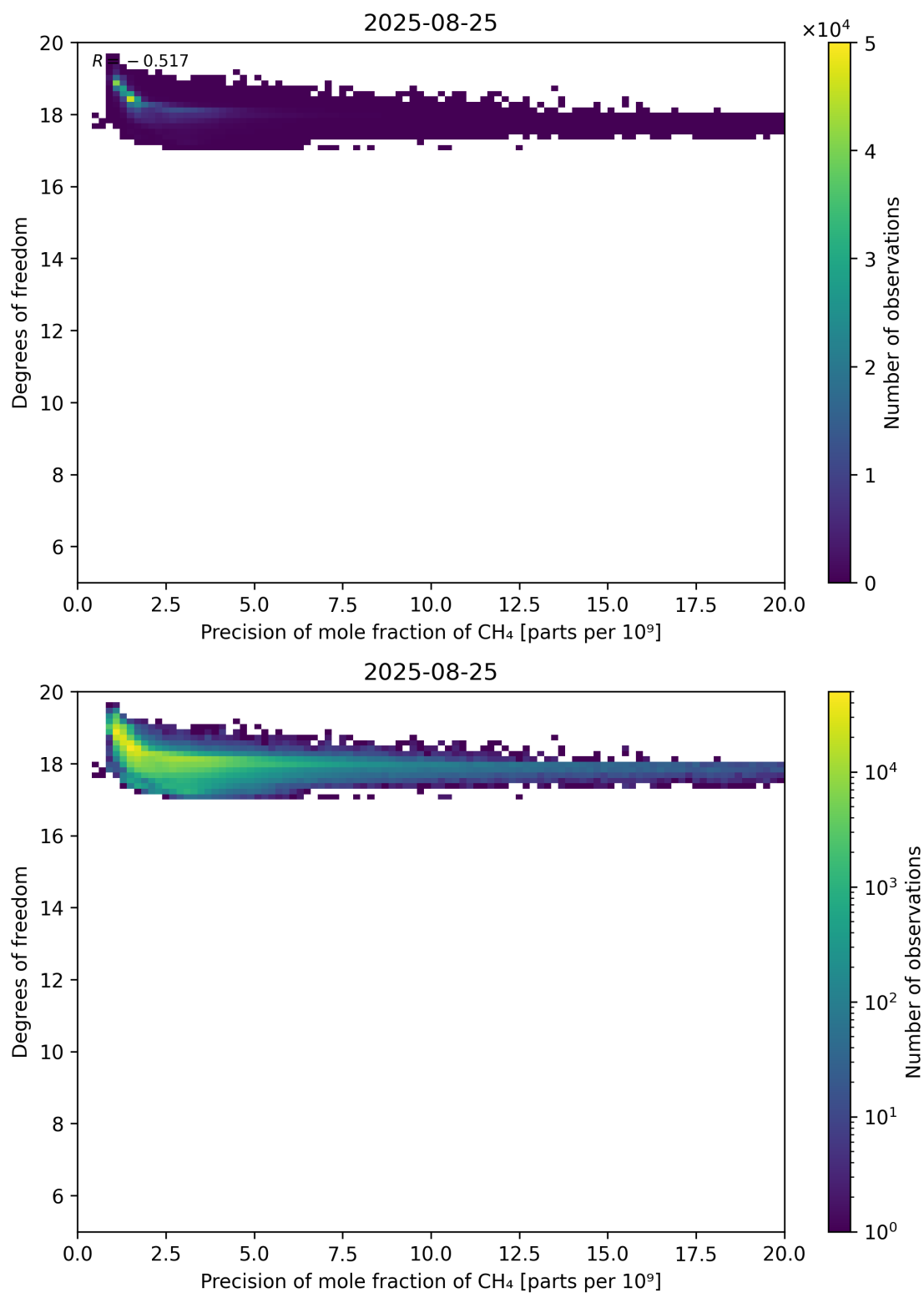
Figure 80: Scatter density plot of “Precision of mole fraction of CH 4 ” against “Degrees of freedom” for 2025-08-25 to 2025-08-26.
