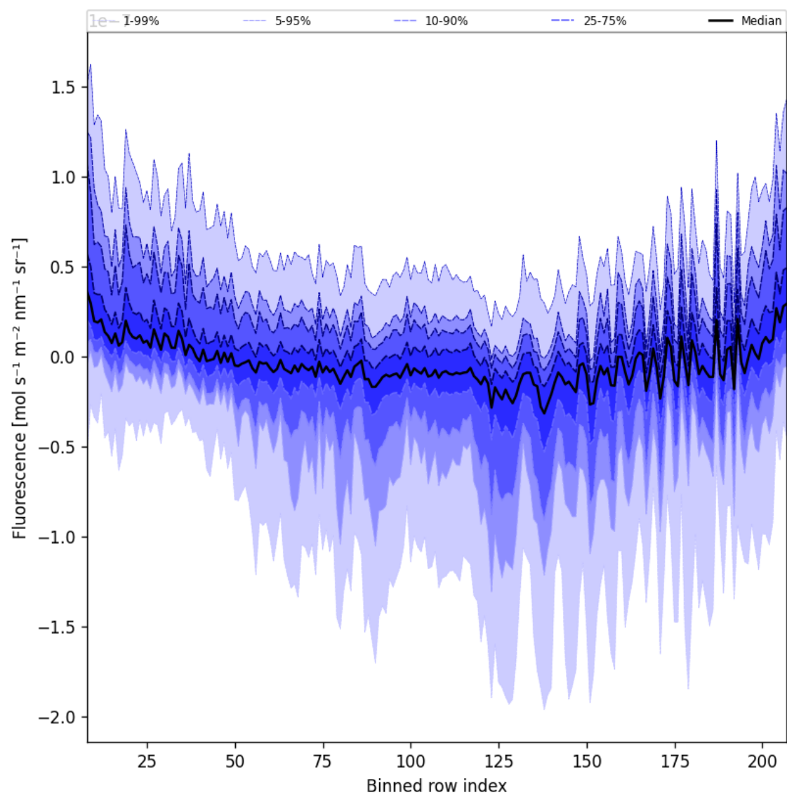
Figure 43: Along track statistics of “Fluorescence” for 2025-08-25 to 2025-08-26
