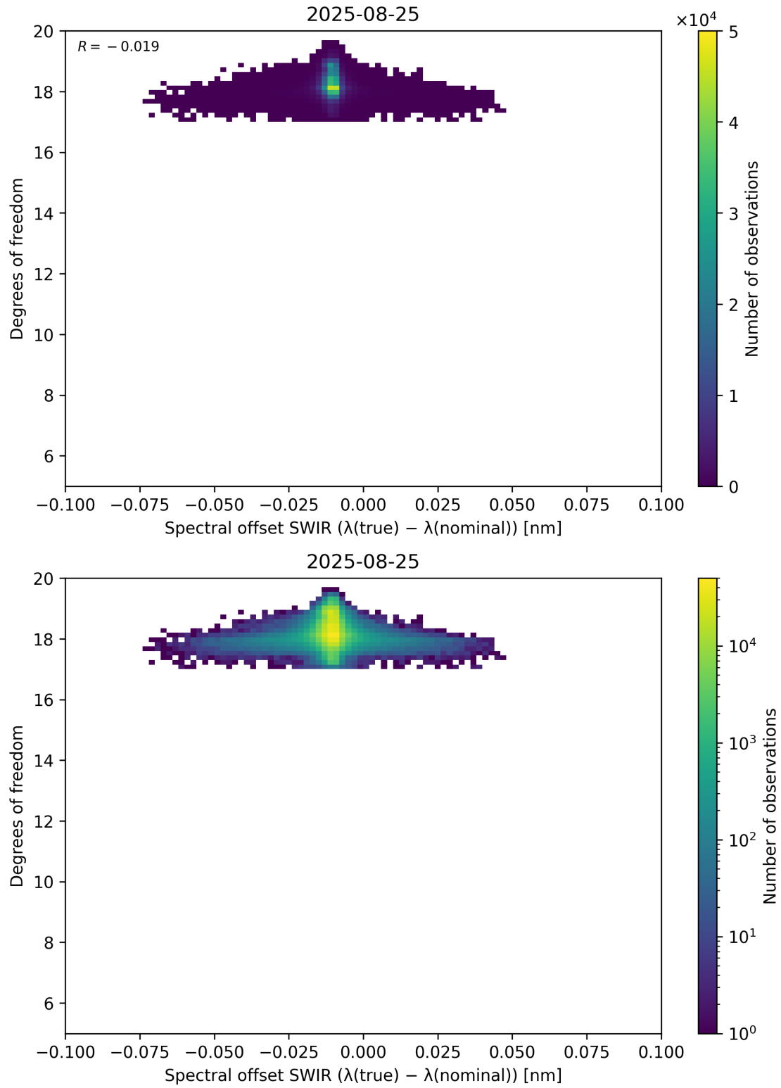
Figure 119: Scatter density plot of “Spectral offset SWIR ( \lambda_{\text{true}} - \lambda_{\text{nominal}} )” against “Degrees of freedom” for 2025-08-25 to 2025-08-26.
