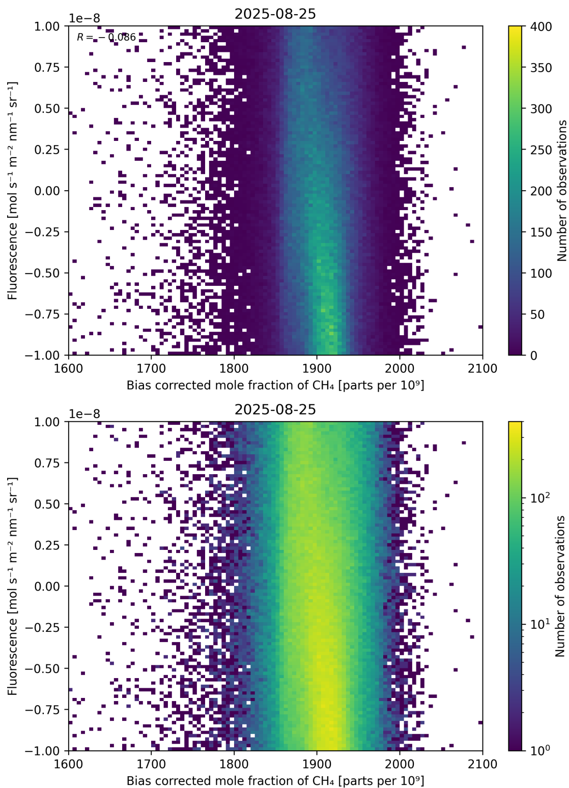
Figure 66: Scatter density plot of “Bias corrected mole fraction of CH 4 ” against “Fluorescence” for 2025-08-25 to 2025-08-26.
