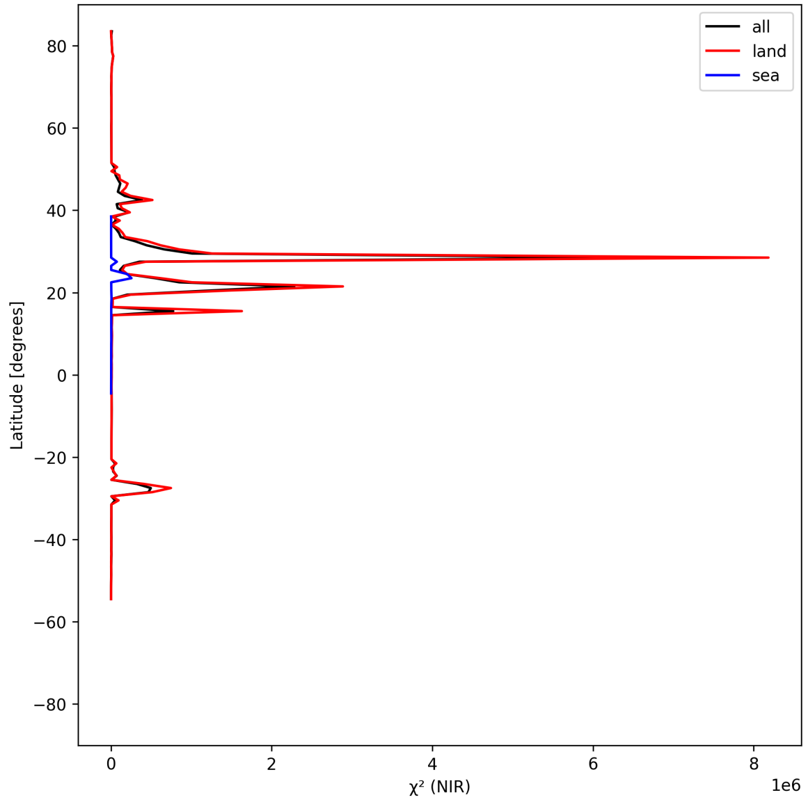
Figure 18: Zonal average of “ \chi^2 (NIR)” for 2025-08-25 to 2025-08-26.
