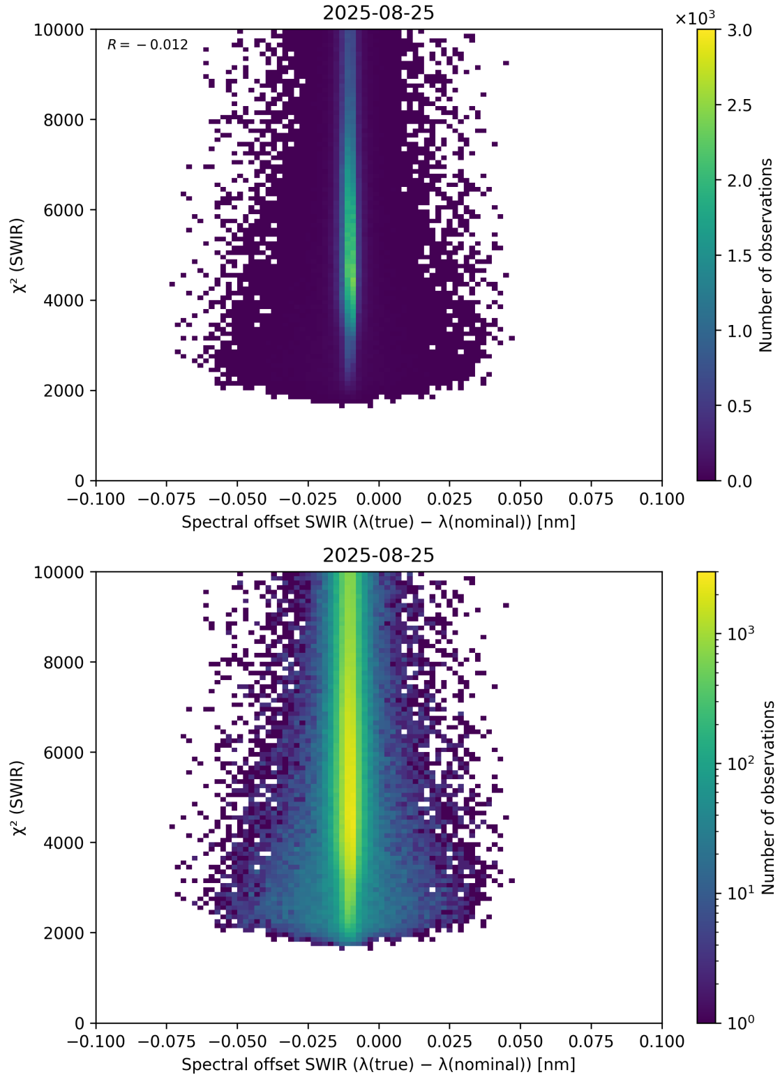
Figure 118: Scatter density plot of “Spectral offset SWIR ( \lambda_{\text{true}} - \lambda_{\text{nominal}} )” against “ \chi^2 (SWIR)” for 2025-08-25 to 2025-08-26.
