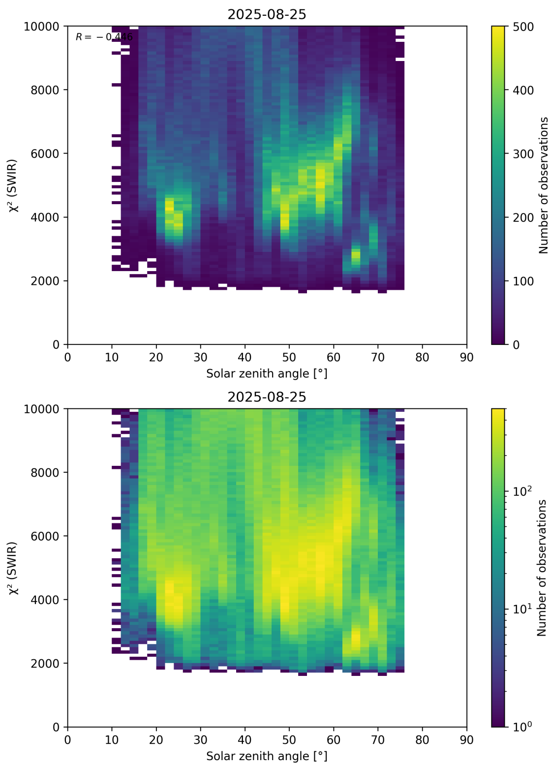
Figure 95: Scatter density plot of “Solar zenith angle” against “ \chi^2 (SWIR)” for 2025-08-25 to 2025-08-26.
