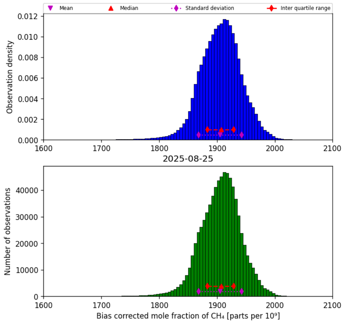
Figure 25: Histogram of “Bias corrected mole fraction of CH 4 ” for 2025-08-25 to 2025-08-26
