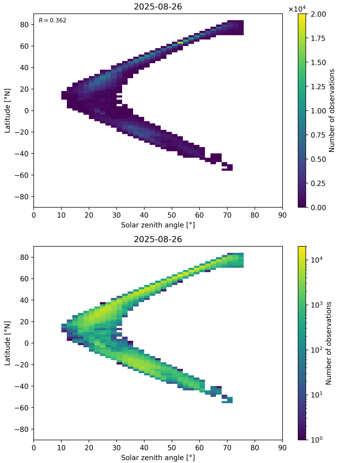
Figure 98: Scatter density plot of “Solar zenith angle” against “Latitude” for 2025-08-25 to 2025-08-27.
