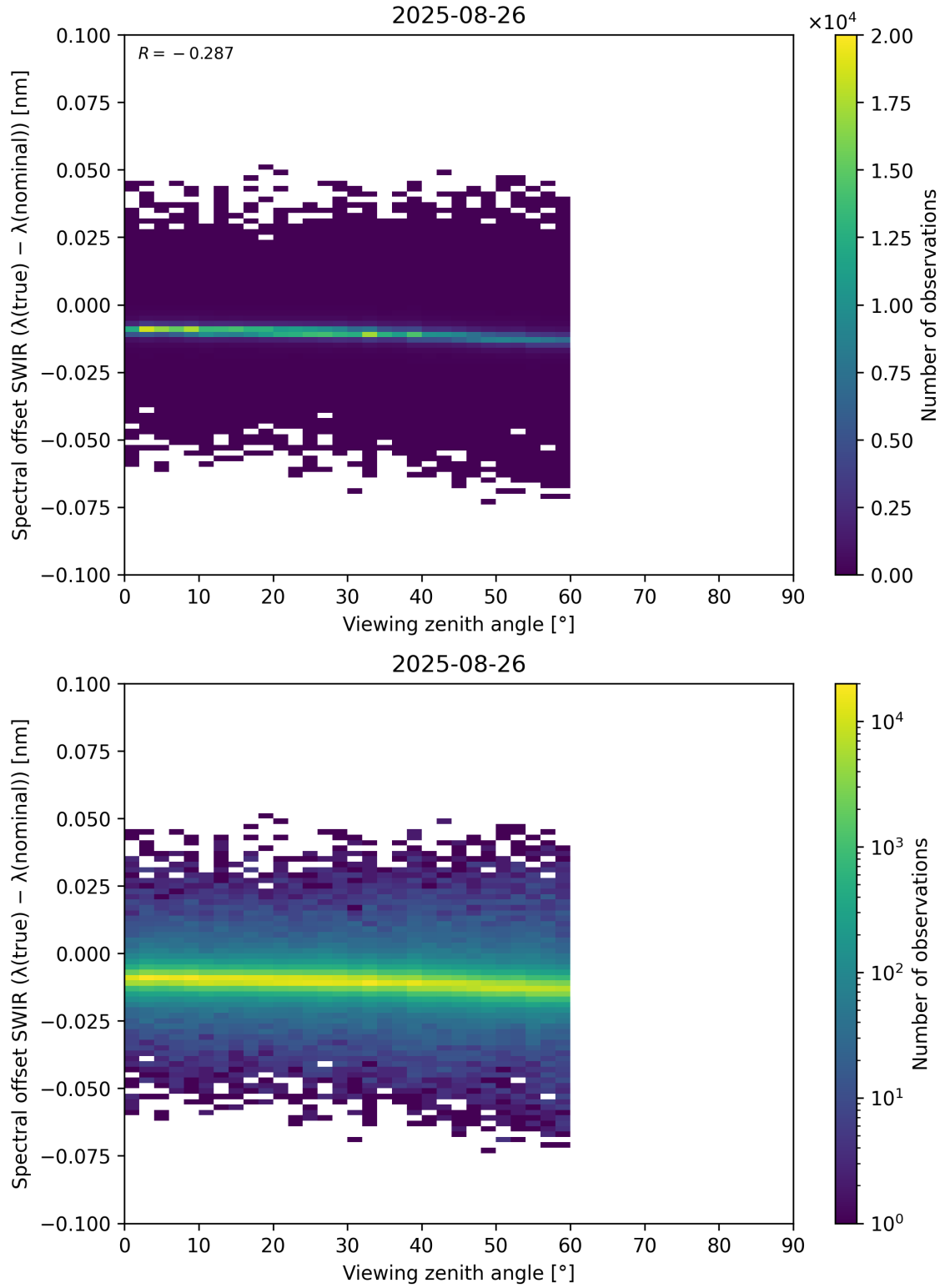
Figure 116: Scatter density plot of “Viewing zenith angle” against “Spectral offset SWIR ( \lambda_{\text{true}} - \lambda_{\text{nominal}} )” for 2025-08-25 to 2025-08-27.
