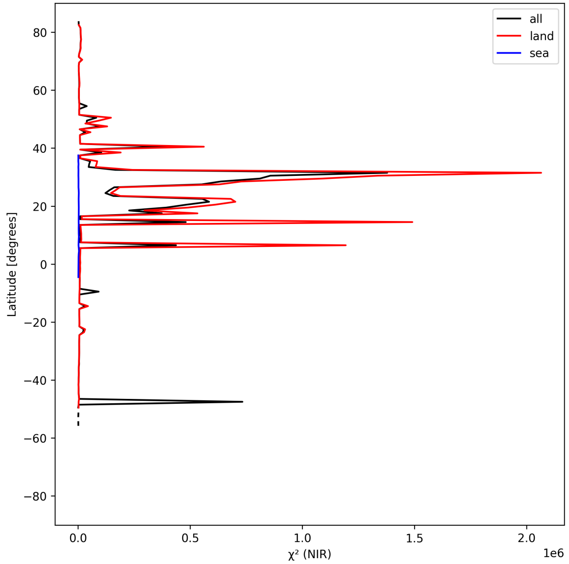
Figure 18: Zonal average of “ \chi^2 (NIR)” for 2025-08-25 to 2025-08-27.
