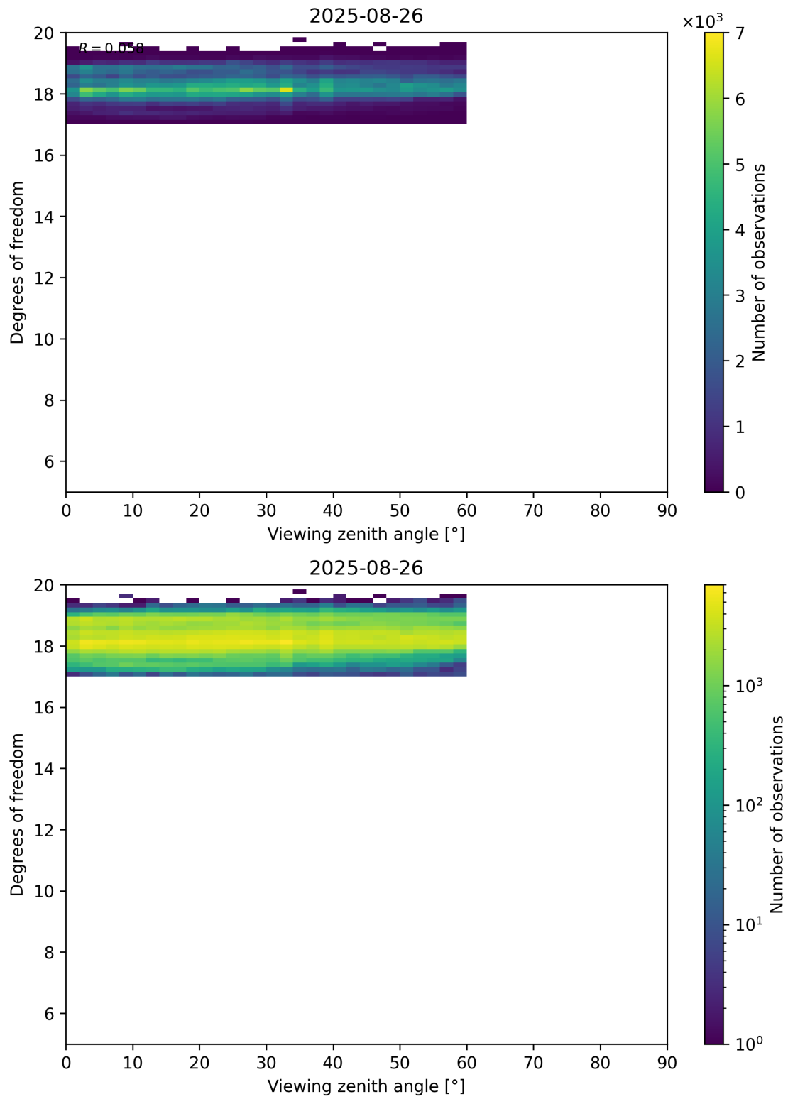
Figure 107: Scatter density plot of “Viewing zenith angle” against “Degrees of freedom” for 2025-08-25 to 2025-08-27.
