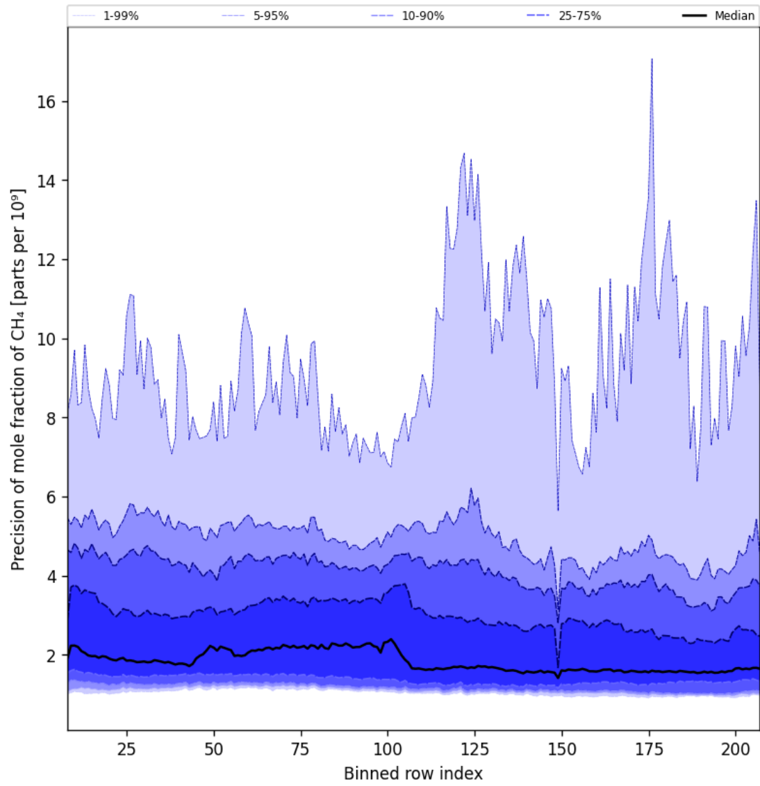
Figure 35: Along track statistics of “Precision of mole fraction of CH 4 ” for 2025-08-25 to 2025-08-27
