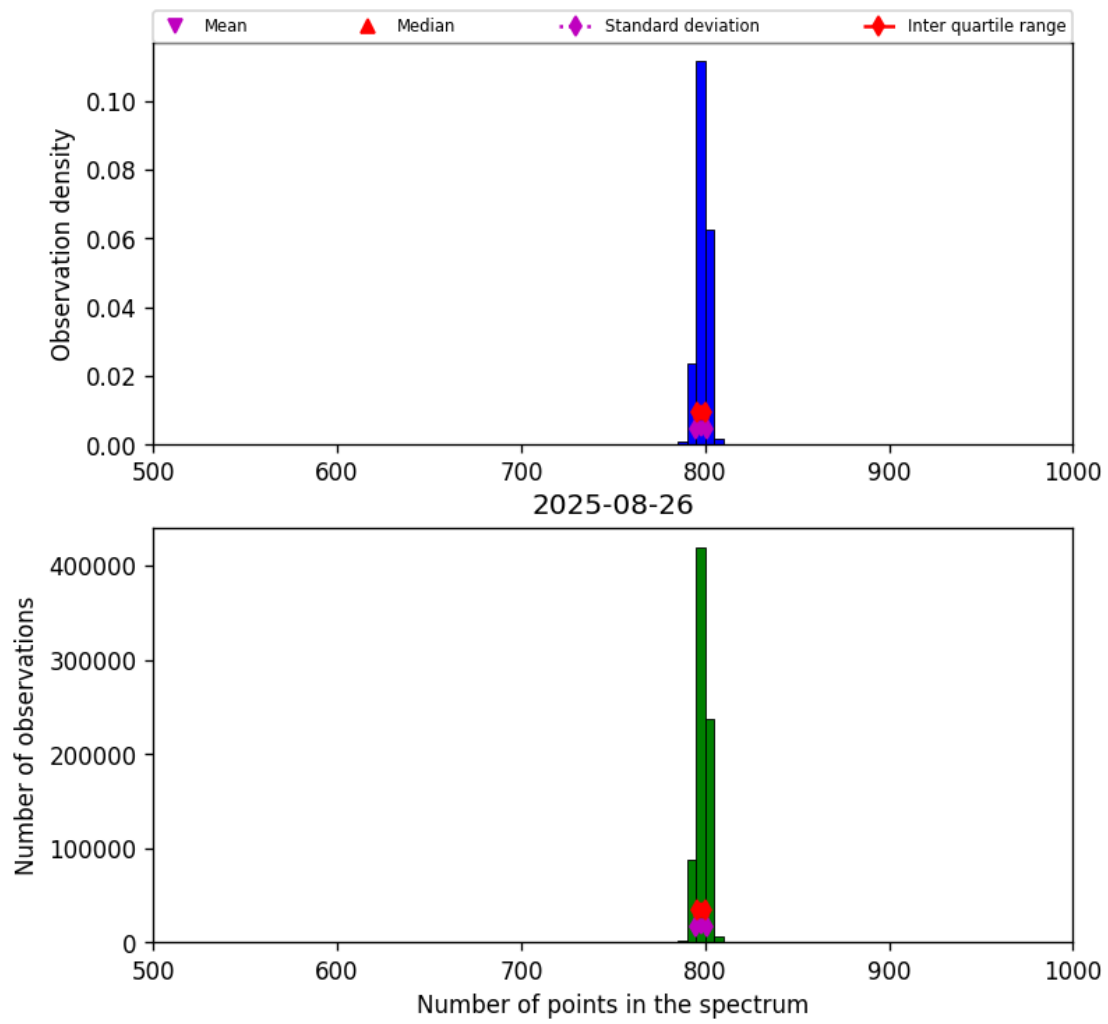
Figure 26: Histogram of “Number of points in the spectrum” for 2025-08-25 to 2025-08-27
