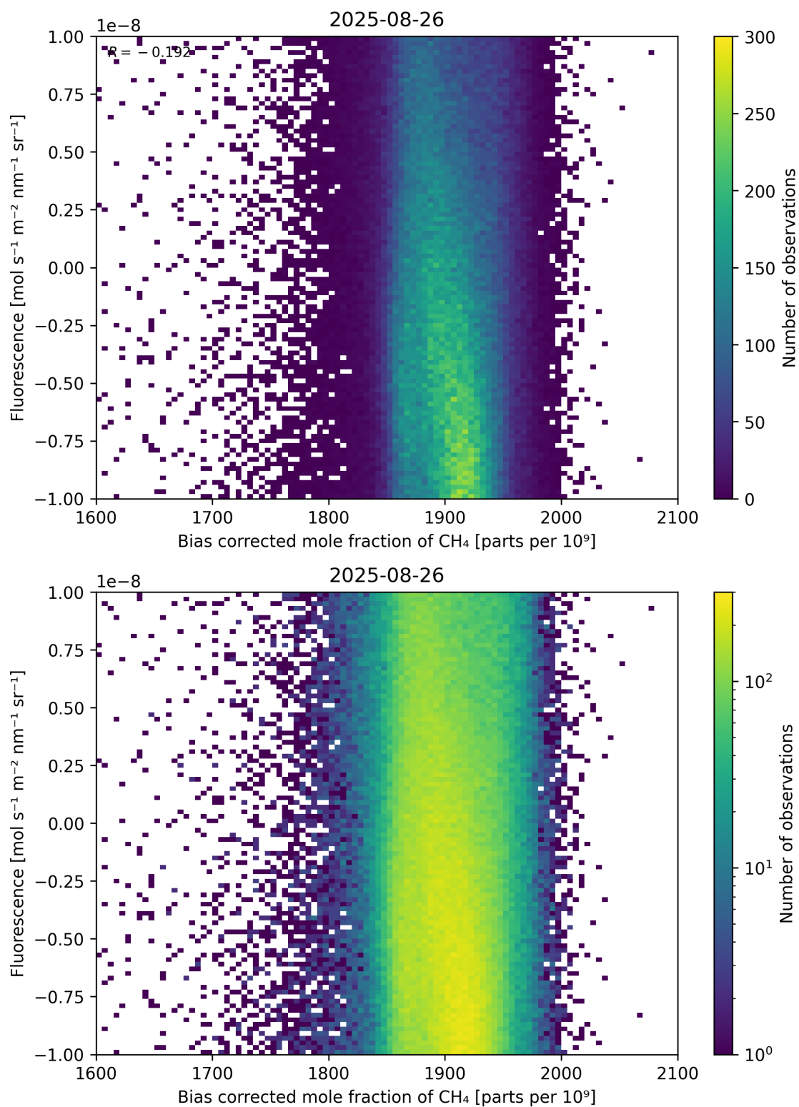
Figure 66: Scatter density plot of “Bias corrected mole fraction of \text{CH}_4 ” against “Fluorescence” for 2025-08-25 to 2025-08-27.
