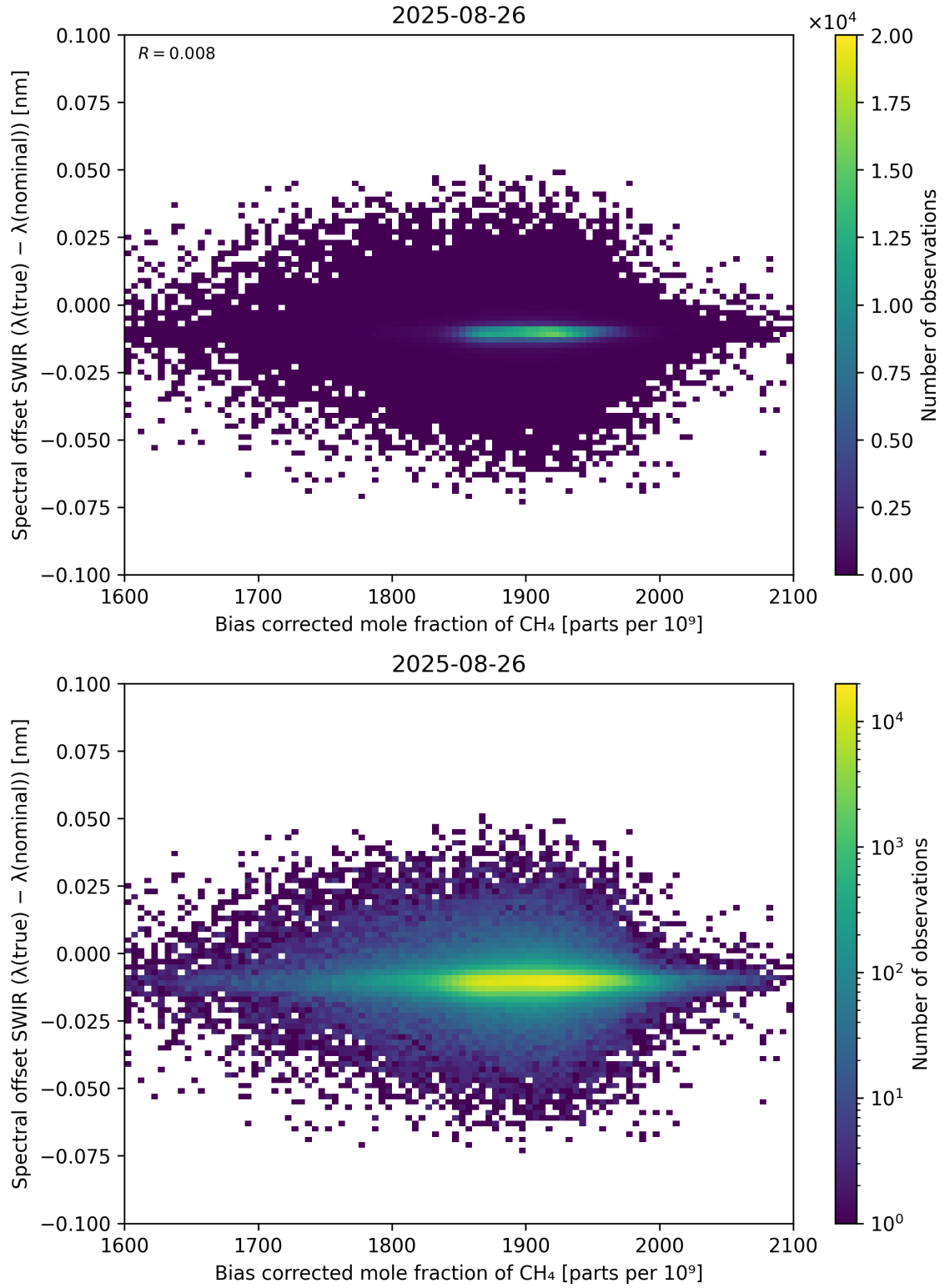
Figure 69: Scatter density plot of “Bias corrected mole fraction of \text{CH}_4 ” against “Spectral offset SWIR ( \lambda_{\text{true}} - \lambda_{\text{nominal}} )” for 2025-08-25 to 2025-08-27.
