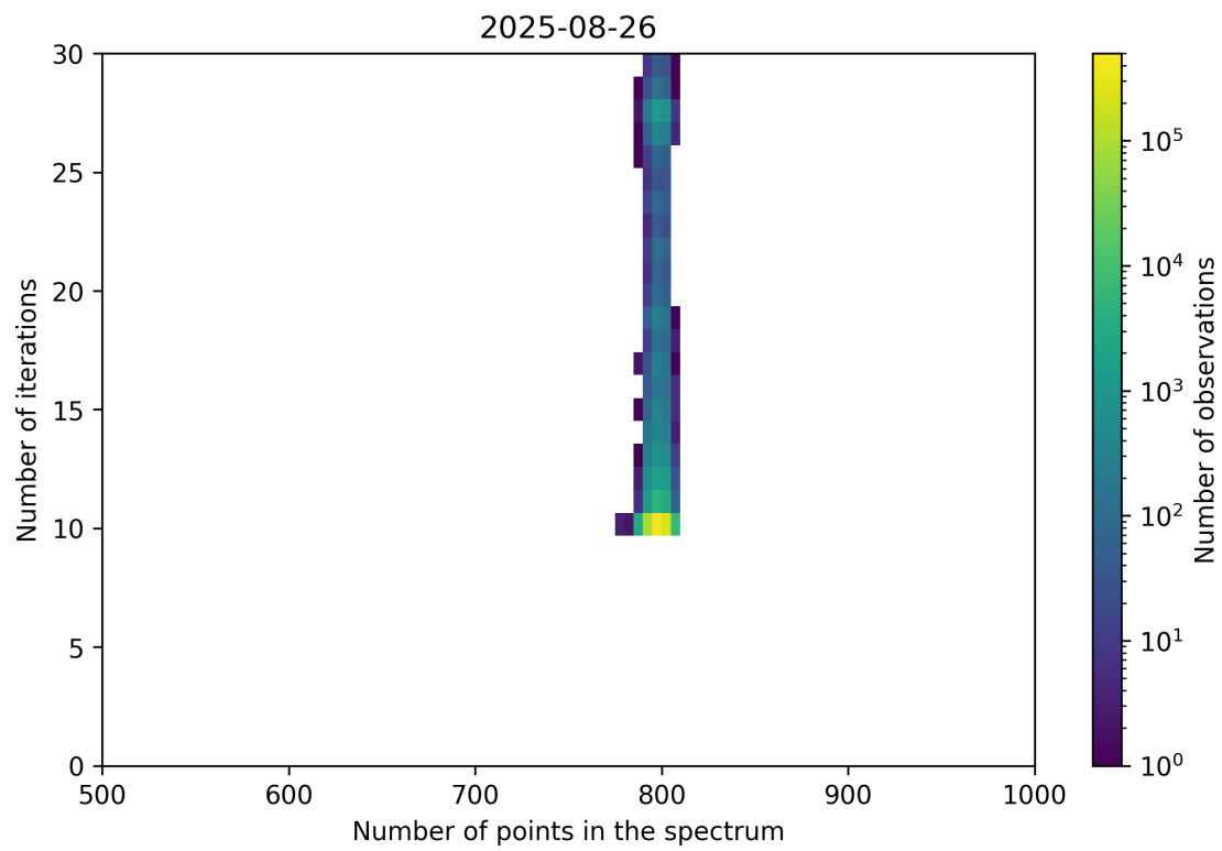
Figure 92: Scatter density plot of “Number of points in the spectrum” against “Number of iterations” for 2025-08-25 to 2025-08-27.
