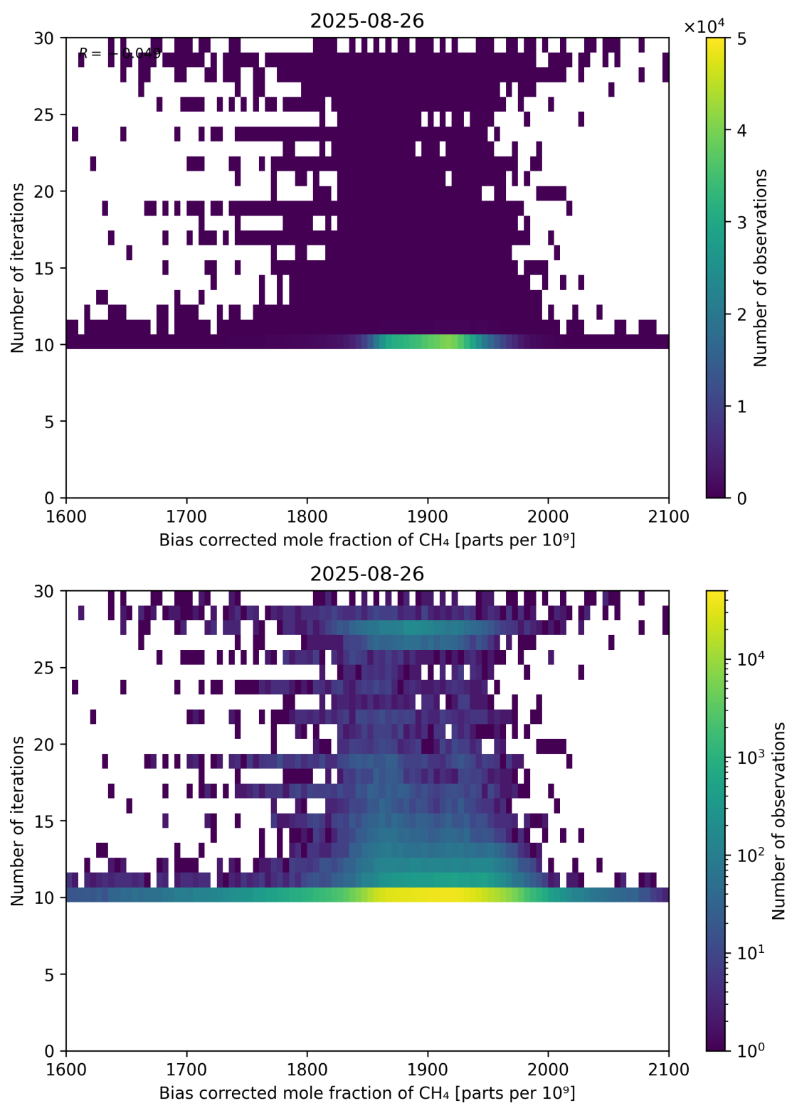
Figure 67: Scatter density plot of “Bias corrected mole fraction of \text{CH}_4 ” against “Number of iterations” for 2025-08-25 to 2025-08-27.
