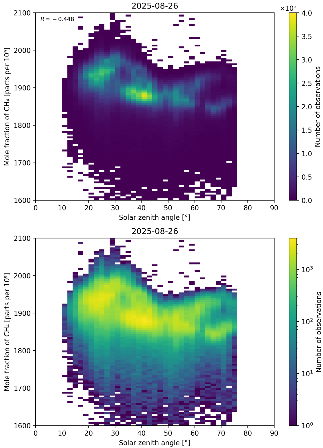
Figure 99: Scatter density plot of “Solar zenith angle” against “Mole fraction of CH 4 ” for 2025-08-25 to 2025-08-27.
