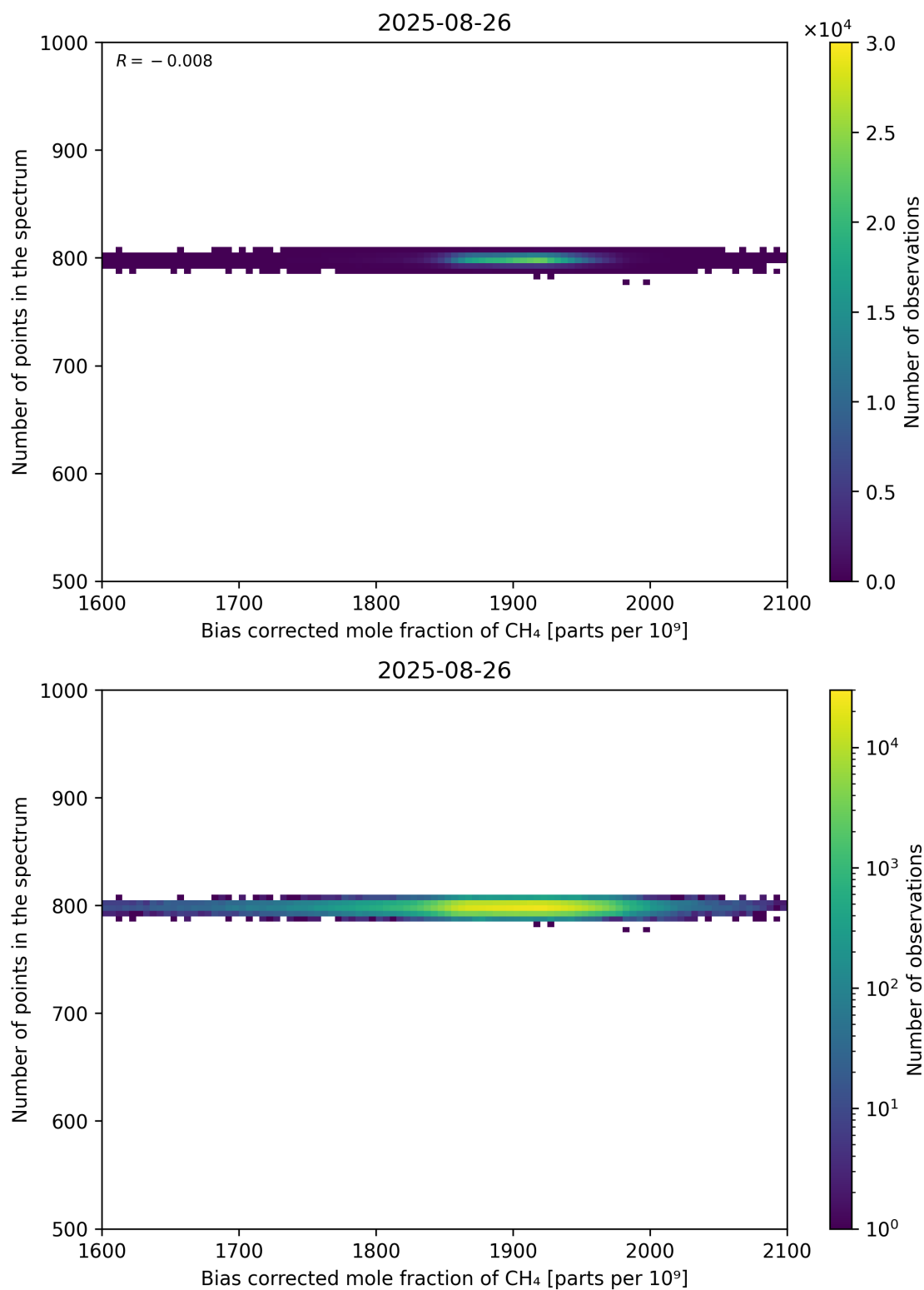
Figure 68: Scatter density plot of “Bias corrected mole fraction of CH 4 ” against “Number of points in the spectrum” for 2025-08-25 to 2025-08-27.
