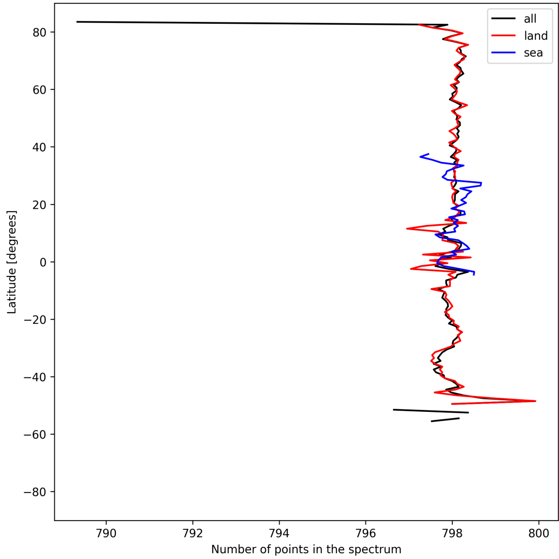
Figure 15: Zonal average of “Number of points in the spectrum” for 2025-08-25 to 2025-08-27.
