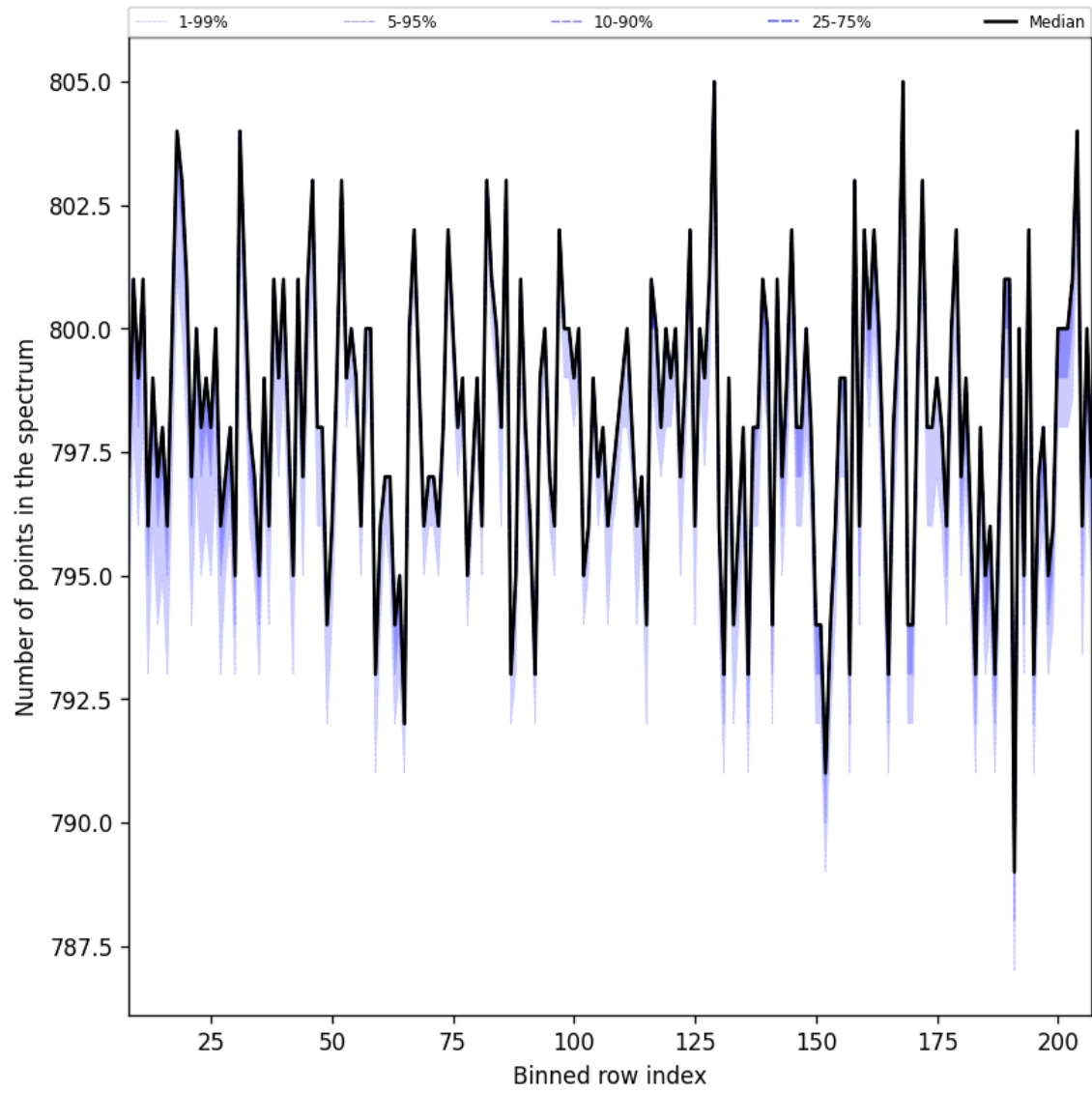
Figure 37: Along track statistics of “Number of points in the spectrum” for 2025-08-25 to 2025-08-27
