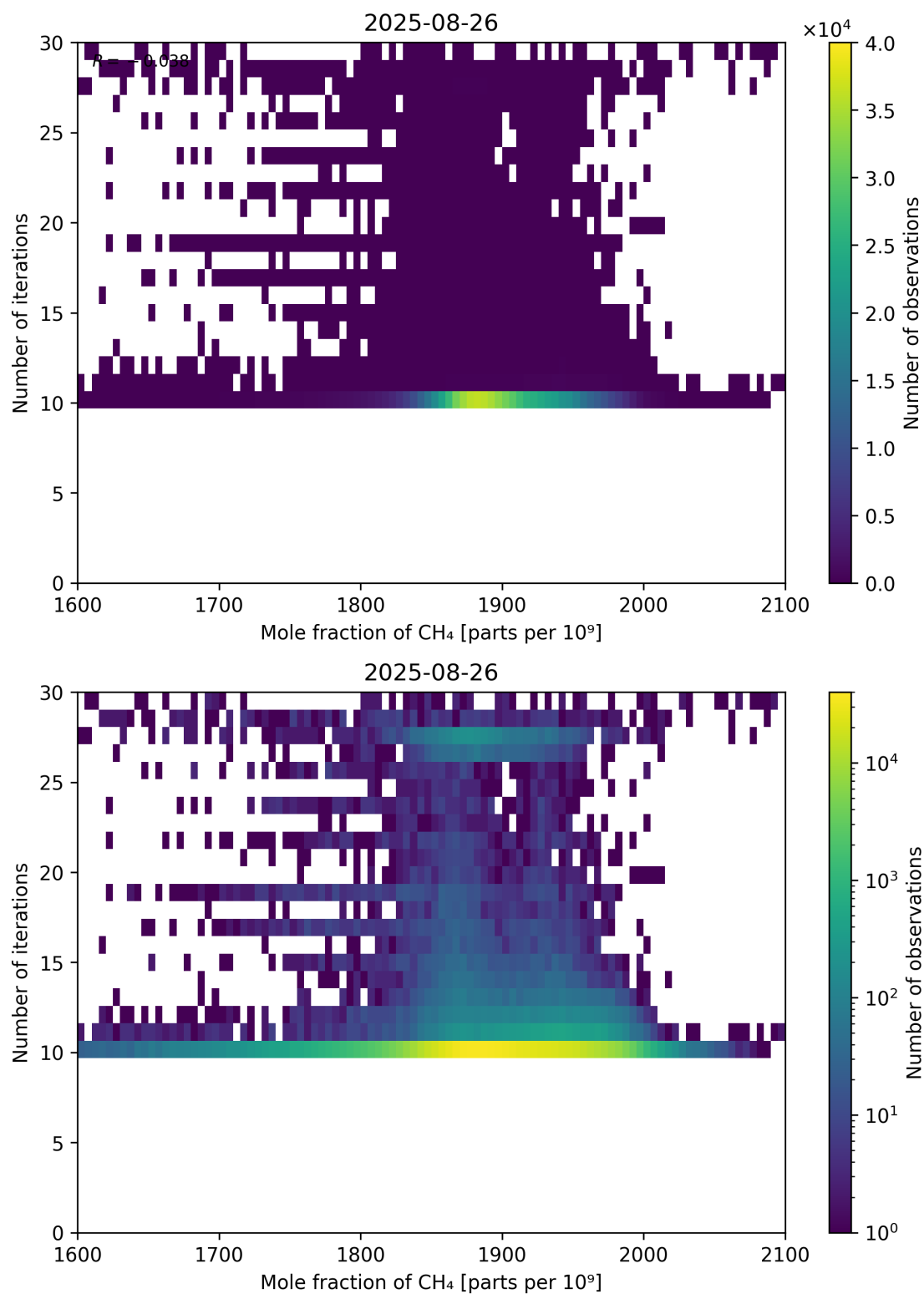
Figure 76: Scatter density plot of “Mole fraction of CH 4 ” against “Number of iterations” for 2025-08-25 to 2025-08-27.
