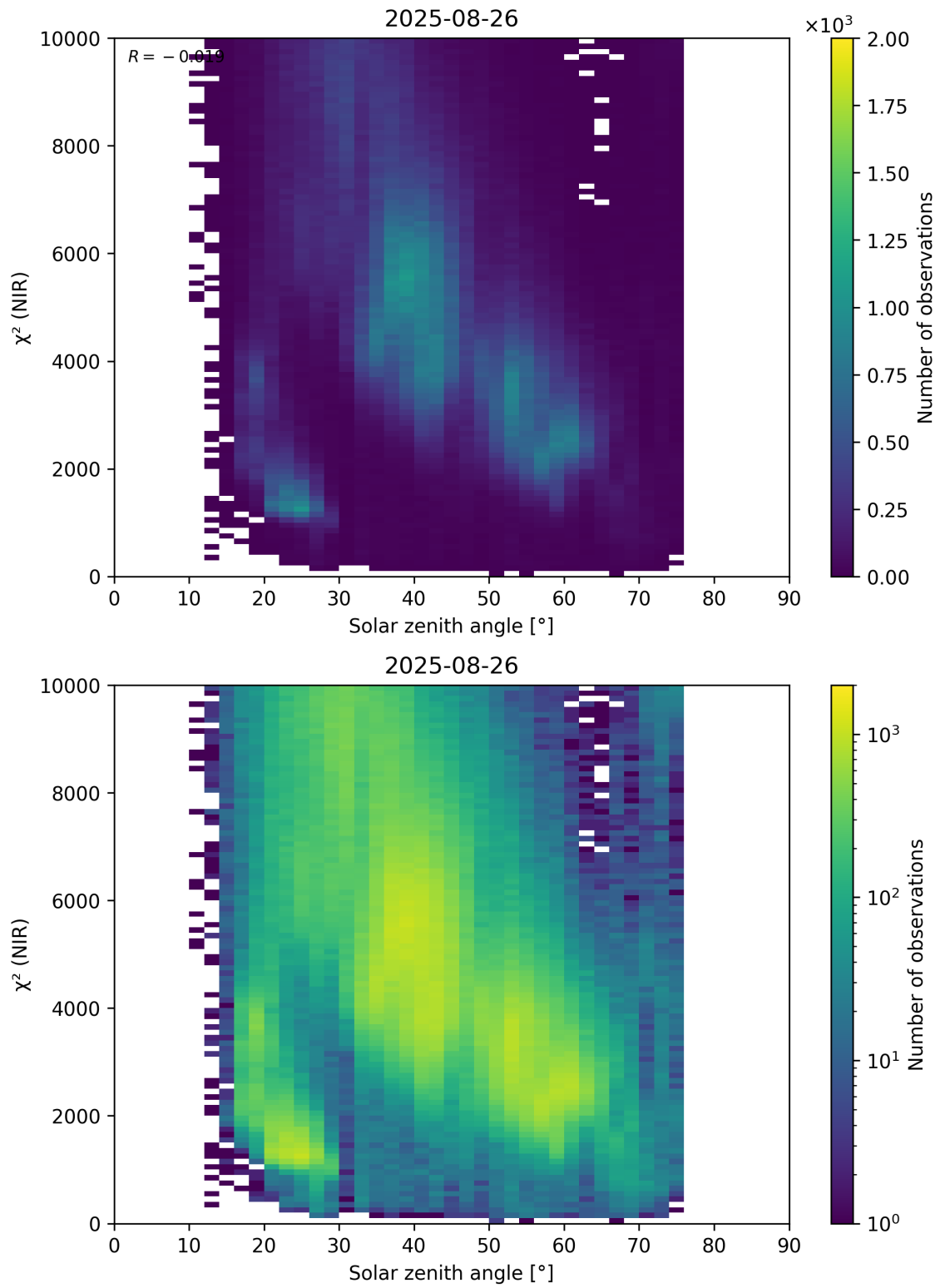
Figure 94: Scatter density plot of “Solar zenith angle” against “ \chi^2 (NIR)” for 2025-08-25 to 2025-08-27.
