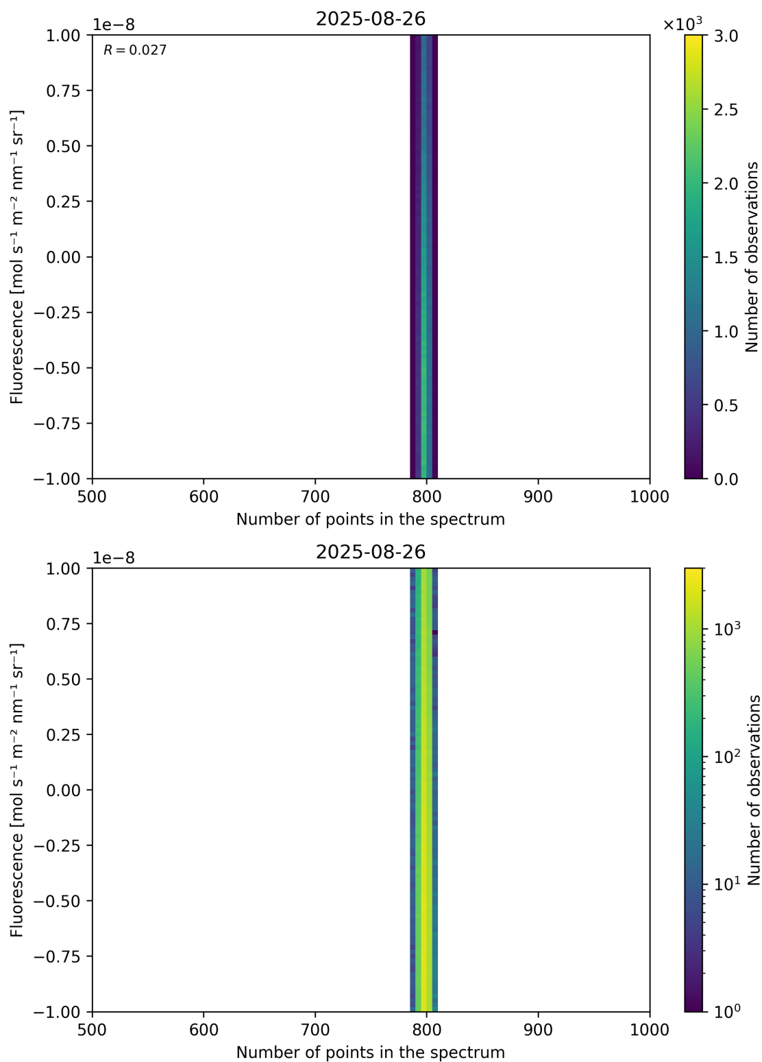
Figure 91: Scatter density plot of “Number of points in the spectrum” against “Fluorescence” for 2025-08-25 to 2025-08-27.
