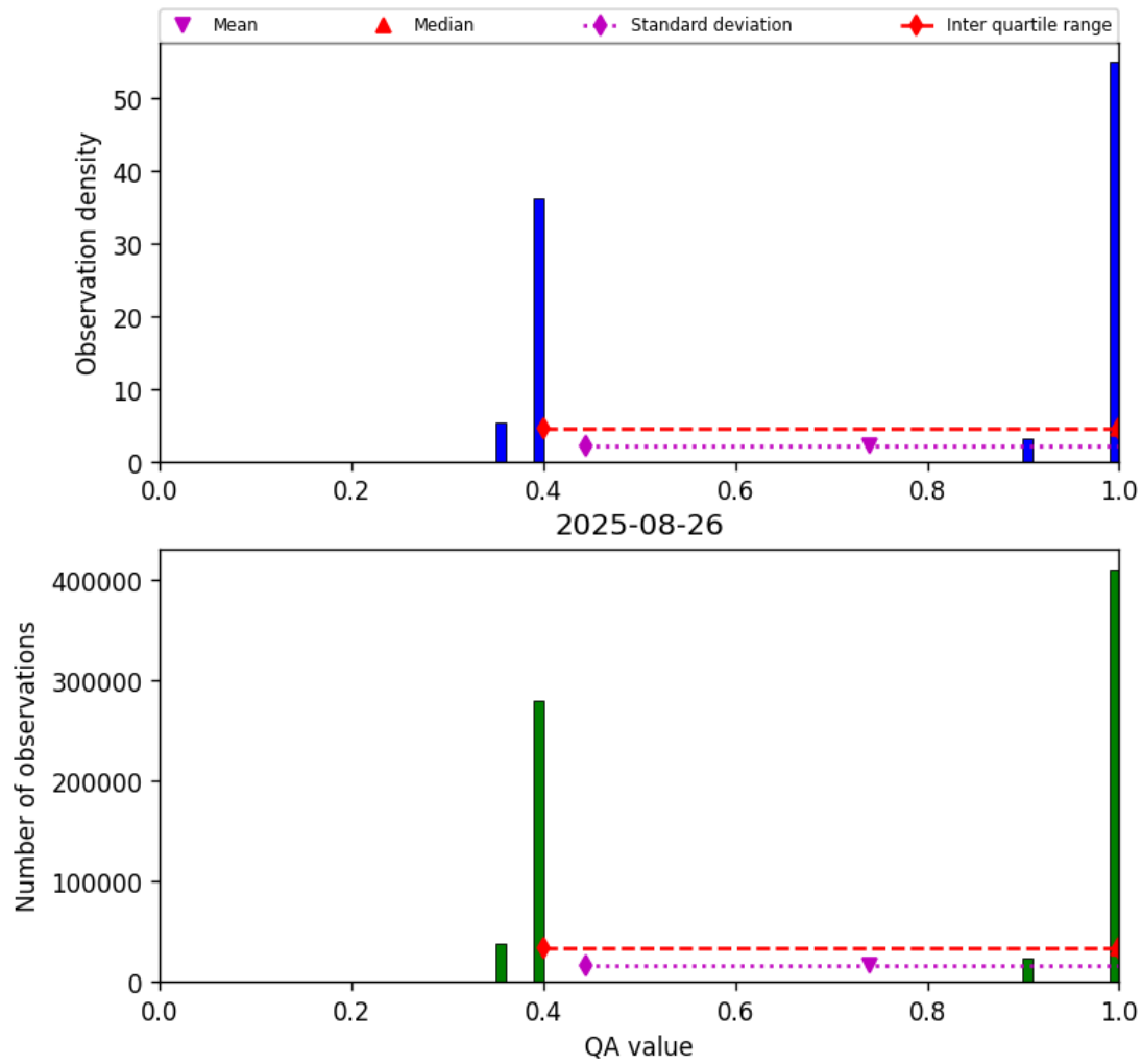
Figure 22: Histogram of “QA value” for 2025-08-25 to 2025-08-27
