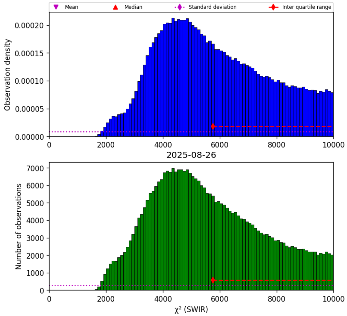
Figure 28: Histogram of “ \chi^2 (SWIR)” for 2025-08-25 to 2025-08-27
