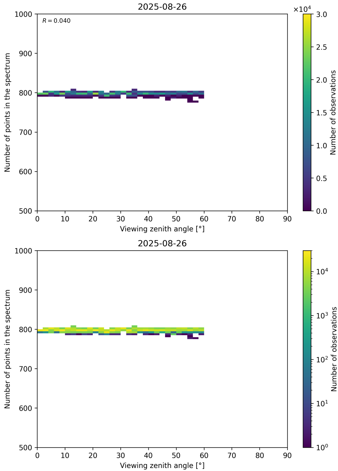
Figure 114: Scatter density plot of “Viewing zenith angle” against “Number of points in the spectrum” for 2025-08-25 to 2025-08-27.
