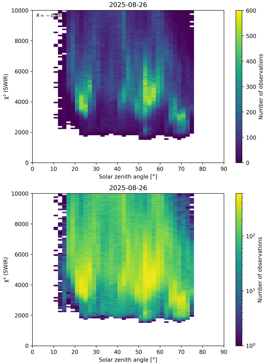
Figure 95: Scatter density plot of “Solar zenith angle” against “ \chi^2 (SWIR)” for 2025-08-25 to 2025-08-27.
