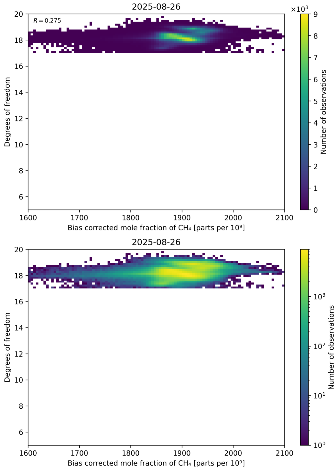
Figure 65: Scatter density plot of “Bias corrected mole fraction of CH 4 ” against “Degrees of freedom” for 2025-08-25 to 2025-08-27.
