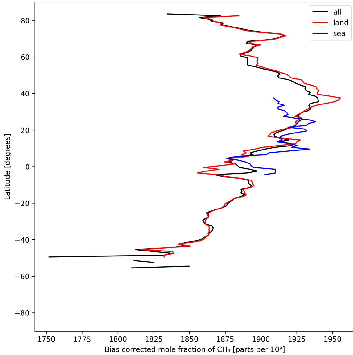
Figure 14: Zonal average of “Bias corrected mole fraction of CH 4 ” for 2025-08-25 to 2025-08-27.
