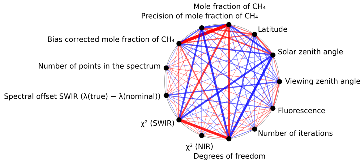
Figure 1: Map of correlation graph for 2025-08-25 to 2025-08-27.
