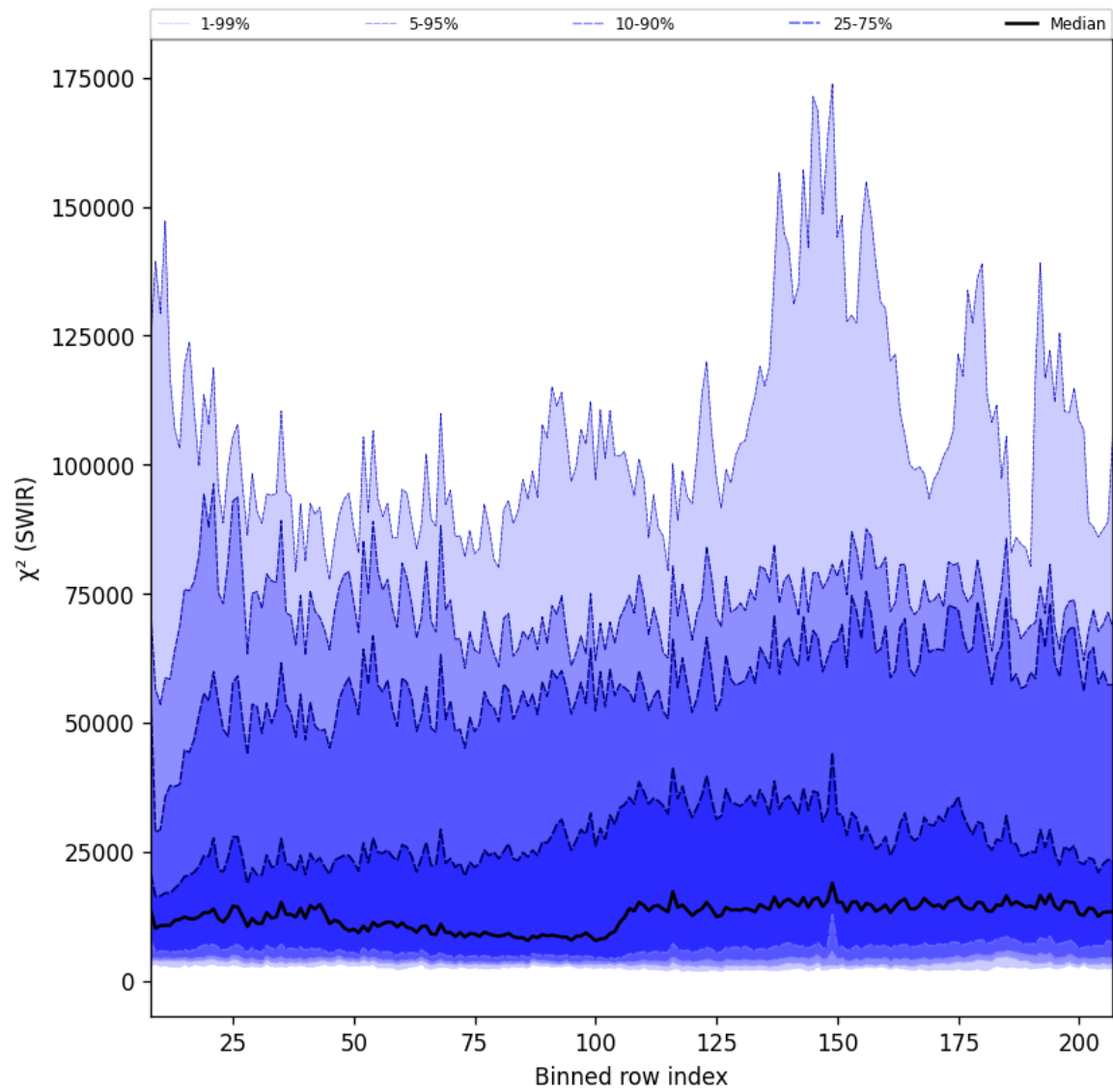
Figure 39: Along track statistics of “ \chi^2 (SWIR)” for 2025-08-25 to 2025-08-27
