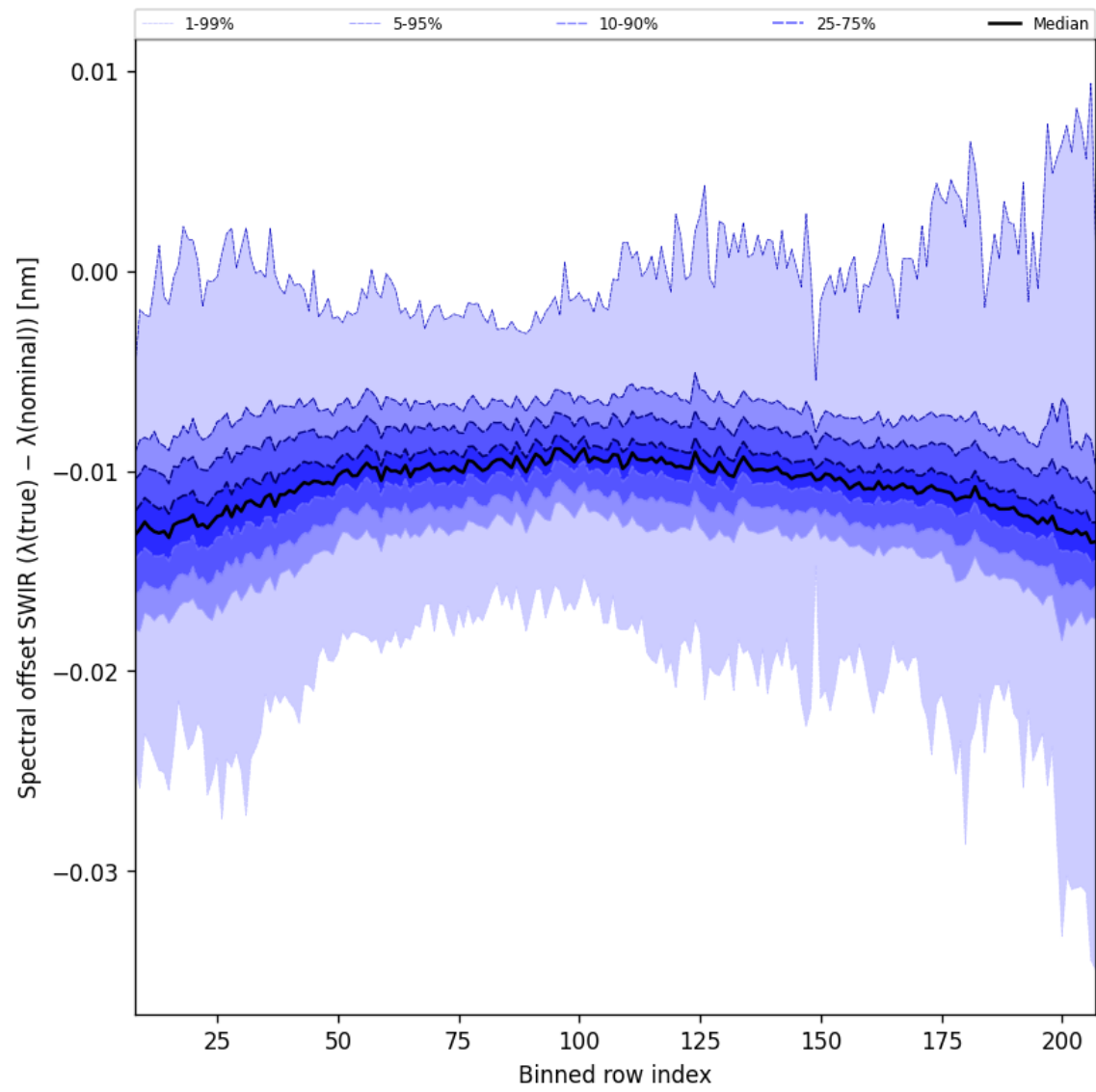
Figure 38: Along track statistics of “Spectral offset SWIR ( \lambda_{\text{true}} - \lambda_{\text{nominal}} )” for 2025-08-25 to 2025-08-27
