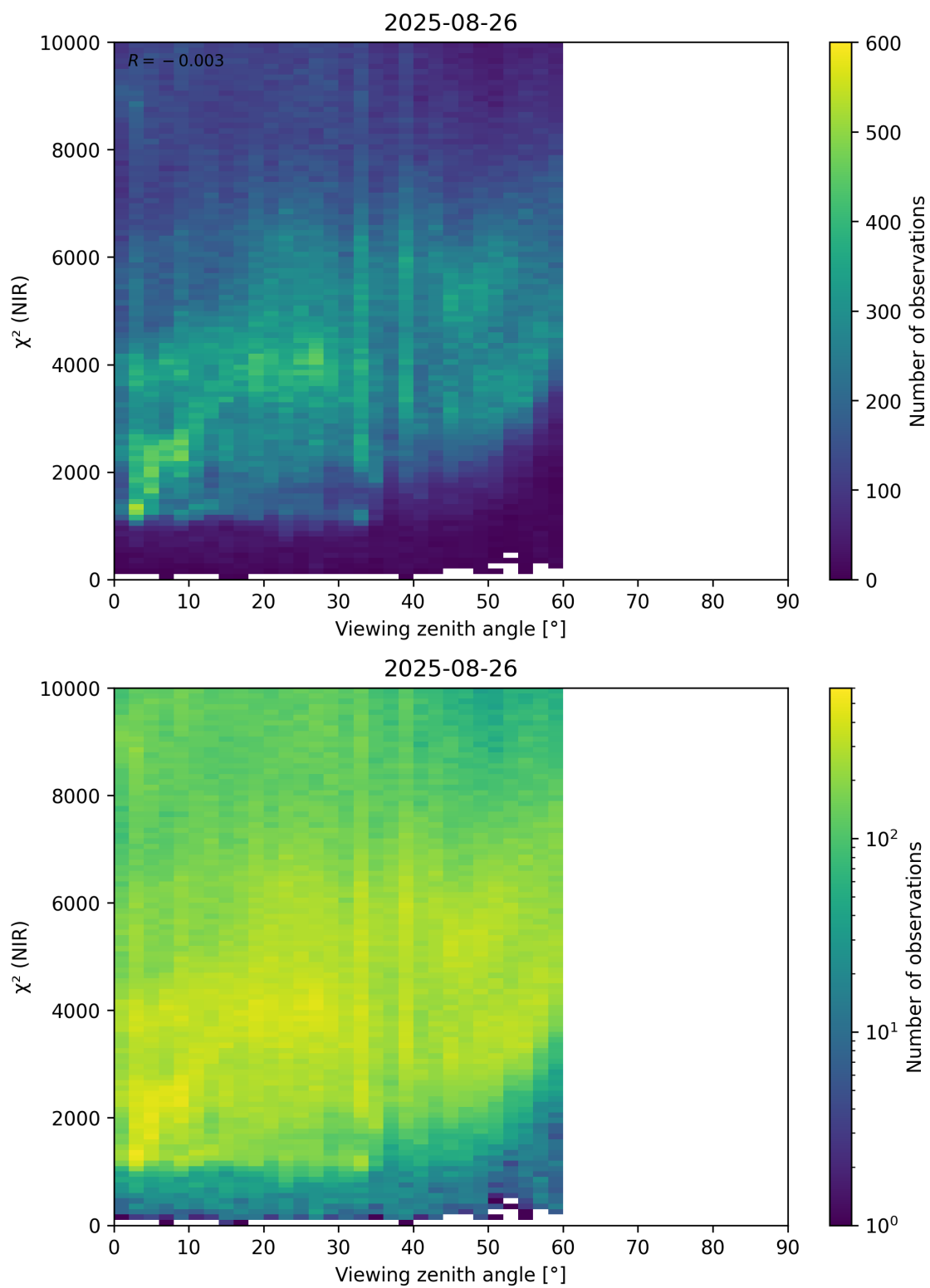
Figure 105: Scatter density plot of “Viewing zenith angle” against “ \chi^2 (NIR)” for 2025-08-25 to 2025-08-27.
