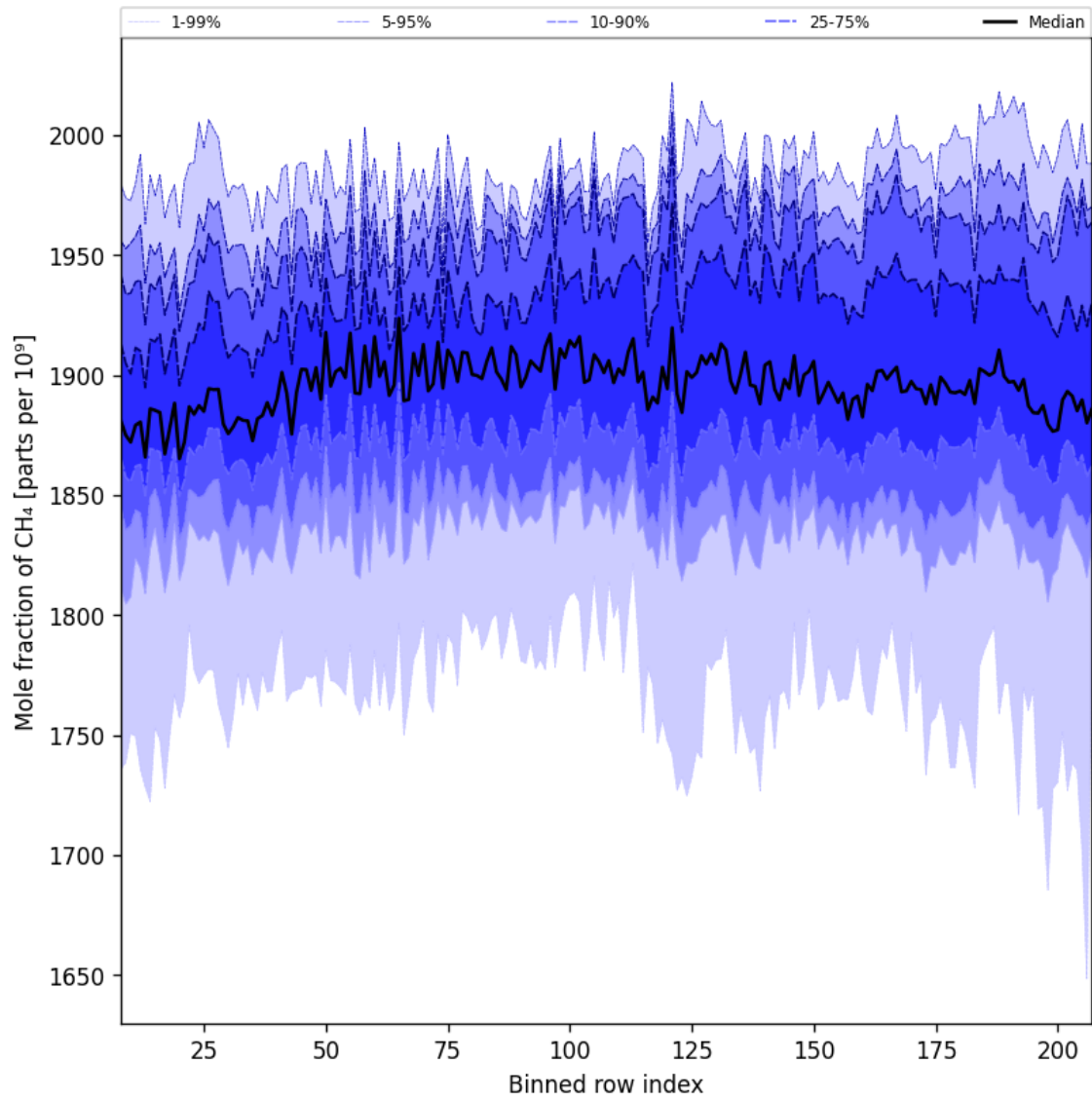
Figure 34: Along track statistics of “Mole fraction of CH 4 ” for 2025-08-25 to 2025-08-27
