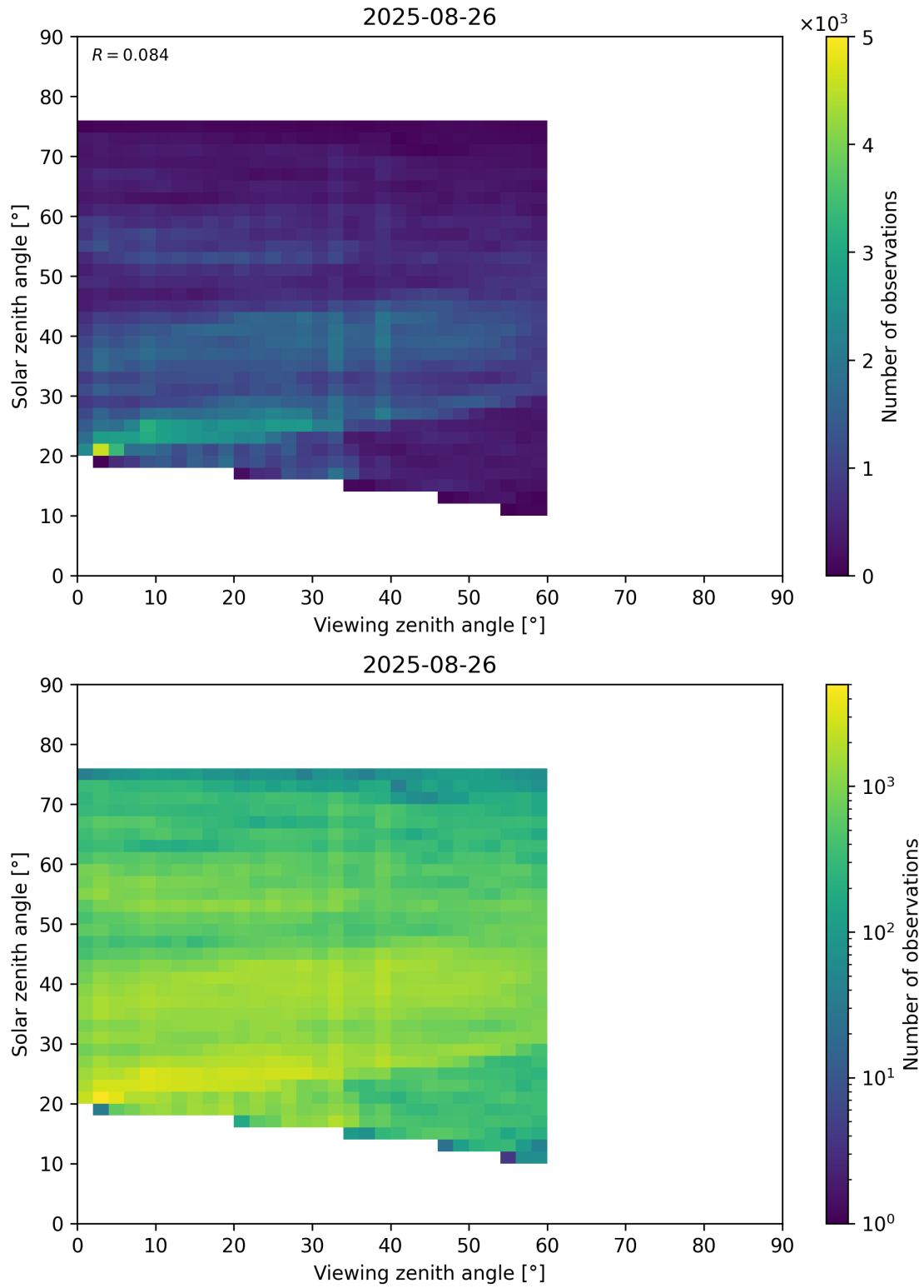
Figure 115: Scatter density plot of “Viewing zenith angle” against “Solar zenith angle” for 2025-08-25 to 2025-08-27.
