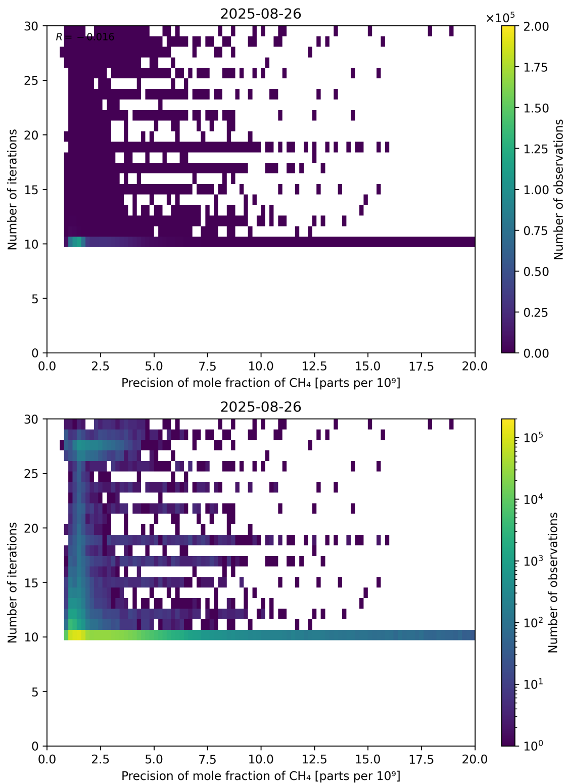
Figure 83: Scatter density plot of “Precision of mole fraction of CH 4 ” against “Number of iterations” for 2025-08-25 to 2025-08-27.
