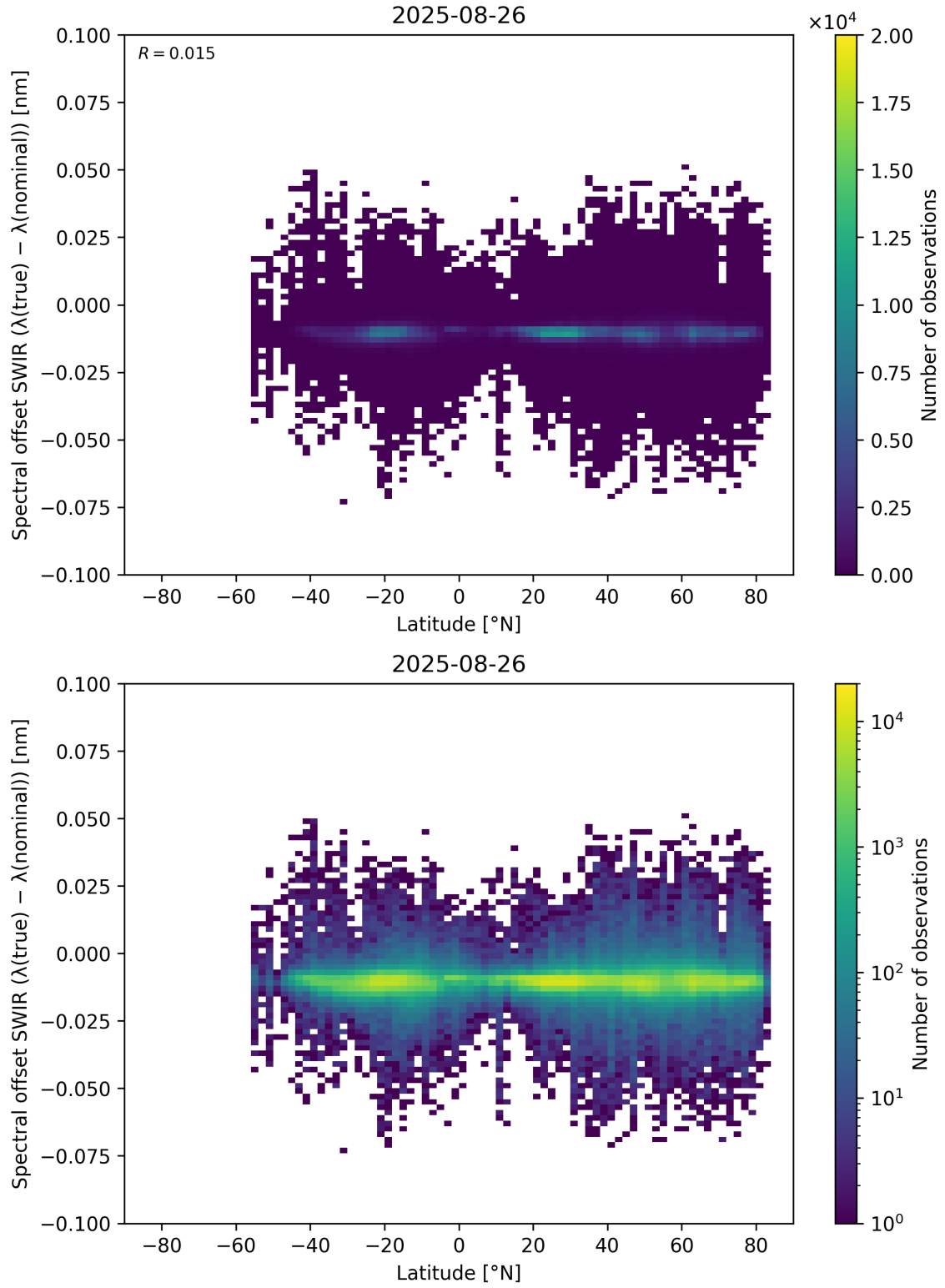
Figure 62: Scatter density plot of “Latitude” against “Spectral offset SWIR ( \lambda_{\text{true}} - \lambda_{\text{nominal}} )” for 2025-08-25 to 2025-08-27.
