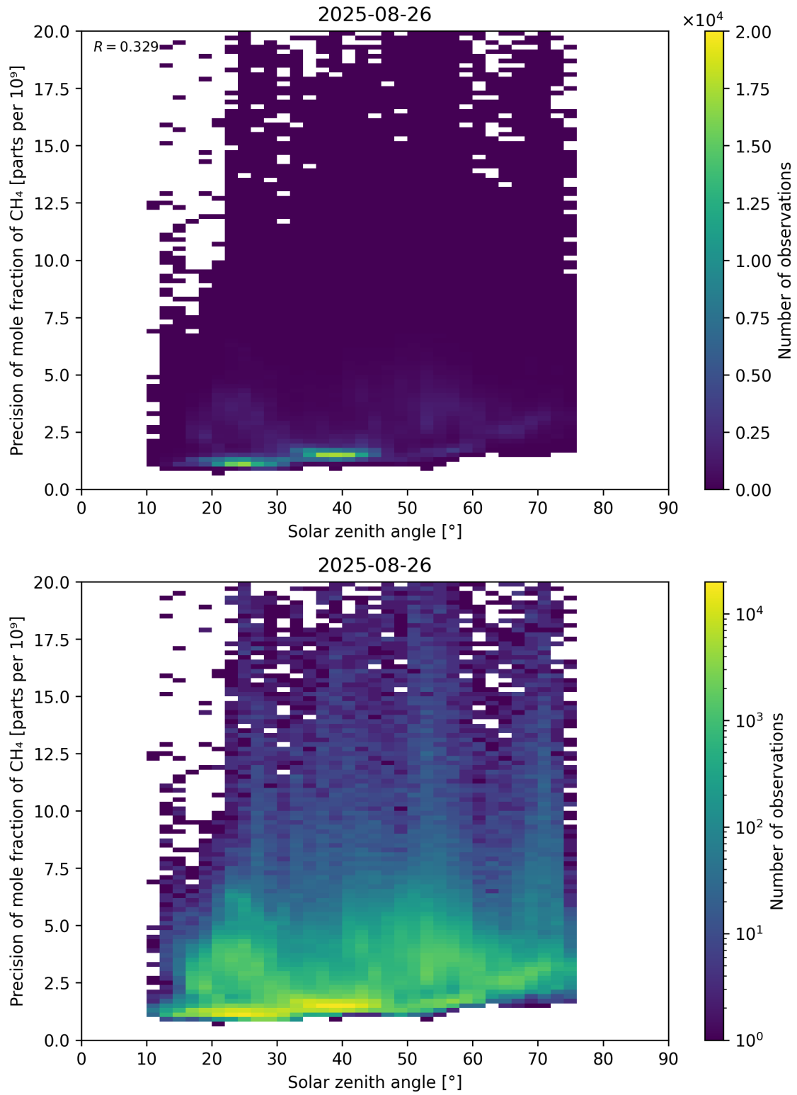
Figure 101: Scatter density plot of “Solar zenith angle” against “Precision of mole fraction of \text{CH}_4 ” for 2025-08-25 to 2025-08-27.
