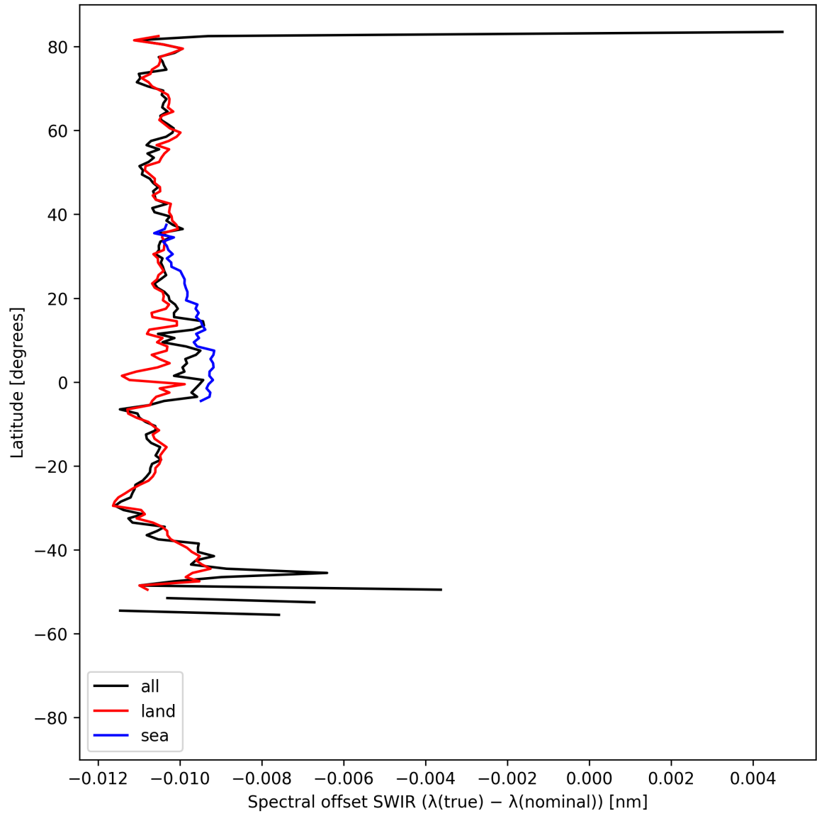
Figure 16: Zonal average of “Spectral offset SWIR ( \lambda_{\text{true}} - \lambda_{\text{nominal}} )” for 2025-08-25 to 2025-08-27.
