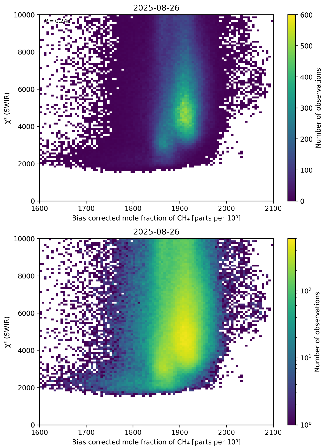
Figure 64: Scatter density plot of “Bias corrected mole fraction of \text{CH}_4 ” against “ \chi^2 (SWIR)” for 2025-08-25 to 2025-08-27.
