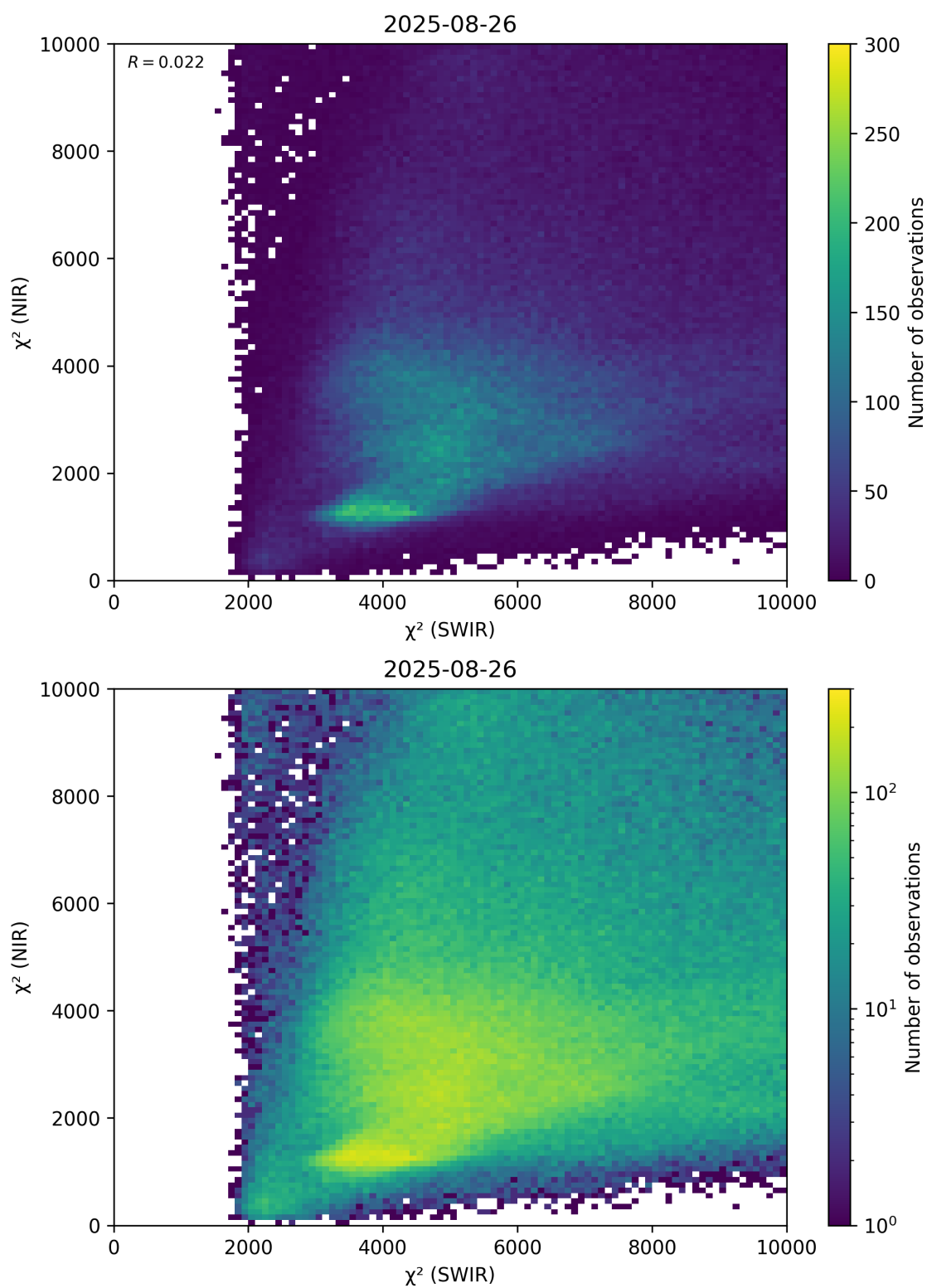
Figure 47: Scatter density plot of “ \chi^2 (SWIR)” against “ \chi^2 (NIR)” for 2025-08-25 to 2025-08-27.
