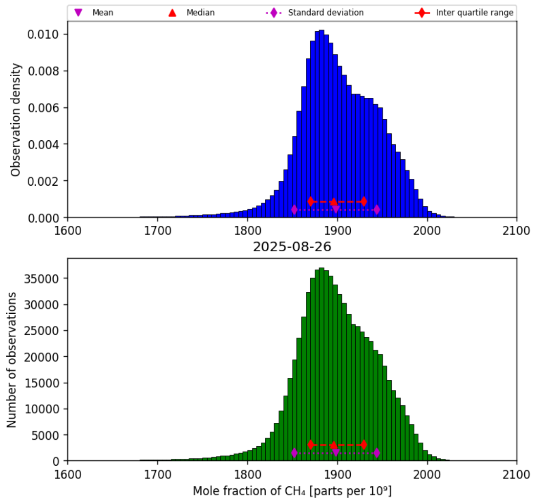
Figure 23: Histogram of “Mole fraction of CH 4 ” for 2025-08-25 to 2025-08-27
