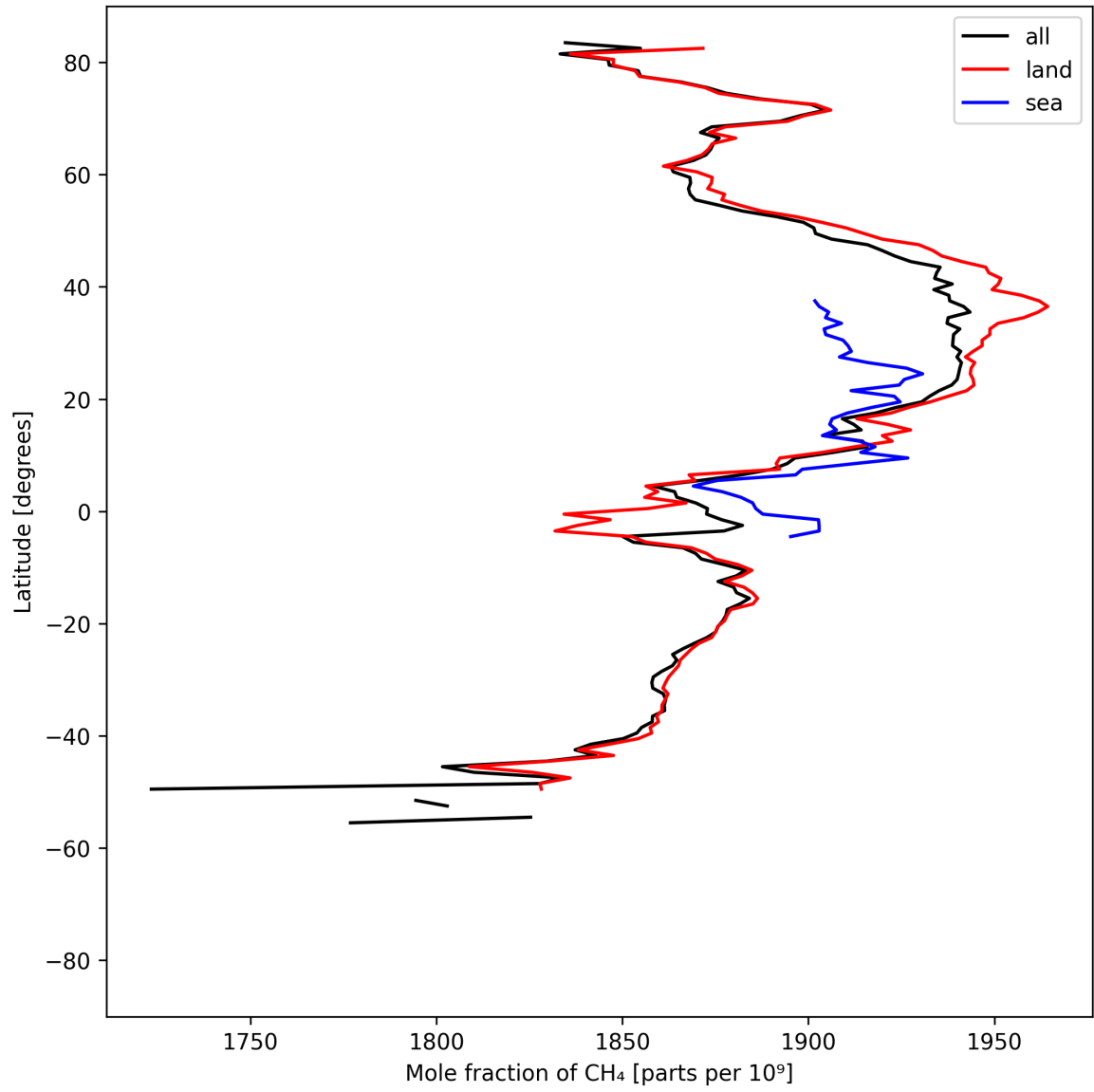
Figure 12: Zonal average of “Mole fraction of \text{CH}_4 ” for 2025-08-25 to 2025-08-27.
