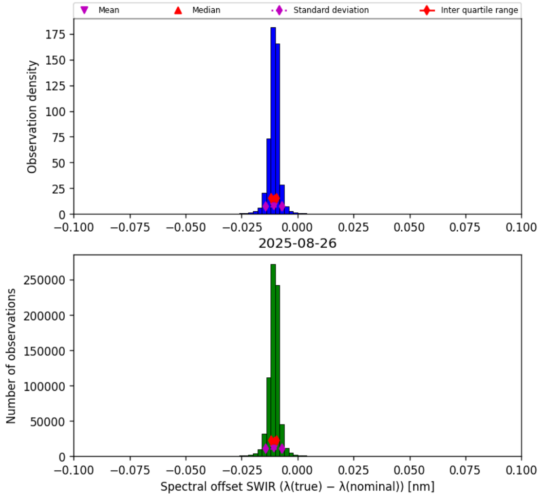
Figure 27: Histogram of “Spectral offset SWIR ( \lambda_{\text{true}} - \lambda_{\text{nominal}} )” for 2025-08-25 to 2025-08-27
