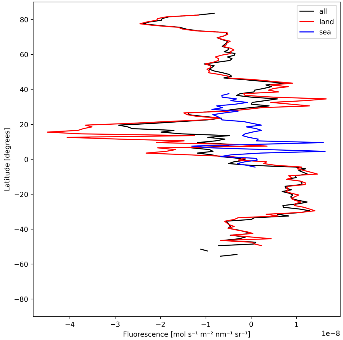
Figure 21: Zonal average of “Fluorescence” for 2025-08-25 to 2025-08-27.
