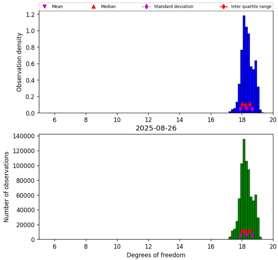
Figure 30: Histogram of “Degrees of freedom” for 2025-08-25 to 2025-08-27
