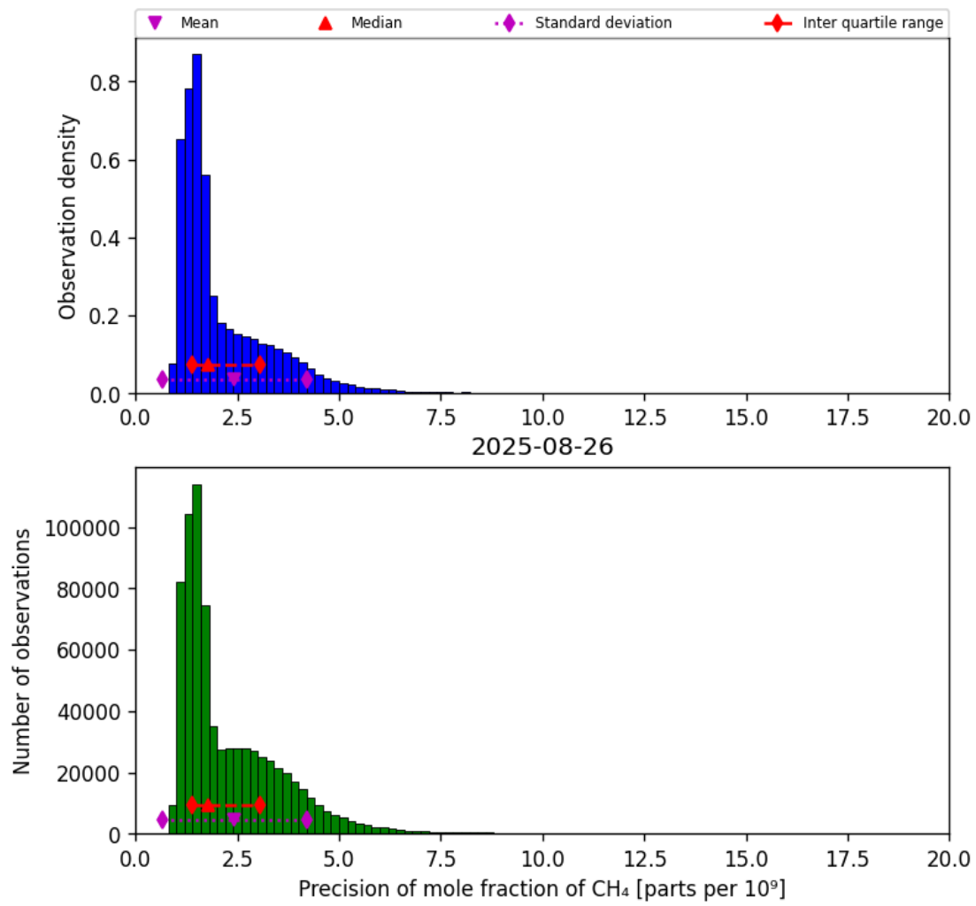
Figure 24: Histogram of “Precision of mole fraction of CH 4 ” for 2025-08-25 to 2025-08-27
