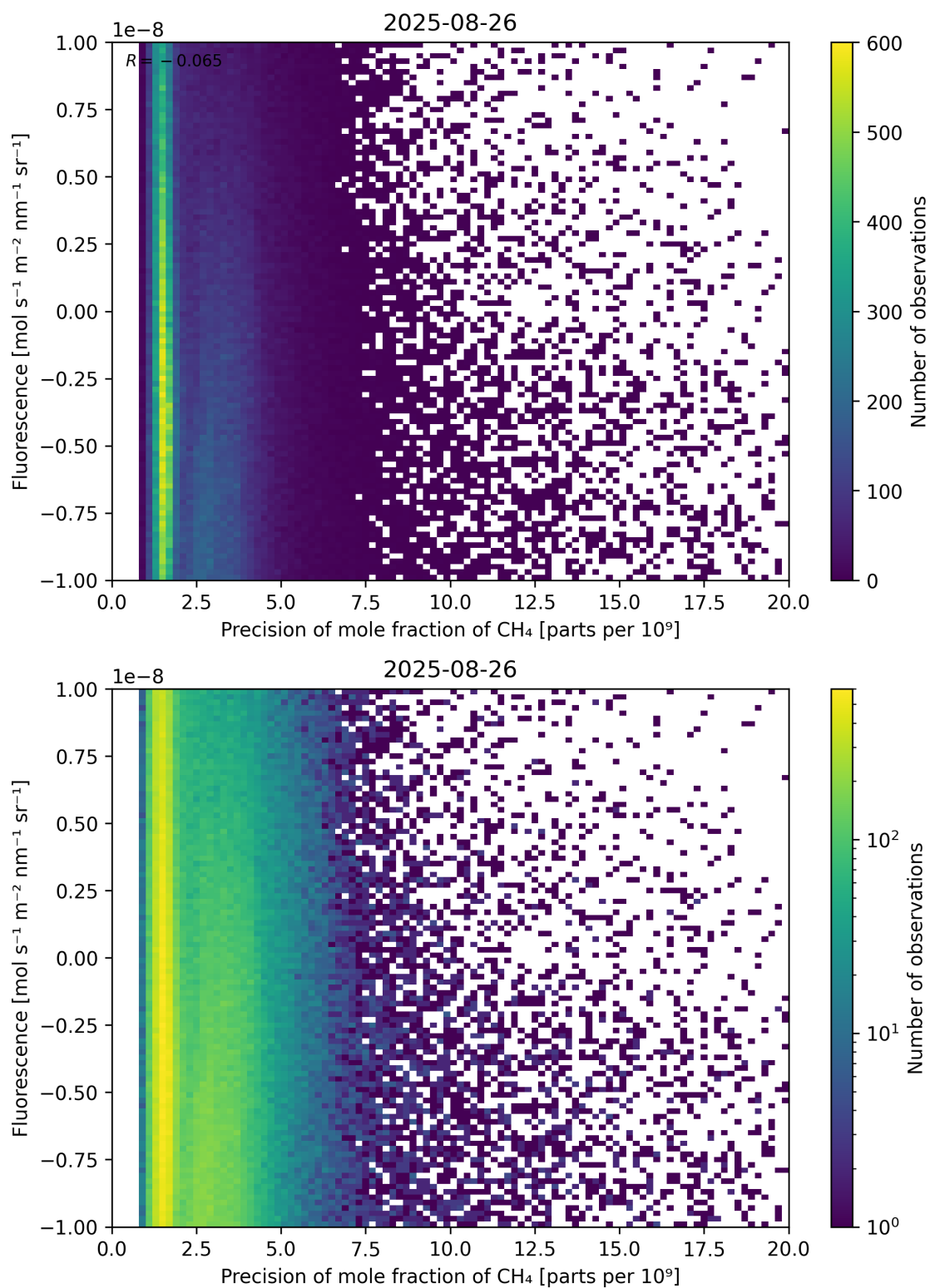
Figure 81: Scatter density plot of “Precision of mole fraction of \text{CH}_4 ” against “Fluorescence” for 2025-08-25 to 2025-08-27.
