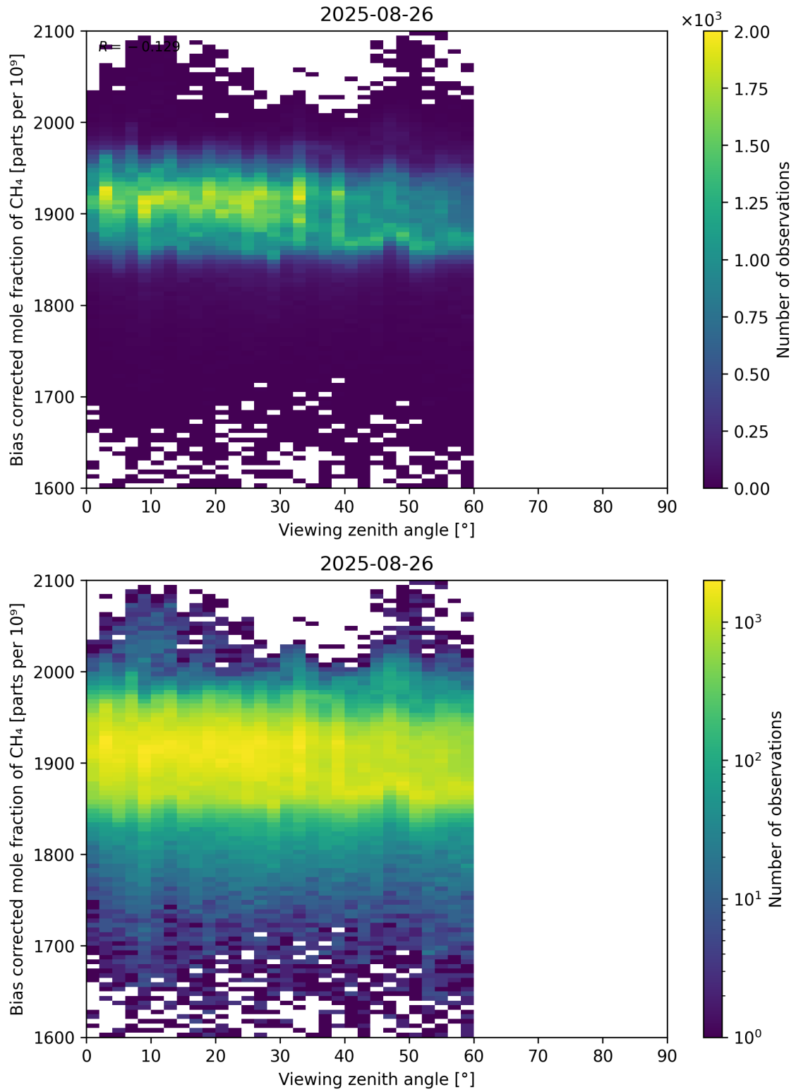
Figure 111: Scatter density plot of “Viewing zenith angle” against “Bias corrected mole fraction of CH 4 ” for 2025-08-25 to 2025-08-27.
