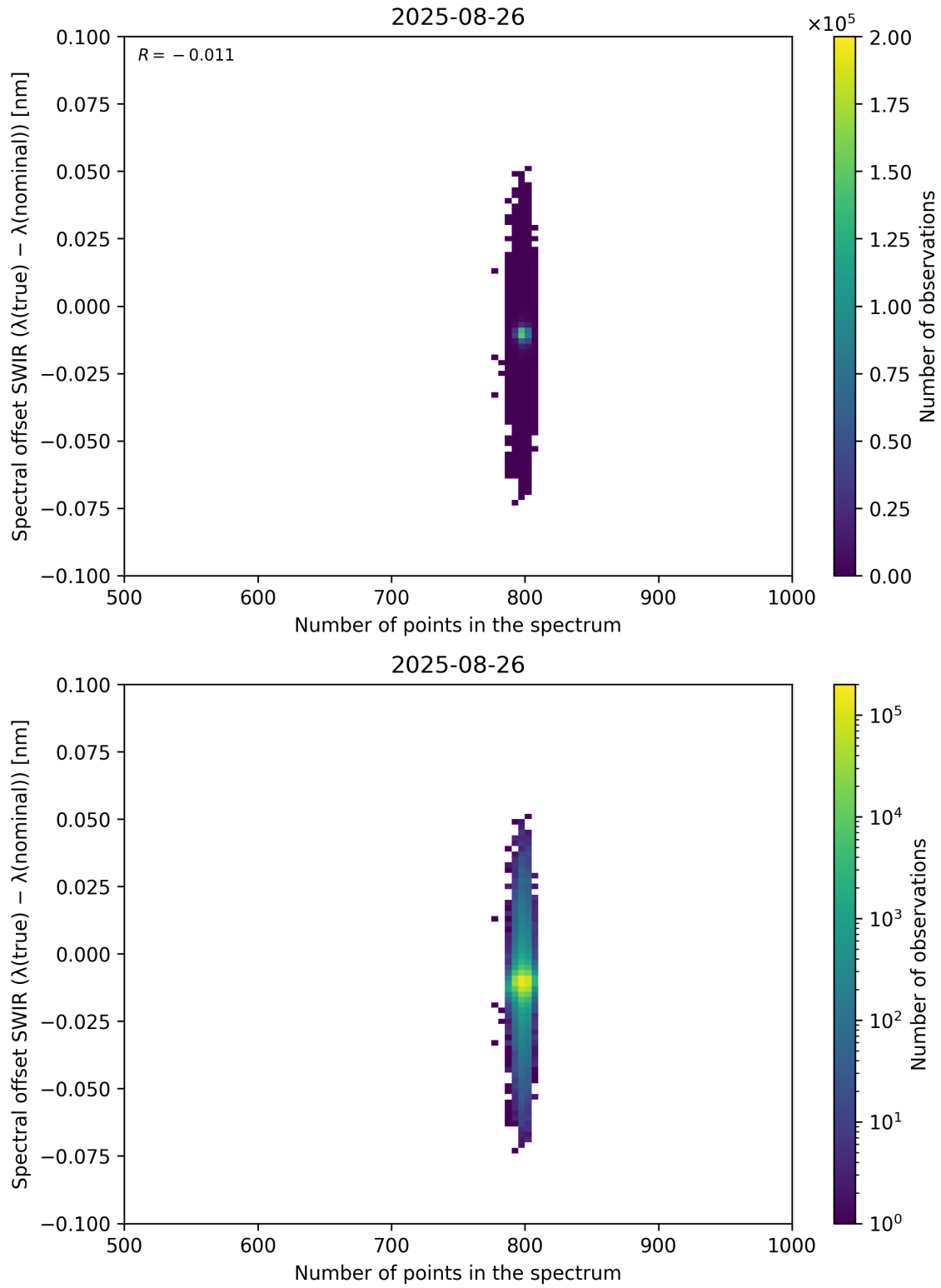
Figure 93: Scatter density plot of “Number of points in the spectrum” against “Spectral offset SWIR ( \lambda_{\text{true}} - \lambda_{\text{nominal}} )” for 2025-08-25 to 2025-08-27.
