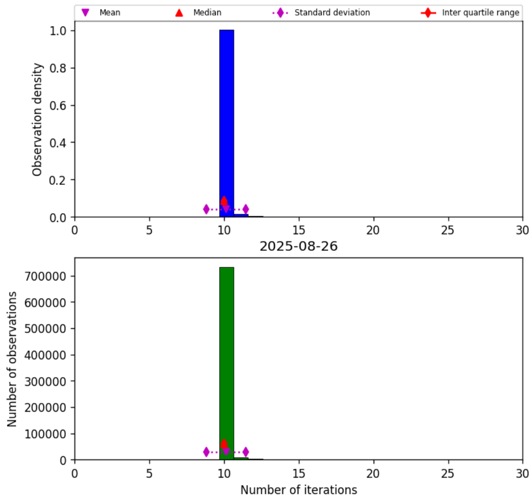
Figure 31: Histogram of “Number of iterations” for 2025-08-25 to 2025-08-27
