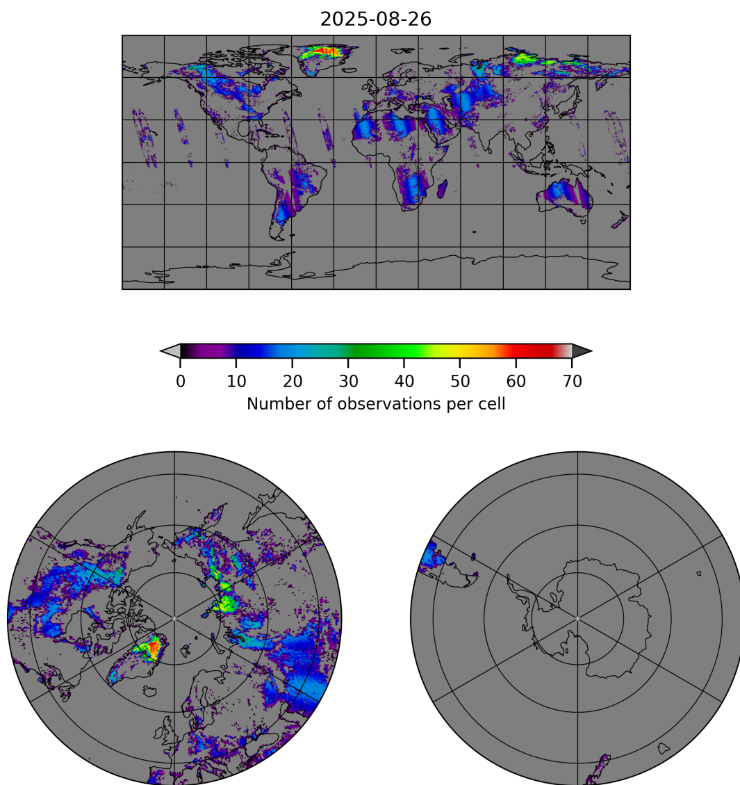
Figure 10: Map of the number of observations for 2025-08-25 to 2025-08-27
