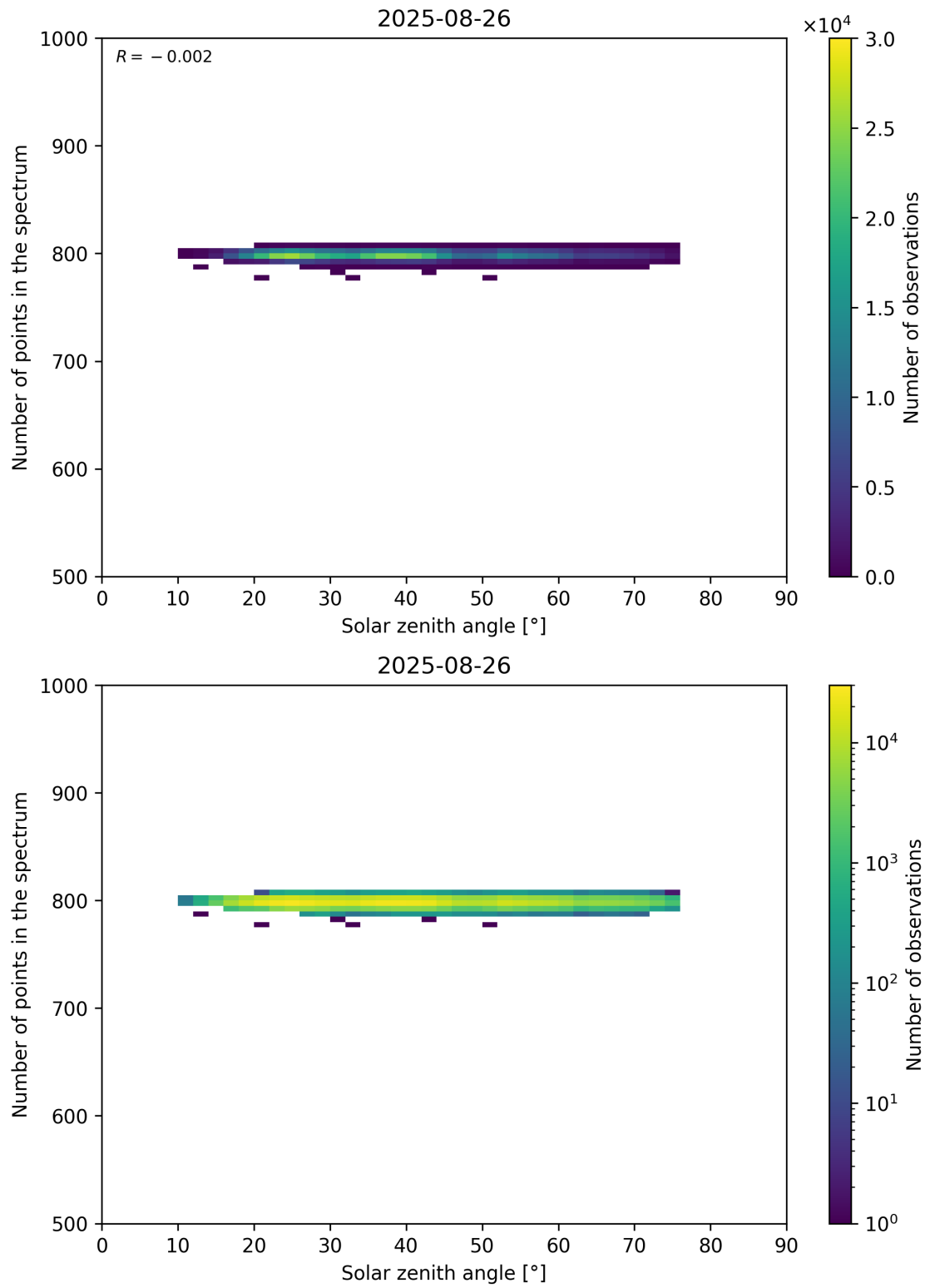
Figure 103: Scatter density plot of “Solar zenith angle” against “Number of points in the spectrum” for 2025-08-25 to 2025-08-27.
