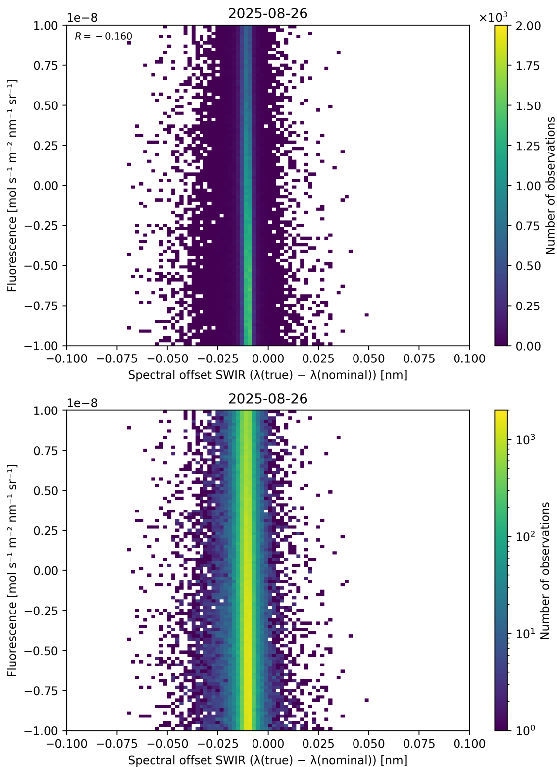
Figure 120: Scatter density plot of “Spectral offset SWIR ( \lambda_{\text{true}} - \lambda_{\text{nominal}} )” against “Fluorescence” for 2025-08-25 to 2025-08-27.
