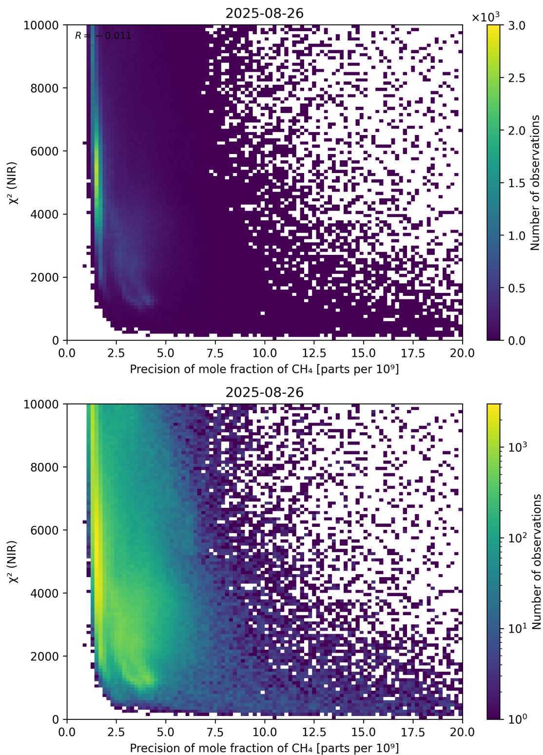
Figure 78: Scatter density plot of “Precision of mole fraction of CH 4 ” against “ \chi^2 (NIR)” for 2025-08-25 to 2025-08-27.
