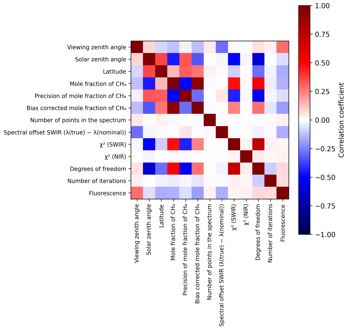
Figure 2: Map of correlation matrix for 2025-08-25 to 2025-08-27.
