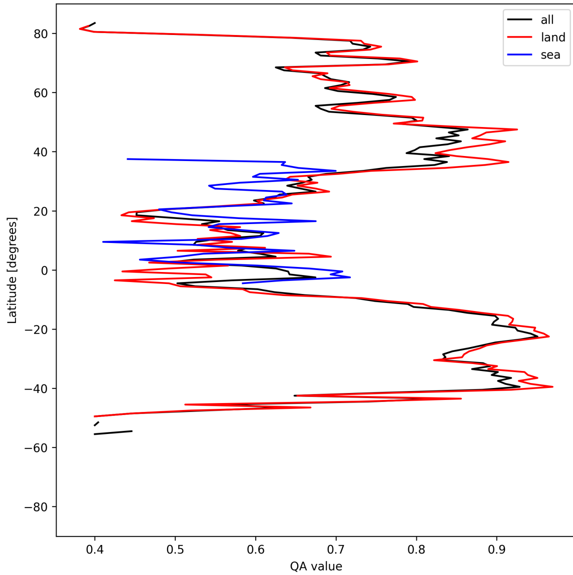
Figure 11: Zonal average of “QA value” for 2025-08-25 to 2025-08-27.
