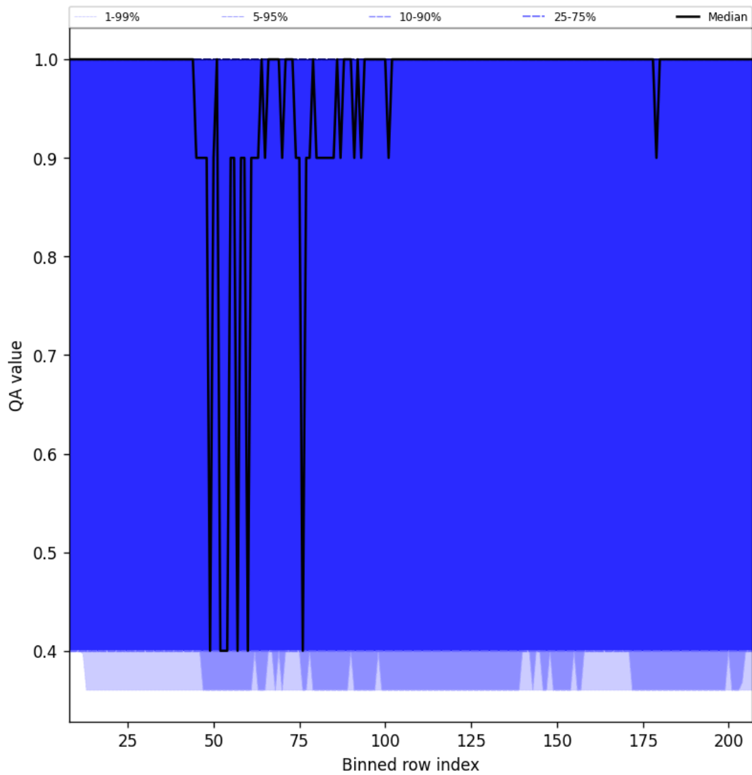
Figure 33: Along track statistics of “QA value” for 2025-08-25 to 2025-08-27
