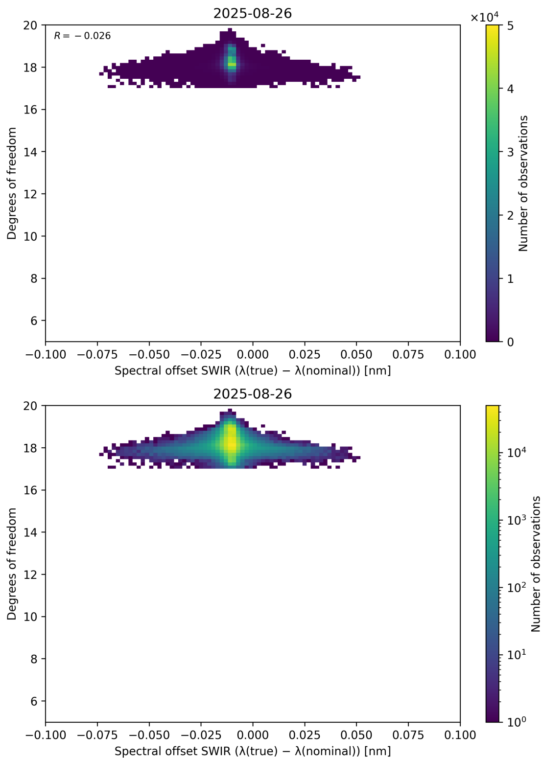
Figure 119: Scatter density plot of “Spectral offset SWIR ( \lambda_{\text{true}} - \lambda_{\text{nominal}} )” against “Degrees of freedom” for 2025-08-25 to 2025-08-27.
