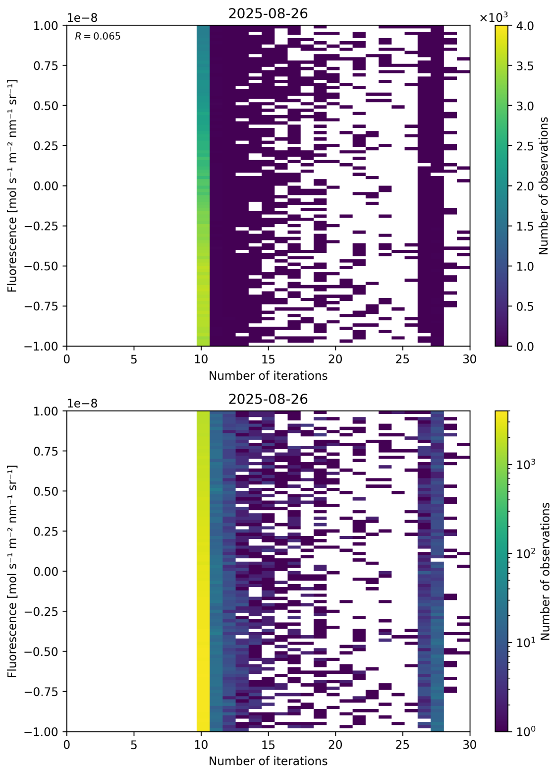
Figure 87: Scatter density plot of “Number of iterations” against “Fluorescence” for 2025-08-25 to 2025-08-27.
