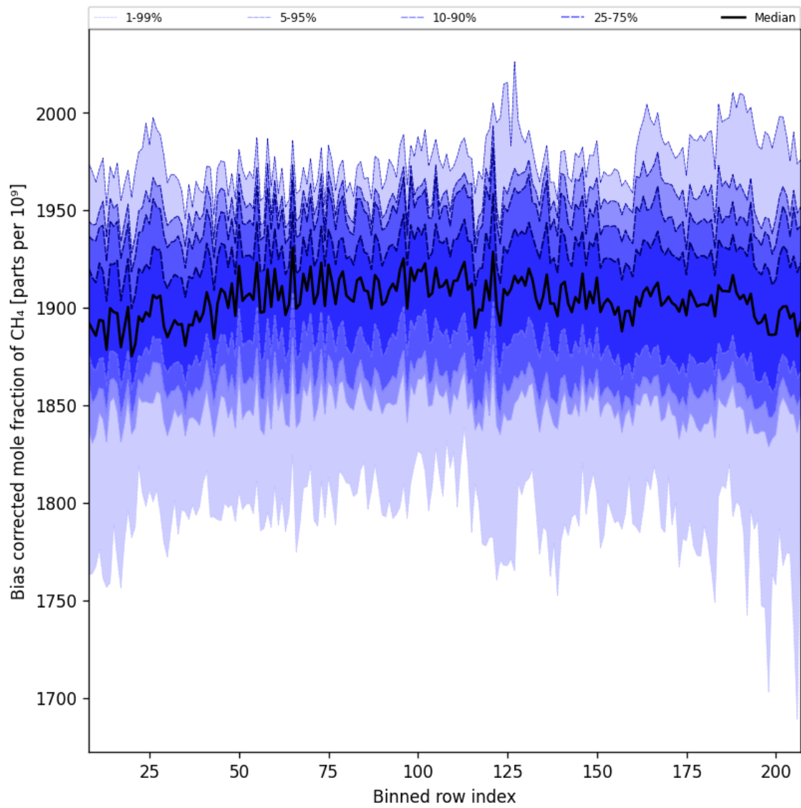
Figure 36: Along track statistics of “Bias corrected mole fraction of \text{CH}_4 ” for 2025-08-25 to 2025-08-27
