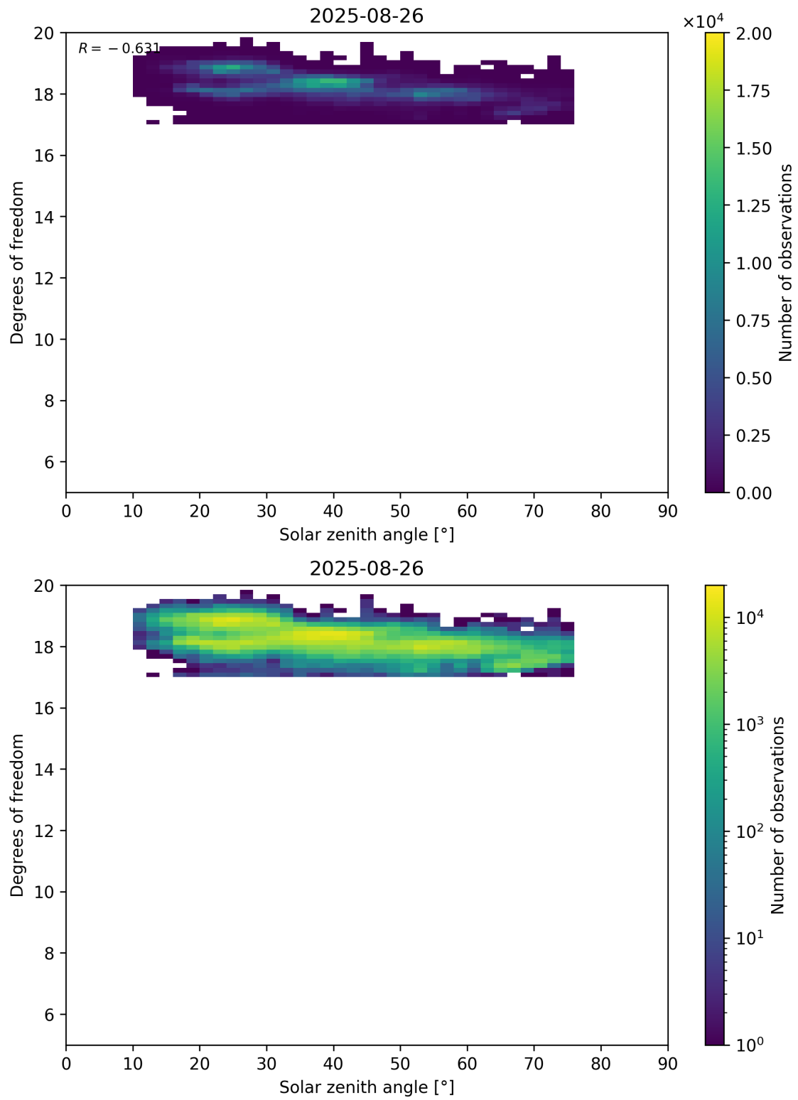
Figure 96: Scatter density plot of “Solar zenith angle” against “Degrees of freedom” for 2025-08-25 to 2025-08-27.
