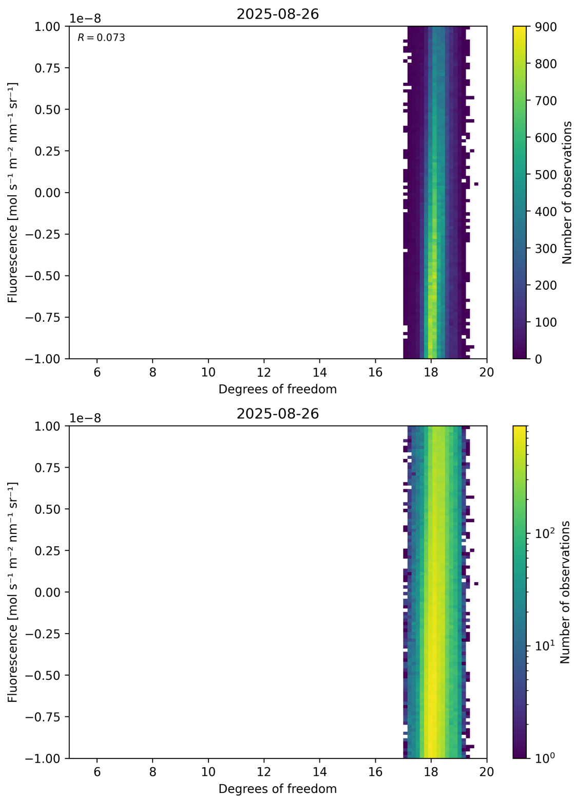
Figure 51: Scatter density plot of “Degrees of freedom” against “Fluorescence” for 2025-08-25 to 2025-08-27.
