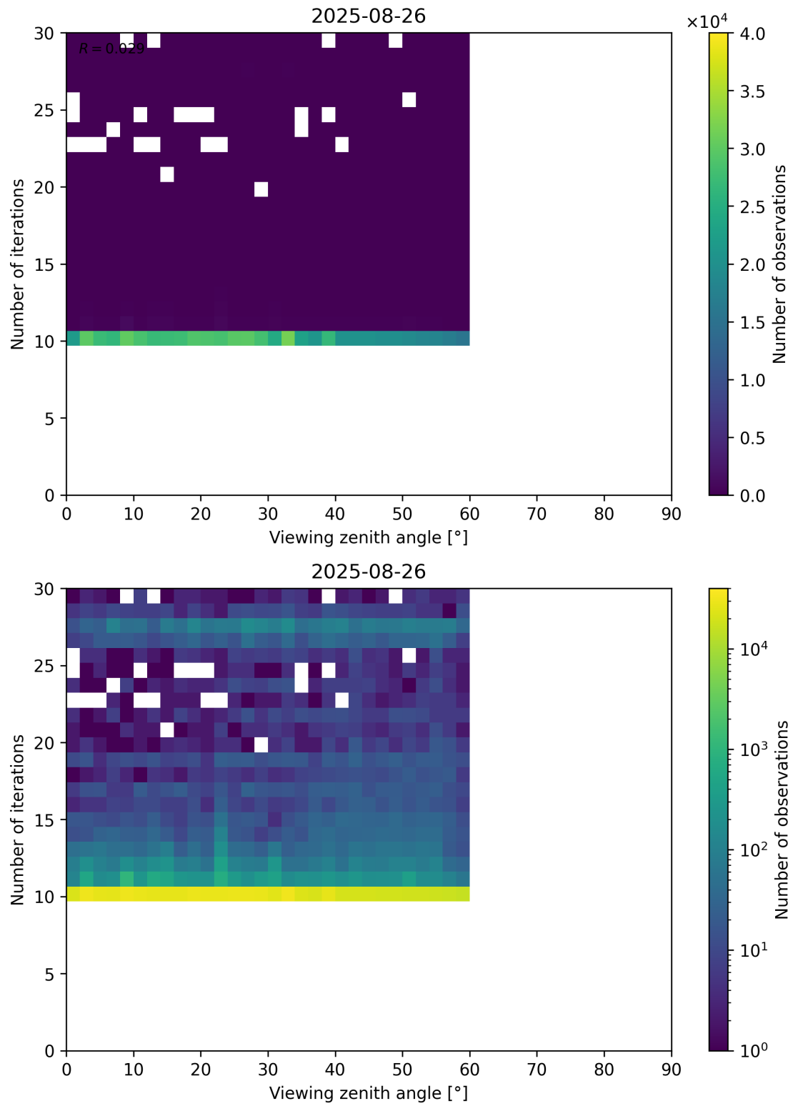
Figure 113: Scatter density plot of “Viewing zenith angle” against “Number of iterations” for 2025-08-25 to 2025-08-27.
