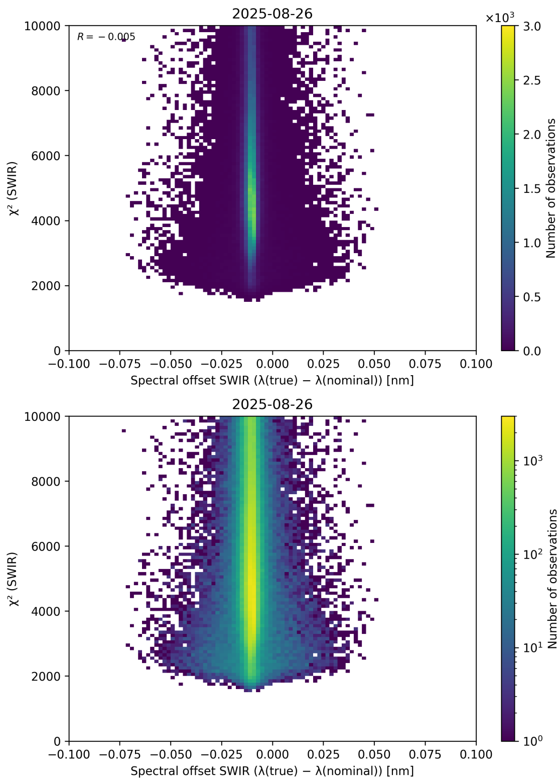
Figure 118: Scatter density plot of “Spectral offset SWIR ( \lambda_{\text{true}} - \lambda_{\text{nominal}} )” against “ \chi^2 (SWIR)” for 2025-08-25 to 2025-08-27.
