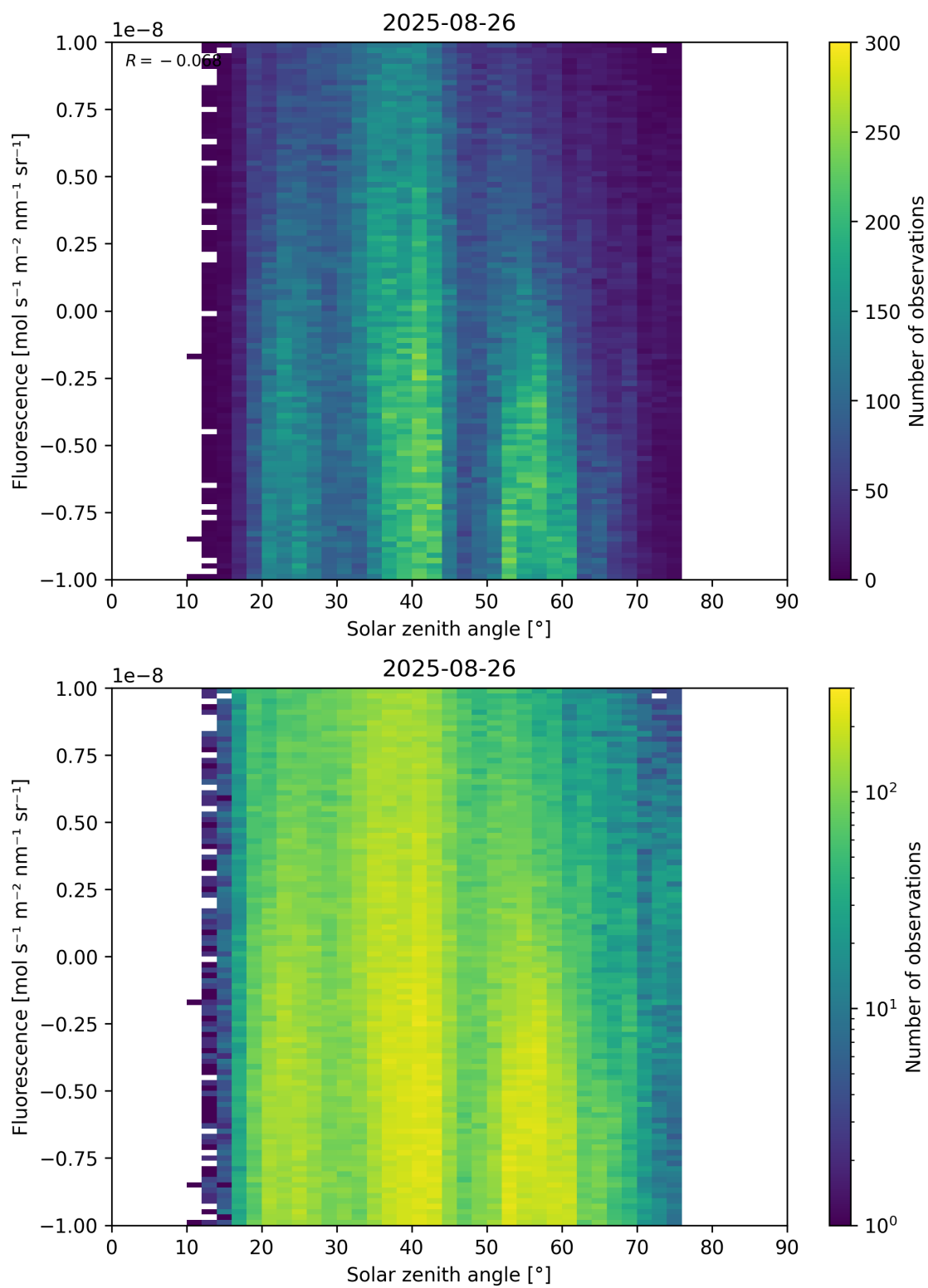
Figure 97: Scatter density plot of “Solar zenith angle” against “Fluorescence” for 2025-08-25 to 2025-08-27.
