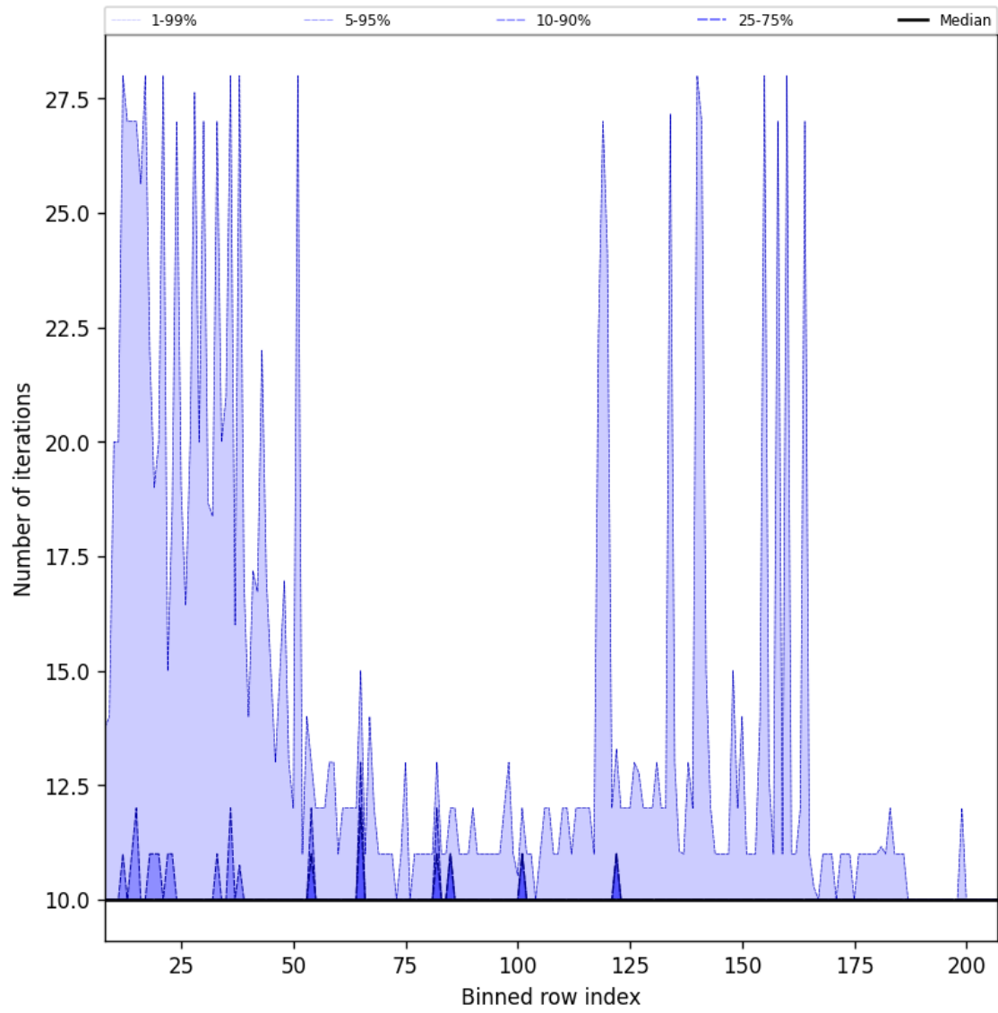
Figure 42: Along track statistics of “Number of iterations” for 2025-08-25 to 2025-08-27
