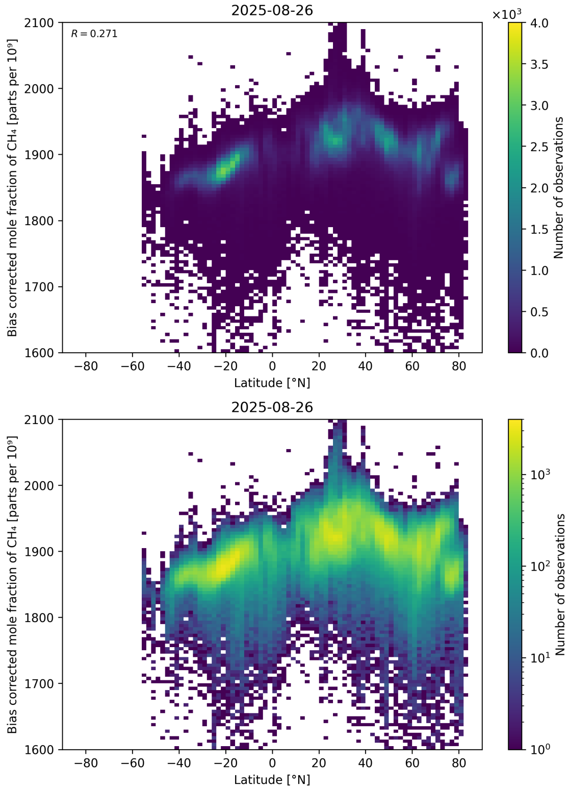
Figure 58: Scatter density plot of “Latitude” against “Bias corrected mole fraction of CH 4 ” for 2025-08-25 to 2025-08-27.
