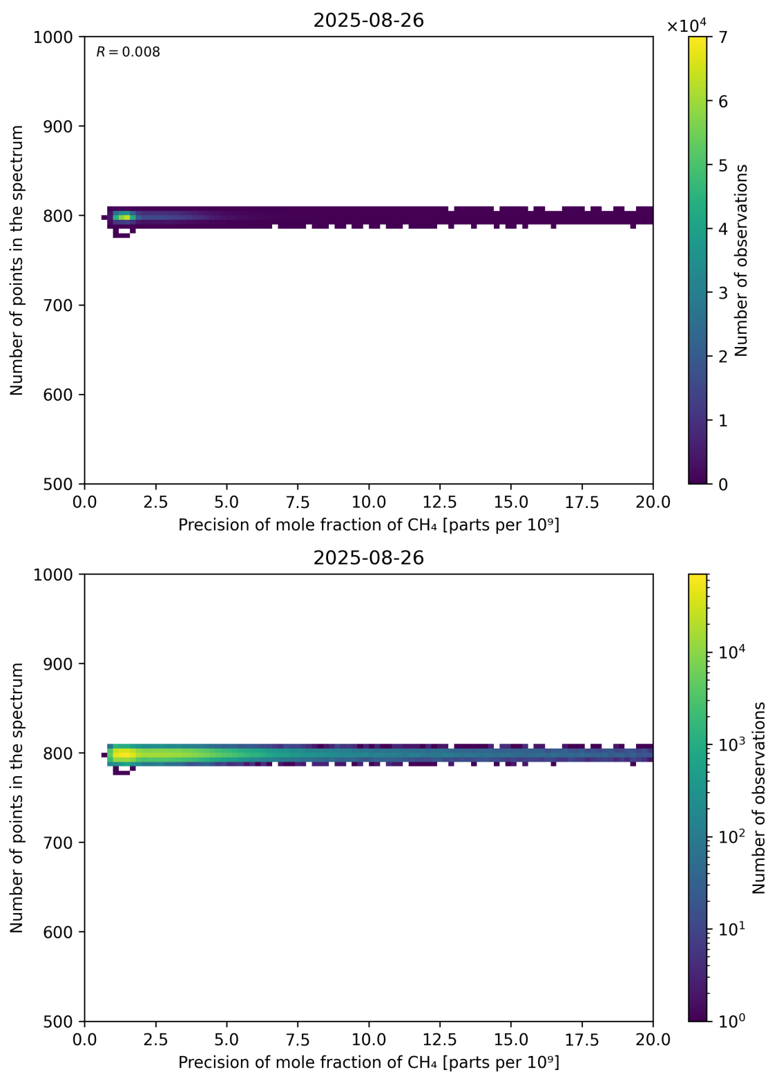
Figure 84: Scatter density plot of “Precision of mole fraction of CH 4 ” against “Number of points in the spectrum” for 2025-08-25 to 2025-08-27.
