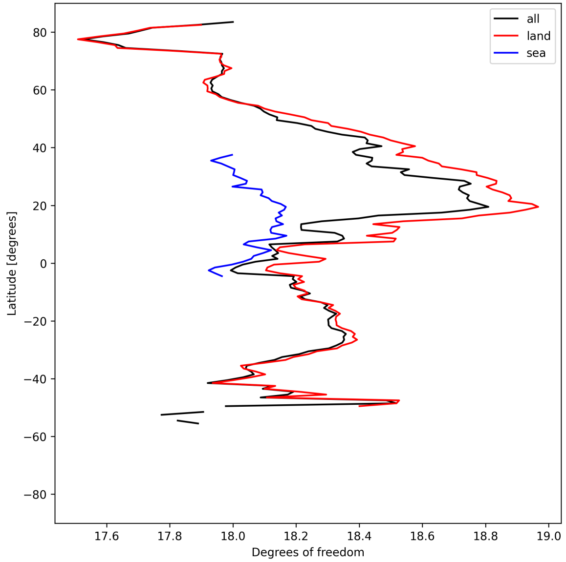
Figure 19: Zonal average of “Degrees of freedom” for 2025-08-25 to 2025-08-27.
