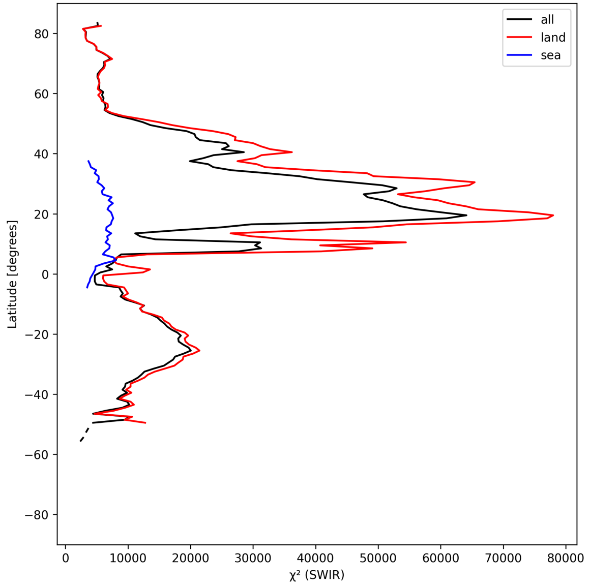
Figure 17: Zonal average of “ \chi^2 (SWIR)” for 2025-08-25 to 2025-08-27.
