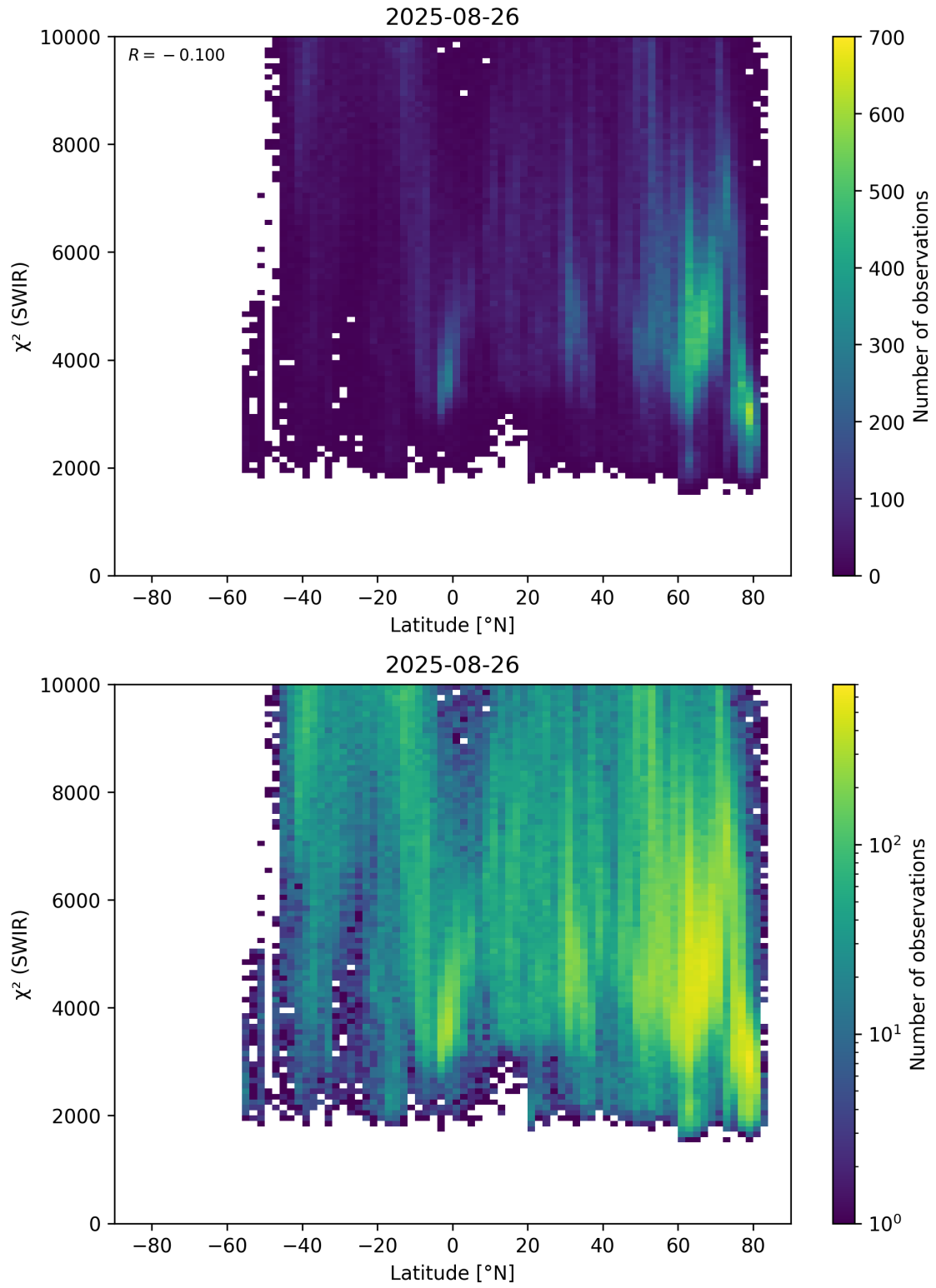
Figure 54: Scatter density plot of “Latitude” against “ \chi^2 (SWIR)” for 2025-08-25 to 2025-08-27.
