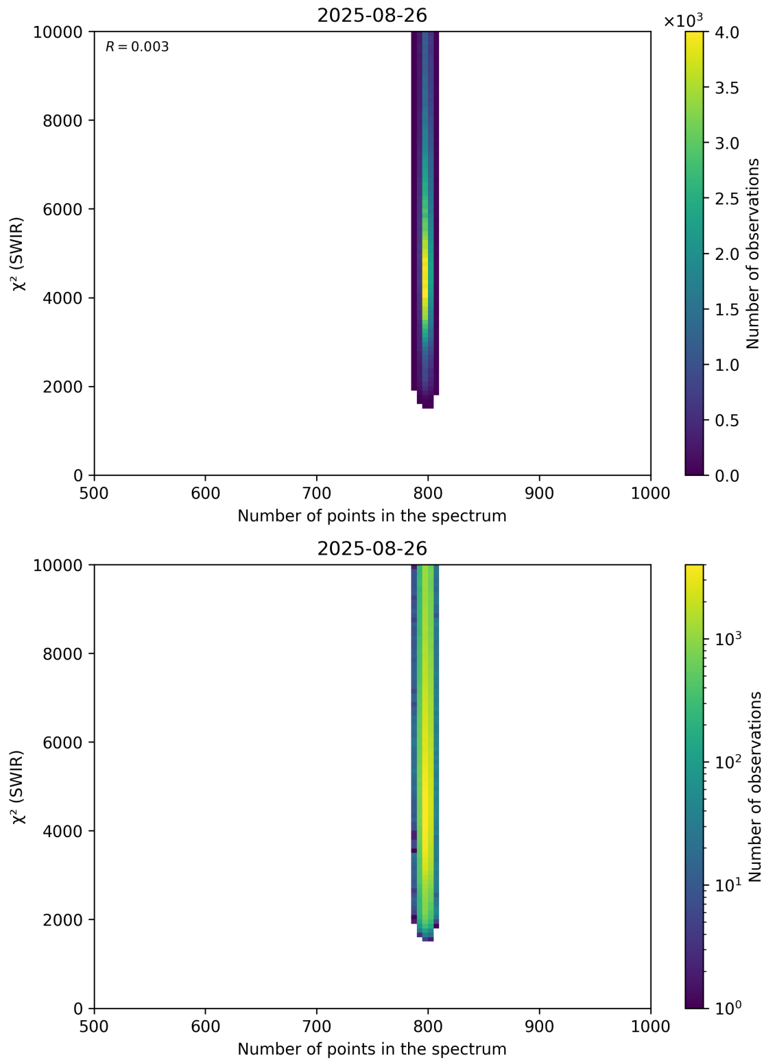
Figure 89: Scatter density plot of “Number of points in the spectrum” against “ \chi^2 (SWIR)” for 2025-08-25 to 2025-08-27.
