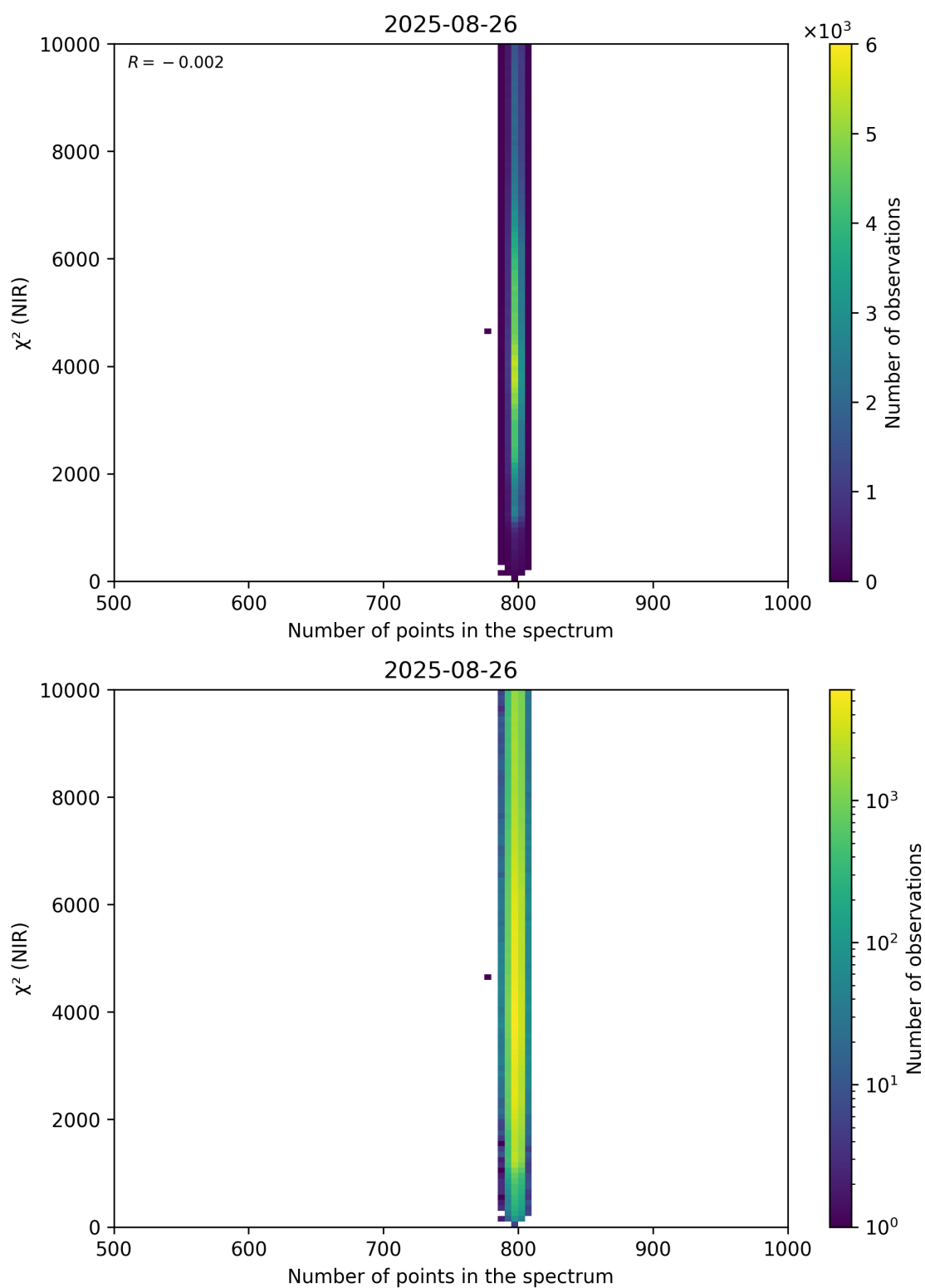
Figure 88: Scatter density plot of “Number of points in the spectrum” against “ \chi^2 (NIR)” for 2025-08-25 to 2025-08-27.
