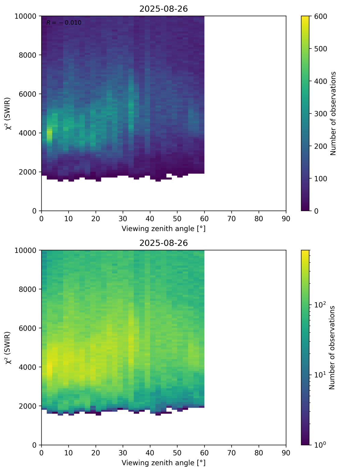
Figure 106: Scatter density plot of “Viewing zenith angle” against “ \chi^2 (SWIR)” for 2025-08-25 to 2025-08-27.
