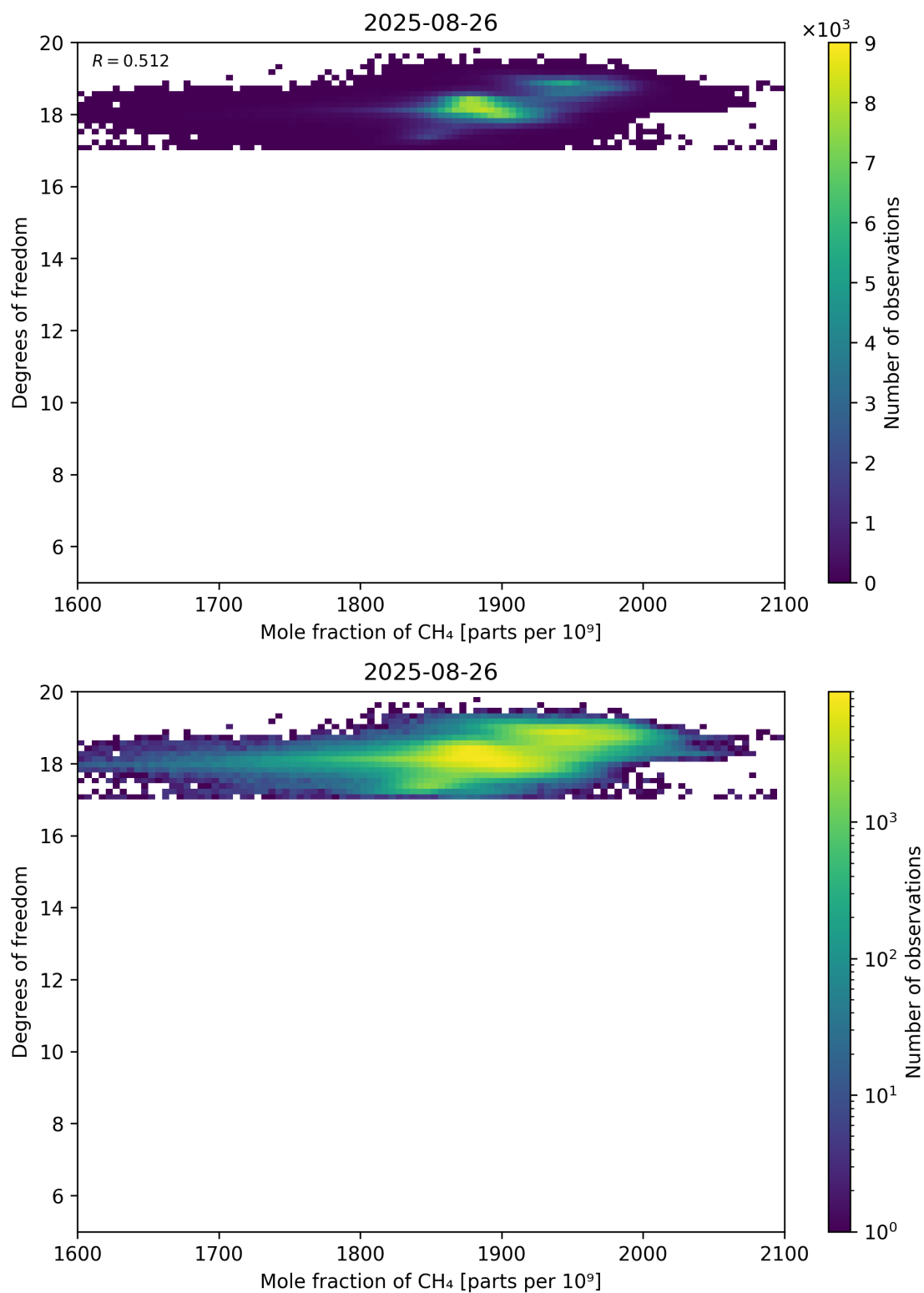
Figure 72: Scatter density plot of “Mole fraction of CH 4 ” against “Degrees of freedom” for 2025-08-25 to 2025-08-27.
