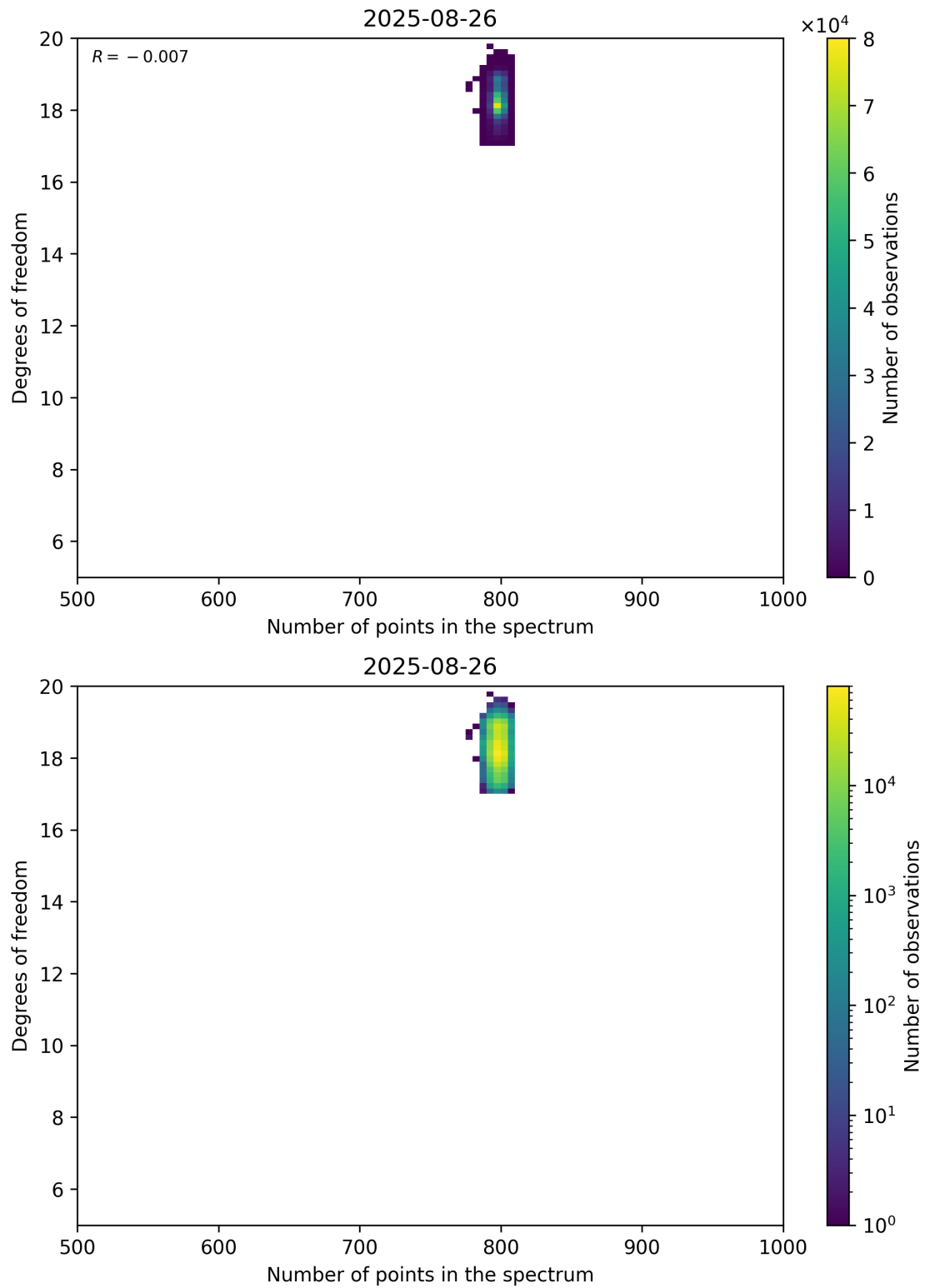
Figure 90: Scatter density plot of “Number of points in the spectrum” against “Degrees of freedom” for 2025-08-25 to 2025-08-27.
