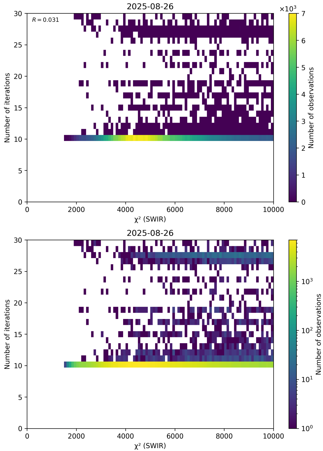
Figure 50: Scatter density plot of “ \chi^2 (SWIR)” against “Number of iterations” for 2025-08-25 to 2025-08-27.
