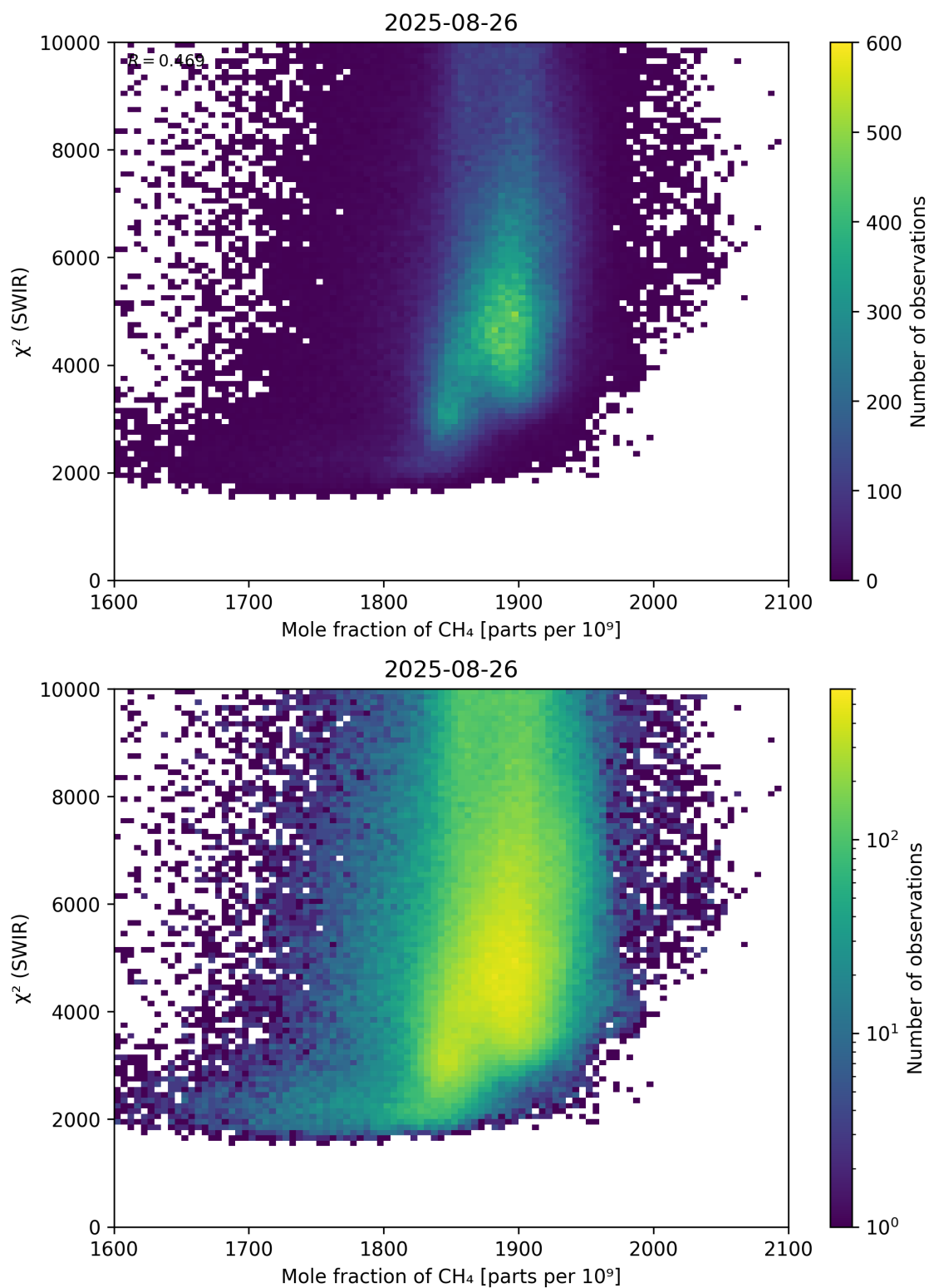
Figure 71: Scatter density plot of “Mole fraction of \text{CH}_4 ” against “ \chi^2 (SWIR)” for 2025-08-25 to 2025-08-27.
