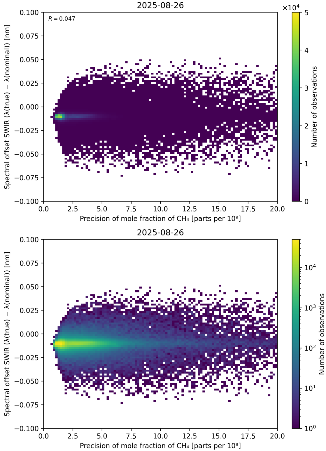
Figure 85: Scatter density plot of “Precision of mole fraction of CH 4 ” against “Spectral offset SWIR ( \lambda_{\text{true}} - \lambda_{\text{nominal}} )” for 2025-08-25 to 2025-08-27.
