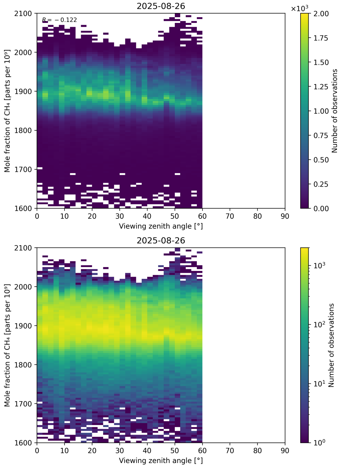
Figure 110: Scatter density plot of “Viewing zenith angle” against “Mole fraction of CH 4 ” for 2025-08-25 to 2025-08-27.
