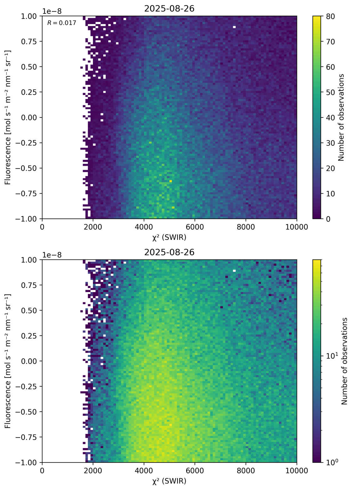
Figure 49: Scatter density plot of “ \chi^2 (SWIR)” against “Fluorescence” for 2025-08-25 to 2025-08-27.
