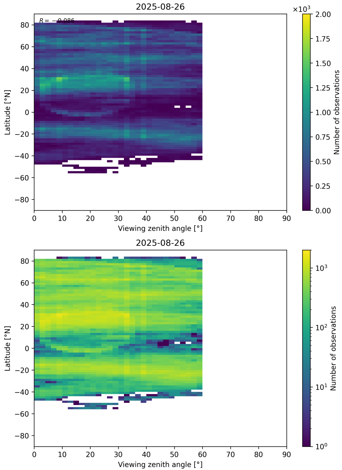
Figure 109: Scatter density plot of “Viewing zenith angle” against “Latitude” for 2025-08-25 to 2025-08-27.
