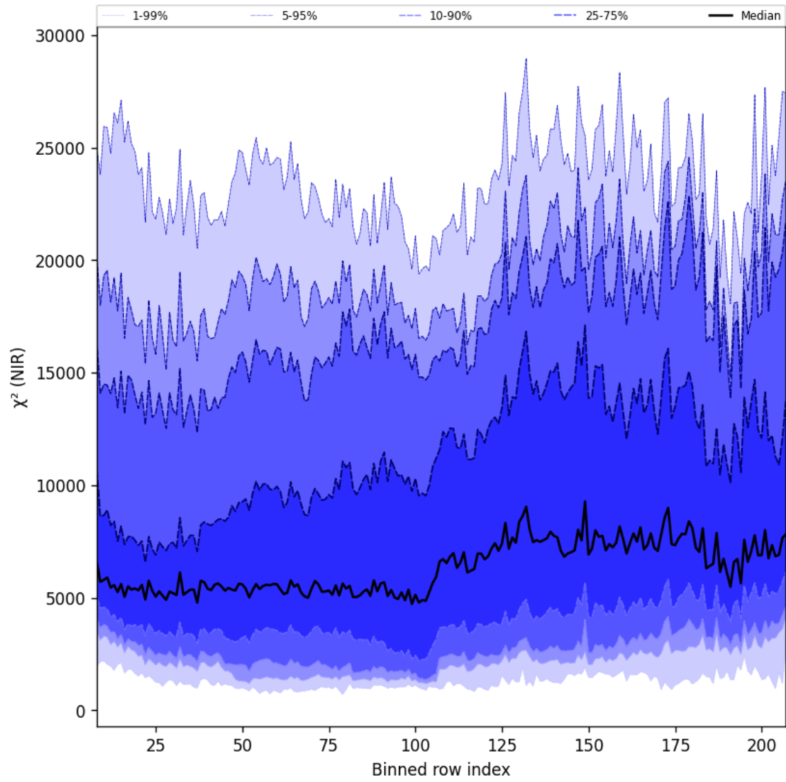
Figure 40: Along track statistics of “ \chi^2 (NIR)” for 2025-08-25 to 2025-08-27
