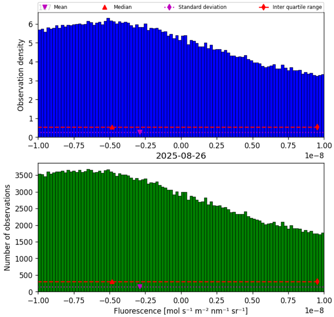
Figure 32: Histogram of “Fluorescence” for 2025-08-25 to 2025-08-27
