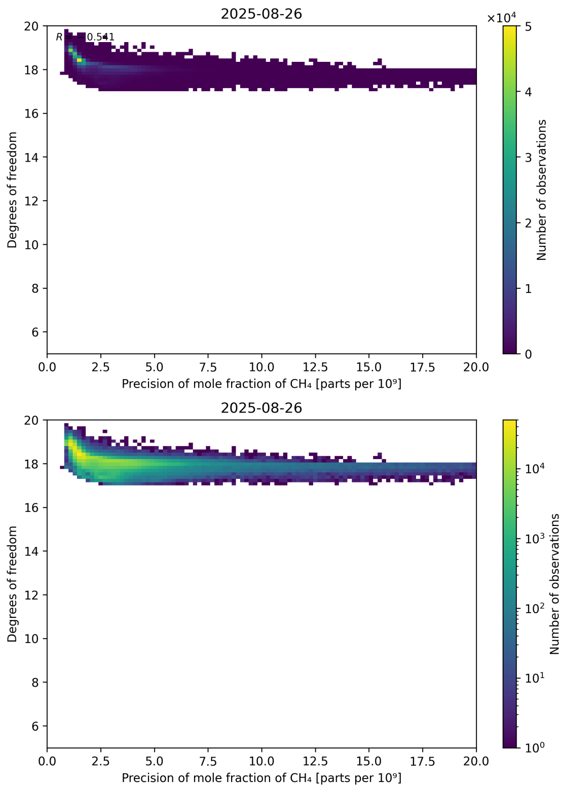
Figure 80: Scatter density plot of “Precision of mole fraction of CH 4 ” against “Degrees of freedom” for 2025-08-25 to 2025-08-27.
