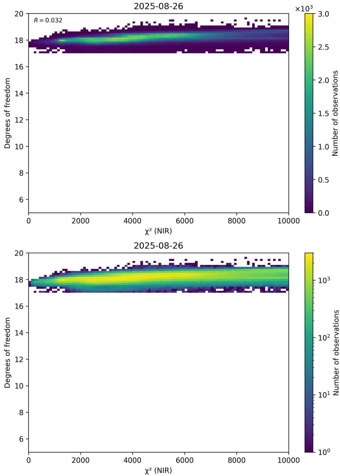
Figure 44: Scatter density plot of “ \chi^2 (NIR)” against “Degrees of freedom” for 2025-08-25 to 2025-08-27.
