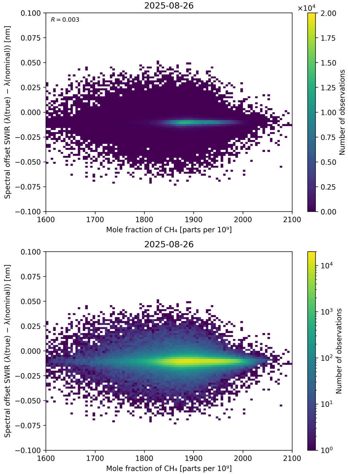
Figure 86: Scatter density plot of “Mole fraction of \text{CH}_4 ” against “Spectral offset SWIR ( \lambda_{\text{true}} - \lambda_{\text{nominal}} )” for 2025-08-25 to 2025-08-27.
