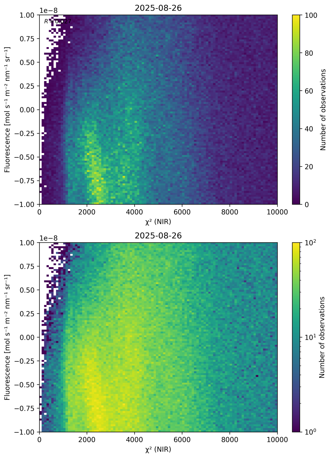
Figure 45: Scatter density plot of “ \chi^2 (NIR)” against “Fluorescence” for 2025-08-25 to 2025-08-27.
