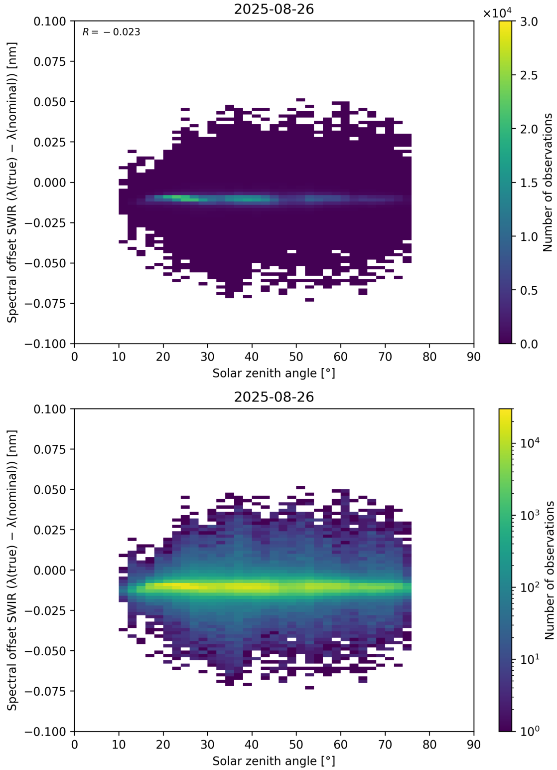
Figure 104: Scatter density plot of “Solar zenith angle” against “Spectral offset SWIR ( \lambda_{\text{true}} - \lambda_{\text{nominal}} )” for 2025-08-25 to 2025-08-27.
