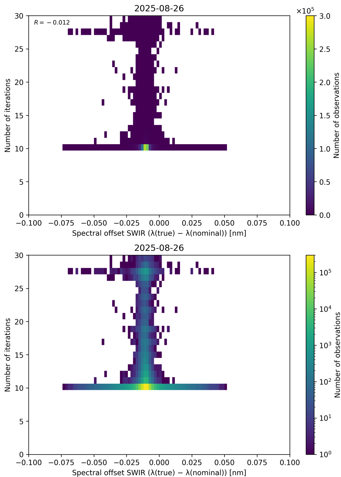
Figure 121: Scatter density plot of “Spectral offset SWIR ( \lambda_{\text{true}} - \lambda_{\text{nominal}} )” against “Number of iterations” for 2025-08-25 to 2025-08-27.
