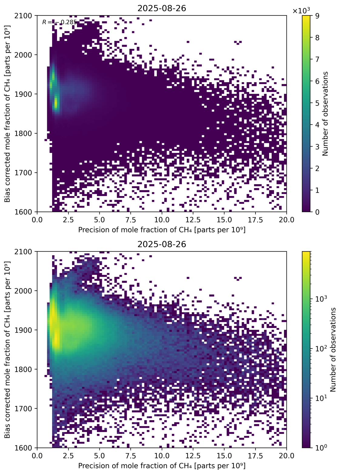
Figure 82: Scatter density plot of “Precision of mole fraction of CH 4 ” against “Bias corrected mole fraction of CH 4 ” for 2025-08-25 to 2025-08-27.
