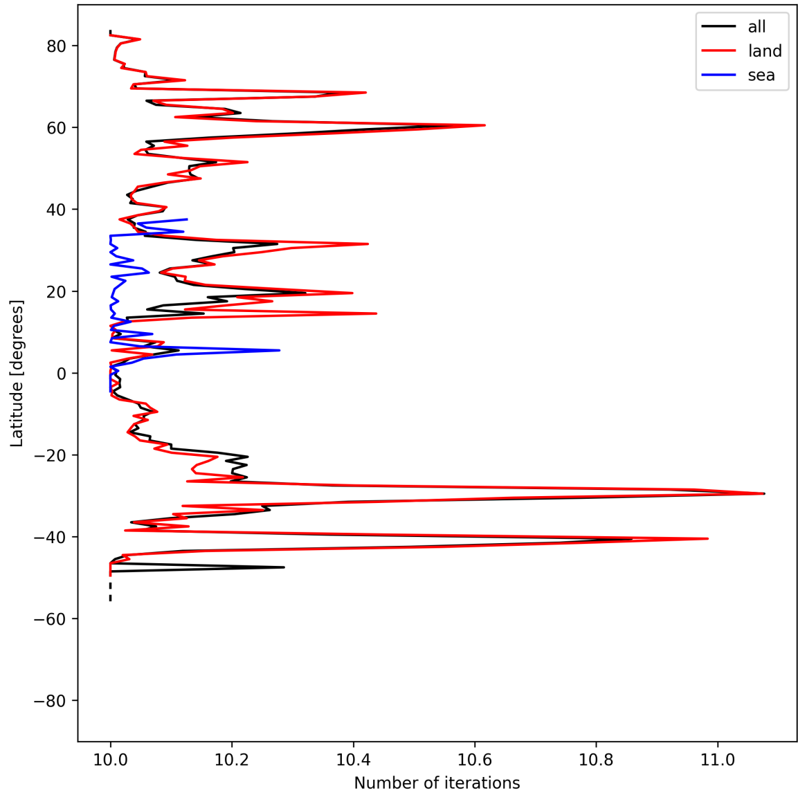
Figure 20: Zonal average of “Number of iterations” for 2025-08-25 to 2025-08-27.
