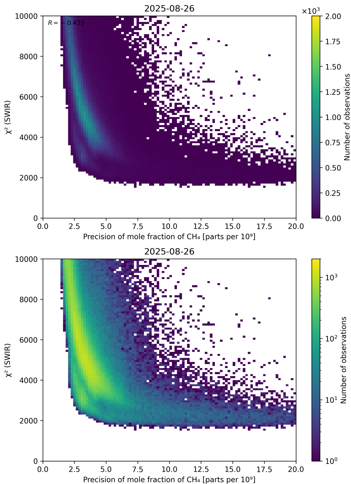
Figure 79: Scatter density plot of “Precision of mole fraction of \text{CH}_4 ” against “ \chi^2 (SWIR)” for 2025-08-25 to 2025-08-27.
