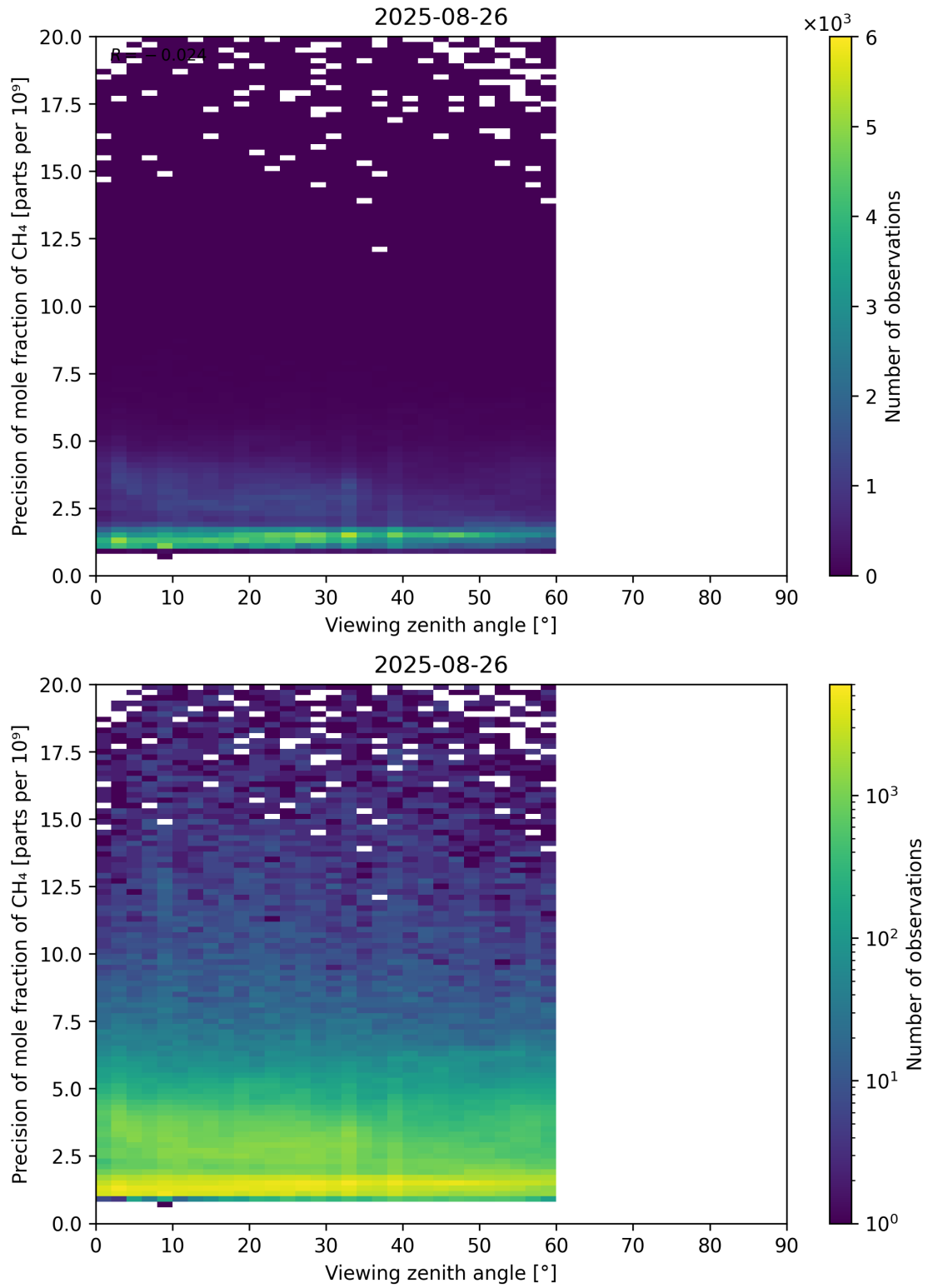
Figure 112: Scatter density plot of “Viewing zenith angle” against “Precision of mole fraction of CH 4 ” for 2025-08-25 to 2025-08-27.
