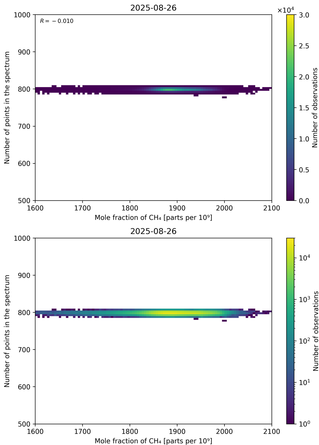
Figure 77: Scatter density plot of “Mole fraction of CH 4 ” against “Number of points in the spectrum” for 2025-08-25 to 2025-08-27.
