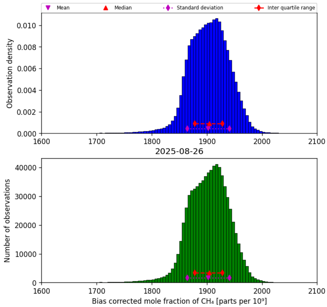
Figure 25: Histogram of “Bias corrected mole fraction of CH 4 ” for 2025-08-25 to 2025-08-27
