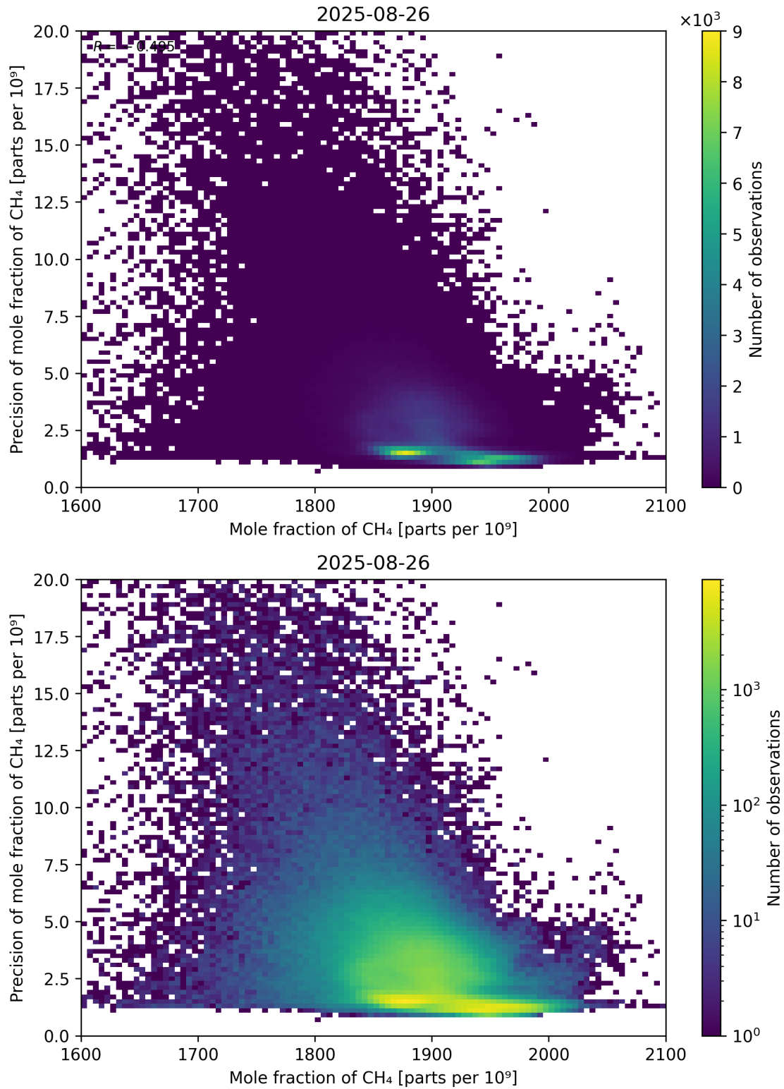
Figure 75: Scatter density plot of “Mole fraction of CH 4 ” against “Precision of mole fraction of CH 4 ” for 2025-08-25 to 2025-08-27.
