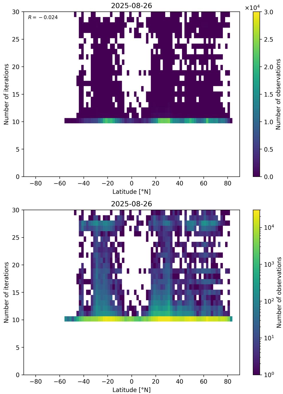
Figure 60: Scatter density plot of “Latitude” against “Number of iterations” for 2025-08-25 to 2025-08-27.
