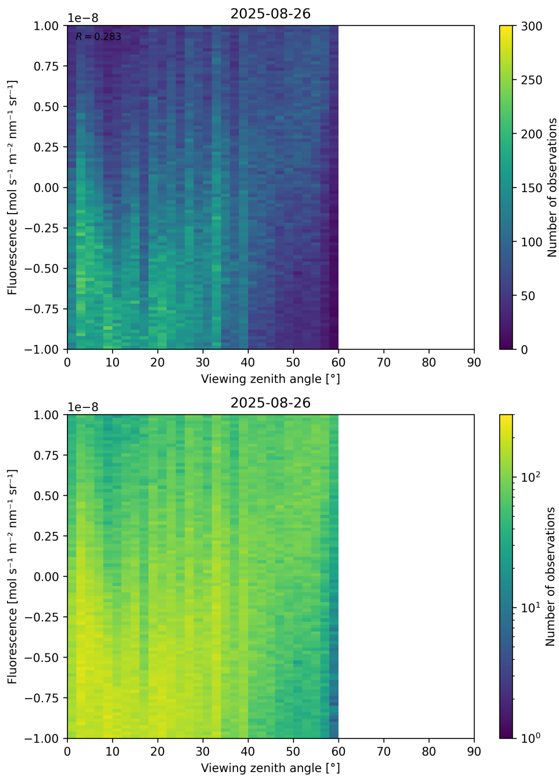
Figure 108: Scatter density plot of “Viewing zenith angle” against “Fluorescence” for 2025-08-25 to 2025-08-27.
