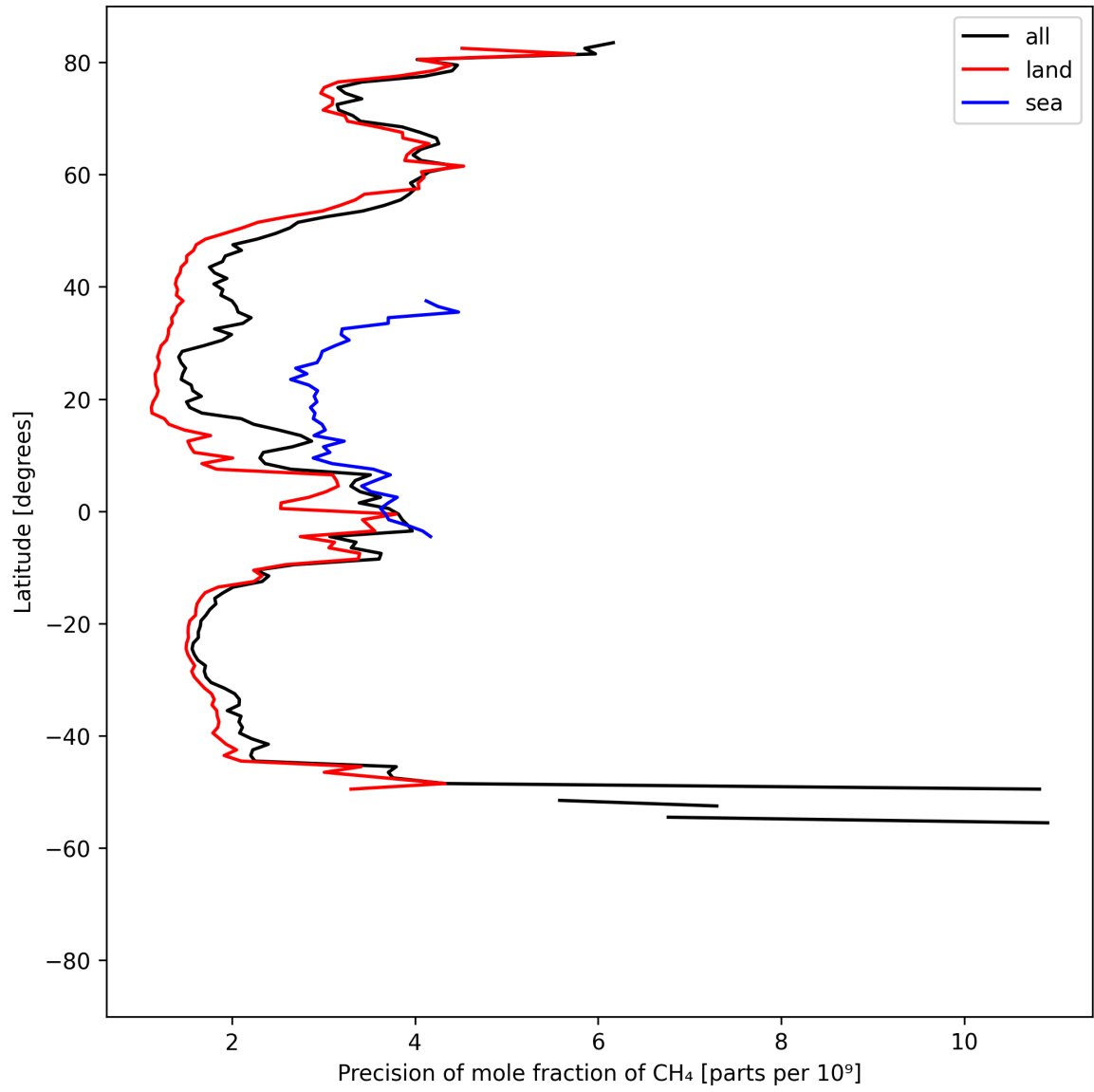
Figure 13: Zonal average of “Precision of mole fraction of CH 4 ” for 2025-08-25 to 2025-08-27.
