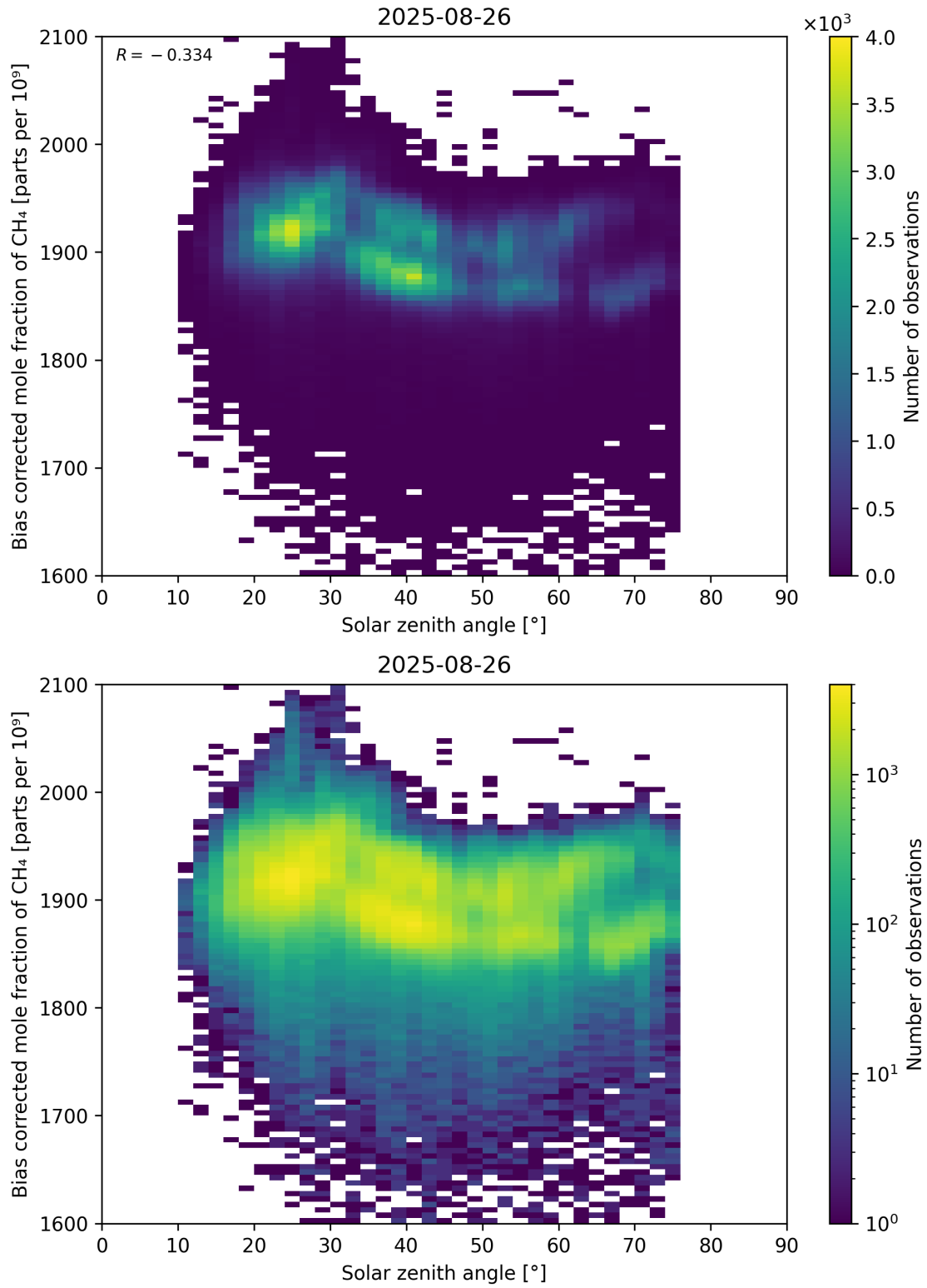
Figure 100: Scatter density plot of “Solar zenith angle” against “Bias corrected mole fraction of CH 4 ” for 2025-08-25 to 2025-08-27.
