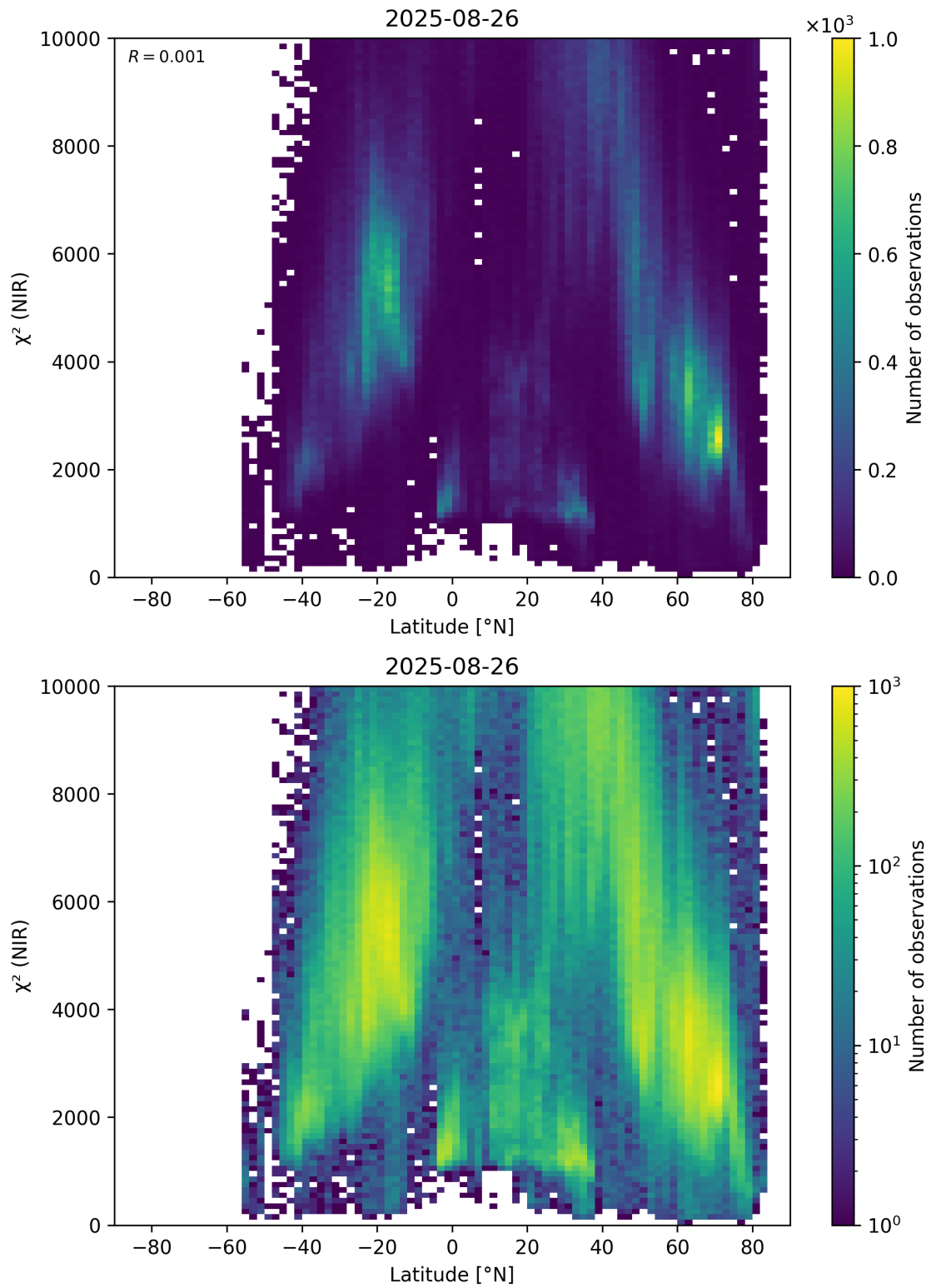
Figure 53: Scatter density plot of “Latitude” against “ \chi^2 (NIR)” for 2025-08-25 to 2025-08-27.
