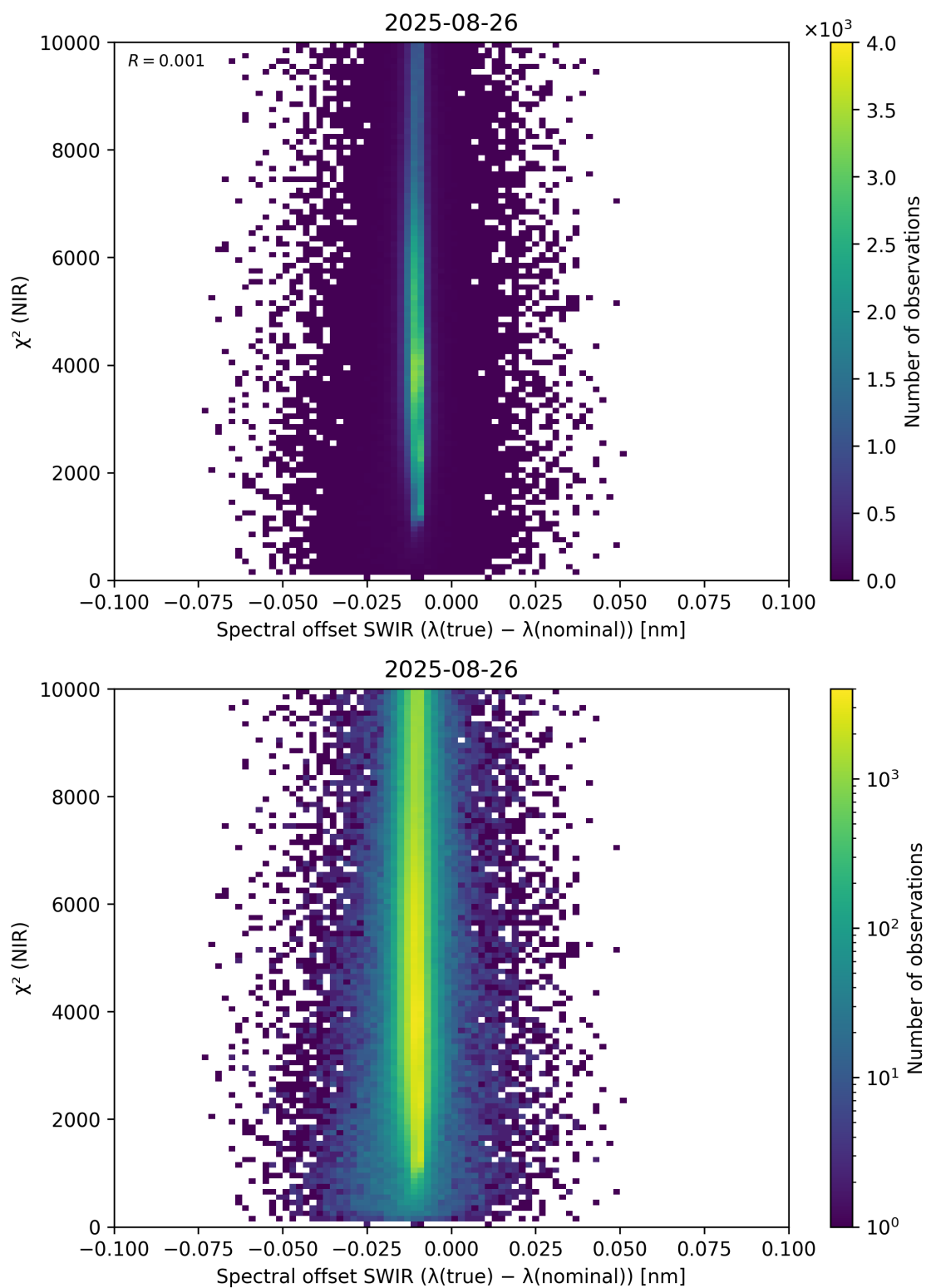
Figure 117: Scatter density plot of “Spectral offset SWIR ( \lambda_{\text{true}} - \lambda_{\text{nominal}} )” against “ \chi^2 (NIR)” for 2025-08-25 to 2025-08-27.
