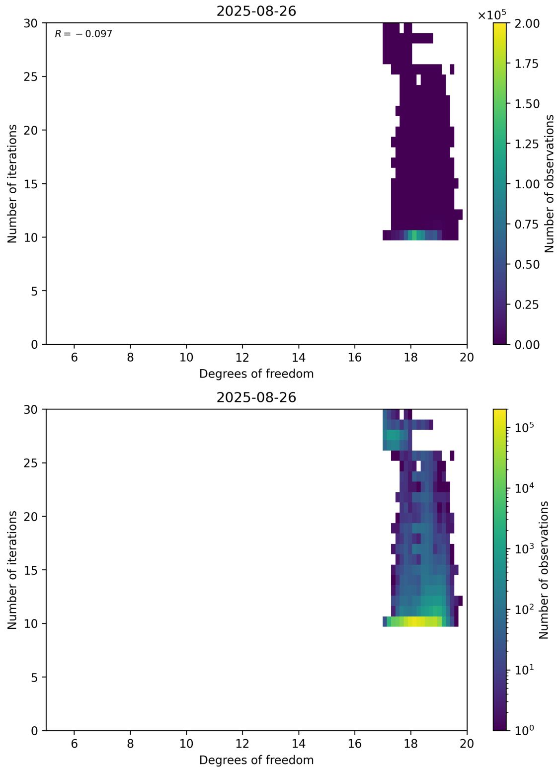
Figure 52: Scatter density plot of “Degrees of freedom” against “Number of iterations” for 2025-08-25 to 2025-08-27.
