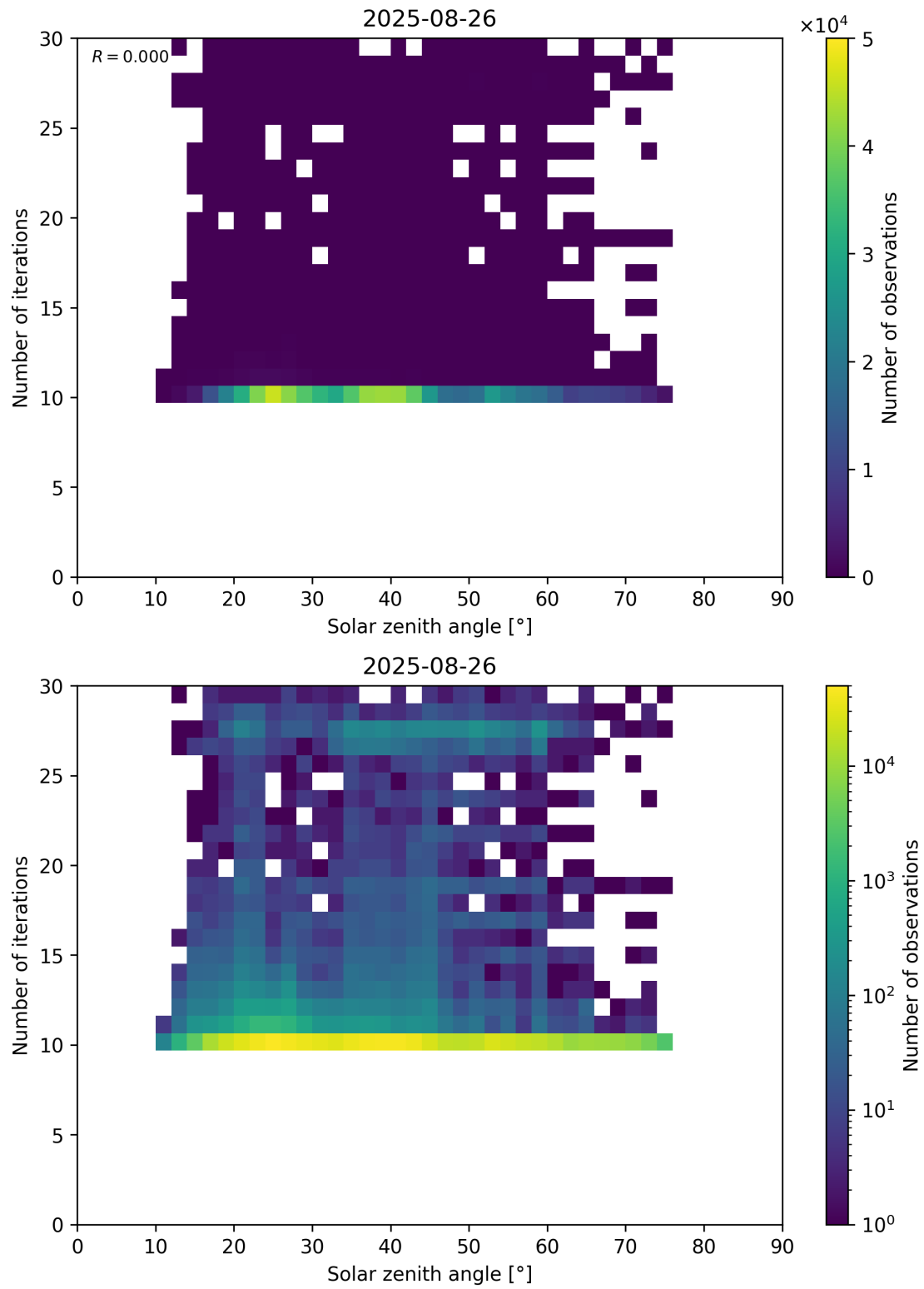
Figure 102: Scatter density plot of “Solar zenith angle” against “Number of iterations” for 2025-08-25 to 2025-08-27.
