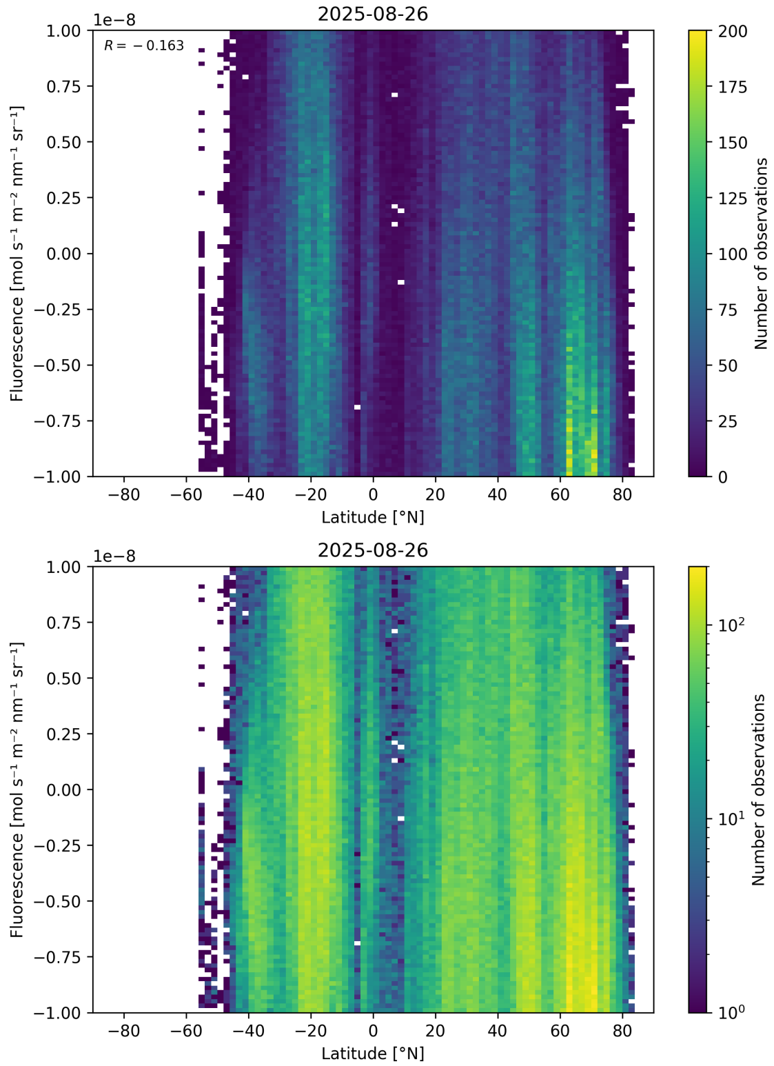
Figure 56: Scatter density plot of “Latitude” against “Fluorescence” for 2025-08-25 to 2025-08-27.
