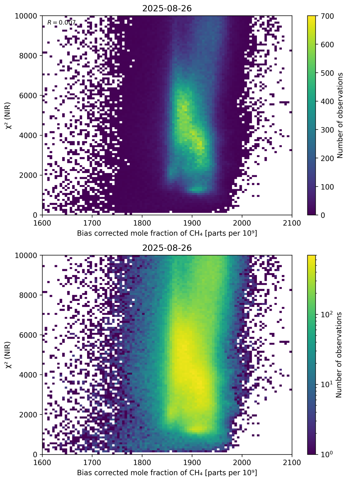
Figure 63: Scatter density plot of “Bias corrected mole fraction of CH 4 ” against “ \chi^2 (NIR)” for 2025-08-25 to 2025-08-27.
