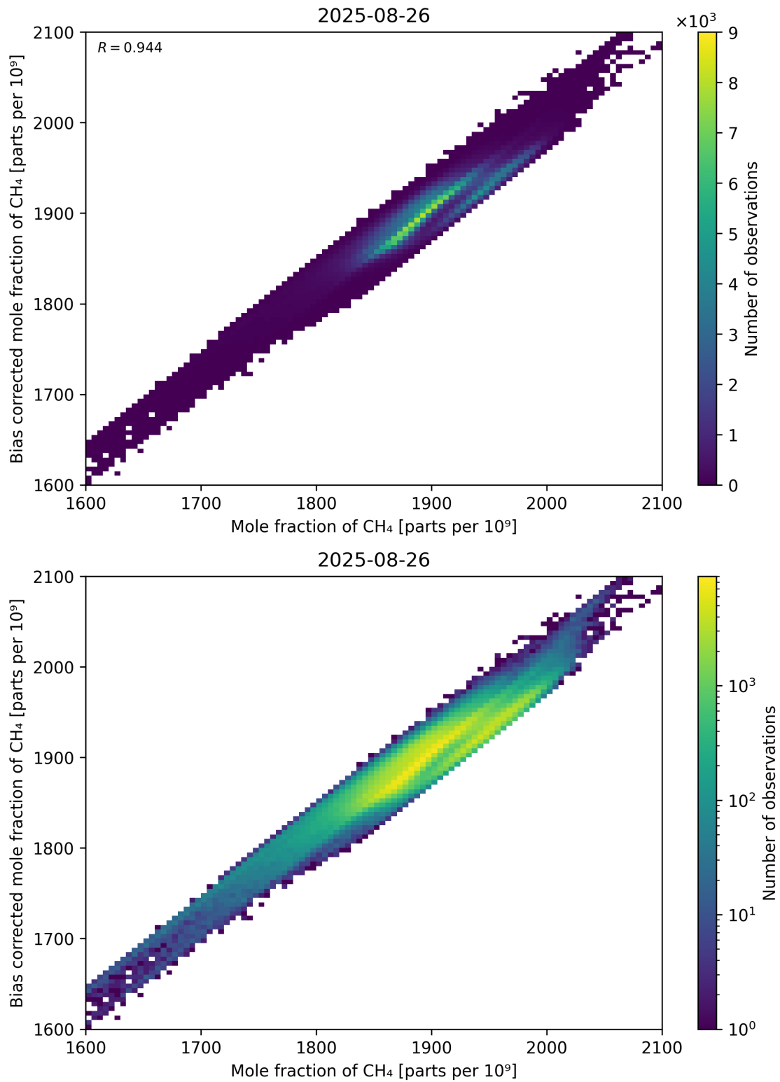
Figure 74: Scatter density plot of “Mole fraction of CH 4 ” against “Bias corrected mole fraction of CH 4 ” for 2025-08-25 to 2025-08-27.
