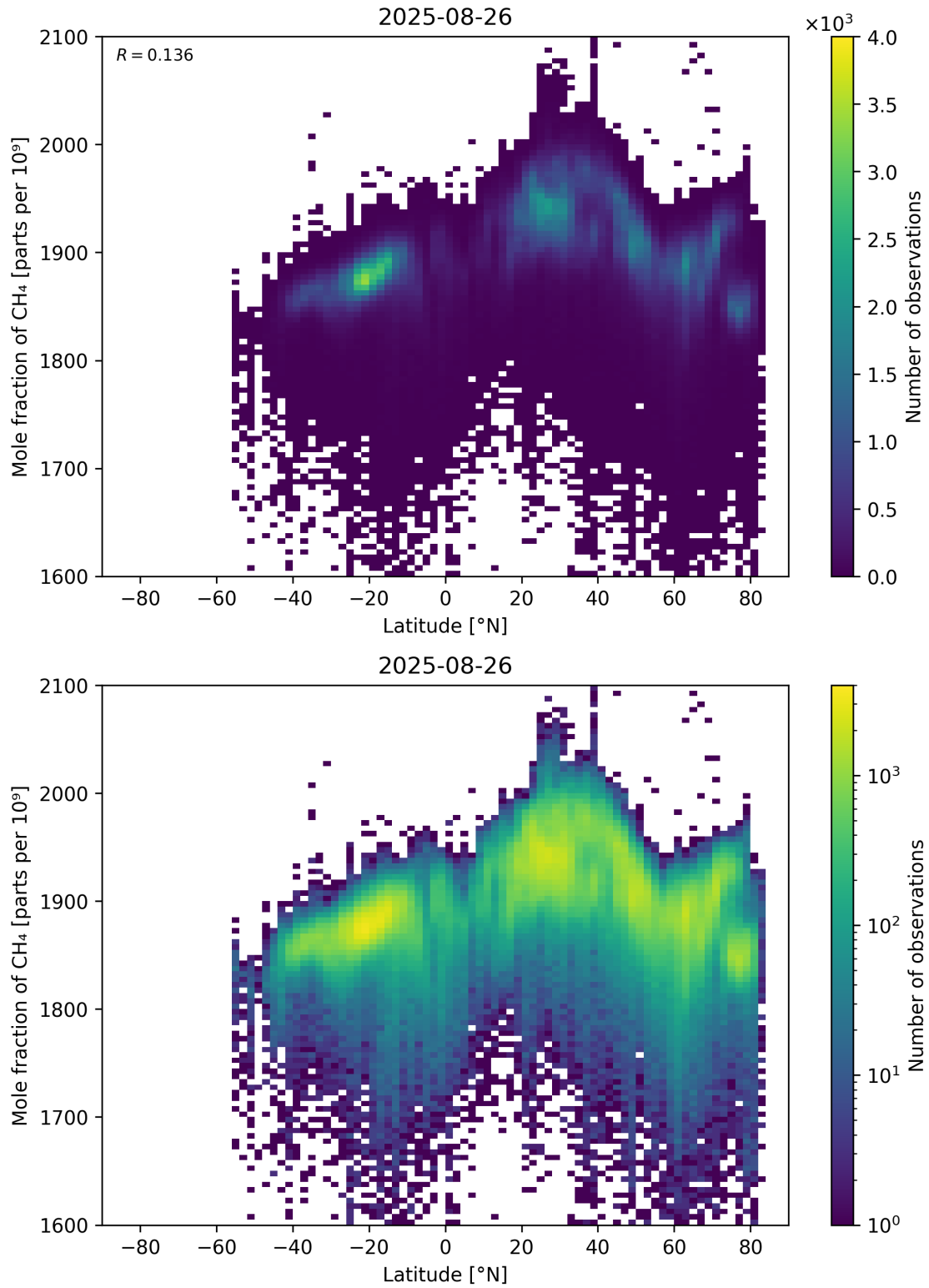
Figure 57: Scatter density plot of “Latitude” against “Mole fraction of CH 4 ” for 2025-08-25 to 2025-08-27.
