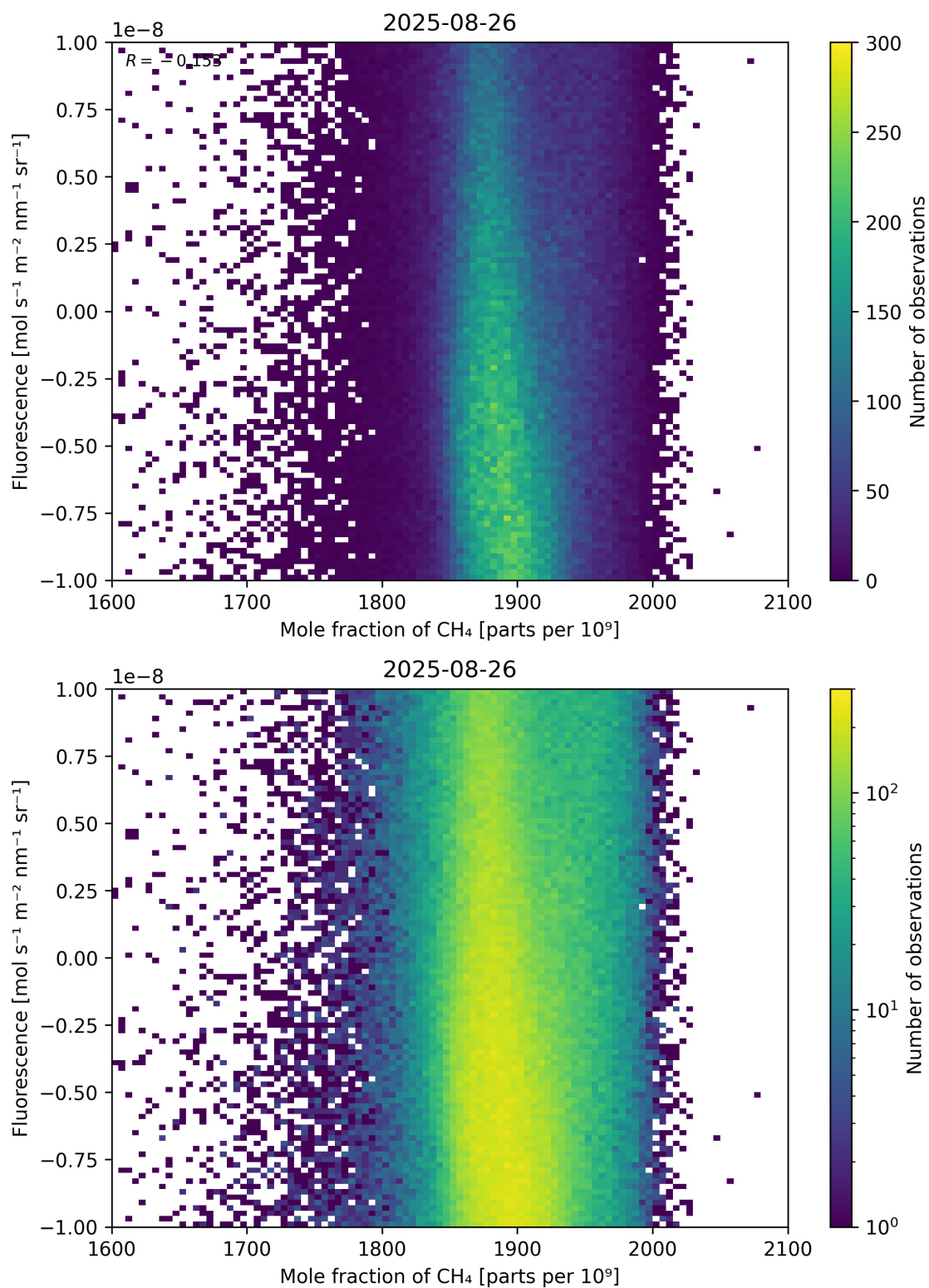
Figure 73: Scatter density plot of “Mole fraction of \text{CH}_4 ” against “Fluorescence” for 2025-08-25 to 2025-08-27.
