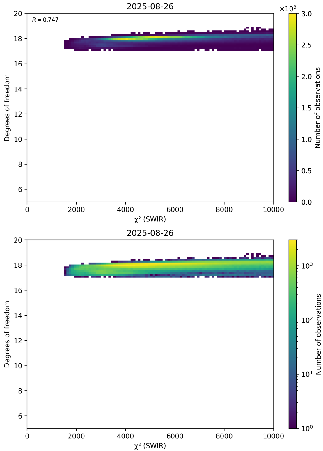
Figure 48: Scatter density plot of “ \chi^2 (SWIR)” against “Degrees of freedom” for 2025-08-25 to 2025-08-27.
