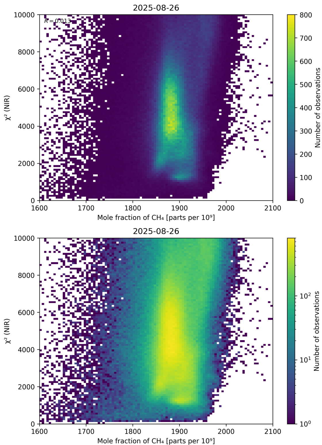
Figure 70: Scatter density plot of “Mole fraction of \text{CH}_4 ” against “ \chi^2 (NIR)” for 2025-08-25 to 2025-08-27.
