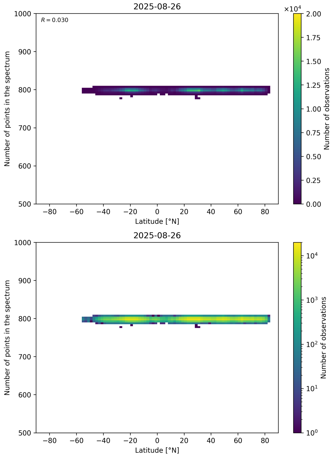
Figure 61: Scatter density plot of “Latitude” against “Number of points in the spectrum” for 2025-08-25 to 2025-08-27.
