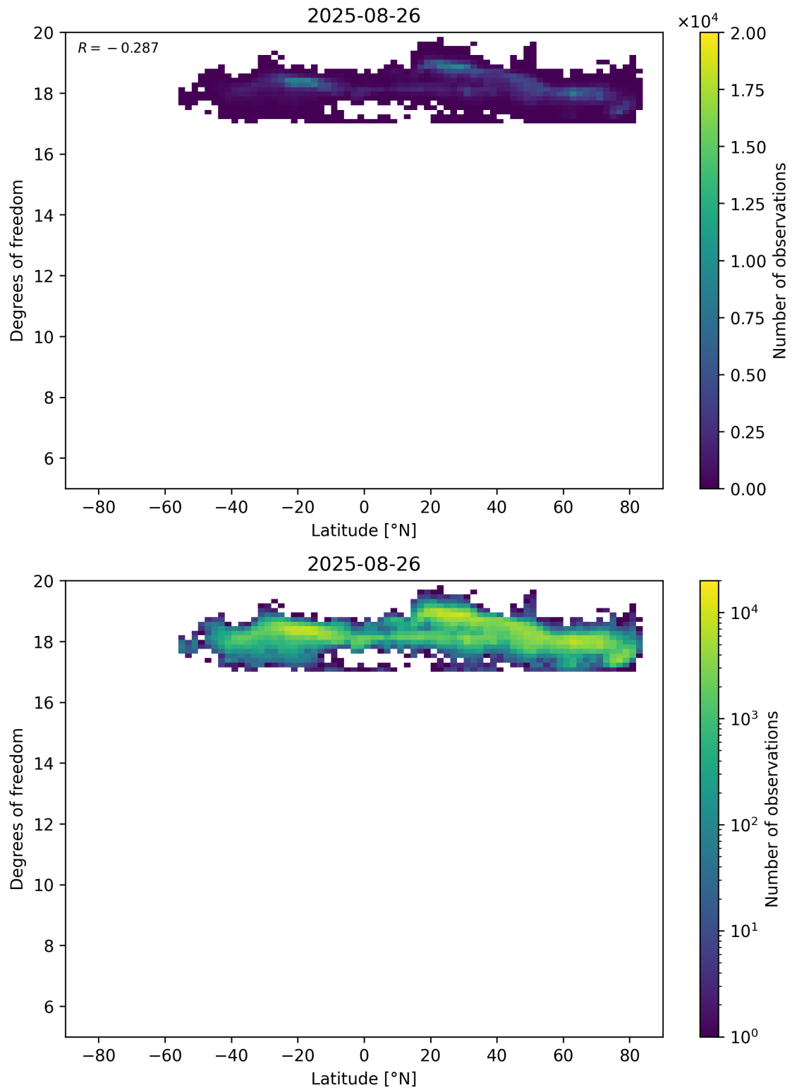
Figure 55: Scatter density plot of “Latitude” against “Degrees of freedom” for 2025-08-25 to 2025-08-27.
