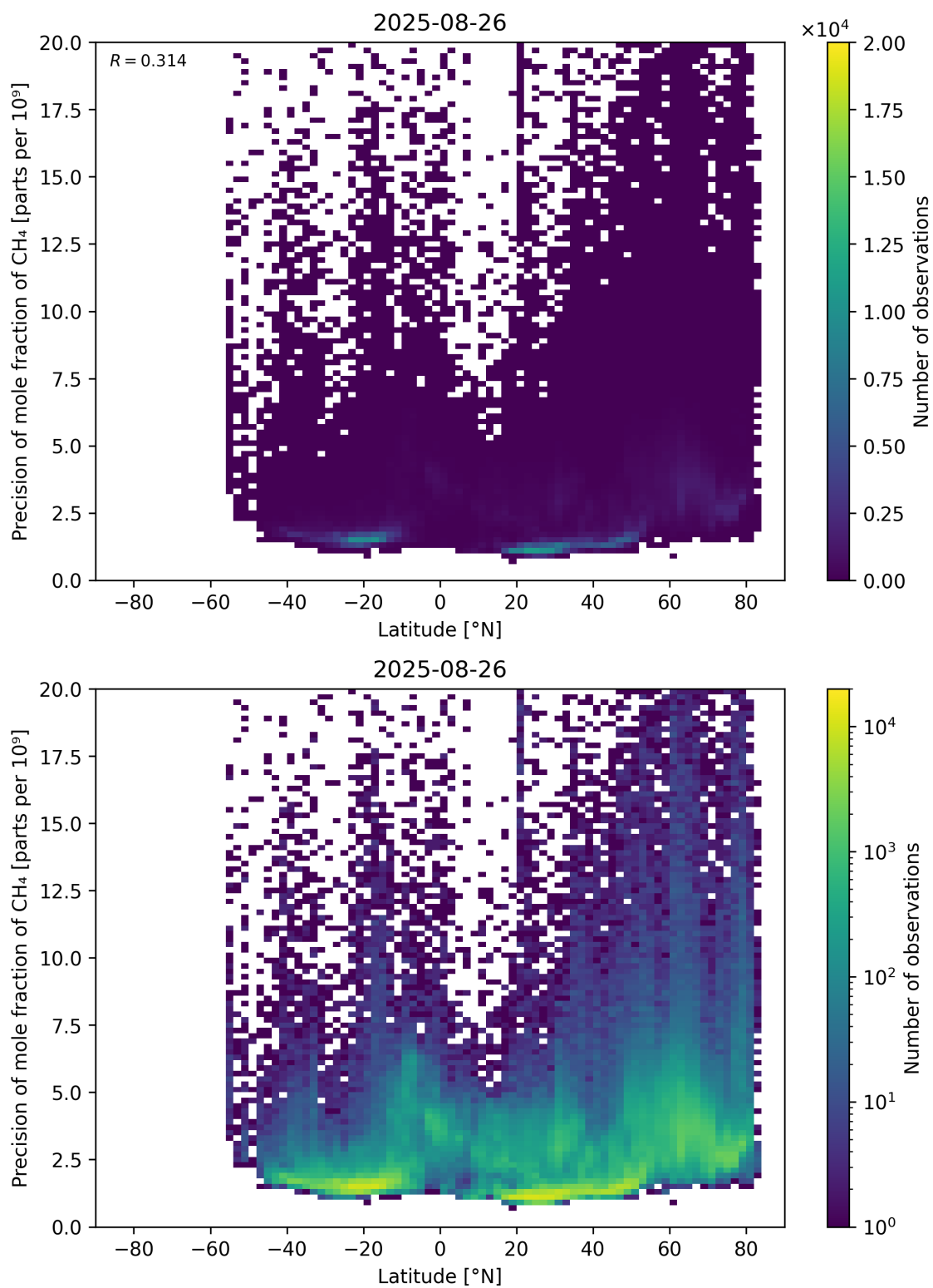
Figure 59: Scatter density plot of “Latitude” against “Precision of mole fraction of \text{CH}_4 ” for 2025-08-25 to 2025-08-27.
