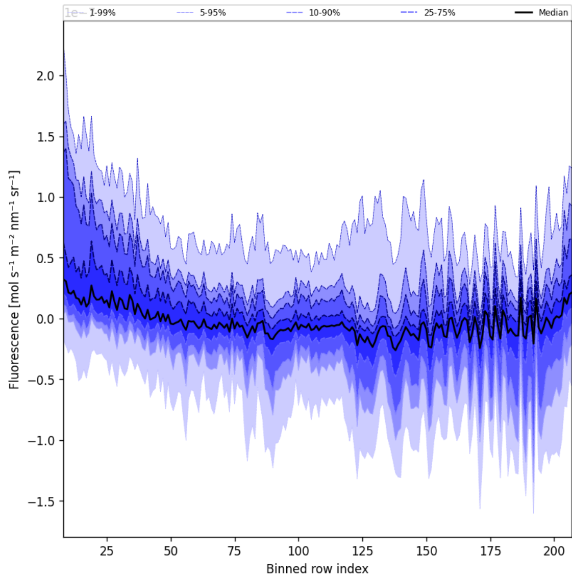
Figure 43: Along track statistics of "Fluorescence" for 2025-08-25 to 2025-08-27
