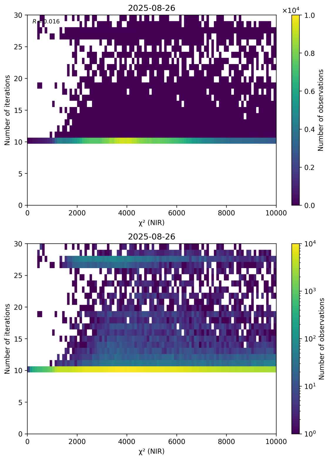
Figure 46: Scatter density plot of “ \chi^2 (NIR)” against “Number of iterations” for 2025-08-25 to 2025-08-27.
