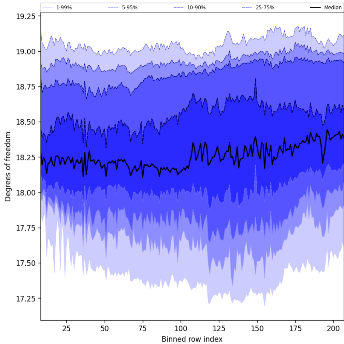
Figure 41: Along track statistics of “Degrees of freedom” for 2025-08-25 to 2025-08-27
