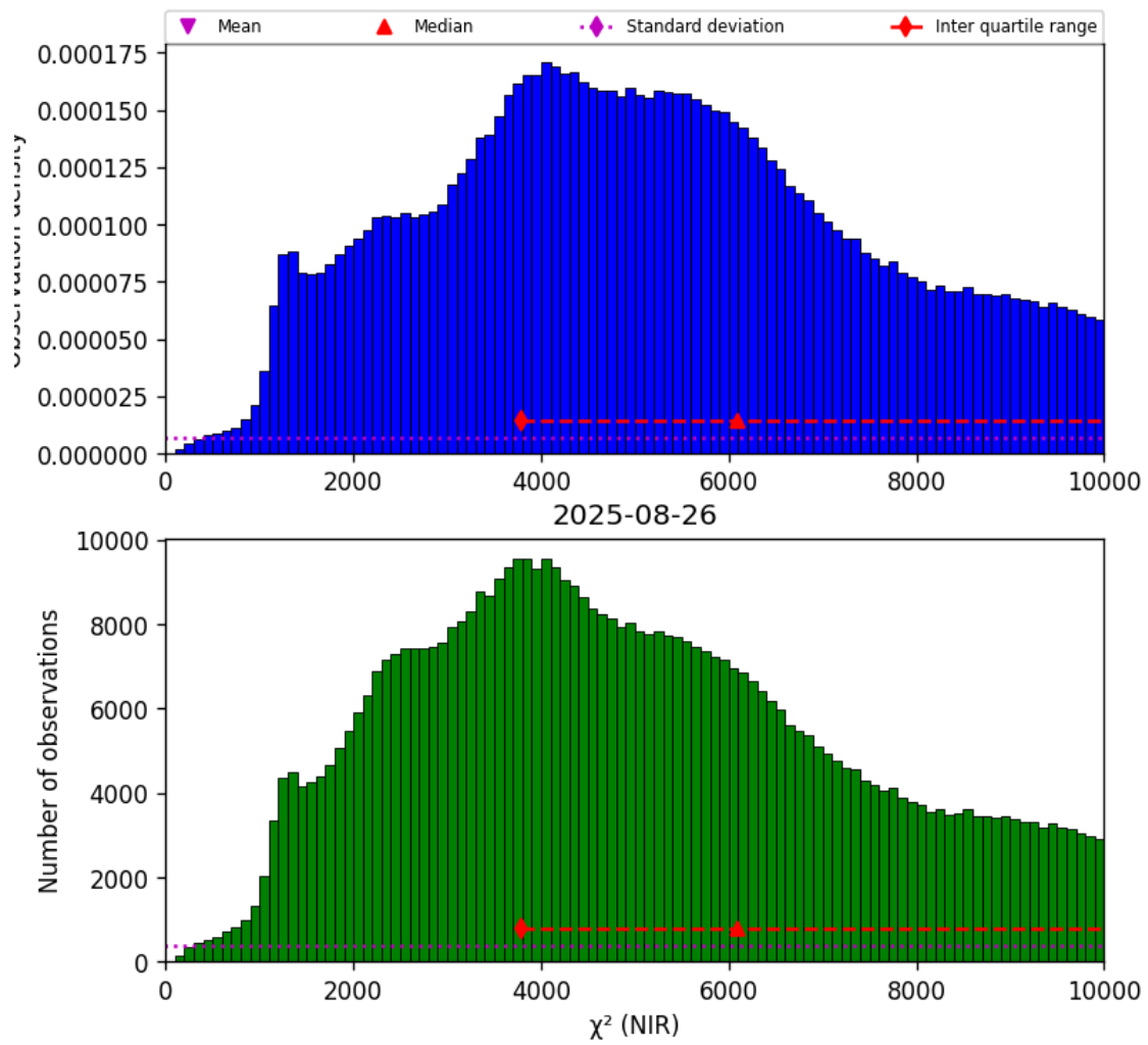
Figure 29: Histogram of “ \chi^2 (NIR)” for 2025-08-25 to 2025-08-27
