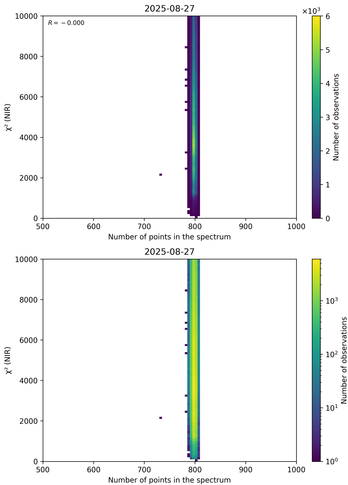
Figure 88: Scatter density plot of “Number of points in the spectrum” against “ \chi^2 (NIR)” for 2025-08-26 to 2025-08-28.
