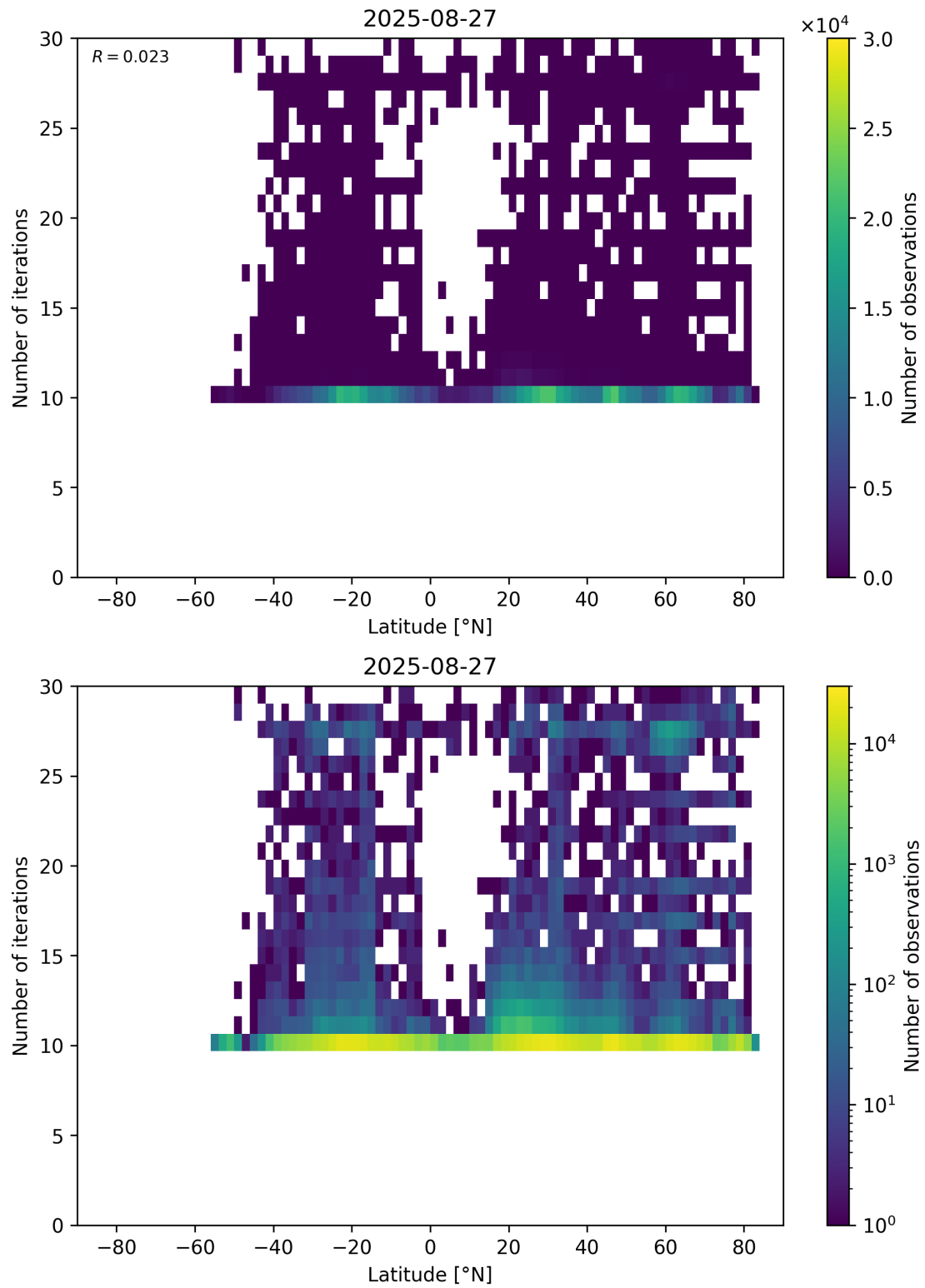
Figure 60: Scatter density plot of “Latitude” against “Number of iterations” for 2025-08-26 to 2025-08-28.
