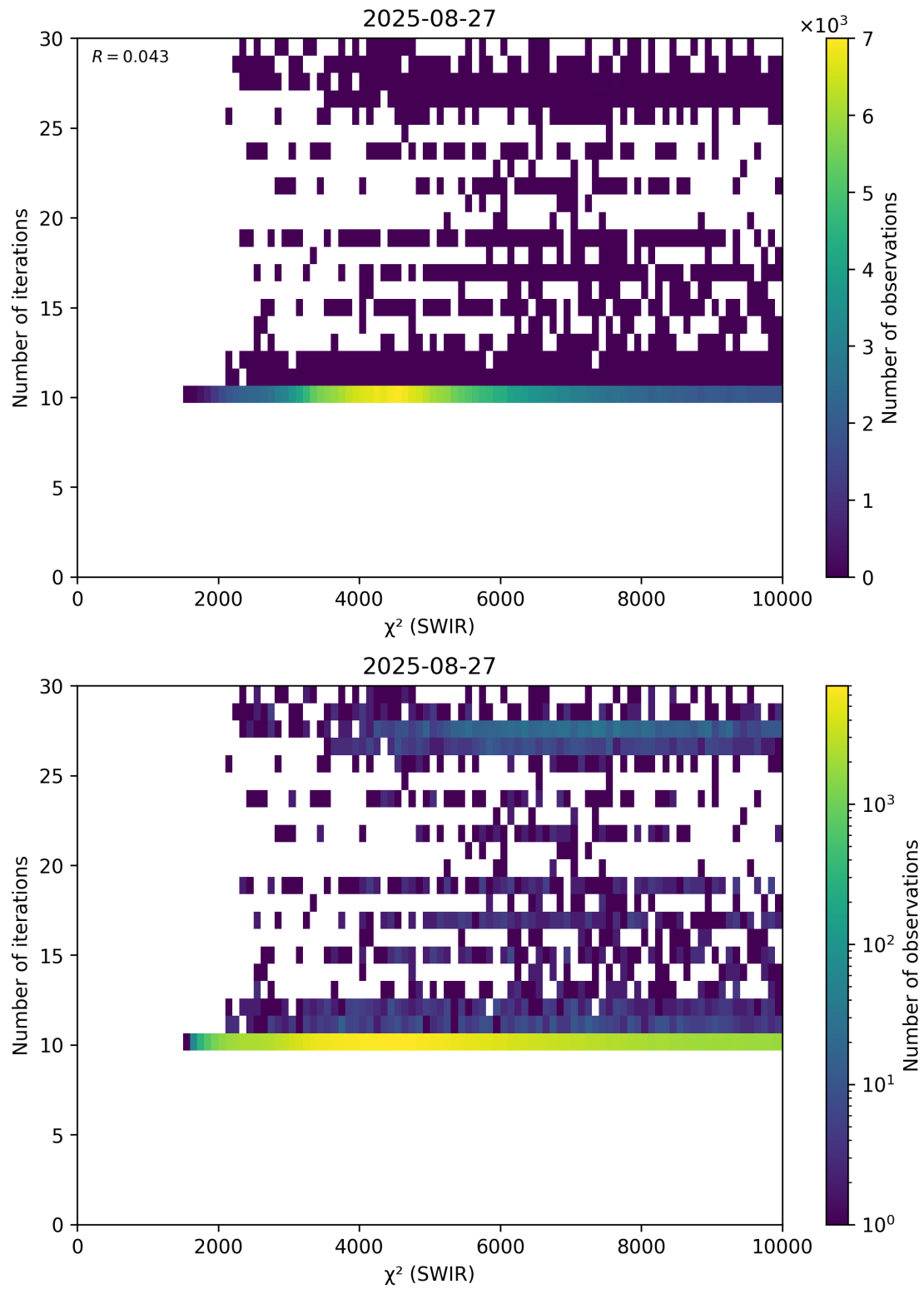
Figure 50: Scatter density plot of “ \chi^2 (SWIR)” against “Number of iterations” for 2025-08-26 to 2025-08-28.
