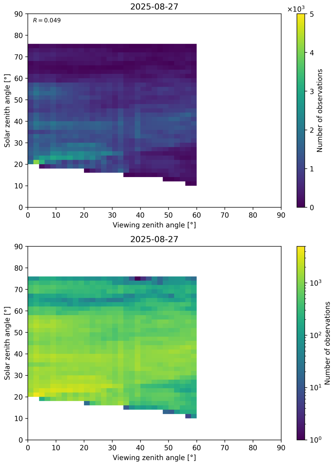
Figure 115: Scatter density plot of “Viewing zenith angle” against “Solar zenith angle” for 2025-08-26 to 2025-08-28.
