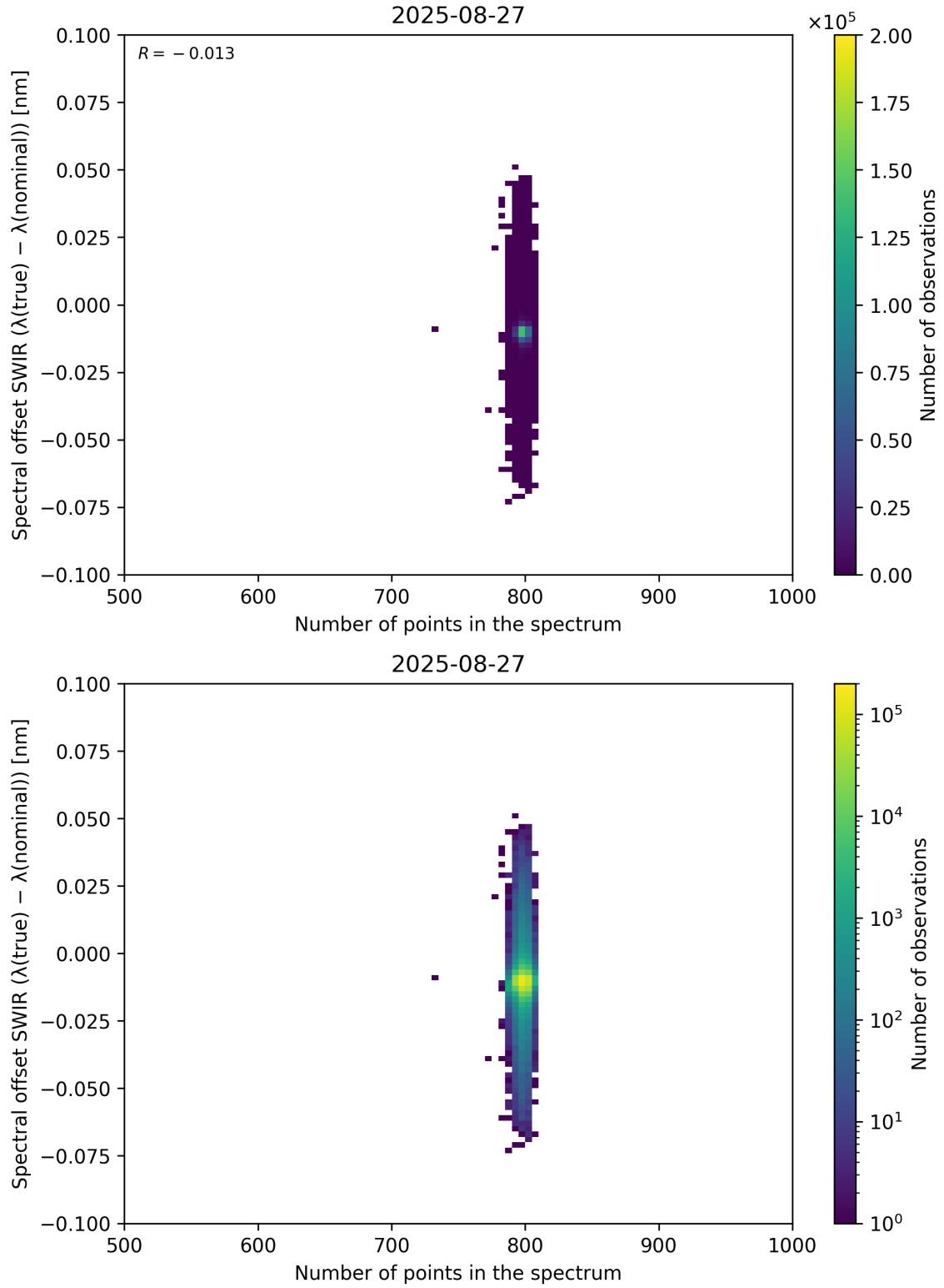
Figure 93: Scatter density plot of “Number of points in the spectrum” against “Spectral offset SWIR ( \lambda_{\text{true}} - \lambda_{\text{nominal}} )” for 2025-08-26 to 2025-08-28.
