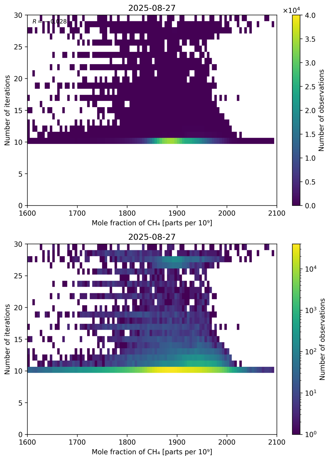
Figure 76: Scatter density plot of “Mole fraction of CH 4 ” against “Number of iterations” for 2025-08-26 to 2025-08-28.
