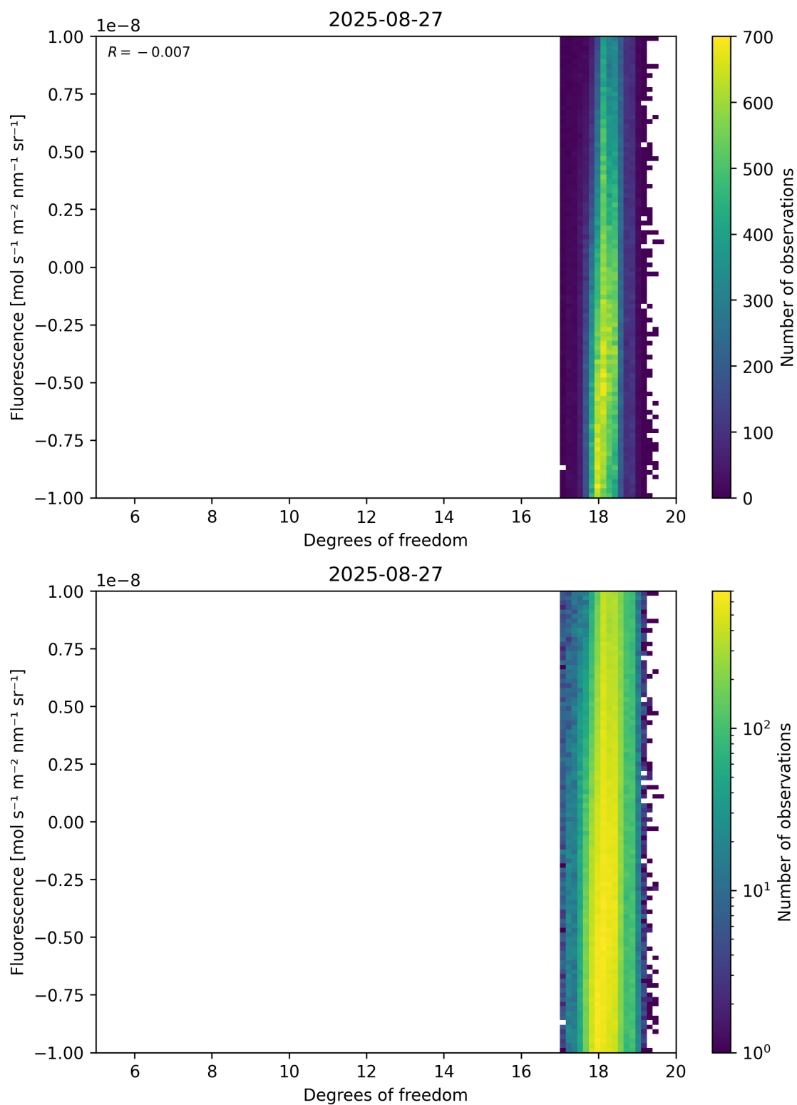
Figure 51: Scatter density plot of “Degrees of freedom” against “Fluorescence” for 2025-08-26 to 2025-08-28.
