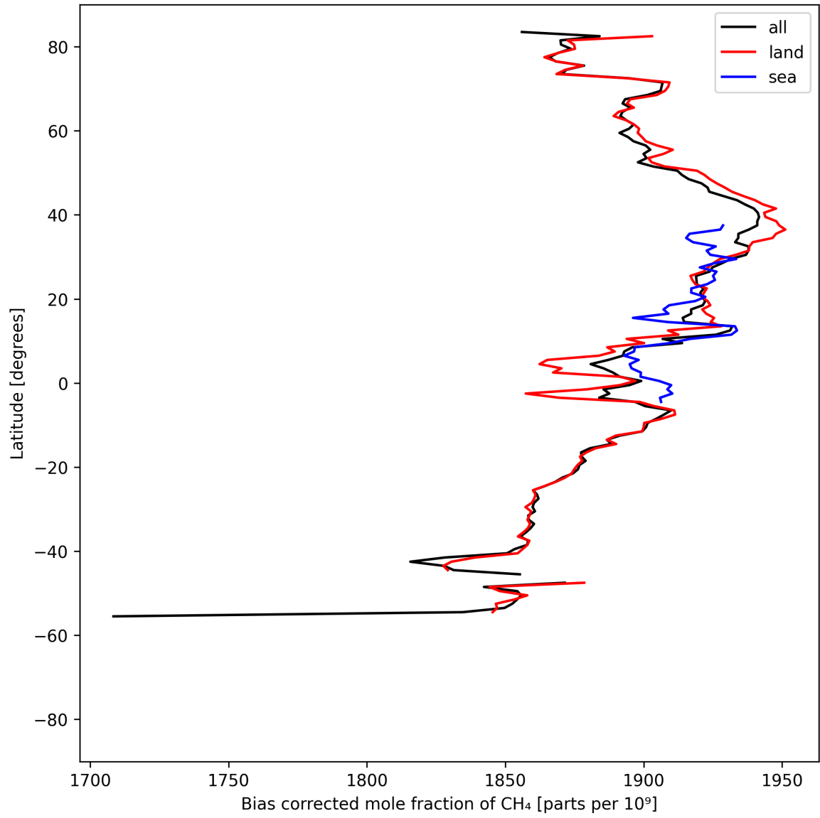
Figure 14: Zonal average of “Bias corrected mole fraction of \text{CH}_4 ” for 2025-08-26 to 2025-08-28.
