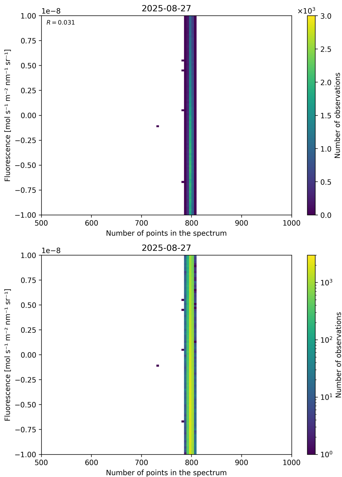
Figure 91: Scatter density plot of “Number of points in the spectrum” against “Fluorescence” for 2025-08-26 to 2025-08-28.
