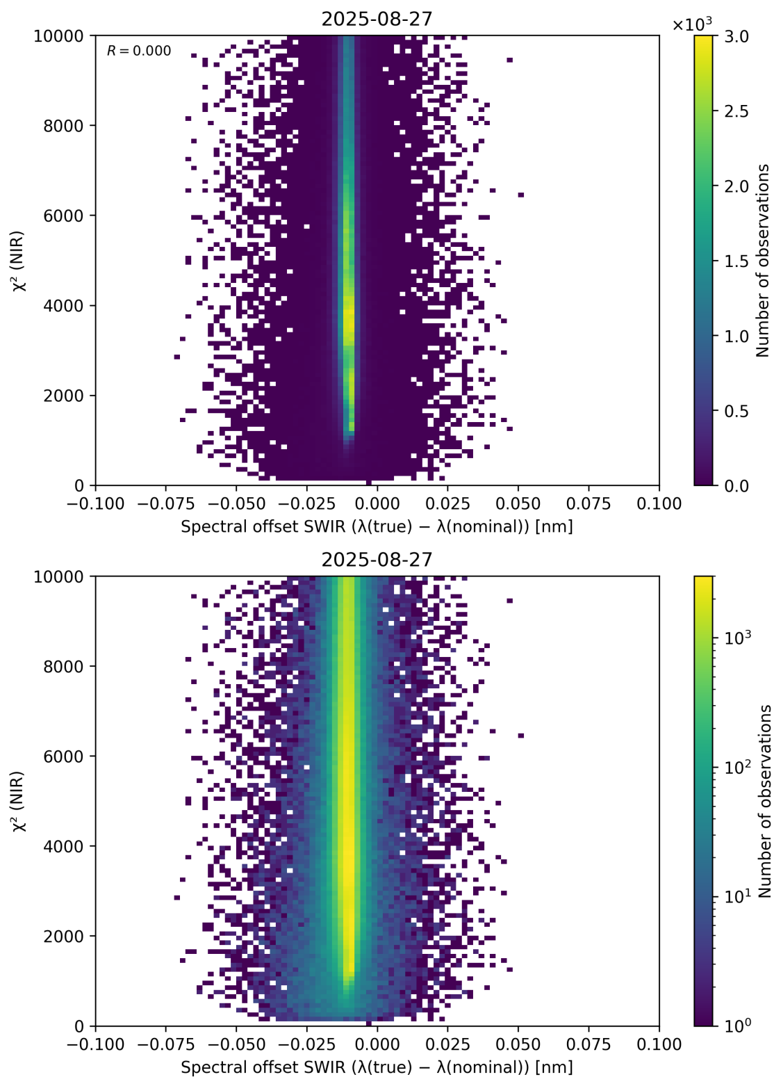
Figure 117: Scatter density plot of “Spectral offset SWIR ( \lambda_{\text{true}} - \lambda_{\text{nominal}} )” against “ \chi^2 (NIR)” for 2025-08-26 to 2025-08-28.
