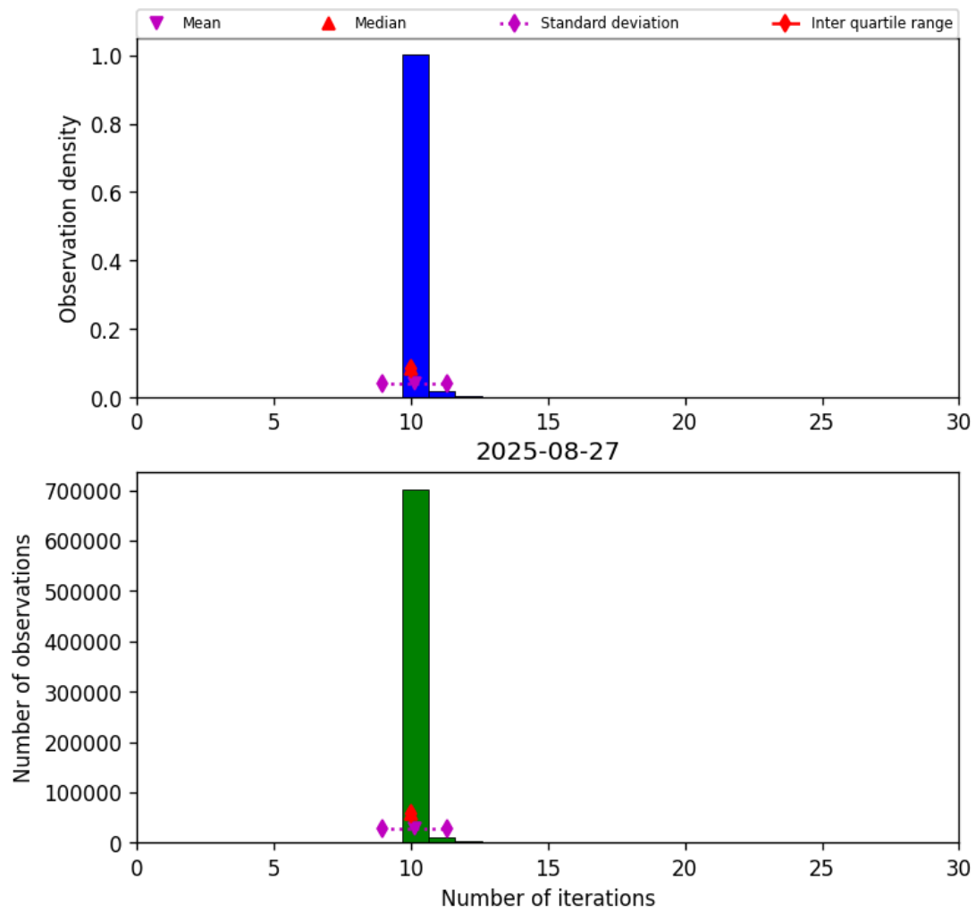
Figure 31: Histogram of “Number of iterations” for 2025-08-26 to 2025-08-28
