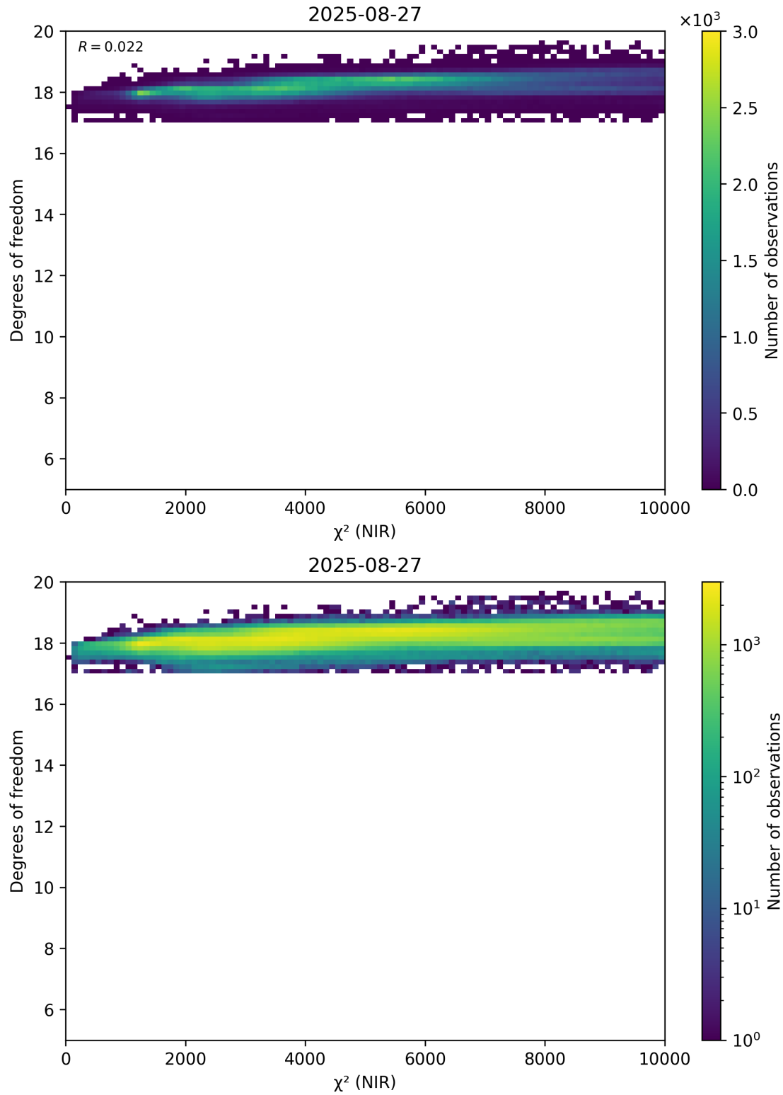
Figure 44: Scatter density plot of “ \chi^2 (NIR)” against “Degrees of freedom” for 2025-08-26 to 2025-08-28.
