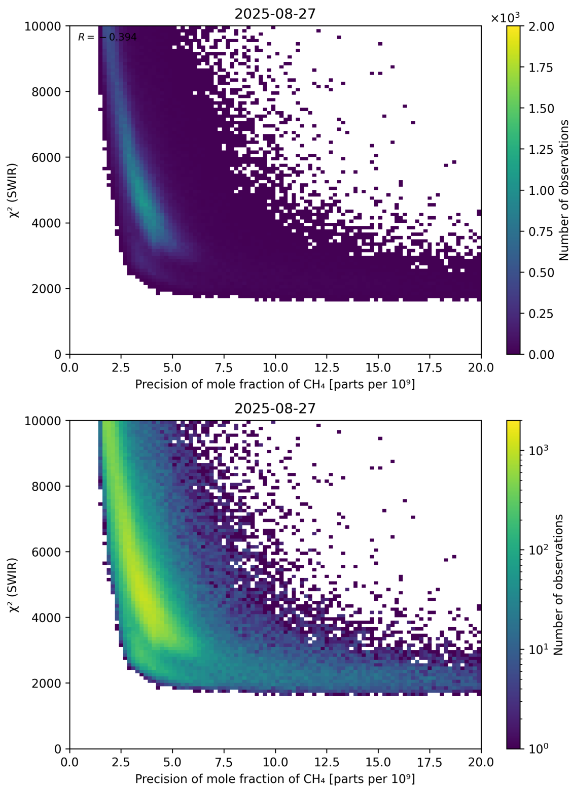
Figure 79: Scatter density plot of “Precision of mole fraction of \text{CH}_4 ” against “ \chi^2 (SWIR)” for 2025-08-26 to 2025-08-28.
