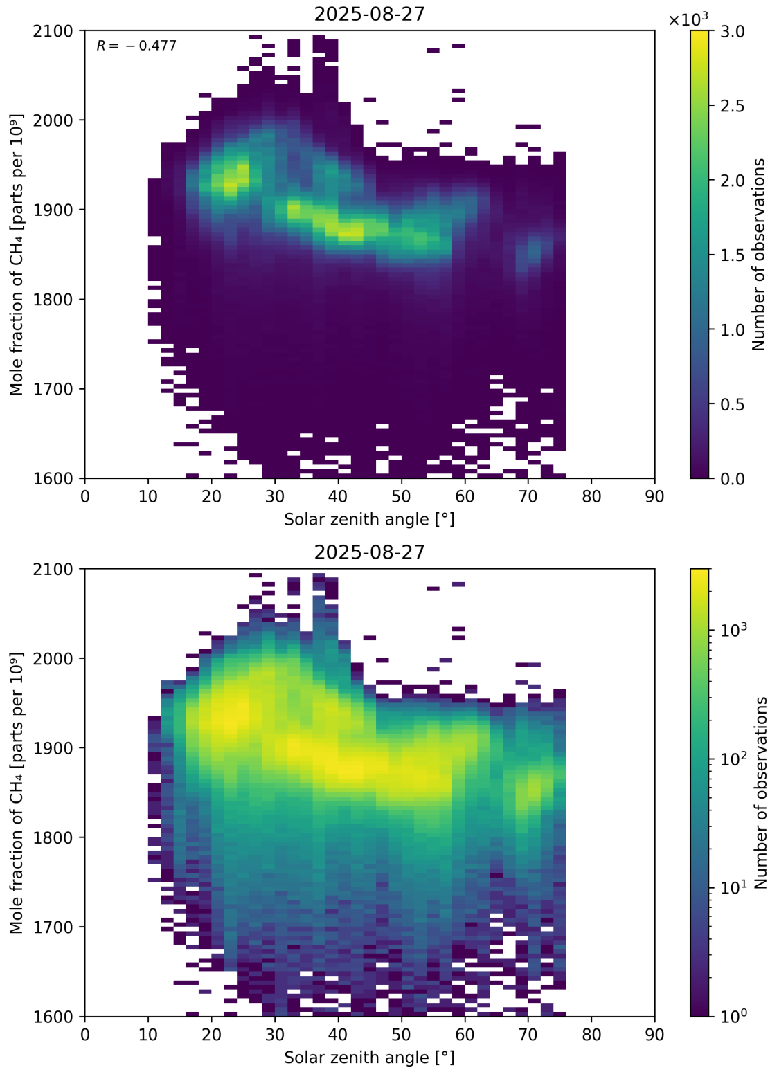
Figure 99: Scatter density plot of “Solar zenith angle” against “Mole fraction of CH 4 ” for 2025-08-26 to 2025-08-28.
