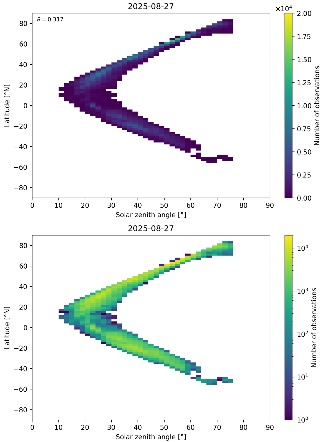
Figure 98: Scatter density plot of “Solar zenith angle” against “Latitude” for 2025-08-26 to 2025-08-28.
