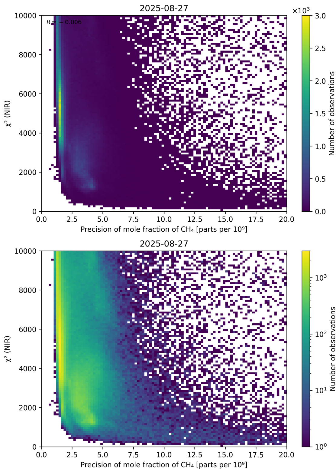
Figure 78: Scatter density plot of “Precision of mole fraction of CH 4 ” against “ \chi^2 (NIR)” for 2025-08-26 to 2025-08-28.
