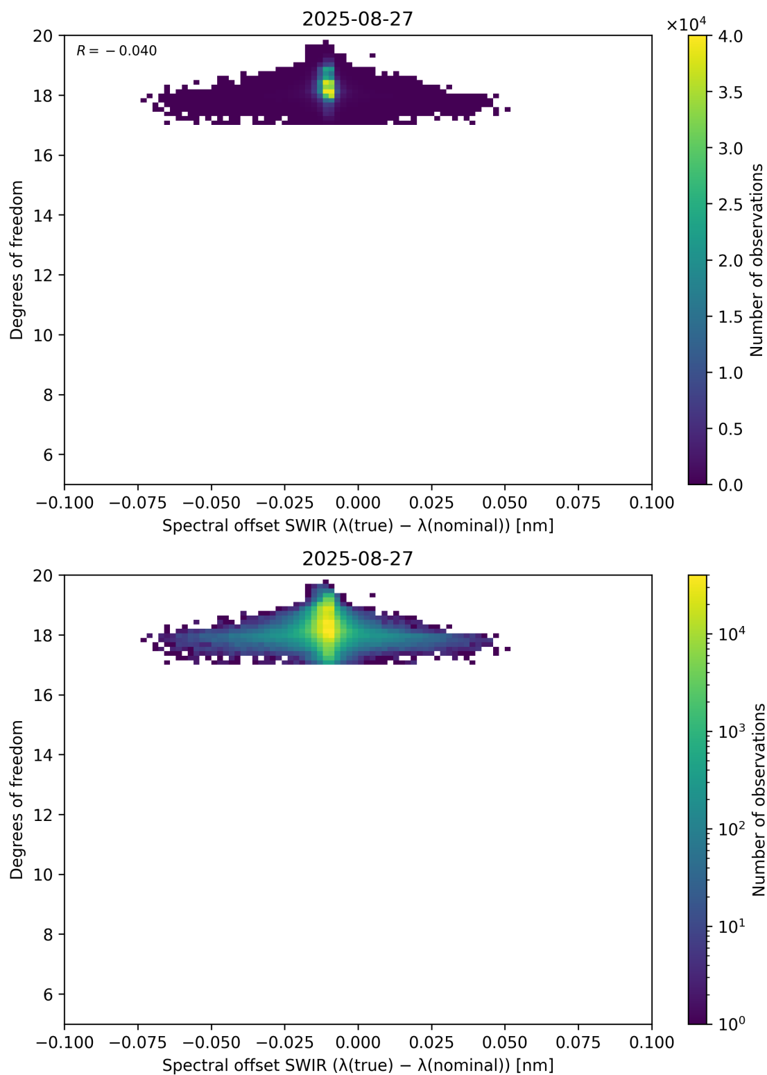
Figure 119: Scatter density plot of “Spectral offset SWIR ( \lambda_{\text{true}} - \lambda_{\text{nominal}} )” against “Degrees of freedom” for 2025-08-26 to 2025-08-28.
