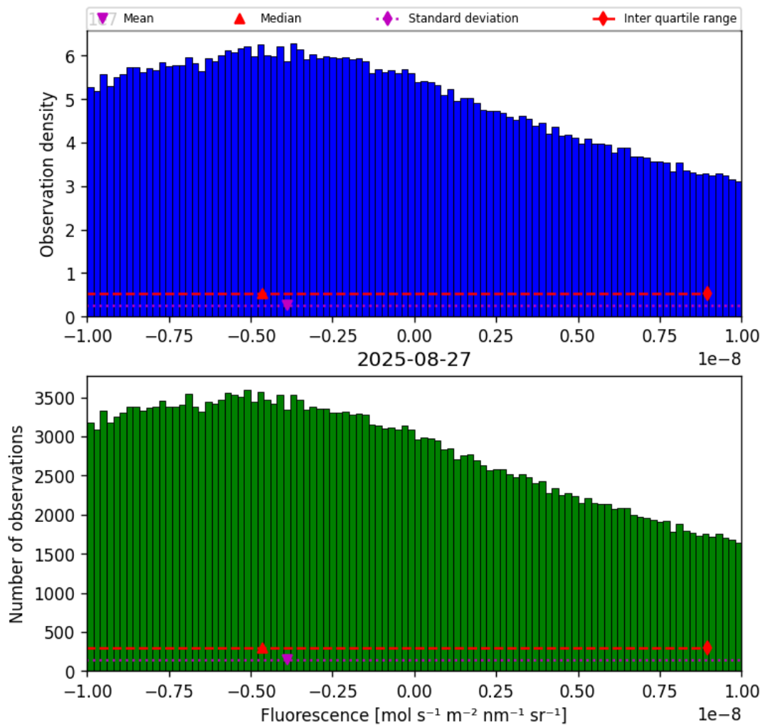
Figure 32: Histogram of “Fluorescence” for 2025-08-26 to 2025-08-28
