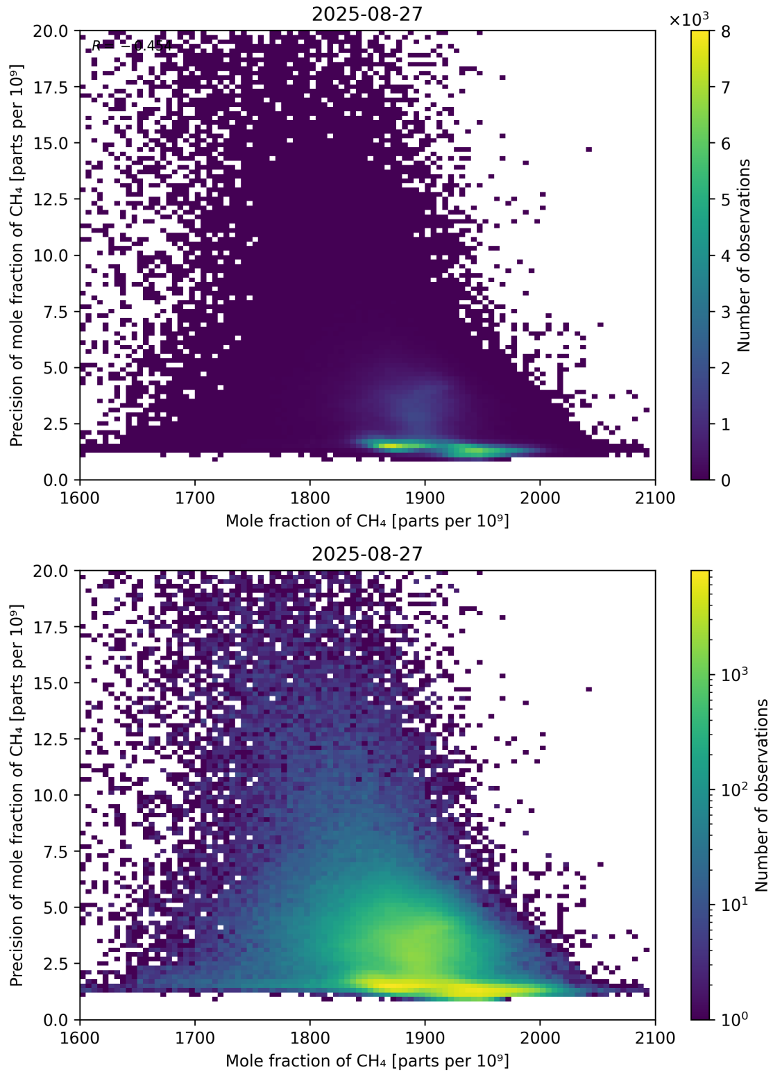
Figure 75: Scatter density plot of “Mole fraction of CH 4 ” against “Precision of mole fraction of CH 4 ” for 2025-08-26 to 2025-08-28.
