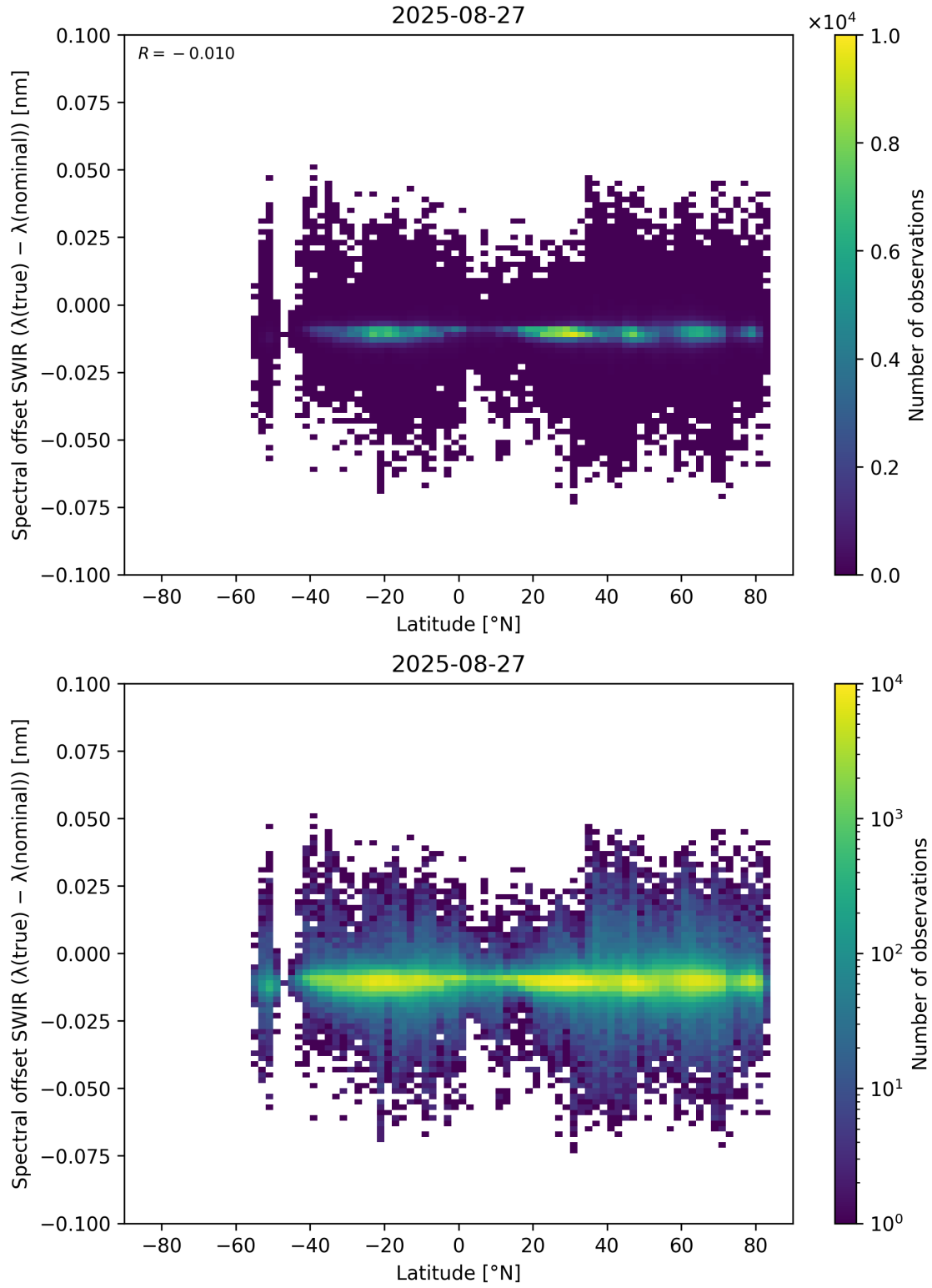
Figure 62: Scatter density plot of “Latitude” against “Spectral offset SWIR ( \lambda_{\text{true}} - \lambda_{\text{nominal}} )” for 2025-08-26 to 2025-08-28.
