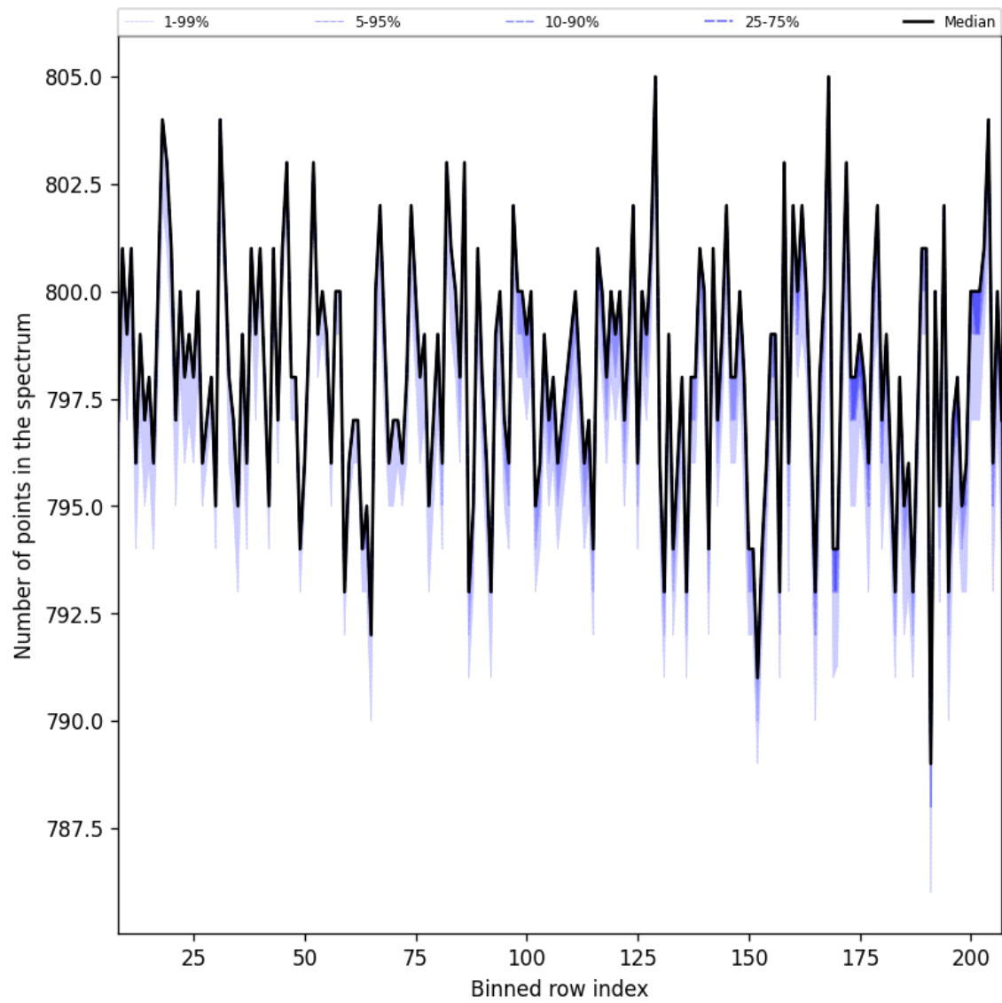
Figure 37: Along track statistics of “Number of points in the spectrum” for 2025-08-26 to 2025-08-28
