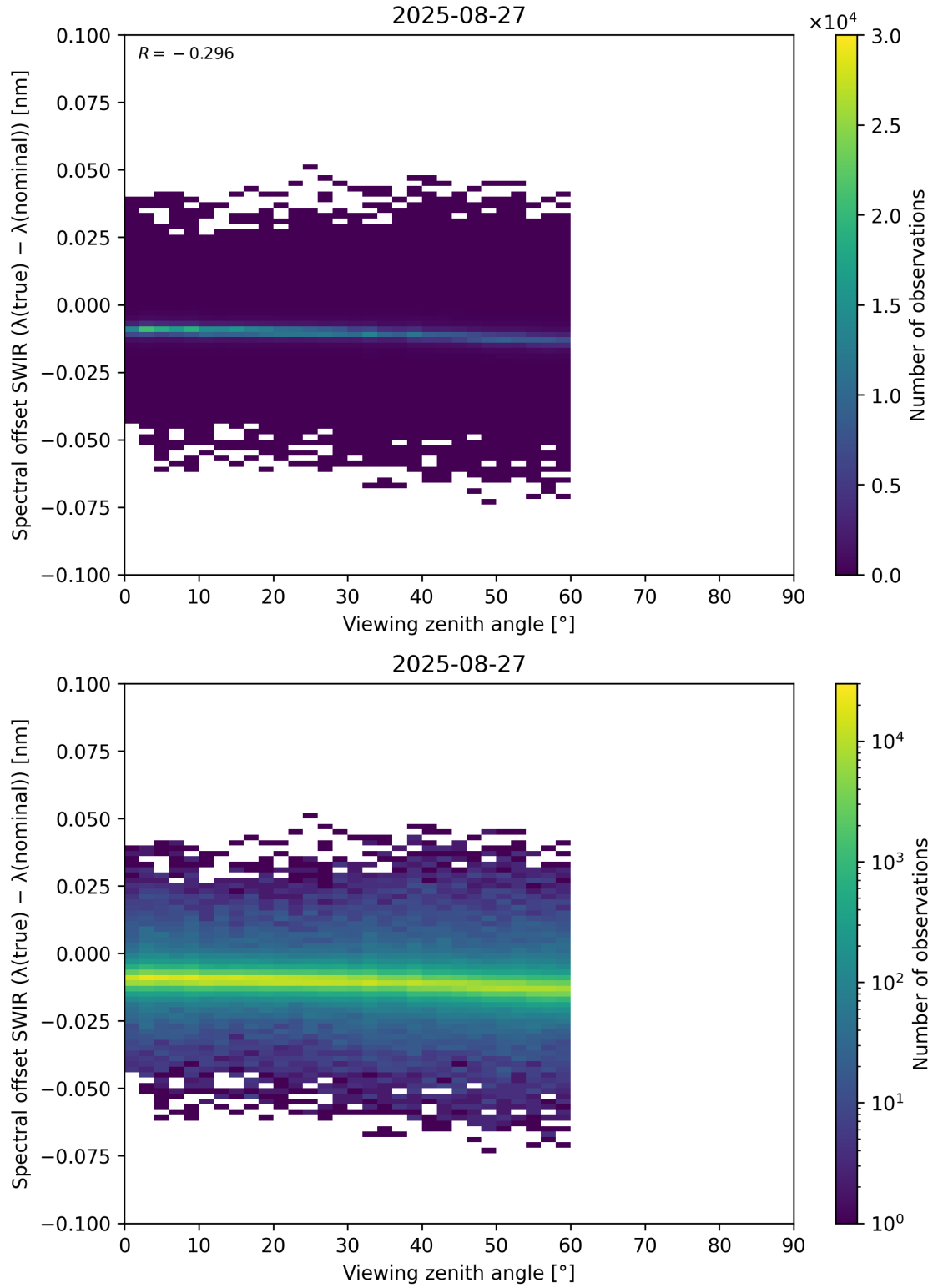
Figure 116: Scatter density plot of “Viewing zenith angle” against “Spectral offset SWIR ( \lambda_{\text{true}} - \lambda_{\text{nominal}} )” for 2025-08-26 to 2025-08-28.
