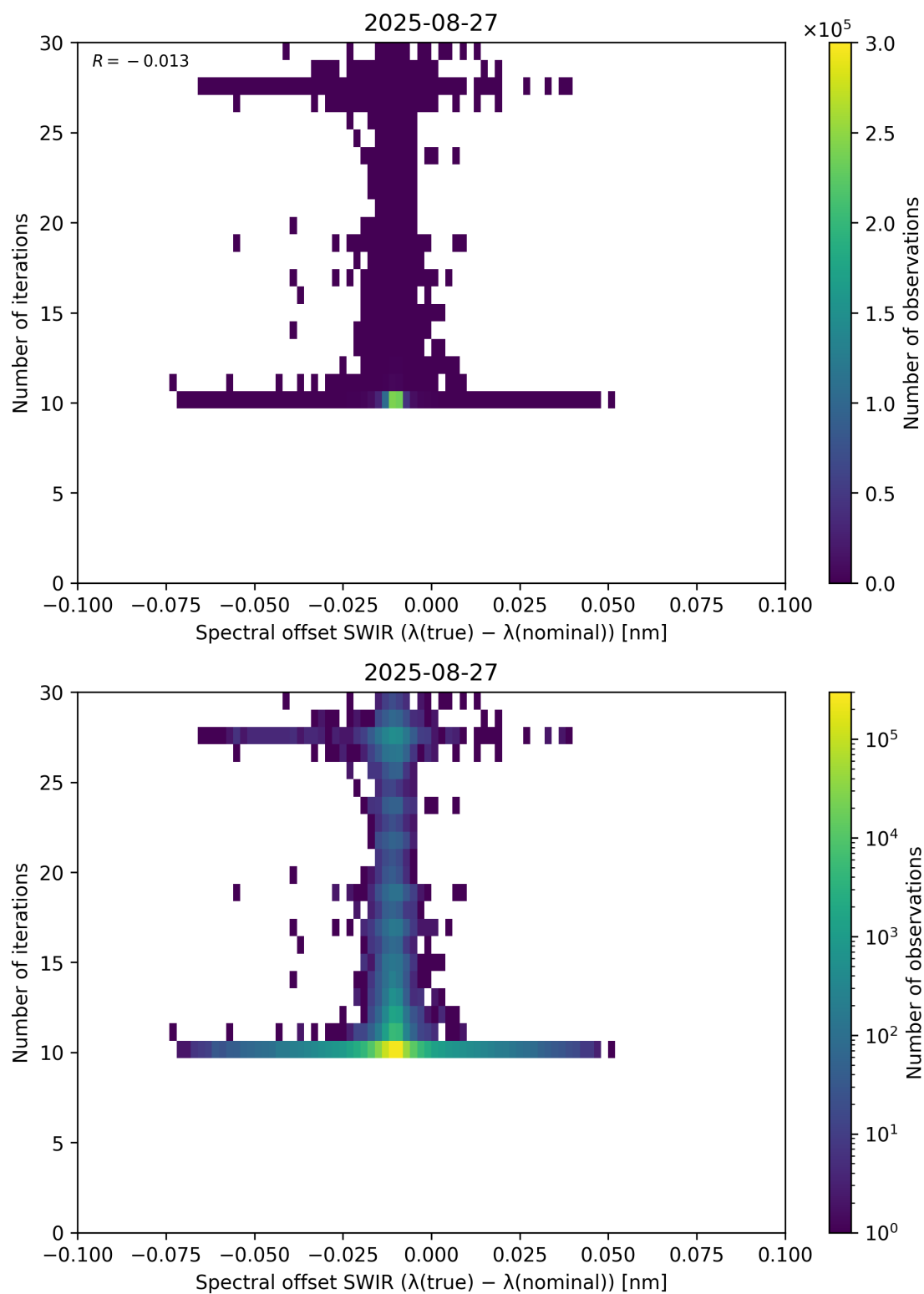
Figure 121: Scatter density plot of “Spectral offset SWIR ( \lambda_{\text{true}} - \lambda_{\text{nominal}} )” against “Number of iterations” for 2025-08-26 to 2025-08-28.
