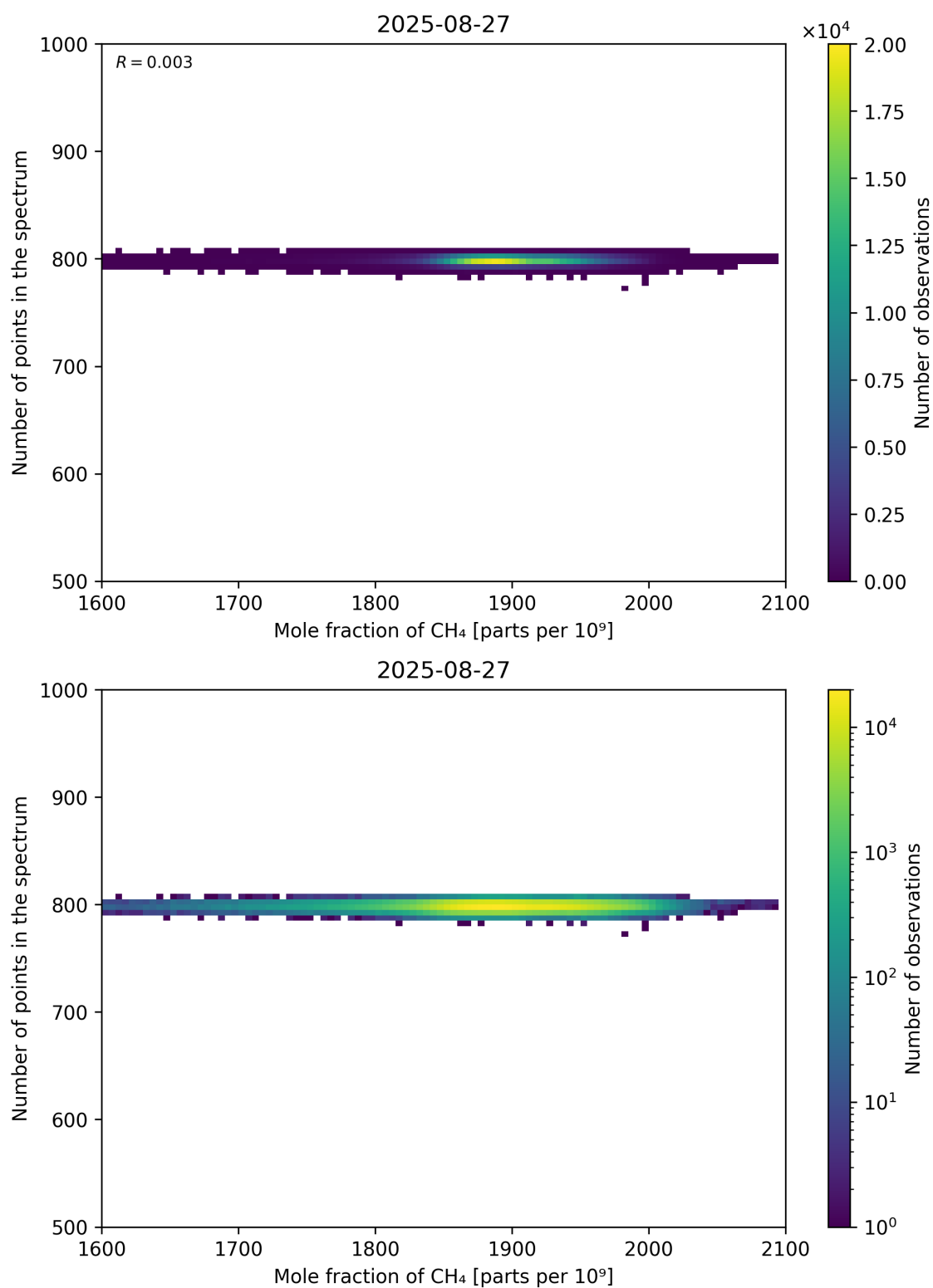
Figure 77: Scatter density plot of “Mole fraction of CH 4 ” against “Number of points in the spectrum” for 2025-08-26 to 2025-08-28.
