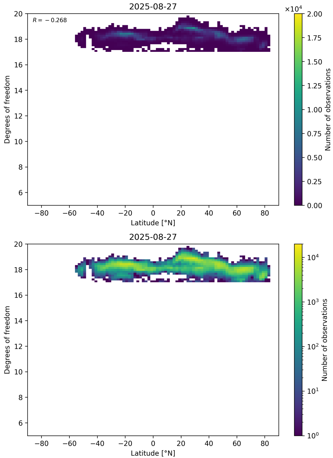
Figure 55: Scatter density plot of “Latitude” against “Degrees of freedom” for 2025-08-26 to 2025-08-28.
