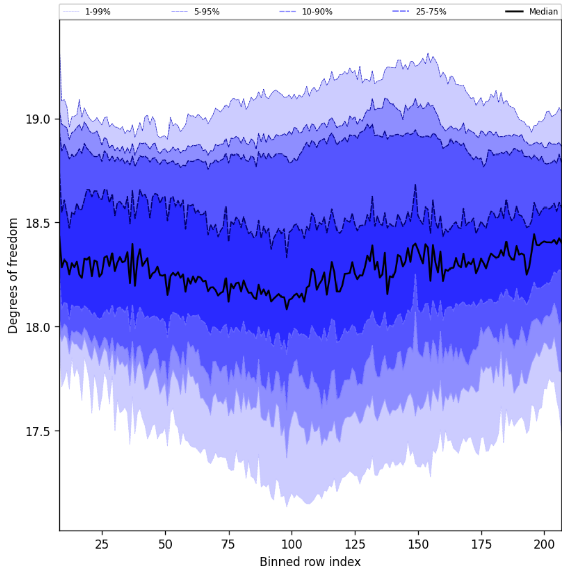
Figure 41: Along track statistics of “Degrees of freedom” for 2025-08-26 to 2025-08-28
