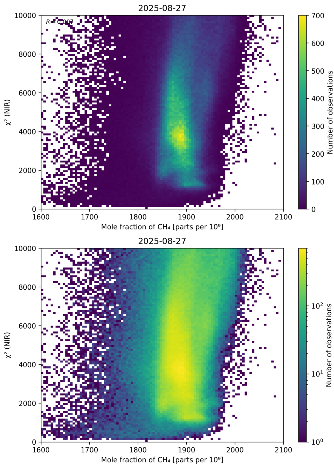
Figure 70: Scatter density plot of “Mole fraction of CH 4 ” against “ \chi^2 (NIR)” for 2025-08-26 to 2025-08-28.
