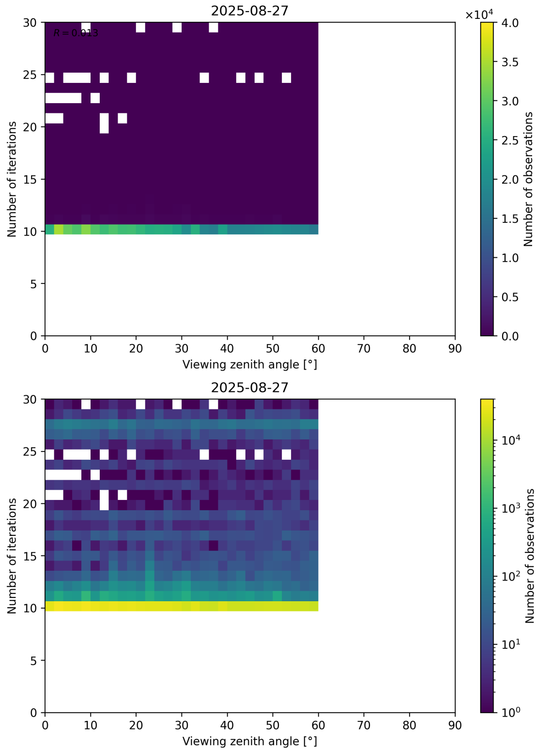
Figure 113: Scatter density plot of “Viewing zenith angle” against “Number of iterations” for 2025-08-26 to 2025-08-28.
