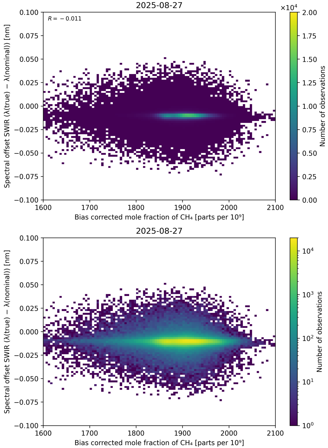
Figure 69: Scatter density plot of “Bias corrected mole fraction of CH 4 ” against “Spectral offset SWIR ( \lambda_{\text{true}} - \lambda_{\text{nominal}} )” for 2025-08-26 to 2025-08-28.
