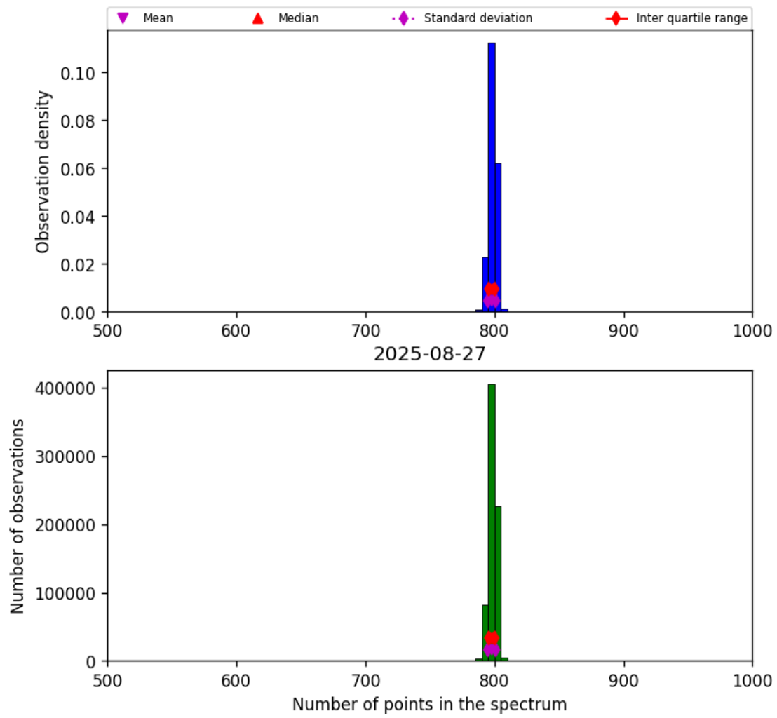
Figure 26: Histogram of “Number of points in the spectrum” for 2025-08-26 to 2025-08-28
