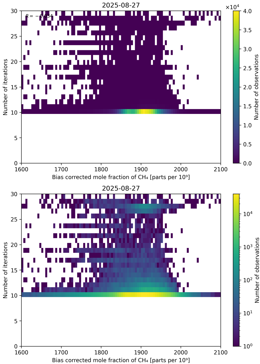
Figure 67: Scatter density plot of “Bias corrected mole fraction of CH 4 ” against “Number of iterations” for 2025-08-26 to 2025-08-28.
