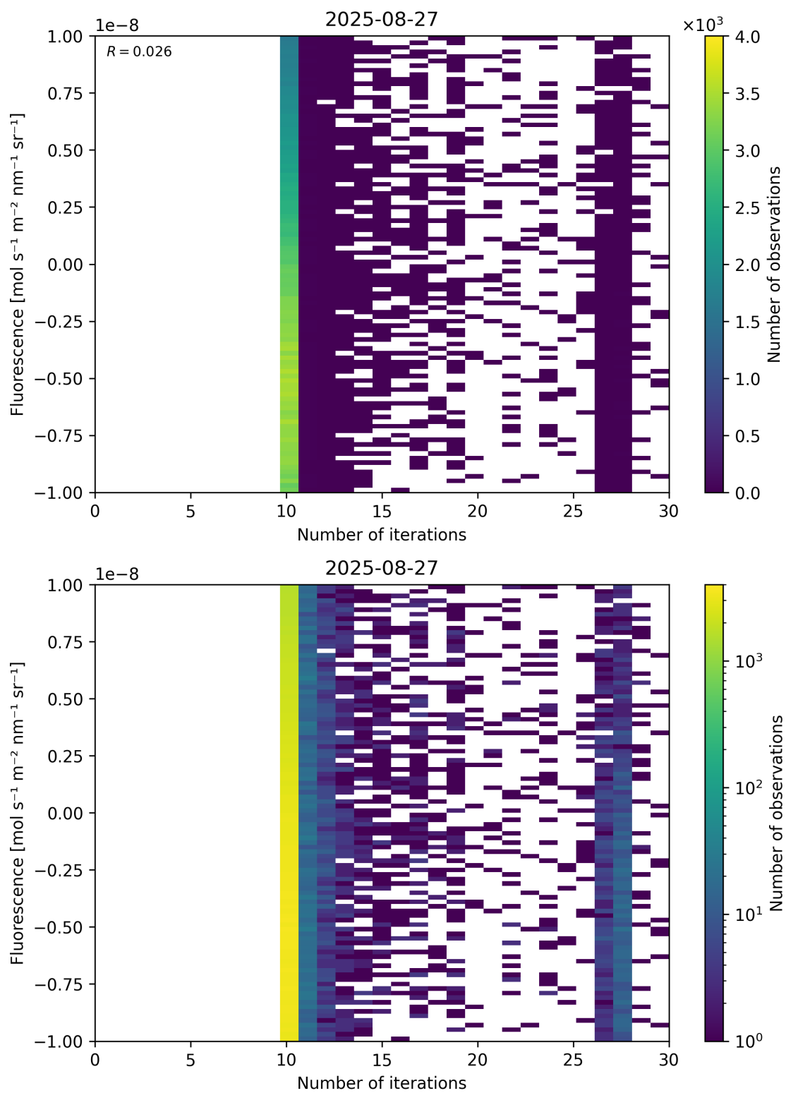
Figure 87: Scatter density plot of “Number of iterations” against “Fluorescence” for 2025-08-26 to 2025-08-28.
