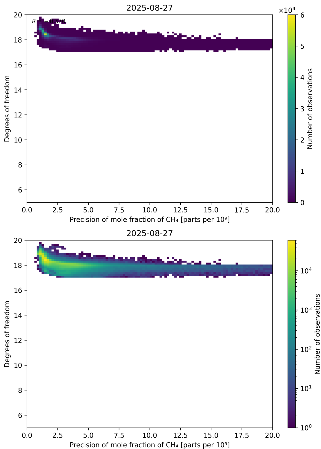
Figure 80: Scatter density plot of “Precision of mole fraction of CH 4 ” against “Degrees of freedom” for 2025-08-26 to 2025-08-28.
