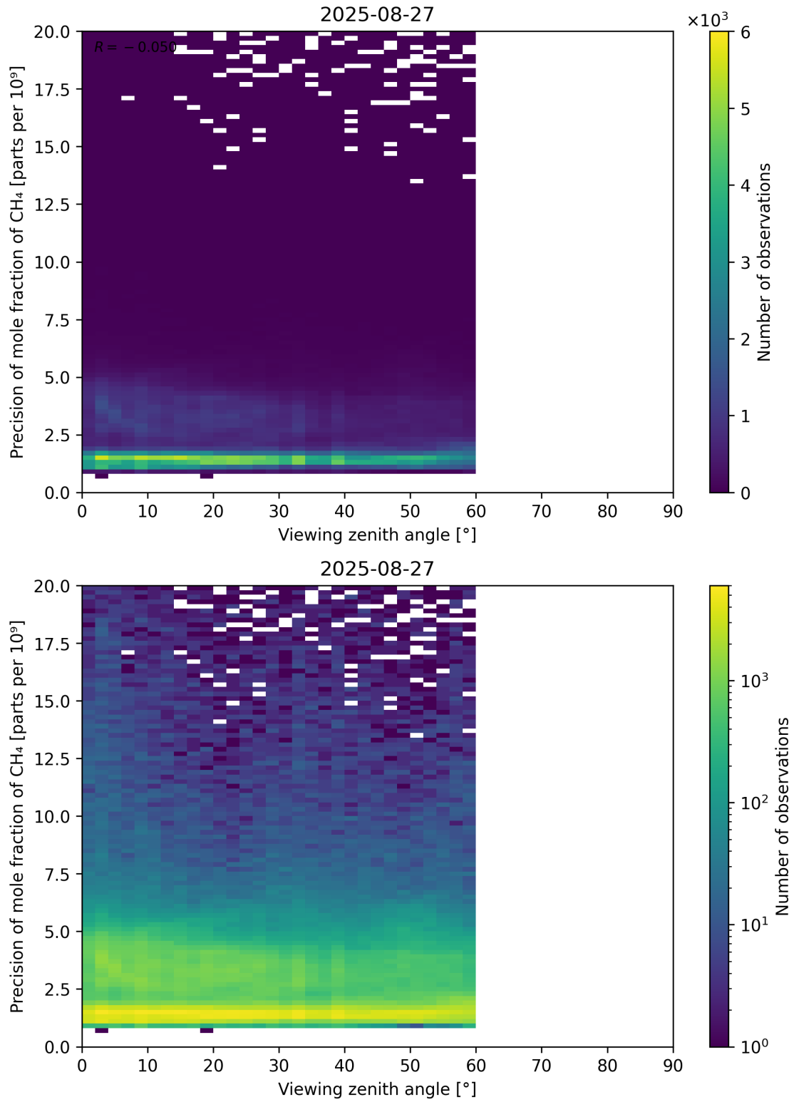
Figure 112: Scatter density plot of “Viewing zenith angle” against “Precision of mole fraction of CH 4 ” for 2025-08-26 to 2025-08-28.
