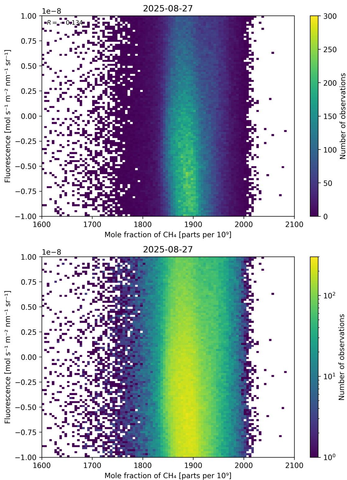
Figure 73: Scatter density plot of “Mole fraction of \text{CH}_4 ” against “Fluorescence” for 2025-08-26 to 2025-08-28.
