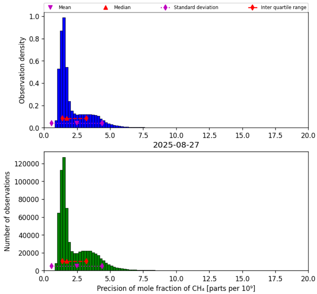
Figure 24: Histogram of “Precision of mole fraction of CH 4 ” for 2025-08-26 to 2025-08-28
