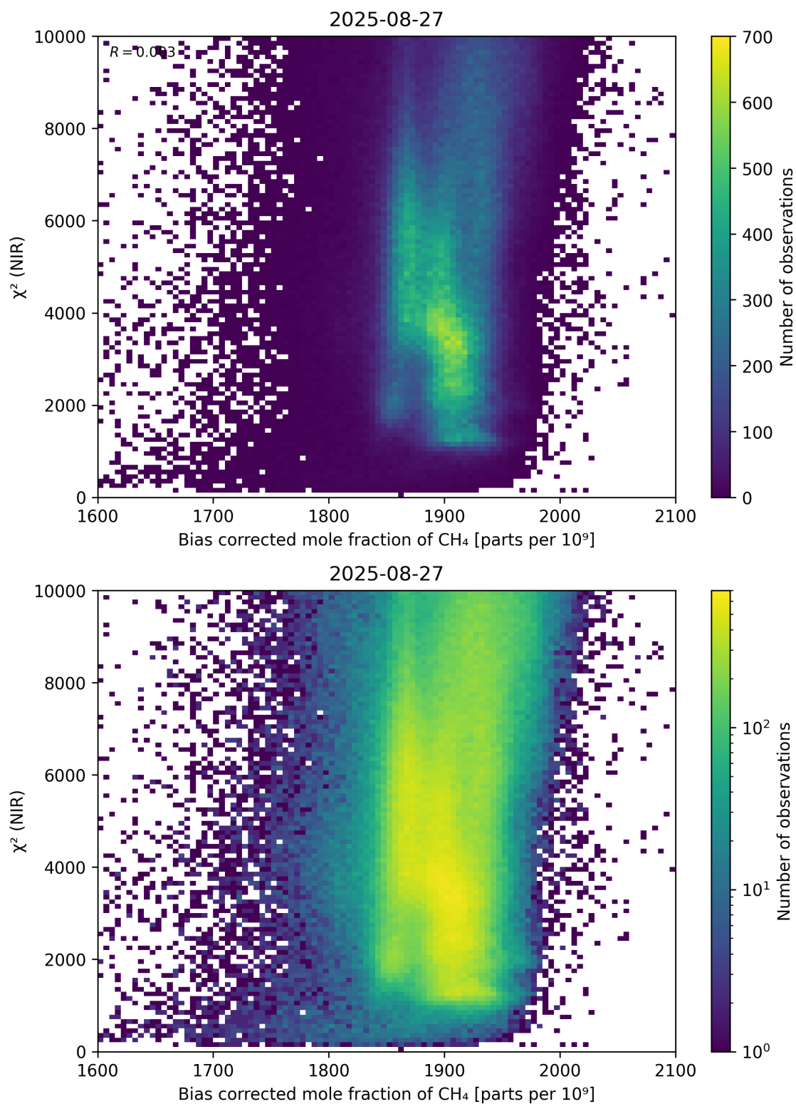
Figure 63: Scatter density plot of “Bias corrected mole fraction of CH 4 ” against “ \chi^2 (NIR)” for 2025-08-26 to 2025-08-28.
