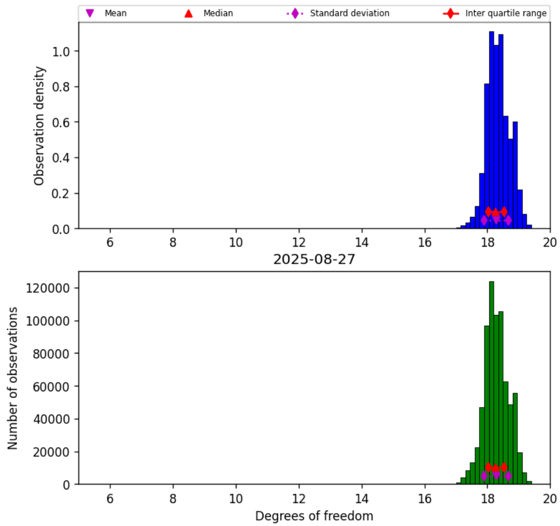
Figure 30: Histogram of “Degrees of freedom” for 2025-08-26 to 2025-08-28
