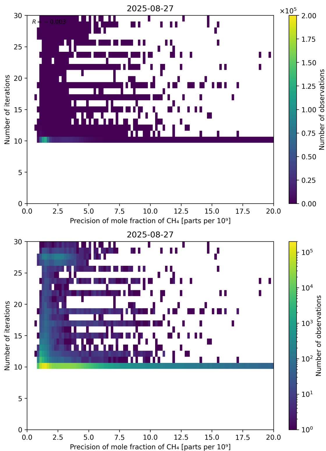
Figure 83: Scatter density plot of “Precision of mole fraction of CH 4 ” against “Number of iterations” for 2025-08-26 to 2025-08-28.
