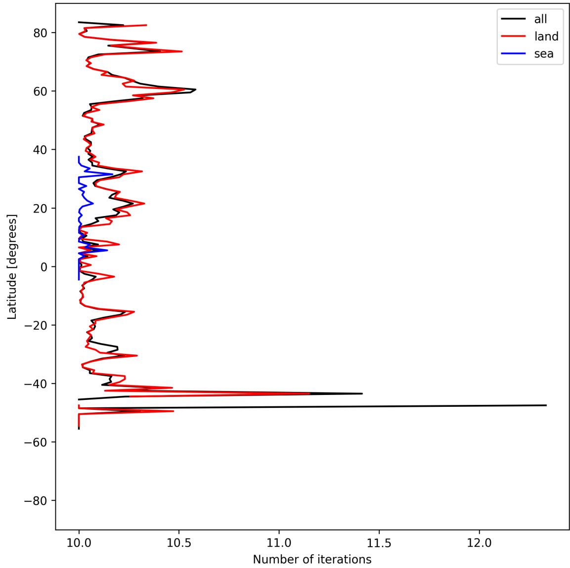
Figure 20: Zonal average of “Number of iterations” for 2025-08-26 to 2025-08-28.
