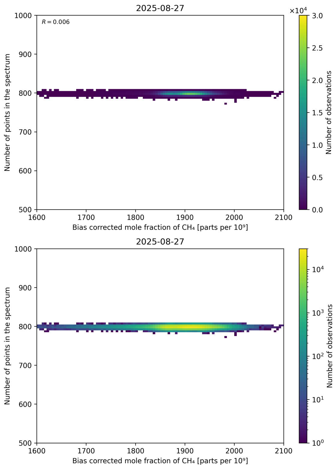
Figure 68: Scatter density plot of “Bias corrected mole fraction of CH 4 ” against “Number of points in the spectrum” for 2025-08-26 to 2025-08-28.
