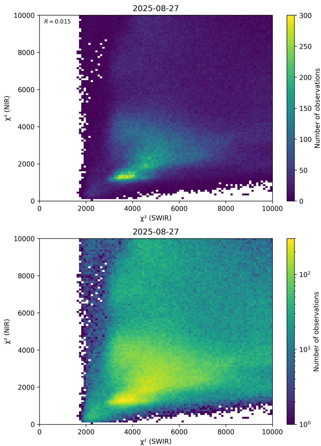
Figure 47: Scatter density plot of “ \chi^2 (SWIR)” against “ \chi^2 (NIR)” for 2025-08-26 to 2025-08-28.
