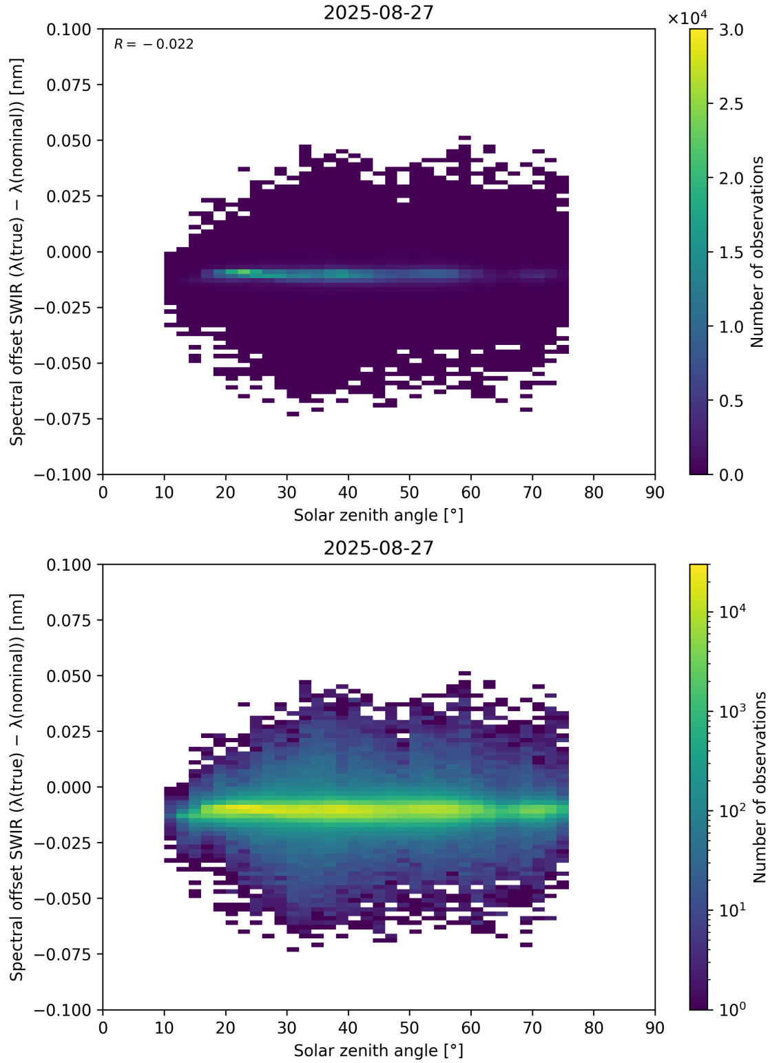
Figure 104: Scatter density plot of “Solar zenith angle” against “Spectral offset SWIR ( \lambda_{\text{true}} - \lambda_{\text{nominal}} )” for 2025-08-26 to 2025-08-28.
