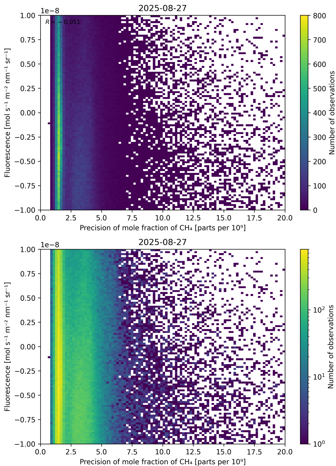
Figure 81: Scatter density plot of “Precision of mole fraction of CH 4 ” against “Fluorescence” for 2025-08-26 to 2025-08-28.
