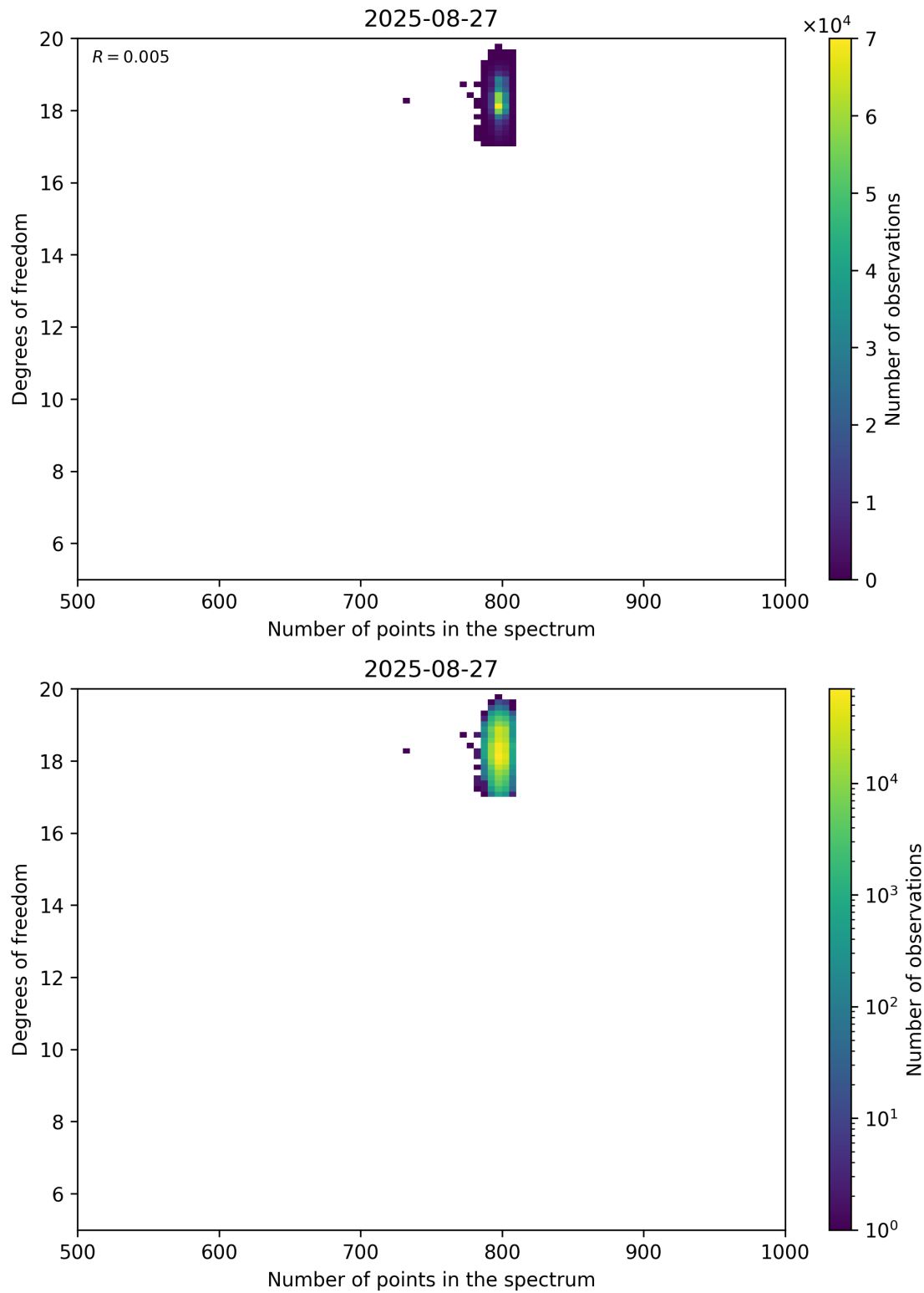
Figure 90: Scatter density plot of “Number of points in the spectrum” against “Degrees of freedom” for 2025-08-26 to 2025-08-28.
