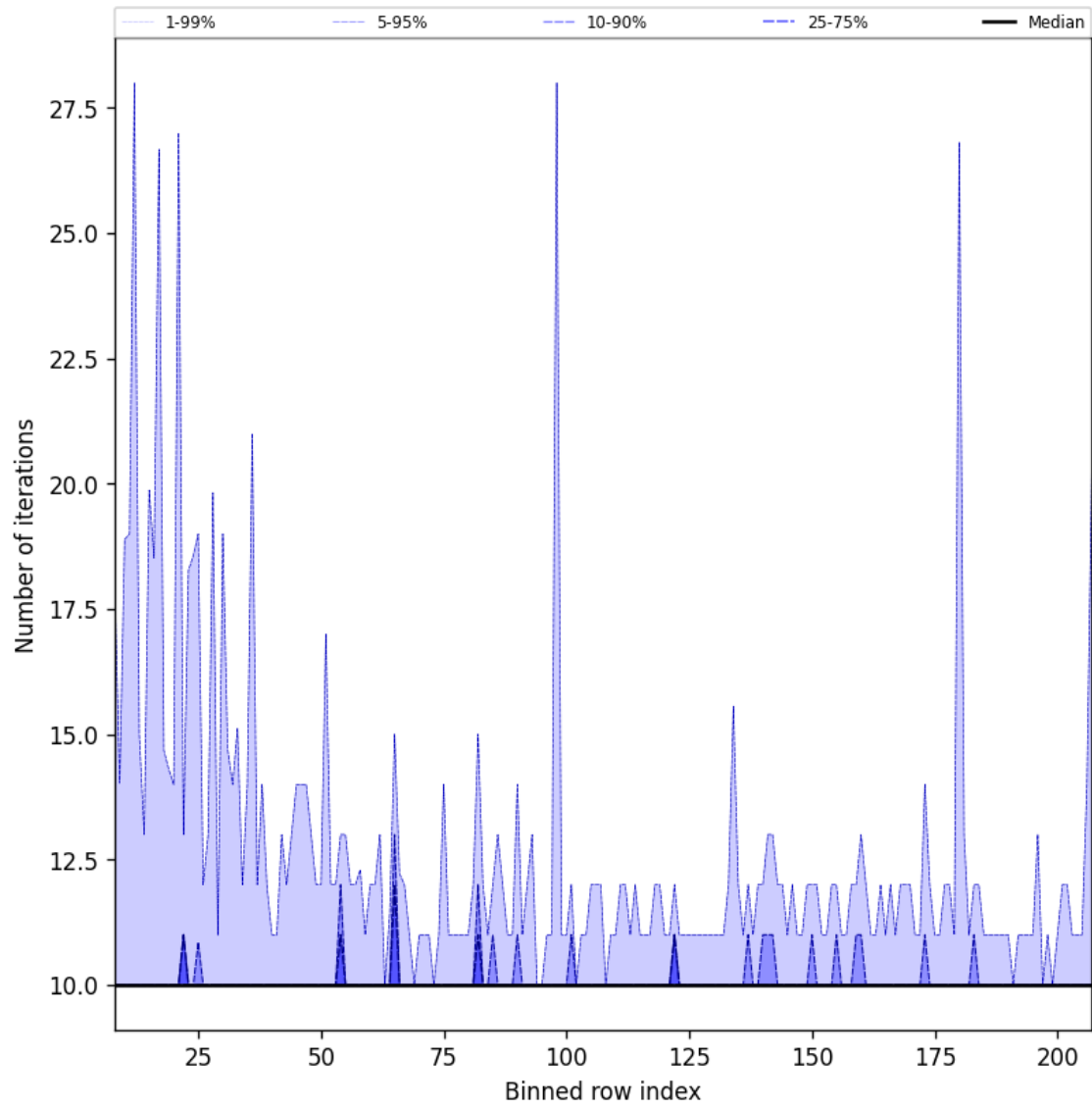
Figure 42: Along track statistics of “Number of iterations” for 2025-08-26 to 2025-08-28
