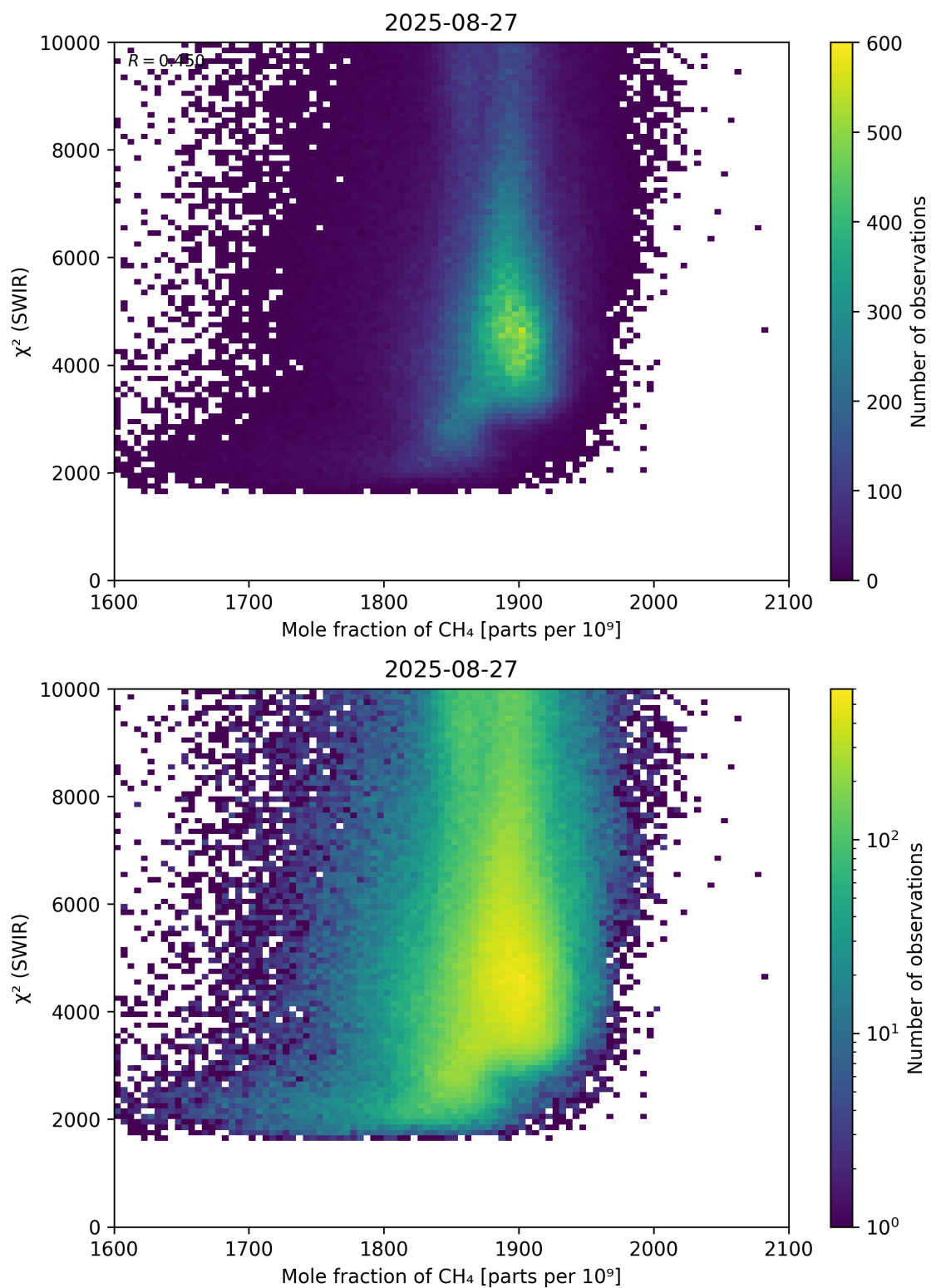
Figure 71: Scatter density plot of “Mole fraction of \text{CH}_4 ” against “ \chi^2 (SWIR)” for 2025-08-26 to 2025-08-28.
