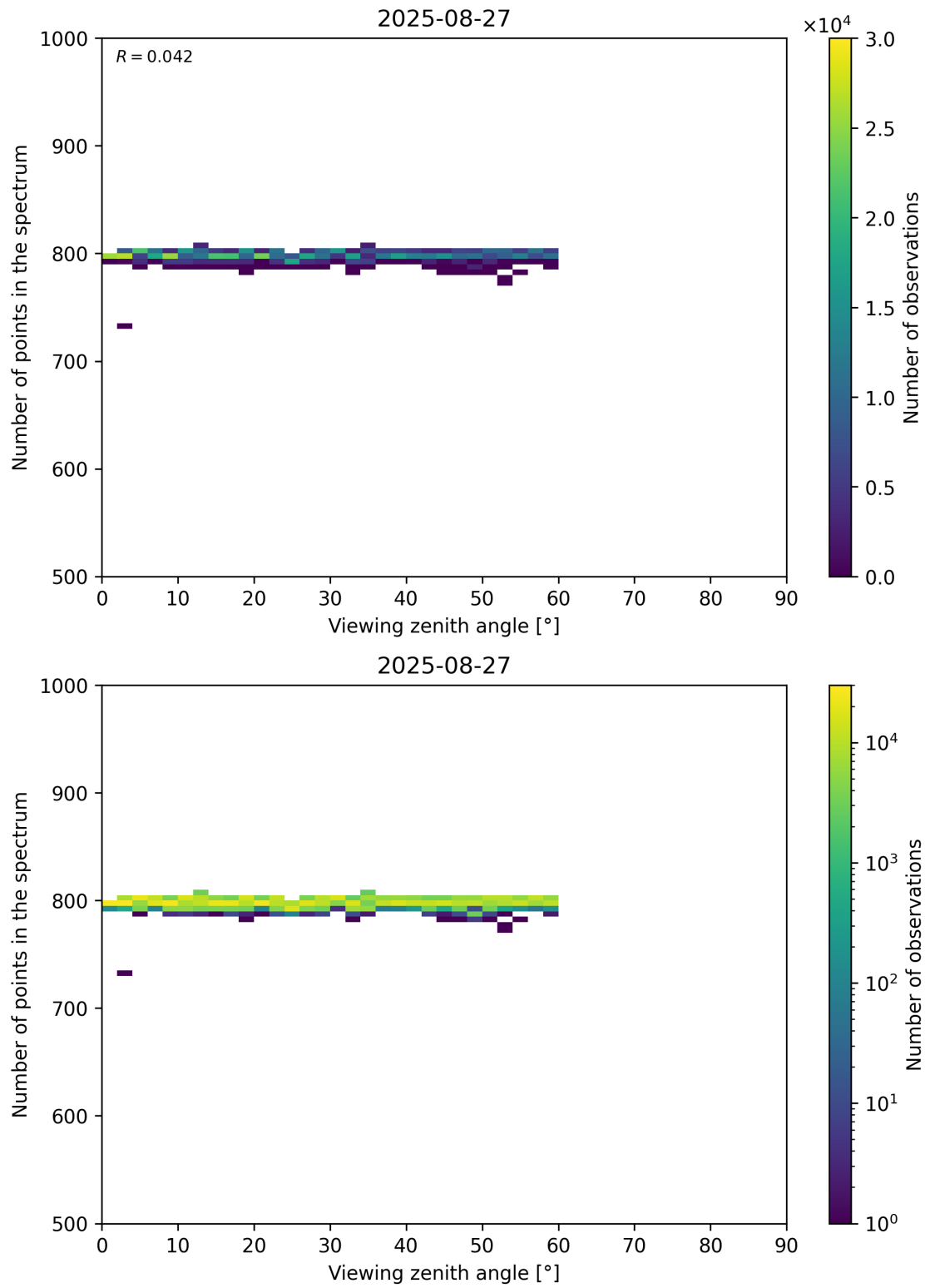
Figure 114: Scatter density plot of “Viewing zenith angle” against “Number of points in the spectrum” for 2025-08-26 to 2025-08-28.
