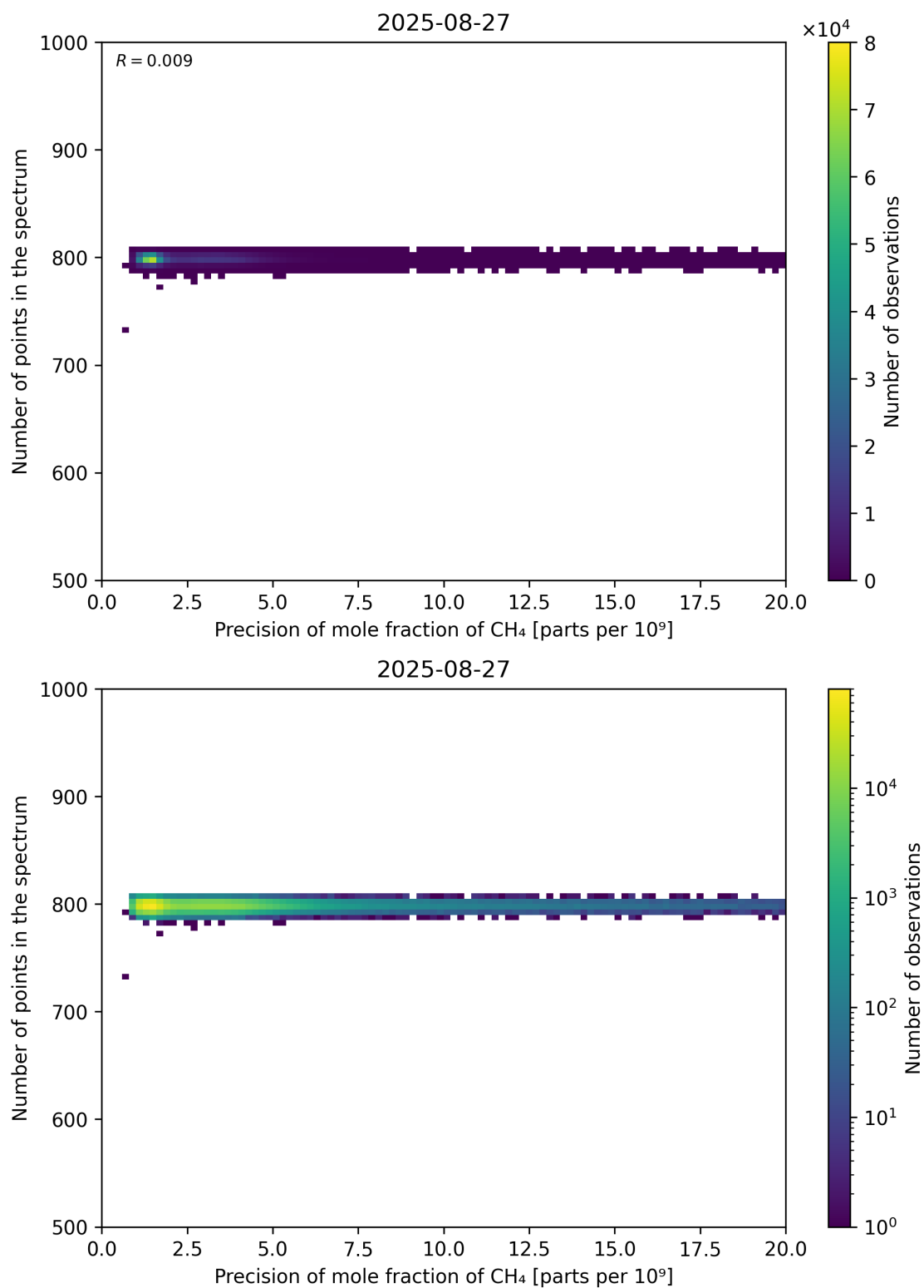
Figure 84: Scatter density plot of “Precision of mole fraction of CH 4 ” against “Number of points in the spectrum” for 2025-08-26 to 2025-08-28.
