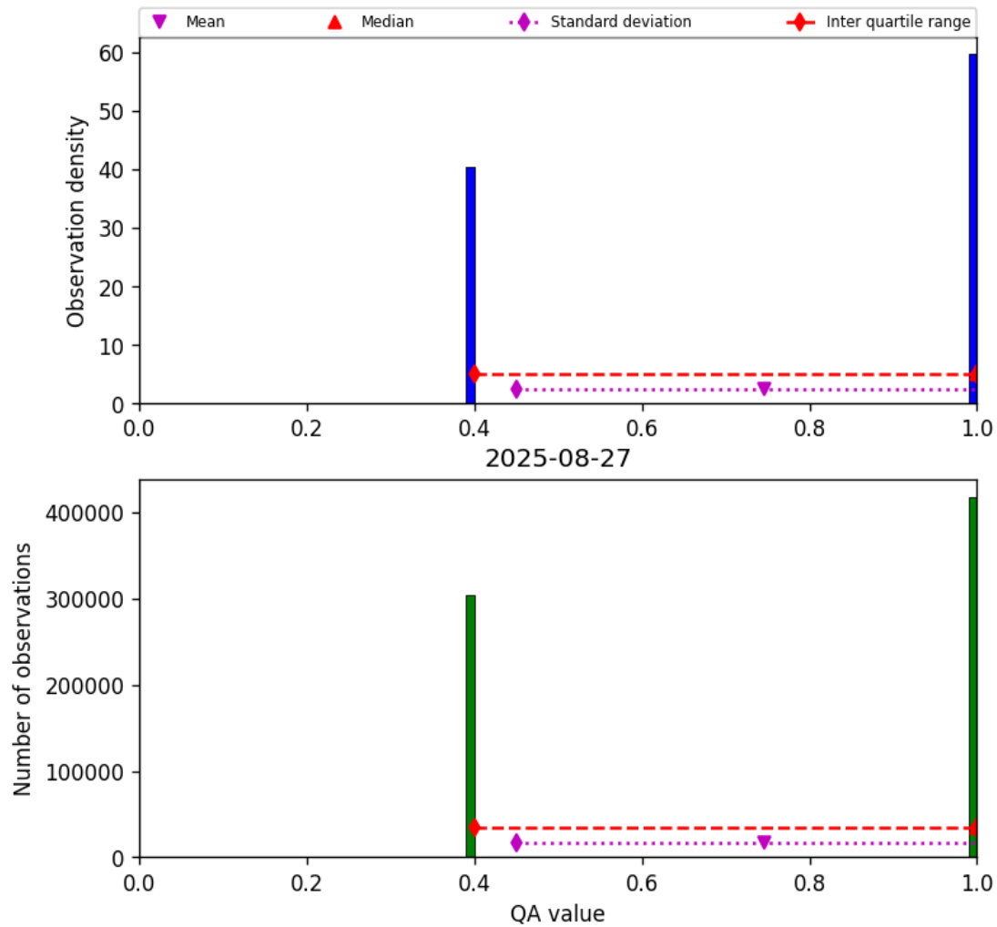
Figure 22: Histogram of “QA value” for 2025-08-26 to 2025-08-28
