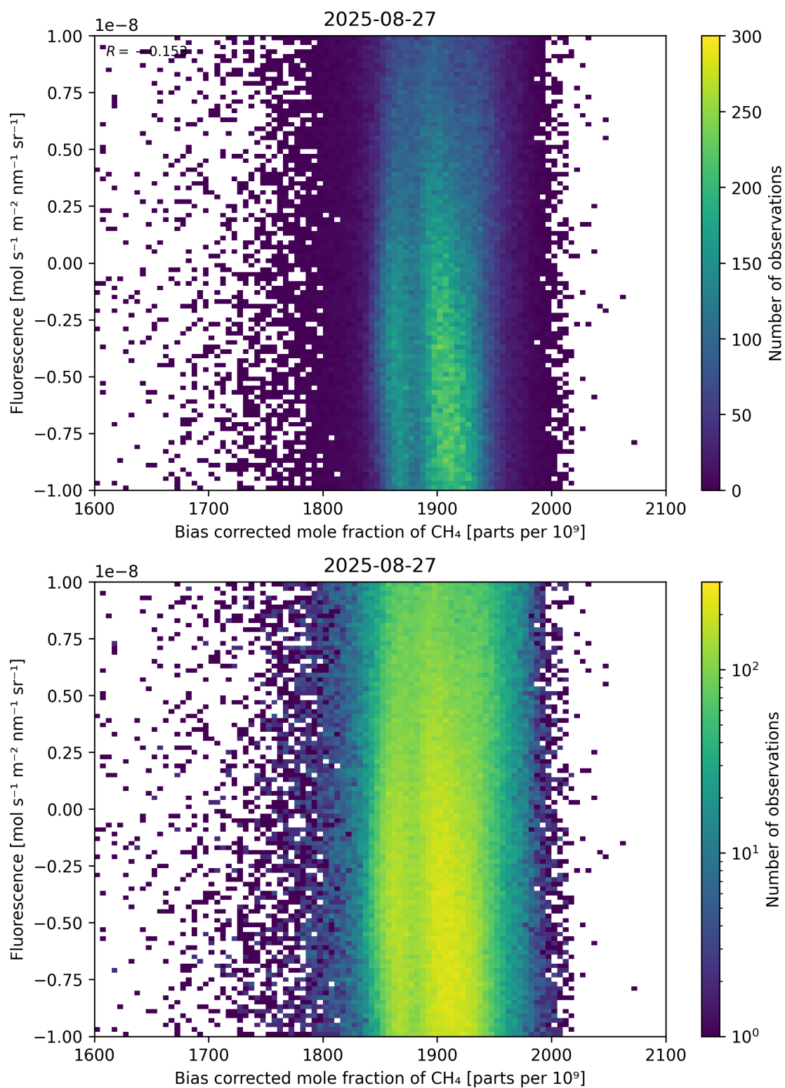
Figure 66: Scatter density plot of “Bias corrected mole fraction of \text{CH}_4 ” against “Fluorescence” for 2025-08-26 to 2025-08-28.
