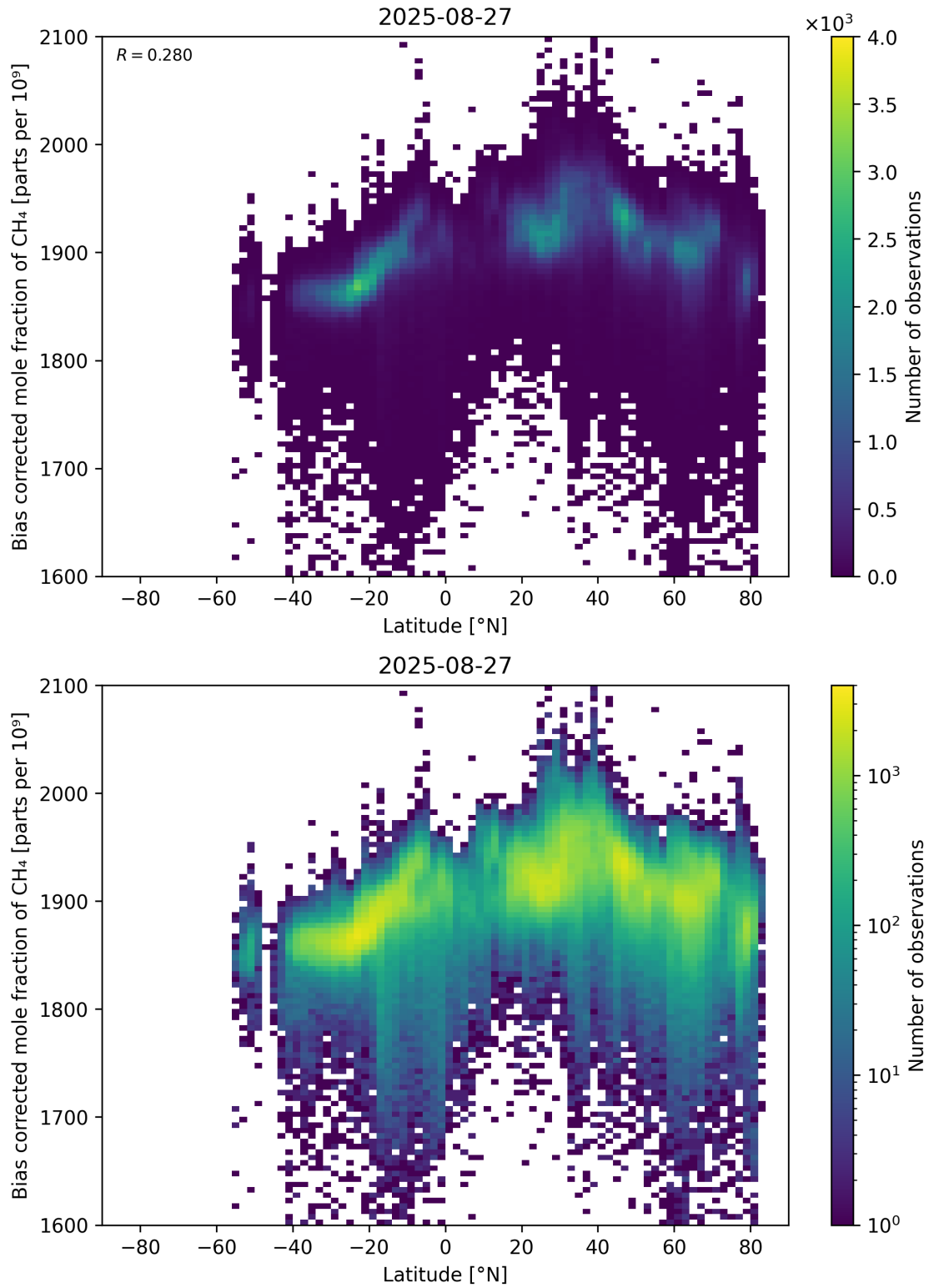
Figure 58: Scatter density plot of “Latitude” against “Bias corrected mole fraction of \text{CH}_4 ” for 2025-08-26 to 2025-08-28.
