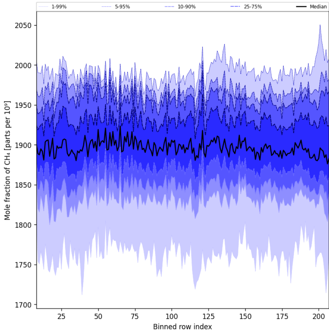
Figure 34: Along track statistics of “Mole fraction of CH 4 ” for 2025-08-26 to 2025-08-28
