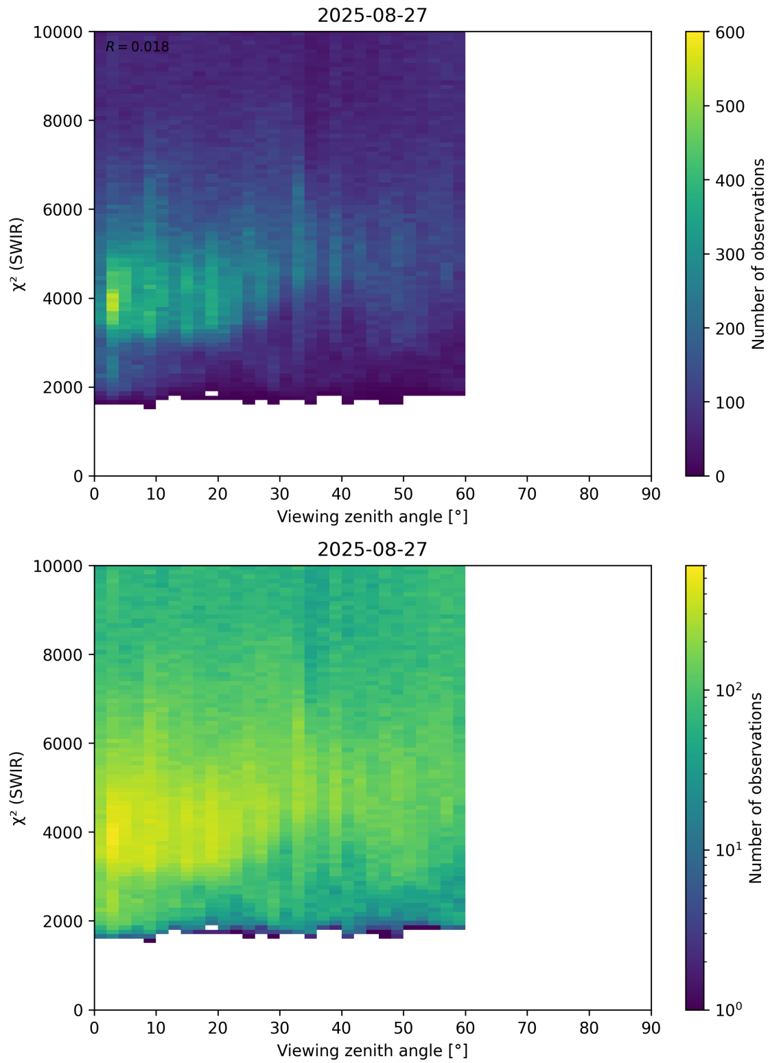
Figure 106: Scatter density plot of “Viewing zenith angle” against “ \chi^2 (SWIR)” for 2025-08-26 to 2025-08-28.
