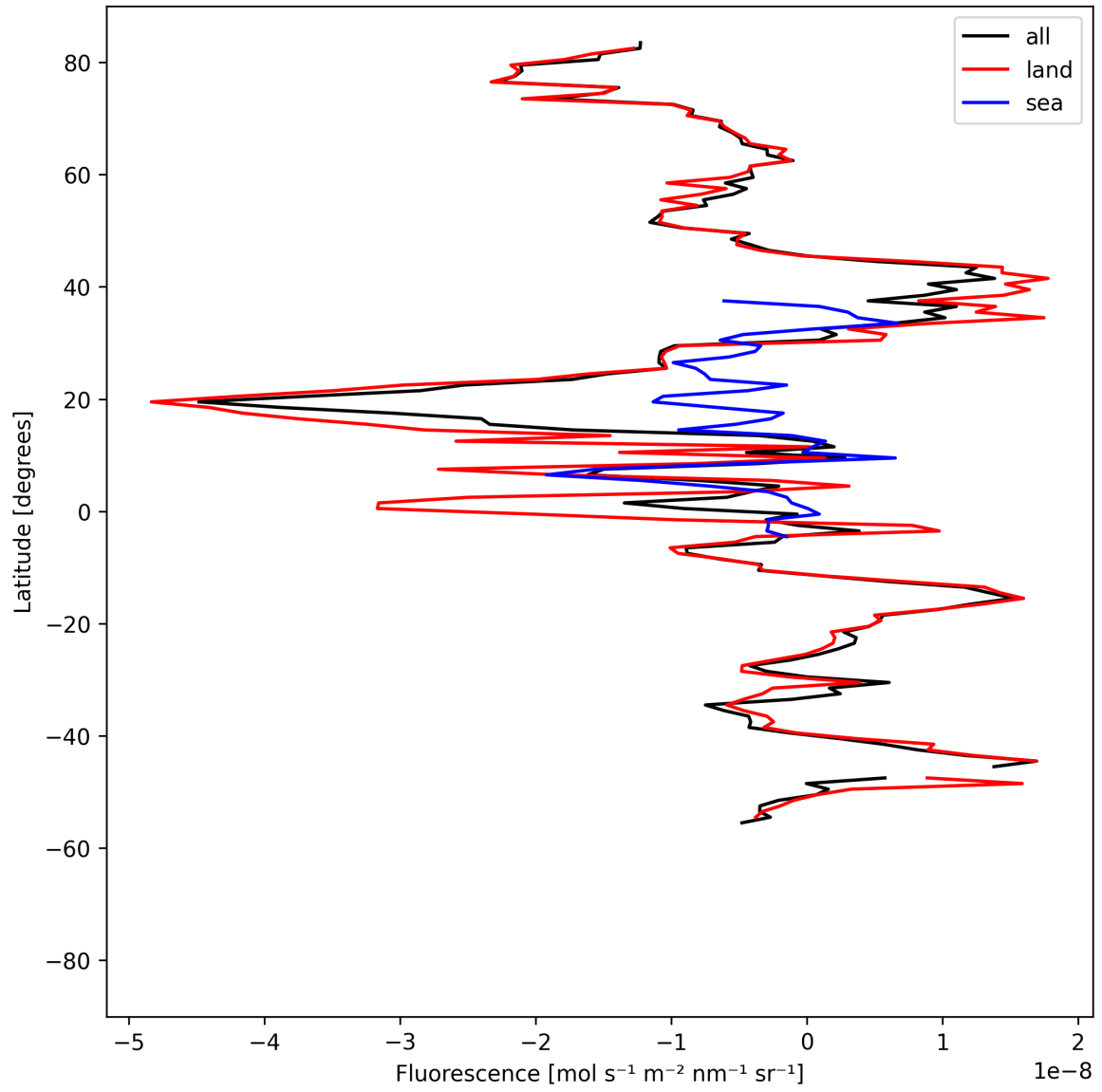
Figure 21: Zonal average of “Fluorescence” for 2025-08-26 to 2025-08-28.
