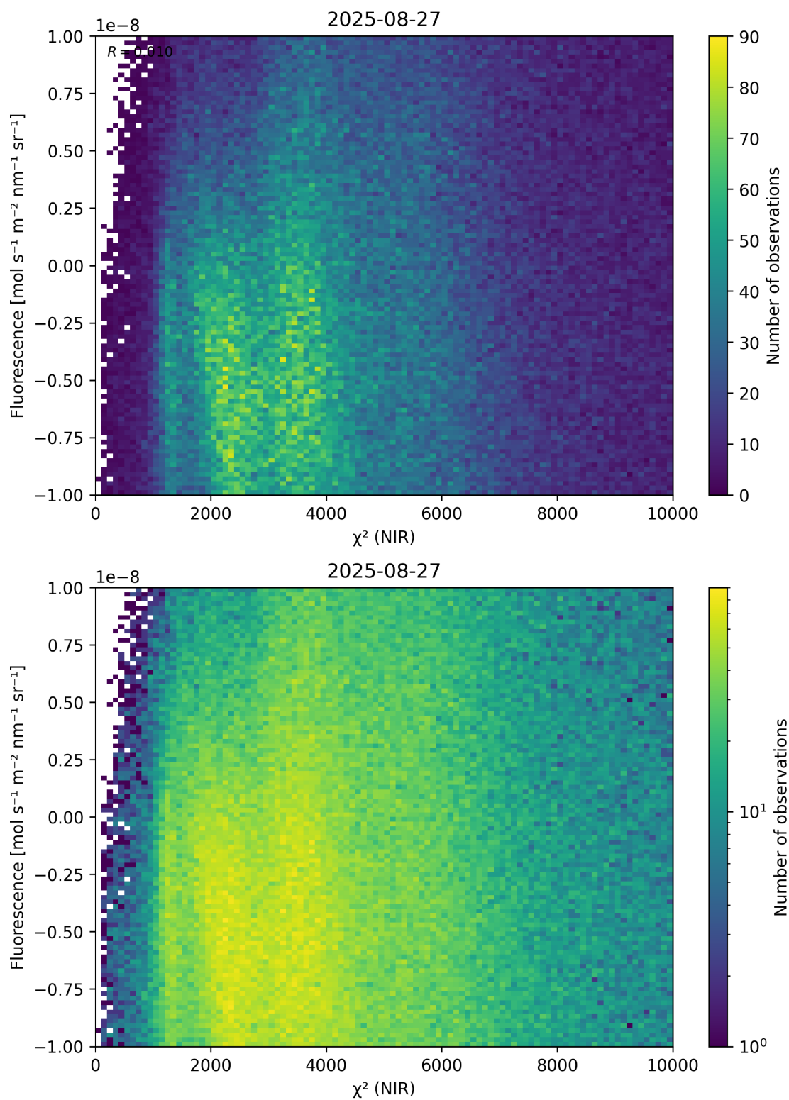
Figure 45: Scatter density plot of “ \chi^2 (NIR)” against “Fluorescence” for 2025-08-26 to 2025-08-28.
