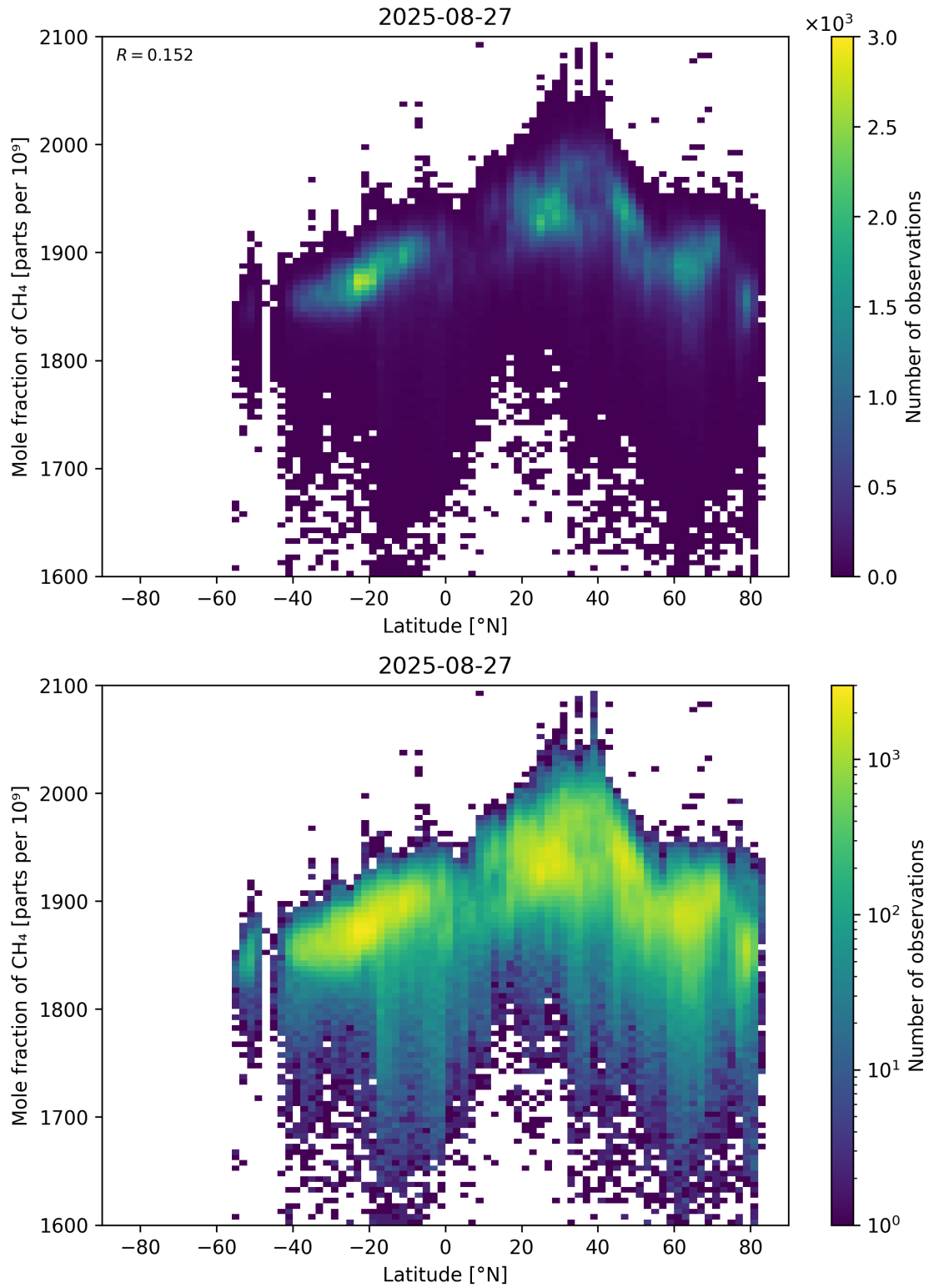
Figure 57: Scatter density plot of “Latitude” against “Mole fraction of CH 4 ” for 2025-08-26 to 2025-08-28.
