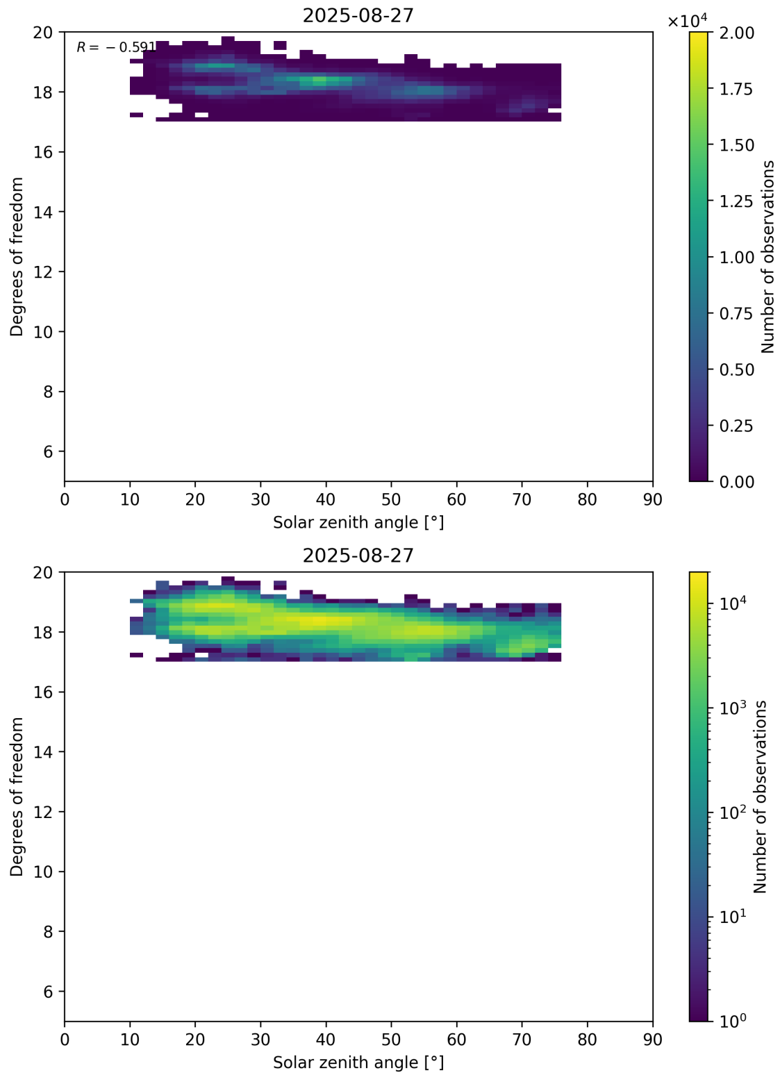
Figure 96: Scatter density plot of “Solar zenith angle” against “Degrees of freedom” for 2025-08-26 to 2025-08-28.
