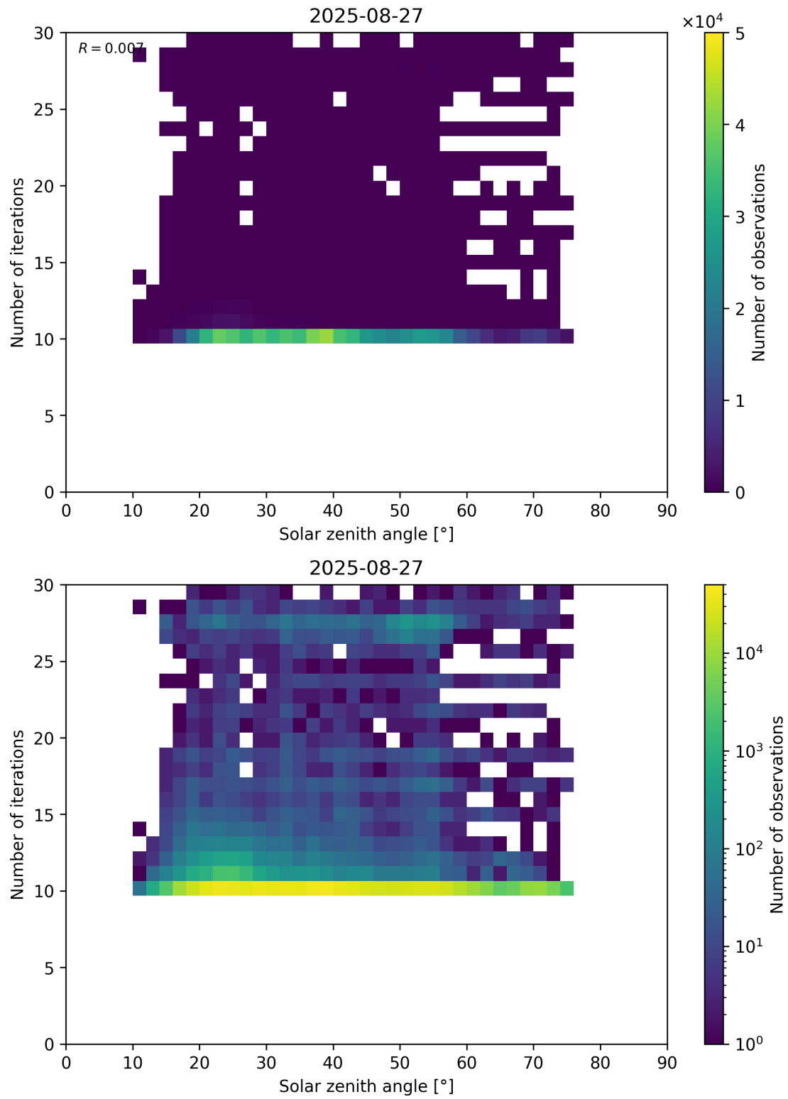
Figure 102: Scatter density plot of “Solar zenith angle” against “Number of iterations” for 2025-08-26 to 2025-08-28.
