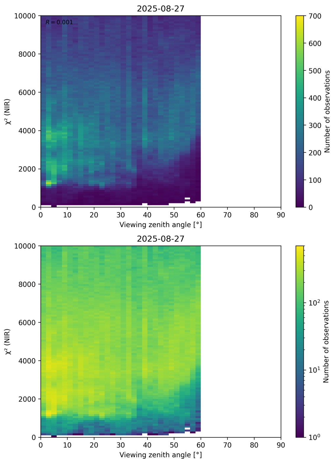
Figure 105: Scatter density plot of “Viewing zenith angle” against “ \chi^2 (NIR)” for 2025-08-26 to 2025-08-28.
