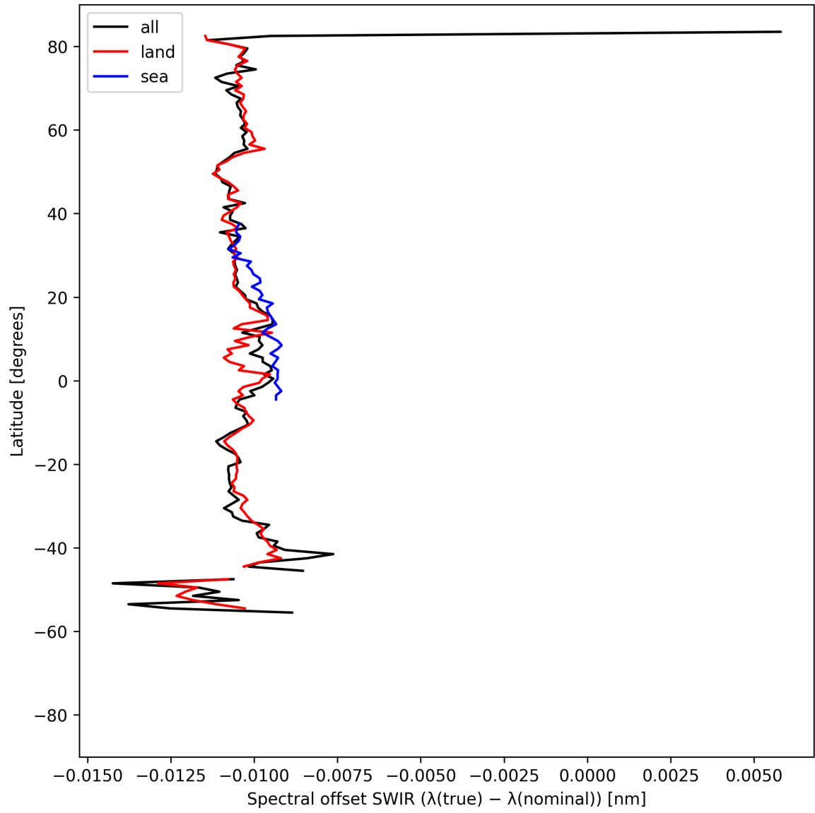
Figure 16: Zonal average of “Spectral offset SWIR ( \lambda_{\text{true}} - \lambda_{\text{nominal}} )” for 2025-08-26 to 2025-08-28.
