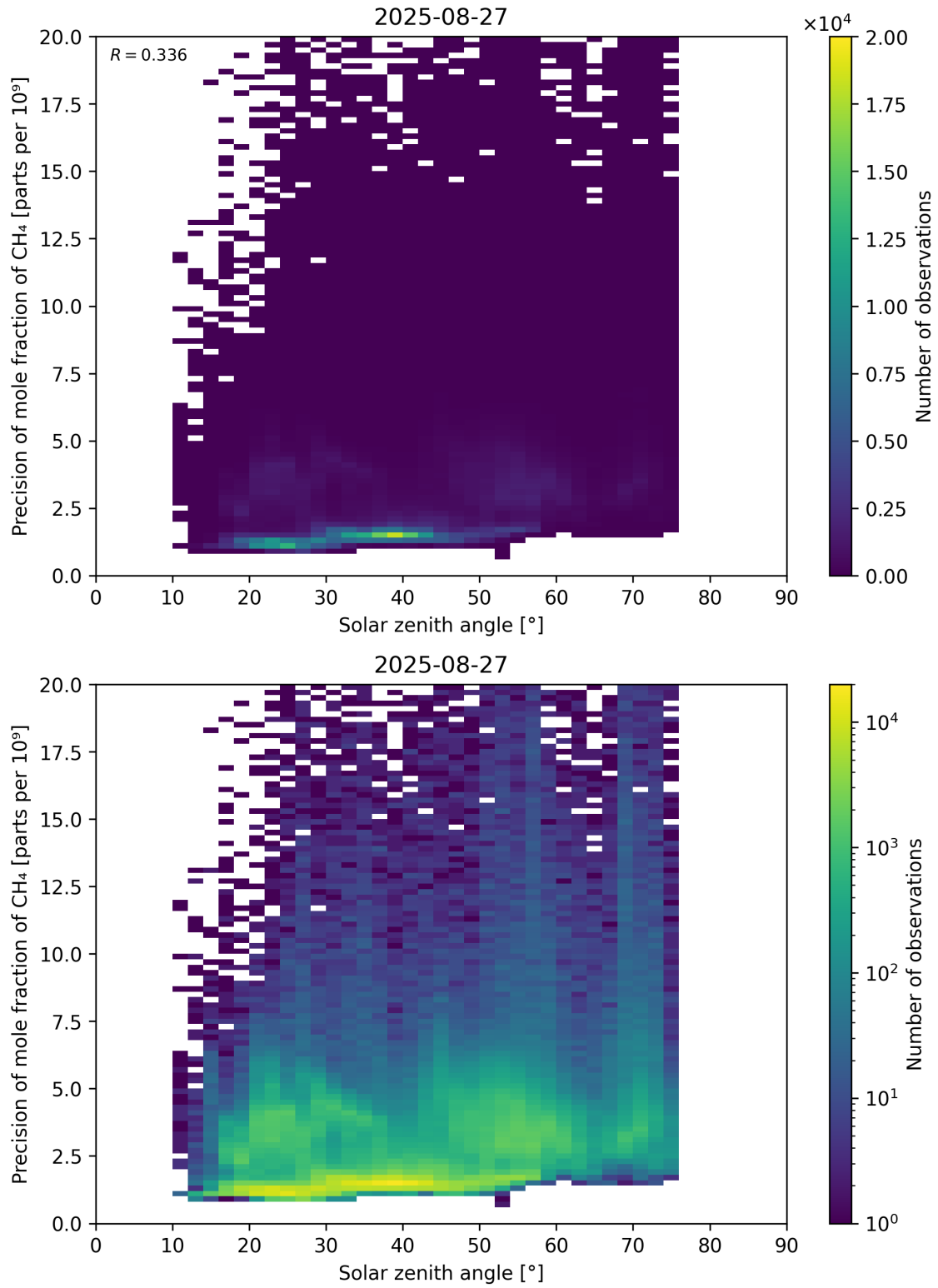
Figure 101: Scatter density plot of “Solar zenith angle” against “Precision of mole fraction of \text{CH}_4 ” for 2025-08-26 to 2025-08-28.
