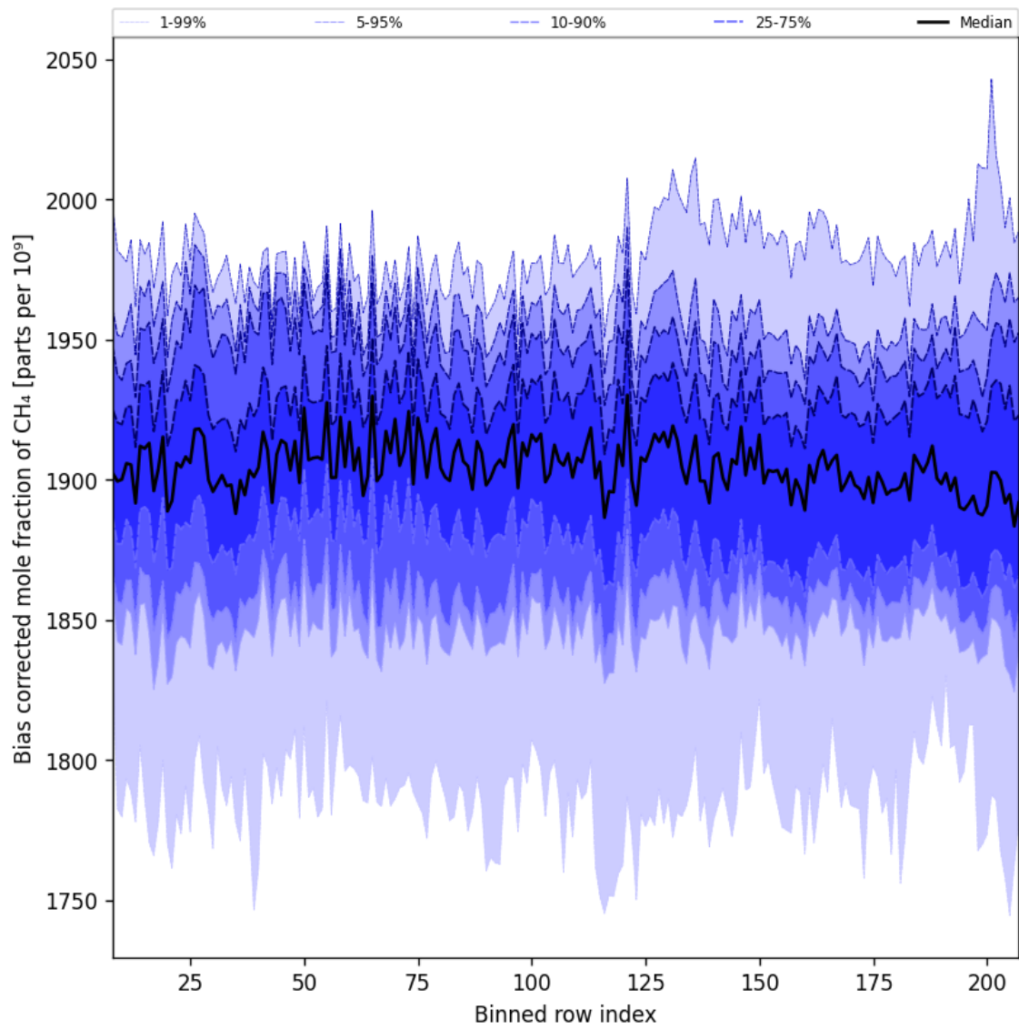
Figure 36: Along track statistics of “Bias corrected mole fraction of CH 4 ” for 2025-08-26 to 2025-08-28
