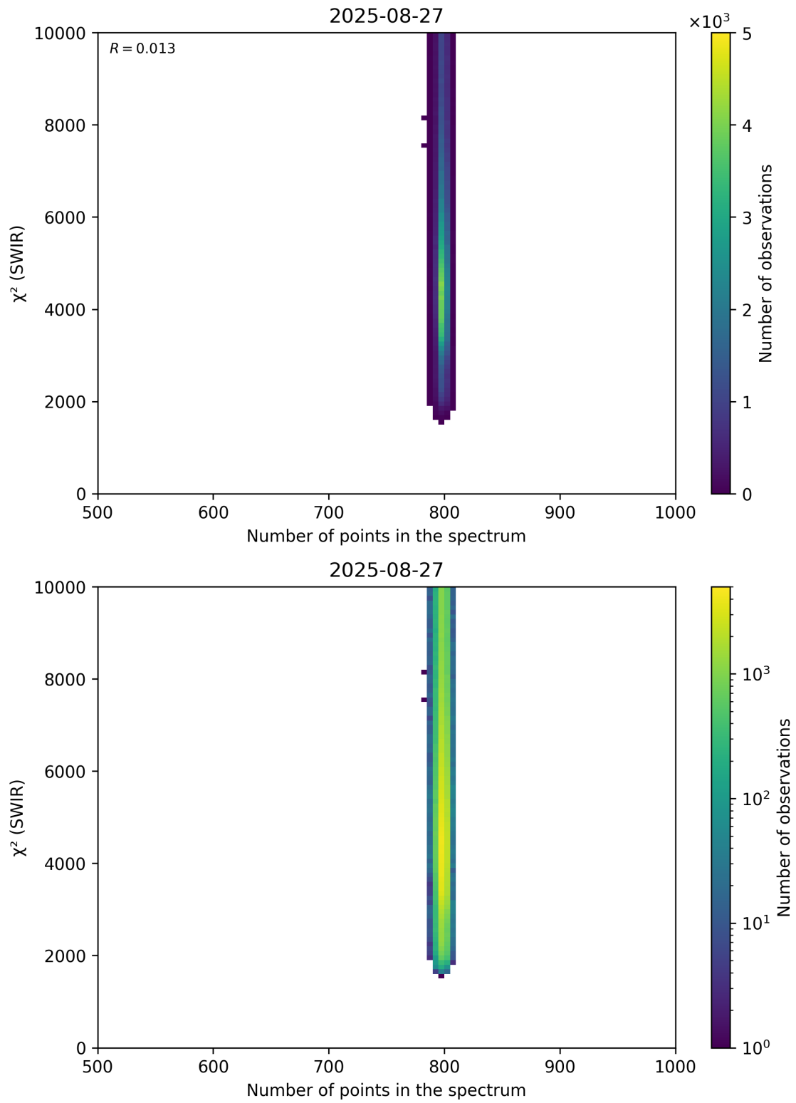
Figure 89: Scatter density plot of “Number of points in the spectrum” against “ \chi^2 (SWIR)” for 2025-08-26 to 2025-08-28.
