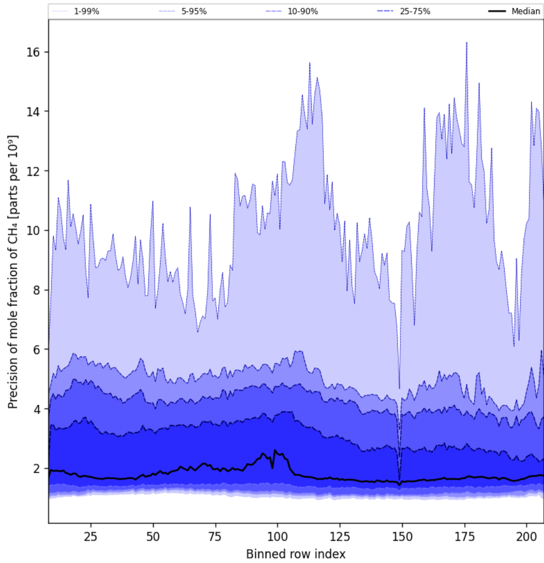
Figure 35: Along track statistics of “Precision of mole fraction of CH 4 ” for 2025-08-26 to 2025-08-28
