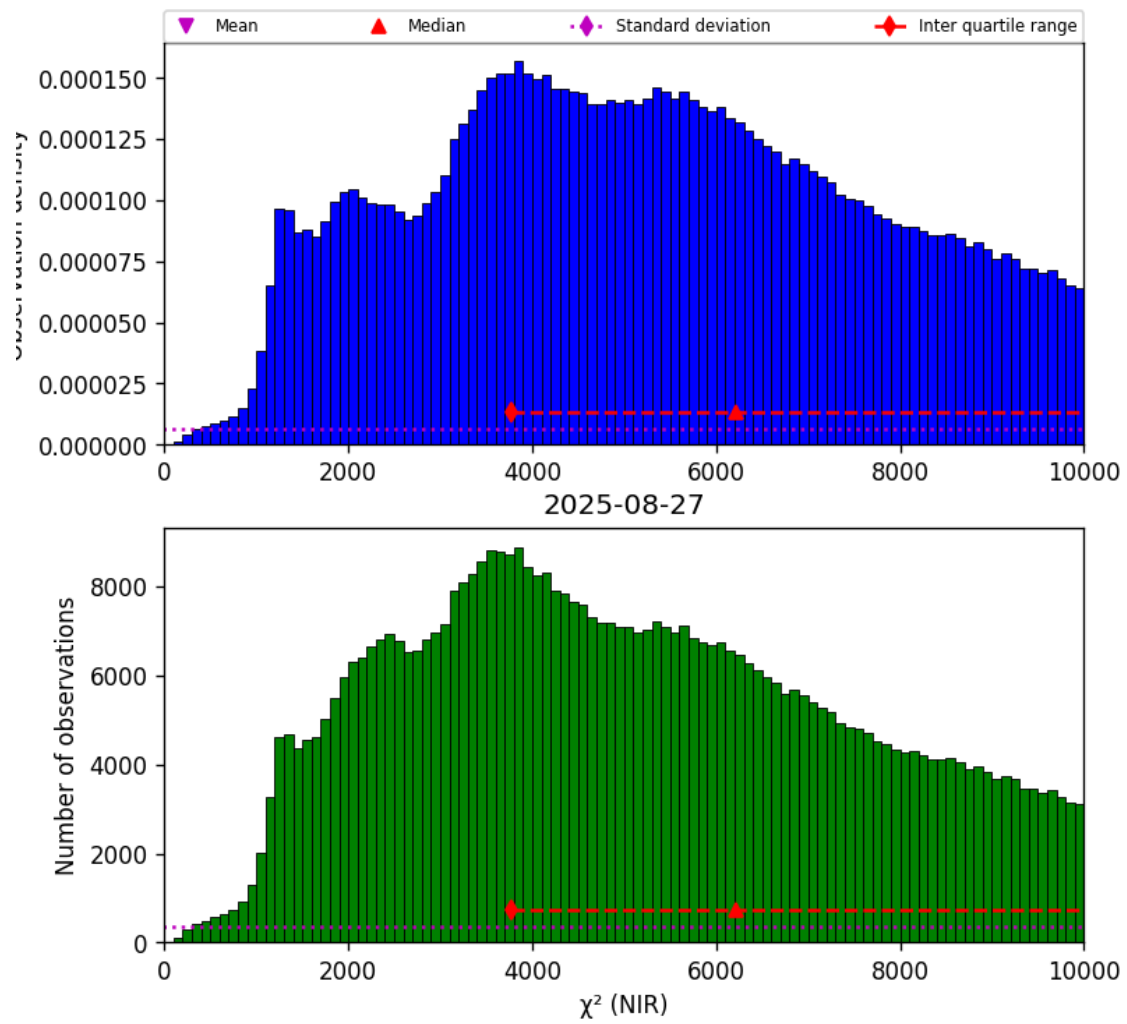
Figure 29: Histogram of “ \chi^2 (NIR)” for 2025-08-26 to 2025-08-28
