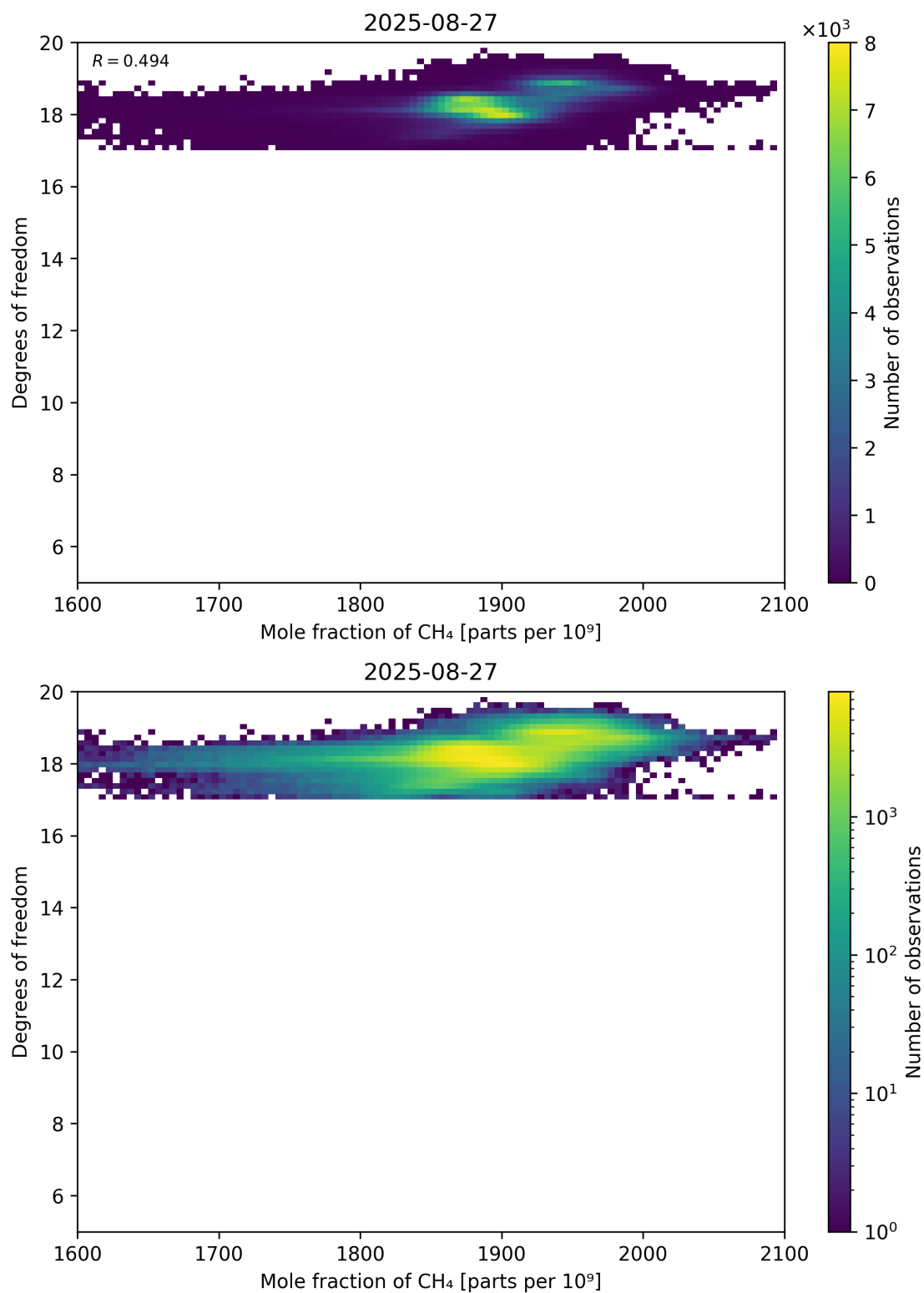
Figure 72: Scatter density plot of “Mole fraction of CH 4 ” against “Degrees of freedom” for 2025-08-26 to 2025-08-28.
