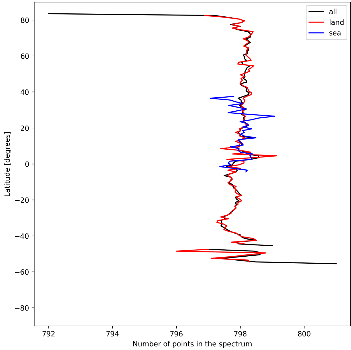
Figure 15: Zonal average of “Number of points in the spectrum” for 2025-08-26 to 2025-08-28.
