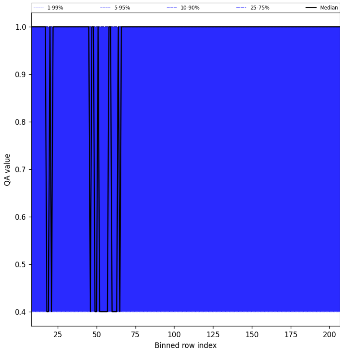
Figure 33: Along track statistics of “QA value” for 2025-08-26 to 2025-08-28
