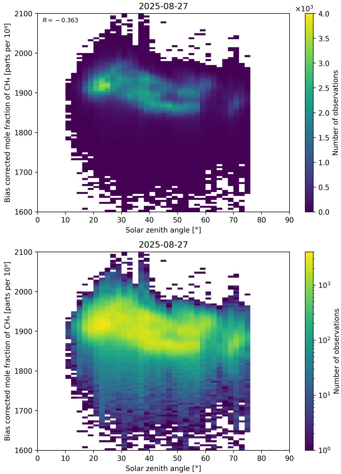
Figure 100: Scatter density plot of “Solar zenith angle” against “Bias corrected mole fraction of CH 4 ” for 2025-08-26 to 2025-08-28.
