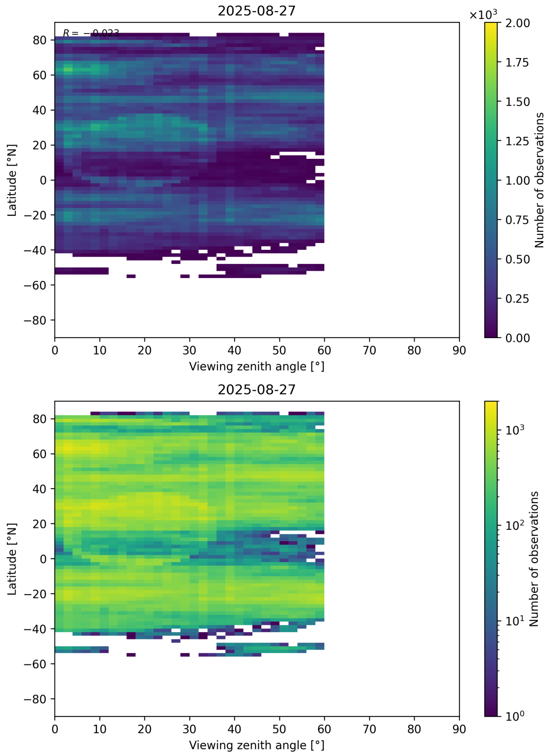
Figure 109: Scatter density plot of “Viewing zenith angle” against “Latitude” for 2025-08-26 to 2025-08-28.
