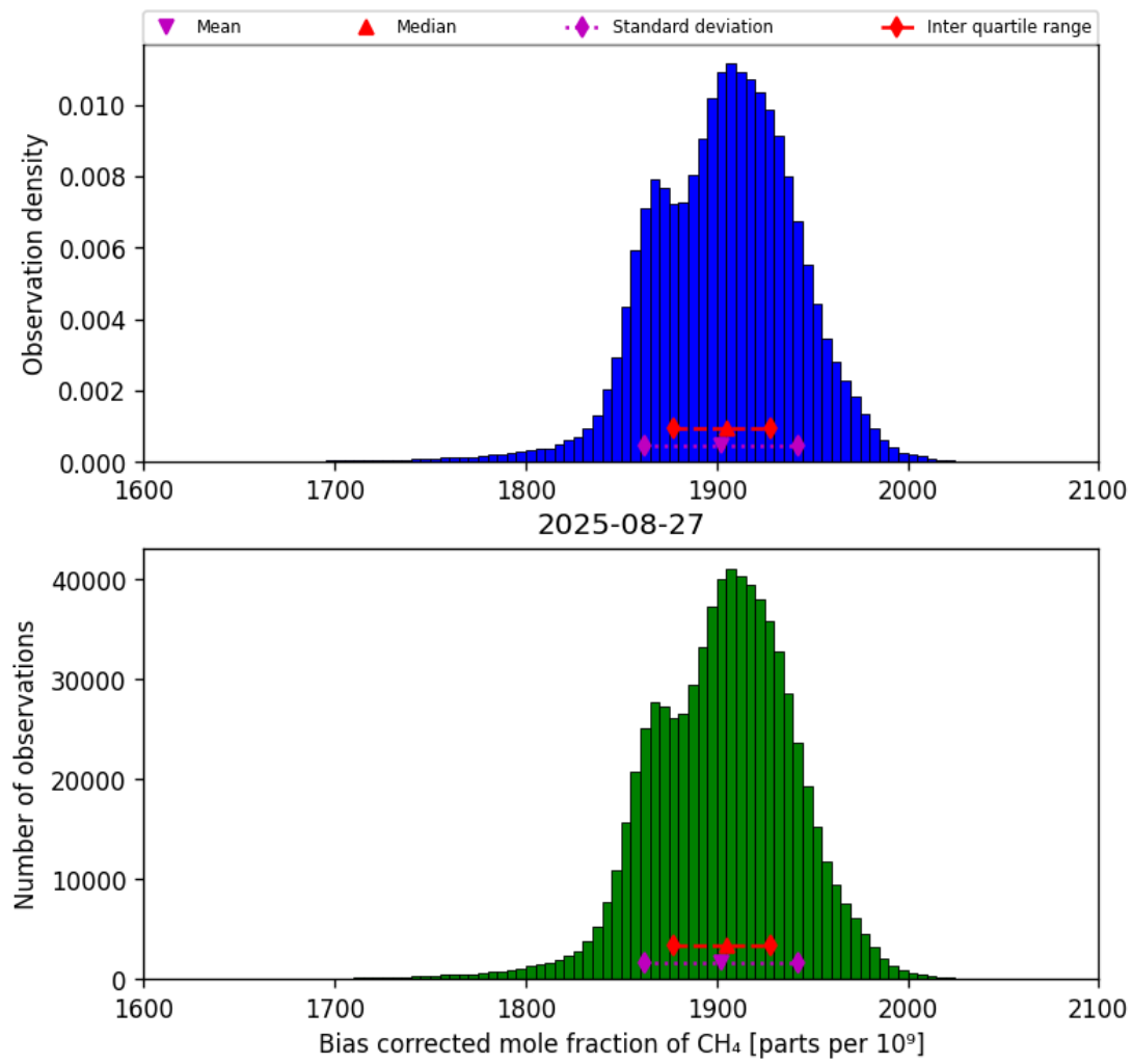
Figure 25: Histogram of “Bias corrected mole fraction of CH 4 ” for 2025-08-26 to 2025-08-28
