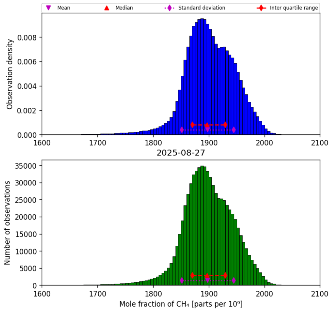
Figure 23: Histogram of “Mole fraction of CH 4 ” for 2025-08-26 to 2025-08-28
