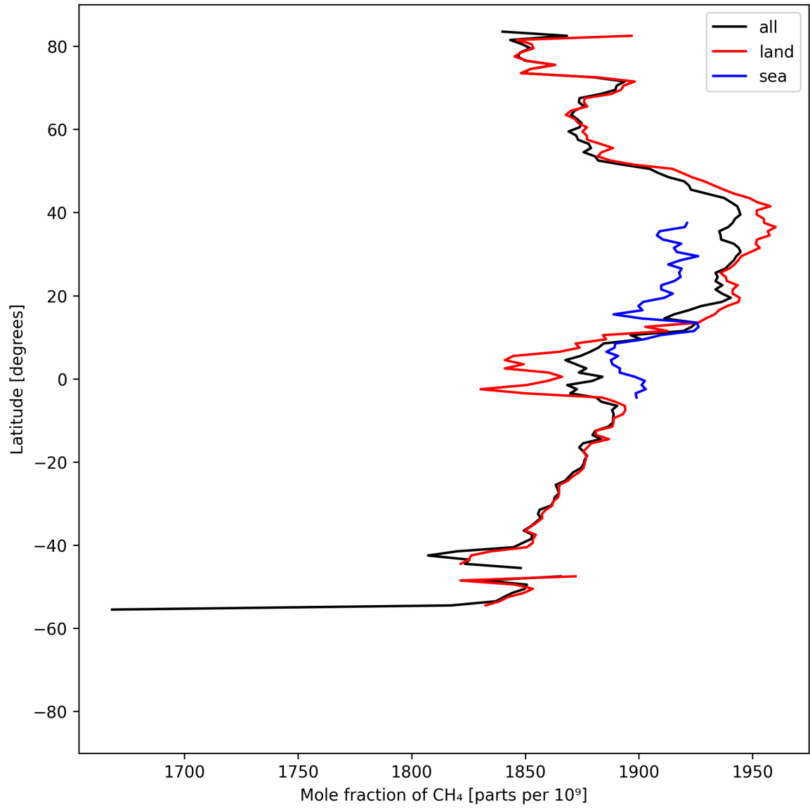
Figure 12: Zonal average of “Mole fraction of CH 4 ” for 2025-08-26 to 2025-08-28.
