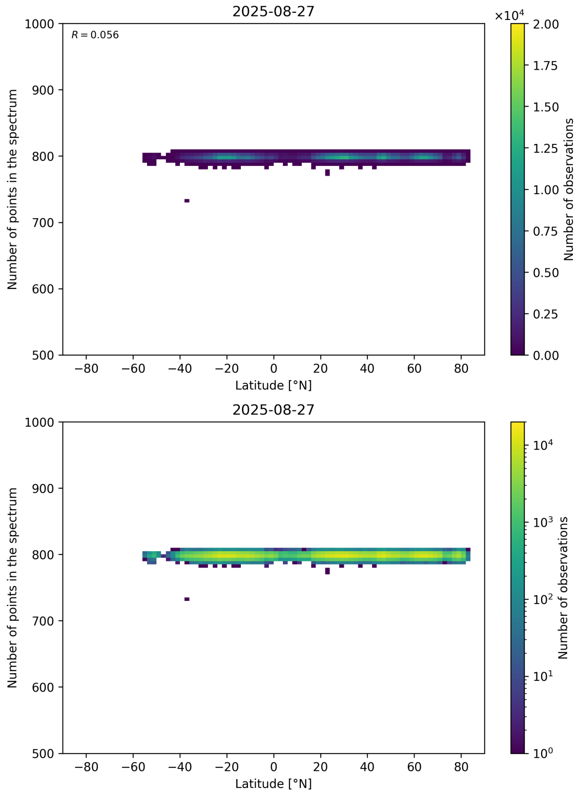
Figure 61: Scatter density plot of “Latitude” against “Number of points in the spectrum” for 2025-08-26 to 2025-08-28.
