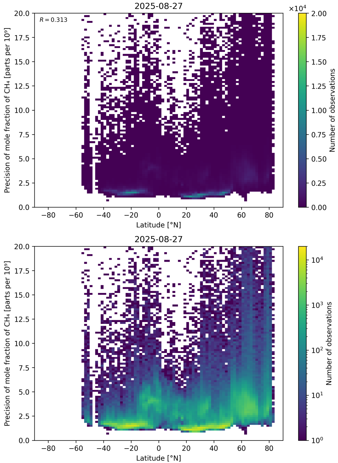
Figure 59: Scatter density plot of “Latitude” against “Precision of mole fraction of \text{CH}_4 ” for 2025-08-26 to 2025-08-28.
