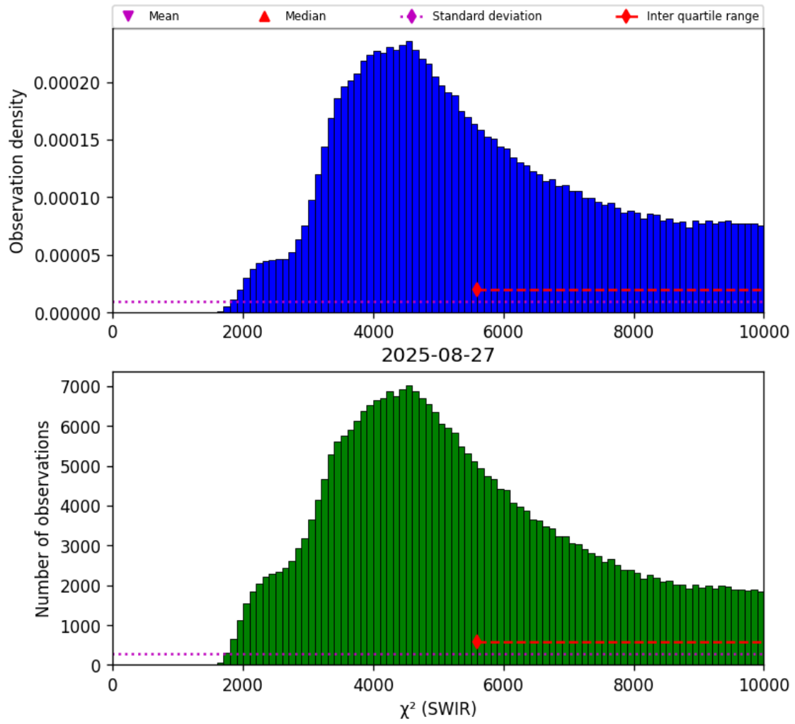
Figure 28: Histogram of “ \chi^2 (SWIR)” for 2025-08-26 to 2025-08-28
