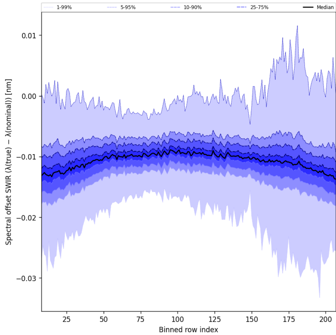
Figure 38: Along track statistics of “Spectral offset SWIR ( \lambda_{\text{true}} - \lambda_{\text{nominal}} )” for 2025-08-26 to 2025-08-28
