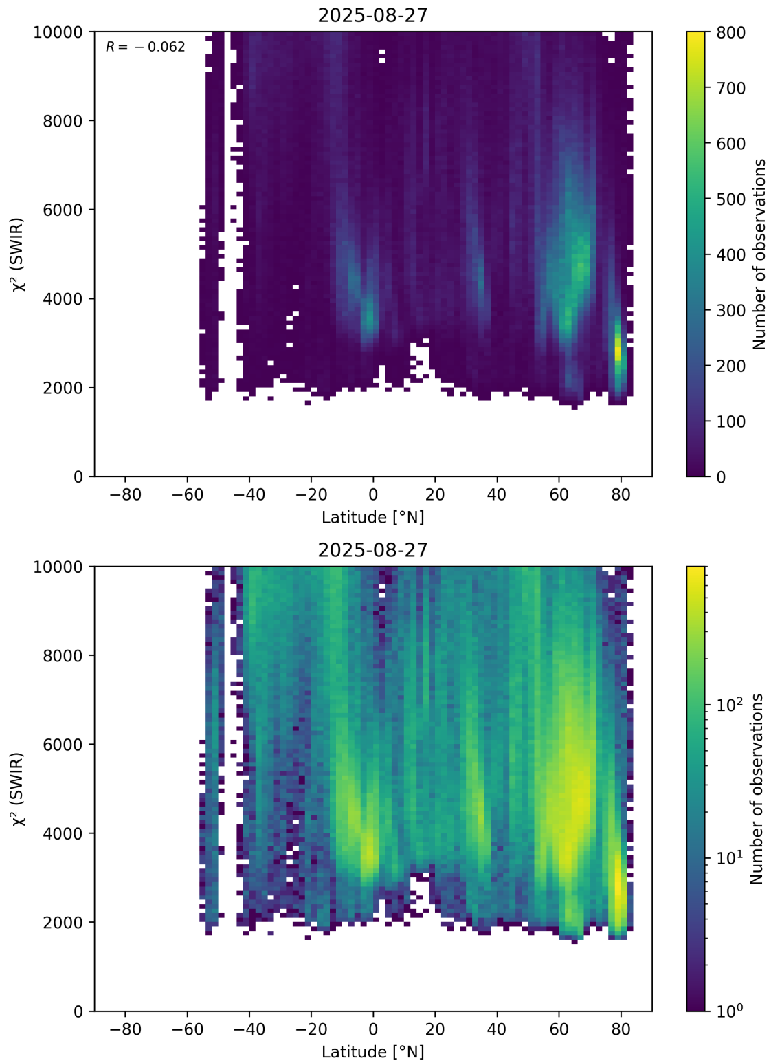
Figure 54: Scatter density plot of “Latitude” against “ \chi^2 (SWIR)” for 2025-08-26 to 2025-08-28.
