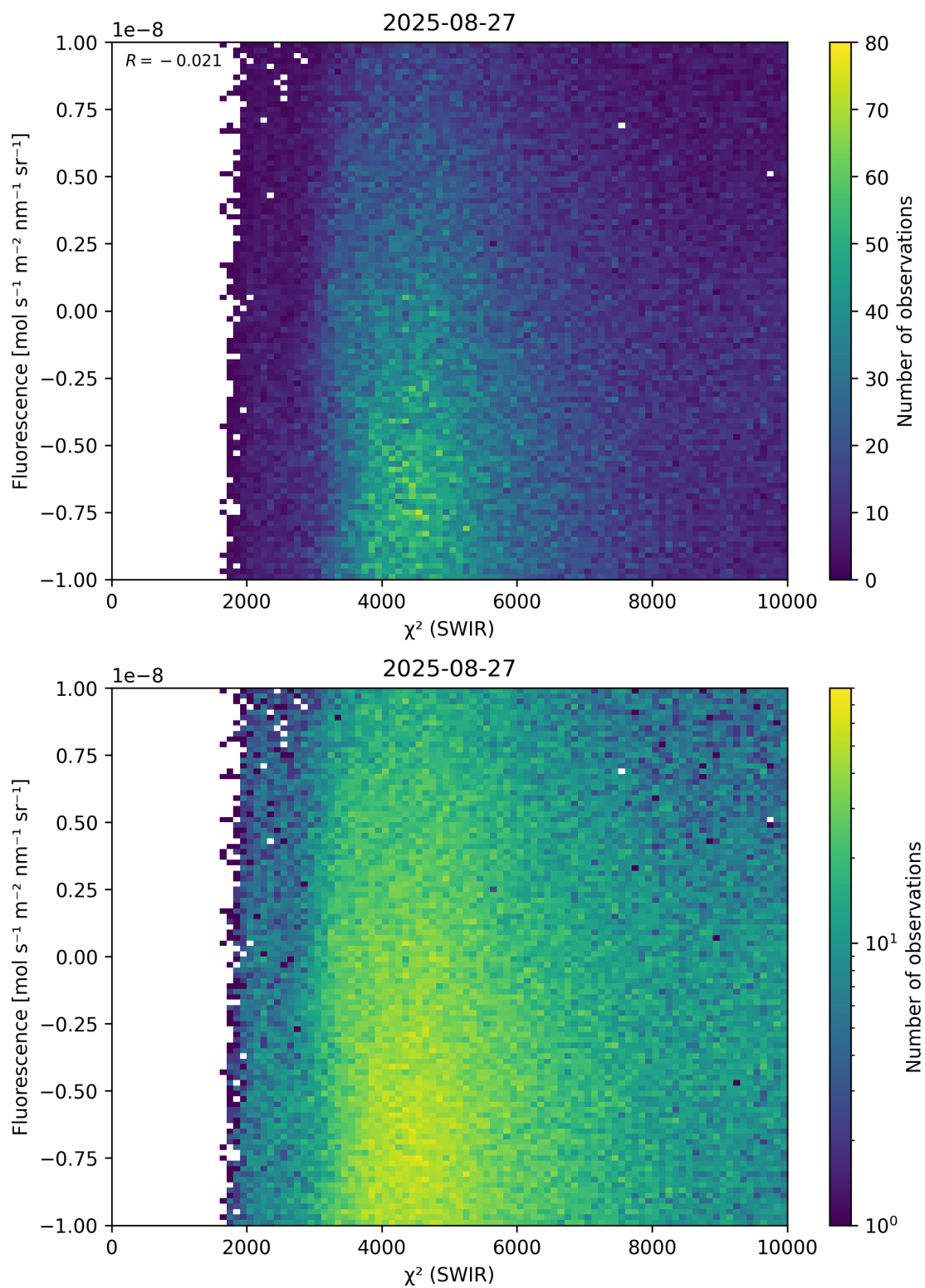
Figure 49: Scatter density plot of “ \chi^2 (SWIR)” against “Fluorescence” for 2025-08-26 to 2025-08-28.
