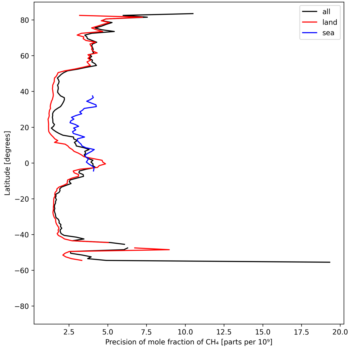
Figure 13: Zonal average of “Precision of mole fraction of CH 4 ” for 2025-08-26 to 2025-08-28.
