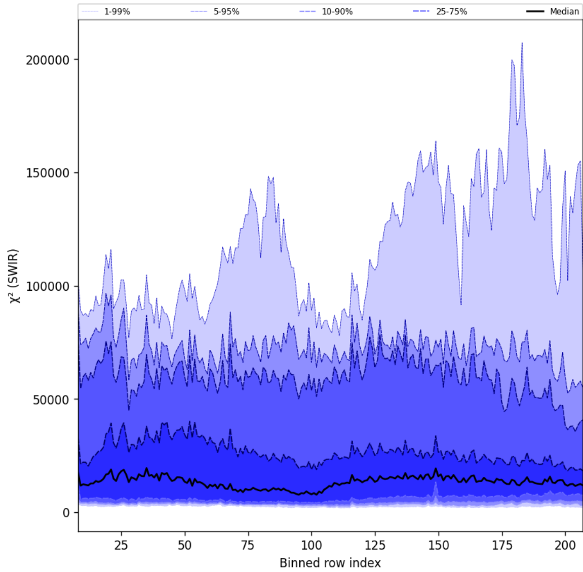
Figure 39: Along track statistics of “ \chi^2 (SWIR)” for 2025-08-26 to 2025-08-28
