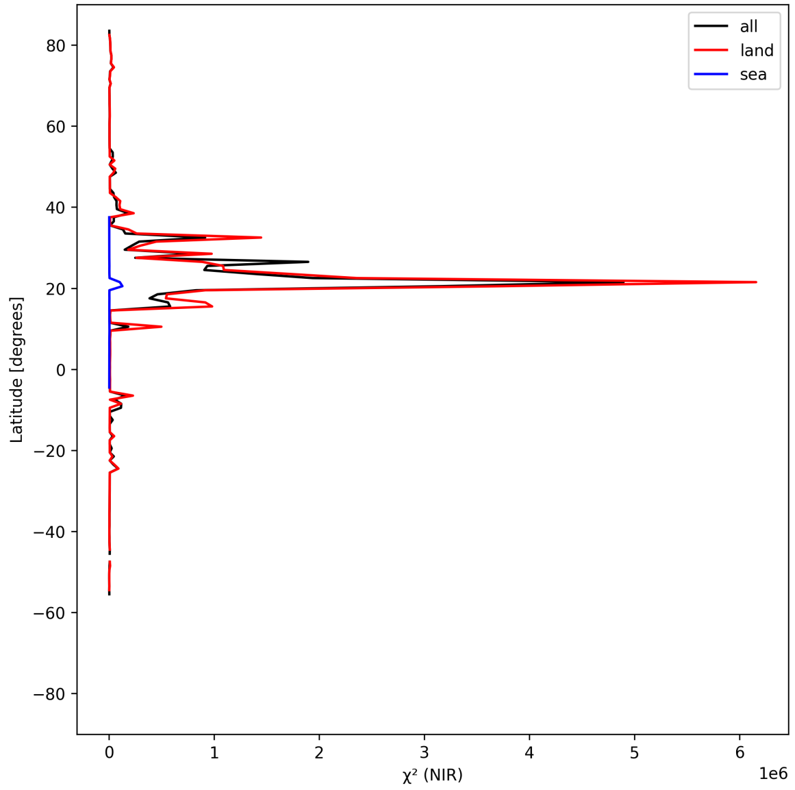
Figure 18: Zonal average of “ \chi^2 (NIR)” for 2025-08-26 to 2025-08-28.
