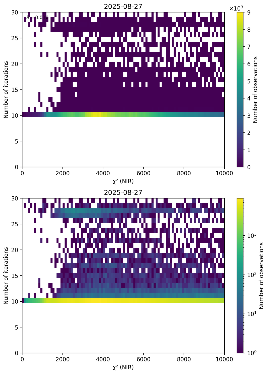
Figure 46: Scatter density plot of “ \chi^2 (NIR)” against “Number of iterations” for 2025-08-26 to 2025-08-28.
