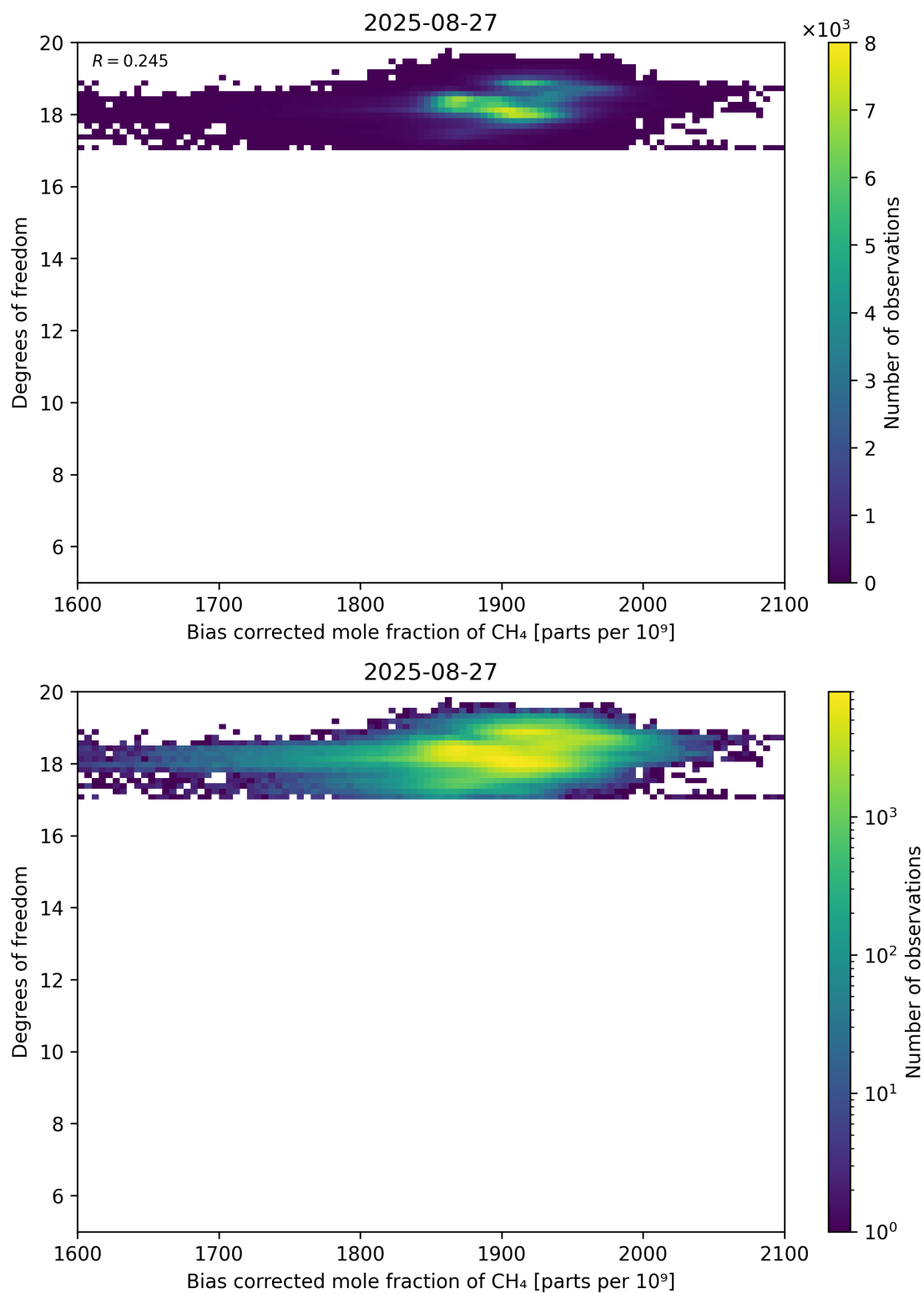
Figure 65: Scatter density plot of “Bias corrected mole fraction of CH 4 ” against “Degrees of freedom” for 2025-08-26 to 2025-08-28.
