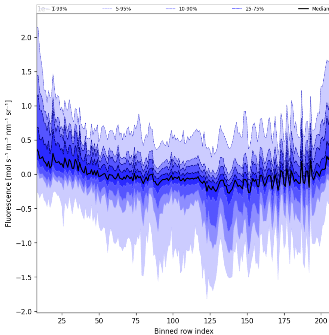
Figure 43: Along track statistics of “Fluorescence” for 2025-08-26 to 2025-08-28
