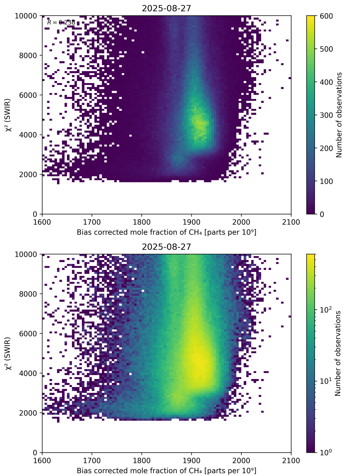
Figure 64: Scatter density plot of “Bias corrected mole fraction of \text{CH}_4 ” against “ \chi^2 (SWIR)” for 2025-08-26 to 2025-08-28.
