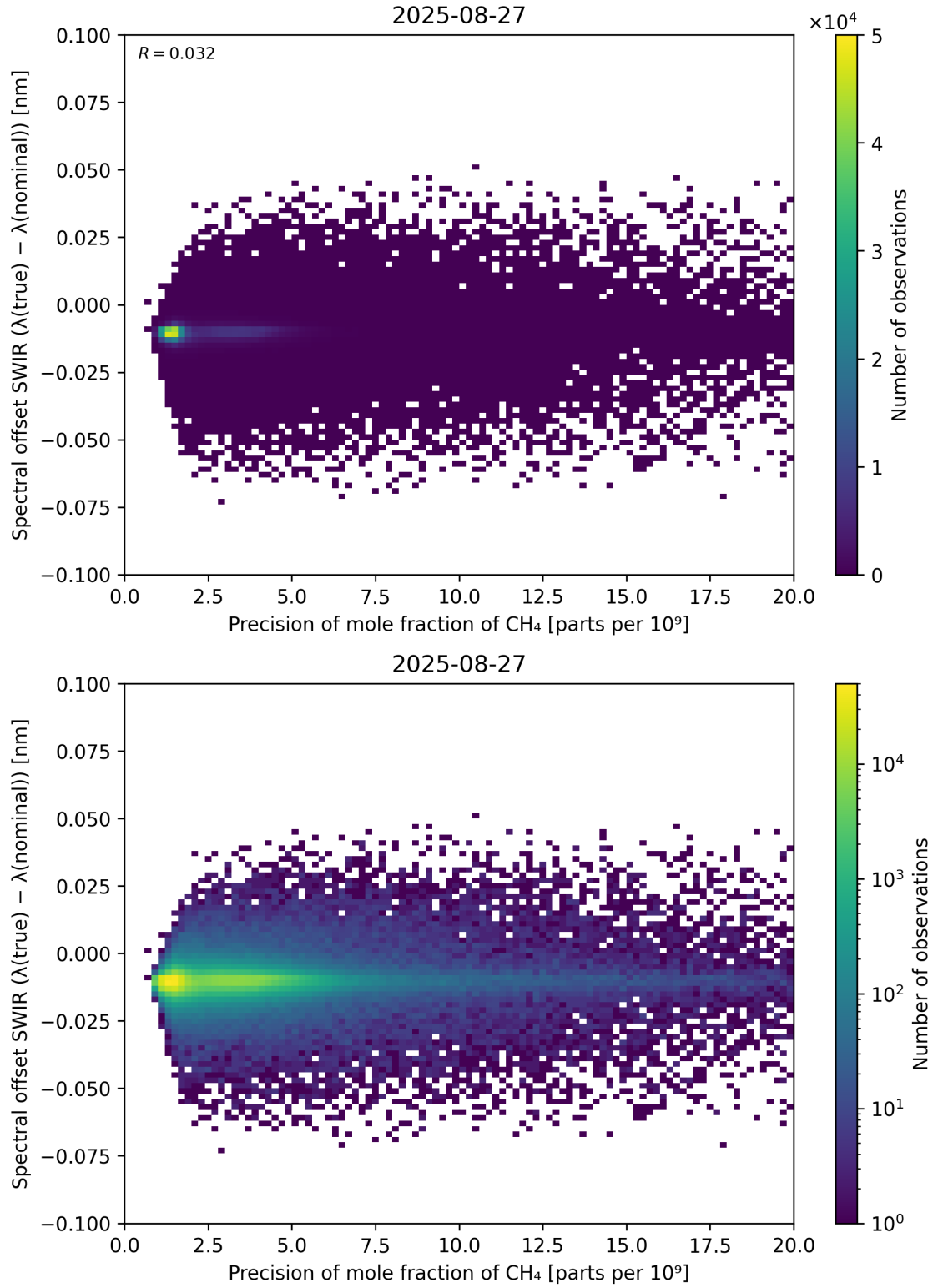
Figure 85: Scatter density plot of “Precision of mole fraction of CH 4 ” against “Spectral offset SWIR ( \lambda_{\text{true}} - \lambda_{\text{nominal}} )” for 2025-08-26 to 2025-08-28.
