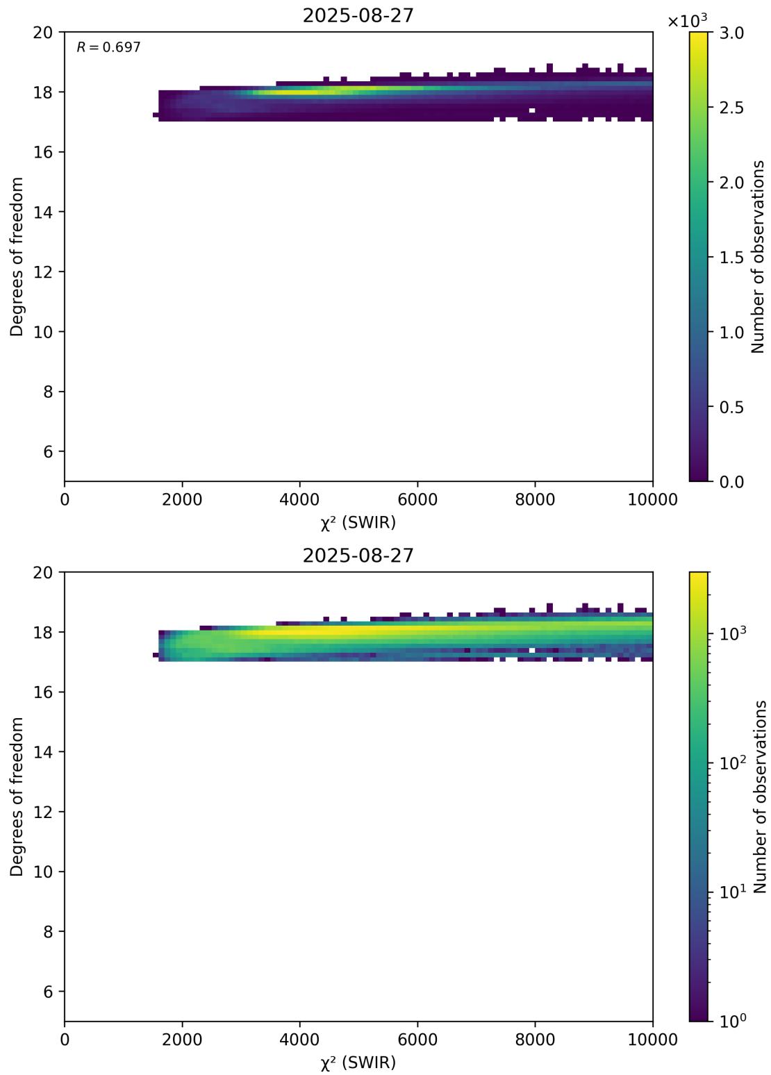
Figure 48: Scatter density plot of “ \chi^2 (SWIR)” against “Degrees of freedom” for 2025-08-26 to 2025-08-28.
