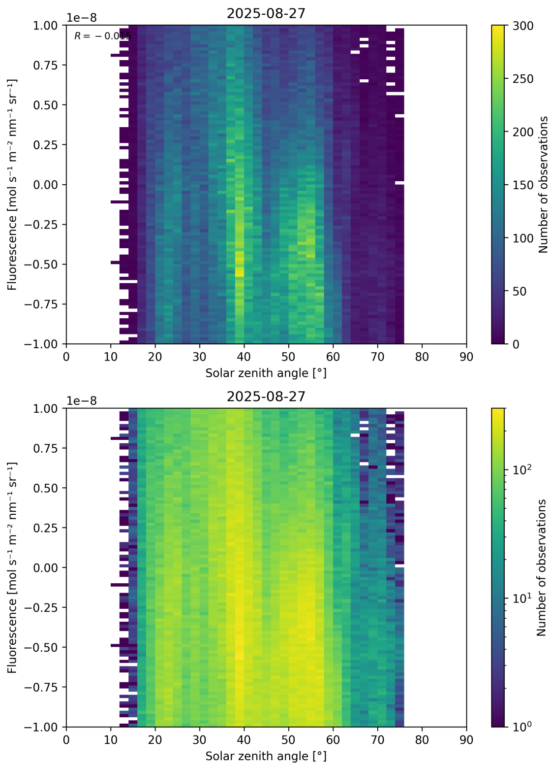
Figure 97: Scatter density plot of “Solar zenith angle” against “Fluorescence” for 2025-08-26 to 2025-08-28.
