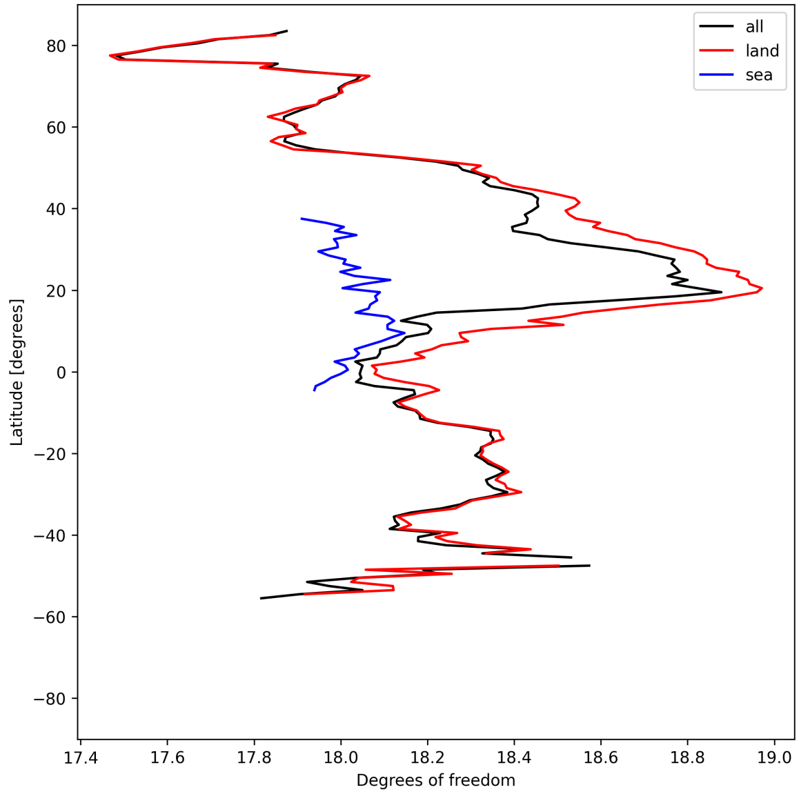
Figure 19: Zonal average of “Degrees of freedom” for 2025-08-26 to 2025-08-28.
