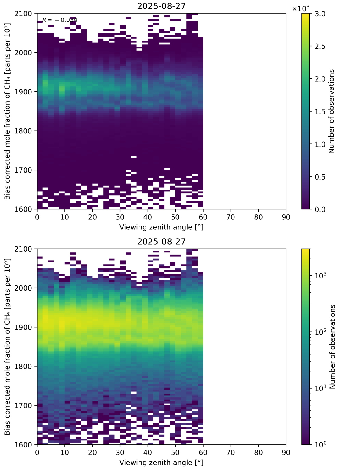
Figure 111: Scatter density plot of “Viewing zenith angle” against “Bias corrected mole fraction of CH 4 ” for 2025-08-26 to 2025-08-28.
