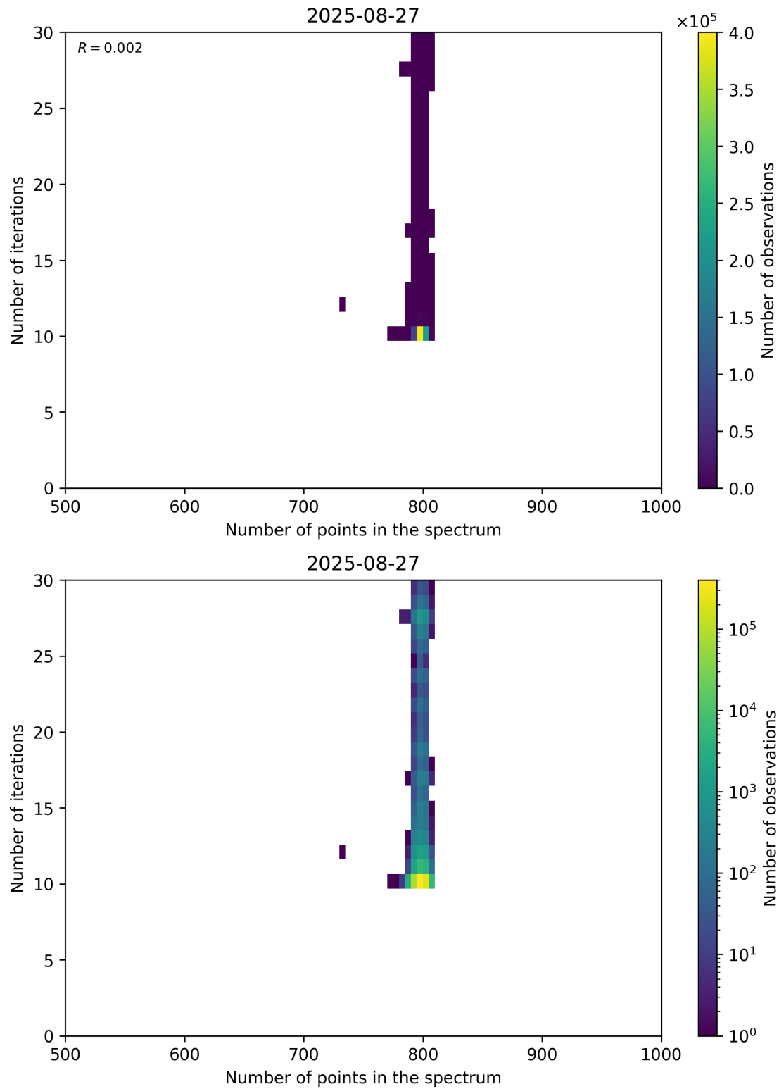
Figure 92: Scatter density plot of “Number of points in the spectrum” against “Number of iterations” for 2025-08-26 to 2025-08-28.
