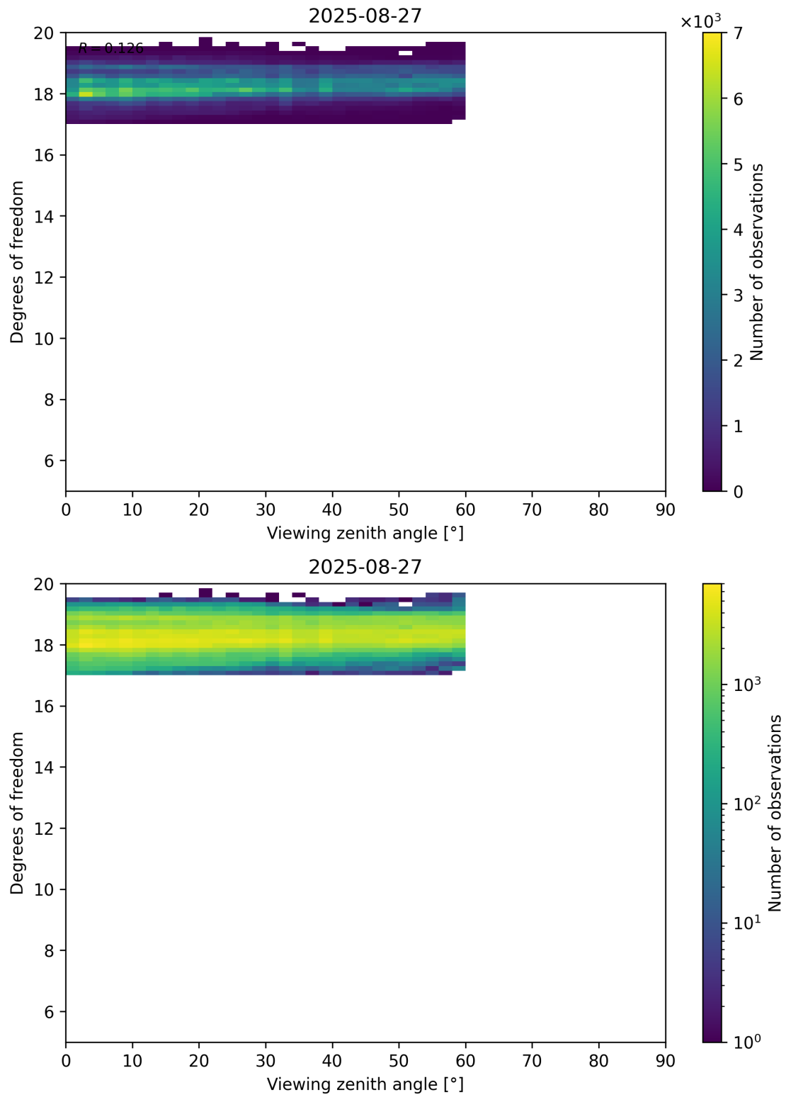
Figure 107: Scatter density plot of “Viewing zenith angle” against “Degrees of freedom” for 2025-08-26 to 2025-08-28.
