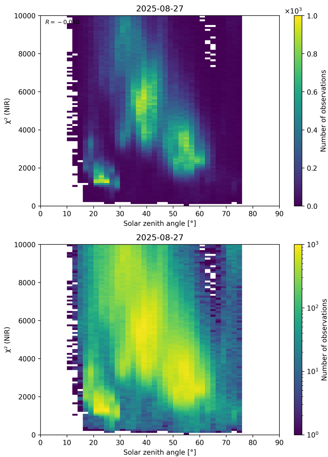
Figure 94: Scatter density plot of “Solar zenith angle” against “ \chi^2 (NIR)” for 2025-08-26 to 2025-08-28.
