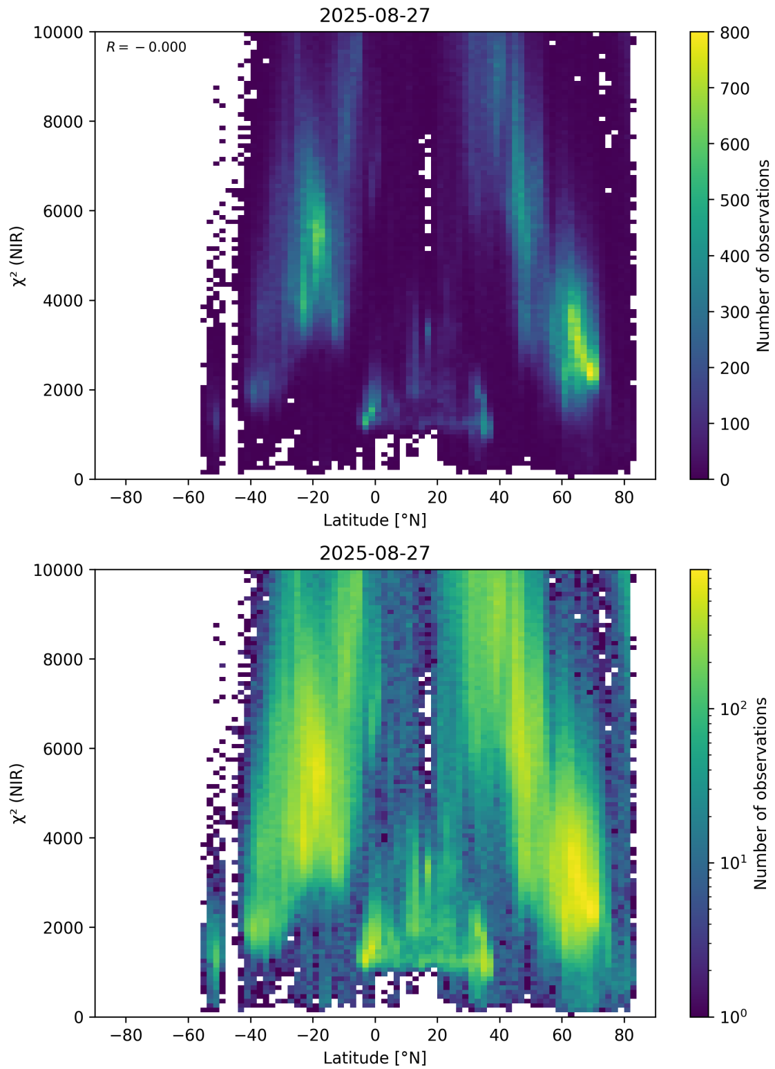
Figure 53: Scatter density plot of “Latitude” against “ \chi^2 (NIR)” for 2025-08-26 to 2025-08-28.
