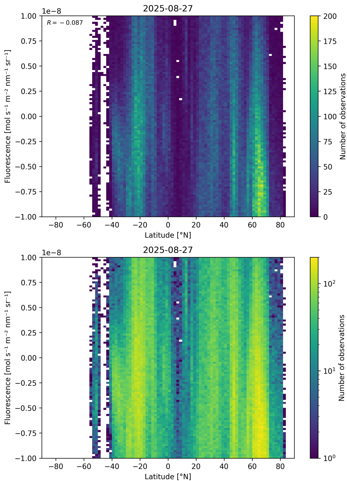
Figure 56: Scatter density plot of “Latitude” against “Fluorescence” for 2025-08-26 to 2025-08-28.
