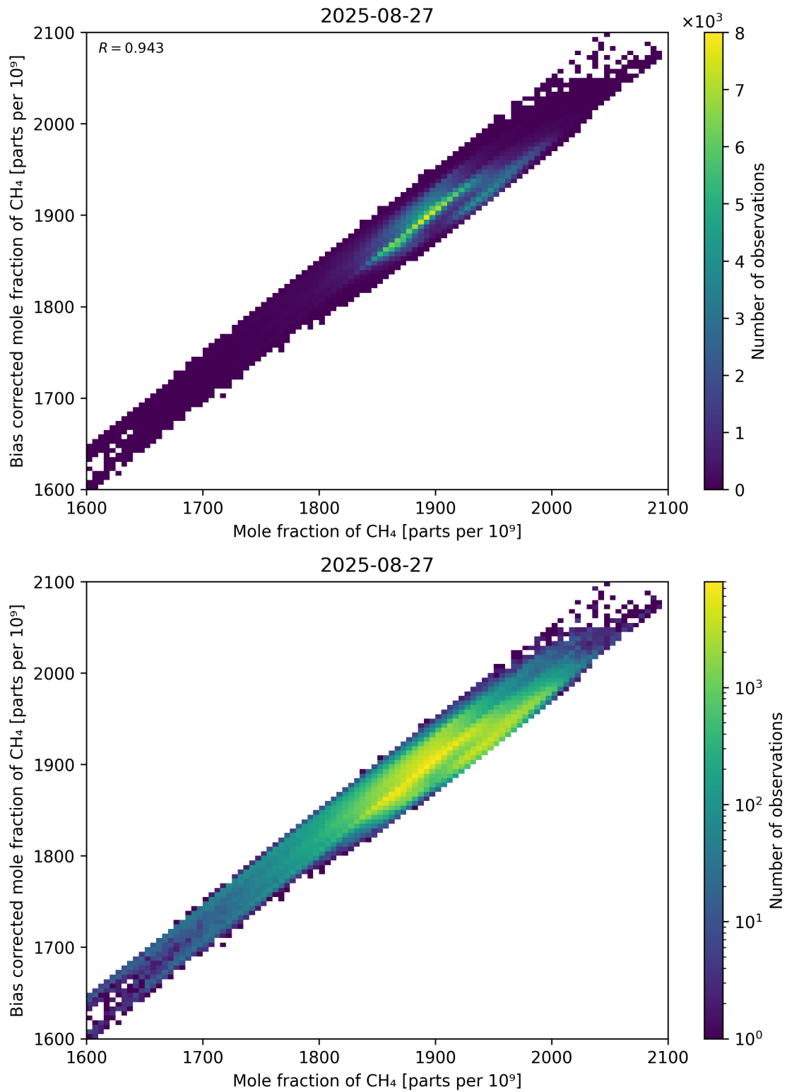
Figure 74: Scatter density plot of “Mole fraction of CH 4 ” against “Bias corrected mole fraction of CH 4 ” for 2025-08-26 to 2025-08-28.
