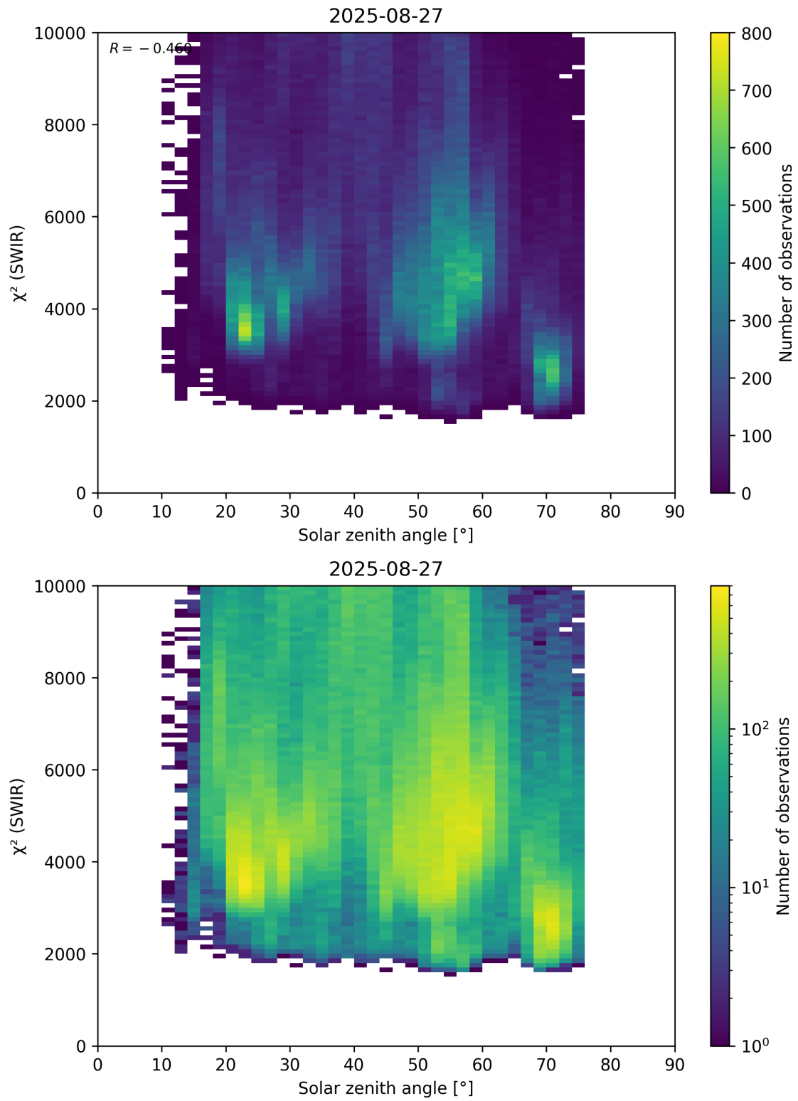
Figure 95: Scatter density plot of “Solar zenith angle” against “ \chi^2 (SWIR)” for 2025-08-26 to 2025-08-28.
