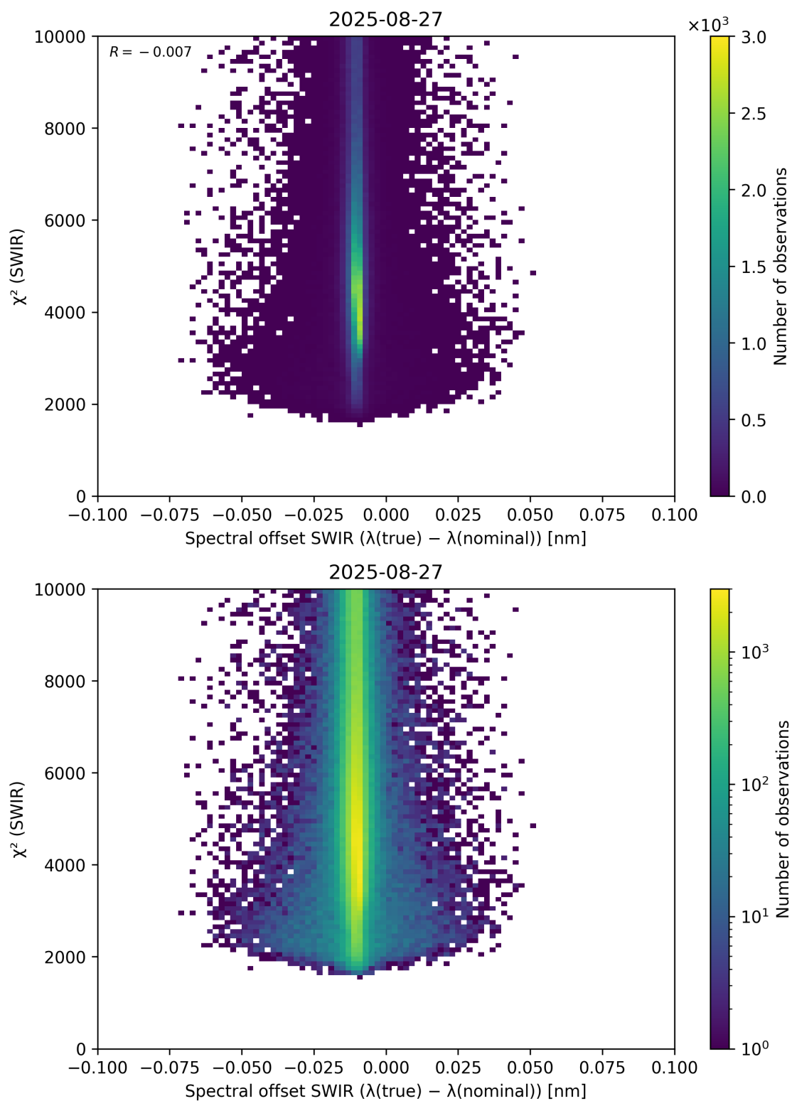
Figure 118: Scatter density plot of “Spectral offset SWIR ( \lambda_{\text{true}} - \lambda_{\text{nominal}} )” against “ \chi^2 (SWIR)” for 2025-08-26 to 2025-08-28.
