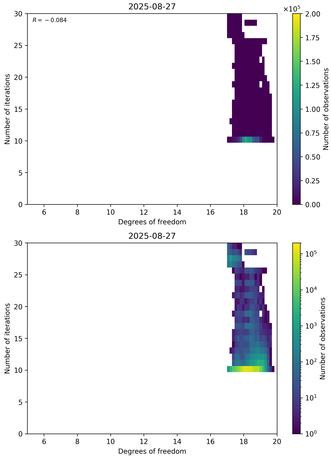
Figure 52: Scatter density plot of “Degrees of freedom” against “Number of iterations” for 2025-08-26 to 2025-08-28.
