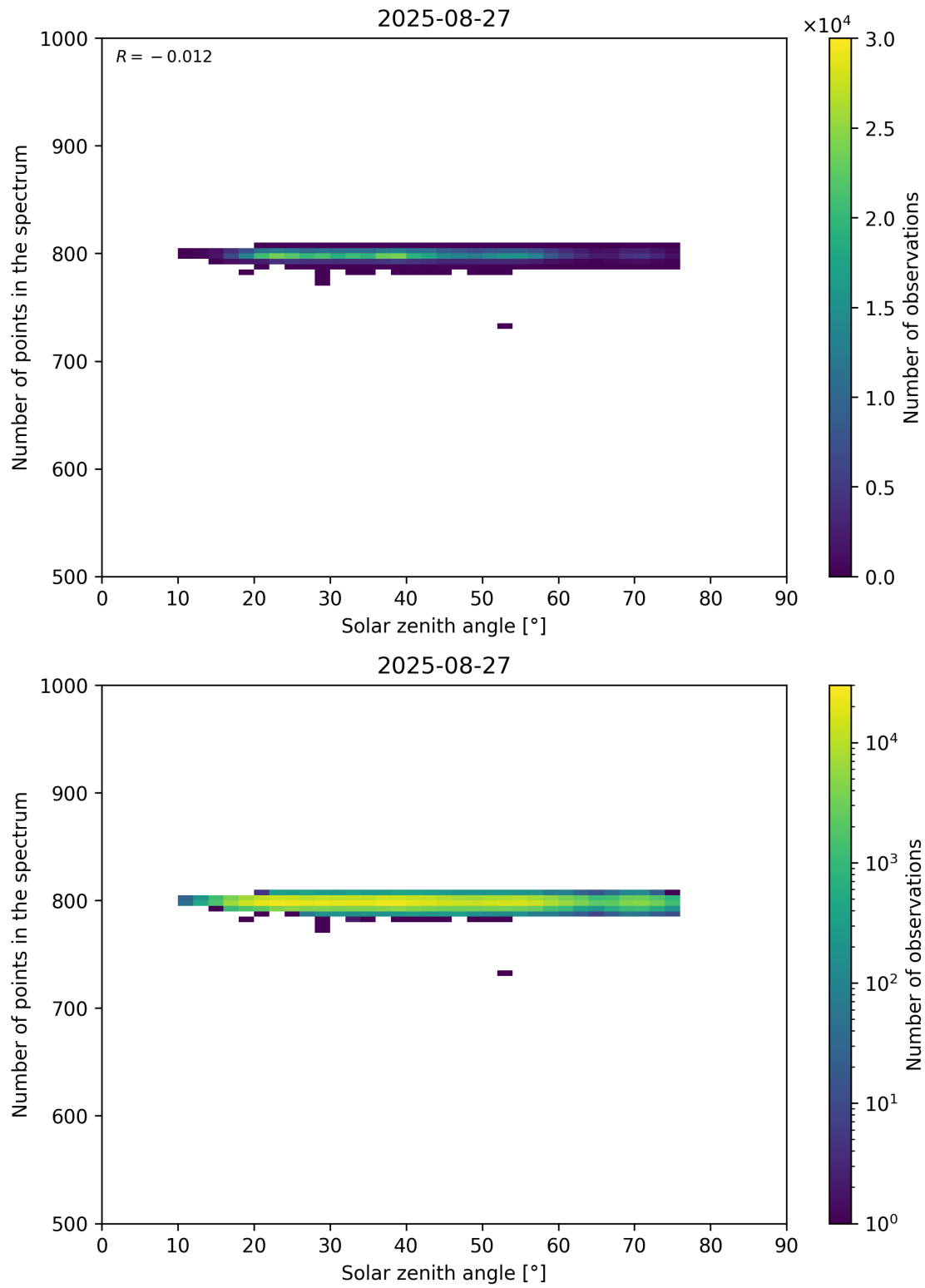
Figure 103: Scatter density plot of “Solar zenith angle” against “Number of points in the spectrum” for 2025-08-26 to 2025-08-28.
