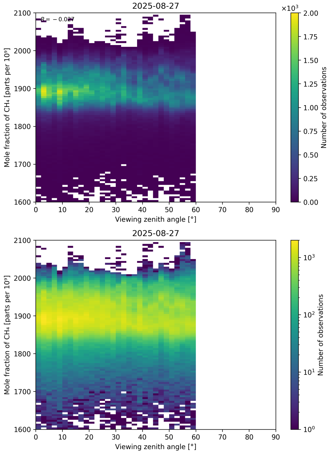
Figure 110: Scatter density plot of “Viewing zenith angle” against “Mole fraction of CH 4 ” for 2025-08-26 to 2025-08-28.
