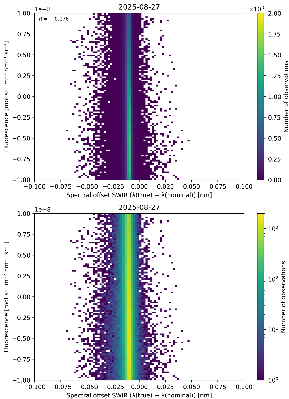
Figure 120: Scatter density plot of “Spectral offset SWIR ( \lambda_{\text{true}} - \lambda_{\text{nominal}} )” against “Fluorescence” for 2025-08-26 to 2025-08-28.
