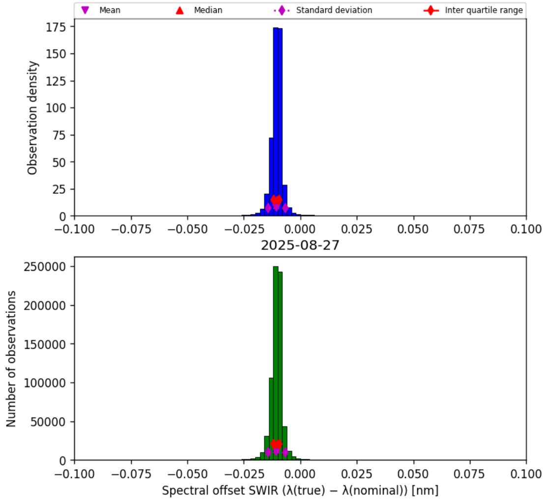
Figure 27: Histogram of “Spectral offset SWIR ( \lambda_{\text{true}} - \lambda_{\text{nominal}} )” for 2025-08-26 to 2025-08-28
