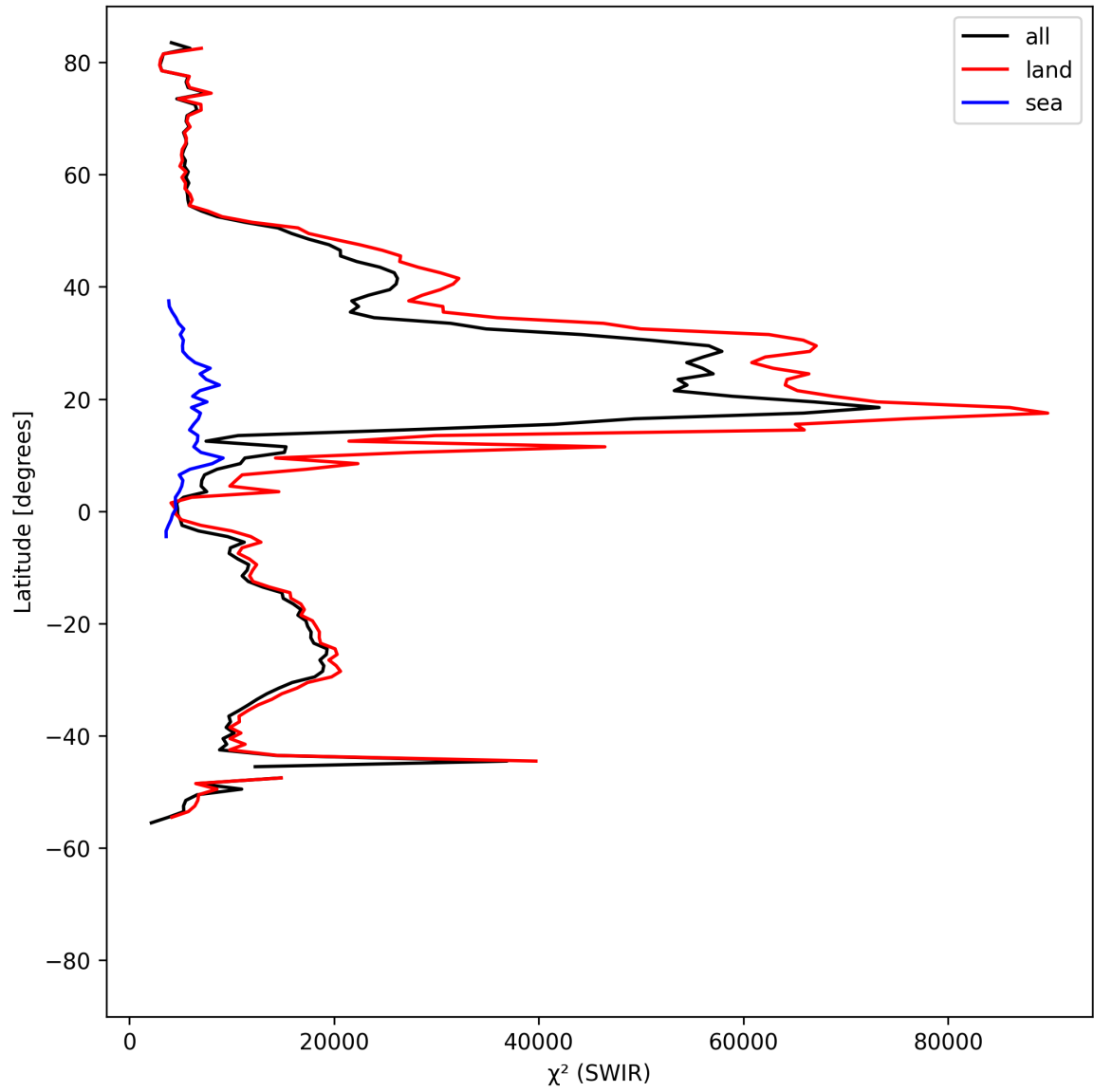
Figure 17: Zonal average of “ \chi^2 (SWIR)” for 2025-08-26 to 2025-08-28.
