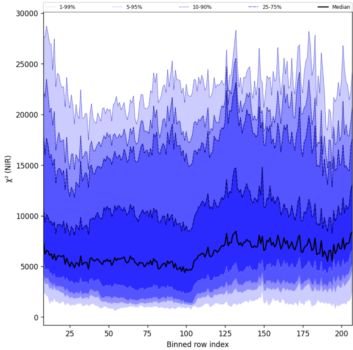
Figure 40: Along track statistics of “ \chi^2 (NIR)” for 2025-08-26 to 2025-08-28
