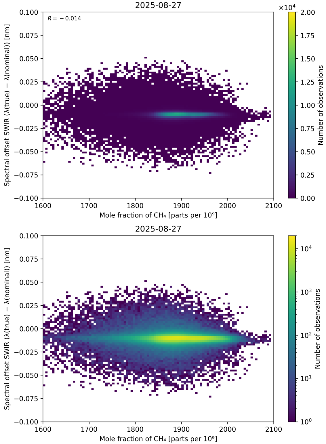
Figure 86: Scatter density plot of “Mole fraction of CH 4 ” against “Spectral offset SWIR ( \lambda_{\text{true}} - \lambda_{\text{nominal}} )” for 2025-08-26 to 2025-08-28.
