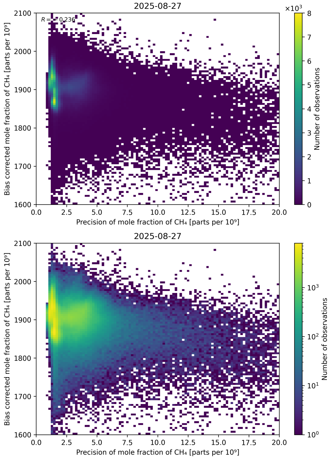
Figure 82: Scatter density plot of “Precision of mole fraction of CH 4 ” against “Bias corrected mole fraction of CH 4 ” for 2025-08-26 to 2025-08-28.
