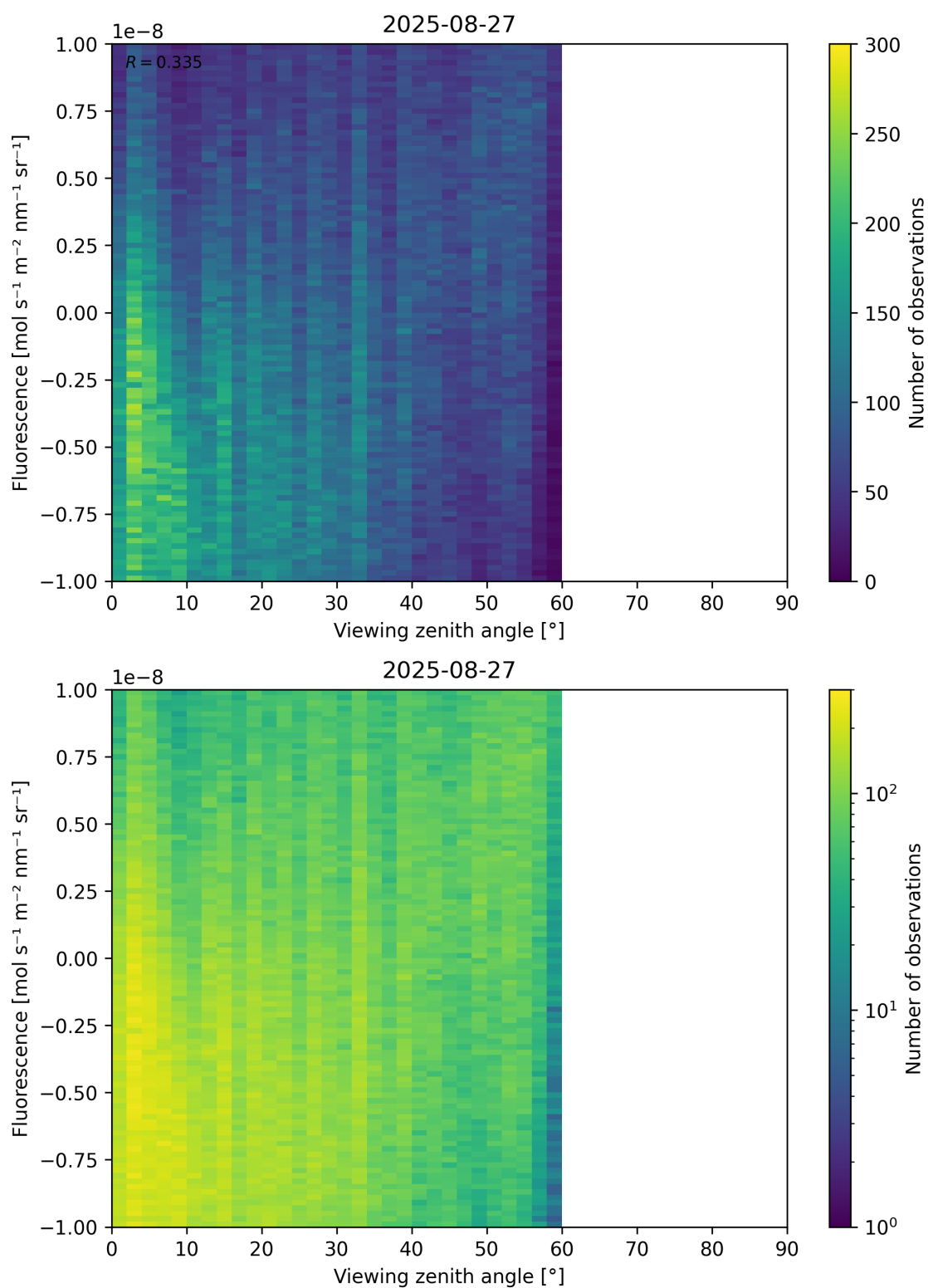
Figure 108: Scatter density plot of “Viewing zenith angle” against “Fluorescence” for 2025-08-26 to 2025-08-28.
