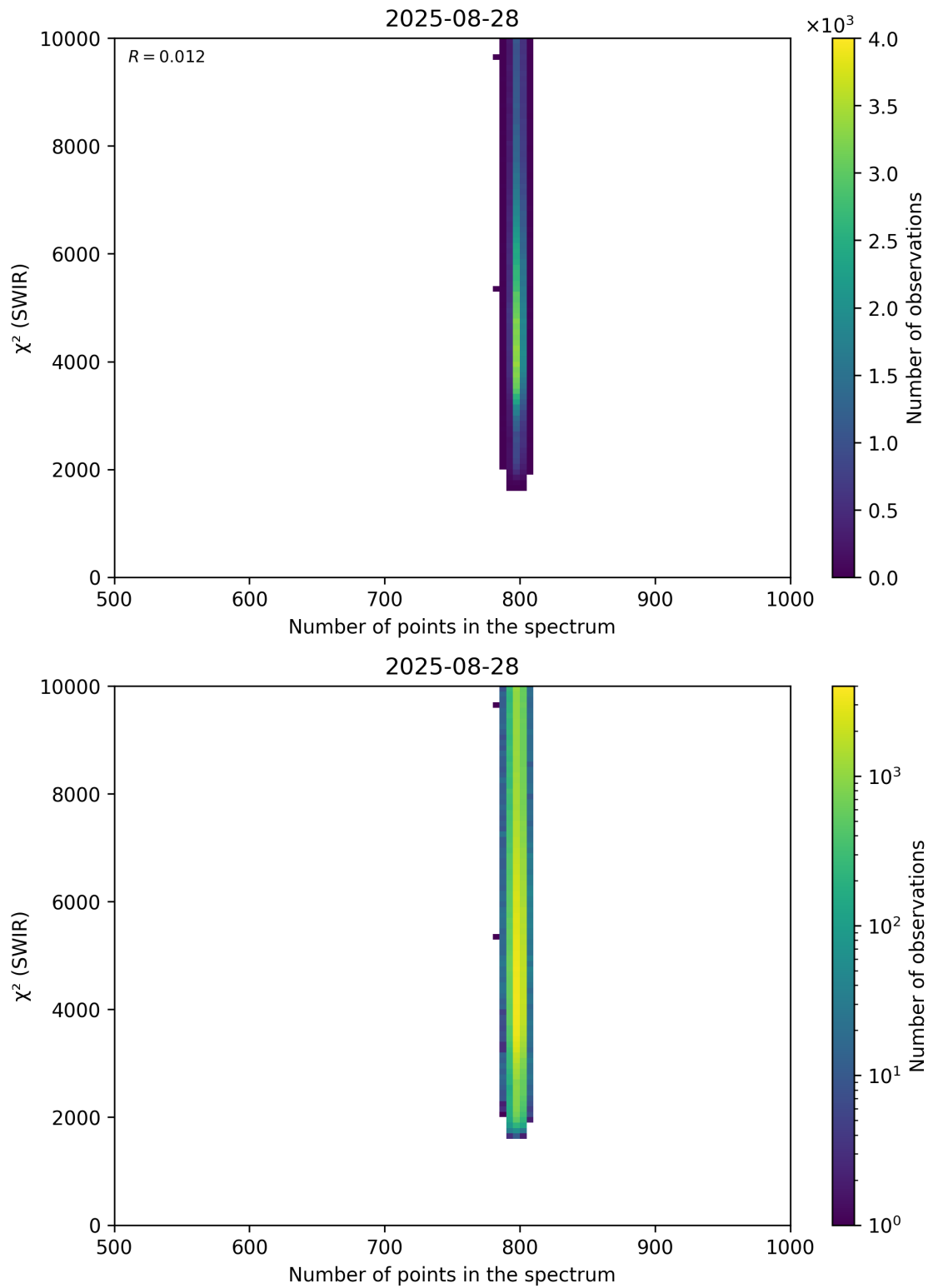
Figure 89: Scatter density plot of “Number of points in the spectrum” against “ \chi^2 (SWIR)” for 2025-08-27 to 2025-08-29.
