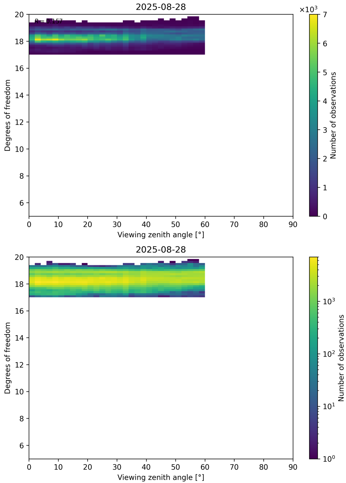
Figure 107: Scatter density plot of “Viewing zenith angle” against “Degrees of freedom” for 2025-08-27 to 2025-08-29.
