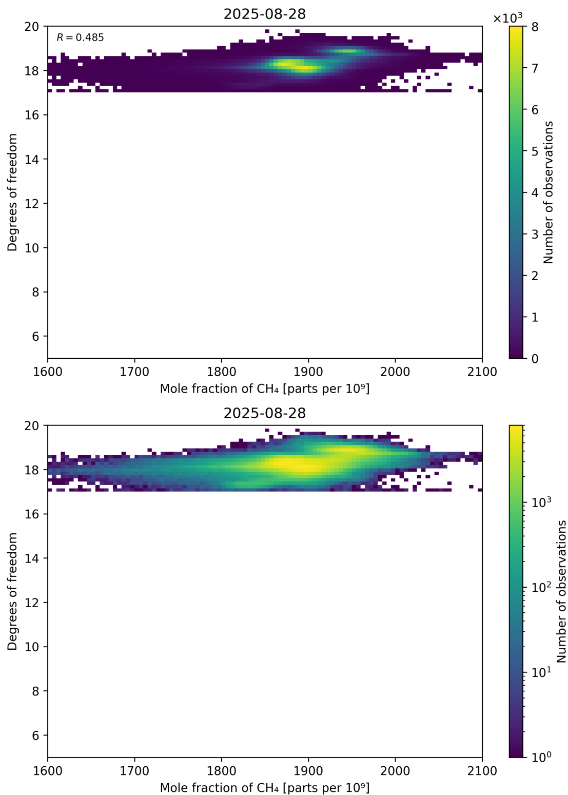
Figure 72: Scatter density plot of “Mole fraction of CH 4 ” against “Degrees of freedom” for 2025-08-27 to 2025-08-29.
