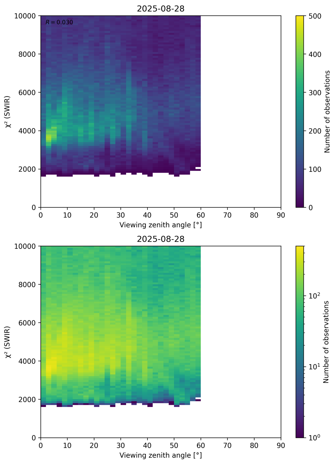
Figure 106: Scatter density plot of “Viewing zenith angle” against “ \chi^2 (SWIR)” for 2025-08-27 to 2025-08-29.
