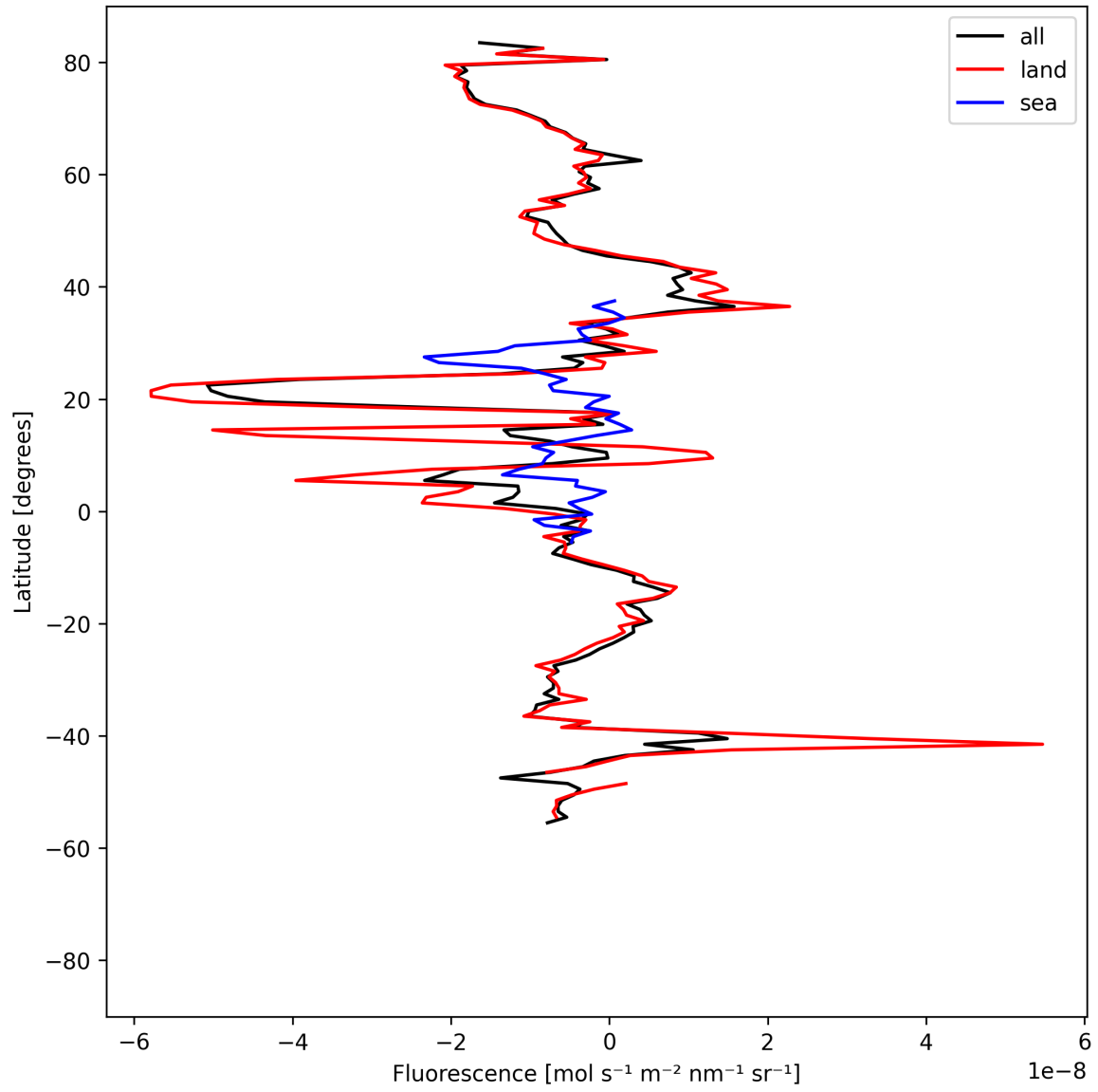
Figure 21: Zonal average of “Fluorescence” for 2025-08-27 to 2025-08-29.
