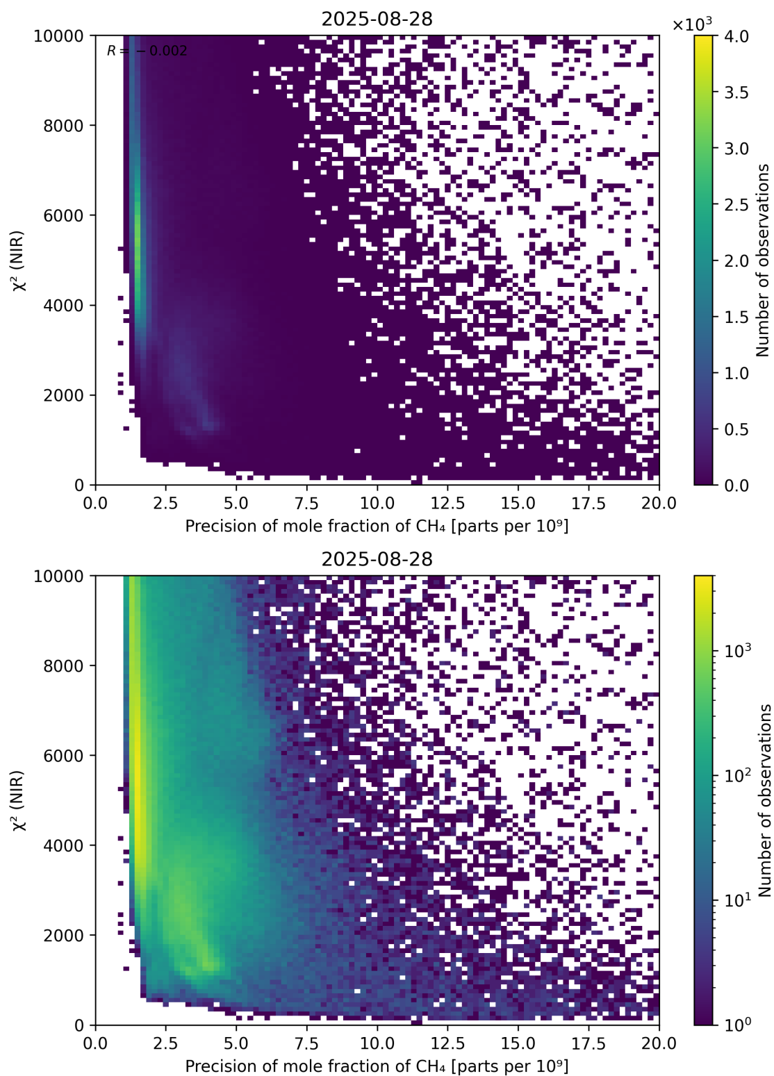
Figure 78: Scatter density plot of “Precision of mole fraction of CH 4 ” against “ \chi^2 (NIR)” for 2025-08-27 to 2025-08-29.
