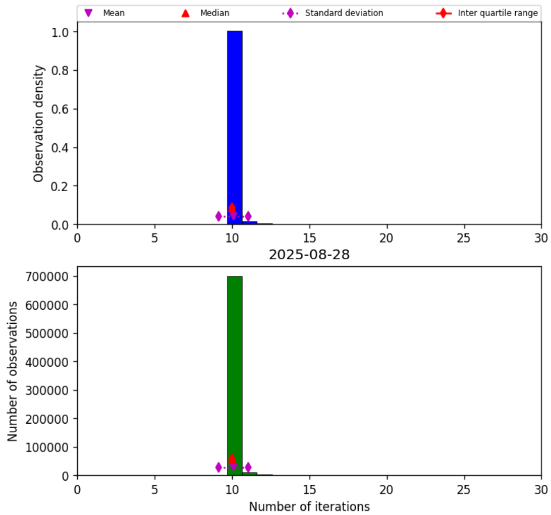
Figure 31: Histogram of “Number of iterations” for 2025-08-27 to 2025-08-29
