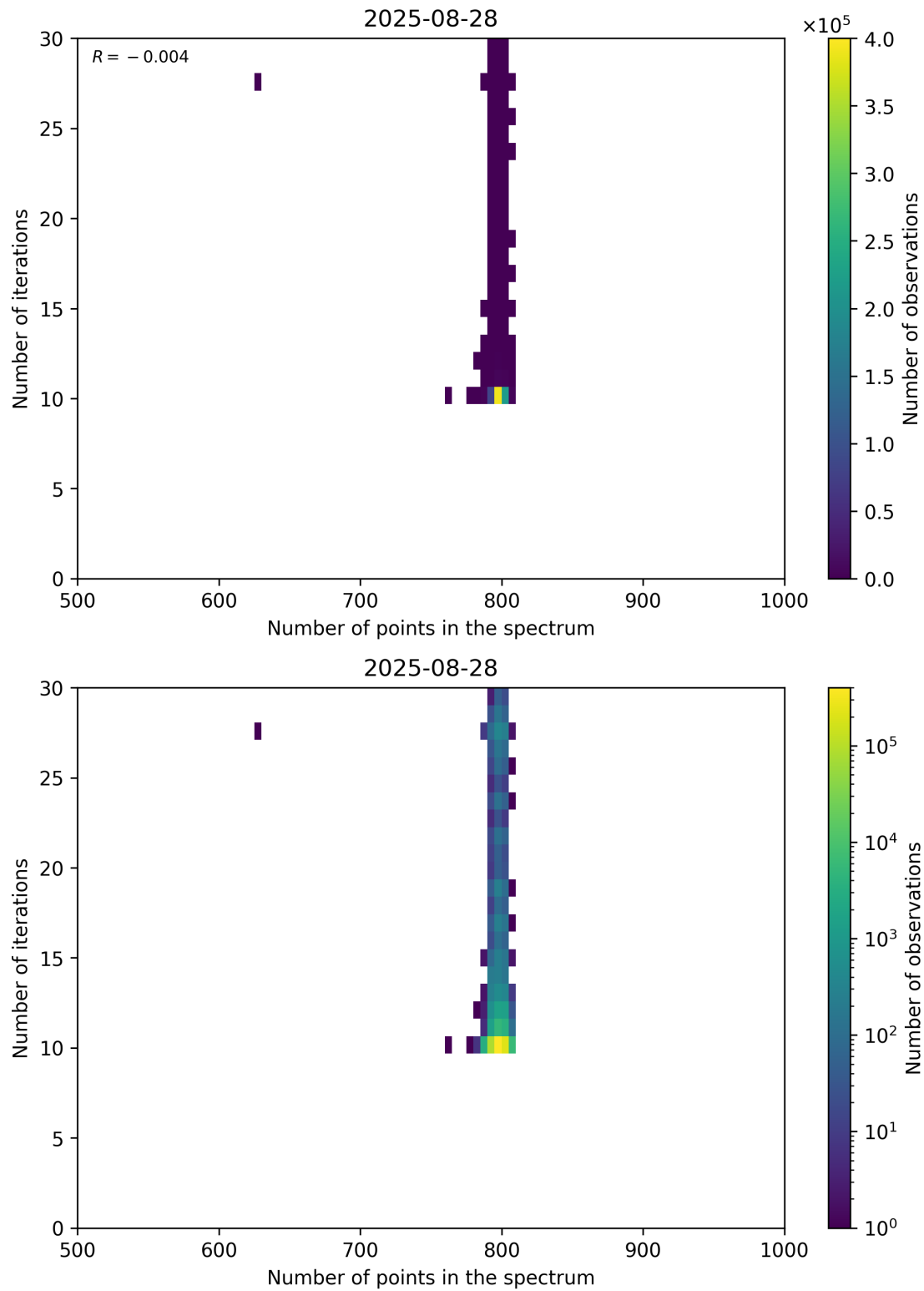
Figure 92: Scatter density plot of “Number of points in the spectrum” against “Number of iterations” for 2025-08-27 to 2025-08-29.
