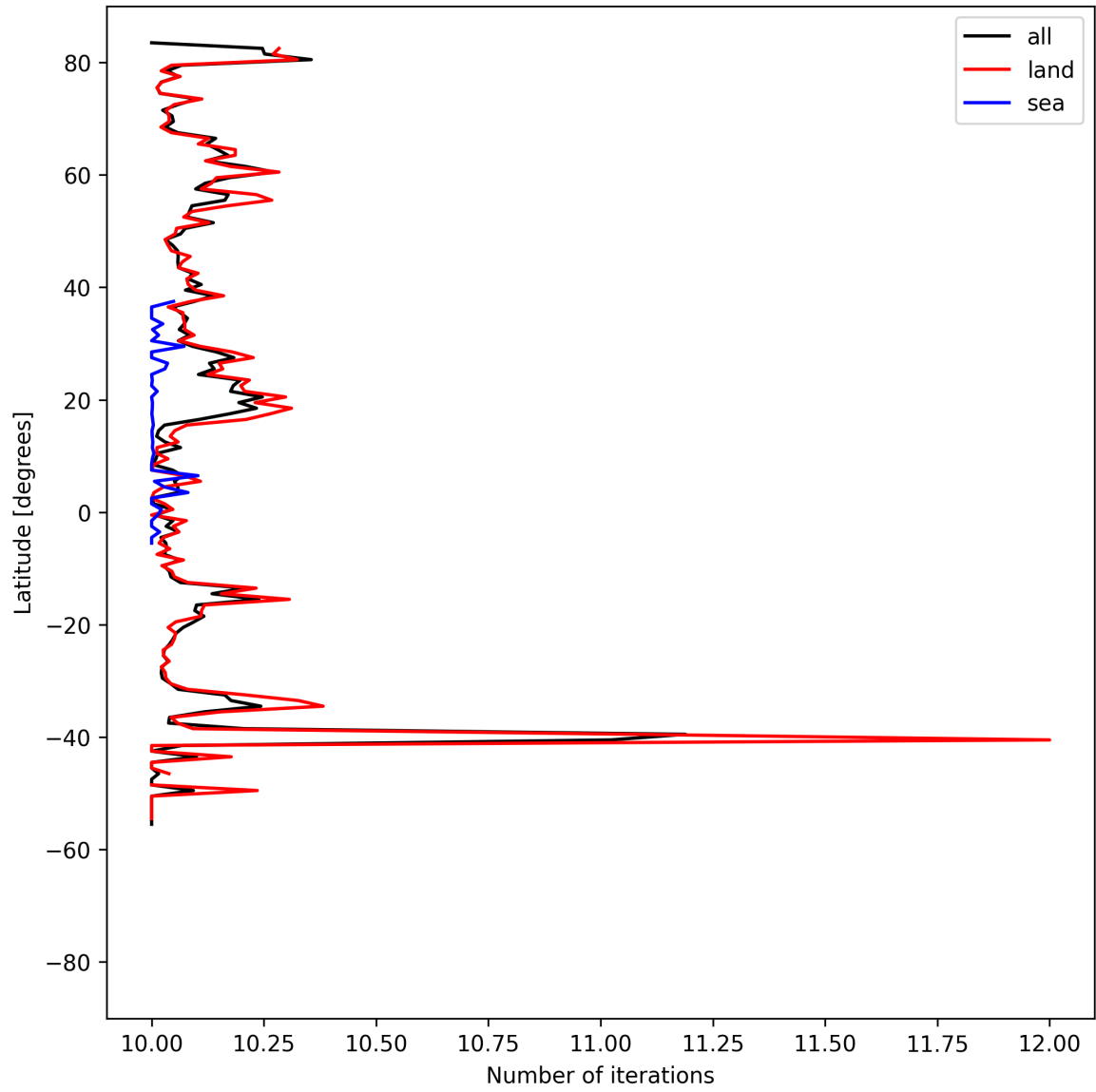
Figure 20: Zonal average of “Number of iterations” for 2025-08-27 to 2025-08-29.
