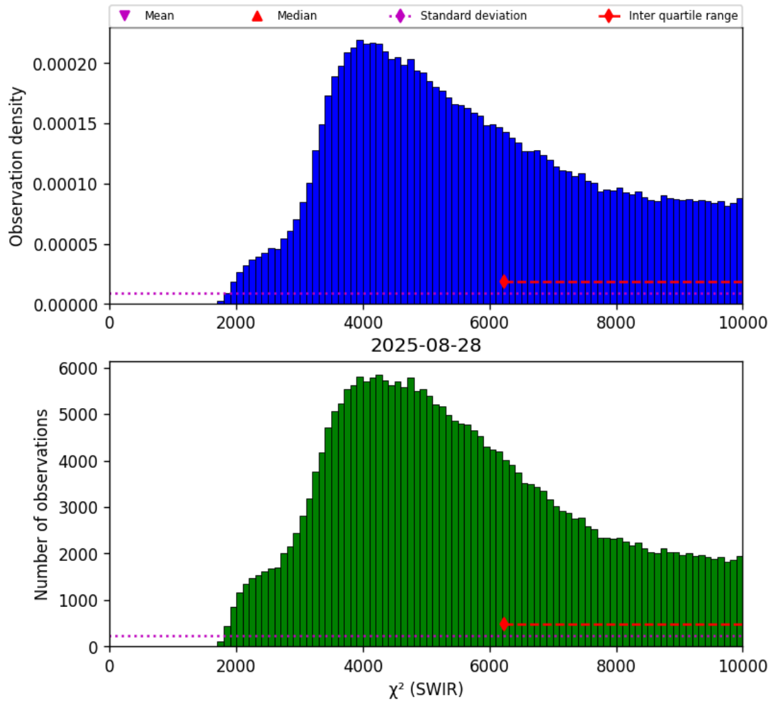
Figure 28: Histogram of “ \chi^2 (SWIR)” for 2025-08-27 to 2025-08-29
