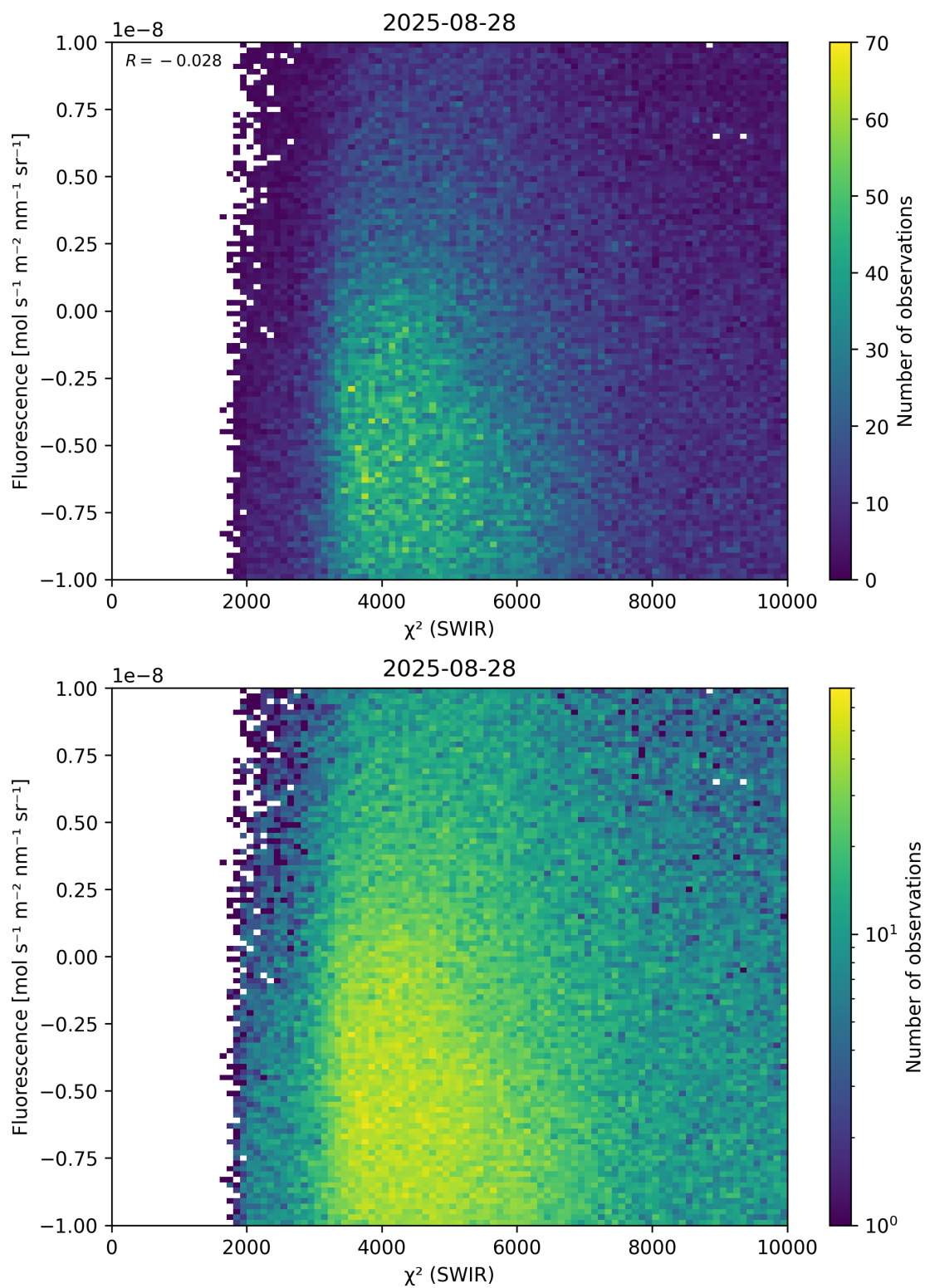
Figure 49: Scatter density plot of “ \chi^2 (SWIR)” against “Fluorescence” for 2025-08-27 to 2025-08-29.
