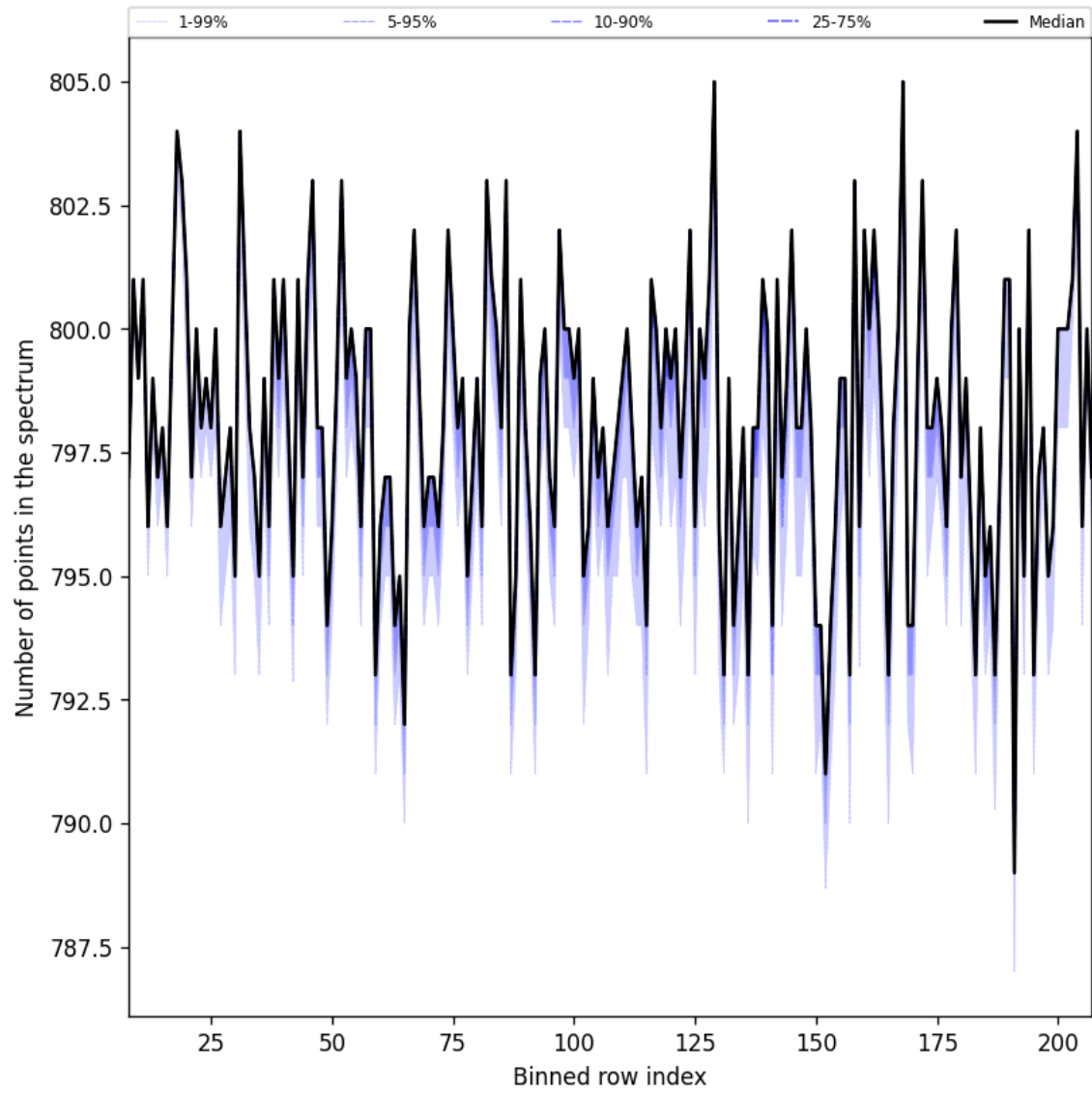
Figure 37: Along track statistics of “Number of points in the spectrum” for 2025-08-27 to 2025-08-29
