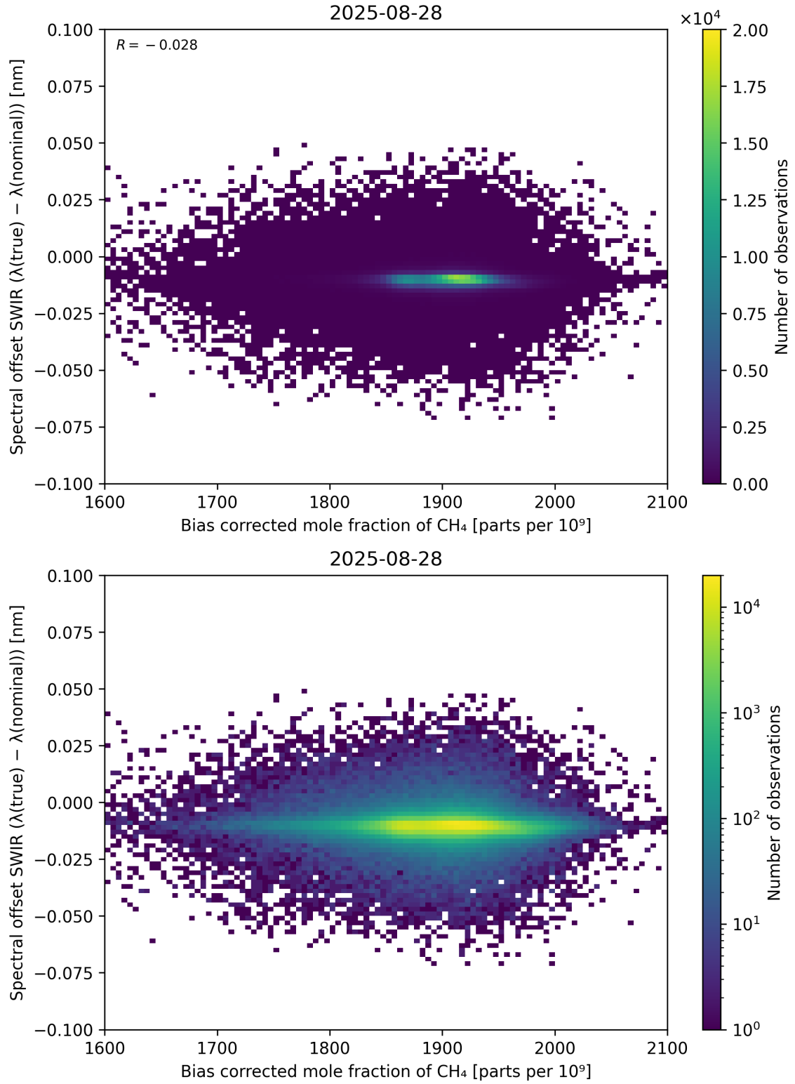
Figure 69: Scatter density plot of “Bias corrected mole fraction of CH 4 ” against “Spectral offset SWIR ( \lambda_{\text{true}} - \lambda_{\text{nominal}} )” for 2025-08-27 to 2025-08-29.
