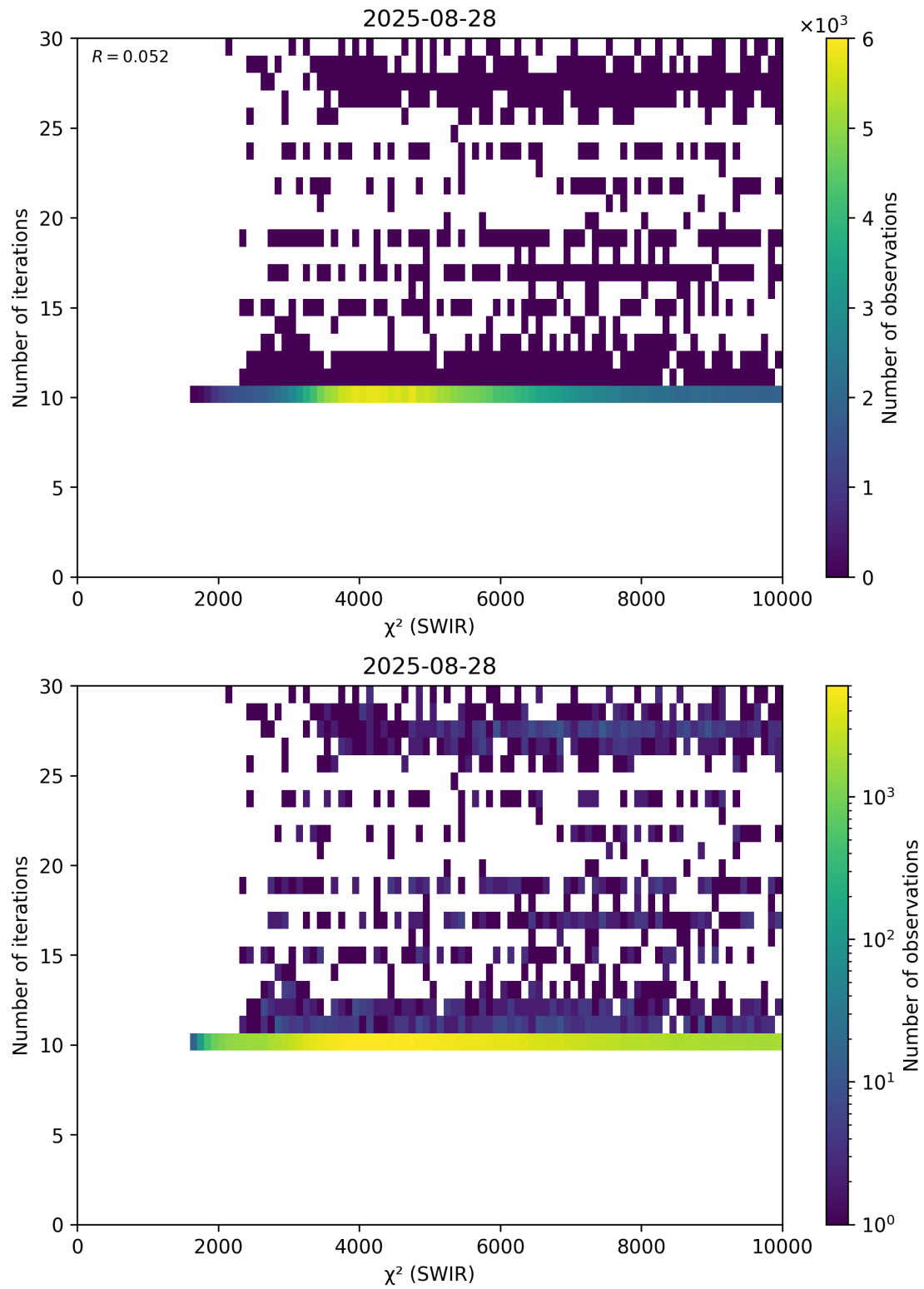
Figure 50: Scatter density plot of “ \chi^2 (SWIR)” against “Number of iterations” for 2025-08-27 to 2025-08-29.
