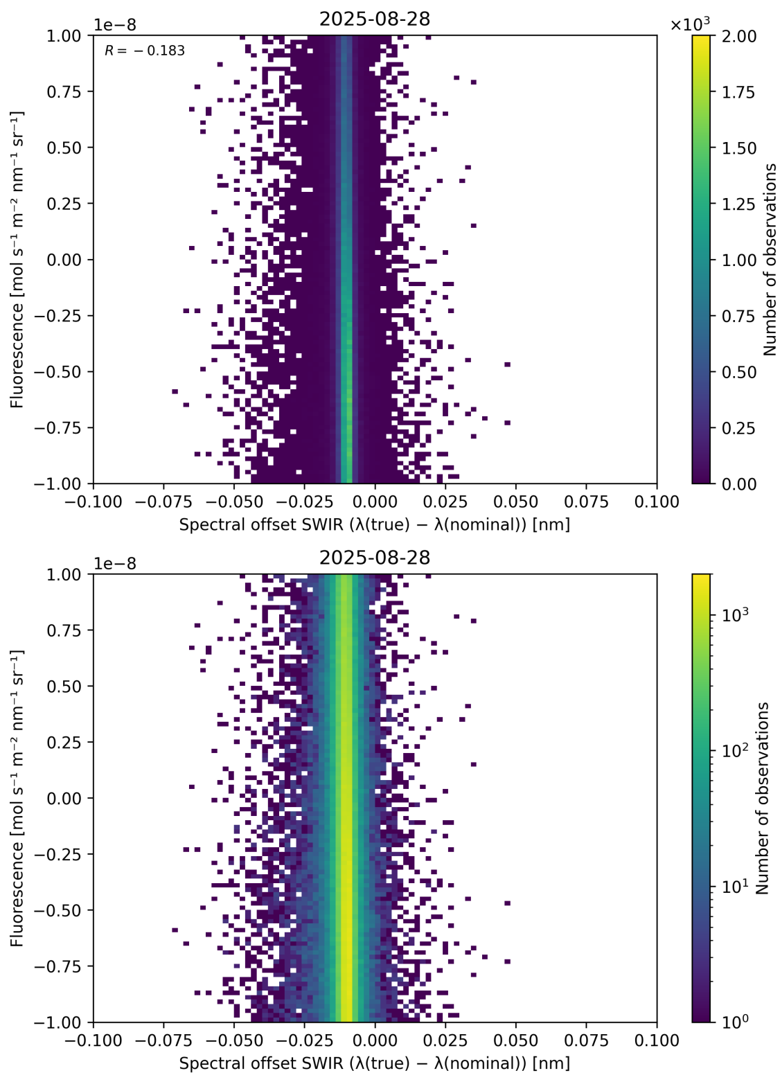
Figure 120: Scatter density plot of “Spectral offset SWIR ( \lambda_{\text{true}} - \lambda_{\text{nominal}} )” against “Fluorescence” for 2025-08-27 to 2025-08-29.
