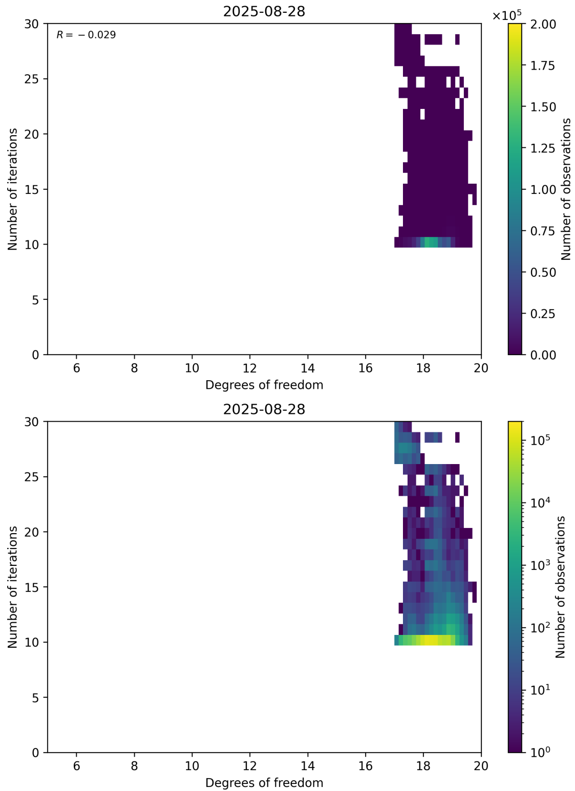
Figure 52: Scatter density plot of “Degrees of freedom” against “Number of iterations” for 2025-08-27 to 2025-08-29.
