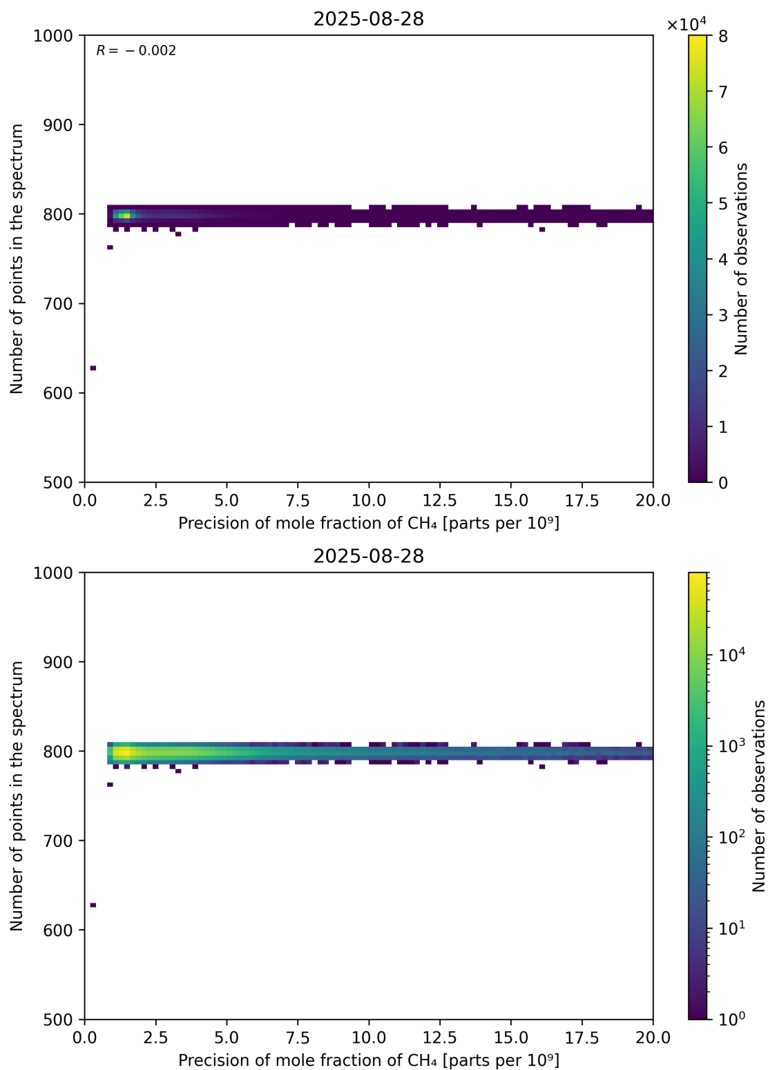
Figure 84: Scatter density plot of “Precision of mole fraction of CH 4 ” against “Number of points in the spectrum” for 2025-08-27 to 2025-08-29.
