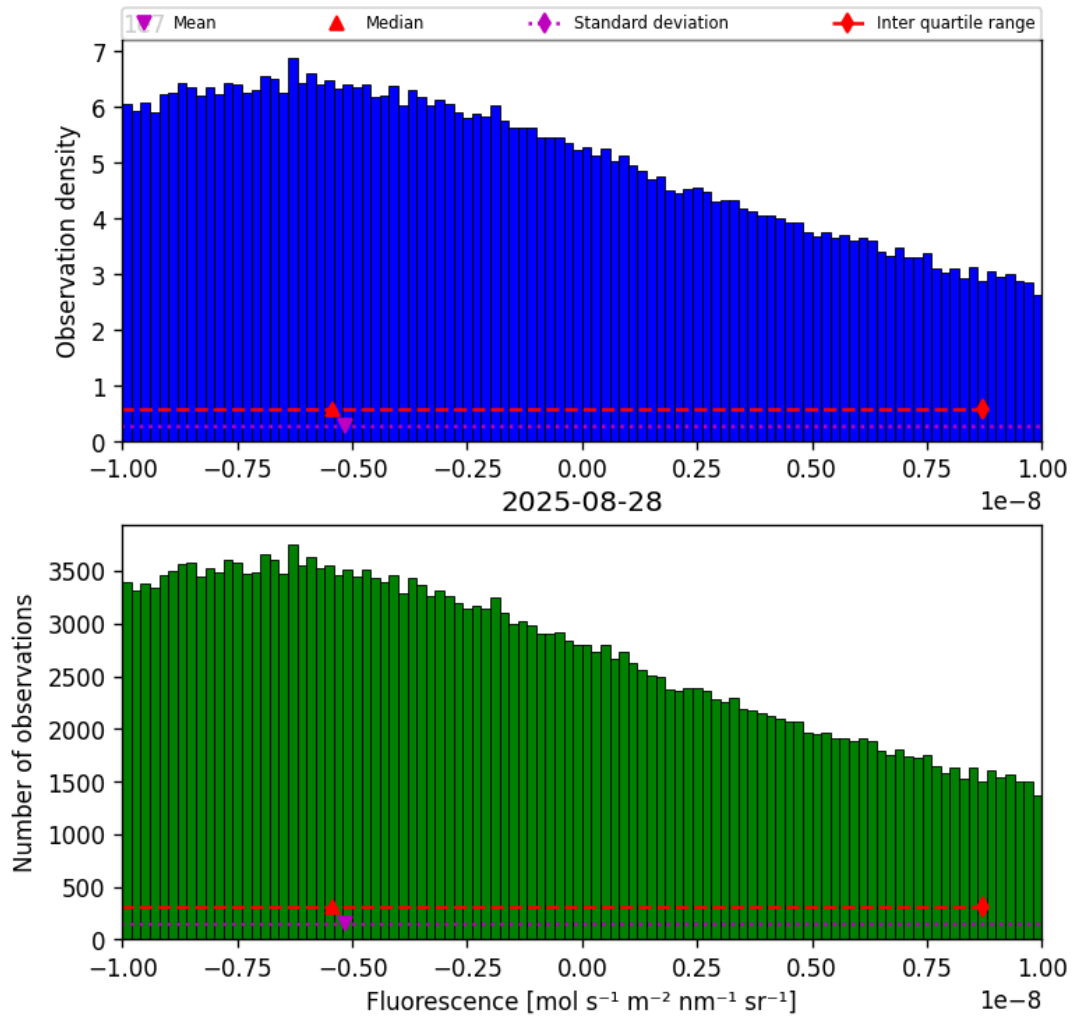
Figure 32: Histogram of “Fluorescence” for 2025-08-27 to 2025-08-29
