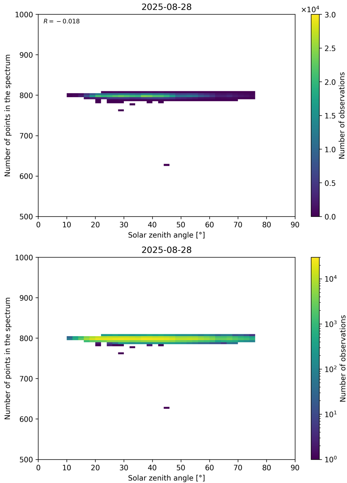
Figure 103: Scatter density plot of “Solar zenith angle” against “Number of points in the spectrum” for 2025-08-27 to 2025-08-29.
