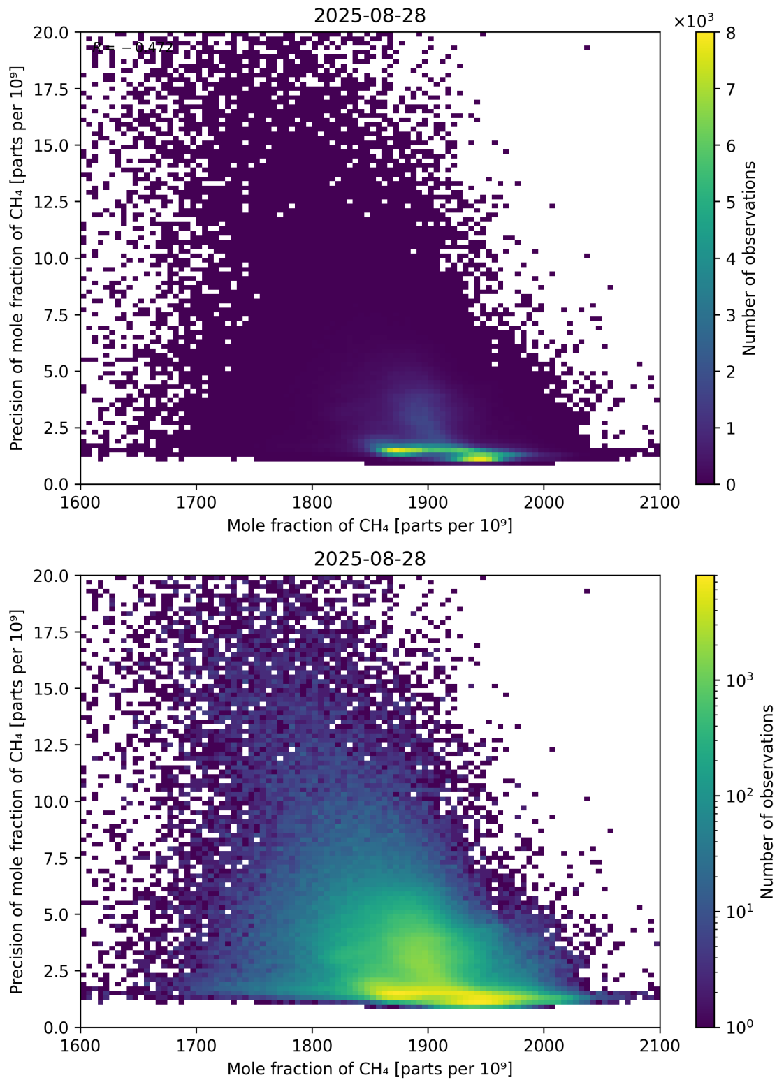
Figure 75: Scatter density plot of “Mole fraction of CH 4 ” against “Precision of mole fraction of CH 4 ” for 2025-08-27 to 2025-08-29.
