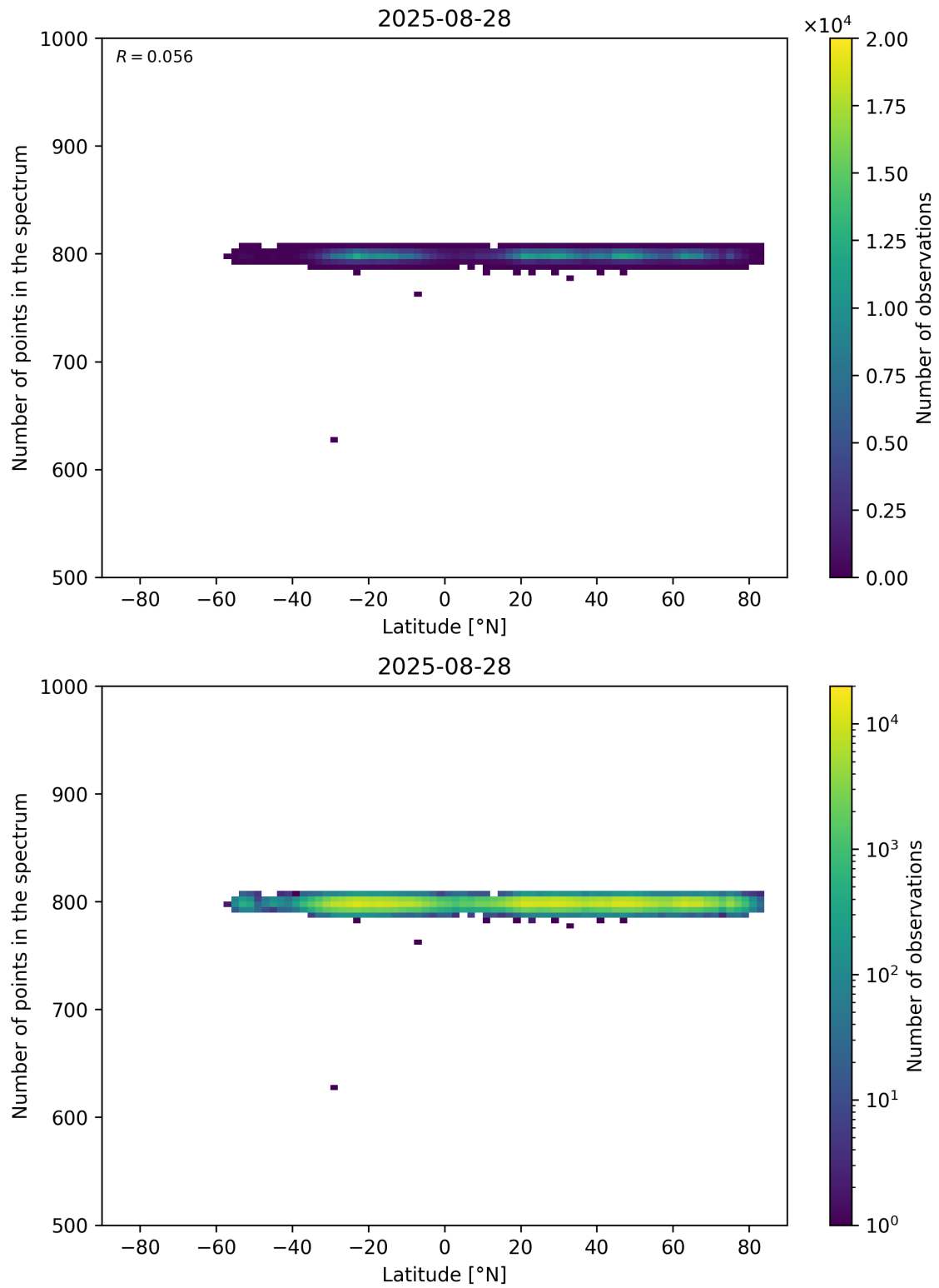
Figure 61: Scatter density plot of “Latitude” against “Number of points in the spectrum” for 2025-08-27 to 2025-08-29.
