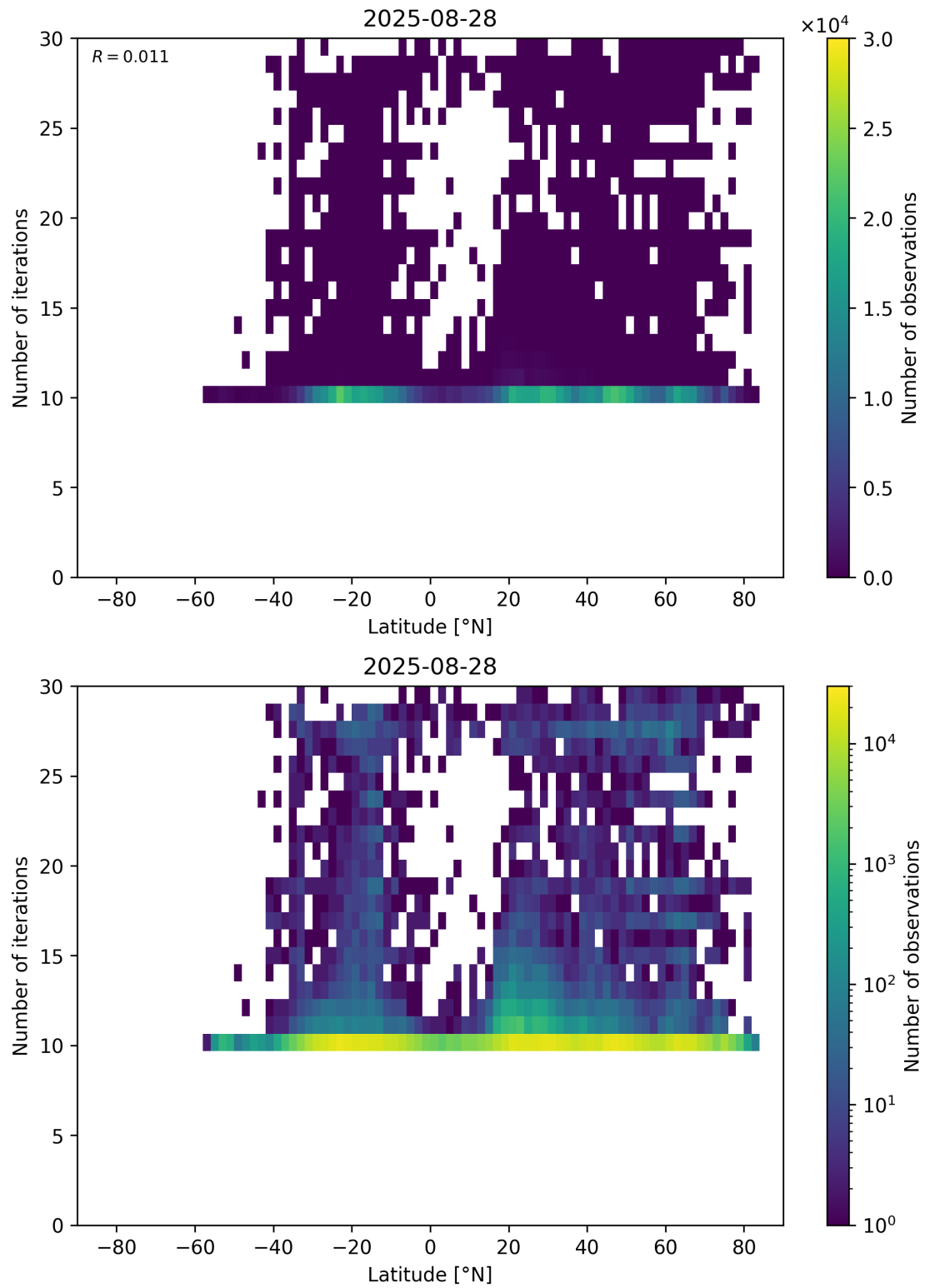
Figure 60: Scatter density plot of “Latitude” against “Number of iterations” for 2025-08-27 to 2025-08-29.
