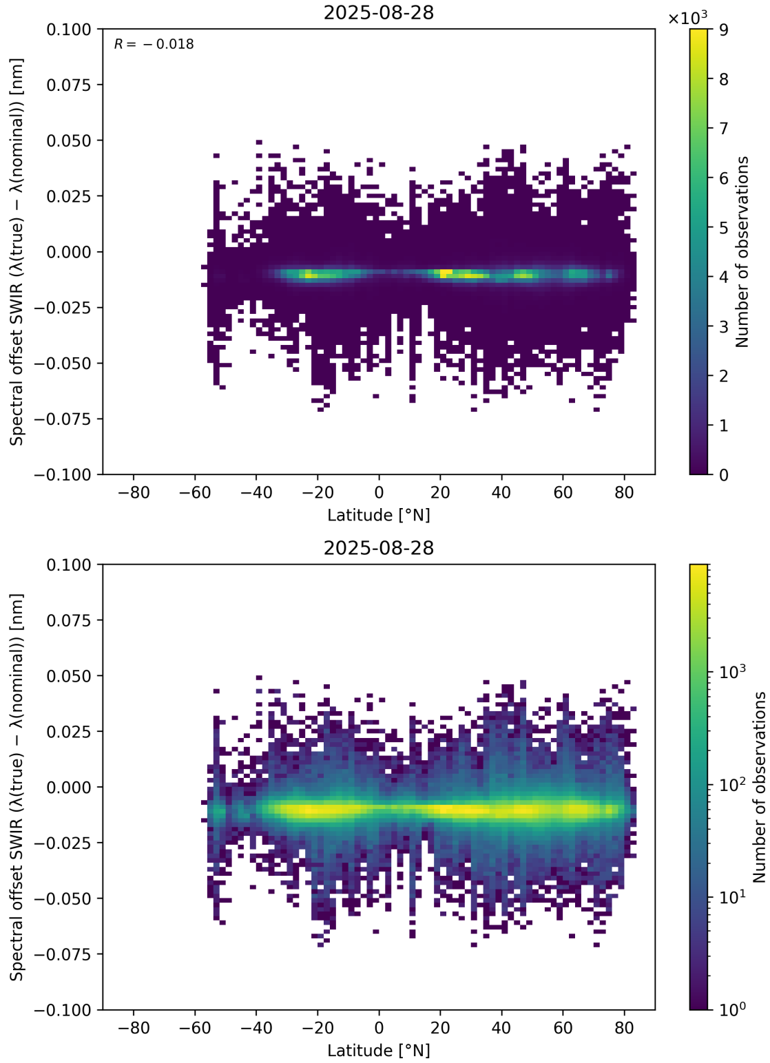
Figure 62: Scatter density plot of “Latitude” against “Spectral offset SWIR ( \lambda_{\text{true}} - \lambda_{\text{nominal}} )” for 2025-08-27 to 2025-08-29.
