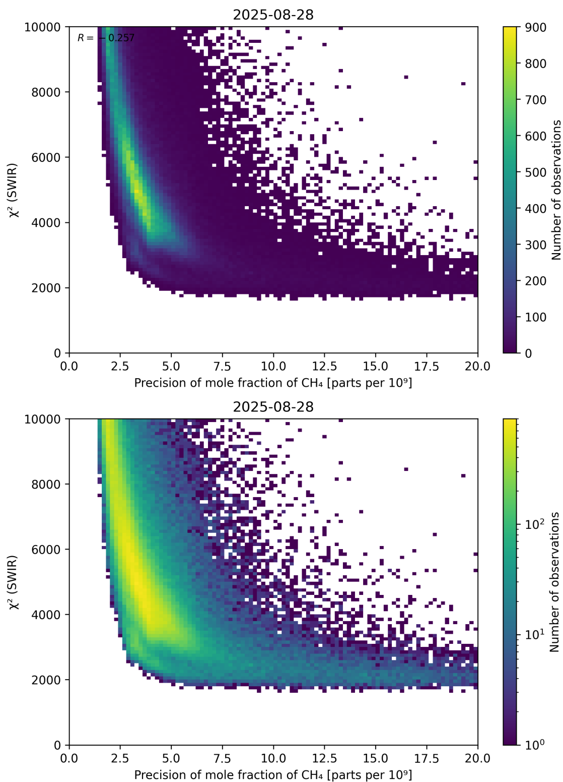
Figure 79: Scatter density plot of “Precision of mole fraction of \text{CH}_4 ” against “ \chi^2 (SWIR)” for 2025-08-27 to 2025-08-29.
