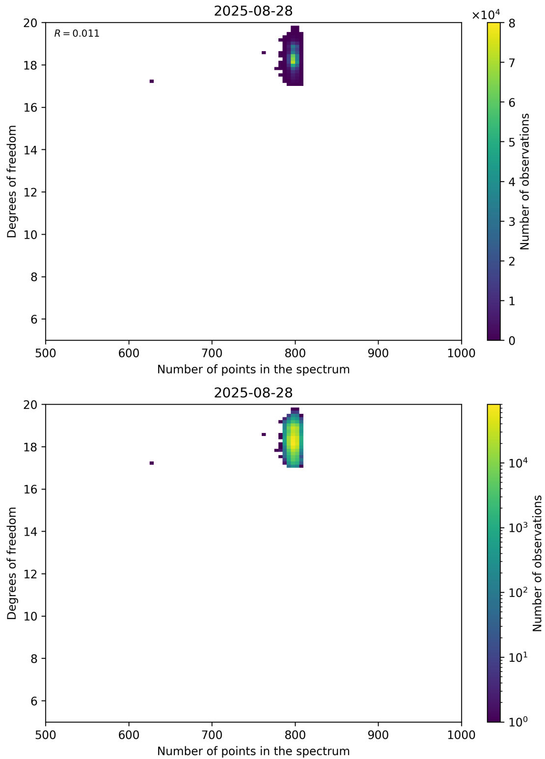
Figure 90: Scatter density plot of “Number of points in the spectrum” against “Degrees of freedom” for 2025-08-27 to 2025-08-29.
