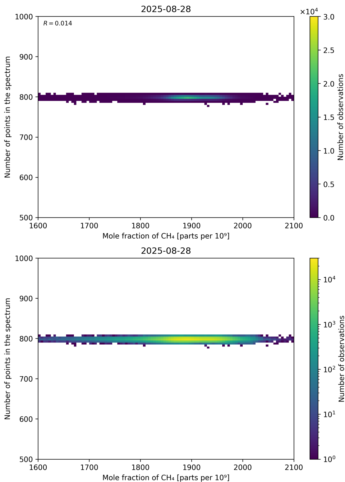
Figure 77: Scatter density plot of “Mole fraction of CH 4 ” against “Number of points in the spectrum” for 2025-08-27 to 2025-08-29.
