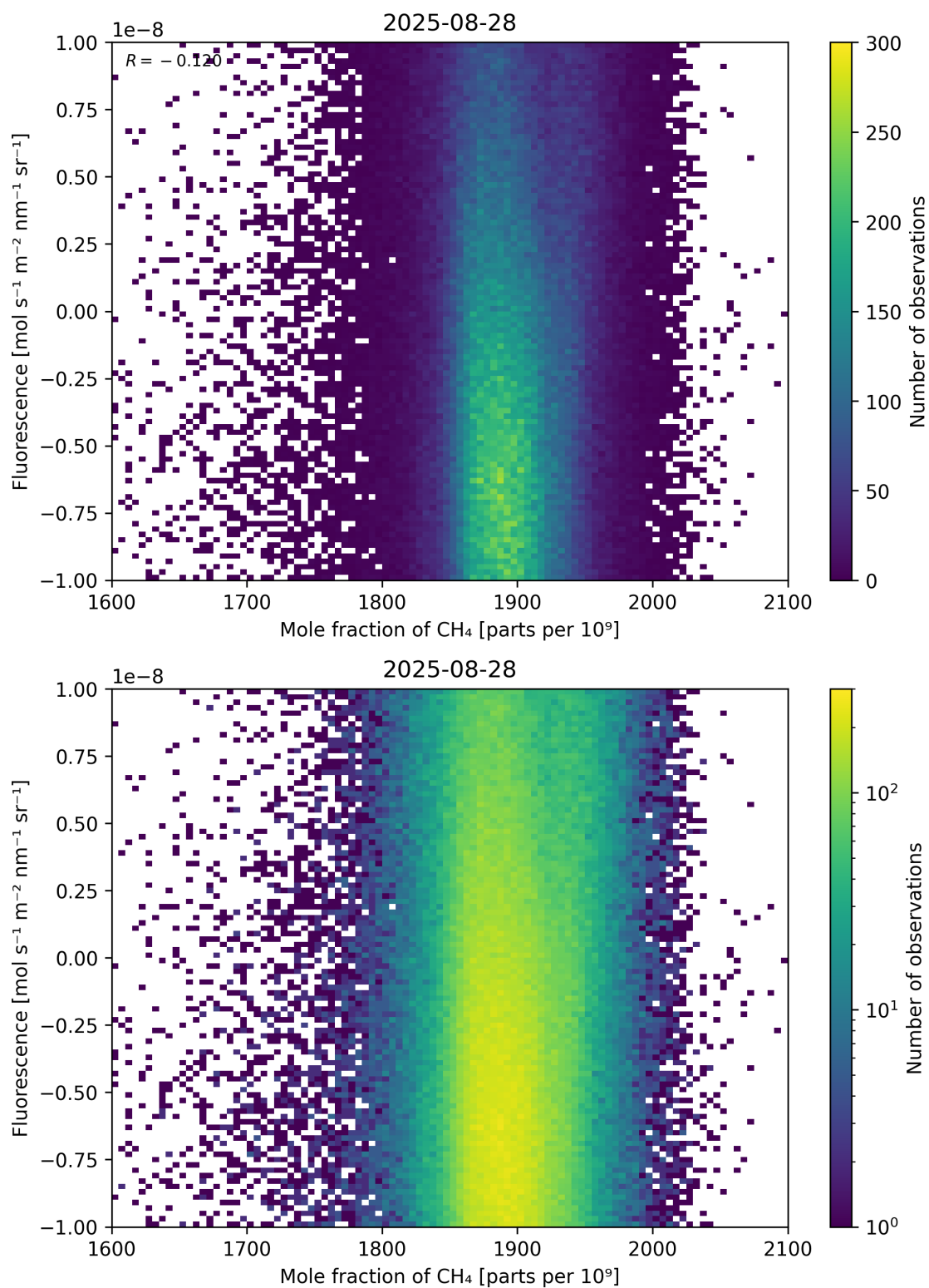
Figure 73: Scatter density plot of “Mole fraction of CH 4 ” against “Fluorescence” for 2025-08-27 to 2025-08-29.
