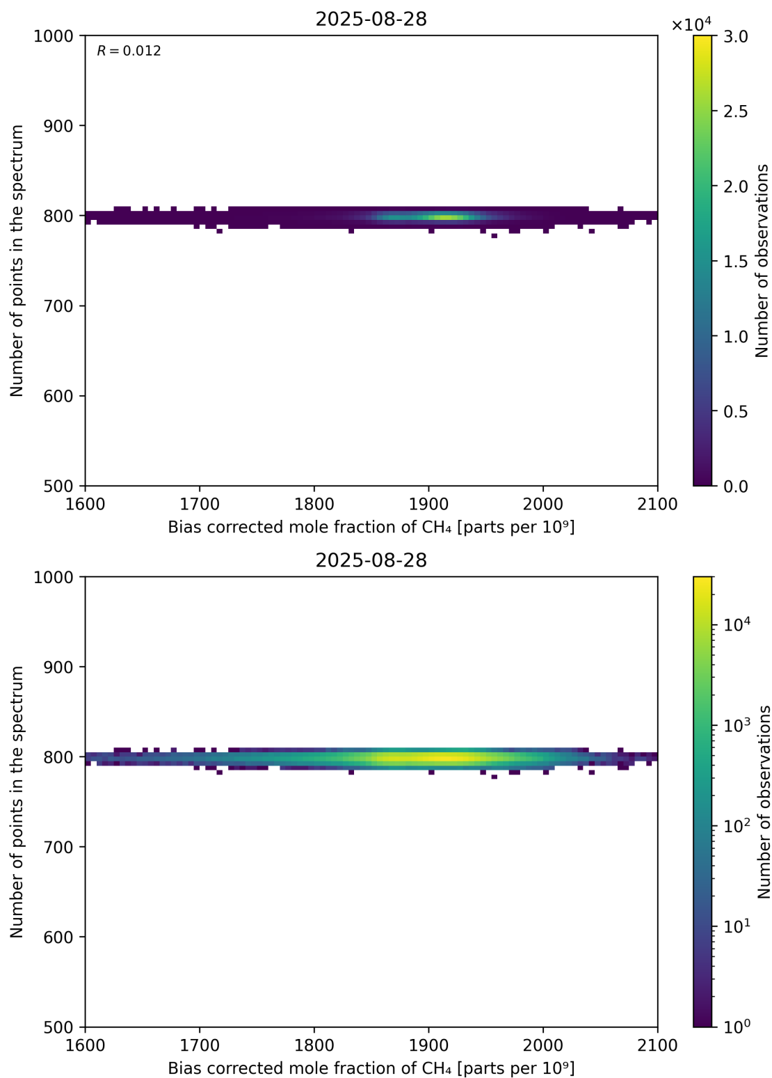
Figure 68: Scatter density plot of “Bias corrected mole fraction of CH 4 ” against “Number of points in the spectrum” for 2025-08-27 to 2025-08-29.
