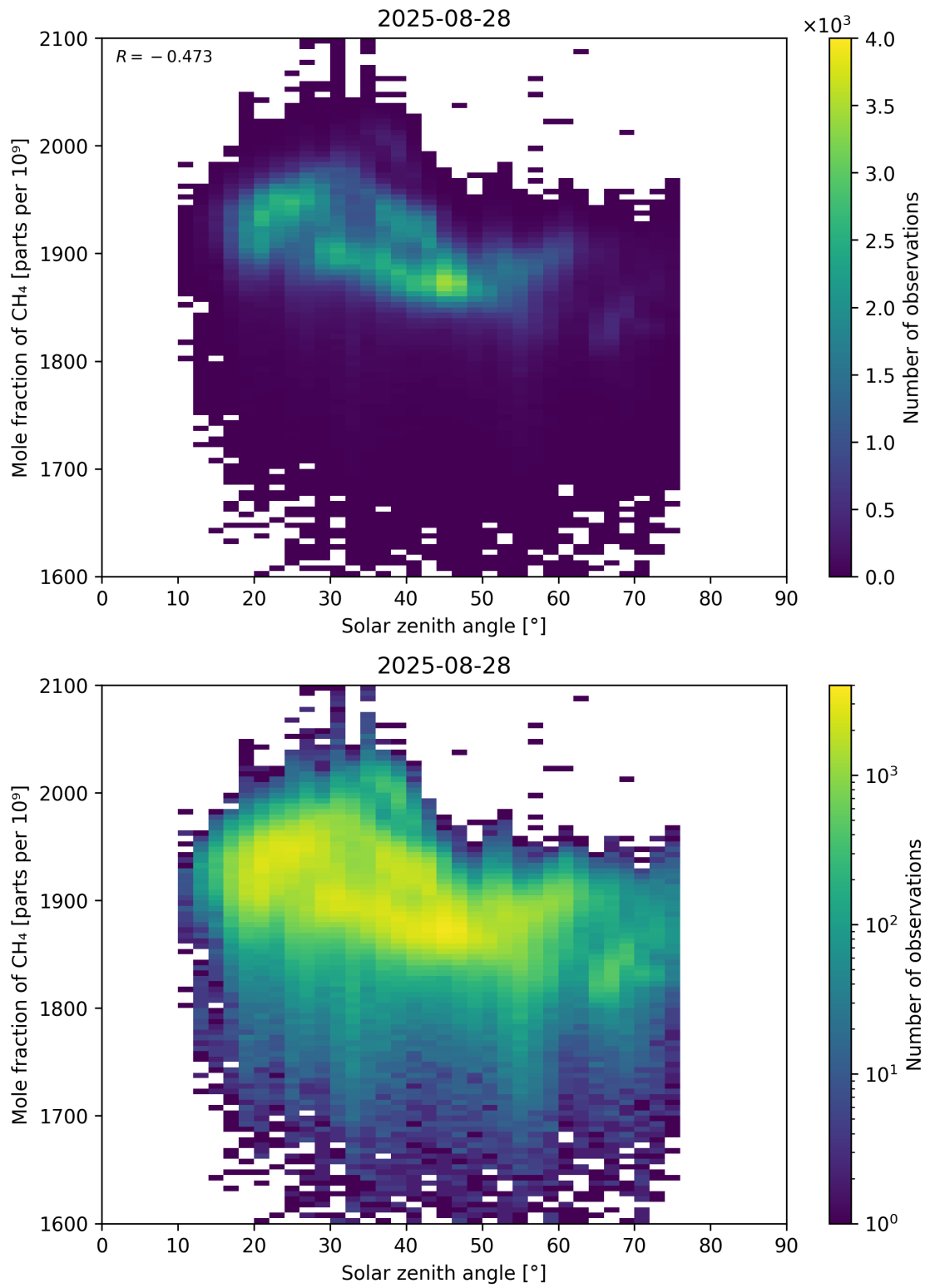
Figure 99: Scatter density plot of “Solar zenith angle” against “Mole fraction of CH 4 ” for 2025-08-27 to 2025-08-29.
