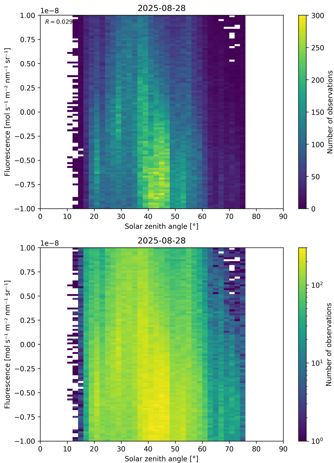
Figure 97: Scatter density plot of “Solar zenith angle” against “Fluorescence” for 2025-08-27 to 2025-08-29.
