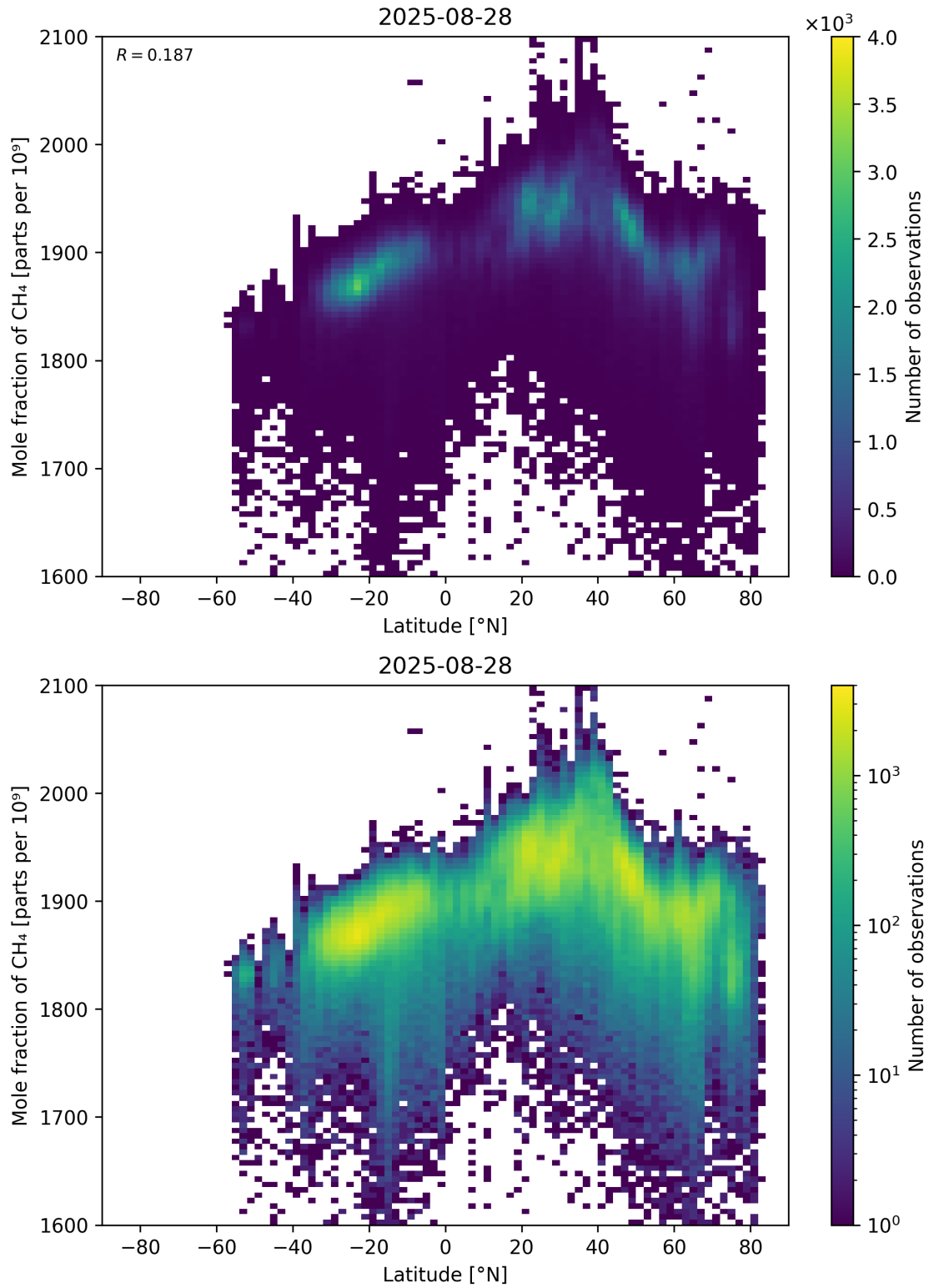
Figure 57: Scatter density plot of “Latitude” against “Mole fraction of \text{CH}_4 ” for 2025-08-27 to 2025-08-29.
