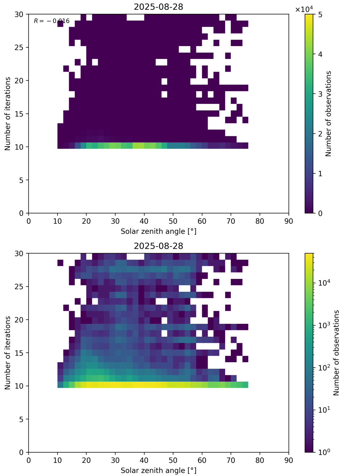
Figure 102: Scatter density plot of “Solar zenith angle” against “Number of iterations” for 2025-08-27 to 2025-08-29.
