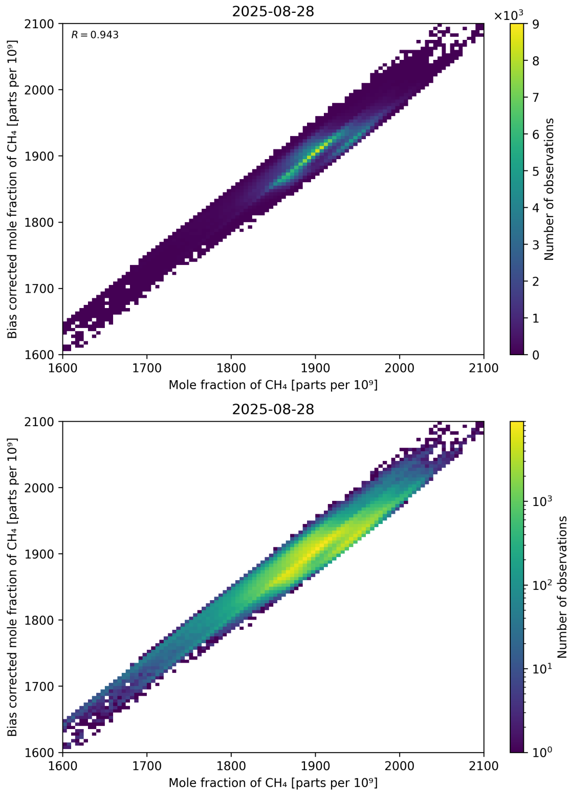
Figure 74: Scatter density plot of “Mole fraction of CH 4 ” against “Bias corrected mole fraction of CH 4 ” for 2025-08-27 to 2025-08-29.
