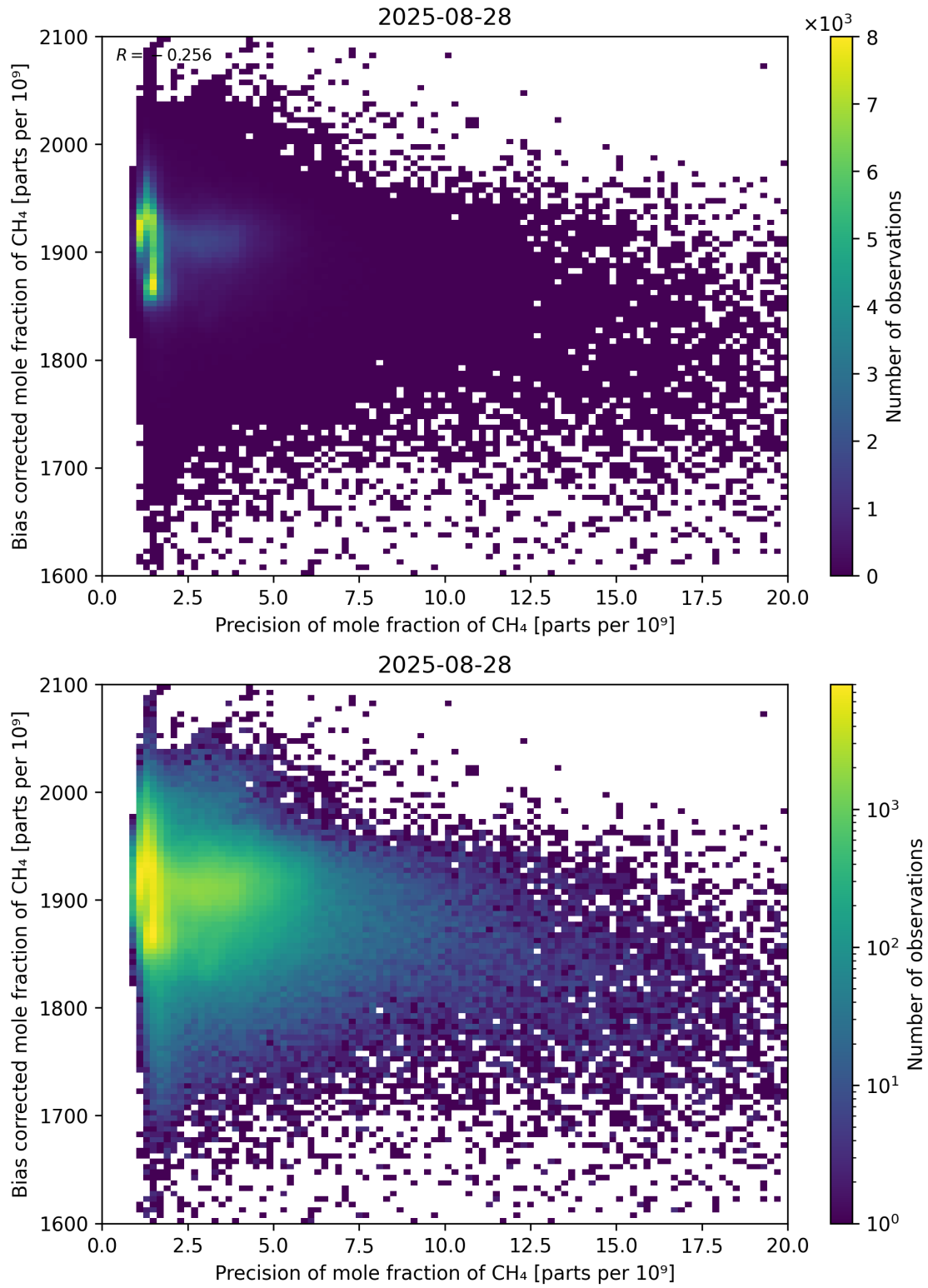
Figure 82: Scatter density plot of “Precision of mole fraction of CH 4 ” against “Bias corrected mole fraction of CH 4 ” for 2025-08-27 to 2025-08-29.
