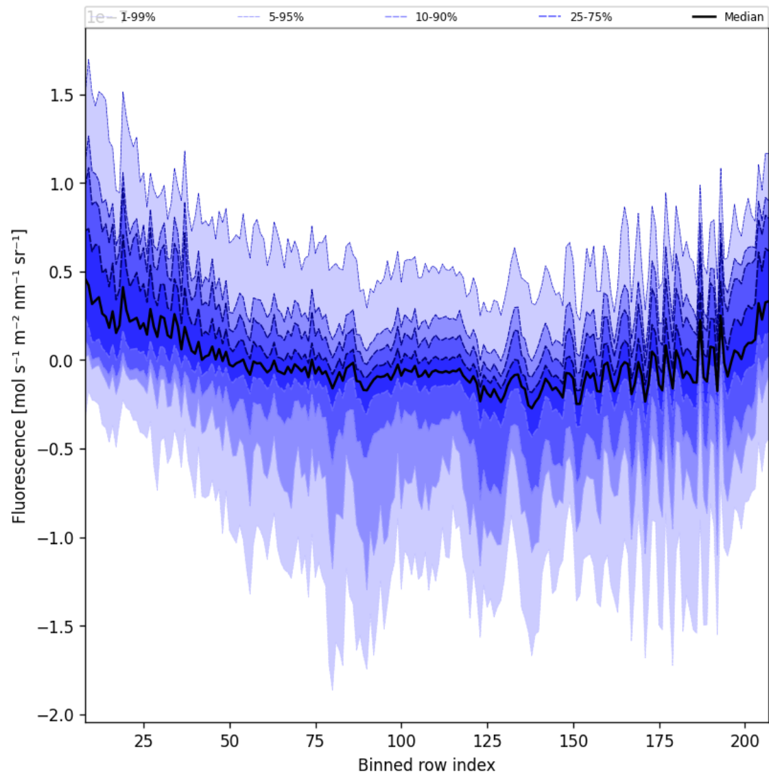
Figure 43: Along track statistics of “Fluorescence” for 2025-08-27 to 2025-08-29
