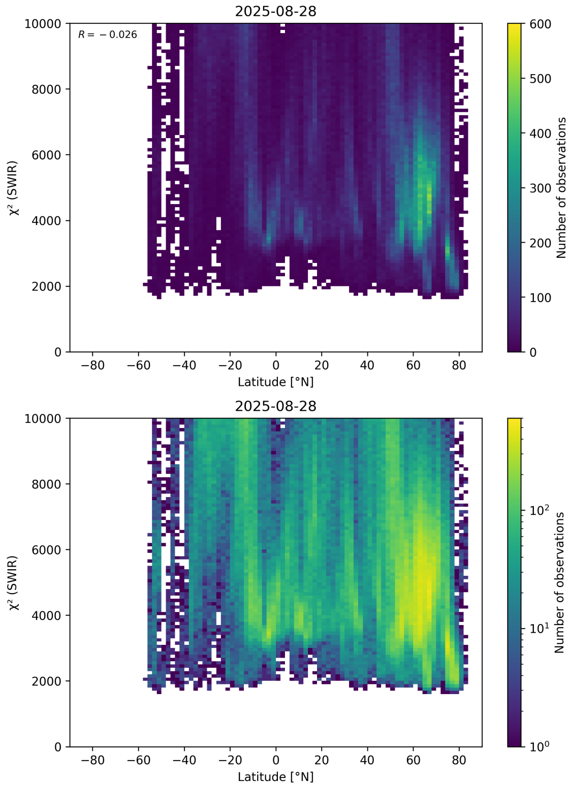
Figure 54: Scatter density plot of “Latitude” against “ \chi^2 (SWIR)” for 2025-08-27 to 2025-08-29.
