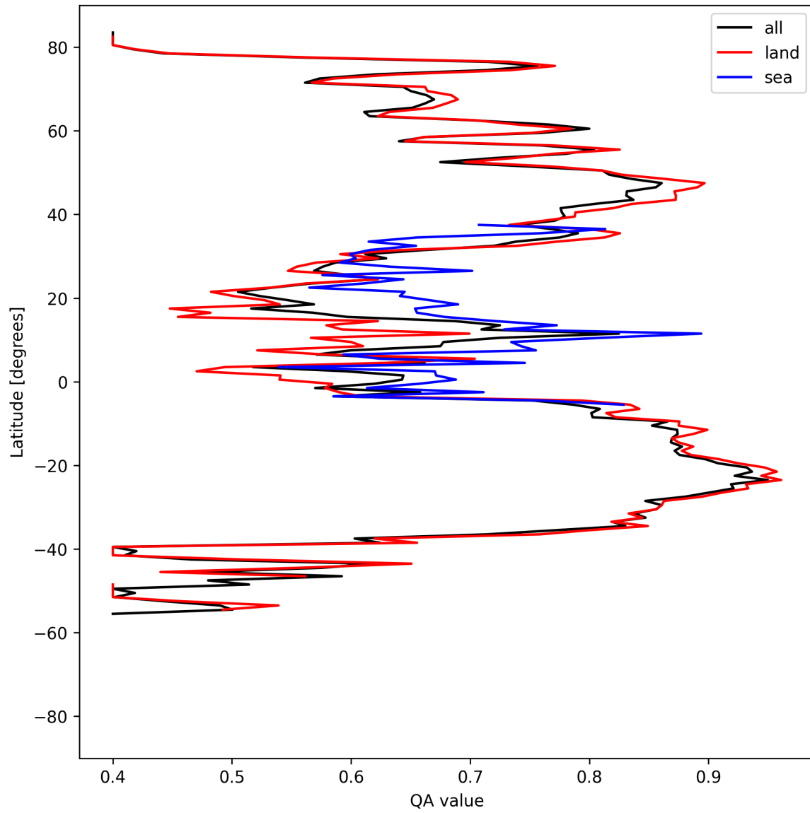
Figure 11: Zonal average of “QA value” for 2025-08-27 to 2025-08-29.
