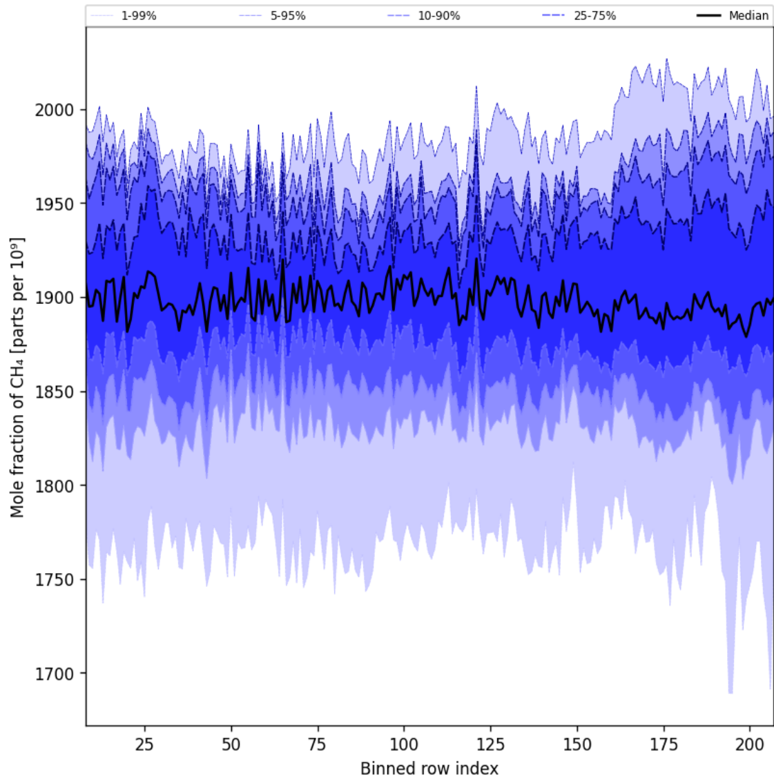
Figure 34: Along track statistics of “Mole fraction of CH 4 ” for 2025-08-27 to 2025-08-29
