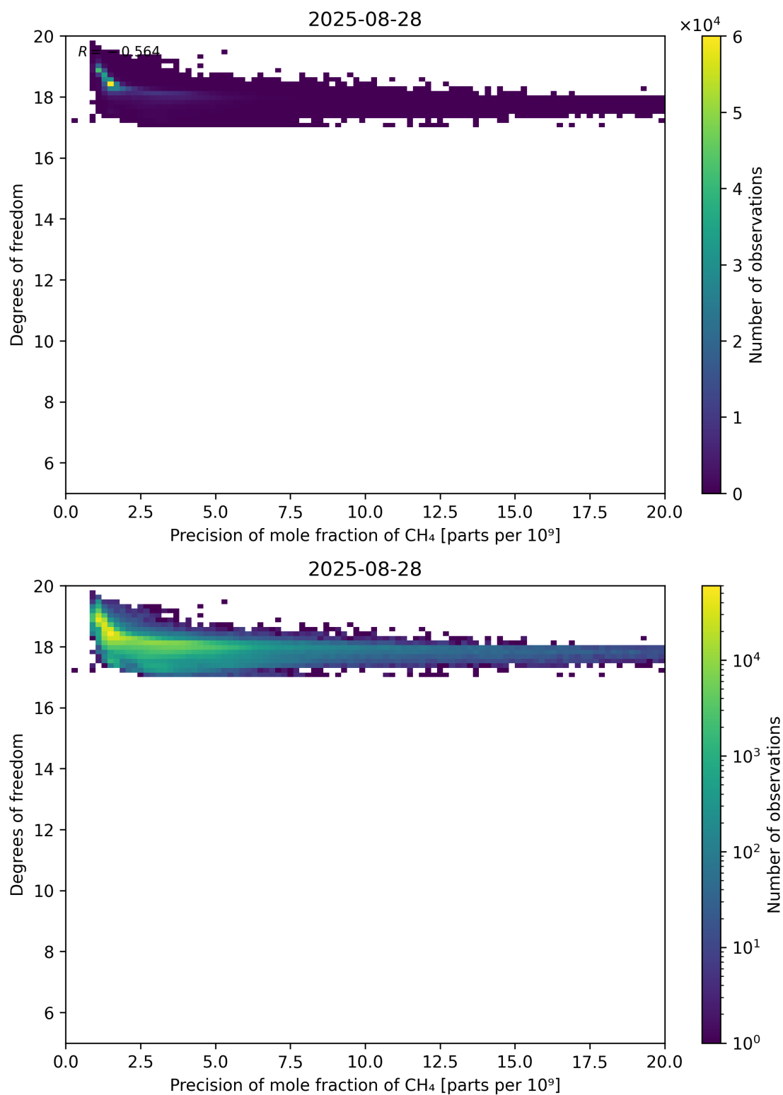
Figure 80: Scatter density plot of “Precision of mole fraction of CH 4 ” against “Degrees of freedom” for 2025-08-27 to 2025-08-29.
