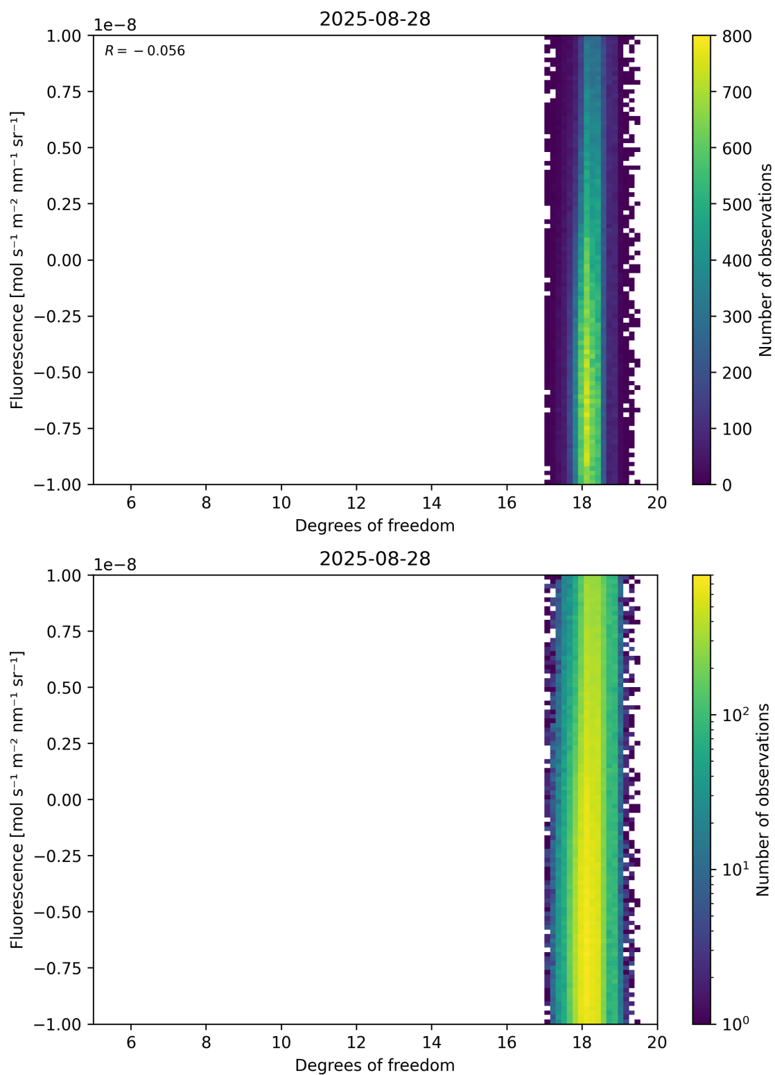
Figure 51: Scatter density plot of “Degrees of freedom” against “Fluorescence” for 2025-08-27 to 2025-08-29.
