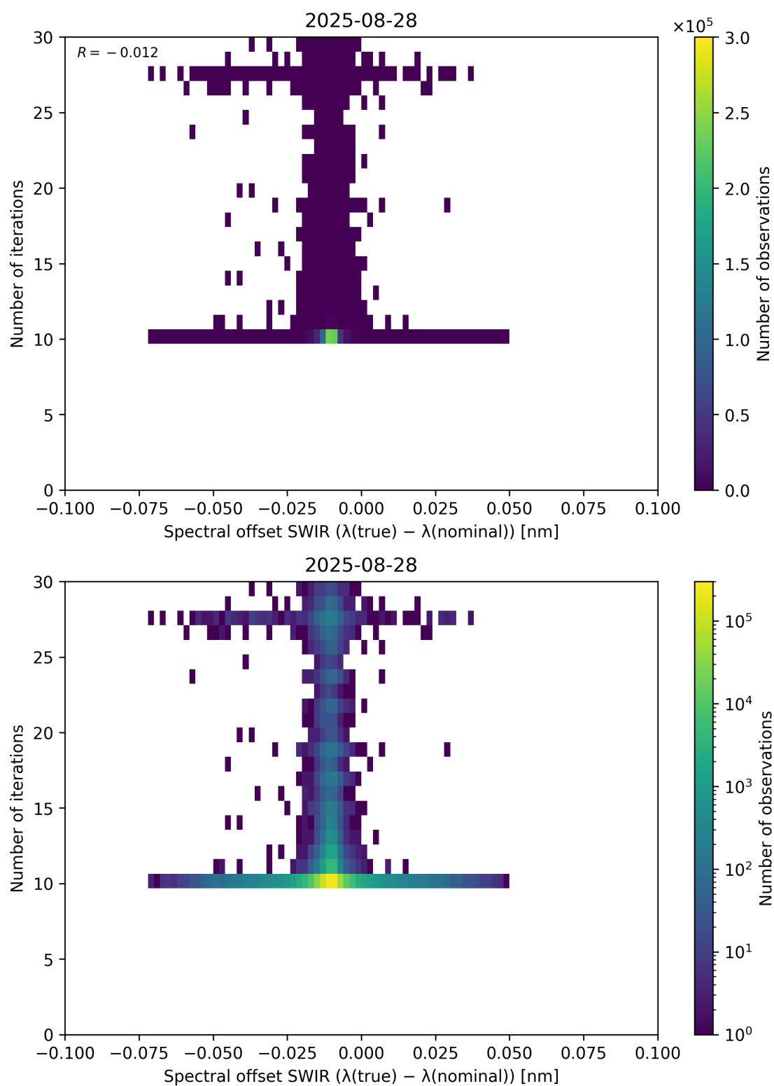
Figure 121: Scatter density plot of “Spectral offset SWIR ( \lambda_{\text{true}} - \lambda_{\text{nominal}} )” against “Number of iterations” for 2025-08-27 to 2025-08-29.
