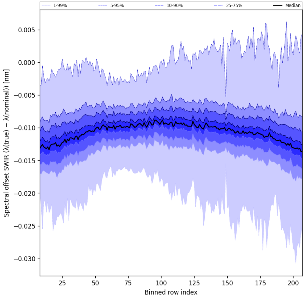
Figure 38: Along track statistics of “Spectral offset SWIR ( \lambda_{\text{true}} - \lambda_{\text{nominal}} )” for 2025-08-27 to 2025-08-29
