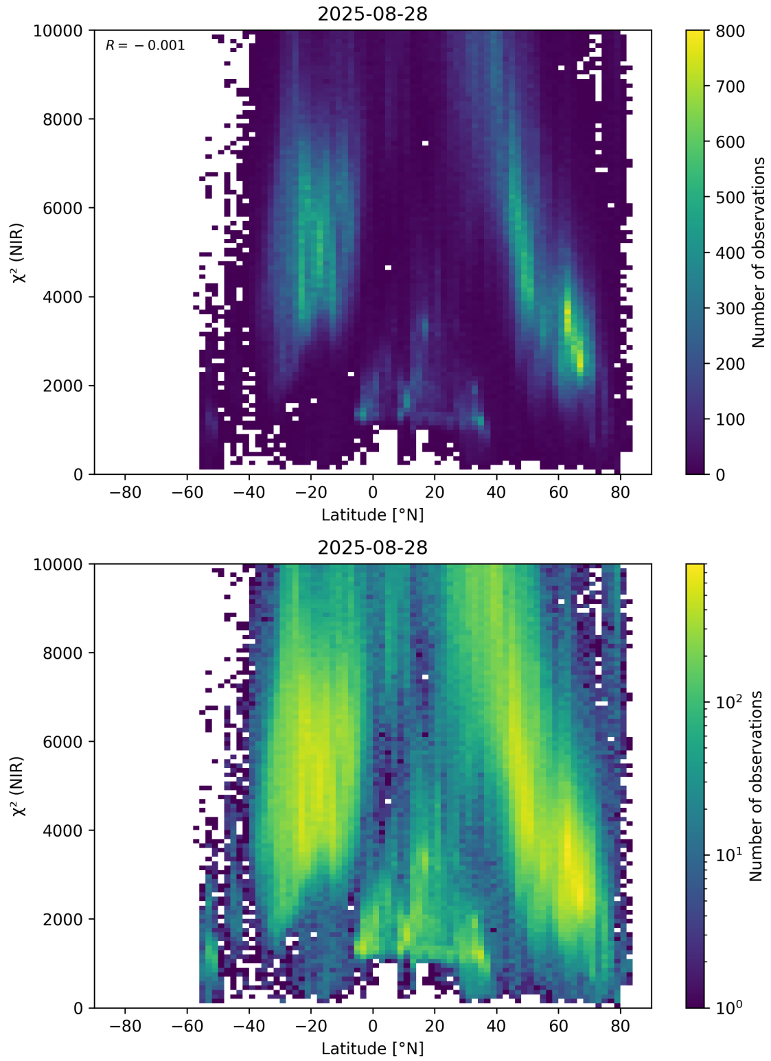
Figure 53: Scatter density plot of “Latitude” against “ \chi^2 (NIR)” for 2025-08-27 to 2025-08-29.
