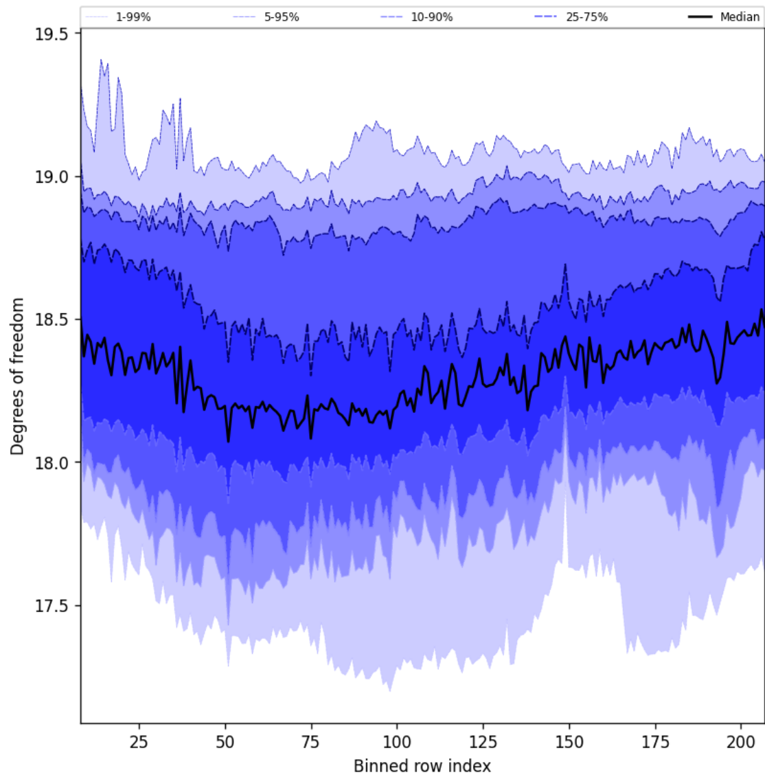
Figure 41: Along track statistics of “Degrees of freedom” for 2025-08-27 to 2025-08-29
