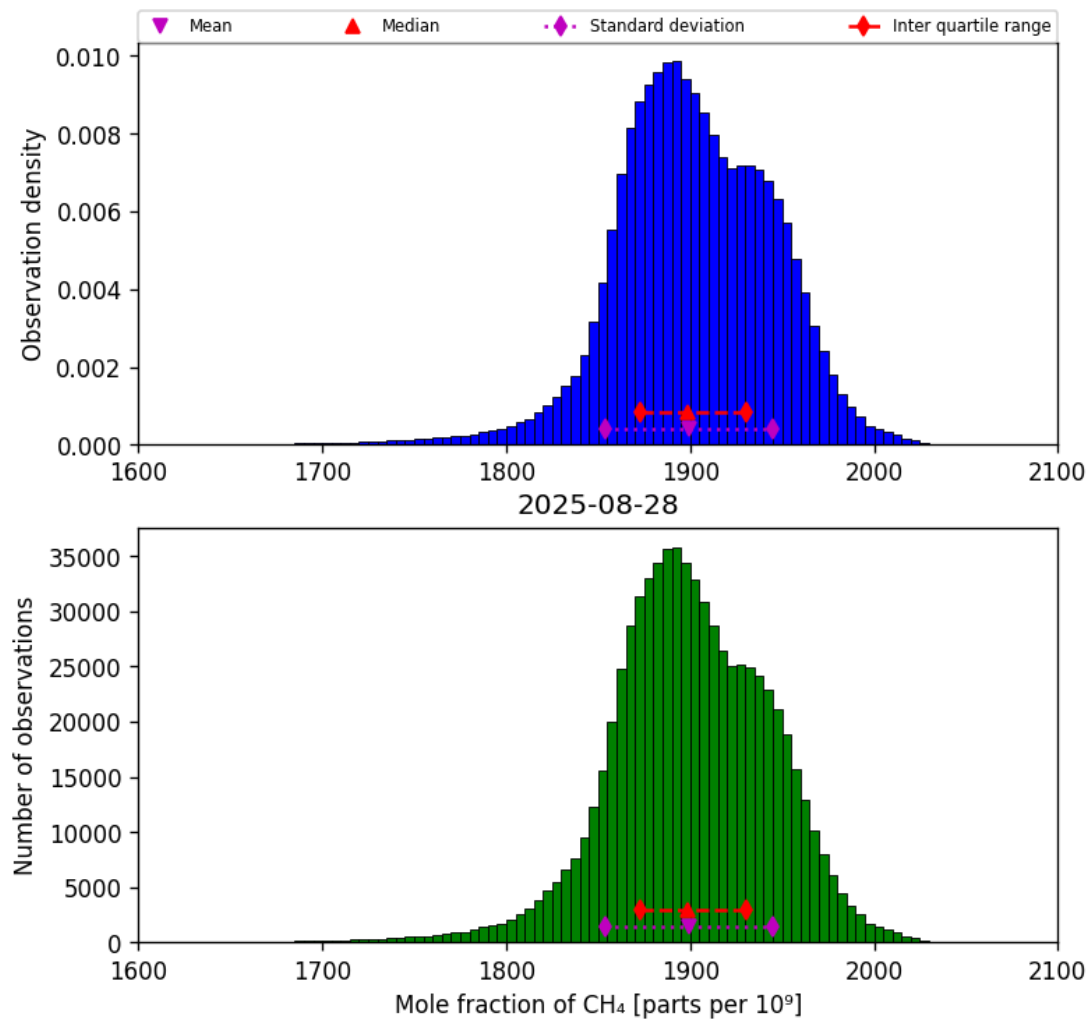
Figure 23: Histogram of “Mole fraction of CH 4 ” for 2025-08-27 to 2025-08-29
