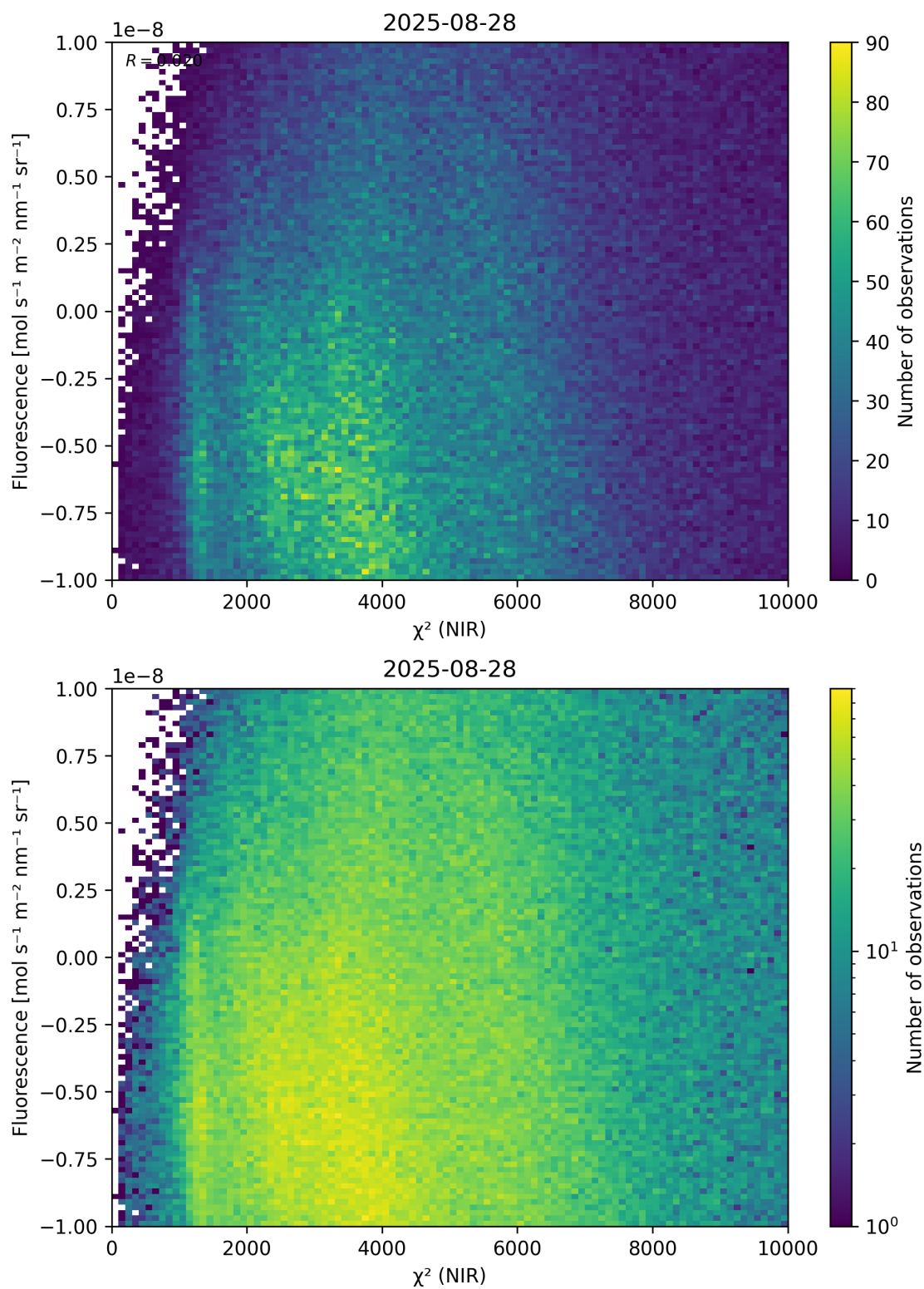
Figure 45: Scatter density plot of “ \chi^2 (NIR)” against “Fluorescence” for 2025-08-27 to 2025-08-29.
