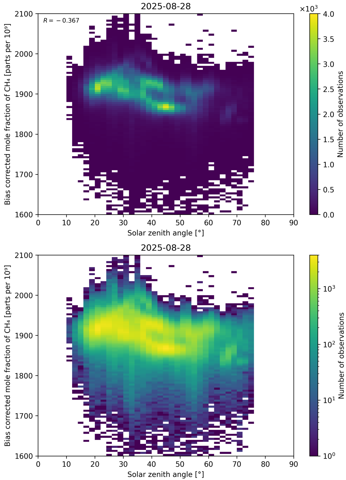
Figure 100: Scatter density plot of “Solar zenith angle” against “Bias corrected mole fraction of CH 4 ” for 2025-08-27 to 2025-08-29.
