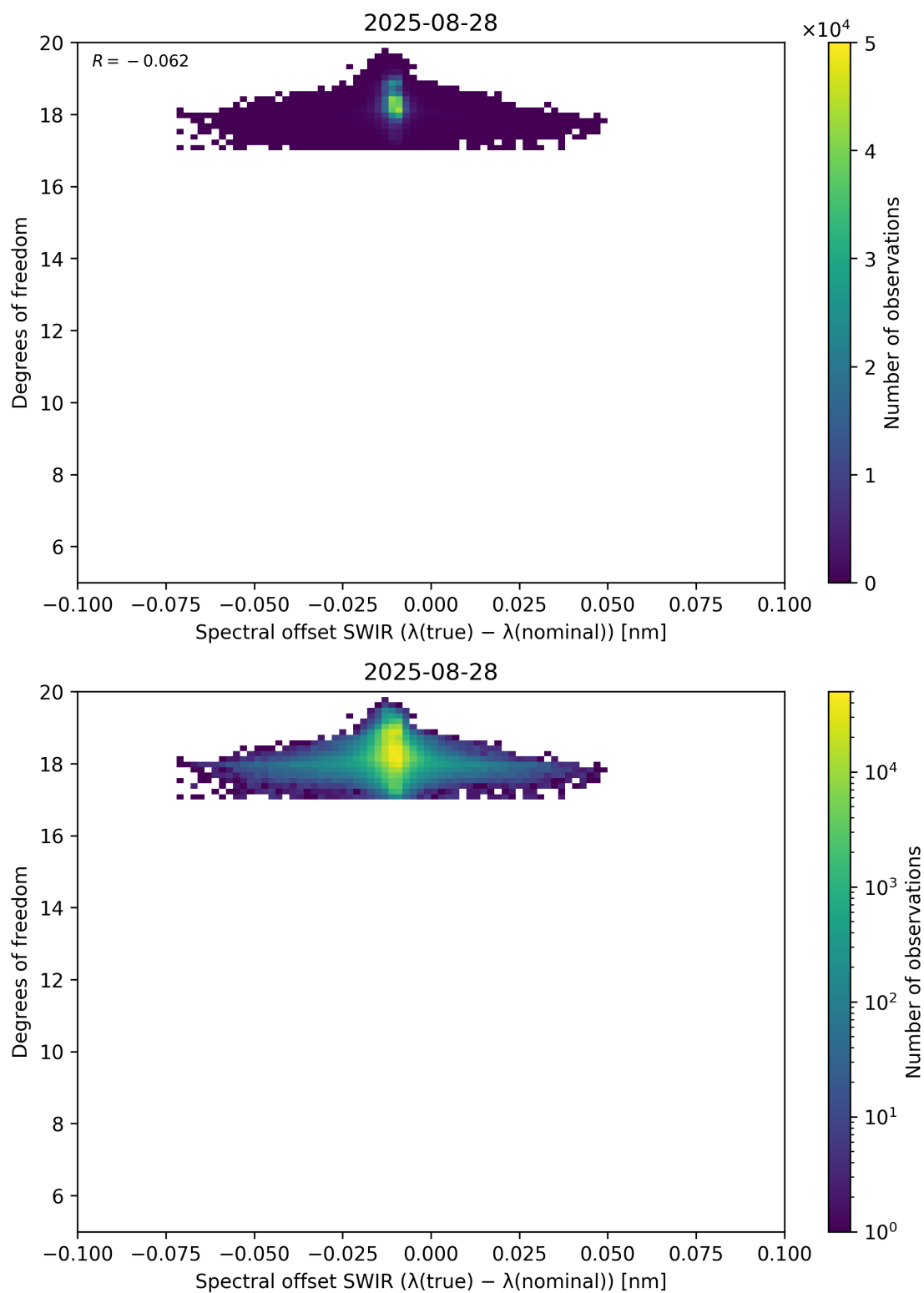
Figure 119: Scatter density plot of “Spectral offset SWIR ( \lambda_{\text{true}} - \lambda_{\text{nominal}} )” against “Degrees of freedom” for 2025-08-27 to 2025-08-29.
