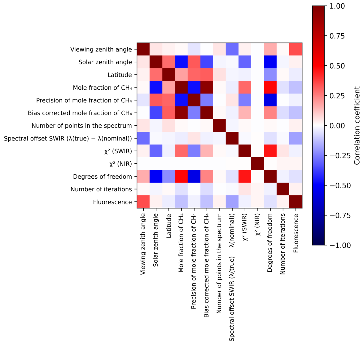
Figure 2: Map of correlation matrix for 2025-08-27 to 2025-08-29.
