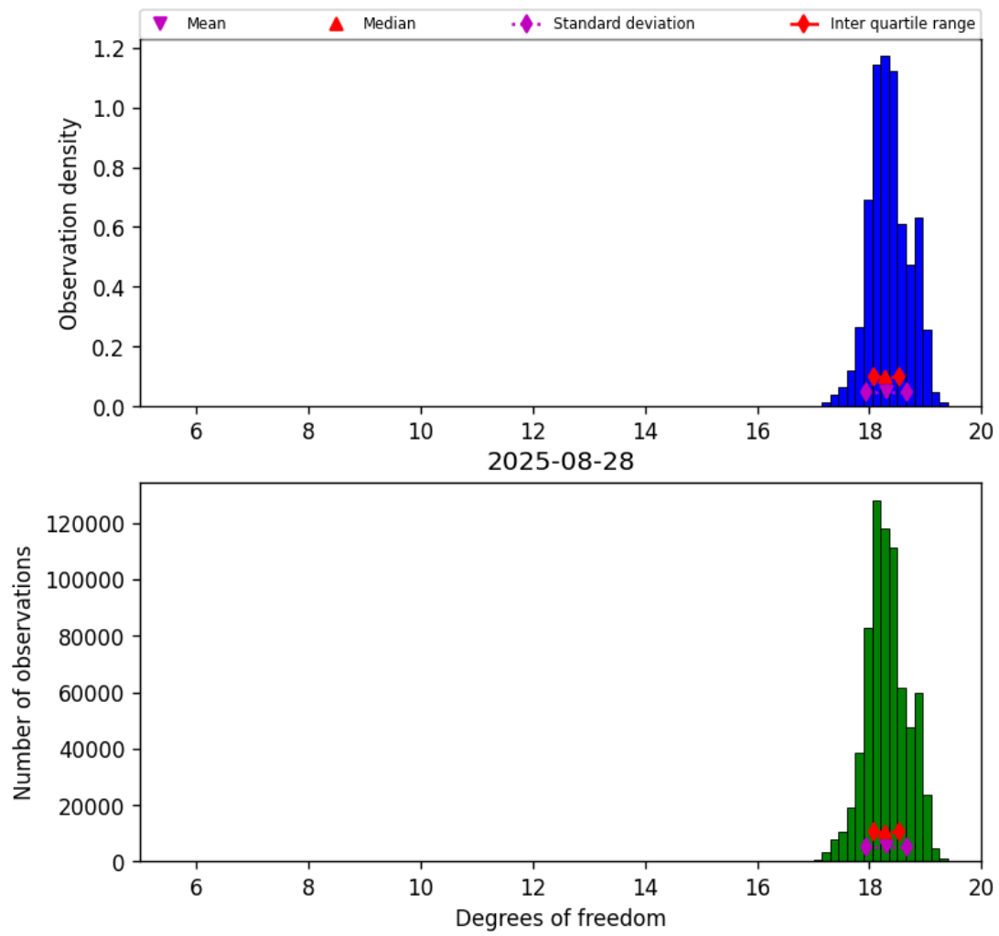
Figure 30: Histogram of “Degrees of freedom” for 2025-08-27 to 2025-08-29
