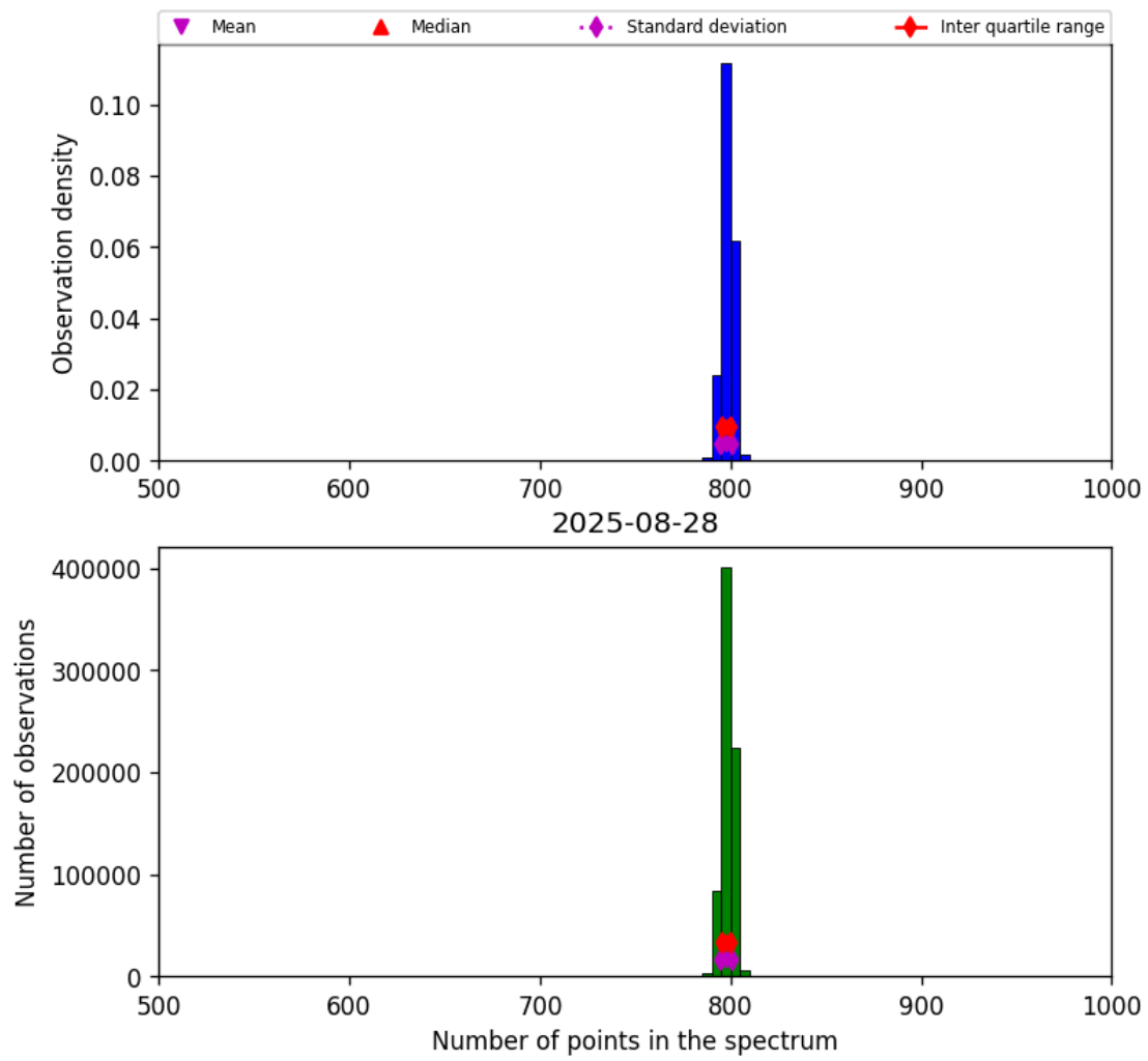
Figure 26: Histogram of “Number of points in the spectrum” for 2025-08-27 to 2025-08-29
