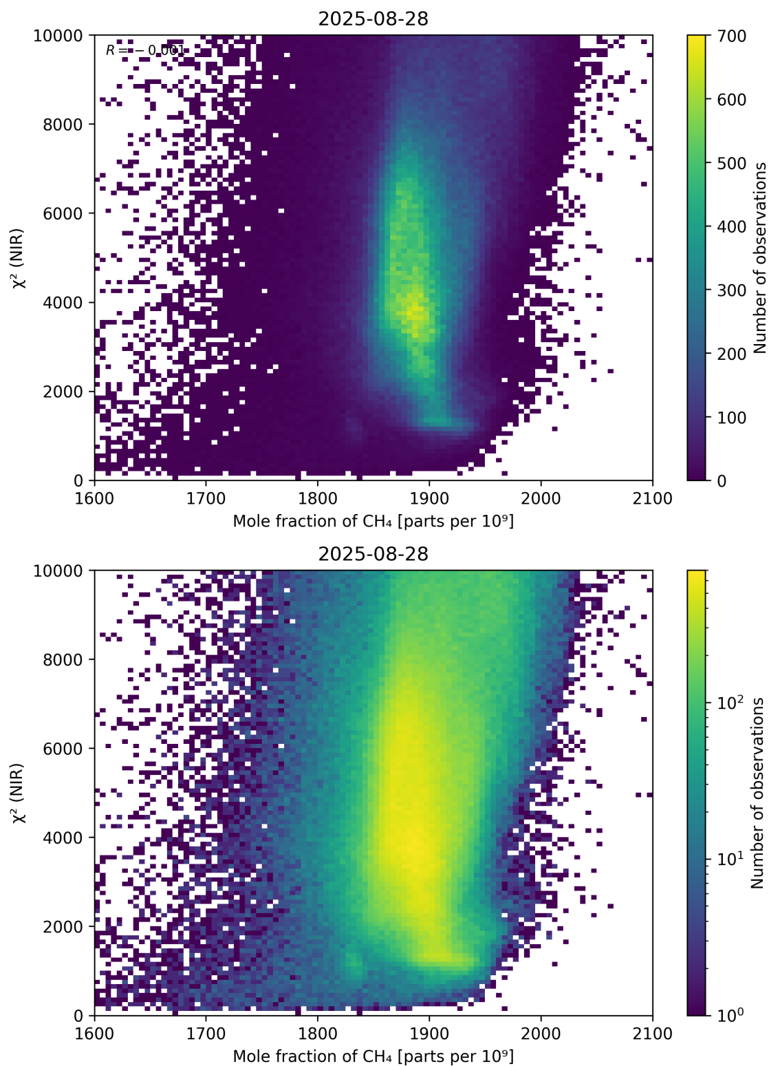
Figure 70: Scatter density plot of “Mole fraction of \text{CH}_4 ” against “ \chi^2 (NIR)” for 2025-08-27 to 2025-08-29.
