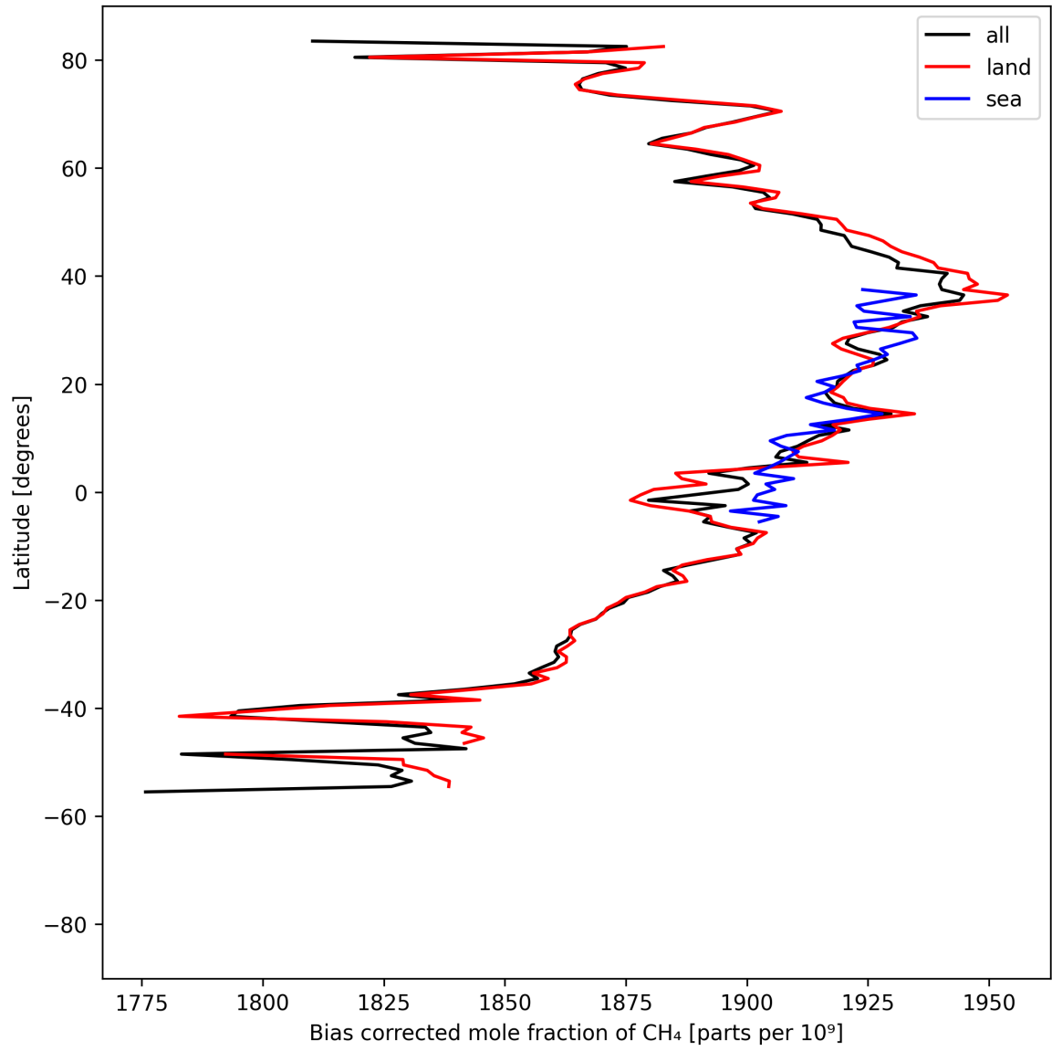
Figure 14: Zonal average of “Bias corrected mole fraction of CH 4 ” for 2025-08-27 to 2025-08-29.
