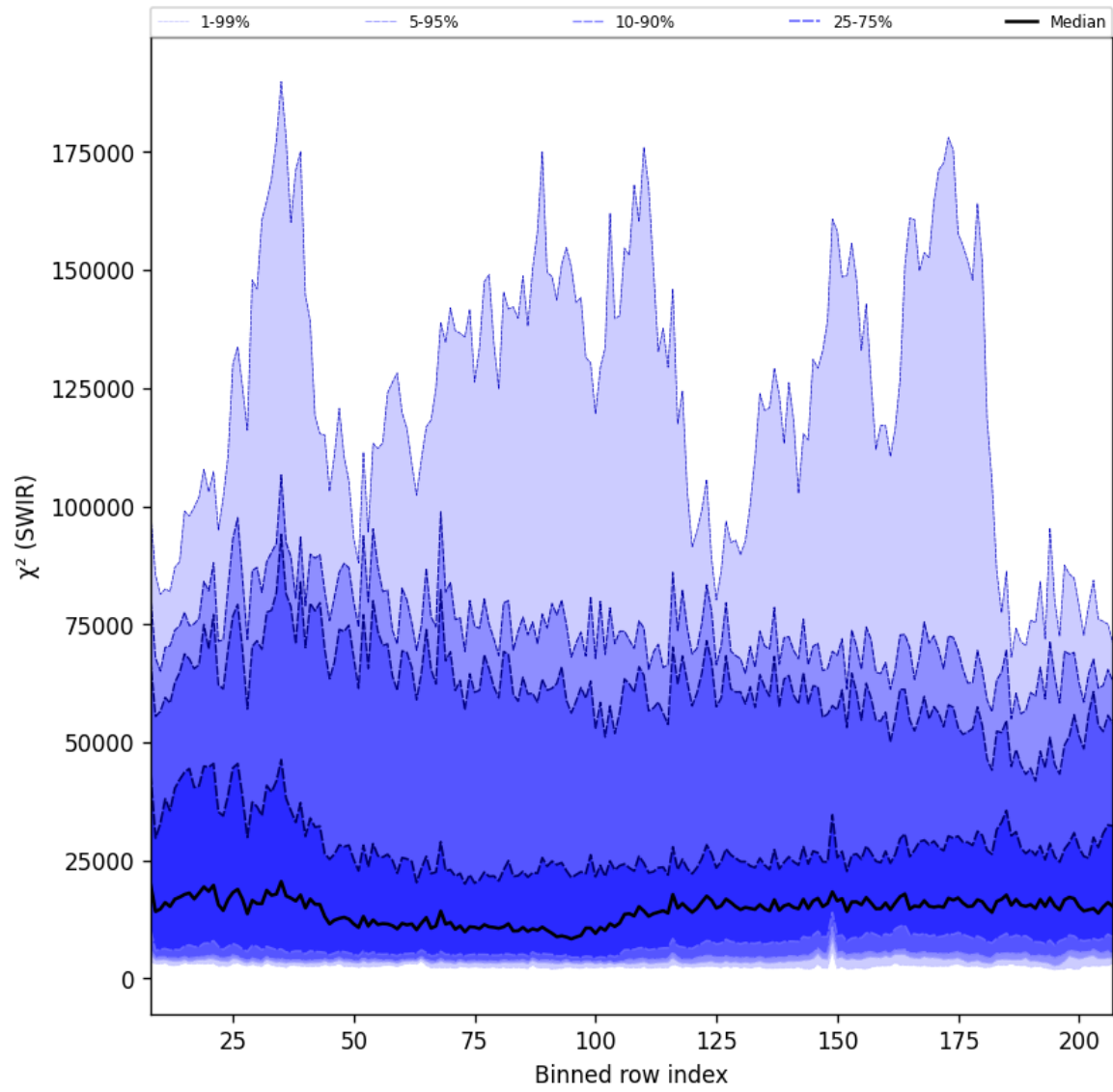
Figure 39: Along track statistics of " \chi^2 (SWIR)" for 2025-08-27 to 2025-08-29
