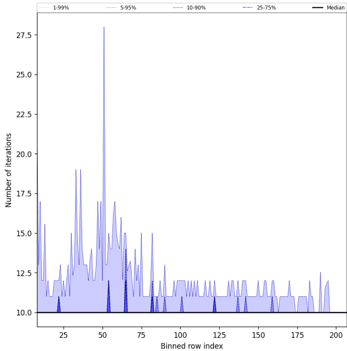
Figure 42: Along track statistics of “Number of iterations” for 2025-08-27 to 2025-08-29
