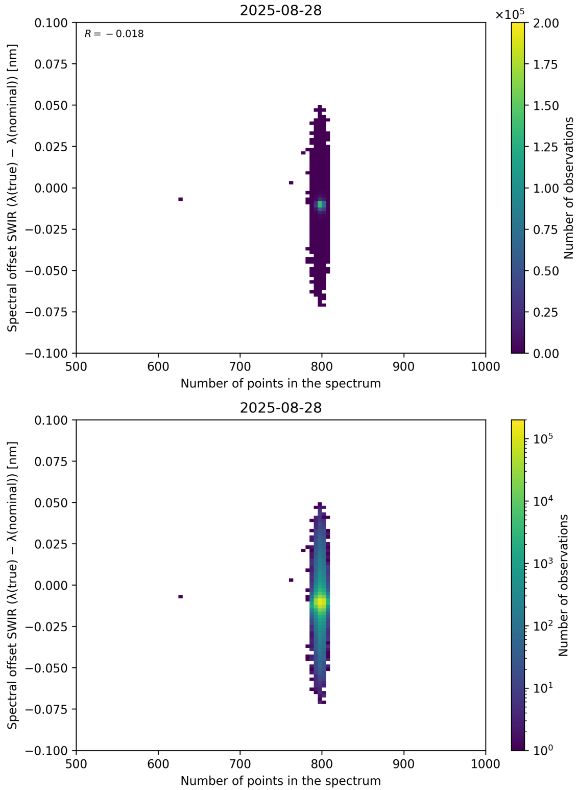
Figure 93: Scatter density plot of “Number of points in the spectrum” against “Spectral offset SWIR ( \lambda_{\text{true}} - \lambda_{\text{nominal}} )” for 2025-08-27 to 2025-08-29.
