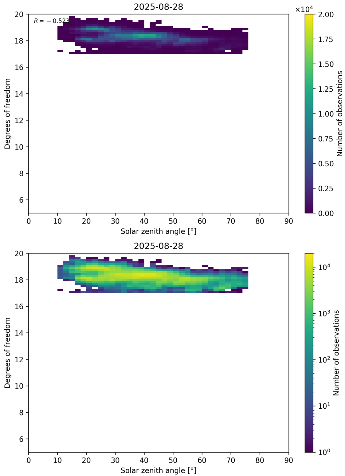
Figure 96: Scatter density plot of “Solar zenith angle” against “Degrees of freedom” for 2025-08-27 to 2025-08-29.
