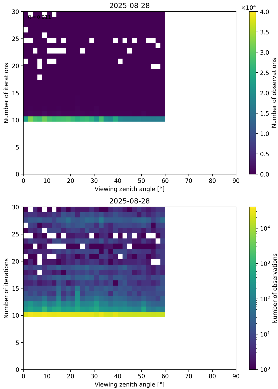
Figure 113: Scatter density plot of “Viewing zenith angle” against “Number of iterations” for 2025-08-27 to 2025-08-29.
