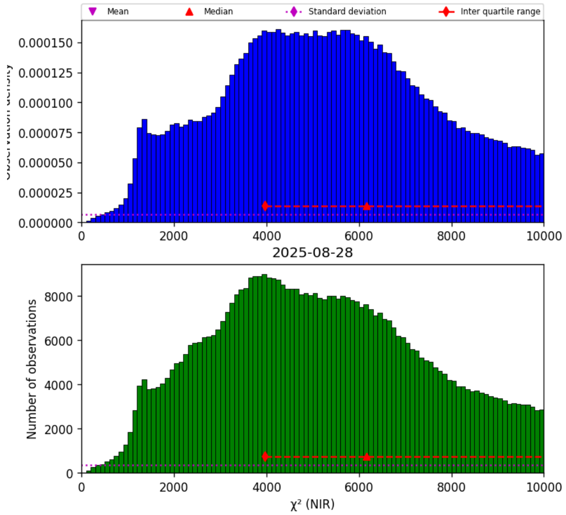
Figure 29: Histogram of “ \chi^2 (NIR)” for 2025-08-27 to 2025-08-29
