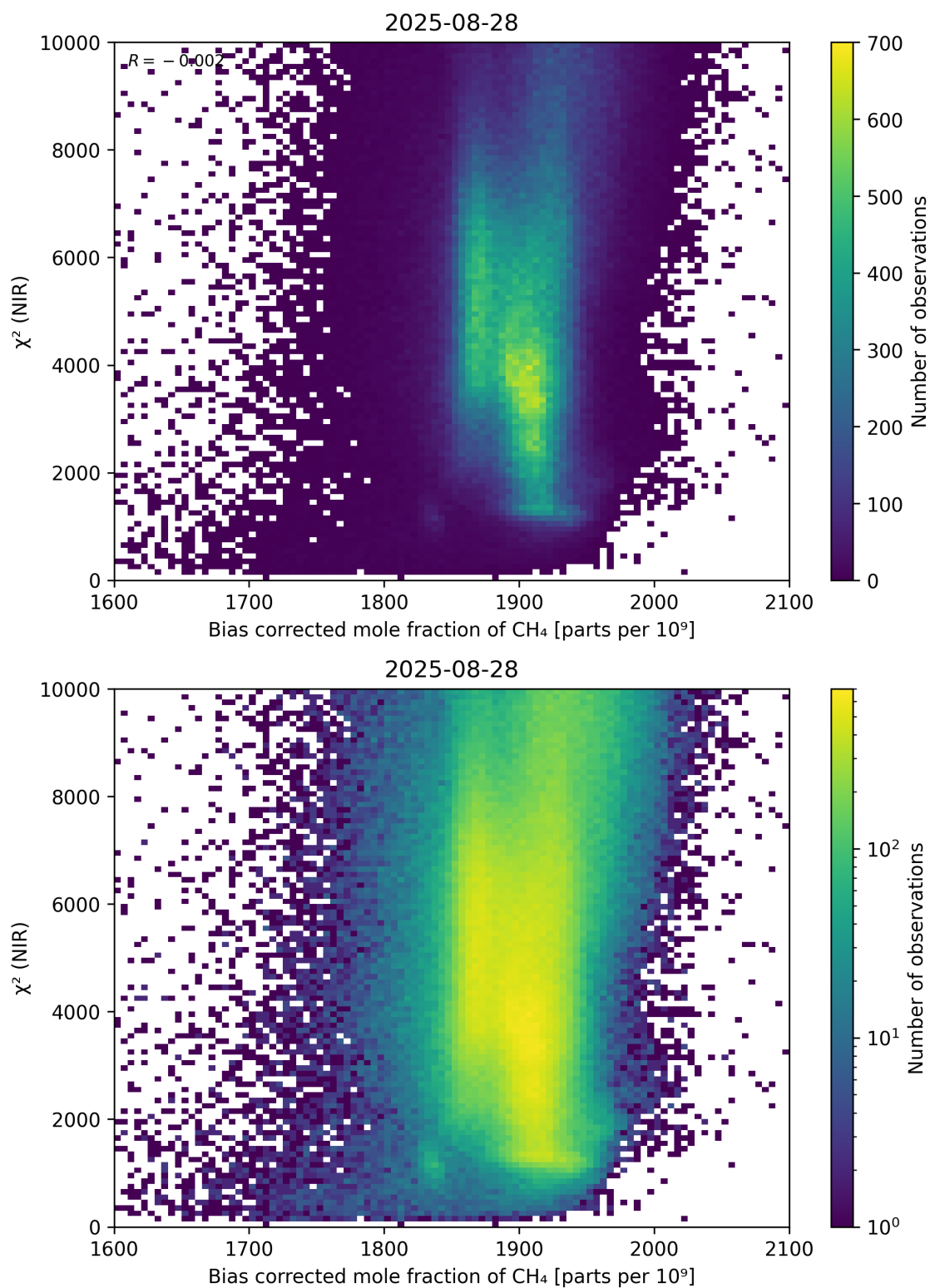
Figure 63: Scatter density plot of “Bias corrected mole fraction of CH 4 ” against “ \chi^2 (NIR)” for 2025-08-27 to 2025-08-29.
