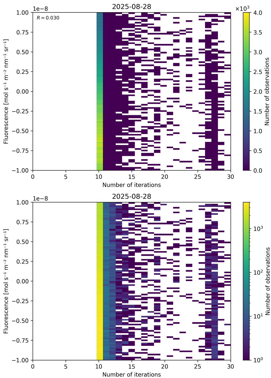
Figure 87: Scatter density plot of “Number of iterations” against “Fluorescence” for 2025-08-27 to 2025-08-29.
