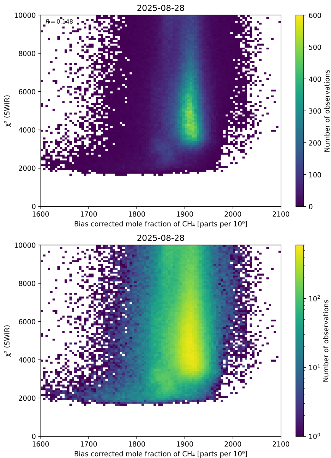
Figure 64: Scatter density plot of “Bias corrected mole fraction of \text{CH}_4 ” against “ \chi^2 (SWIR)” for 2025-08-27 to 2025-08-29.
