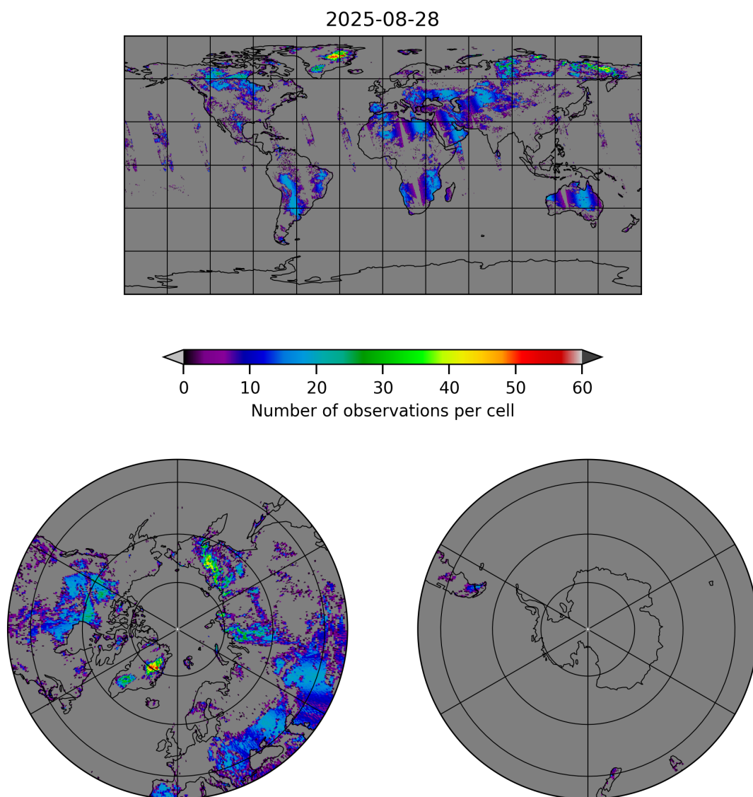
Figure 10: Map of the number of observations for 2025-08-27 to 2025-08-29
