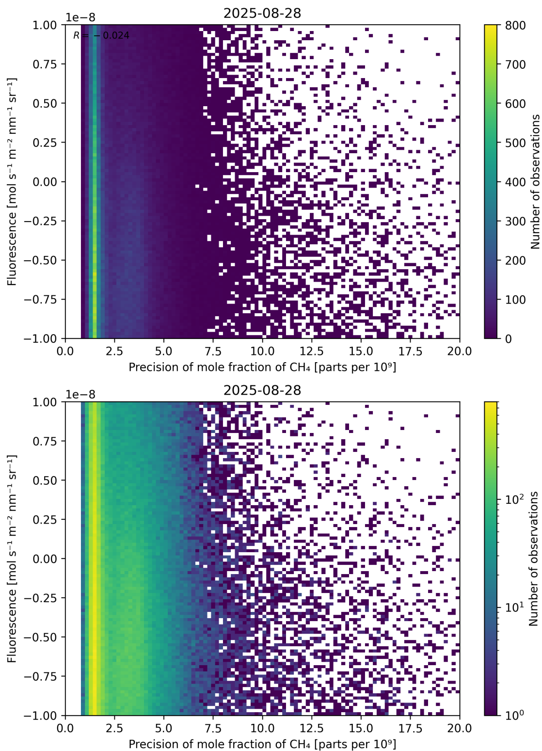
Figure 81: Scatter density plot of “Precision of mole fraction of CH 4 ” against “Fluorescence” for 2025-08-27 to 2025-08-29.
