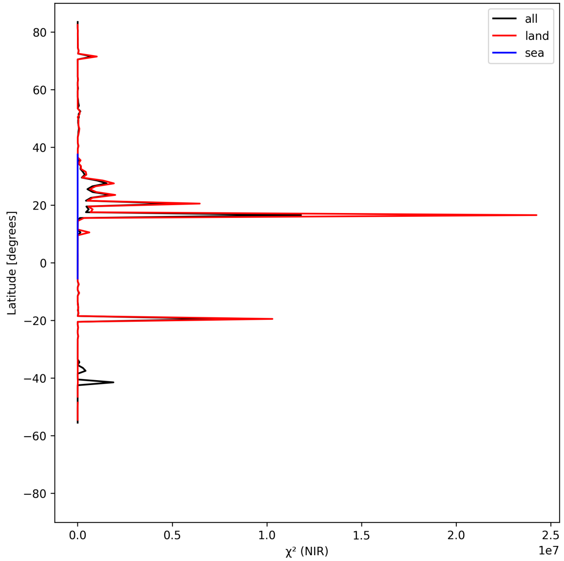
Figure 18: Zonal average of “ \chi^2 (NIR)” for 2025-08-27 to 2025-08-29.
