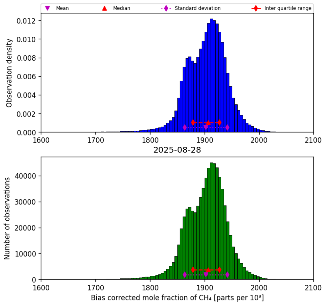
Figure 25: Histogram of “Bias corrected mole fraction of CH 4 ” for 2025-08-27 to 2025-08-29
