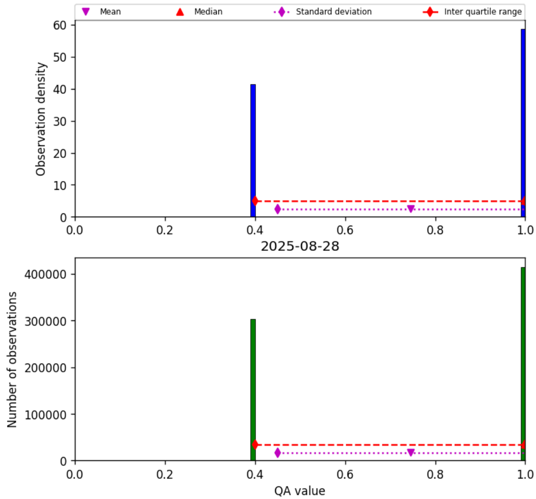
Figure 22: Histogram of “QA value” for 2025-08-27 to 2025-08-29
