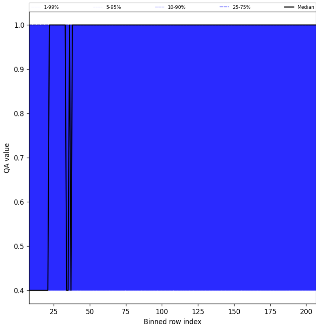
Figure 33: Along track statistics of “QA value” for 2025-08-27 to 2025-08-29
