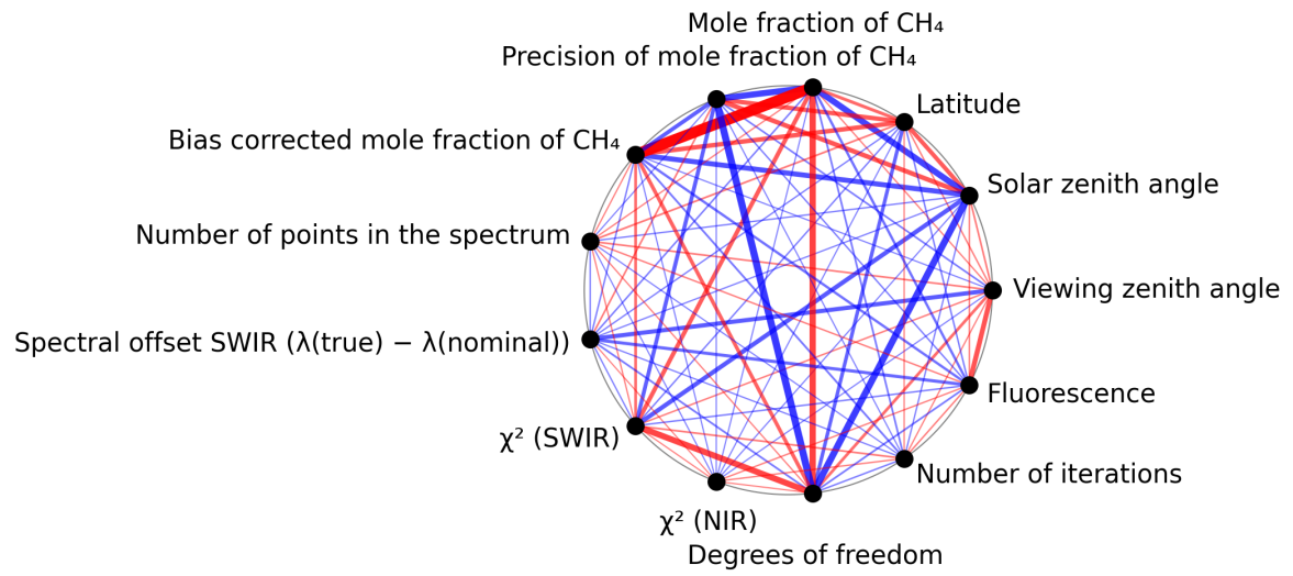
Figure 1: Map of correlation graph for 2025-08-27 to 2025-08-29.
