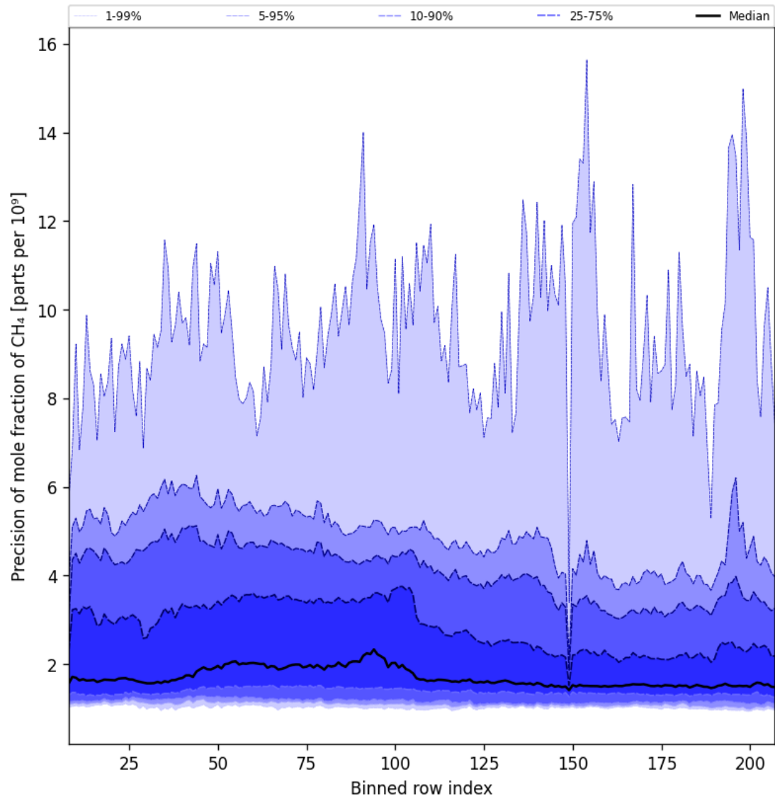
Figure 35: Along track statistics of “Precision of mole fraction of CH 4 ” for 2025-08-27 to 2025-08-29
