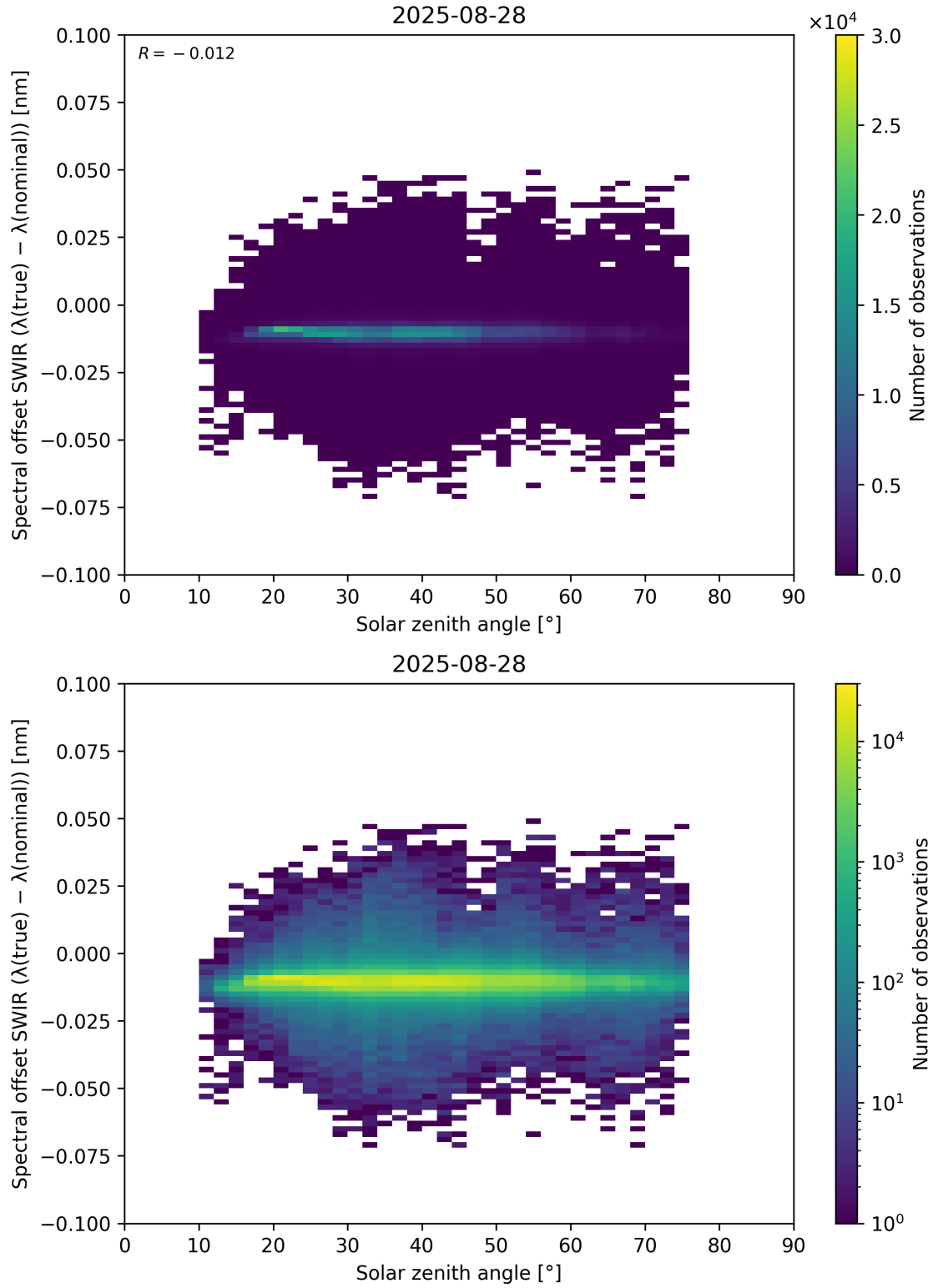
Figure 104: Scatter density plot of “Solar zenith angle” against “Spectral offset SWIR ( \lambda_{\text{true}} - \lambda_{\text{nominal}} )” for 2025-08-27 to 2025-08-29.
