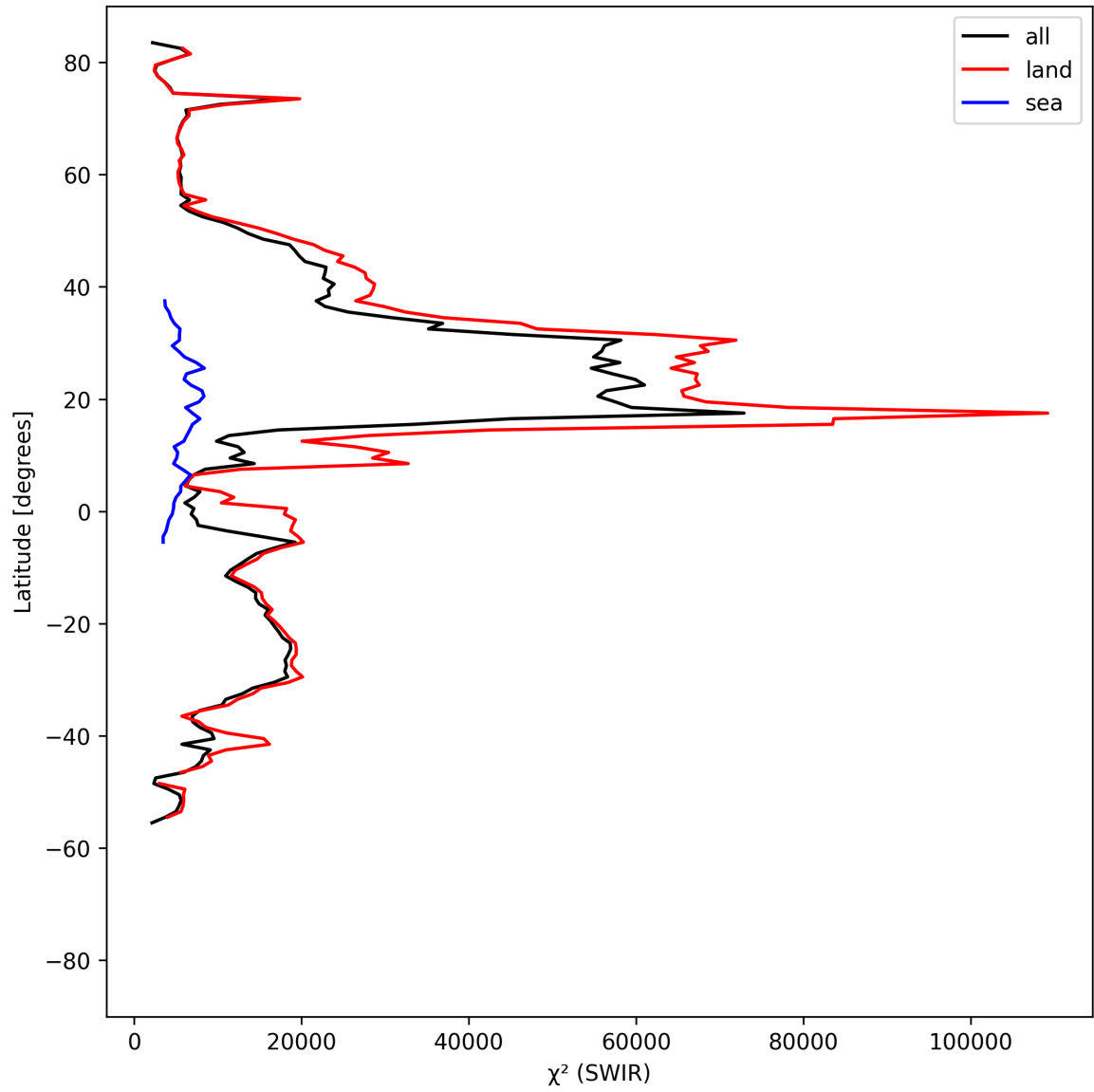
Figure 17: Zonal average of “ \chi^2 (SWIR)” for 2025-08-27 to 2025-08-29.
