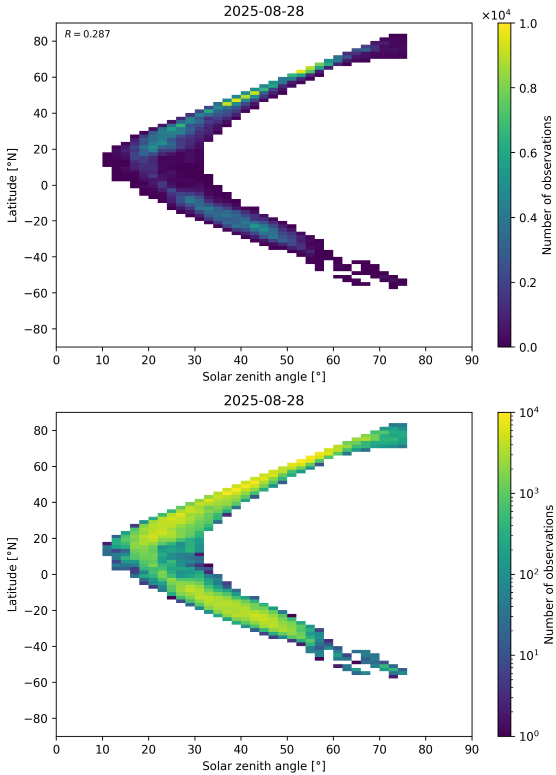
Figure 98: Scatter density plot of “Solar zenith angle” against “Latitude” for 2025-08-27 to 2025-08-29.
