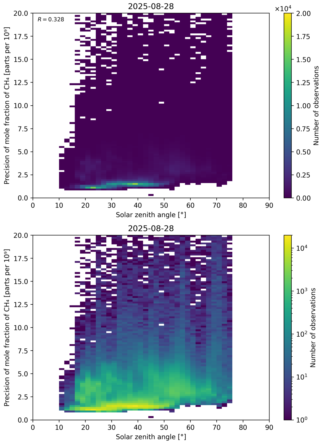
Figure 101: Scatter density plot of “Solar zenith angle” against “Precision of mole fraction of CH 4 ” for 2025-08-27 to 2025-08-29.
