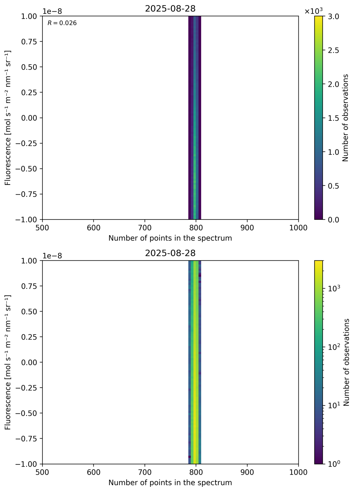
Figure 91: Scatter density plot of “Number of points in the spectrum” against “Fluorescence” for 2025-08-27 to 2025-08-29.
