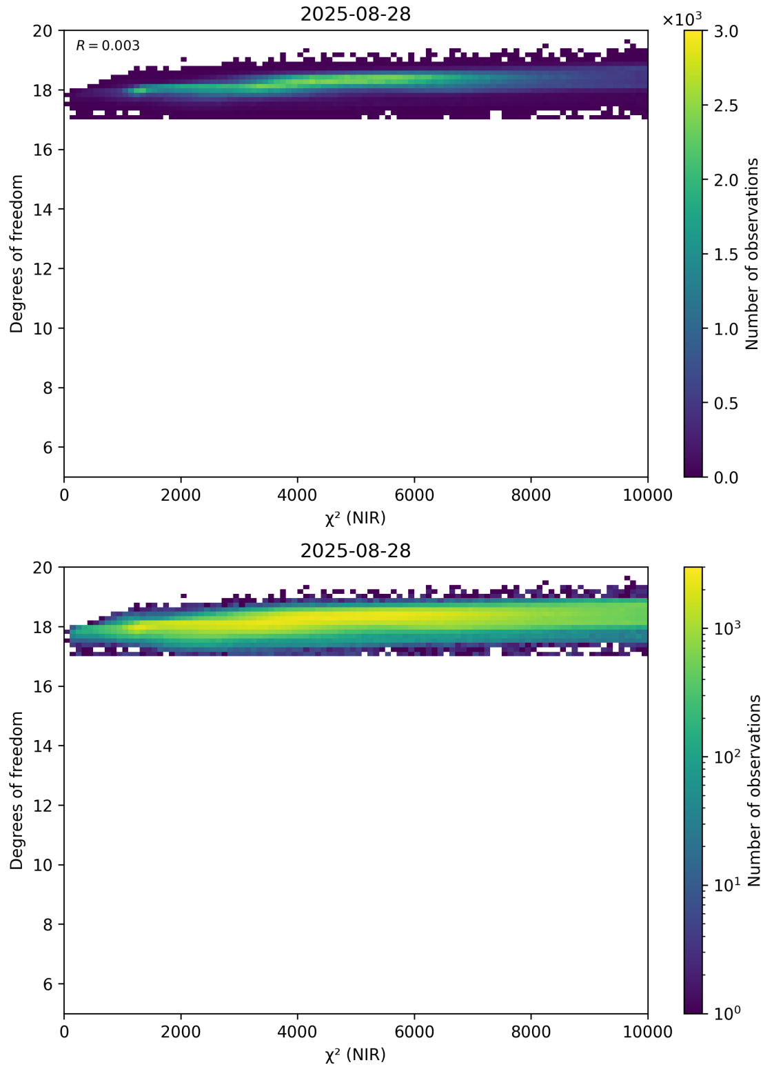
Figure 44: Scatter density plot of “ \chi^2 (NIR)” against “Degrees of freedom” for 2025-08-27 to 2025-08-29.
