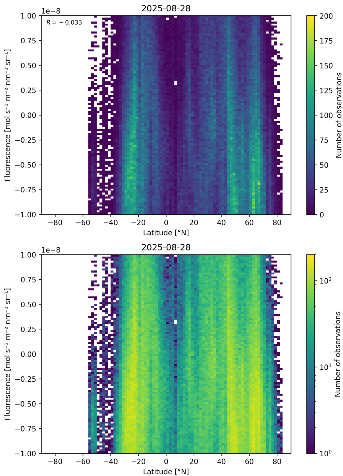
Figure 56: Scatter density plot of “Latitude” against “Fluorescence” for 2025-08-27 to 2025-08-29.
