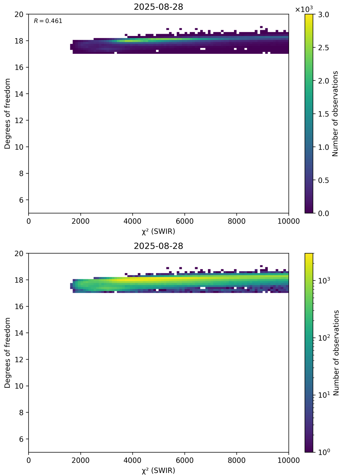
Figure 48: Scatter density plot of “ \chi^2 (SWIR)” against “Degrees of freedom” for 2025-08-27 to 2025-08-29.
