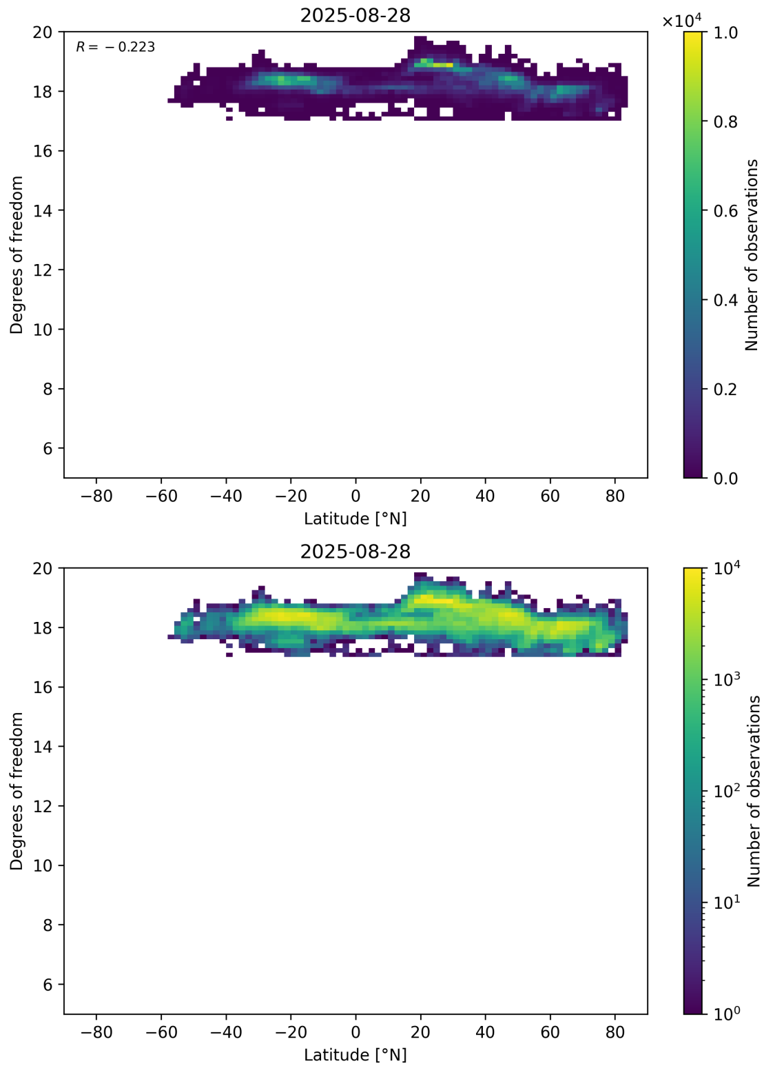
Figure 55: Scatter density plot of “Latitude” against “Degrees of freedom” for 2025-08-27 to 2025-08-29.
