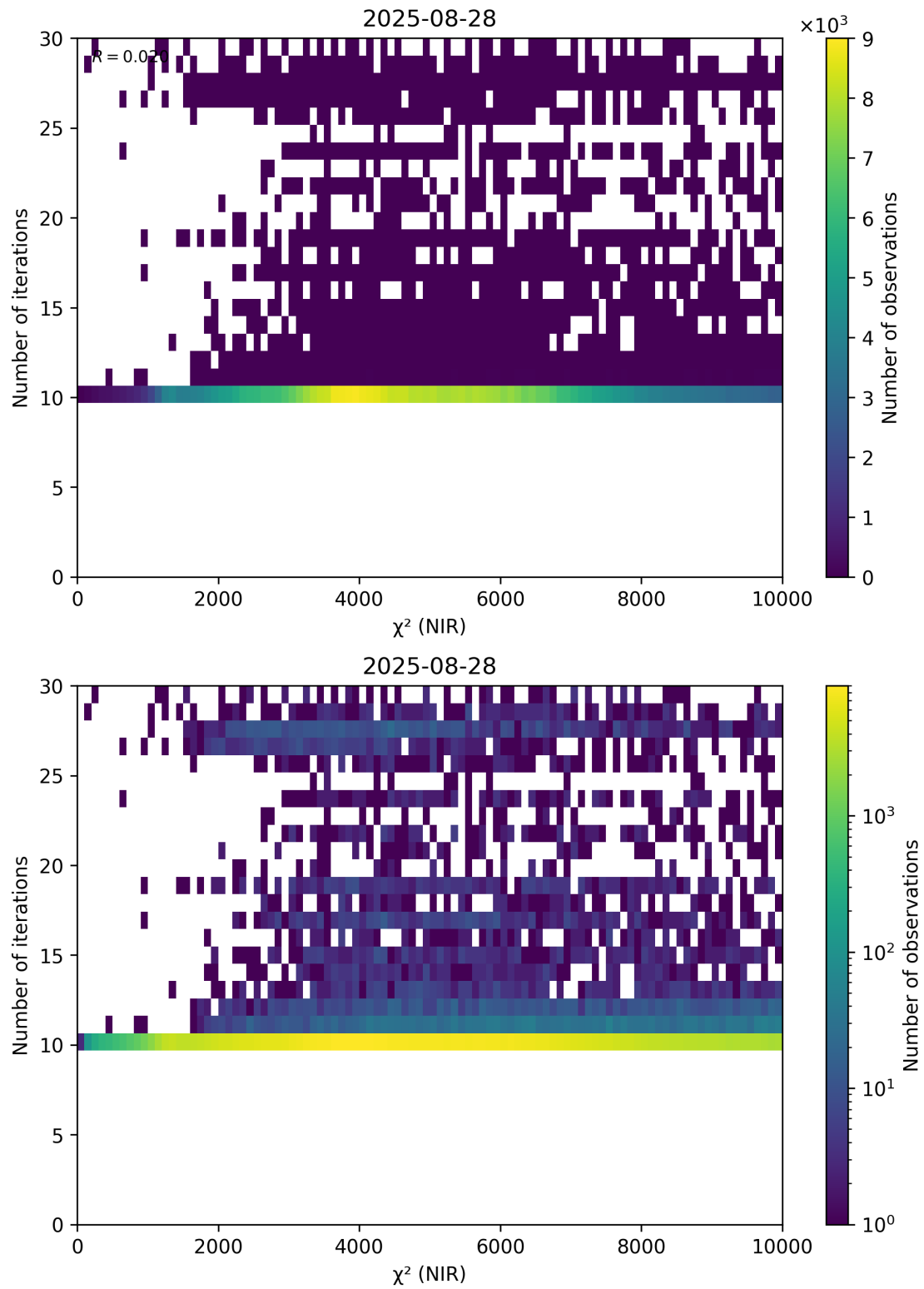
Figure 46: Scatter density plot of “ \chi^2 (NIR)” against “Number of iterations” for 2025-08-27 to 2025-08-29.
