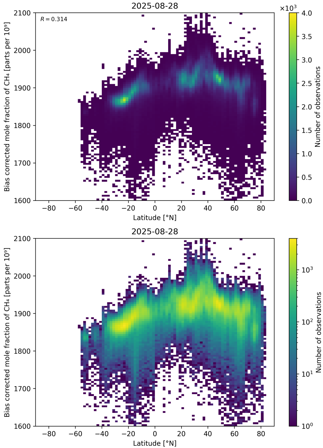
Figure 58: Scatter density plot of “Latitude” against “Bias corrected mole fraction of CH 4 ” for 2025-08-27 to 2025-08-29.
