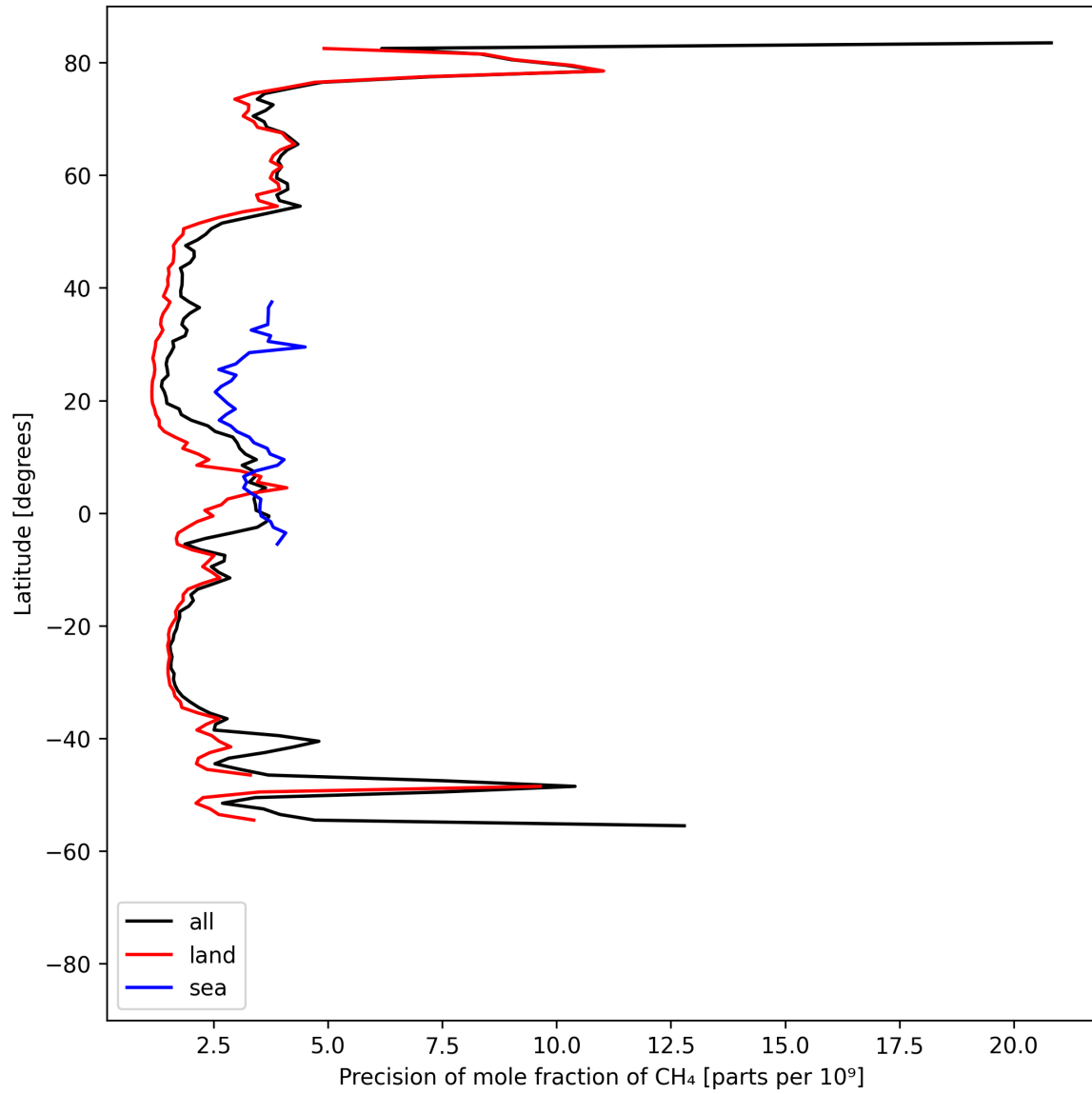
Figure 13: Zonal average of “Precision of mole fraction of CH 4 ” for 2025-08-27 to 2025-08-29.
