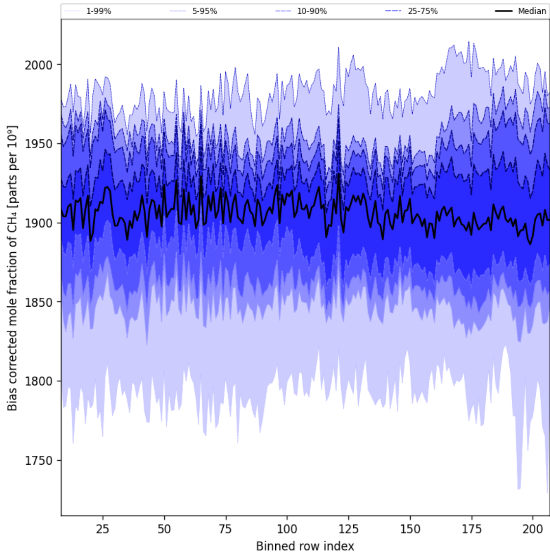
Figure 36: Along track statistics of “Bias corrected mole fraction of CH 4 ” for 2025-08-27 to 2025-08-29
