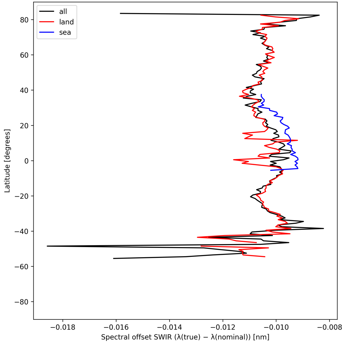
Figure 16: Zonal average of “Spectral offset SWIR ( \lambda_{\text{true}} - \lambda_{\text{nominal}} )” for 2025-08-27 to 2025-08-29.
