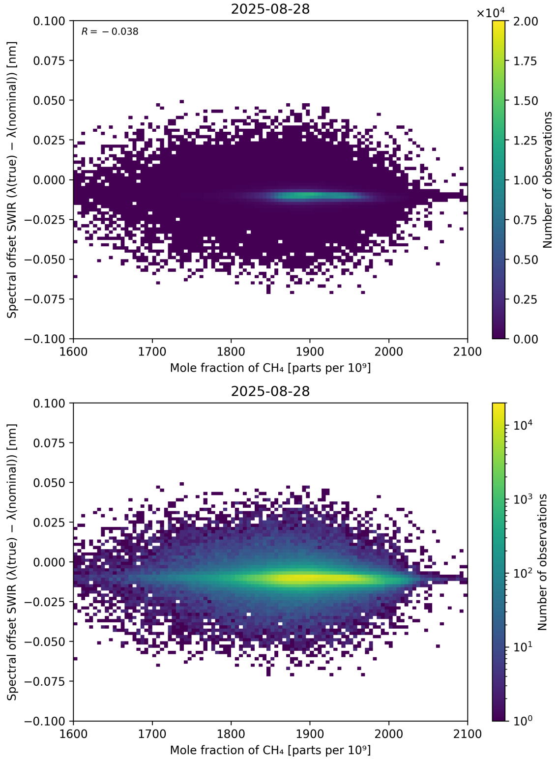
Figure 86: Scatter density plot of “Mole fraction of CH 4 ” against “Spectral offset SWIR ( \lambda_{\text{true}} - \lambda_{\text{nominal}} )” for 2025-08-27 to 2025-08-29.
