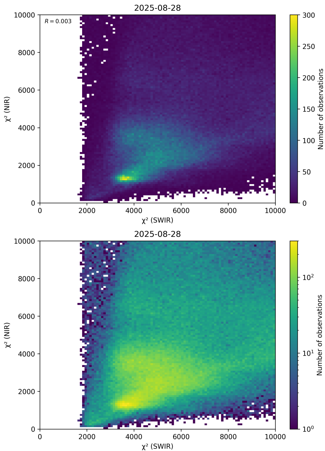
Figure 47: Scatter density plot of “ \chi^2 (SWIR)” against “ \chi^2 (NIR)” for 2025-08-27 to 2025-08-29.
