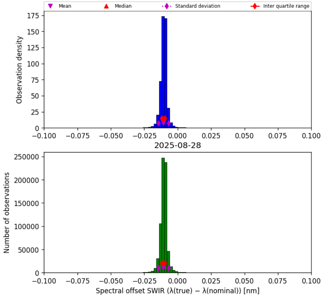
Figure 27: Histogram of “Spectral offset SWIR ( \lambda_{\text{true}} - \lambda_{\text{nominal}} )” for 2025-08-27 to 2025-08-29
