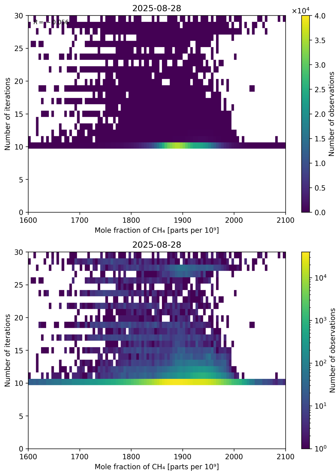
Figure 76: Scatter density plot of “Mole fraction of CH 4 ” against “Number of iterations” for 2025-08-27 to 2025-08-29.
