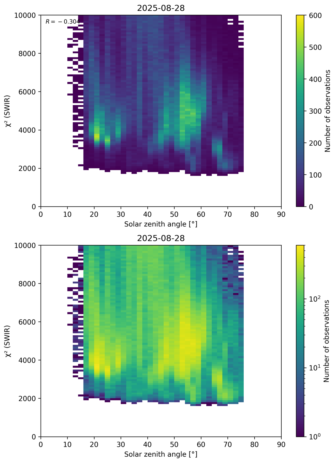
Figure 95: Scatter density plot of “Solar zenith angle” against “ \chi^2 (SWIR)” for 2025-08-27 to 2025-08-29.
