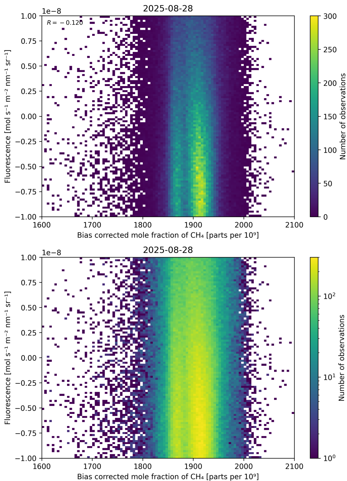
Figure 66: Scatter density plot of “Bias corrected mole fraction of \text{CH}_4 ” against “Fluorescence” for 2025-08-27 to 2025-08-29.
