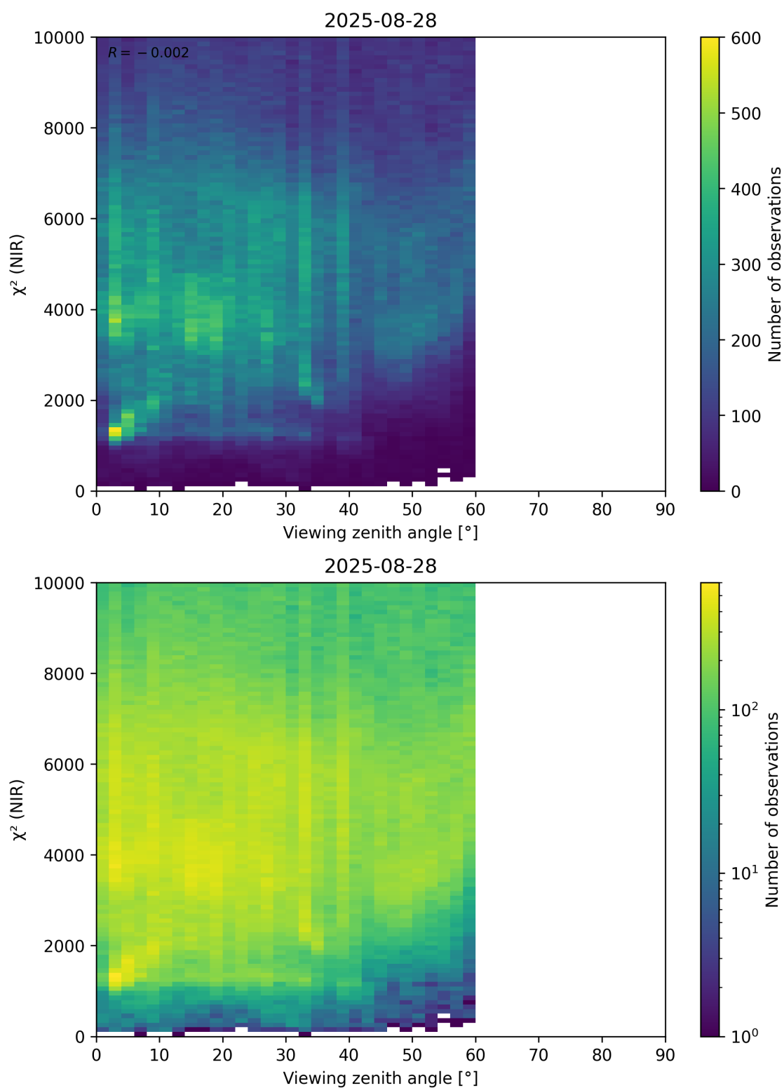
Figure 105: Scatter density plot of “Viewing zenith angle” against “ \chi^2 (NIR)” for 2025-08-27 to 2025-08-29.
