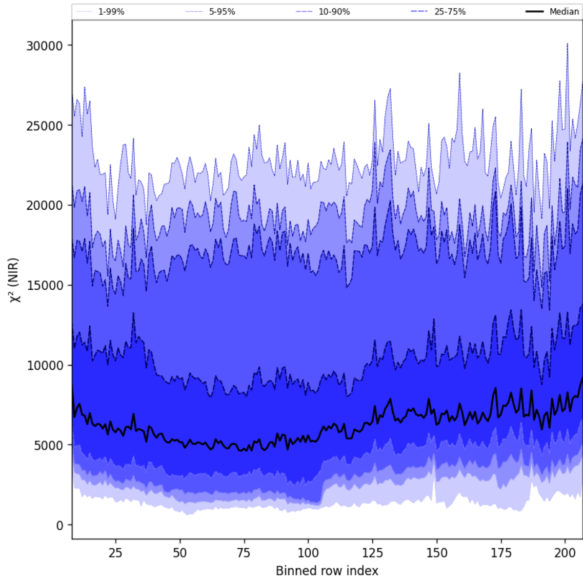
Figure 40: Along track statistics of " \chi^2 (NIR)" for 2025-08-27 to 2025-08-29
