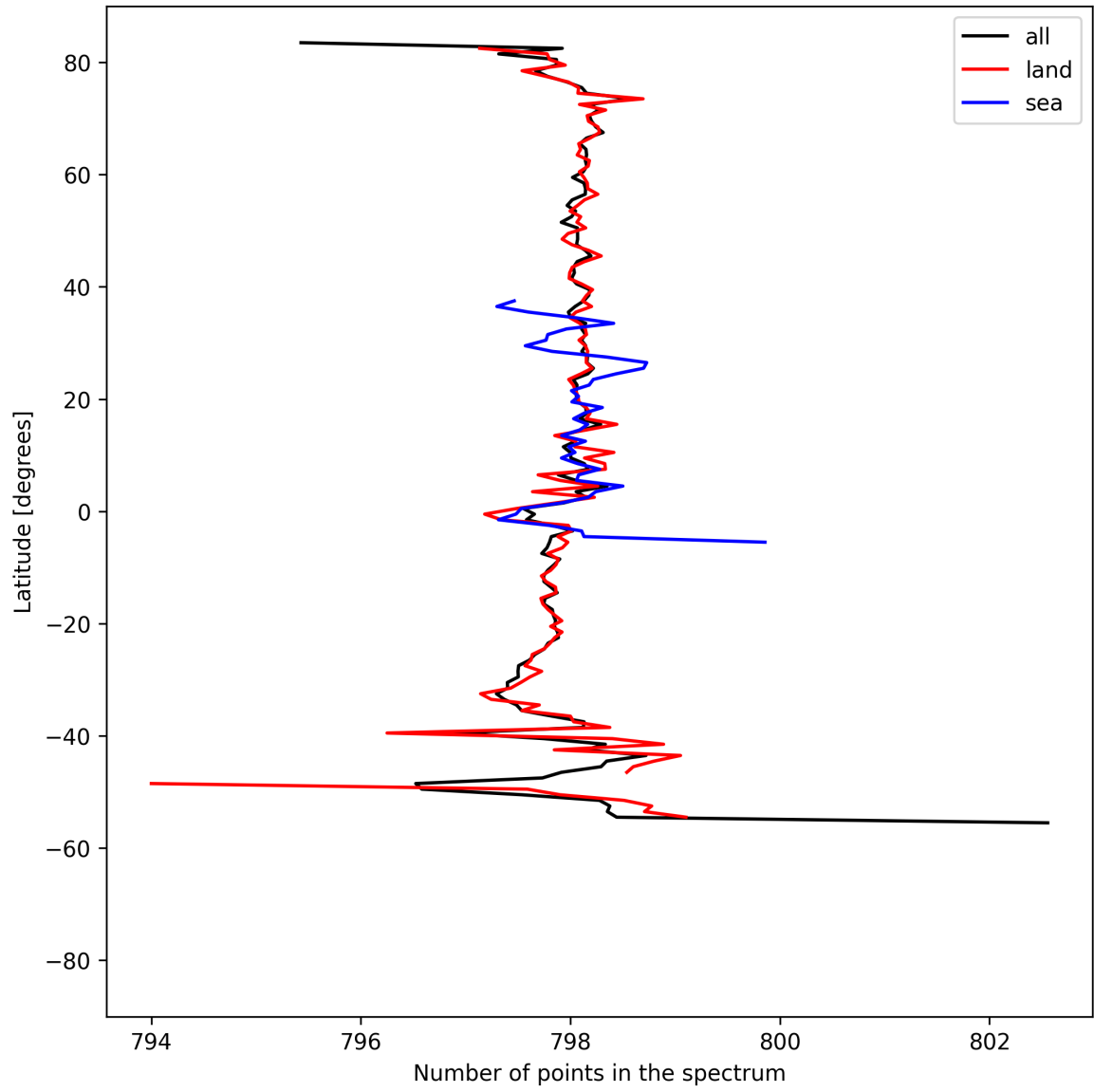
Figure 15: Zonal average of “Number of points in the spectrum” for 2025-08-27 to 2025-08-29.
