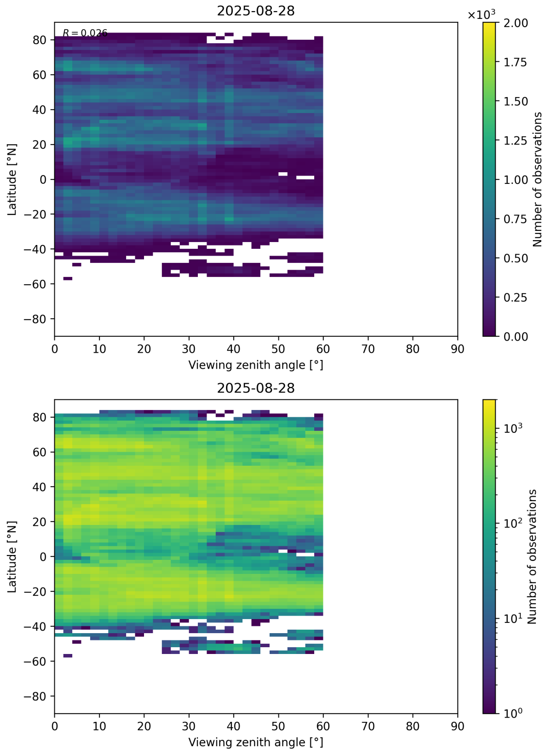
Figure 109: Scatter density plot of “Viewing zenith angle” against “Latitude” for 2025-08-27 to 2025-08-29.
