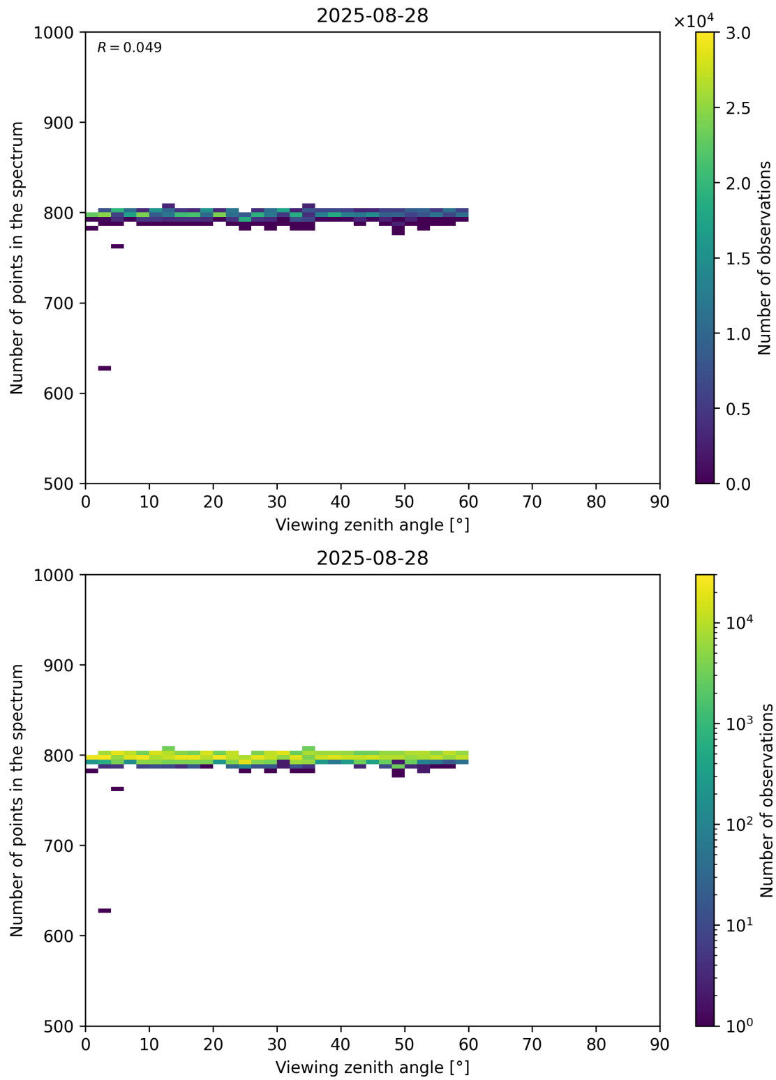
Figure 114: Scatter density plot of “Viewing zenith angle” against “Number of points in the spectrum” for 2025-08-27 to 2025-08-29.
