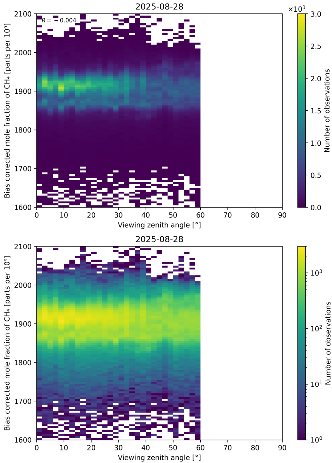
Figure 111: Scatter density plot of “Viewing zenith angle” against “Bias corrected mole fraction of CH 4 ” for 2025-08-27 to 2025-08-29.
