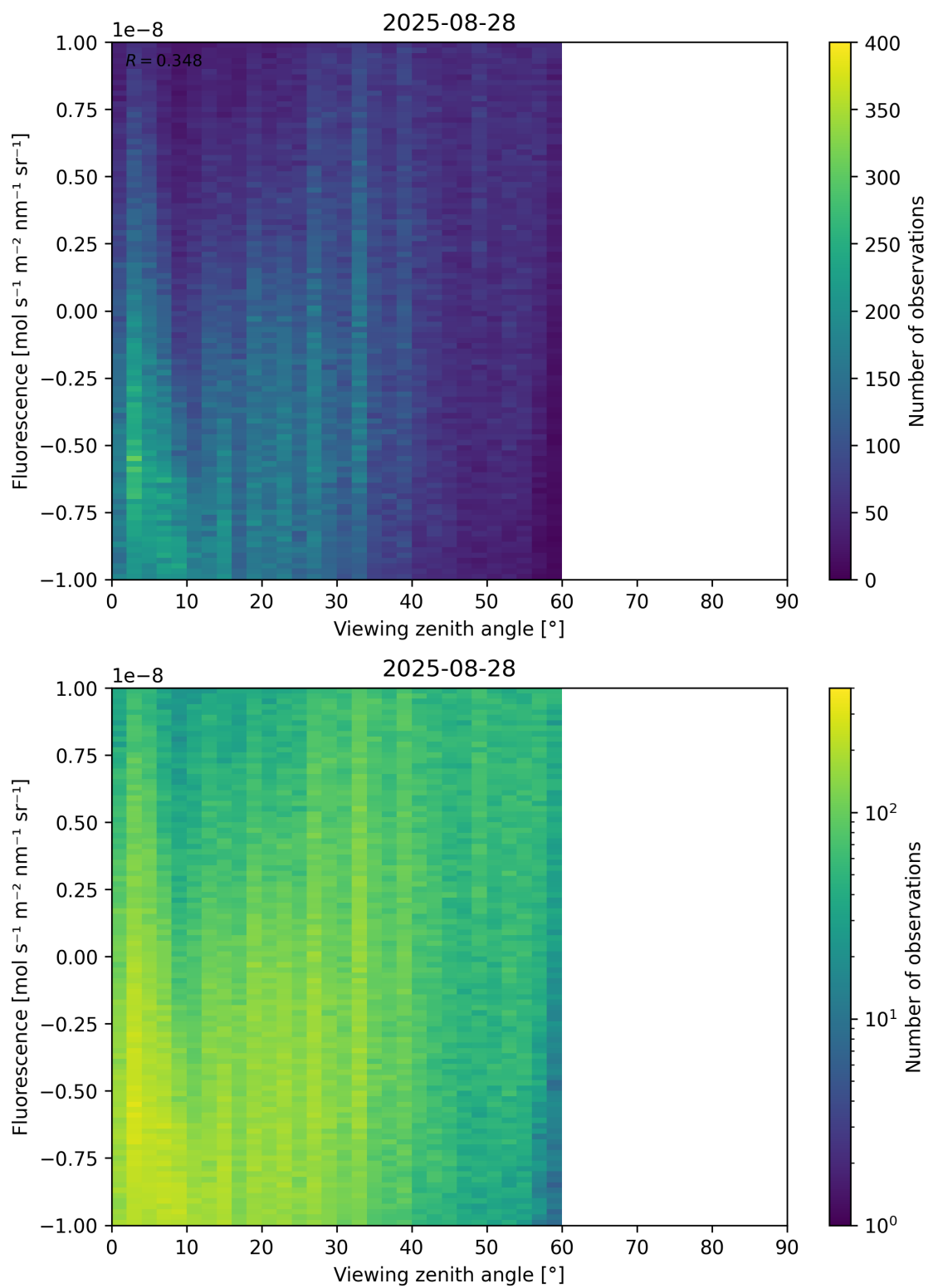
Figure 108: Scatter density plot of “Viewing zenith angle” against “Fluorescence” for 2025-08-27 to 2025-08-29.
