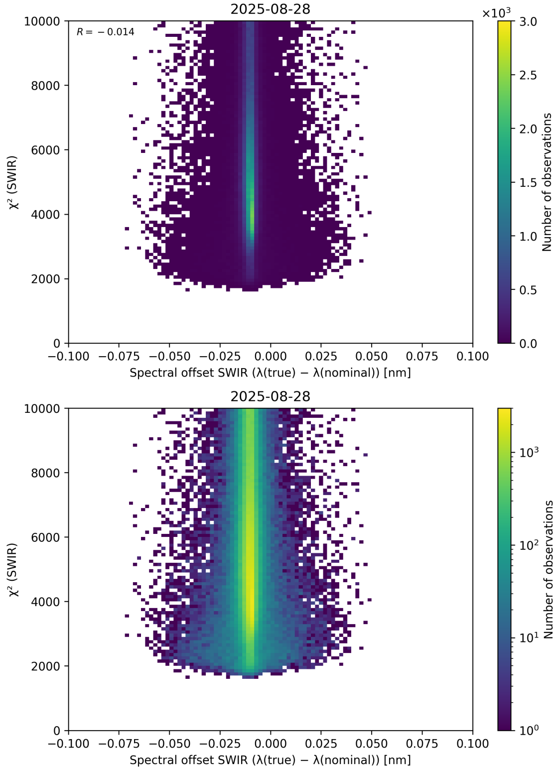
Figure 118: Scatter density plot of “Spectral offset SWIR ( \lambda_{\text{true}} - \lambda_{\text{nominal}} )” against “ \chi^2 (SWIR)” for 2025-08-27 to 2025-08-29.
