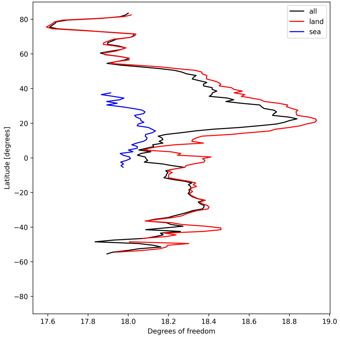
Figure 19: Zonal average of “Degrees of freedom” for 2025-08-27 to 2025-08-29.
