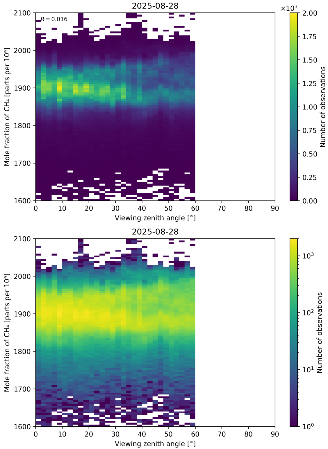
Figure 110: Scatter density plot of “Viewing zenith angle” against “Mole fraction of CH 4 ” for 2025-08-27 to 2025-08-29.
