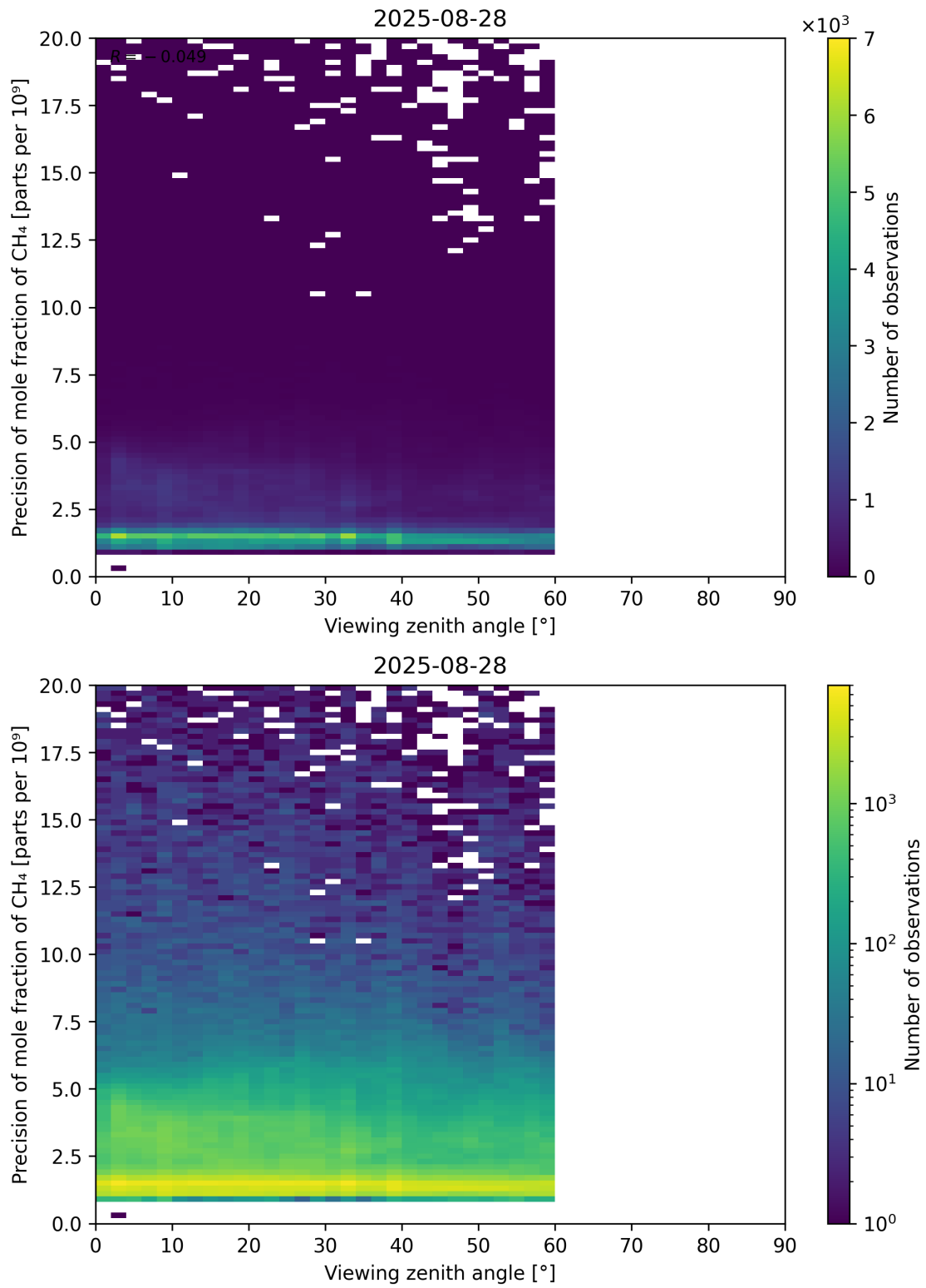
Figure 112: Scatter density plot of “Viewing zenith angle” against “Precision of mole fraction of CH 4 ” for 2025-08-27 to 2025-08-29.
