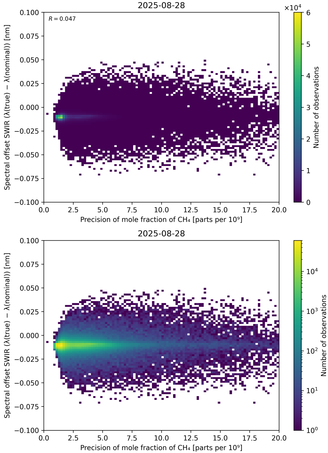
Figure 85: Scatter density plot of “Precision of mole fraction of CH 4 ” against “Spectral offset SWIR ( \lambda_{\text{true}} - \lambda_{\text{nominal}} )” for 2025-08-27 to 2025-08-29.
