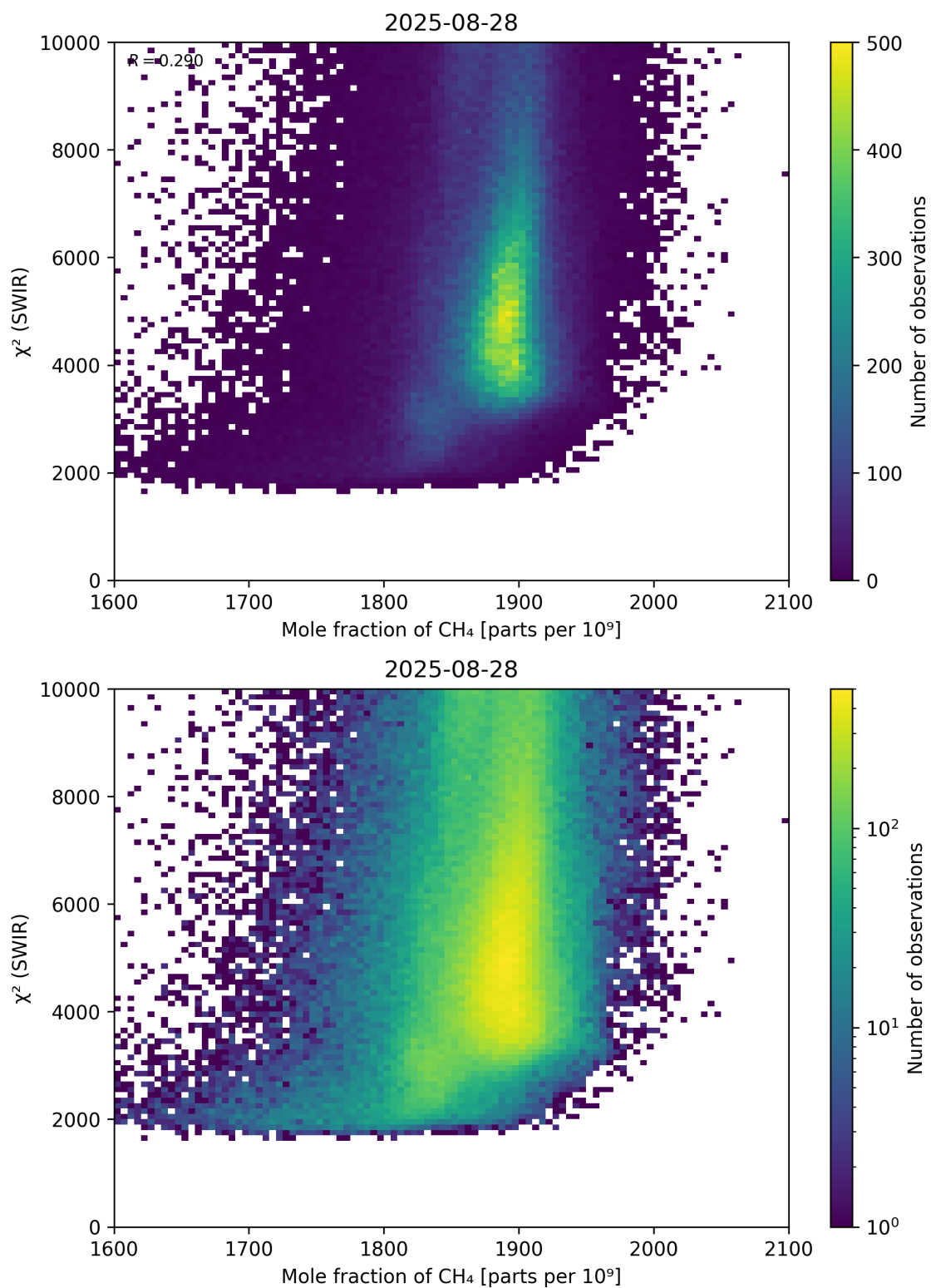
Figure 71: Scatter density plot of “Mole fraction of \text{CH}_4 ” against “ \chi^2 (SWIR)” for 2025-08-27 to 2025-08-29.
