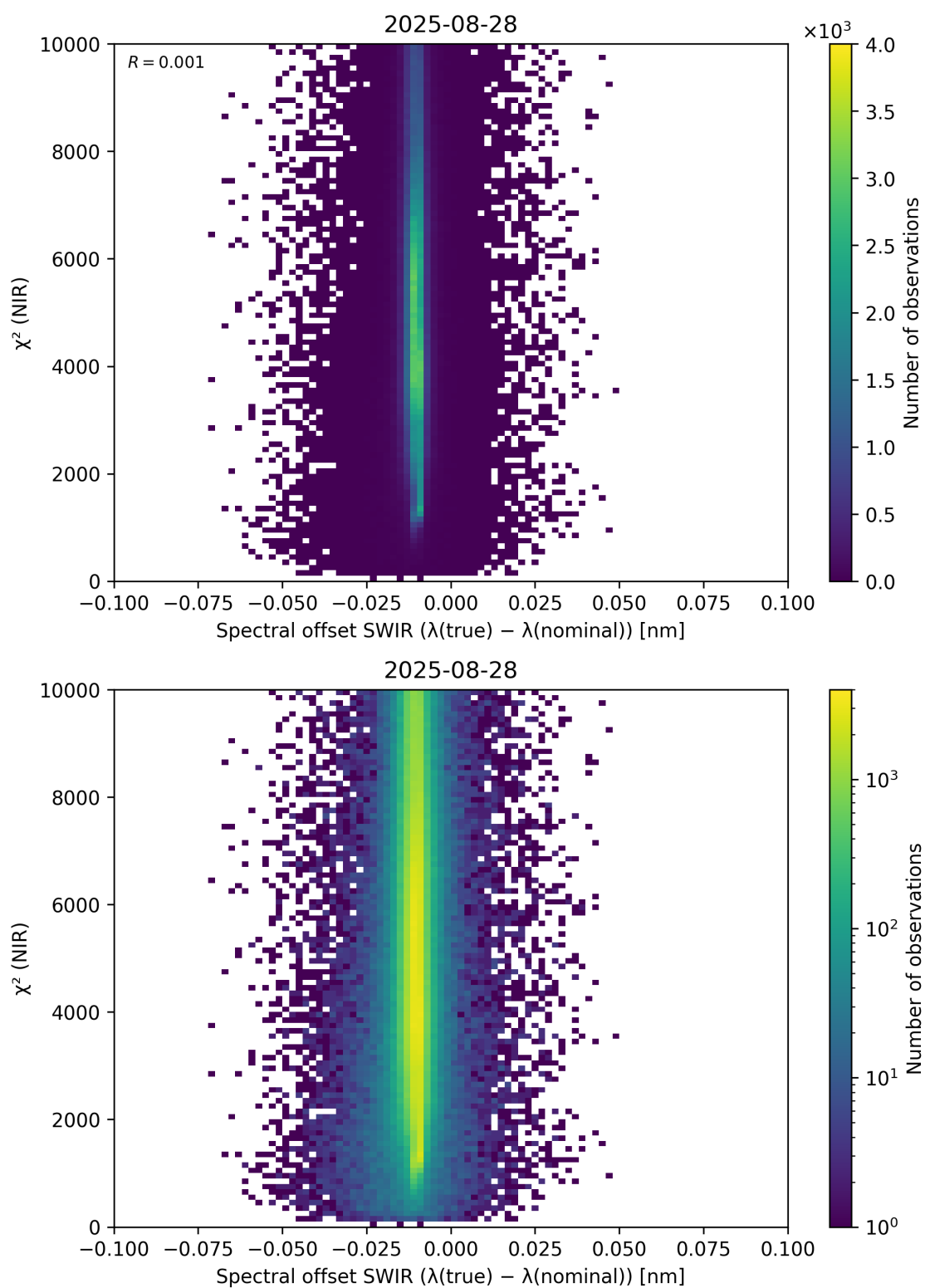
Figure 117: Scatter density plot of “Spectral offset SWIR ( \lambda_{\text{true}} - \lambda_{\text{nominal}} )” against “ \chi^2 (NIR)” for 2025-08-27 to 2025-08-29.
