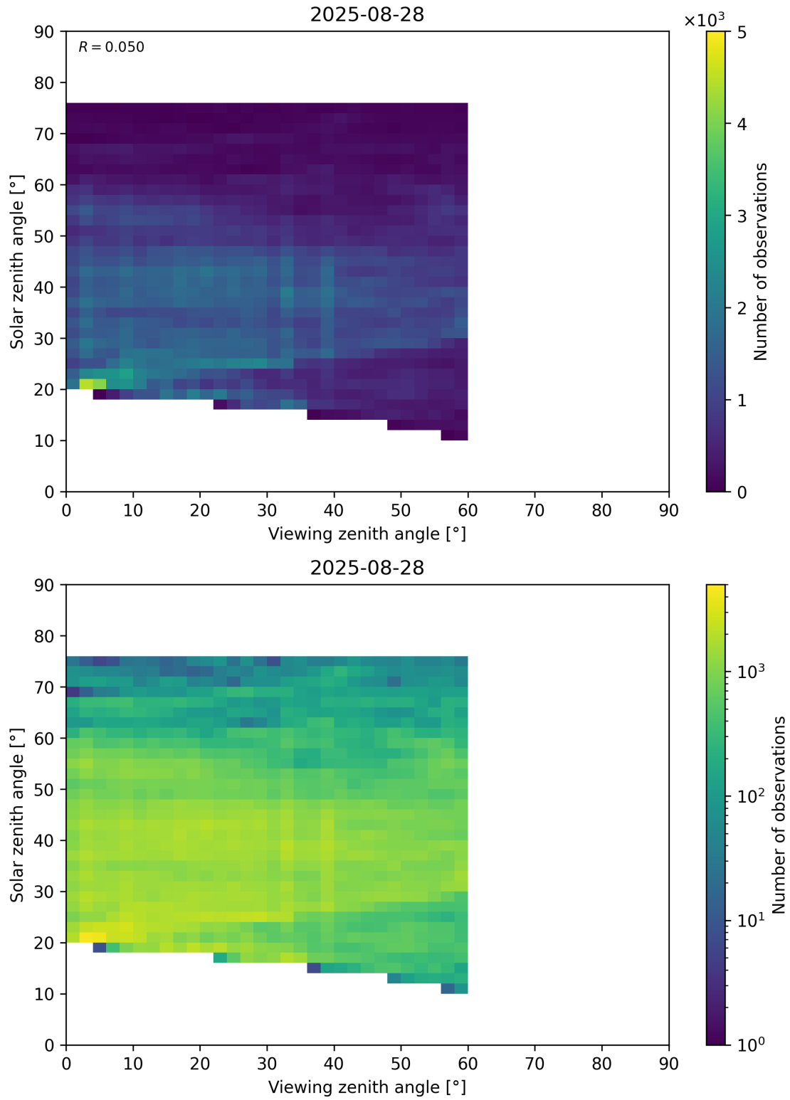
Figure 115: Scatter density plot of “Viewing zenith angle” against “Solar zenith angle” for 2025-08-27 to 2025-08-29.
