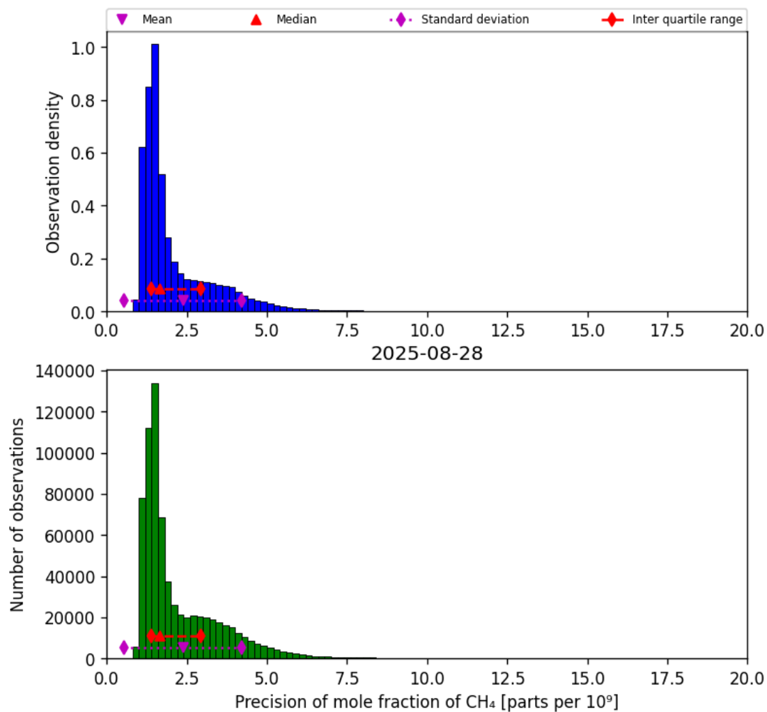
Figure 24: Histogram of “Precision of mole fraction of CH 4 ” for 2025-08-27 to 2025-08-29
