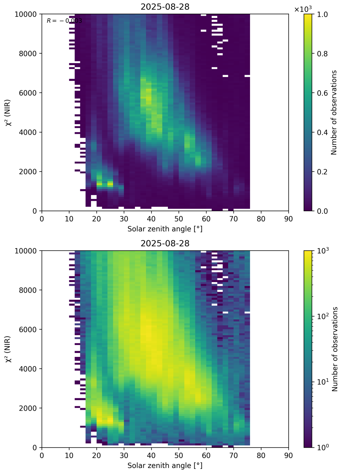
Figure 94: Scatter density plot of “Solar zenith angle” against “ \chi^2 (NIR)” for 2025-08-27 to 2025-08-29.
