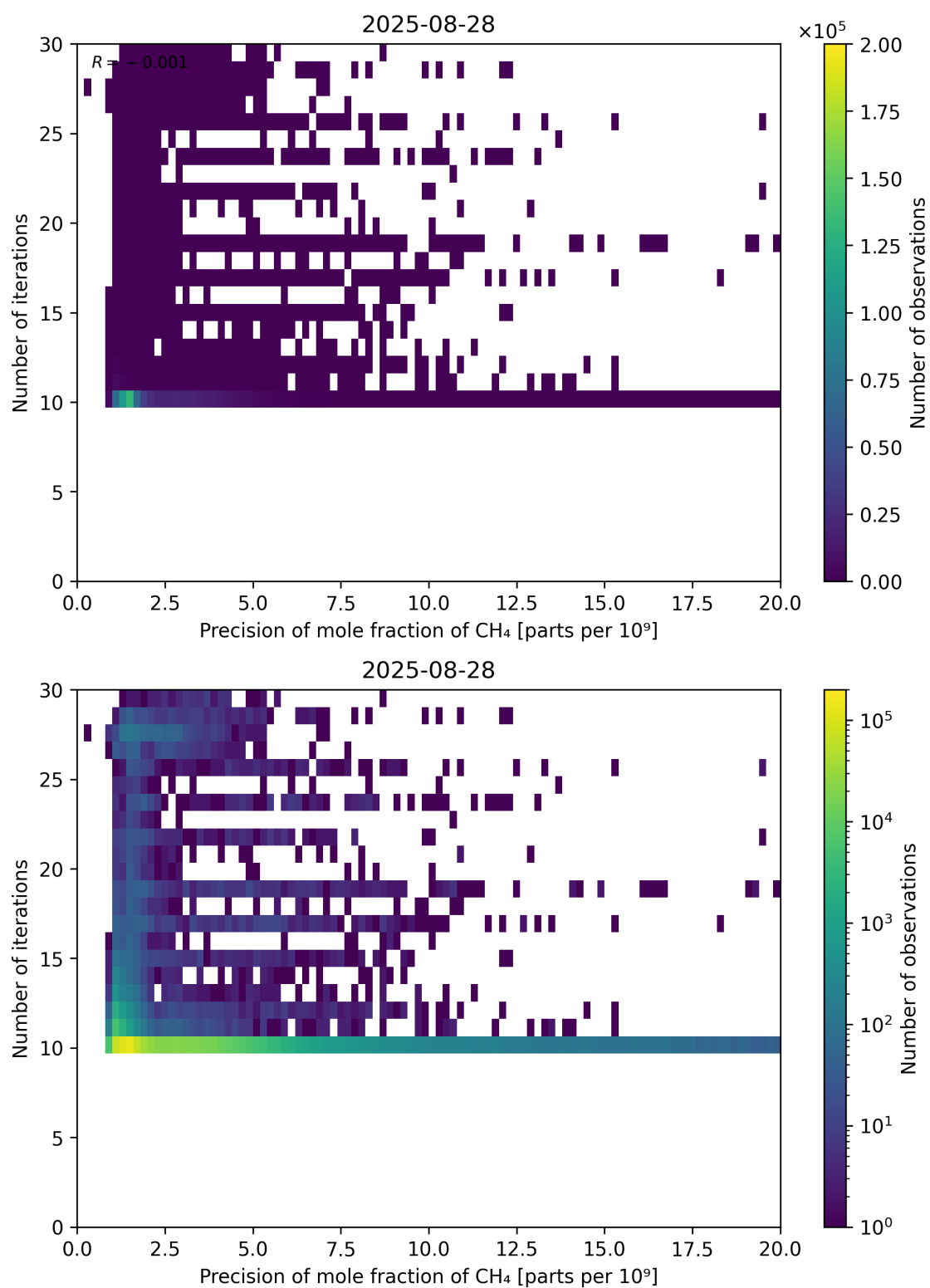
Figure 83: Scatter density plot of “Precision of mole fraction of CH 4 ” against “Number of iterations” for 2025-08-27 to 2025-08-29.
