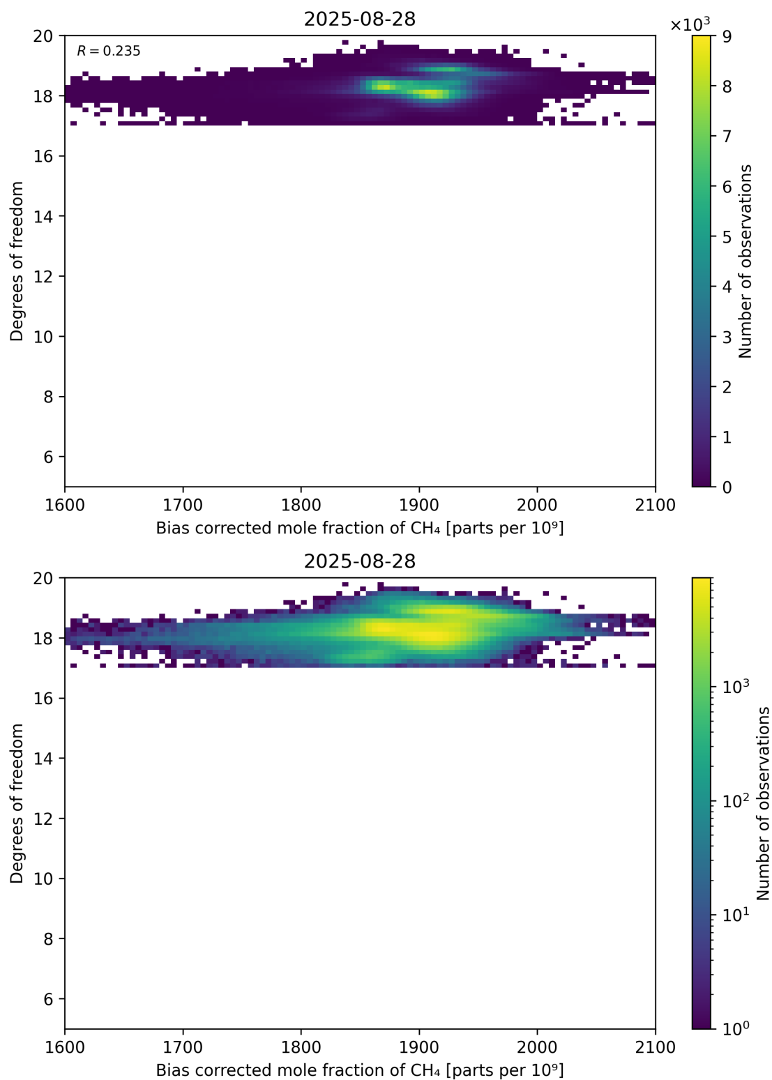
Figure 65: Scatter density plot of “Bias corrected mole fraction of CH 4 ” against “Degrees of freedom” for 2025-08-27 to 2025-08-29.
