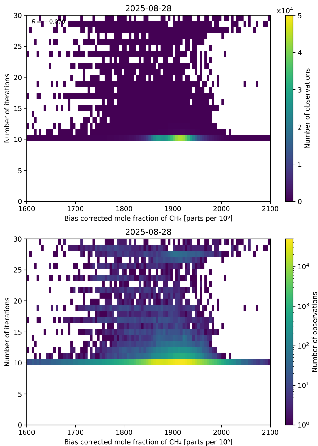
Figure 67: Scatter density plot of “Bias corrected mole fraction of CH 4 ” against “Number of iterations” for 2025-08-27 to 2025-08-29.
