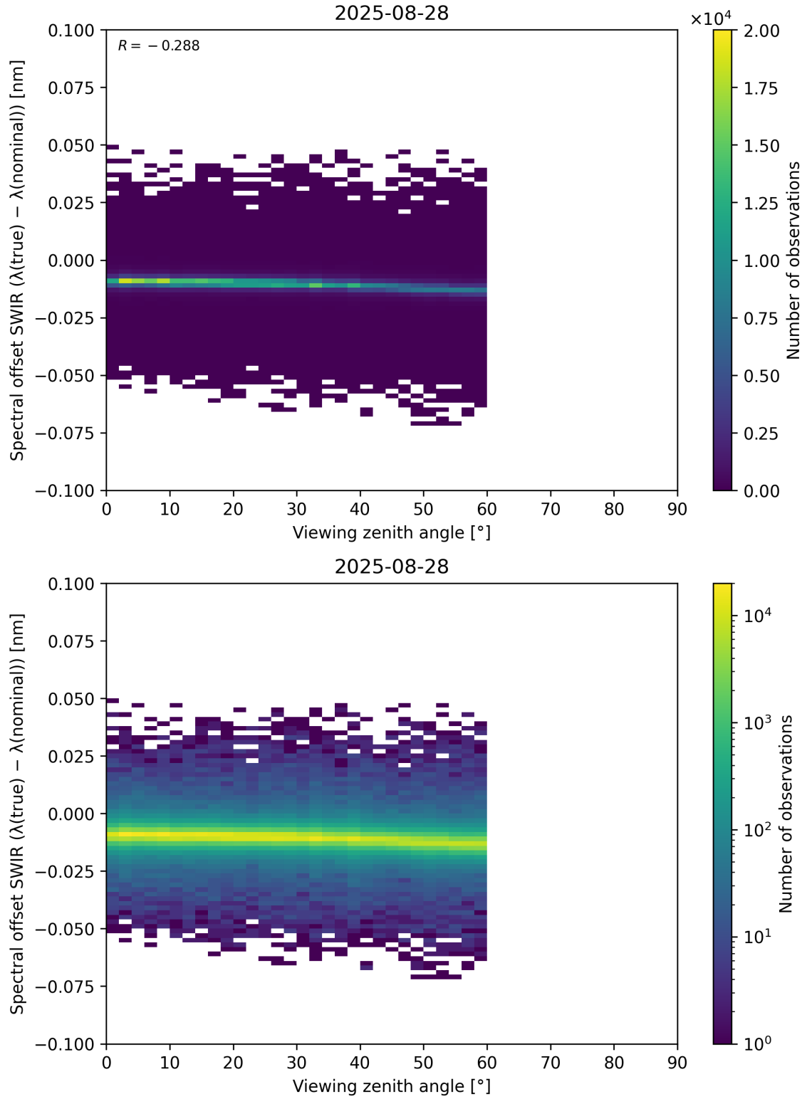
Figure 116: Scatter density plot of “Viewing zenith angle” against “Spectral offset SWIR ( \lambda_{\text{true}} - \lambda_{\text{nominal}} )” for 2025-08-27 to 2025-08-29.
