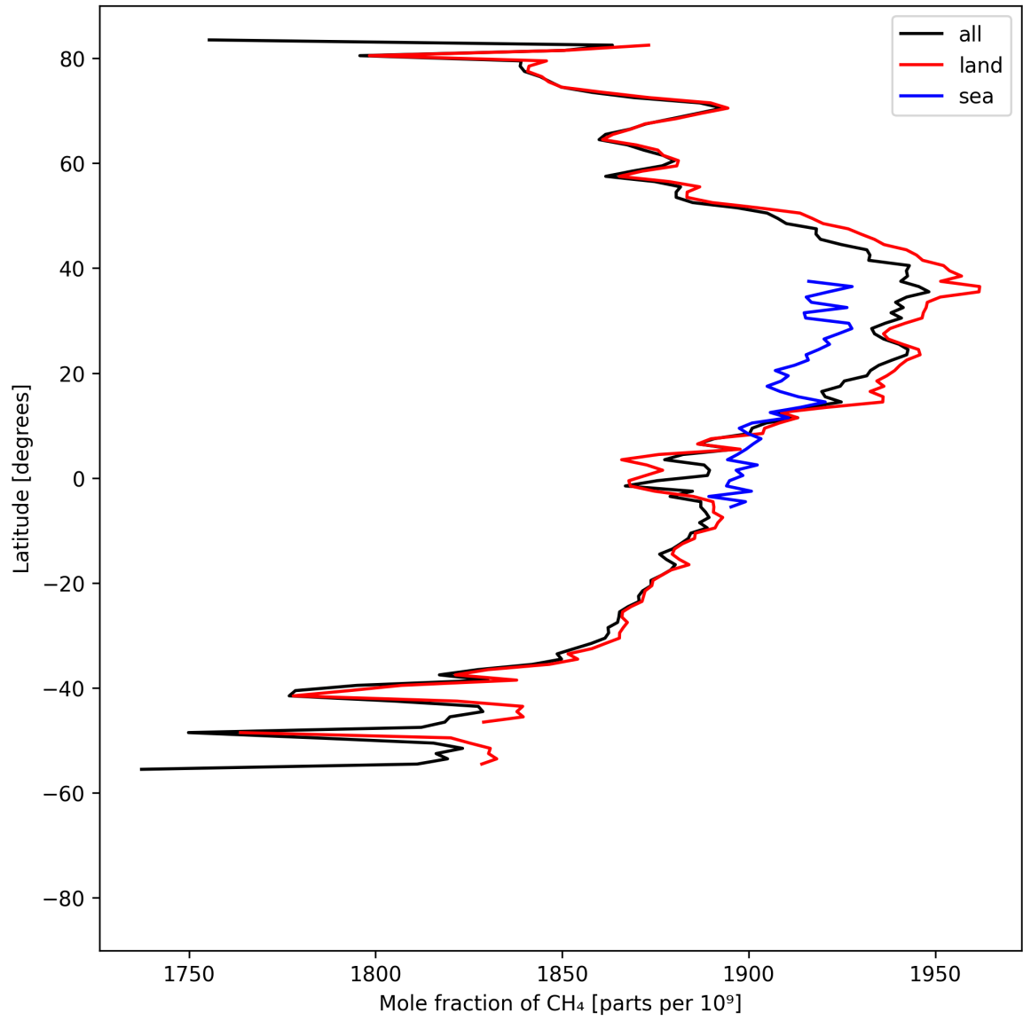
Figure 12: Zonal average of “Mole fraction of \text{CH}_4 ” for 2025-08-27 to 2025-08-29.
