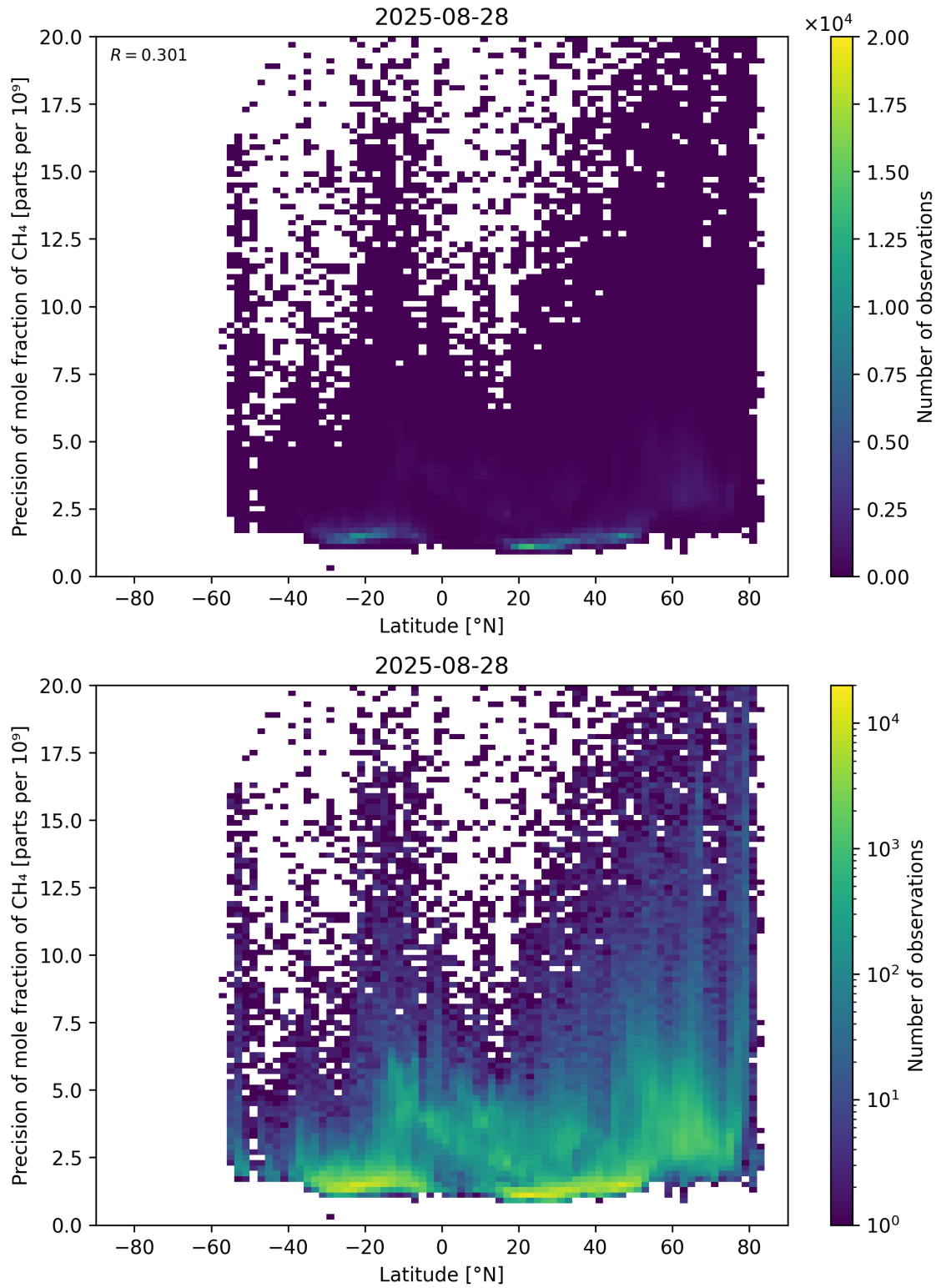
Figure 59: Scatter density plot of “Latitude” against “Precision of mole fraction of \text{CH}_4 ” for 2025-08-27 to 2025-08-29.
