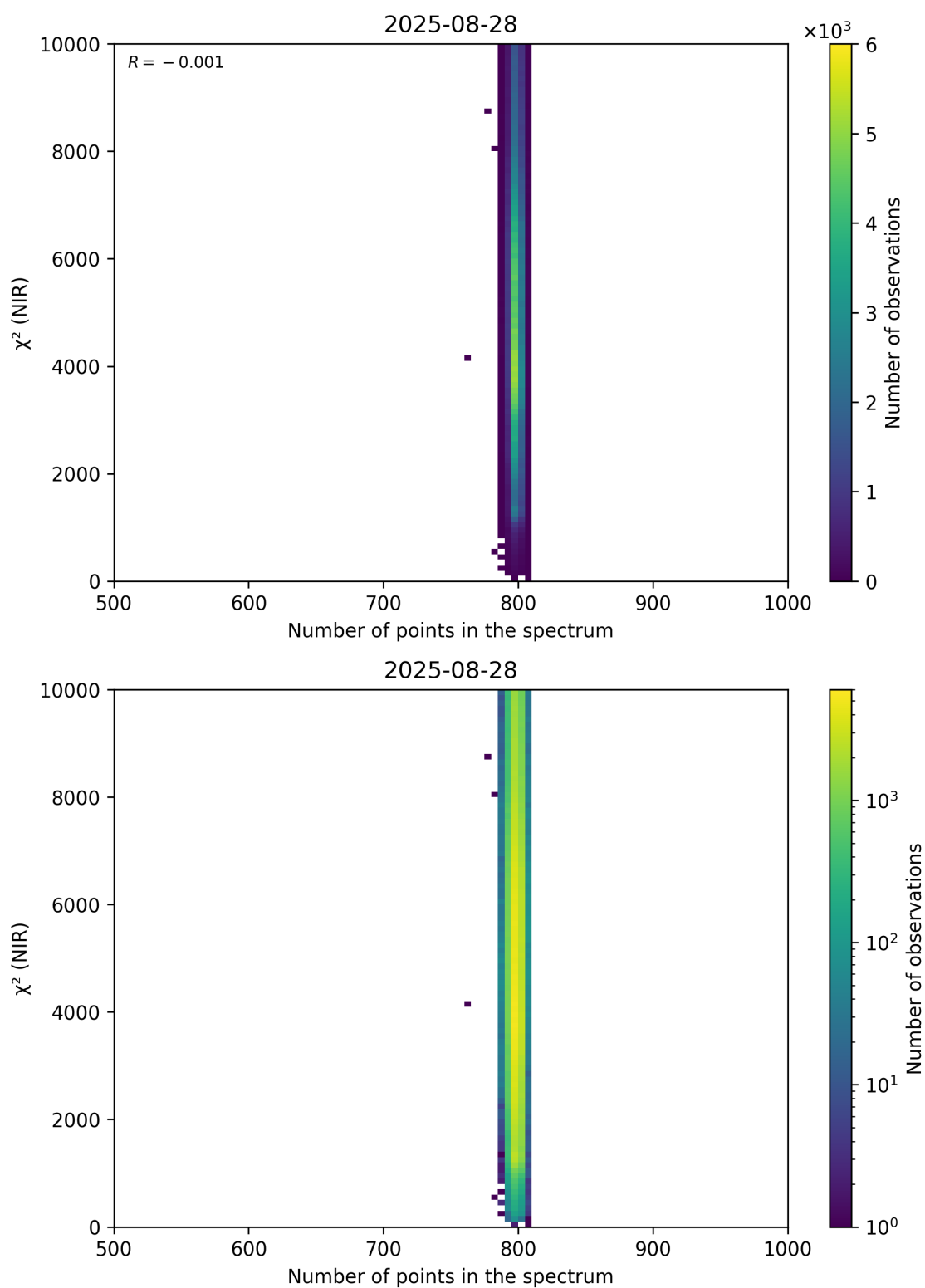
Figure 88: Scatter density plot of “Number of points in the spectrum” against “ \chi^2 (NIR)” for 2025-08-27 to 2025-08-29.
