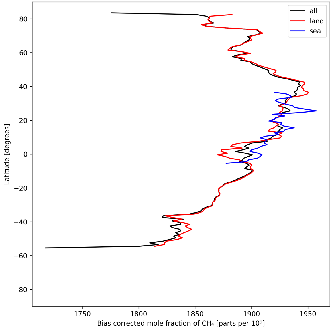
Figure 14: Zonal average of “Bias corrected mole fraction of CH 4 ” for 2025-08-28 to 2025-08-30.
