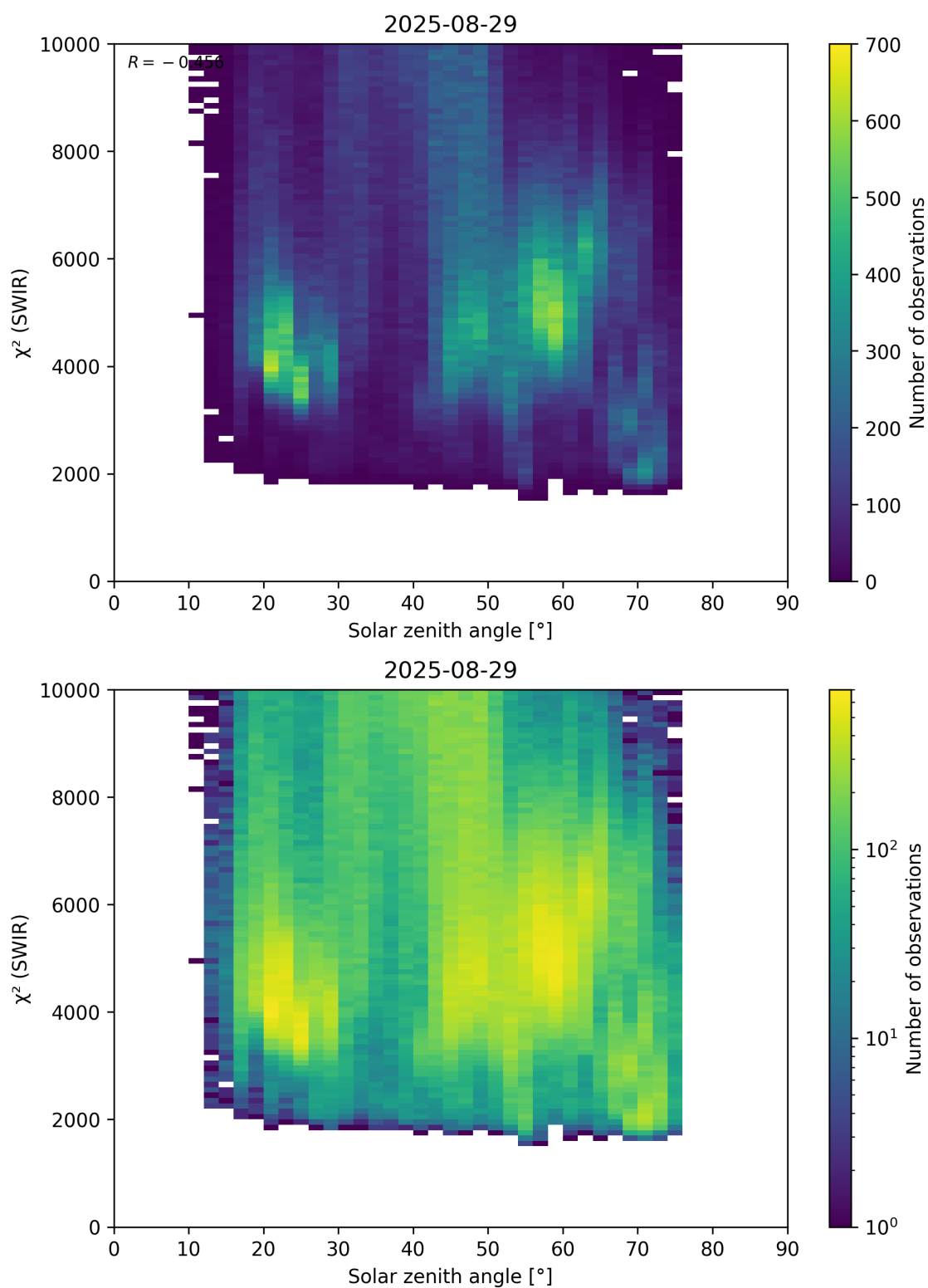
Figure 95: Scatter density plot of “Solar zenith angle” against “ \chi^2 (SWIR)” for 2025-08-28 to 2025-08-30.
