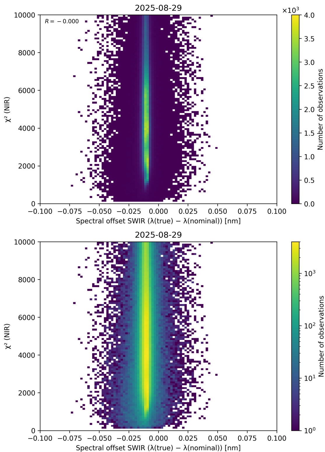
Figure 117: Scatter density plot of “Spectral offset SWIR ( \lambda_{\text{true}} - \lambda_{\text{nominal}} )” against “ \chi^2 (NIR)” for 2025-08-28 to 2025-08-30.
