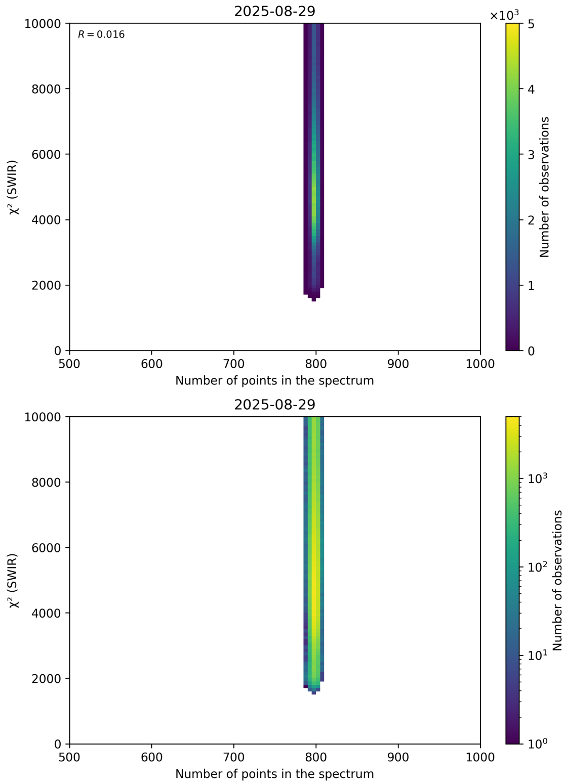
Figure 89: Scatter density plot of “Number of points in the spectrum” against “ \chi^2 (SWIR)” for 2025-08-28 to 2025-08-30.
