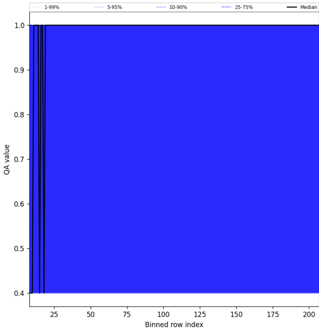
Figure 33: Along track statistics of “QA value” for 2025-08-28 to 2025-08-30
