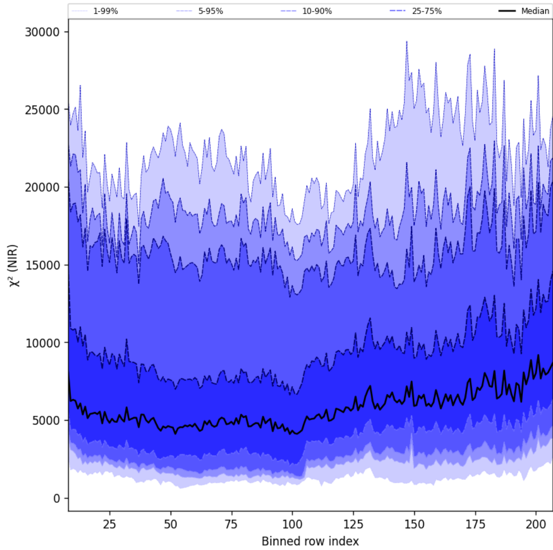
Figure 40: Along track statistics of " \chi^2 (NIR)" for 2025-08-28 to 2025-08-30
