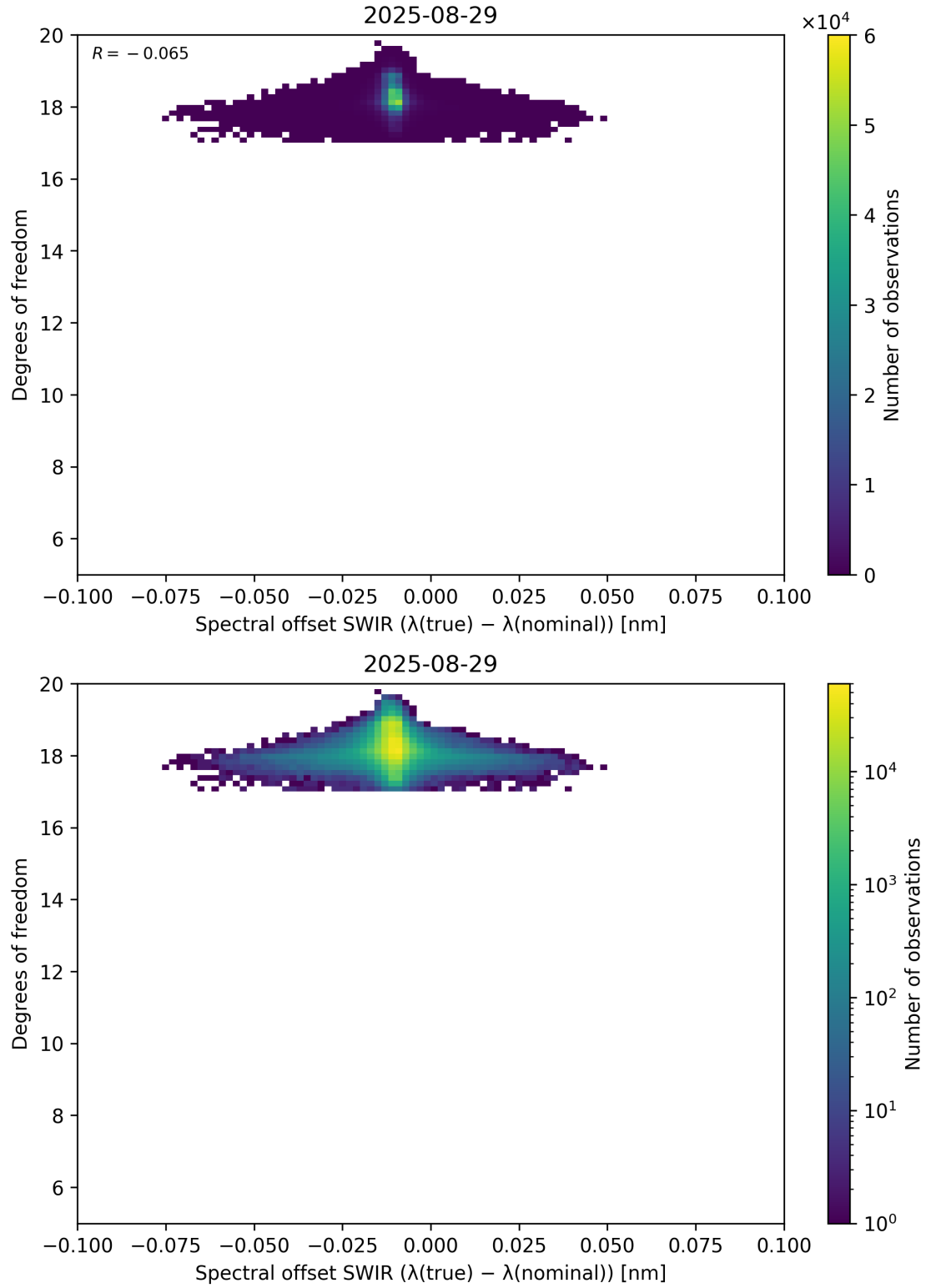
Figure 119: Scatter density plot of “Spectral offset SWIR ( \lambda_{\text{true}} - \lambda_{\text{nominal}} )” against “Degrees of freedom” for 2025-08-28 to 2025-08-30.
