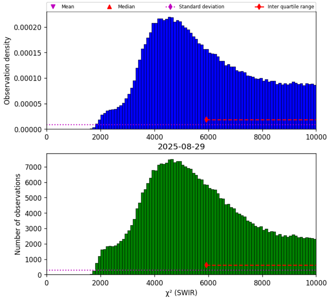
Figure 28: Histogram of " \chi^2 (SWIR)" for 2025-08-28 to 2025-08-30
