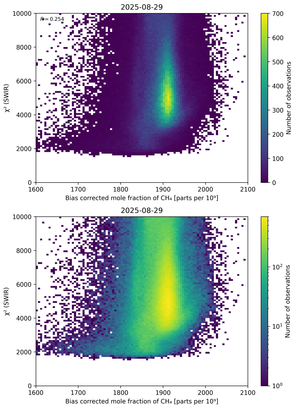
Figure 64: Scatter density plot of “Bias corrected mole fraction of \text{CH}_4 ” against “ \chi^2 (SWIR)” for 2025-08-28 to 2025-08-30.
