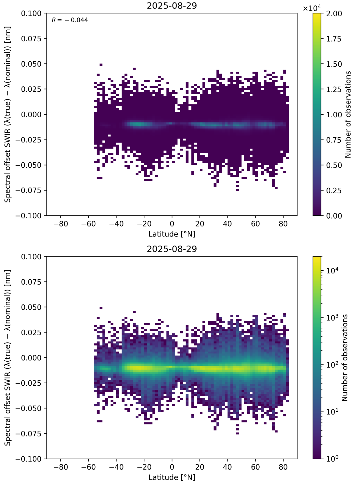
Figure 62: Scatter density plot of “Latitude” against “Spectral offset SWIR ( \lambda_{\text{true}} - \lambda_{\text{nominal}} )” for 2025-08-28 to 2025-08-30.
