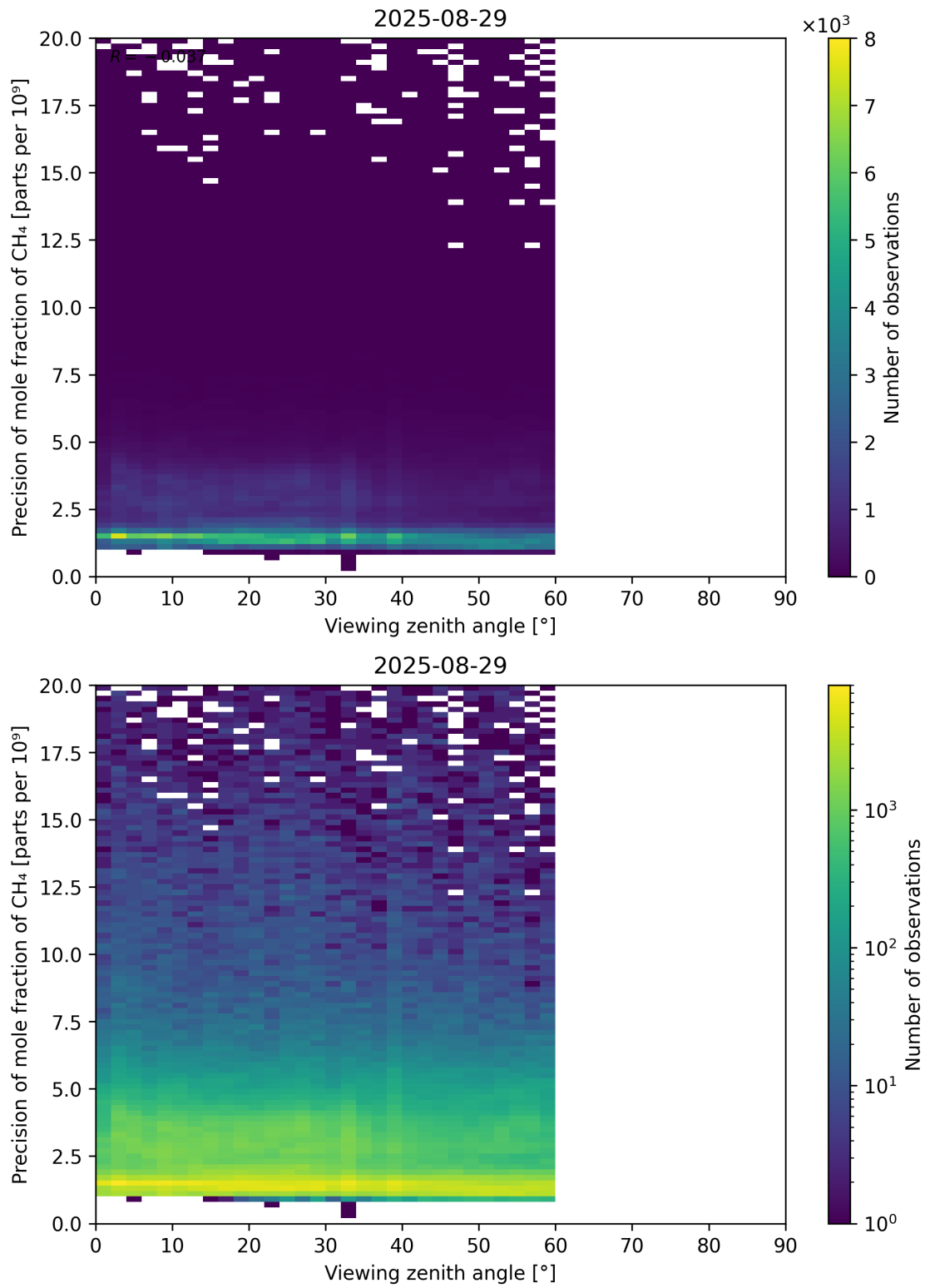
Figure 112: Scatter density plot of “Viewing zenith angle” against “Precision of mole fraction of CH 4 ” for 2025-08-28 to 2025-08-30.
