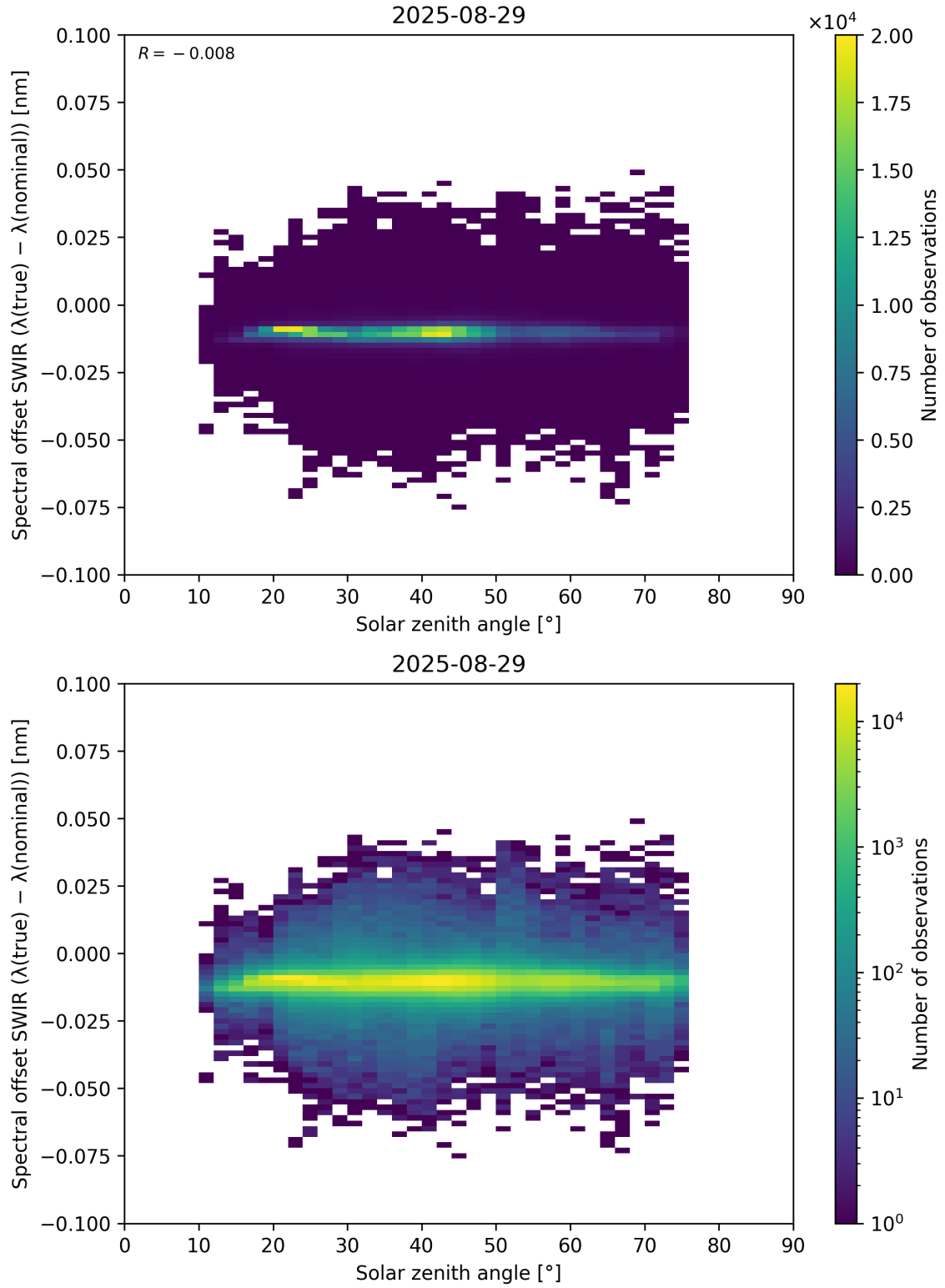
Figure 104: Scatter density plot of “Solar zenith angle” against “Spectral offset SWIR ( \lambda_{\text{true}} - \lambda_{\text{nominal}} )” for 2025-08-28 to 2025-08-30.
