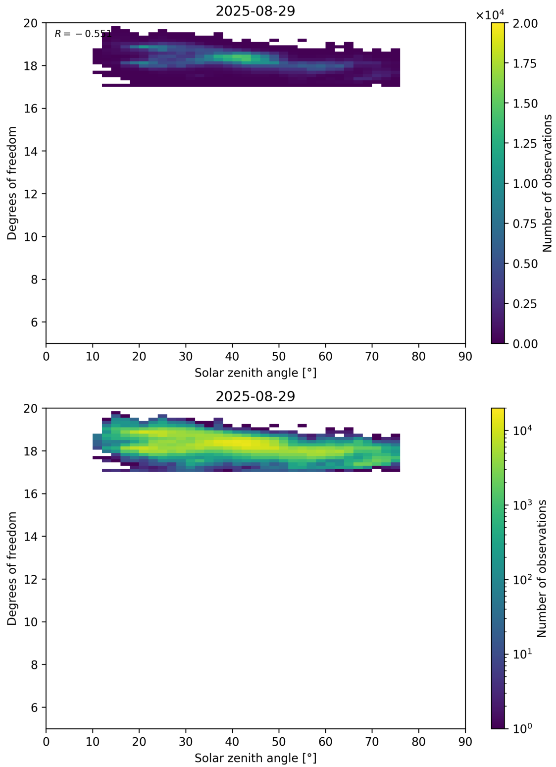
Figure 96: Scatter density plot of “Solar zenith angle” against “Degrees of freedom” for 2025-08-28 to 2025-08-30.
