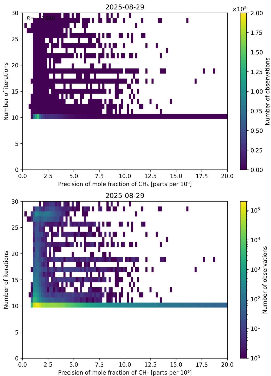
Figure 83: Scatter density plot of “Precision of mole fraction of CH 4 ” against “Number of iterations” for 2025-08-28 to 2025-08-30.
