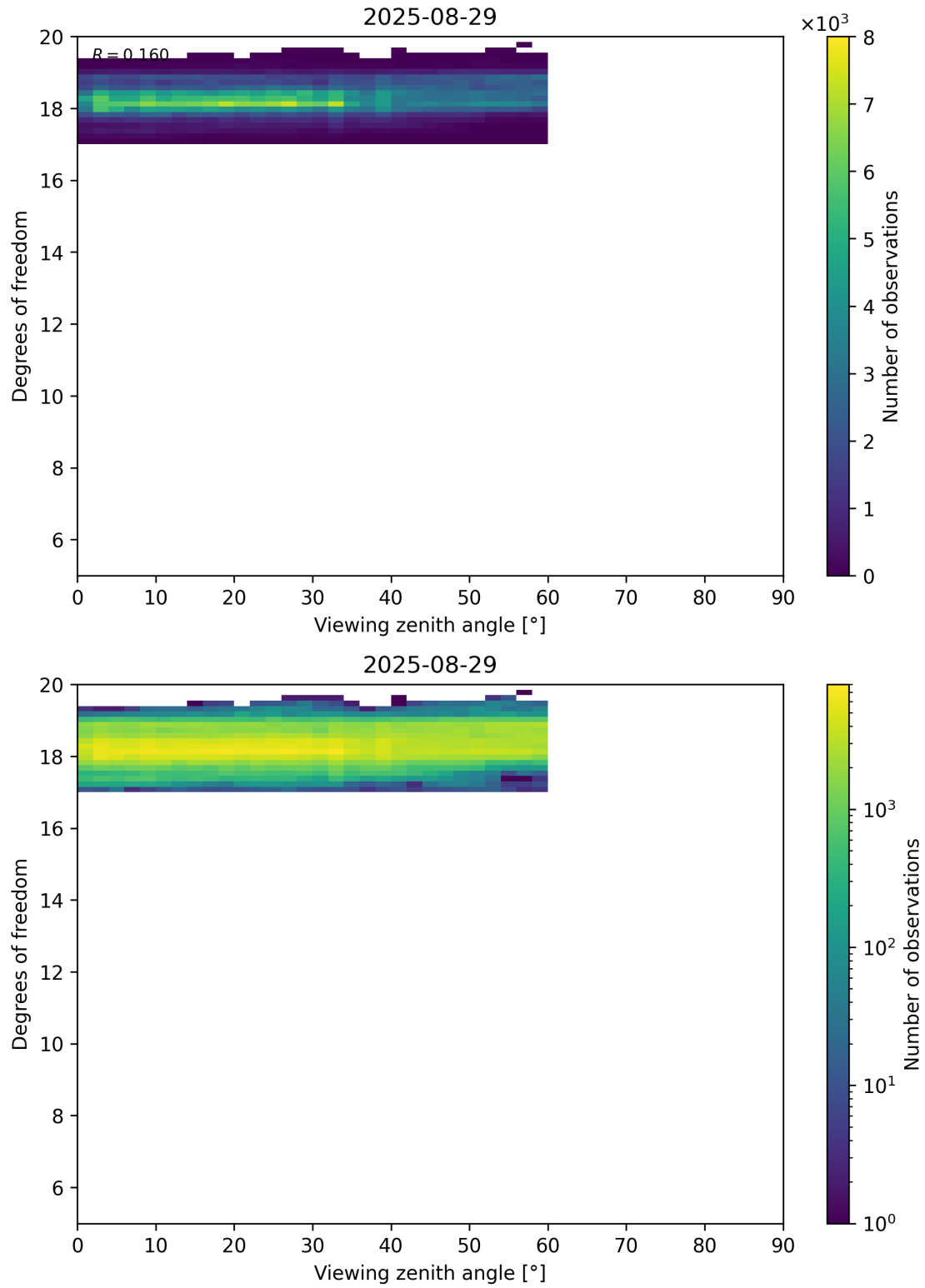
Figure 107: Scatter density plot of “Viewing zenith angle” against “Degrees of freedom” for 2025-08-28 to 2025-08-30.
