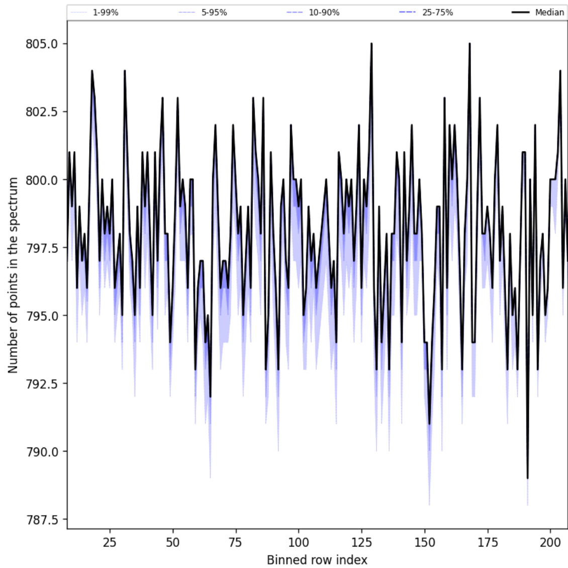
Figure 37: Along track statistics of “Number of points in the spectrum” for 2025-08-28 to 2025-08-30
