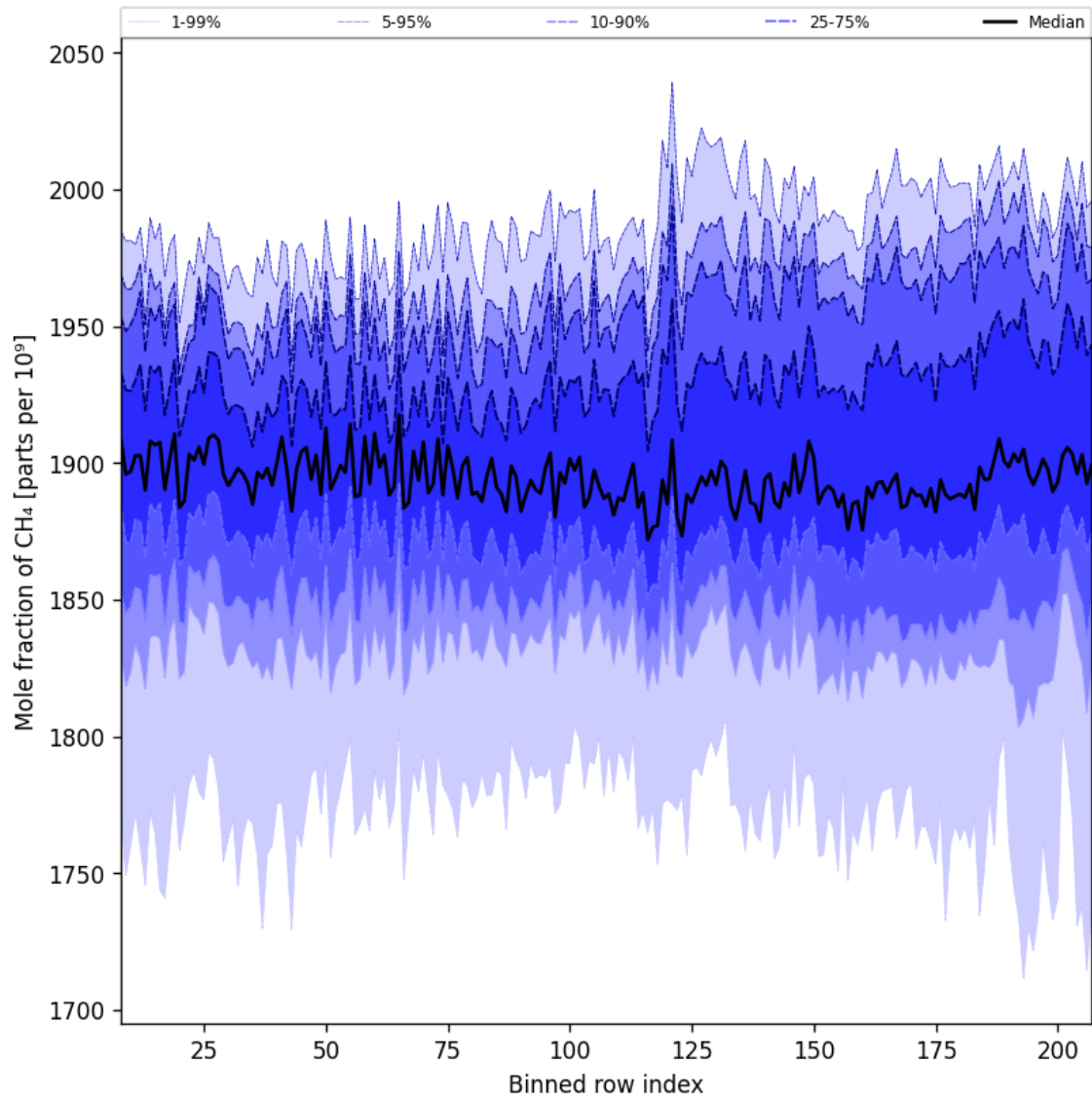
Figure 34: Along track statistics of “Mole fraction of CH 4 ” for 2025-08-28 to 2025-08-30
