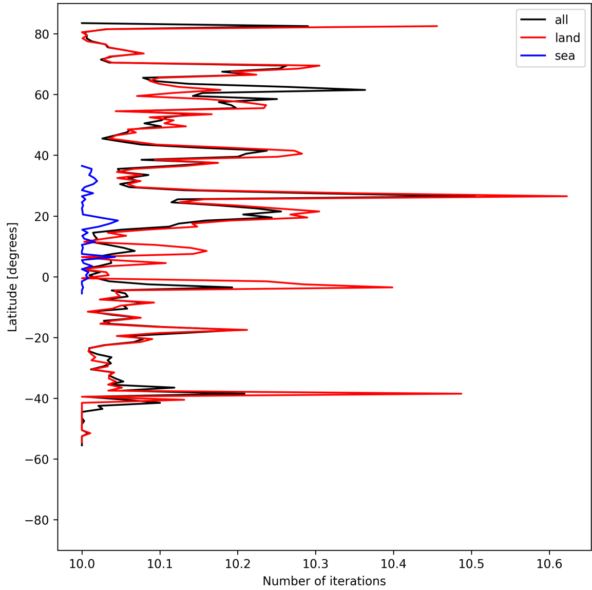
Figure 20: Zonal average of “Number of iterations” for 2025-08-28 to 2025-08-30.
