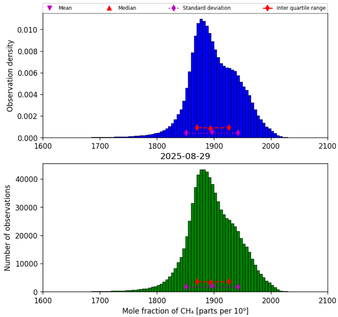
Figure 23: Histogram of “Mole fraction of CH 4 ” for 2025-08-28 to 2025-08-30
