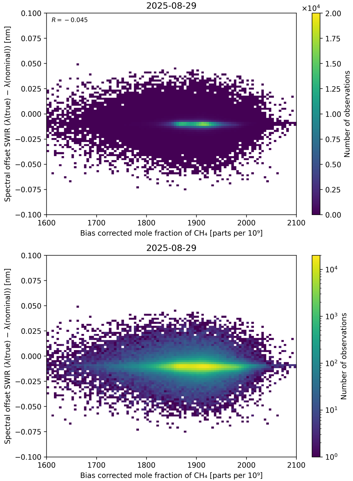
Figure 69: Scatter density plot of “Bias corrected mole fraction of \text{CH}_4 ” against “Spectral offset SWIR ( \lambda_{\text{true}} - \lambda_{\text{nominal}} )” for 2025-08-28 to 2025-08-30.
