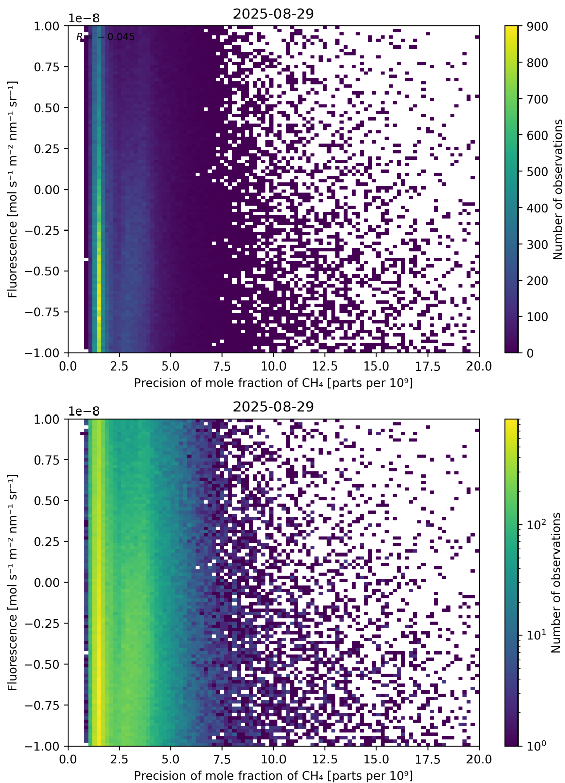
Figure 81: Scatter density plot of “Precision of mole fraction of \text{CH}_4 ” against “Fluorescence” for 2025-08-28 to 2025-08-30.
