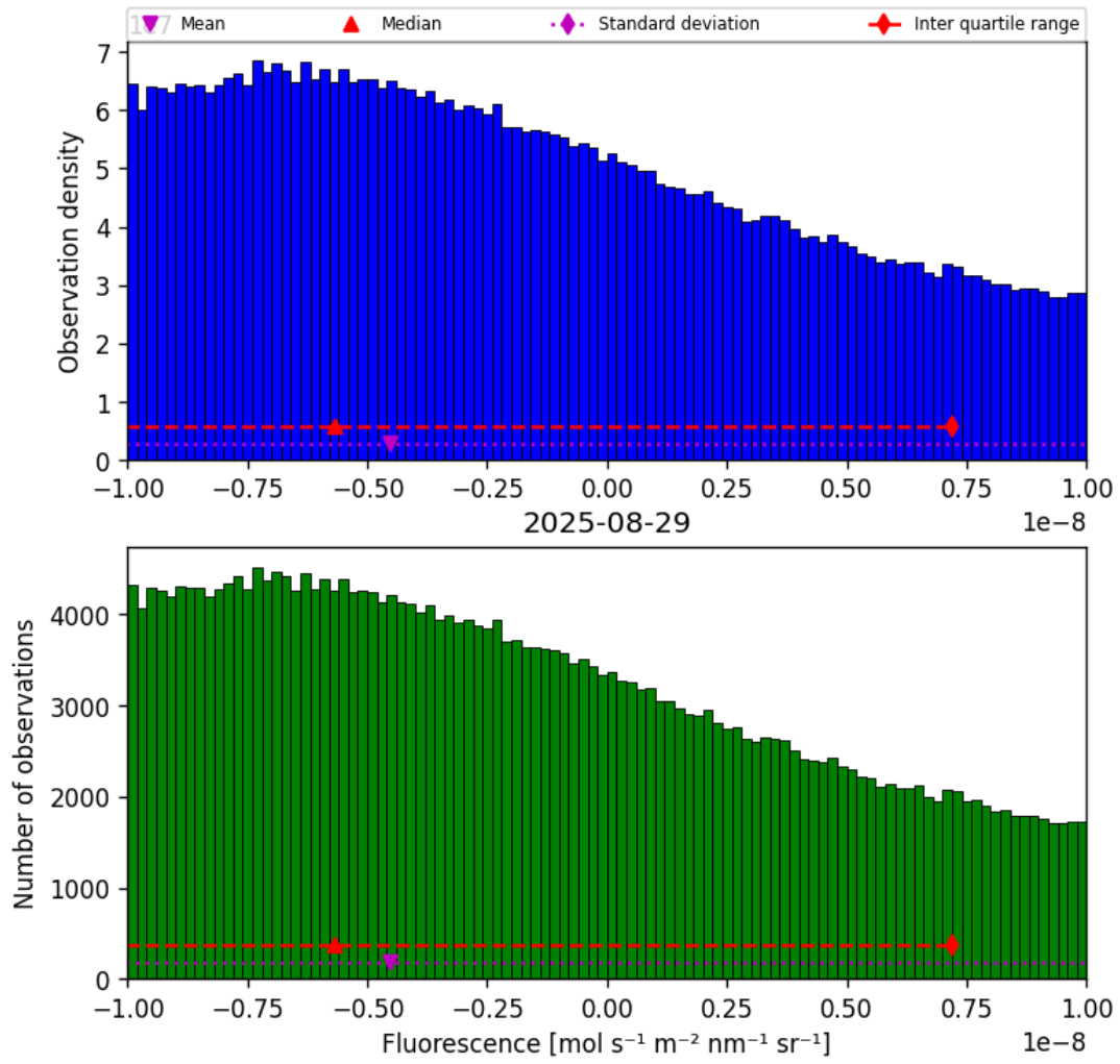
Figure 32: Histogram of “Fluorescence” for 2025-08-28 to 2025-08-30
