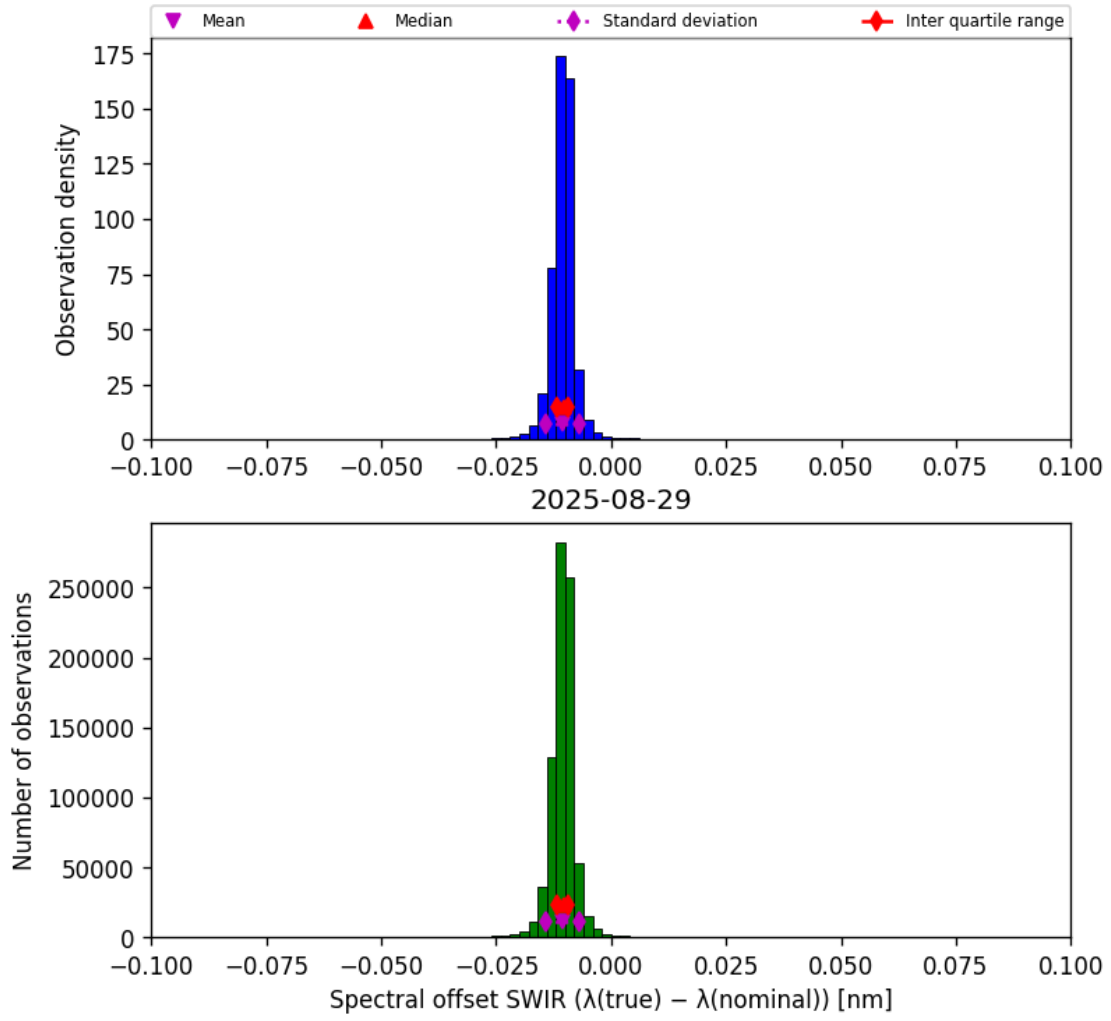
Figure 27: Histogram of “Spectral offset SWIR ( \lambda_{\text{true}} - \lambda_{\text{nominal}} )” for 2025-08-28 to 2025-08-30
