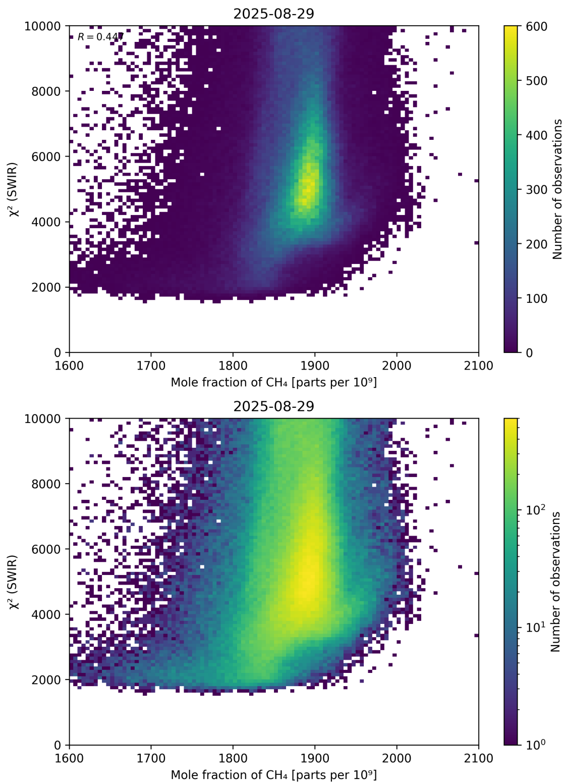
Figure 71: Scatter density plot of “Mole fraction of \text{CH}_4 ” against “ \chi^2 (SWIR)” for 2025-08-28 to 2025-08-30.
