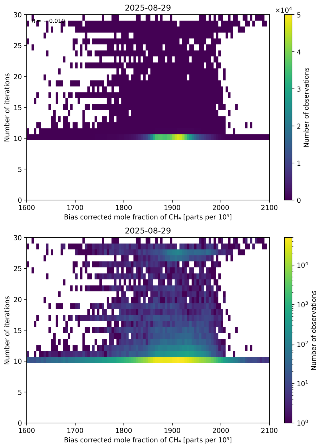
Figure 67: Scatter density plot of “Bias corrected mole fraction of \text{CH}_4 ” against “Number of iterations” for 2025-08-28 to 2025-08-30.
