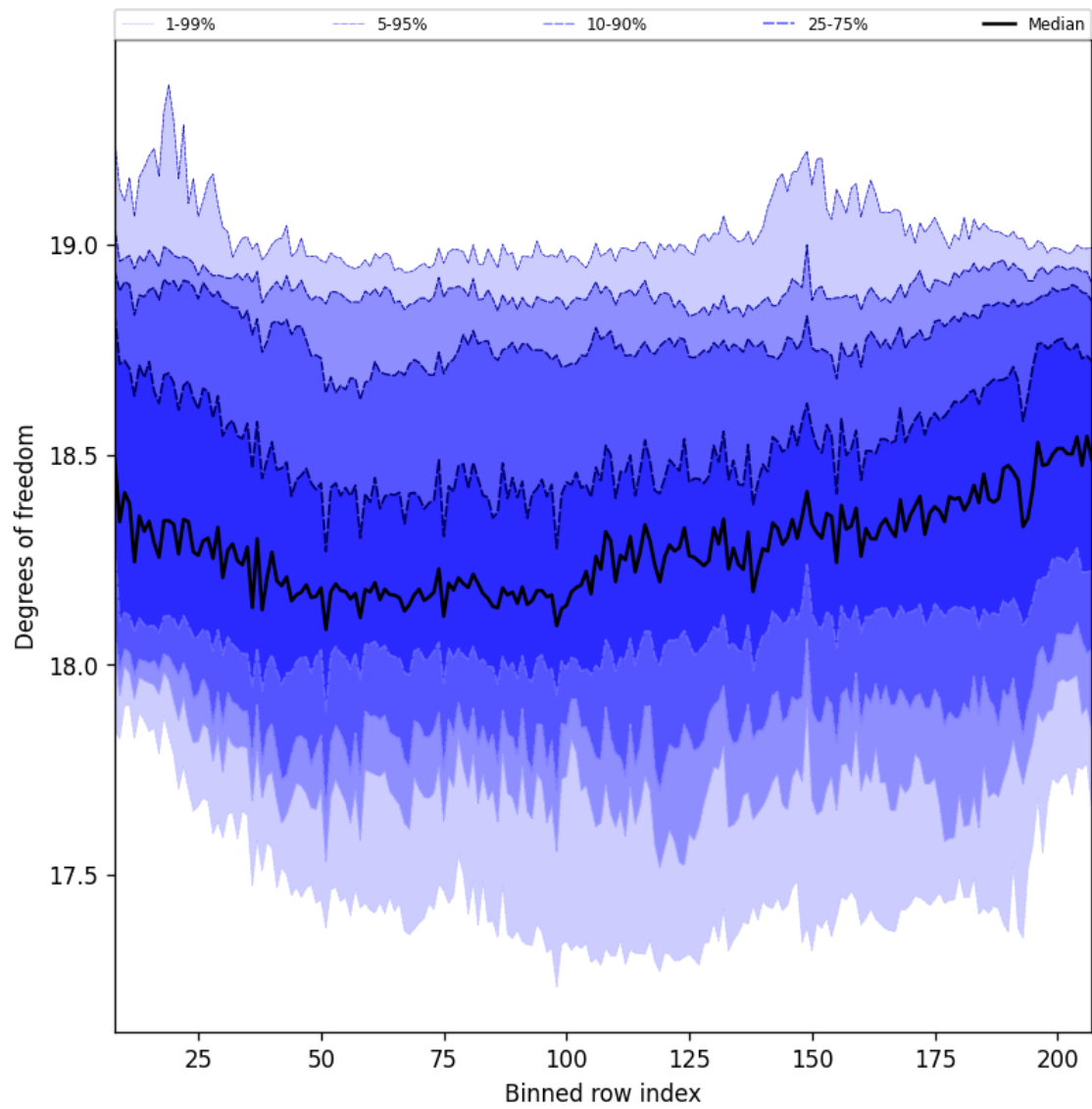
Figure 41: Along track statistics of “Degrees of freedom” for 2025-08-28 to 2025-08-30
