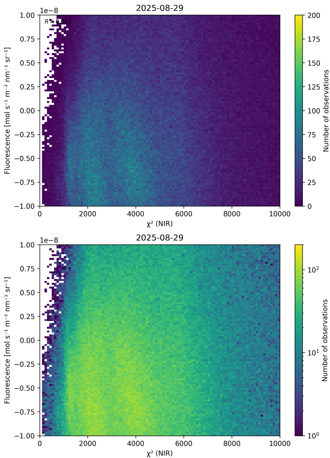
Figure 45: Scatter density plot of “ \chi^2 (NIR)” against “Fluorescence” for 2025-08-28 to 2025-08-30.
