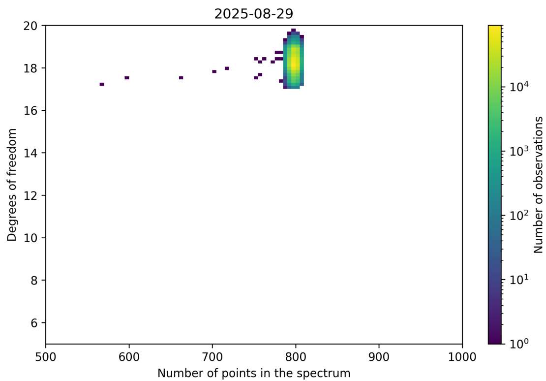
Figure 90: Scatter density plot of “Number of points in the spectrum” against “Degrees of freedom” for 2025-08-28 to 2025-08-30.
