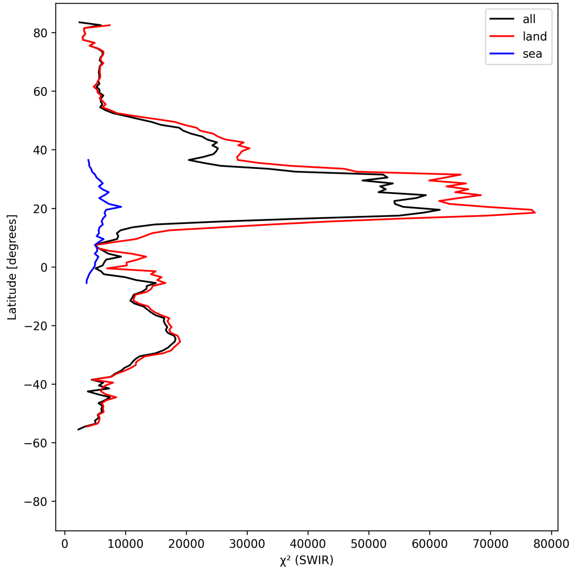
Figure 17: Zonal average of “ \chi^2 (SWIR)” for 2025-08-28 to 2025-08-30.
