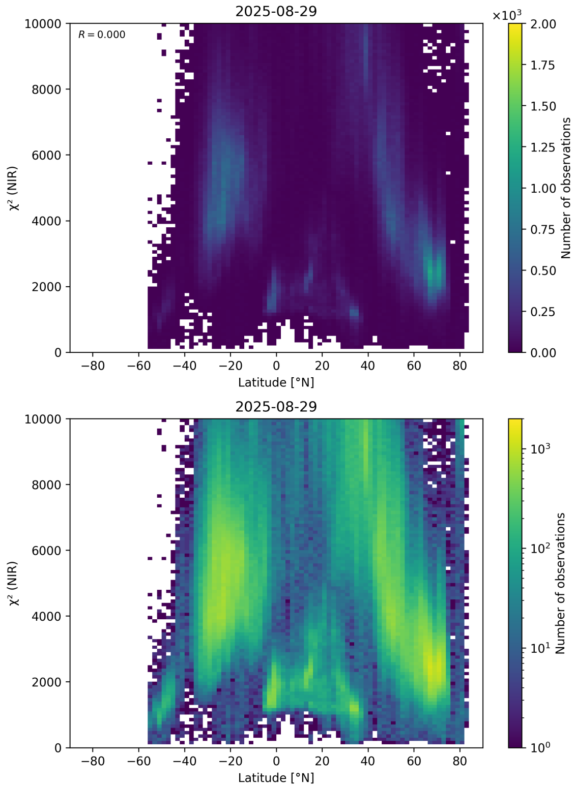
Figure 53: Scatter density plot of “Latitude” against “ \chi^2 (NIR)” for 2025-08-28 to 2025-08-30.
