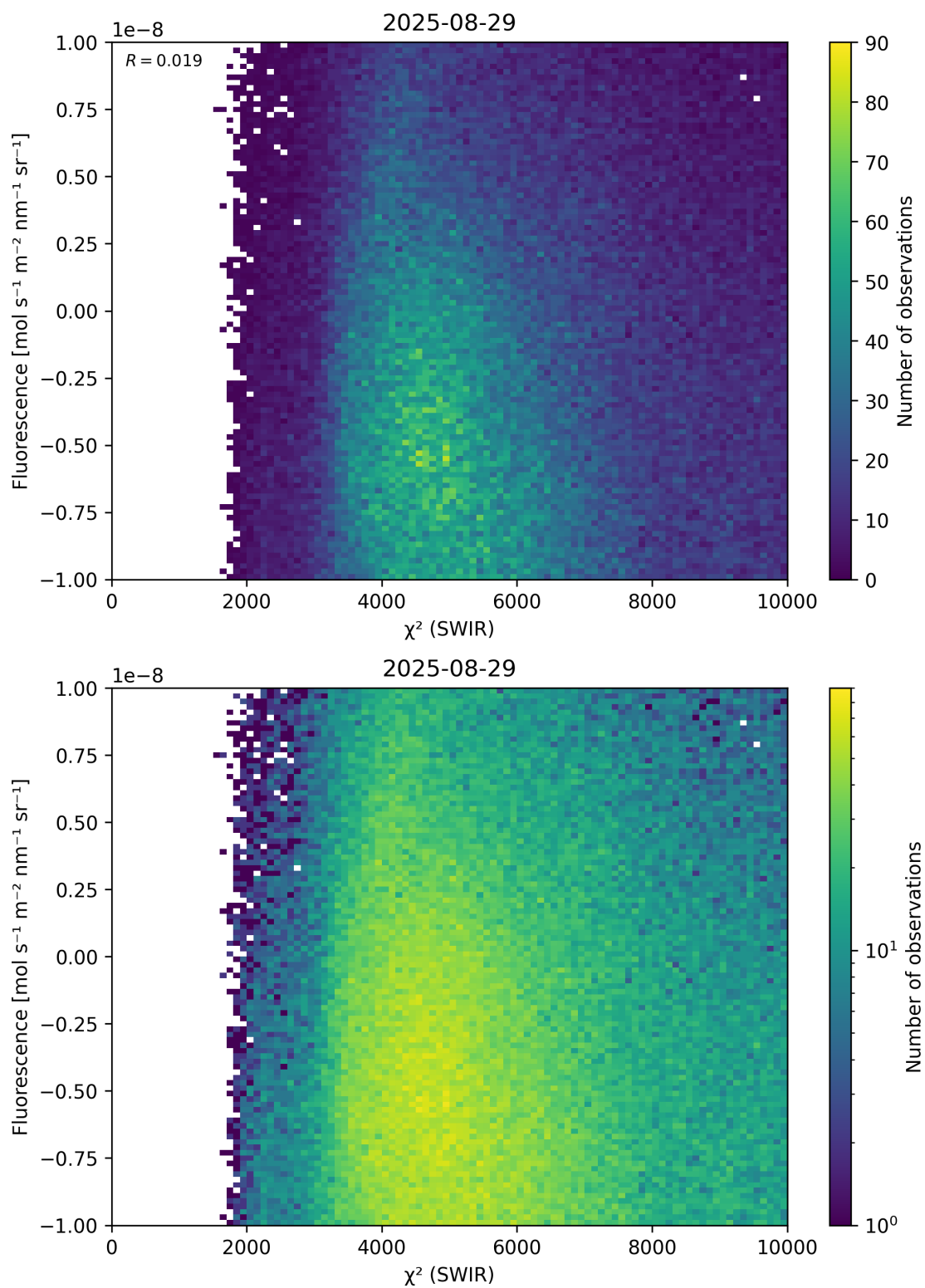
Figure 49: Scatter density plot of “ \chi^2 (SWIR)” against “Fluorescence” for 2025-08-28 to 2025-08-30.
