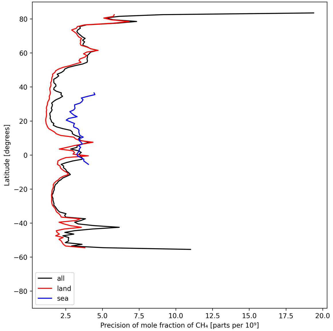
Figure 13: Zonal average of “Precision of mole fraction of CH 4 ” for 2025-08-28 to 2025-08-30.
