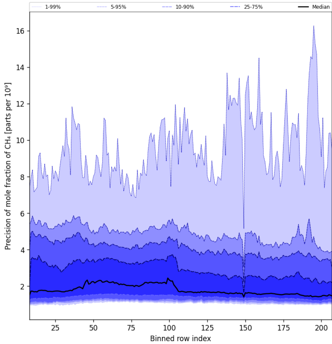
Figure 35: Along track statistics of “Precision of mole fraction of CH 4 ” for 2025-08-28 to 2025-08-30
