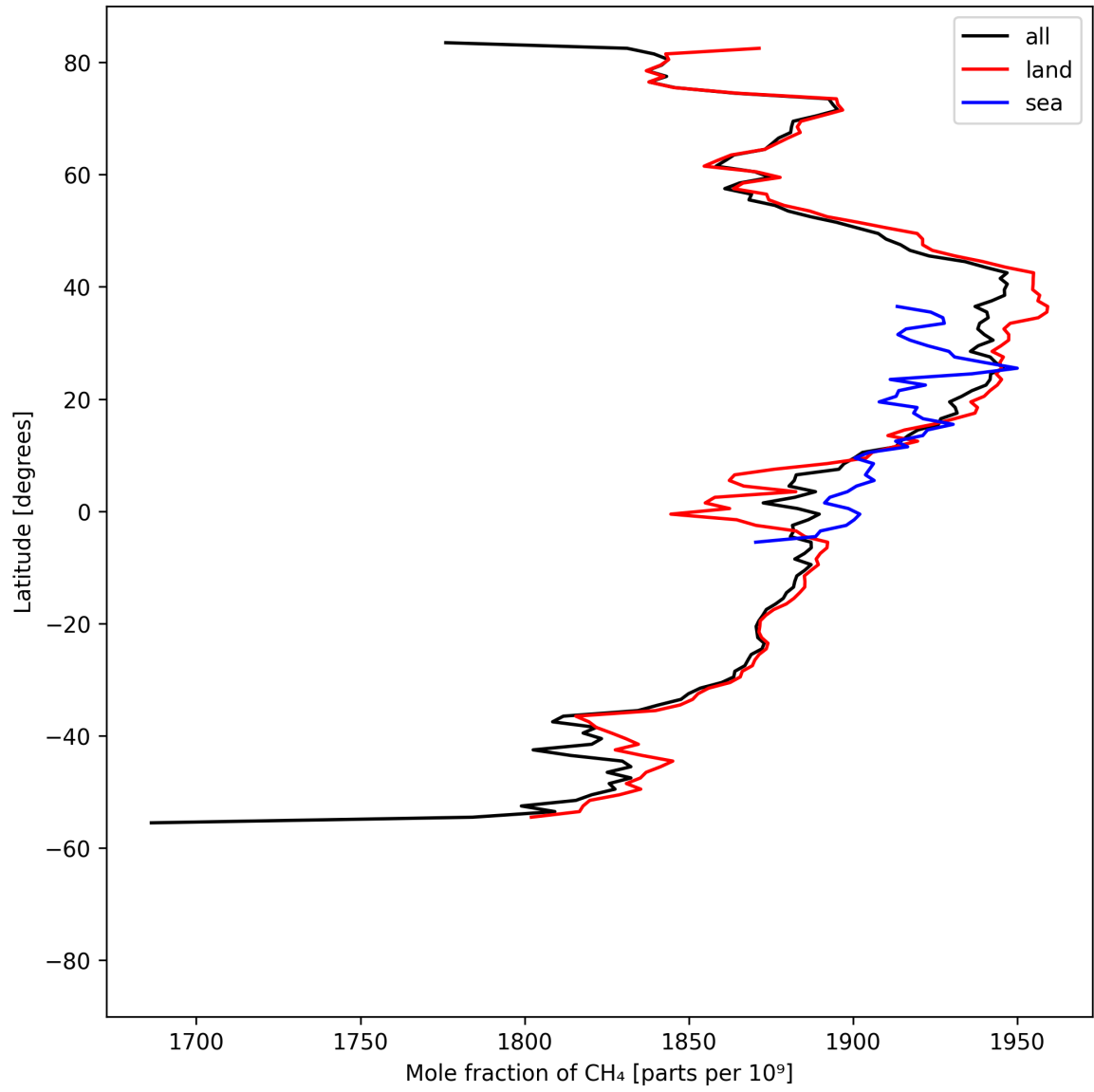
Figure 12: Zonal average of “Mole fraction of \text{CH}_4 ” for 2025-08-28 to 2025-08-30.
