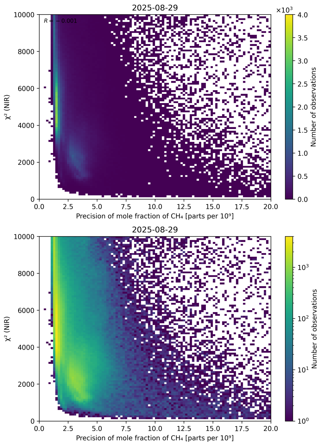
Figure 78: Scatter density plot of “Precision of mole fraction of CH 4 ” against “ \chi^2 (NIR)” for 2025-08-28 to 2025-08-30.
