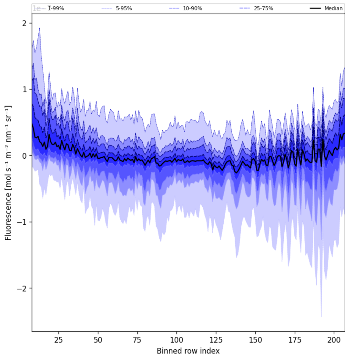
Figure 43: Along track statistics of “Fluorescence” for 2025-08-28 to 2025-08-30
