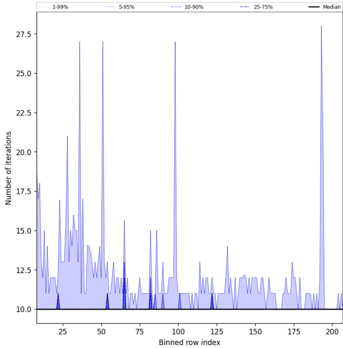
Figure 42: Along track statistics of “Number of iterations” for 2025-08-28 to 2025-08-30
