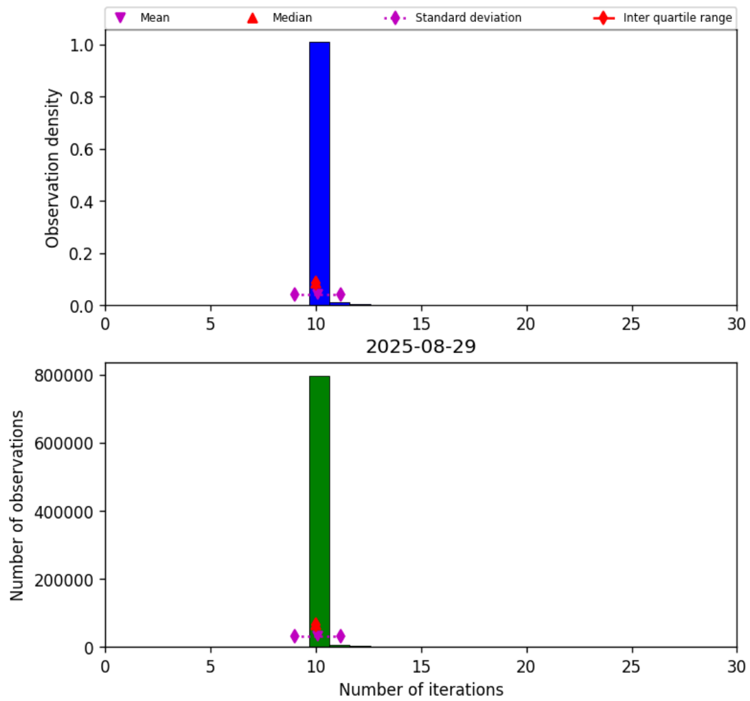
Figure 31: Histogram of “Number of iterations” for 2025-08-28 to 2025-08-30
