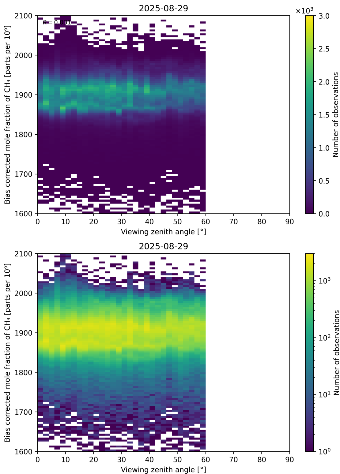
Figure 111: Scatter density plot of “Viewing zenith angle” against “Bias corrected mole fraction of CH 4 ” for 2025-08-28 to 2025-08-30.
