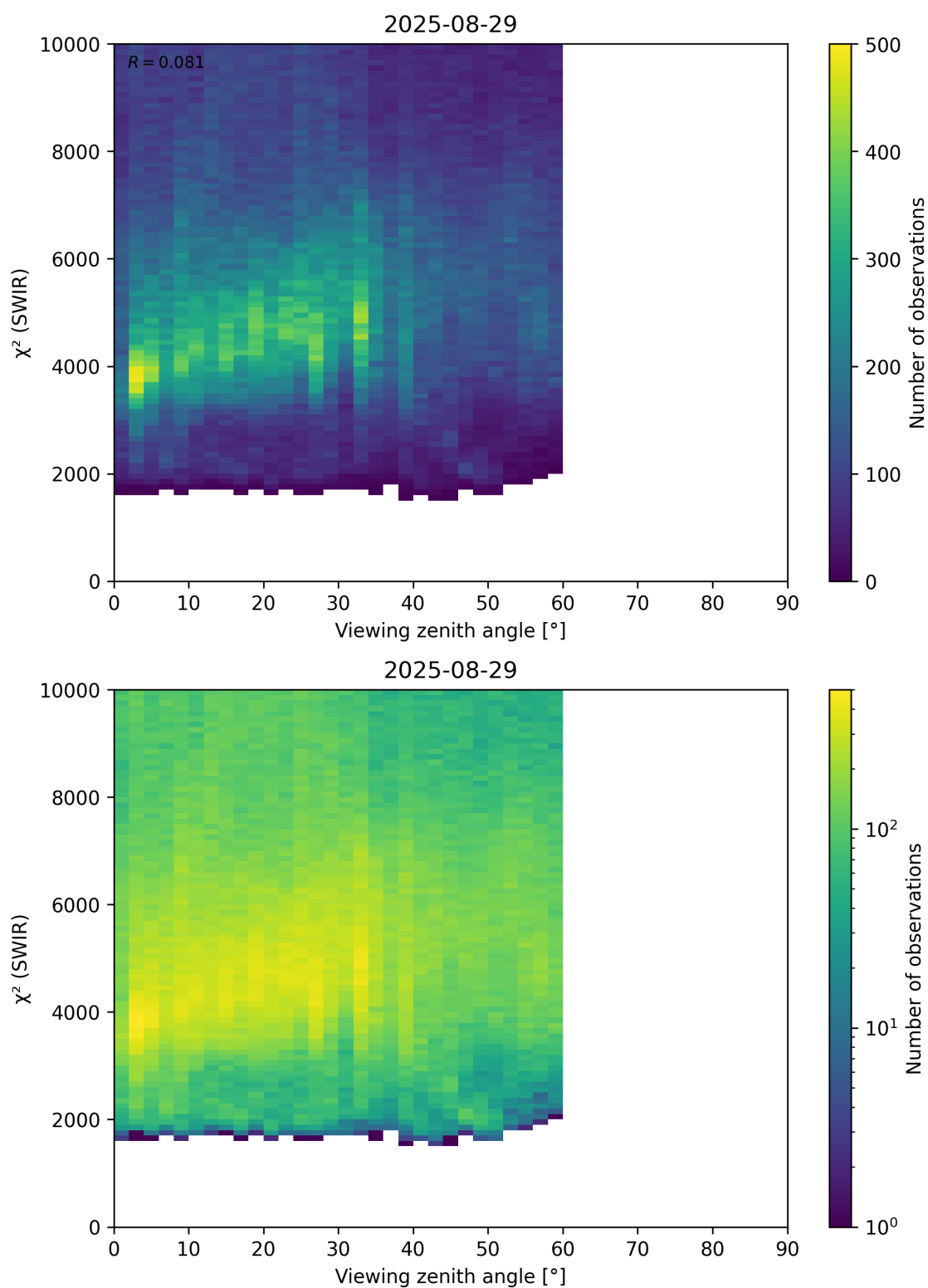
Figure 106: Scatter density plot of “Viewing zenith angle” against “ \chi^2 (SWIR)” for 2025-08-28 to 2025-08-30.
