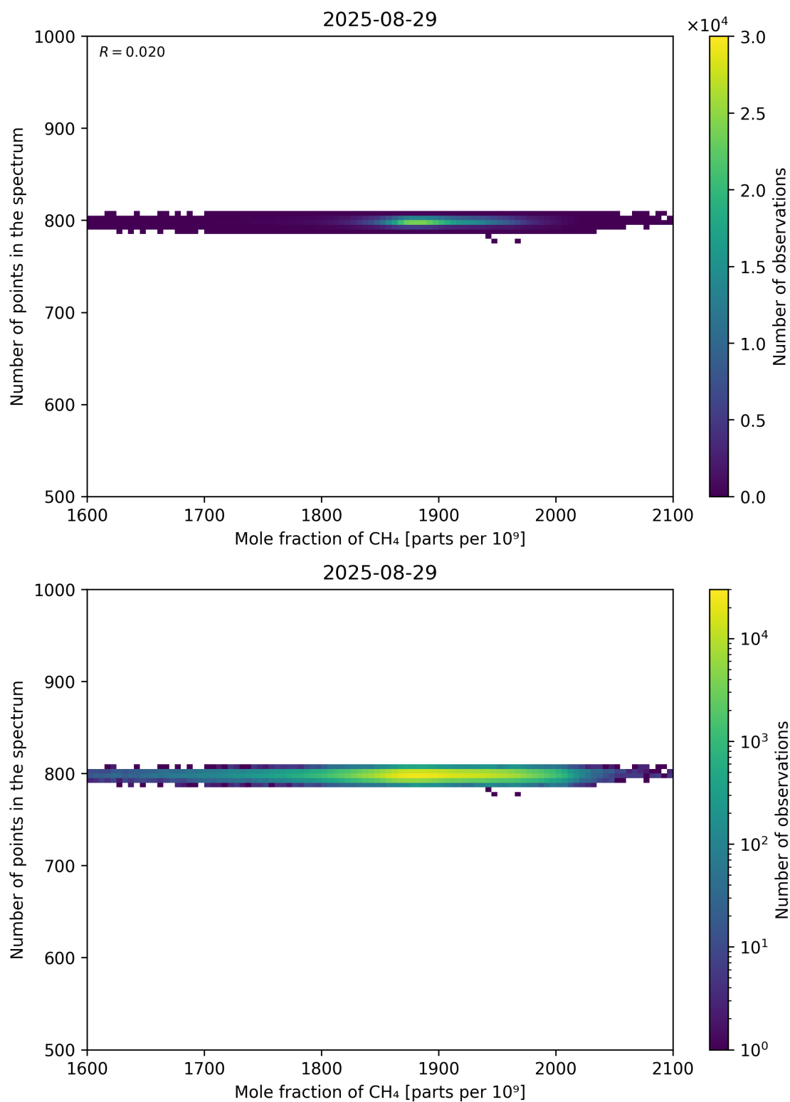
Figure 77: Scatter density plot of “Mole fraction of CH 4 ” against “Number of points in the spectrum” for 2025-08-28 to 2025-08-30.
