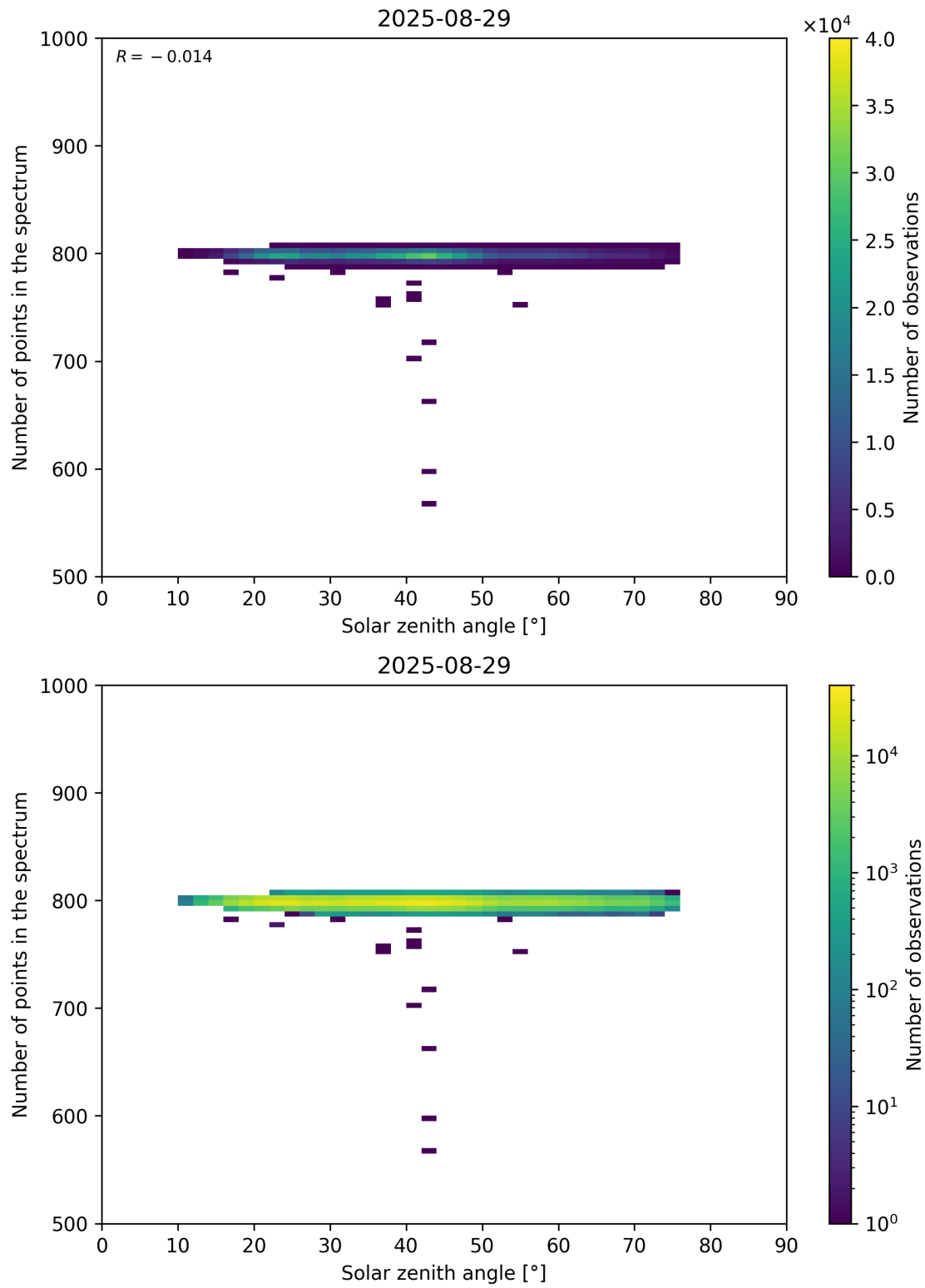
Figure 103: Scatter density plot of “Solar zenith angle” against “Number of points in the spectrum” for 2025-08-28 to 2025-08-30.
