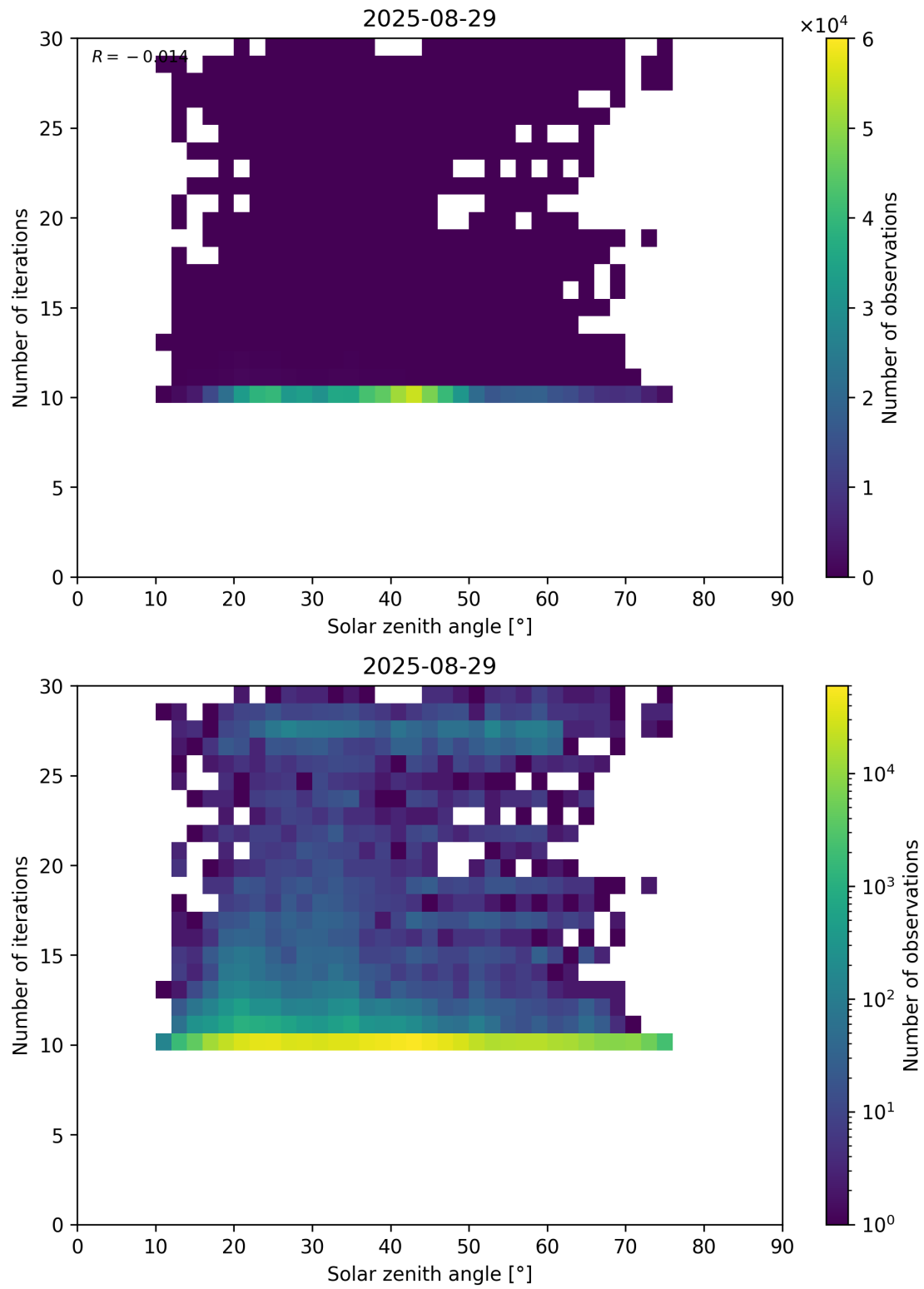
Figure 102: Scatter density plot of “Solar zenith angle” against “Number of iterations” for 2025-08-28 to 2025-08-30.
