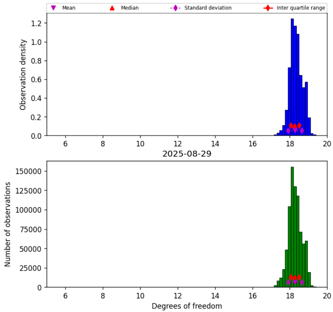
Figure 30: Histogram of “Degrees of freedom” for 2025-08-28 to 2025-08-30
