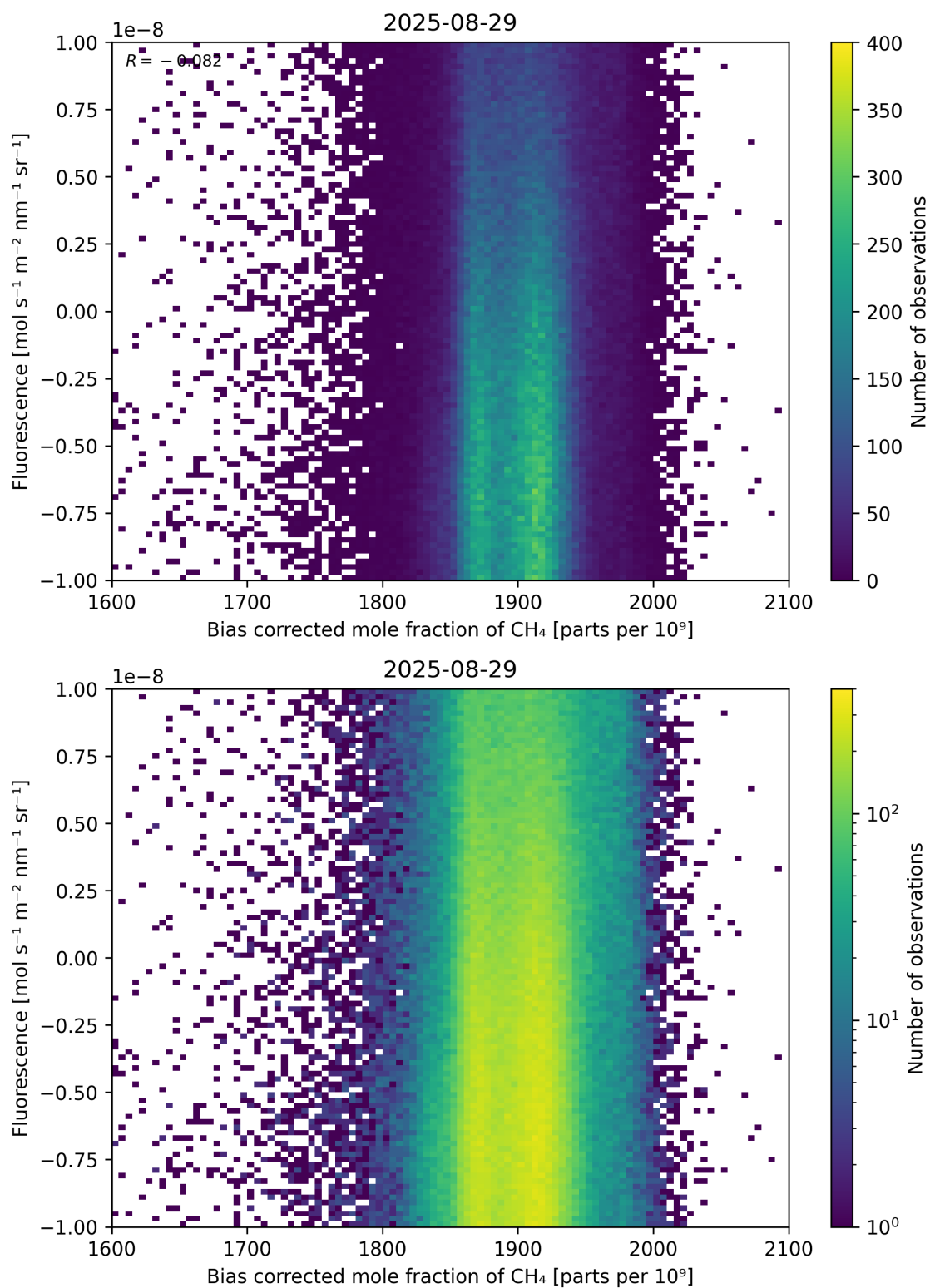
Figure 66: Scatter density plot of “Bias corrected mole fraction of \text{CH}_4 ” against “Fluorescence” for 2025-08-28 to 2025-08-30.
