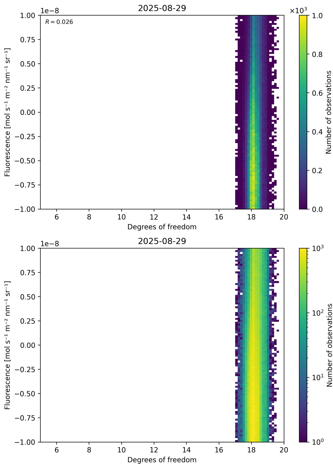
Figure 51: Scatter density plot of “Degrees of freedom” against “Fluorescence” for 2025-08-28 to 2025-08-30.
