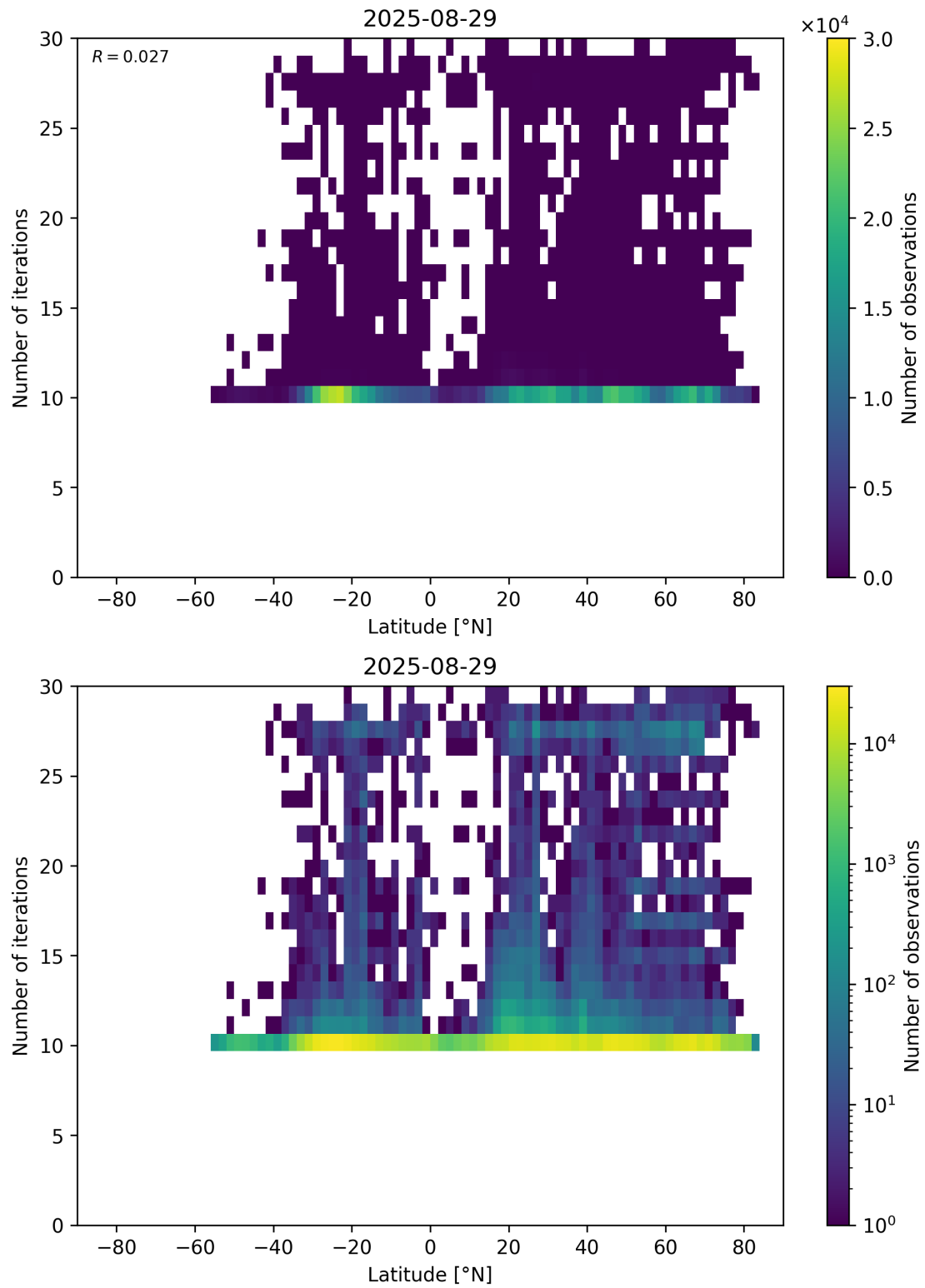
Figure 60: Scatter density plot of “Latitude” against “Number of iterations” for 2025-08-28 to 2025-08-30.
