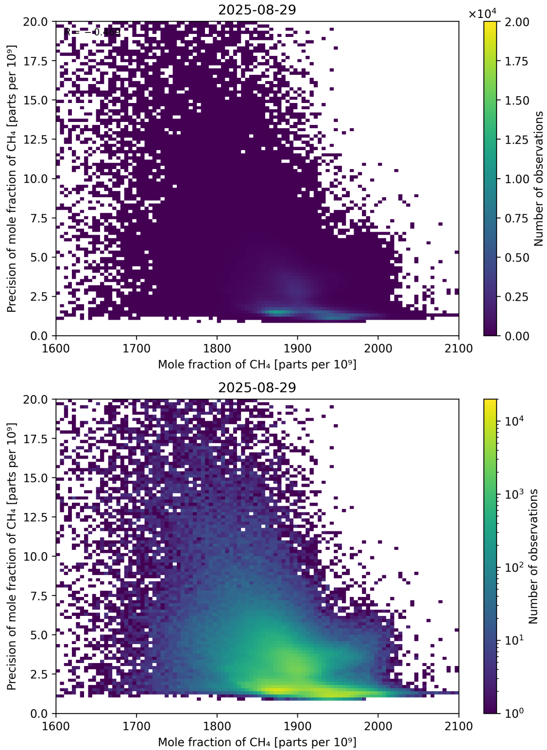
Figure 75: Scatter density plot of “Mole fraction of CH 4 ” against “Precision of mole fraction of CH 4 ” for 2025-08-28 to 2025-08-30.
