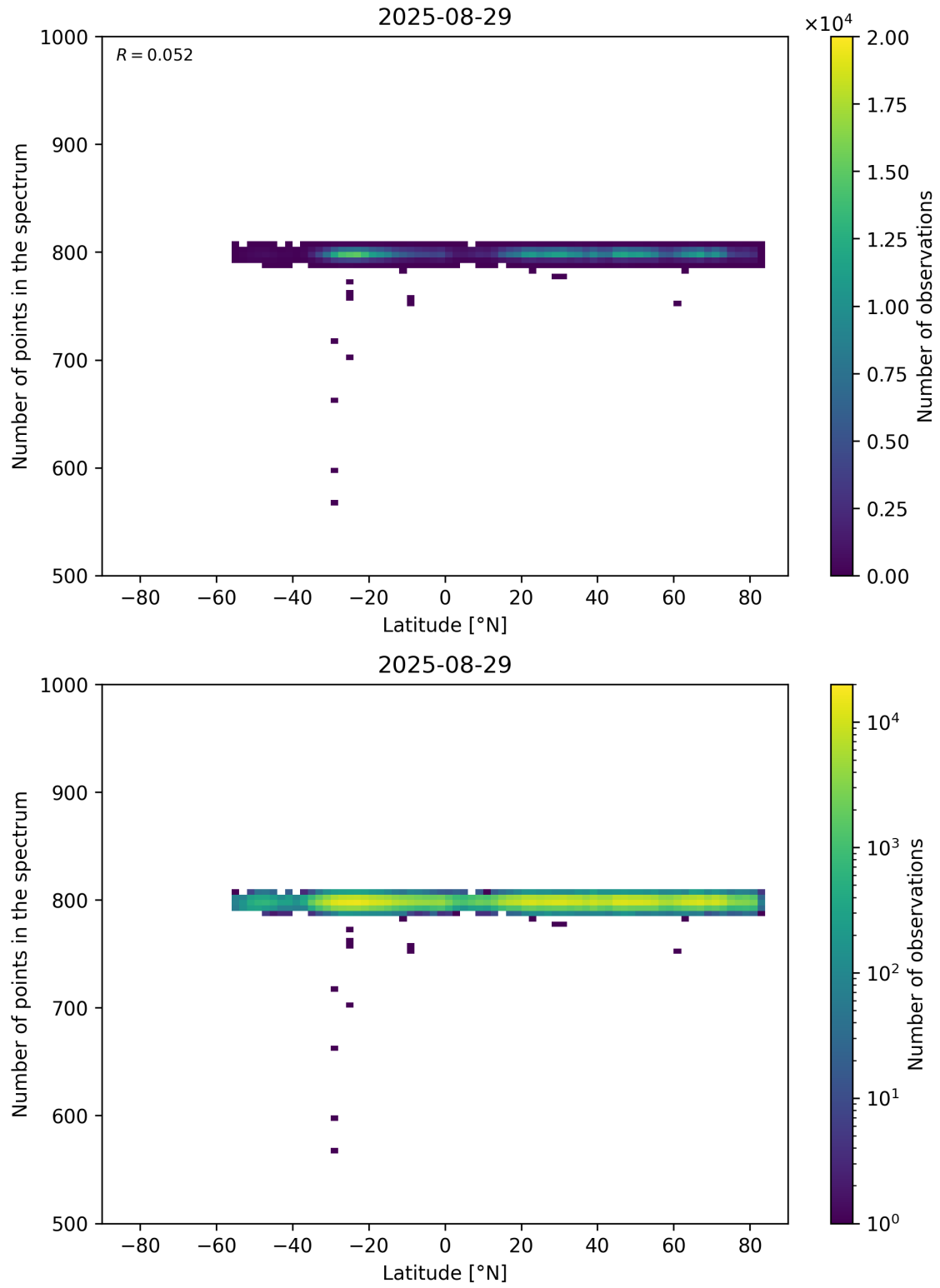
Figure 61: Scatter density plot of “Latitude” against “Number of points in the spectrum” for 2025-08-28 to 2025-08-30.
