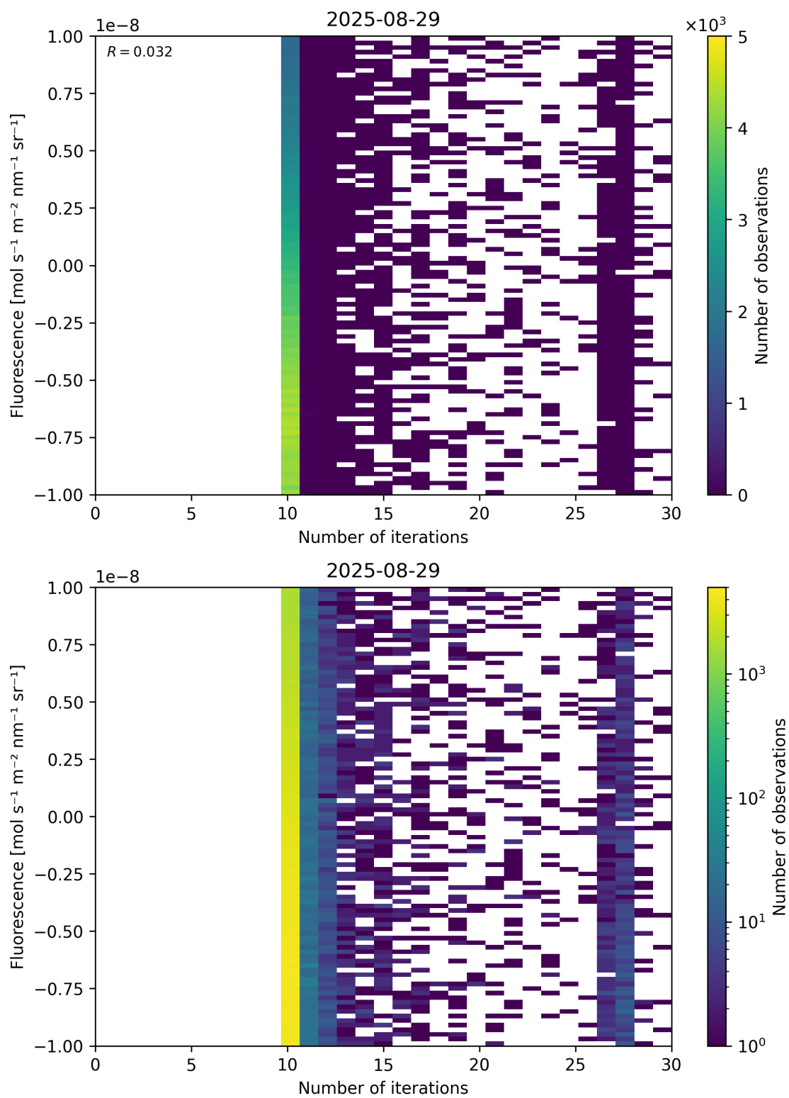
Figure 87: Scatter density plot of “Number of iterations” against “Fluorescence” for 2025-08-28 to 2025-08-30.
