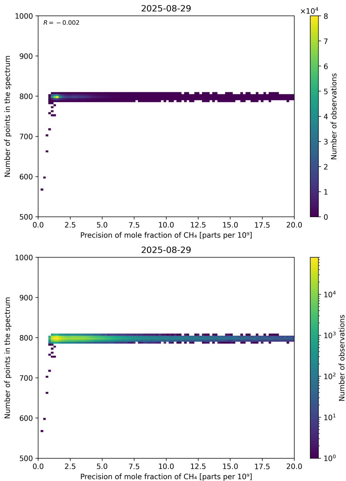
Figure 84: Scatter density plot of “Precision of mole fraction of CH 4 ” against “Number of points in the spectrum” for 2025-08-28 to 2025-08-30.
