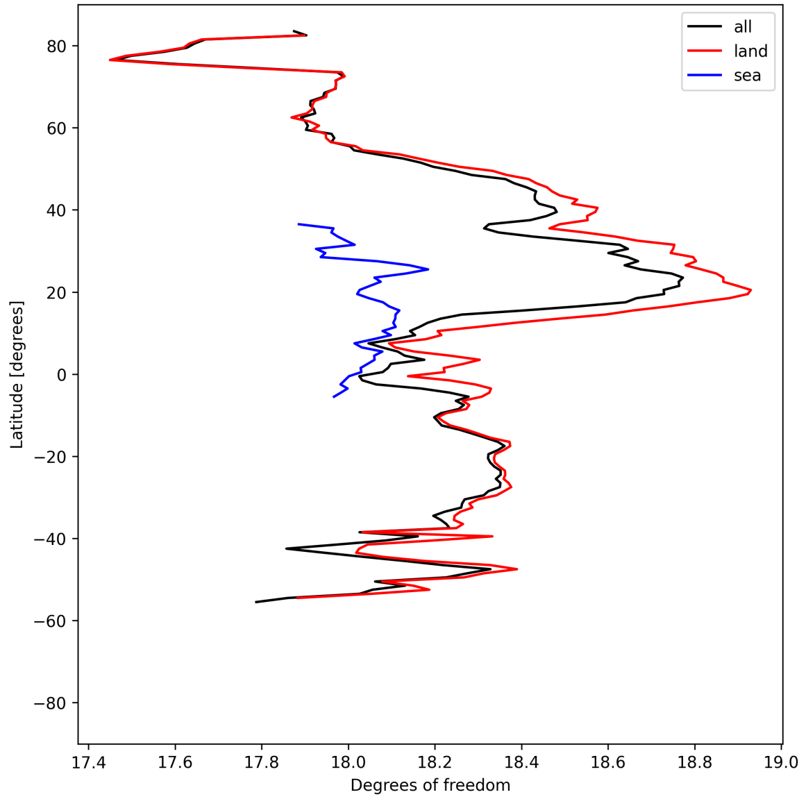
Figure 19: Zonal average of “Degrees of freedom” for 2025-08-28 to 2025-08-30.
