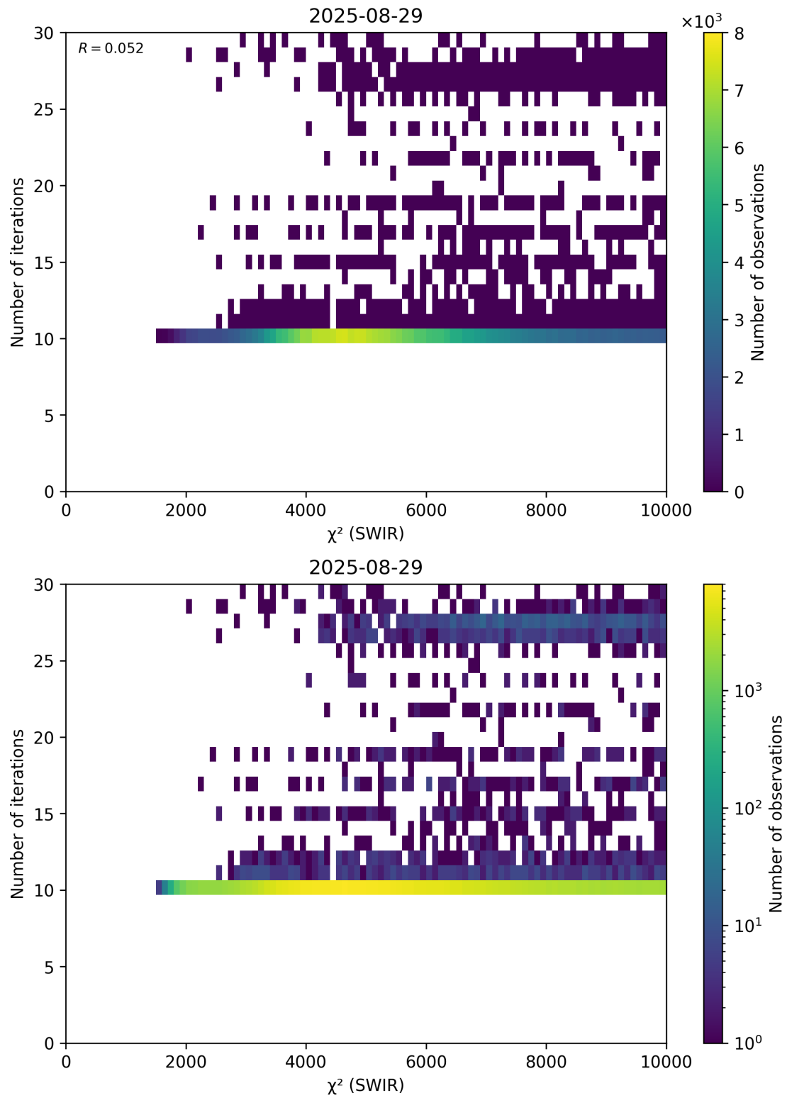
Figure 50: Scatter density plot of “ \chi^2 (SWIR)” against “Number of iterations” for 2025-08-28 to 2025-08-30.
