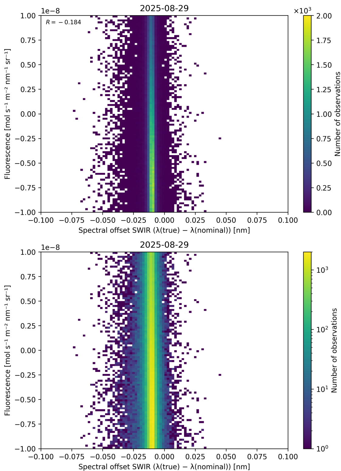
Figure 120: Scatter density plot of “Spectral offset SWIR ( \lambda_{\text{true}} - \lambda_{\text{nominal}} )” against “Fluorescence” for 2025-08-28 to 2025-08-30.
