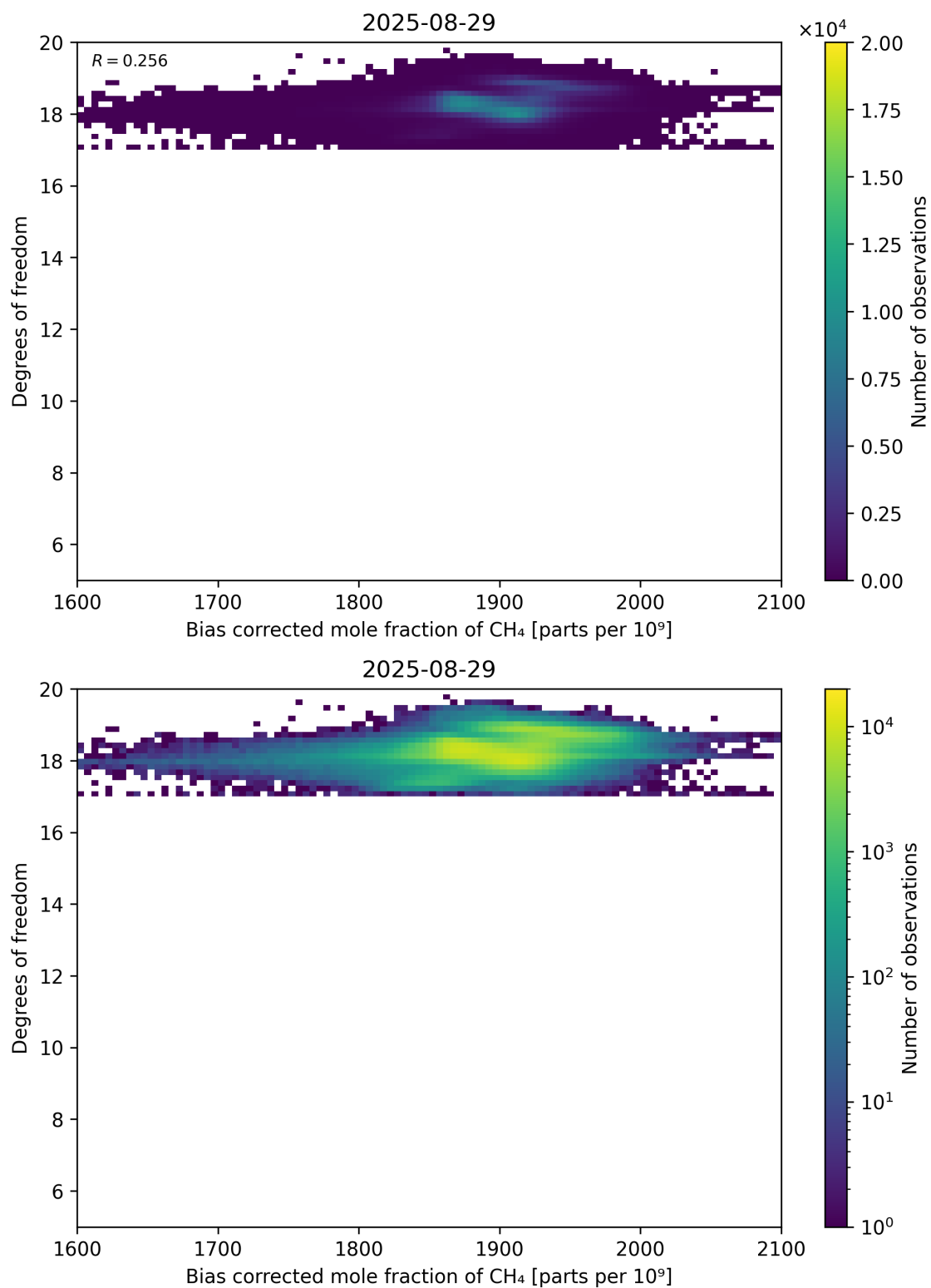
Figure 65: Scatter density plot of “Bias corrected mole fraction of CH 4 ” against “Degrees of freedom” for 2025-08-28 to 2025-08-30.
