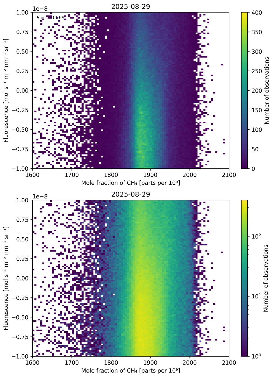
Figure 73: Scatter density plot of “Mole fraction of \text{CH}_4 ” against “Fluorescence” for 2025-08-28 to 2025-08-30.
