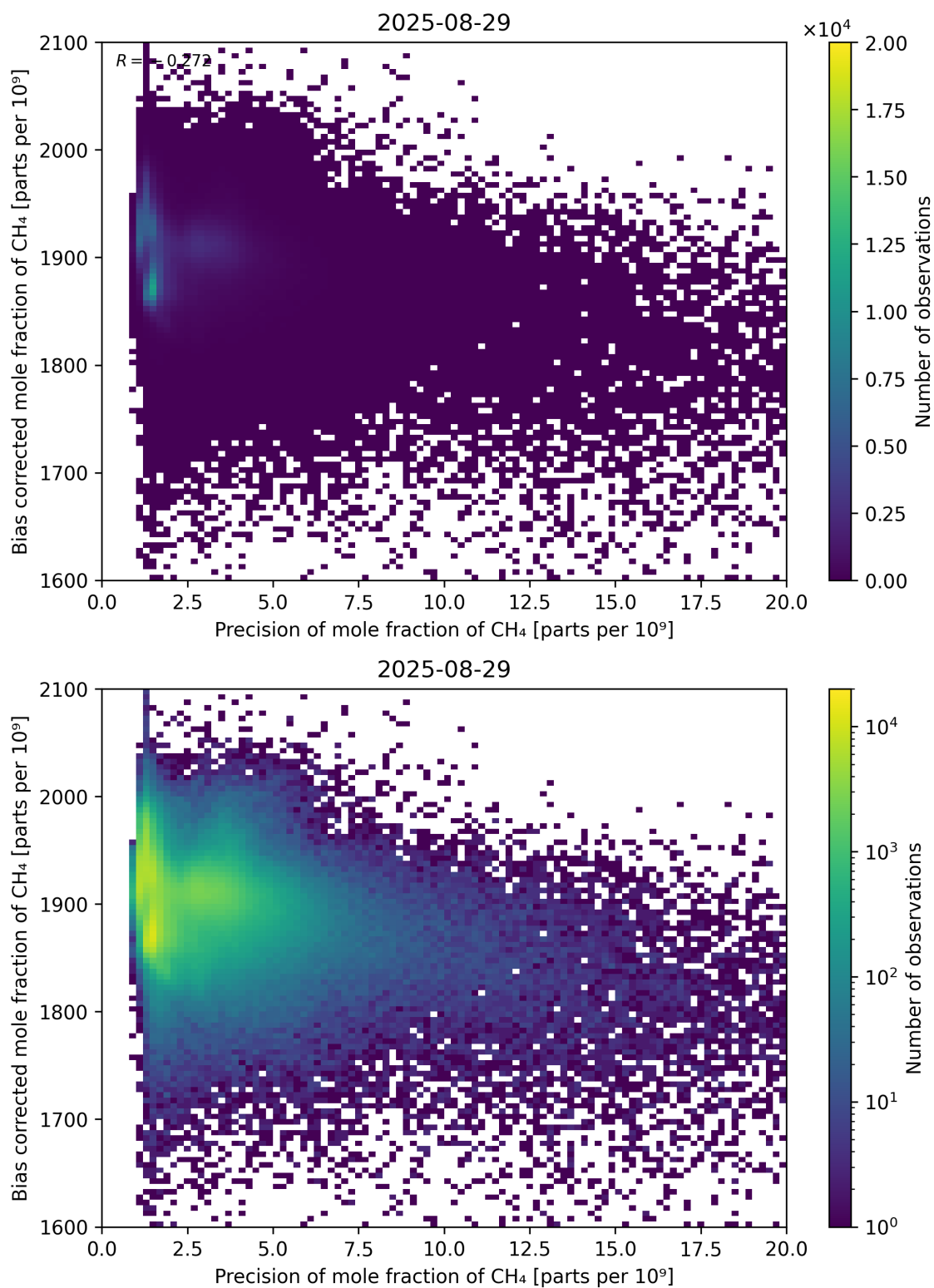
Figure 82: Scatter density plot of “Precision of mole fraction of CH 4 ” against “Bias corrected mole fraction of CH 4 ” for 2025-08-28 to 2025-08-30.
