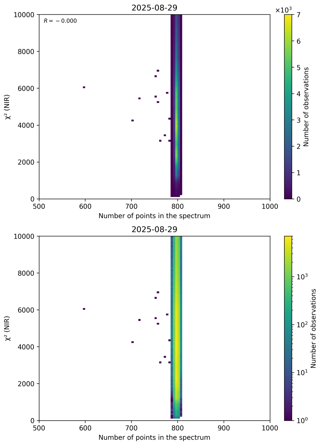
Figure 88: Scatter density plot of “Number of points in the spectrum” against “ \chi^2 (NIR)” for 2025-08-28 to 2025-08-30.
