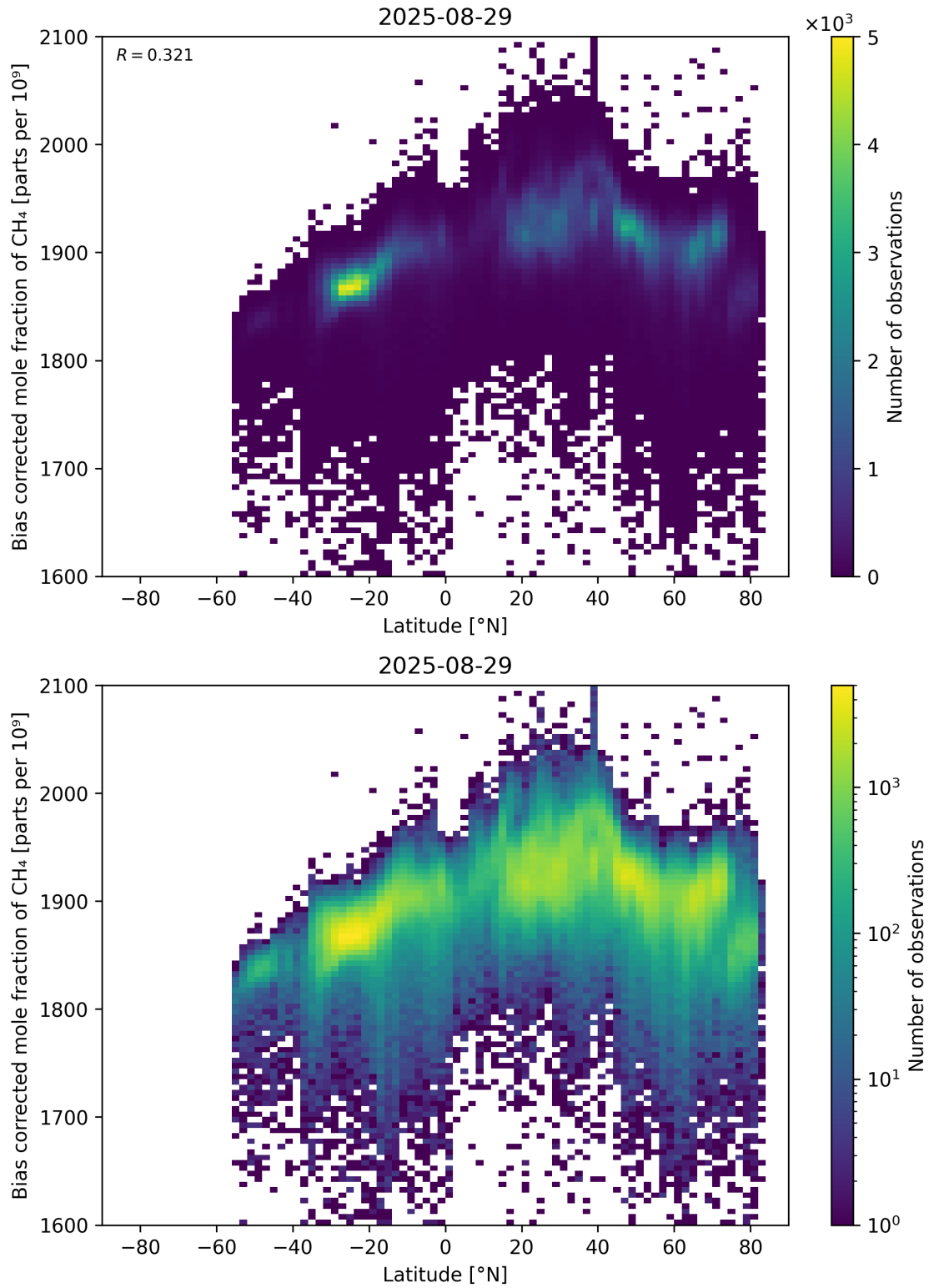
Figure 58: Scatter density plot of “Latitude” against “Bias corrected mole fraction of \text{CH}_4 ” for 2025-08-28 to 2025-08-30.
