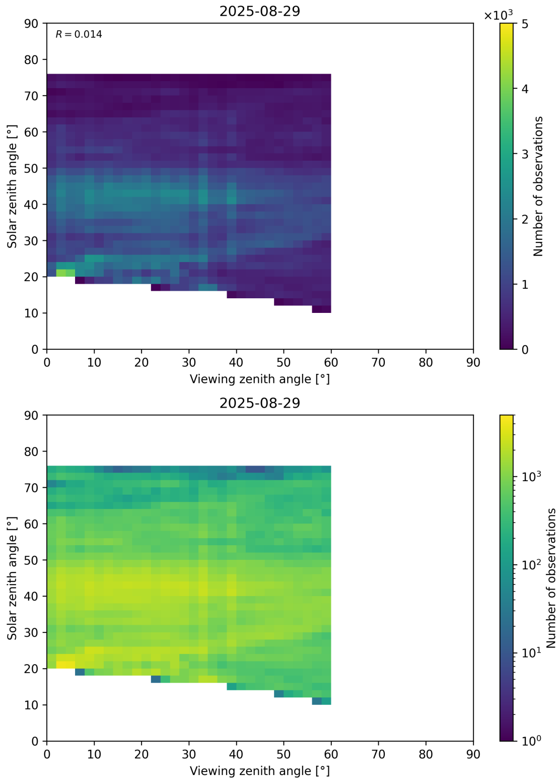
Figure 115: Scatter density plot of “Viewing zenith angle” against “Solar zenith angle” for 2025-08-28 to 2025-08-30.
