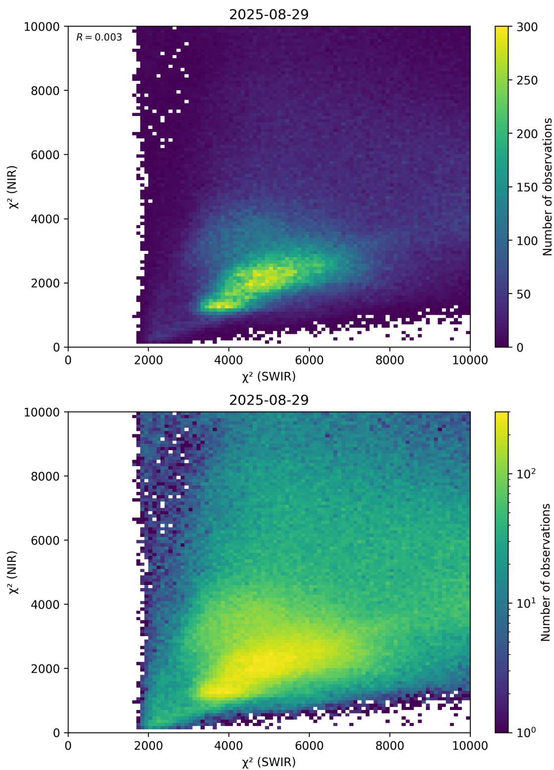
Figure 47: Scatter density plot of “ \chi^2 (SWIR)” against “ \chi^2 (NIR)” for 2025-08-28 to 2025-08-30.
