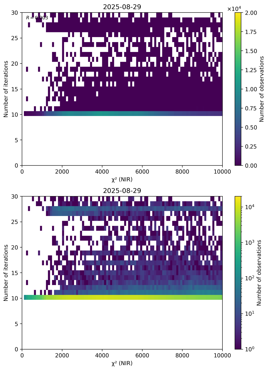
Figure 46: Scatter density plot of “ \chi^2 (NIR)” against “Number of iterations” for 2025-08-28 to 2025-08-30.
