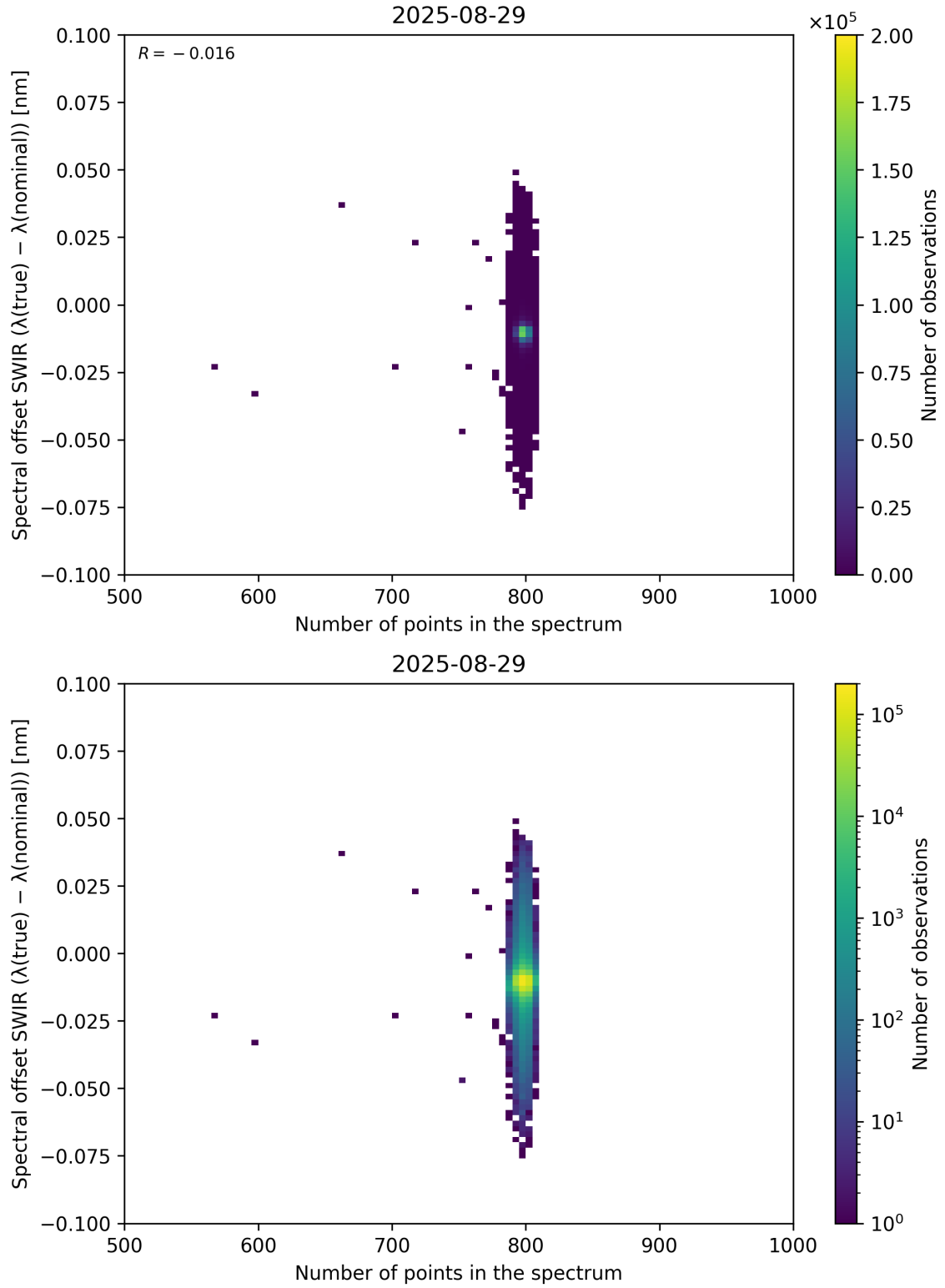
Figure 93: Scatter density plot of “Number of points in the spectrum” against “Spectral offset SWIR ( \lambda_{\text{true}} - \lambda_{\text{nominal}} )” for 2025-08-28 to 2025-08-30.
