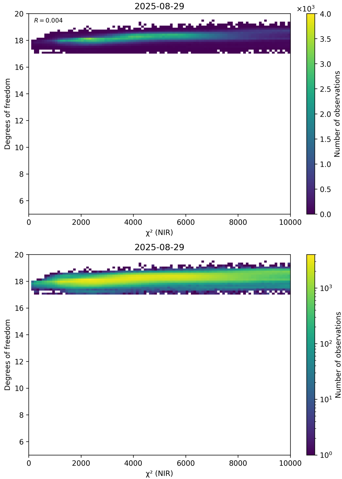
Figure 44: Scatter density plot of “ \chi^2 (NIR)” against “Degrees of freedom” for 2025-08-28 to 2025-08-30.
