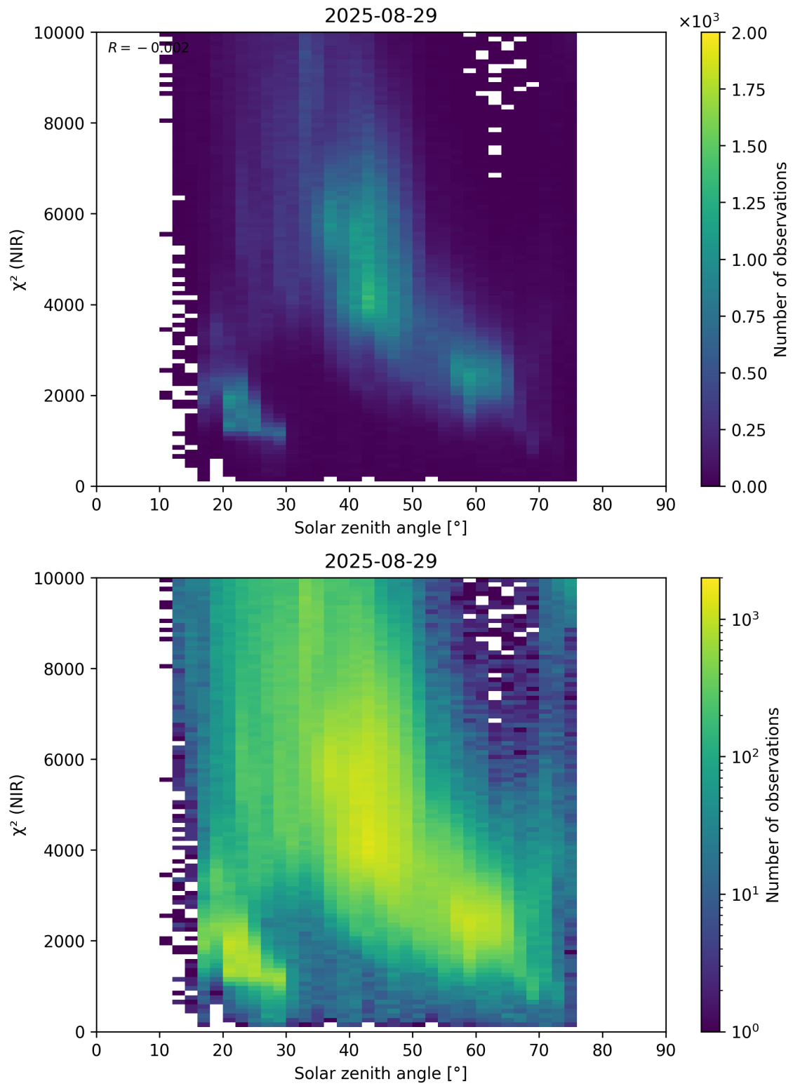
Figure 94: Scatter density plot of “Solar zenith angle” against “ \chi^2 (NIR)” for 2025-08-28 to 2025-08-30.
