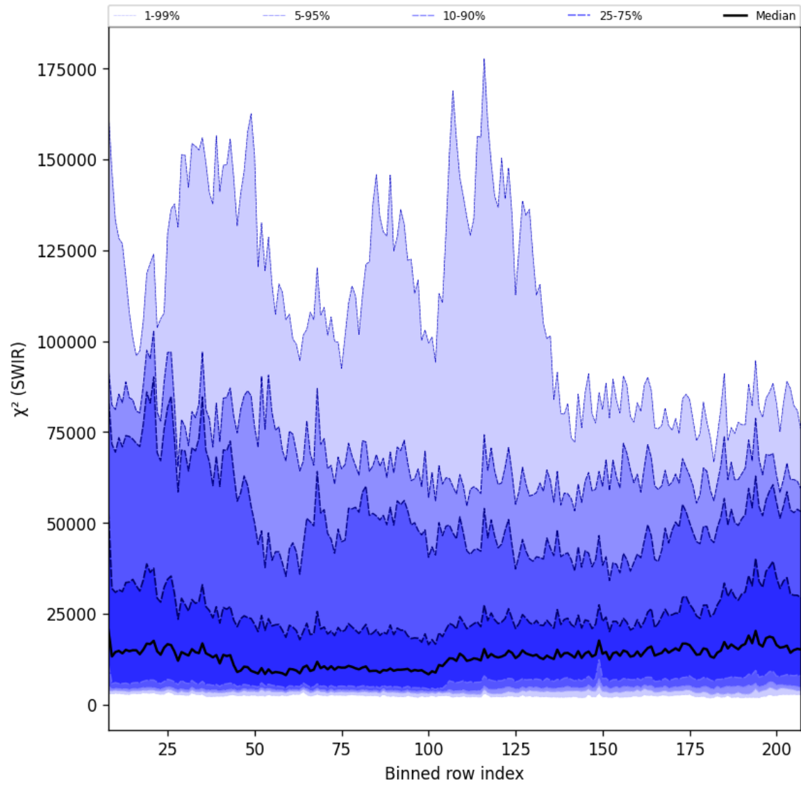
Figure 39: Along track statistics of “ \chi^2 (SWIR)” for 2025-08-28 to 2025-08-30
