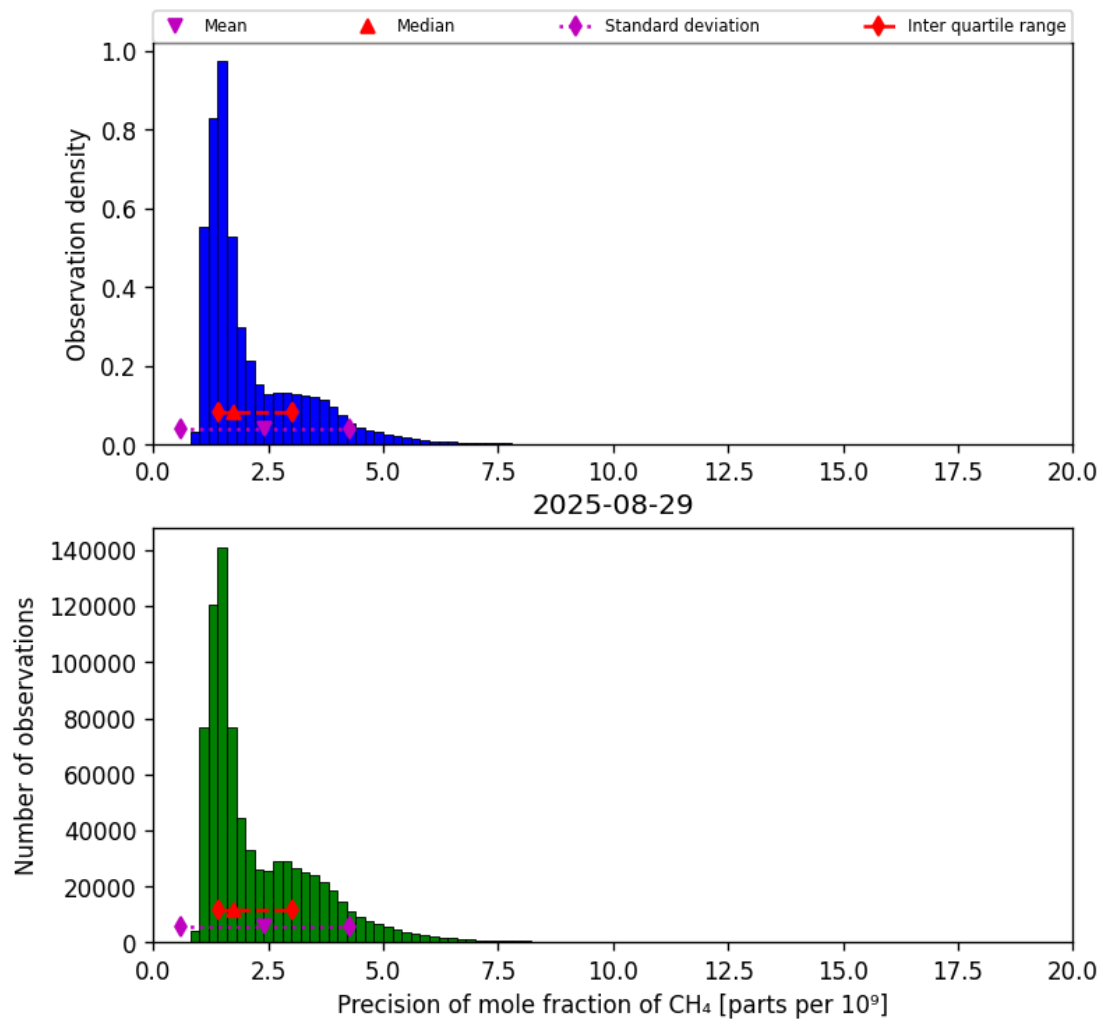
Figure 24: Histogram of “Precision of mole fraction of CH 4 ” for 2025-08-28 to 2025-08-30
