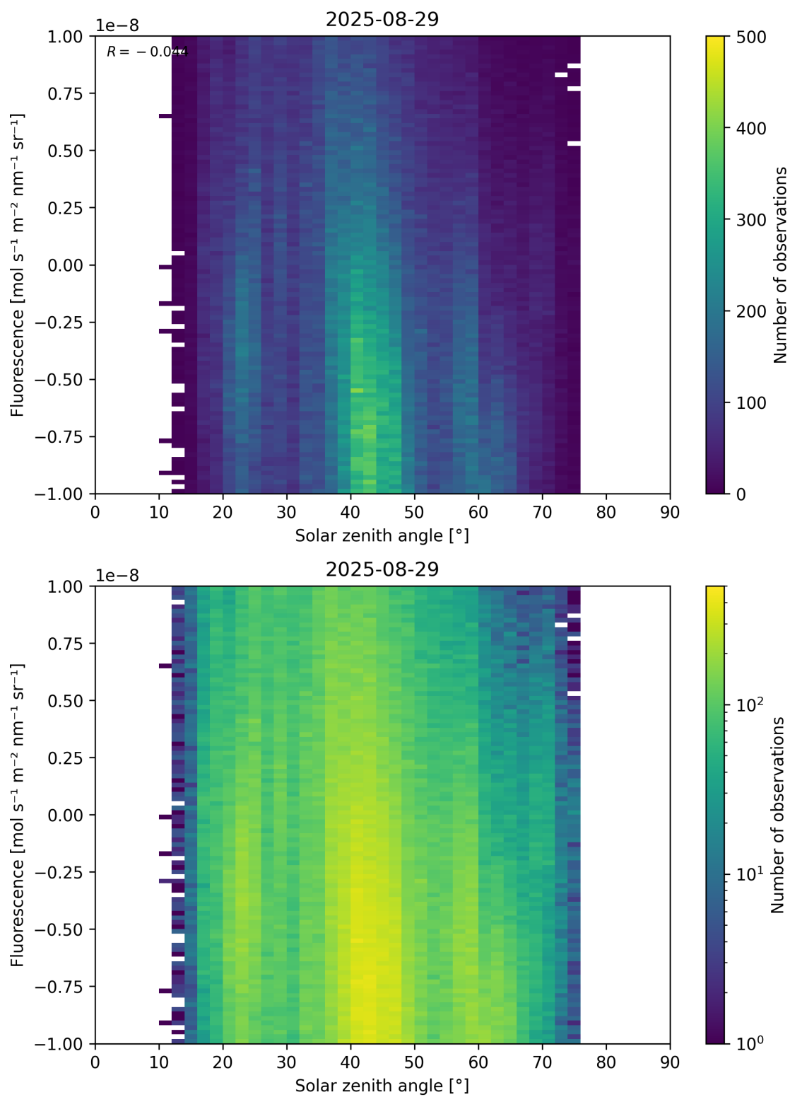
Figure 97: Scatter density plot of “Solar zenith angle” against “Fluorescence” for 2025-08-28 to 2025-08-30.
