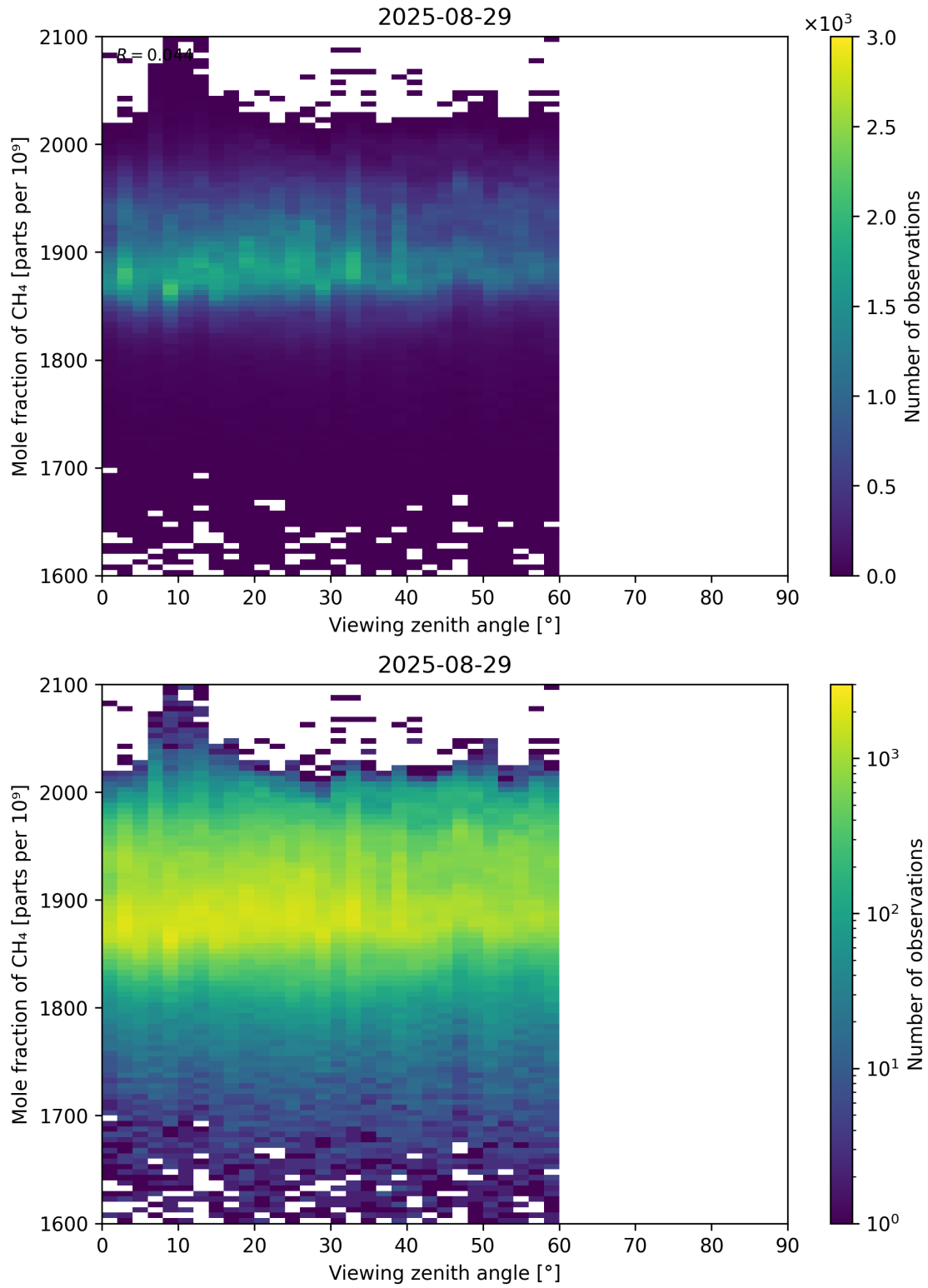
Figure 110: Scatter density plot of “Viewing zenith angle” against “Mole fraction of CH 4 ” for 2025-08-28 to 2025-08-30.
