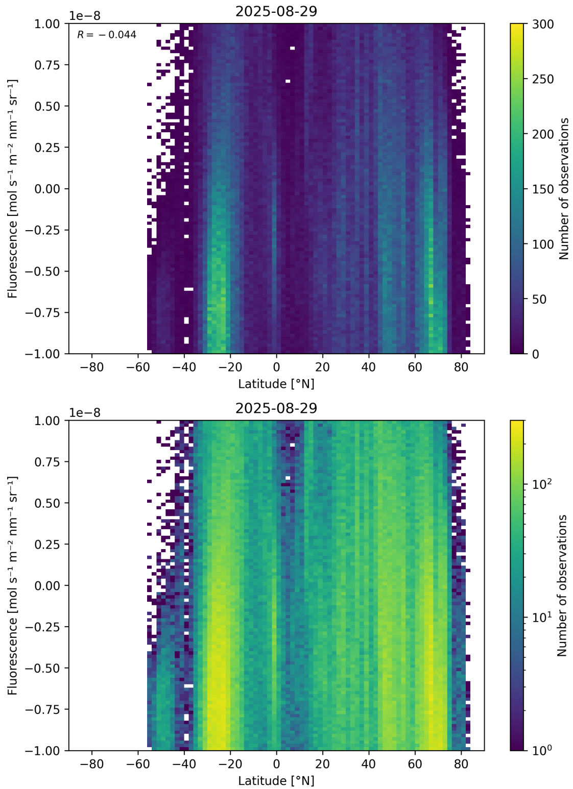
Figure 56: Scatter density plot of “Latitude” against “Fluorescence” for 2025-08-28 to 2025-08-30.
