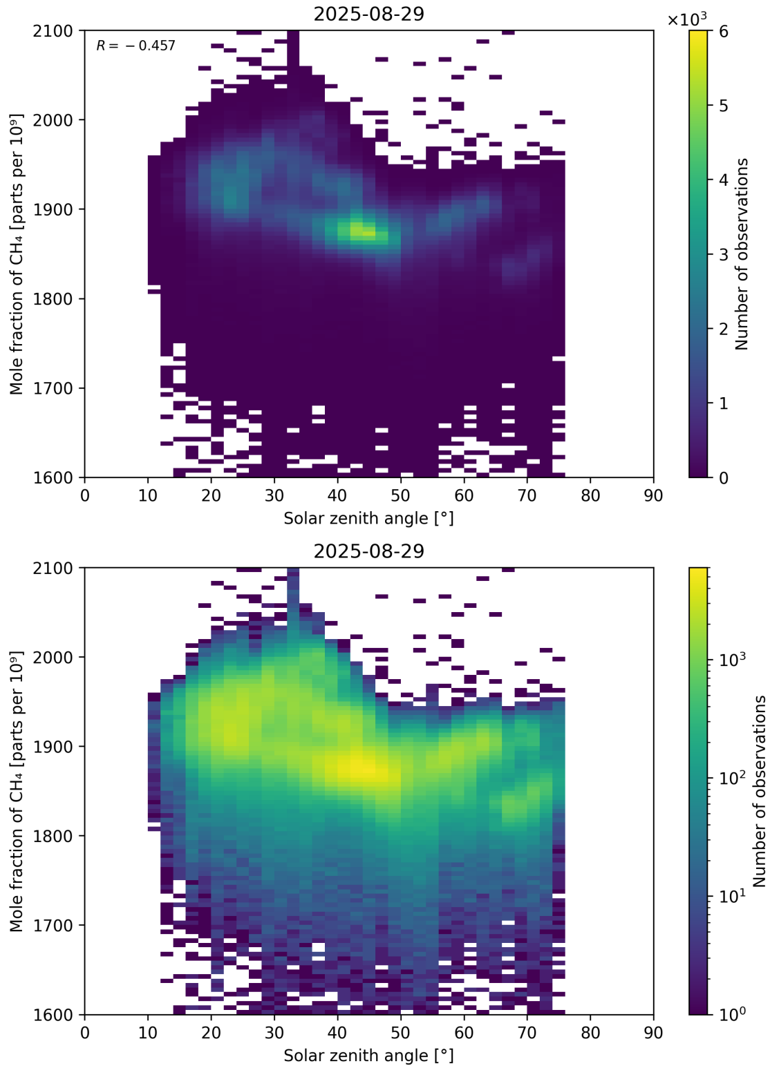
Figure 99: Scatter density plot of “Solar zenith angle” against “Mole fraction of \text{CH}_4 ” for 2025-08-28 to 2025-08-30.
