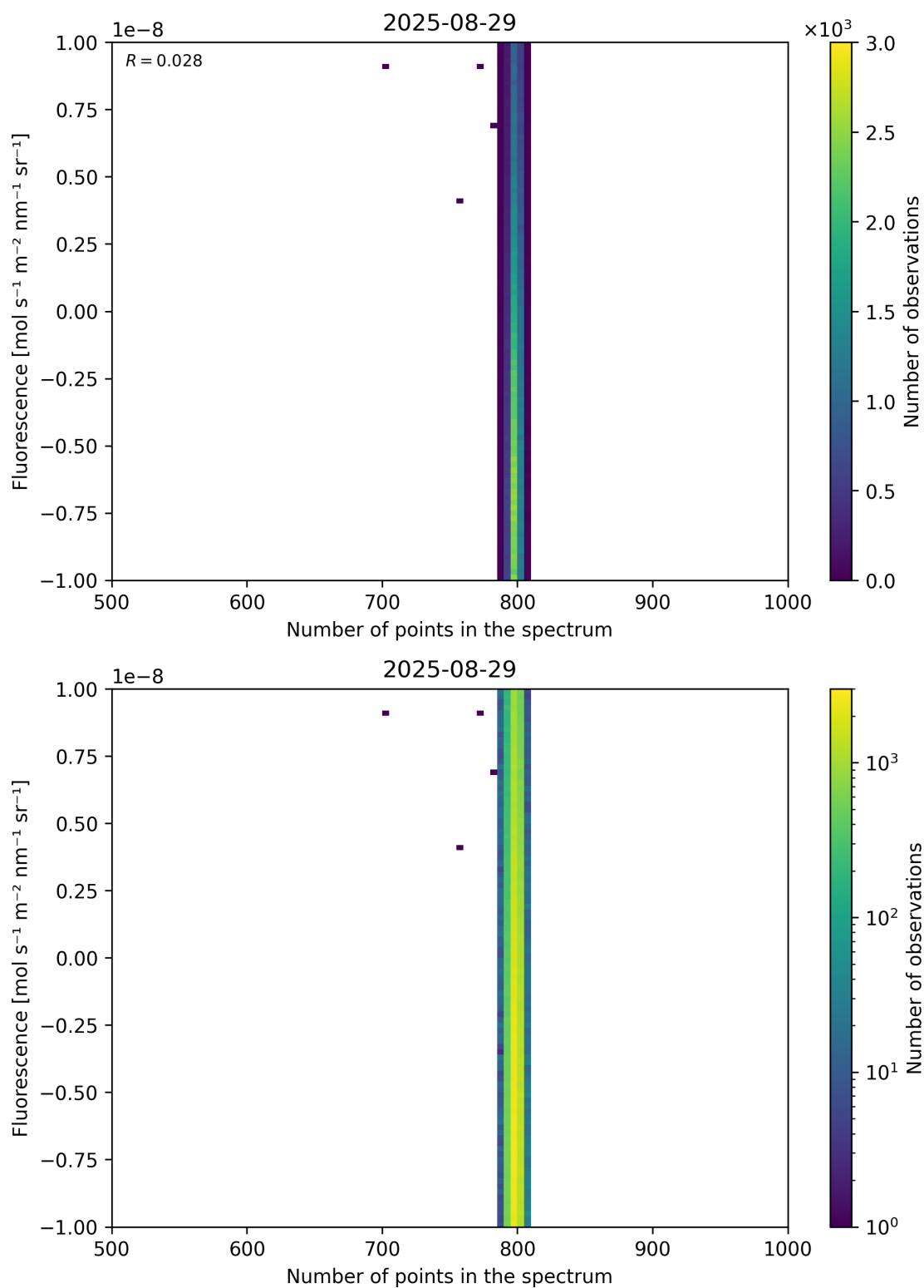
Figure 91: Scatter density plot of “Number of points in the spectrum” against “Fluorescence” for 2025-08-28 to 2025-08-30.
