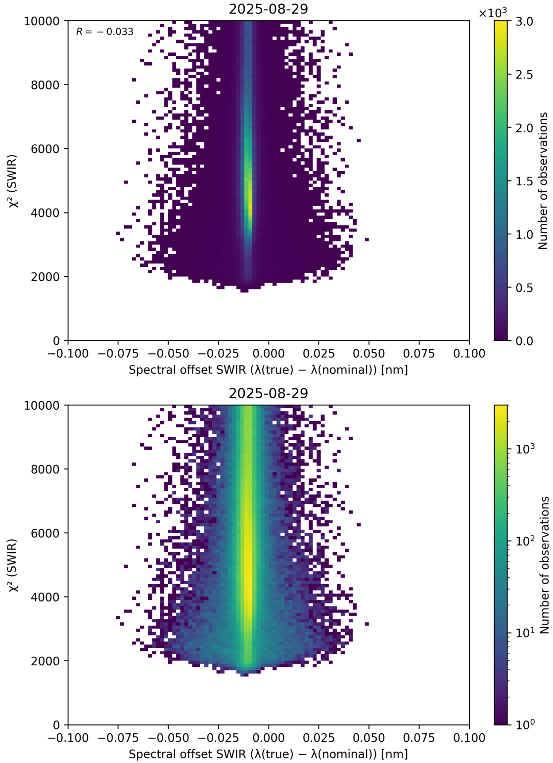
Figure 118: Scatter density plot of “Spectral offset SWIR ( \lambda_{\text{true}} - \lambda_{\text{nominal}} )” against “ \chi^2 (SWIR)” for 2025-08-28 to 2025-08-30.
