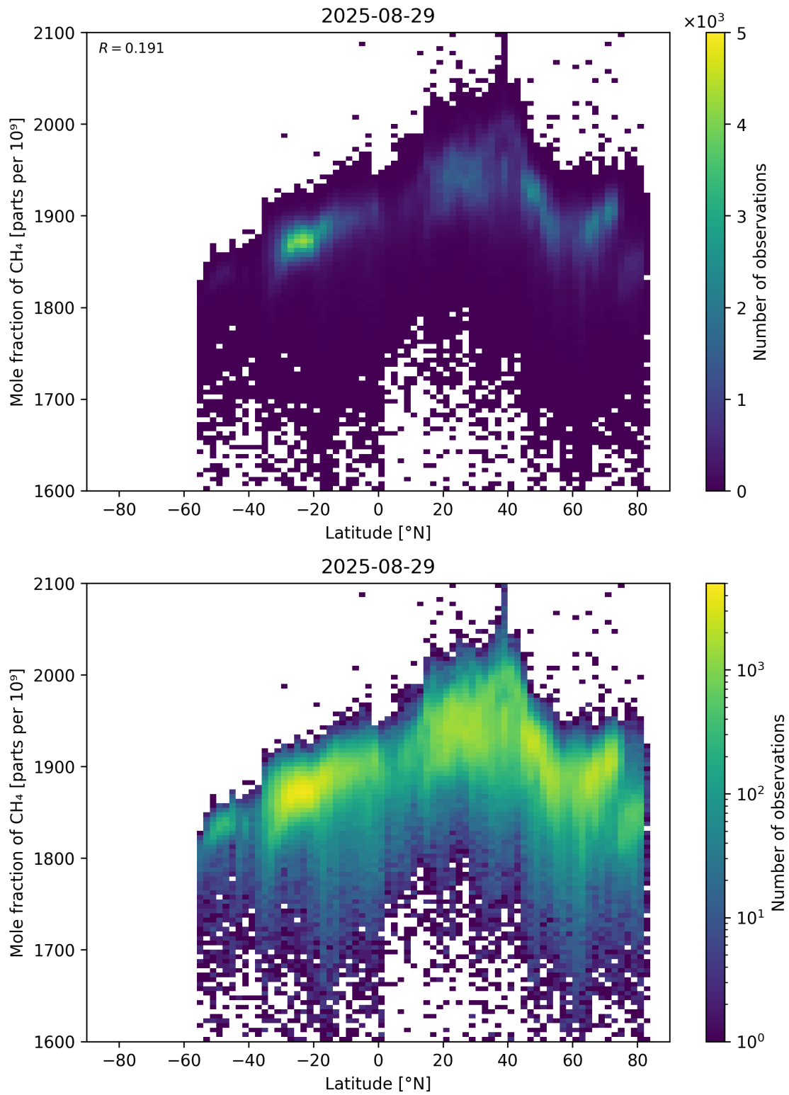
Figure 57: Scatter density plot of “Latitude” against “Mole fraction of CH 4 ” for 2025-08-28 to 2025-08-30.
