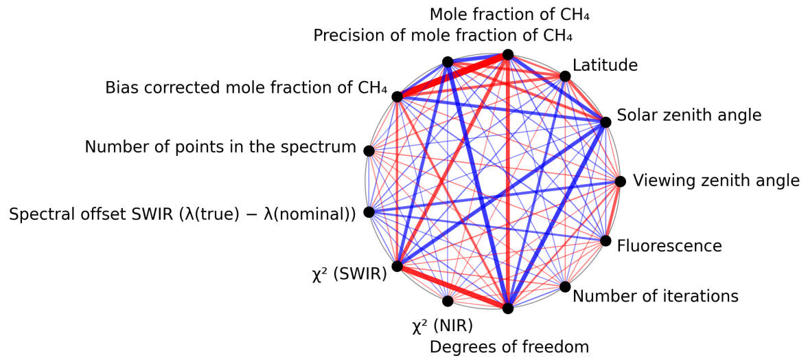
Figure 1: Map of correlation graph for 2025-08-28 to 2025-08-30.
