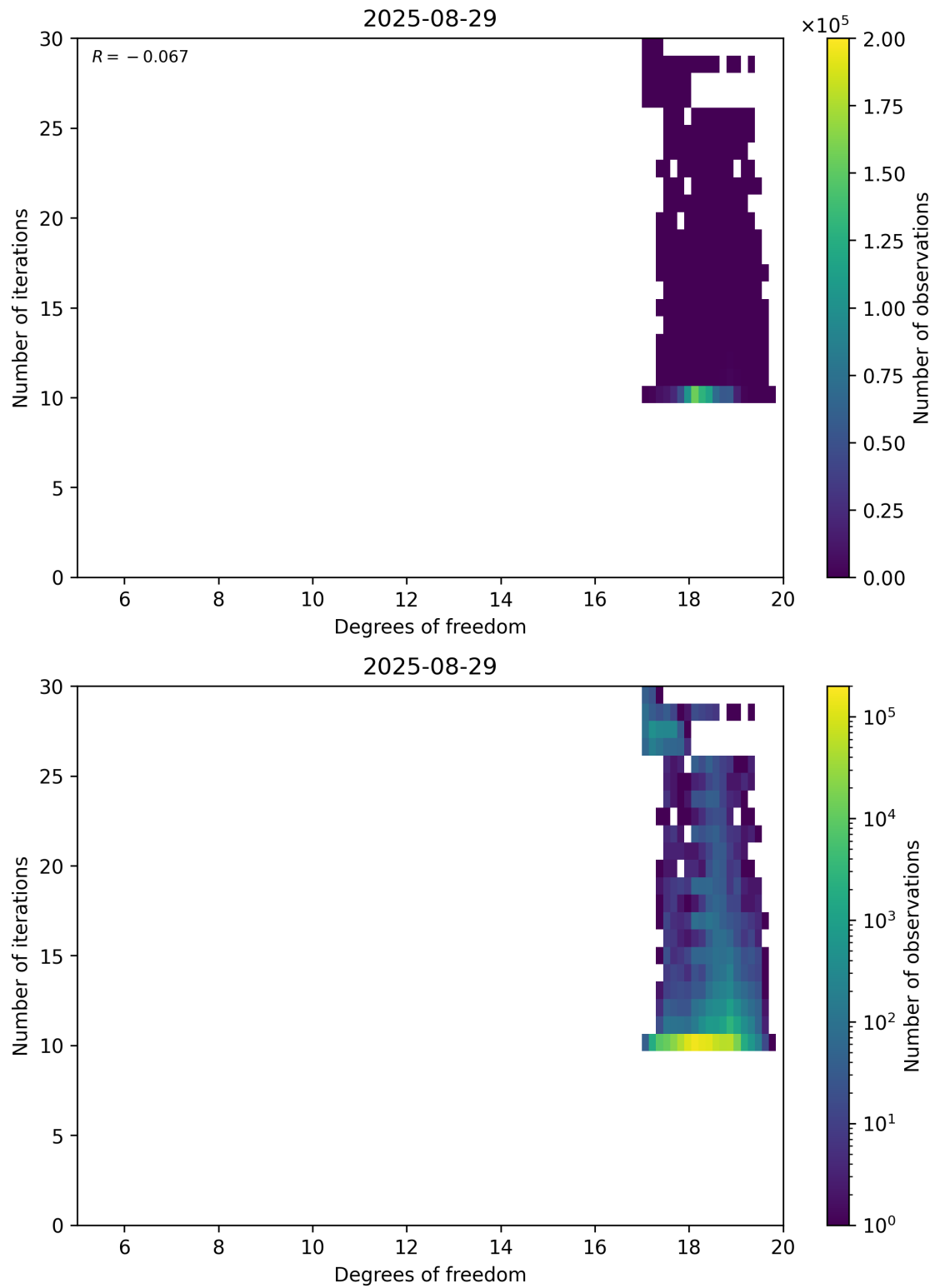
Figure 52: Scatter density plot of “Degrees of freedom” against “Number of iterations” for 2025-08-28 to 2025-08-30.
