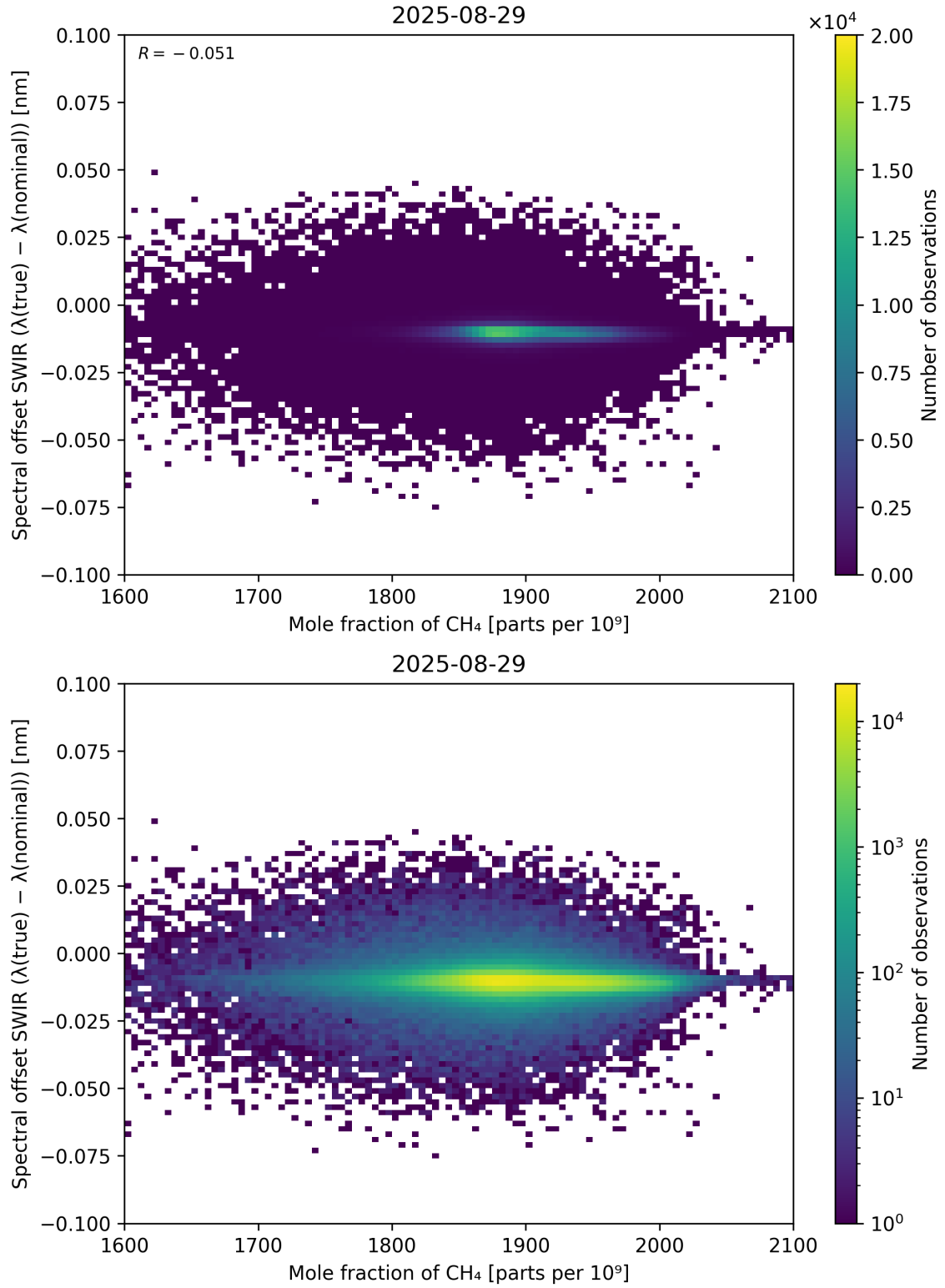
Figure 86: Scatter density plot of “Mole fraction of \text{CH}_4 ” against “Spectral offset SWIR ( \lambda_{\text{true}} - \lambda_{\text{nominal}} )” for 2025-08-28 to 2025-08-30.
