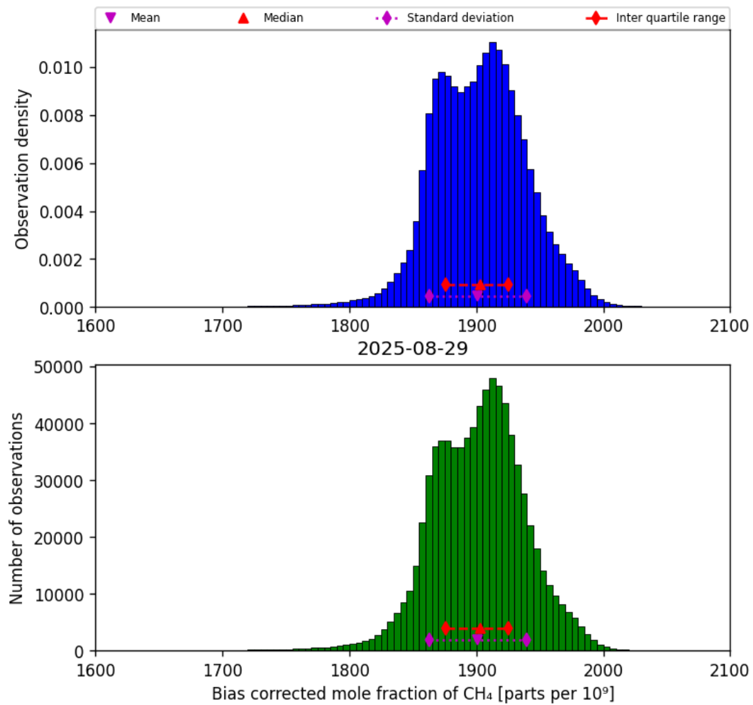
Figure 25: Histogram of “Bias corrected mole fraction of CH 4 ” for 2025-08-28 to 2025-08-30
