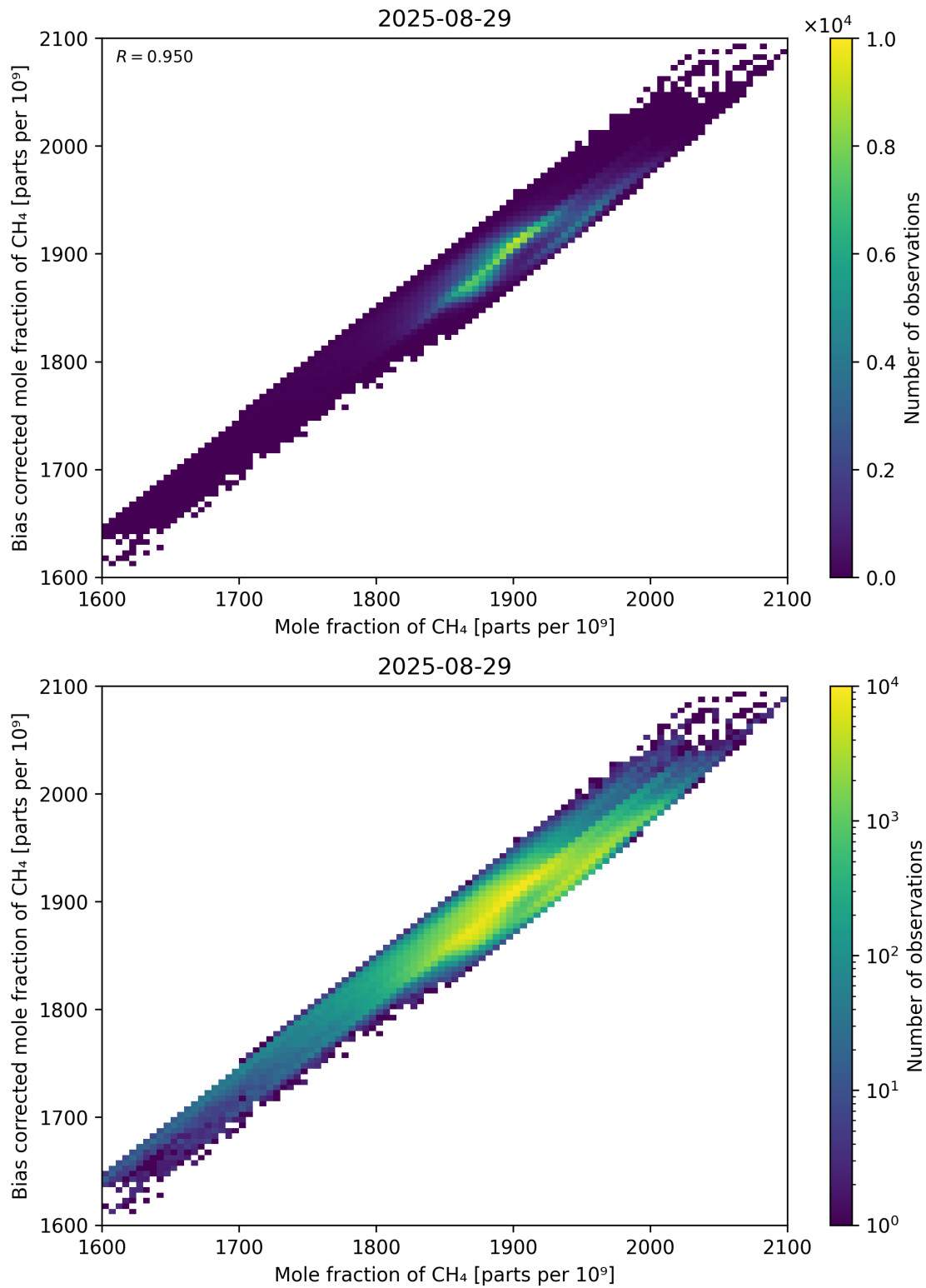
Figure 74: Scatter density plot of “Mole fraction of \text{CH}_4 ” against “Bias corrected mole fraction of \text{CH}_4 ” for 2025-08-28 to 2025-08-30.
