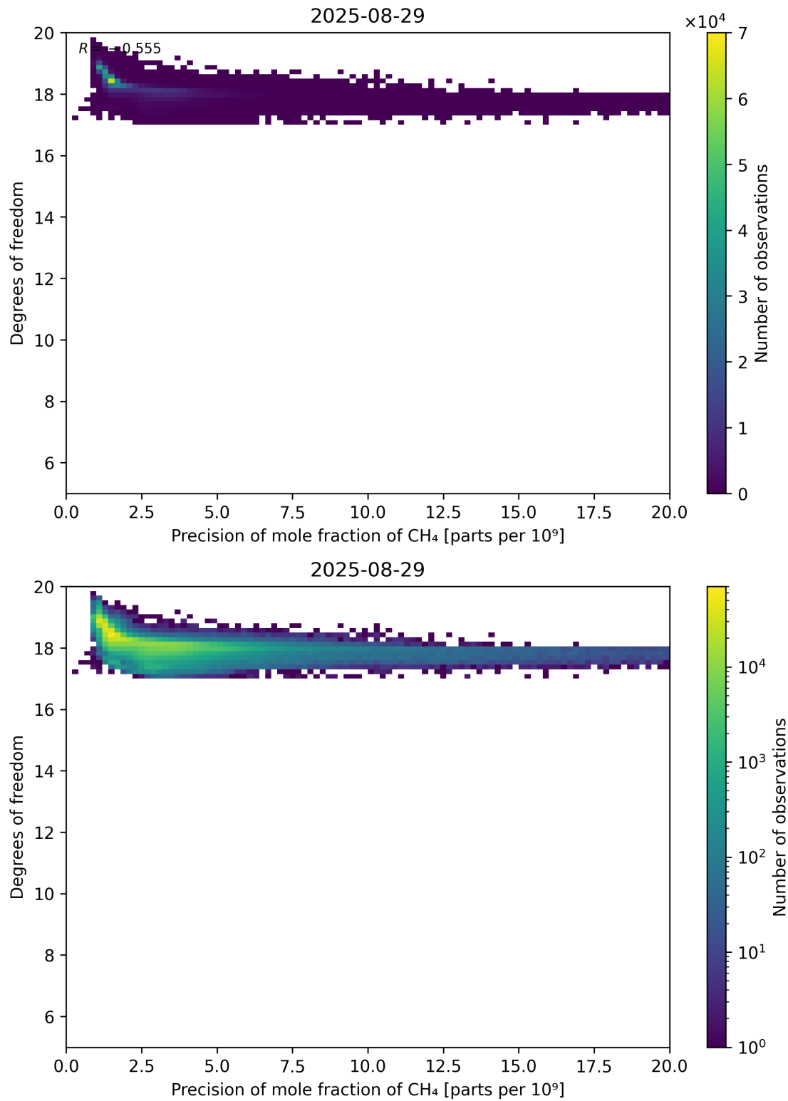
Figure 80: Scatter density plot of “Precision of mole fraction of CH 4 ” against “Degrees of freedom” for 2025-08-28 to 2025-08-30.
