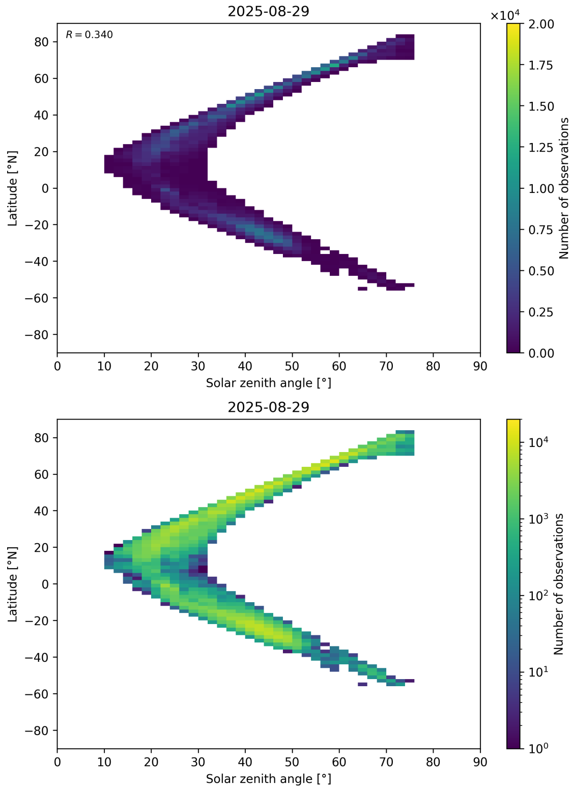
Figure 98: Scatter density plot of “Solar zenith angle” against “Latitude” for 2025-08-28 to 2025-08-30.
