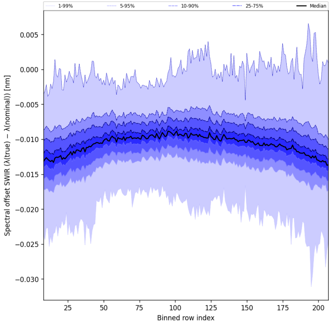
Figure 38: Along track statistics of “Spectral offset SWIR ( \lambda_{\text{true}} - \lambda_{\text{nominal}} )” for 2025-08-28 to 2025-08-30
