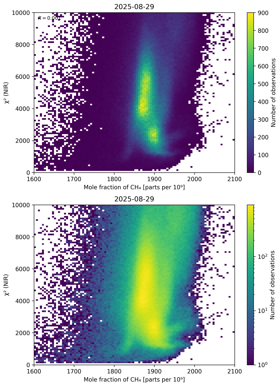
Figure 70: Scatter density plot of “Mole fraction of \text{CH}_4 ” against “ \chi^2 (NIR)” for 2025-08-28 to 2025-08-30.
