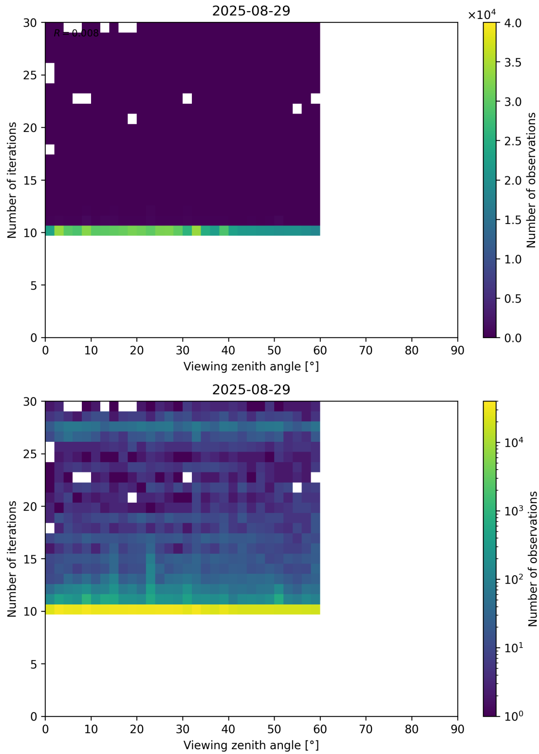
Figure 113: Scatter density plot of “Viewing zenith angle” against “Number of iterations” for 2025-08-28 to 2025-08-30.
