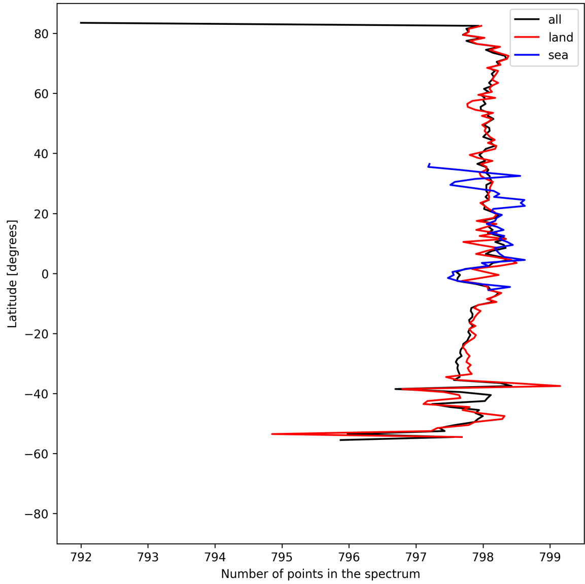
Figure 15: Zonal average of “Number of points in the spectrum” for 2025-08-28 to 2025-08-30.
