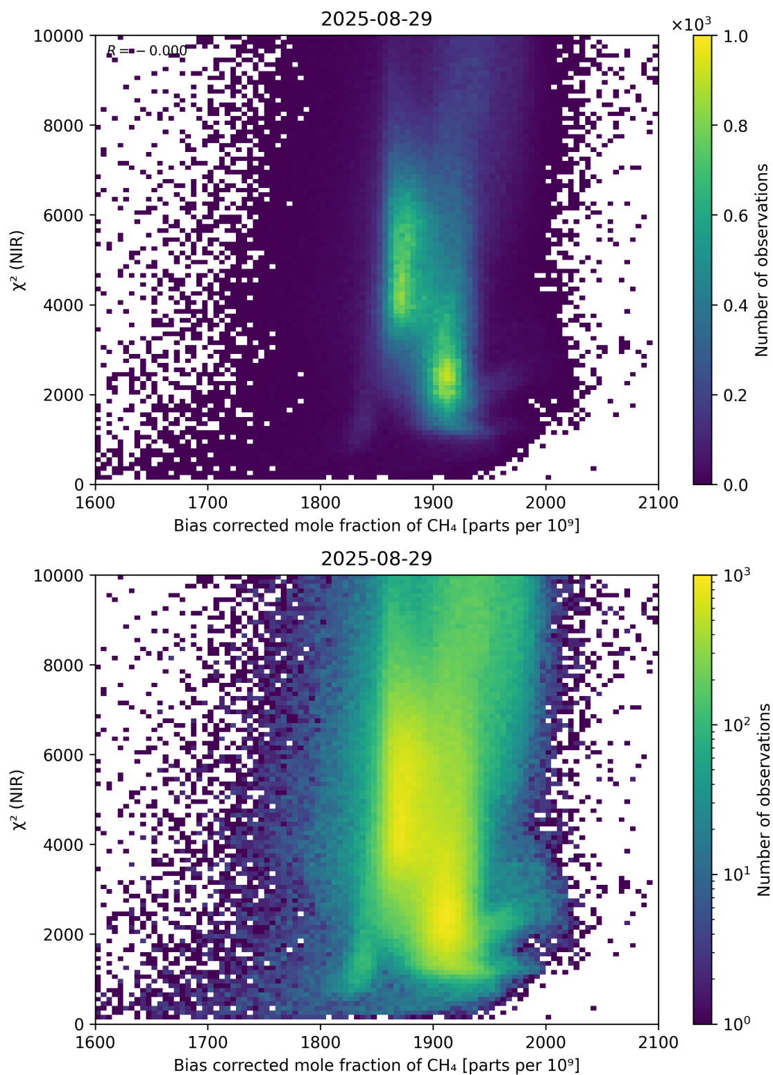
Figure 63: Scatter density plot of “Bias corrected mole fraction of CH 4 ” against “ \chi^2 (NIR)” for 2025-08-28 to 2025-08-30.
