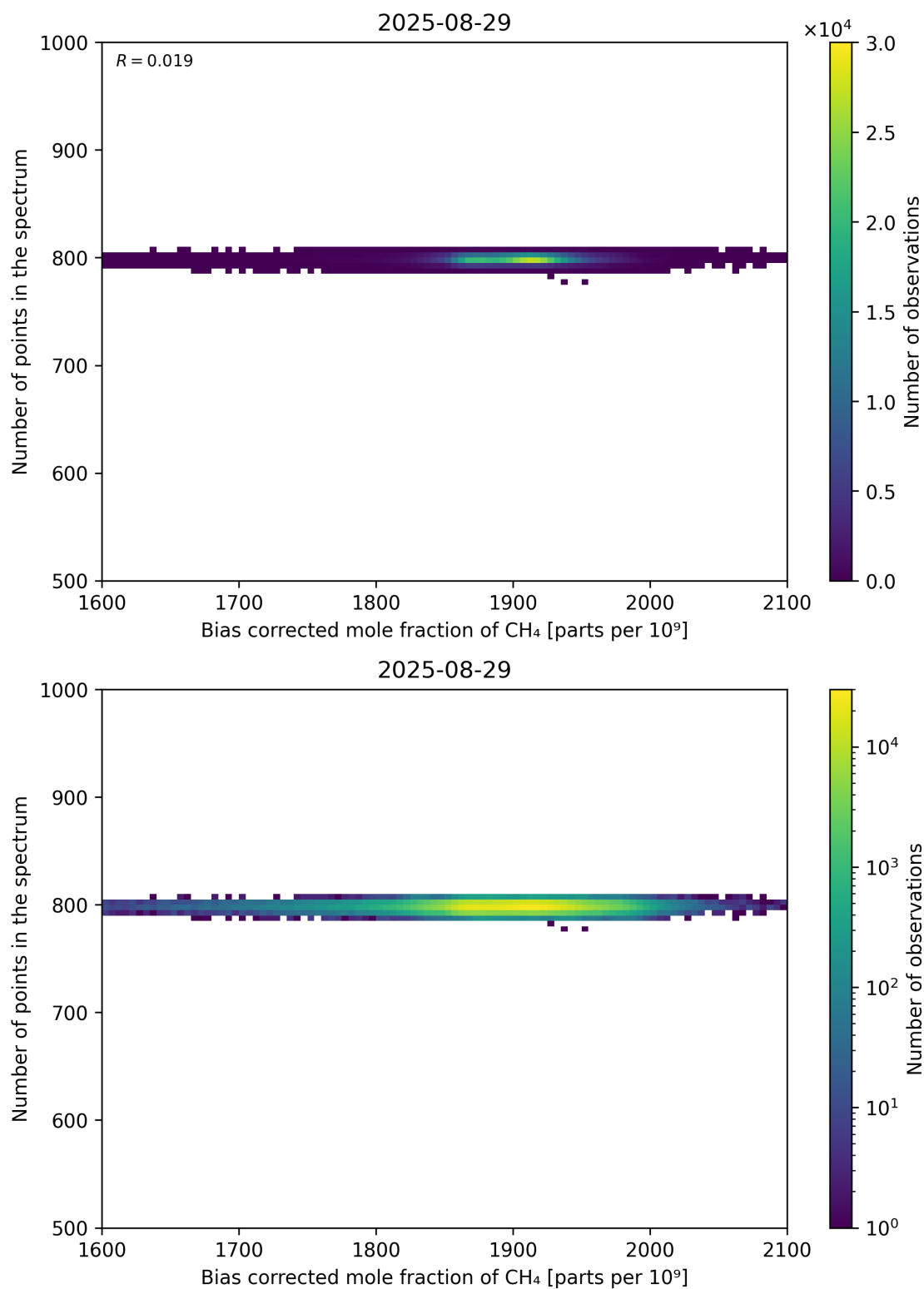
Figure 68: Scatter density plot of “Bias corrected mole fraction of CH 4 ” against “Number of points in the spectrum” for 2025-08-28 to 2025-08-30.
