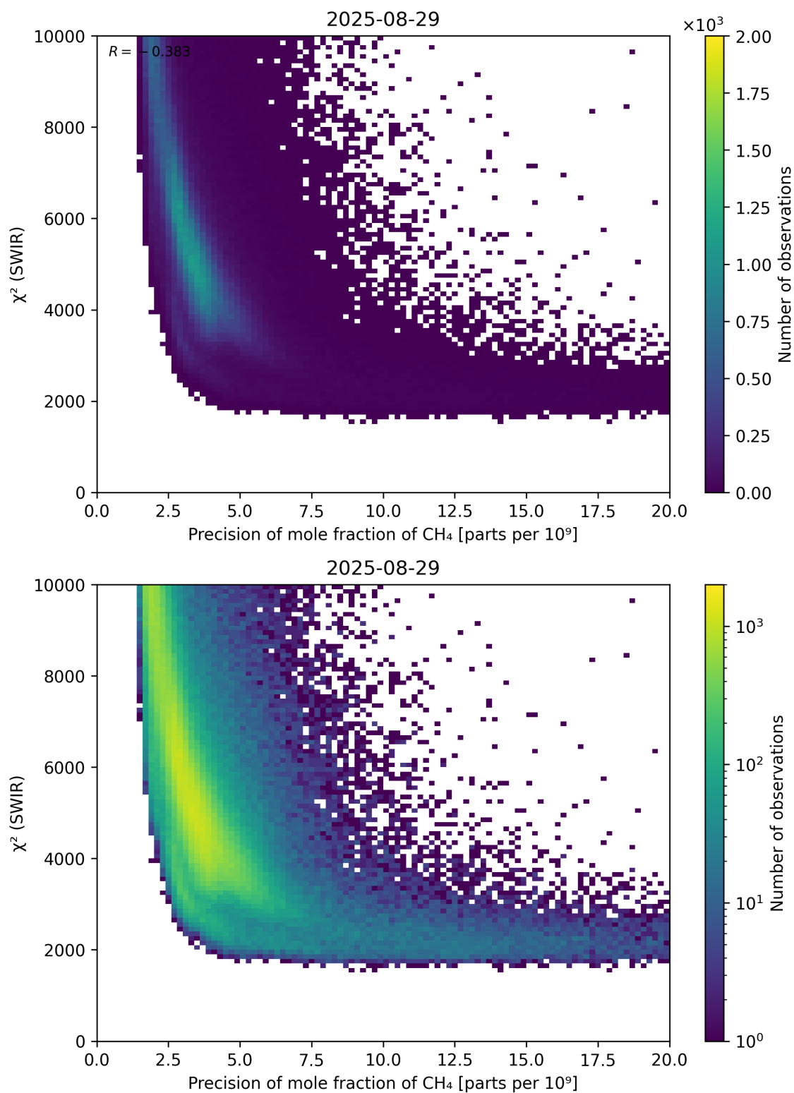
Figure 79: Scatter density plot of “Precision of mole fraction of \text{CH}_4 ” against “ \chi^2 (SWIR)” for 2025-08-28 to 2025-08-30.
