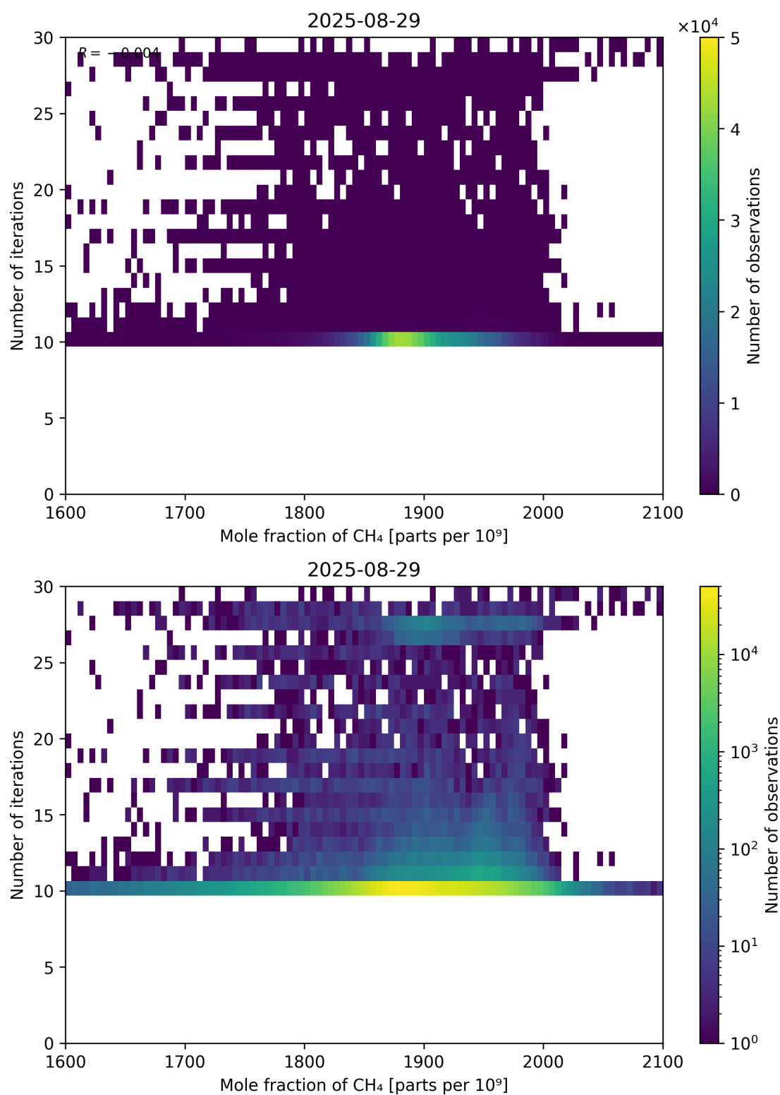
Figure 76: Scatter density plot of “Mole fraction of CH 4 ” against “Number of iterations” for 2025-08-28 to 2025-08-30.
