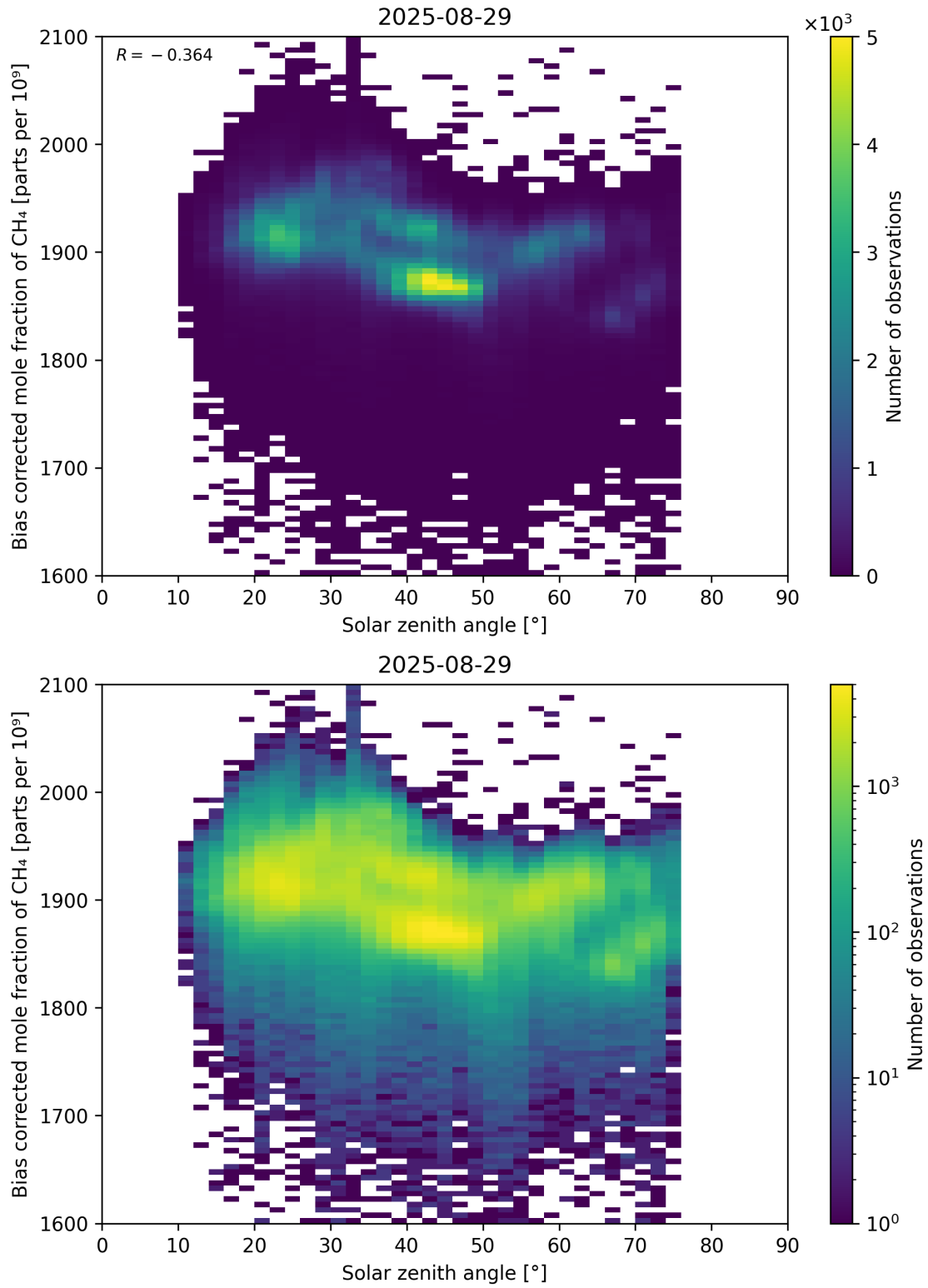
Figure 100: Scatter density plot of “Solar zenith angle” against “Bias corrected mole fraction of CH 4 ” for 2025-08-28 to 2025-08-30.
