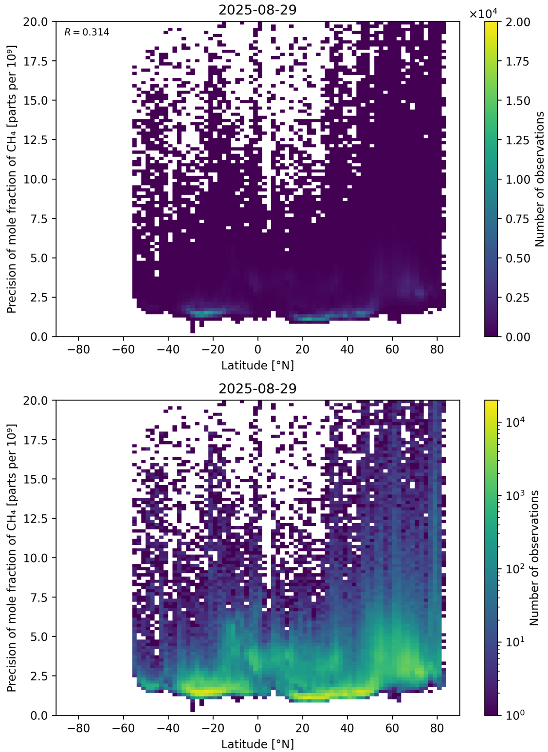
Figure 59: Scatter density plot of “Latitude” against “Precision of mole fraction of \text{CH}_4 ” for 2025-08-28 to 2025-08-30.
