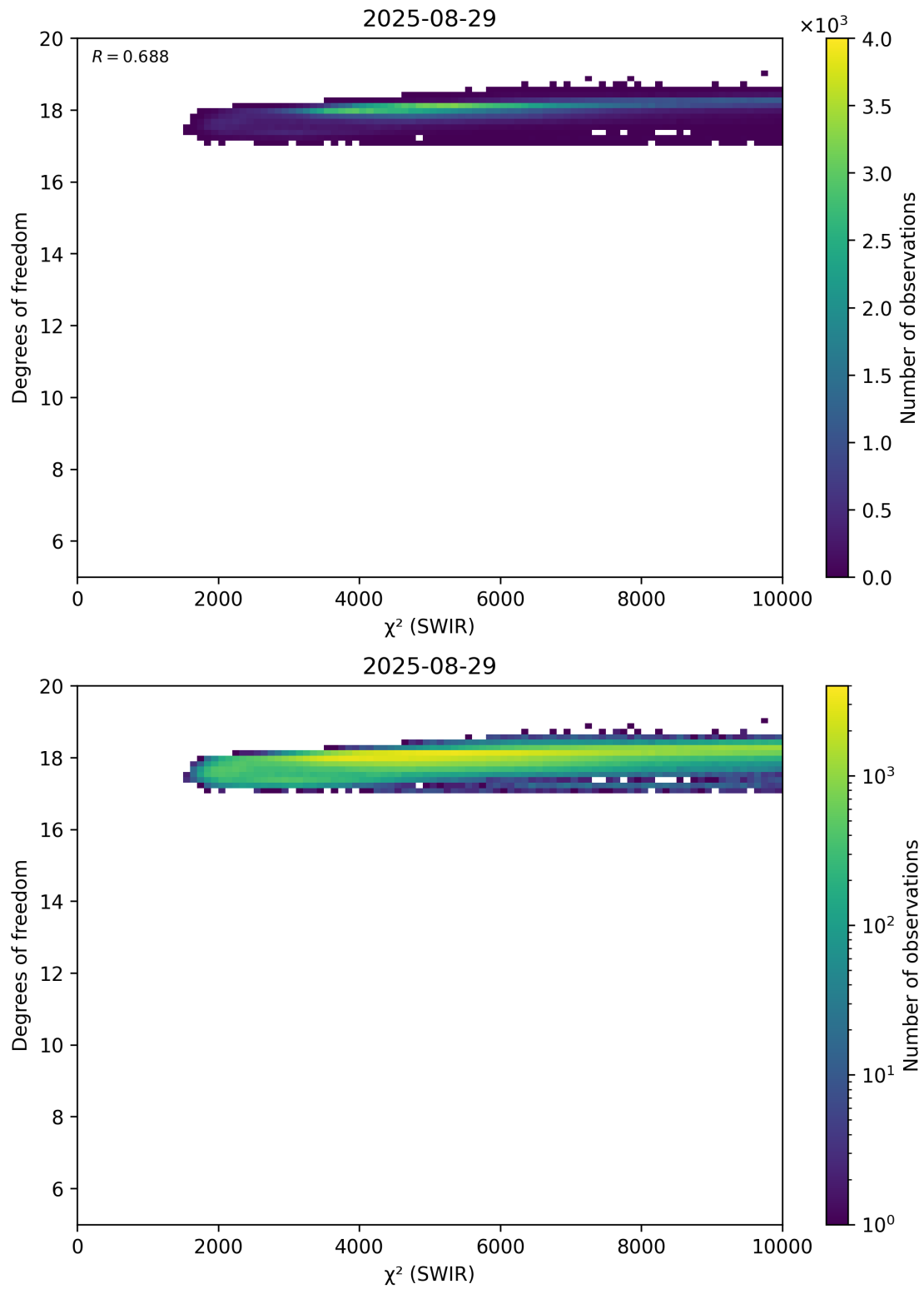
Figure 48: Scatter density plot of “ \chi^2 (SWIR)” against “Degrees of freedom” for 2025-08-28 to 2025-08-30.
