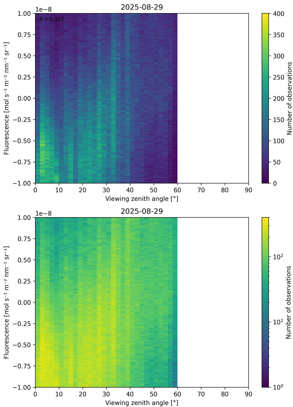
Figure 108: Scatter density plot of “Viewing zenith angle” against “Fluorescence” for 2025-08-28 to 2025-08-30.
