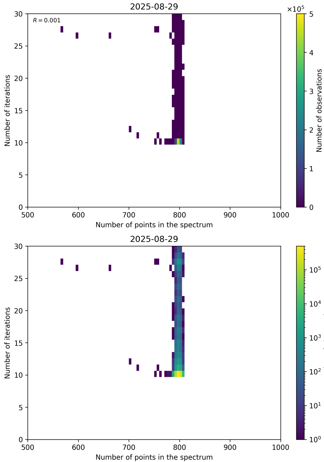
Figure 92: Scatter density plot of “Number of points in the spectrum” against “Number of iterations” for 2025-08-28 to 2025-08-30.
