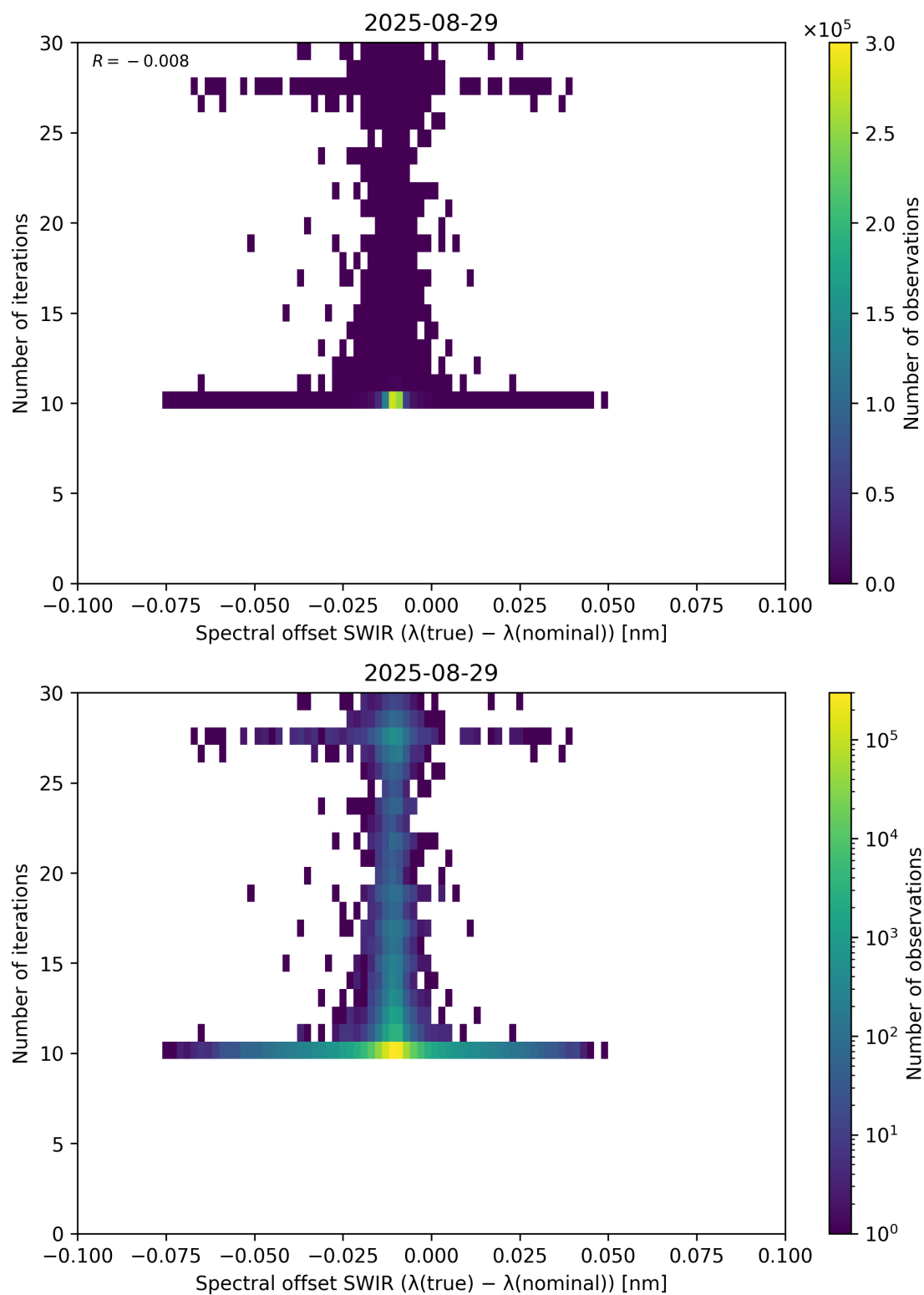
Figure 121: Scatter density plot of “Spectral offset SWIR ( \lambda_{\text{true}} - \lambda_{\text{nominal}} )” against “Number of iterations” for 2025-08-28 to 2025-08-30.
