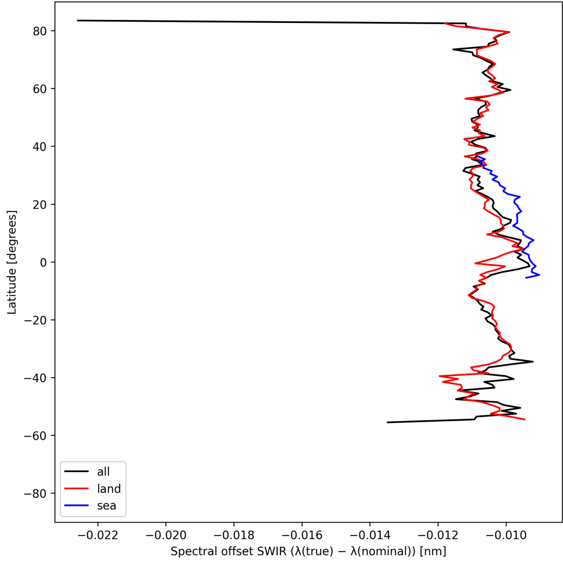
Figure 16: Zonal average of “Spectral offset SWIR ( \lambda_{\text{true}} - \lambda_{\text{nominal}} )” for 2025-08-28 to 2025-08-30.
