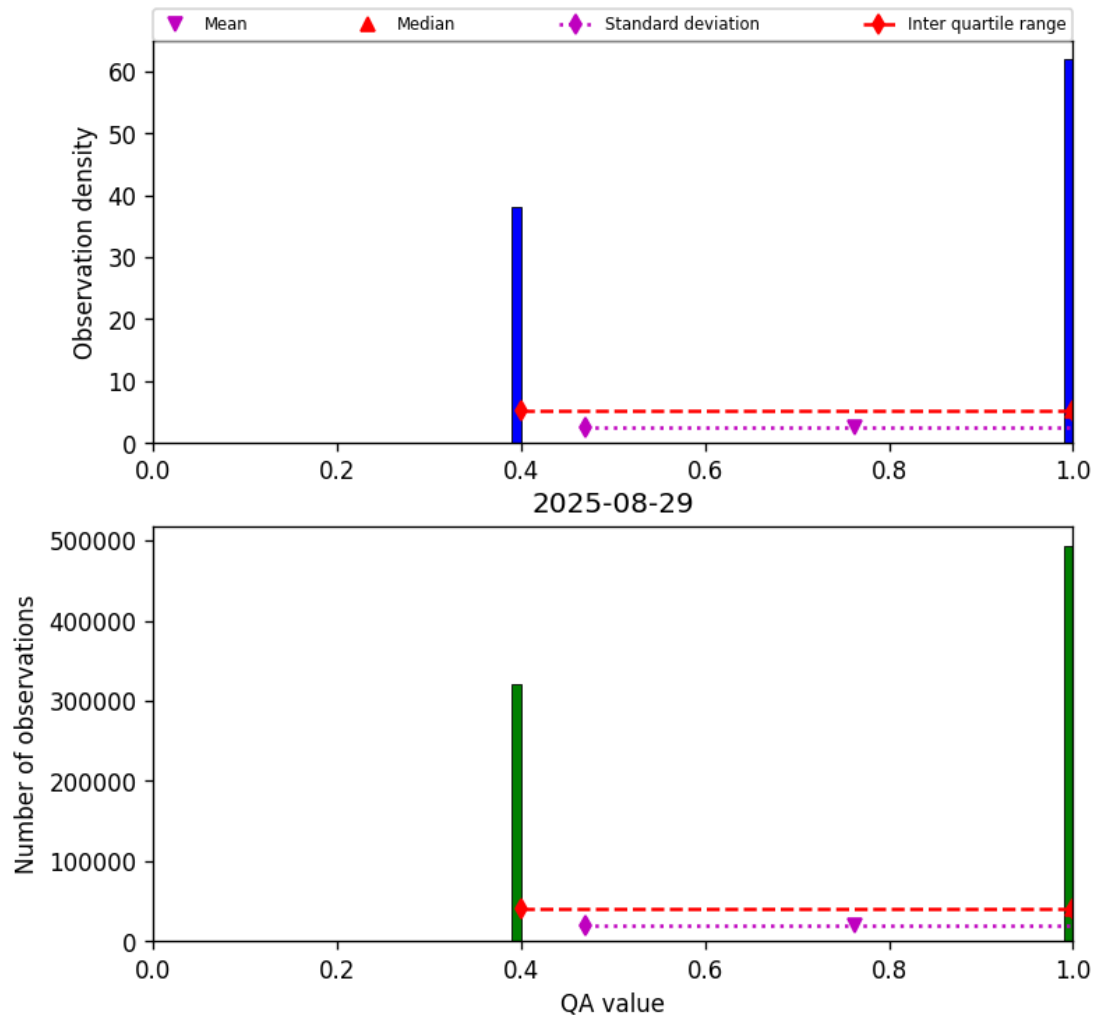
Figure 22: Histogram of “QA value” for 2025-08-28 to 2025-08-30
