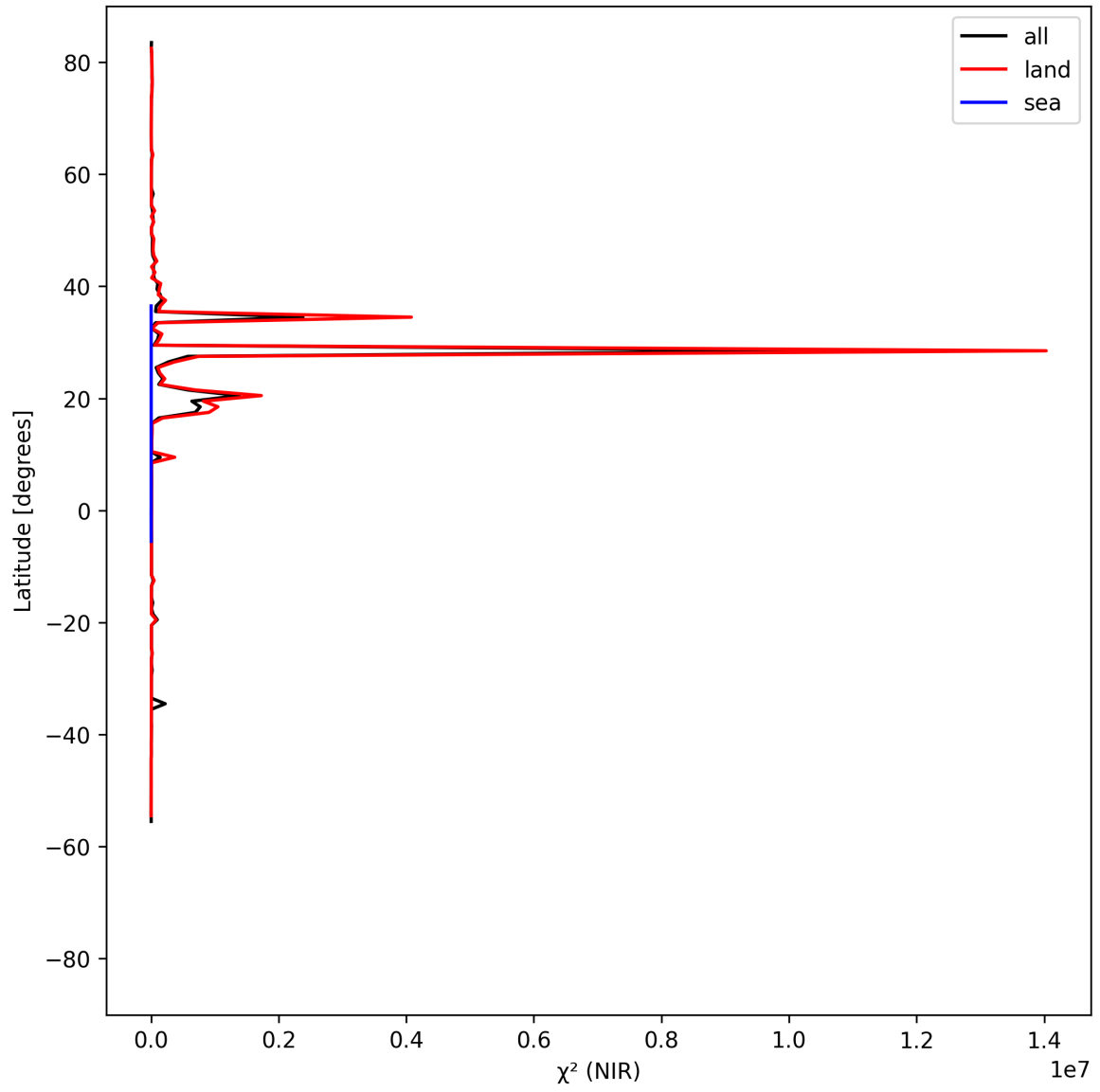
Figure 18: Zonal average of “ \chi^2 (NIR)” for 2025-08-28 to 2025-08-30.
