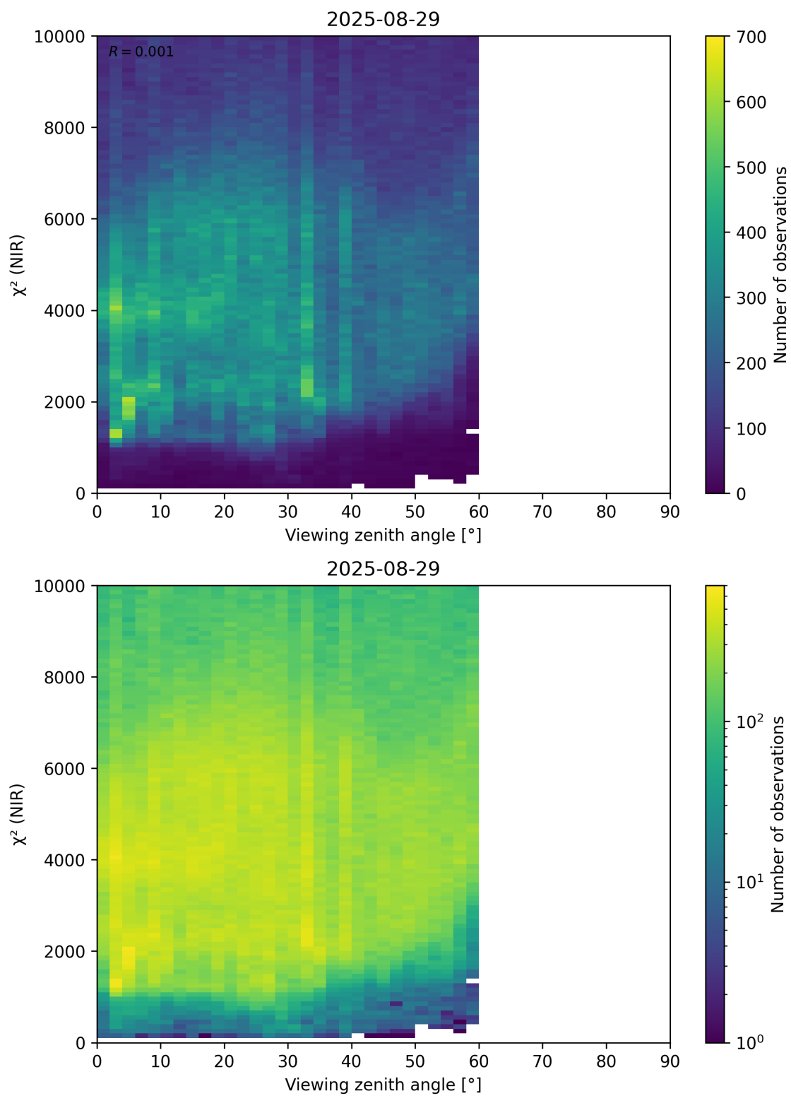
Figure 105: Scatter density plot of “Viewing zenith angle” against “ \chi^2 (NIR)” for 2025-08-28 to 2025-08-30.
