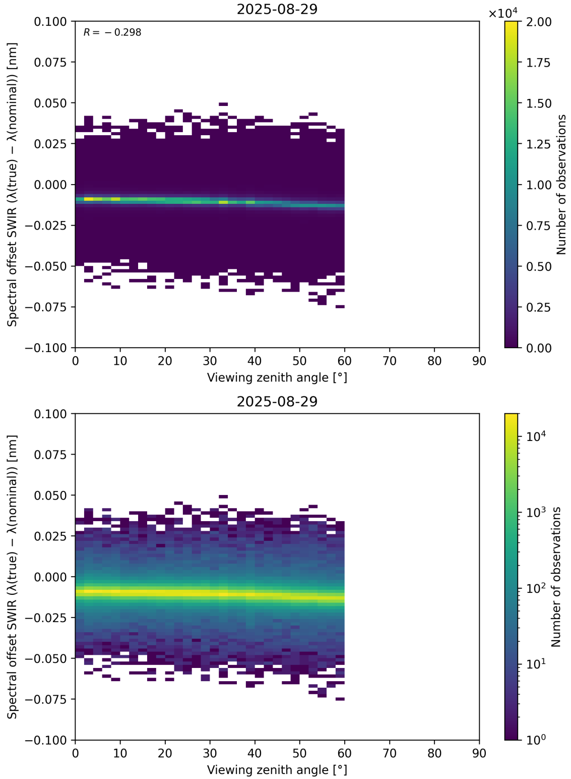
Figure 116: Scatter density plot of “Viewing zenith angle” against “Spectral offset SWIR ( \lambda_{\text{true}} - \lambda_{\text{nominal}} )” for 2025-08-28 to 2025-08-30.
