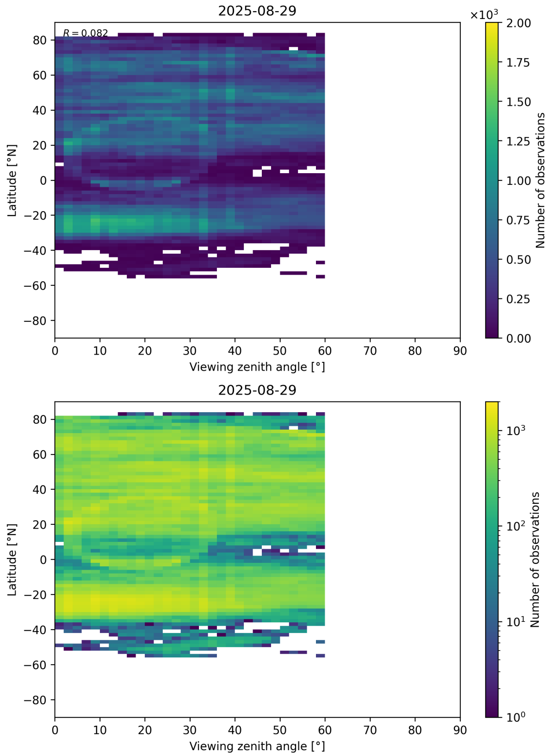
Figure 109: Scatter density plot of “Viewing zenith angle” against “Latitude” for 2025-08-28 to 2025-08-30.
