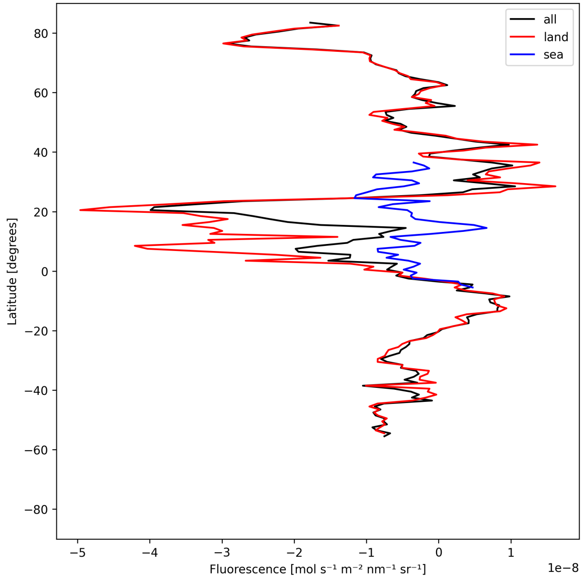
Figure 21: Zonal average of “Fluorescence” for 2025-08-28 to 2025-08-30.
