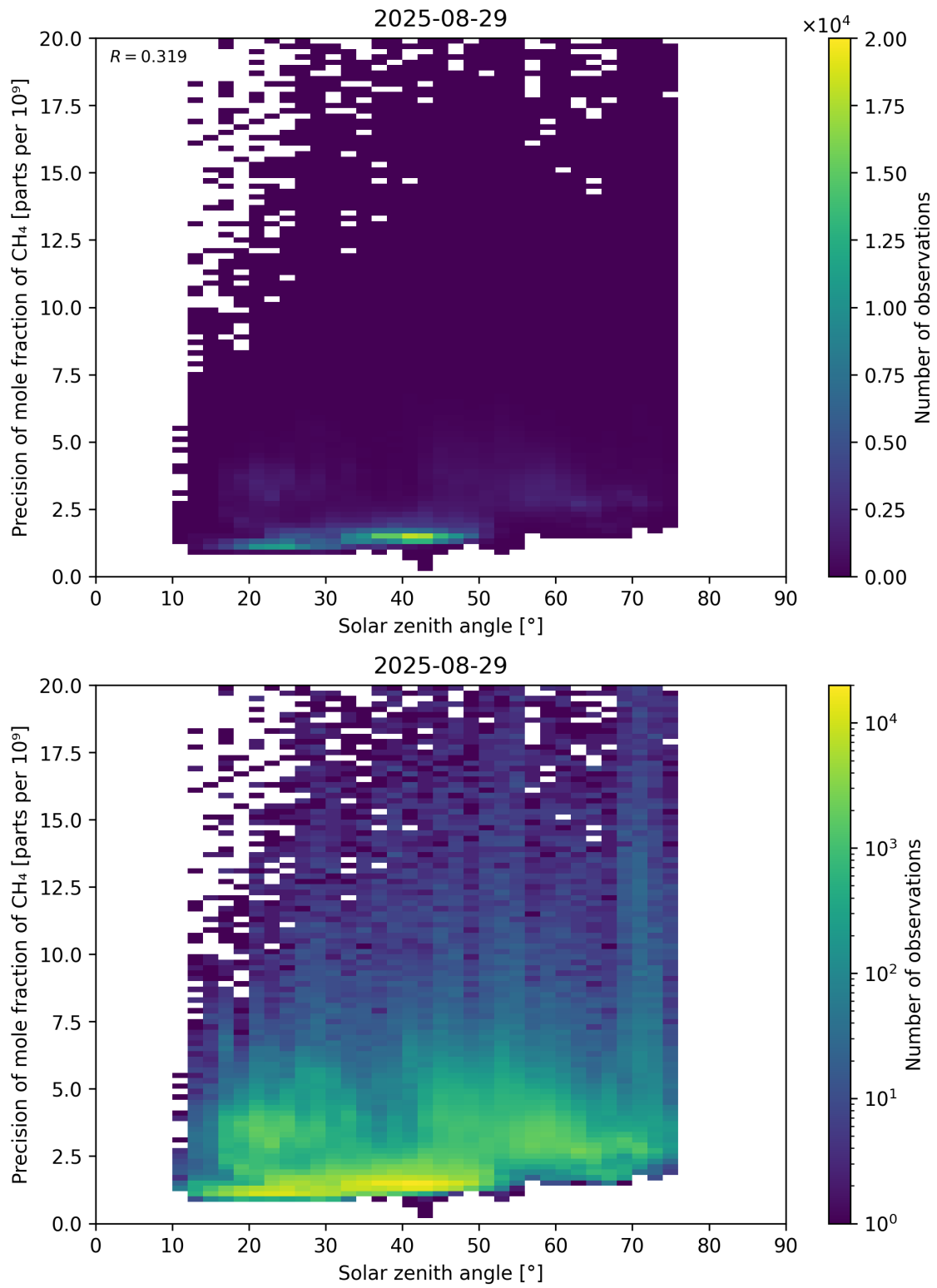
Figure 101: Scatter density plot of “Solar zenith angle” against “Precision of mole fraction of \text{CH}_4 ” for 2025-08-28 to 2025-08-30.
