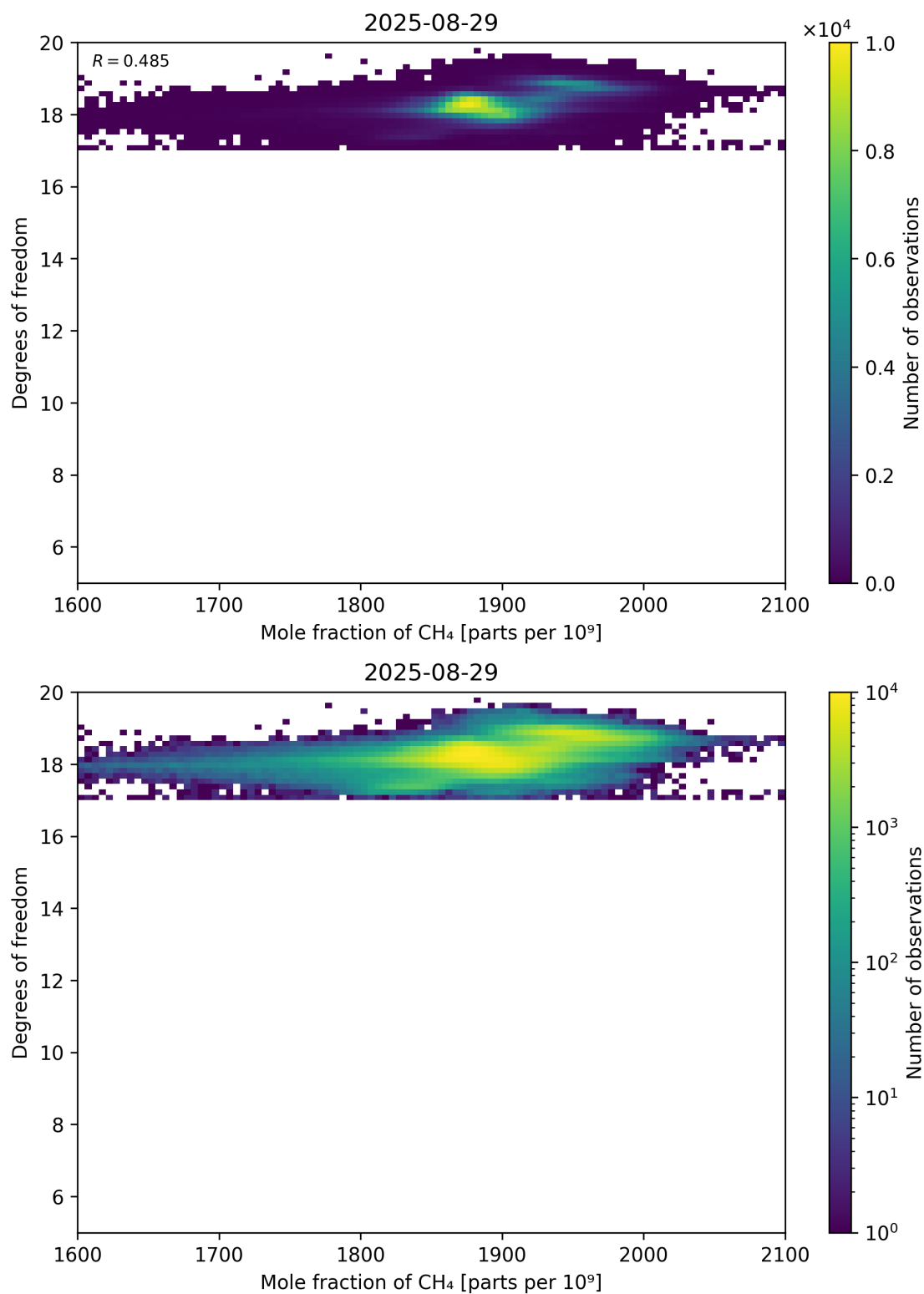
Figure 72: Scatter density plot of “Mole fraction of CH 4 ” against “Degrees of freedom” for 2025-08-28 to 2025-08-30.
