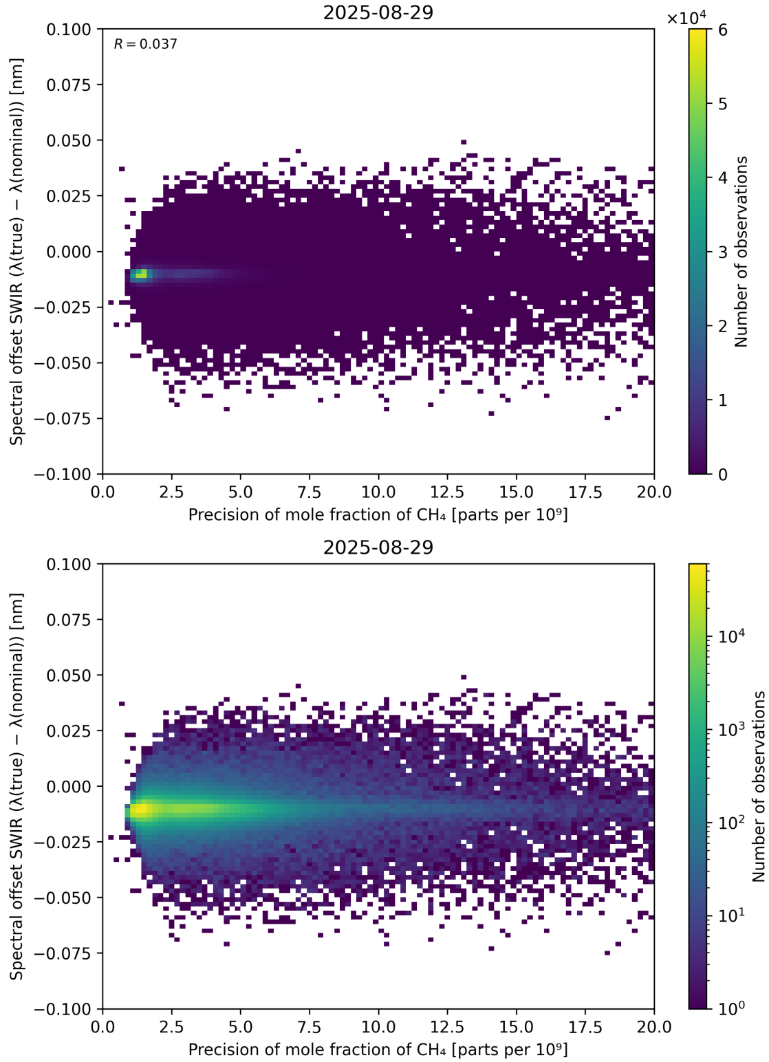
Figure 85: Scatter density plot of “Precision of mole fraction of CH 4 ” against “Spectral offset SWIR ( \lambda_{\text{true}} - \lambda_{\text{nominal}} )” for 2025-08-28 to 2025-08-30.
