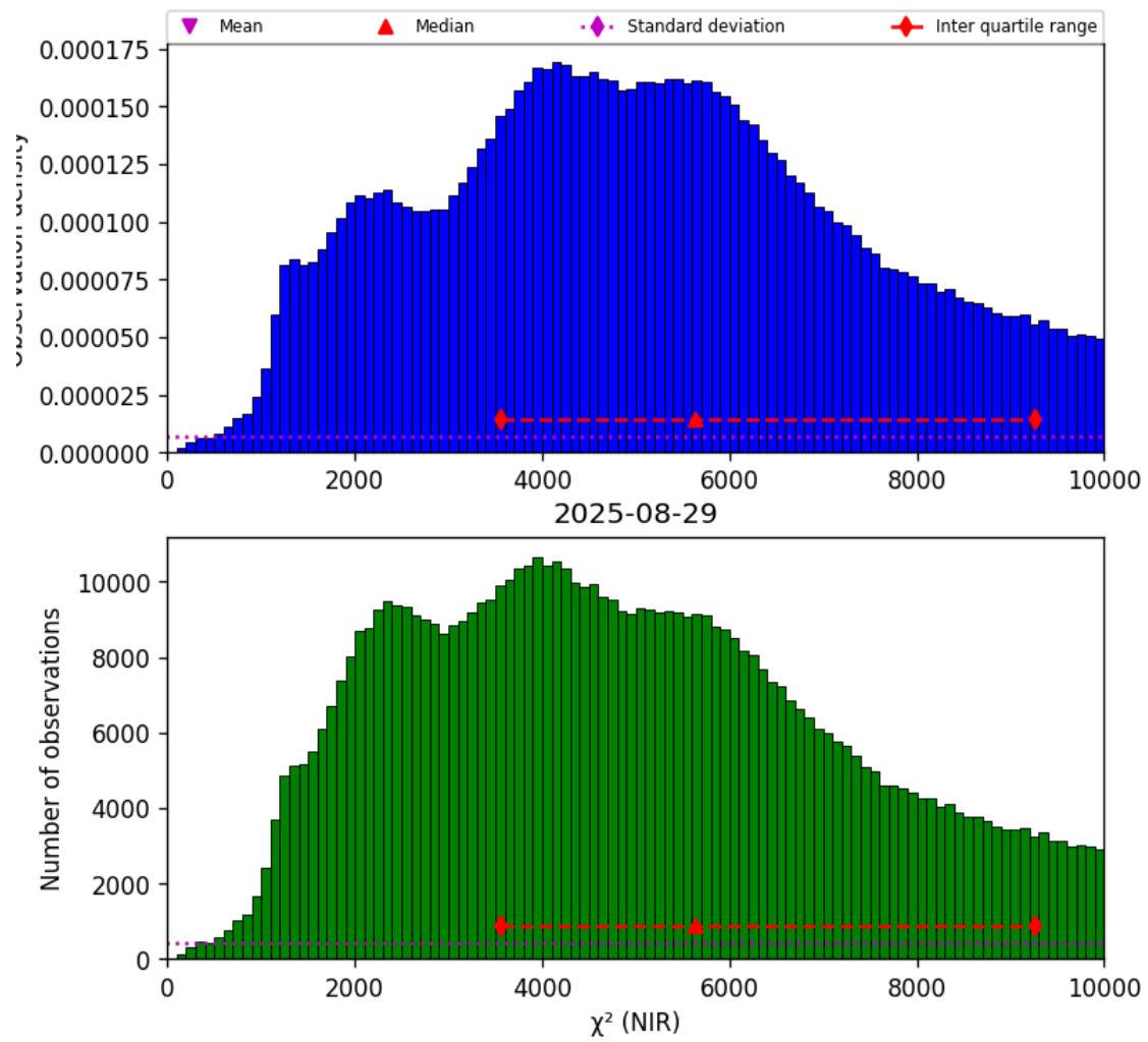
Figure 29: Histogram of “ \chi^2 (NIR)” for 2025-08-28 to 2025-08-30
