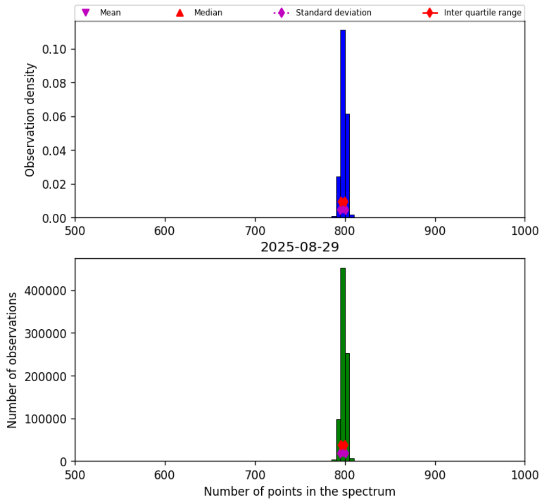
Figure 26: Histogram of “Number of points in the spectrum” for 2025-08-28 to 2025-08-30
