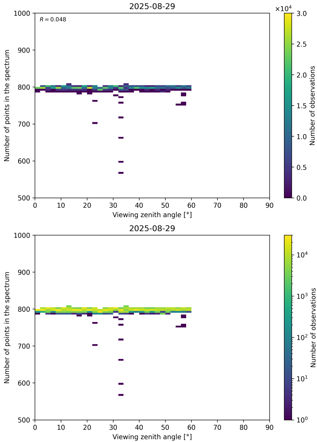
Figure 114: Scatter density plot of “Viewing zenith angle” against “Number of points in the spectrum” for 2025-08-28 to 2025-08-30.
