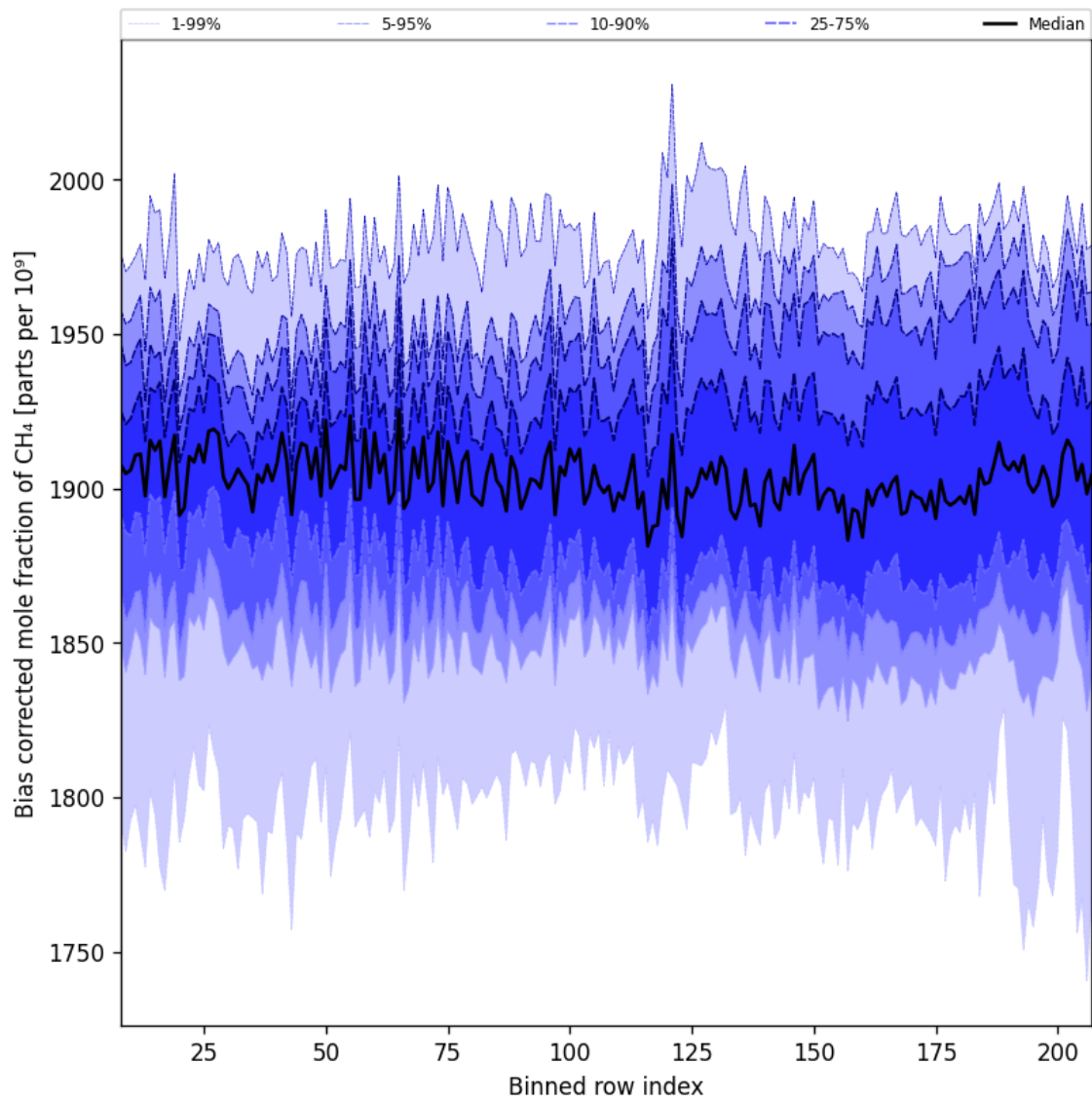
Figure 36: Along track statistics of “Bias corrected mole fraction of CH 4 ” for 2025-08-28 to 2025-08-30
