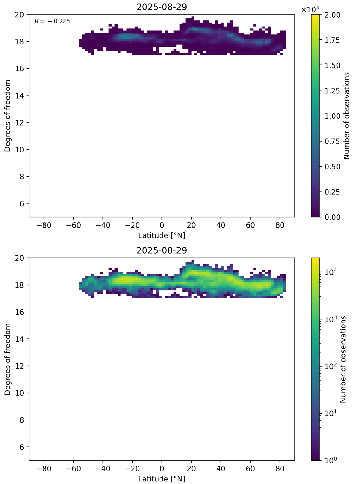
Figure 55: Scatter density plot of “Latitude” against “Degrees of freedom” for 2025-08-28 to 2025-08-30.
