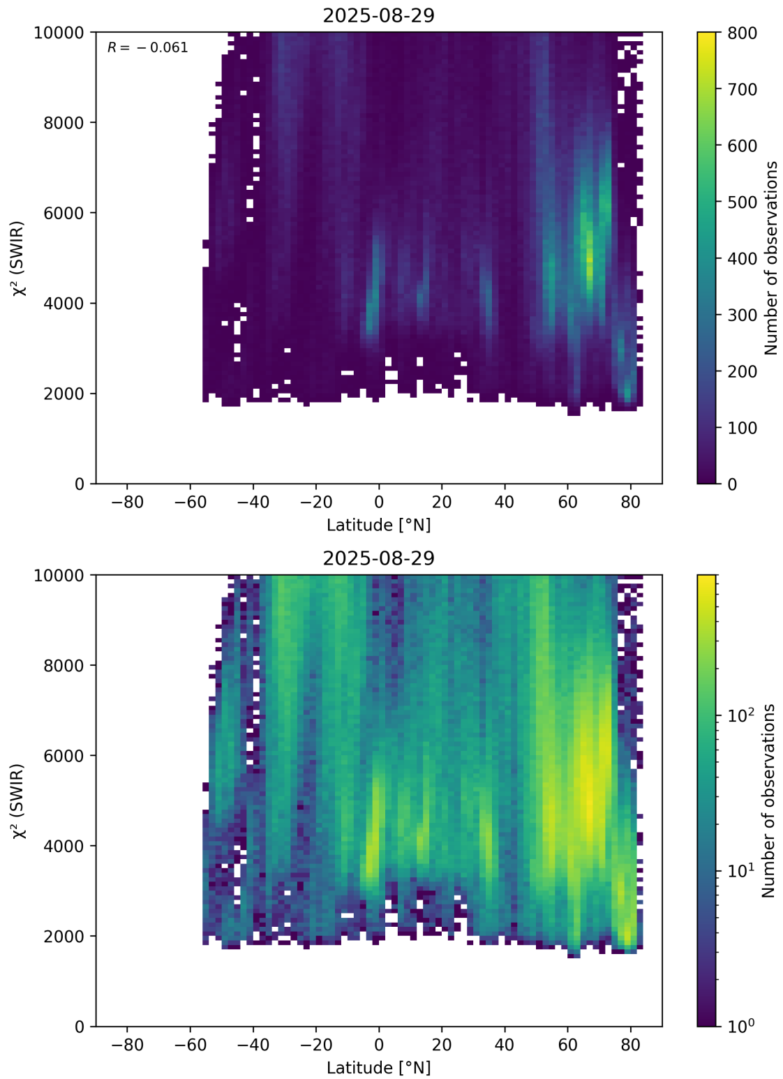
Figure 54: Scatter density plot of “Latitude” against “ \chi^2 (SWIR)” for 2025-08-28 to 2025-08-30.
