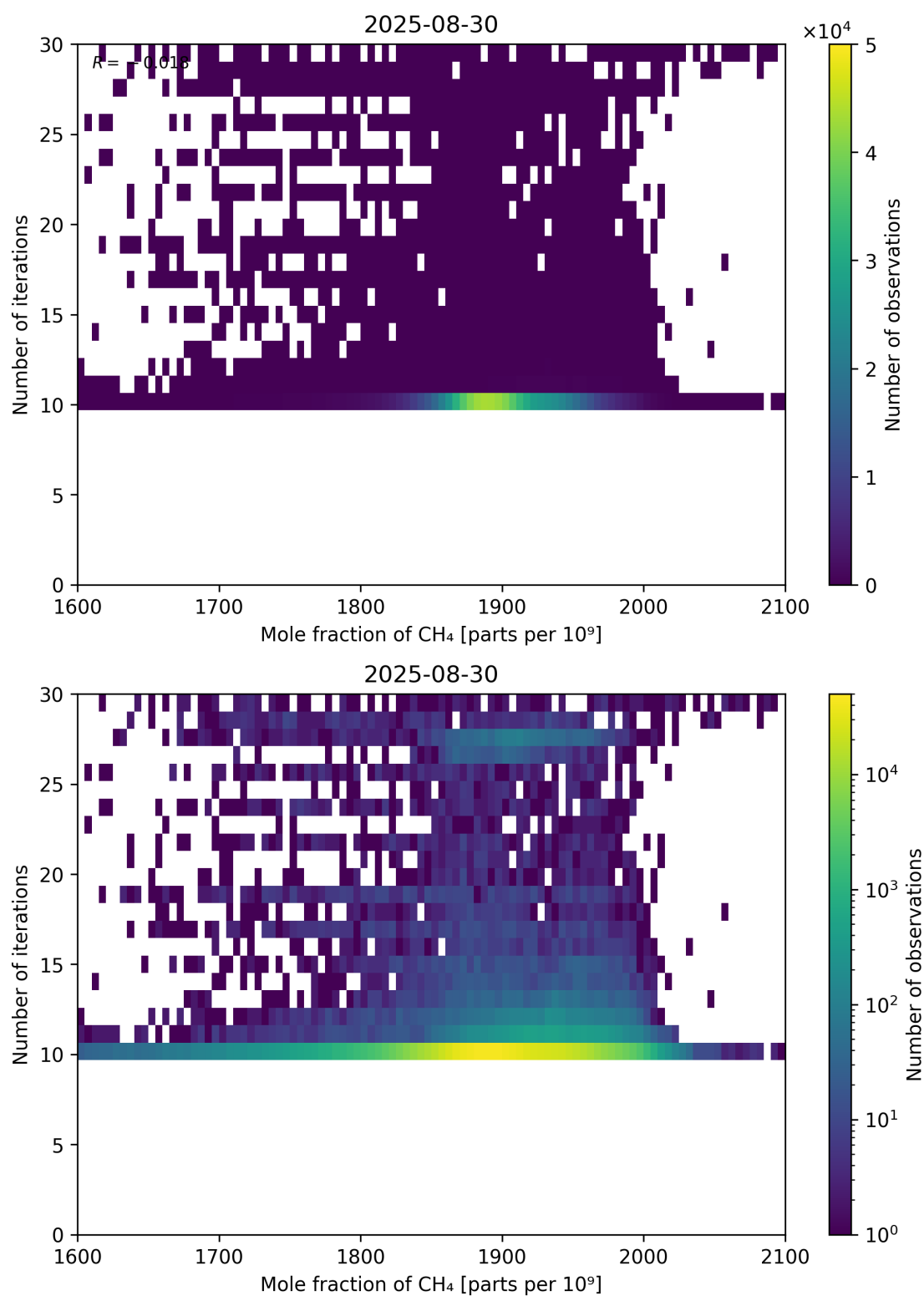
Figure 76: Scatter density plot of “Mole fraction of CH 4 ” against “Number of iterations” for 2025-08-30 to 2025-08-31.
