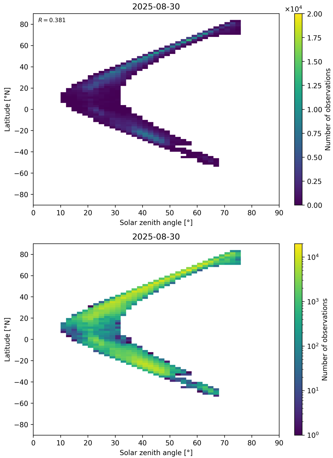
Figure 98: Scatter density plot of “Solar zenith angle” against “Latitude” for 2025-08-30 to 2025-08-31.
