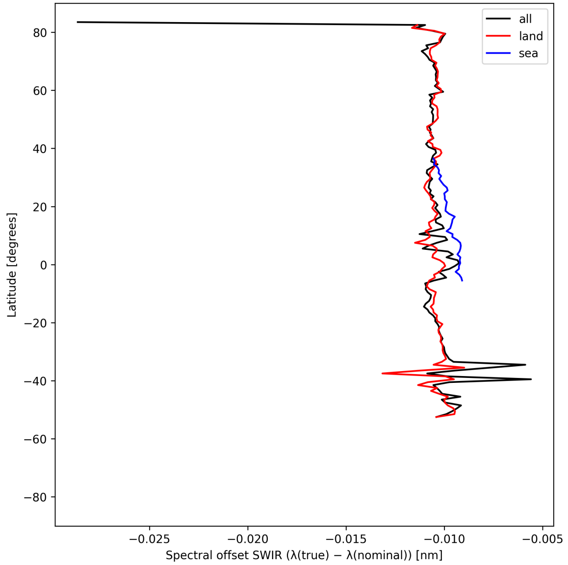
Figure 16: Zonal average of “Spectral offset SWIR ( \lambda_{\text{true}} - \lambda_{\text{nominal}} )” for 2025-08-30 to 2025-08-31.
