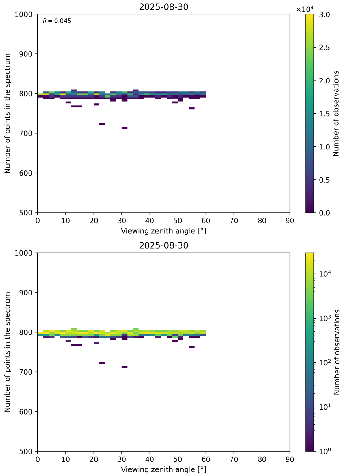
Figure 114: Scatter density plot of “Viewing zenith angle” against “Number of points in the spectrum” for 2025-08-30 to 2025-08-31.
