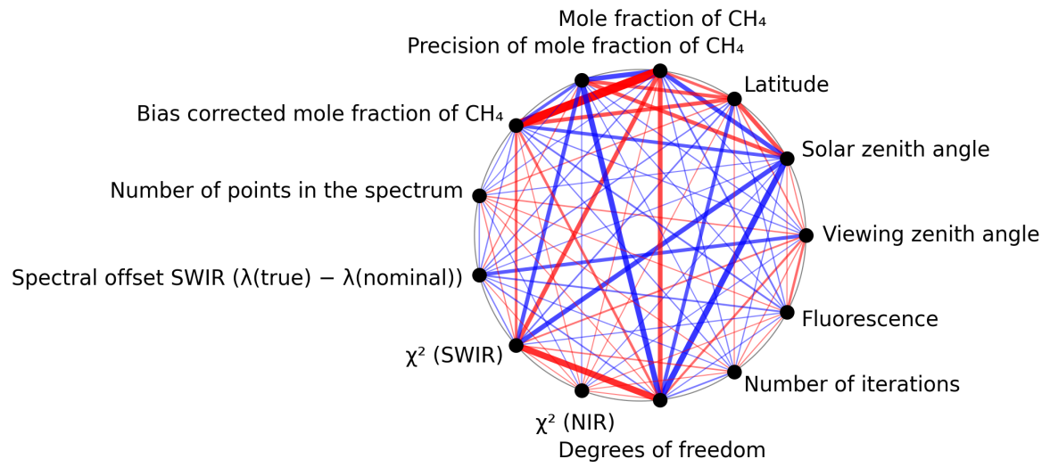
Figure 1: Map of correlation graph for 2025-08-30 to 2025-08-31.
