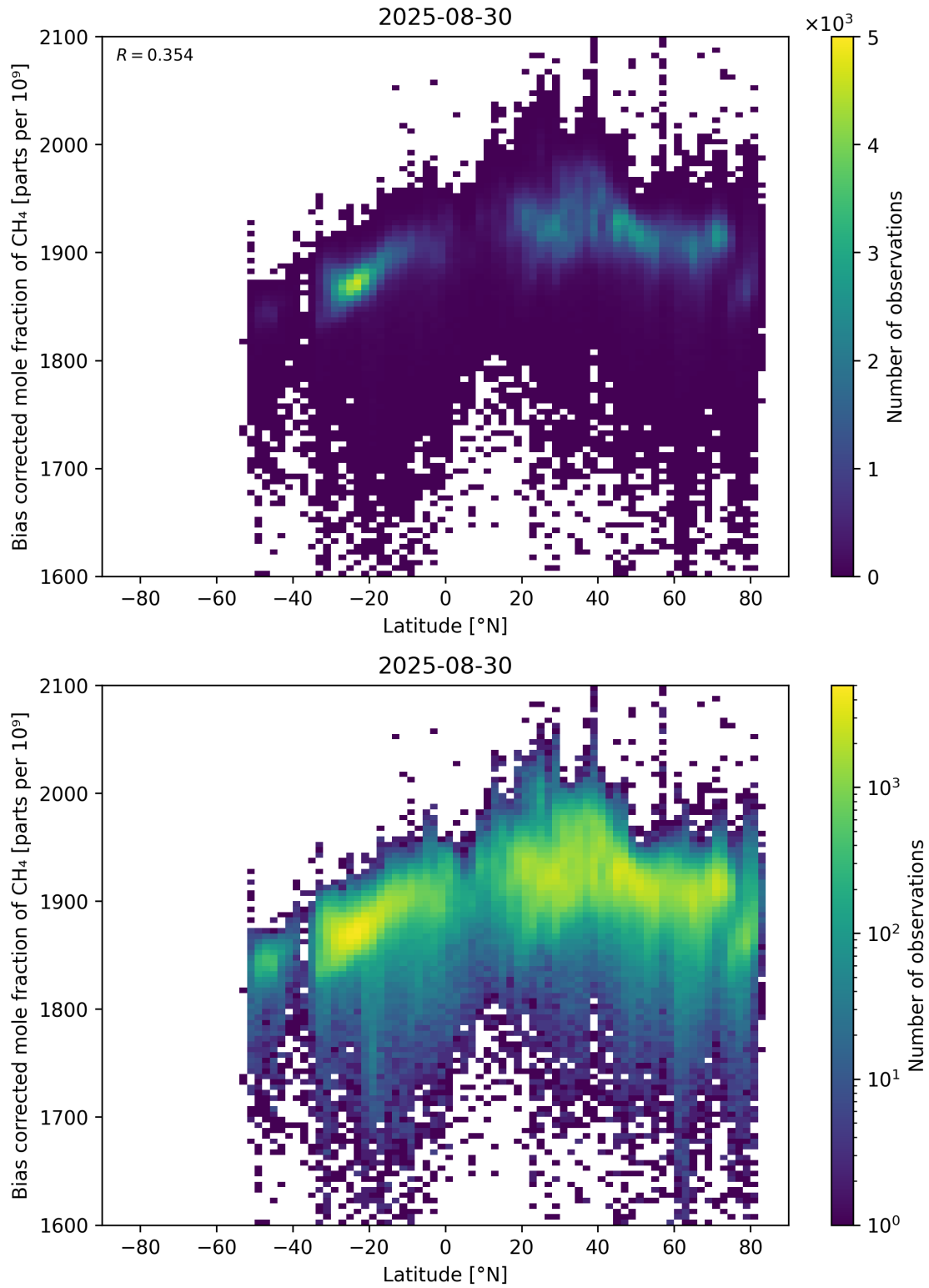
Figure 58: Scatter density plot of “Latitude” against “Bias corrected mole fraction of CH 4 ” for 2025-08-30 to 2025-08-31.
