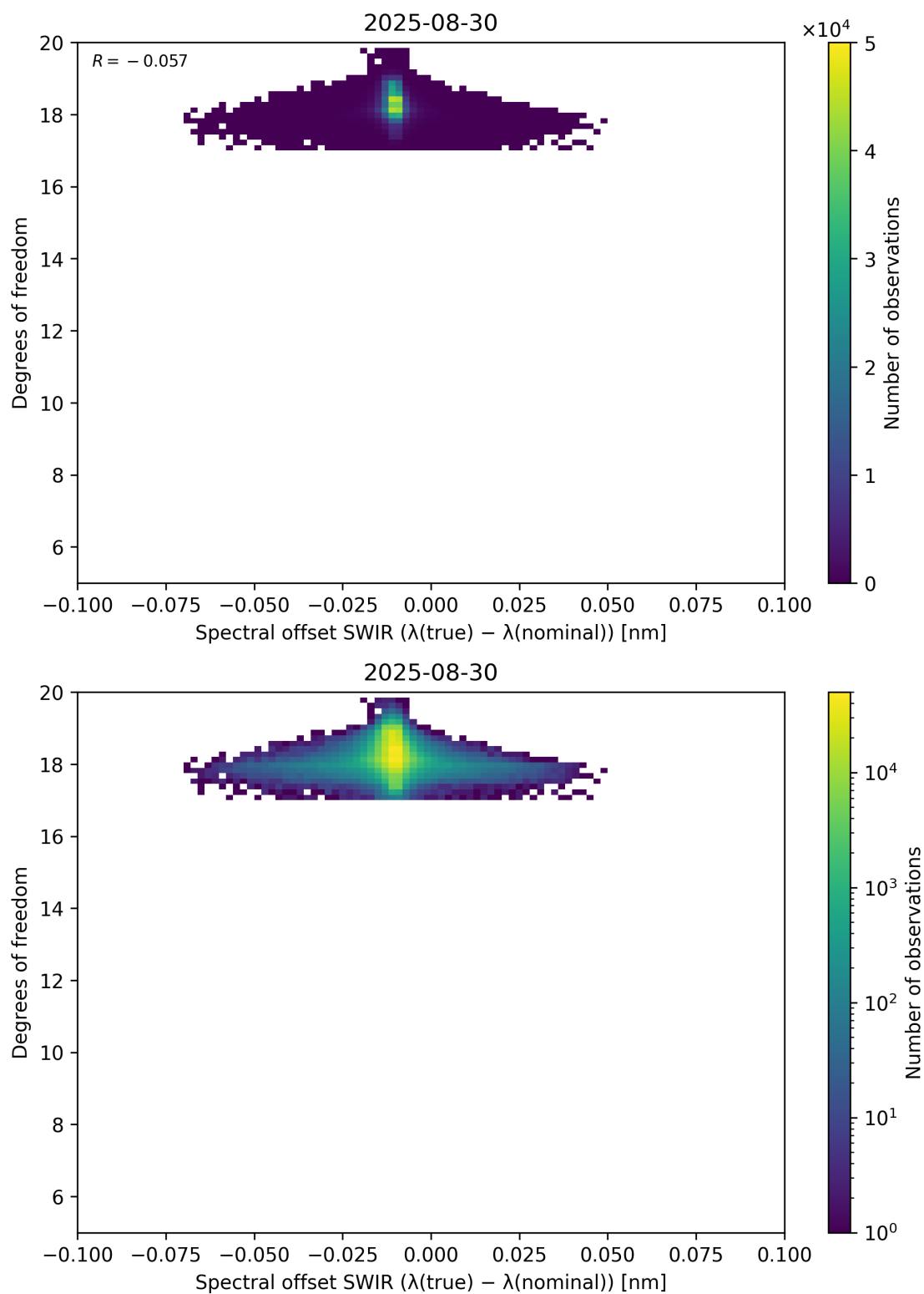
Figure 119: Scatter density plot of “Spectral offset SWIR ( \lambda_{\text{true}} - \lambda_{\text{nominal}} )” against “Degrees of freedom” for 2025-08-30 to 2025-08-31.
