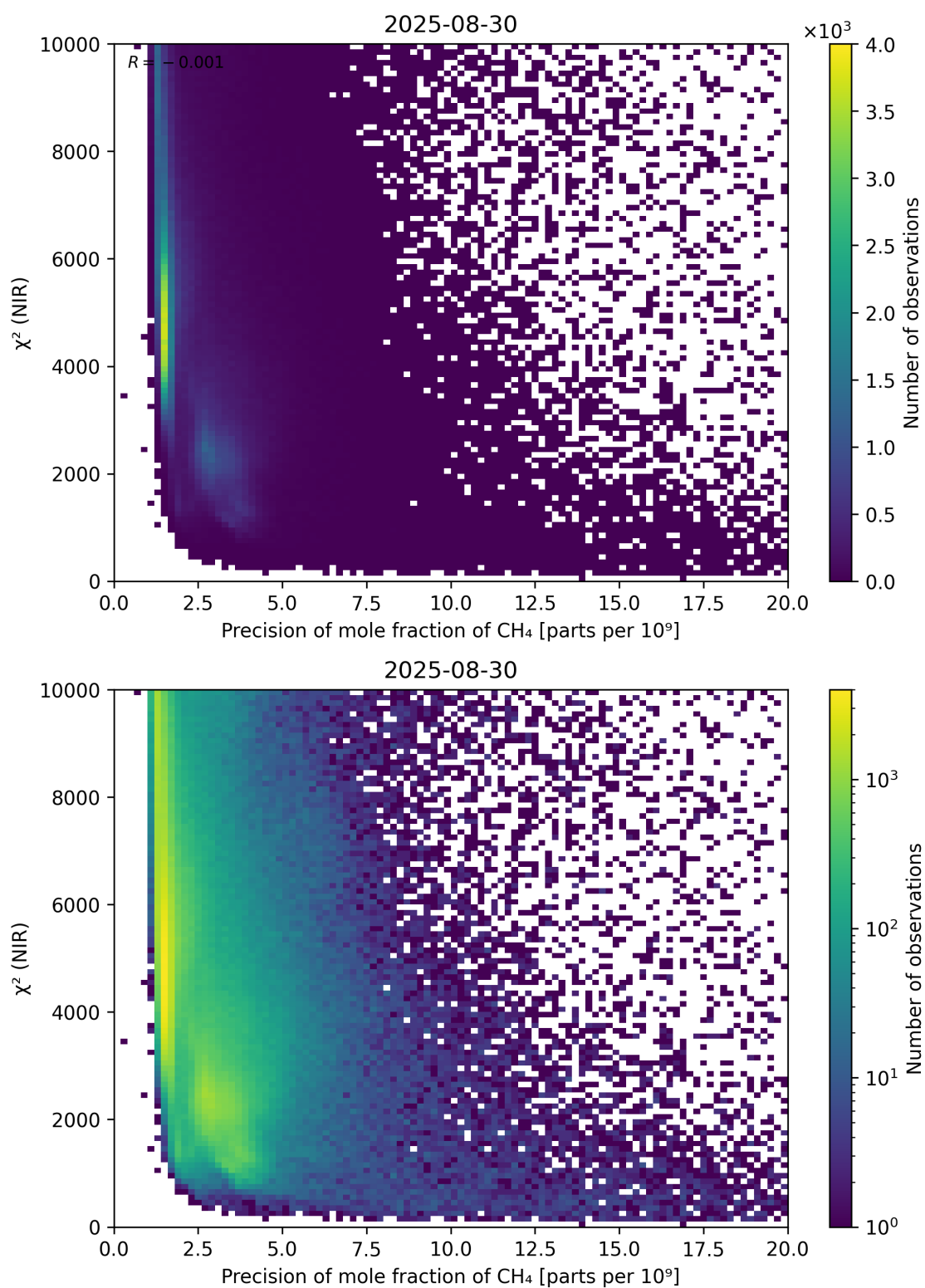
Figure 78: Scatter density plot of “Precision of mole fraction of CH 4 ” against “ \chi^2 (NIR)” for 2025-08-30 to 2025-08-31.
