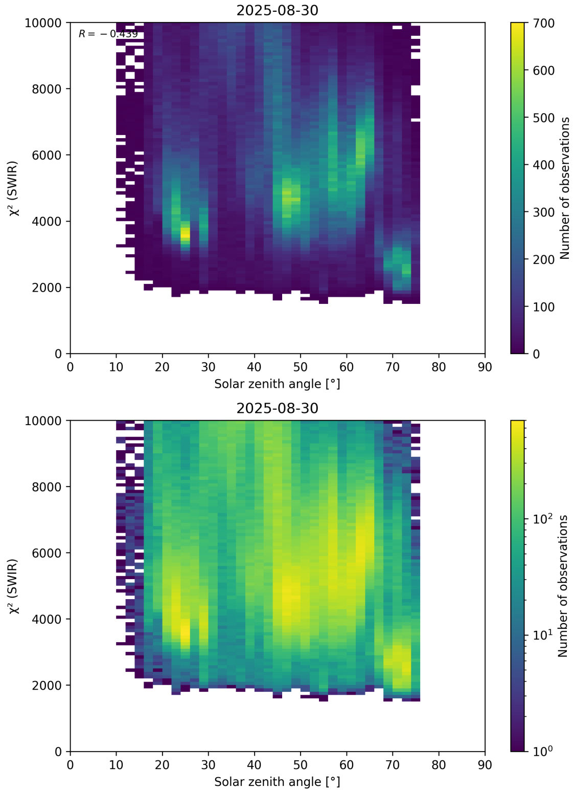
Figure 95: Scatter density plot of “Solar zenith angle” against “ \chi^2 (SWIR)” for 2025-08-30 to 2025-08-31.
