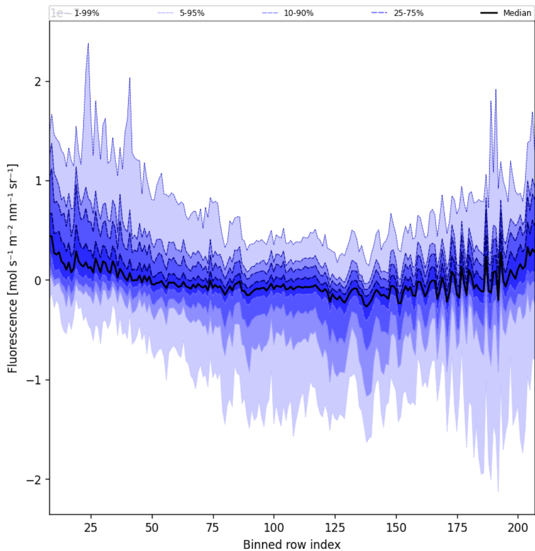
Figure 43: Along track statistics of “Fluorescence” for 2025-08-30 to 2025-08-31
