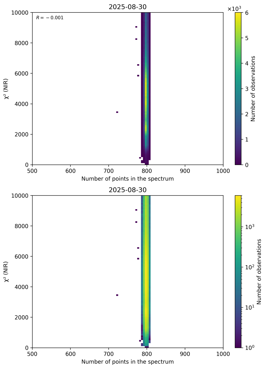
Figure 88: Scatter density plot of “Number of points in the spectrum” against “ \chi^2 (NIR)” for 2025-08-30 to 2025-08-31.
