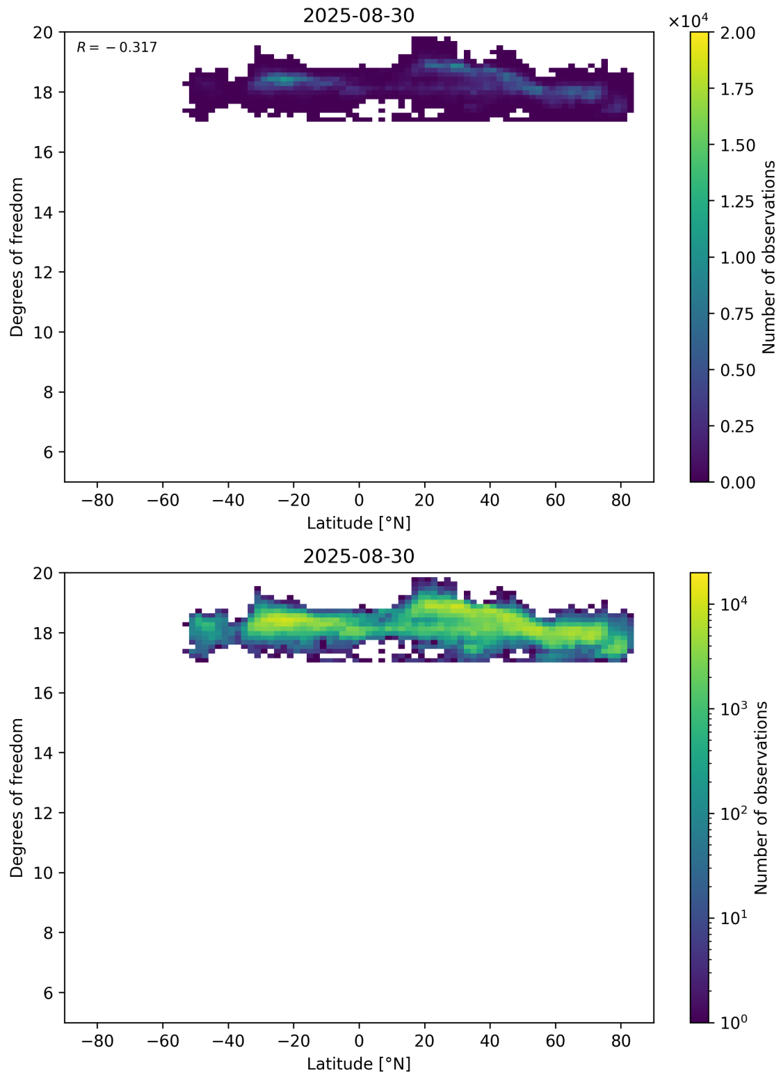
Figure 55: Scatter density plot of “Latitude” against “Degrees of freedom” for 2025-08-30 to 2025-08-31.
