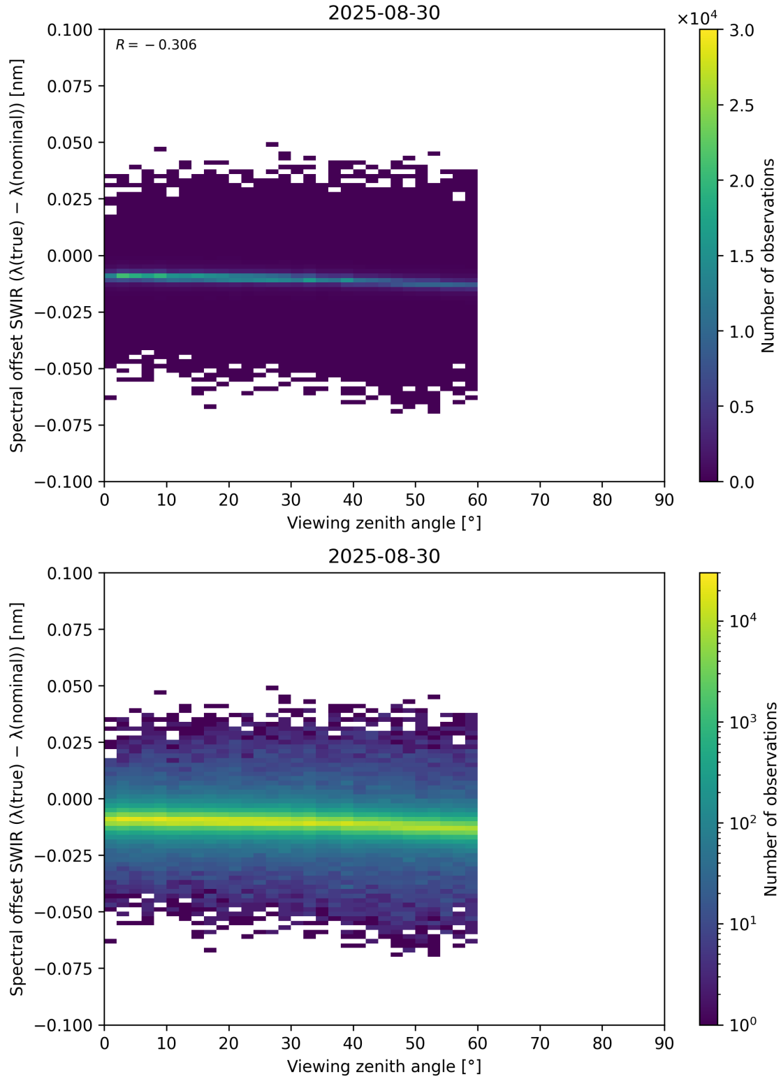
Figure 116: Scatter density plot of “Viewing zenith angle” against “Spectral offset SWIR ( \lambda_{\text{true}} - \lambda_{\text{nominal}} )” for 2025-08-30 to 2025-08-31.
