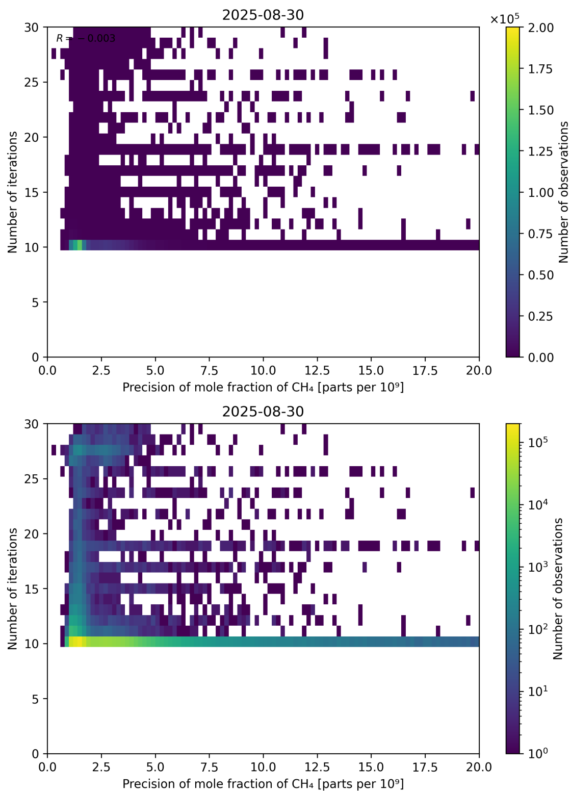
Figure 83: Scatter density plot of “Precision of mole fraction of CH 4 ” against “Number of iterations” for 2025-08-30 to 2025-08-31.
