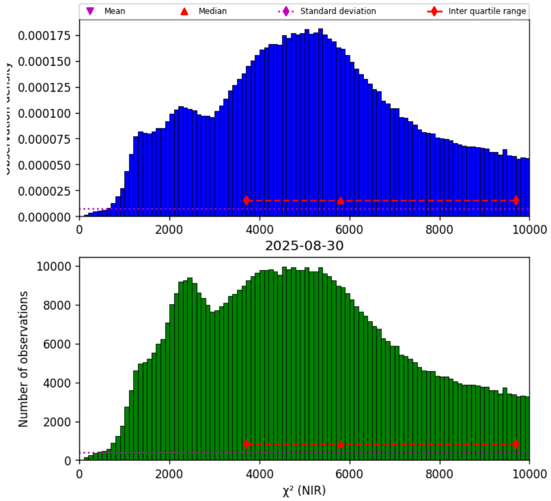
Figure 29: Histogram of “ \chi^2 (NIR)” for 2025-08-30 to 2025-08-31
