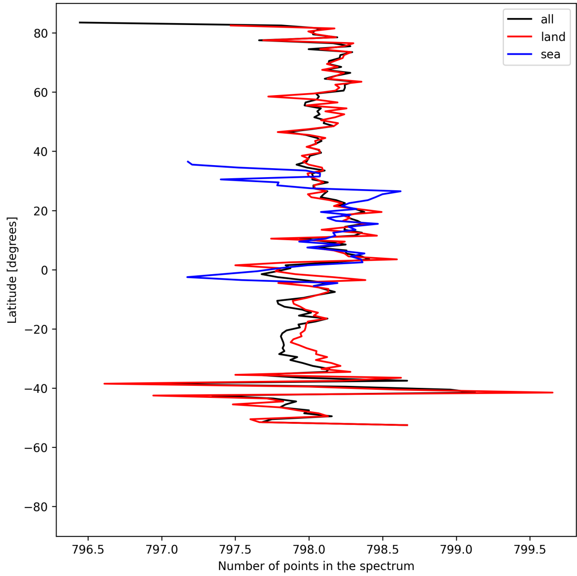
Figure 15: Zonal average of “Number of points in the spectrum” for 2025-08-30 to 2025-08-31.
