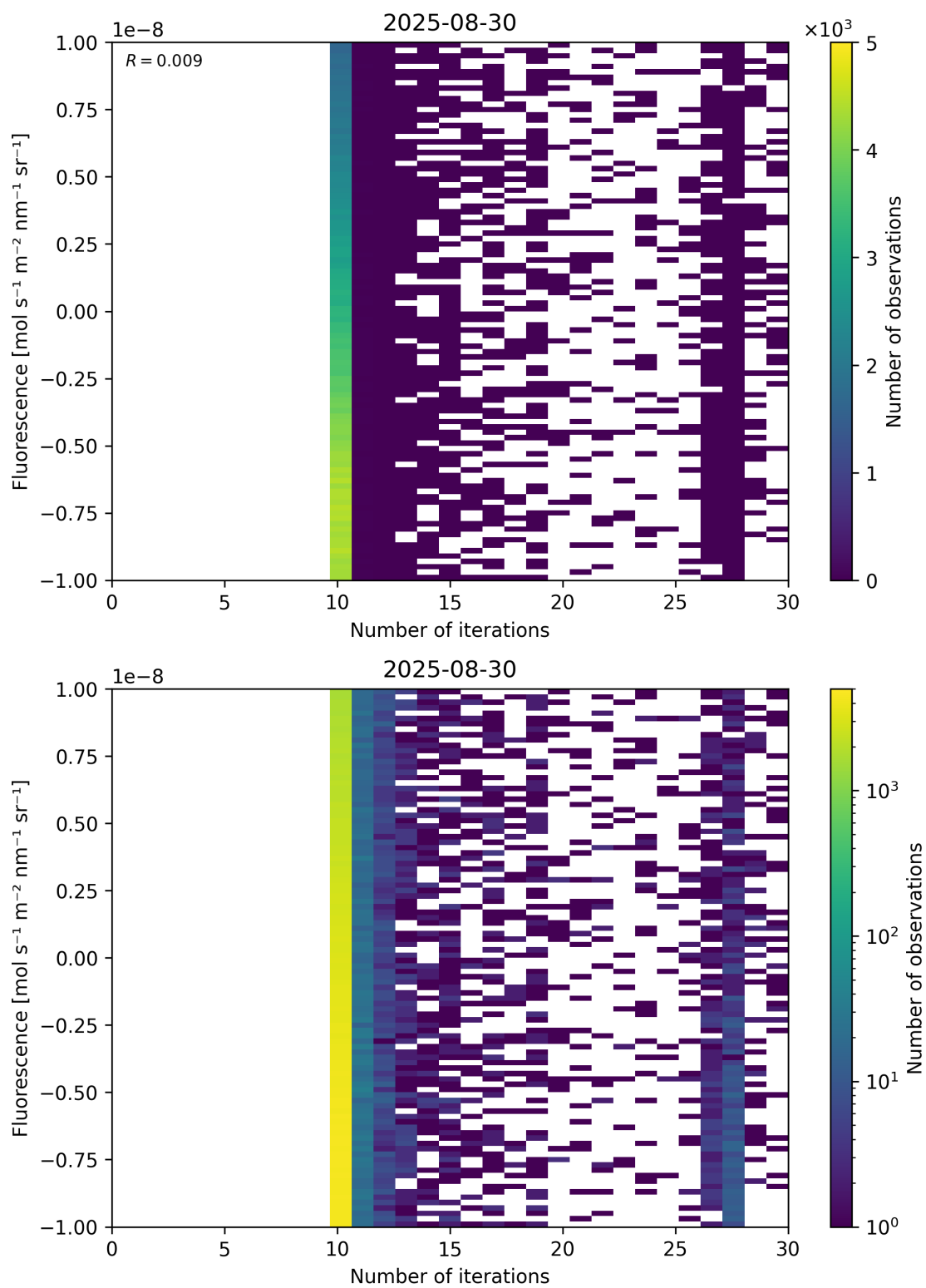
Figure 87: Scatter density plot of “Number of iterations” against “Fluorescence” for 2025-08-30 to 2025-08-31.
