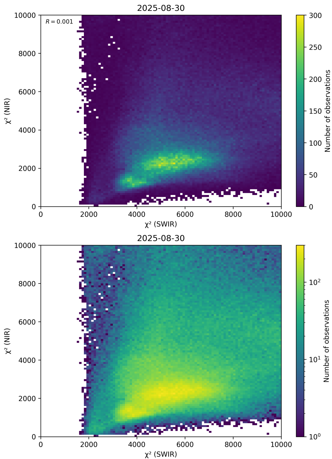
Figure 47: Scatter density plot of “ \chi^2 (SWIR)” against “ \chi^2 (NIR)” for 2025-08-30 to 2025-08-31.
