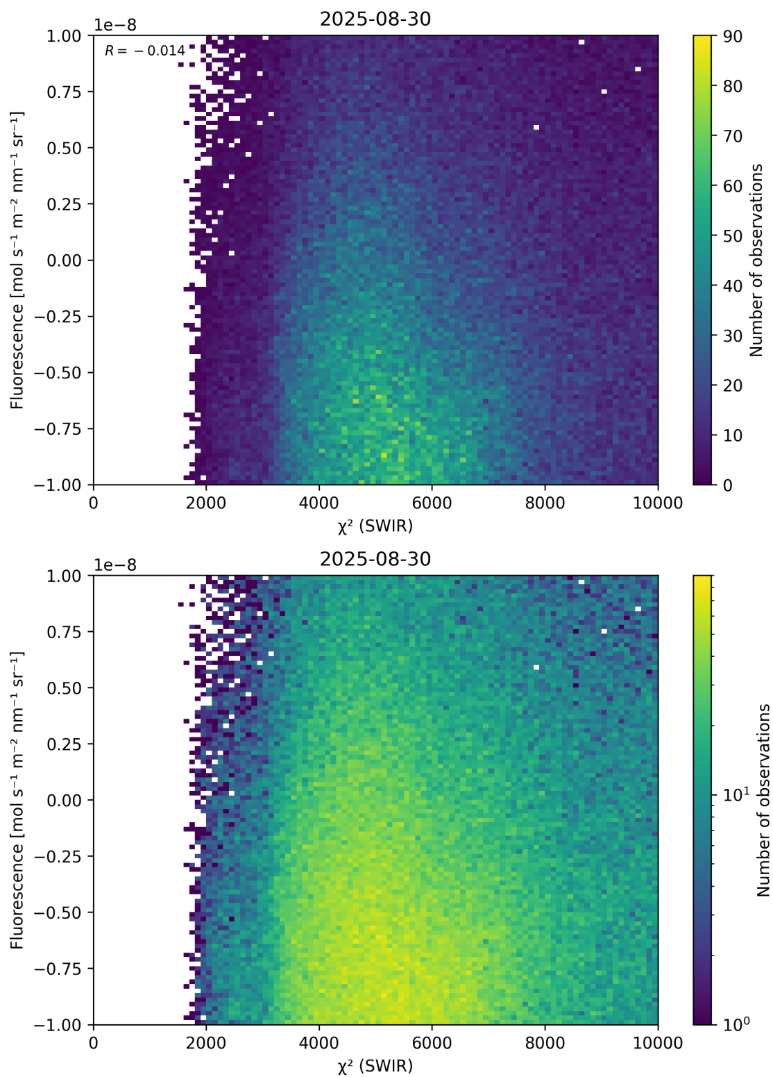
Figure 49: Scatter density plot of “ \chi^2 (SWIR)” against “Fluorescence” for 2025-08-30 to 2025-08-31.
