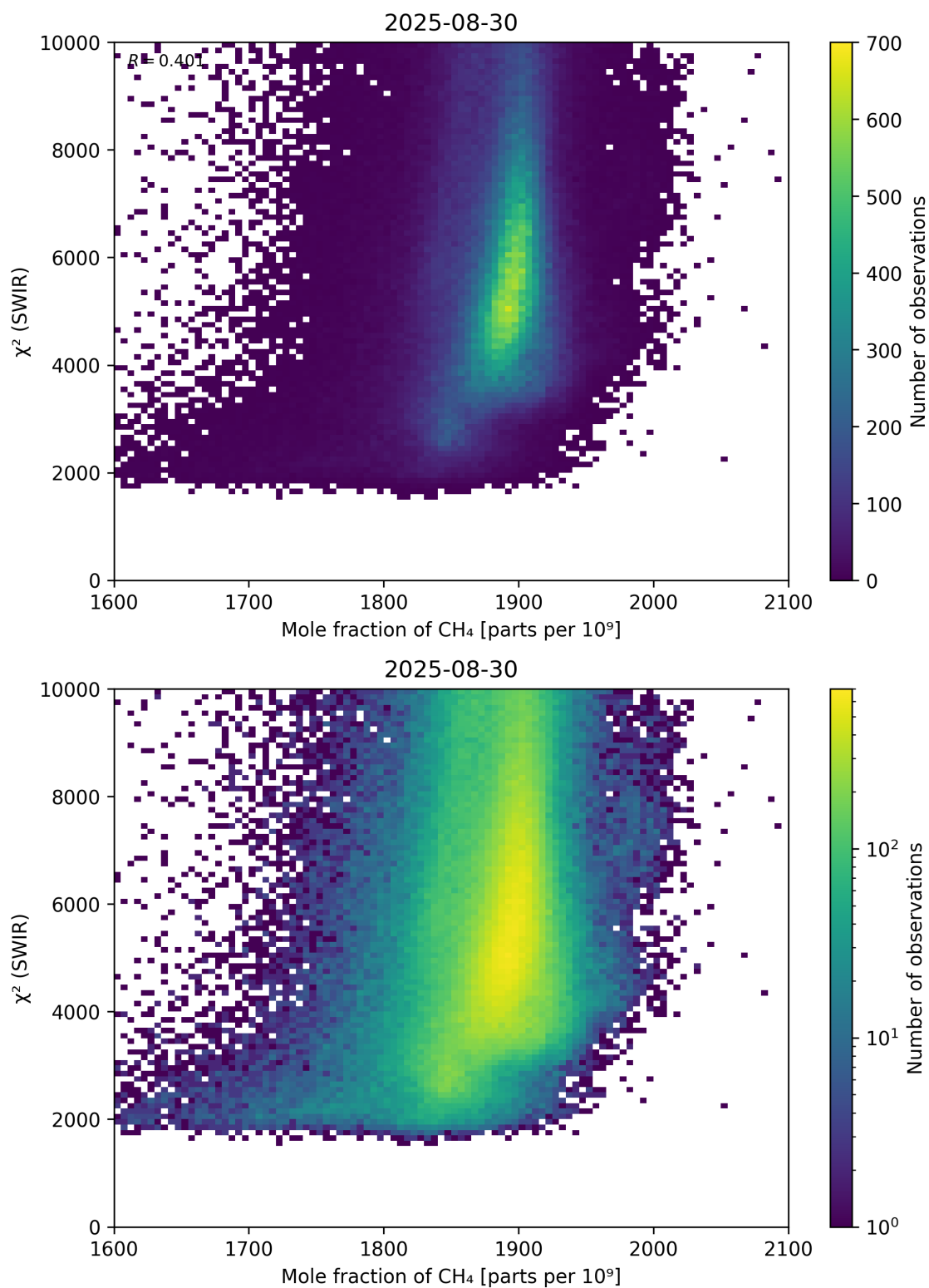
Figure 71: Scatter density plot of “Mole fraction of \text{CH}_4 ” against “ \chi^2 (SWIR)” for 2025-08-30 to 2025-08-31.
