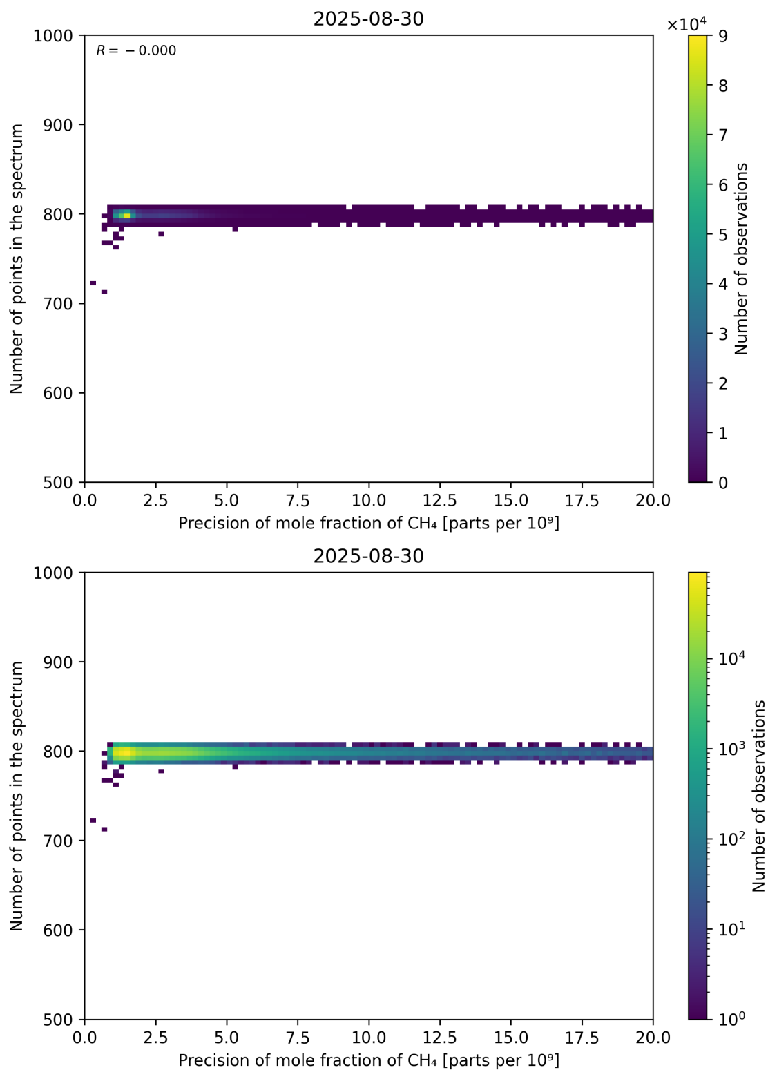
Figure 84: Scatter density plot of “Precision of mole fraction of CH 4 ” against “Number of points in the spectrum” for 2025-08-30 to 2025-08-31.
