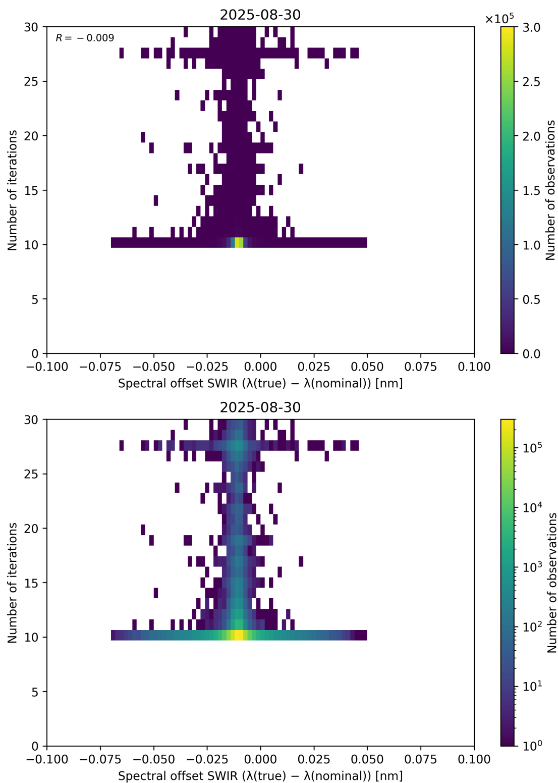
Figure 121: Scatter density plot of “Spectral offset SWIR ( \lambda_{\text{true}} - \lambda_{\text{nominal}} )” against “Number of iterations” for 2025-08-30 to 2025-08-31.
