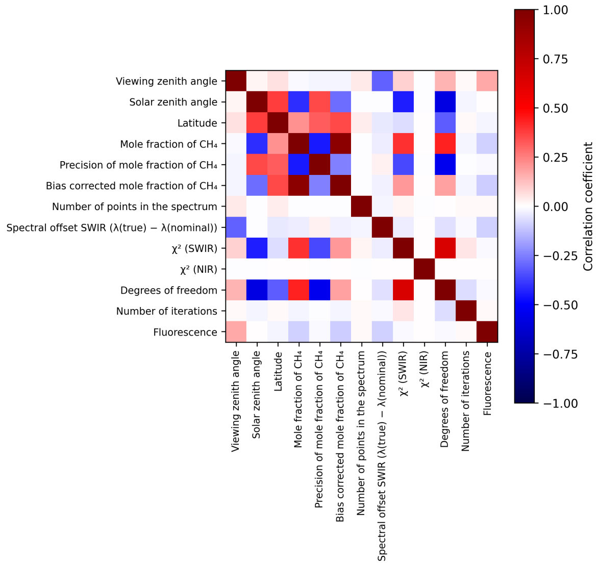
Figure 2: Map of correlation matrix for 2025-08-30 to 2025-08-31.
