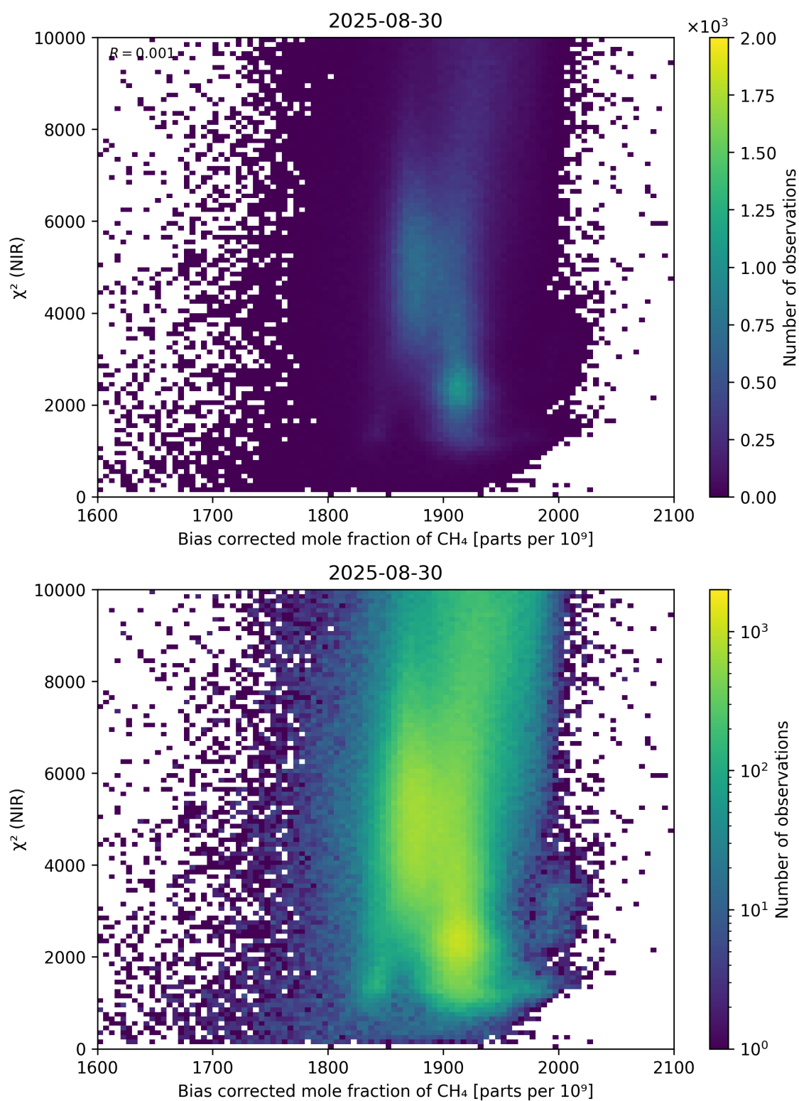
Figure 63: Scatter density plot of “Bias corrected mole fraction of \text{CH}_4 ” against “ \chi^2 (NIR)” for 2025-08-30 to 2025-08-31.
