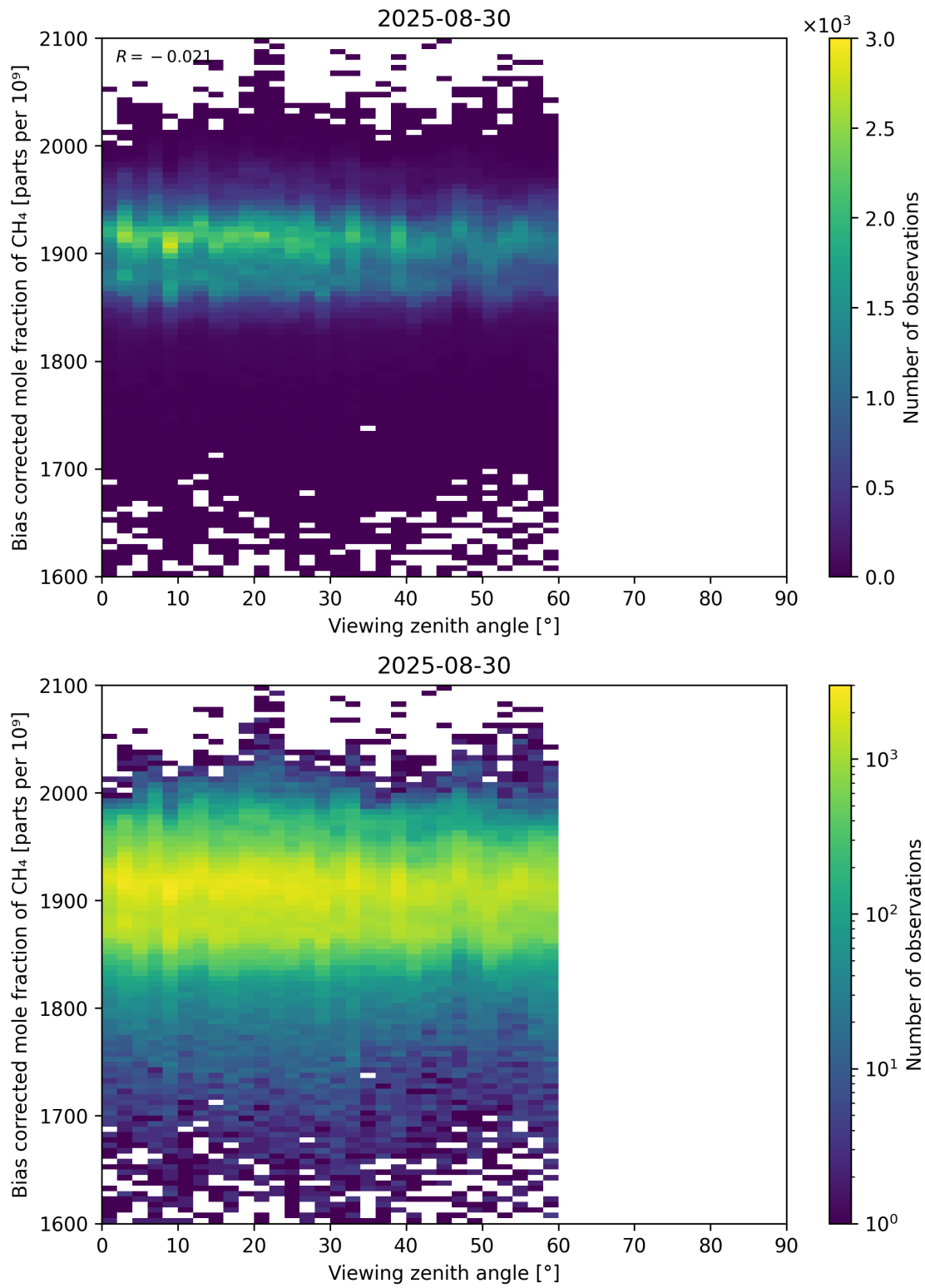
Figure 111: Scatter density plot of “Viewing zenith angle” against “Bias corrected mole fraction of CH 4 ” for 2025-08-30 to 2025-08-31.
