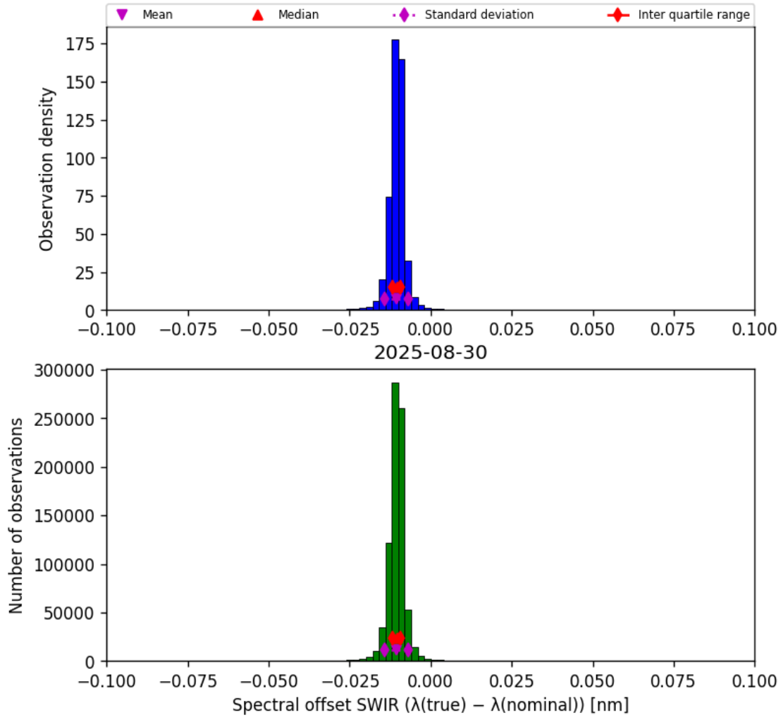
Figure 27: Histogram of “Spectral offset SWIR ( \lambda_{\text{true}} - \lambda_{\text{nominal}} )” for 2025-08-30 to 2025-08-31
