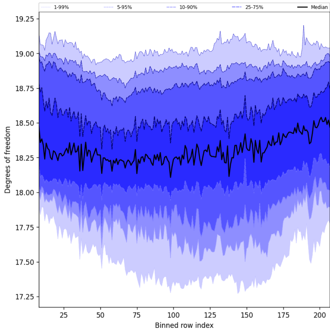
Figure 41: Along track statistics of “Degrees of freedom” for 2025-08-30 to 2025-08-31
