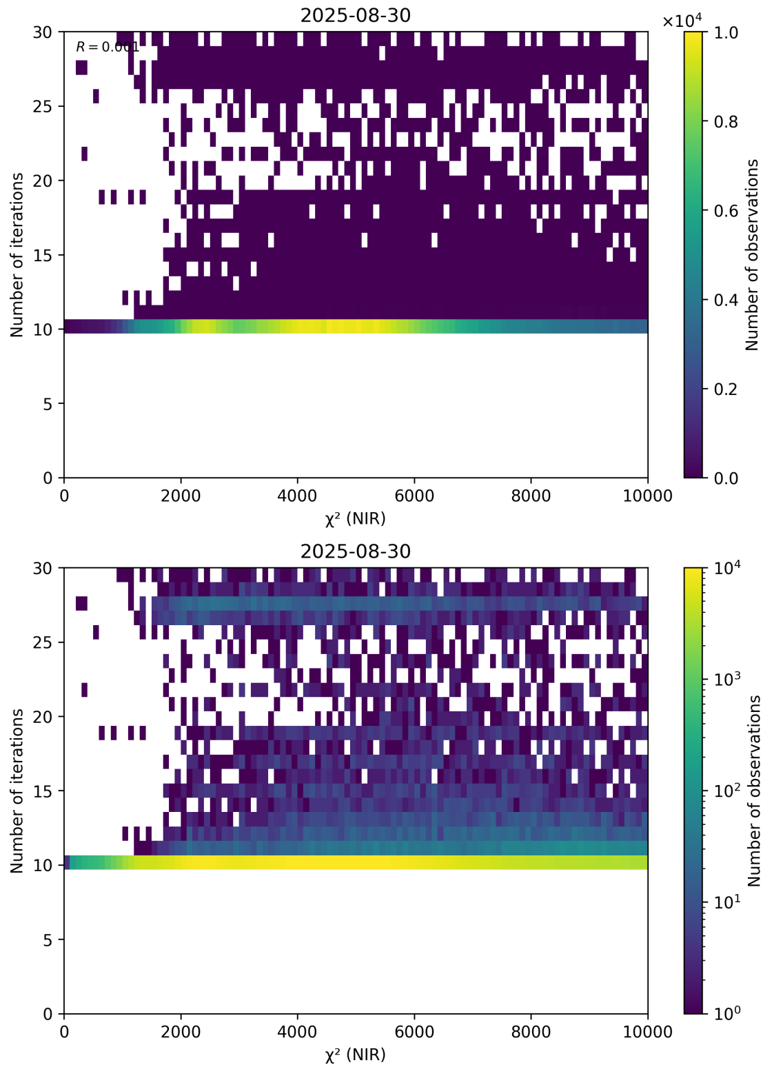
Figure 46: Scatter density plot of “ \chi^2 (NIR)” against “Number of iterations” for 2025-08-30 to 2025-08-31.
