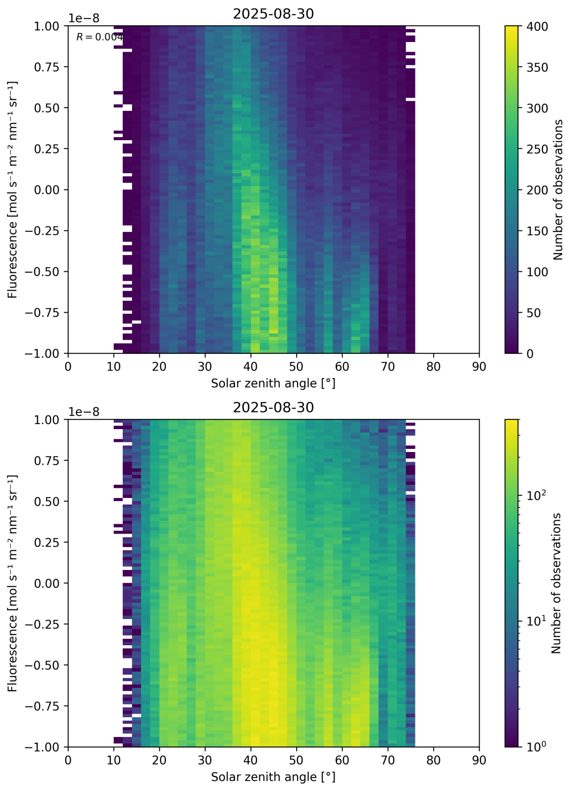
Figure 97: Scatter density plot of “Solar zenith angle” against “Fluorescence” for 2025-08-30 to 2025-08-31.
