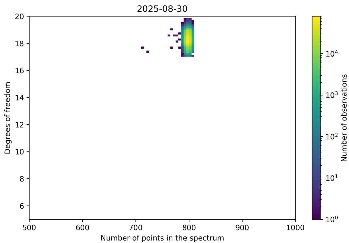
Figure 90: Scatter density plot of “Number of points in the spectrum” against “Degrees of freedom” for 2025-08-30 to 2025-08-31.
