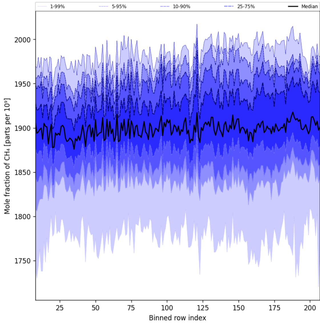
Figure 34: Along track statistics of “Mole fraction of CH 4 ” for 2025-08-30 to 2025-08-31
