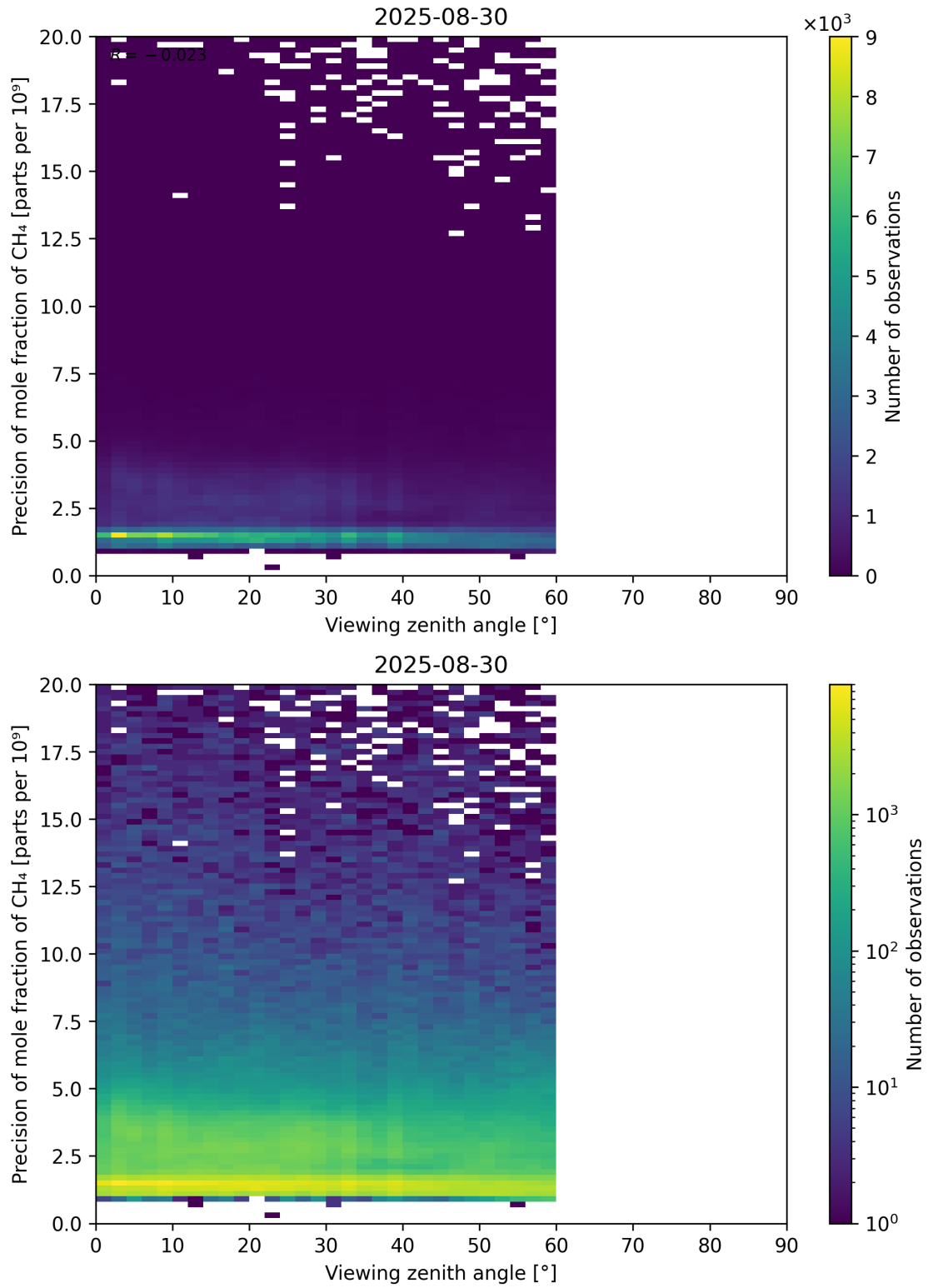
Figure 112: Scatter density plot of “Viewing zenith angle” against “Precision of mole fraction of CH 4 ” for 2025-08-30 to 2025-08-31.
