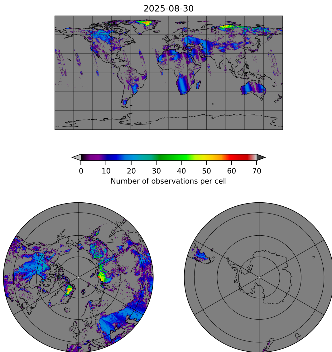
Figure 10: Map of the number of observations for 2025-08-30 to 2025-08-31
