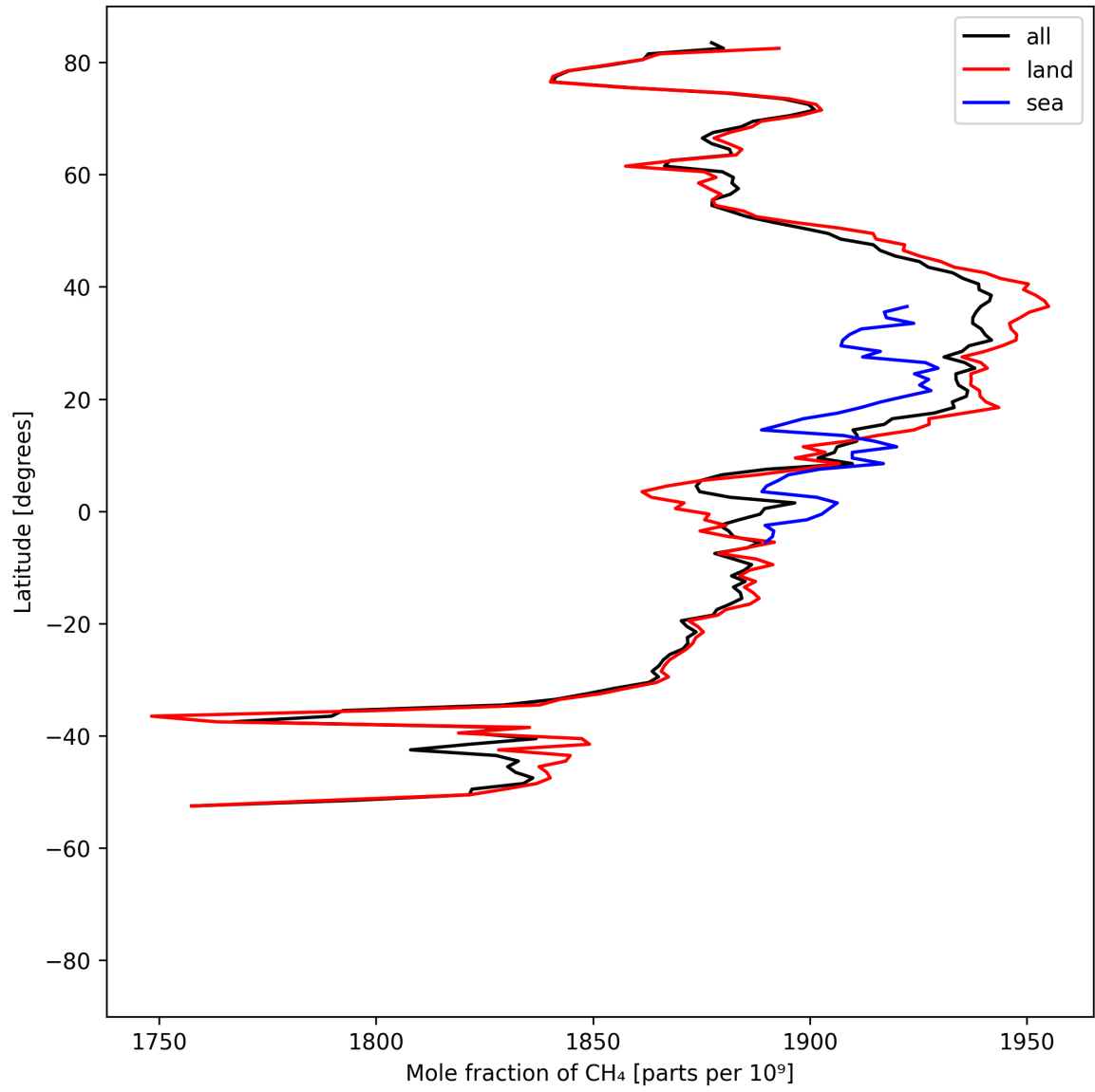
Figure 12: Zonal average of “Mole fraction of \text{CH}_4 ” for 2025-08-30 to 2025-08-31.
