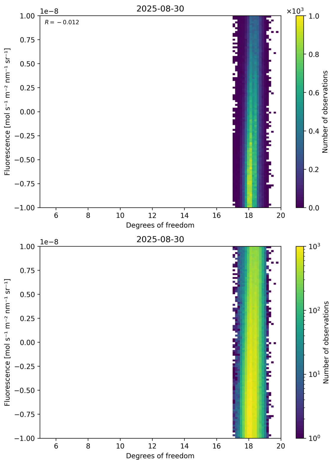
Figure 51: Scatter density plot of “Degrees of freedom” against “Fluorescence” for 2025-08-30 to 2025-08-31.
