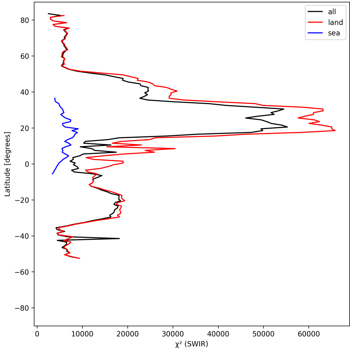
Figure 17: Zonal average of “ \chi^2 (SWIR)” for 2025-08-30 to 2025-08-31.
