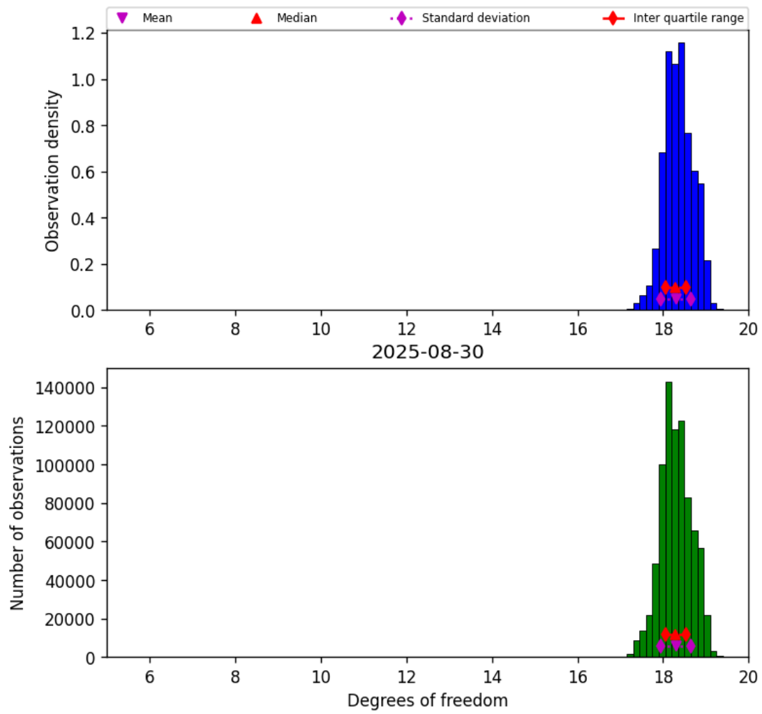
Figure 30: Histogram of “Degrees of freedom” for 2025-08-30 to 2025-08-31
