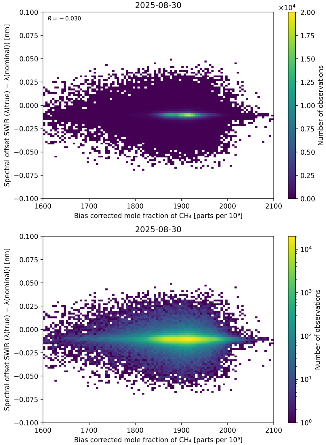
Figure 69: Scatter density plot of “Bias corrected mole fraction of \text{CH}_4 ” against “Spectral offset SWIR ( \lambda_{\text{true}} - \lambda_{\text{nominal}} )” for 2025-08-30 to 2025-08-31.
