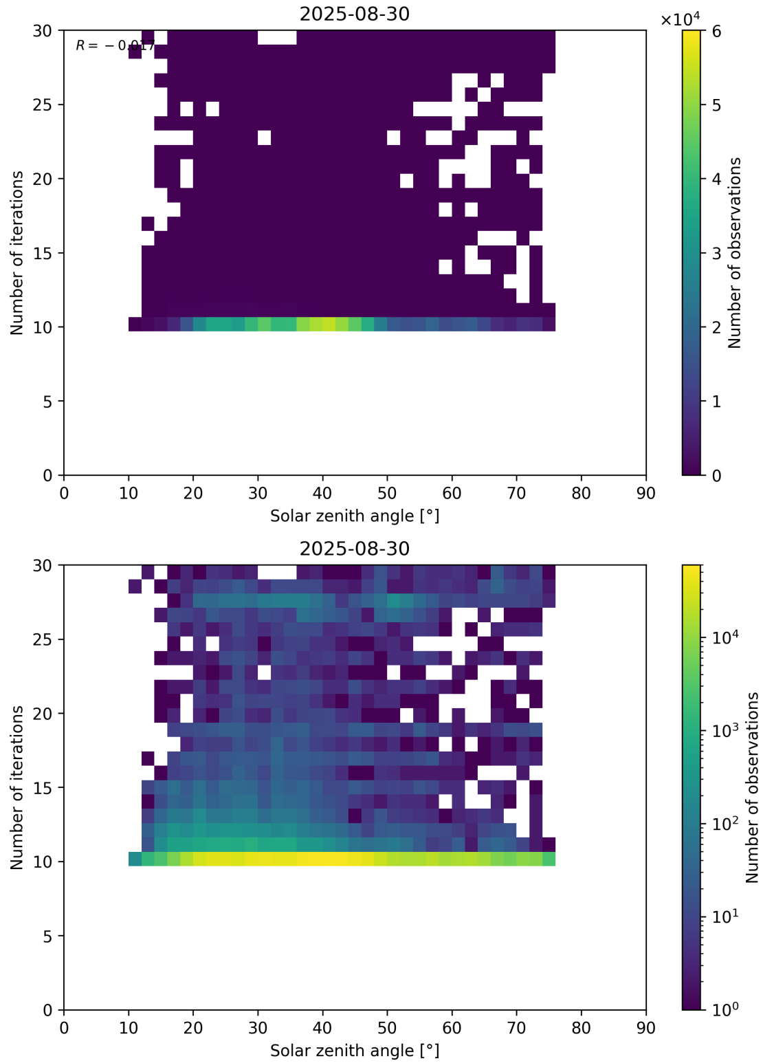
Figure 102: Scatter density plot of “Solar zenith angle” against “Number of iterations” for 2025-08-30 to 2025-08-31.
