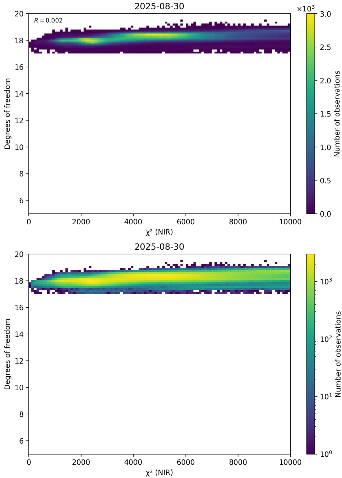
Figure 44: Scatter density plot of “ \chi^2 (NIR)” against “Degrees of freedom” for 2025-08-30 to 2025-08-31.
