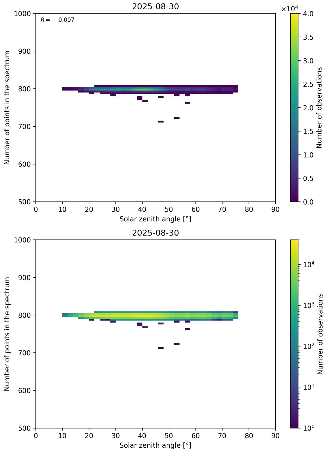
Figure 103: Scatter density plot of “Solar zenith angle” against “Number of points in the spectrum” for 2025-08-30 to 2025-08-31.
