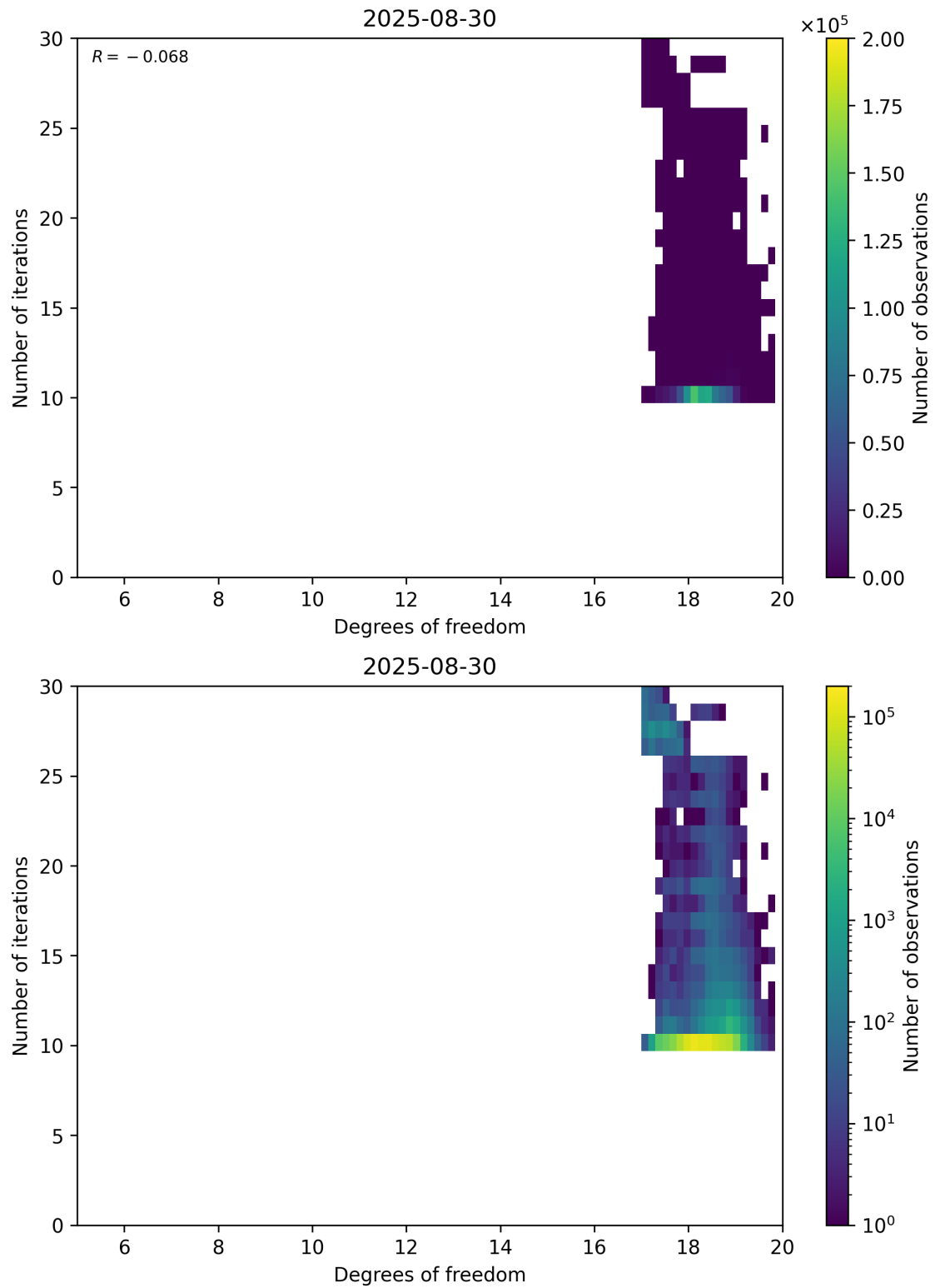
Figure 52: Scatter density plot of “Degrees of freedom” against “Number of iterations” for 2025-08-30 to 2025-08-31.
