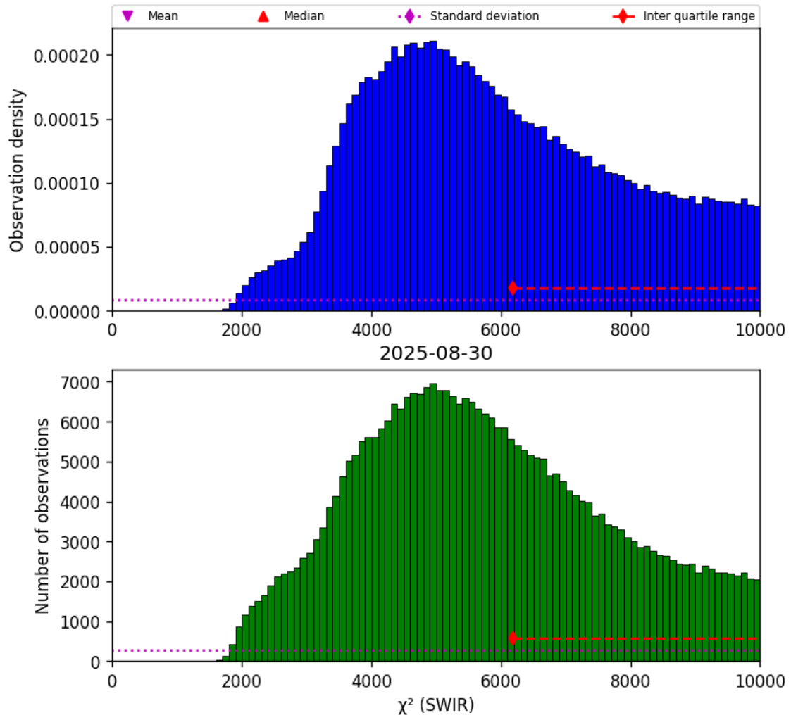
Figure 28: Histogram of " \chi^2 (SWIR)" for 2025-08-30 to 2025-08-31
