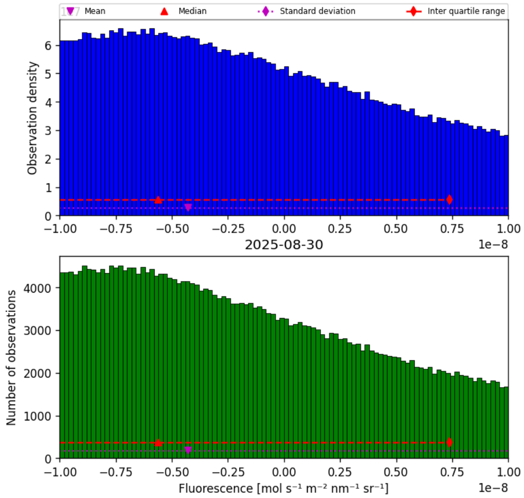
Figure 32: Histogram of “Fluorescence” for 2025-08-30 to 2025-08-31
