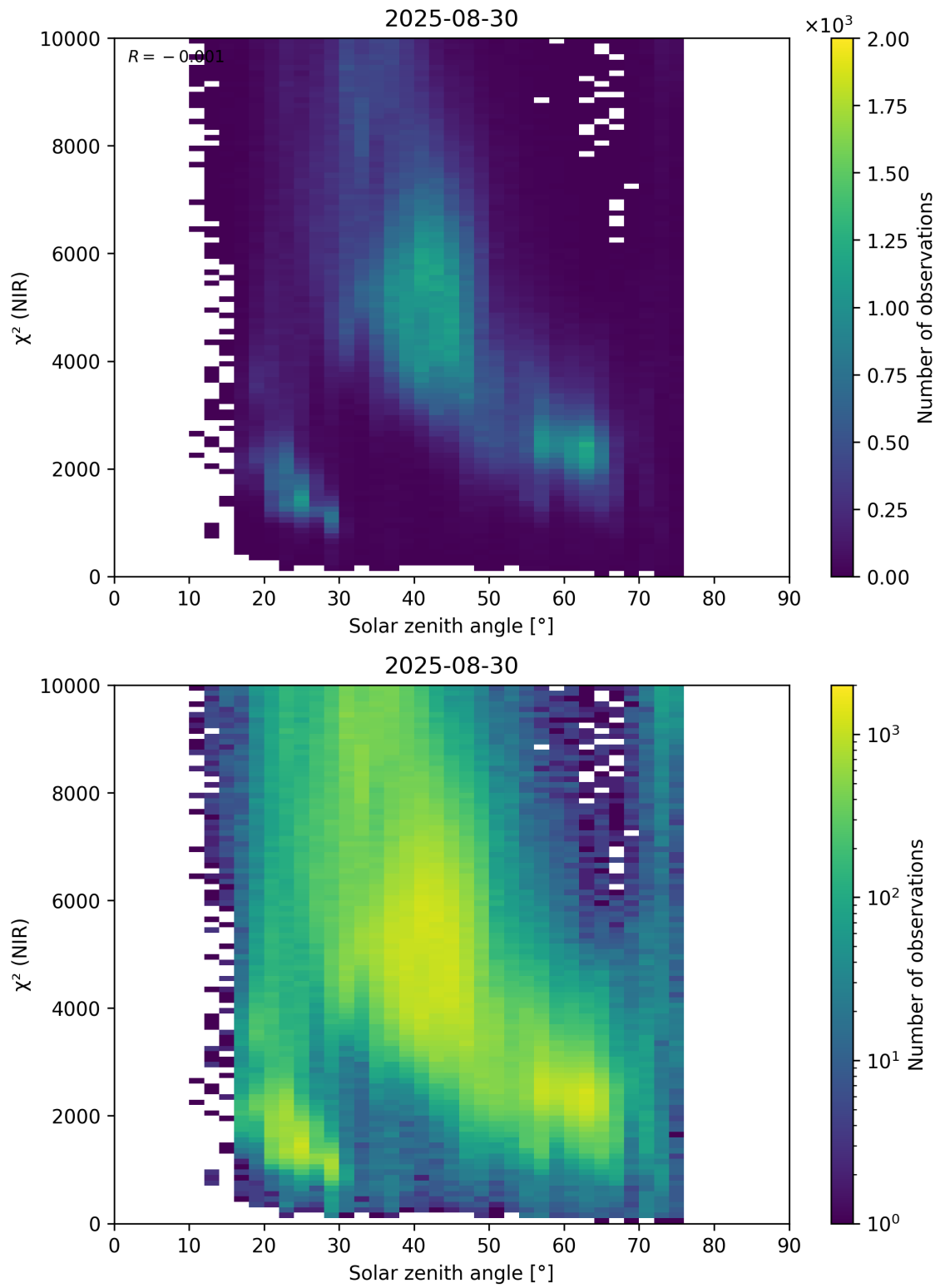
Figure 94: Scatter density plot of “Solar zenith angle” against “ \chi^2 (NIR)” for 2025-08-30 to 2025-08-31.
