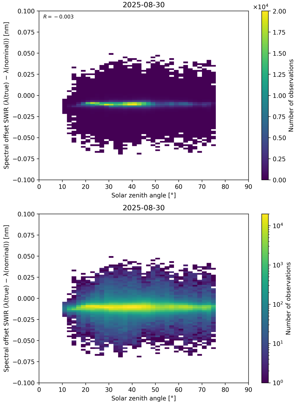
Figure 104: Scatter density plot of “Solar zenith angle” against “Spectral offset SWIR ( \lambda_{\text{true}} - \lambda_{\text{nominal}} )” for 2025-08-30 to 2025-08-31.
