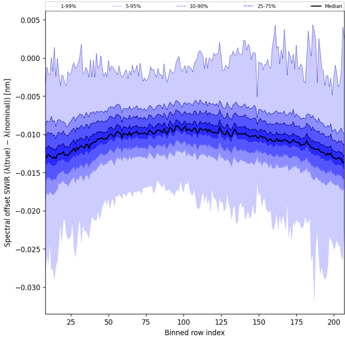
Figure 38: Along track statistics of “Spectral offset SWIR ( \lambda_{\text{true}} - \lambda_{\text{nominal}} )” for 2025-08-30 to 2025-08-31
