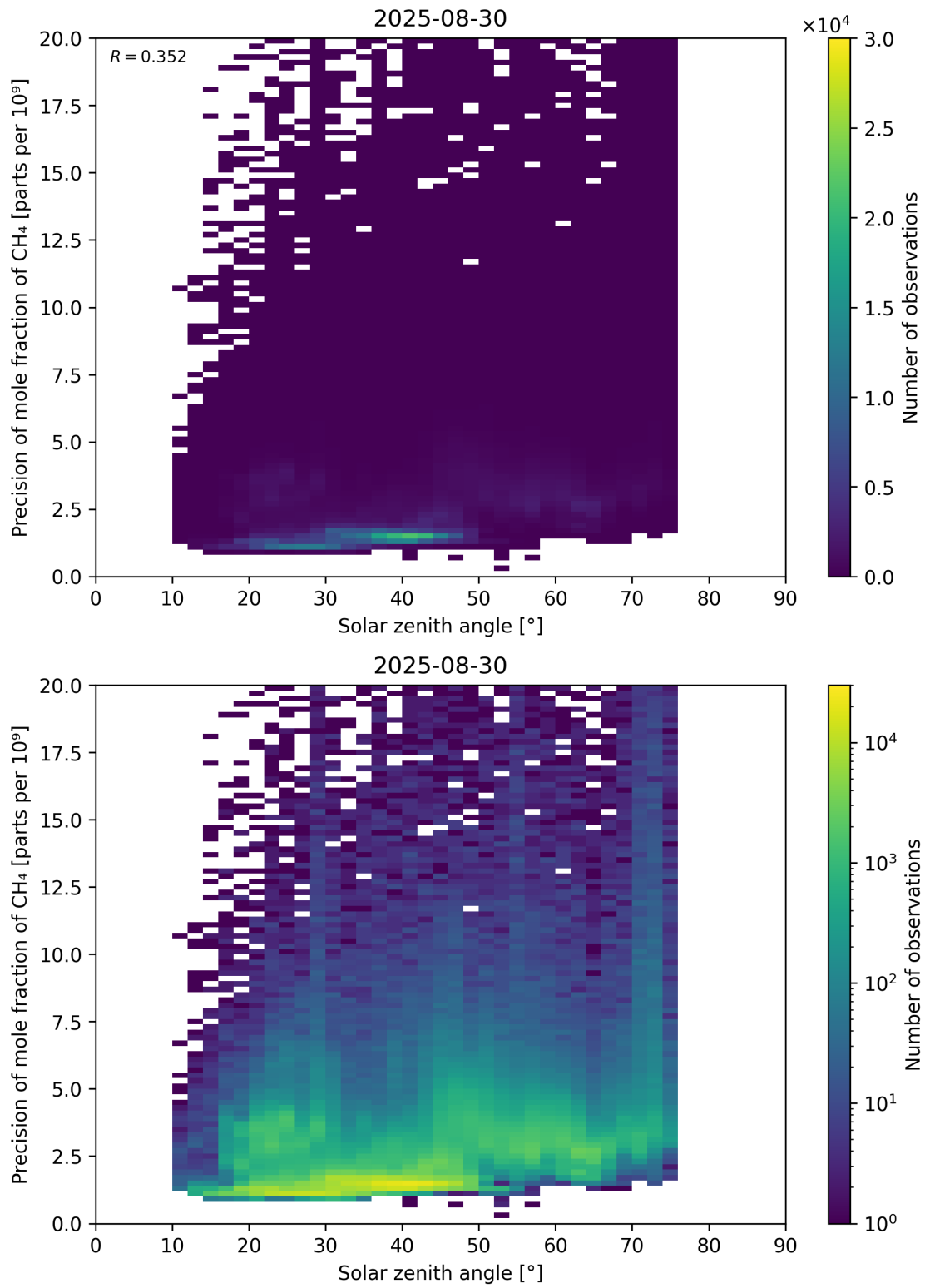
Figure 101: Scatter density plot of “Solar zenith angle” against “Precision of mole fraction of CH 4 ” for 2025-08-30 to 2025-08-31.
