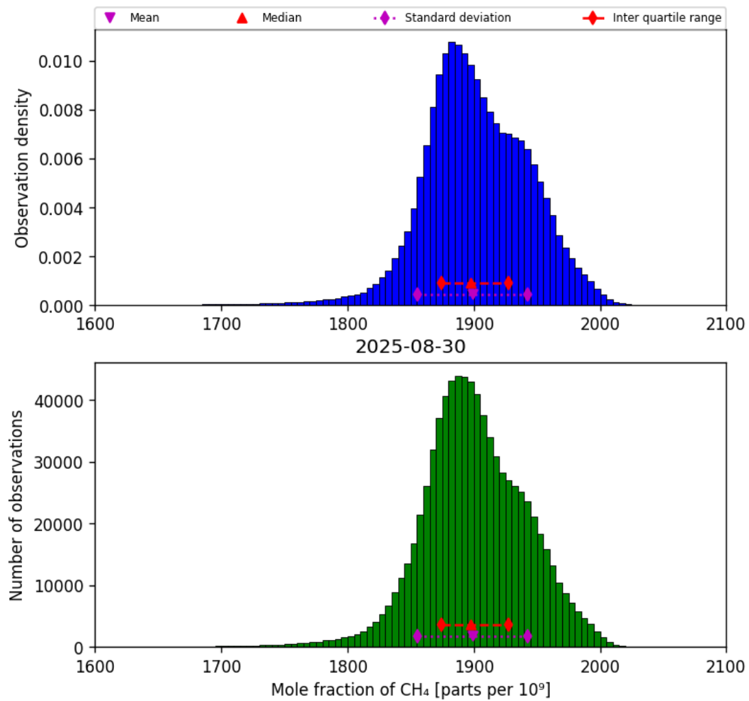
Figure 23: Histogram of “Mole fraction of CH 4 ” for 2025-08-30 to 2025-08-31
