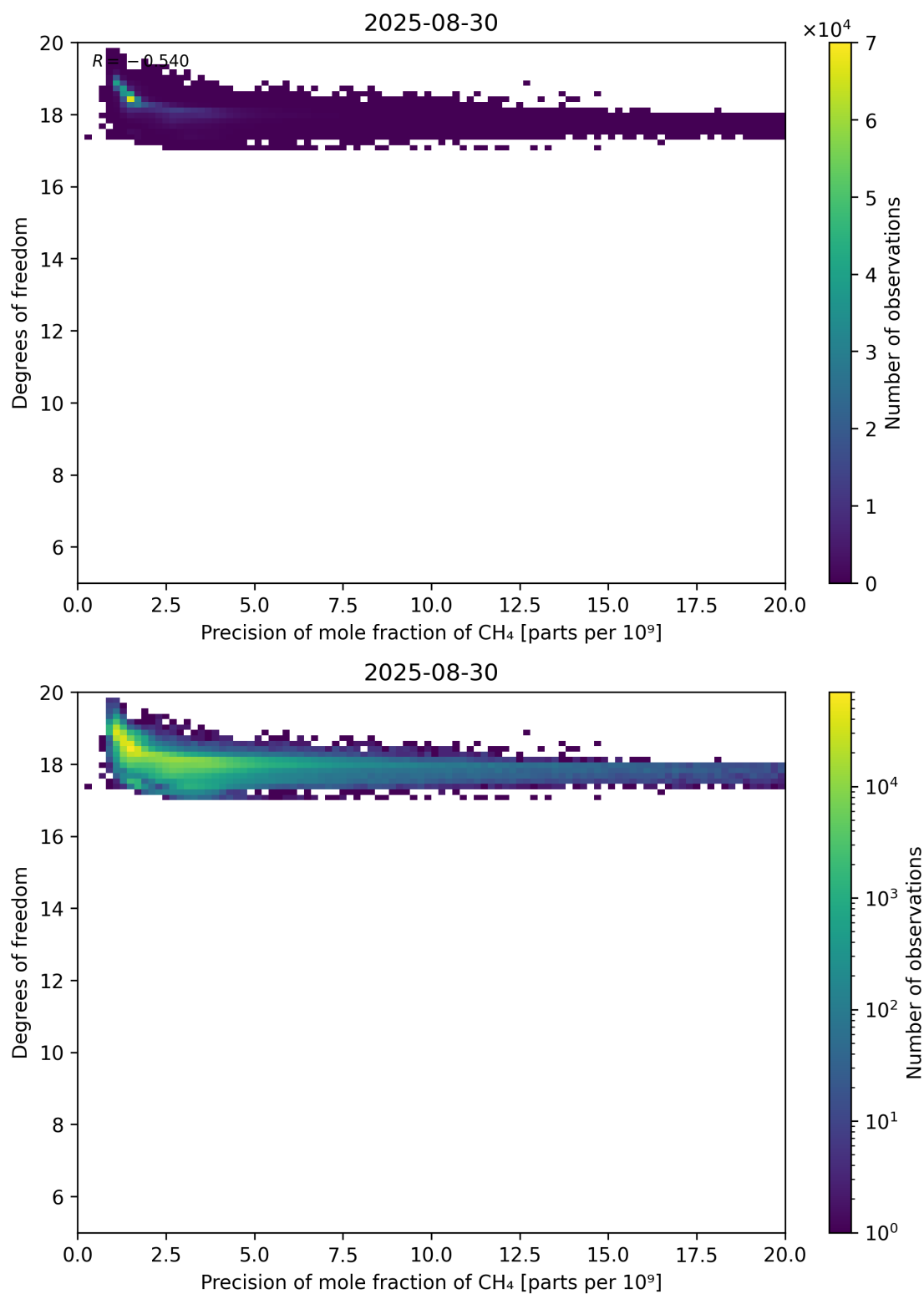
Figure 80: Scatter density plot of “Precision of mole fraction of CH 4 ” against “Degrees of freedom” for 2025-08-30 to 2025-08-31.
