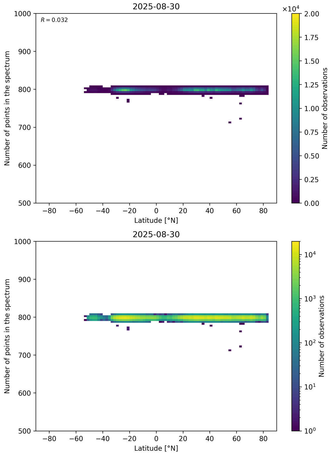
Figure 61: Scatter density plot of “Latitude” against “Number of points in the spectrum” for 2025-08-30 to 2025-08-31.
