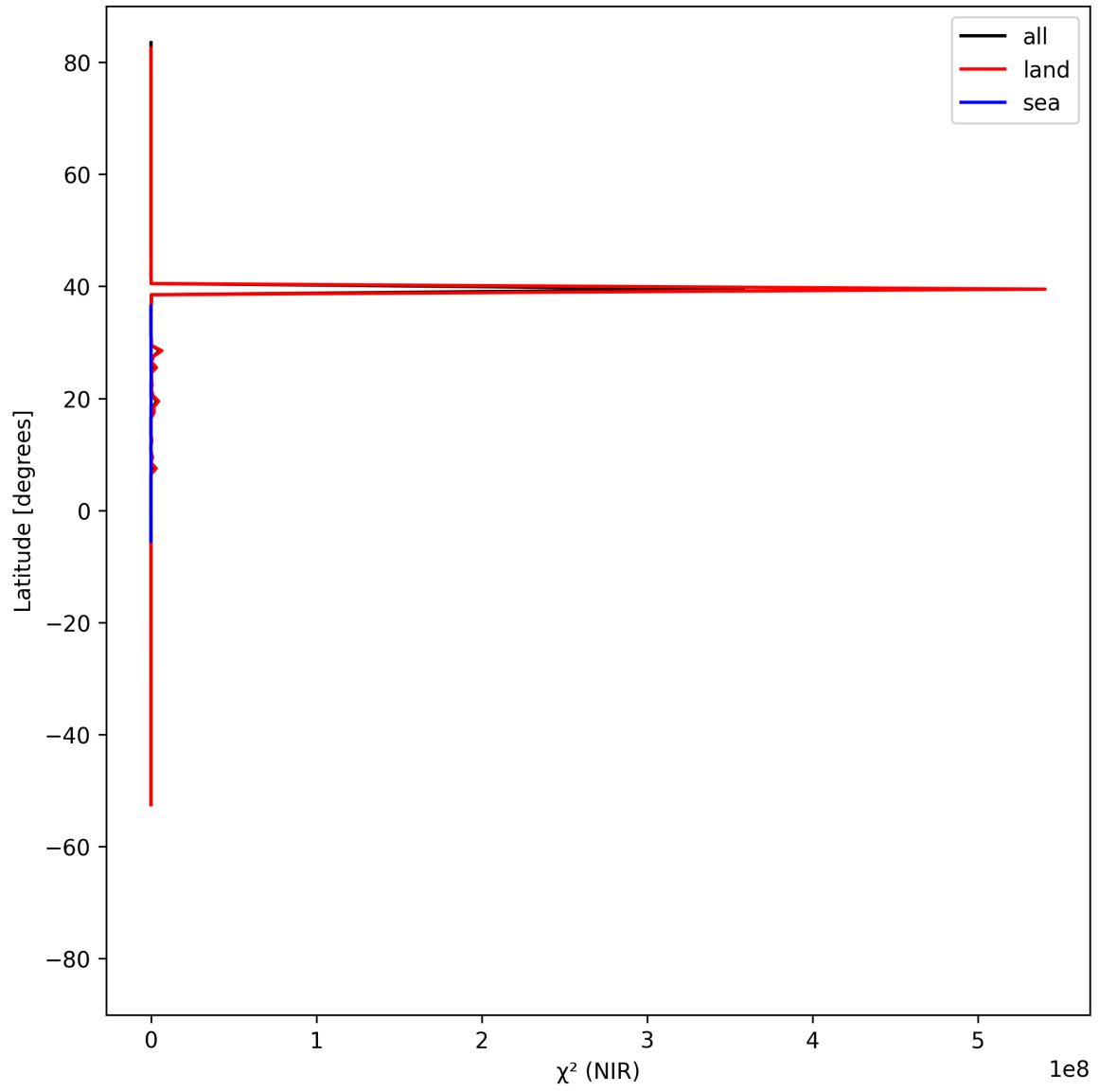
Figure 18: Zonal average of “ \chi^2 (NIR)” for 2025-08-30 to 2025-08-31.
