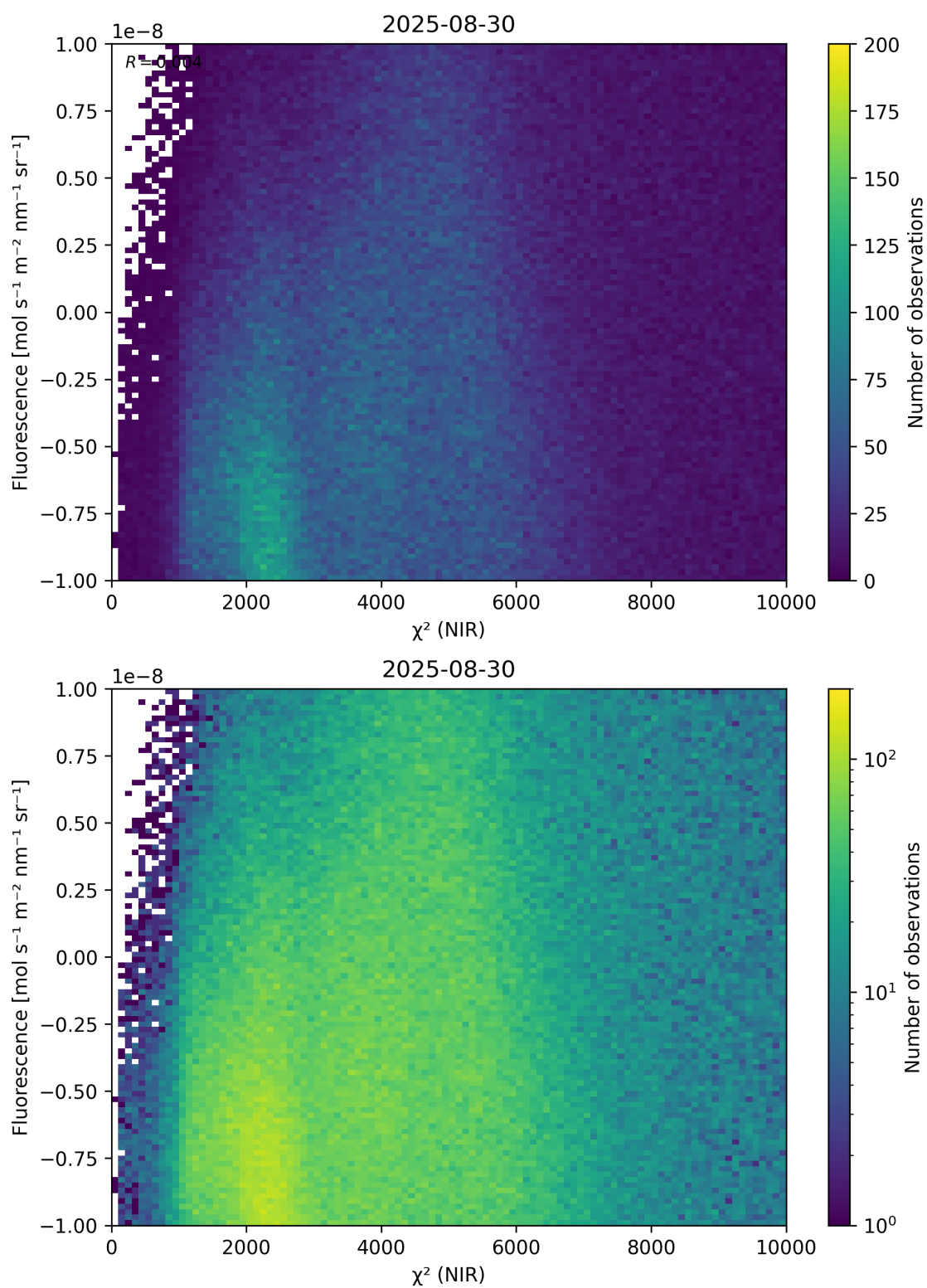
Figure 45: Scatter density plot of “ \chi^2 (NIR)” against “Fluorescence” for 2025-08-30 to 2025-08-31.
