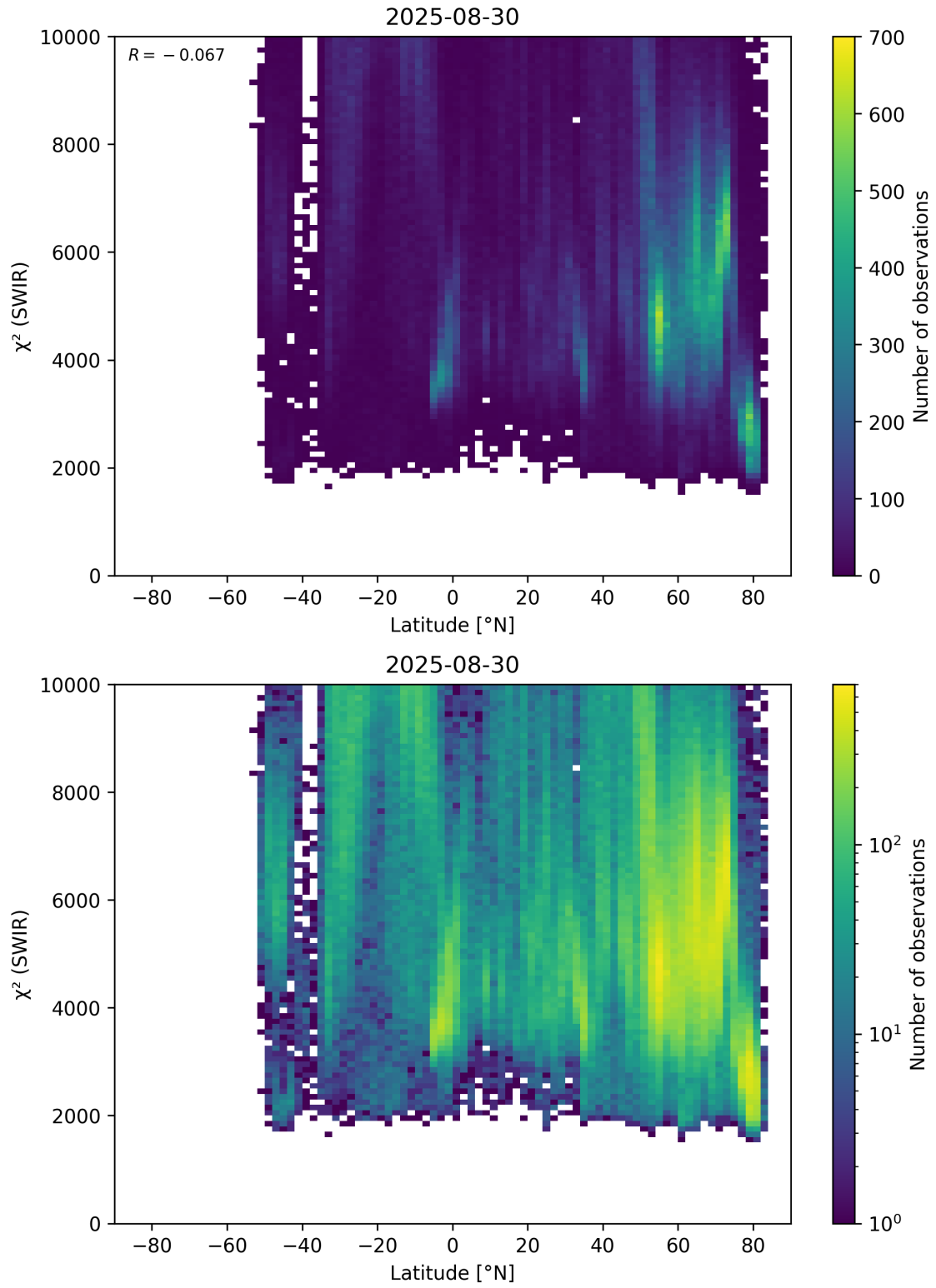
Figure 54: Scatter density plot of “Latitude” against “ \chi^2 (SWIR)” for 2025-08-30 to 2025-08-31.
