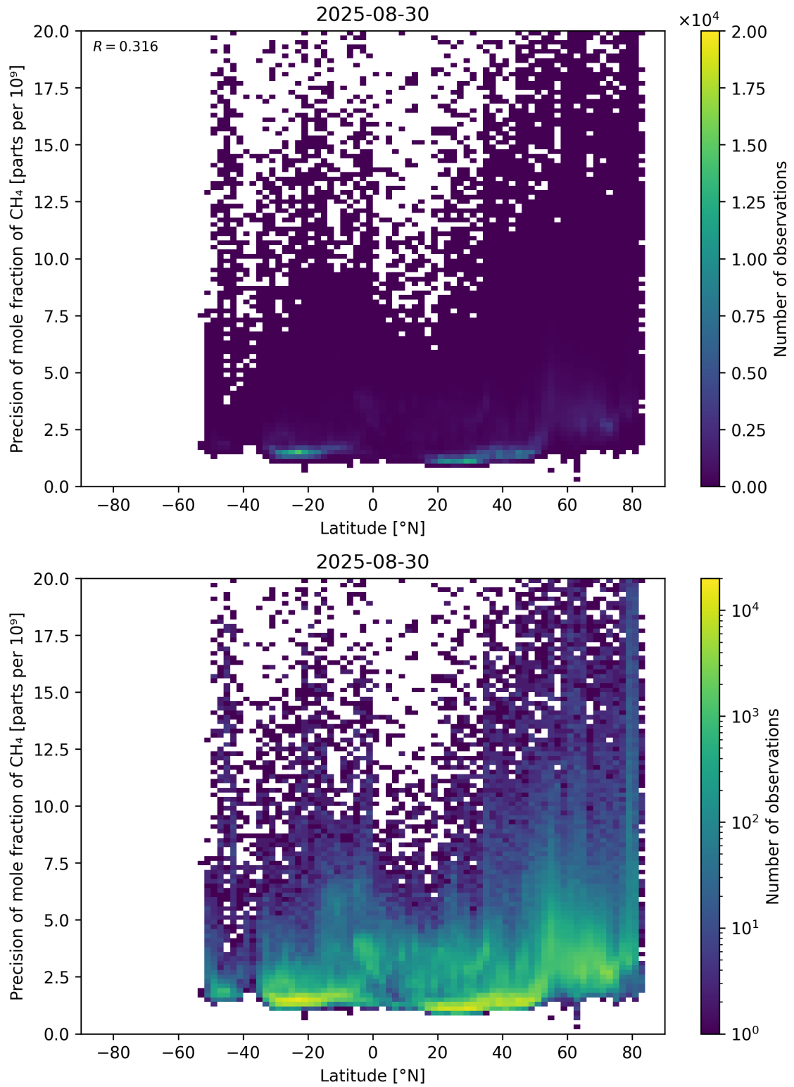
Figure 59: Scatter density plot of “Latitude” against “Precision of mole fraction of \text{CH}_4 ” for 2025-08-30 to 2025-08-31.
