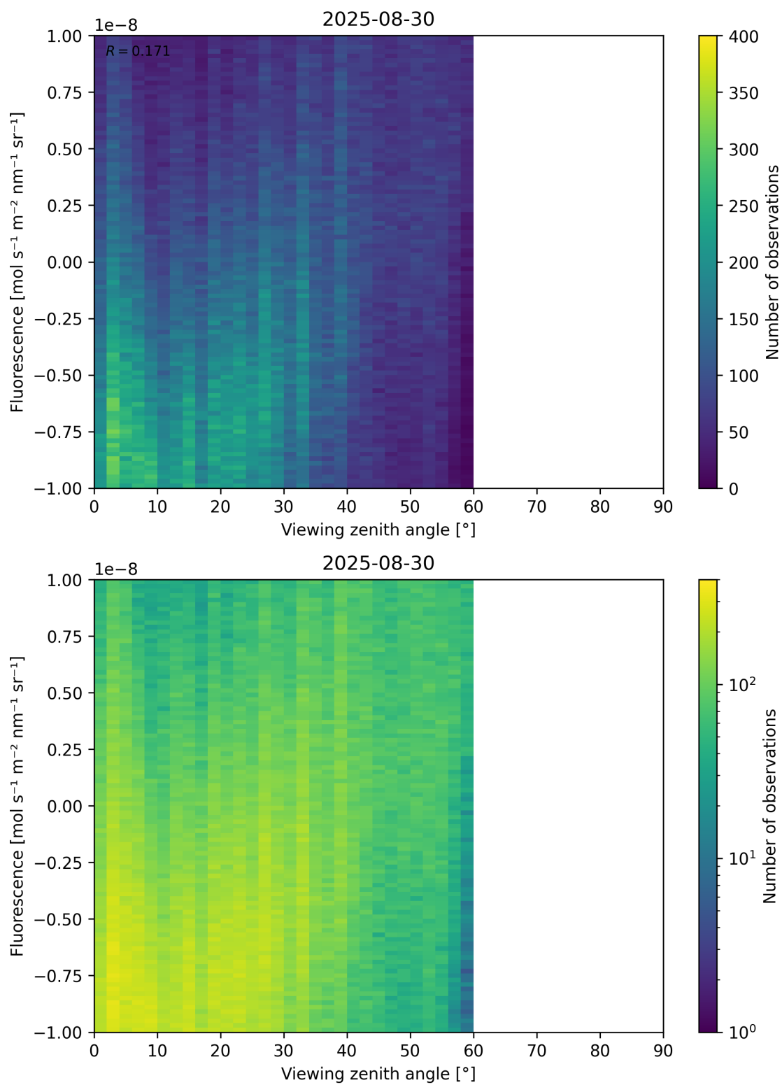
Figure 108: Scatter density plot of “Viewing zenith angle” against “Fluorescence” for 2025-08-30 to 2025-08-31.
