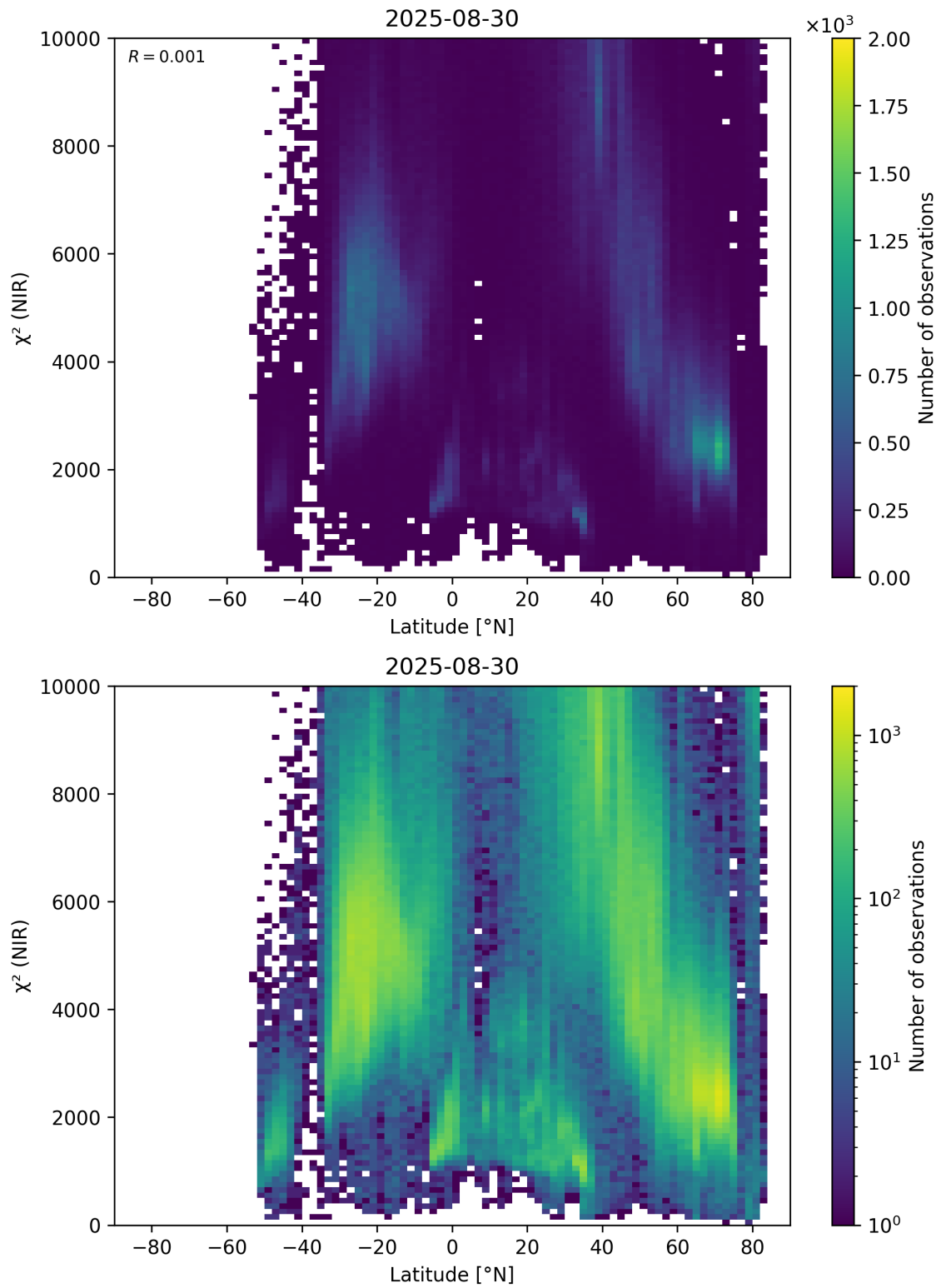
Figure 53: Scatter density plot of “Latitude” against “ \chi^2 (NIR)” for 2025-08-30 to 2025-08-31.
