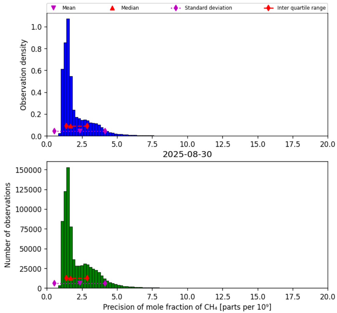
Figure 24: Histogram of “Precision of mole fraction of CH 4 ” for 2025-08-30 to 2025-08-31
