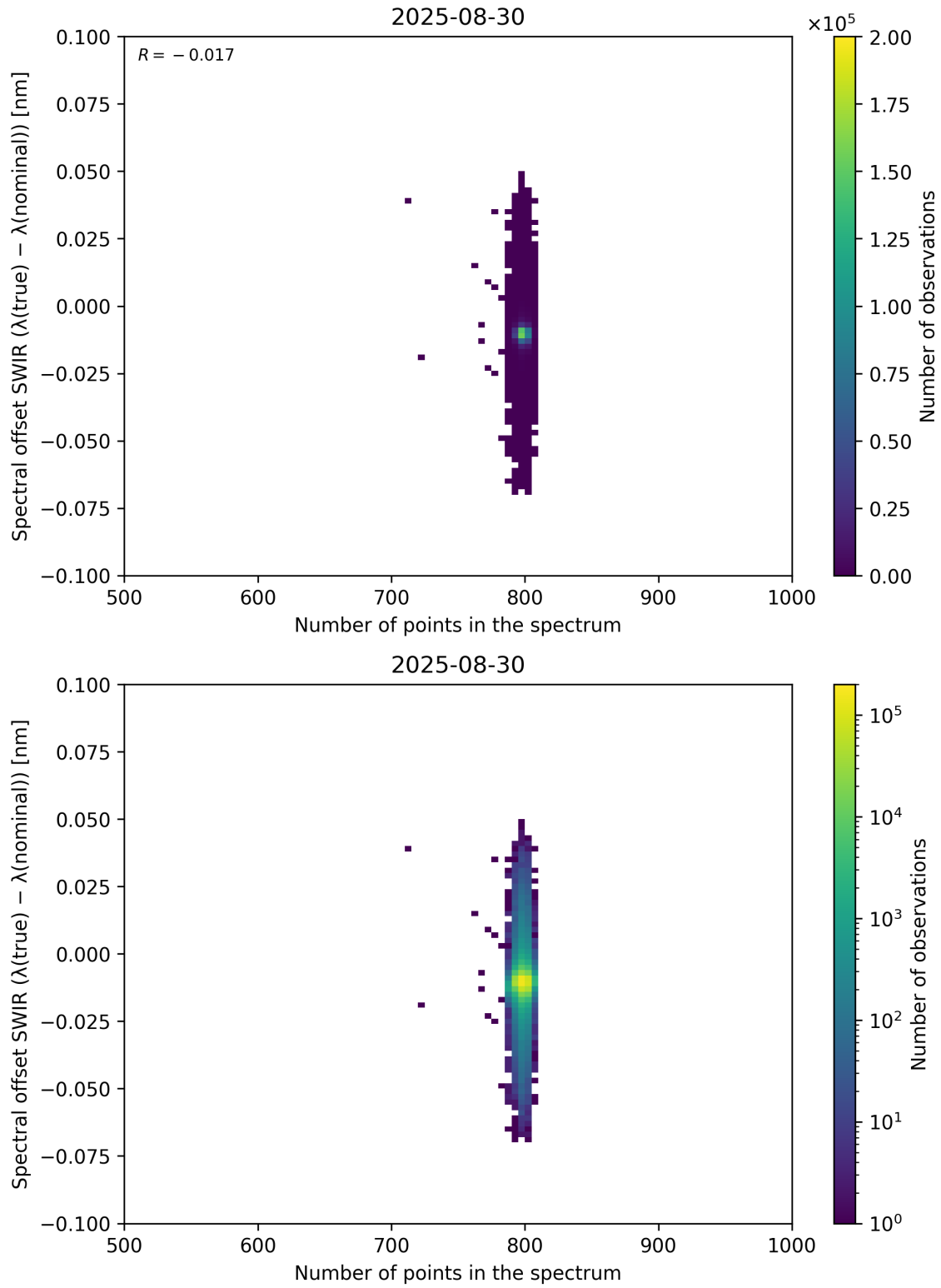
Figure 93: Scatter density plot of “Number of points in the spectrum” against “Spectral offset SWIR ( \lambda_{\text{true}} - \lambda_{\text{nominal}} )” for 2025-08-30 to 2025-08-31.
