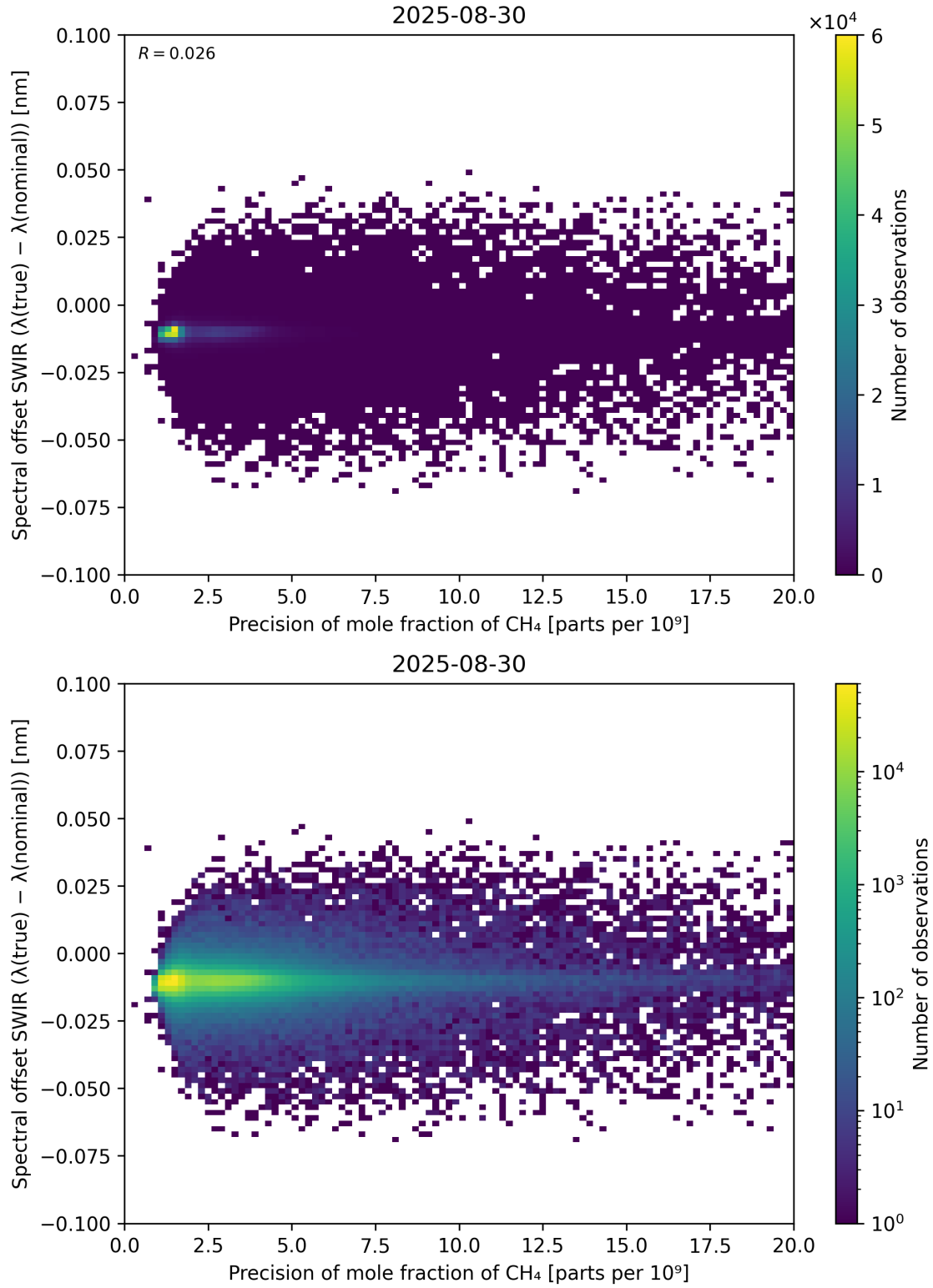
Figure 85: Scatter density plot of “Precision of mole fraction of CH 4 ” against “Spectral offset SWIR ( \lambda_{\text{true}} - \lambda_{\text{nominal}} )” for 2025-08-30 to 2025-08-31.
