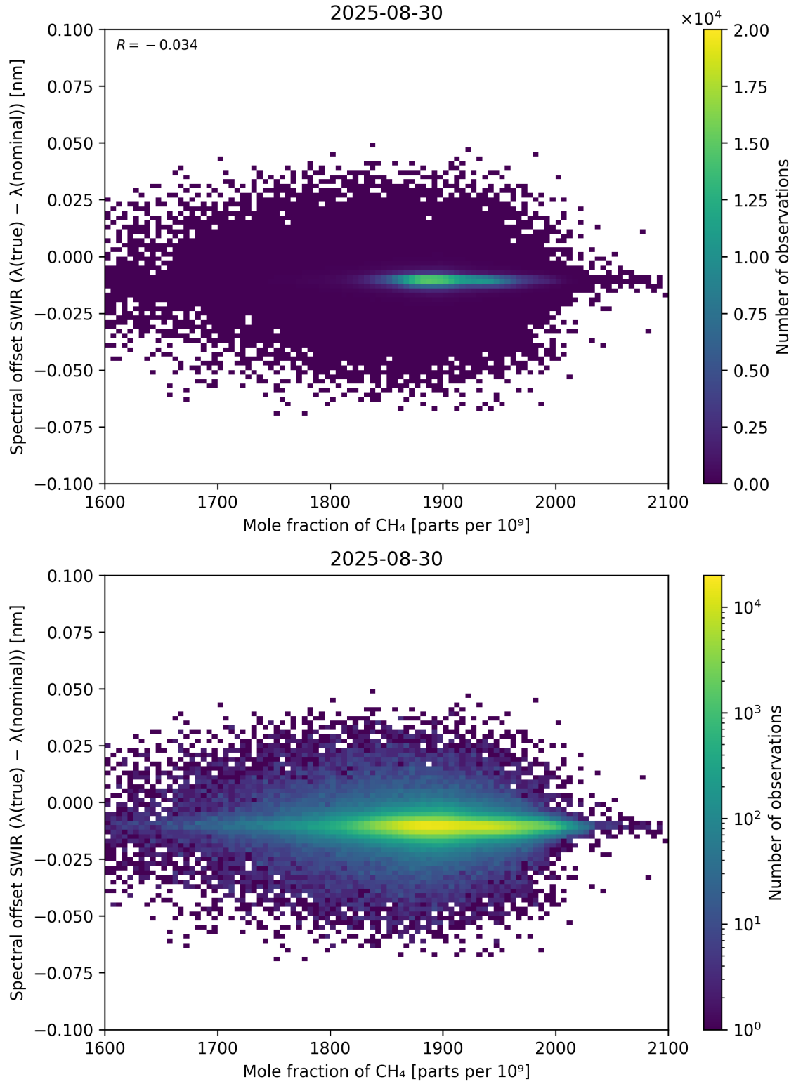
Figure 86: Scatter density plot of “Mole fraction of \text{CH}_4 ” against “Spectral offset SWIR ( \lambda_{\text{true}} - \lambda_{\text{nominal}} )” for 2025-08-30 to 2025-08-31.
