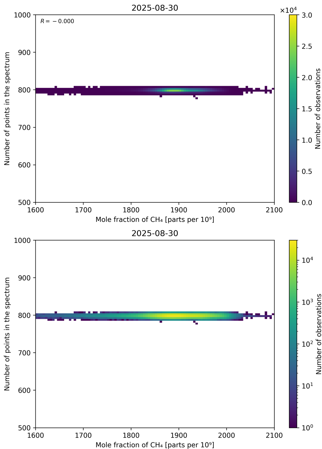
Figure 77: Scatter density plot of “Mole fraction of CH 4 ” against “Number of points in the spectrum” for 2025-08-30 to 2025-08-31.
