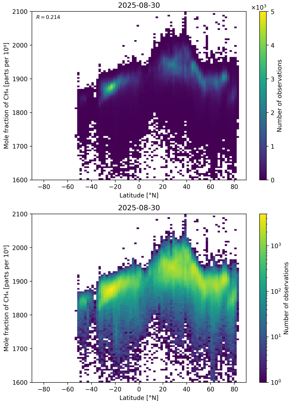
Figure 57: Scatter density plot of “Latitude” against “Mole fraction of \text{CH}_4 ” for 2025-08-30 to 2025-08-31.
