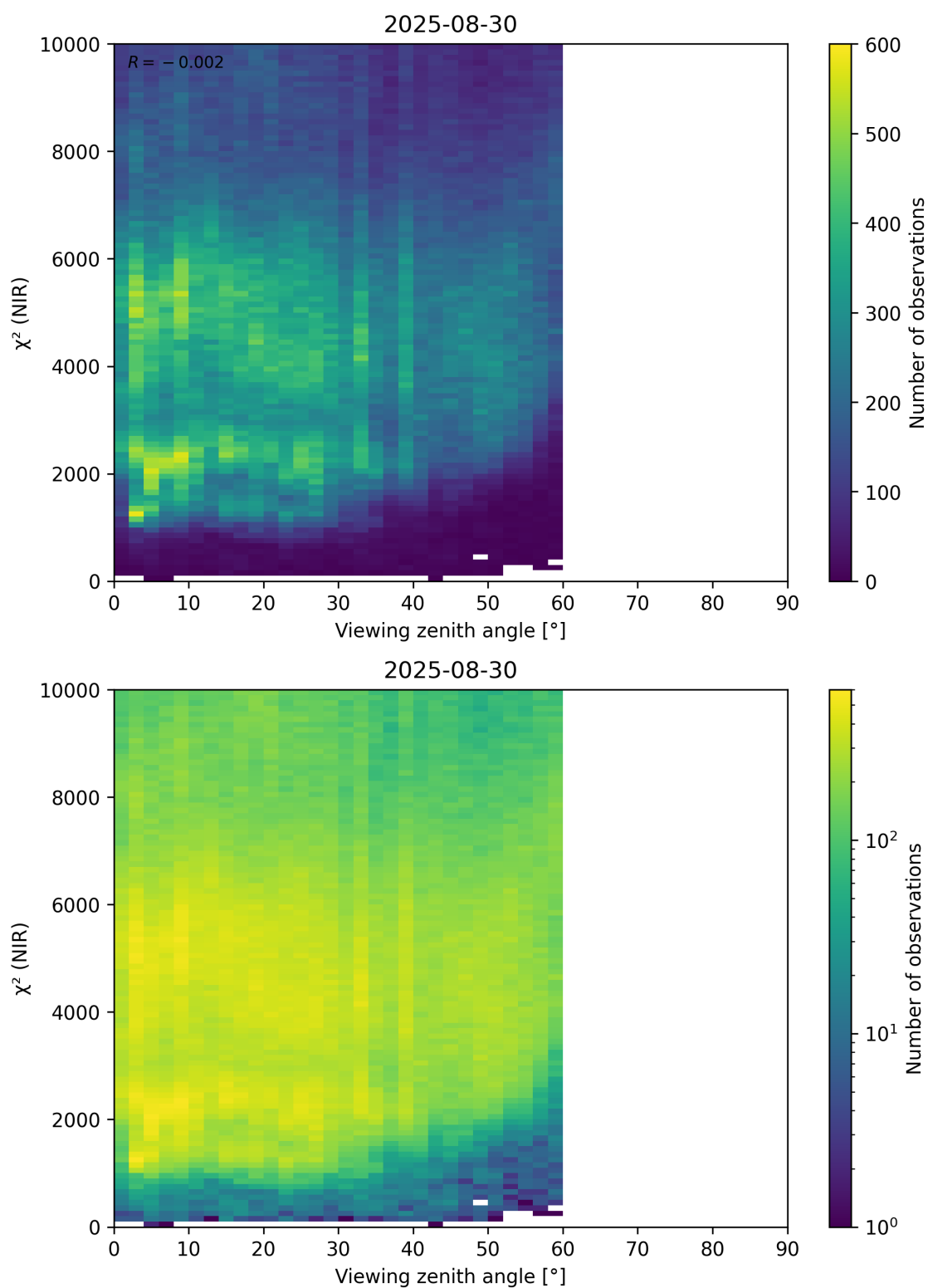
Figure 105: Scatter density plot of “Viewing zenith angle” against “ \chi^2 (NIR)” for 2025-08-30 to 2025-08-31.
