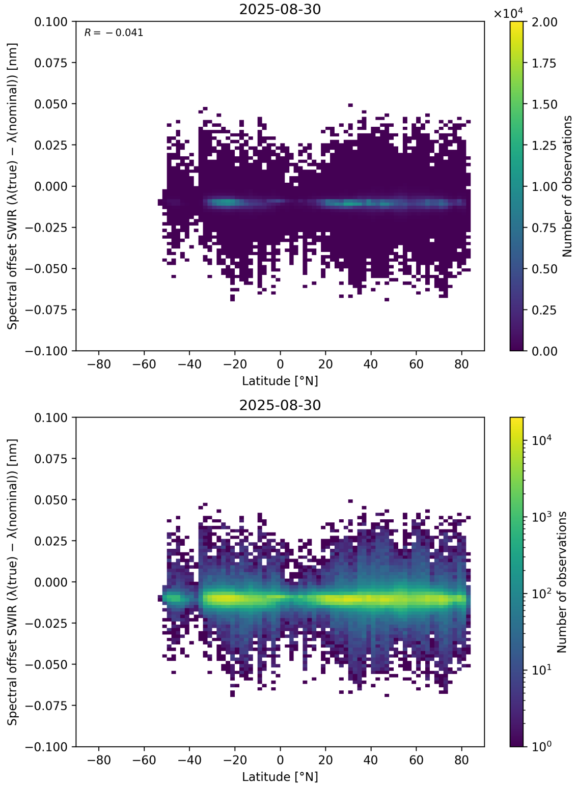
Figure 62: Scatter density plot of “Latitude” against “Spectral offset SWIR ( \lambda_{\text{true}} - \lambda_{\text{nominal}} )” for 2025-08-30 to 2025-08-31.
