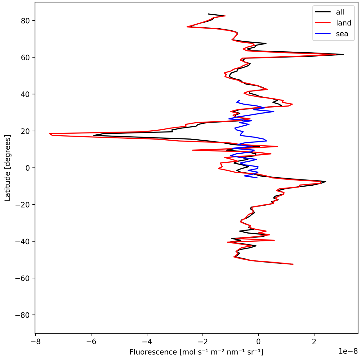
Figure 21: Zonal average of “Fluorescence” for 2025-08-30 to 2025-08-31.
