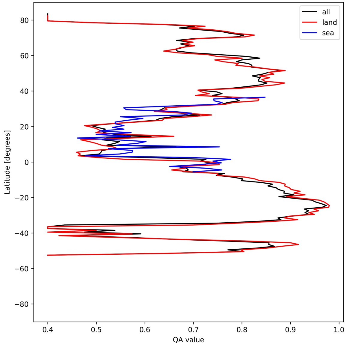
Figure 11: Zonal average of “QA value” for 2025-08-30 to 2025-08-31.
