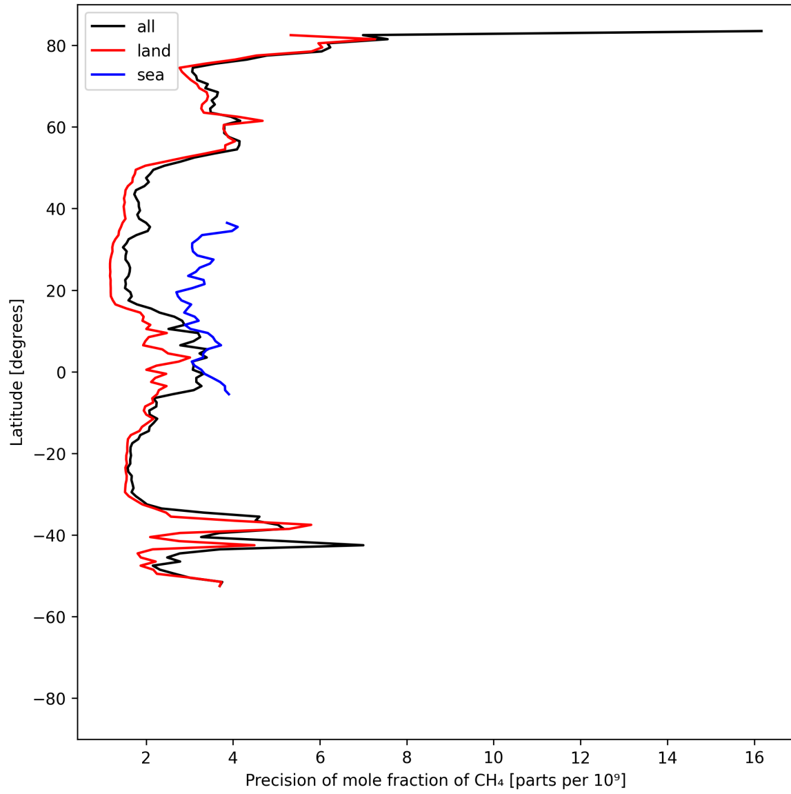
Figure 13: Zonal average of “Precision of mole fraction of CH 4 ” for 2025-08-30 to 2025-08-31.
