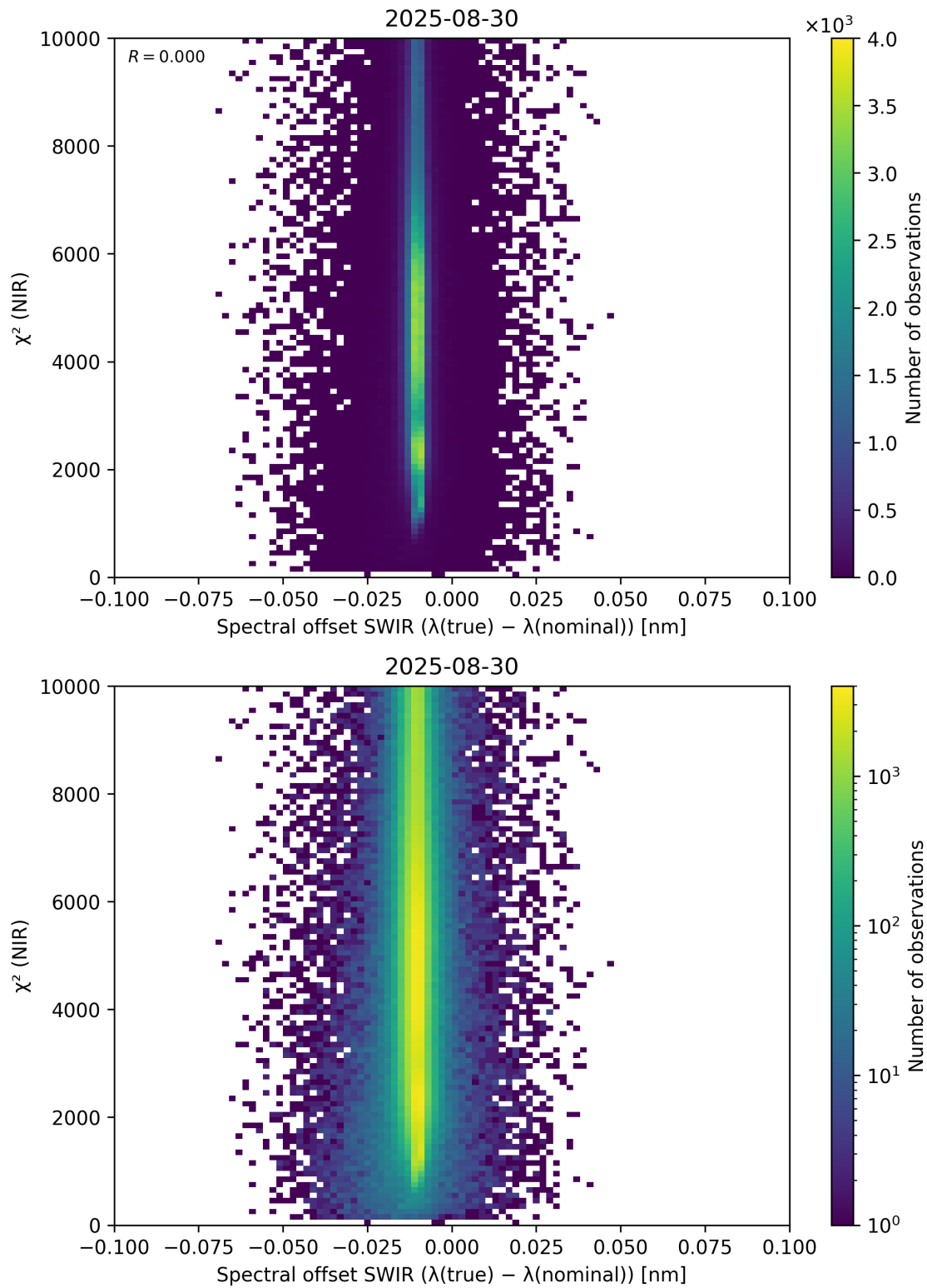
Figure 117: Scatter density plot of “Spectral offset SWIR ( \lambda_{\text{true}} - \lambda_{\text{nominal}} )” against “ \chi^2 (NIR)” for 2025-08-30 to 2025-08-31.
