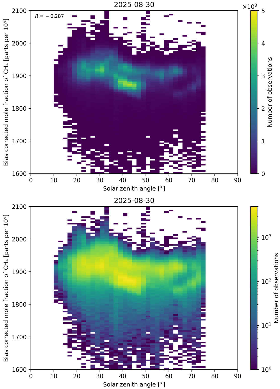
Figure 100: Scatter density plot of “Solar zenith angle” against “Bias corrected mole fraction of \text{CH}_4 ” for 2025-08-30 to 2025-08-31.
