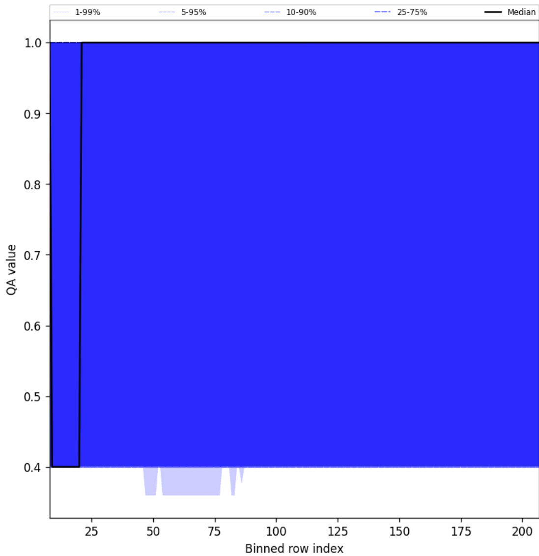
Figure 33: Along track statistics of “QA value” for 2025-08-30 to 2025-08-31
