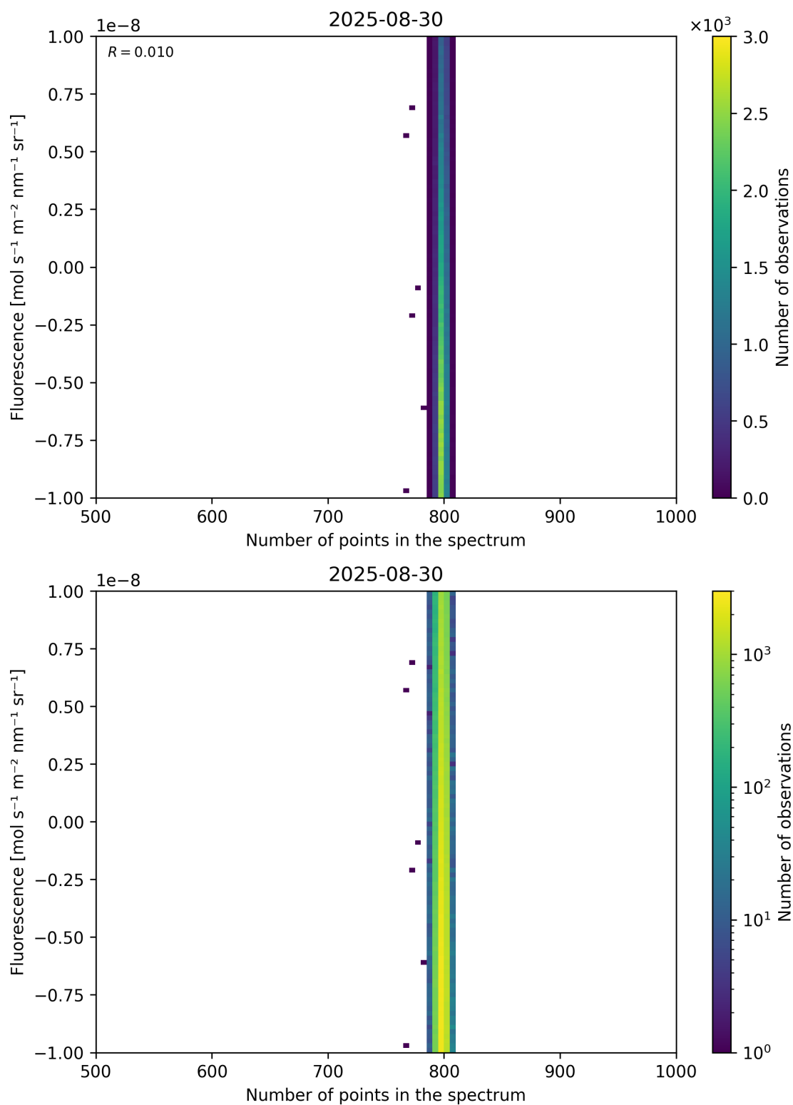
Figure 91: Scatter density plot of “Number of points in the spectrum” against “Fluorescence” for 2025-08-30 to 2025-08-31.
