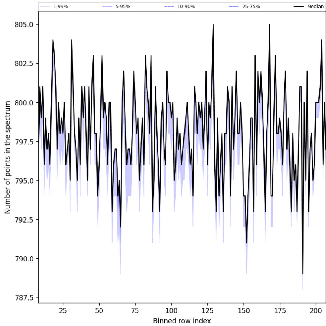
Figure 37: Along track statistics of “Number of points in the spectrum” for 2025-08-30 to 2025-08-31
