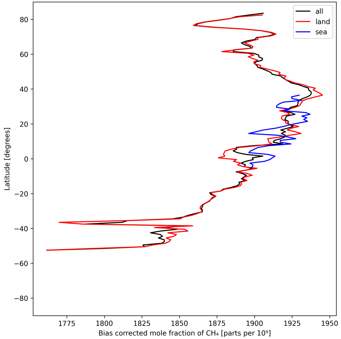
Figure 14: Zonal average of “Bias corrected mole fraction of CH 4 ” for 2025-08-30 to 2025-08-31.
