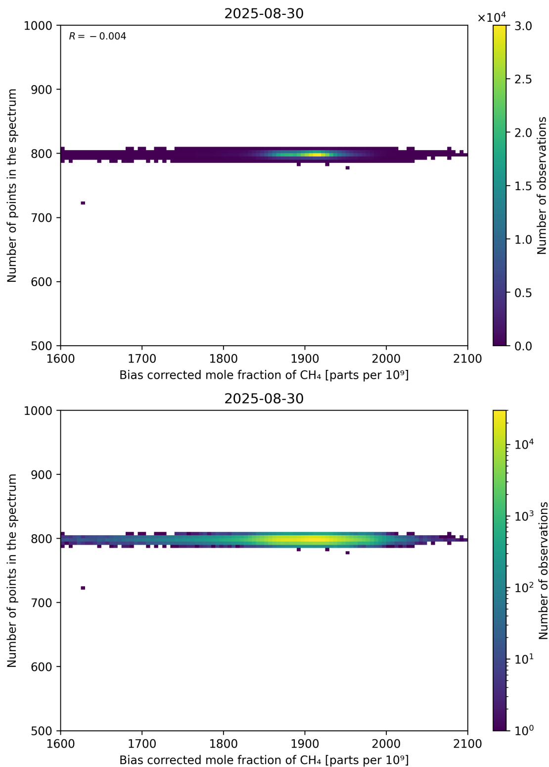
Figure 68: Scatter density plot of “Bias corrected mole fraction of CH 4 ” against “Number of points in the spectrum” for 2025-08-30 to 2025-08-31.
