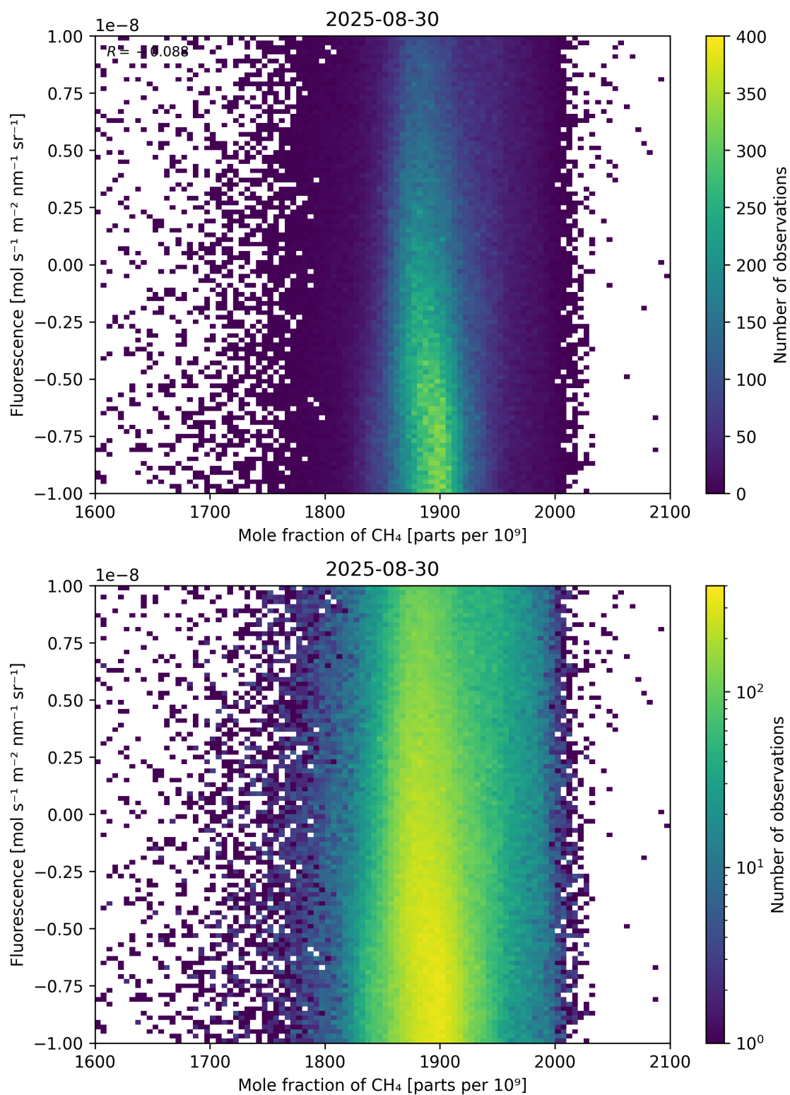
Figure 73: Scatter density plot of “Mole fraction of \text{CH}_4 ” against “Fluorescence” for 2025-08-30 to 2025-08-31.
