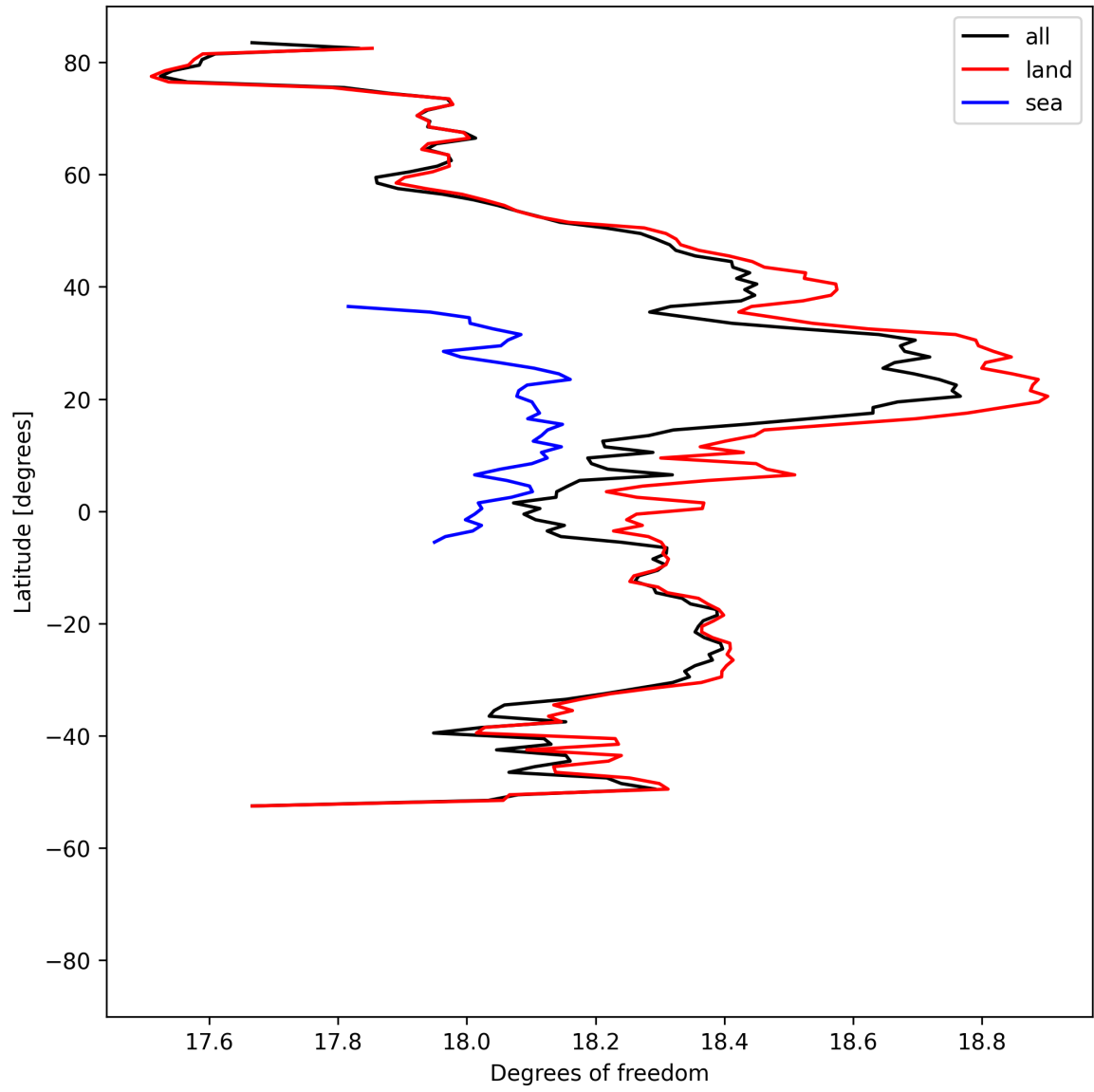
Figure 19: Zonal average of “Degrees of freedom” for 2025-08-30 to 2025-08-31.
