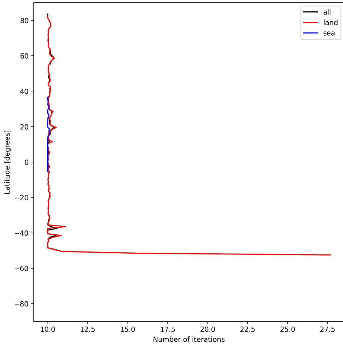
Figure 20: Zonal average of “Number of iterations” for 2025-08-30 to 2025-08-31.
