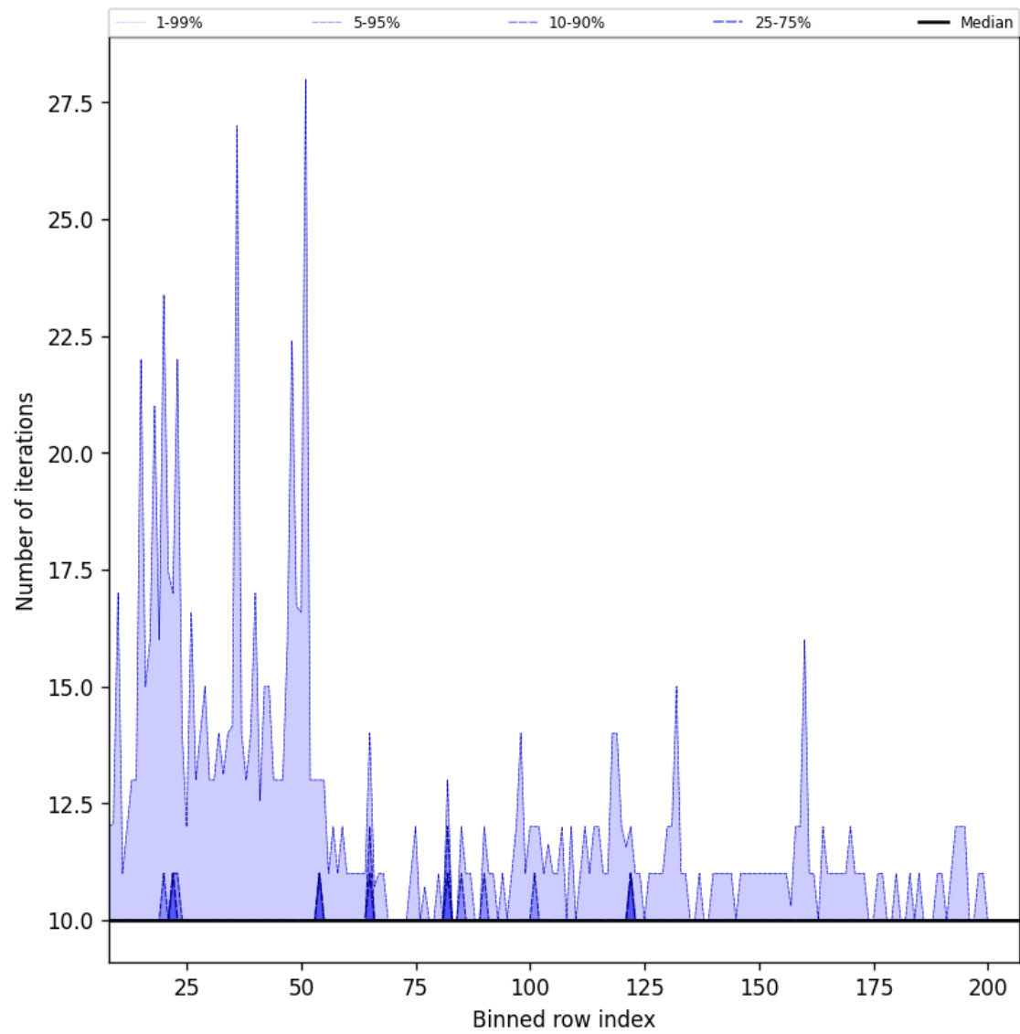
Figure 42: Along track statistics of “Number of iterations” for 2025-08-30 to 2025-08-31
