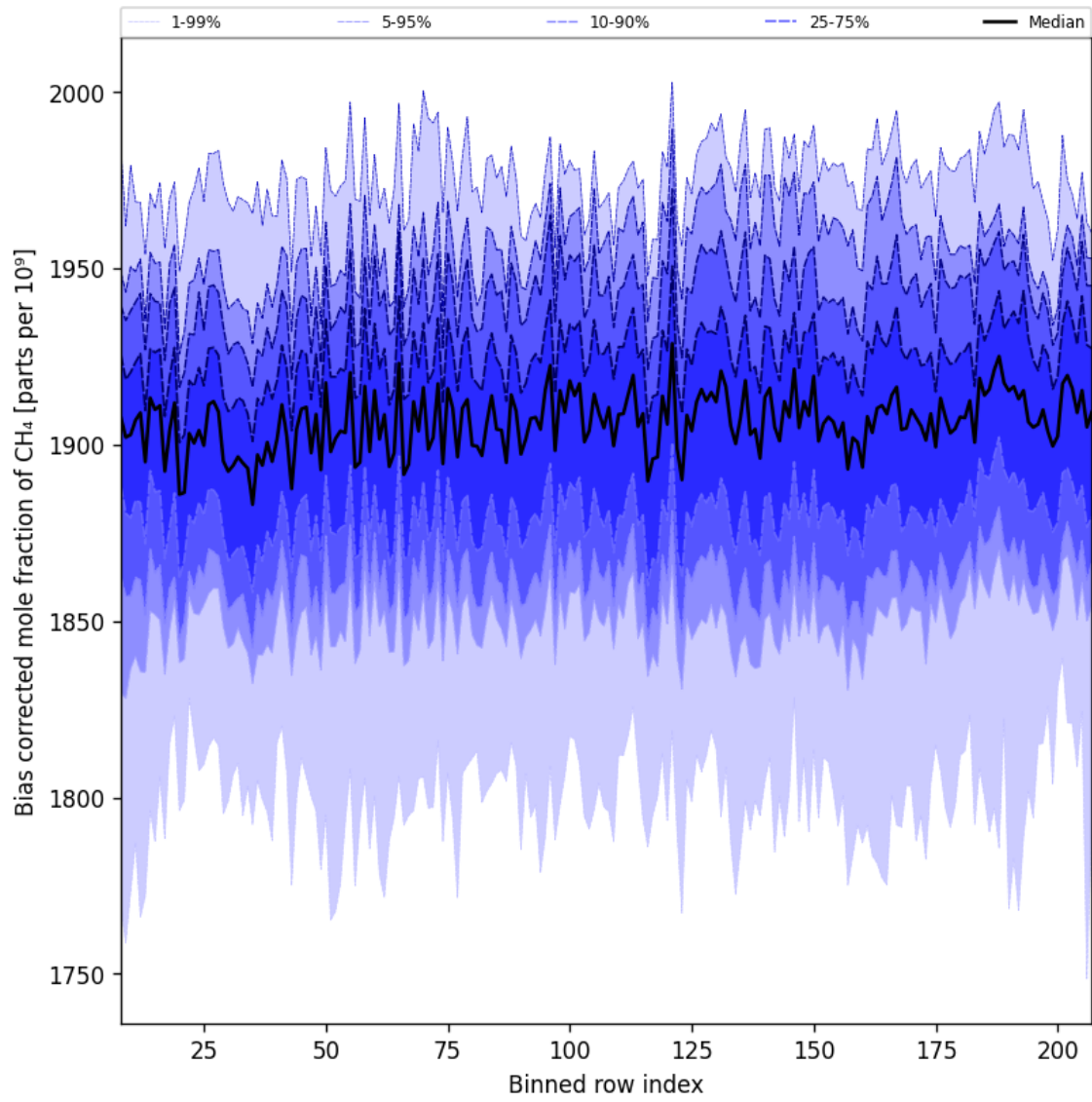
Figure 36: Along track statistics of “Bias corrected mole fraction of CH 4 ” for 2025-08-30 to 2025-08-31
