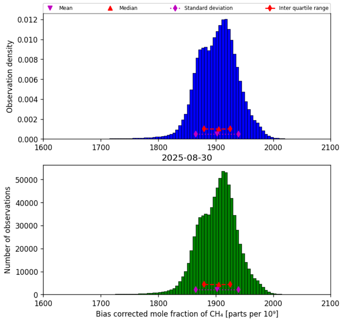
Figure 25: Histogram of “Bias corrected mole fraction of CH 4 ” for 2025-08-30 to 2025-08-31
