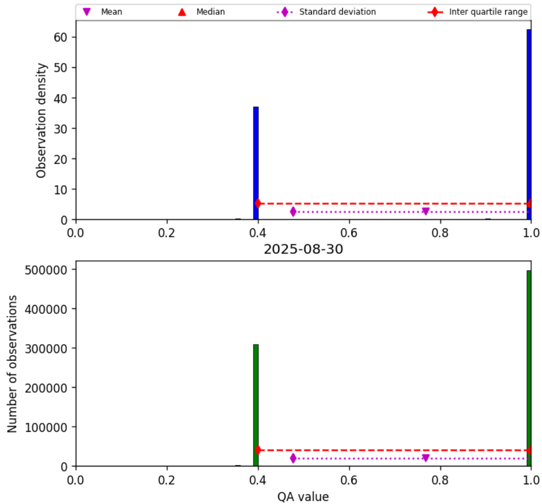
Figure 22: Histogram of “QA value” for 2025-08-30 to 2025-08-31
