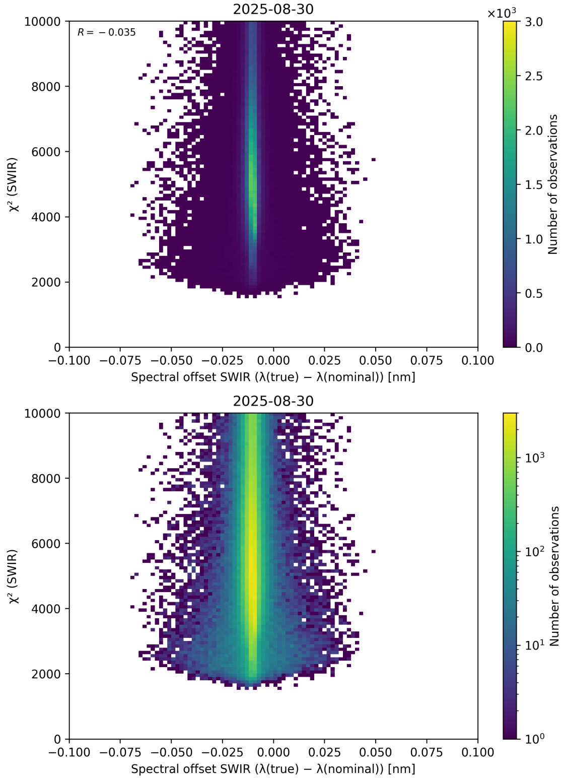
Figure 118: Scatter density plot of “Spectral offset SWIR ( \lambda_{\text{true}} - \lambda_{\text{nominal}} )” against “ \chi^2 (SWIR)” for 2025-08-30 to 2025-08-31.
