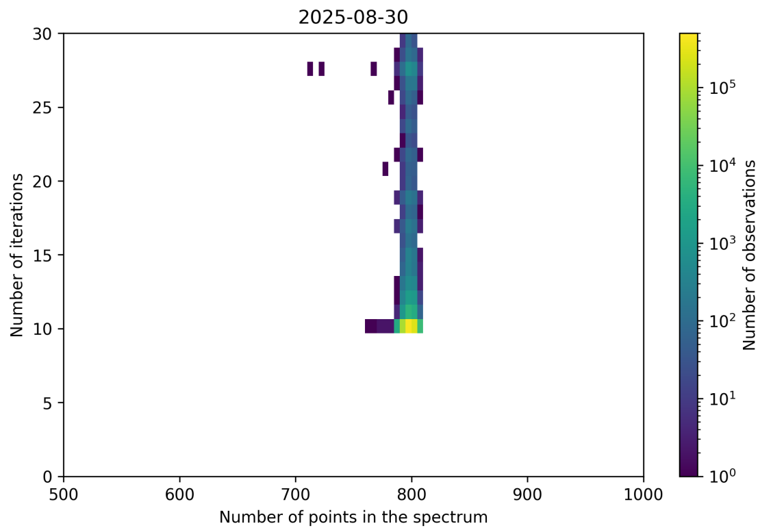
Figure 92: Scatter density plot of “Number of points in the spectrum” against “Number of iterations” for 2025-08-30 to 2025-08-31.
