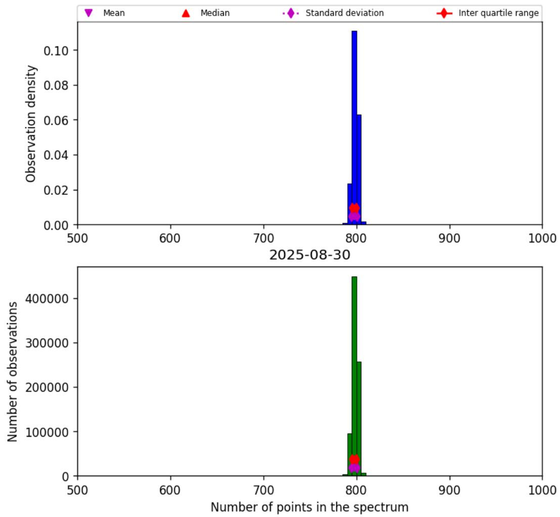
Figure 26: Histogram of “Number of points in the spectrum” for 2025-08-30 to 2025-08-31
