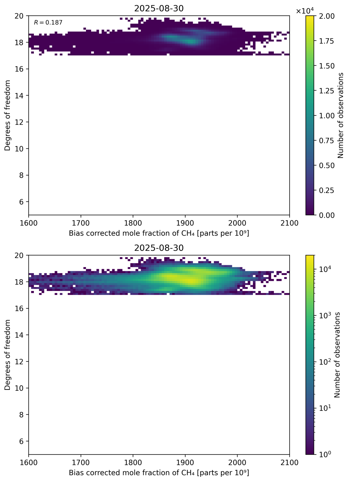
Figure 65: Scatter density plot of “Bias corrected mole fraction of CH 4 ” against “Degrees of freedom” for 2025-08-30 to 2025-08-31.
