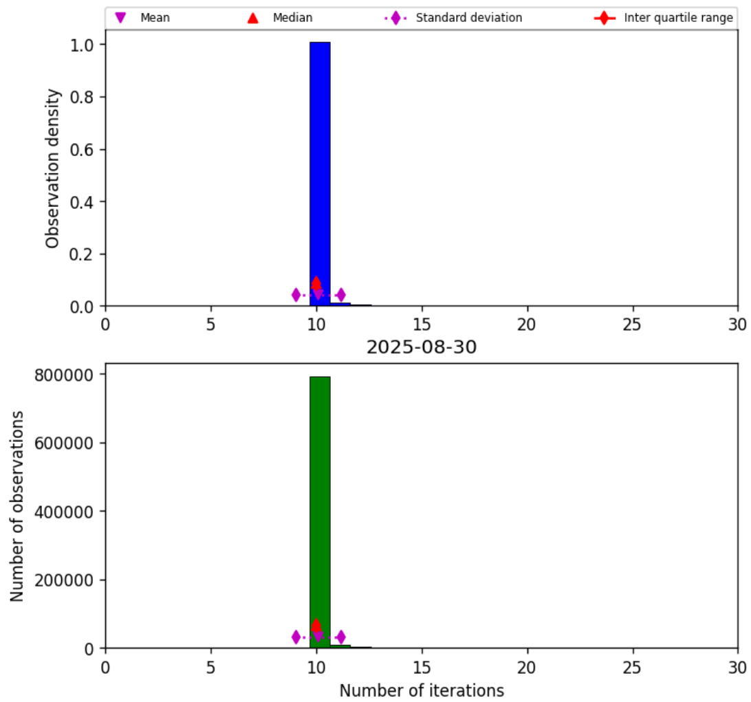
Figure 31: Histogram of “Number of iterations” for 2025-08-30 to 2025-08-31
