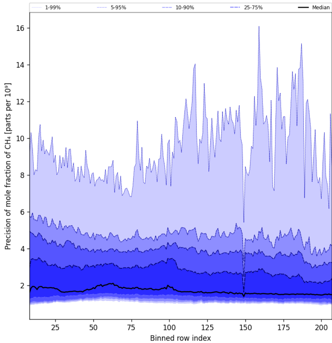
Figure 35: Along track statistics of “Precision of mole fraction of CH 4 ” for 2025-08-30 to 2025-08-31
