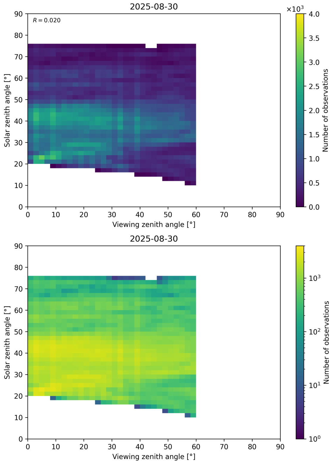
Figure 115: Scatter density plot of “Viewing zenith angle” against “Solar zenith angle” for 2025-08-30 to 2025-08-31.
