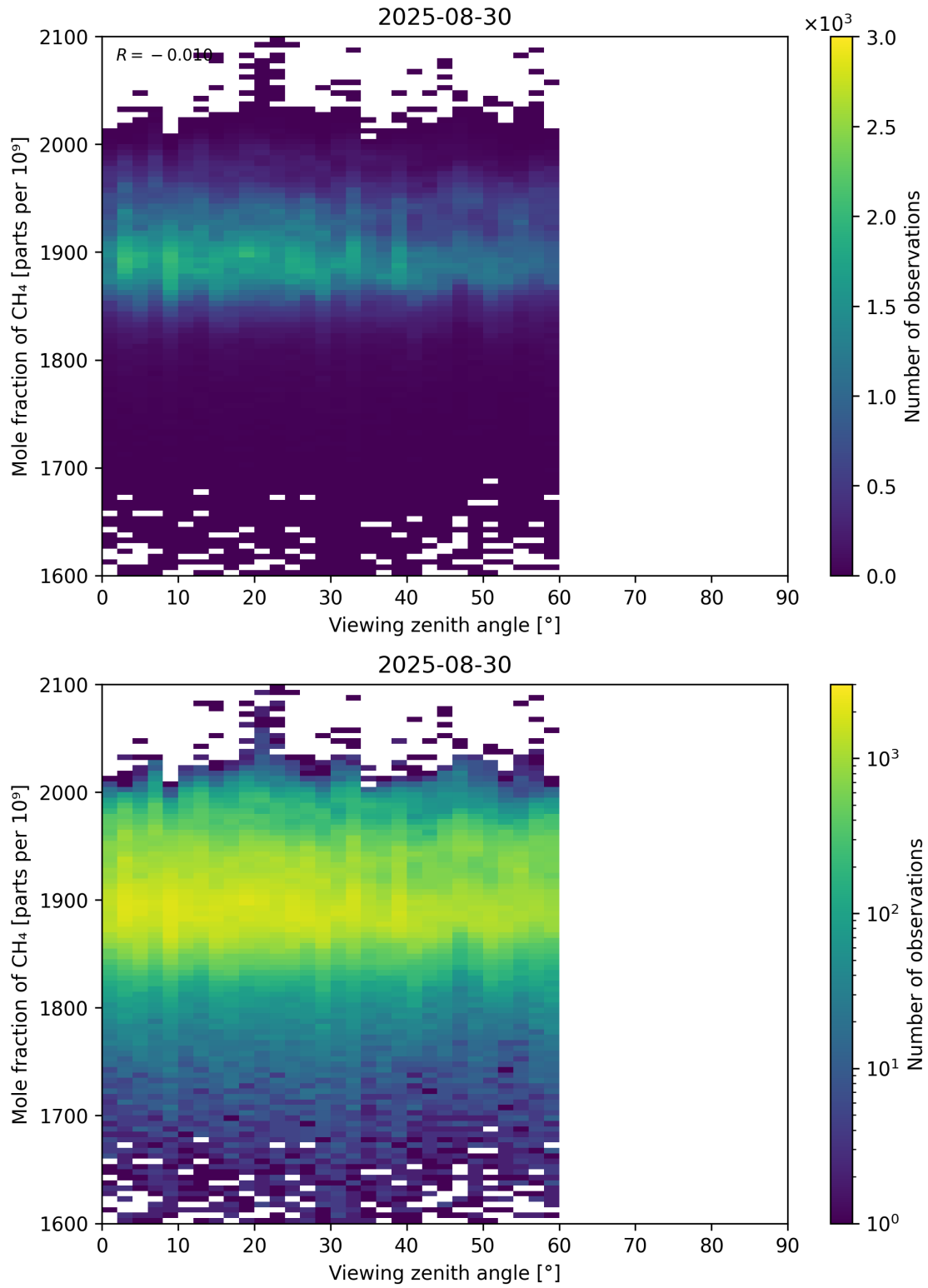
Figure 110: Scatter density plot of “Viewing zenith angle” against “Mole fraction of CH 4 ” for 2025-08-30 to 2025-08-31.
