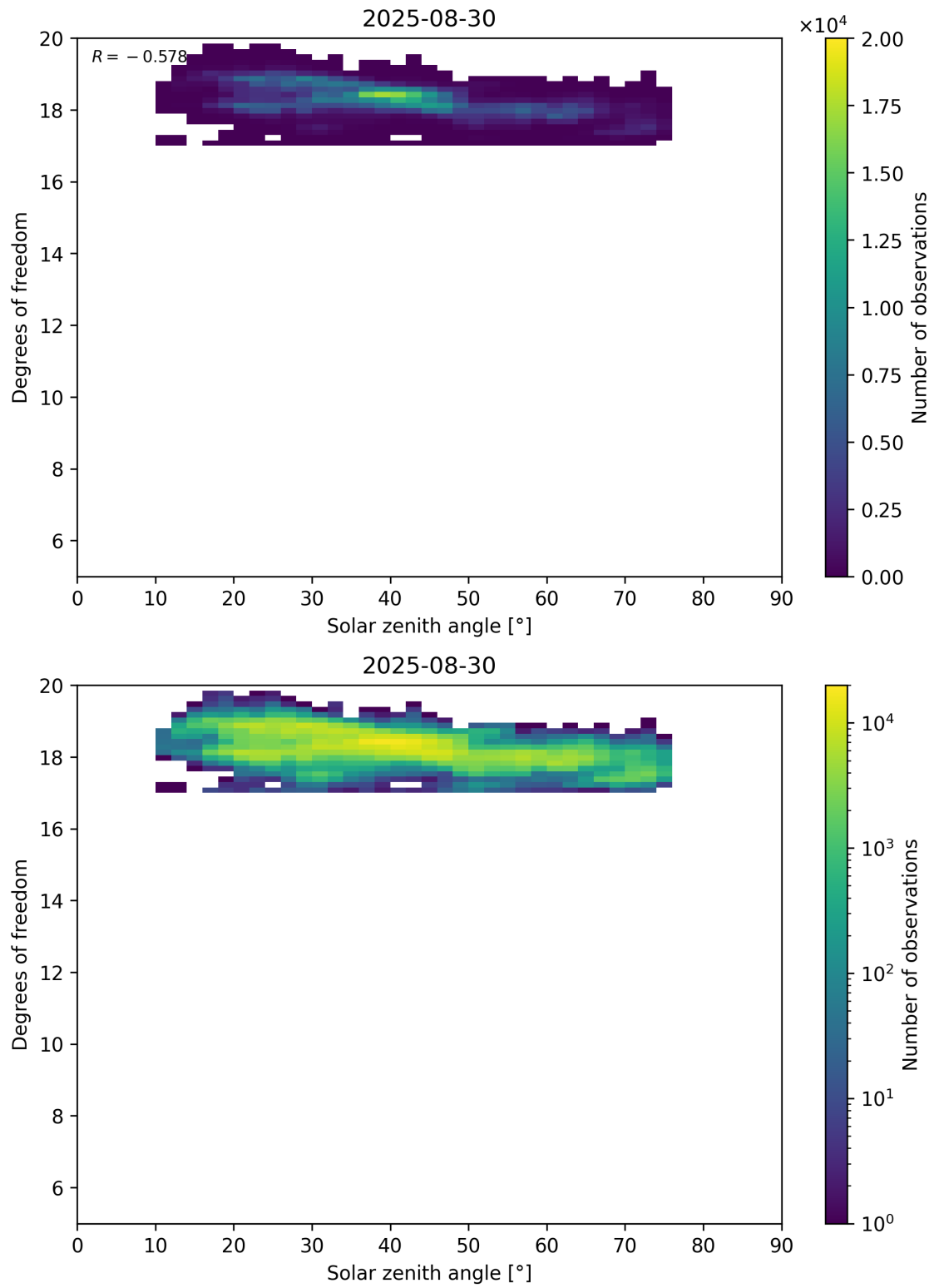
Figure 96: Scatter density plot of “Solar zenith angle” against “Degrees of freedom” for 2025-08-30 to 2025-08-31.
