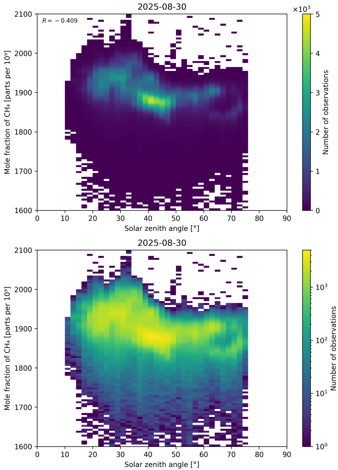
Figure 99: Scatter density plot of “Solar zenith angle” against “Mole fraction of CH 4 ” for 2025-08-30 to 2025-08-31.
