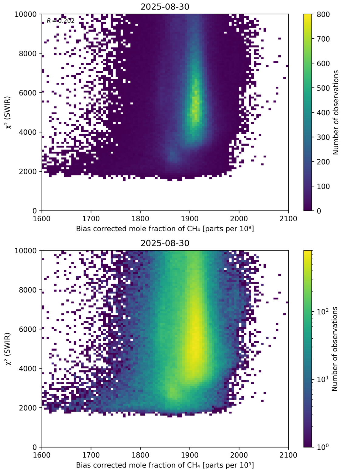
Figure 64: Scatter density plot of “Bias corrected mole fraction of \text{CH}_4 ” against “ \chi^2 (SWIR)” for 2025-08-30 to 2025-08-31.
