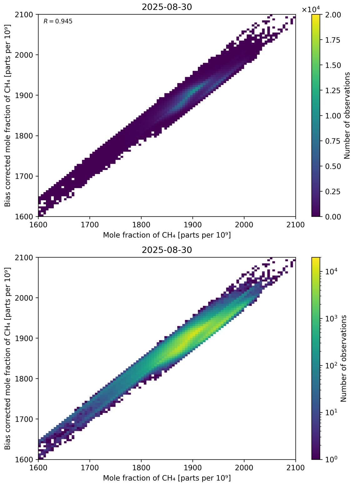
Figure 74: Scatter density plot of “Mole fraction of \text{CH}_4 ” against “Bias corrected mole fraction of \text{CH}_4 ” for 2025-08-30 to 2025-08-31.
