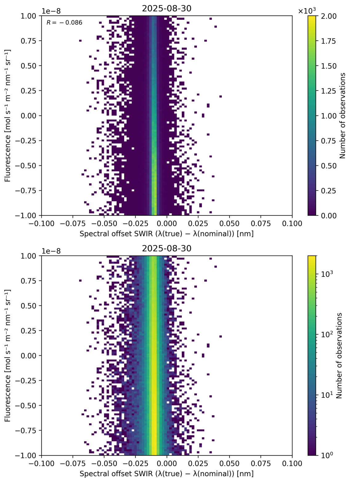
Figure 120: Scatter density plot of “Spectral offset SWIR ( \lambda_{\text{true}} - \lambda_{\text{nominal}} )” against “Fluorescence” for 2025-08-30 to 2025-08-31.
