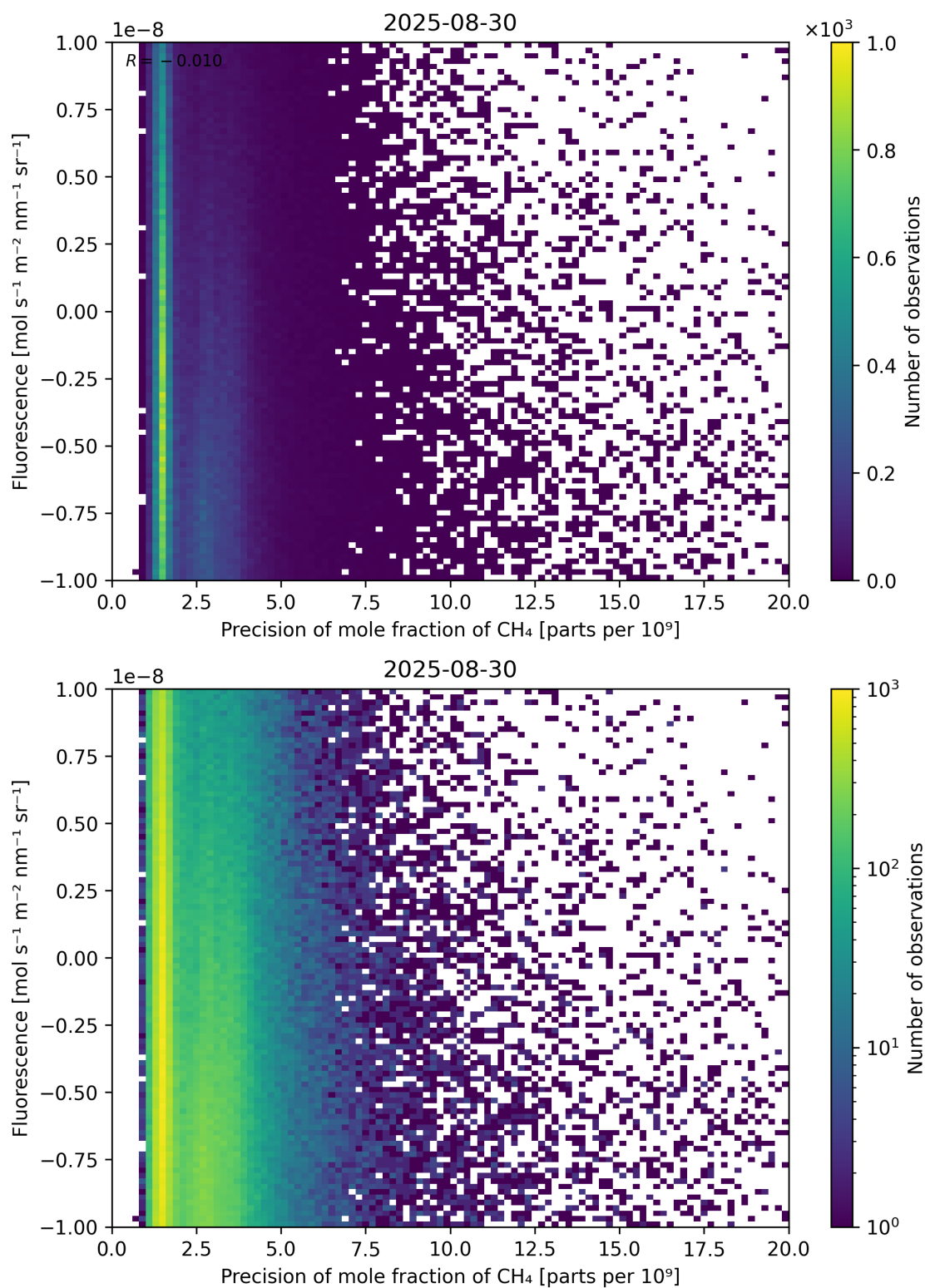
Figure 81: Scatter density plot of “Precision of mole fraction of \text{CH}_4 ” against “Fluorescence” for 2025-08-30 to 2025-08-31.
