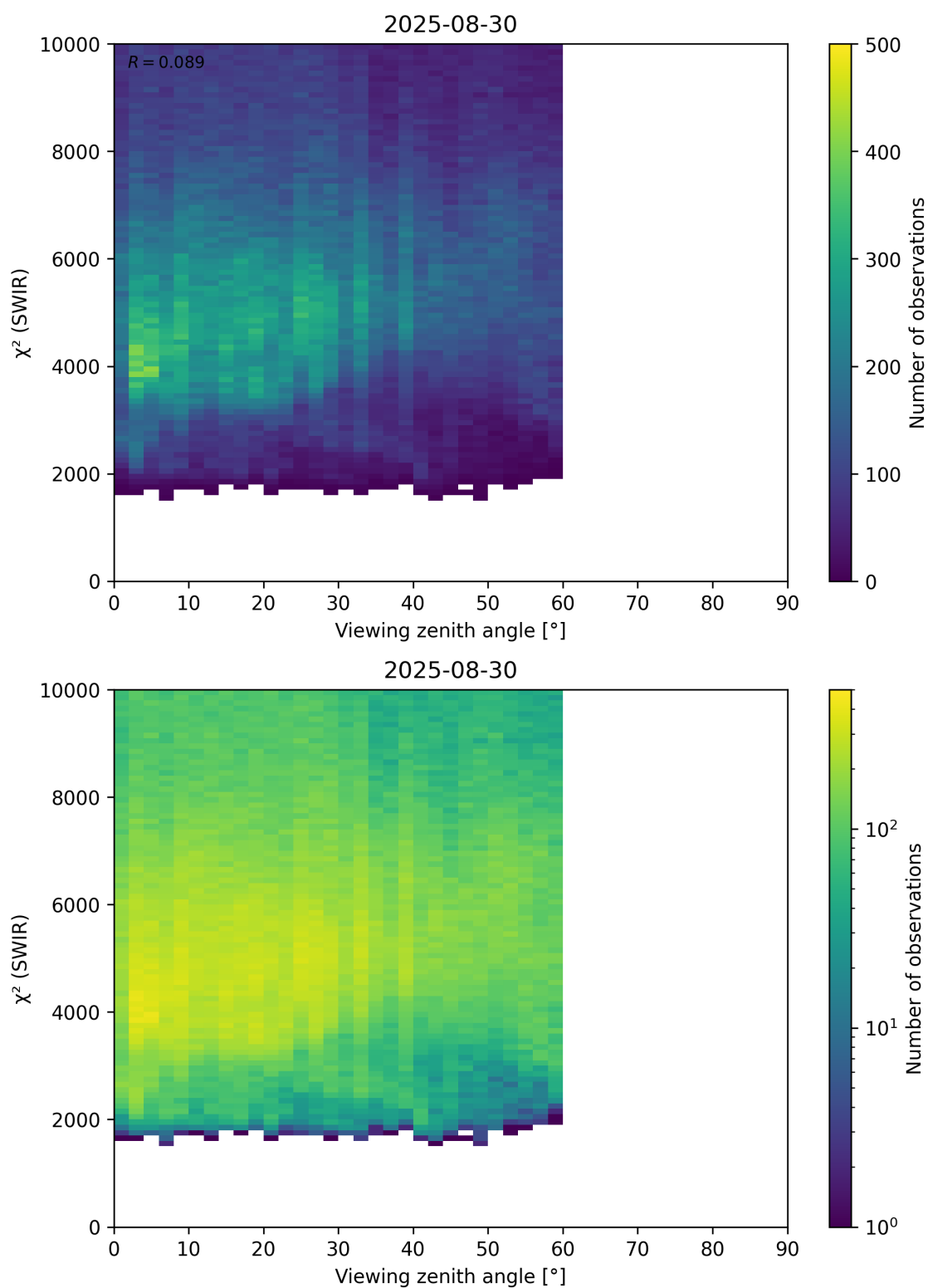
Figure 106: Scatter density plot of “Viewing zenith angle” against “ \chi^2 (SWIR)” for 2025-08-30 to 2025-08-31.
