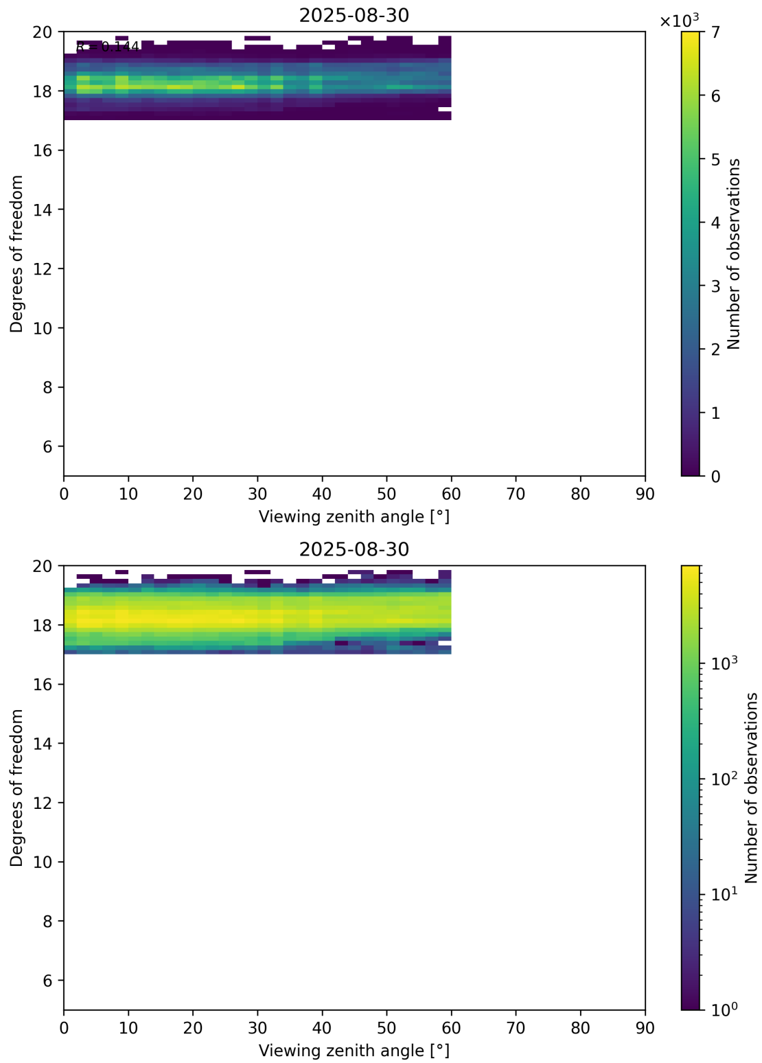
Figure 107: Scatter density plot of “Viewing zenith angle” against “Degrees of freedom” for 2025-08-30 to 2025-08-31.
