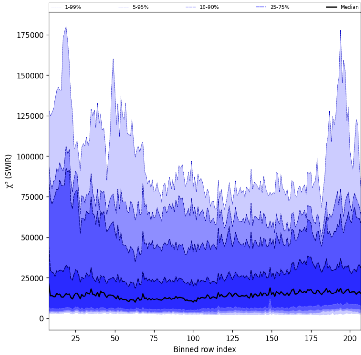
Figure 39: Along track statistics of “ \chi^2 (SWIR)” for 2025-08-30 to 2025-08-31
