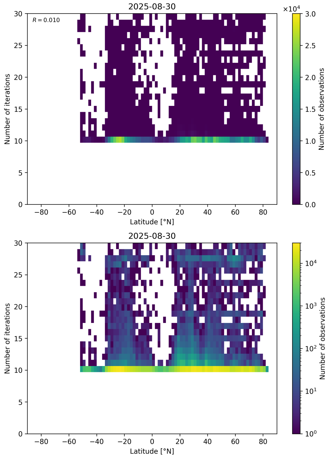
Figure 60: Scatter density plot of “Latitude” against “Number of iterations” for 2025-08-30 to 2025-08-31.
