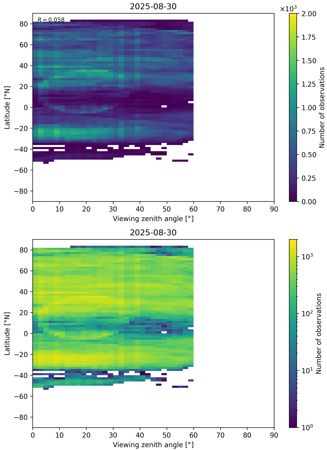
Figure 109: Scatter density plot of “Viewing zenith angle” against “Latitude” for 2025-08-30 to 2025-08-31.
