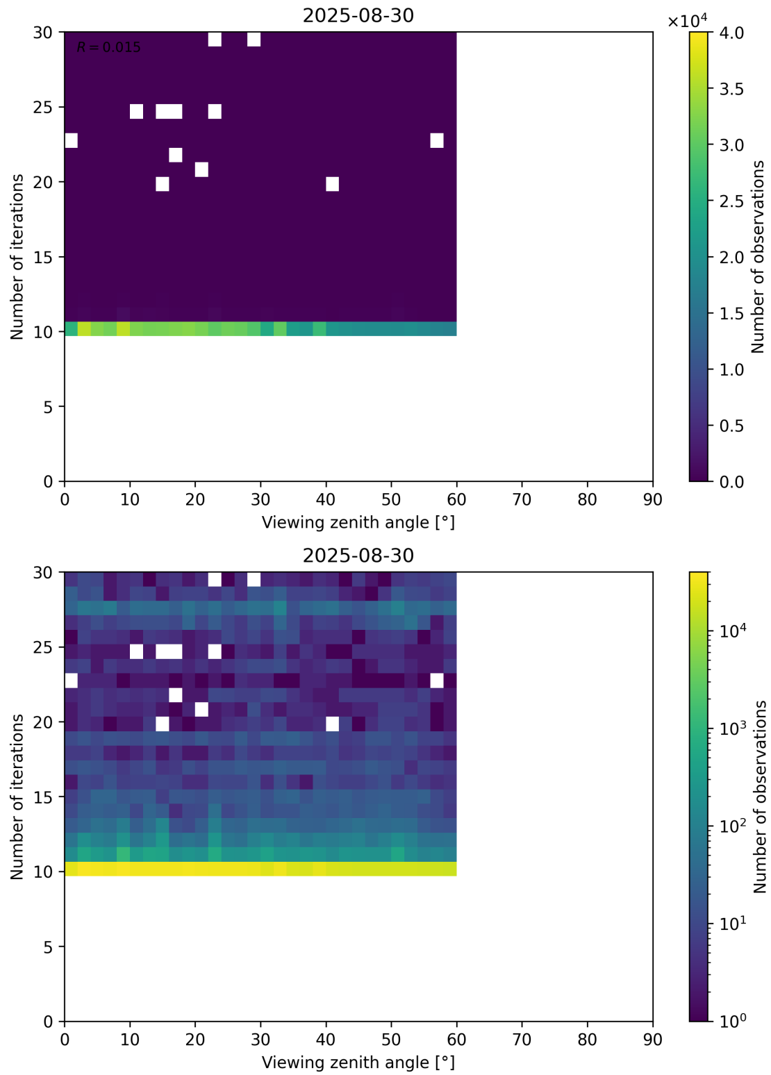
Figure 113: Scatter density plot of “Viewing zenith angle” against “Number of iterations” for 2025-08-30 to 2025-08-31.
