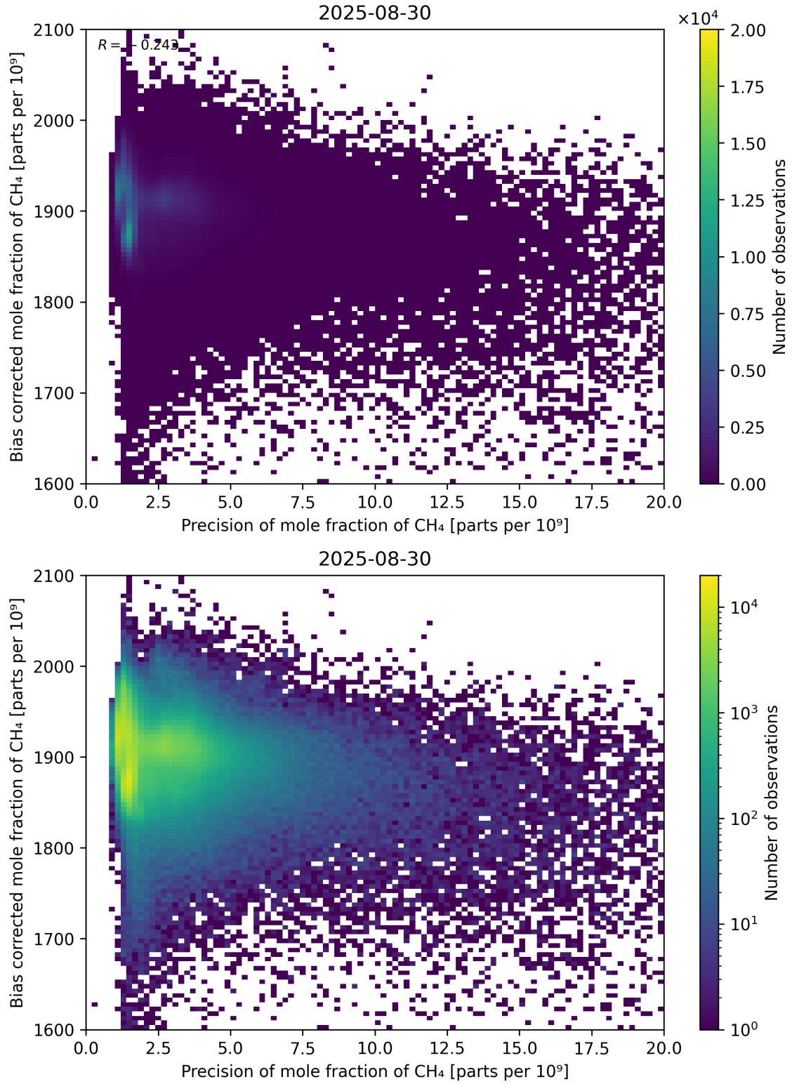
Figure 82: Scatter density plot of “Precision of mole fraction of CH 4 ” against “Bias corrected mole fraction of CH 4 ” for 2025-08-30 to 2025-08-31.
