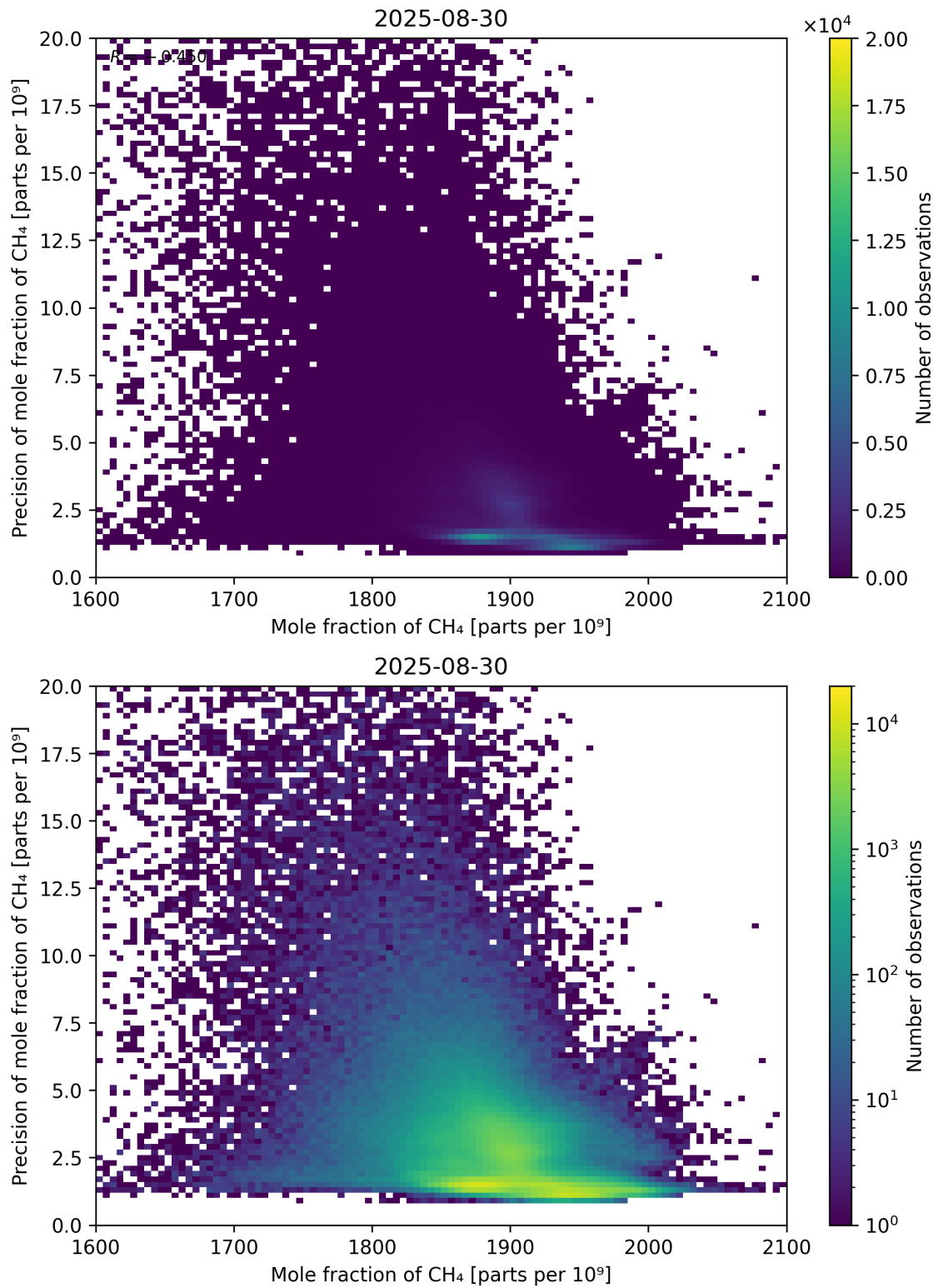
Figure 75: Scatter density plot of “Mole fraction of CH 4 ” against “Precision of mole fraction of CH 4 ” for 2025-08-30 to 2025-08-31.
