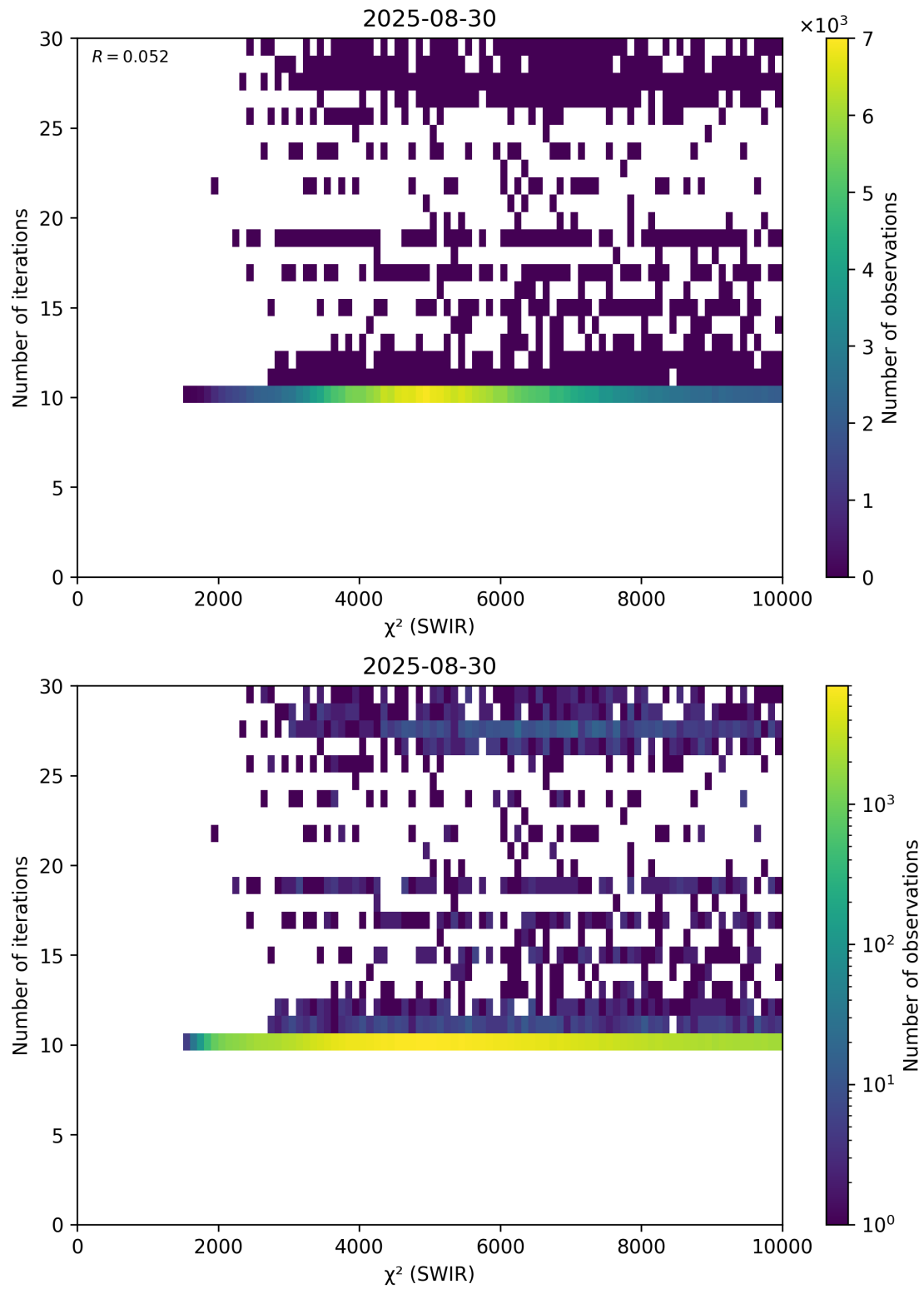
Figure 50: Scatter density plot of “ \chi^2 (SWIR)” against “Number of iterations” for 2025-08-30 to 2025-08-31.
