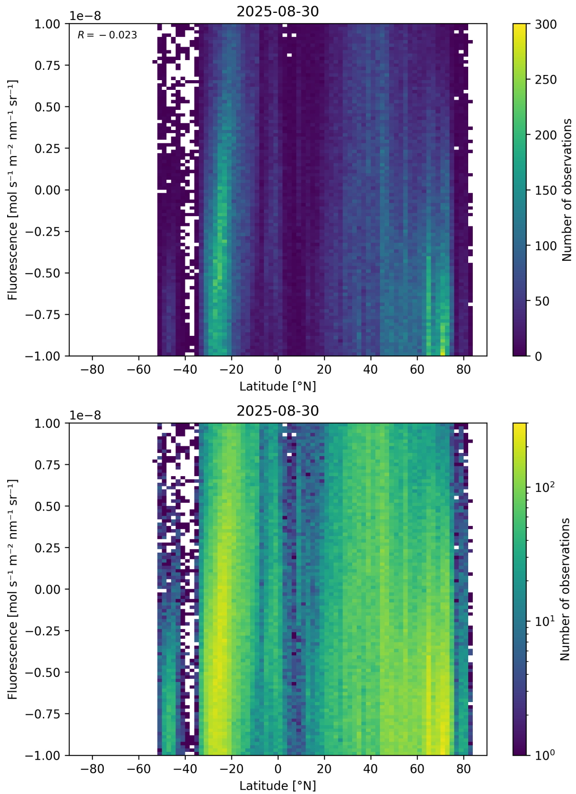
Figure 56: Scatter density plot of “Latitude” against “Fluorescence” for 2025-08-30 to 2025-08-31.
