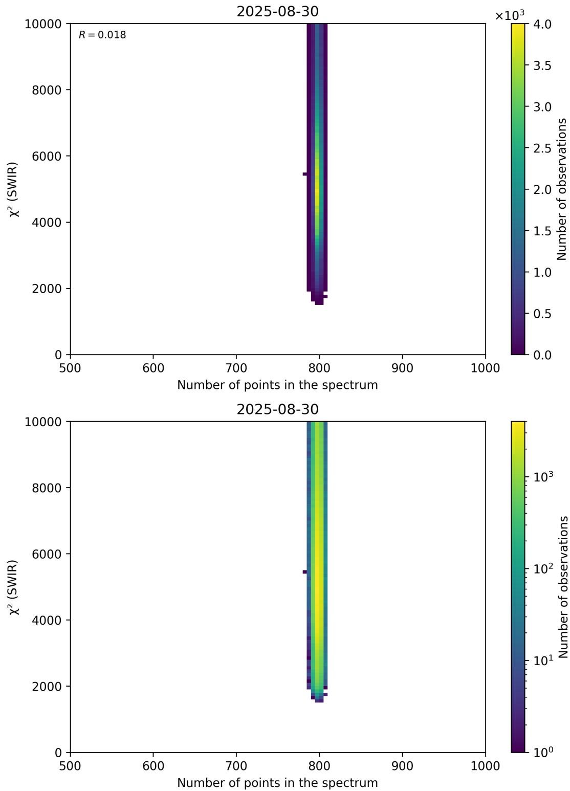
Figure 89: Scatter density plot of “Number of points in the spectrum” against “ \chi^2 (SWIR)” for 2025-08-30 to 2025-08-31.
