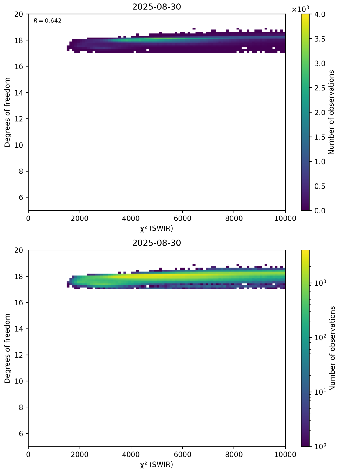
Figure 48: Scatter density plot of “ \chi^2 (SWIR)” against “Degrees of freedom” for 2025-08-30 to 2025-08-31.
