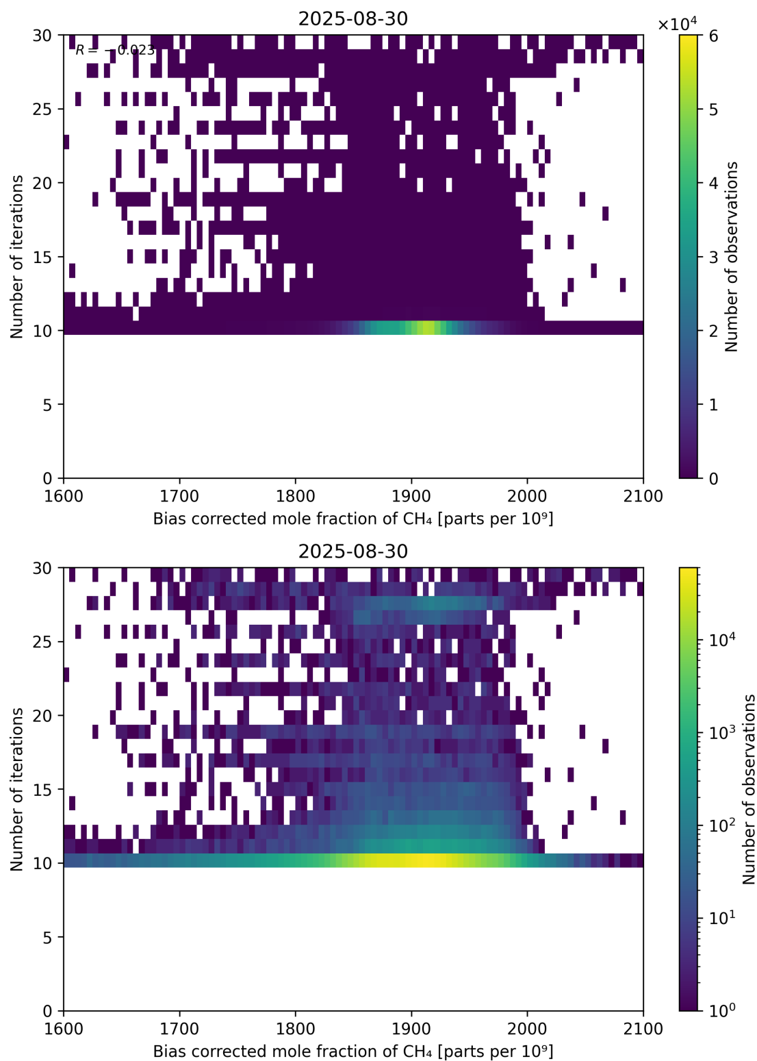
Figure 67: Scatter density plot of “Bias corrected mole fraction of CH 4 ” against “Number of iterations” for 2025-08-30 to 2025-08-31.
