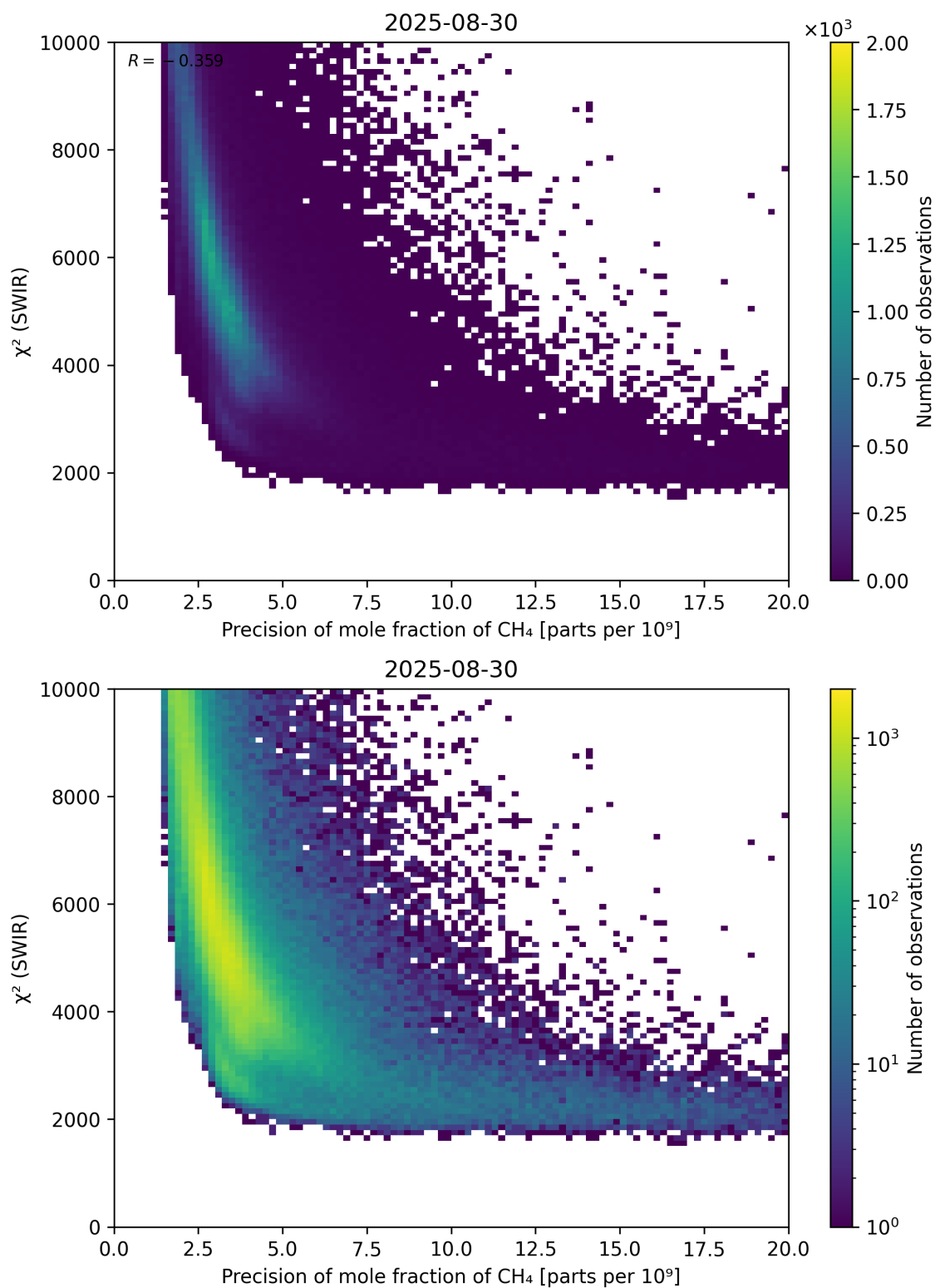
Figure 79: Scatter density plot of “Precision of mole fraction of \text{CH}_4 ” against “ \chi^2 (SWIR)” for 2025-08-30 to 2025-08-31.
