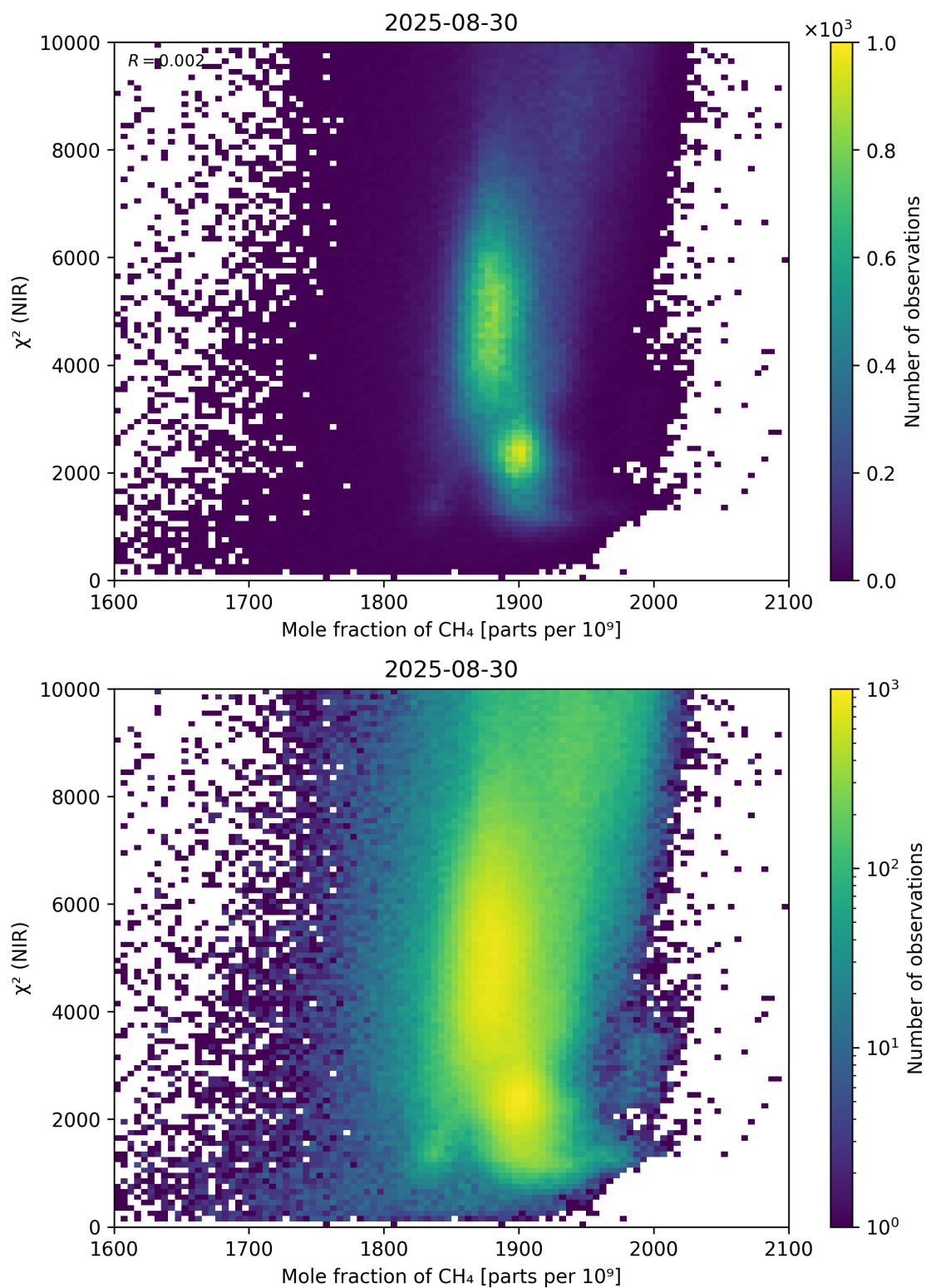
Figure 70: Scatter density plot of “Mole fraction of \text{CH}_4 ” against “ \chi^2 (NIR)” for 2025-08-30 to 2025-08-31.
