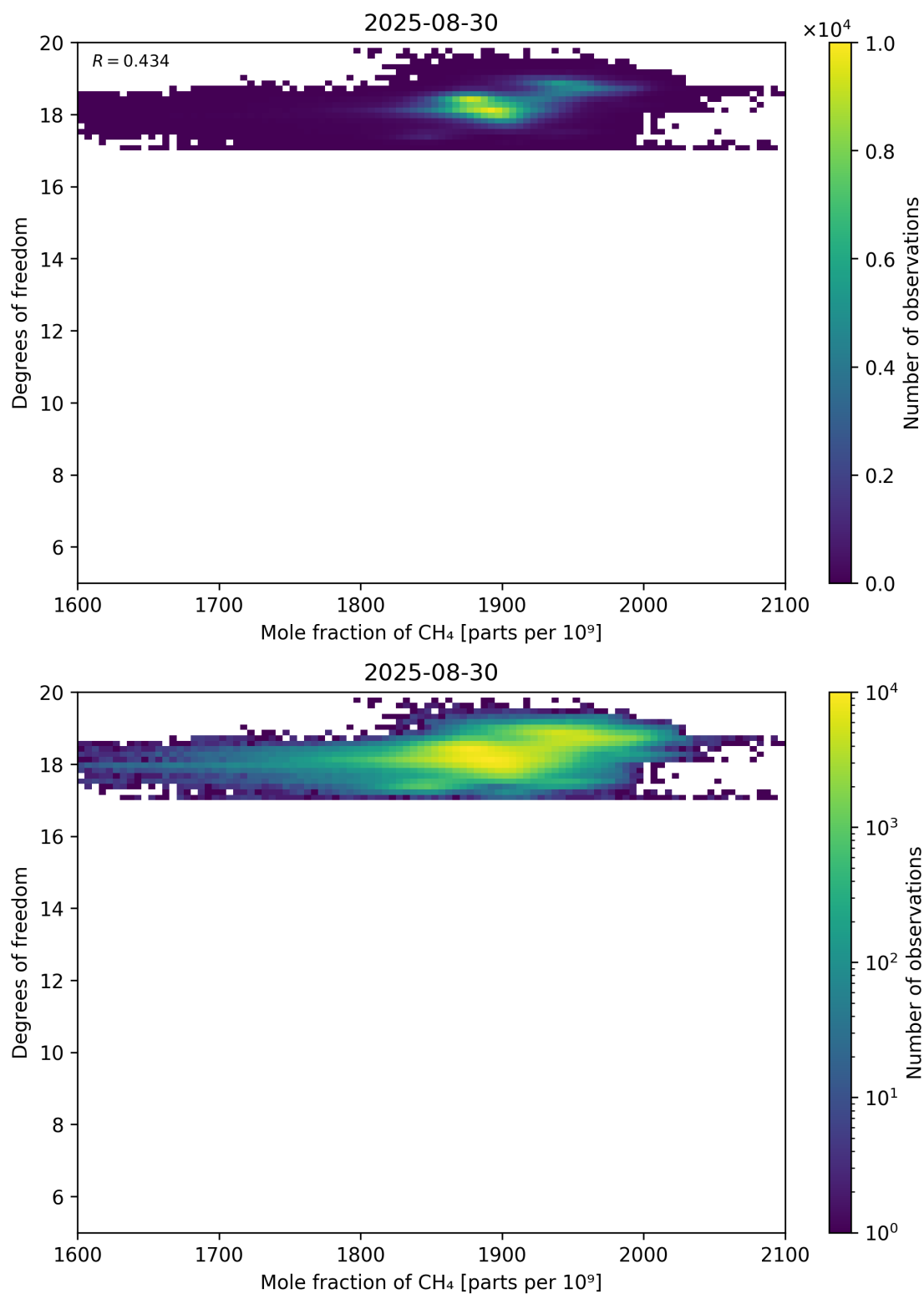
Figure 72: Scatter density plot of “Mole fraction of CH 4 ” against “Degrees of freedom” for 2025-08-30 to 2025-08-31.
