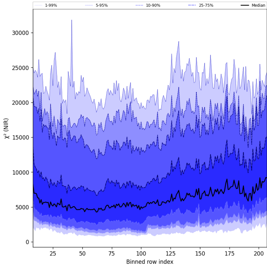
Figure 40: Along track statistics of “ \chi^2 (NIR)” for 2025-08-30 to 2025-08-31
