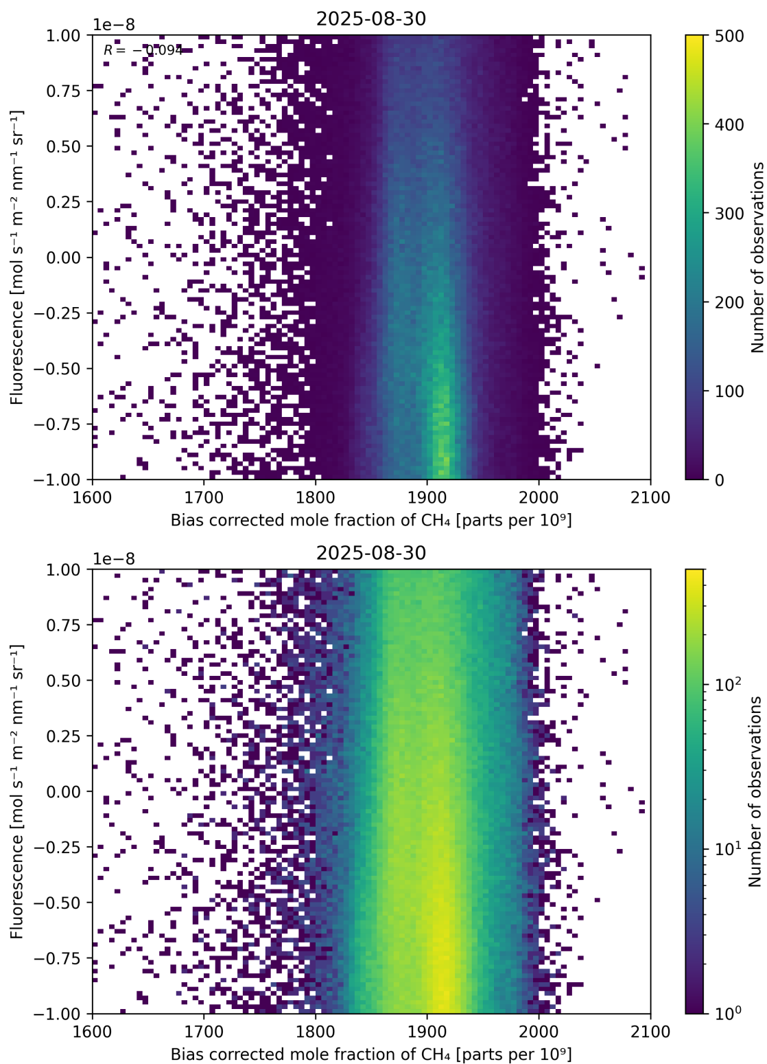
Figure 66: Scatter density plot of “Bias corrected mole fraction of \text{CH}_4 ” against “Fluorescence” for 2025-08-30 to 2025-08-31.
