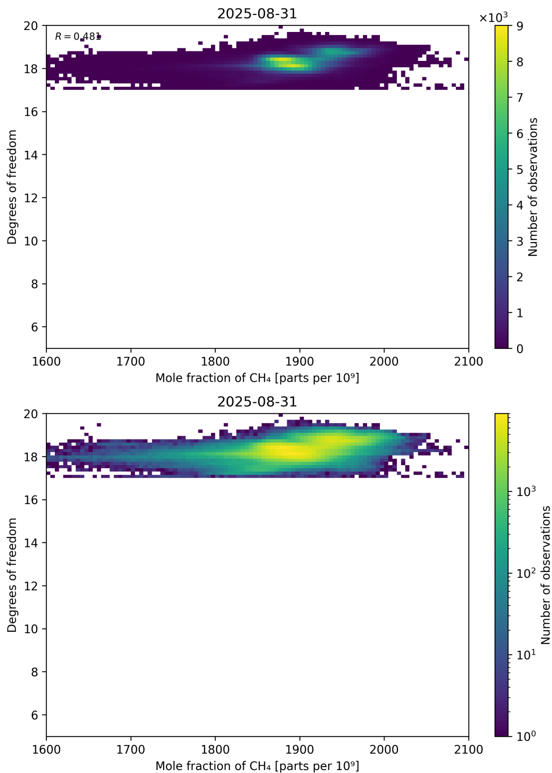
Figure 72: Scatter density plot of “Mole fraction of CH 4 ” against “Degrees of freedom” for 2025-08-30 to 2025-09-01.
