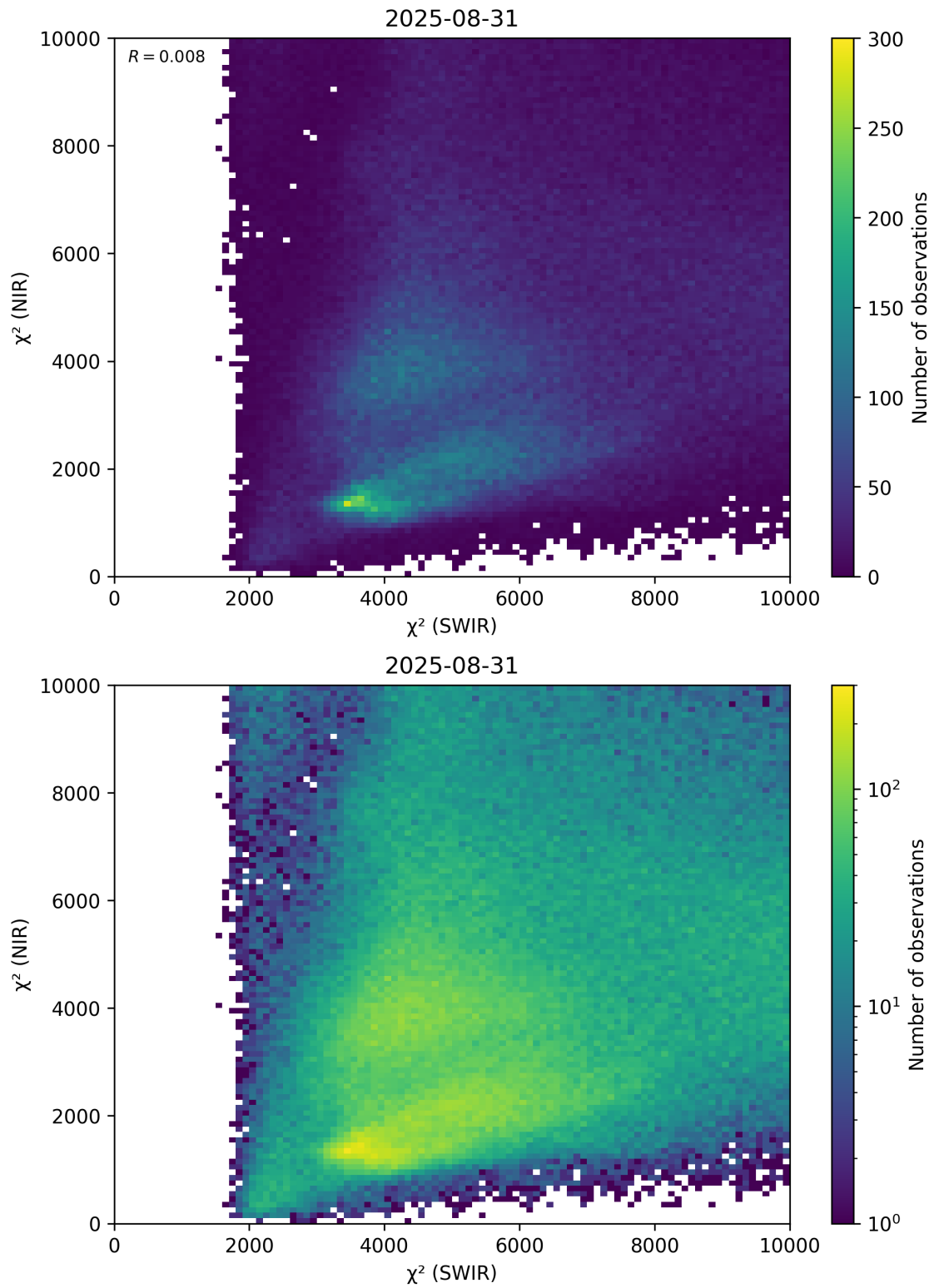
Figure 47: Scatter density plot of “ \chi^2 (SWIR)” against “ \chi^2 (NIR)” for 2025-08-30 to 2025-09-01.
