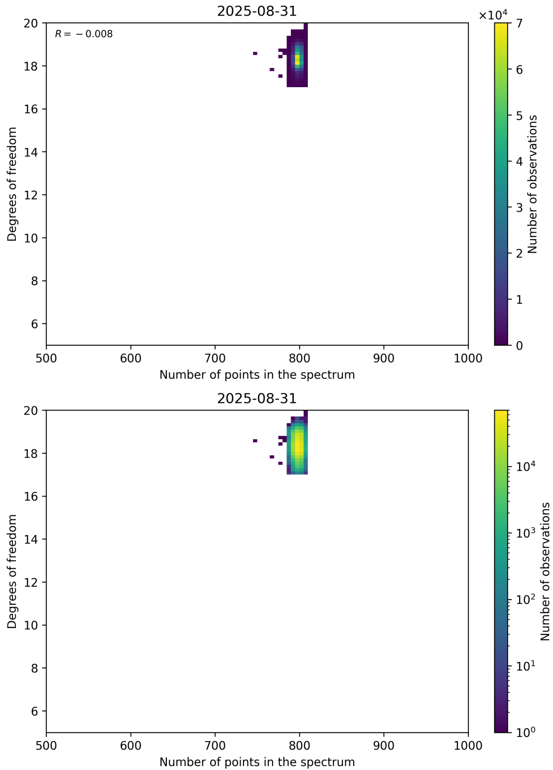
Figure 90: Scatter density plot of “Number of points in the spectrum” against “Degrees of freedom” for 2025-08-30 to 2025-09-01.
