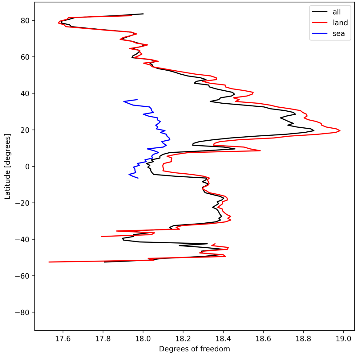
Figure 19: Zonal average of “Degrees of freedom” for 2025-08-30 to 2025-09-01.
