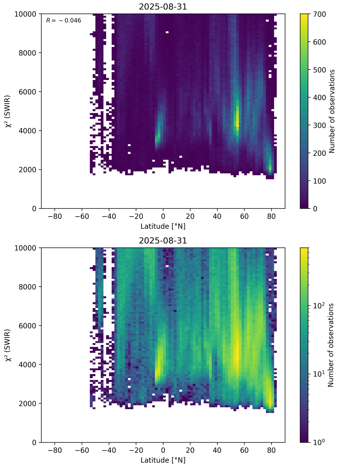
Figure 54: Scatter density plot of “Latitude” against “ \chi^2 (SWIR)” for 2025-08-30 to 2025-09-01.
