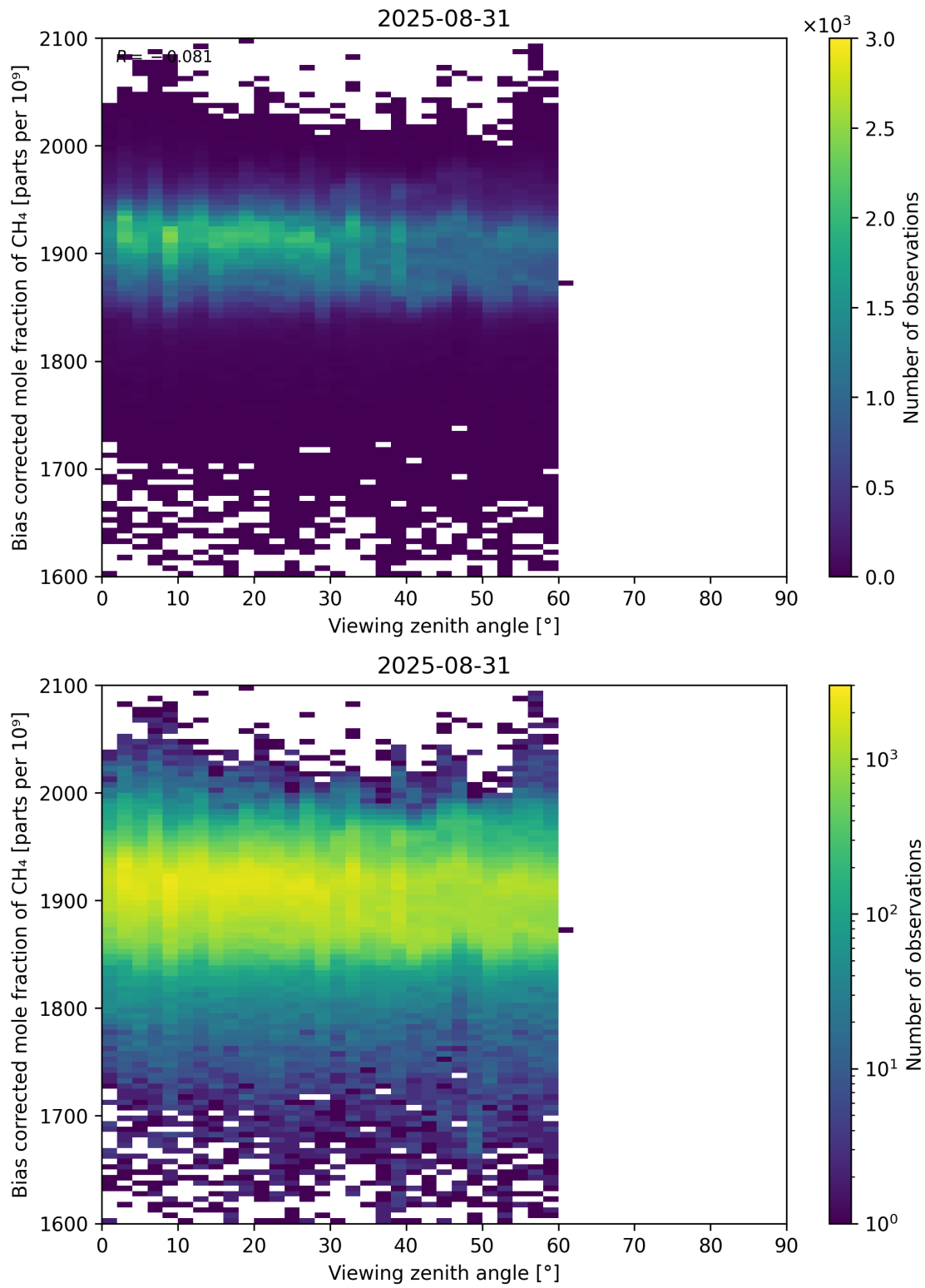
Figure 111: Scatter density plot of “Viewing zenith angle” against “Bias corrected mole fraction of CH 4 ” for 2025-08-30 to 2025-09-01.
