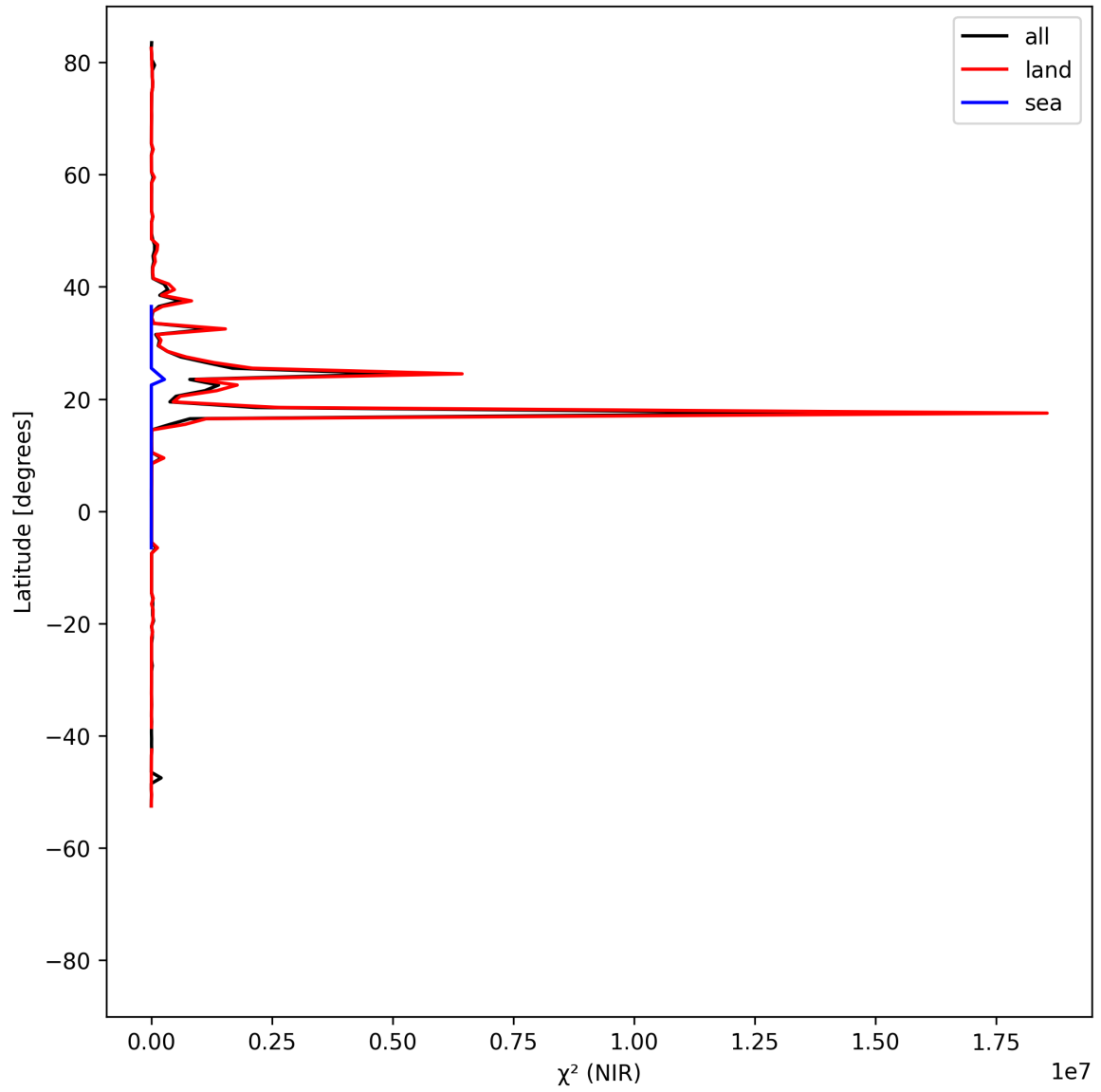
Figure 18: Zonal average of “ \chi^2 (NIR)” for 2025-08-30 to 2025-09-01.
