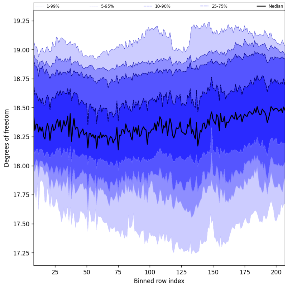
Figure 41: Along track statistics of “Degrees of freedom” for 2025-08-30 to 2025-09-01
