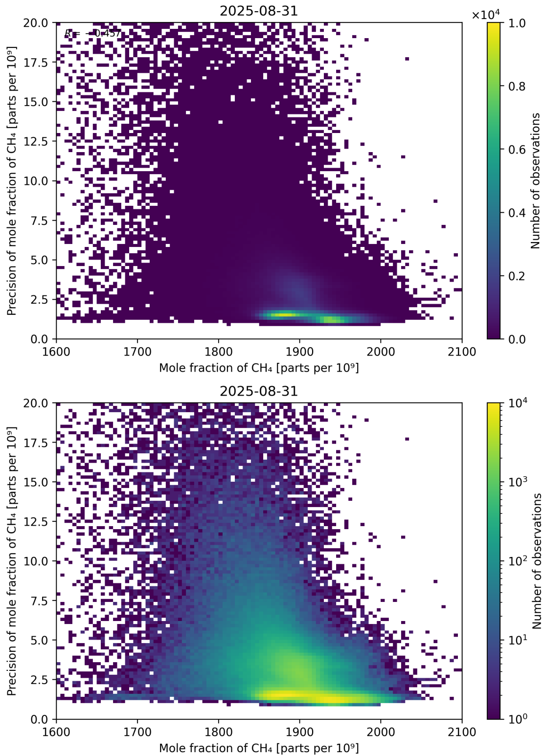
Figure 75: Scatter density plot of “Mole fraction of CH 4 ” against “Precision of mole fraction of CH 4 ” for 2025-08-30 to 2025-09-01.
