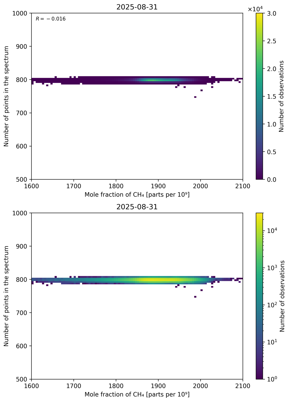
Figure 77: Scatter density plot of “Mole fraction of CH 4 ” against “Number of points in the spectrum” for 2025-08-30 to 2025-09-01.
