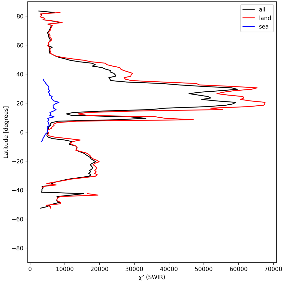
Figure 17: Zonal average of “ \chi^2 (SWIR)” for 2025-08-30 to 2025-09-01.
