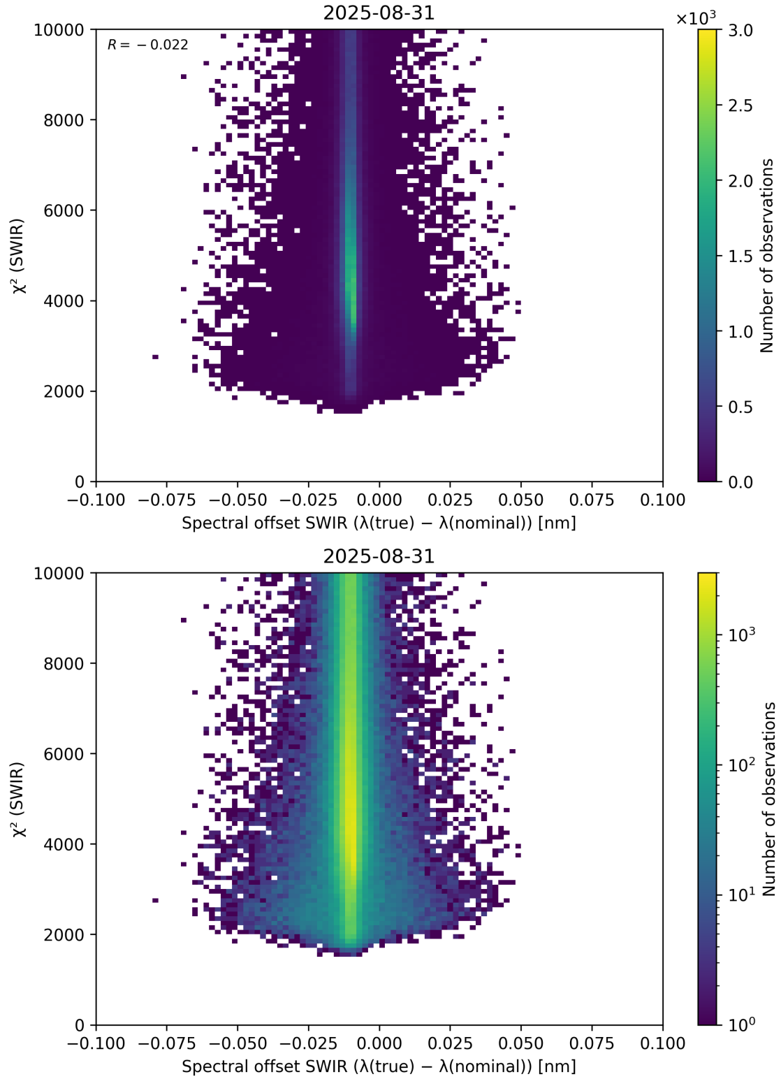
Figure 118: Scatter density plot of “Spectral offset SWIR ( \lambda_{\text{true}} - \lambda_{\text{nominal}} )” against “ \chi^2 (SWIR)” for 2025-08-30 to 2025-09-01.
