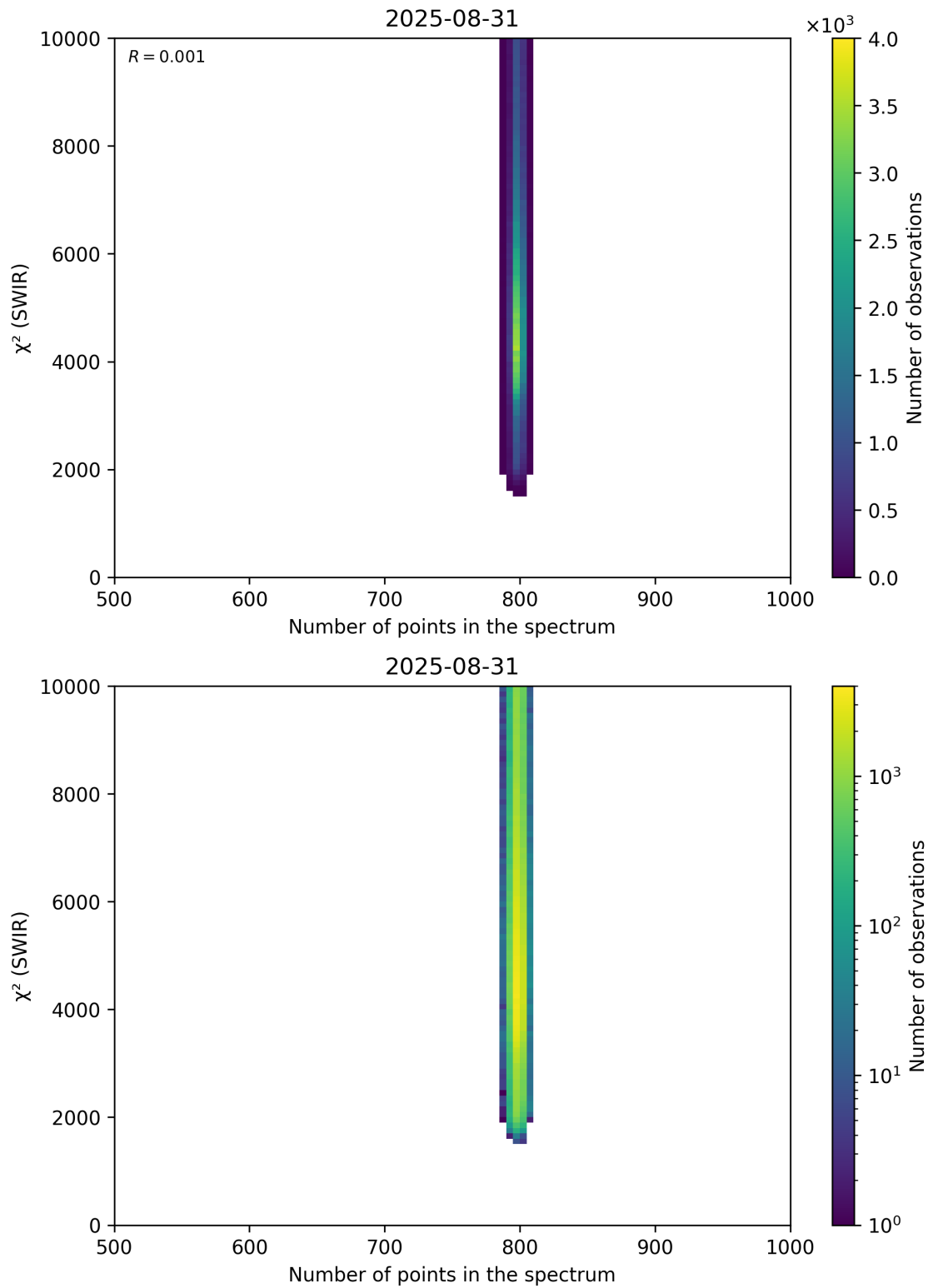
Figure 89: Scatter density plot of “Number of points in the spectrum” against “ \chi^2 (SWIR)” for 2025-08-30 to 2025-09-01.
