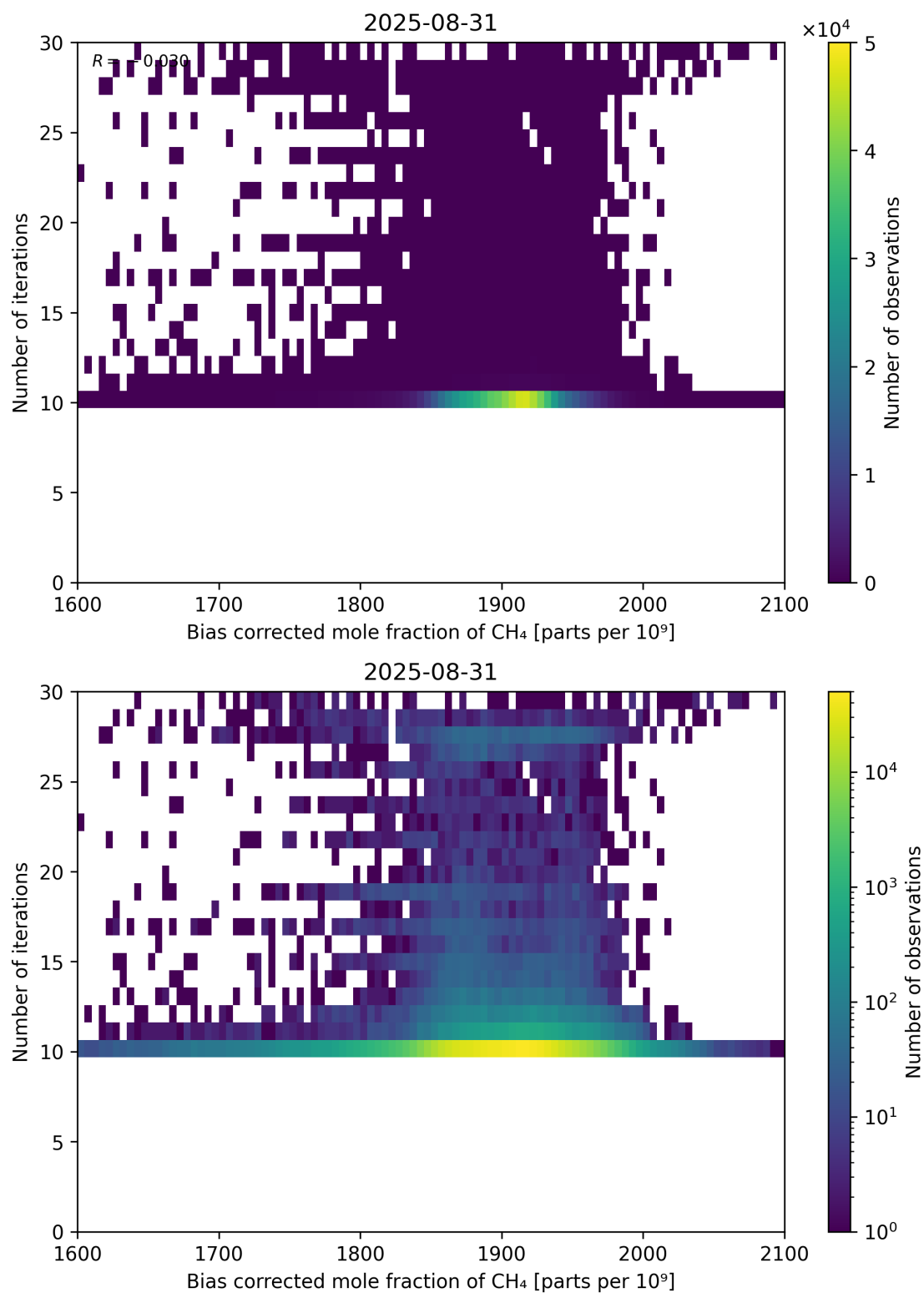
Figure 67: Scatter density plot of “Bias corrected mole fraction of CH 4 ” against “Number of iterations” for 2025-08-30 to 2025-09-01.
