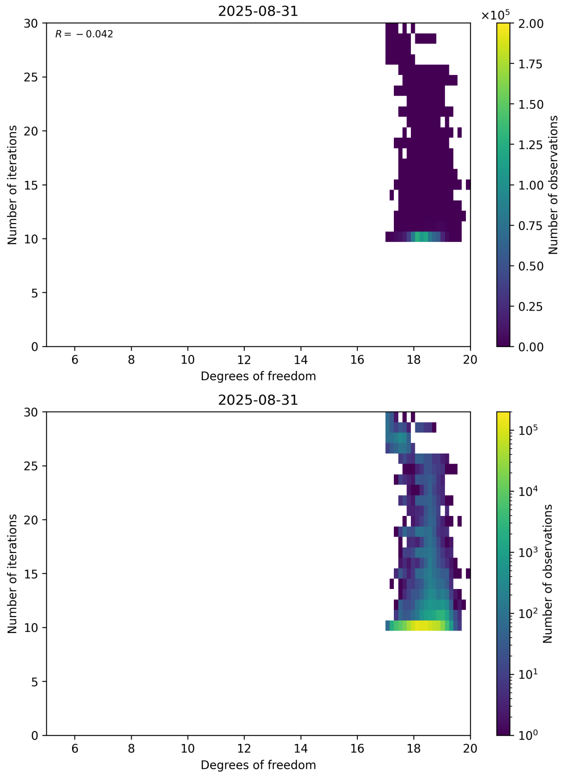
Figure 52: Scatter density plot of “Degrees of freedom” against “Number of iterations” for 2025-08-30 to 2025-09-01.
