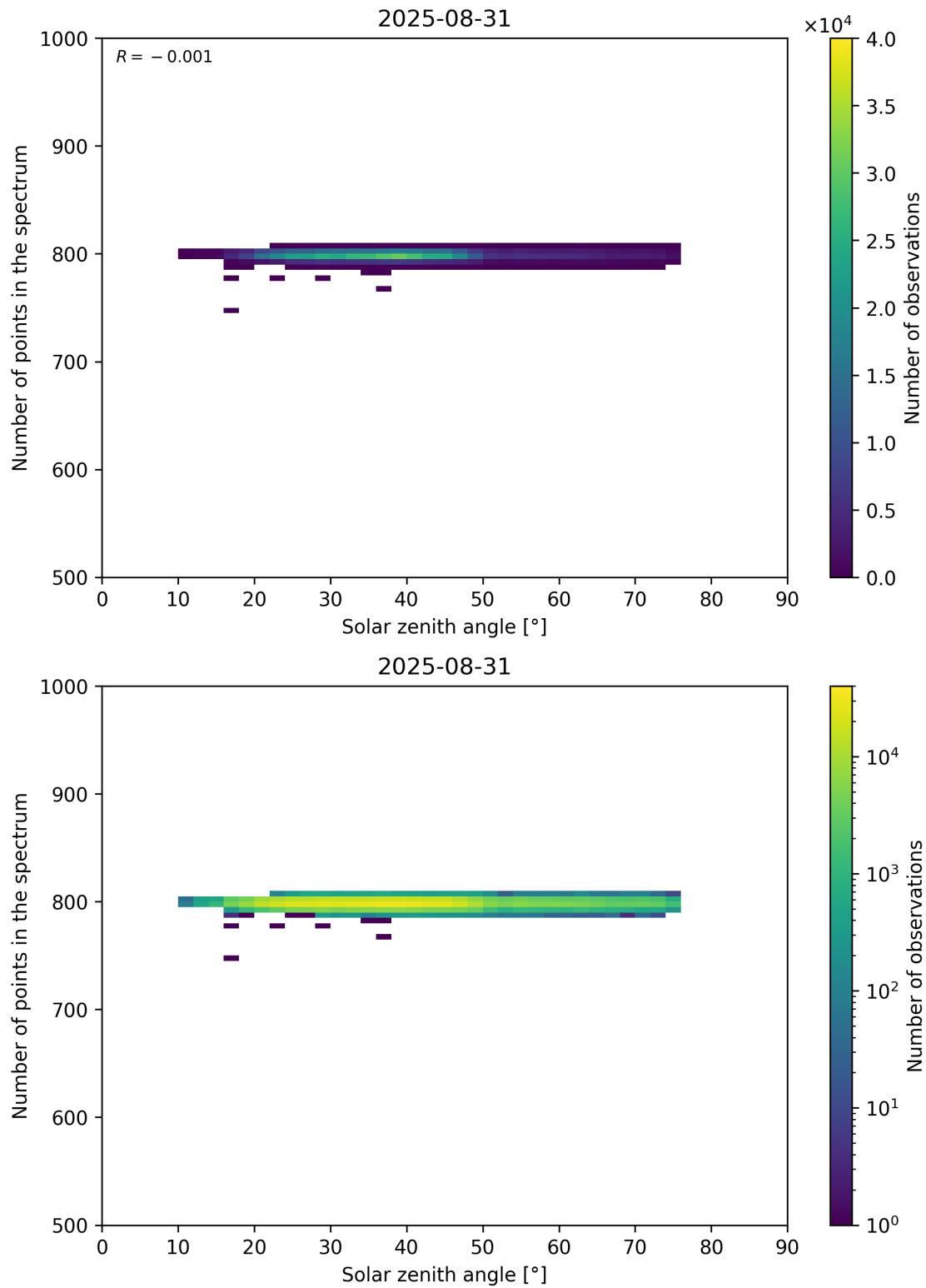
Figure 103: Scatter density plot of “Solar zenith angle” against “Number of points in the spectrum” for 2025-08-30 to 2025-09-01.
