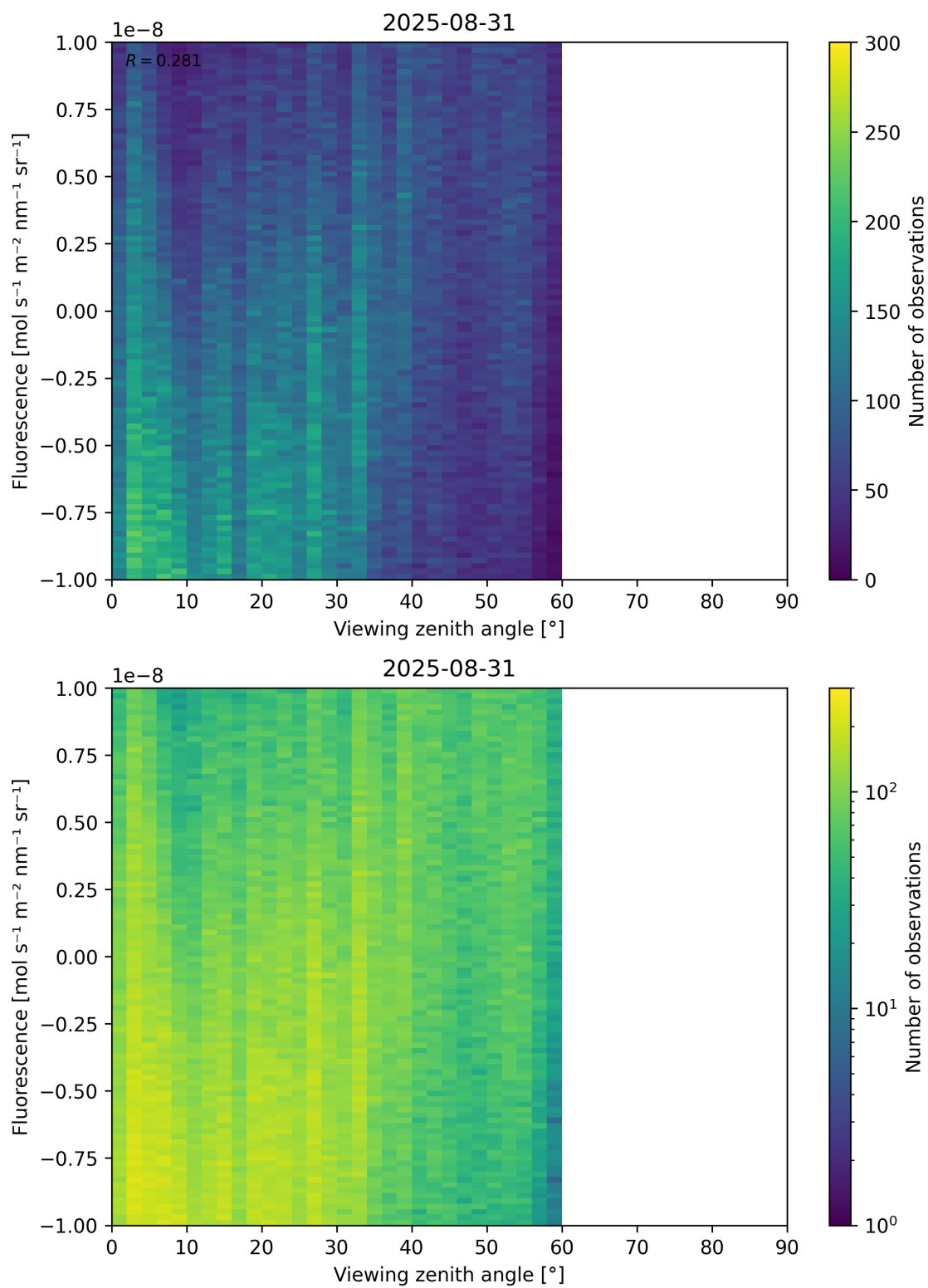
Figure 108: Scatter density plot of “Viewing zenith angle” against “Fluorescence” for 2025-08-30 to 2025-09-01.
