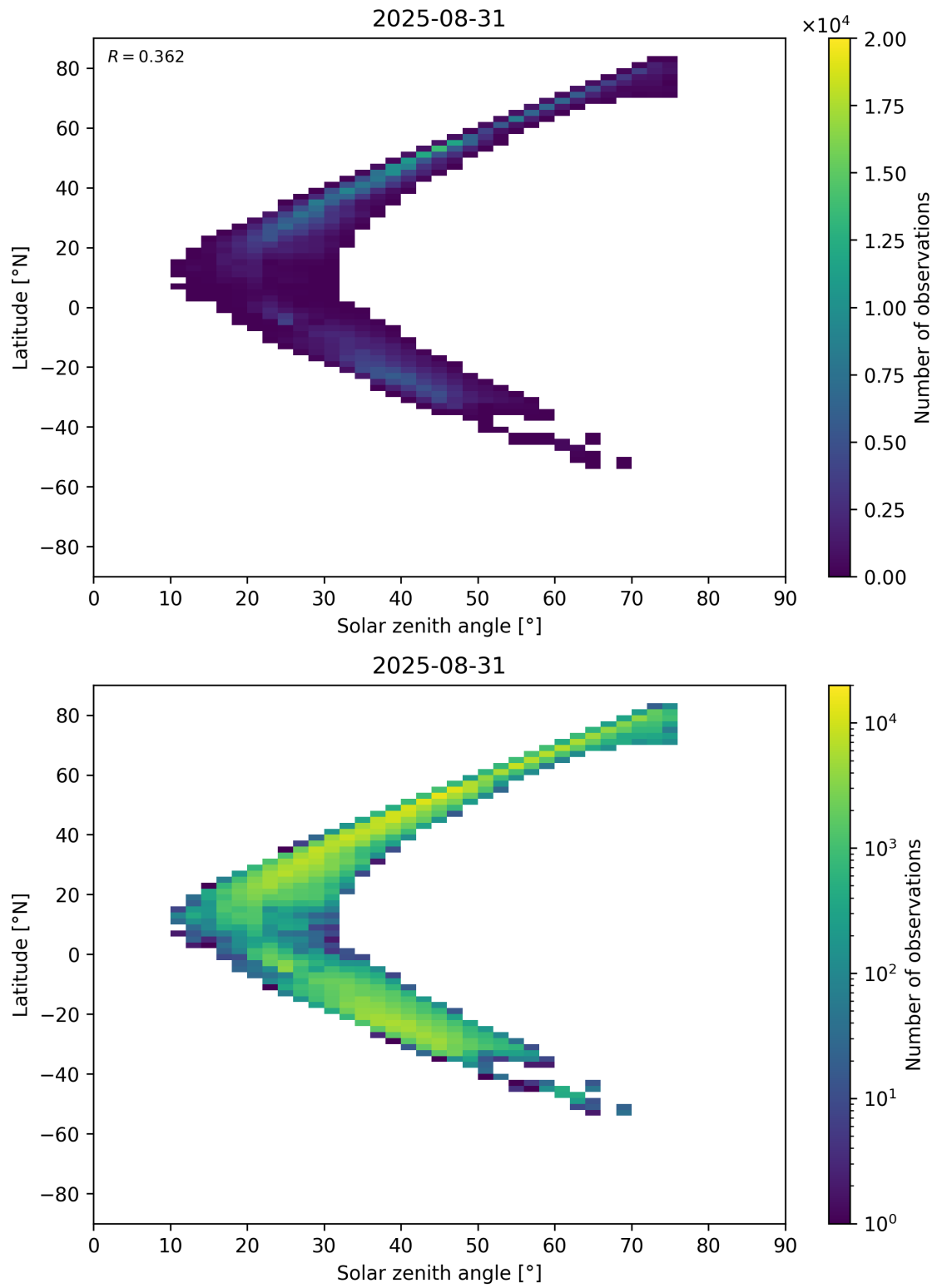
Figure 98: Scatter density plot of “Solar zenith angle” against “Latitude” for 2025-08-30 to 2025-09-01.
