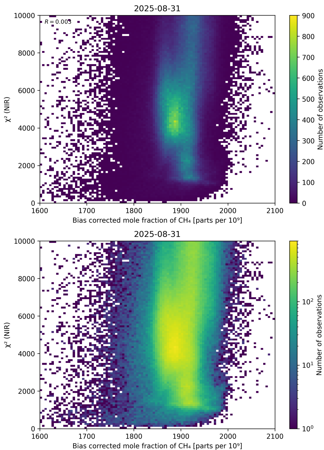
Figure 63: Scatter density plot of “Bias corrected mole fraction of \text{CH}_4 ” against “ \chi^2 (NIR)” for 2025-08-30 to 2025-09-01.
