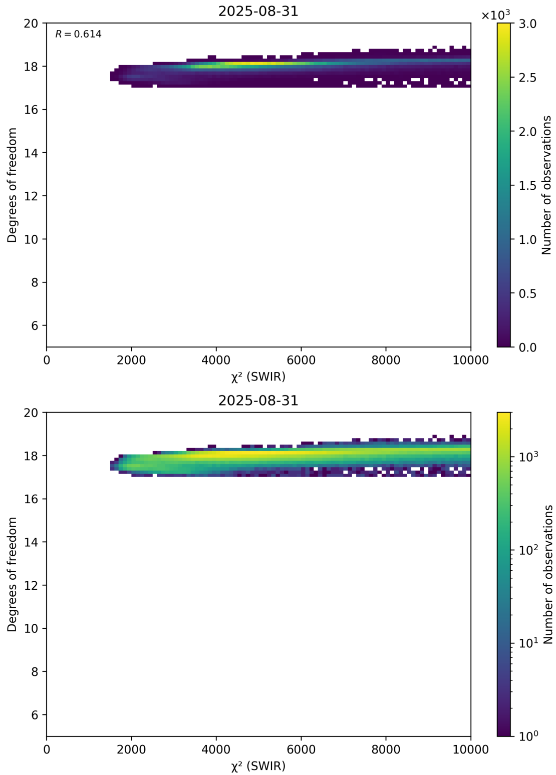
Figure 48: Scatter density plot of " \chi^2 (SWIR)" against "Degrees of freedom" for 2025-08-30 to 2025-09-01.
