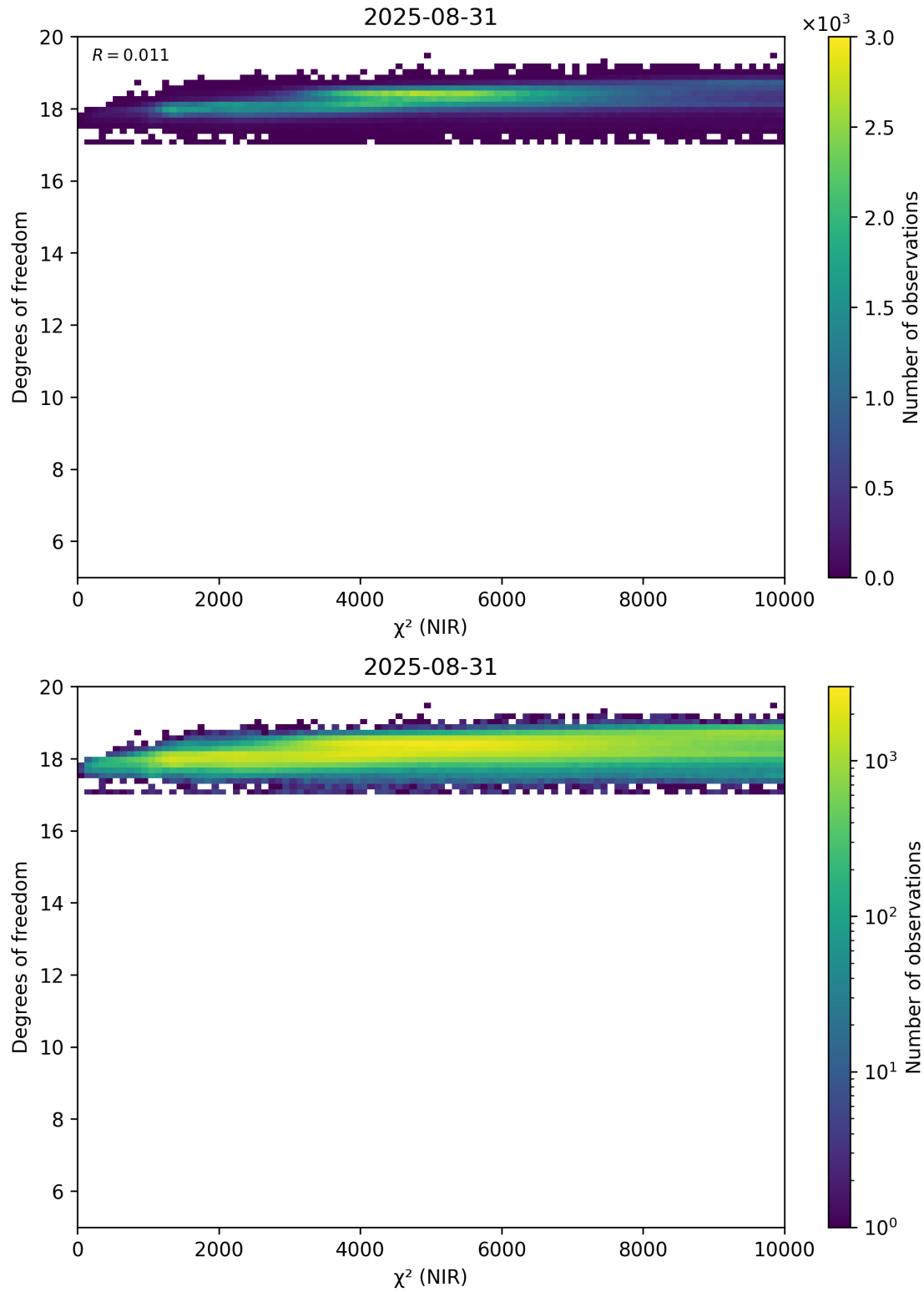
Figure 44: Scatter density plot of “ \chi^2 (NIR)” against “Degrees of freedom” for 2025-08-30 to 2025-09-01.
