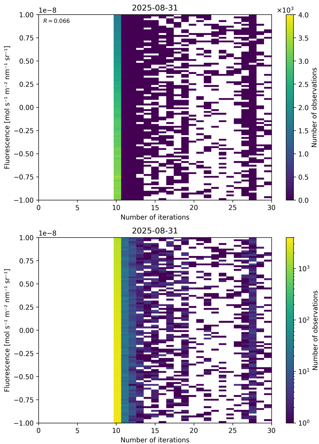
Figure 87: Scatter density plot of "Number of iterations" against "Fluorescence" for 2025-08-30 to 2025-09-01.
