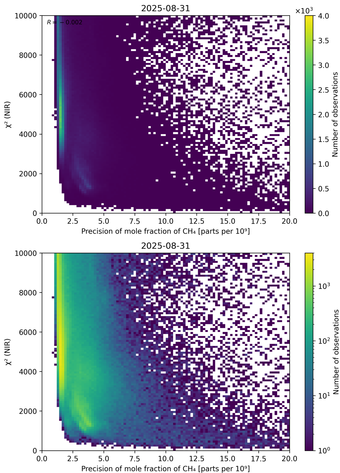
Figure 78: Scatter density plot of “Precision of mole fraction of CH 4 ” against “ \chi^2 (NIR)” for 2025-08-30 to 2025-09-01.
