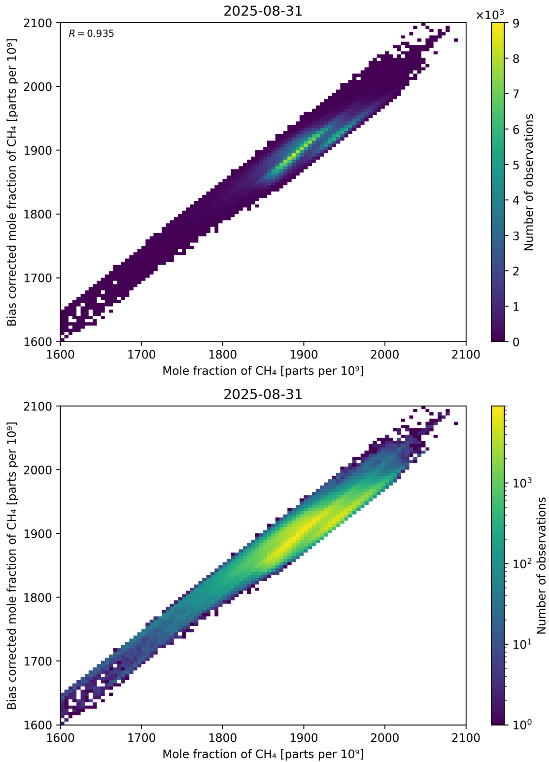
Figure 74: Scatter density plot of “Mole fraction of CH 4 ” against “Bias corrected mole fraction of CH 4 ” for 2025-08-30 to 2025-09-01.
