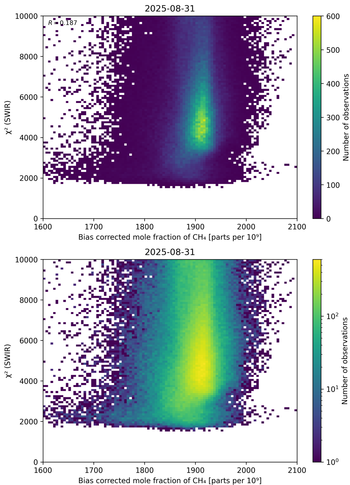
Figure 64: Scatter density plot of “Bias corrected mole fraction of \text{CH}_4 ” against “ \chi^2 (SWIR)” for 2025-08-30 to 2025-09-01.
