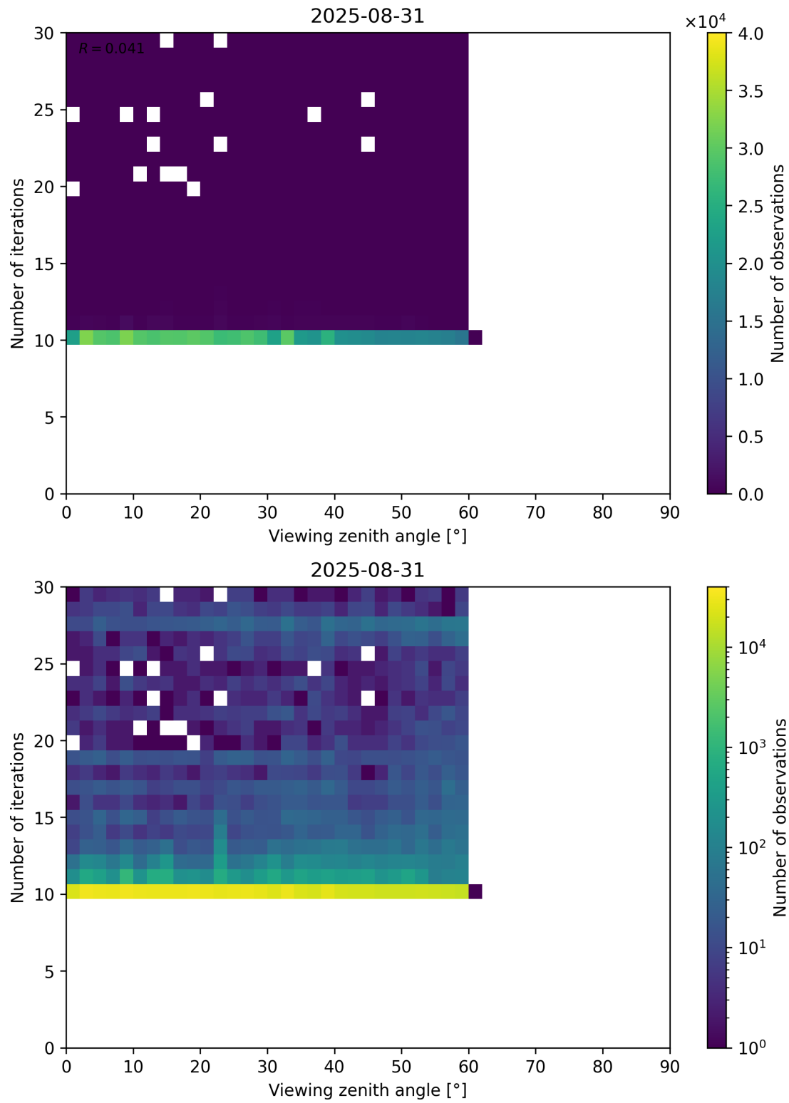
Figure 113: Scatter density plot of “Viewing zenith angle” against “Number of iterations” for 2025-08-30 to 2025-09-01.
