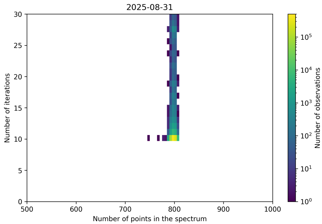
Figure 92: Scatter density plot of “Number of points in the spectrum” against “Number of iterations” for 2025-08-30 to 2025-09-01.
