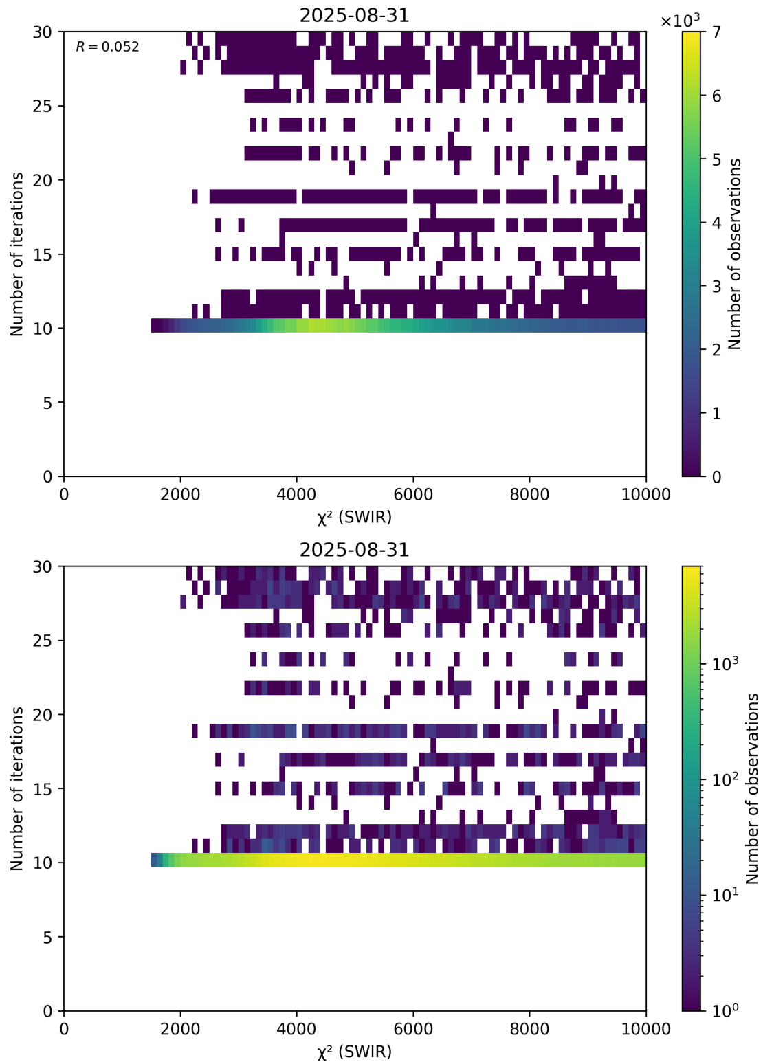
Figure 50: Scatter density plot of “ \chi^2 (SWIR)” against “Number of iterations” for 2025-08-30 to 2025-09-01.
