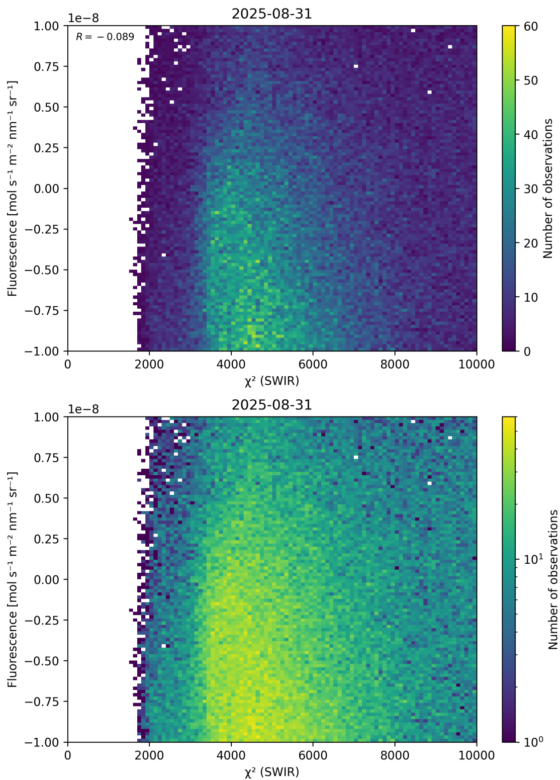
Figure 49: Scatter density plot of “ \chi^2 (SWIR)” against “Fluorescence” for 2025-08-30 to 2025-09-01.
