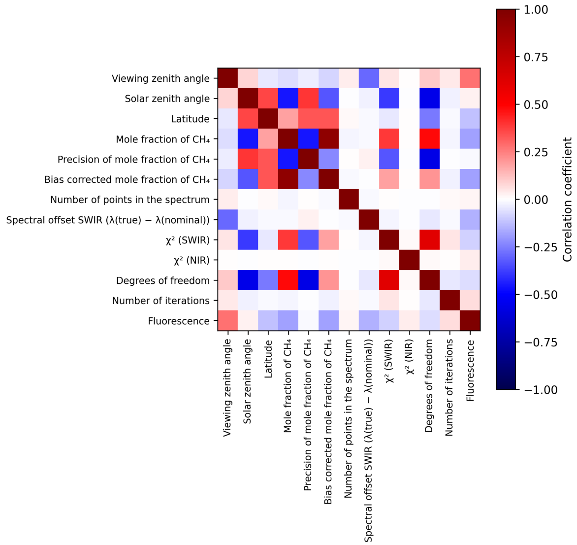
Figure 2: Map of correlation matrix for 2025-08-30 to 2025-09-01.
