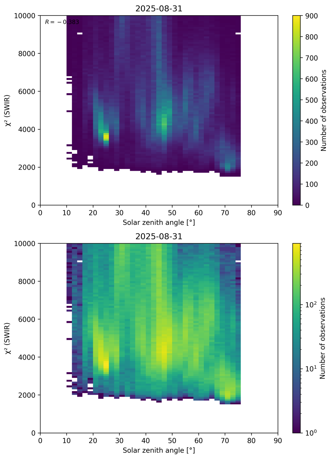
Figure 95: Scatter density plot of “Solar zenith angle” against “ \chi^2 (SWIR)” for 2025-08-30 to 2025-09-01.
