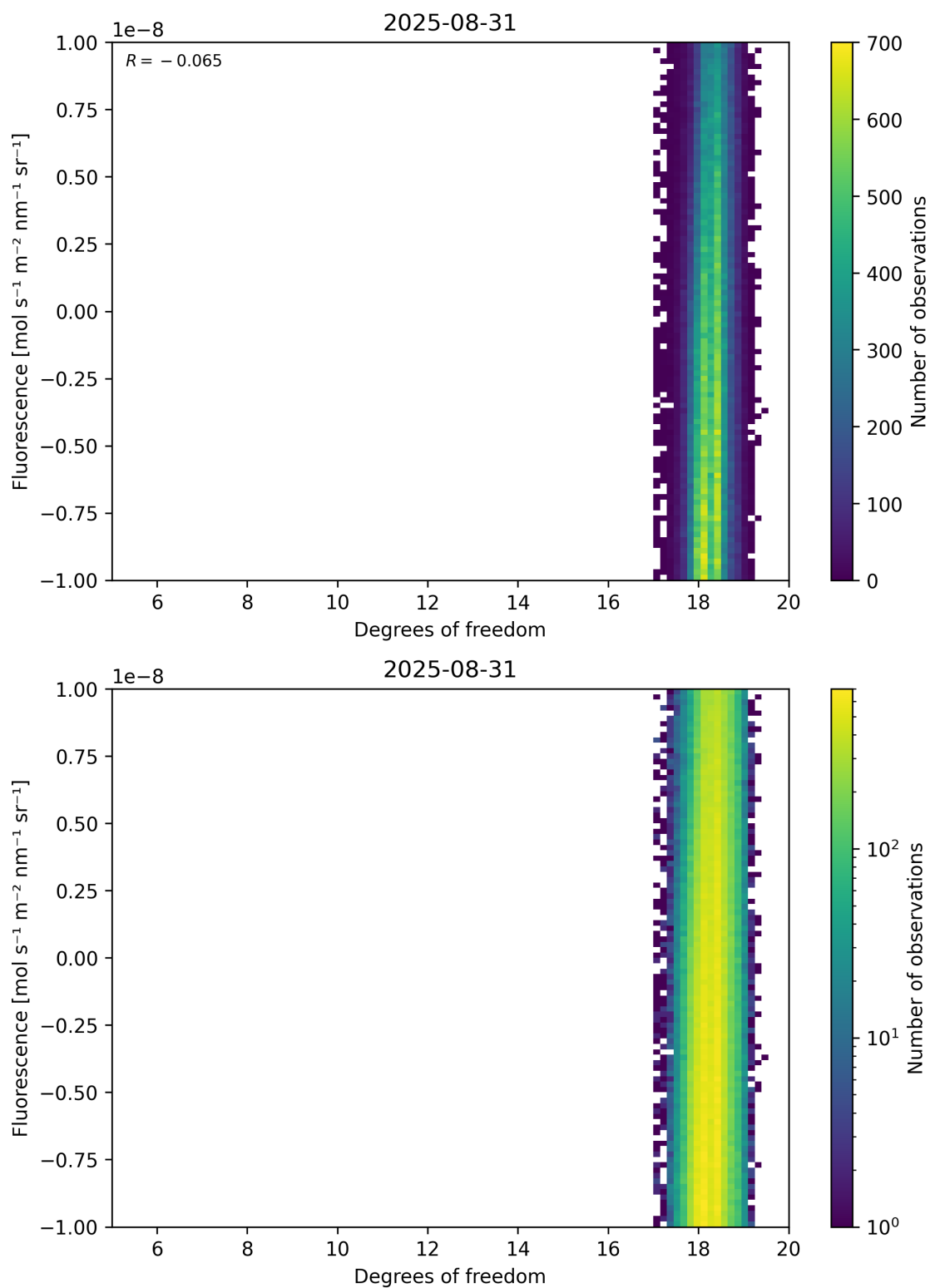
Figure 51: Scatter density plot of “Degrees of freedom” against “Fluorescence” for 2025-08-30 to 2025-09-01.
