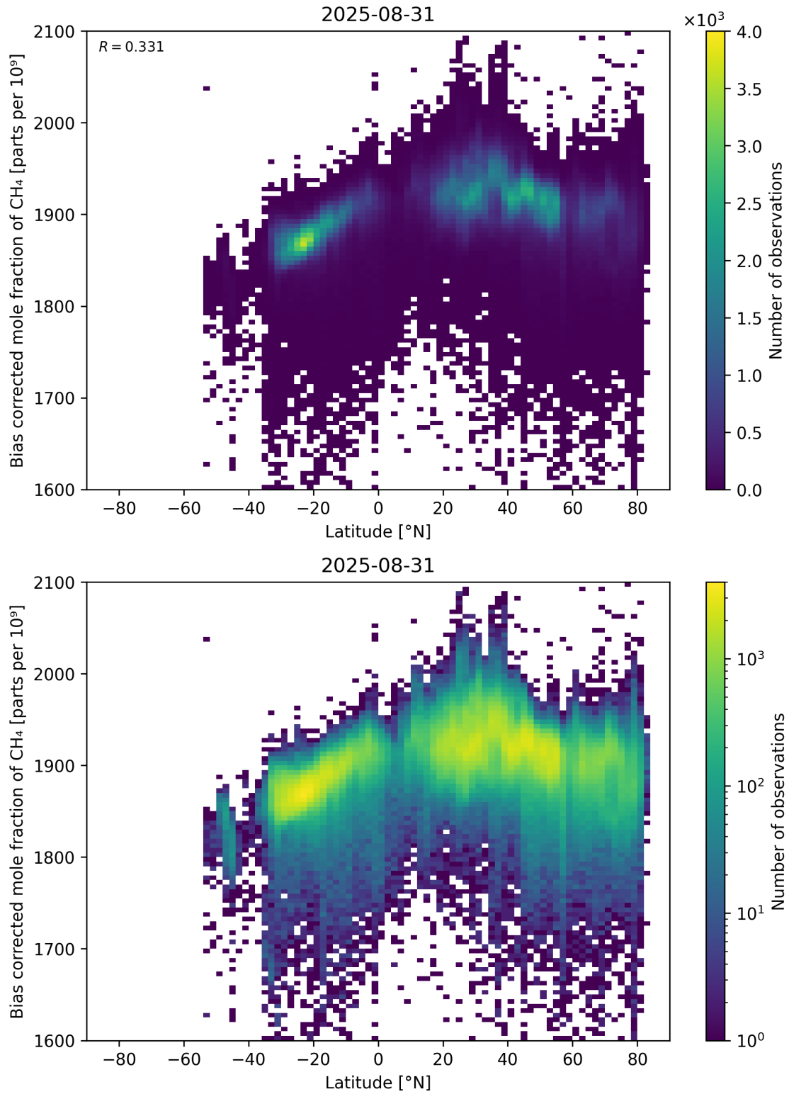
Figure 58: Scatter density plot of “Latitude” against “Bias corrected mole fraction of CH 4 ” for 2025-08-30 to 2025-09-01.
