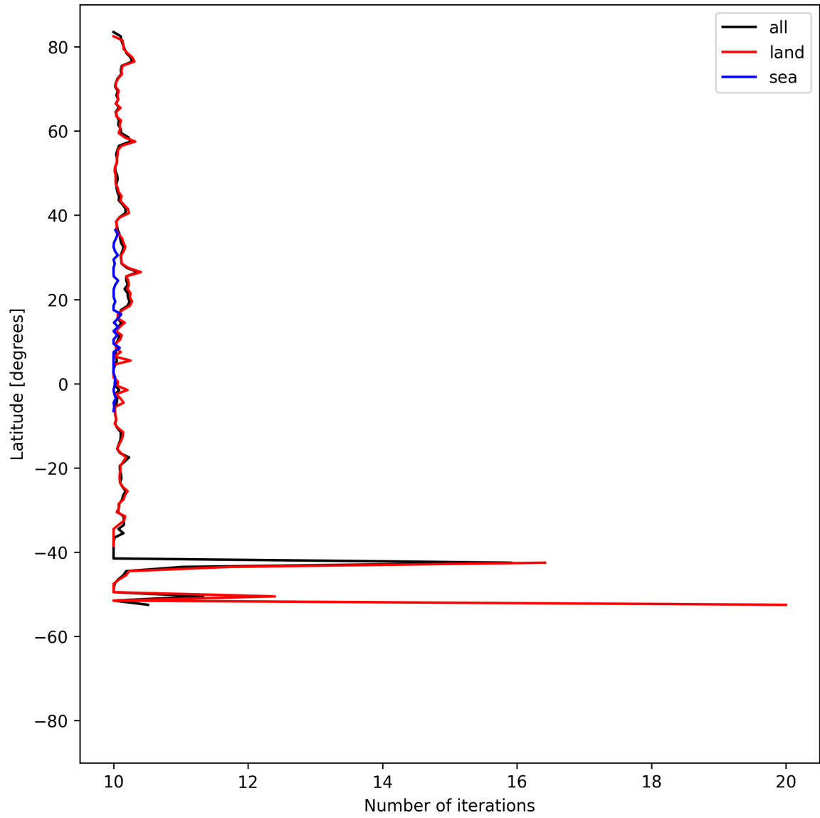
Figure 20: Zonal average of “Number of iterations” for 2025-08-30 to 2025-09-01.
