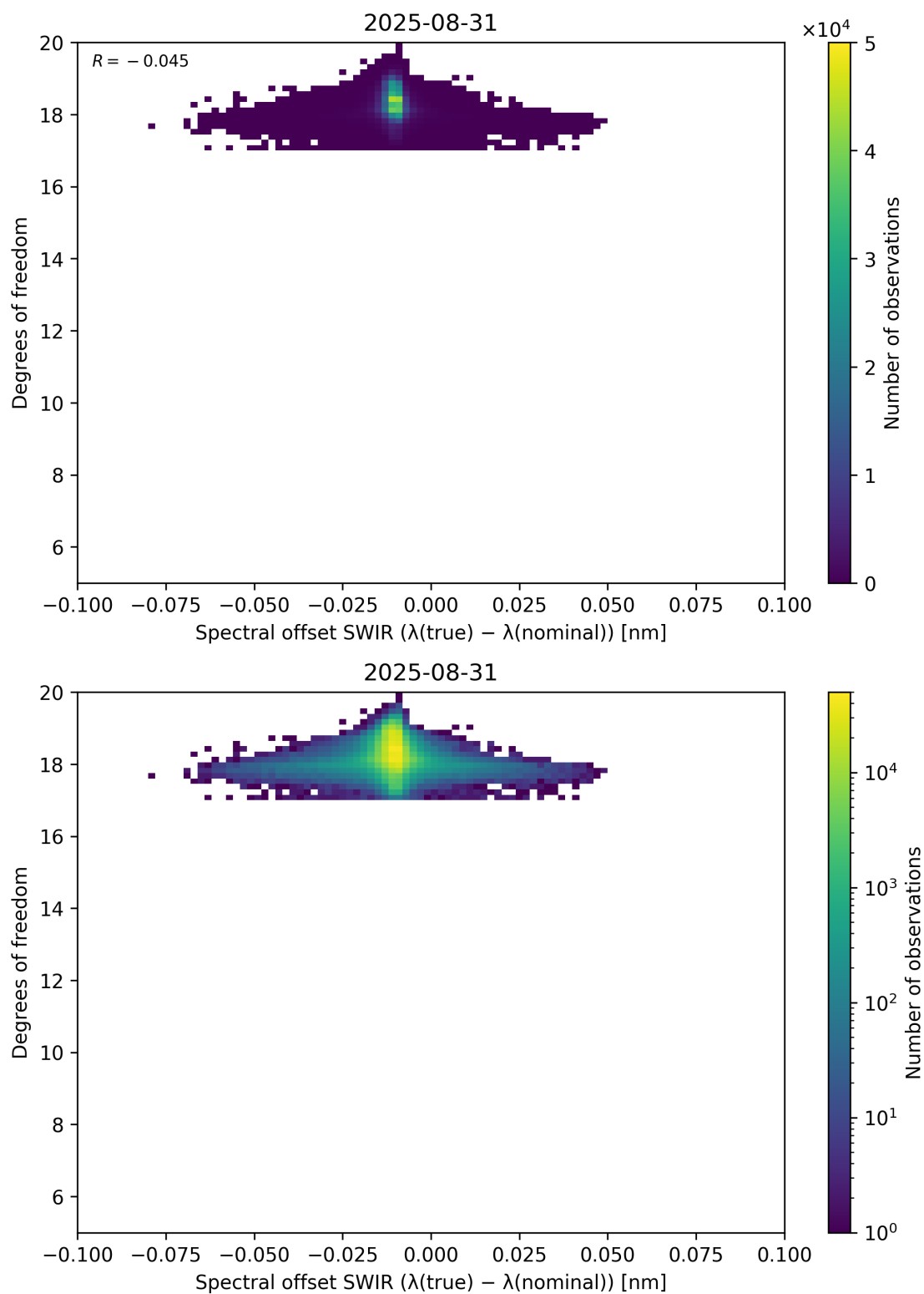
Figure 119: Scatter density plot of “Spectral offset SWIR ( \lambda_{\text{true}} - \lambda_{\text{nominal}} )” against “Degrees of freedom” for 2025-08-30 to 2025-09-01.
