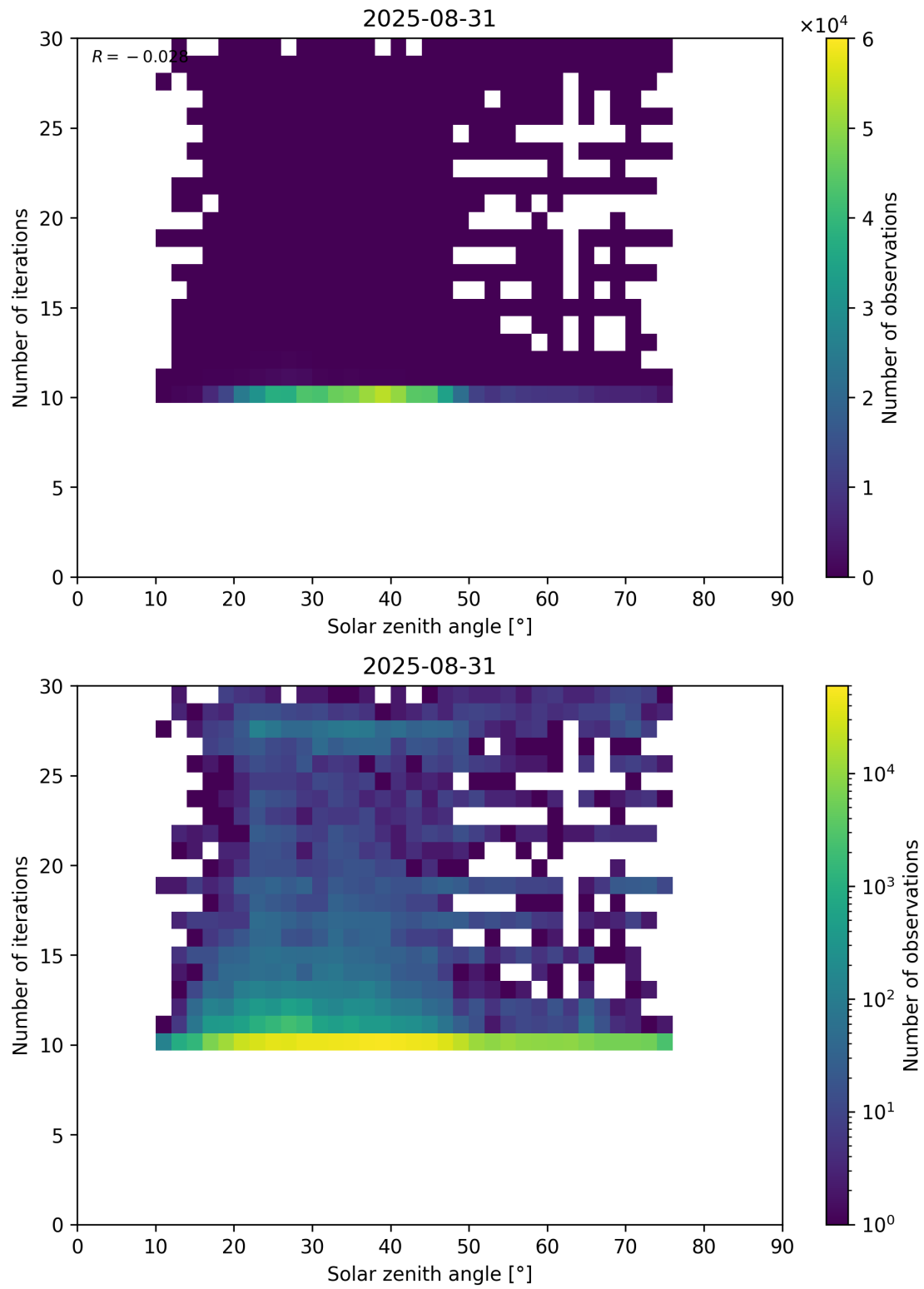
Figure 102: Scatter density plot of “Solar zenith angle” against “Number of iterations” for 2025-08-30 to 2025-09-01.
