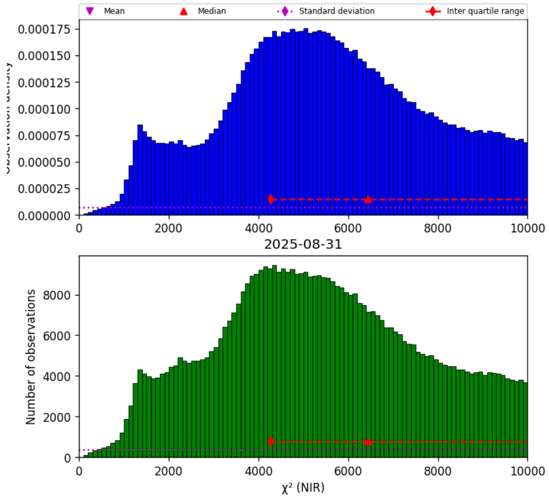
Figure 29: Histogram of “ \chi^2 (NIR)” for 2025-08-30 to 2025-09-01
