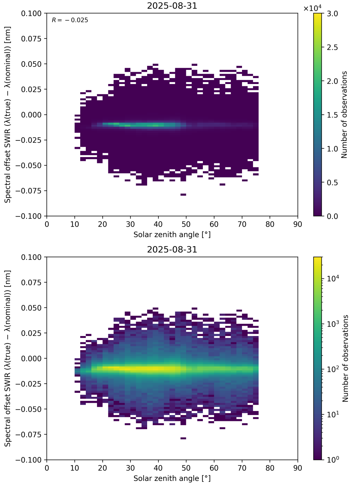
Figure 104: Scatter density plot of “Solar zenith angle” against “Spectral offset SWIR ( \lambda_{\text{true}} - \lambda_{\text{nominal}} )” for 2025-08-30 to 2025-09-01.
