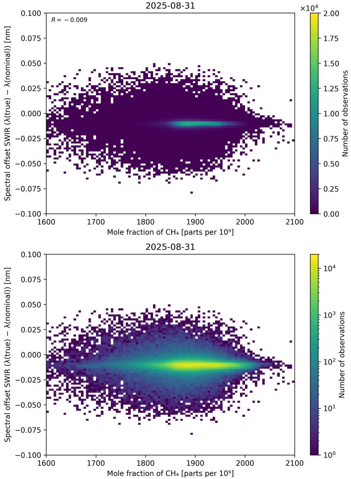
Figure 86: Scatter density plot of “Mole fraction of CH 4 ” against “Spectral offset SWIR ( \lambda_{\text{true}} - \lambda_{\text{nominal}} )” for 2025-08-30 to 2025-09-01.
