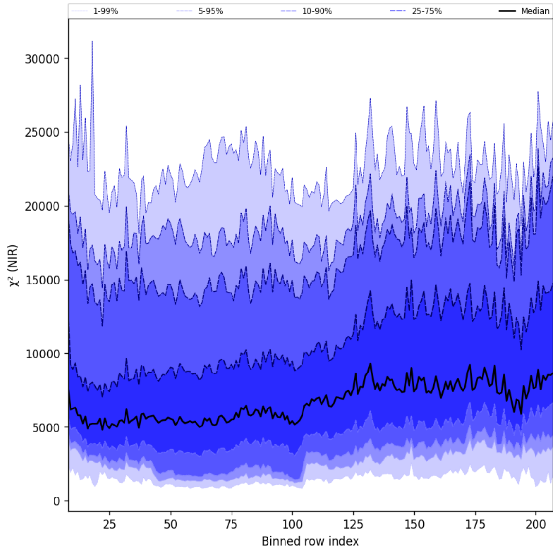
Figure 40: Along track statistics of “ \chi^2 (NIR)” for 2025-08-30 to 2025-09-01
