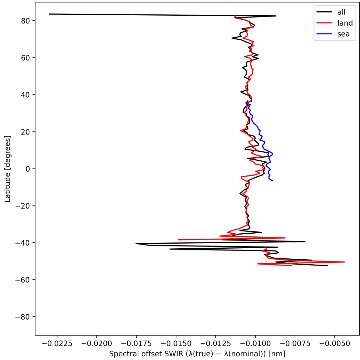
Figure 16: Zonal average of “Spectral offset SWIR ( \lambda_{\text{true}} - \lambda_{\text{nominal}} )” for 2025-08-30 to 2025-09-01.
