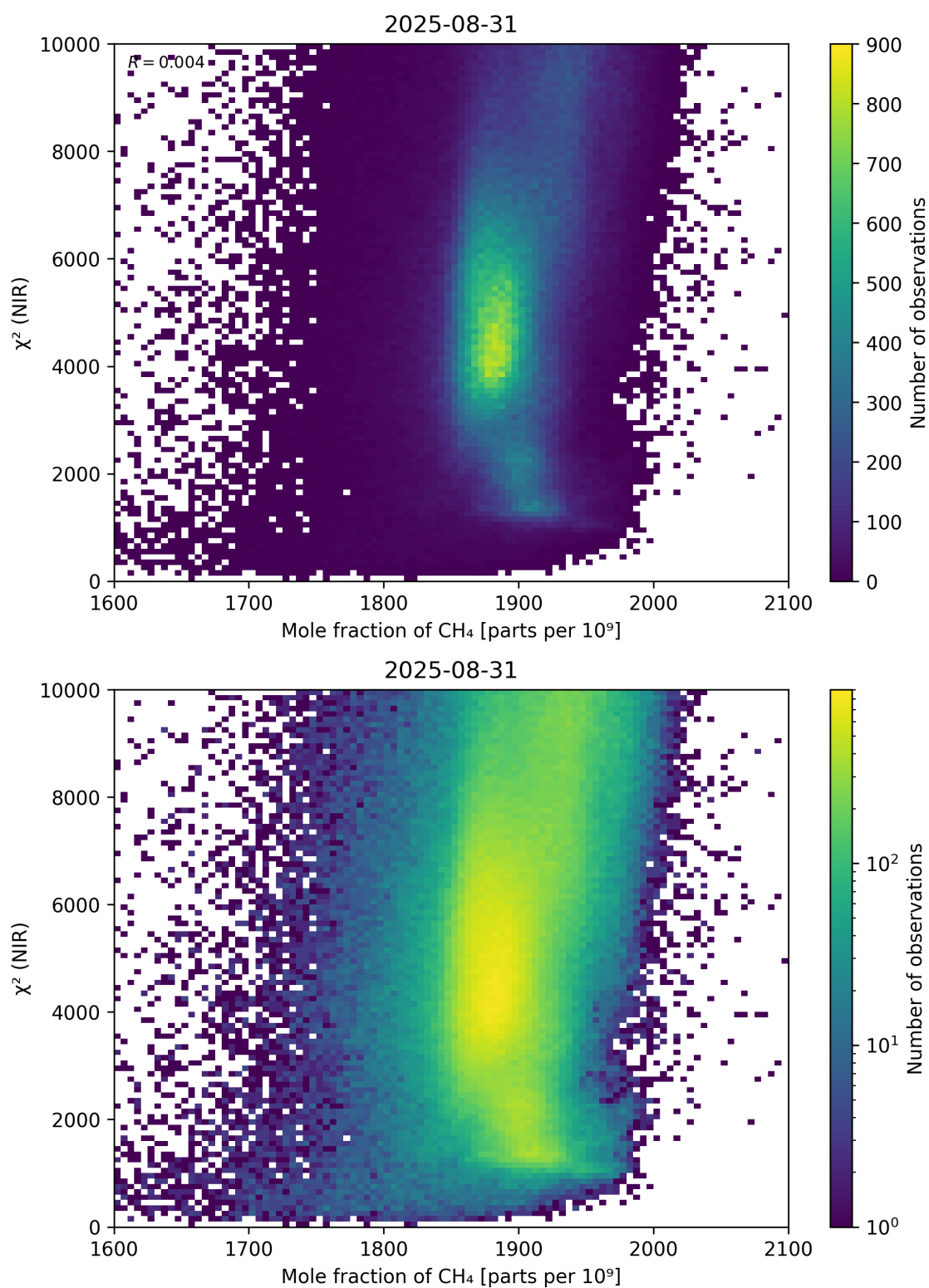
Figure 70: Scatter density plot of “Mole fraction of \text{CH}_4 ” against “ \chi^2 (NIR)” for 2025-08-30 to 2025-09-01.
