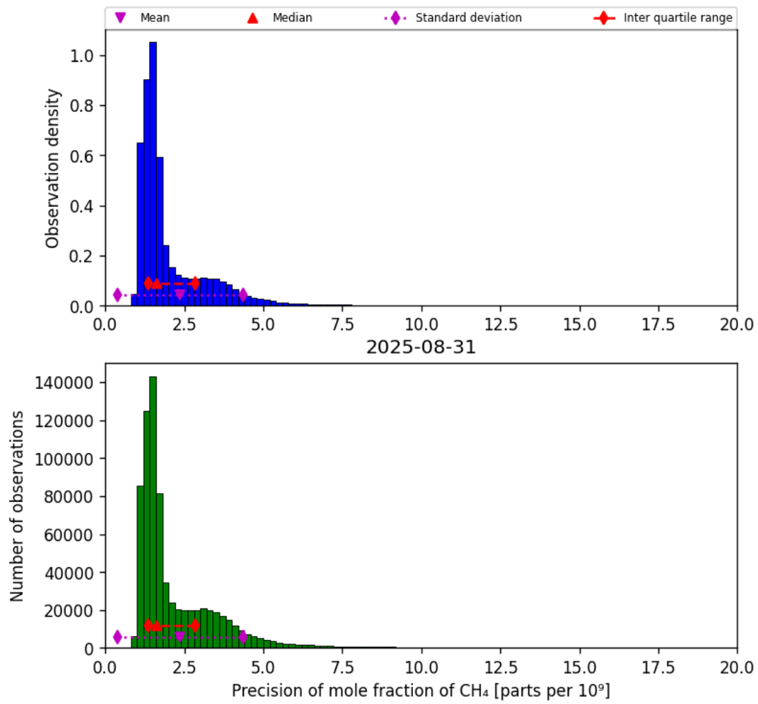
Figure 24: Histogram of “Precision of mole fraction of CH 4 ” for 2025-08-30 to 2025-09-01
