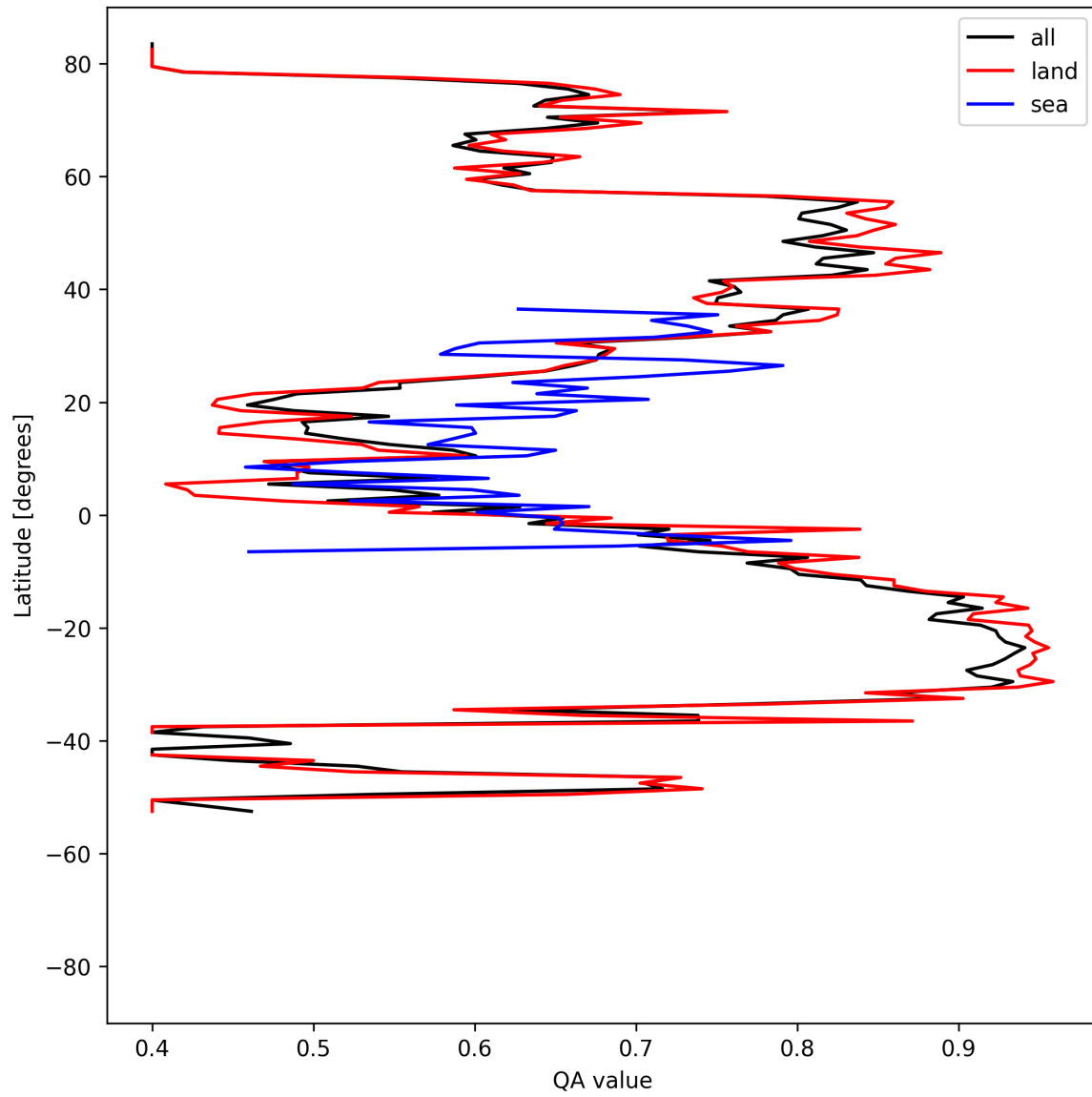
Figure 11: Zonal average of “QA value” for 2025-08-30 to 2025-09-01.
