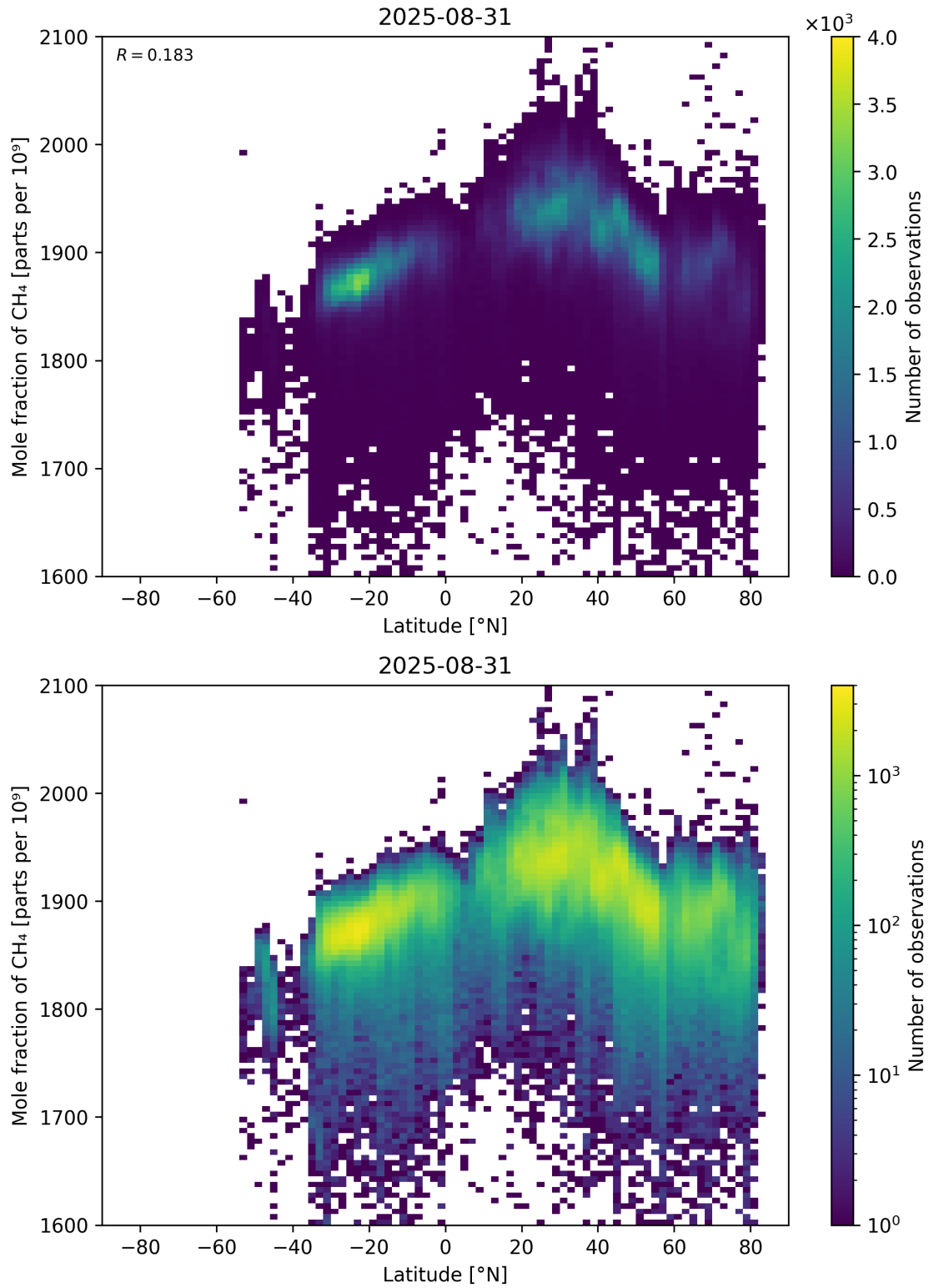
Figure 57: Scatter density plot of “Latitude” against “Mole fraction of CH 4 ” for 2025-08-30 to 2025-09-01.
