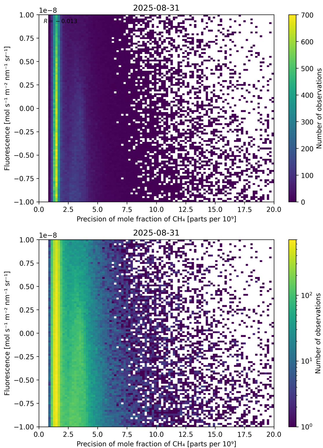
Figure 81: Scatter density plot of “Precision of mole fraction of \text{CH}_4 ” against “Fluorescence” for 2025-08-30 to 2025-09-01.
