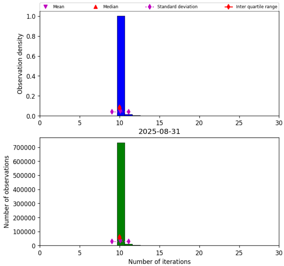
Figure 31: Histogram of "Number of iterations" for 2025-08-30 to 2025-09-01
