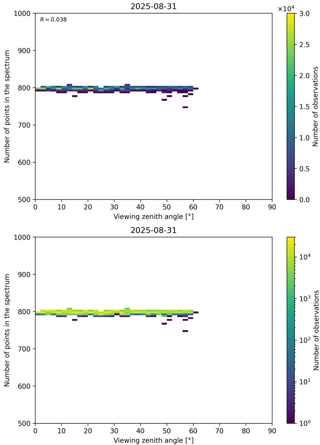
Figure 114: Scatter density plot of “Viewing zenith angle” against “Number of points in the spectrum” for 2025-08-30 to 2025-09-01.
