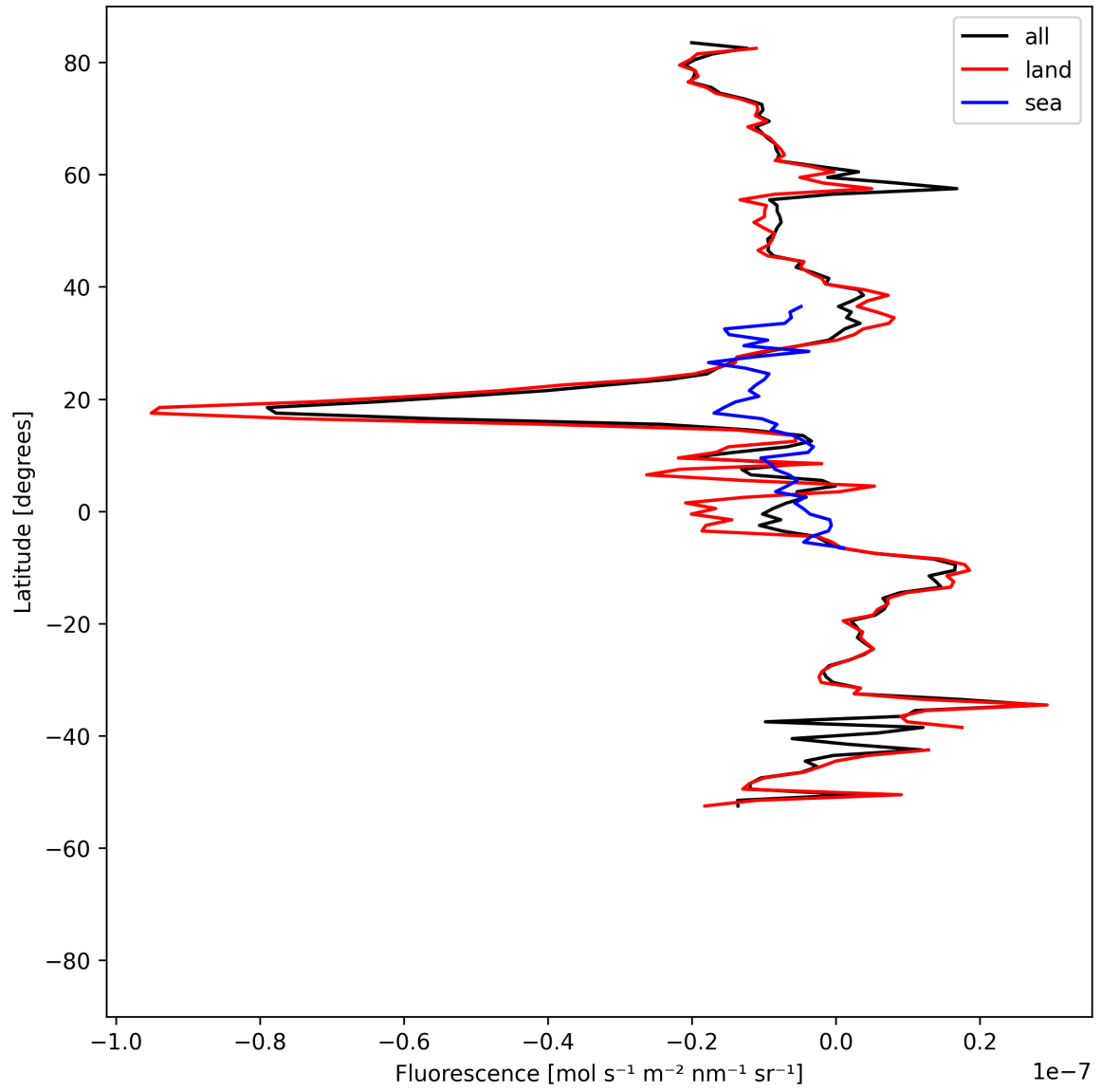
Figure 21: Zonal average of “Fluorescence” for 2025-08-30 to 2025-09-01.
