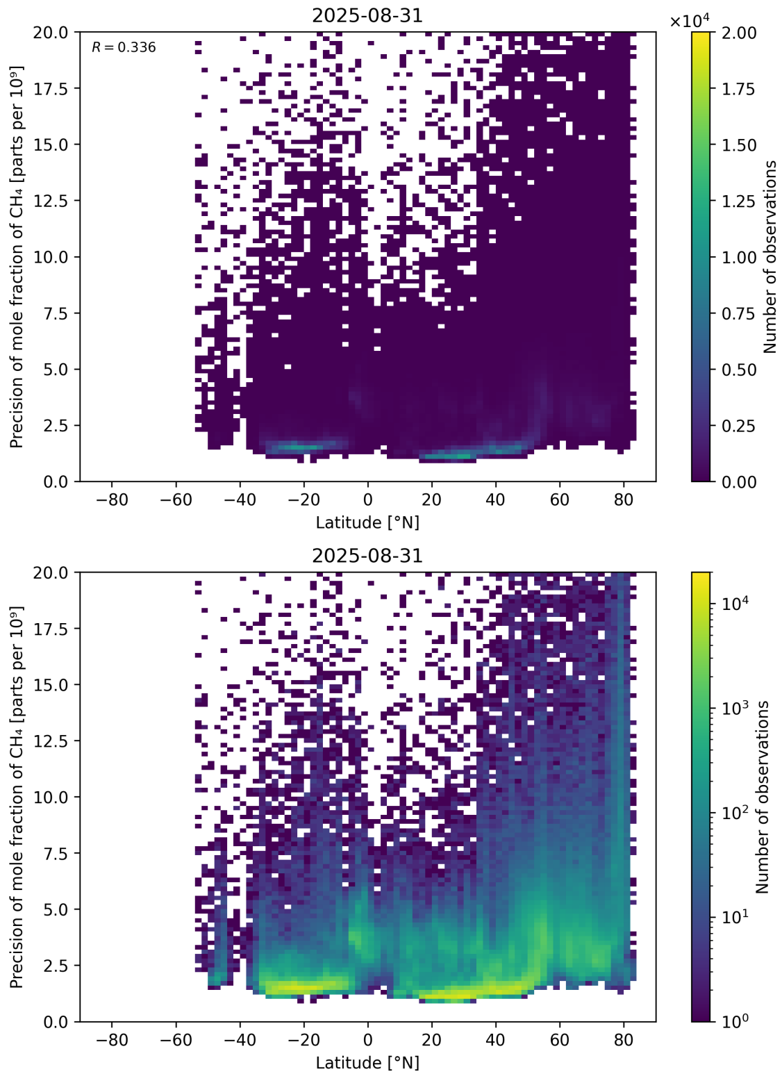
Figure 59: Scatter density plot of “Latitude” against “Precision of mole fraction of \text{CH}_4 ” for 2025-08-30 to 2025-09-01.
