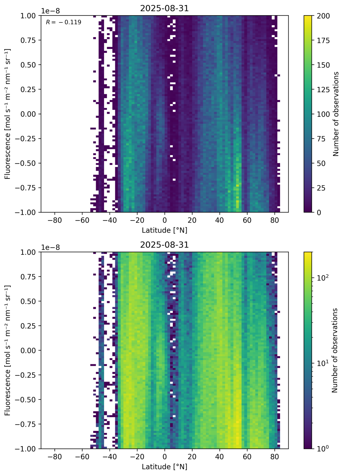
Figure 56: Scatter density plot of “Latitude” against “Fluorescence” for 2025-08-30 to 2025-09-01.
