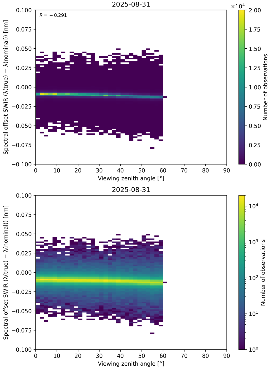
Figure 116: Scatter density plot of “Viewing zenith angle” against “Spectral offset SWIR ( \lambda_{\text{true}} - \lambda_{\text{nominal}} )” for 2025-08-30 to 2025-09-01.
