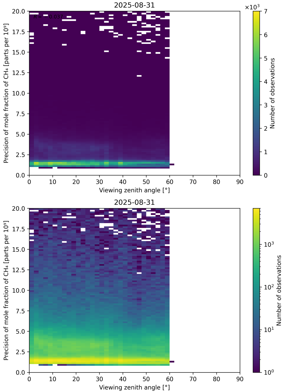
Figure 112: Scatter density plot of “Viewing zenith angle” against “Precision of mole fraction of CH 4 ” for 2025-08-30 to 2025-09-01.
