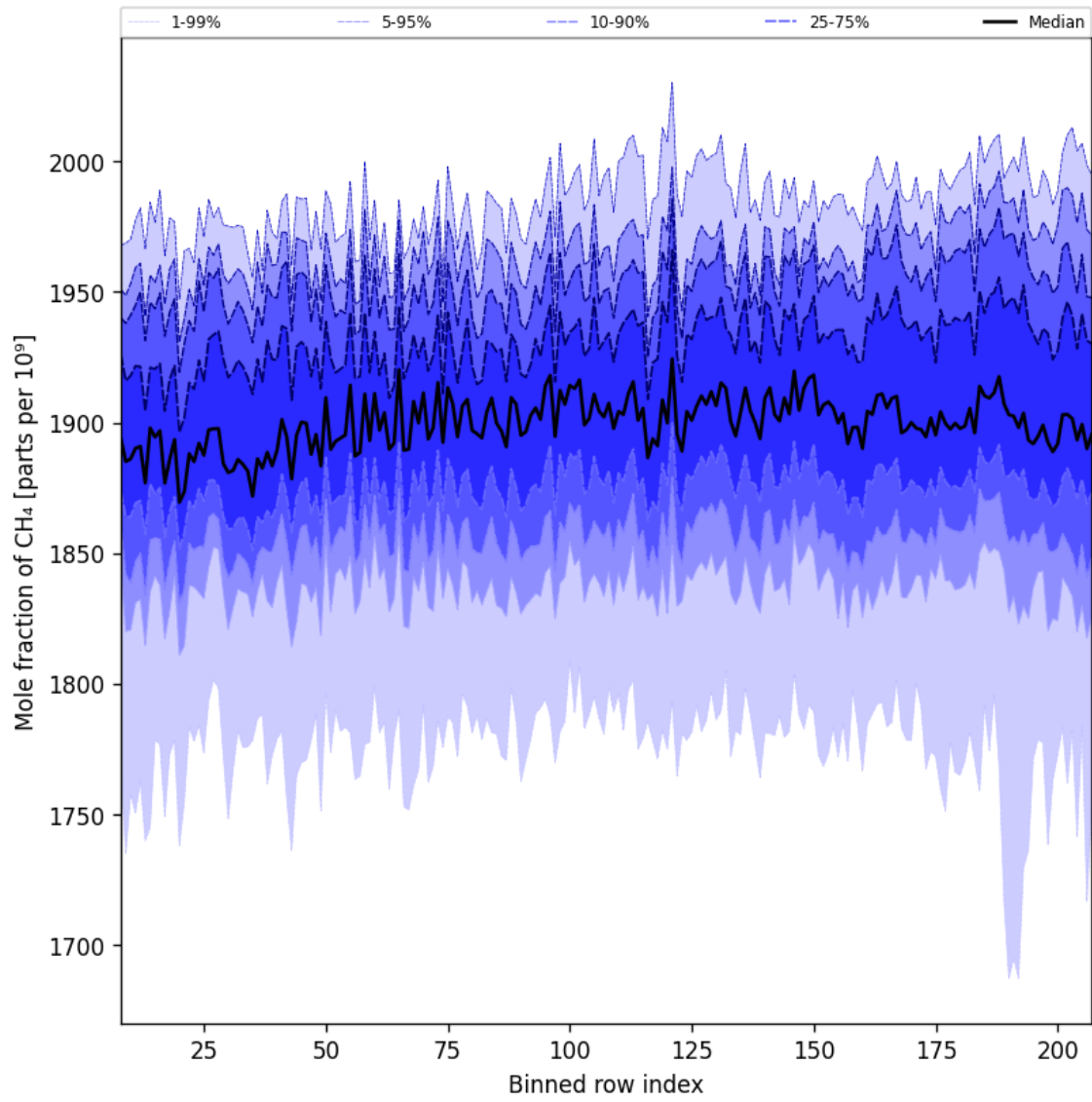
Figure 34: Along track statistics of “Mole fraction of CH 4 ” for 2025-08-30 to 2025-09-01
