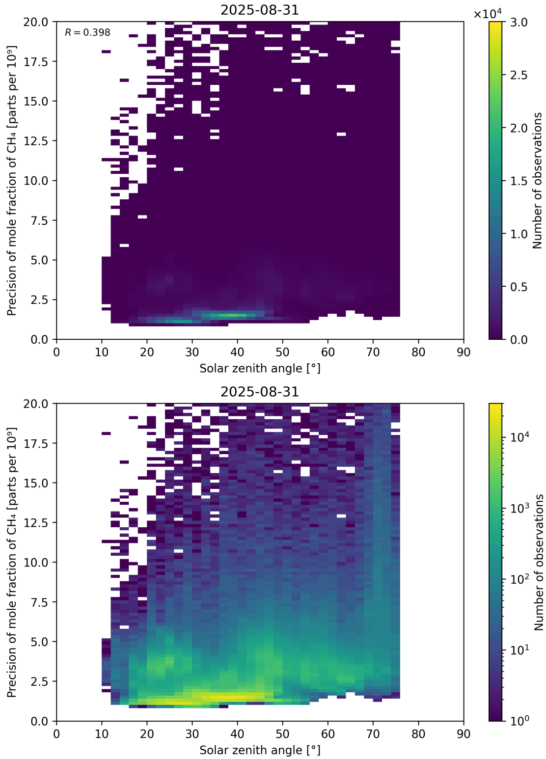
Figure 101: Scatter density plot of “Solar zenith angle” against “Precision of mole fraction of \text{CH}_4 ” for 2025-08-30 to 2025-09-01.
