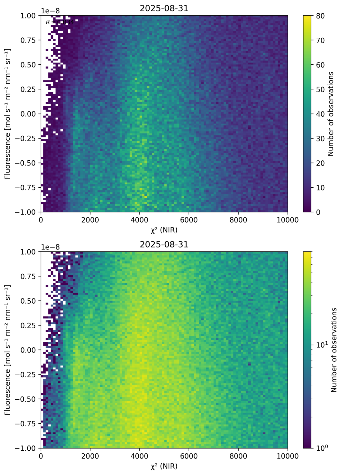
Figure 45: Scatter density plot of “ \chi^2 (NIR)” against “Fluorescence” for 2025-08-30 to 2025-09-01.
