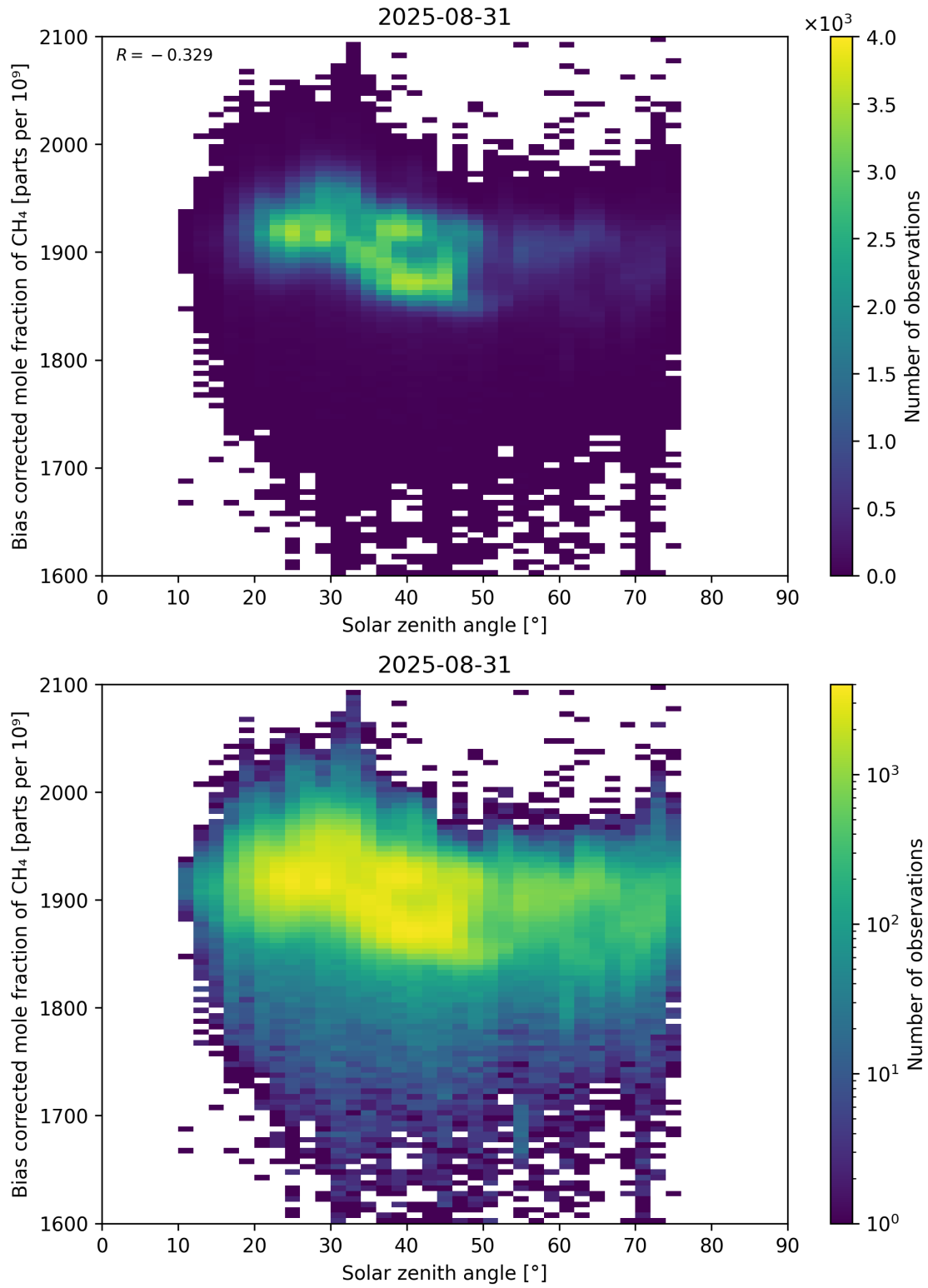
Figure 100: Scatter density plot of “Solar zenith angle” against “Bias corrected mole fraction of CH 4 ” for 2025-08-30 to 2025-09-01.
