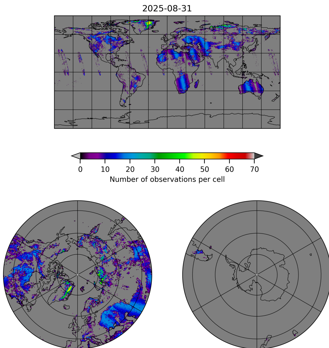
Figure 10: Map of the number of observations for 2025-08-30 to 2025-09-01
