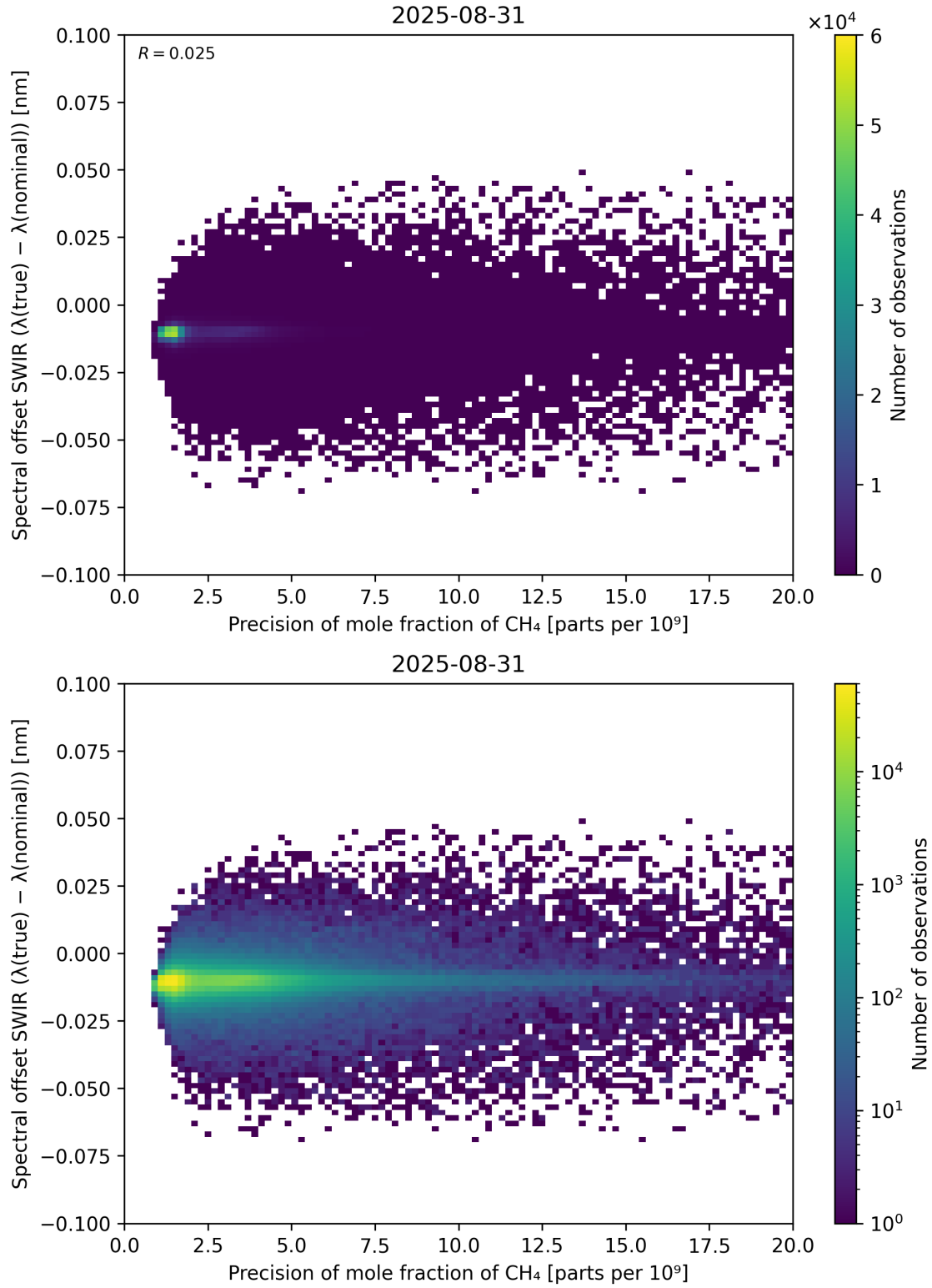
Figure 85: Scatter density plot of “Precision of mole fraction of CH 4 ” against “Spectral offset SWIR ( \lambda_{\text{true}} - \lambda_{\text{nominal}} )” for 2025-08-30 to 2025-09-01.
