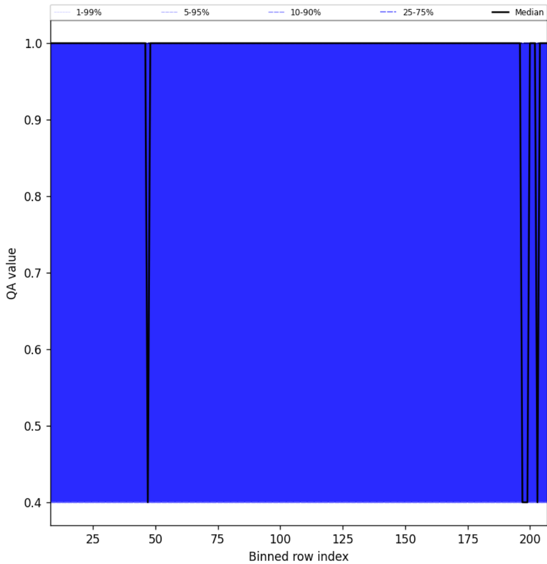
Figure 33: Along track statistics of “QA value” for 2025-08-30 to 2025-09-01
