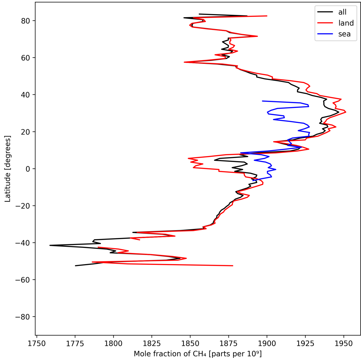
Figure 12: Zonal average of “Mole fraction of CH 4 ” for 2025-08-30 to 2025-09-01.
