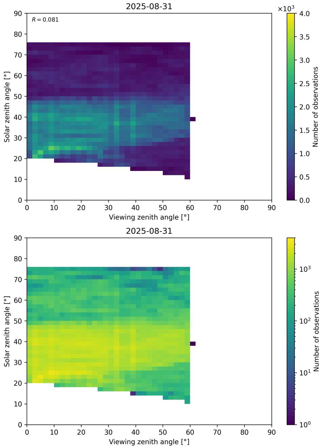
Figure 115: Scatter density plot of “Viewing zenith angle” against “Solar zenith angle” for 2025-08-30 to 2025-09-01.
