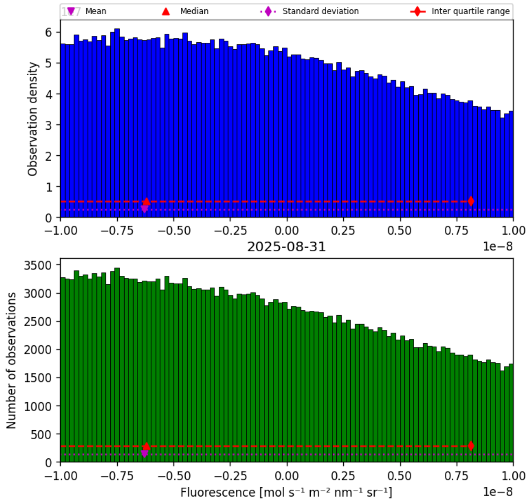
Figure 32: Histogram of “Fluorescence” for 2025-08-30 to 2025-09-01
