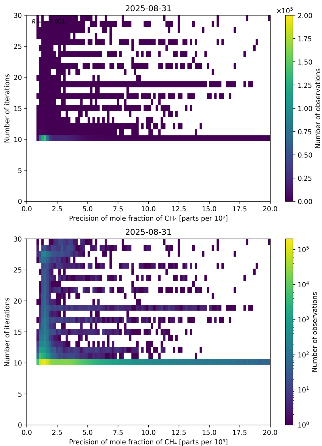
Figure 83: Scatter density plot of “Precision of mole fraction of CH 4 ” against “Number of iterations” for 2025-08-30 to 2025-09-01.
