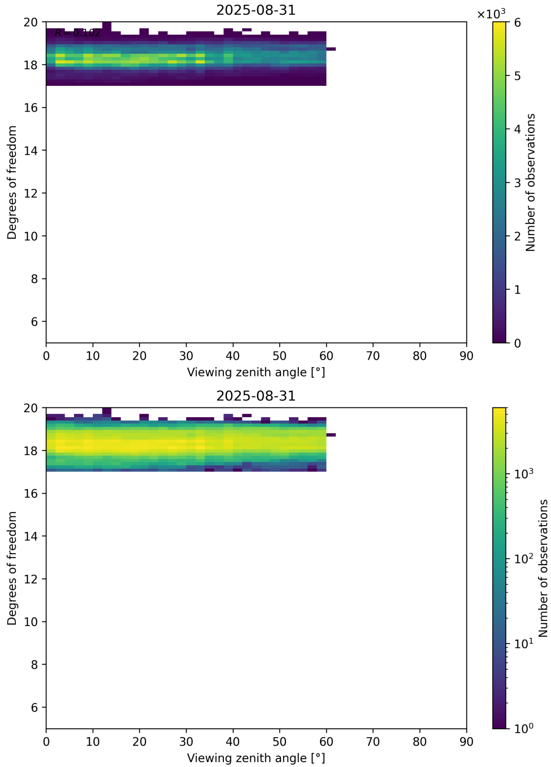
Figure 107: Scatter density plot of “Viewing zenith angle” against “Degrees of freedom” for 2025-08-30 to 2025-09-01.
