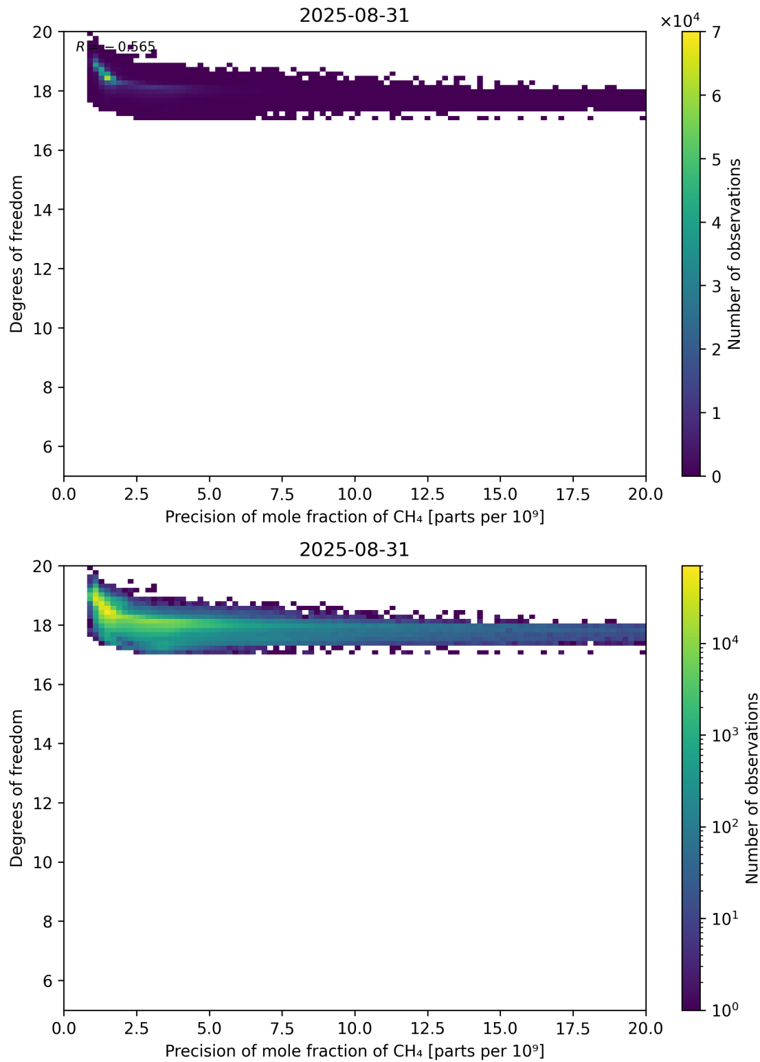
Figure 80: Scatter density plot of “Precision of mole fraction of CH 4 ” against “Degrees of freedom” for 2025-08-30 to 2025-09-01.
