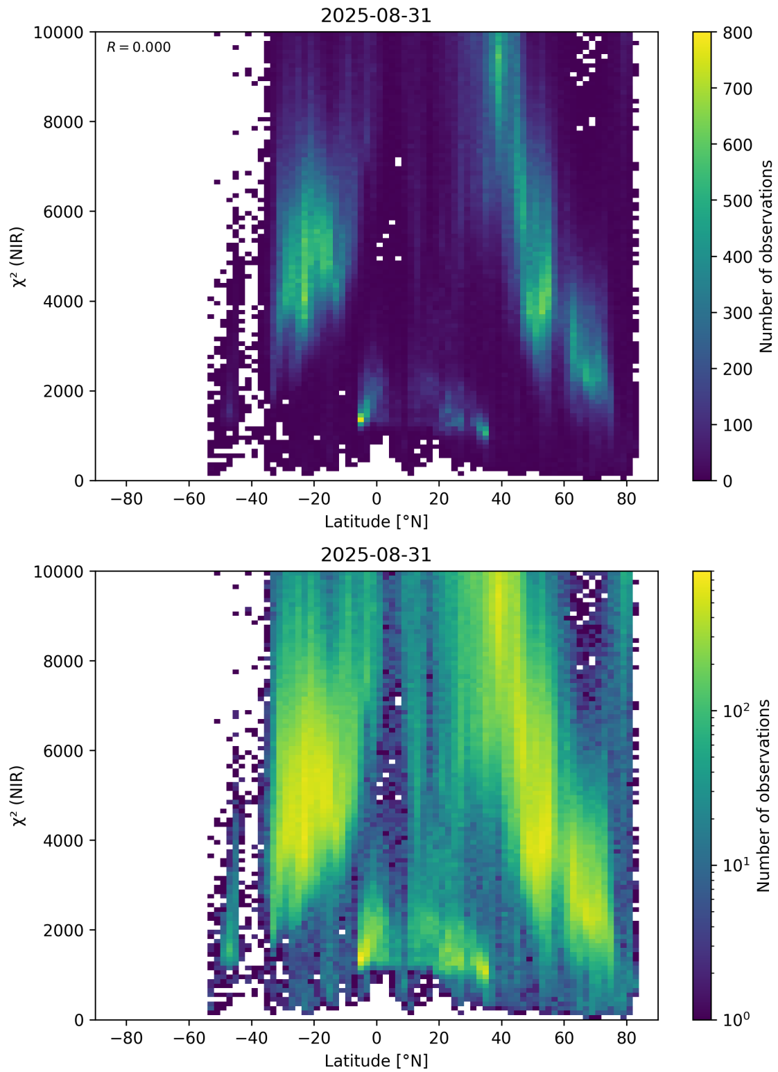
Figure 53: Scatter density plot of “Latitude” against “ \chi^2 (NIR)” for 2025-08-30 to 2025-09-01.
