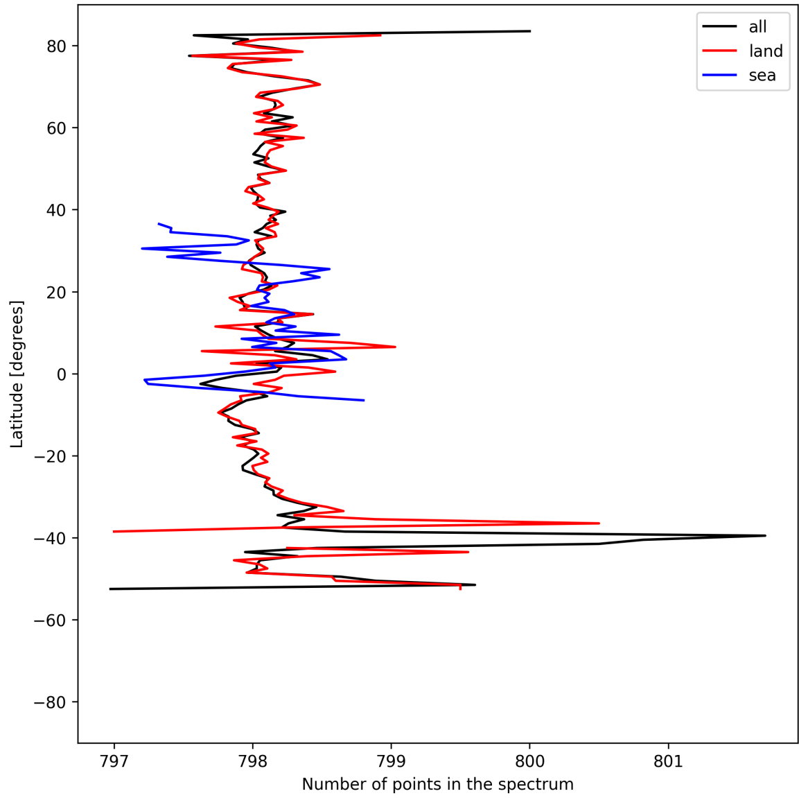
Figure 15: Zonal average of “Number of points in the spectrum” for 2025-08-30 to 2025-09-01.
