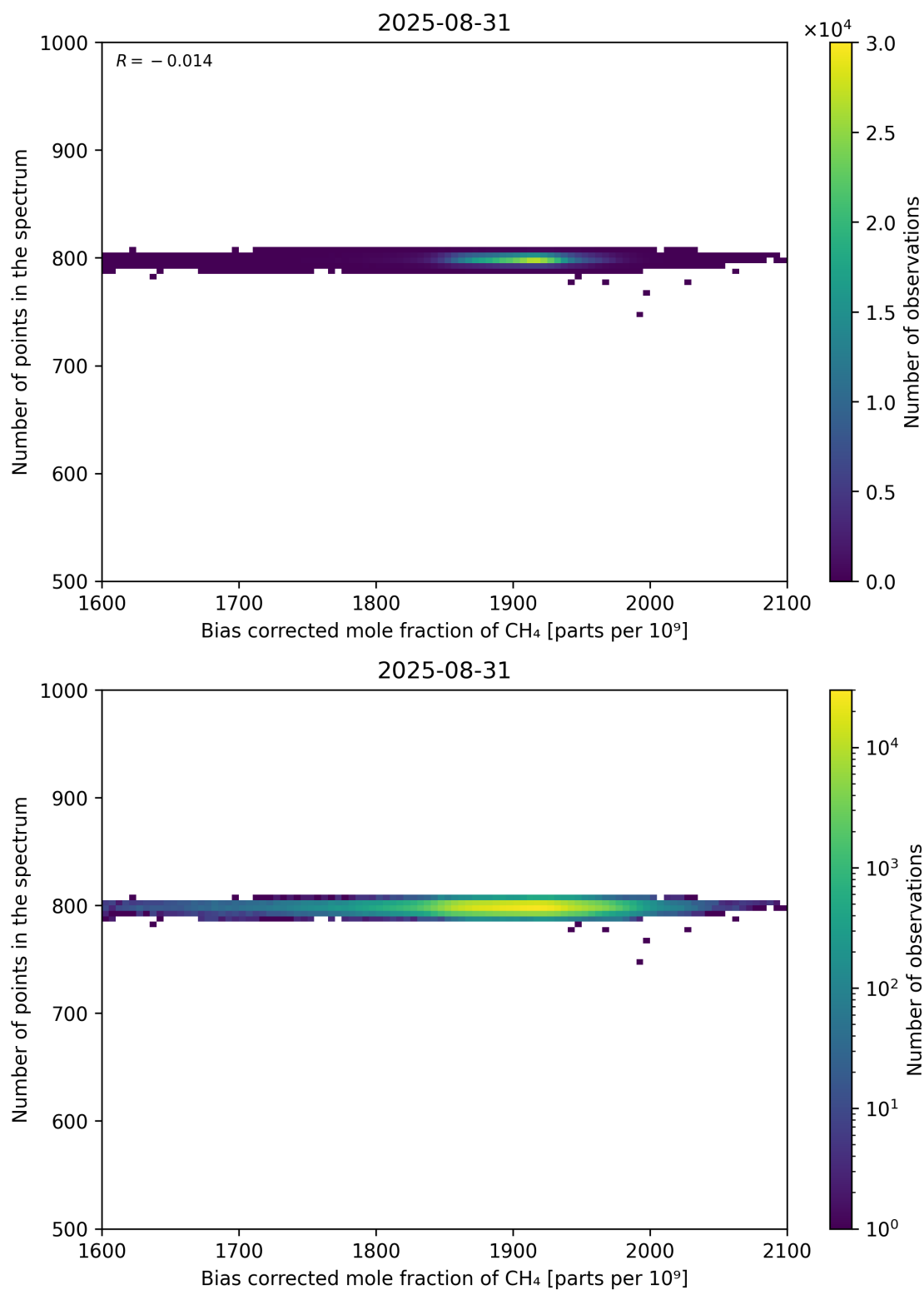
Figure 68: Scatter density plot of “Bias corrected mole fraction of CH 4 ” against “Number of points in the spectrum” for 2025-08-30 to 2025-09-01.
