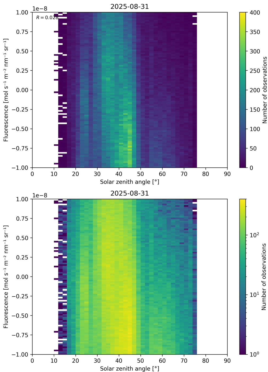
Figure 97: Scatter density plot of “Solar zenith angle” against “Fluorescence” for 2025-08-30 to 2025-09-01.
