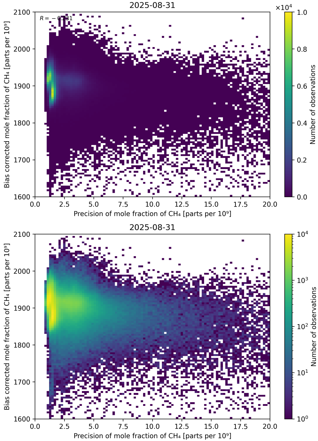
Figure 82: Scatter density plot of “Precision of mole fraction of CH 4 ” against “Bias corrected mole fraction of CH 4 ” for 2025-08-30 to 2025-09-01.
