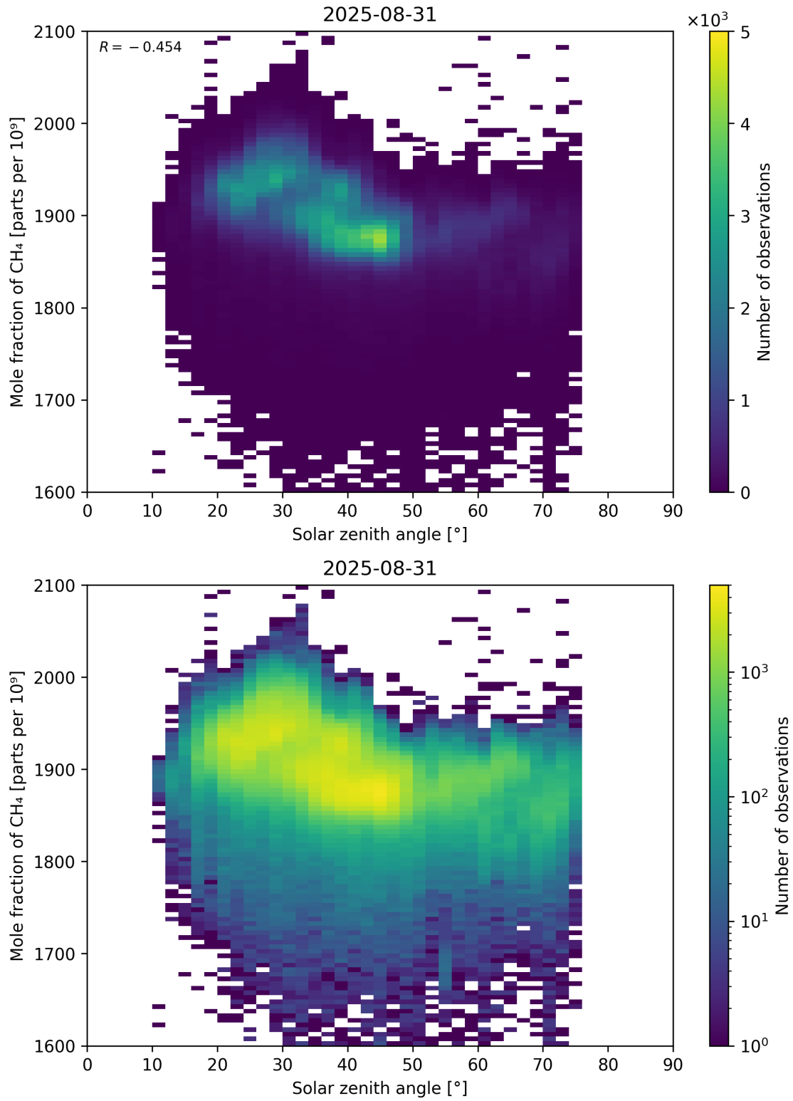
Figure 99: Scatter density plot of “Solar zenith angle” against “Mole fraction of \text{CH}_4 ” for 2025-08-30 to 2025-09-01.
