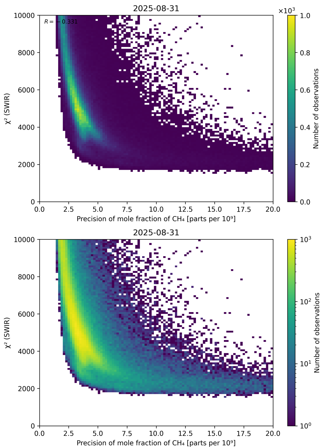
Figure 79: Scatter density plot of “Precision of mole fraction of \text{CH}_4 ” against “ \chi^2 (SWIR)” for 2025-08-30 to 2025-09-01.
