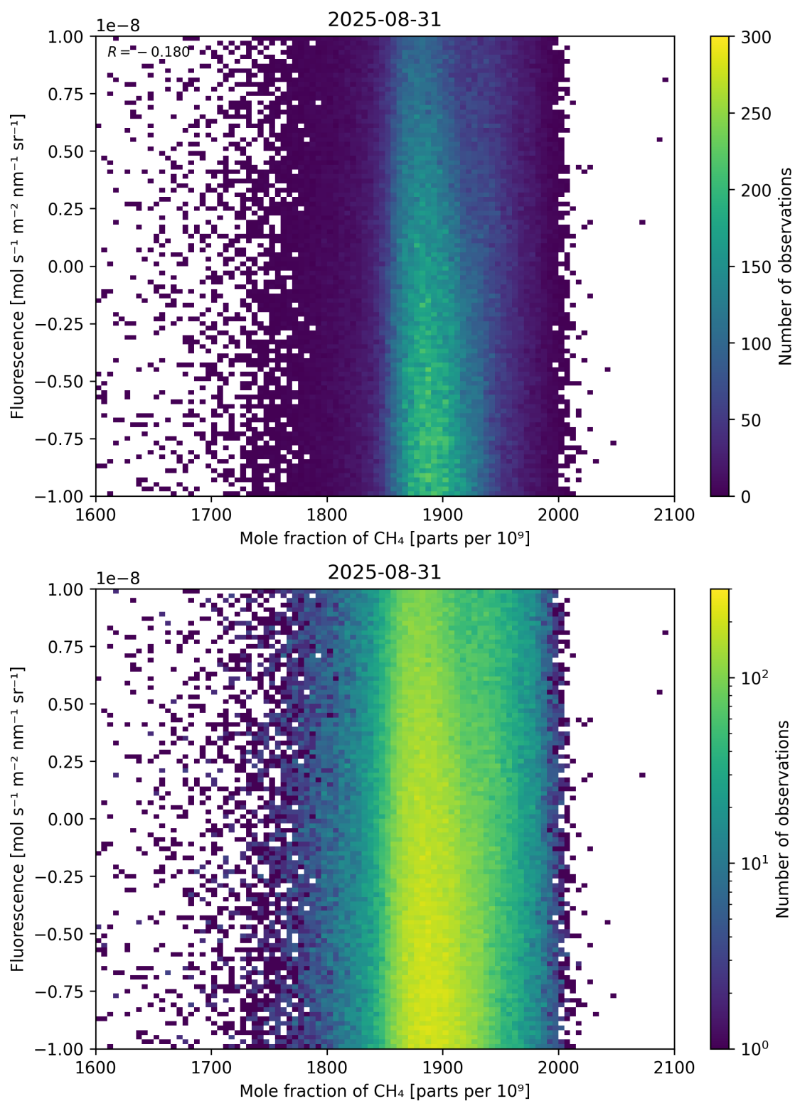
Figure 73: Scatter density plot of “Mole fraction of \text{CH}_4 ” against “Fluorescence” for 2025-08-30 to 2025-09-01.
