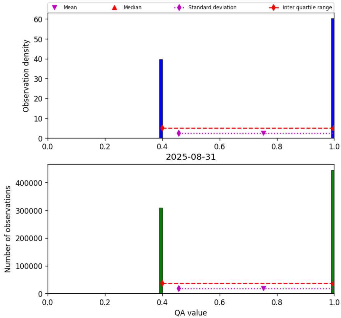
Figure 22: Histogram of “QA value” for 2025-08-30 to 2025-09-01
