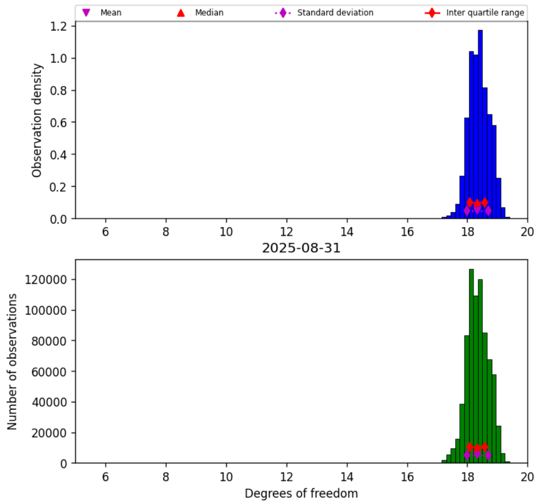
Figure 30: Histogram of “Degrees of freedom” for 2025-08-30 to 2025-09-01
