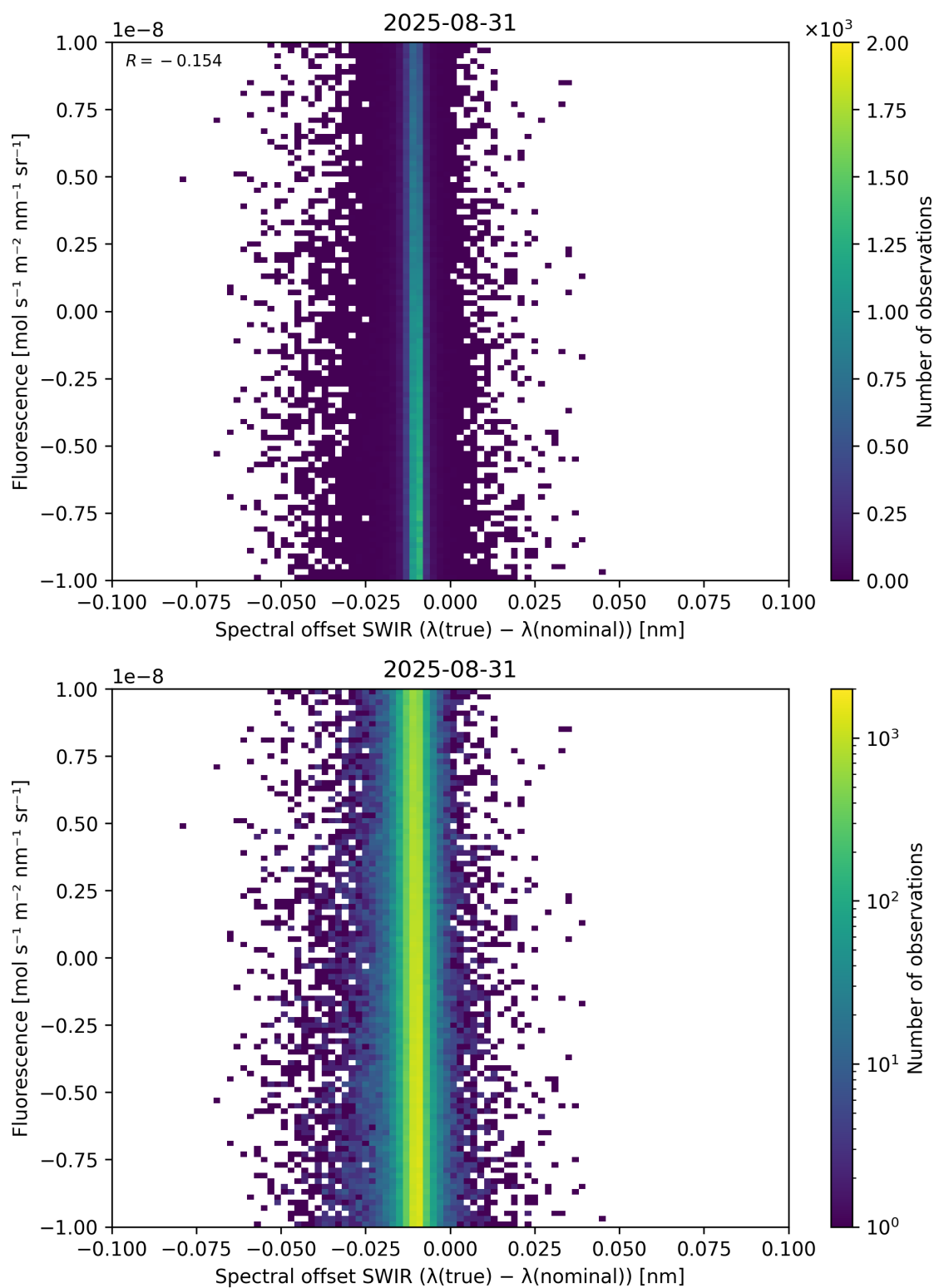
Figure 120: Scatter density plot of “Spectral offset SWIR ( \lambda_{\text{true}} - \lambda_{\text{nominal}} )” against “Fluorescence” for 2025-08-30 to 2025-09-01.
