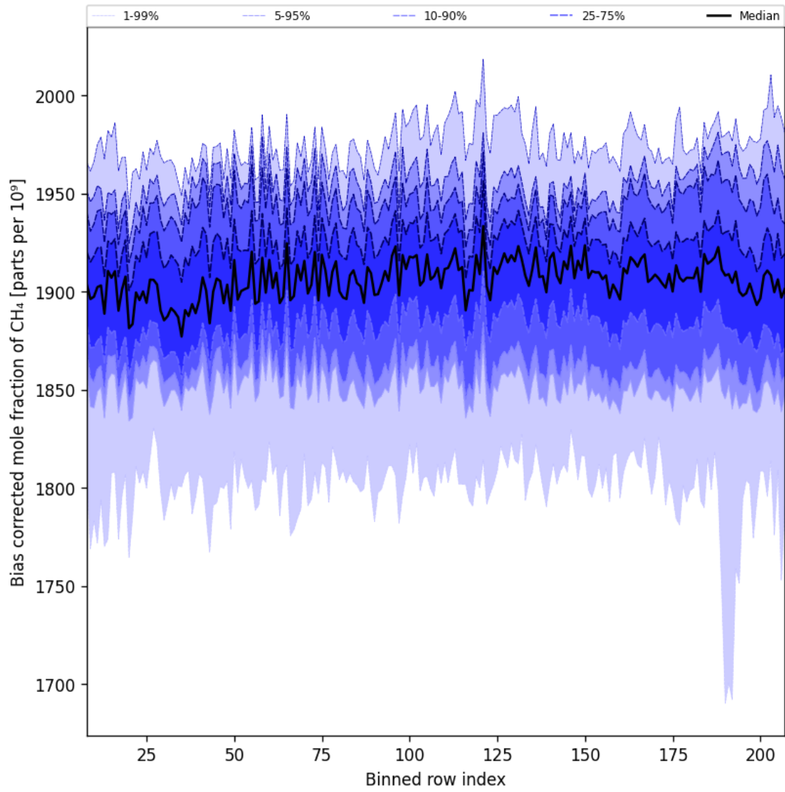
Figure 36: Along track statistics of “Bias corrected mole fraction of CH 4 ” for 2025-08-30 to 2025-09-01
