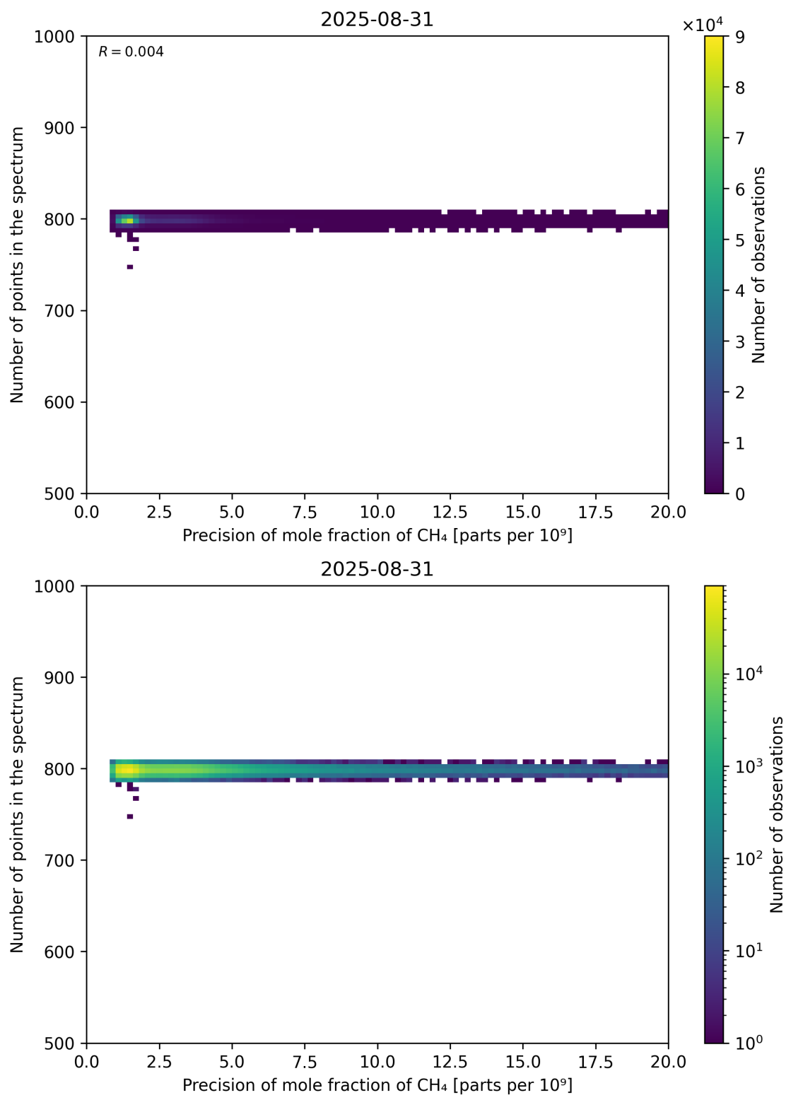
Figure 84: Scatter density plot of “Precision of mole fraction of CH 4 ” against “Number of points in the spectrum” for 2025-08-30 to 2025-09-01.
