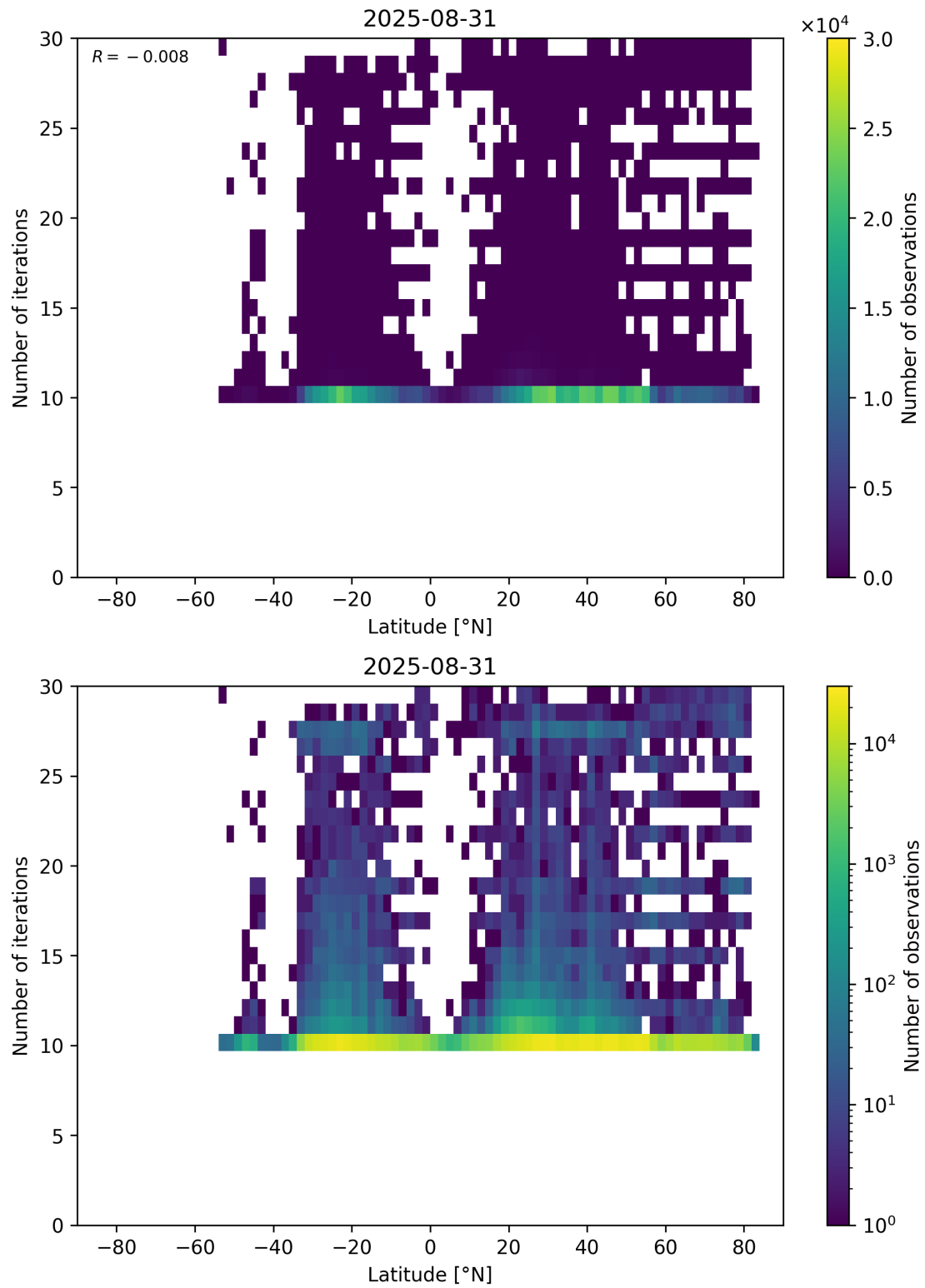
Figure 60: Scatter density plot of “Latitude” against “Number of iterations” for 2025-08-30 to 2025-09-01.
