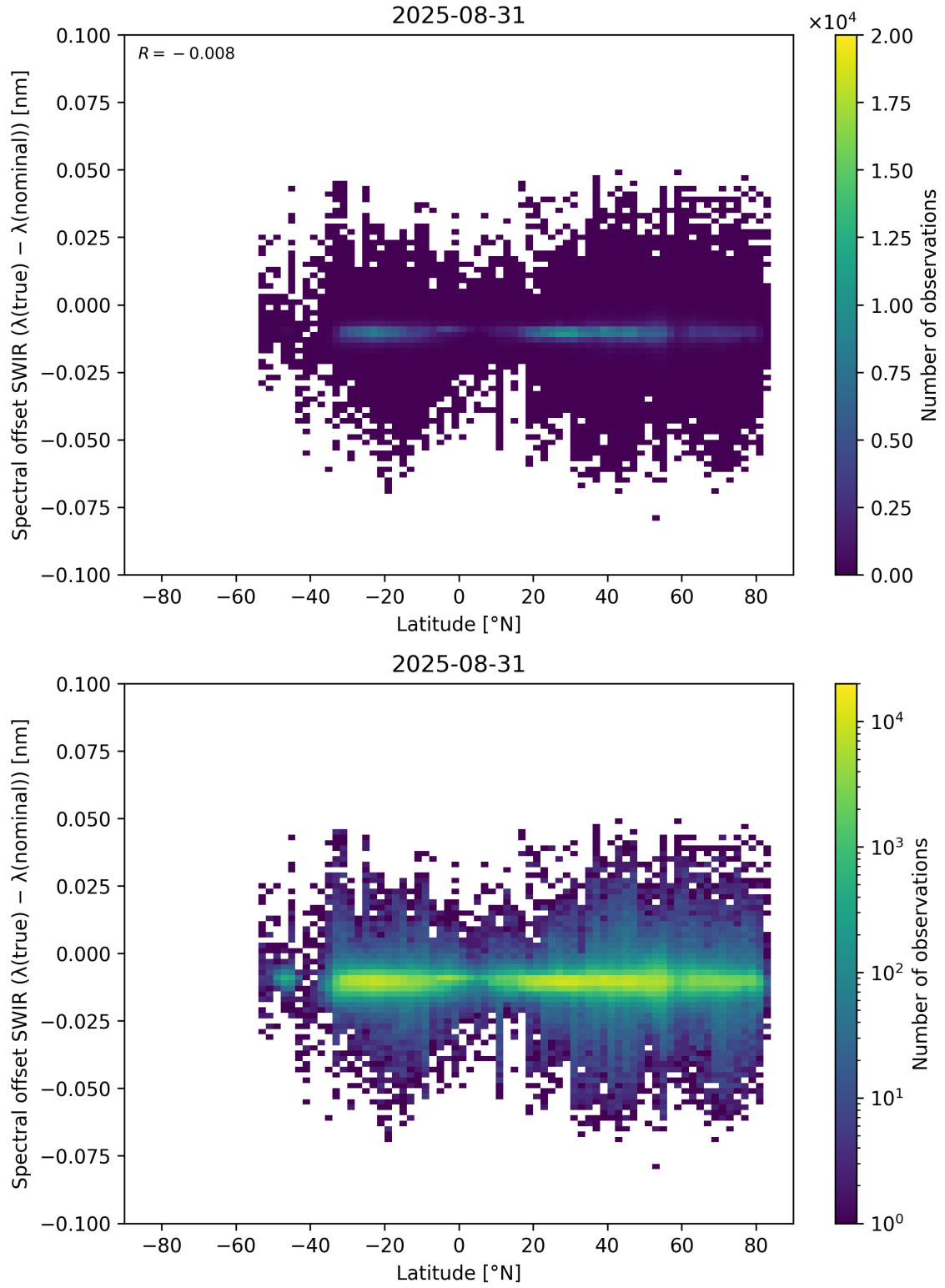
Figure 62: Scatter density plot of “Latitude” against “Spectral offset SWIR ( \lambda_{\text{true}} - \lambda_{\text{nominal}} )” for 2025-08-30 to 2025-09-01.
