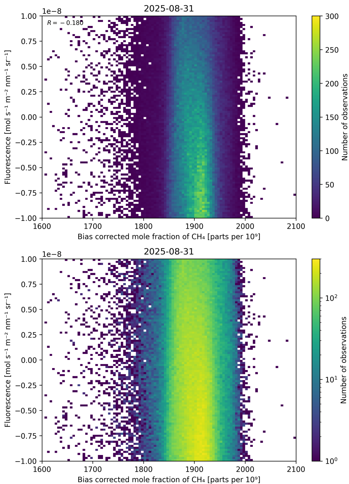
Figure 66: Scatter density plot of “Bias corrected mole fraction of \text{CH}_4 ” against “Fluorescence” for 2025-08-30 to 2025-09-01.
