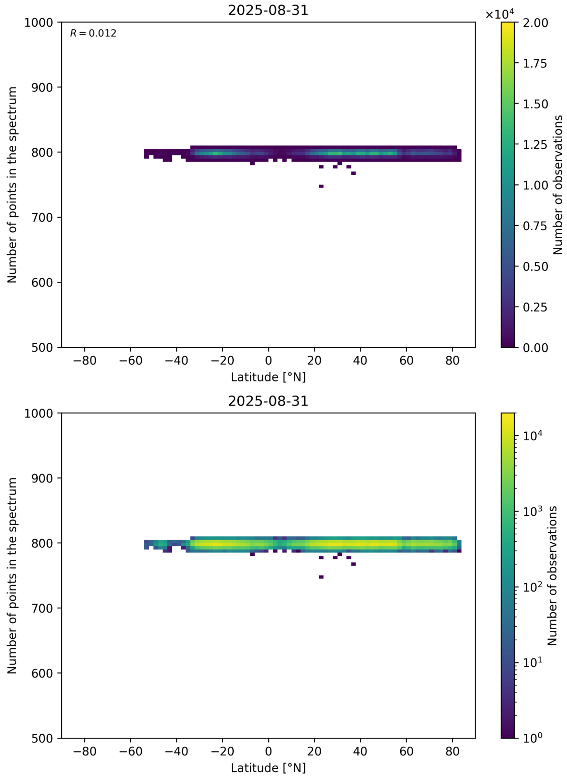
Figure 61: Scatter density plot of “Latitude” against “Number of points in the spectrum” for 2025-08-30 to 2025-09-01.
