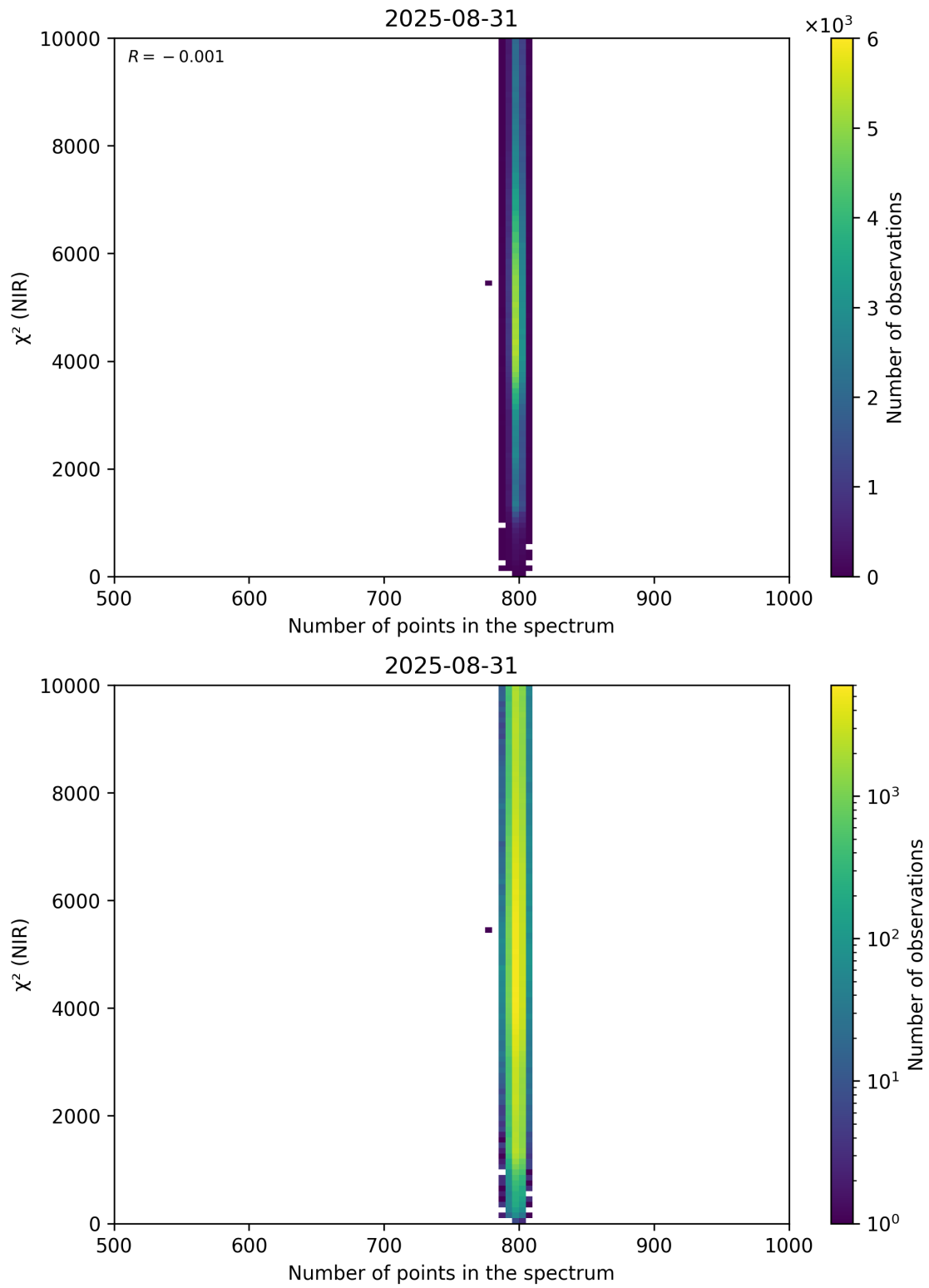
Figure 88: Scatter density plot of “Number of points in the spectrum” against “ \chi^2 (NIR)” for 2025-08-30 to 2025-09-01.
