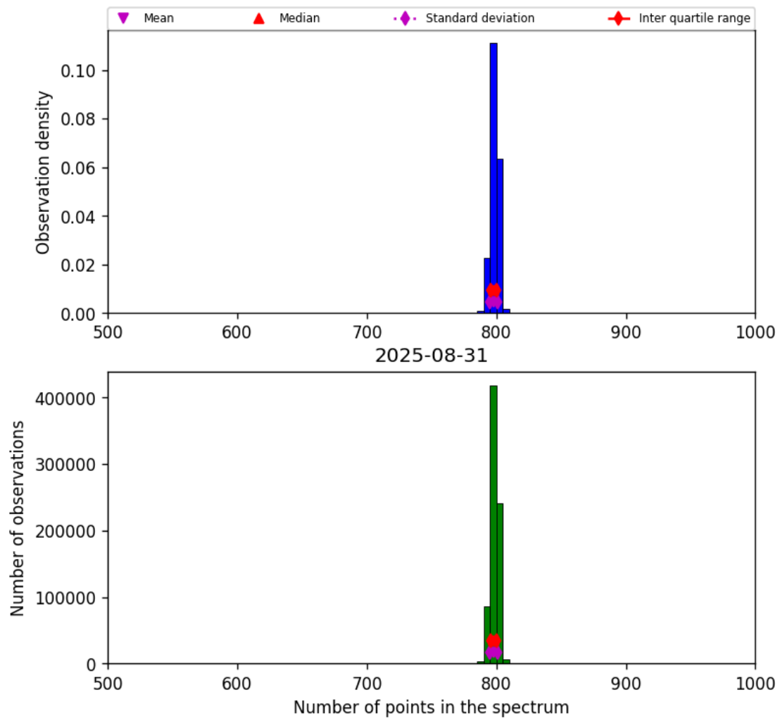
Figure 26: Histogram of “Number of points in the spectrum” for 2025-08-30 to 2025-09-01
