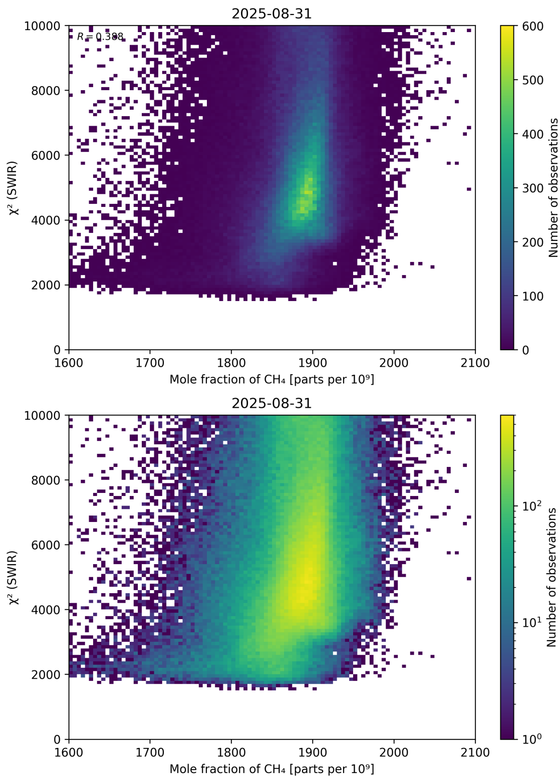
Figure 71: Scatter density plot of “Mole fraction of \text{CH}_4 ” against “ \chi^2 (SWIR)” for 2025-08-30 to 2025-09-01.
