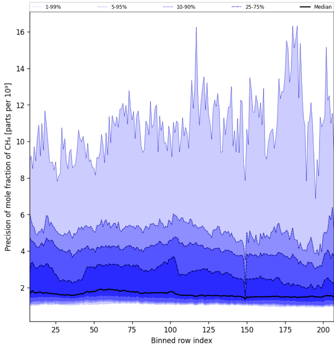
Figure 35: Along track statistics of “Precision of mole fraction of CH 4 ” for 2025-08-30 to 2025-09-01
