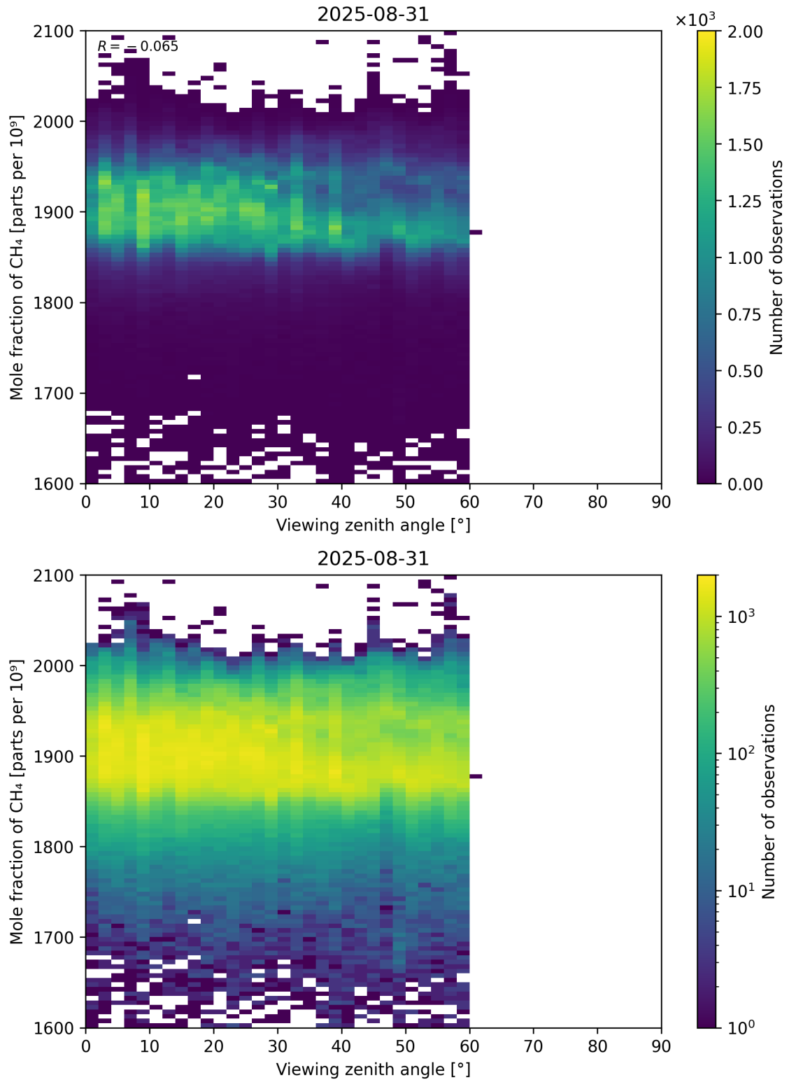
Figure 110: Scatter density plot of “Viewing zenith angle” against “Mole fraction of CH 4 ” for 2025-08-30 to 2025-09-01.
