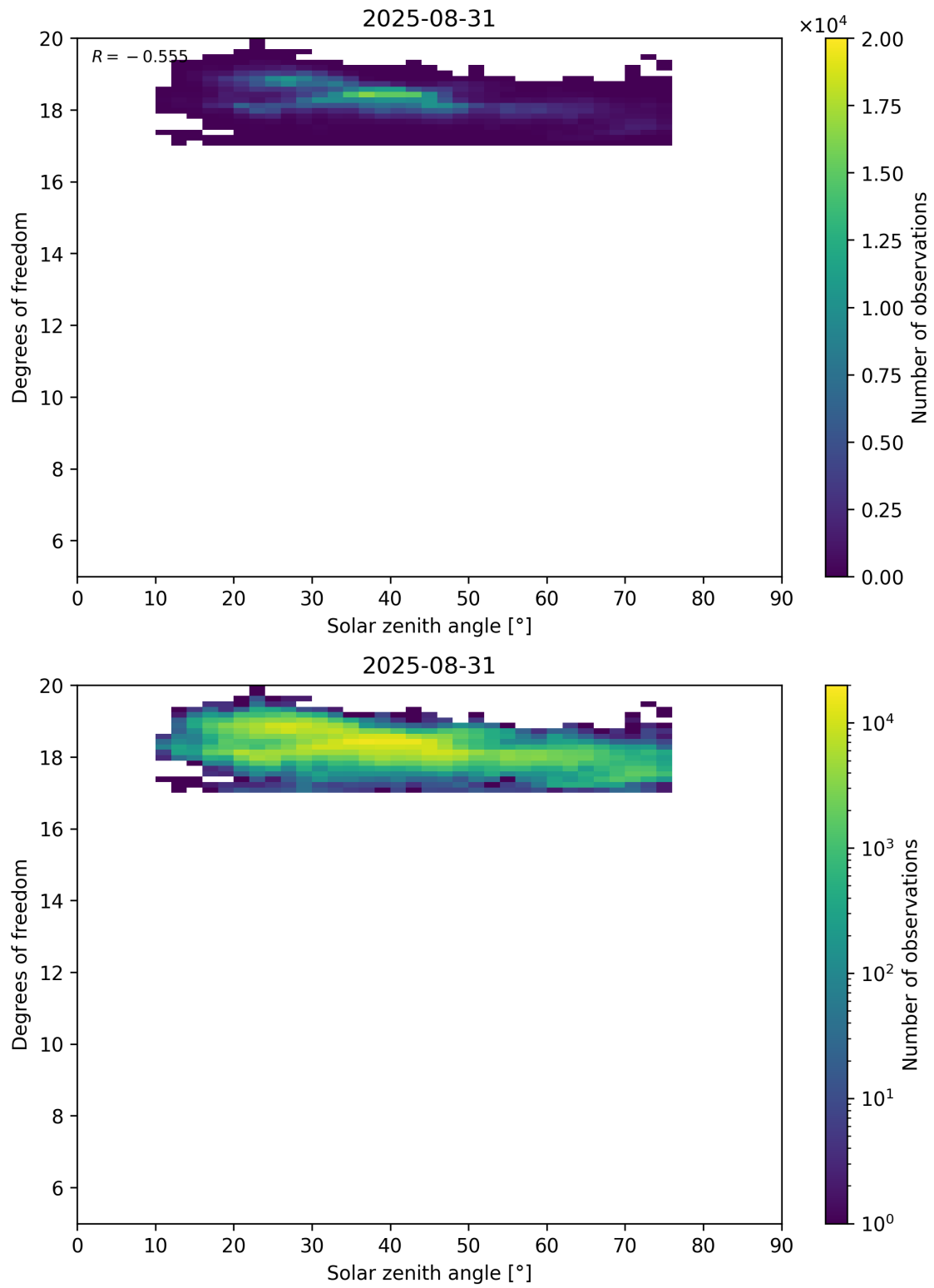
Figure 96: Scatter density plot of “Solar zenith angle” against “Degrees of freedom” for 2025-08-30 to 2025-09-01.
