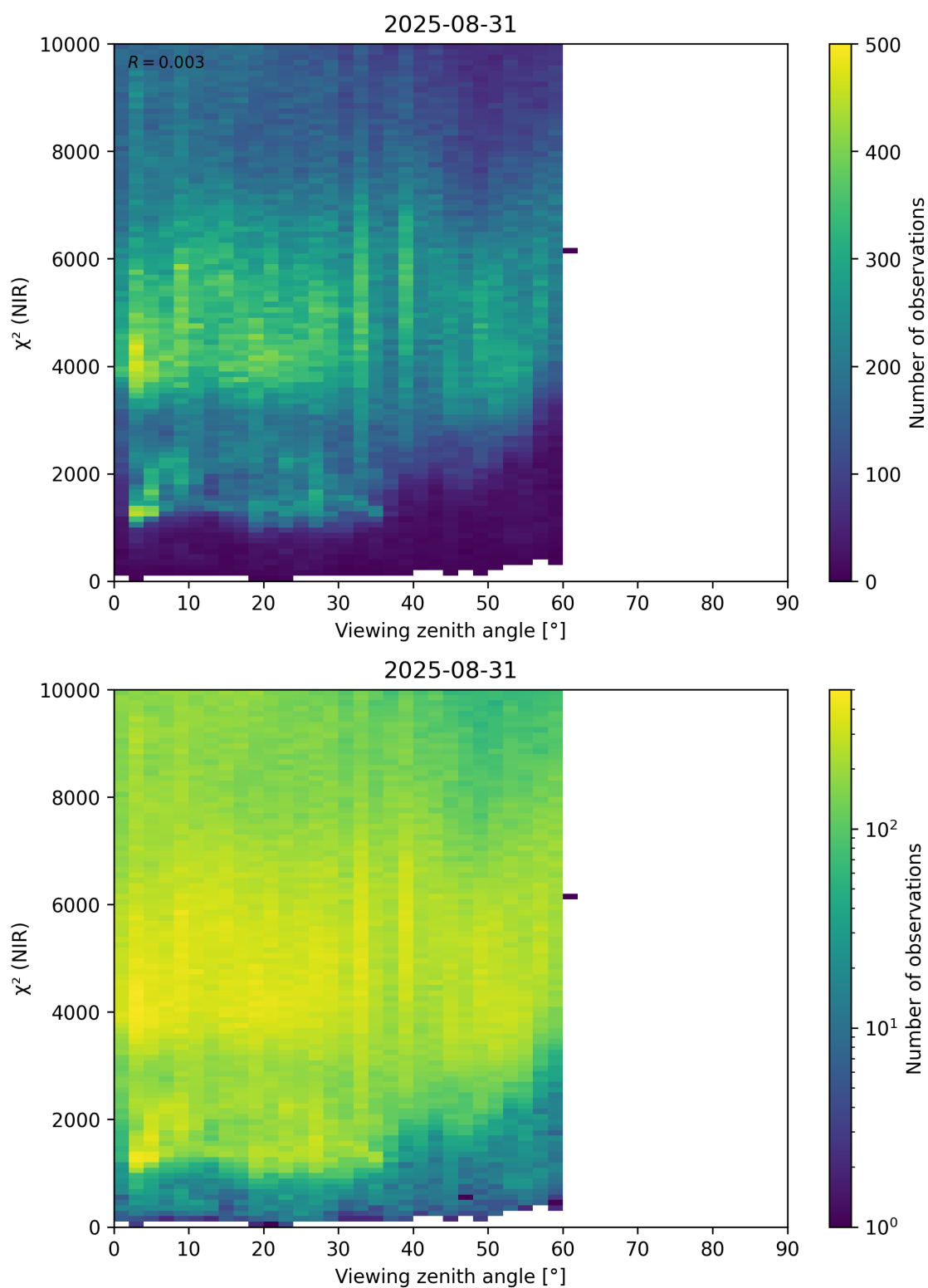
Figure 105: Scatter density plot of “Viewing zenith angle” against “ \chi^2 (NIR)” for 2025-08-30 to 2025-09-01.
