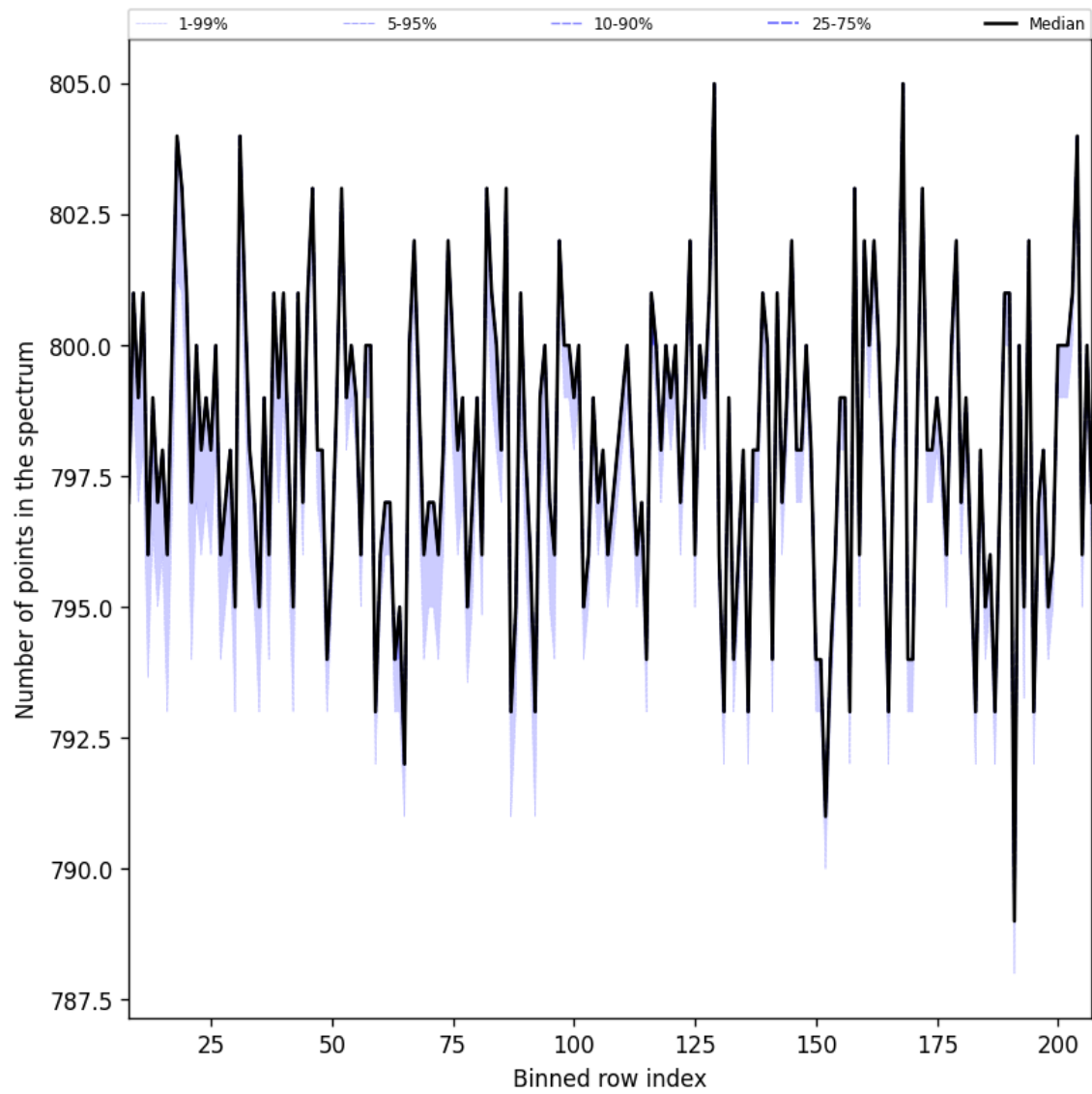
Figure 37: Along track statistics of “Number of points in the spectrum” for 2025-08-30 to 2025-09-01
