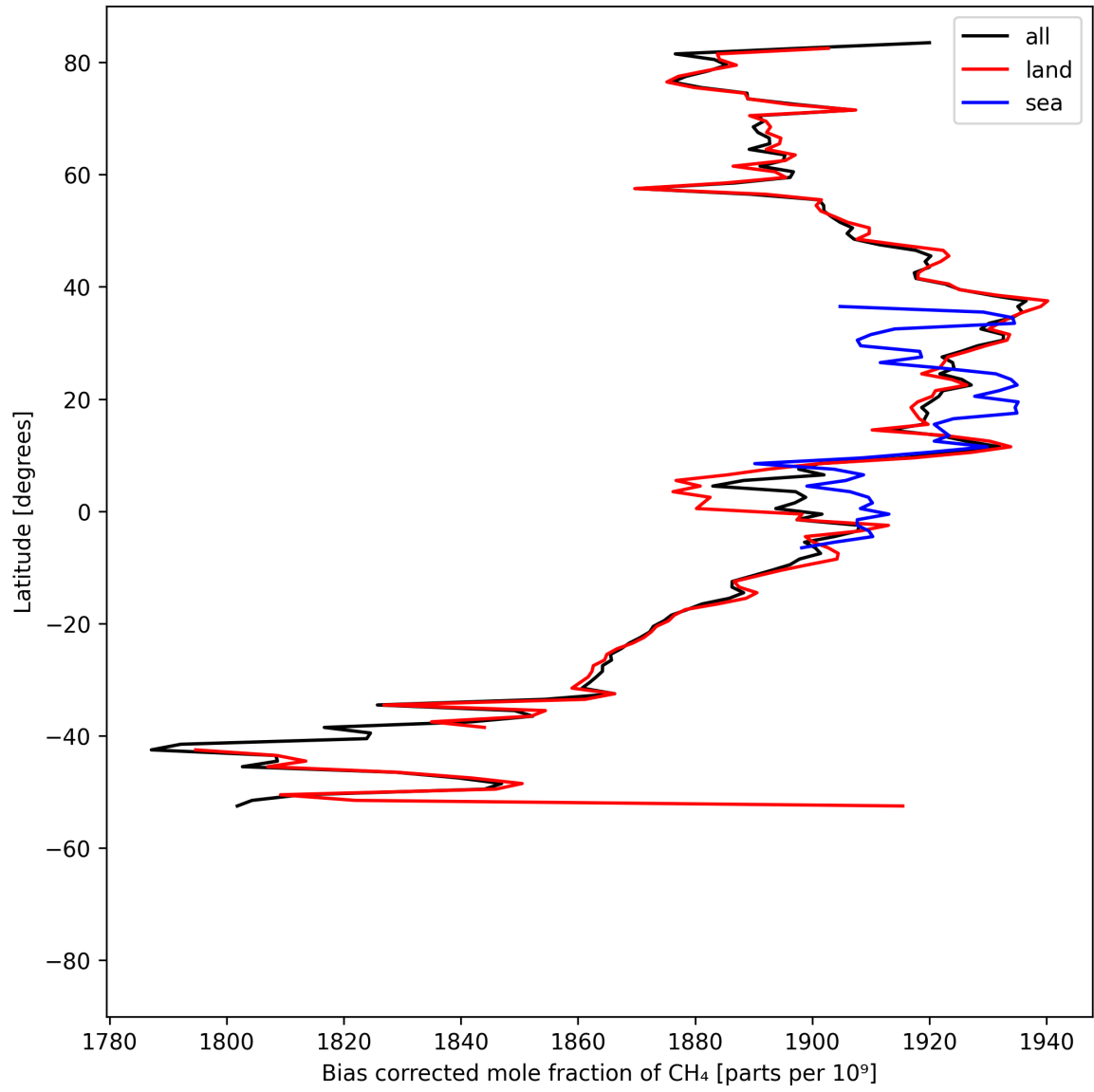
Figure 14: Zonal average of “Bias corrected mole fraction of \text{CH}_4 ” for 2025-08-30 to 2025-09-01.
