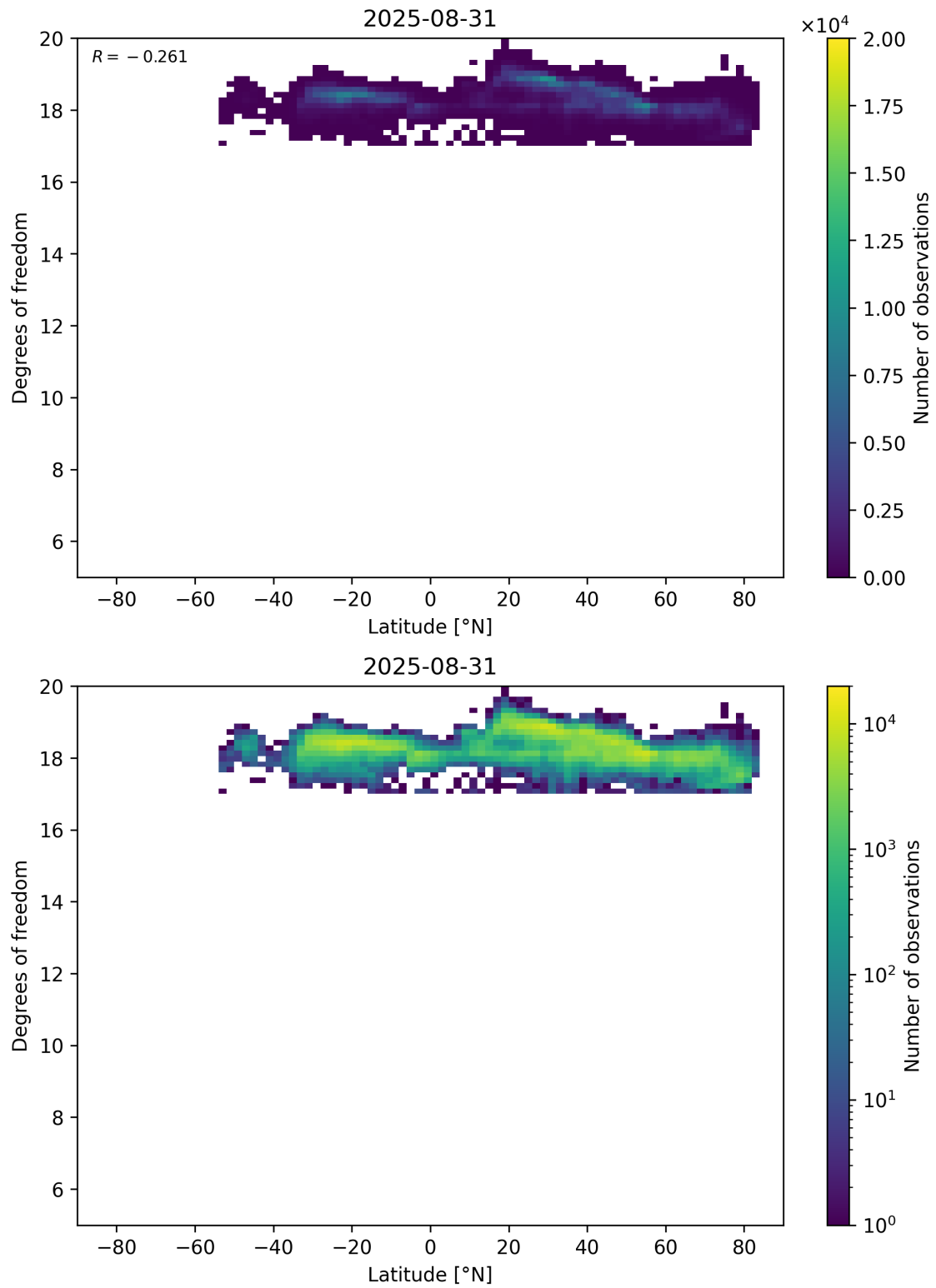
Figure 55: Scatter density plot of “Latitude” against “Degrees of freedom” for 2025-08-30 to 2025-09-01.
