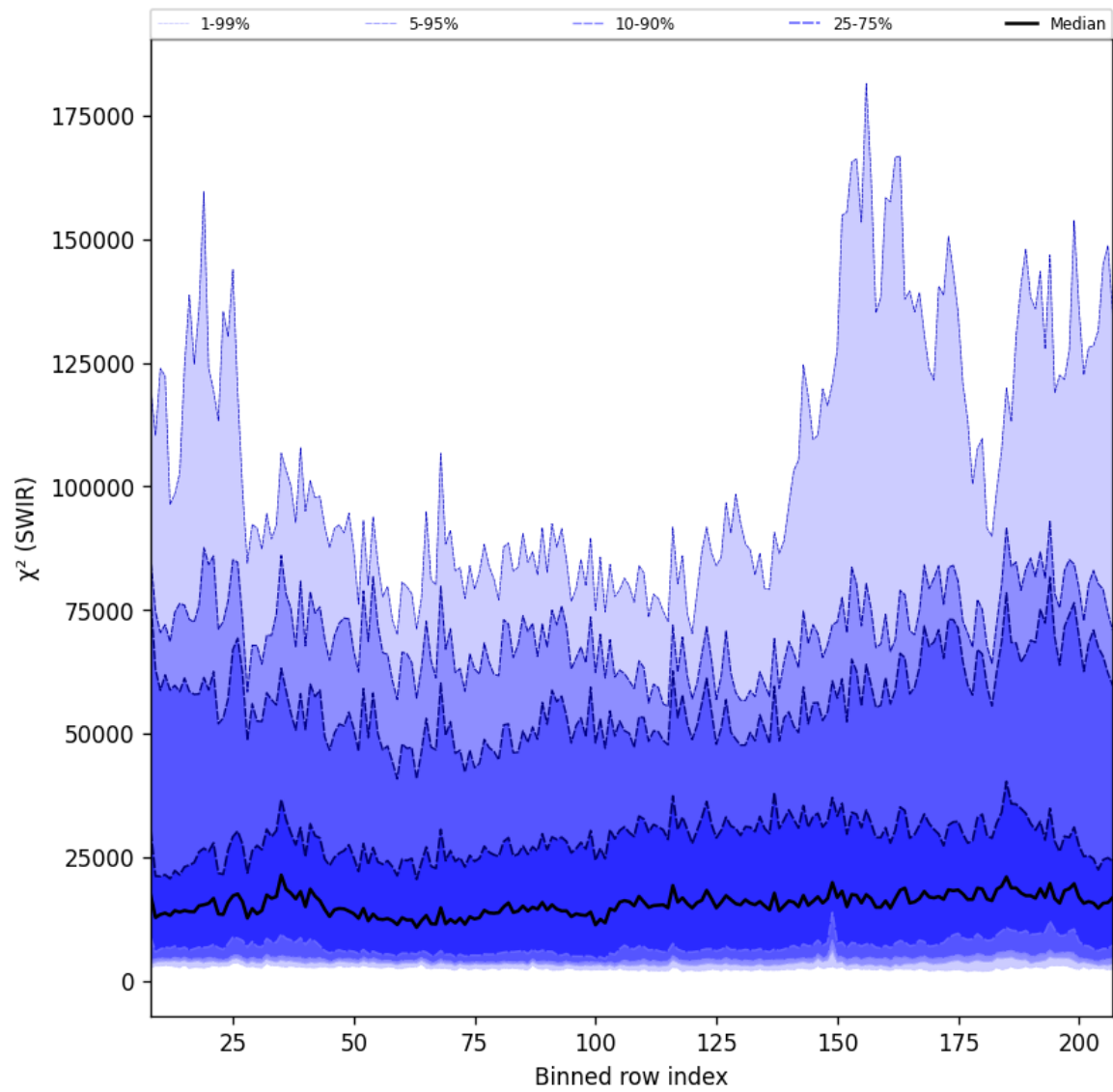
Figure 39: Along track statistics of “ \chi^2 (SWIR)” for 2025-08-30 to 2025-09-01
