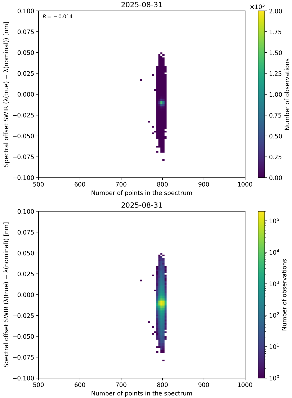
Figure 93: Scatter density plot of “Number of points in the spectrum” against “Spectral offset SWIR ( \lambda_{\text{true}} - \lambda_{\text{nominal}} )” for 2025-08-30 to 2025-09-01.
