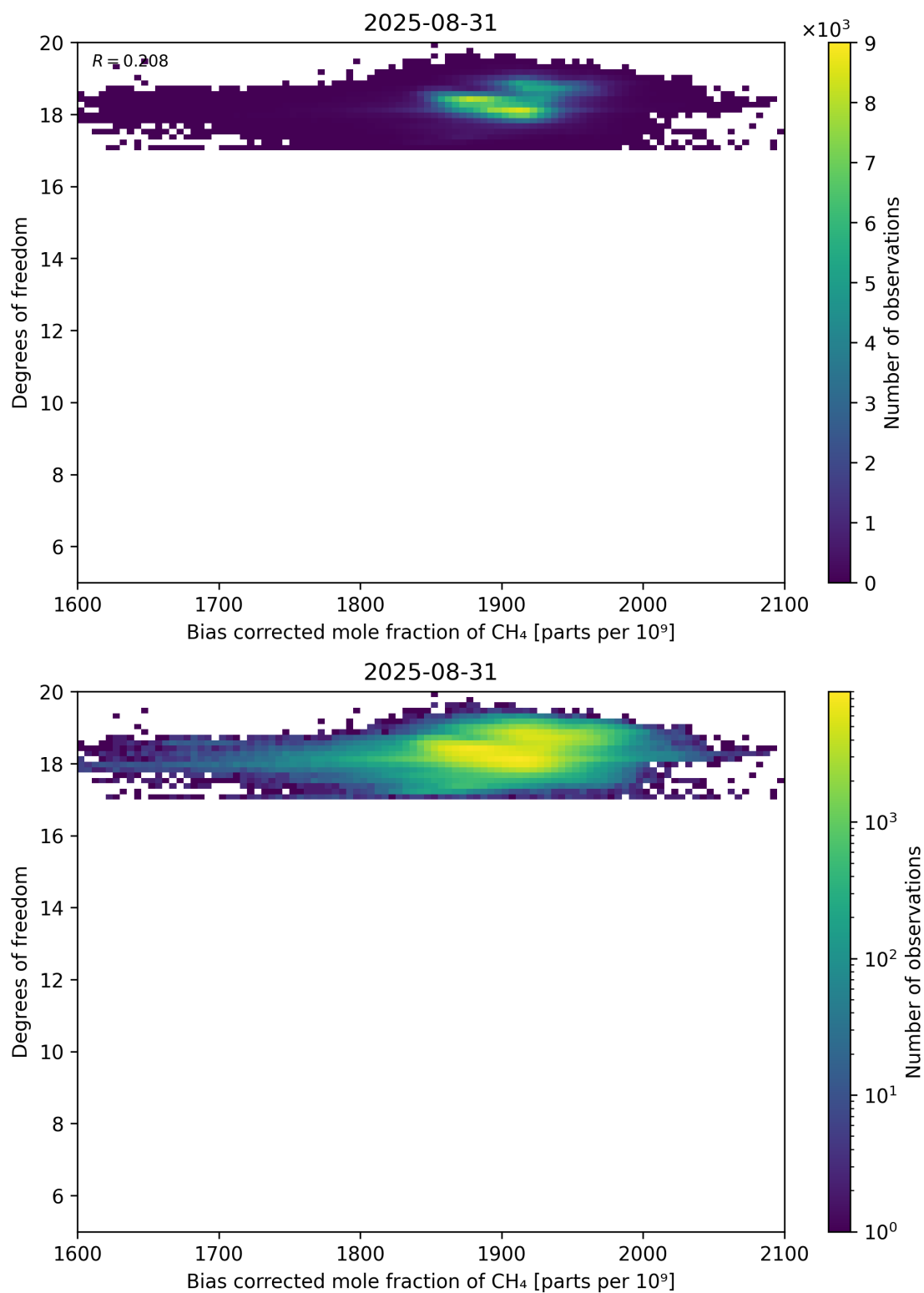
Figure 65: Scatter density plot of “Bias corrected mole fraction of CH 4 ” against “Degrees of freedom” for 2025-08-30 to 2025-09-01.
