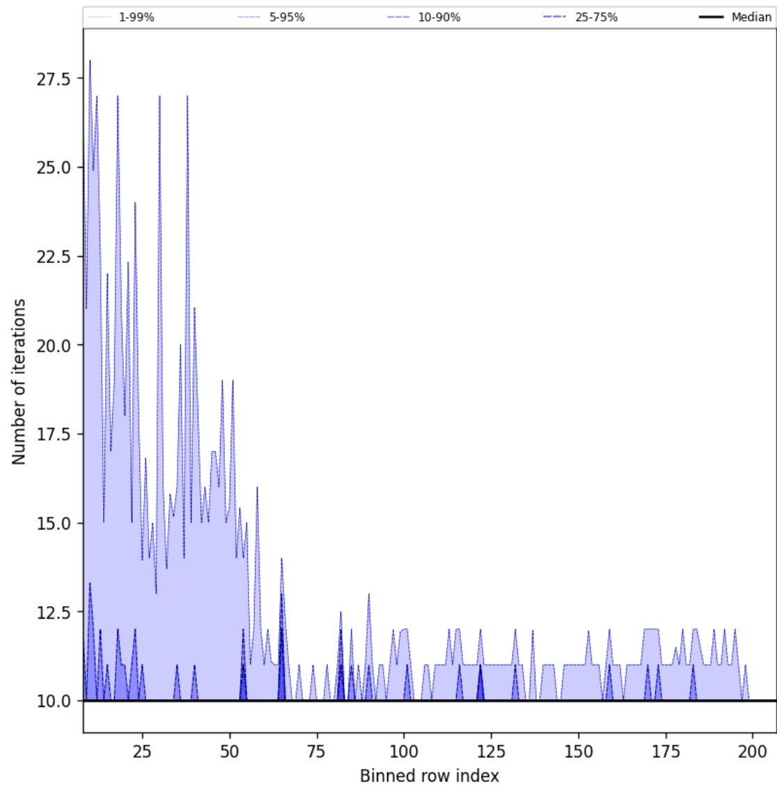
Figure 42: Along track statistics of “Number of iterations” for 2025-08-30 to 2025-09-01
