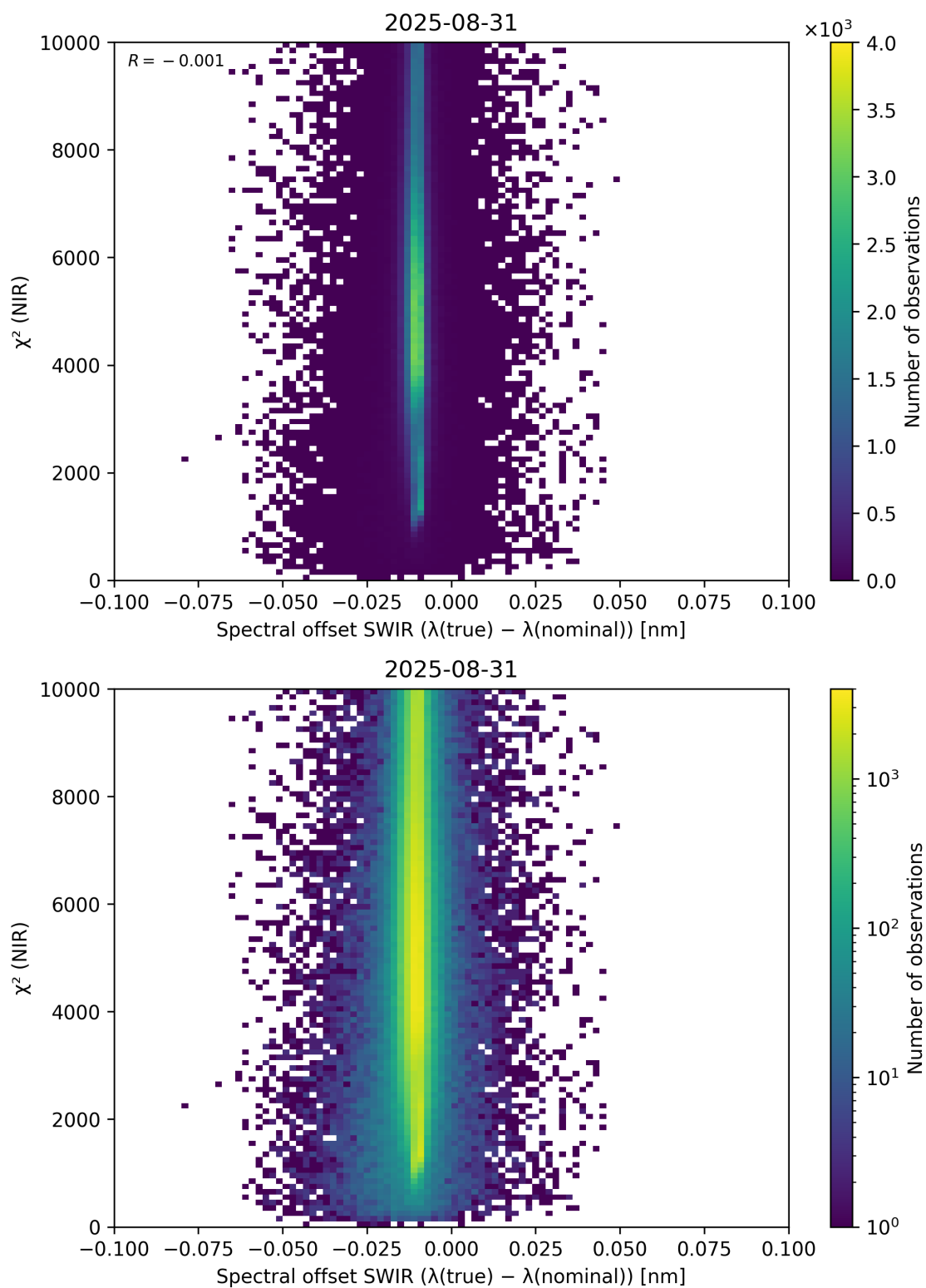
Figure 117: Scatter density plot of “Spectral offset SWIR ( \lambda_{\text{true}} - \lambda_{\text{nominal}} )” against “ \chi^2 (NIR)” for 2025-08-30 to 2025-09-01.
