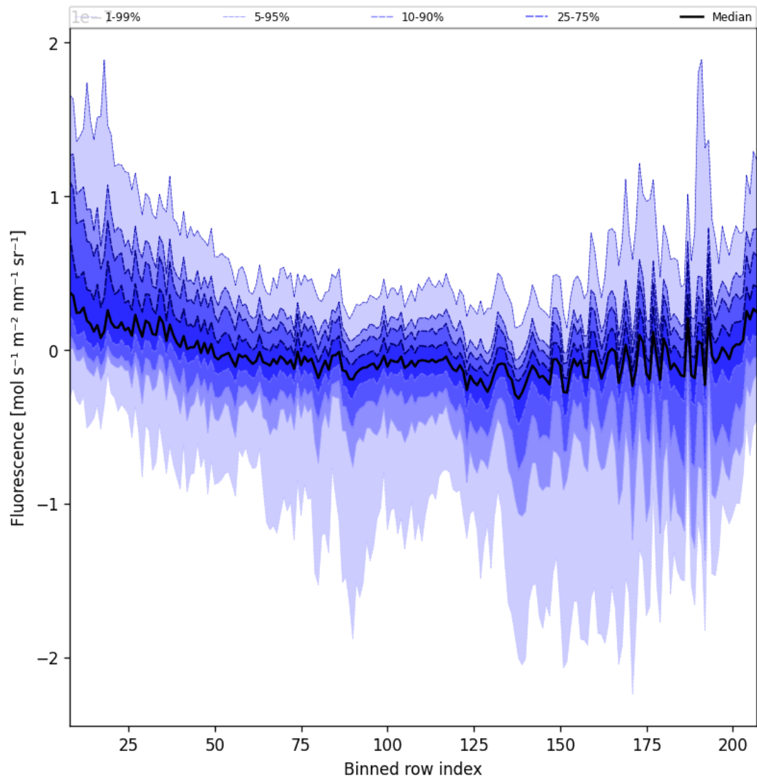
Figure 43: Along track statistics of “Fluorescence” for 2025-08-30 to 2025-09-01
