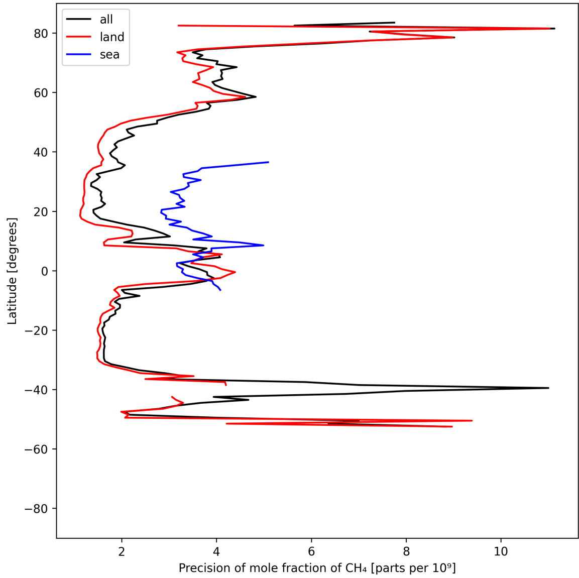
Figure 13: Zonal average of “Precision of mole fraction of CH 4 ” for 2025-08-30 to 2025-09-01.
