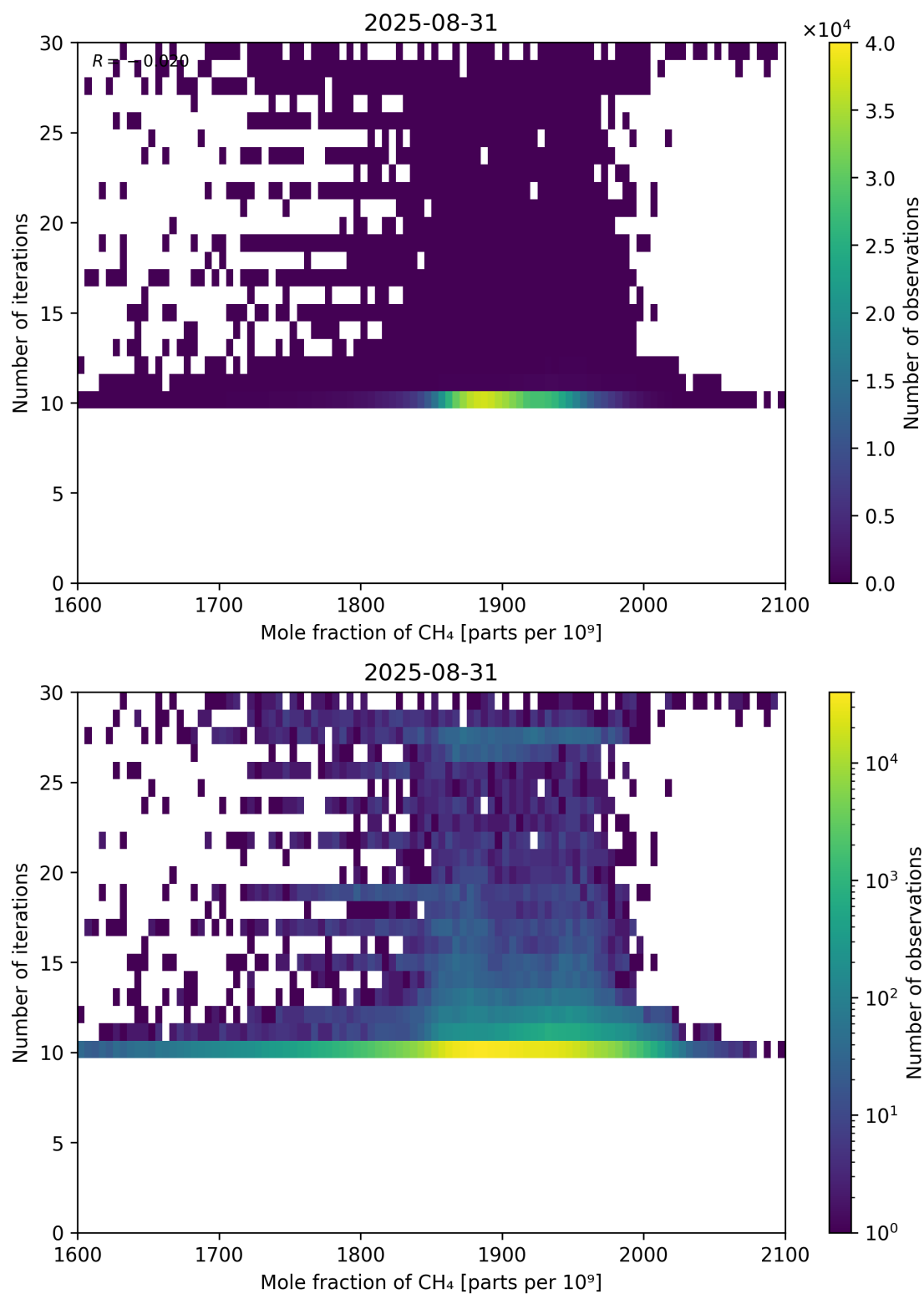
Figure 76: Scatter density plot of “Mole fraction of CH 4 ” against “Number of iterations” for 2025-08-30 to 2025-09-01.
