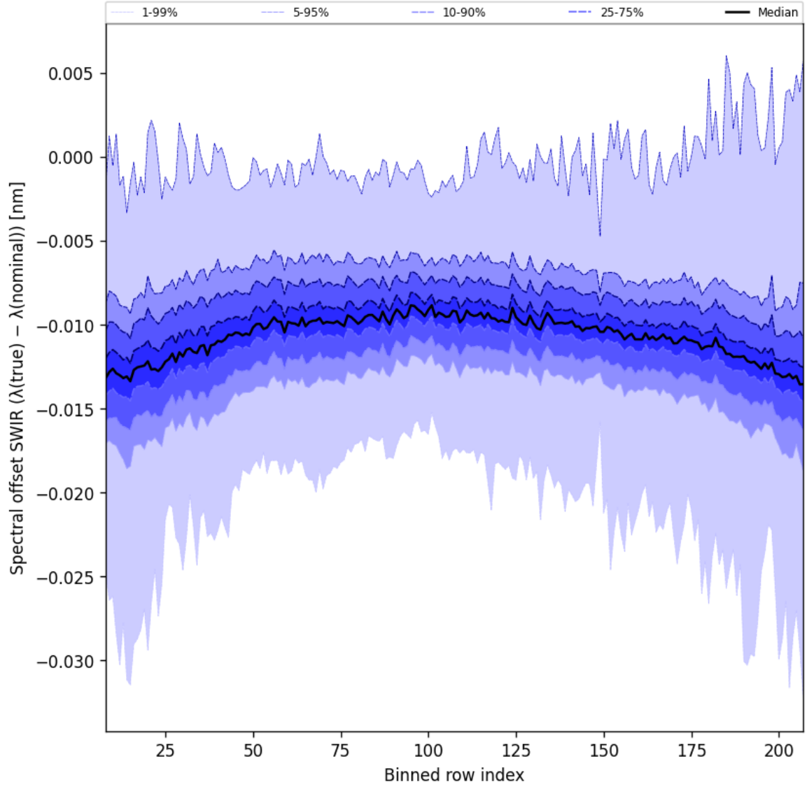
Figure 38: Along track statistics of “Spectral offset SWIR ( \lambda_{\text{true}} - \lambda_{\text{nominal}} )” for 2025-08-30 to 2025-09-01
