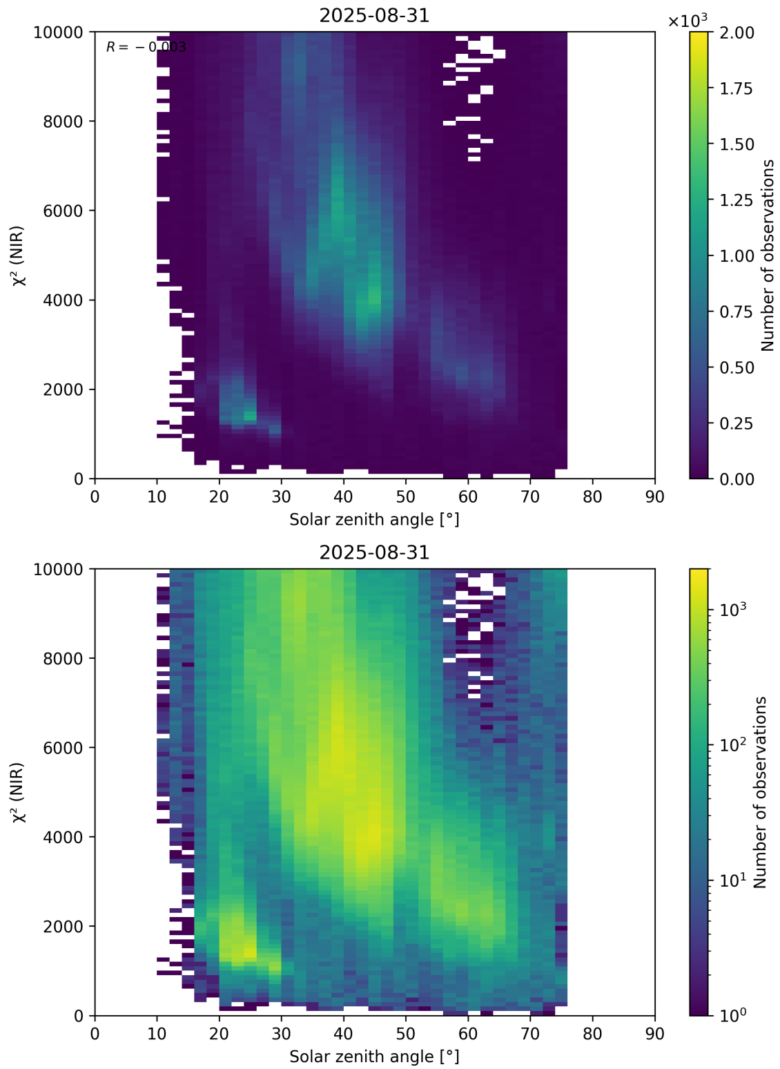
Figure 94: Scatter density plot of “Solar zenith angle” against “ \chi^2 (NIR)” for 2025-08-30 to 2025-09-01.
