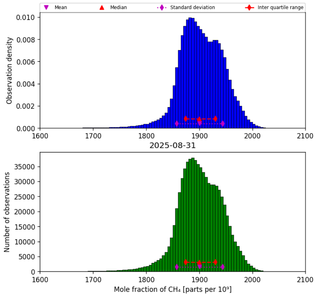
Figure 23: Histogram of “Mole fraction of CH 4 ” for 2025-08-30 to 2025-09-01
