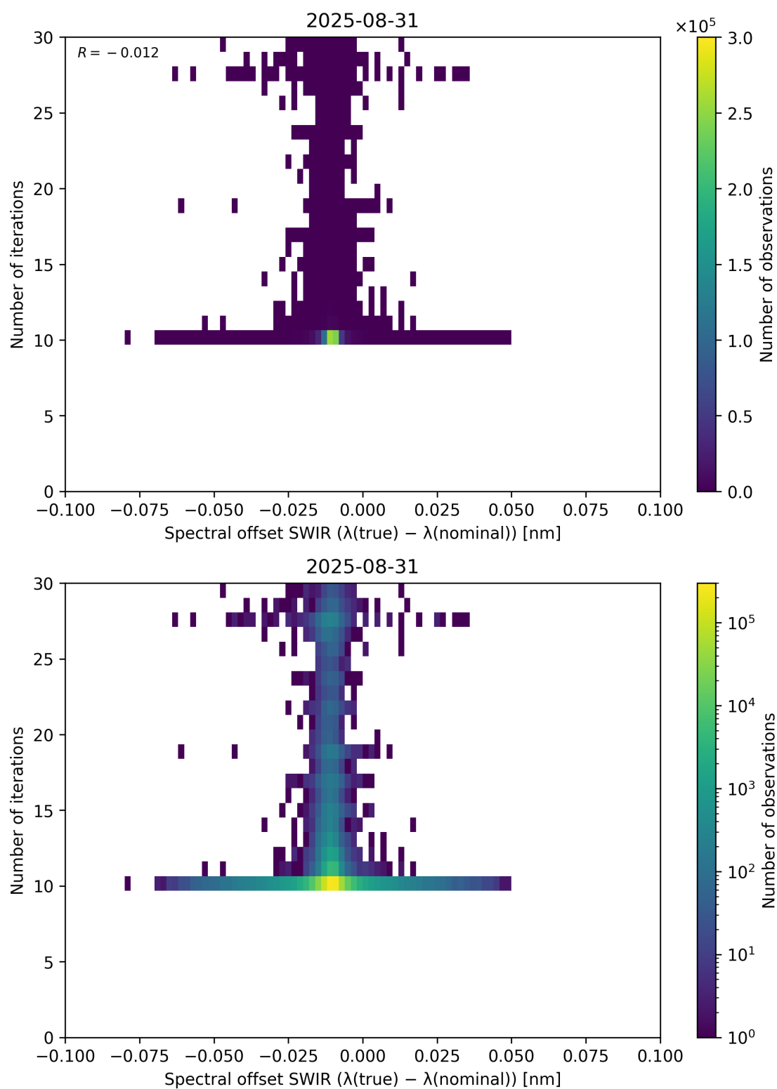
Figure 121: Scatter density plot of “Spectral offset SWIR ( \lambda_{\text{true}} - \lambda_{\text{nominal}} )” against “Number of iterations” for 2025-08-30 to 2025-09-01.
