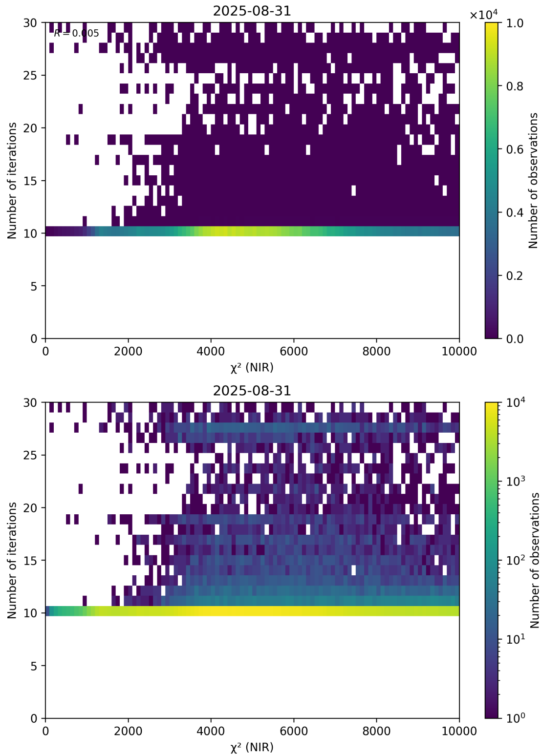
Figure 46: Scatter density plot of “ \chi^2 (NIR)” against “Number of iterations” for 2025-08-30 to 2025-09-01.
