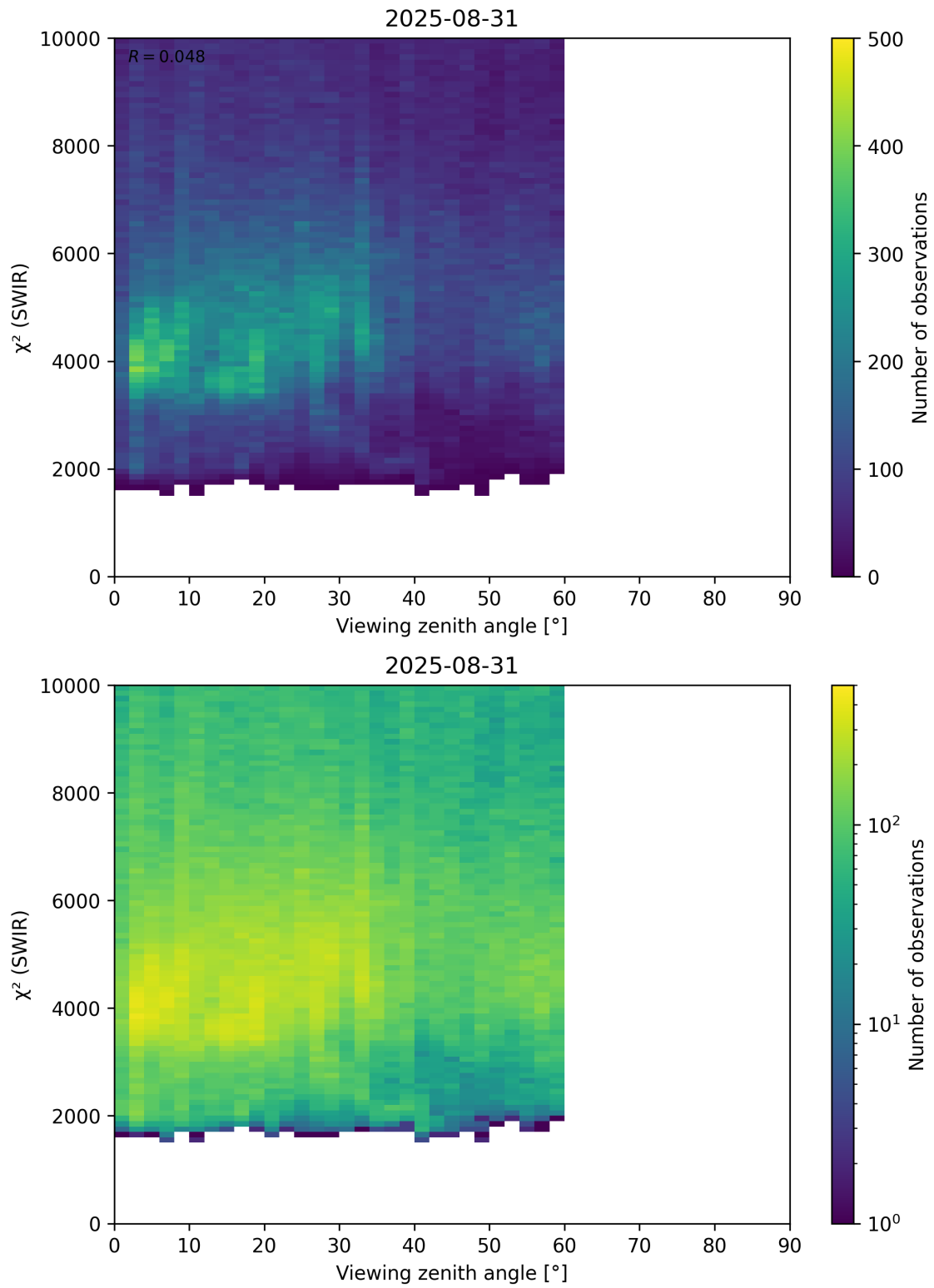
Figure 106: Scatter density plot of “Viewing zenith angle” against “ \chi^2 (SWIR)” for 2025-08-30 to 2025-09-01.
