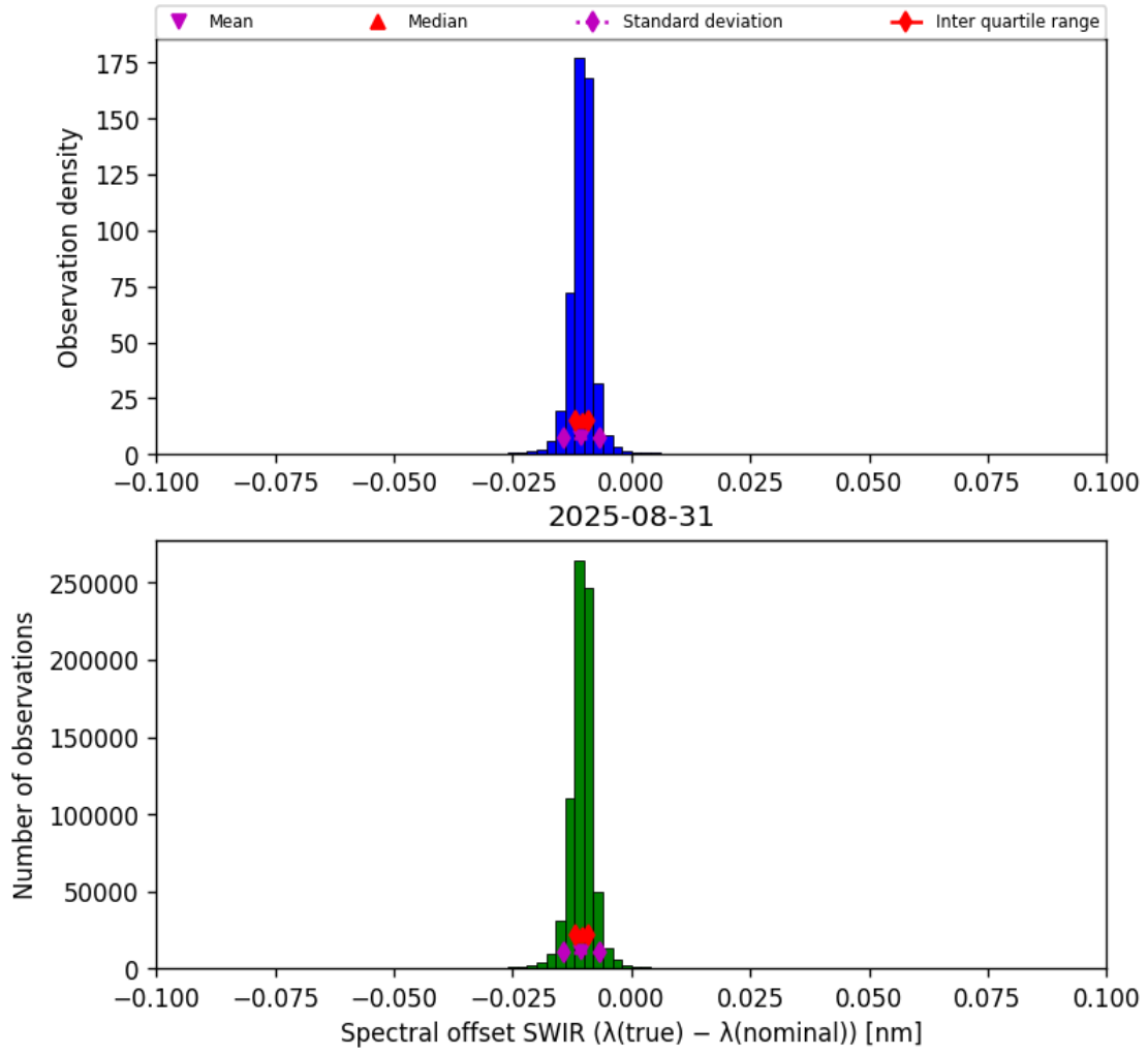
Figure 27: Histogram of “Spectral offset SWIR ( \lambda_{\text{true}} - \lambda_{\text{nominal}} )” for 2025-08-30 to 2025-09-01
