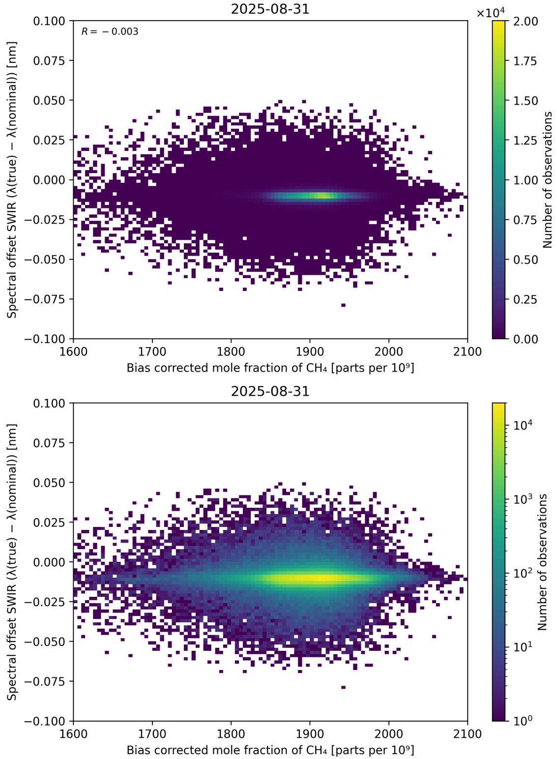
Figure 69: Scatter density plot of “Bias corrected mole fraction of \text{CH}_4 ” against “Spectral offset SWIR ( \lambda_{\text{true}} - \lambda_{\text{nominal}} )” for 2025-08-30 to 2025-09-01.
