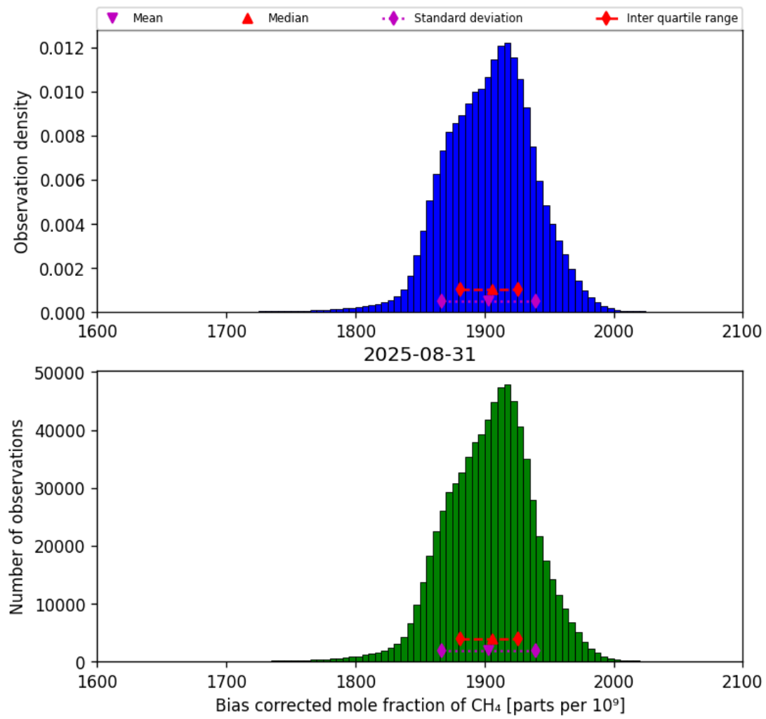
Figure 25: Histogram of “Bias corrected mole fraction of CH 4 ” for 2025-08-30 to 2025-09-01
