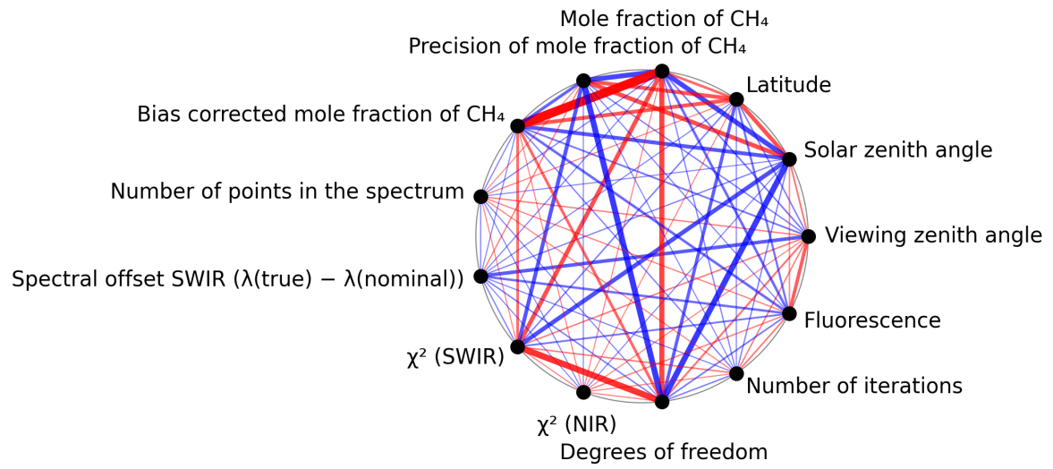
Figure 1: Map of correlation graph for 2025-08-30 to 2025-09-01.
