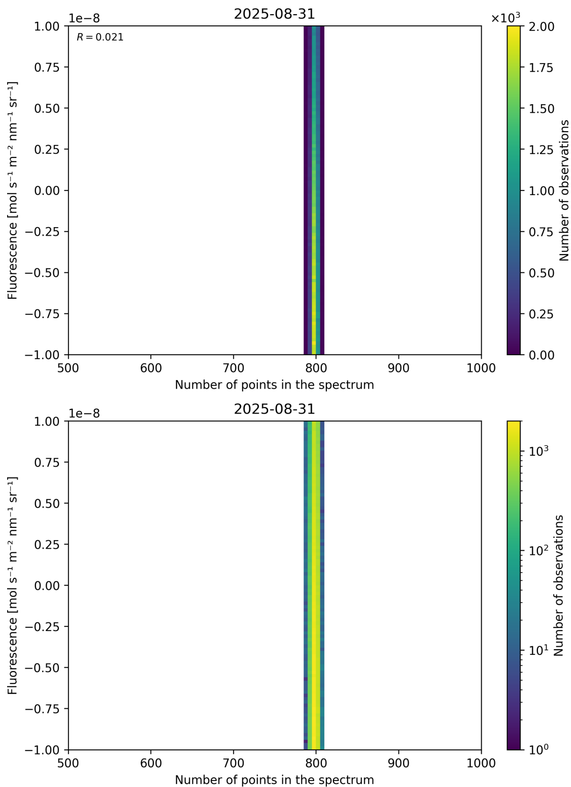
Figure 91: Scatter density plot of “Number of points in the spectrum” against “Fluorescence” for 2025-08-30 to 2025-09-01.
