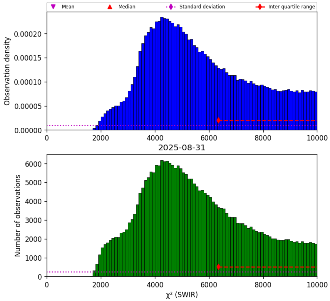
Figure 28: Histogram of “ \chi^2 (SWIR)” for 2025-08-30 to 2025-09-01
