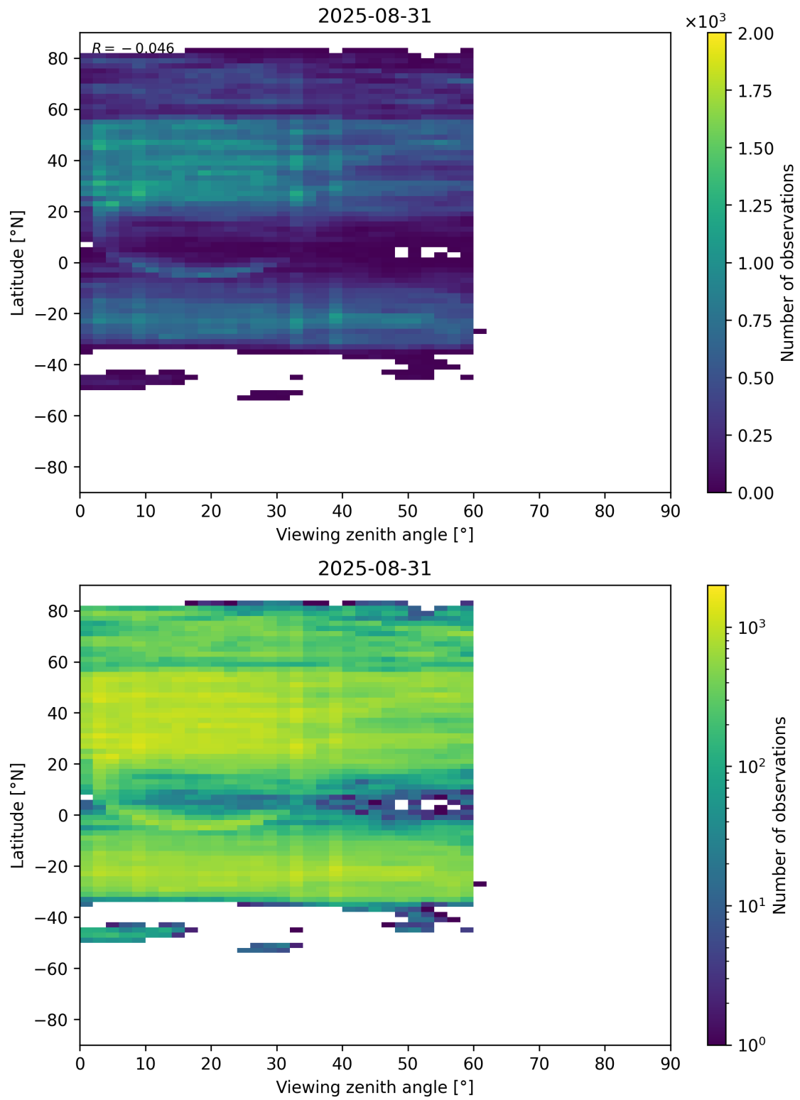
Figure 109: Scatter density plot of “Viewing zenith angle” against “Latitude” for 2025-08-30 to 2025-09-01.
