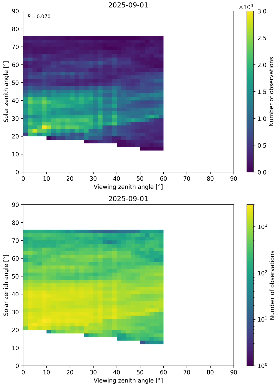
Figure 115: Scatter density plot of “Viewing zenith angle” against “Solar zenith angle” for 2025-08-31 to 2025-09-02.
