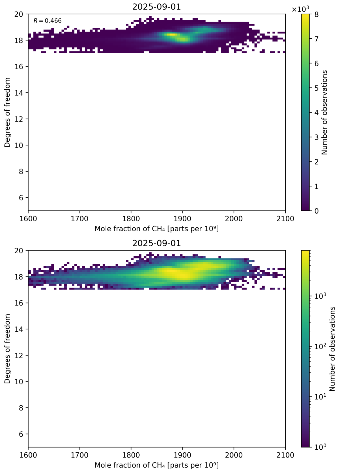
Figure 72: Scatter density plot of “Mole fraction of CH 4 ” against “Degrees of freedom” for 2025-08-31 to 2025-09-02.
