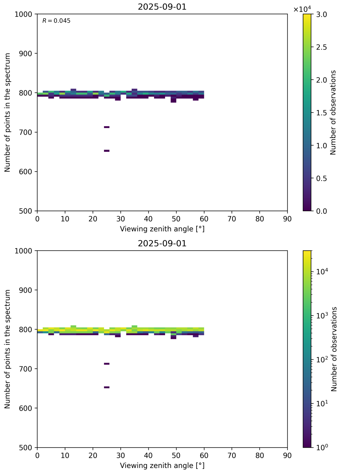
Figure 114: Scatter density plot of “Viewing zenith angle” against “Number of points in the spectrum” for 2025-08-31 to 2025-09-02.
