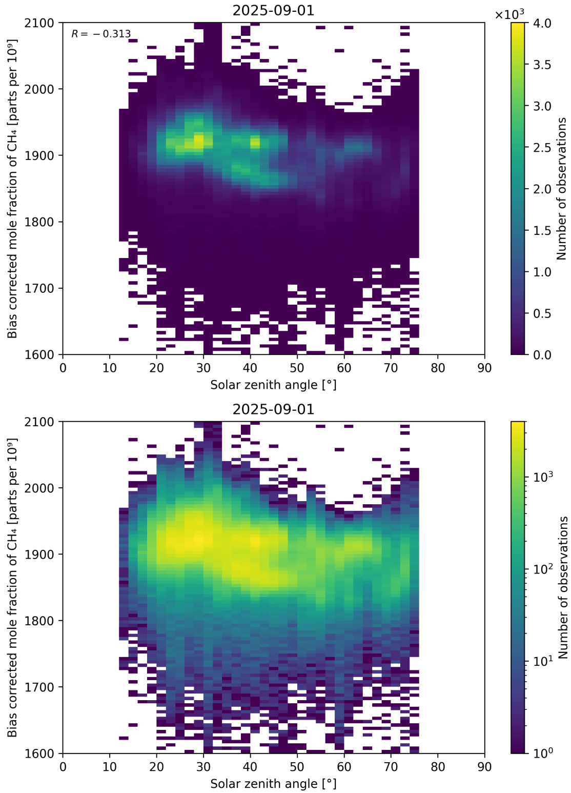
Figure 100: Scatter density plot of “Solar zenith angle” against “Bias corrected mole fraction of CH 4 ” for 2025-08-31 to 2025-09-02.
