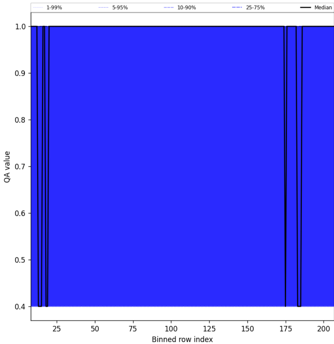
Figure 33: Along track statistics of “QA value” for 2025-08-31 to 2025-09-02
