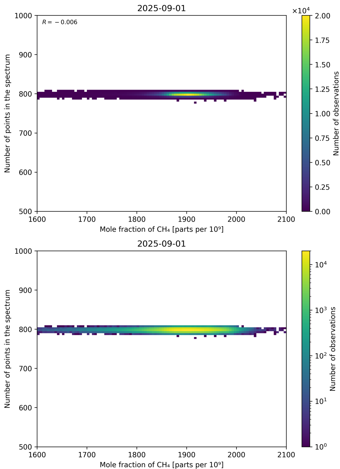
Figure 77: Scatter density plot of “Mole fraction of CH 4 ” against “Number of points in the spectrum” for 2025-08-31 to 2025-09-02.
