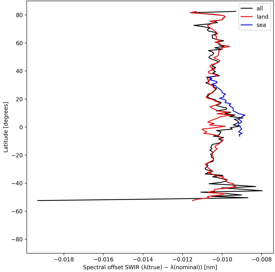
Figure 16: Zonal average of “Spectral offset SWIR ( \lambda_{\text{true}} - \lambda_{\text{nominal}} )” for 2025-08-31 to 2025-09-02.
