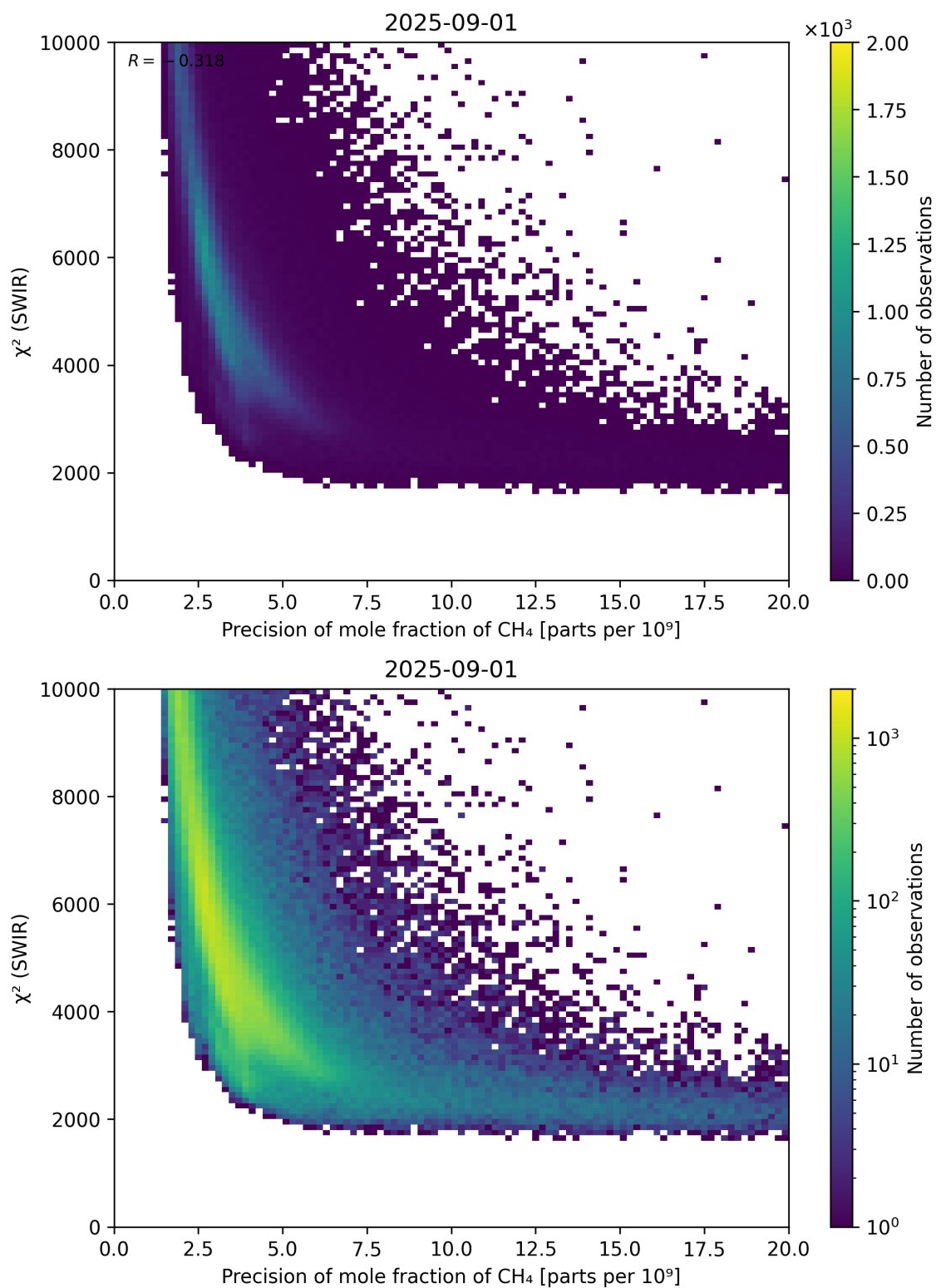
Figure 79: Scatter density plot of “Precision of mole fraction of CH 4 ” against “ \chi^2 (SWIR)” for 2025-08-31 to 2025-09-02.
