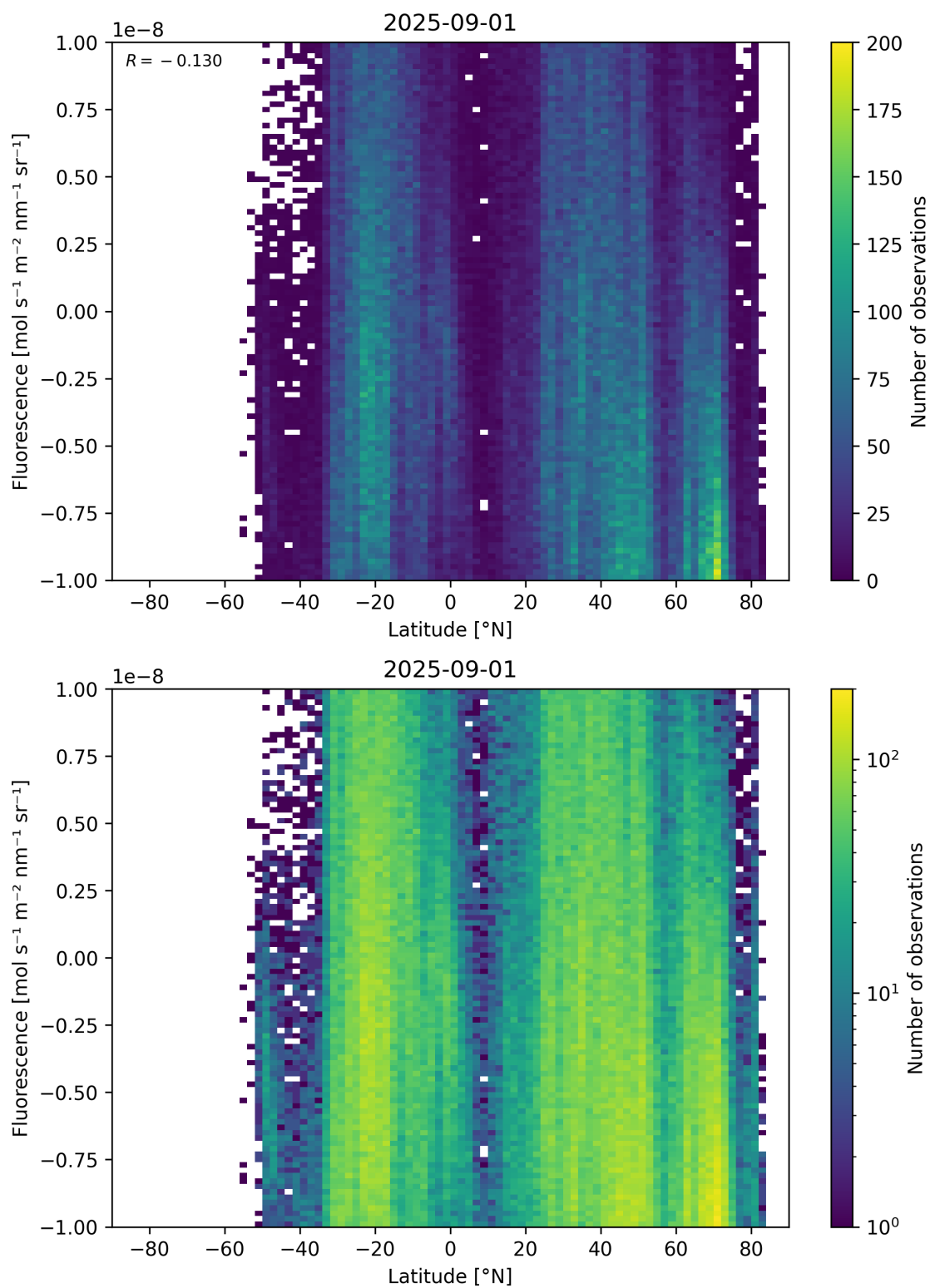
Figure 56: Scatter density plot of “Latitude” against “Fluorescence” for 2025-08-31 to 2025-09-02.
