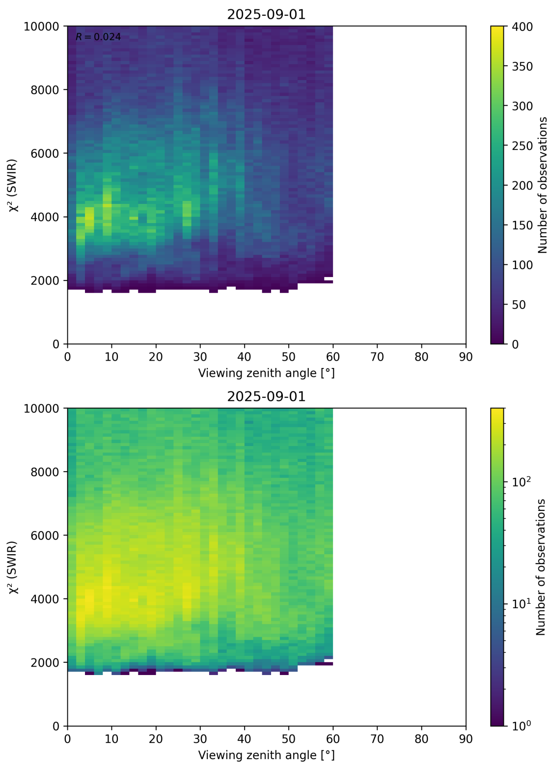
Figure 106: Scatter density plot of “Viewing zenith angle” against “ \chi^2 (SWIR)” for 2025-08-31 to 2025-09-02.
