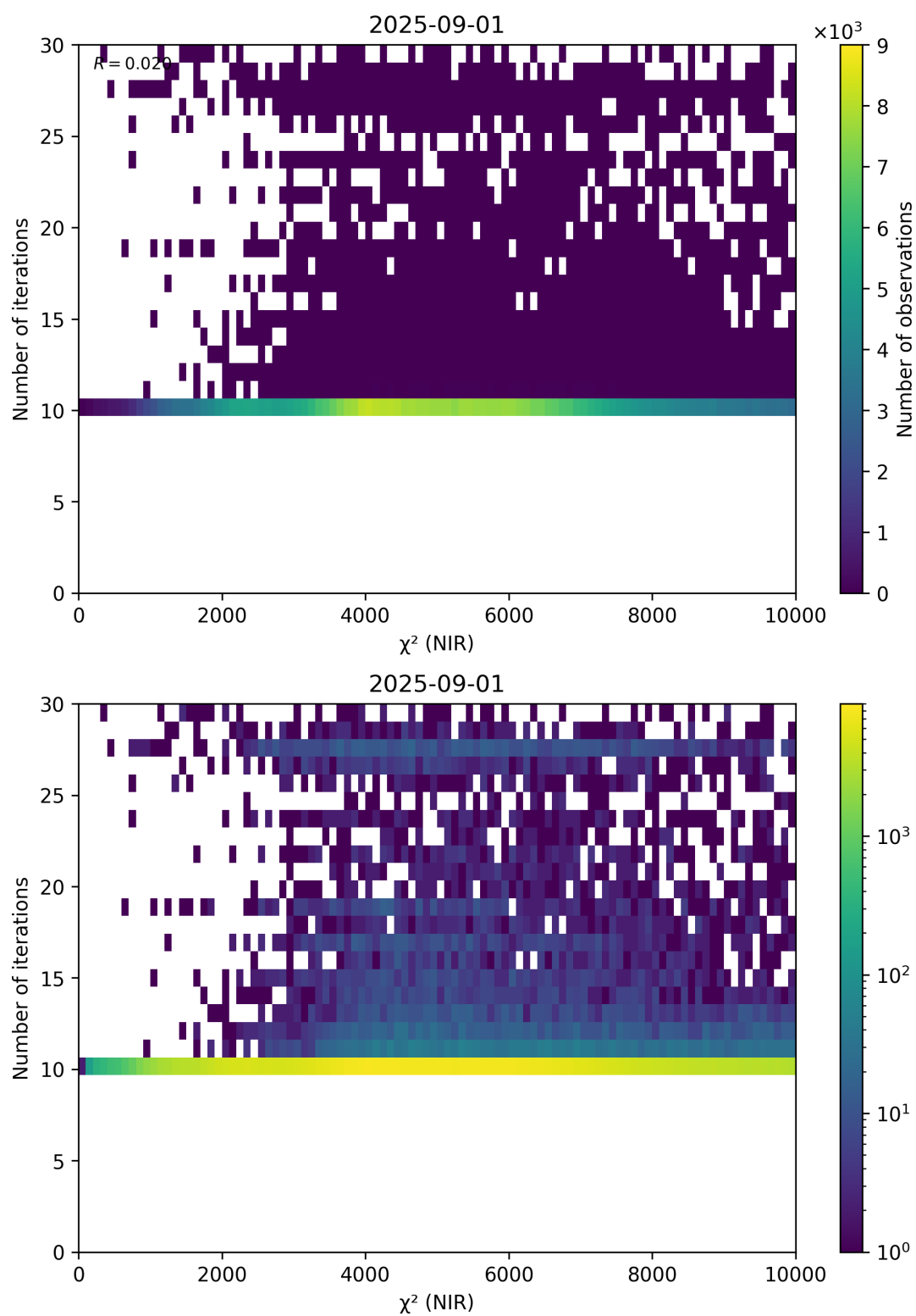
Figure 46: Scatter density plot of “ \chi^2 (NIR)” against “Number of iterations” for 2025-08-31 to 2025-09-02.
