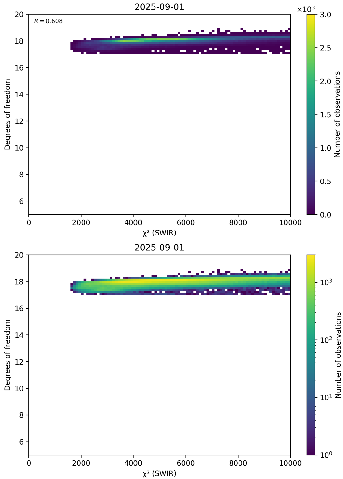
Figure 48: Scatter density plot of “ \chi^2 (SWIR)” against “Degrees of freedom” for 2025-08-31 to 2025-09-02.
