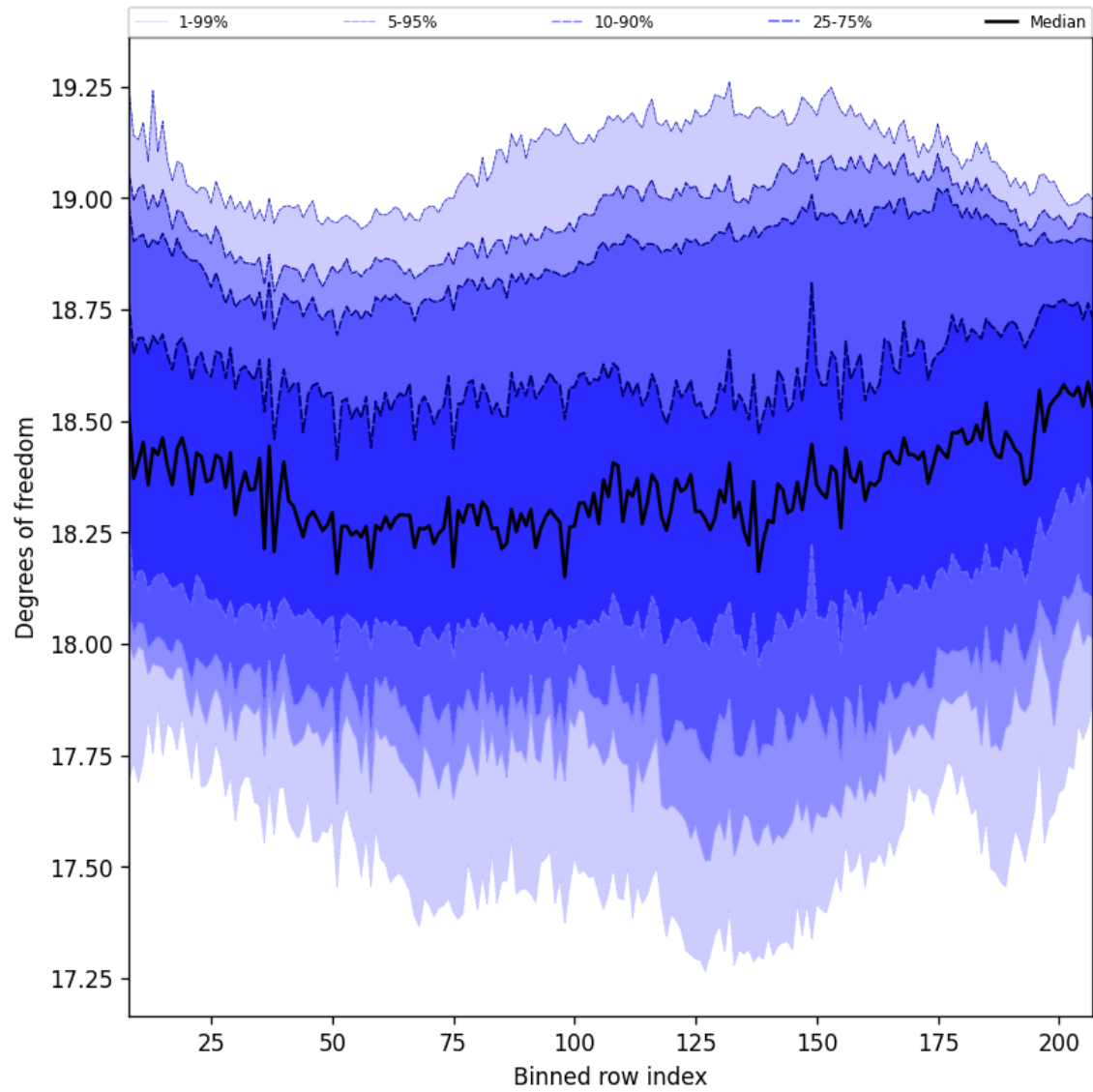
Figure 41: Along track statistics of “Degrees of freedom” for 2025-08-31 to 2025-09-02
