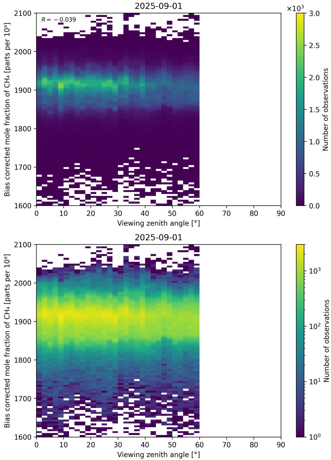
Figure 111: Scatter density plot of “Viewing zenith angle” against “Bias corrected mole fraction of CH 4 ” for 2025-08-31 to 2025-09-02.
