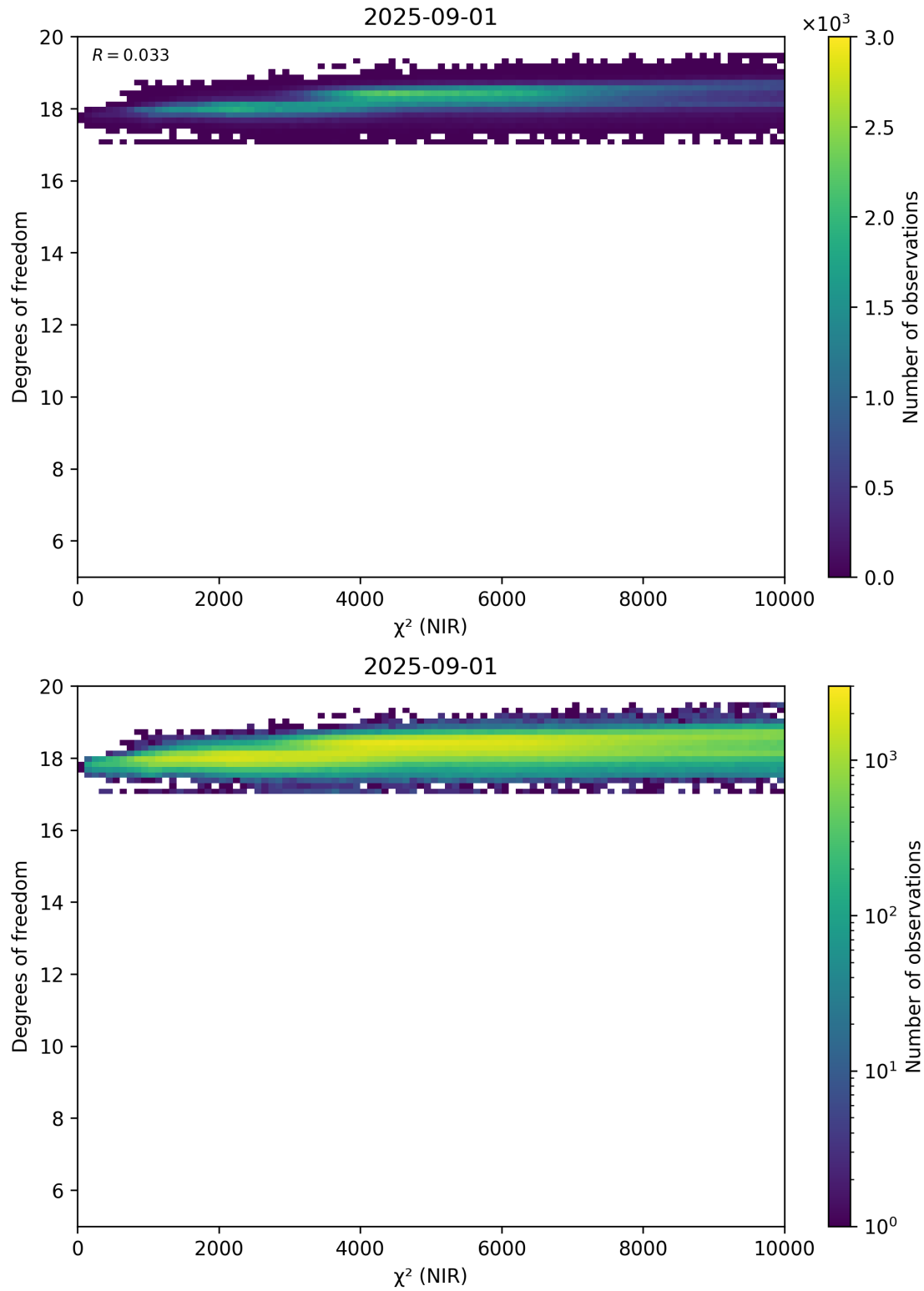
Figure 44: Scatter density plot of “ \chi^2 (NIR)” against “Degrees of freedom” for 2025-08-31 to 2025-09-02.
