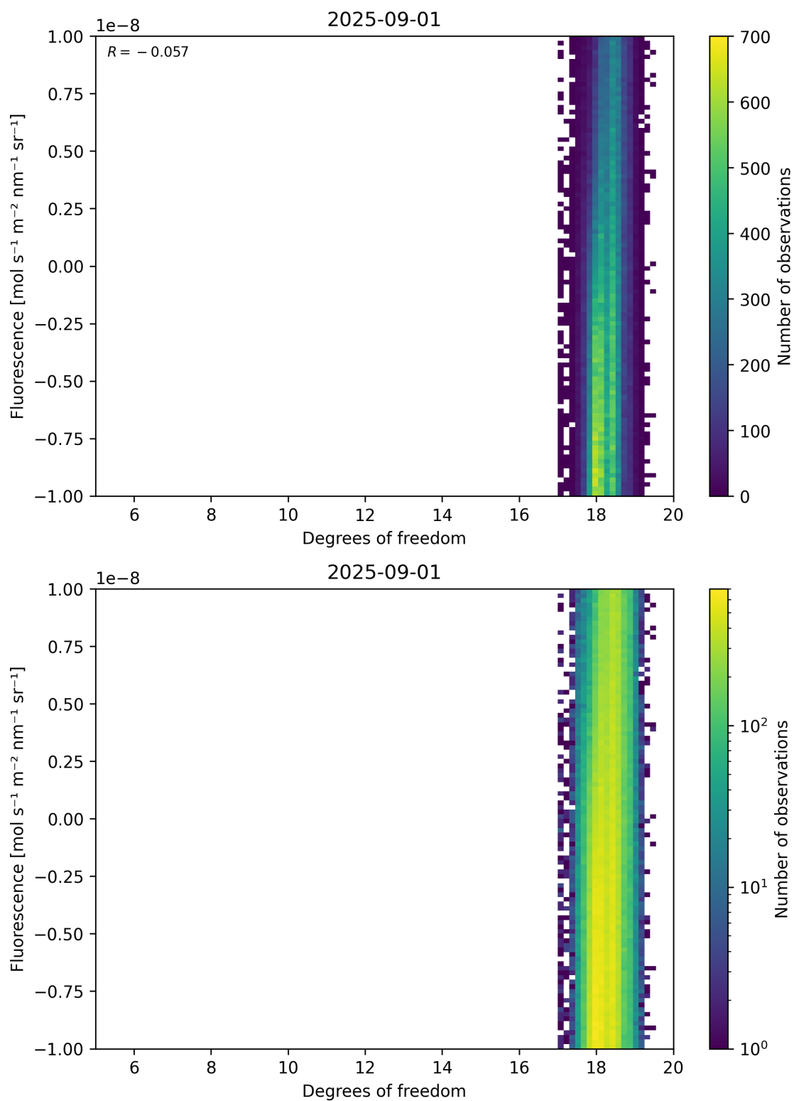
Figure 51: Scatter density plot of “Degrees of freedom” against “Fluorescence” for 2025-08-31 to 2025-09-02.
