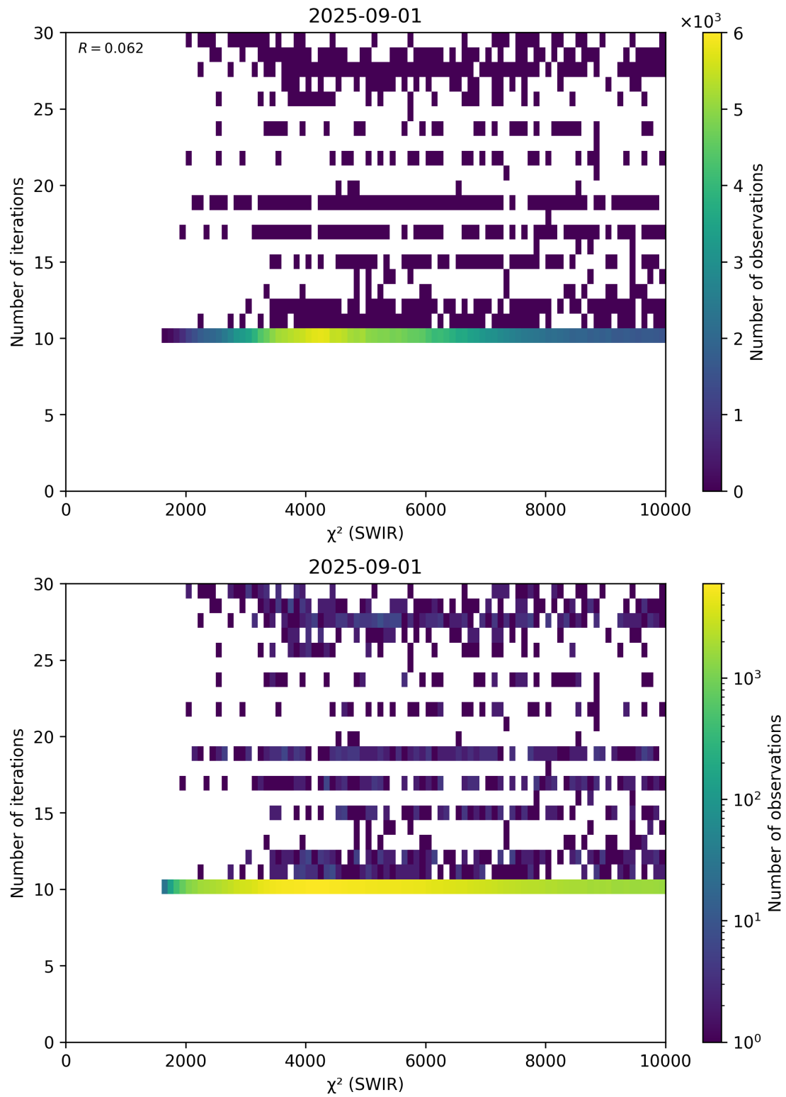
Figure 50: Scatter density plot of “ \chi^2 (SWIR)” against “Number of iterations” for 2025-08-31 to 2025-09-02.
