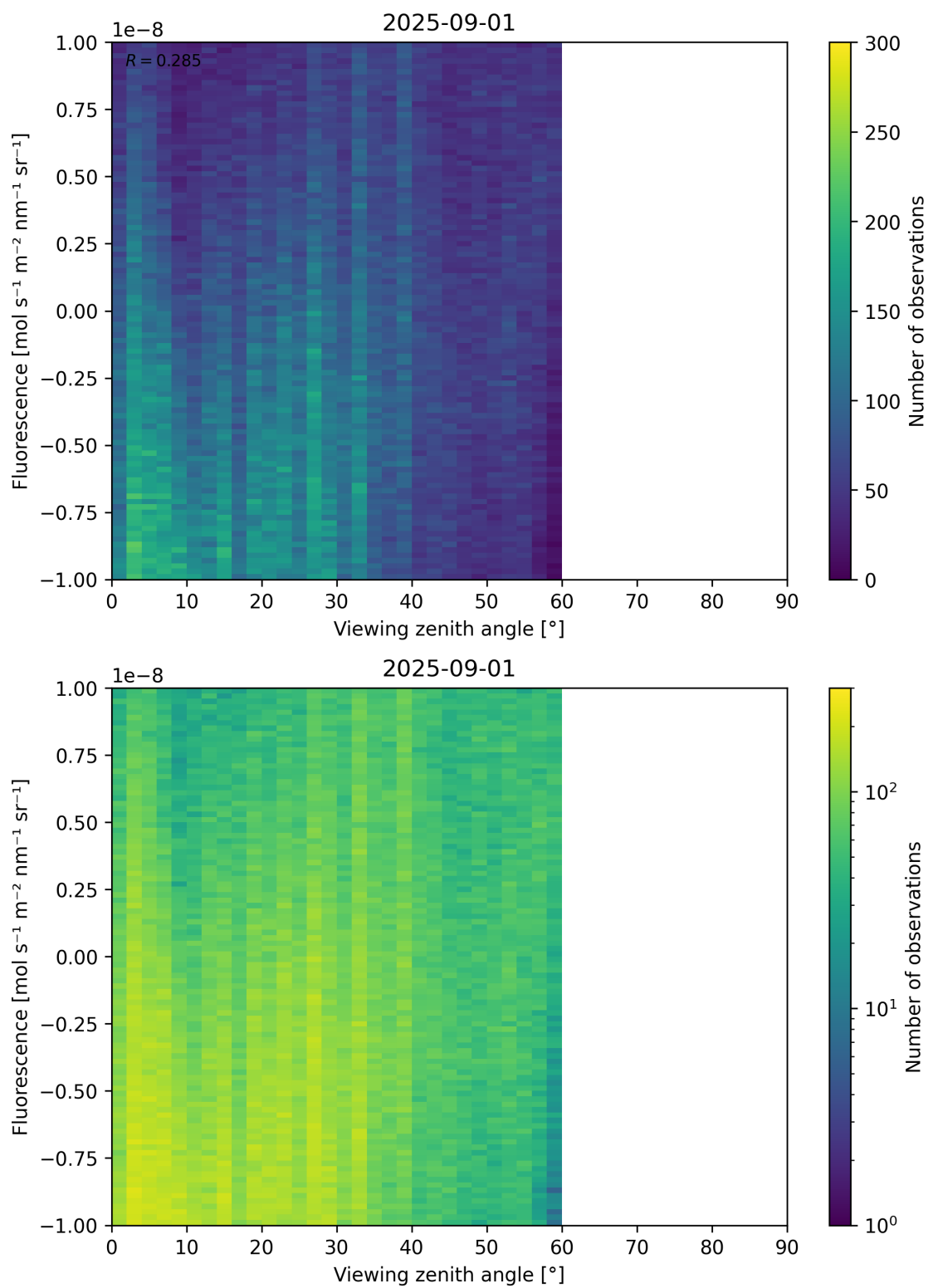
Figure 108: Scatter density plot of “Viewing zenith angle” against “Fluorescence” for 2025-08-31 to 2025-09-02.
