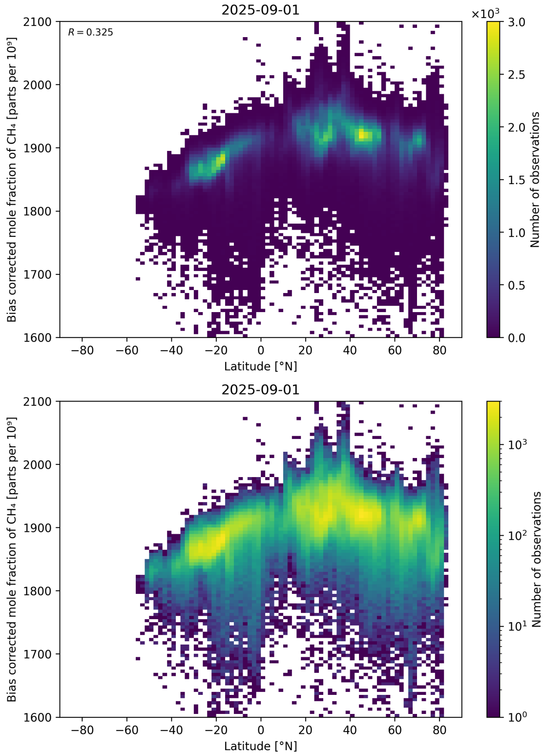
Figure 58: Scatter density plot of “Latitude” against “Bias corrected mole fraction of CH 4 ” for 2025-08-31 to 2025-09-02.
