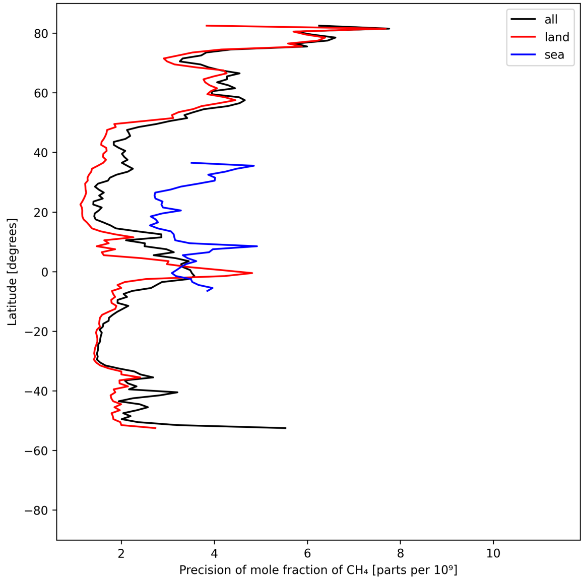
Figure 13: Zonal average of “Precision of mole fraction of CH 4 ” for 2025-08-31 to 2025-09-02.
