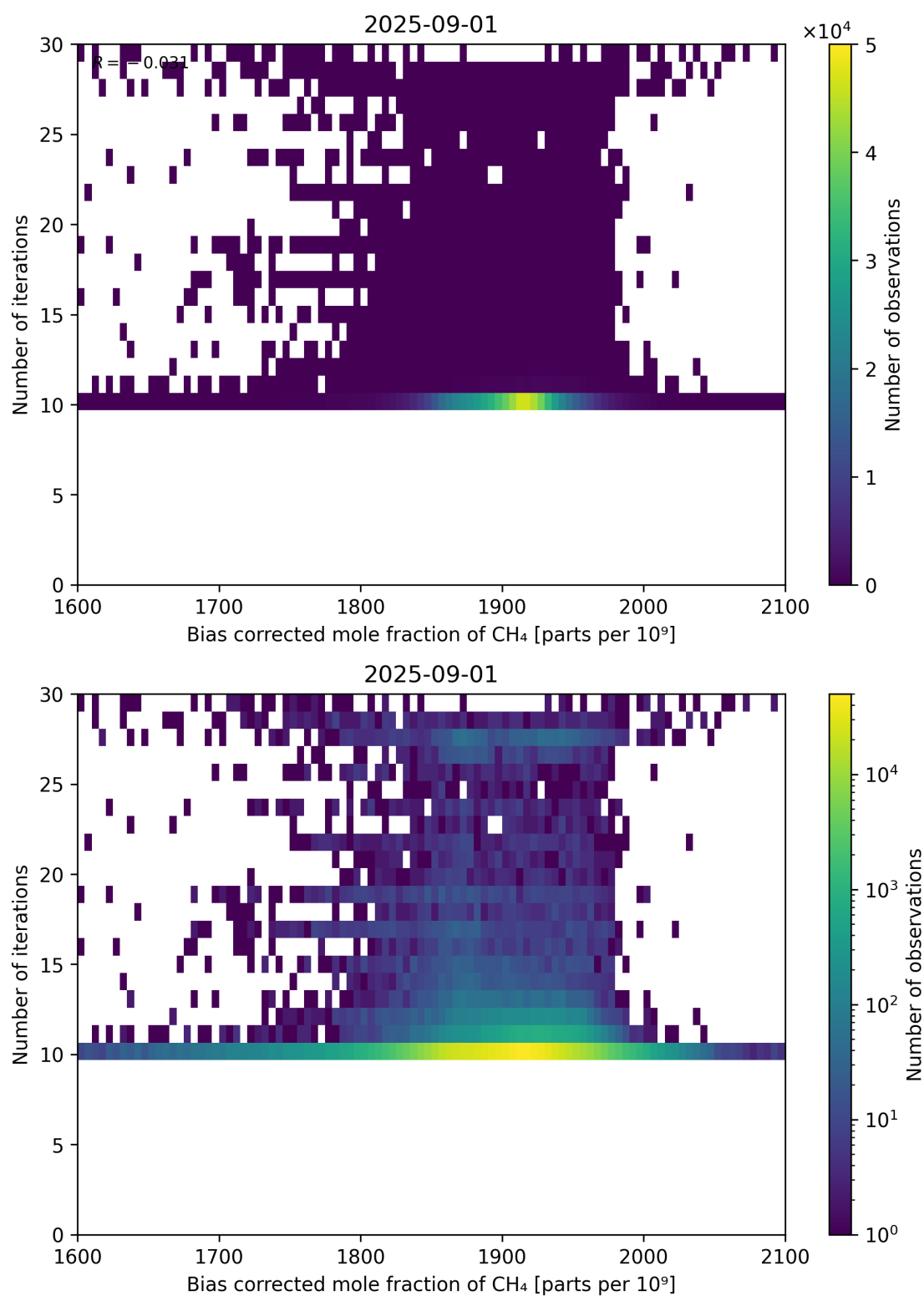
Figure 67: Scatter density plot of “Bias corrected mole fraction of CH 4 ” against “Number of iterations” for 2025-08-31 to 2025-09-02.
