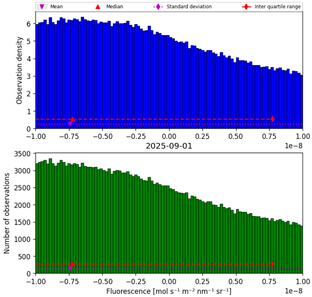
Figure 32: Histogram of “Fluorescence” for 2025-08-31 to 2025-09-02
