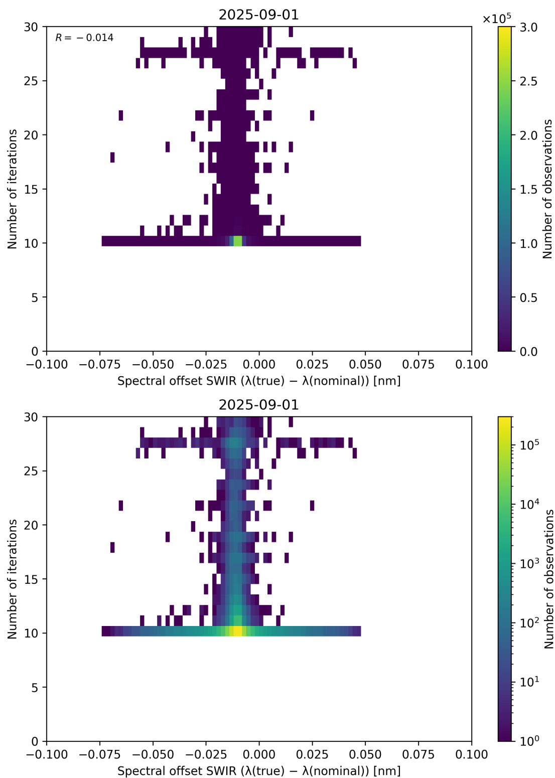
Figure 121: Scatter density plot of “Spectral offset SWIR ( \lambda_{\text{true}} - \lambda_{\text{nominal}} )” against “Number of iterations” for 2025-08-31 to 2025-09-02.
