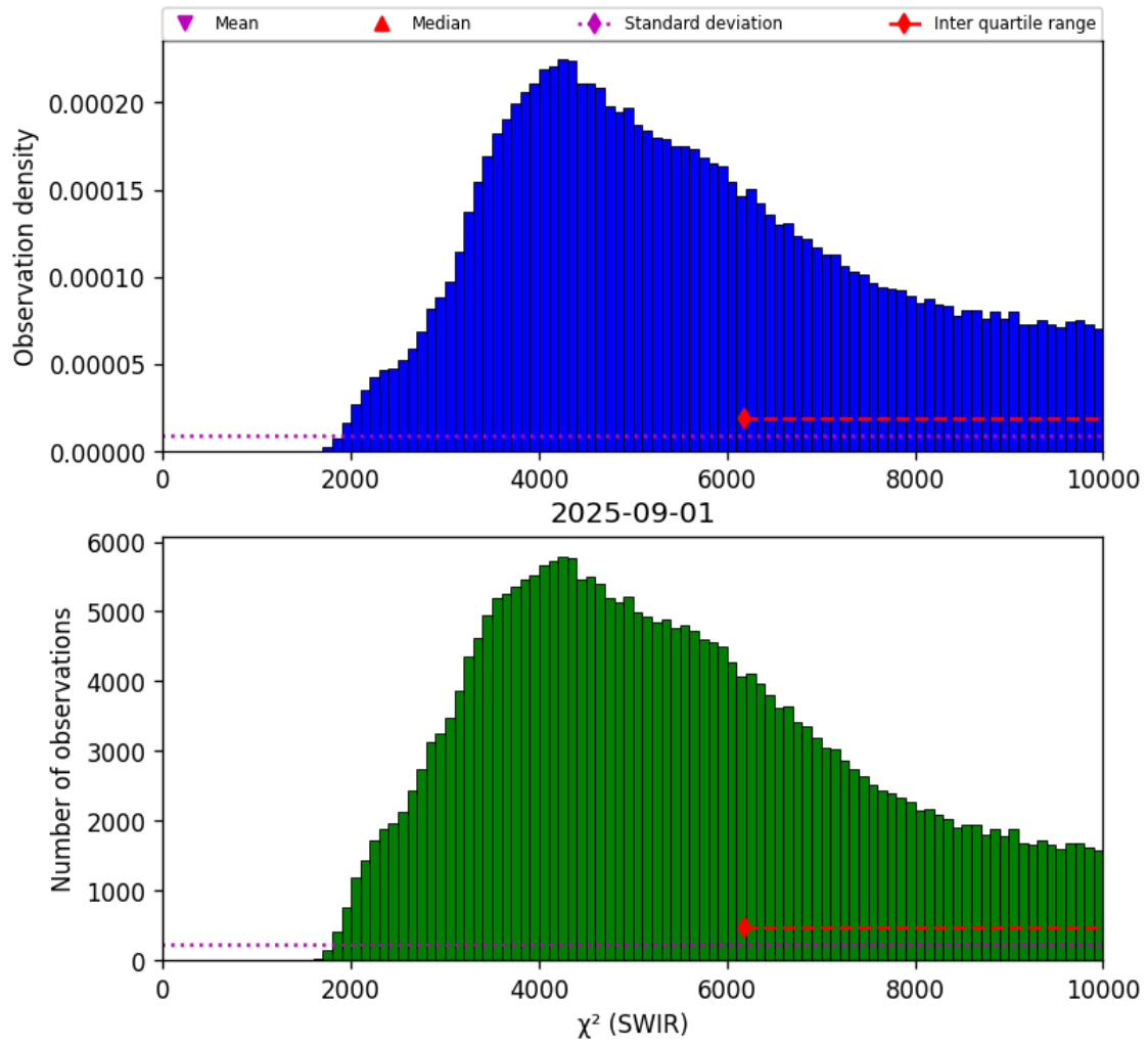
Figure 28: Histogram of " \chi^2 (SWIR)" for 2025-08-31 to 2025-09-02
