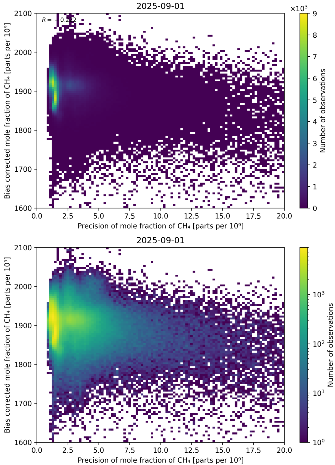
Figure 82: Scatter density plot of “Precision of mole fraction of CH 4 ” against “Bias corrected mole fraction of CH 4 ” for 2025-08-31 to 2025-09-02.
