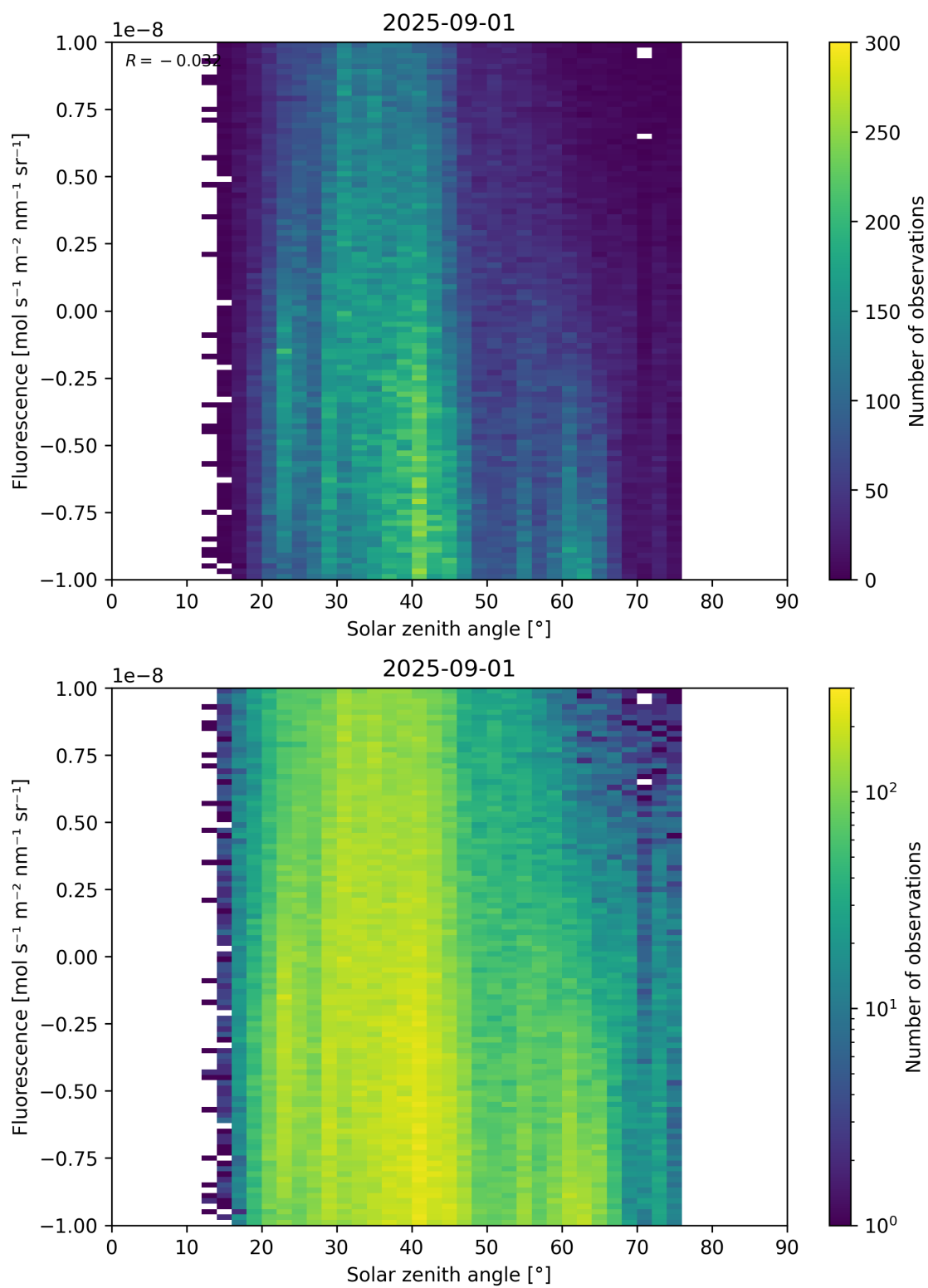
Figure 97: Scatter density plot of “Solar zenith angle” against “Fluorescence” for 2025-08-31 to 2025-09-02.
