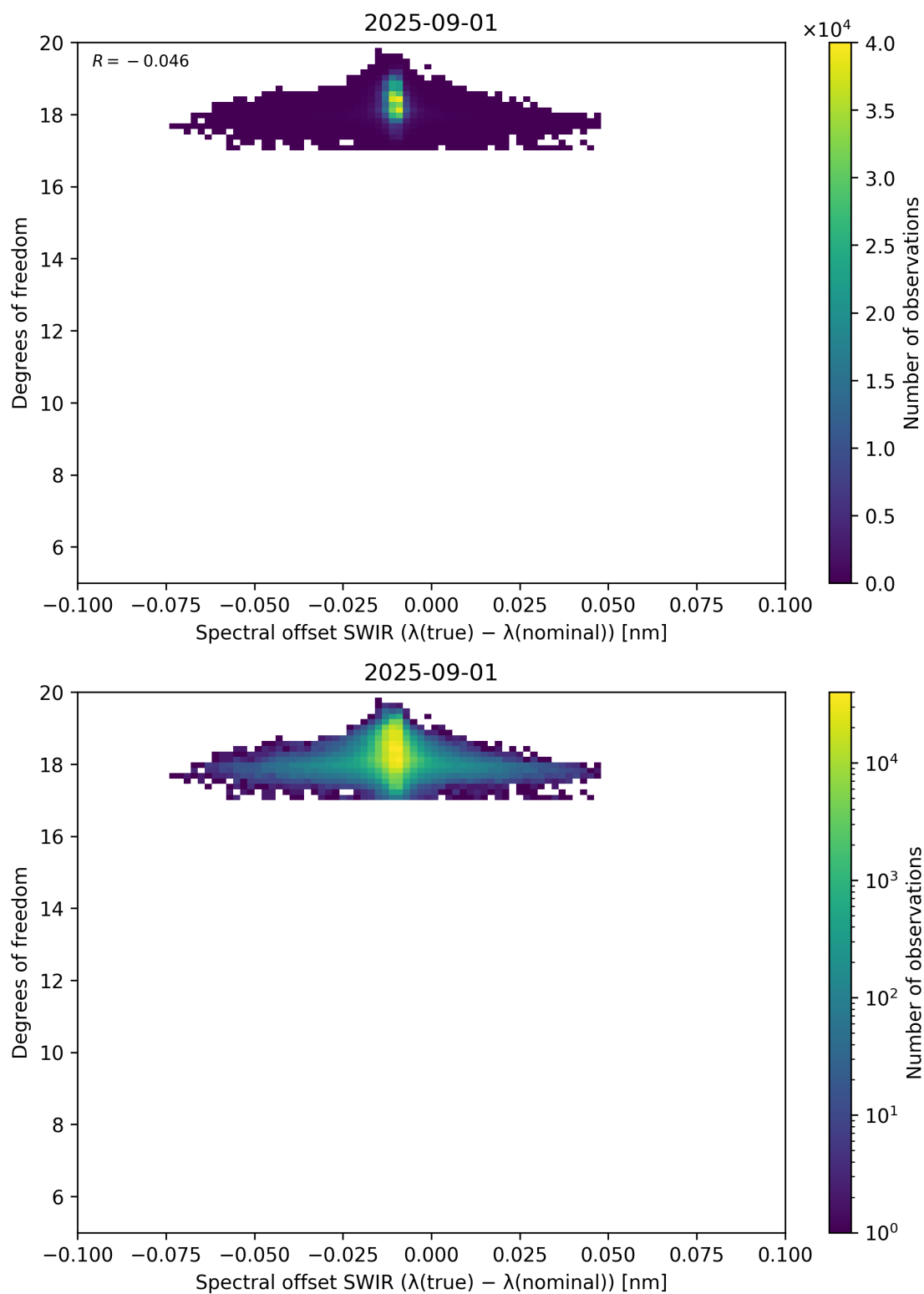
Figure 119: Scatter density plot of “Spectral offset SWIR ( \lambda_{\text{true}} - \lambda_{\text{nominal}} )” against “Degrees of freedom” for 2025-08-31 to 2025-09-02.
