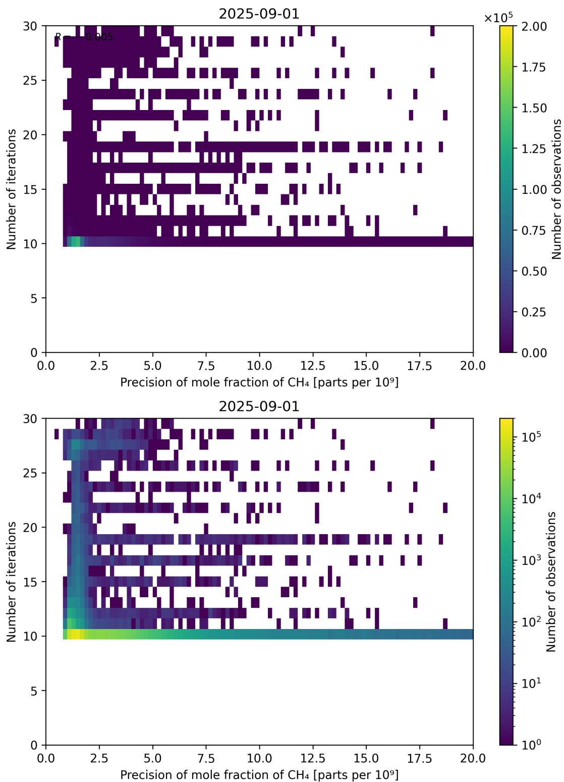
Figure 83: Scatter density plot of “Precision of mole fraction of CH 4 ” against “Number of iterations” for 2025-08-31 to 2025-09-02.
