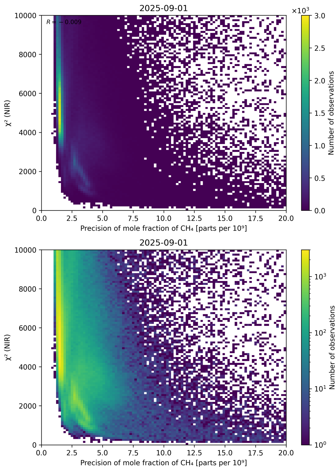
Figure 78: Scatter density plot of “Precision of mole fraction of CH 4 ” against “ \chi^2 (NIR)” for 2025-08-31 to 2025-09-02.
