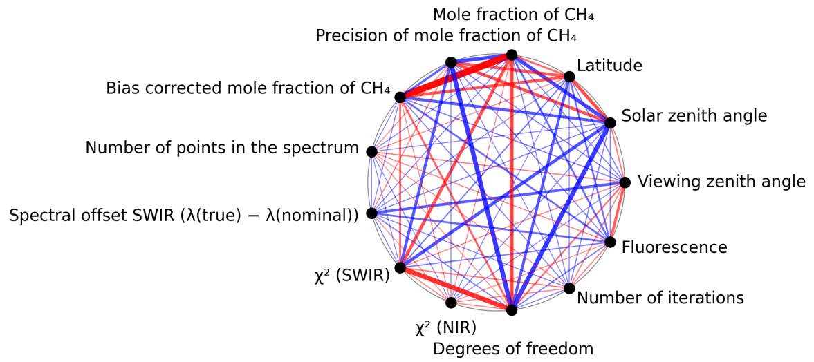
Figure 1: Map of correlation graph for 2025-08-31 to 2025-09-02.
