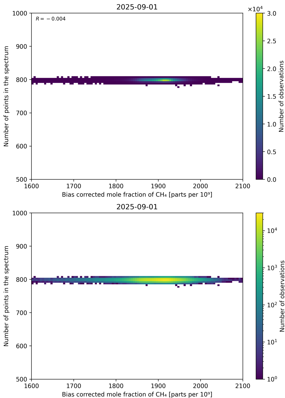
Figure 68: Scatter density plot of “Bias corrected mole fraction of CH 4 ” against “Number of points in the spectrum” for 2025-08-31 to 2025-09-02.
