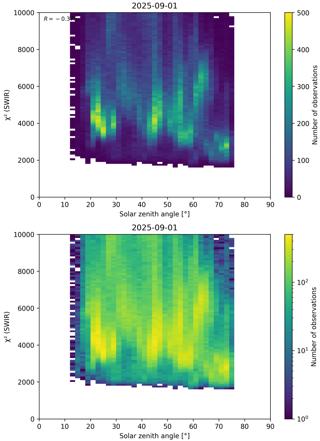
Figure 95: Scatter density plot of “Solar zenith angle” against “ \chi^2 (SWIR)” for 2025-08-31 to 2025-09-02.
