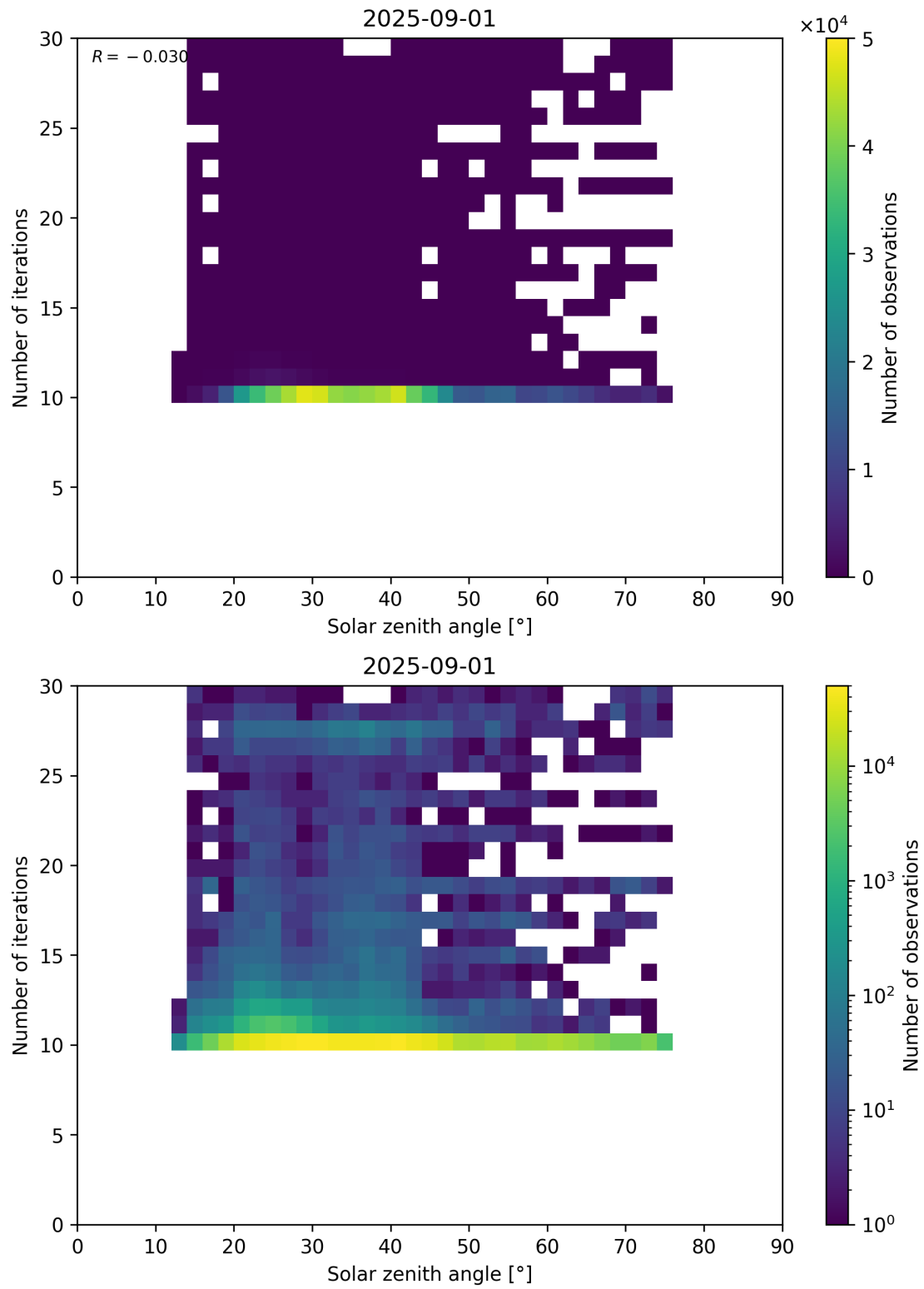
Figure 102: Scatter density plot of “Solar zenith angle” against “Number of iterations” for 2025-08-31 to 2025-09-02.
