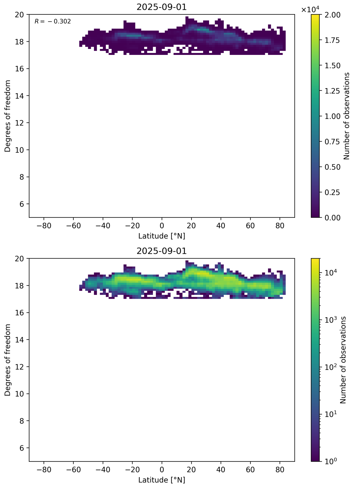
Figure 55: Scatter density plot of “Latitude” against “Degrees of freedom” for 2025-08-31 to 2025-09-02.
