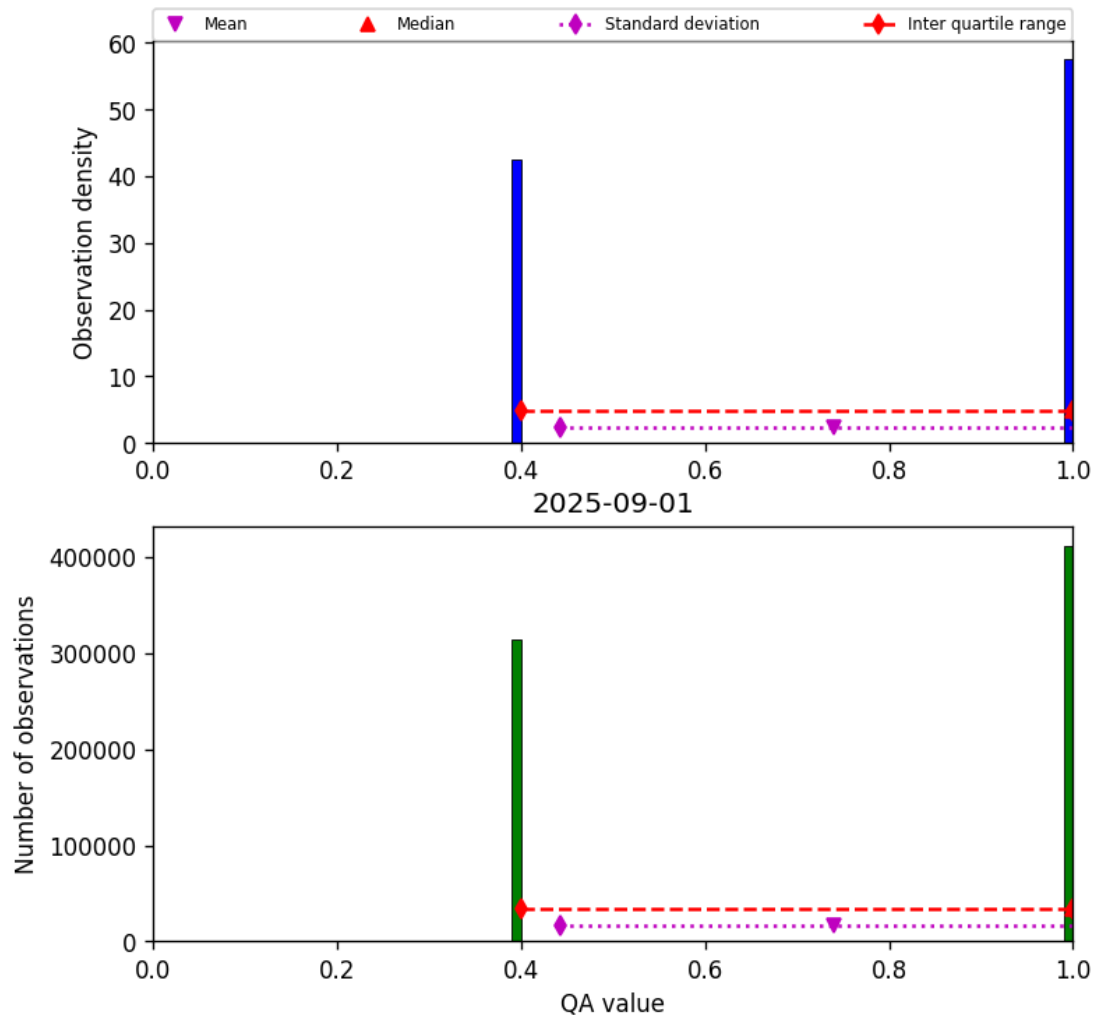
Figure 22: Histogram of “QA value” for 2025-08-31 to 2025-09-02
