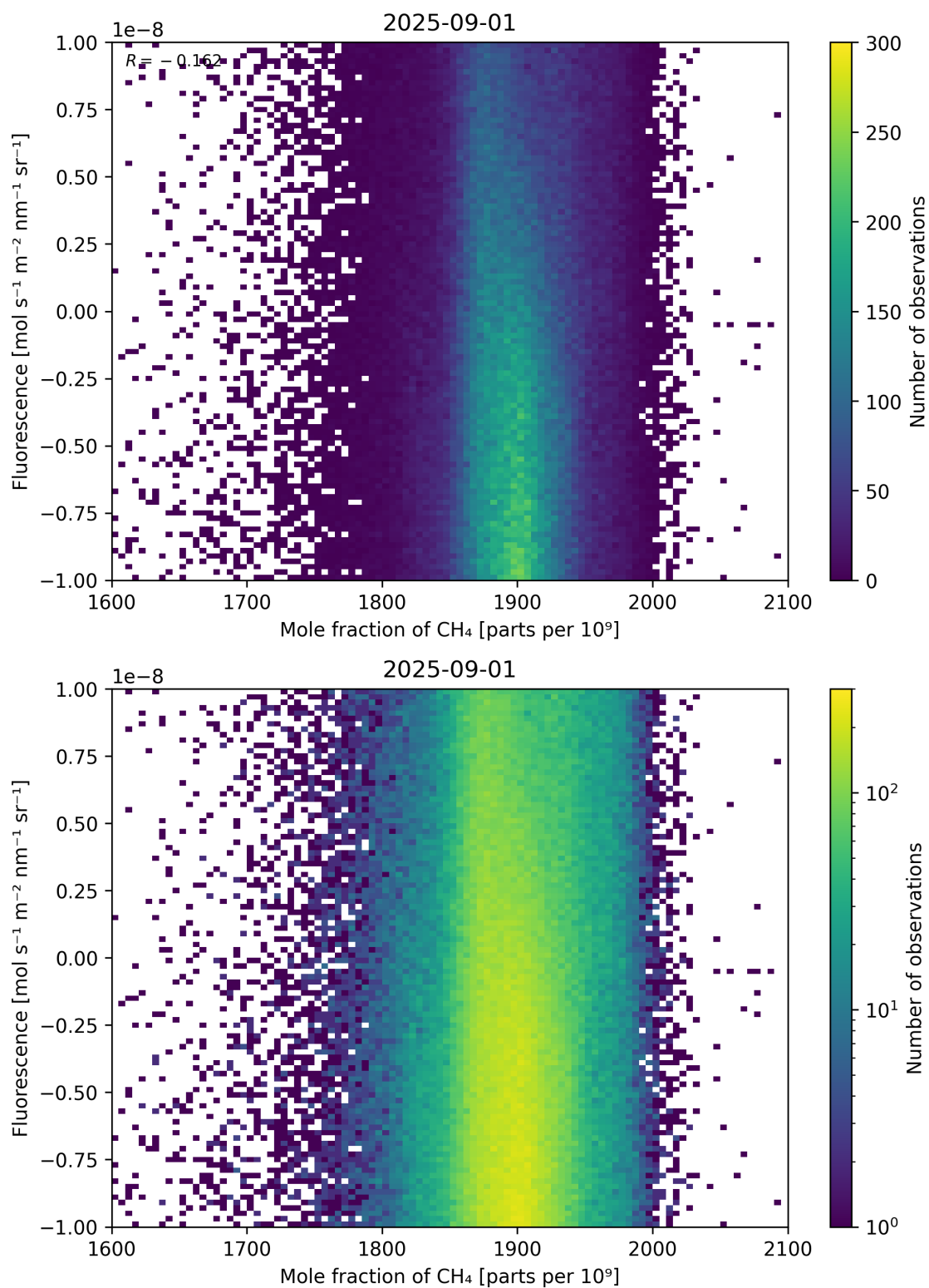
Figure 73: Scatter density plot of “Mole fraction of \text{CH}_4 ” against “Fluorescence” for 2025-08-31 to 2025-09-02.
