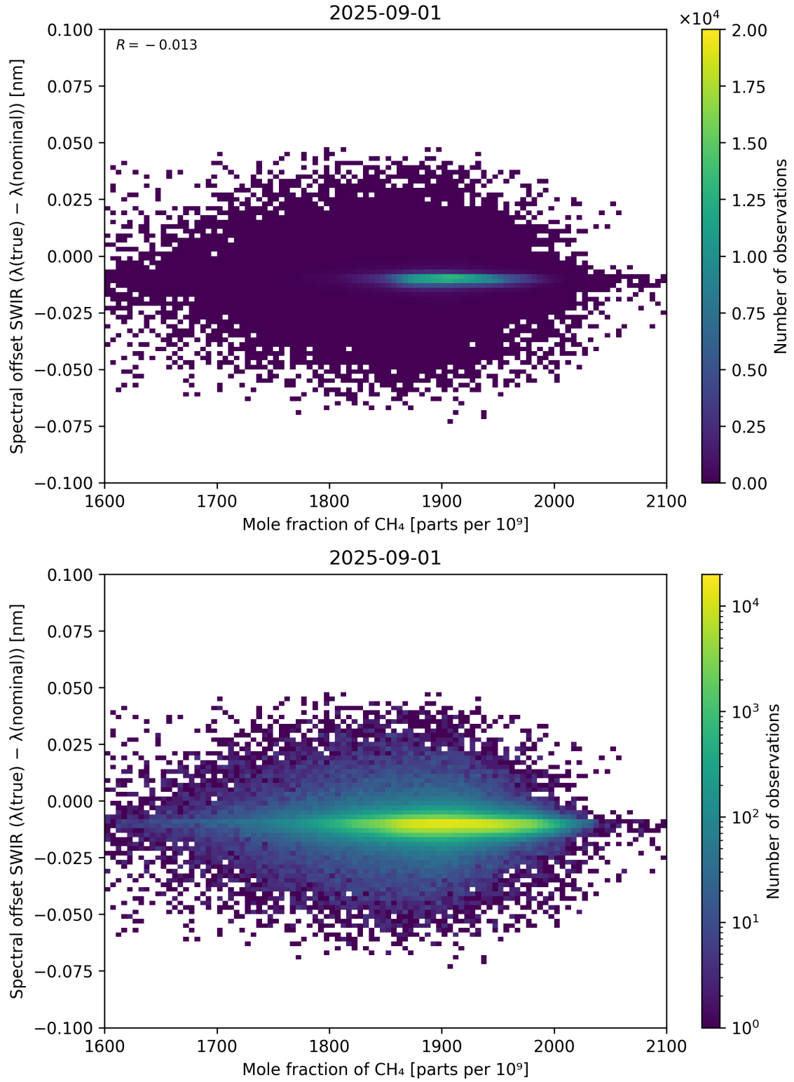
Figure 86: Scatter density plot of “Mole fraction of \text{CH}_4 ” against “Spectral offset SWIR ( \lambda_{\text{true}} - \lambda_{\text{nominal}} )” for 2025-08-31 to 2025-09-02.
