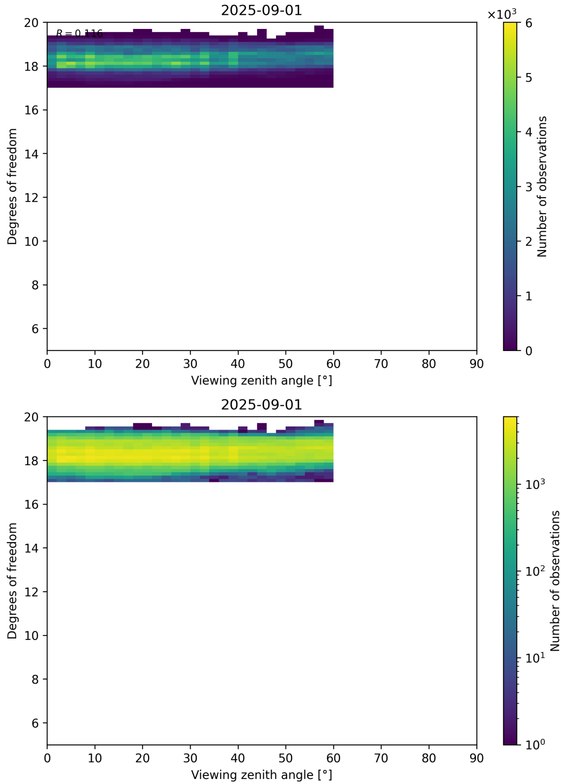
Figure 107: Scatter density plot of “Viewing zenith angle” against “Degrees of freedom” for 2025-08-31 to 2025-09-02.
