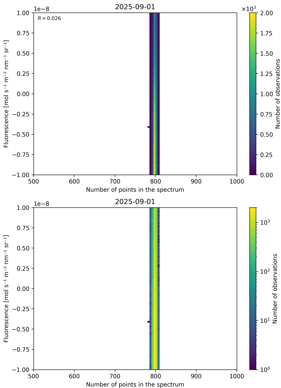
Figure 91: Scatter density plot of “Number of points in the spectrum” against “Fluorescence” for 2025-08-31 to 2025-09-02.
