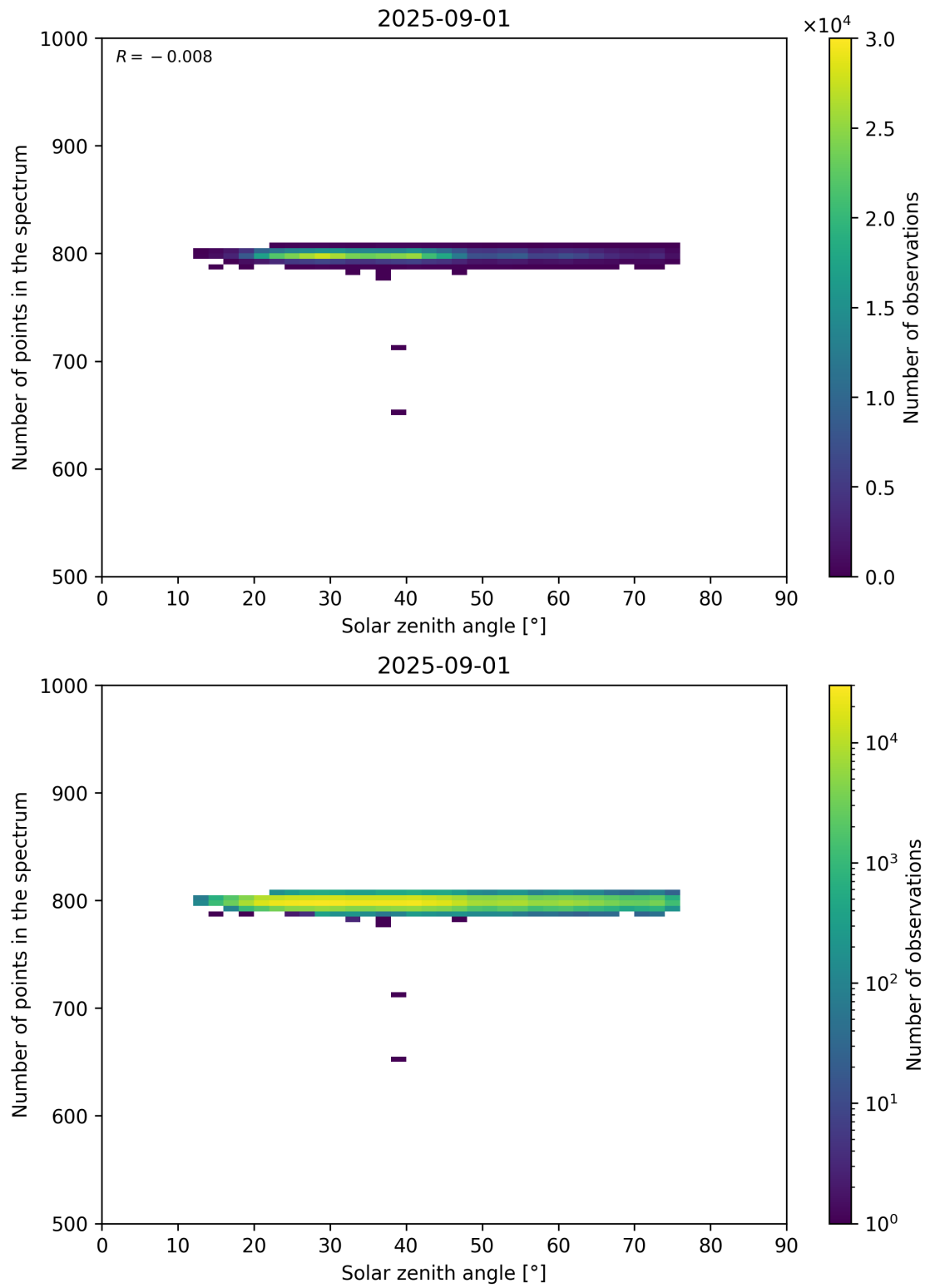
Figure 103: Scatter density plot of “Solar zenith angle” against “Number of points in the spectrum” for 2025-08-31 to 2025-09-02.
