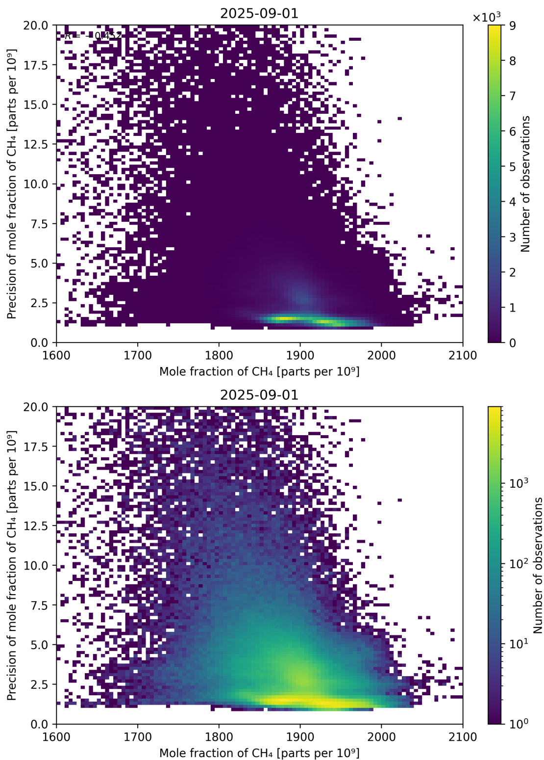
Figure 75: Scatter density plot of “Mole fraction of CH 4 ” against “Precision of mole fraction of CH 4 ” for 2025-08-31 to 2025-09-02.
