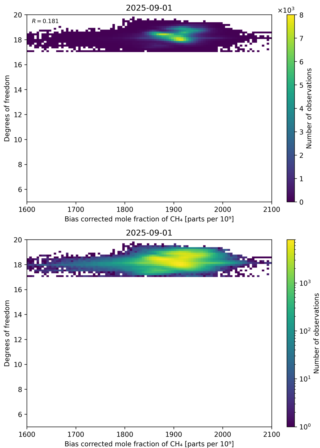
Figure 65: Scatter density plot of “Bias corrected mole fraction of CH 4 ” against “Degrees of freedom” for 2025-08-31 to 2025-09-02.
