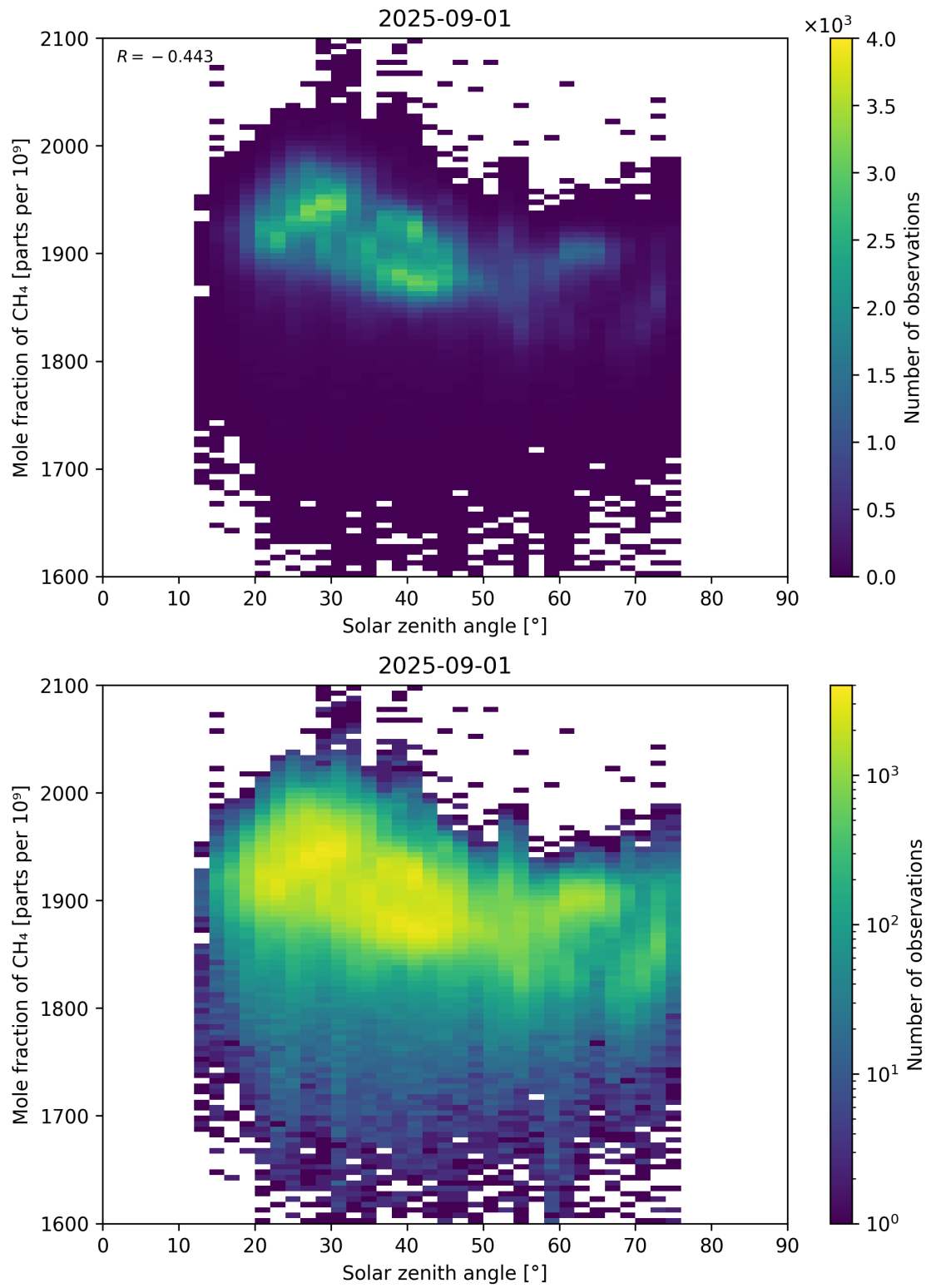
Figure 99: Scatter density plot of “Solar zenith angle” against “Mole fraction of CH 4 ” for 2025-08-31 to 2025-09-02.
