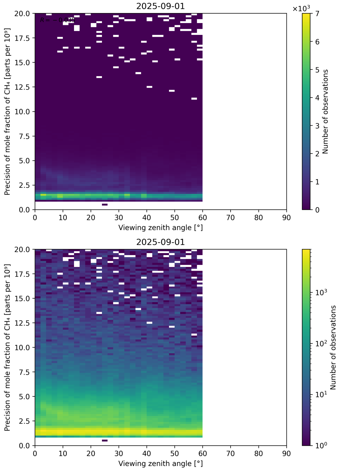
Figure 112: Scatter density plot of “Viewing zenith angle” against “Precision of mole fraction of CH 4 ” for 2025-08-31 to 2025-09-02.
