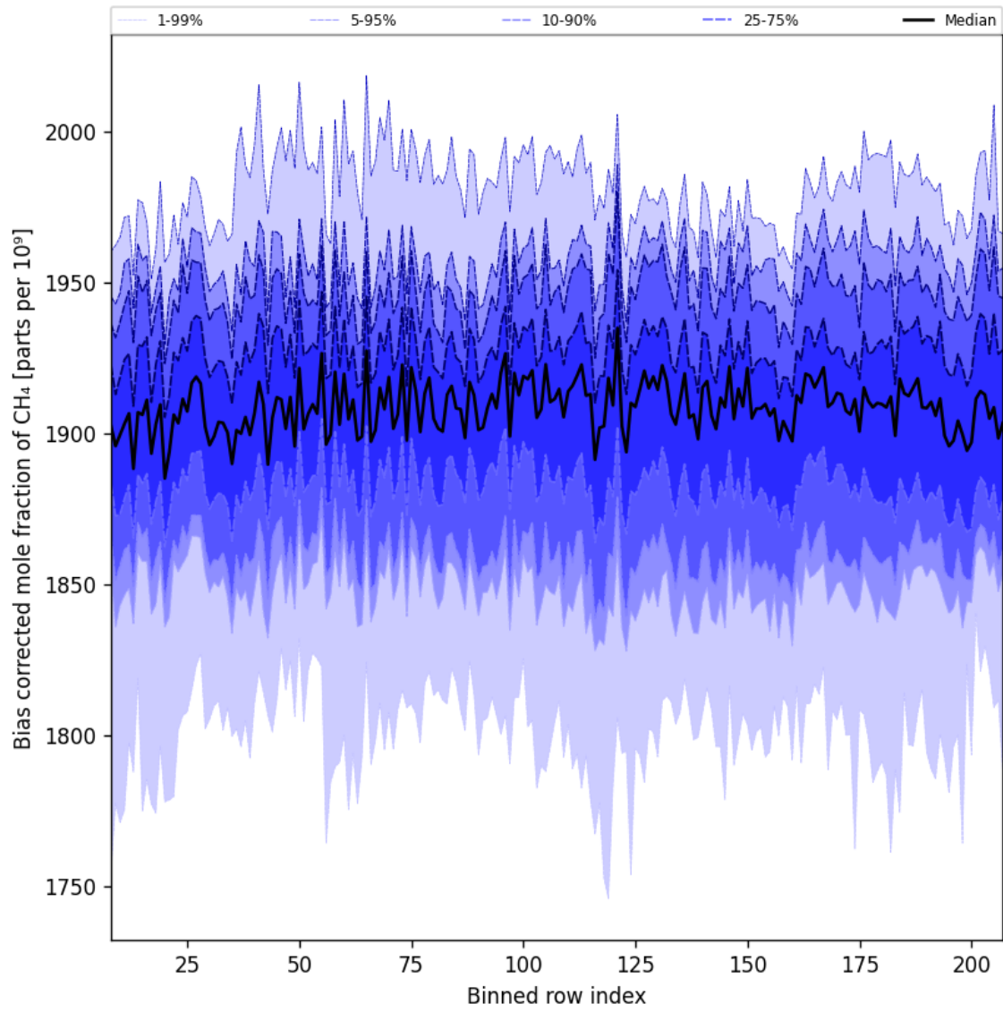
Figure 36: Along track statistics of “Bias corrected mole fraction of CH 4 ” for 2025-08-31 to 2025-09-02
