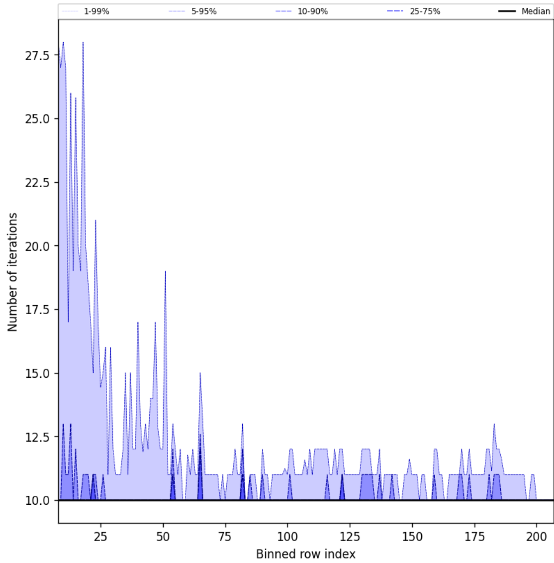
Figure 42: Along track statistics of “Number of iterations” for 2025-08-31 to 2025-09-02
