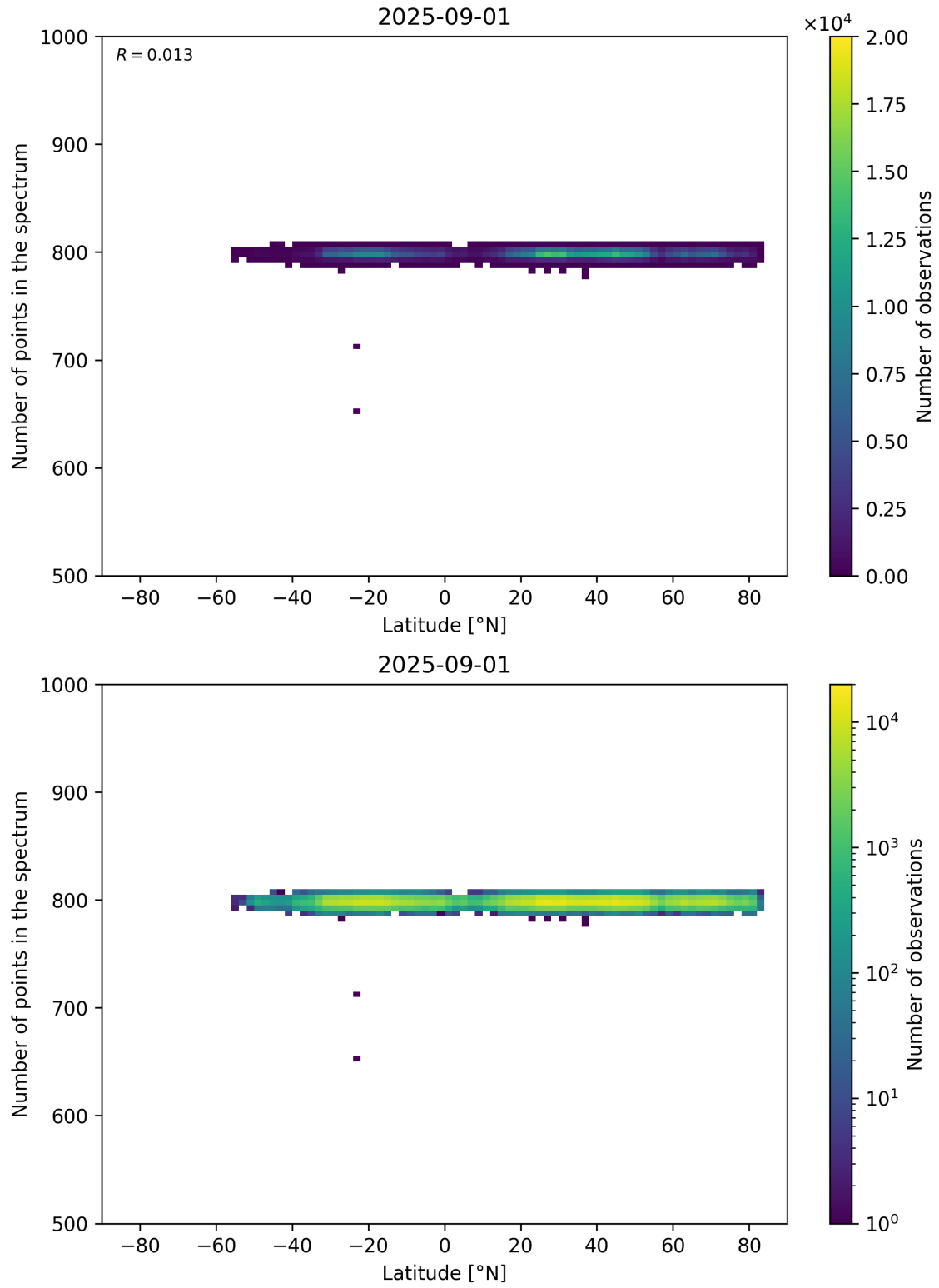
Figure 61: Scatter density plot of “Latitude” against “Number of points in the spectrum” for 2025-08-31 to 2025-09-02.
