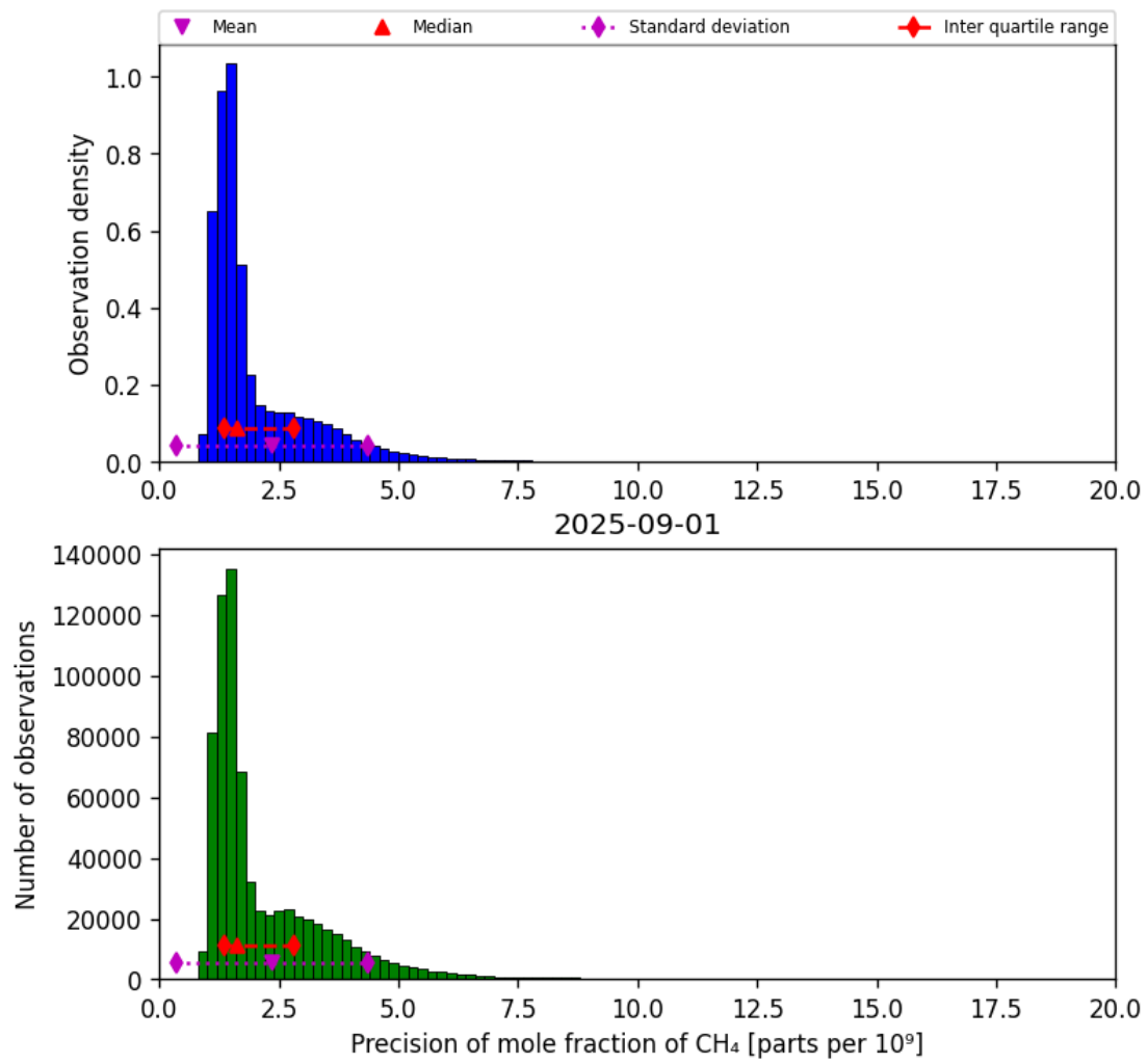
Figure 24: Histogram of “Precision of mole fraction of CH 4 ” for 2025-08-31 to 2025-09-02
