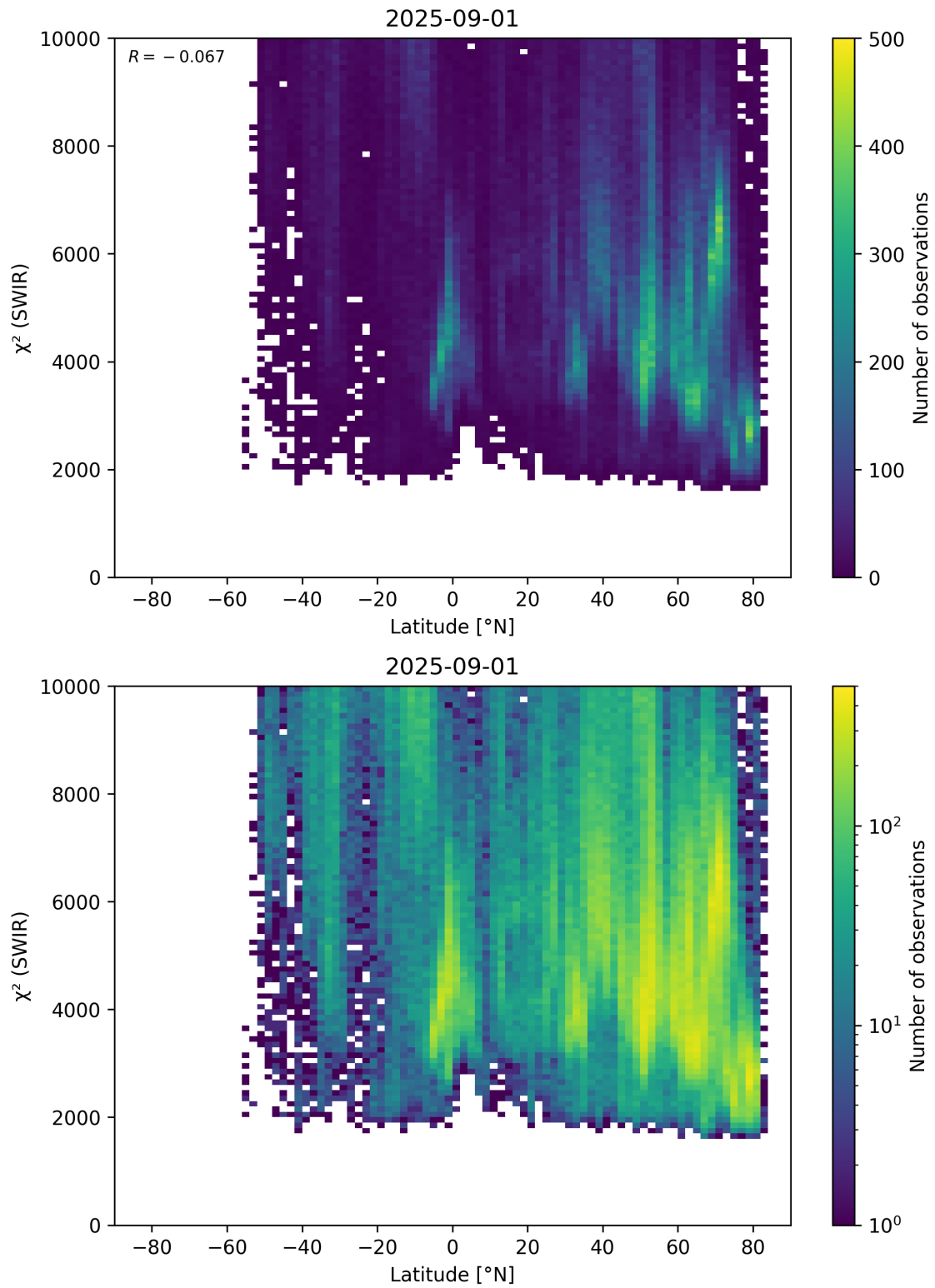
Figure 54: Scatter density plot of “Latitude” against “ \chi^2 (SWIR)” for 2025-08-31 to 2025-09-02.
