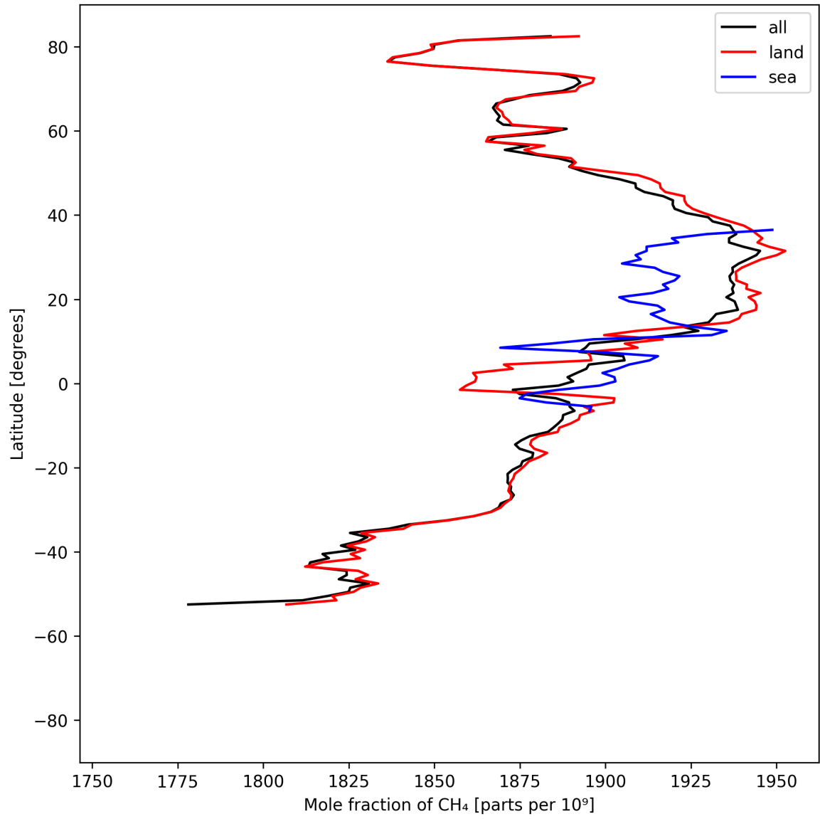
Figure 12: Zonal average of “Mole fraction of \text{CH}_4 ” for 2025-08-31 to 2025-09-02.
