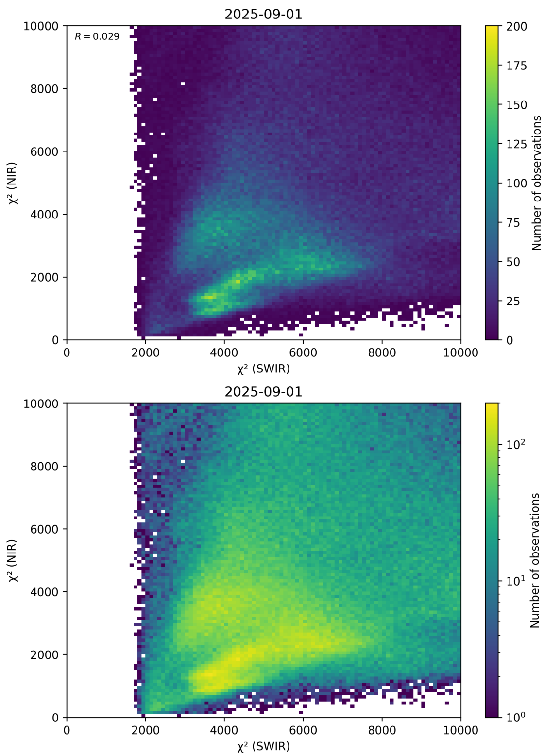
Figure 47: Scatter density plot of “ \chi^2 (SWIR)” against “ \chi^2 (NIR)” for 2025-08-31 to 2025-09-02.
