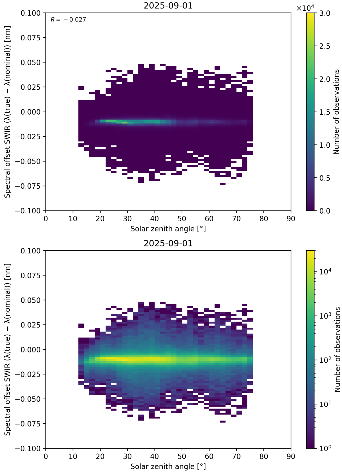
Figure 104: Scatter density plot of “Solar zenith angle” against “Spectral offset SWIR ( \lambda_{\text{true}} - \lambda_{\text{nominal}} )” for 2025-08-31 to 2025-09-02.
