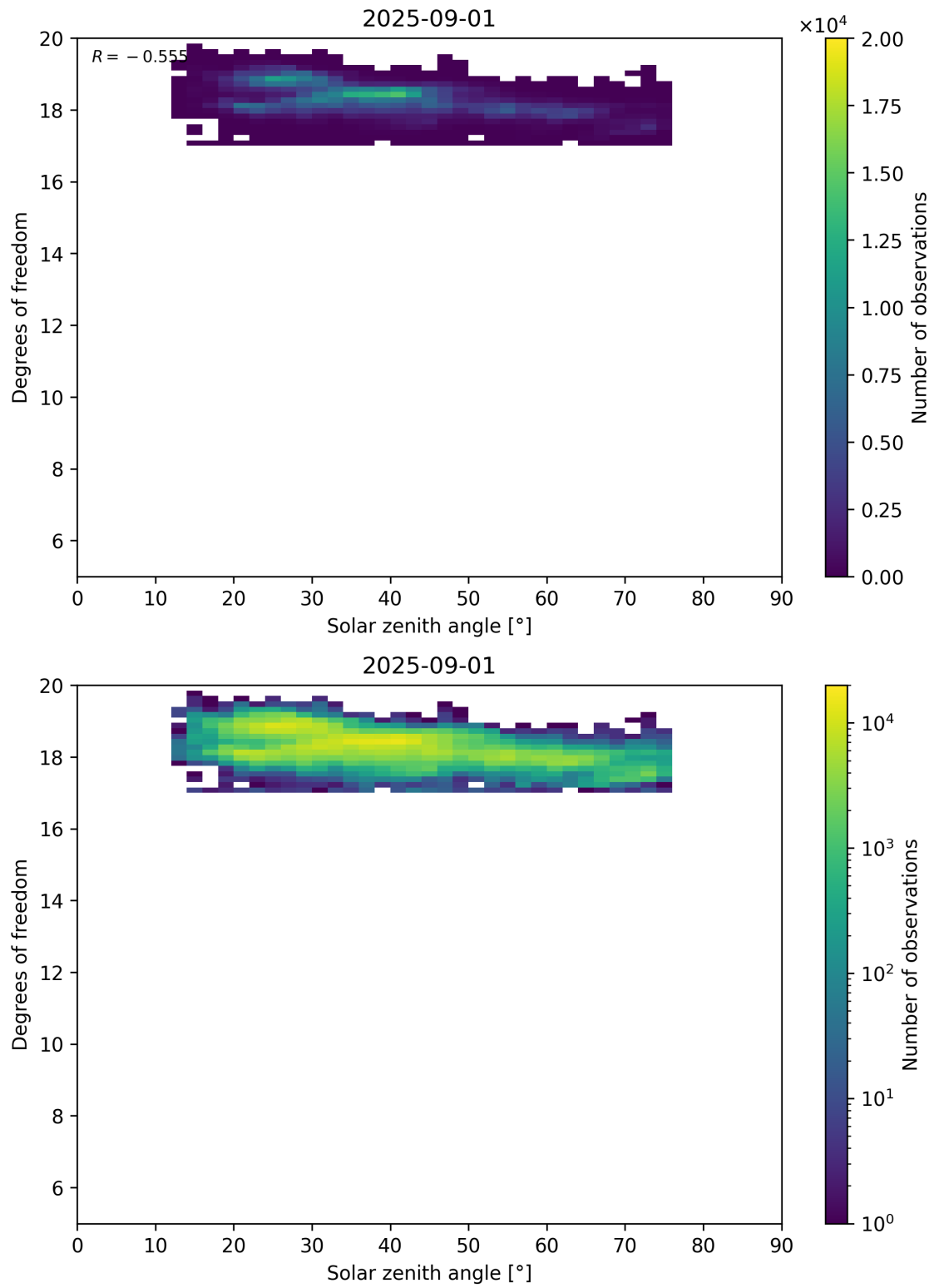
Figure 96: Scatter density plot of “Solar zenith angle” against “Degrees of freedom” for 2025-08-31 to 2025-09-02.
