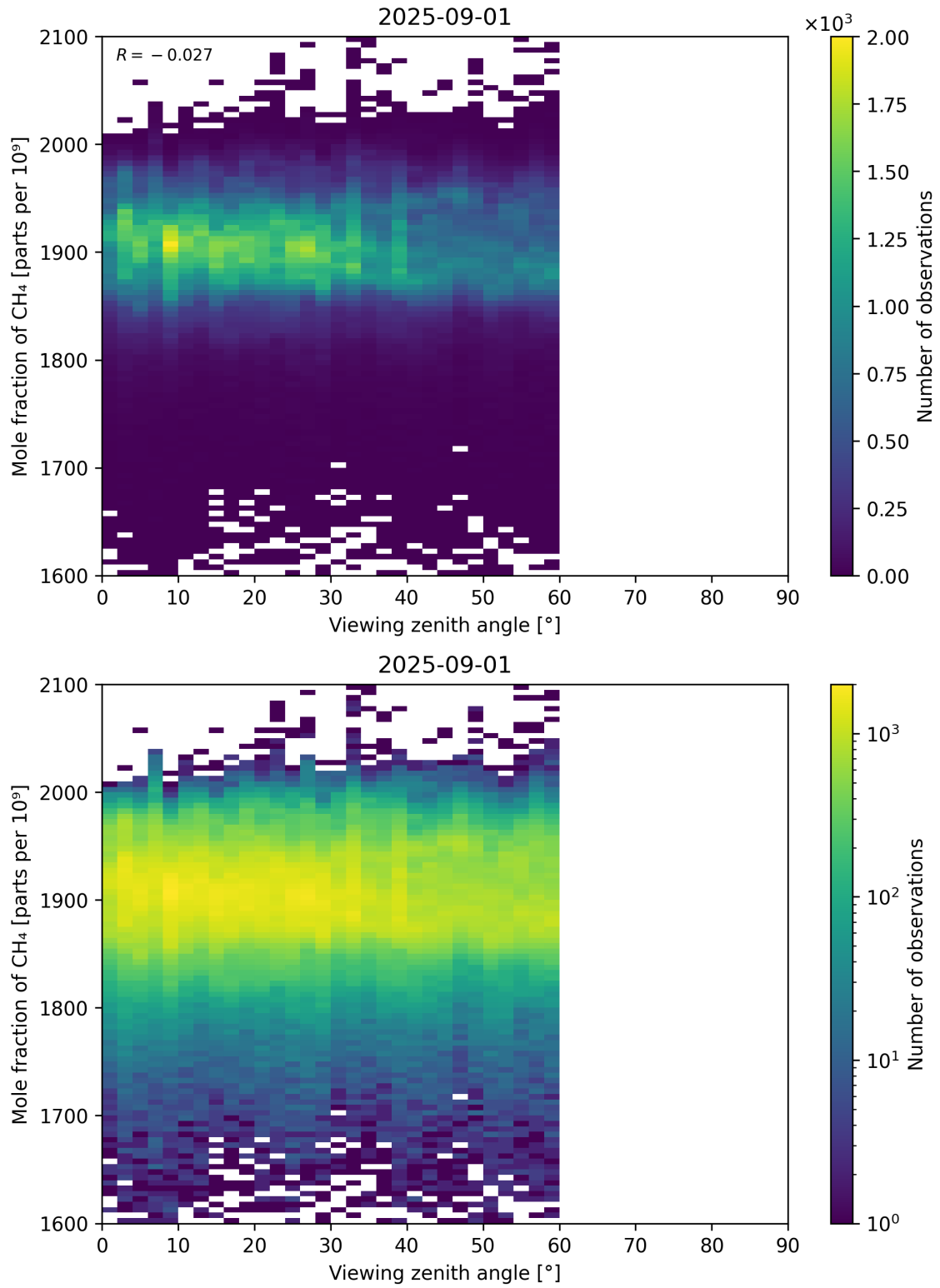
Figure 110: Scatter density plot of “Viewing zenith angle” against “Mole fraction of CH 4 ” for 2025-08-31 to 2025-09-02.
