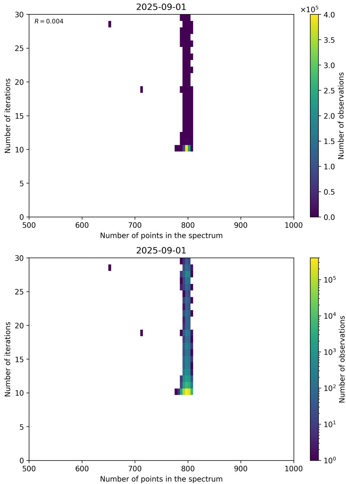
Figure 92: Scatter density plot of “Number of points in the spectrum” against “Number of iterations” for 2025-08-31 to 2025-09-02.
