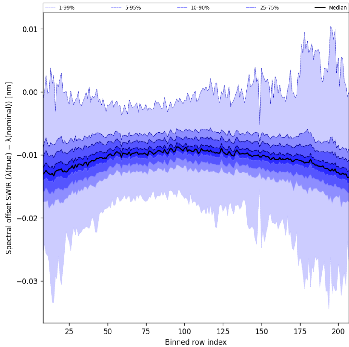
Figure 38: Along track statistics of “Spectral offset SWIR ( \lambda_{\text{true}} - \lambda_{\text{nominal}} )” for 2025-08-31 to 2025-09-02
