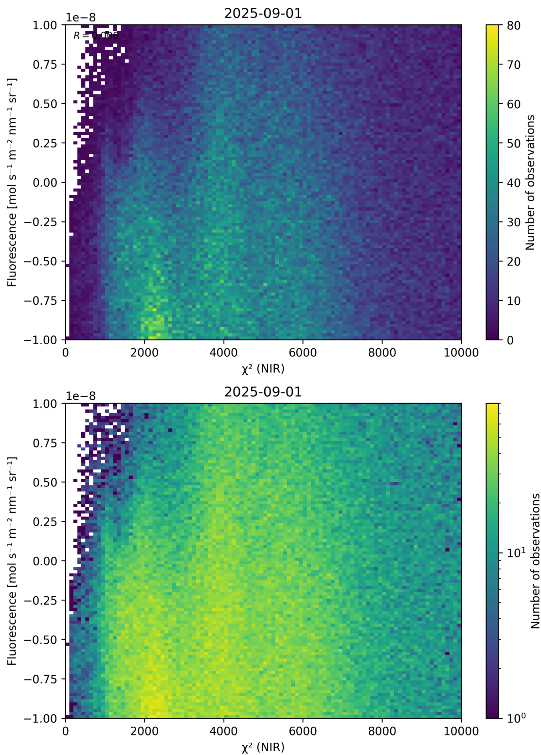
Figure 45: Scatter density plot of “ \chi^2 (NIR)” against “Fluorescence” for 2025-08-31 to 2025-09-02.
