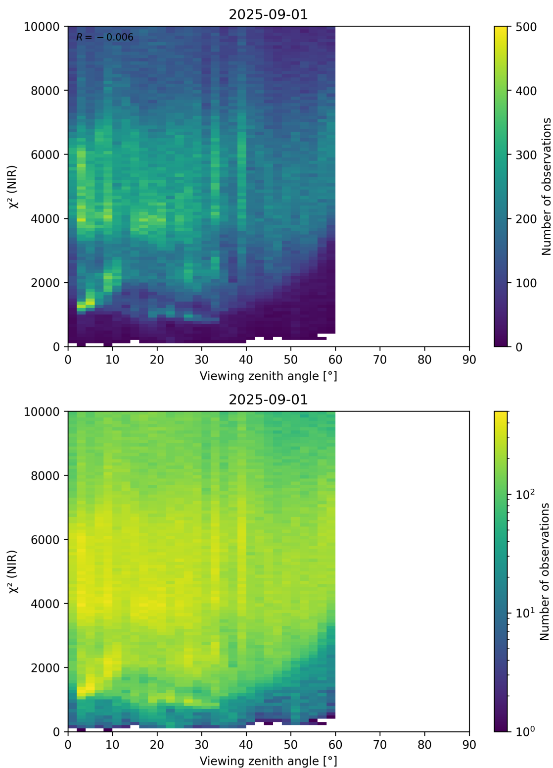
Figure 105: Scatter density plot of “Viewing zenith angle” against “ \chi^2 (NIR)” for 2025-08-31 to 2025-09-02.
