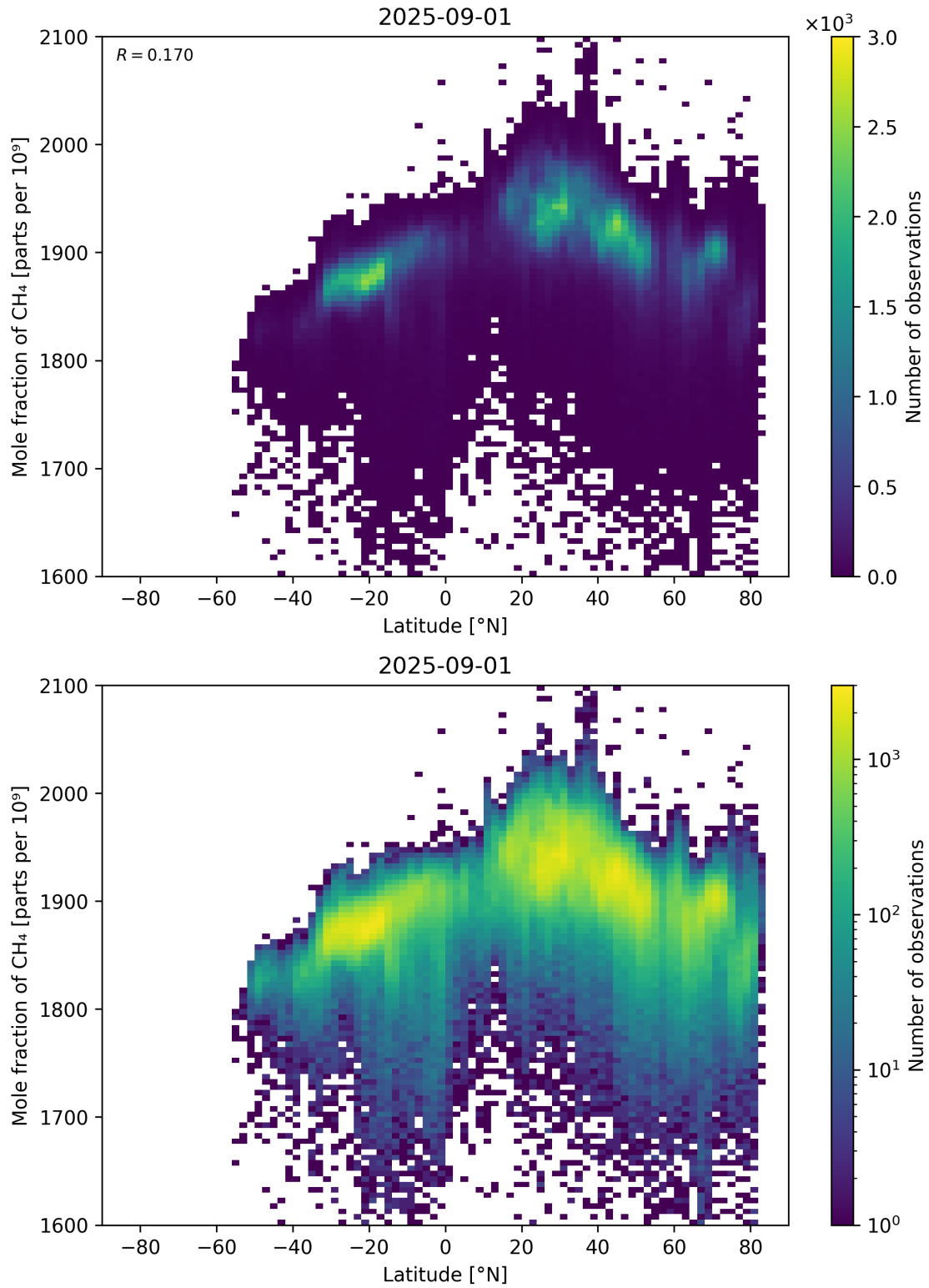
Figure 57: Scatter density plot of “Latitude” against “Mole fraction of \text{CH}_4 ” for 2025-08-31 to 2025-09-02.
