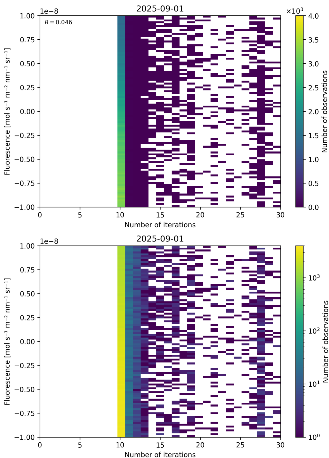
Figure 87: Scatter density plot of "Number of iterations" against "Fluorescence" for 2025-08-31 to 2025-09-02.
