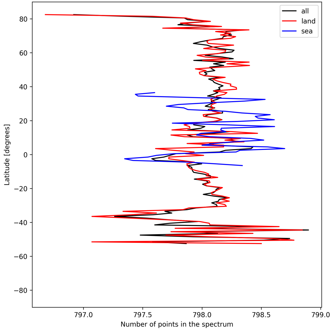
Figure 15: Zonal average of “Number of points in the spectrum” for 2025-08-31 to 2025-09-02.
