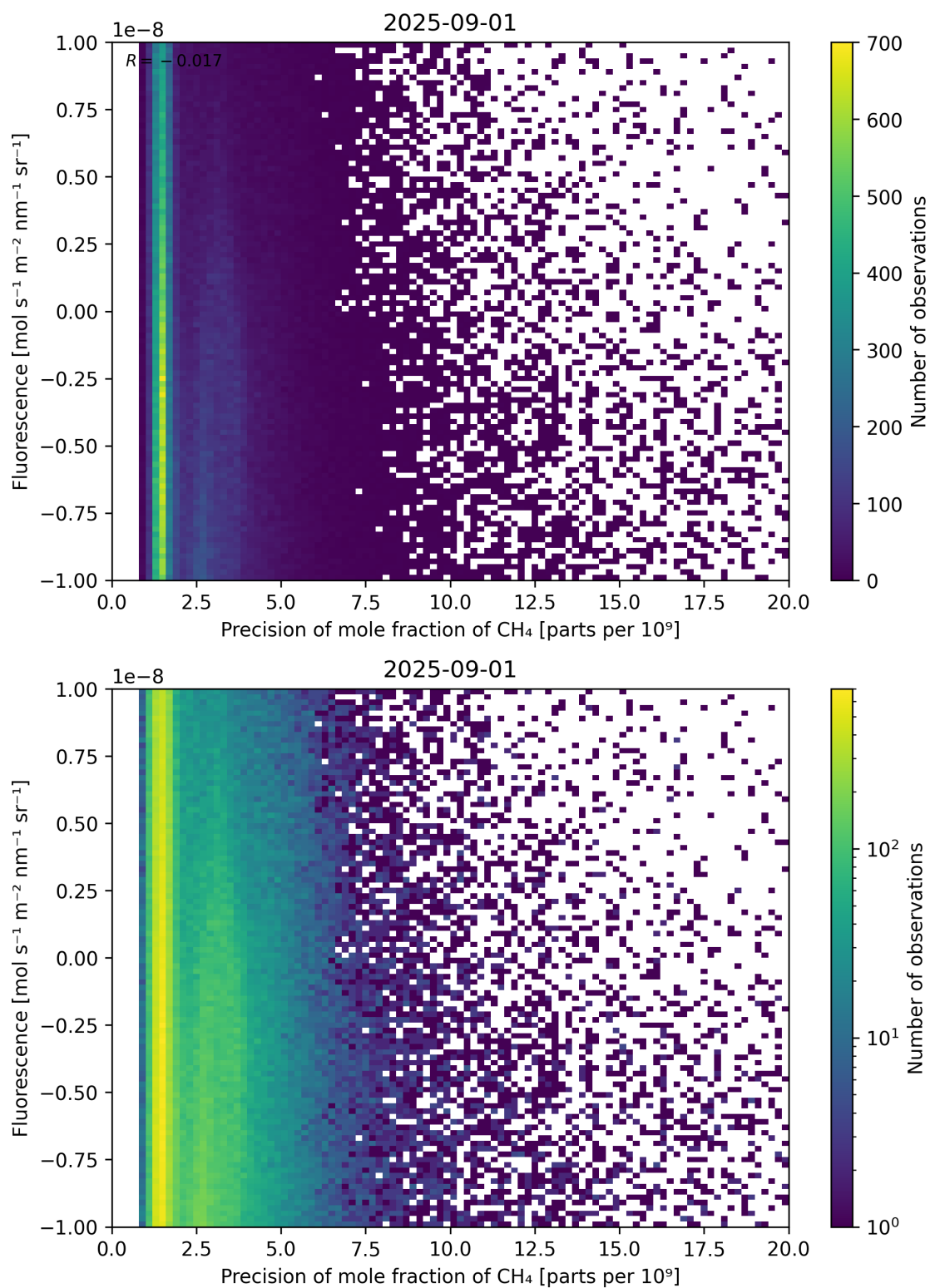
Figure 81: Scatter density plot of “Precision of mole fraction of \text{CH}_4 ” against “Fluorescence” for 2025-08-31 to 2025-09-02.
