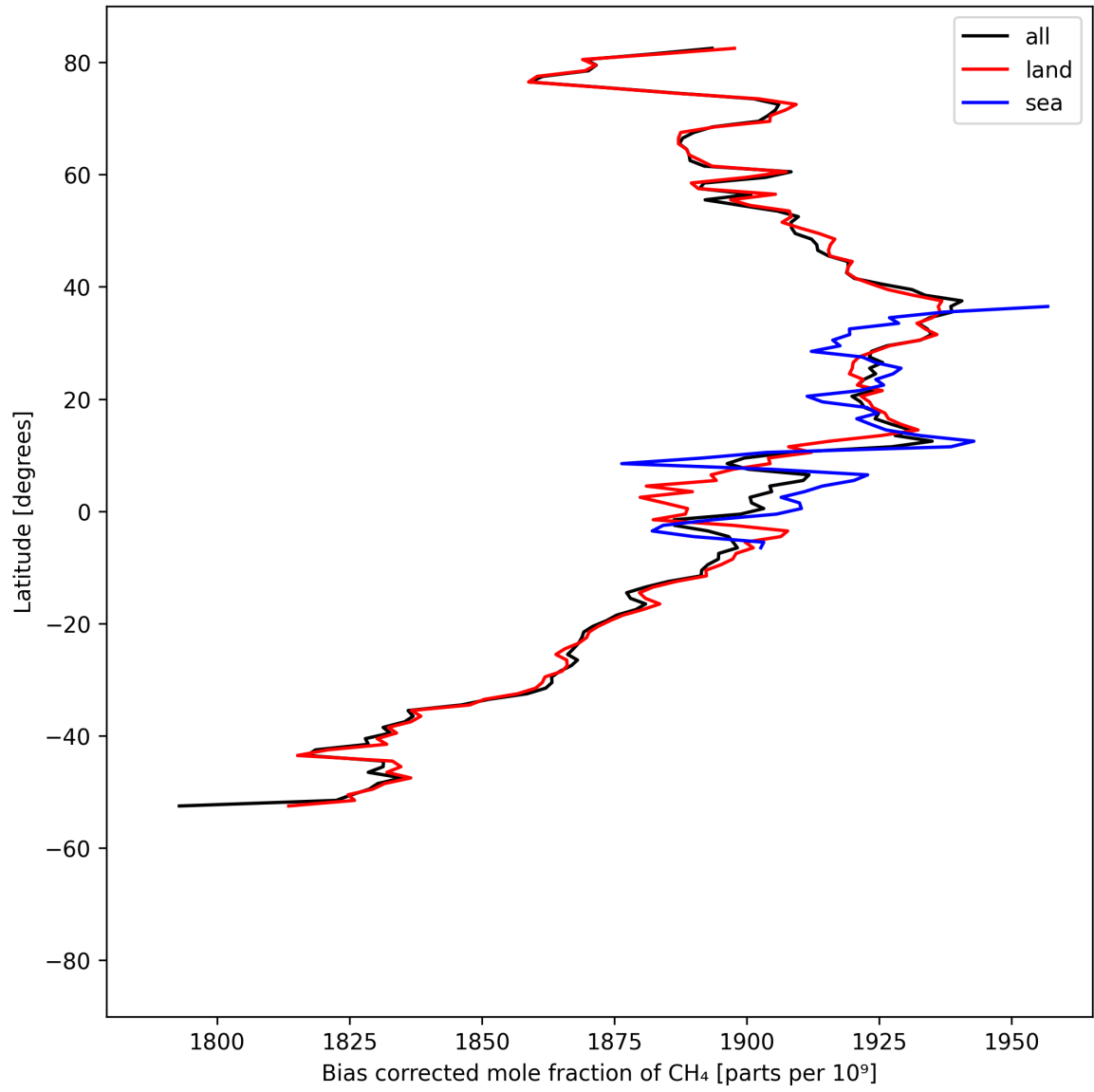
Figure 14: Zonal average of “Bias corrected mole fraction of CH 4 ” for 2025-08-31 to 2025-09-02.
