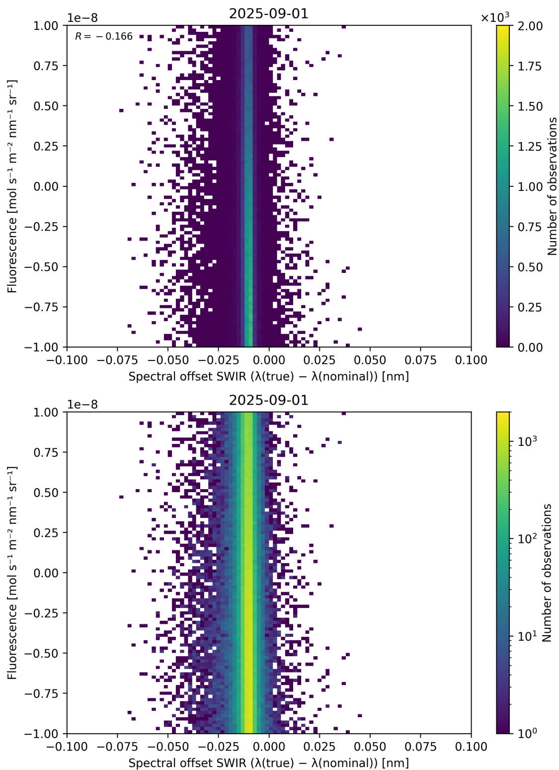
Figure 120: Scatter density plot of “Spectral offset SWIR ( \lambda_{\text{true}} - \lambda_{\text{nominal}} )” against “Fluorescence” for 2025-08-31 to 2025-09-02.
