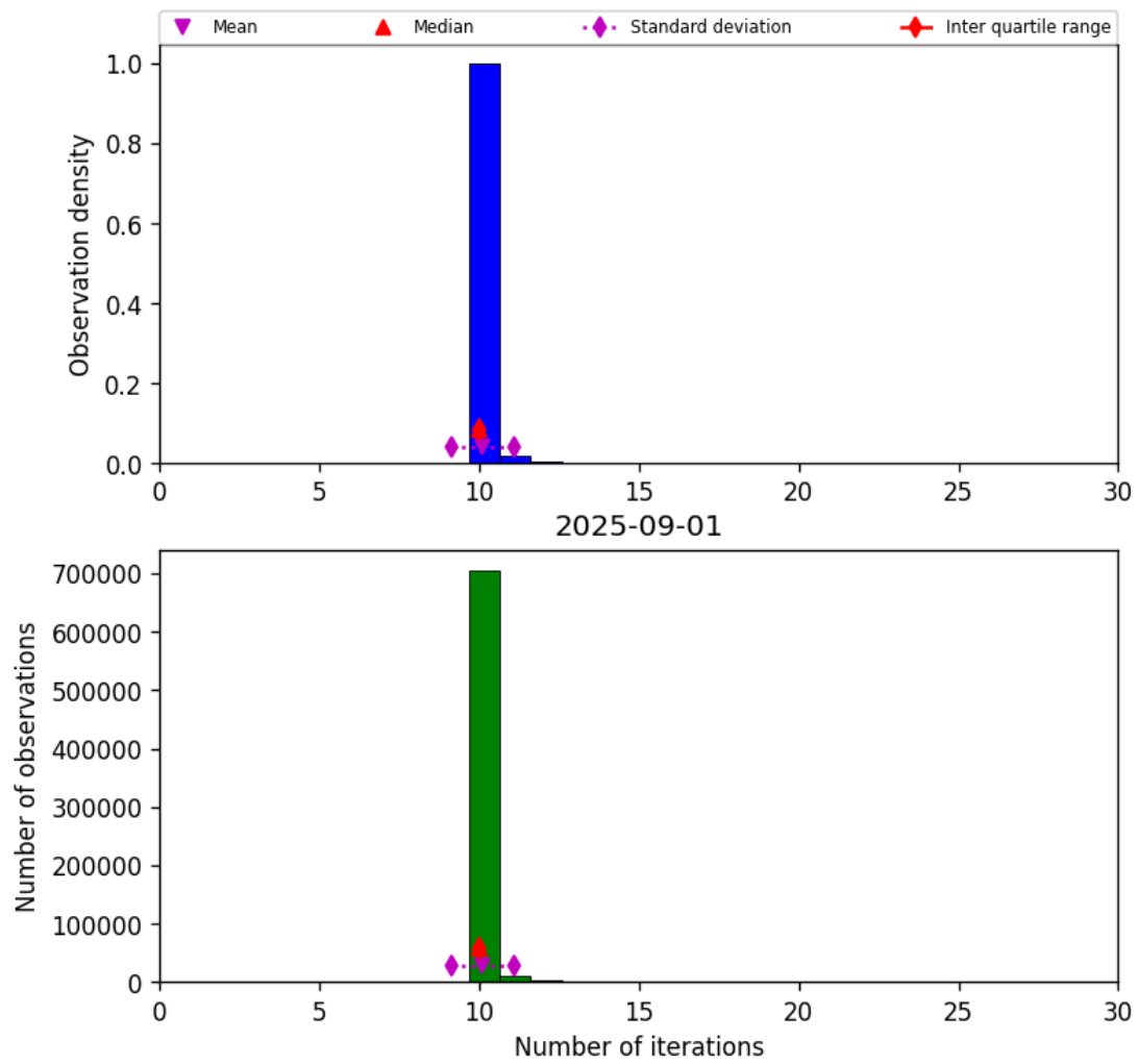
Figure 31: Histogram of “Number of iterations” for 2025-08-31 to 2025-09-02
