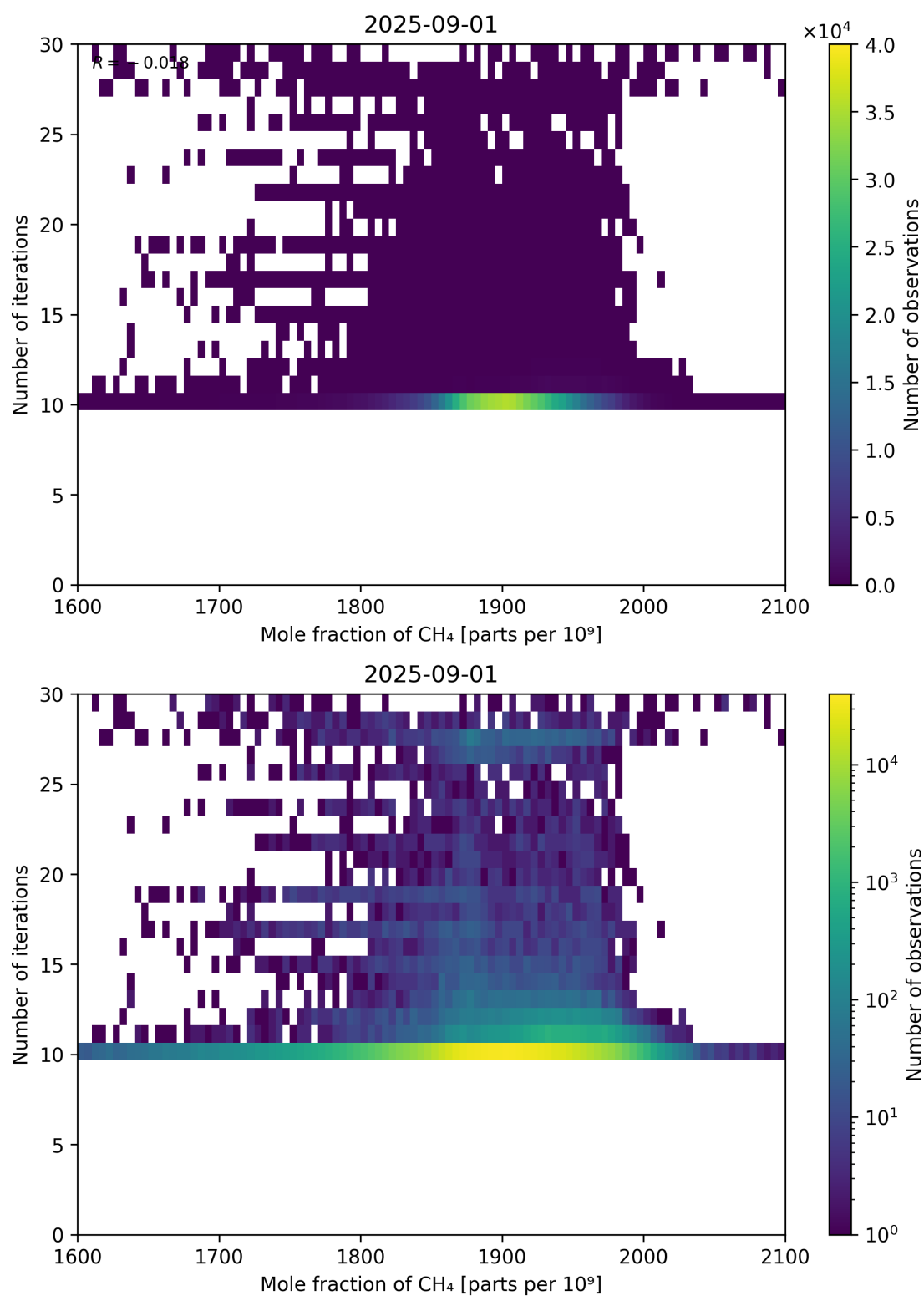
Figure 76: Scatter density plot of “Mole fraction of CH 4 ” against “Number of iterations” for 2025-08-31 to 2025-09-02.
