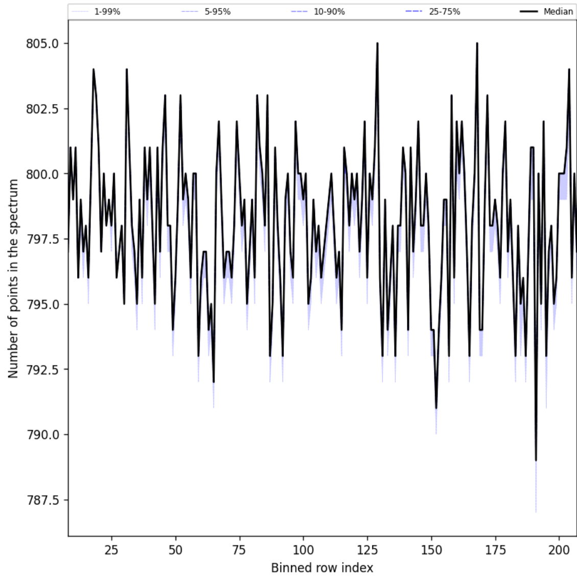
Figure 37: Along track statistics of “Number of points in the spectrum” for 2025-08-31 to 2025-09-02
