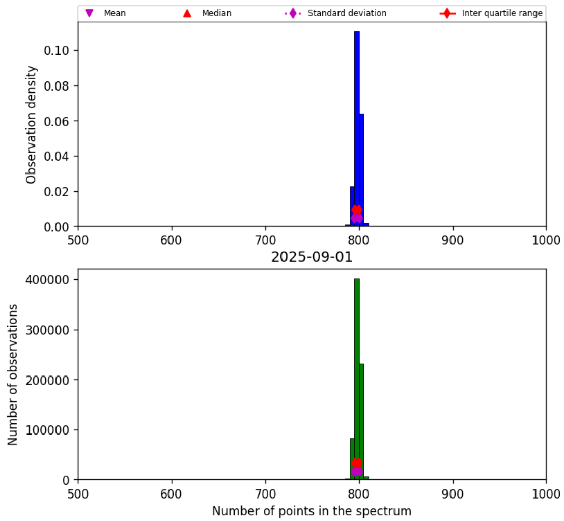
Figure 26: Histogram of “Number of points in the spectrum” for 2025-08-31 to 2025-09-02
