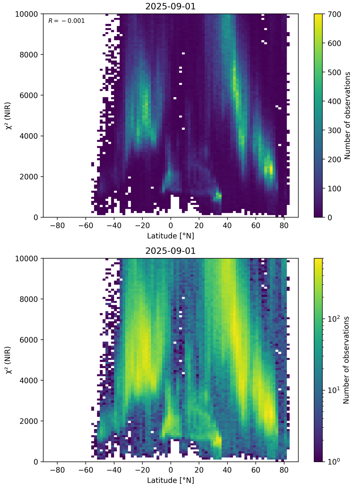
Figure 53: Scatter density plot of “Latitude” against “ \chi^2 (NIR)” for 2025-08-31 to 2025-09-02.
