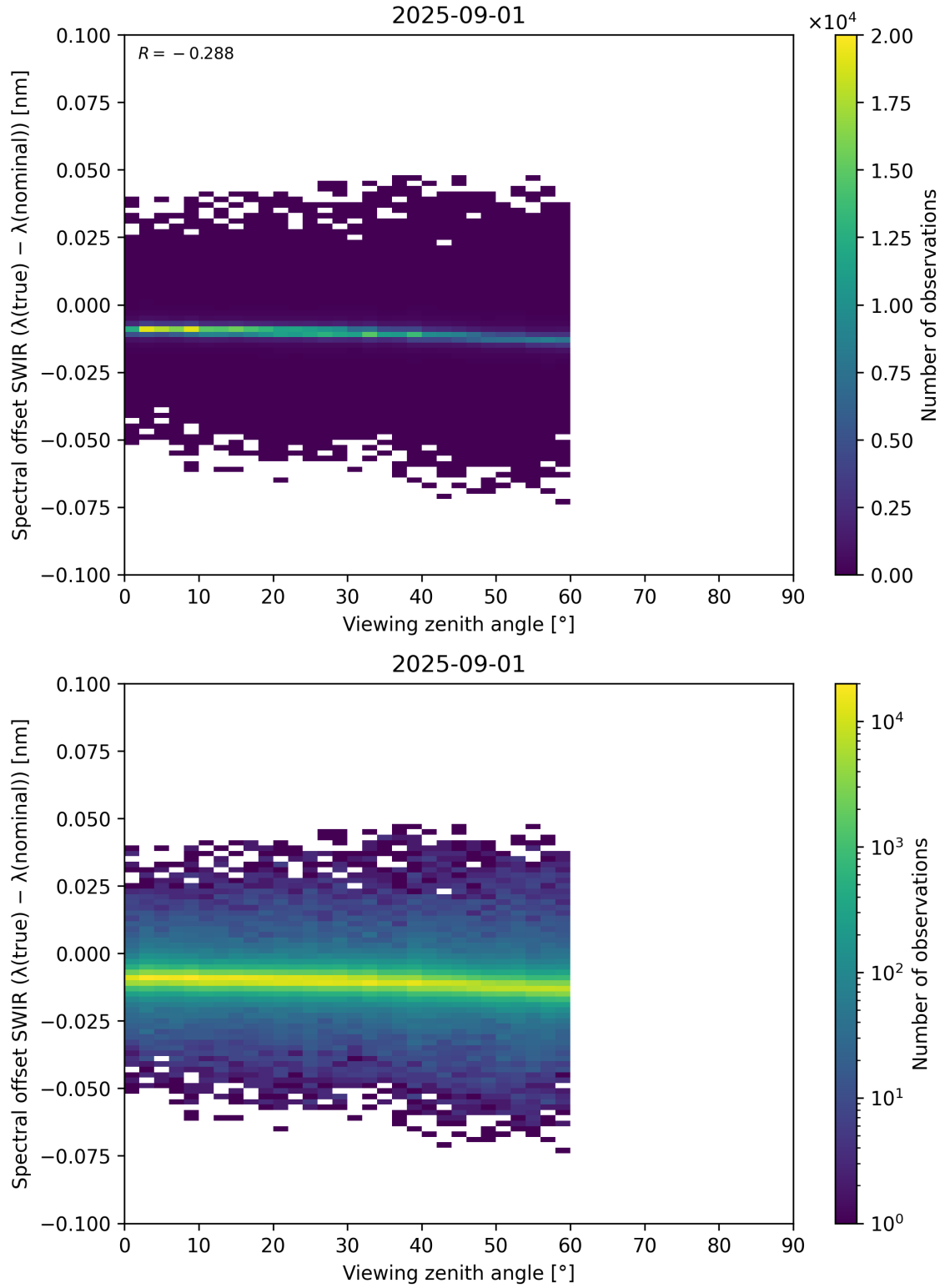
Figure 116: Scatter density plot of “Viewing zenith angle” against “Spectral offset SWIR ( \lambda_{\text{true}} - \lambda_{\text{nominal}} )” for 2025-08-31 to 2025-09-02.
