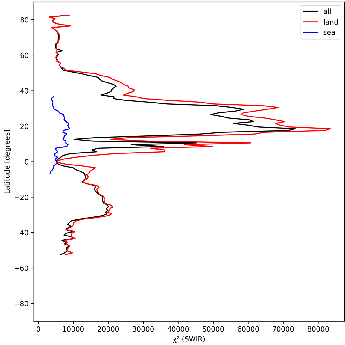
Figure 17: Zonal average of “ \chi^2 (SWIR)” for 2025-08-31 to 2025-09-02.
