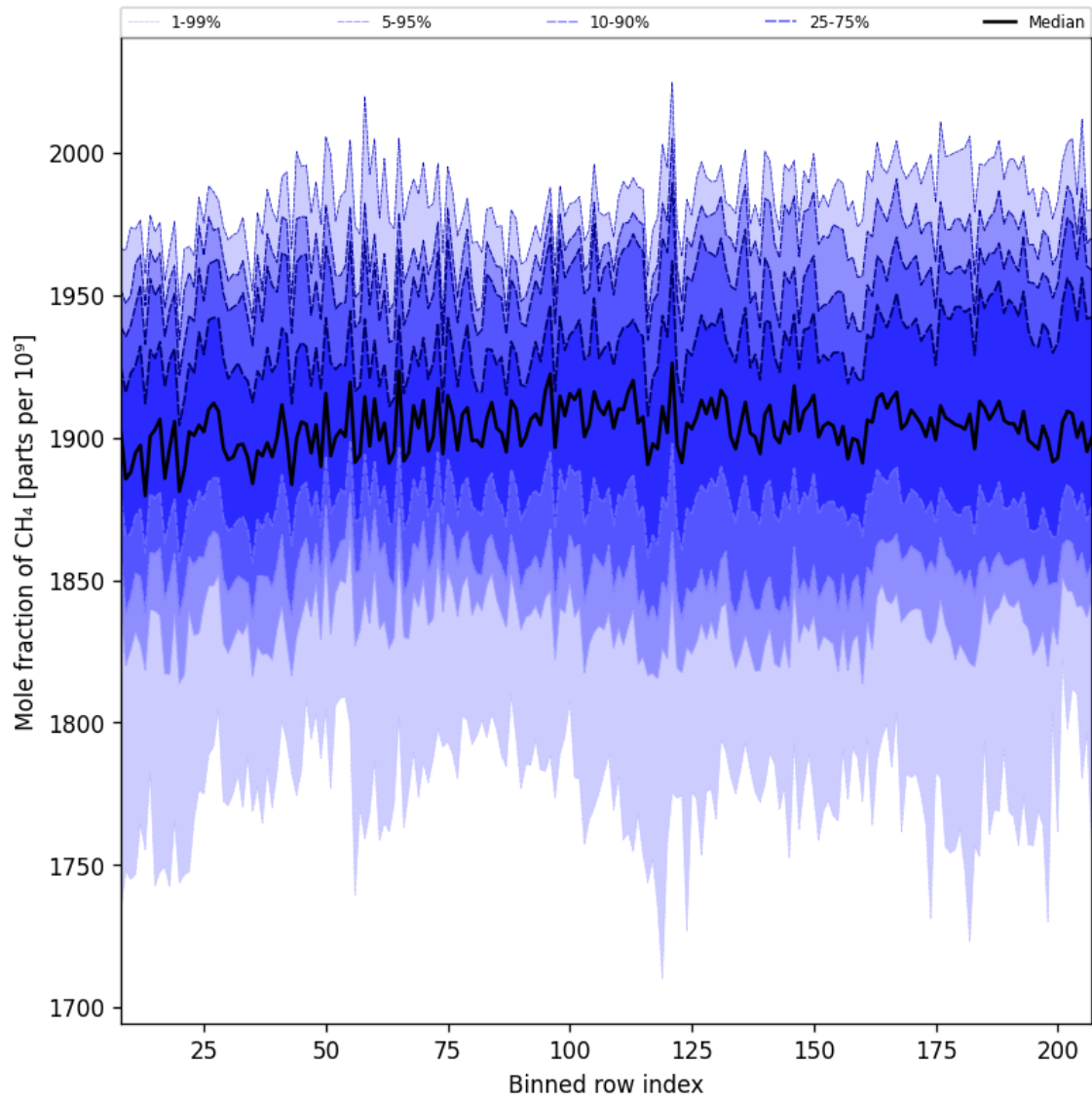
Figure 34: Along track statistics of “Mole fraction of CH 4 ” for 2025-08-31 to 2025-09-02
