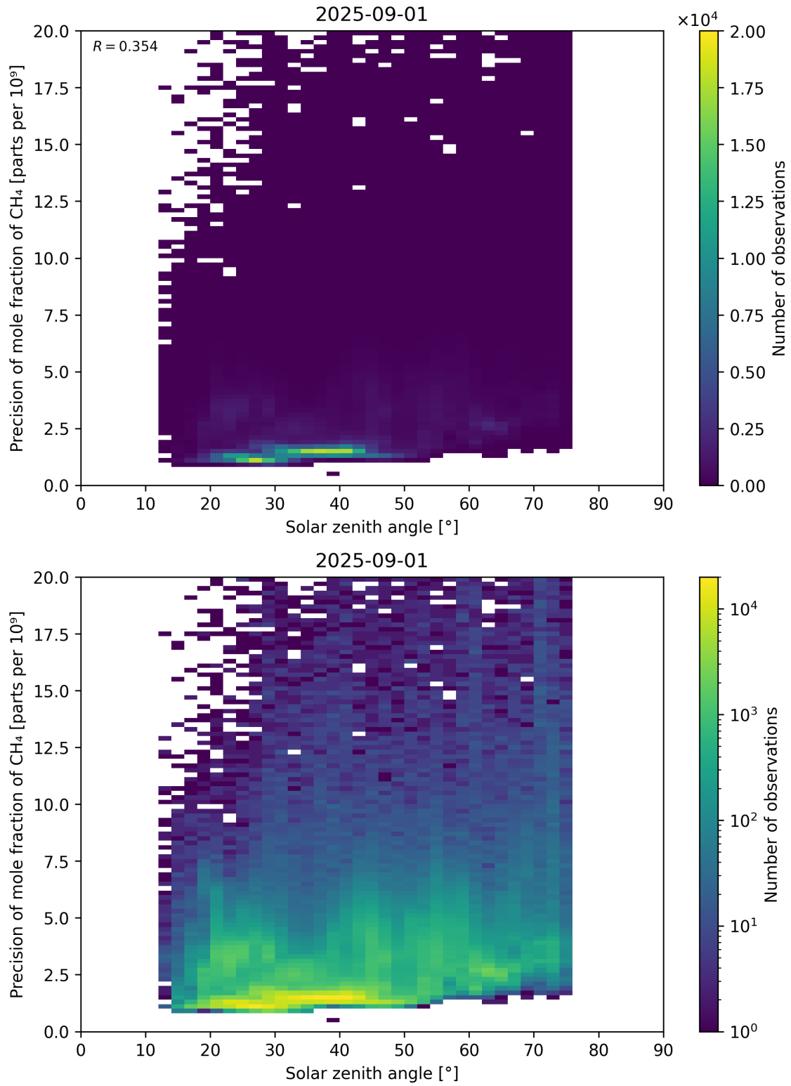
Figure 101: Scatter density plot of “Solar zenith angle” against “Precision of mole fraction of \text{CH}_4 ” for 2025-08-31 to 2025-09-02.
