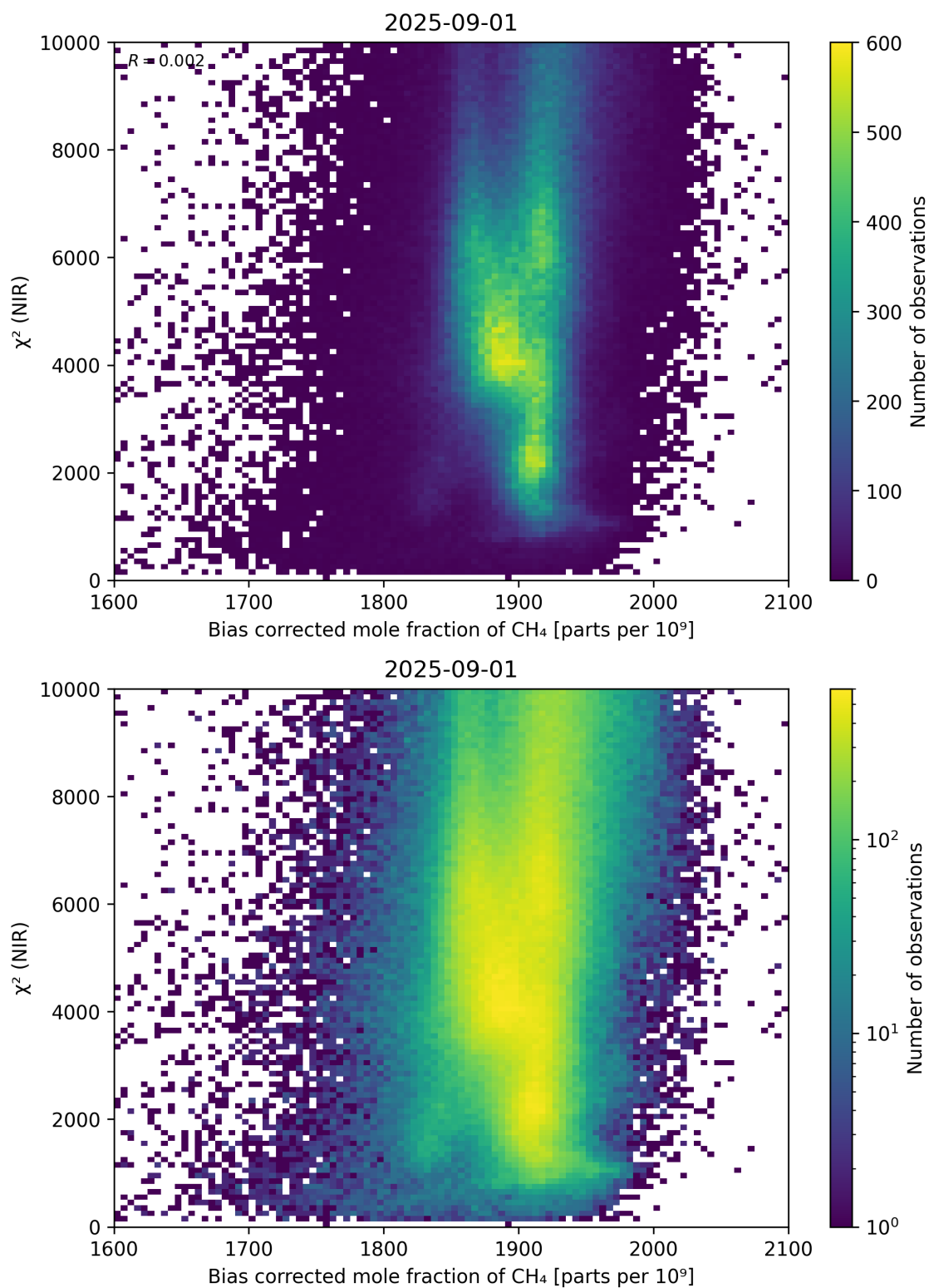
Figure 63: Scatter density plot of “Bias corrected mole fraction of \text{CH}_4 ” against “ \chi^2 (NIR)” for 2025-08-31 to 2025-09-02.
