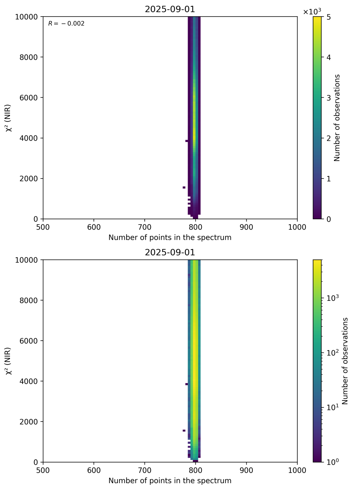
Figure 88: Scatter density plot of “Number of points in the spectrum” against “ \chi^2 (NIR)” for 2025-08-31 to 2025-09-02.
