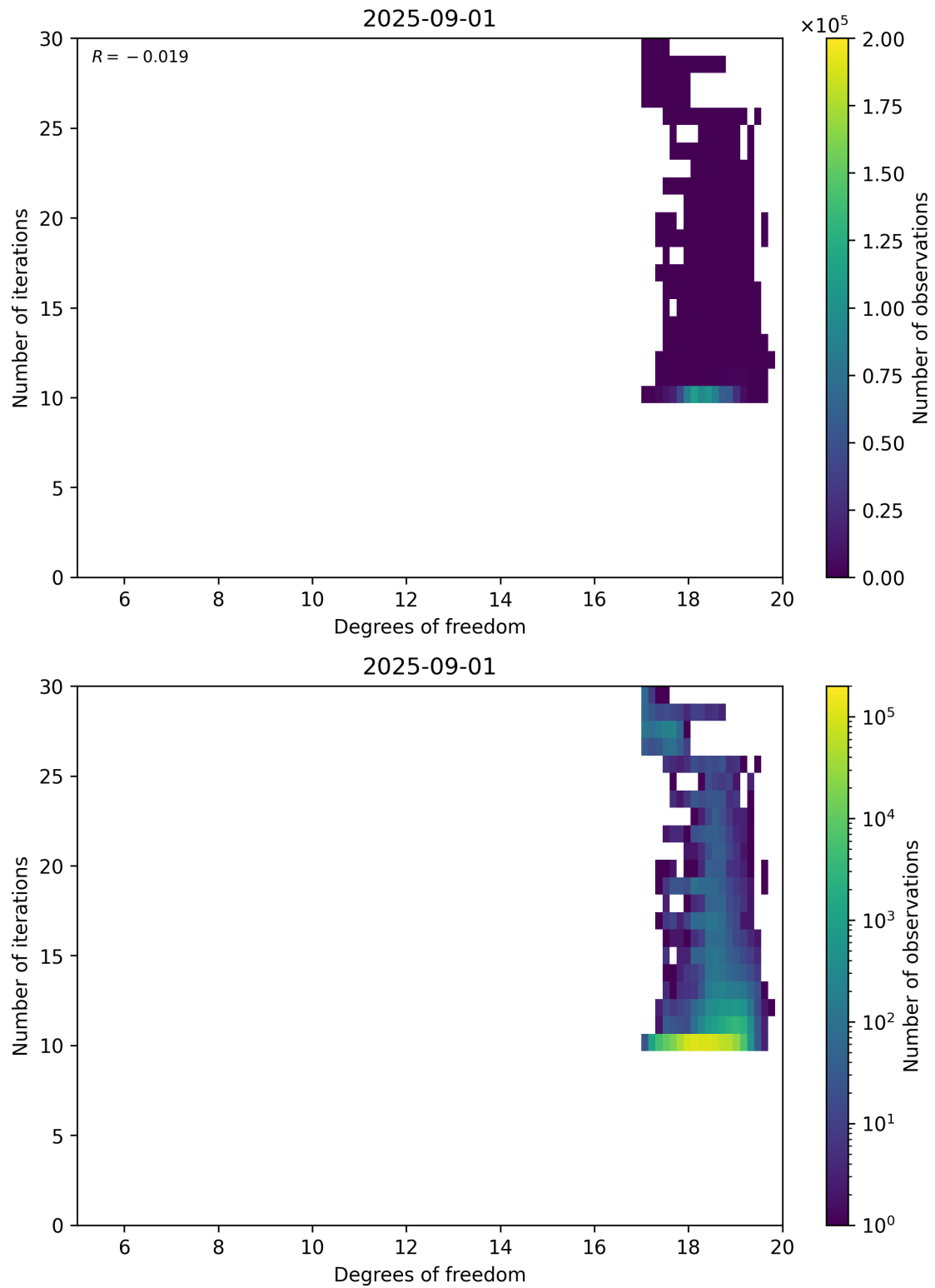
Figure 52: Scatter density plot of “Degrees of freedom” against “Number of iterations” for 2025-08-31 to 2025-09-02.
