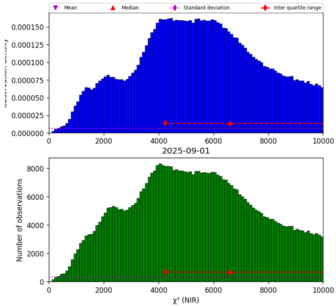
Figure 29: Histogram of “ \chi^2 (NIR)” for 2025-08-31 to 2025-09-02
