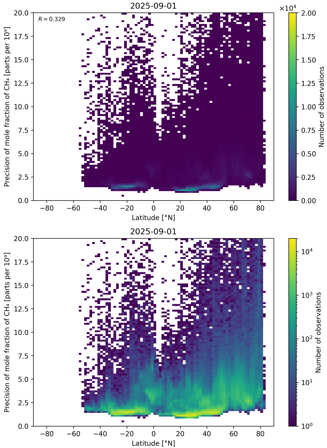
Figure 59: Scatter density plot of “Latitude” against “Precision of mole fraction of \text{CH}_4 ” for 2025-08-31 to 2025-09-02.
