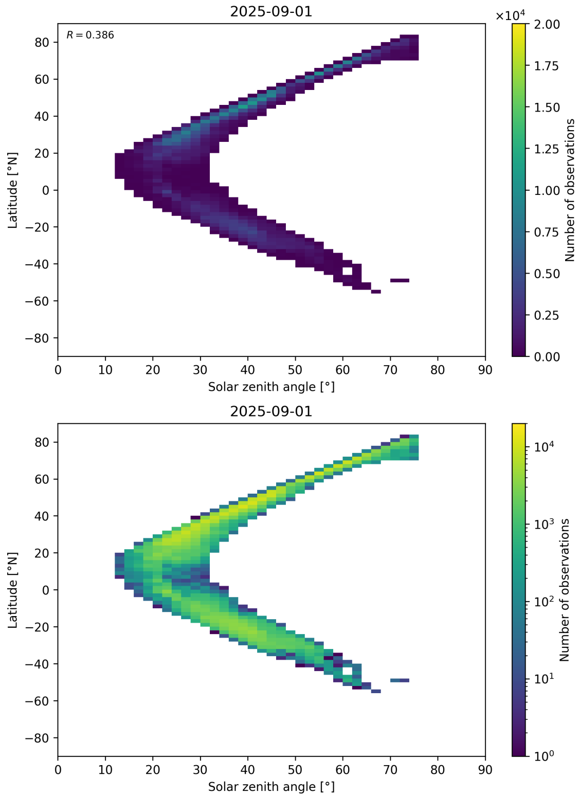
Figure 98: Scatter density plot of “Solar zenith angle” against “Latitude” for 2025-08-31 to 2025-09-02.
