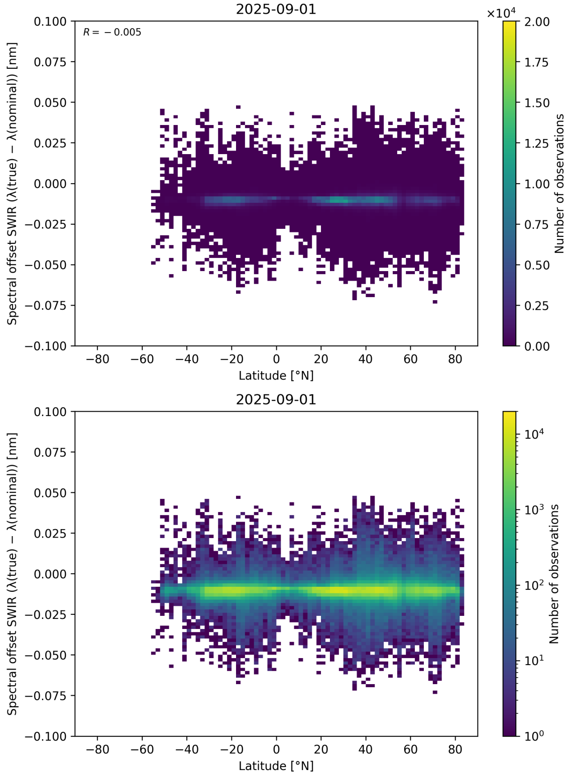
Figure 62: Scatter density plot of “Latitude” against “Spectral offset SWIR ( \lambda_{\text{true}} - \lambda_{\text{nominal}} )” for 2025-08-31 to 2025-09-02.
