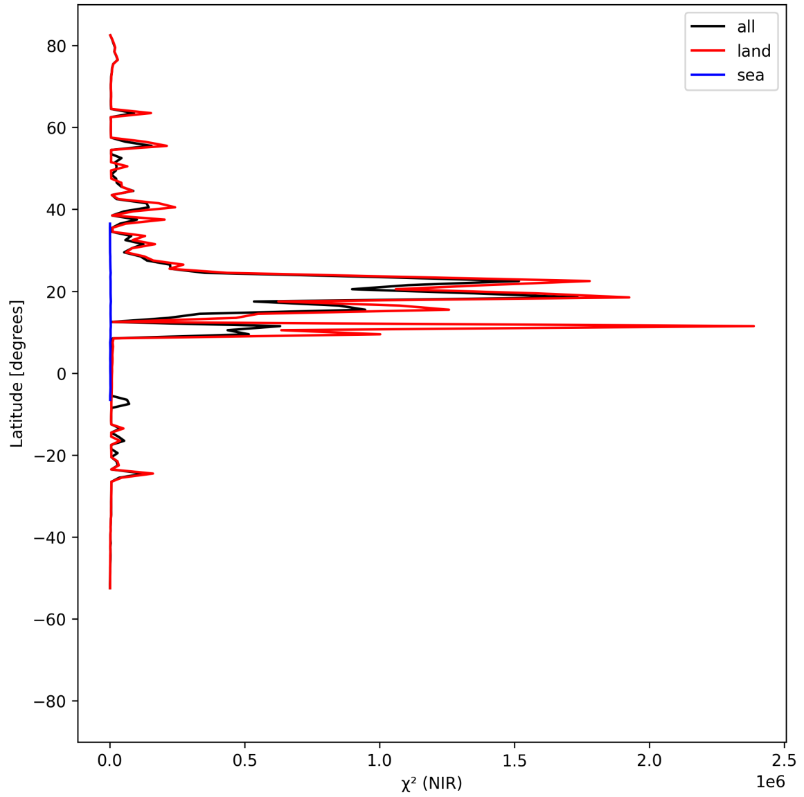
Figure 18: Zonal average of “ \chi^2 (NIR)” for 2025-08-31 to 2025-09-02.
