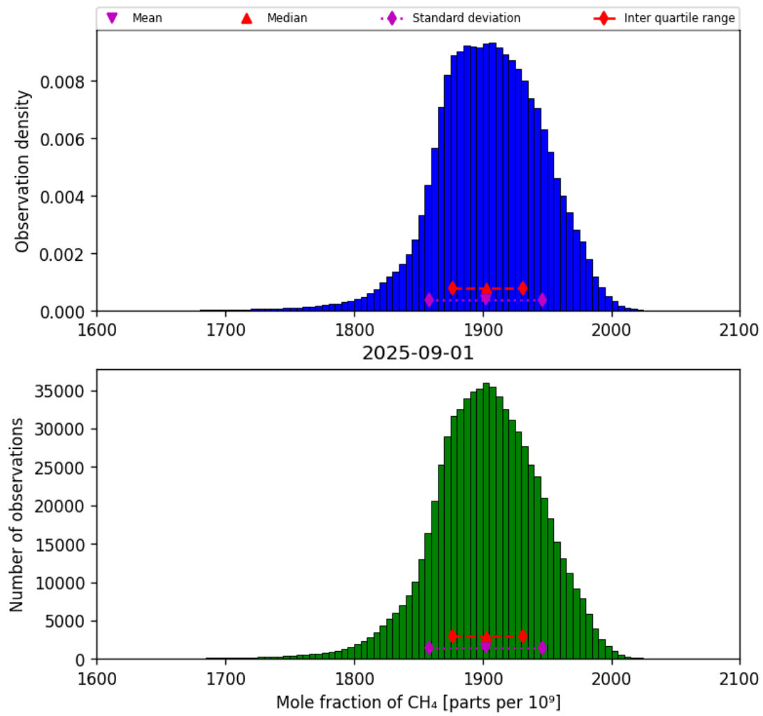
Figure 23: Histogram of “Mole fraction of CH 4 ” for 2025-08-31 to 2025-09-02
