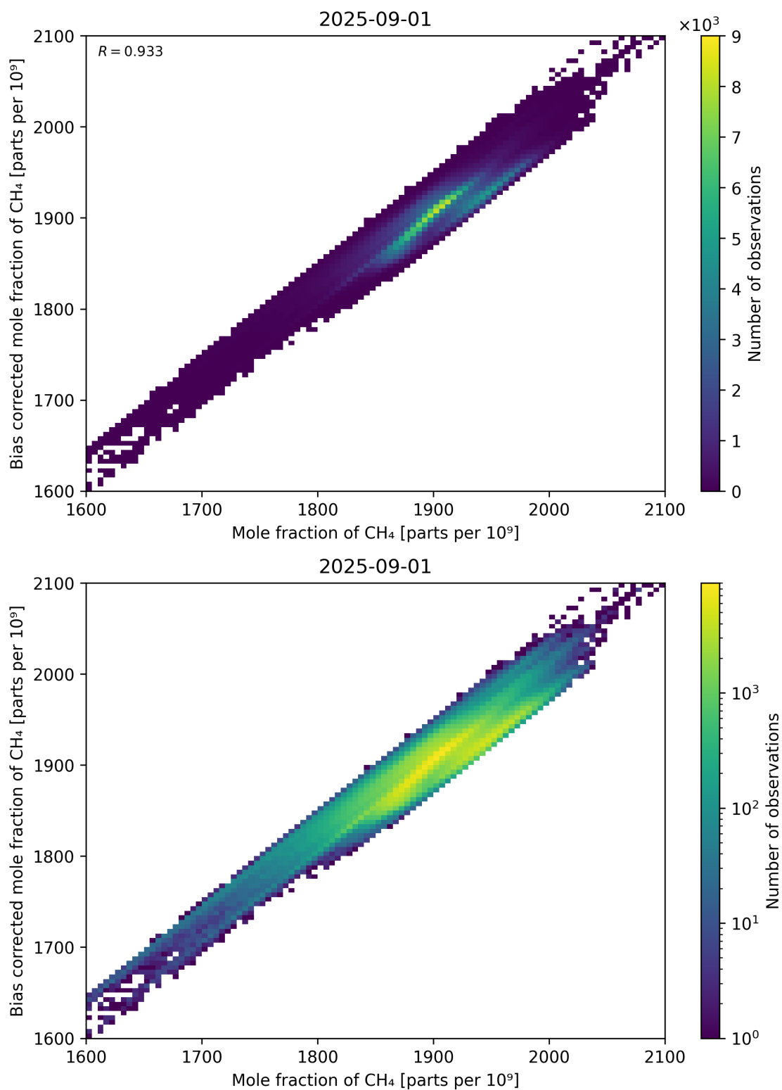
Figure 74: Scatter density plot of “Mole fraction of CH 4 ” against “Bias corrected mole fraction of CH 4 ” for 2025-08-31 to 2025-09-02.
