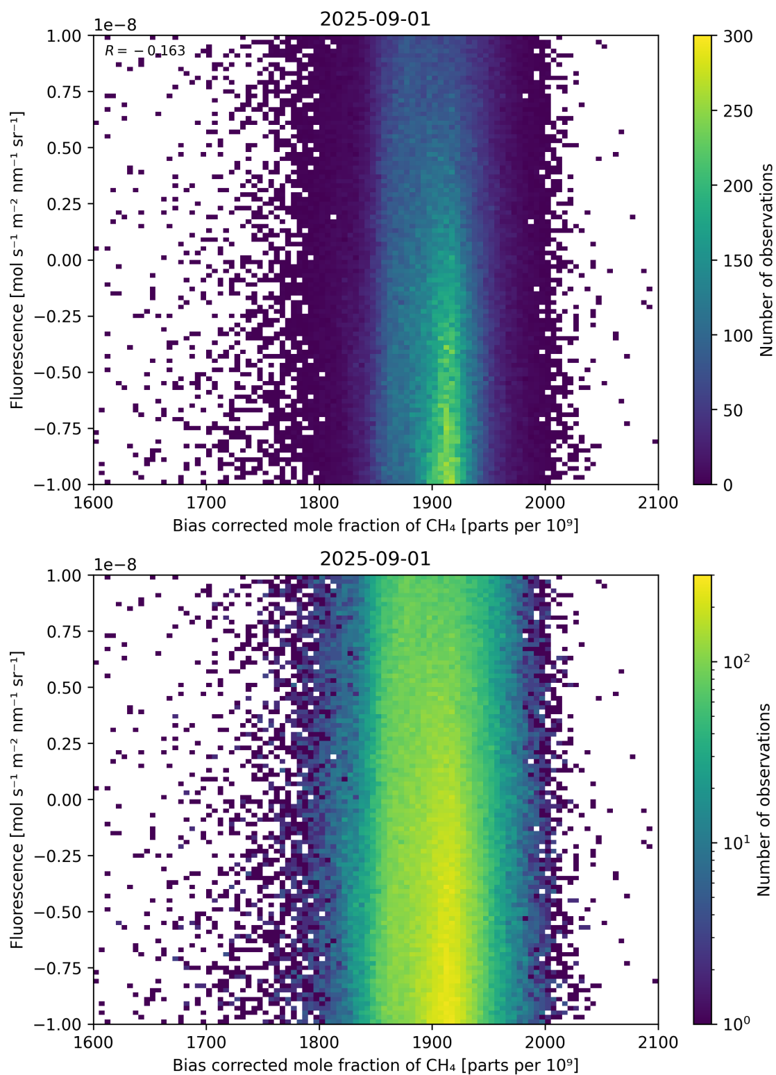
Figure 66: Scatter density plot of “Bias corrected mole fraction of CH 4 ” against “Fluorescence” for 2025-08-31 to 2025-09-02.
