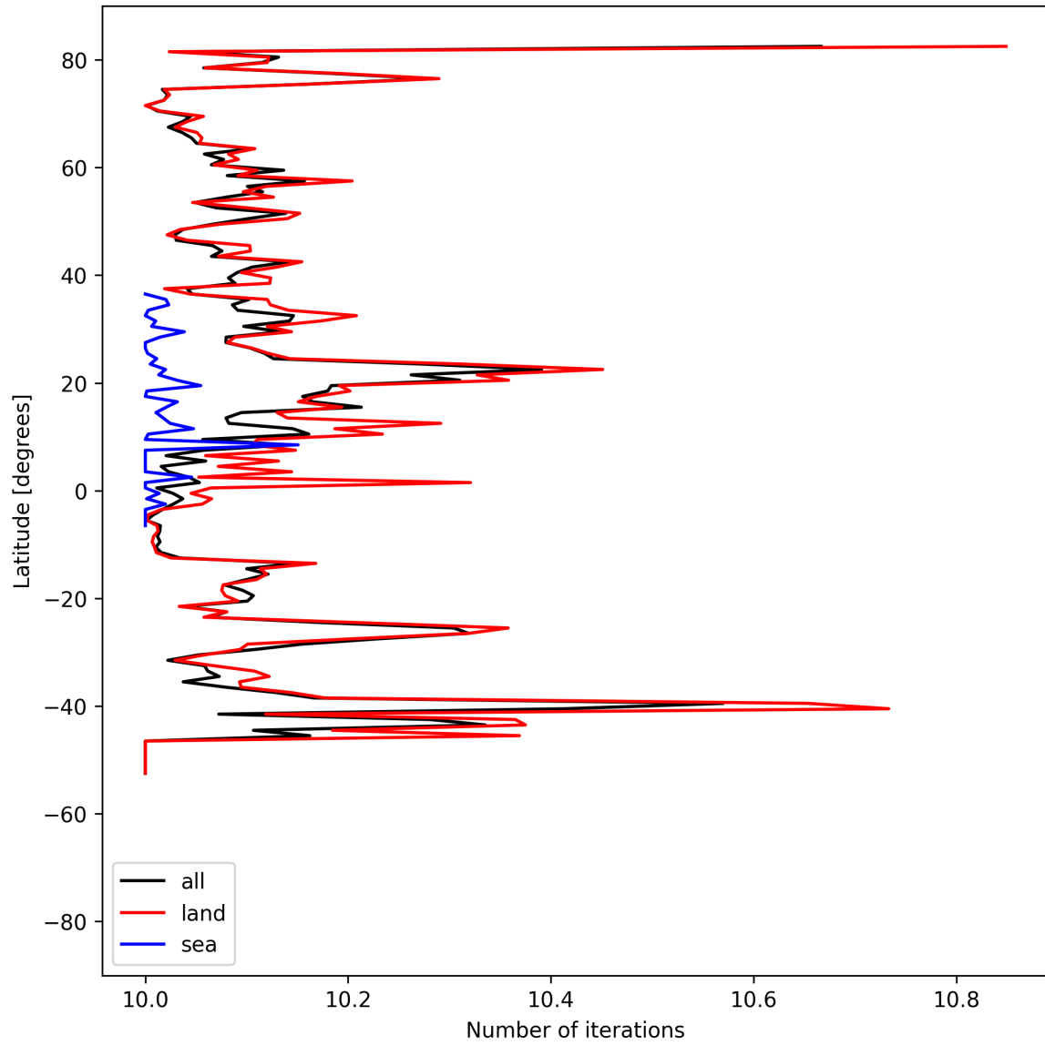
Figure 20: Zonal average of “Number of iterations” for 2025-08-31 to 2025-09-02.
