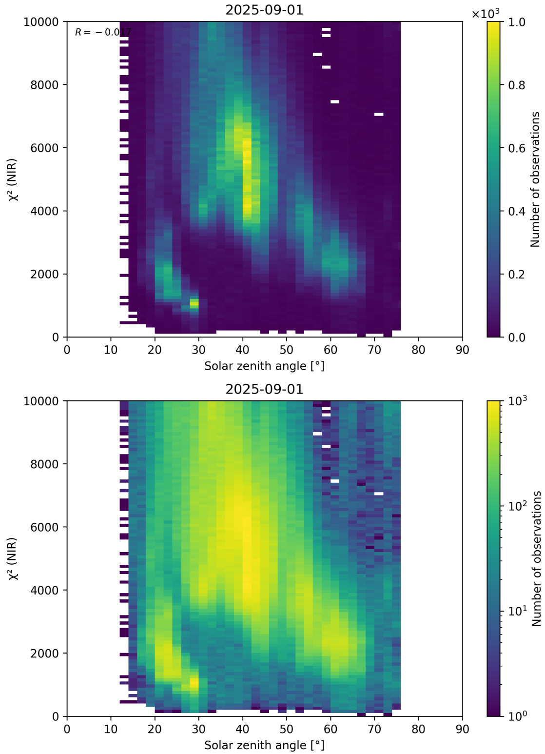
Figure 94: Scatter density plot of “Solar zenith angle” against “ \chi^2 (NIR)” for 2025-08-31 to 2025-09-02.
