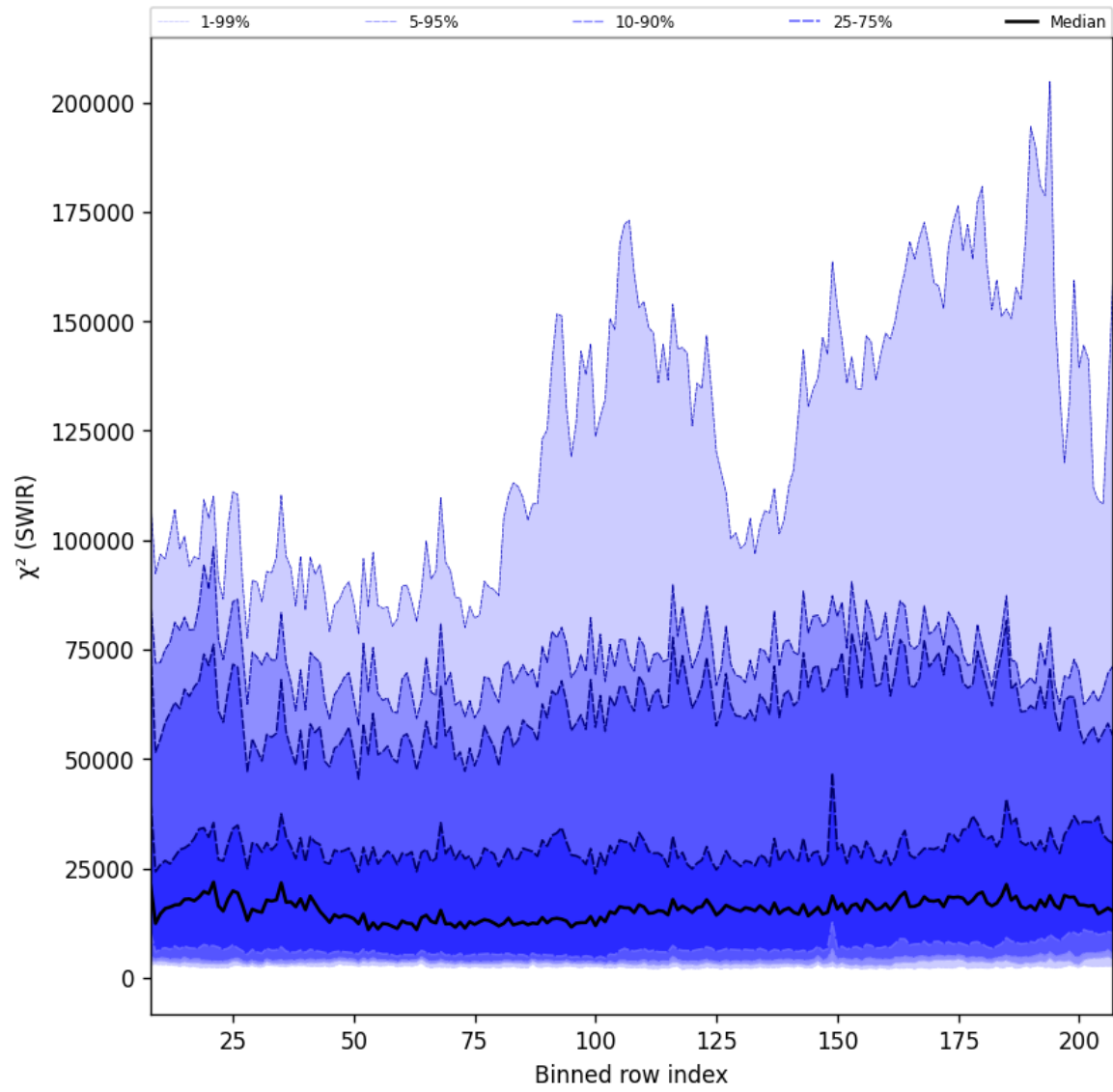
Figure 39: Along track statistics of “ \chi^2 (SWIR)” for 2025-08-31 to 2025-09-02
