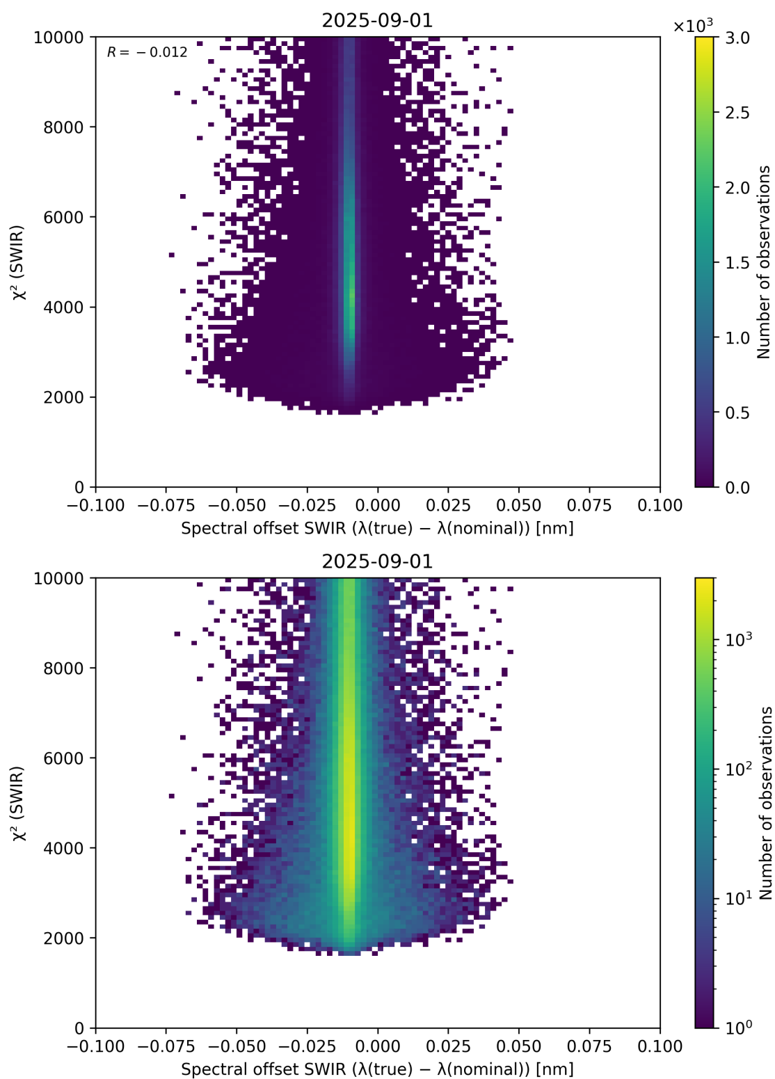
Figure 118: Scatter density plot of “Spectral offset SWIR ( \lambda_{\text{true}} - \lambda_{\text{nominal}} )” against “ \chi^2 (SWIR)” for 2025-08-31 to 2025-09-02.
