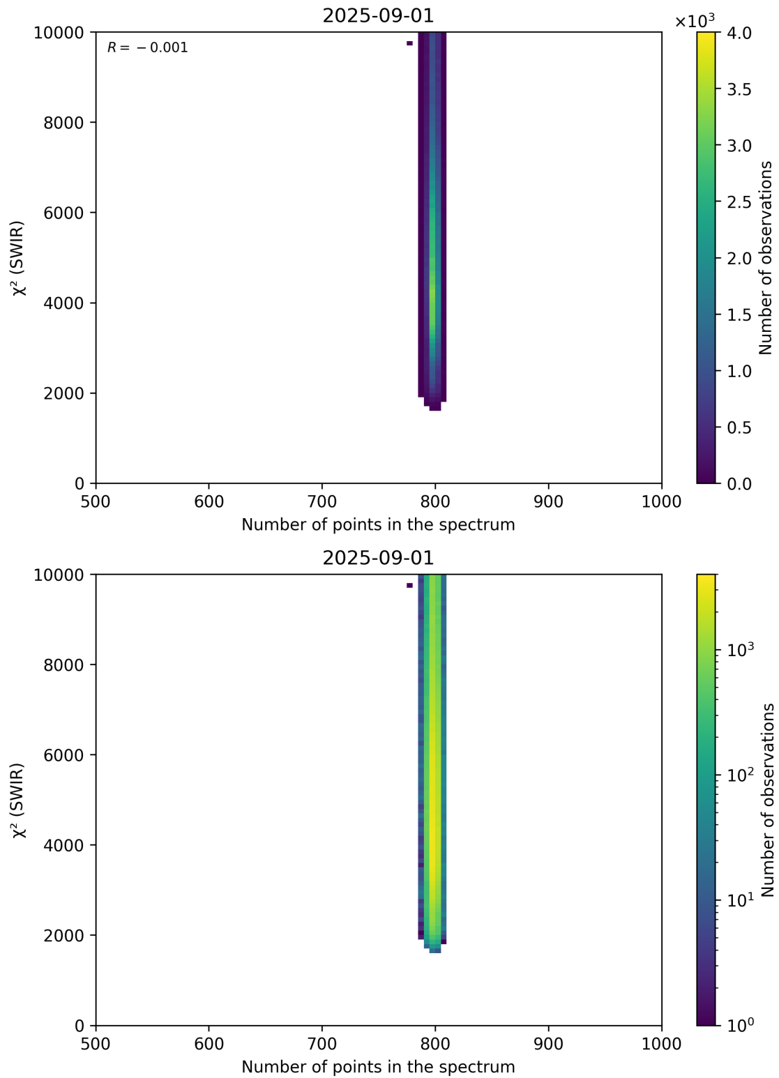
Figure 89: Scatter density plot of “Number of points in the spectrum” against “ \chi^2 (SWIR)” for 2025-08-31 to 2025-09-02.
