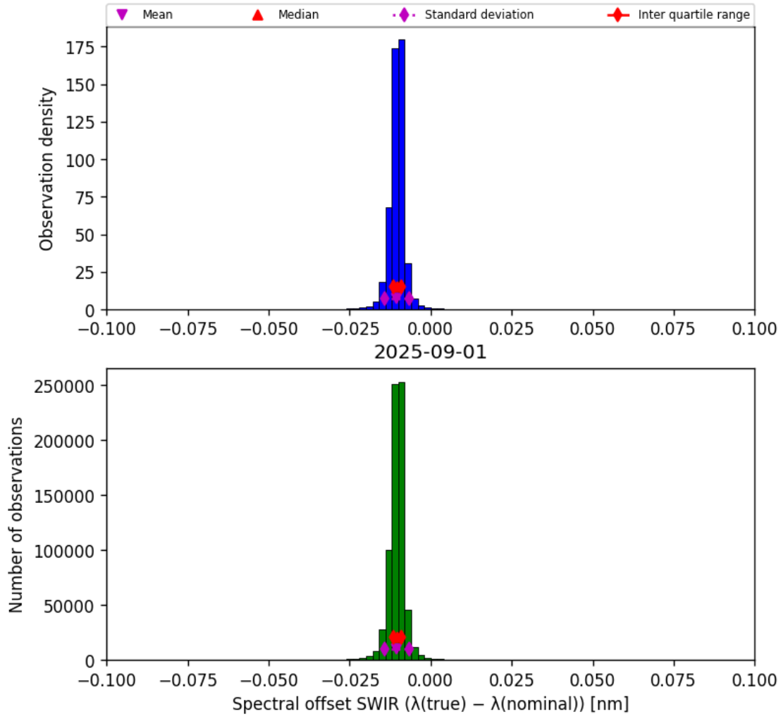
Figure 27: Histogram of “Spectral offset SWIR ( \lambda_{\text{true}} - \lambda_{\text{nominal}} )” for 2025-08-31 to 2025-09-02
