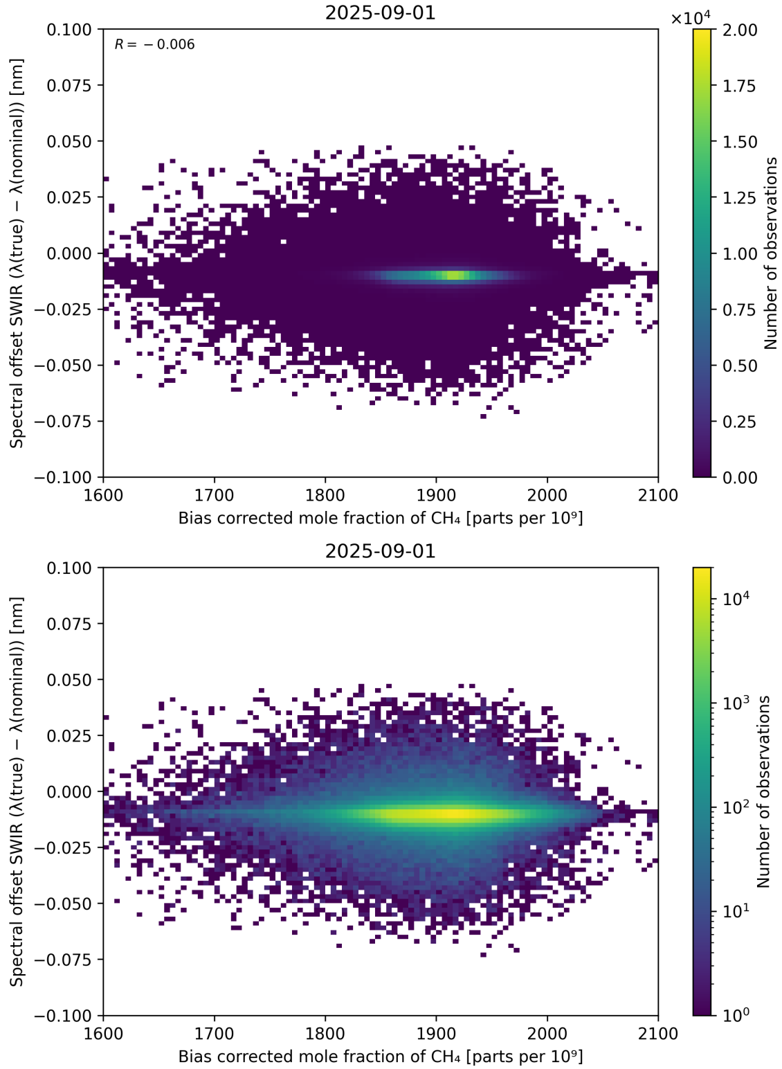
Figure 69: Scatter density plot of “Bias corrected mole fraction of \text{CH}_4 ” against “Spectral offset SWIR ( \lambda_{\text{true}} - \lambda_{\text{nominal}} )” for 2025-08-31 to 2025-09-02.
