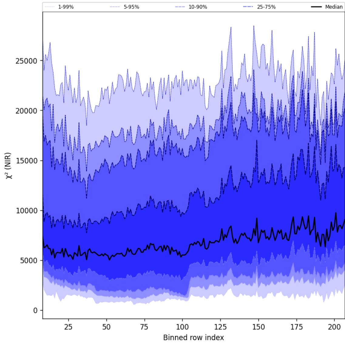
Figure 40: Along track statistics of “ \chi^2 (NIR)” for 2025-08-31 to 2025-09-02
