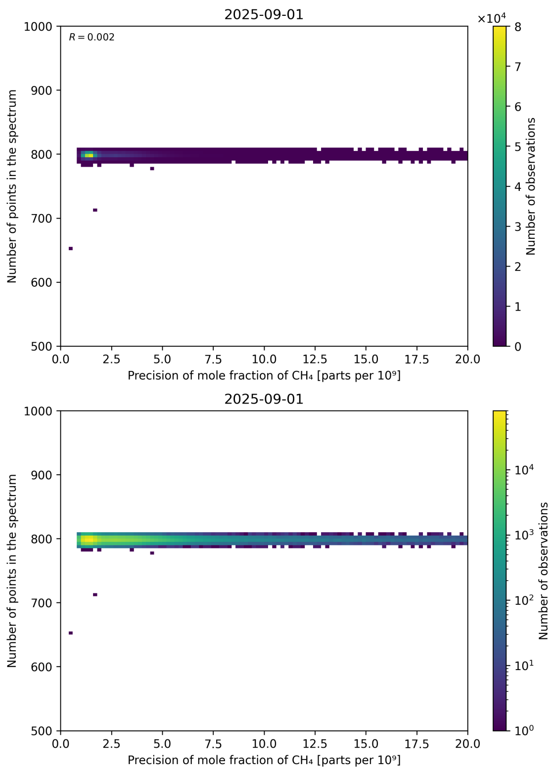
Figure 84: Scatter density plot of “Precision of mole fraction of CH 4 ” against “Number of points in the spectrum” for 2025-08-31 to 2025-09-02.
