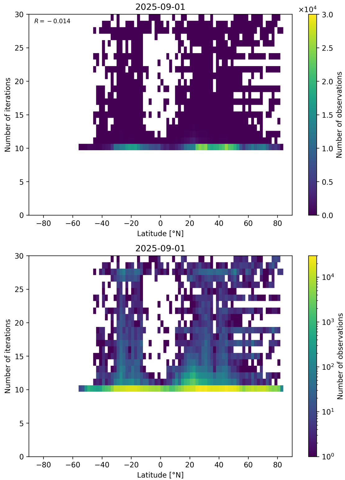
Figure 60: Scatter density plot of “Latitude” against “Number of iterations” for 2025-08-31 to 2025-09-02.
