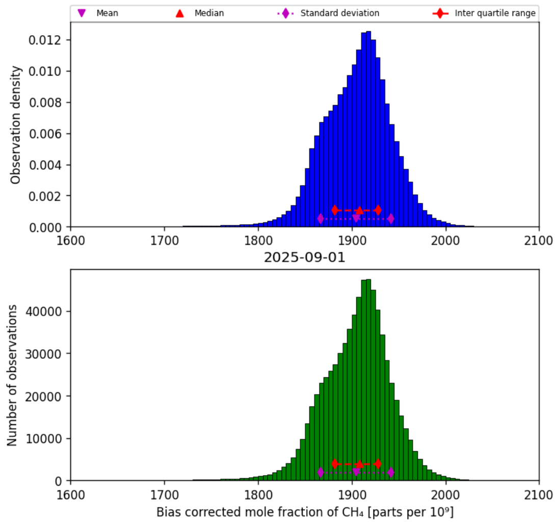
Figure 25: Histogram of “Bias corrected mole fraction of CH 4 ” for 2025-08-31 to 2025-09-02
