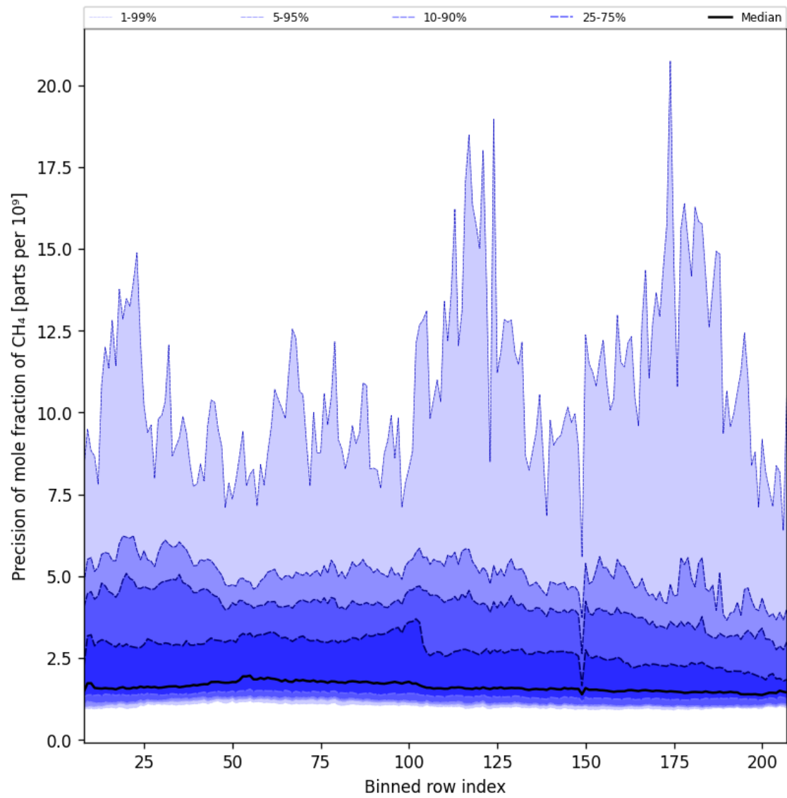
Figure 35: Along track statistics of “Precision of mole fraction of CH 4 ” for 2025-08-31 to 2025-09-02
