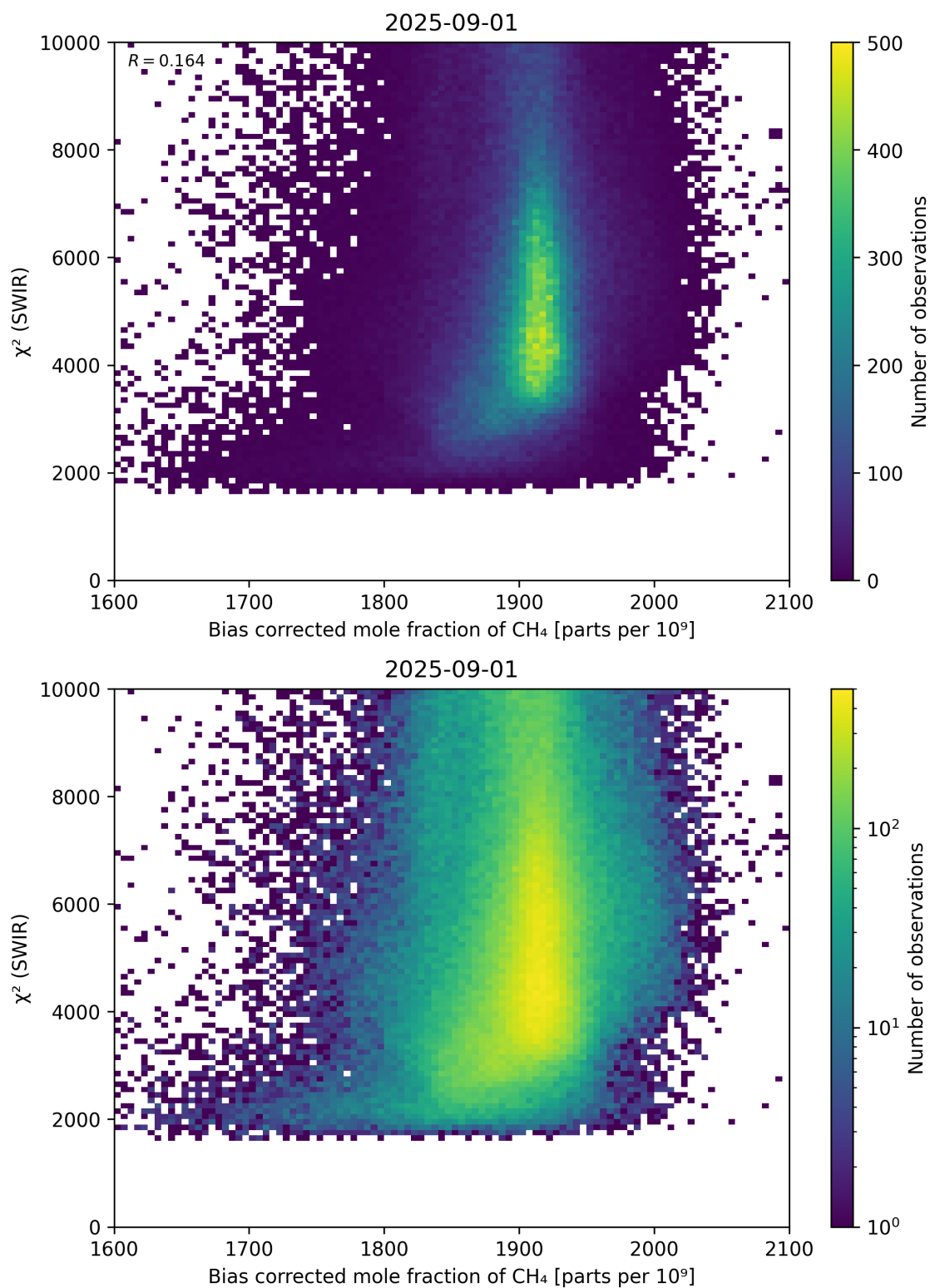
Figure 64: Scatter density plot of “Bias corrected mole fraction of \text{CH}_4 ” against “ \chi^2 (SWIR)” for 2025-08-31 to 2025-09-02.
