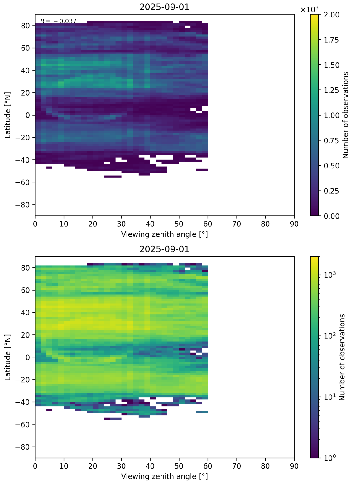
Figure 109: Scatter density plot of “Viewing zenith angle” against “Latitude” for 2025-08-31 to 2025-09-02.
