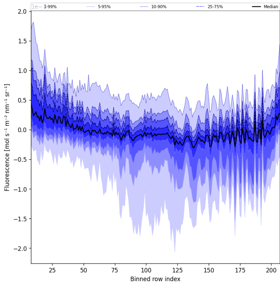
Figure 43: Along track statistics of “Fluorescence” for 2025-08-31 to 2025-09-02
