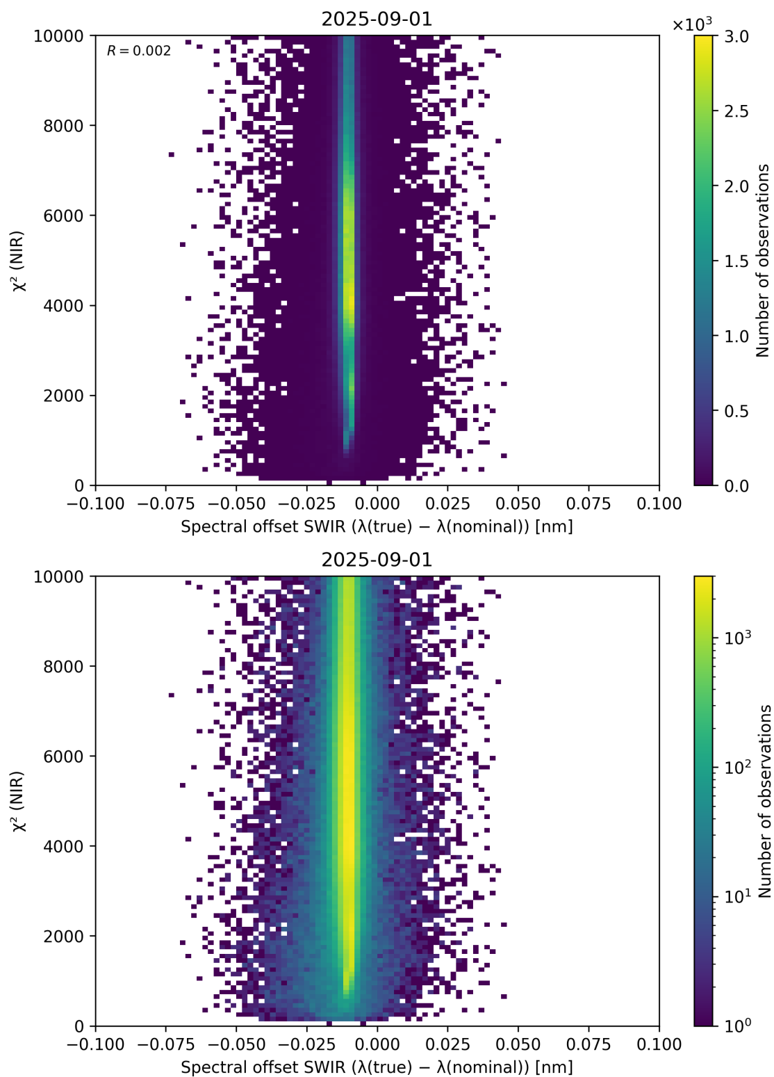
Figure 117: Scatter density plot of “Spectral offset SWIR ( \lambda_{\text{true}} - \lambda_{\text{nominal}} )” against “ \chi^2 (NIR)” for 2025-08-31 to 2025-09-02.
