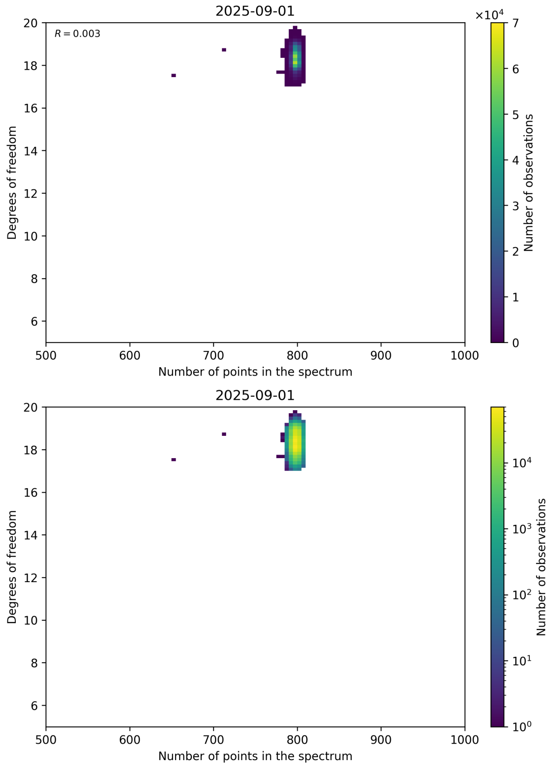
Figure 90: Scatter density plot of “Number of points in the spectrum” against “Degrees of freedom” for 2025-08-31 to 2025-09-02.
