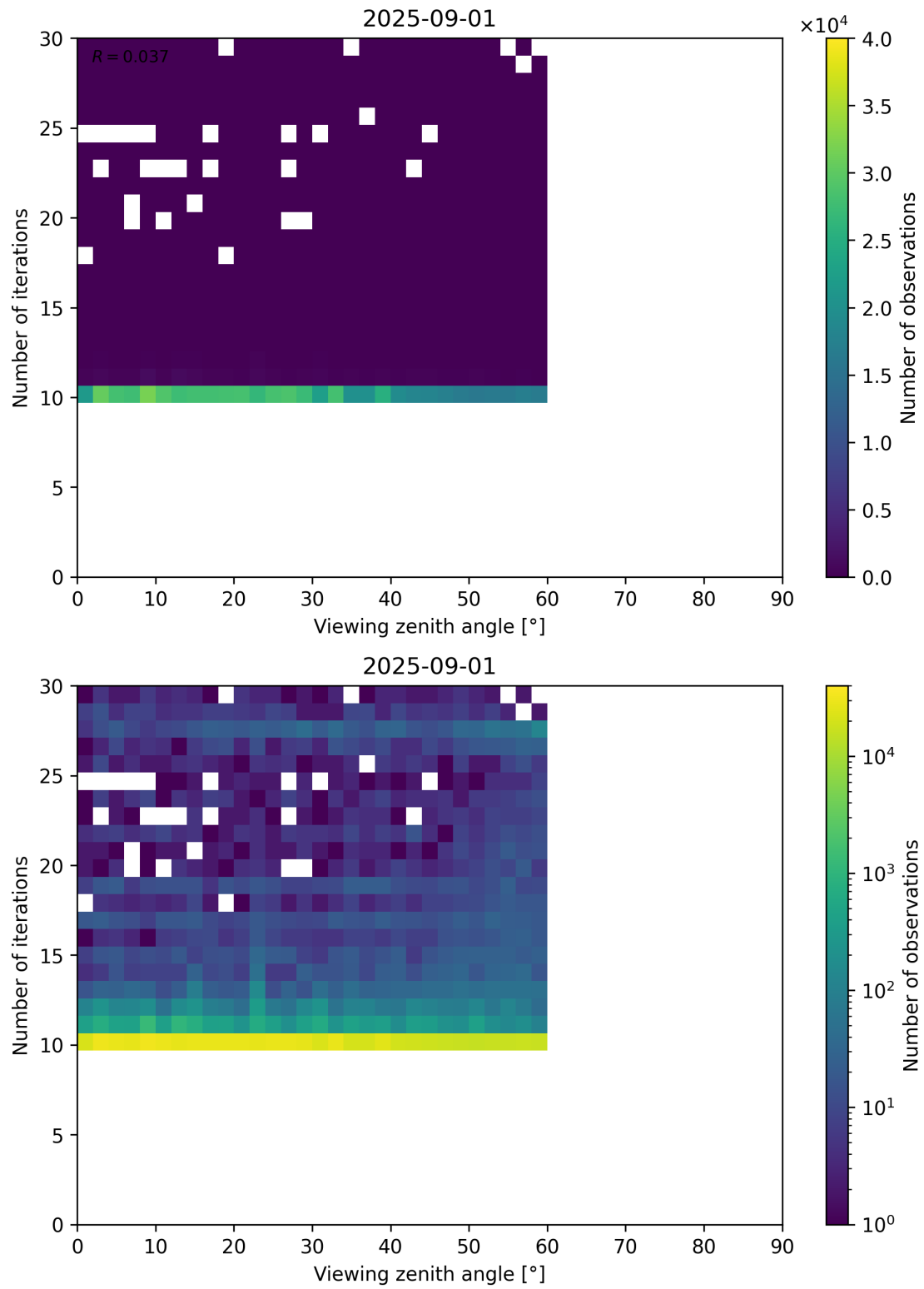
Figure 113: Scatter density plot of “Viewing zenith angle” against “Number of iterations” for 2025-08-31 to 2025-09-02.
