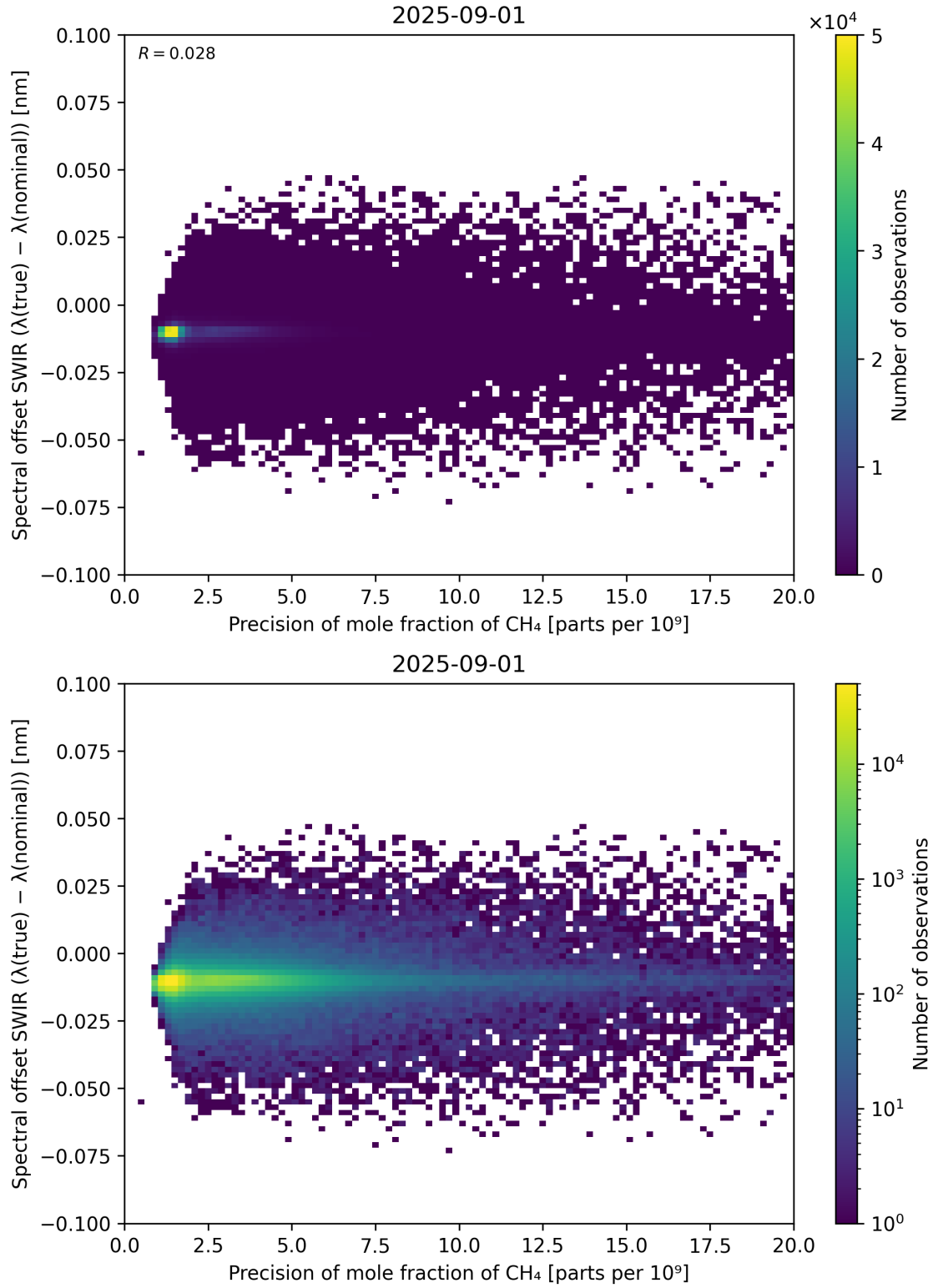
Figure 85: Scatter density plot of “Precision of mole fraction of \text{CH}_4 ” against “Spectral offset SWIR ( \lambda_{\text{true}} - \lambda_{\text{nominal}} )” for 2025-08-31 to 2025-09-02.
