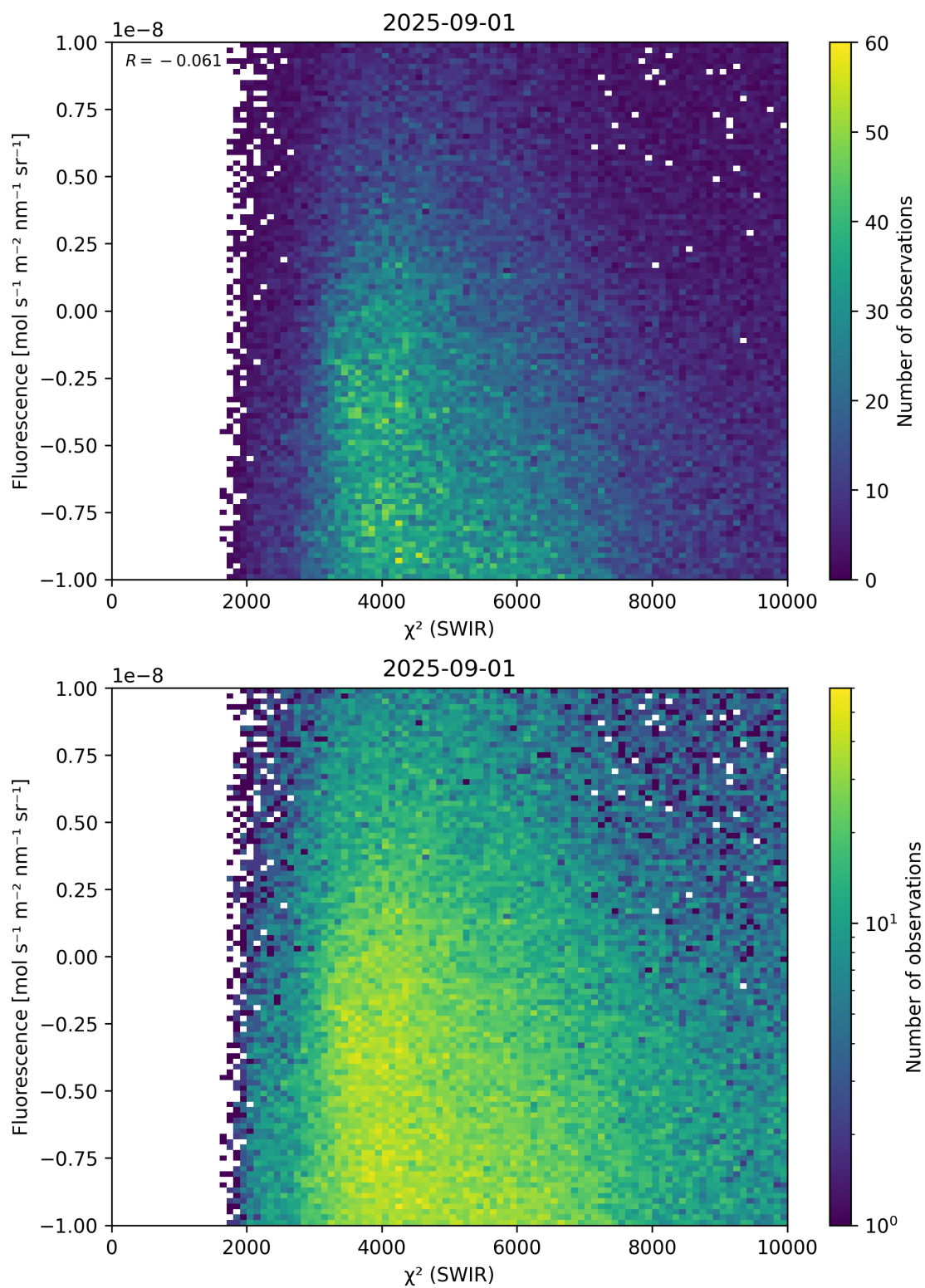
Figure 49: Scatter density plot of “ \chi^2 (SWIR)” against “Fluorescence” for 2025-08-31 to 2025-09-02.
