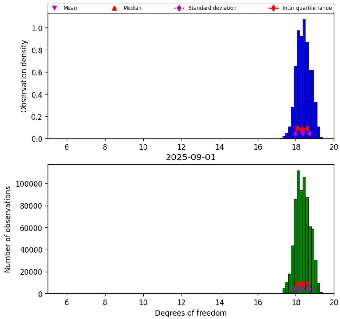
Figure 30: Histogram of “Degrees of freedom” for 2025-08-31 to 2025-09-02
