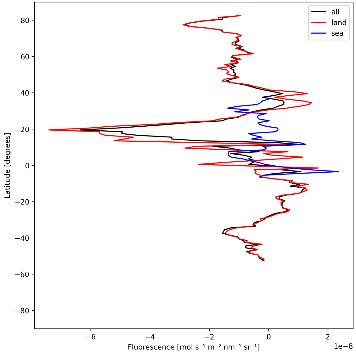
Figure 21: Zonal average of “Fluorescence” for 2025-08-31 to 2025-09-02.
