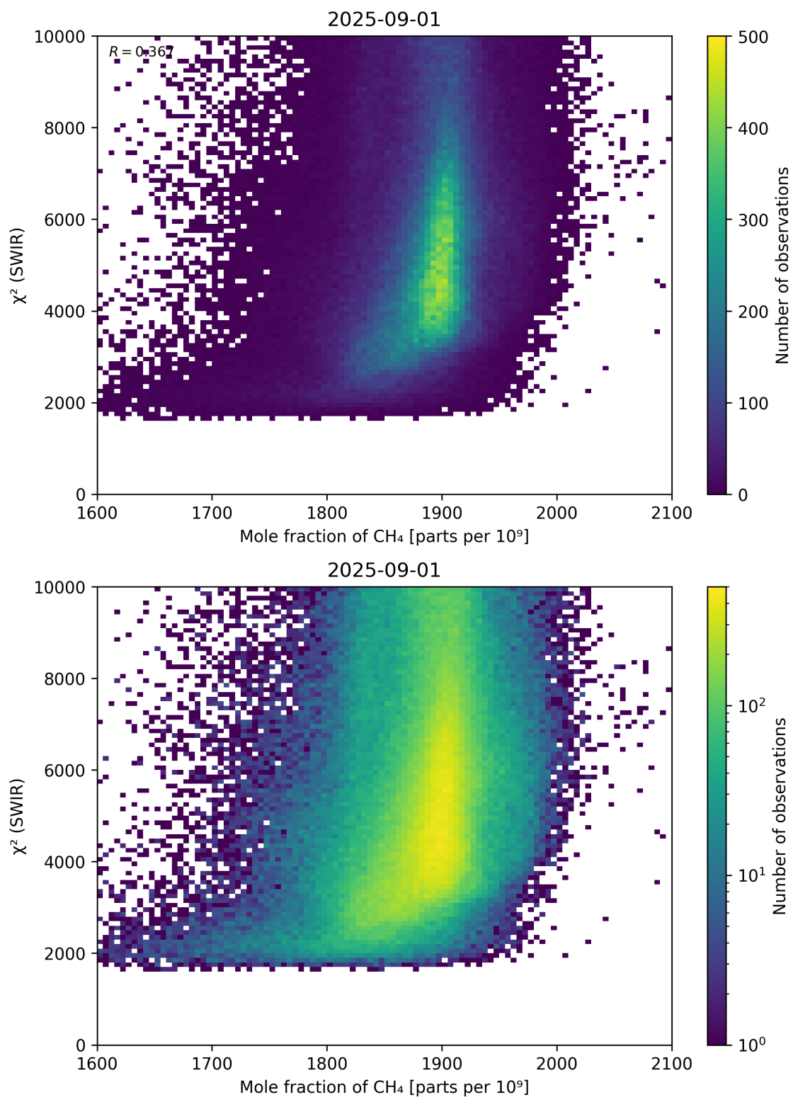
Figure 71: Scatter density plot of “Mole fraction of CH 4 ” against “ \chi^2 (SWIR)” for 2025-08-31 to 2025-09-02.
