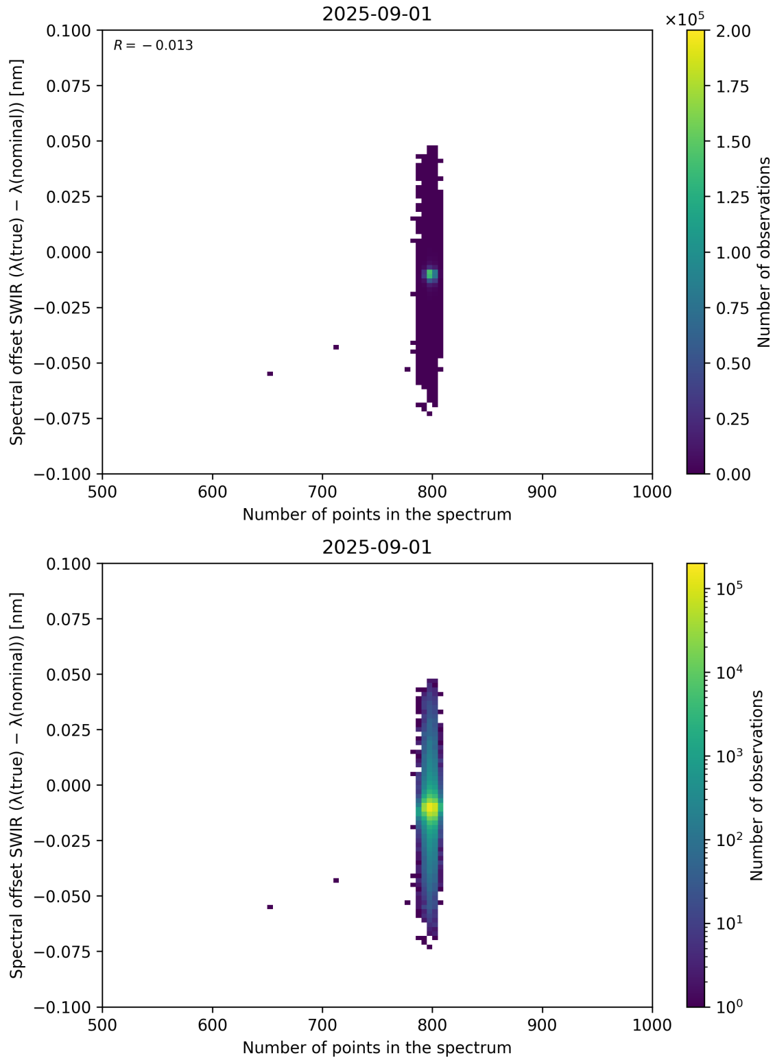
Figure 93: Scatter density plot of “Number of points in the spectrum” against “Spectral offset SWIR ( \lambda_{\text{true}} - \lambda_{\text{nominal}} )” for 2025-08-31 to 2025-09-02.
