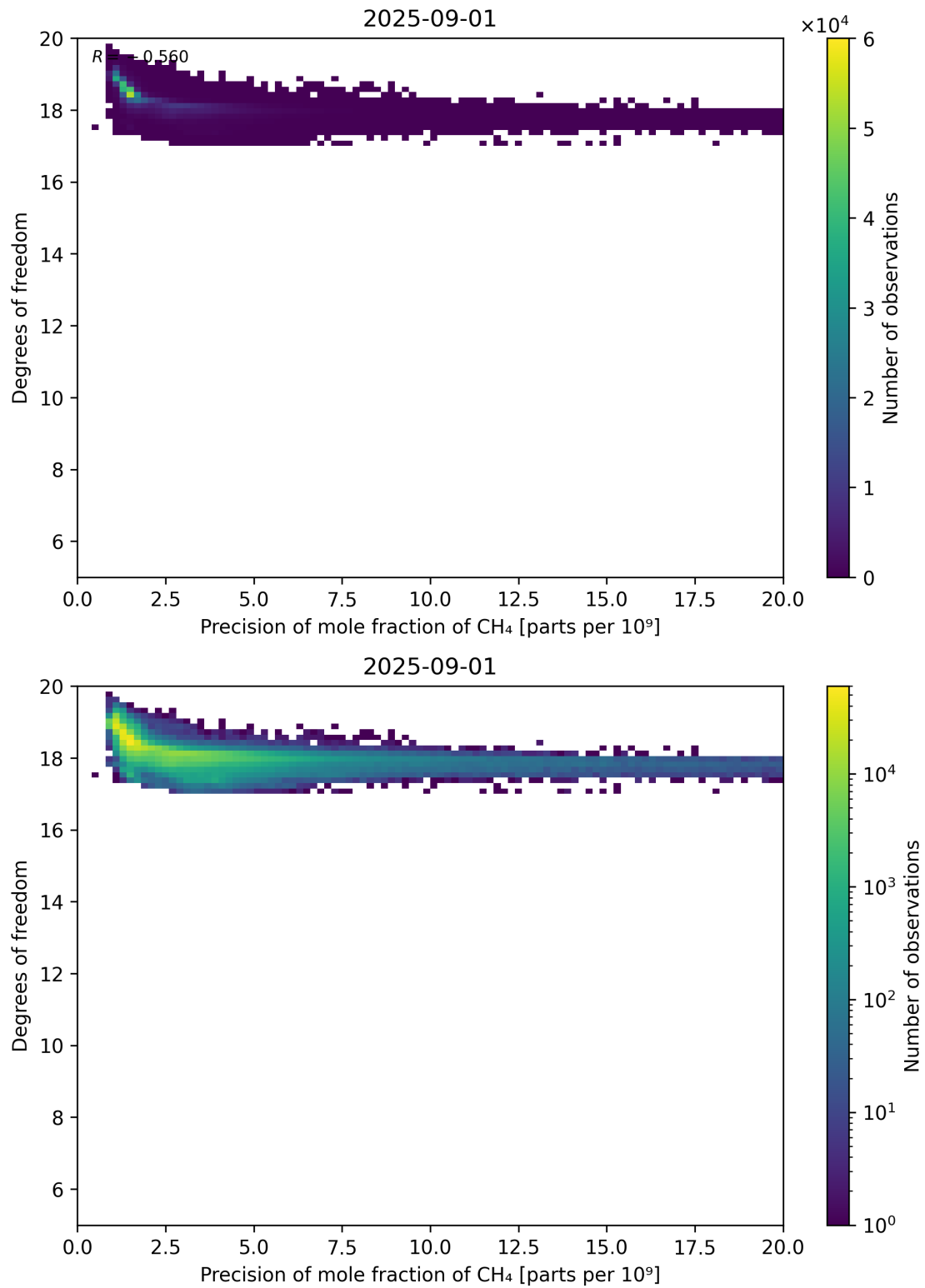
Figure 80: Scatter density plot of “Precision of mole fraction of CH 4 ” against “Degrees of freedom” for 2025-08-31 to 2025-09-02.
