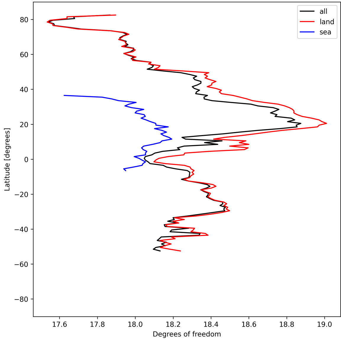
Figure 19: Zonal average of “Degrees of freedom” for 2025-08-31 to 2025-09-02.
