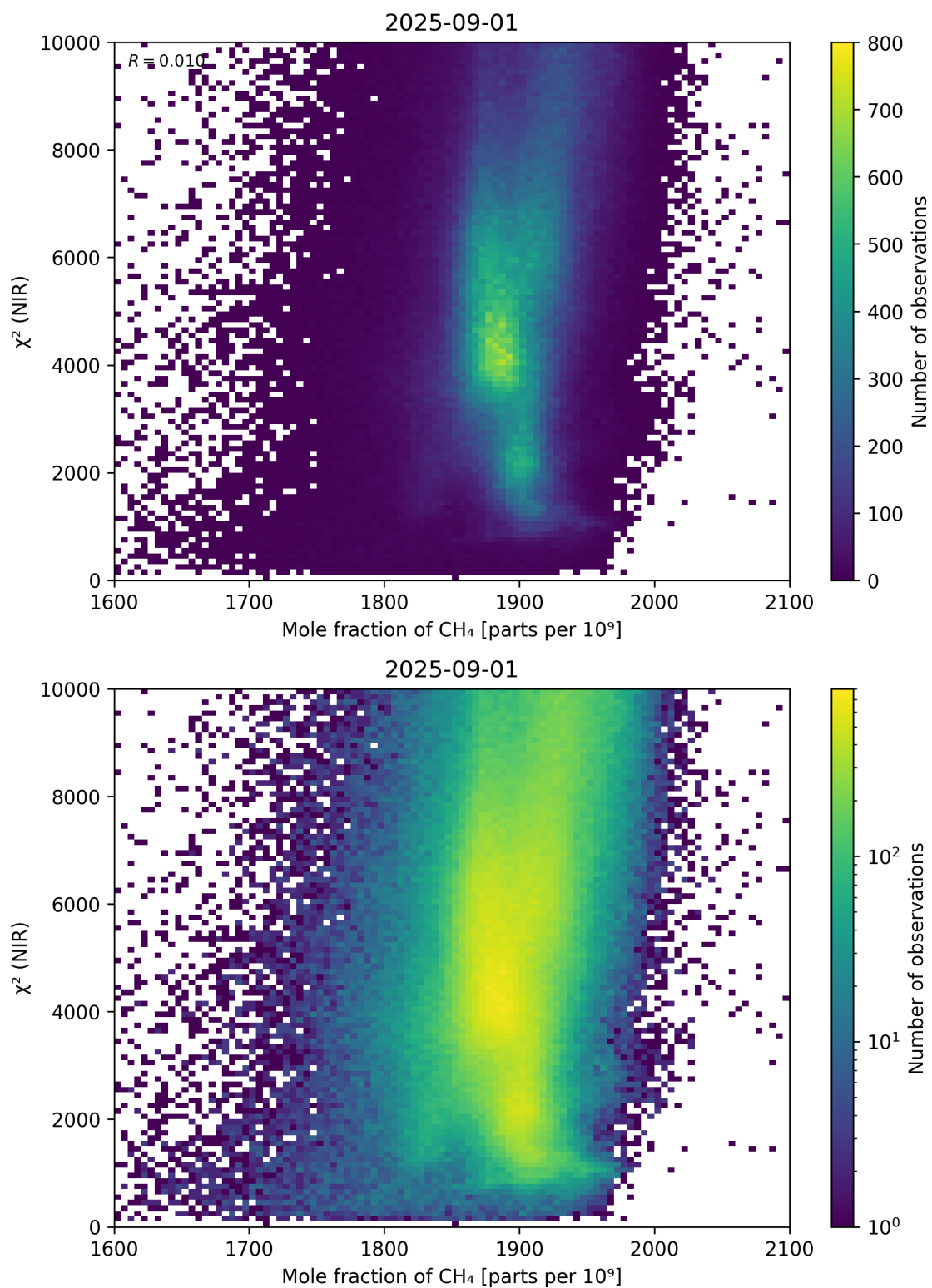
Figure 70: Scatter density plot of “Mole fraction of \text{CH}_4 ” against “ \chi^2 (NIR)” for 2025-08-31 to 2025-09-02.
