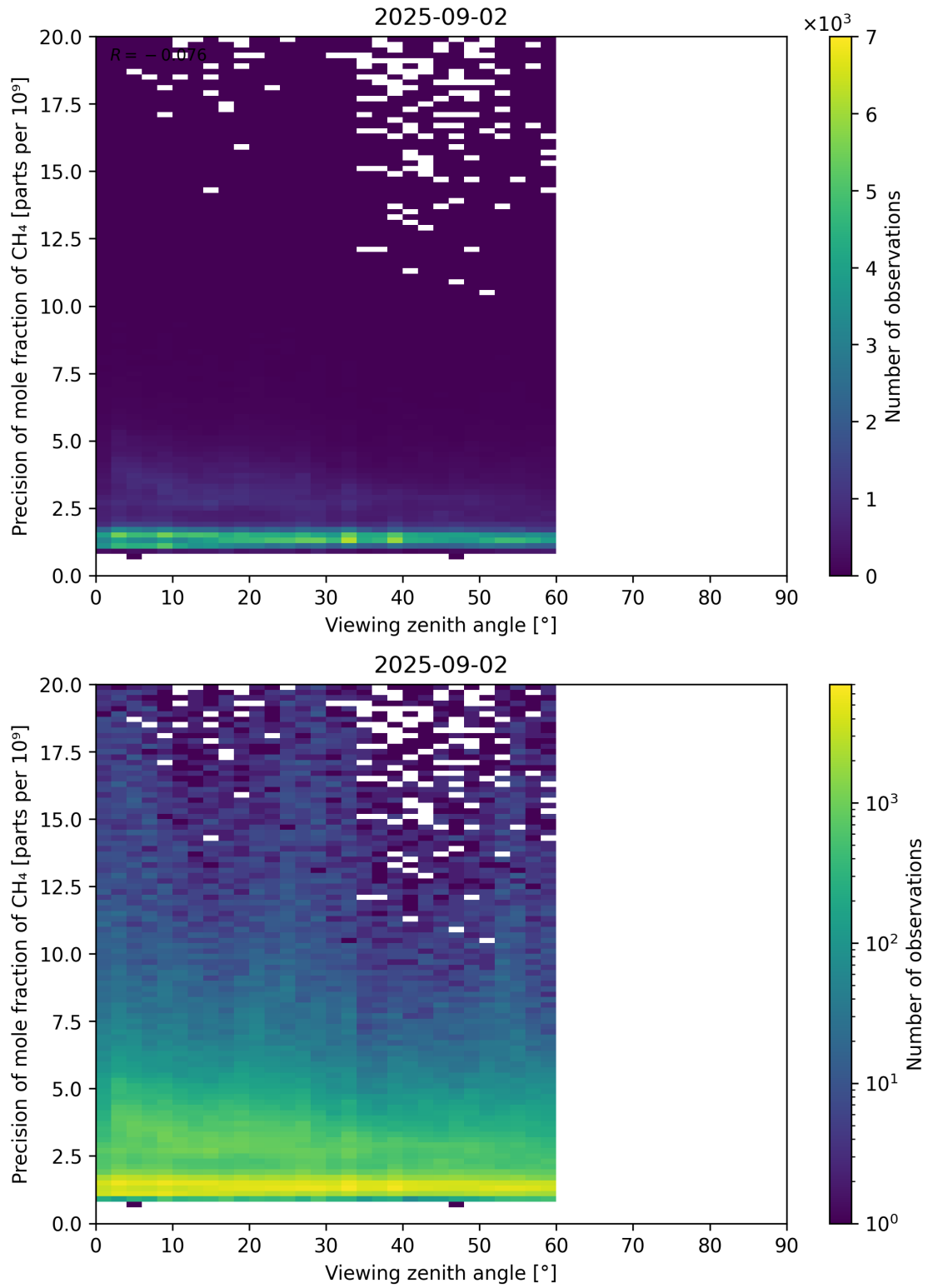
Figure 112: Scatter density plot of “Viewing zenith angle” against “Precision of mole fraction of CH 4 ” for 2025-09-01 to 2025-09-03.
