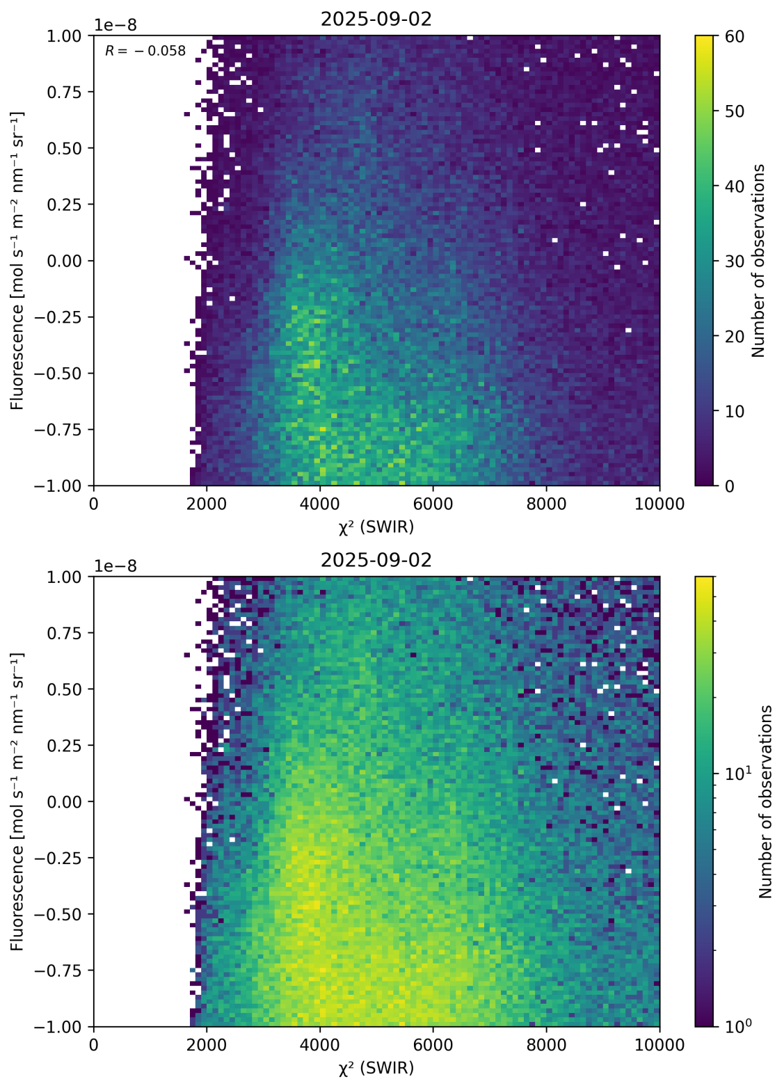
Figure 49: Scatter density plot of “ \chi^2 (SWIR)” against “Fluorescence” for 2025-09-01 to 2025-09-03.
