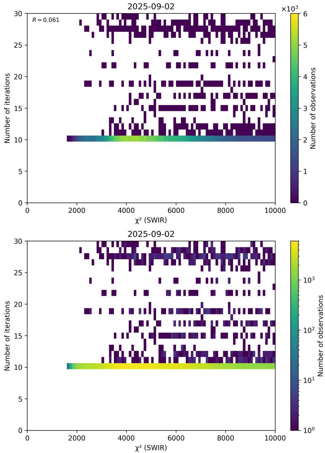
Figure 50: Scatter density plot of “ \chi^2 (SWIR)” against “Number of iterations” for 2025-09-01 to 2025-09-03.
