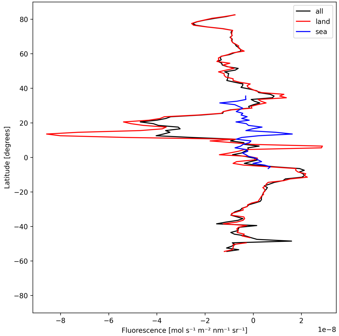
Figure 21: Zonal average of “Fluorescence” for 2025-09-01 to 2025-09-03.
