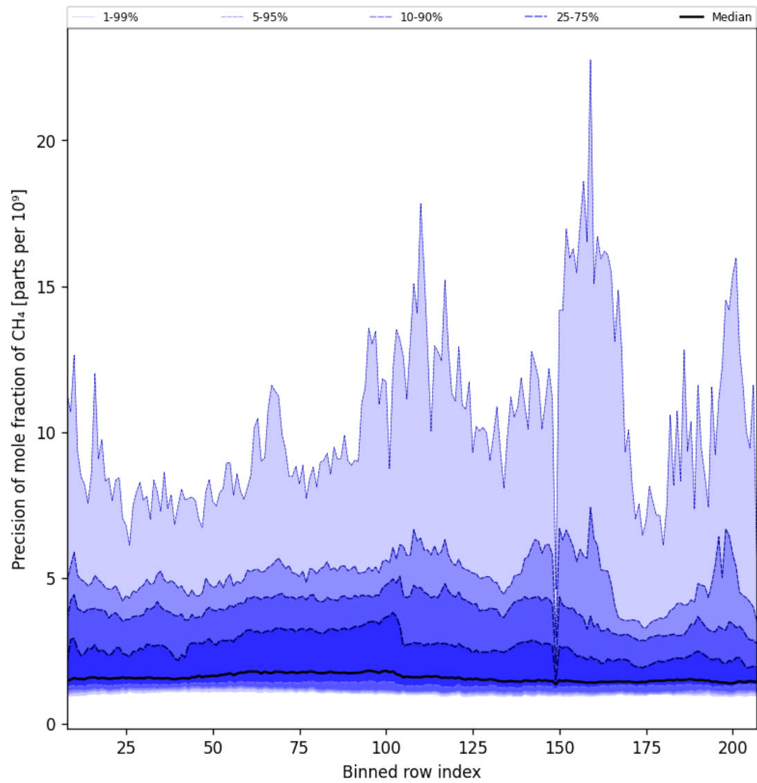
Figure 35: Along track statistics of “Precision of mole fraction of CH 4 ” for 2025-09-01 to 2025-09-03
