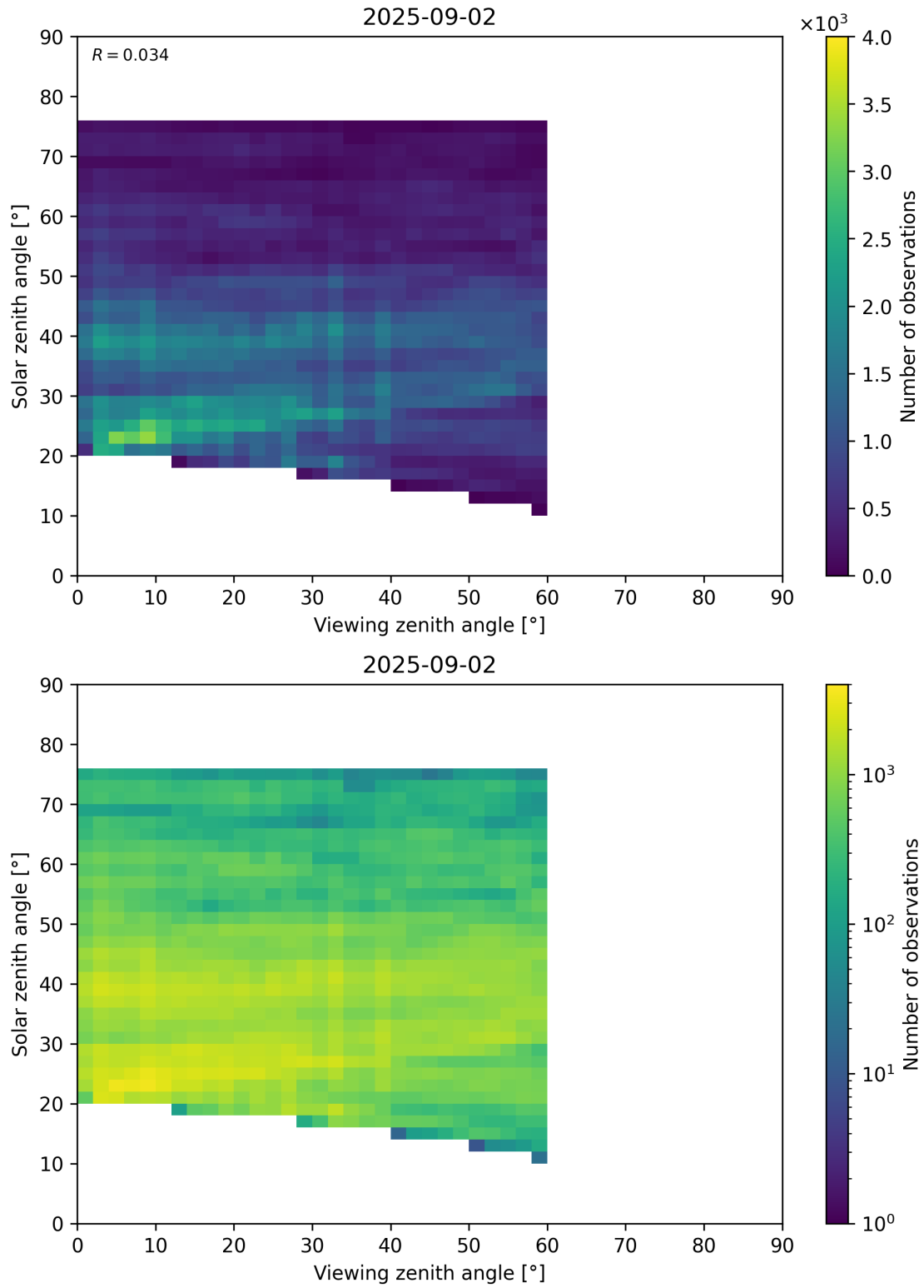
Figure 115: Scatter density plot of “Viewing zenith angle” against “Solar zenith angle” for 2025-09-01 to 2025-09-03.
