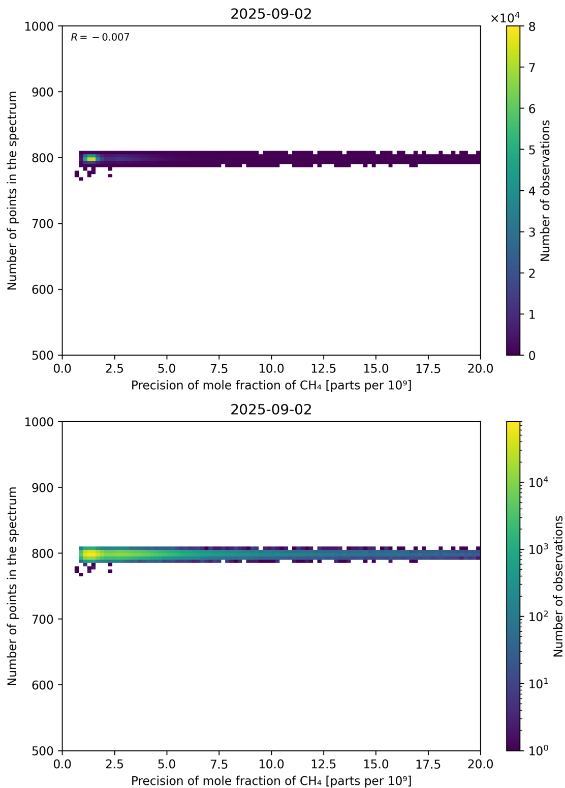
Figure 84: Scatter density plot of “Precision of mole fraction of CH 4 ” against “Number of points in the spectrum” for 2025-09-01 to 2025-09-03.
