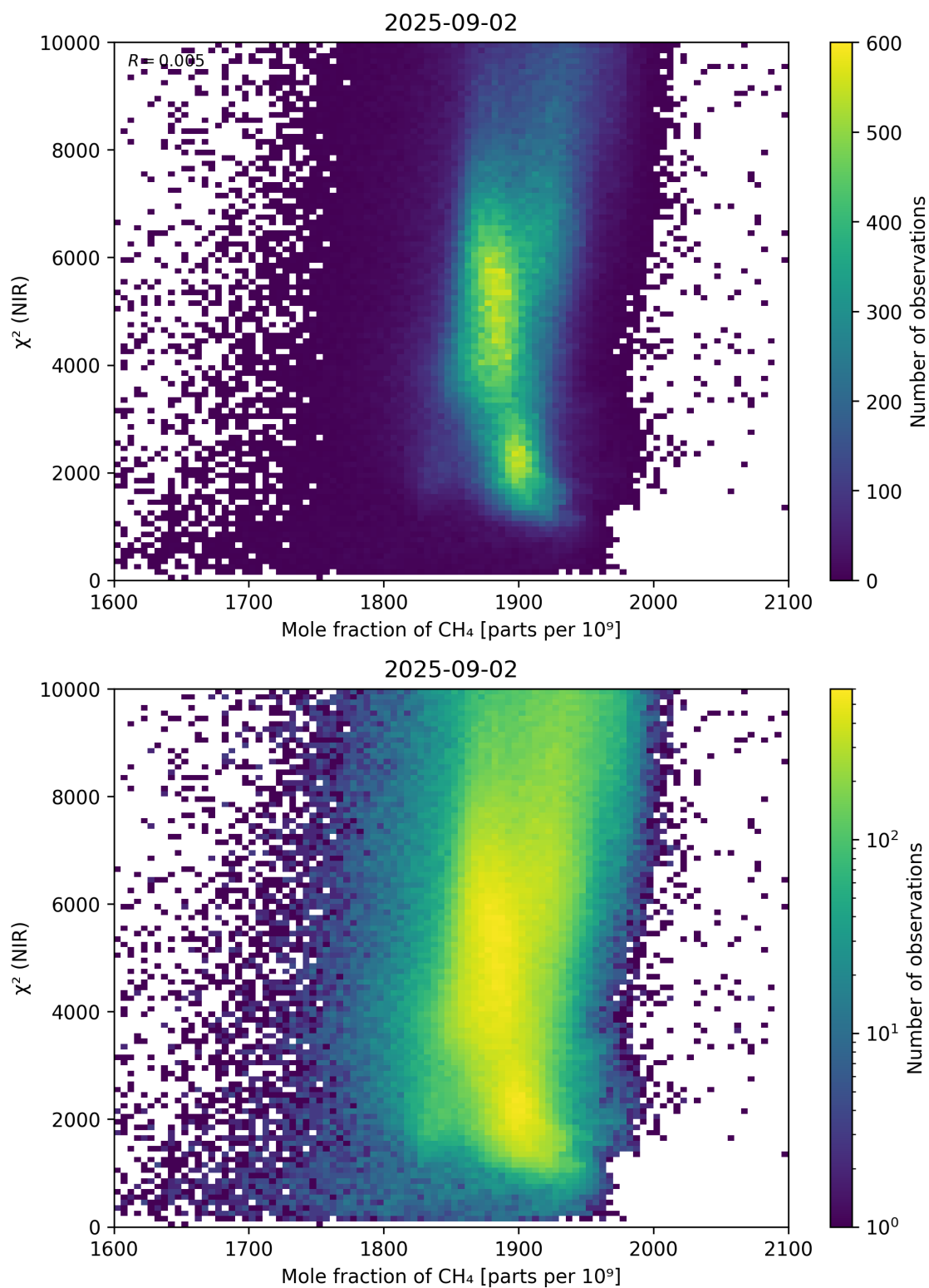
Figure 70: Scatter density plot of “Mole fraction of CH 4 ” against “ \chi^2 (NIR)” for 2025-09-01 to 2025-09-03.
