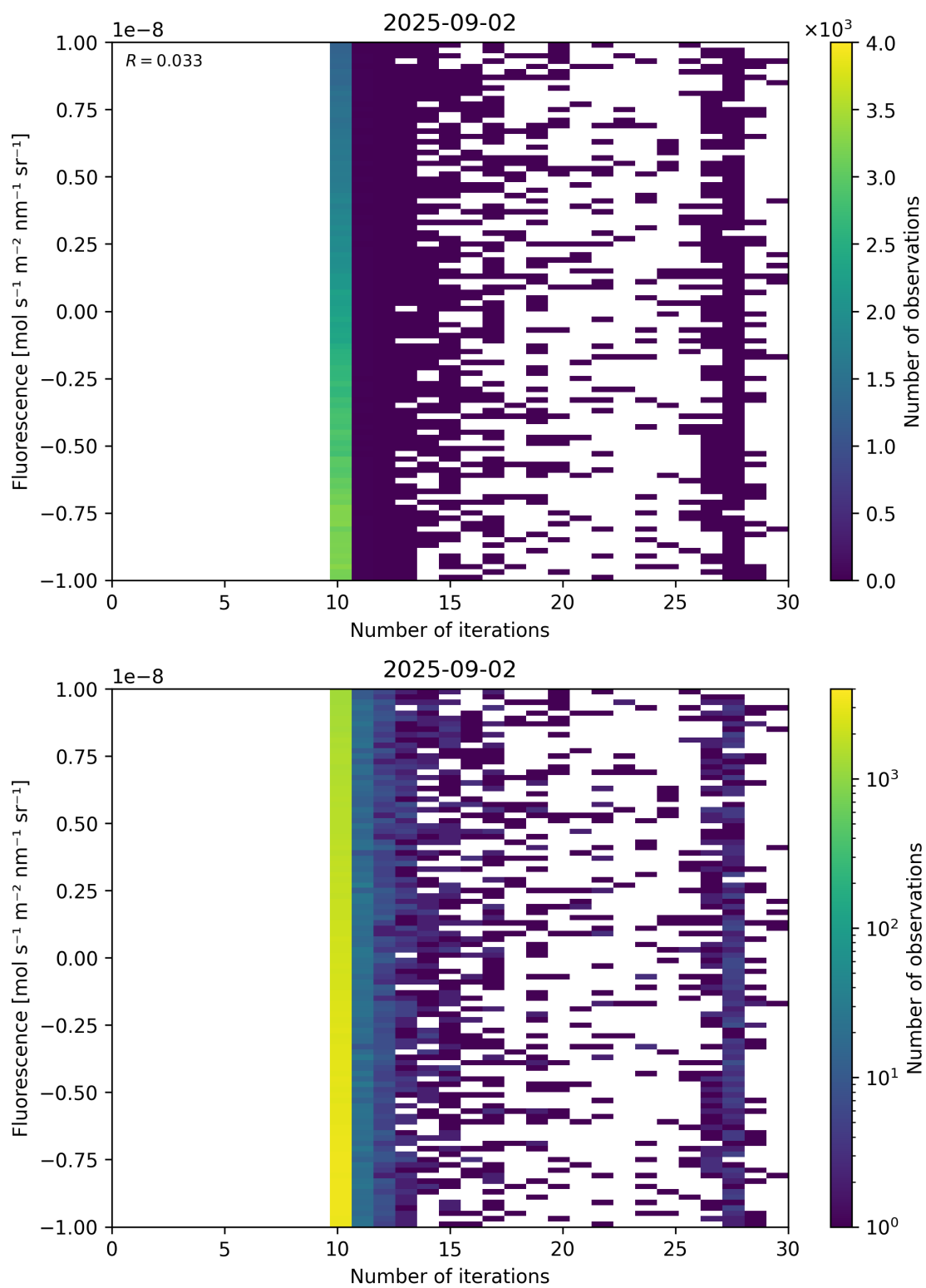
Figure 87: Scatter density plot of “Number of iterations” against “Fluorescence” for 2025-09-01 to 2025-09-03.
