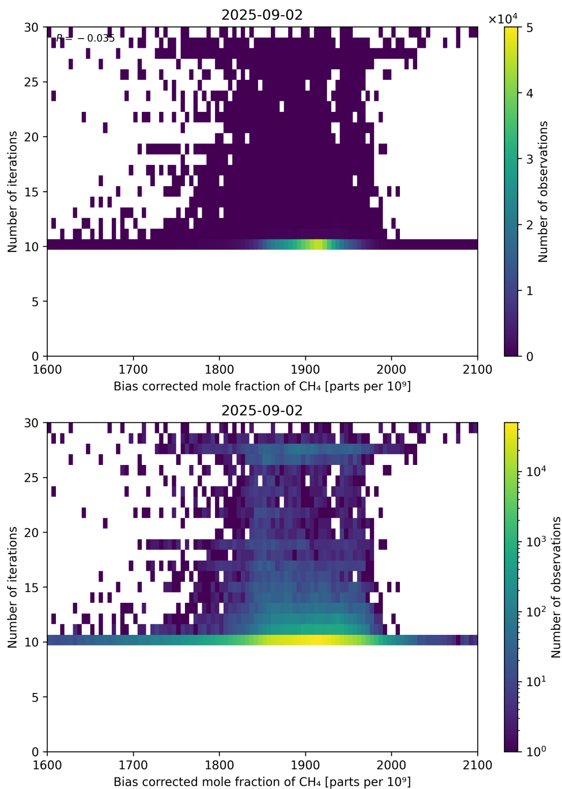
Figure 67: Scatter density plot of “Bias corrected mole fraction of CH 4 ” against “Number of iterations” for 2025-09-01 to 2025-09-03.
