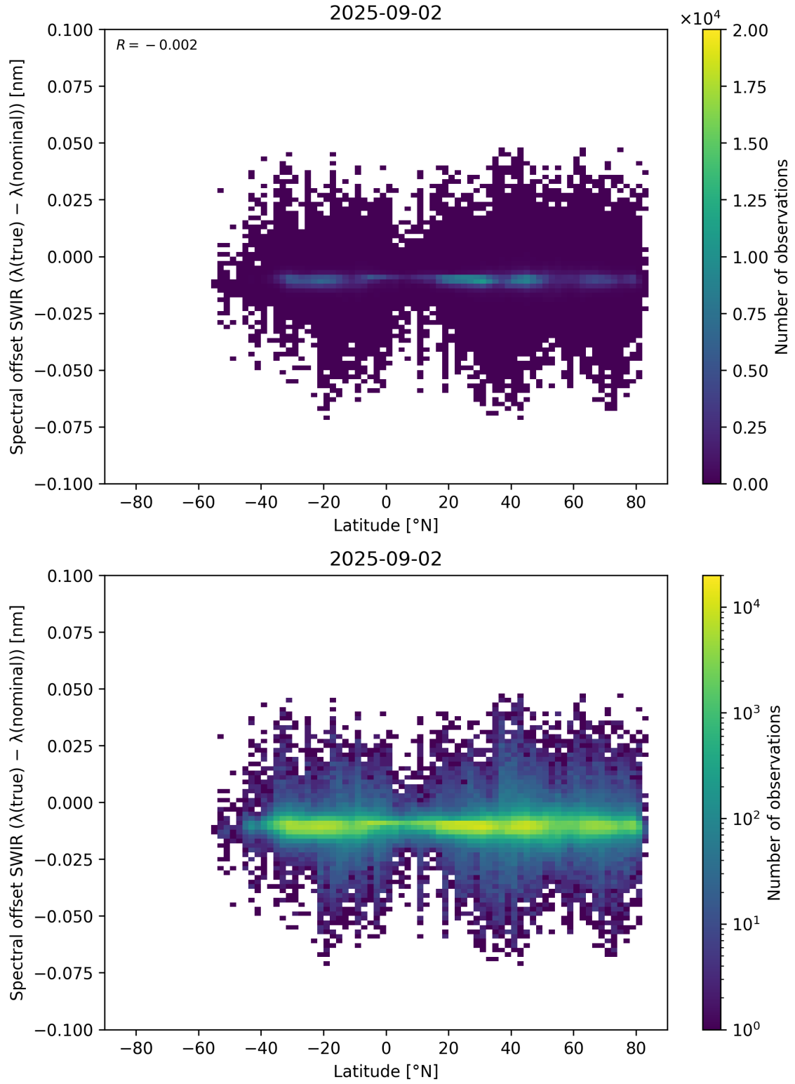
Figure 62: Scatter density plot of “Latitude” against “Spectral offset SWIR ( \lambda_{\text{true}} - \lambda_{\text{nominal}} )” for 2025-09-01 to 2025-09-03.
