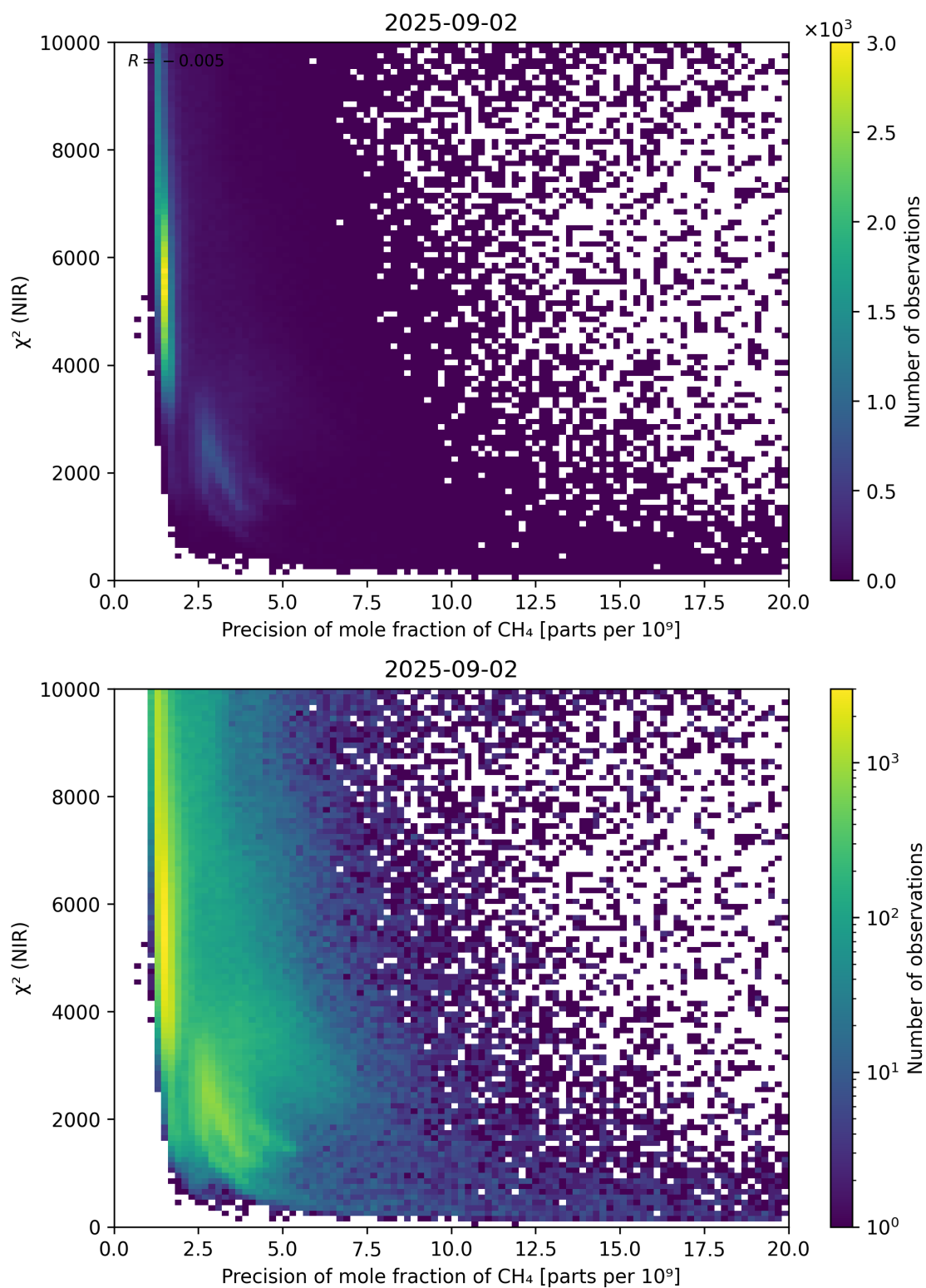
Figure 78: Scatter density plot of “Precision of mole fraction of CH 4 ” against “ \chi^2 (NIR)” for 2025-09-01 to 2025-09-03.
