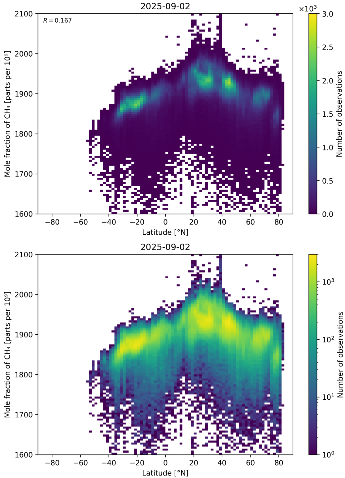
Figure 57: Scatter density plot of “Latitude” against “Mole fraction of CH 4 ” for 2025-09-01 to 2025-09-03.
