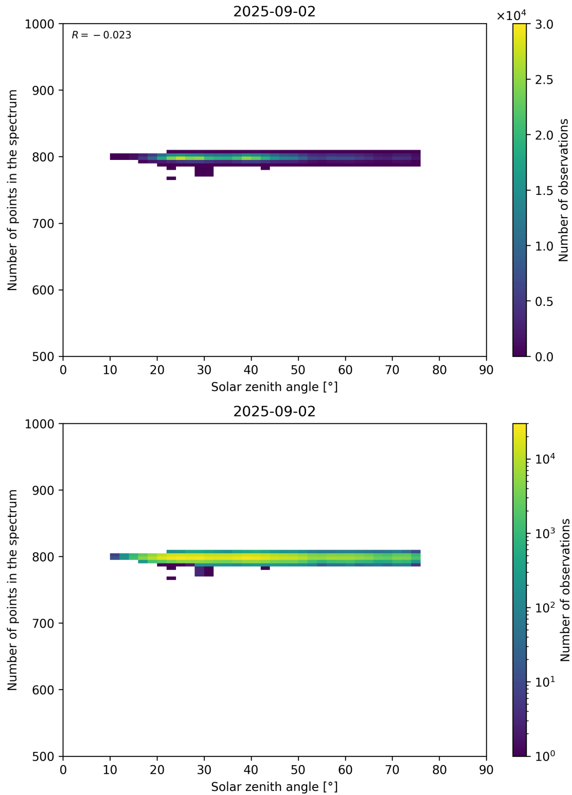
Figure 103: Scatter density plot of “Solar zenith angle” against “Number of points in the spectrum” for 2025-09-01 to 2025-09-03.
