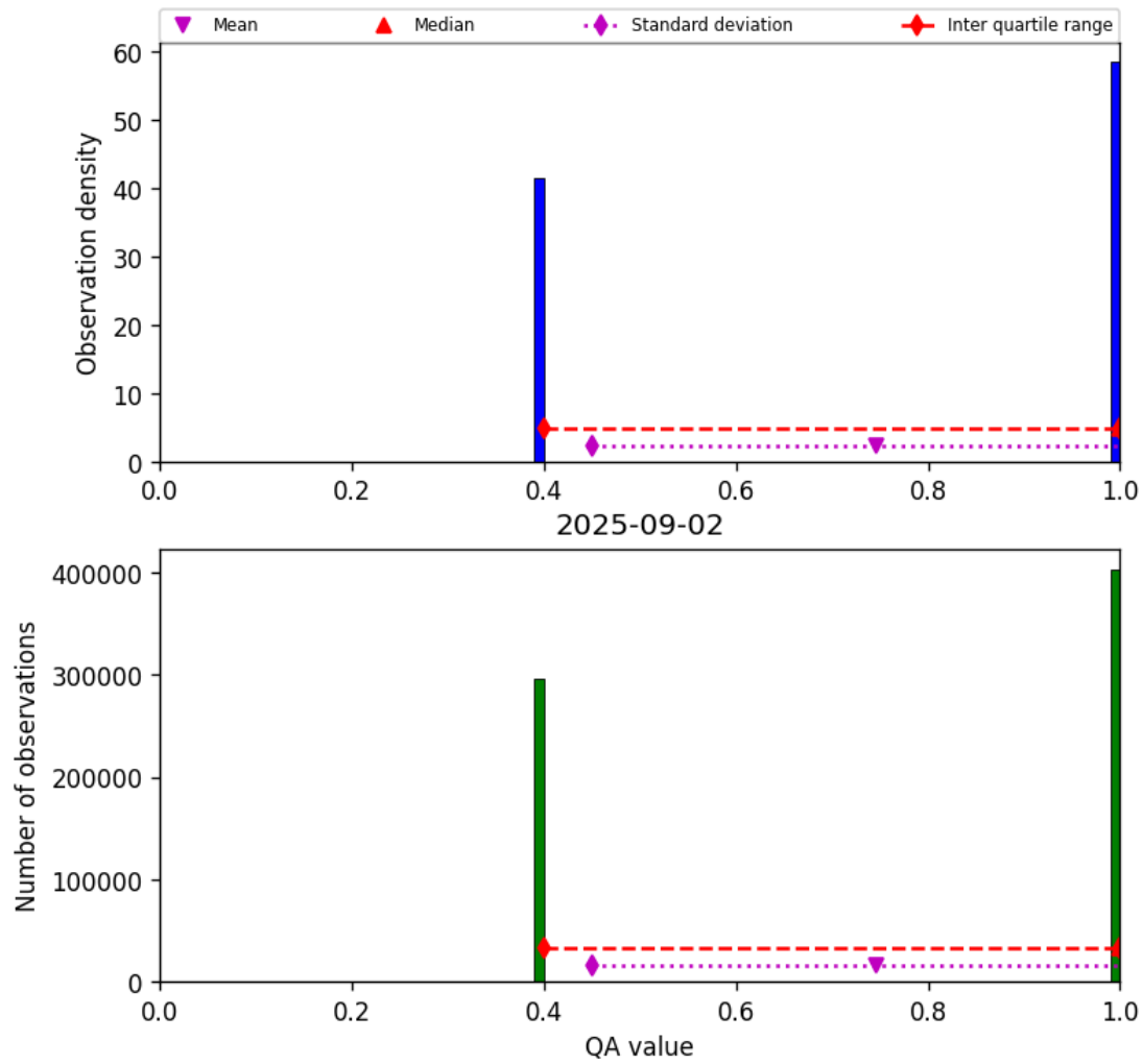
Figure 22: Histogram of “QA value” for 2025-09-01 to 2025-09-03
