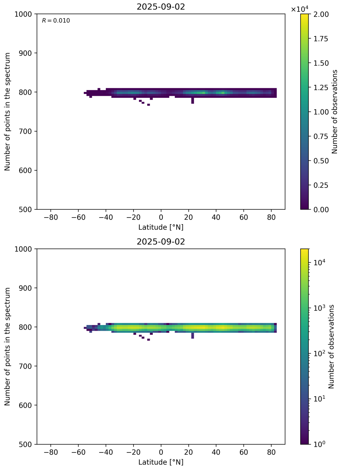
Figure 61: Scatter density plot of “Latitude” against “Number of points in the spectrum” for 2025-09-01 to 2025-09-03.
