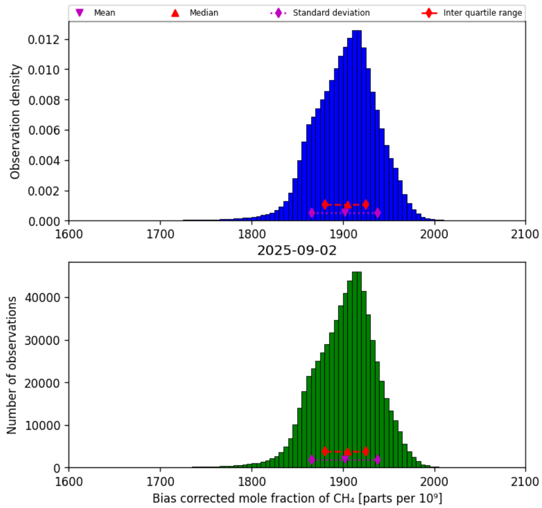
Figure 25: Histogram of “Bias corrected mole fraction of CH 4 ” for 2025-09-01 to 2025-09-03
