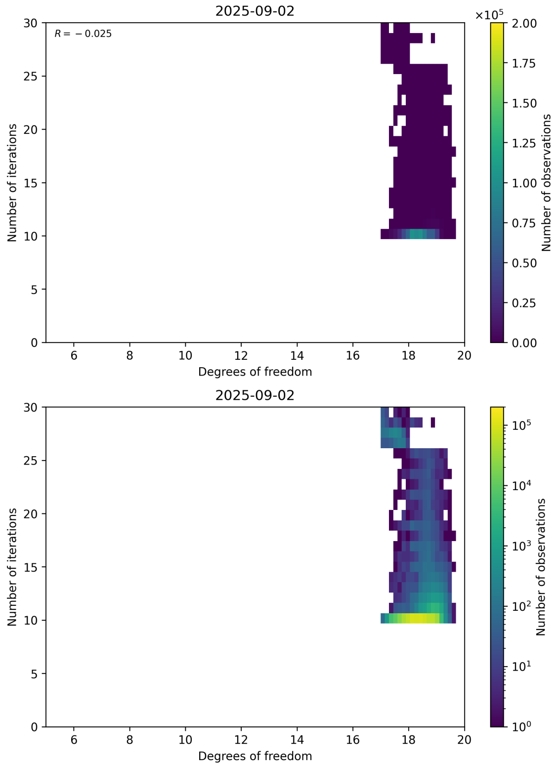
Figure 52: Scatter density plot of “Degrees of freedom” against “Number of iterations” for 2025-09-01 to 2025-09-03.
