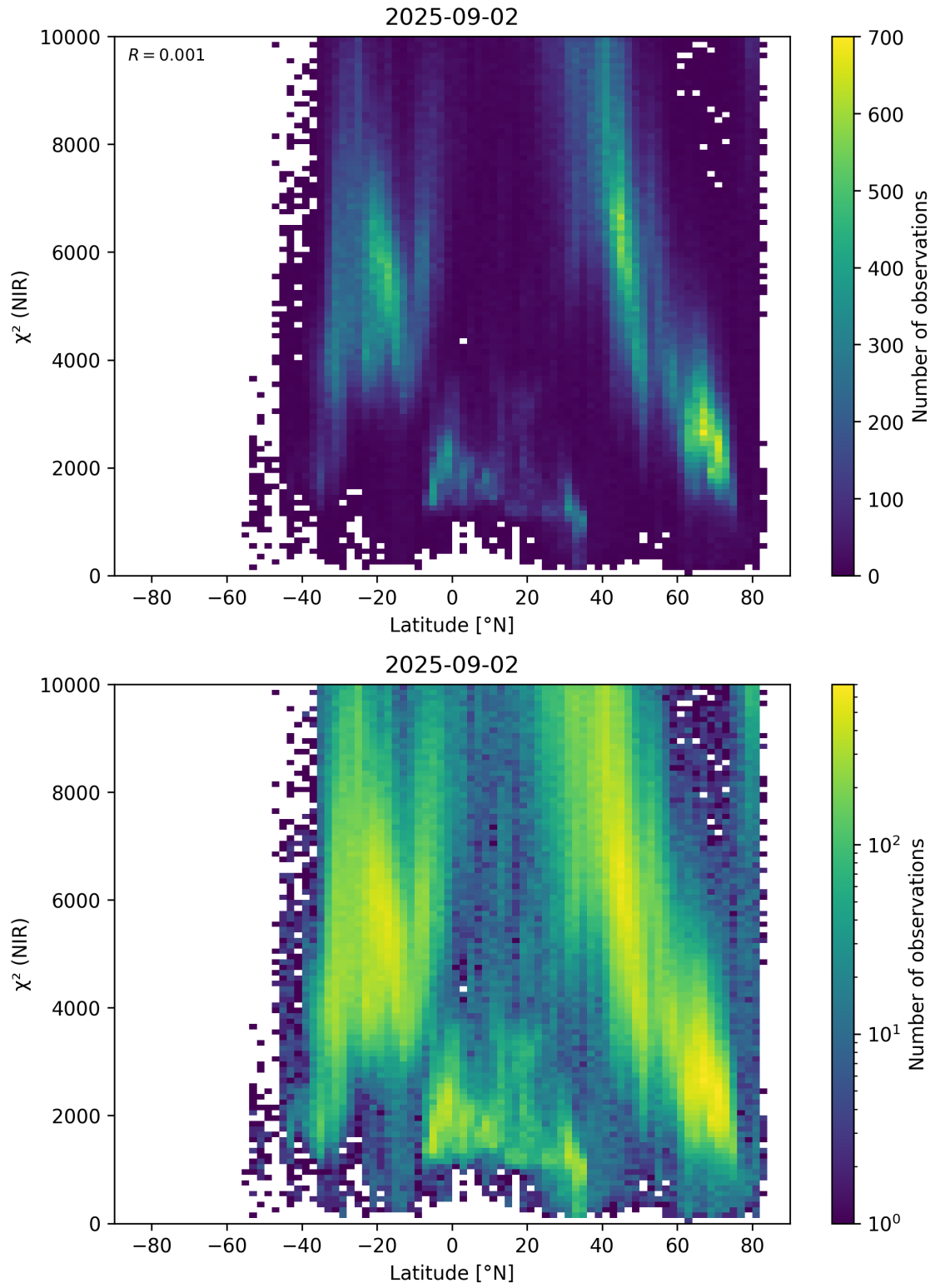
Figure 53: Scatter density plot of “Latitude” against “ \chi^2 (NIR)” for 2025-09-01 to 2025-09-03.
