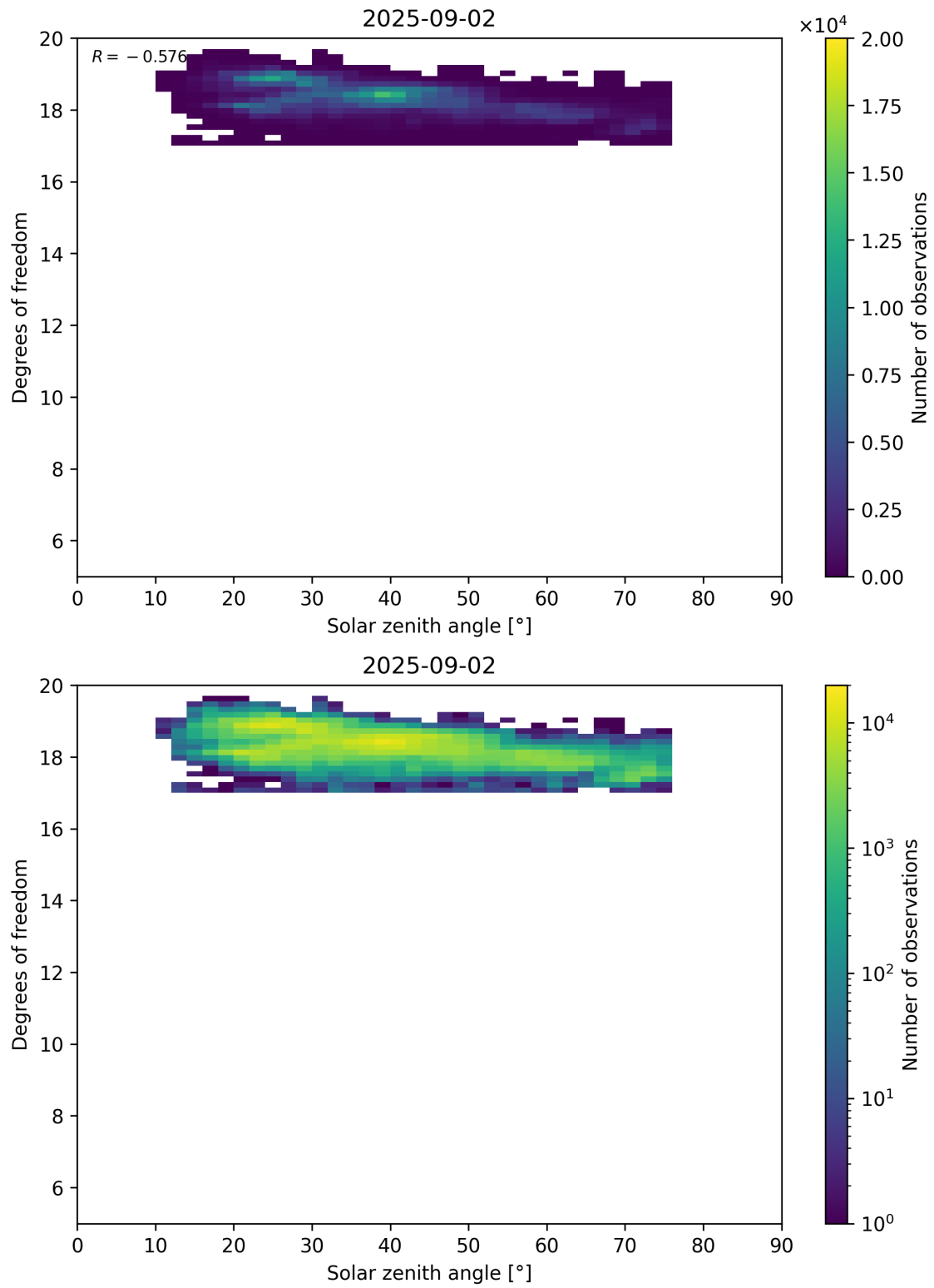
Figure 96: Scatter density plot of “Solar zenith angle” against “Degrees of freedom” for 2025-09-01 to 2025-09-03.
