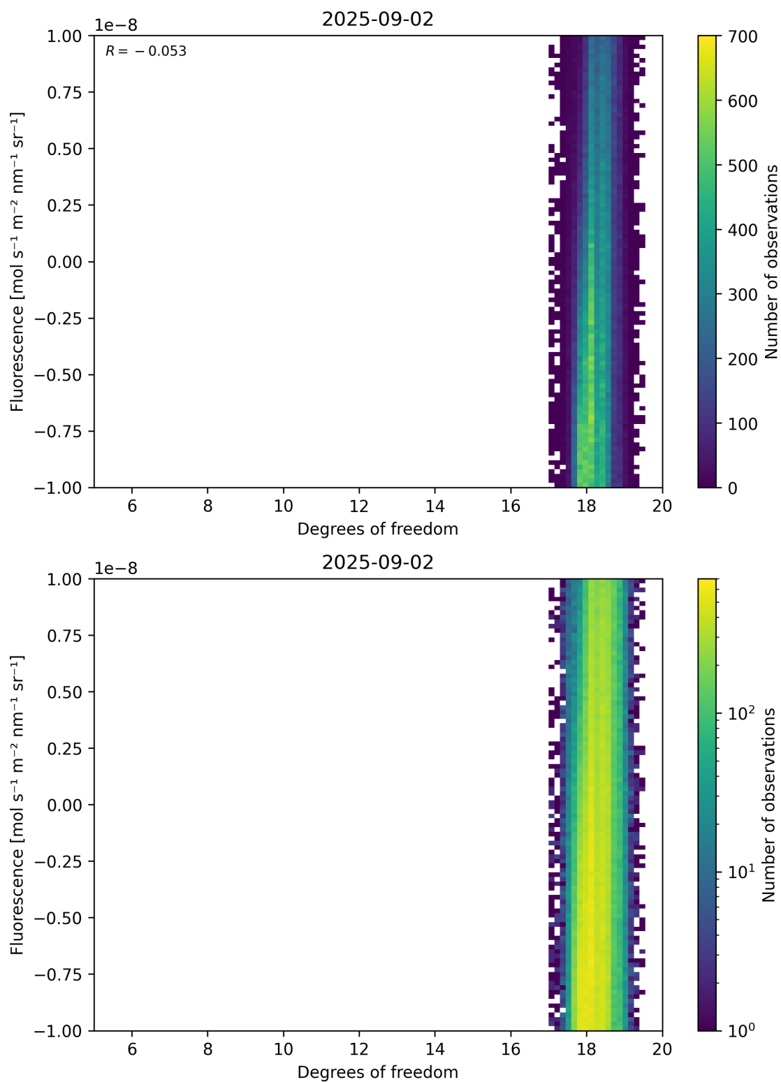
Figure 51: Scatter density plot of “Degrees of freedom” against “Fluorescence” for 2025-09-01 to 2025-09-03.
