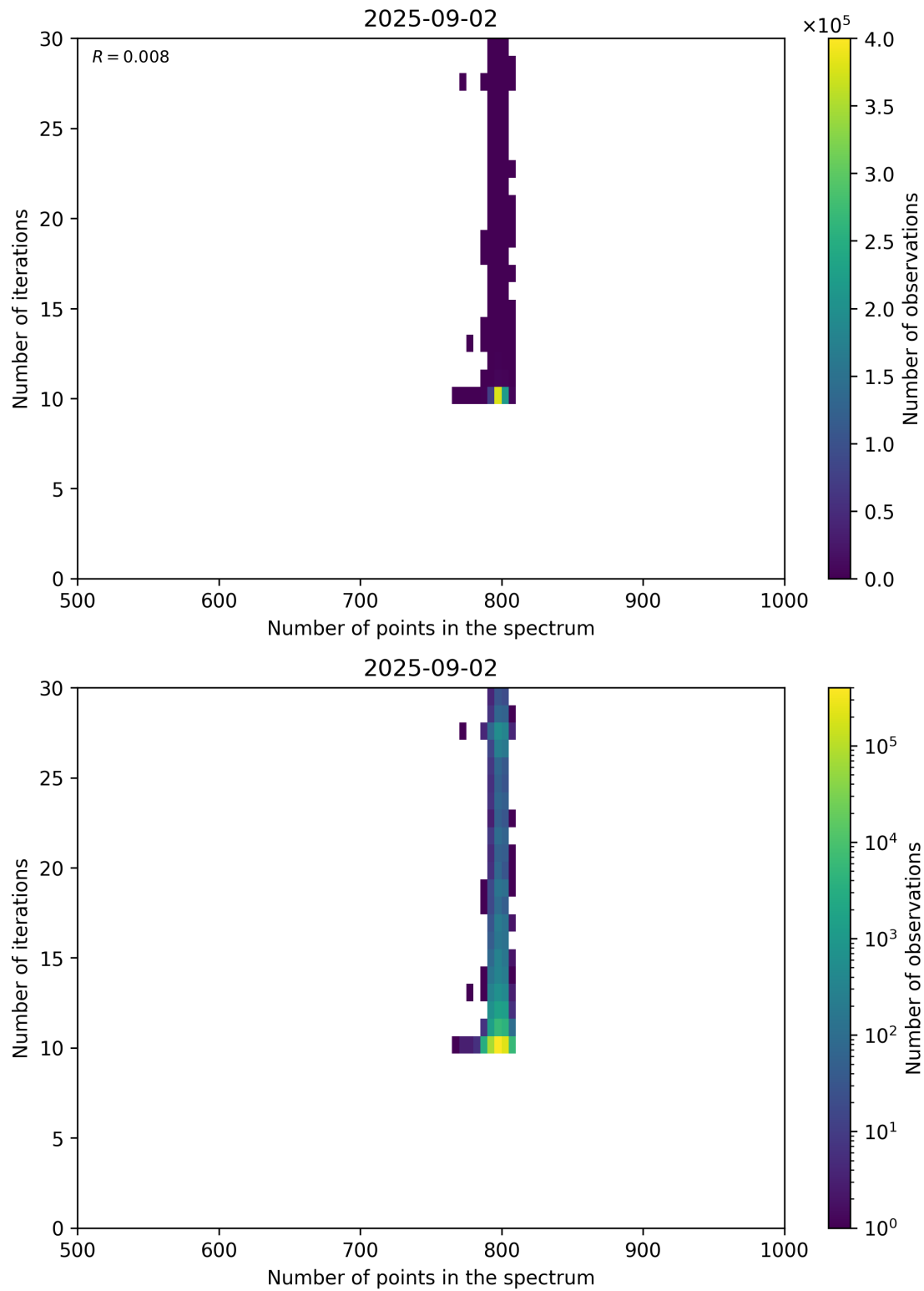
Figure 92: Scatter density plot of “Number of points in the spectrum” against “Number of iterations” for 2025-09-01 to 2025-09-03.
