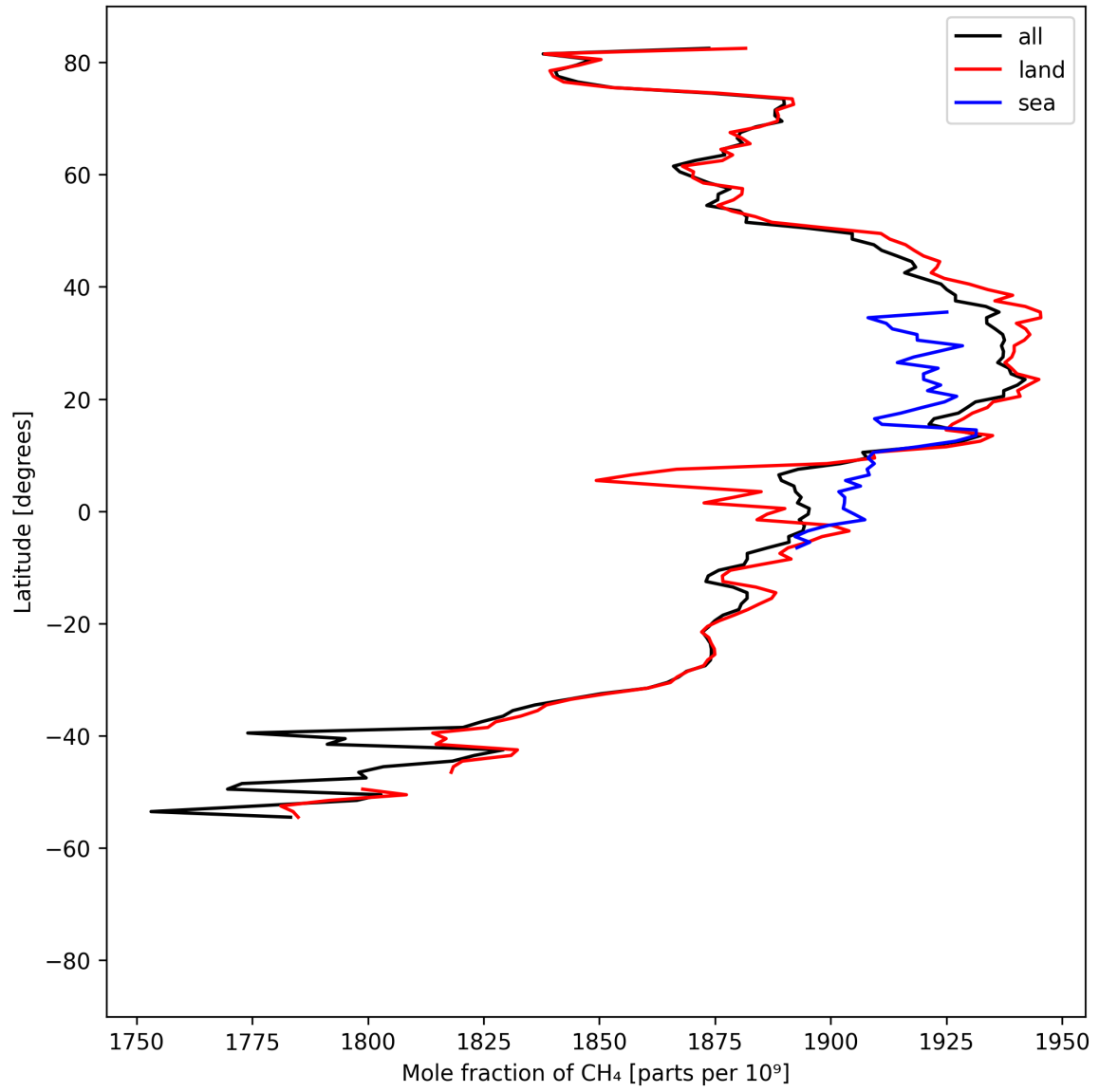
Figure 12: Zonal average of “Mole fraction of CH 4 ” for 2025-09-01 to 2025-09-03.
