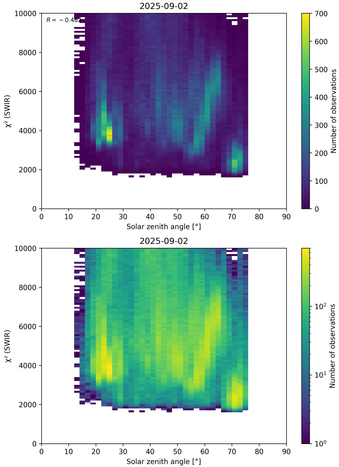
Figure 95: Scatter density plot of “Solar zenith angle” against “ \chi^2 (SWIR)” for 2025-09-01 to 2025-09-03.
