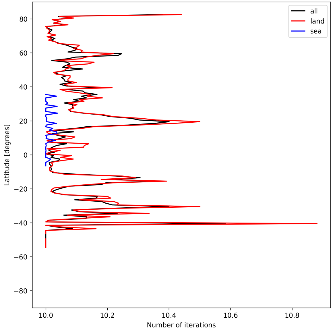
Figure 20: Zonal average of “Number of iterations” for 2025-09-01 to 2025-09-03.
