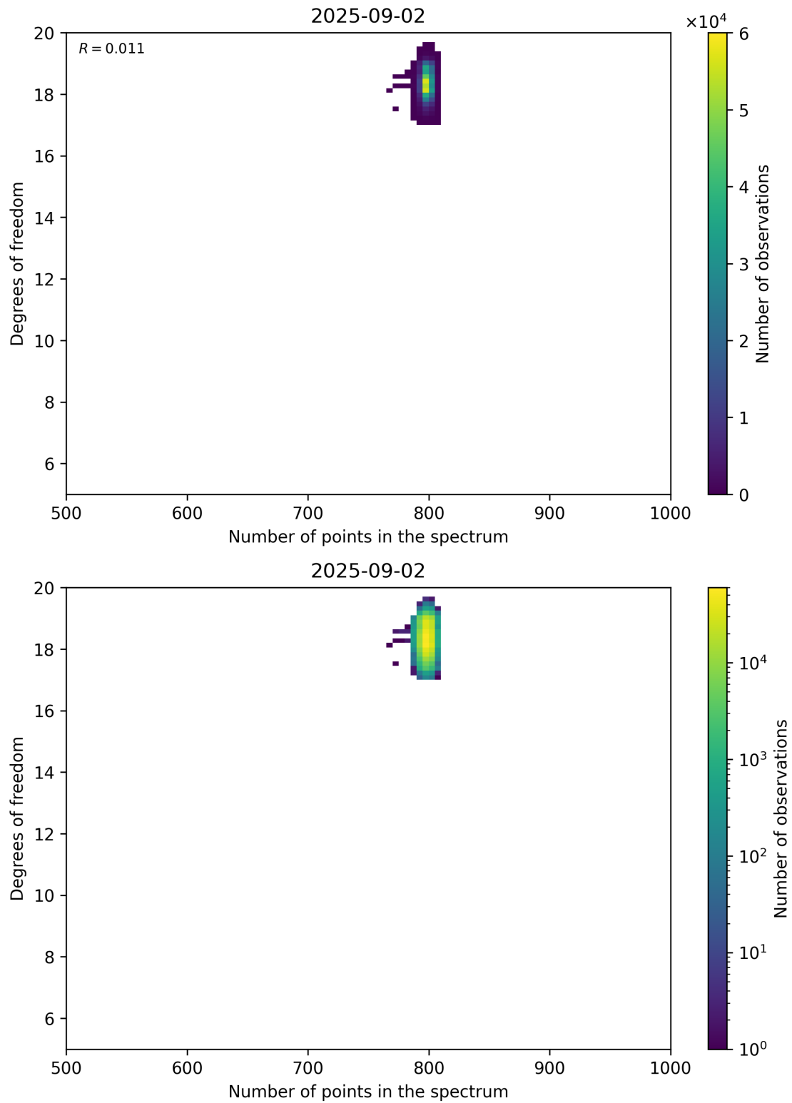
Figure 90: Scatter density plot of “Number of points in the spectrum” against “Degrees of freedom” for 2025-09-01 to 2025-09-03.
