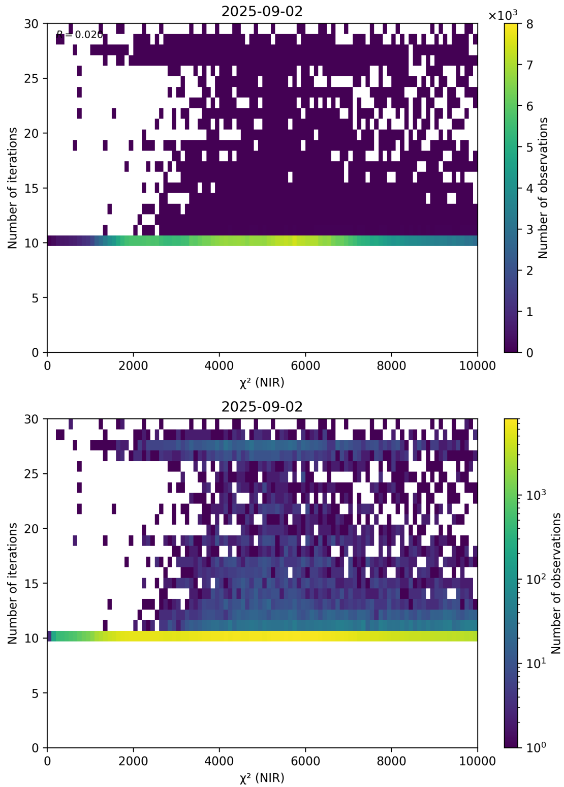
Figure 46: Scatter density plot of “ \chi^2 (NIR)” against “Number of iterations” for 2025-09-01 to 2025-09-03.
