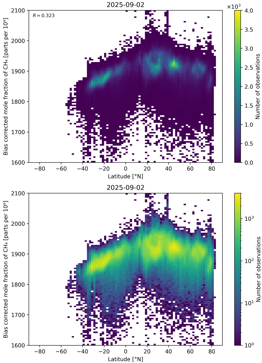
Figure 58: Scatter density plot of “Latitude” against “Bias corrected mole fraction of CH 4 ” for 2025-09-01 to 2025-09-03.
