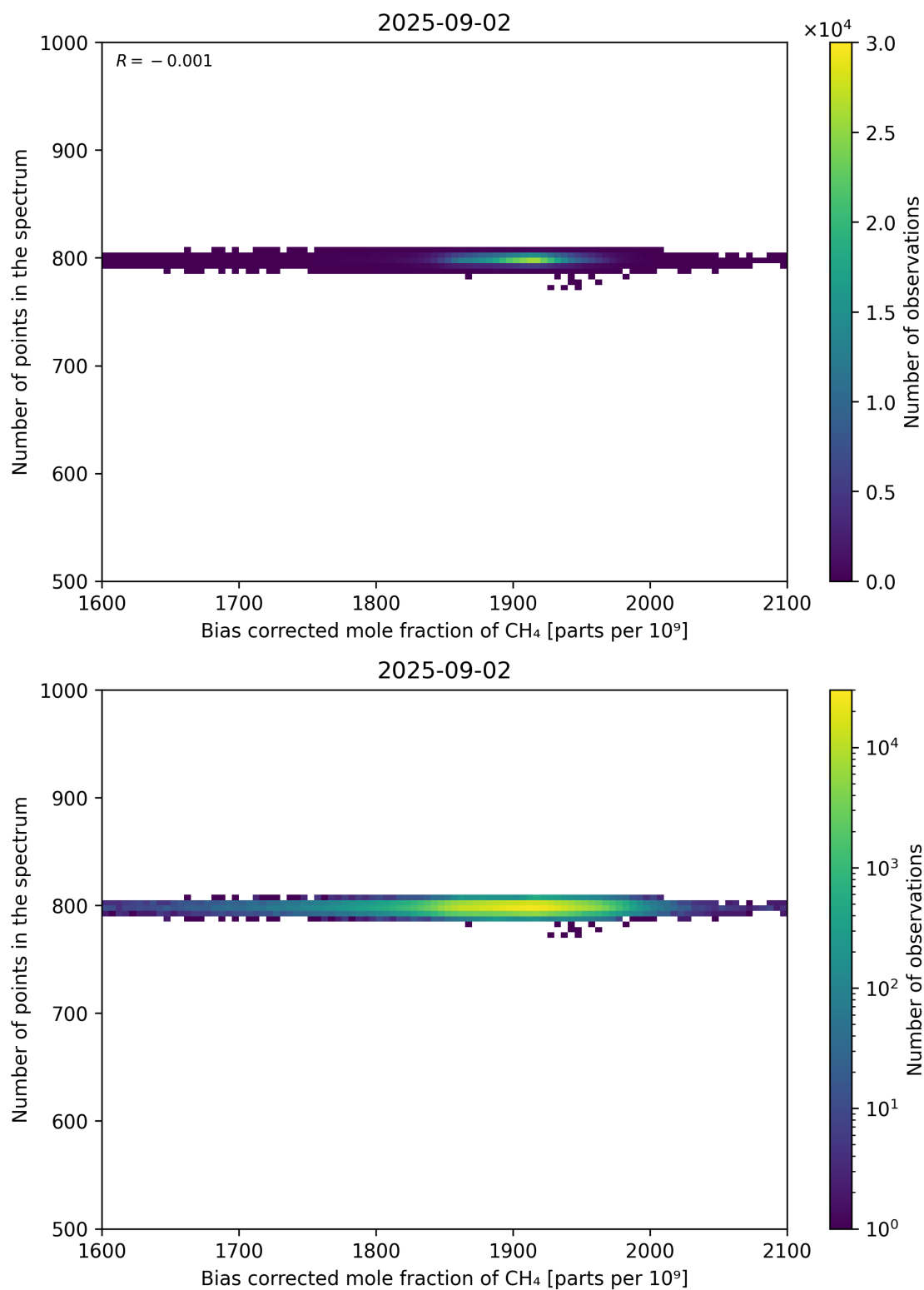
Figure 68: Scatter density plot of “Bias corrected mole fraction of CH 4 ” against “Number of points in the spectrum” for 2025-09-01 to 2025-09-03.
