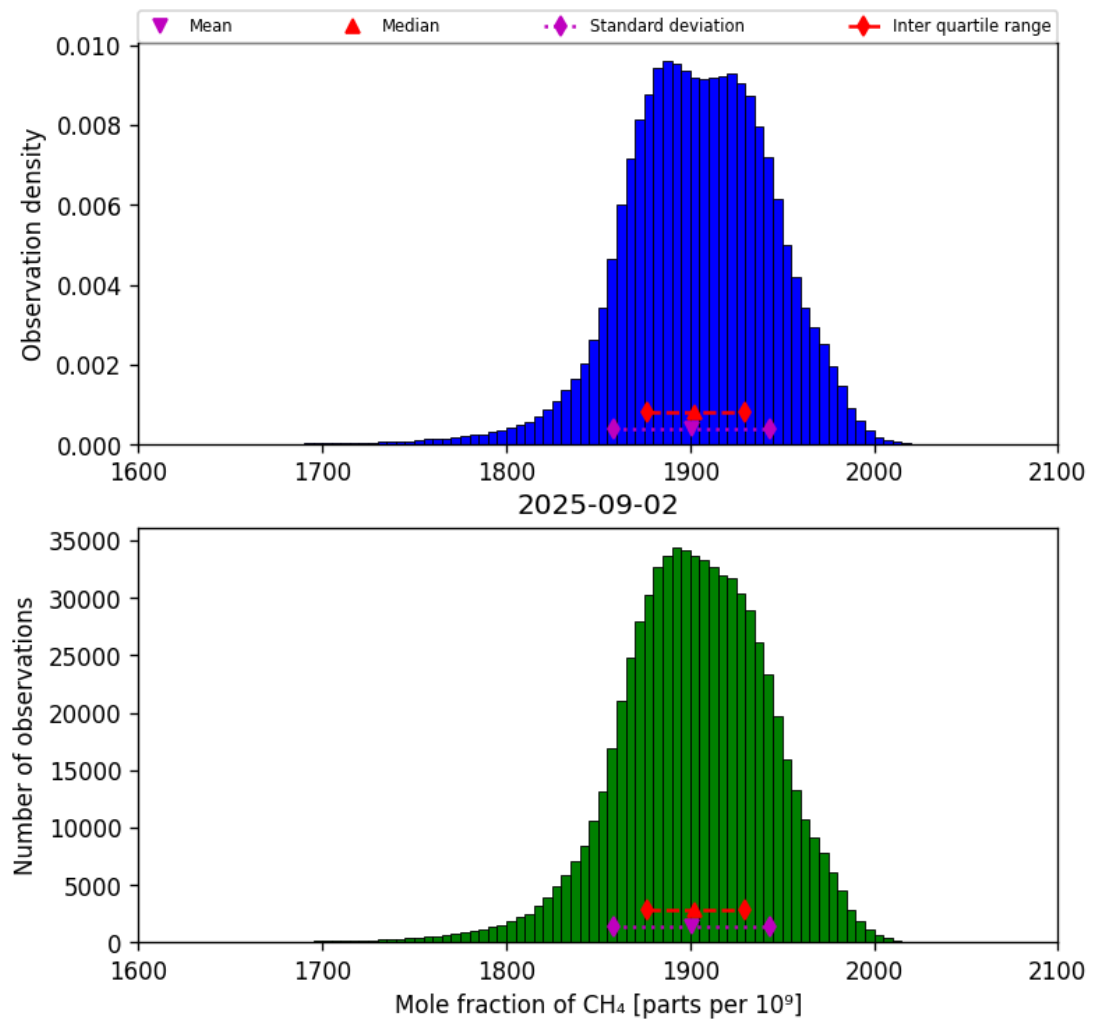
Figure 23: Histogram of “Mole fraction of CH 4 ” for 2025-09-01 to 2025-09-03
