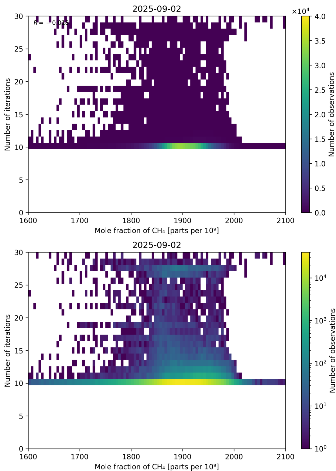
Figure 76: Scatter density plot of “Mole fraction of CH 4 ” against “Number of iterations” for 2025-09-01 to 2025-09-03.
