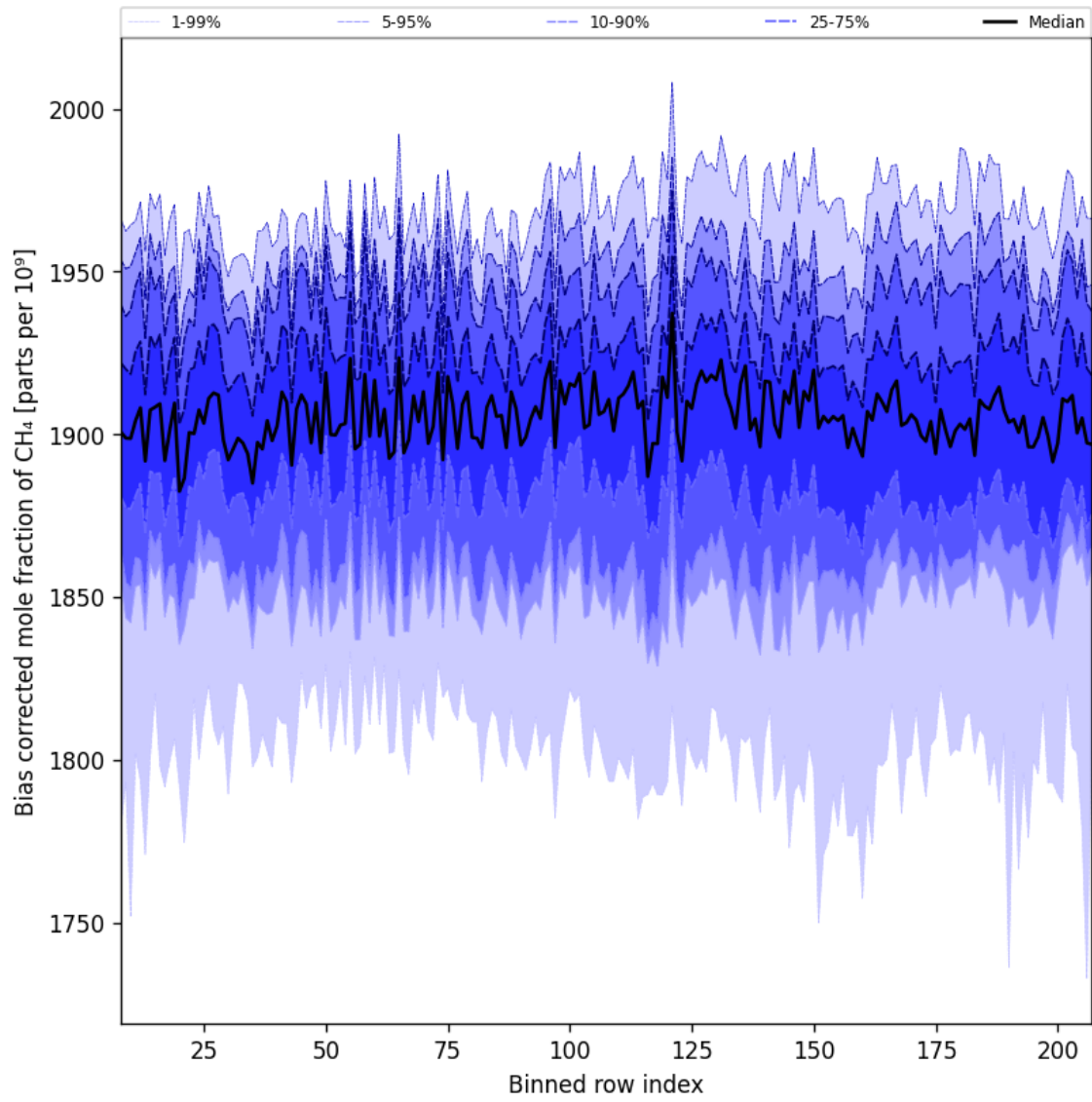
Figure 36: Along track statistics of “Bias corrected mole fraction of CH 4 ” for 2025-09-01 to 2025-09-03
