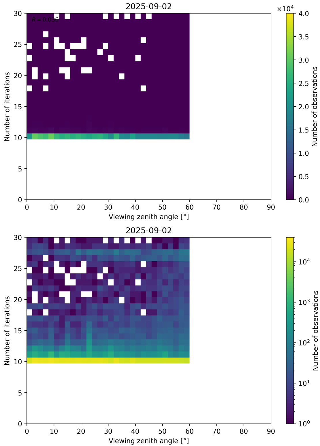
Figure 113: Scatter density plot of “Viewing zenith angle” against “Number of iterations” for 2025-09-01 to 2025-09-03.
