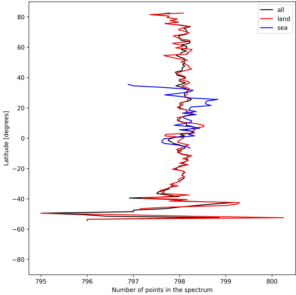
Figure 15: Zonal average of “Number of points in the spectrum” for 2025-09-01 to 2025-09-03.
