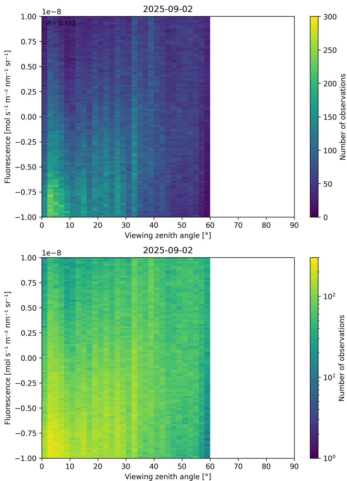
Figure 108: Scatter density plot of “Viewing zenith angle” against “Fluorescence” for 2025-09-01 to 2025-09-03.
