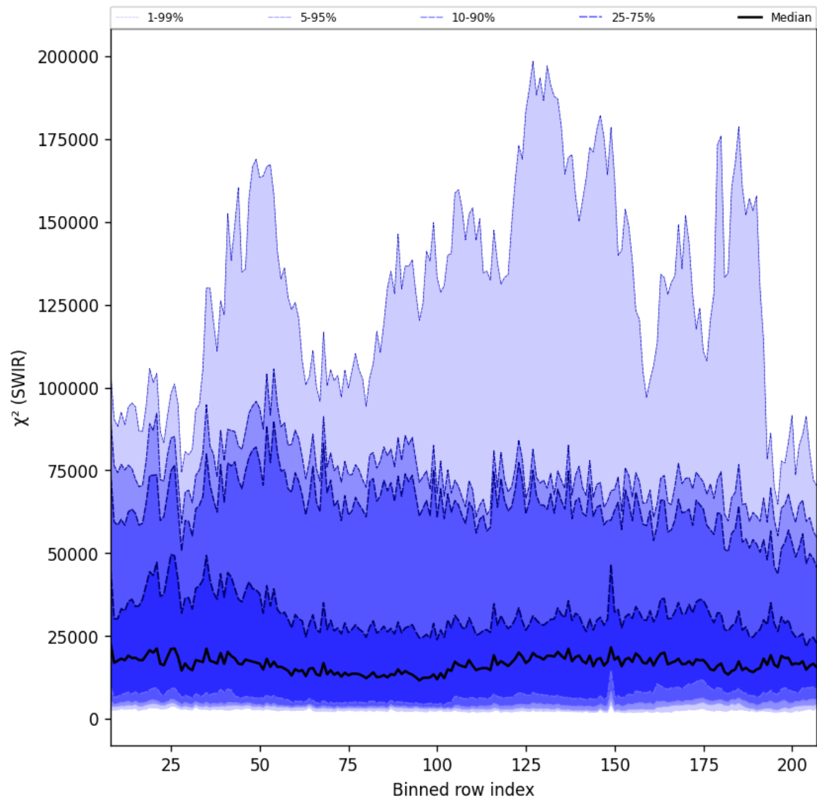
Figure 39: Along track statistics of " \chi^2 (SWIR)" for 2025-09-01 to 2025-09-03
