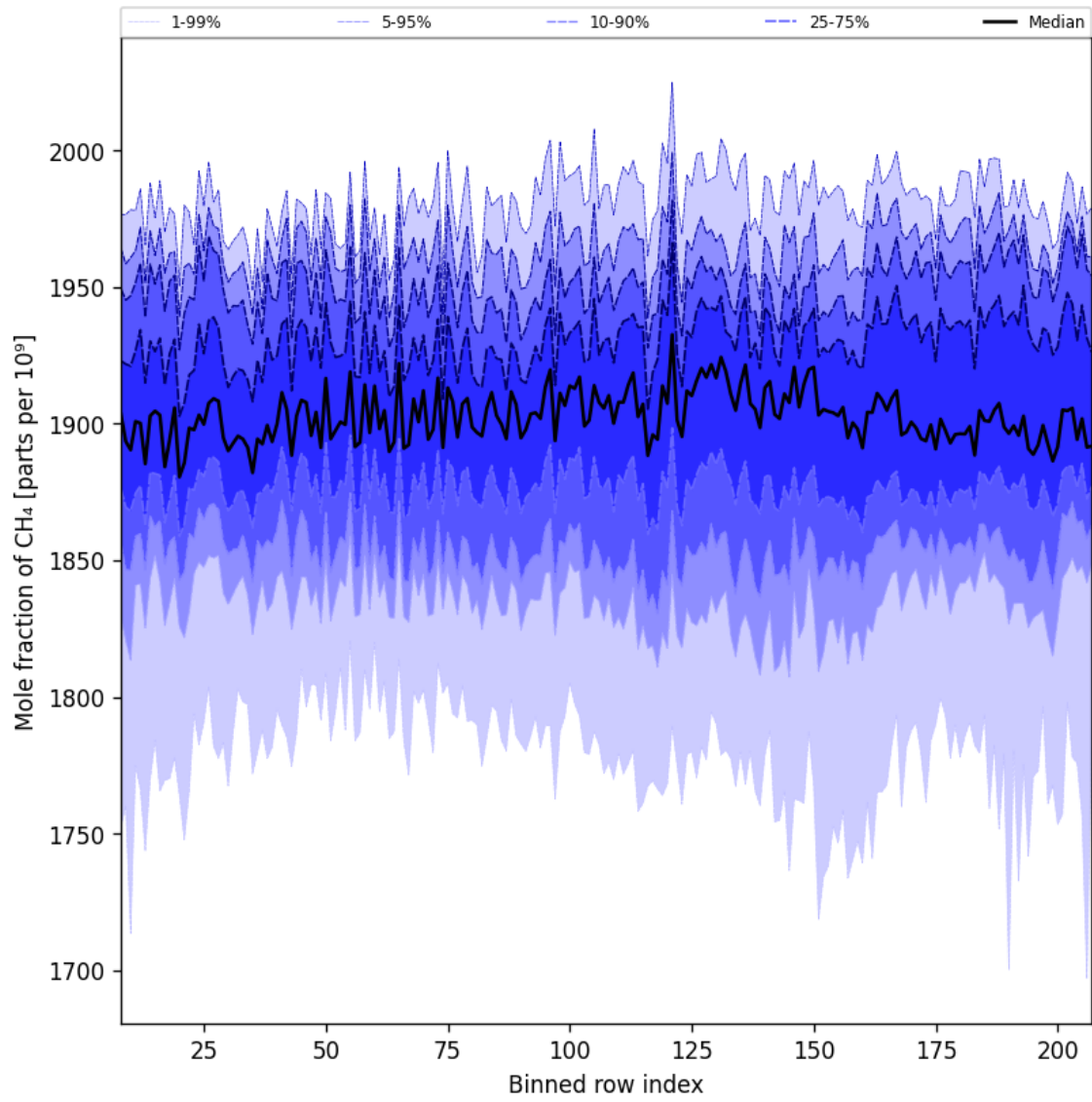
Figure 34: Along track statistics of “Mole fraction of CH 4 ” for 2025-09-01 to 2025-09-03
