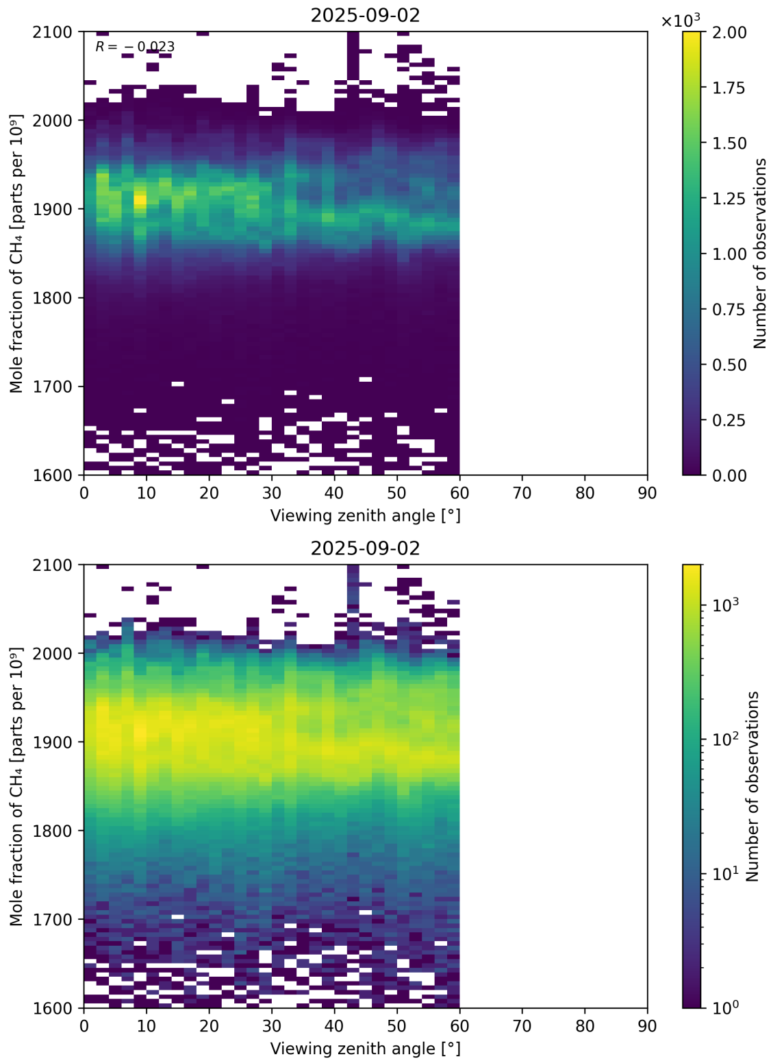
Figure 110: Scatter density plot of “Viewing zenith angle” against “Mole fraction of CH 4 ” for 2025-09-01 to 2025-09-03.
