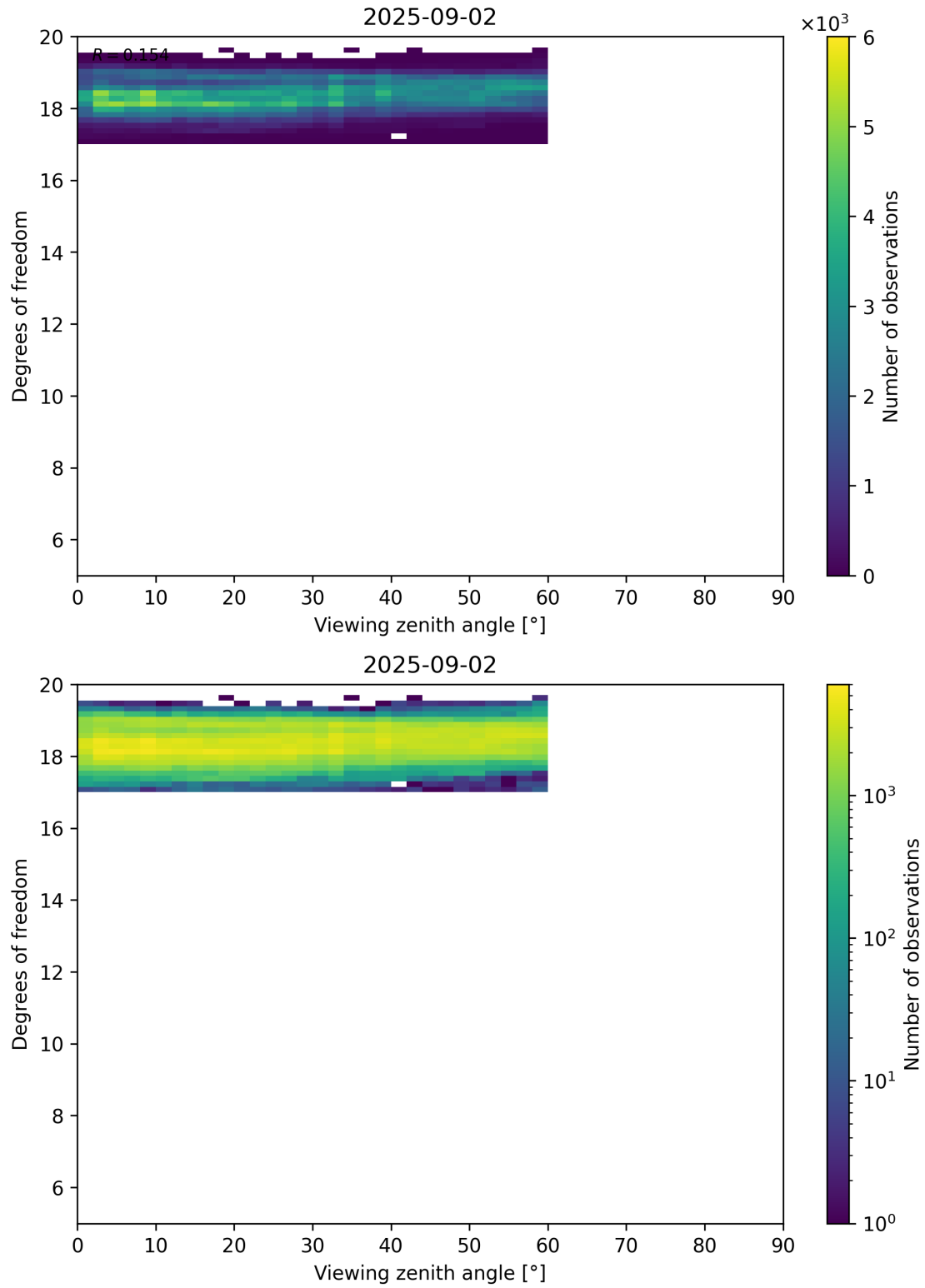
Figure 107: Scatter density plot of “Viewing zenith angle” against “Degrees of freedom” for 2025-09-01 to 2025-09-03.
