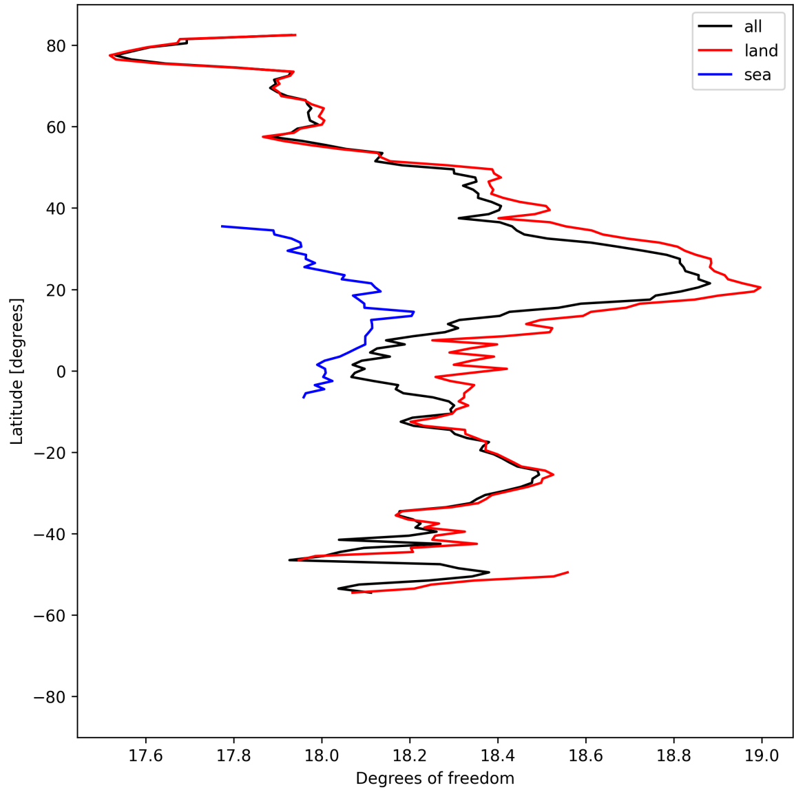
Figure 19: Zonal average of “Degrees of freedom” for 2025-09-01 to 2025-09-03.
