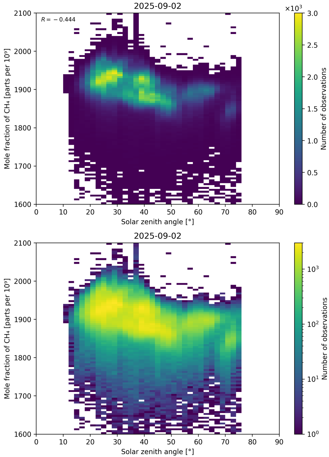
Figure 99: Scatter density plot of “Solar zenith angle” against “Mole fraction of CH 4 ” for 2025-09-01 to 2025-09-03.
