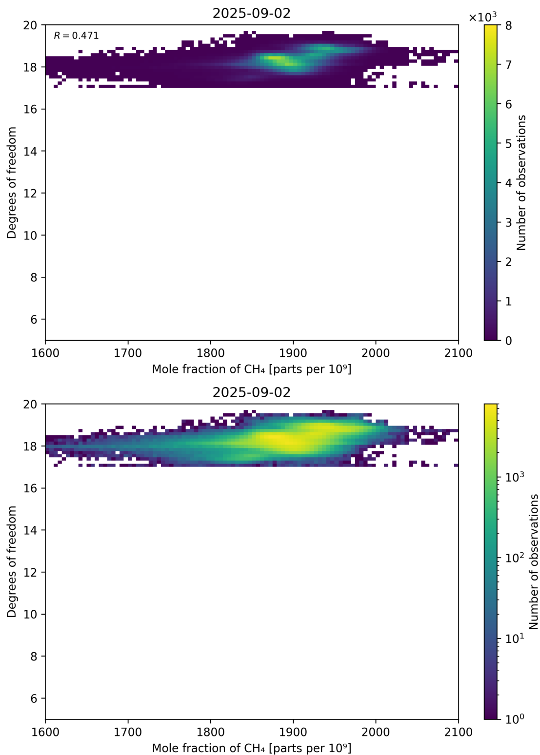
Figure 72: Scatter density plot of “Mole fraction of CH 4 ” against “Degrees of freedom” for 2025-09-01 to 2025-09-03.
