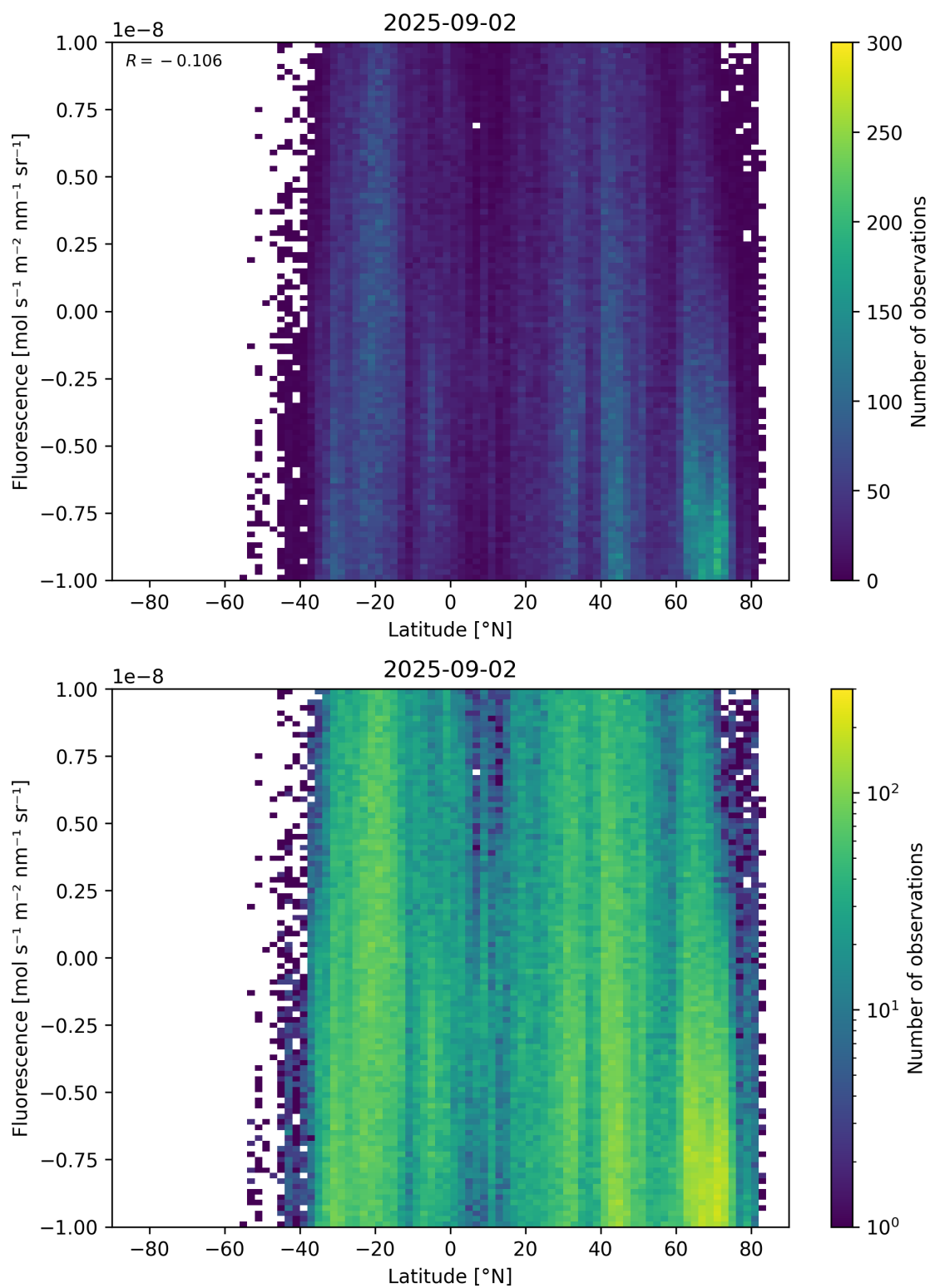
Figure 56: Scatter density plot of “Latitude” against “Fluorescence” for 2025-09-01 to 2025-09-03.
