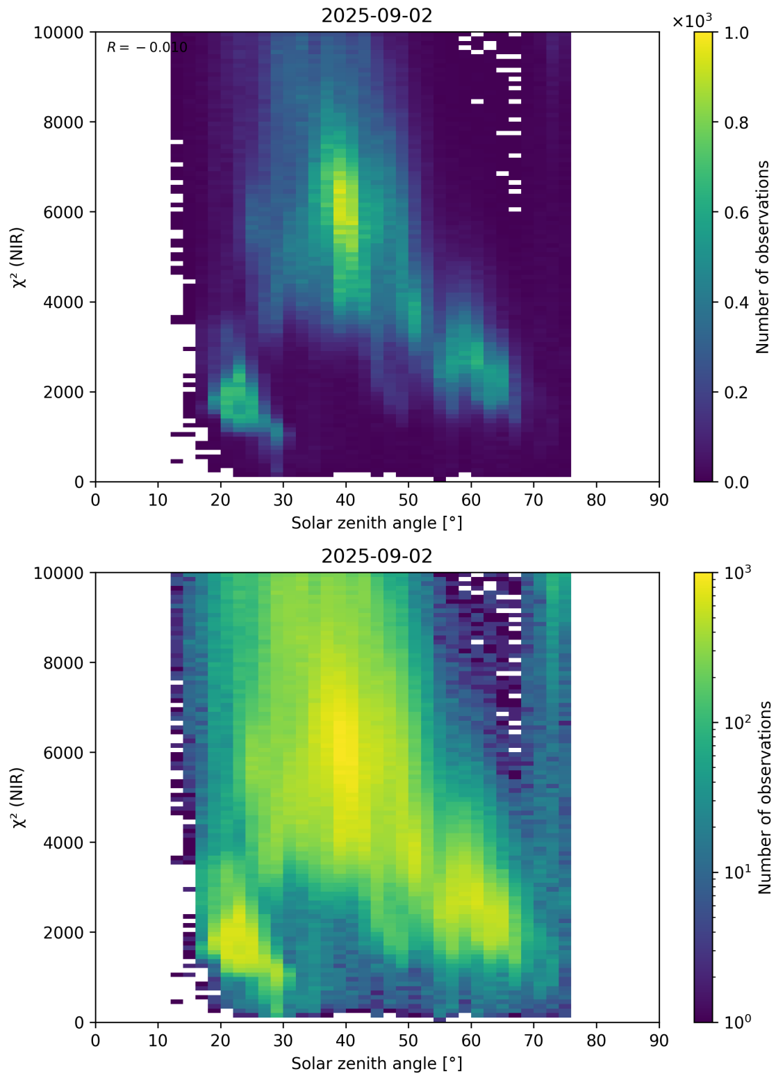
Figure 94: Scatter density plot of “Solar zenith angle” against “ \chi^2 (NIR)” for 2025-09-01 to 2025-09-03.
