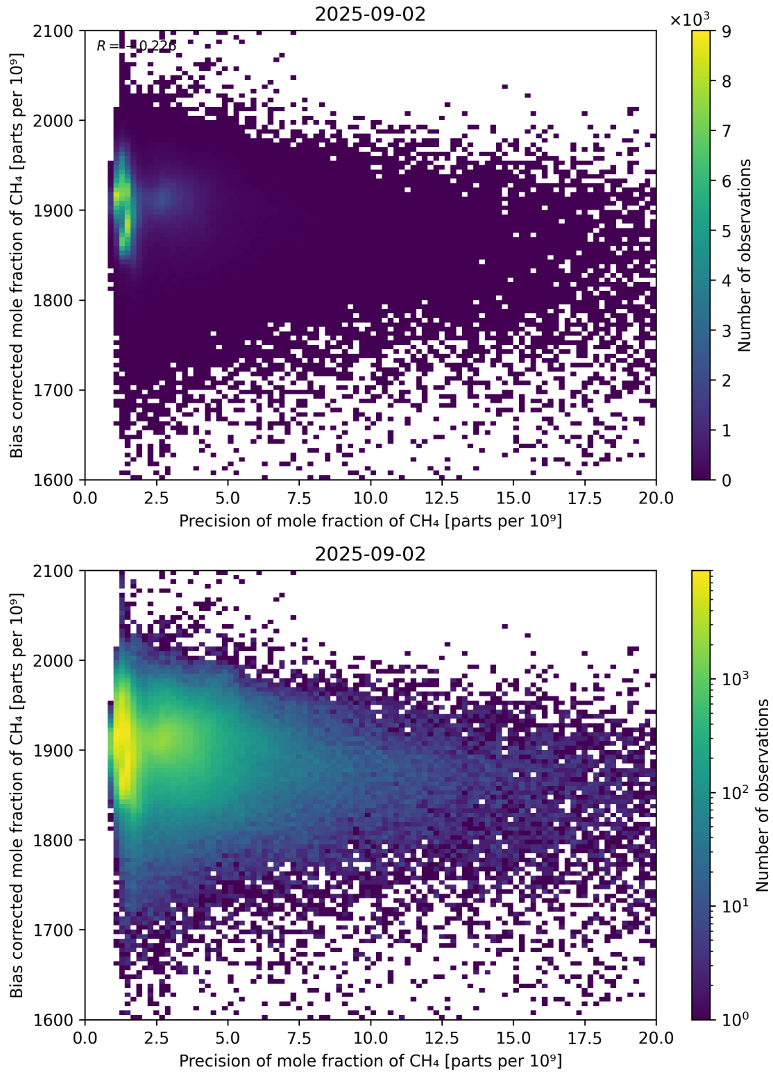
Figure 82: Scatter density plot of “Precision of mole fraction of CH 4 ” against “Bias corrected mole fraction of CH 4 ” for 2025-09-01 to 2025-09-03.
