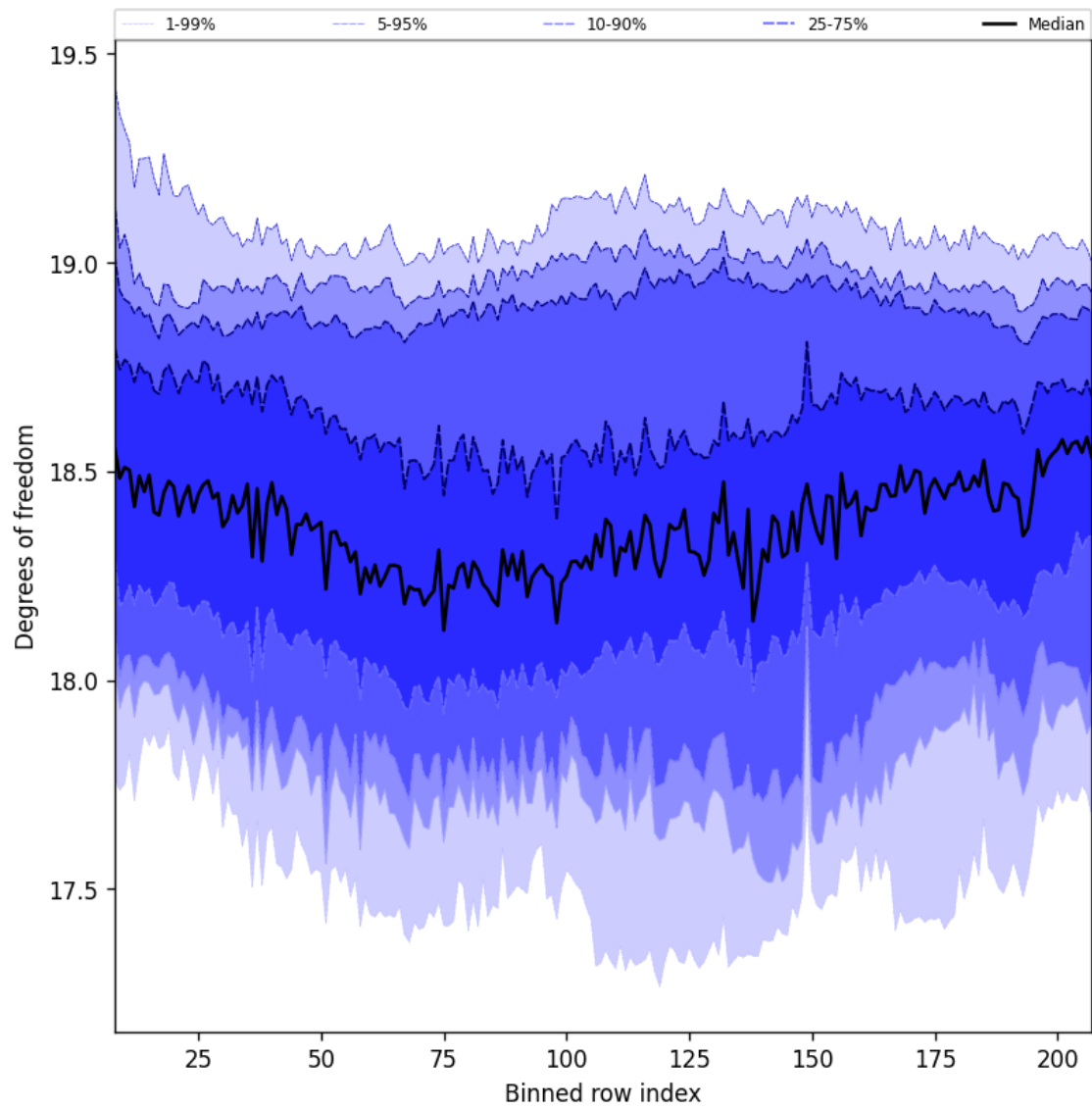
Figure 41: Along track statistics of “Degrees of freedom” for 2025-09-01 to 2025-09-03
