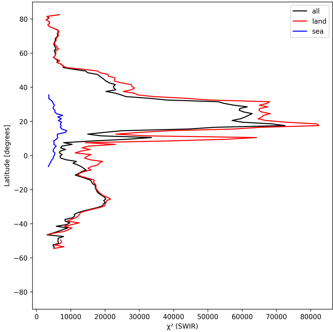
Figure 17: Zonal average of “ \chi^2 (SWIR)” for 2025-09-01 to 2025-09-03.
