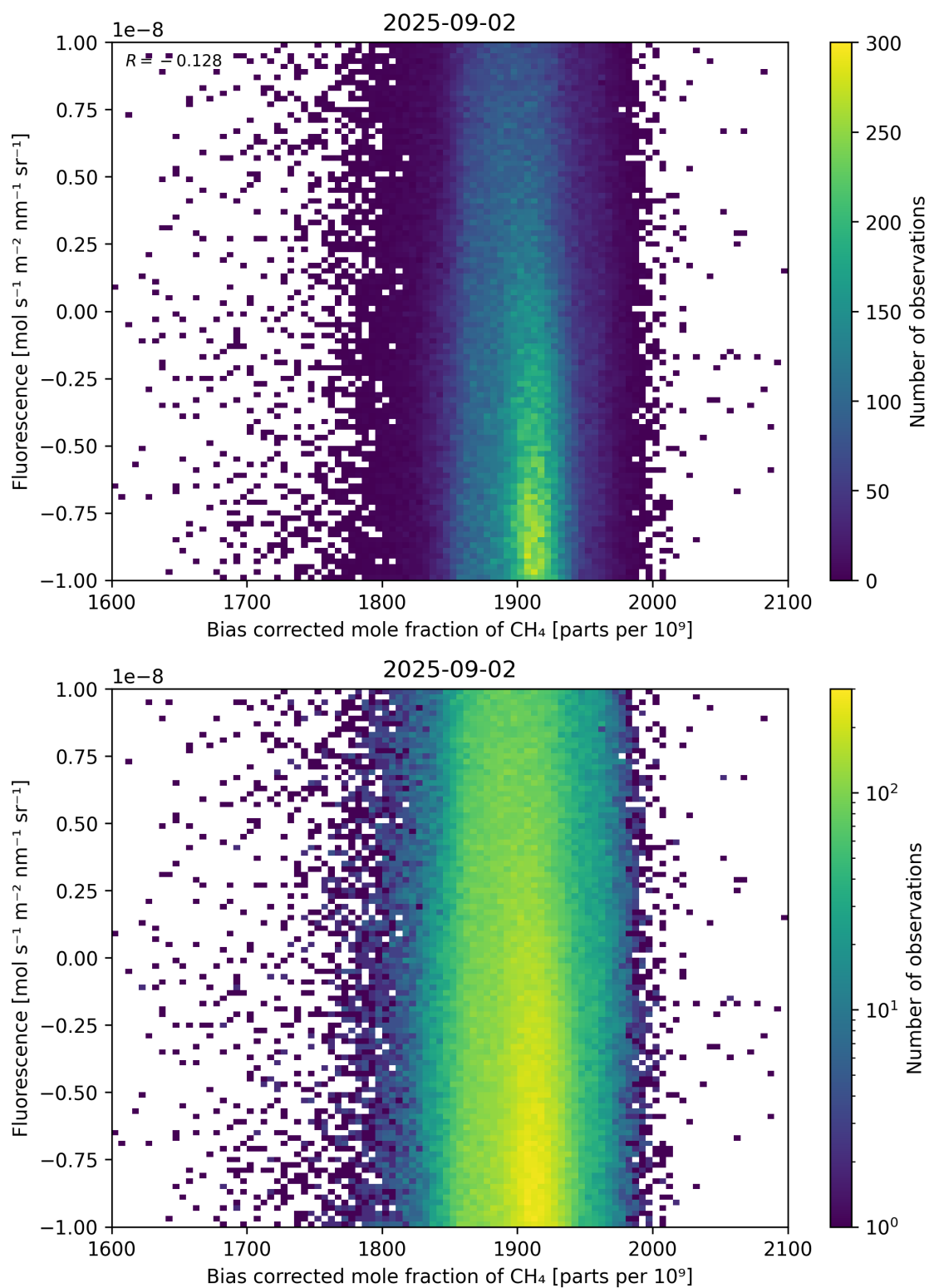
Figure 66: Scatter density plot of “Bias corrected mole fraction of \text{CH}_4 ” against “Fluorescence” for 2025-09-01 to 2025-09-03.
