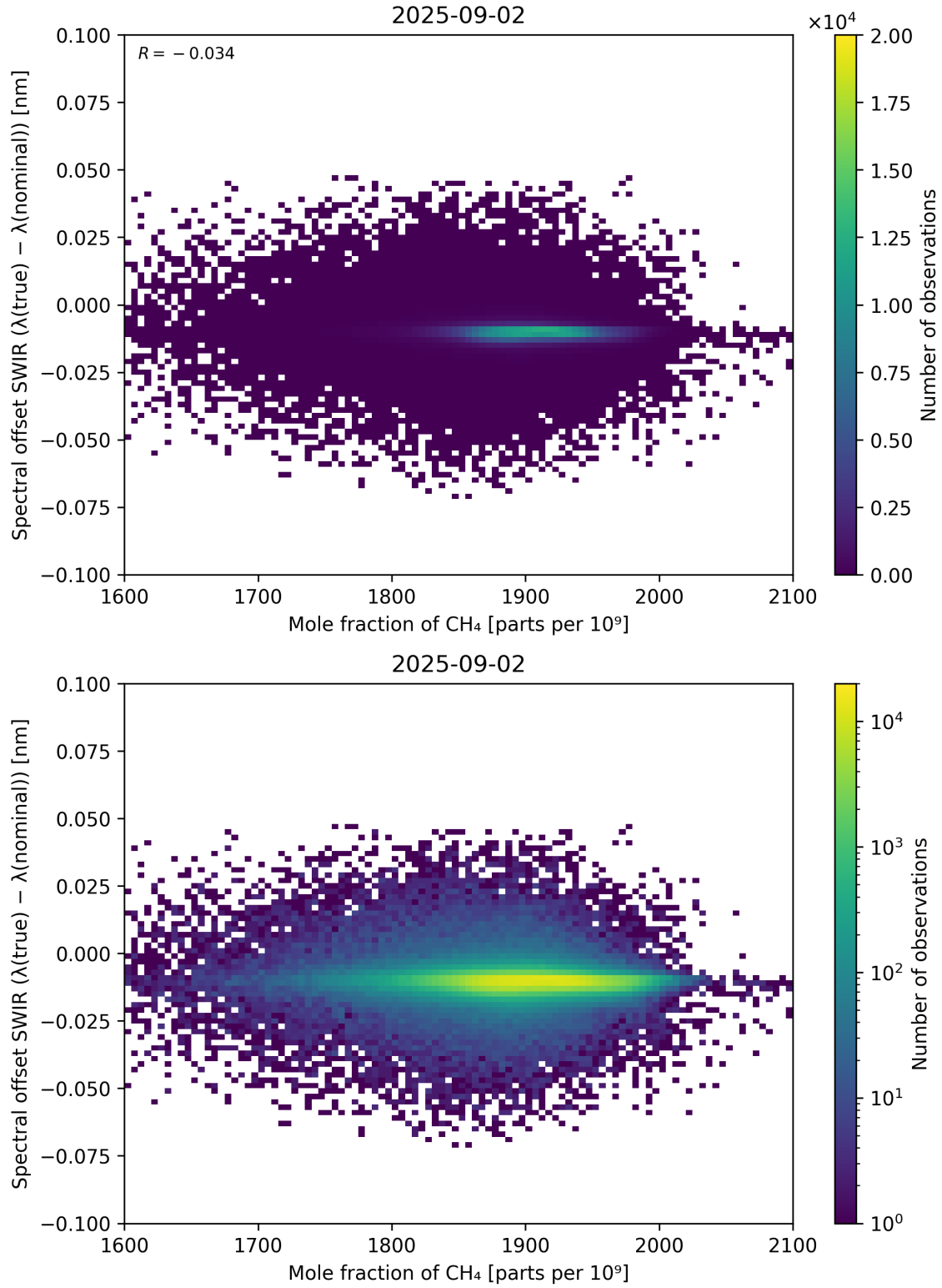
Figure 86: Scatter density plot of “Mole fraction of CH 4 ” against “Spectral offset SWIR ( \lambda_{\text{true}} - \lambda_{\text{nominal}} )” for 2025-09-01 to 2025-09-03.
