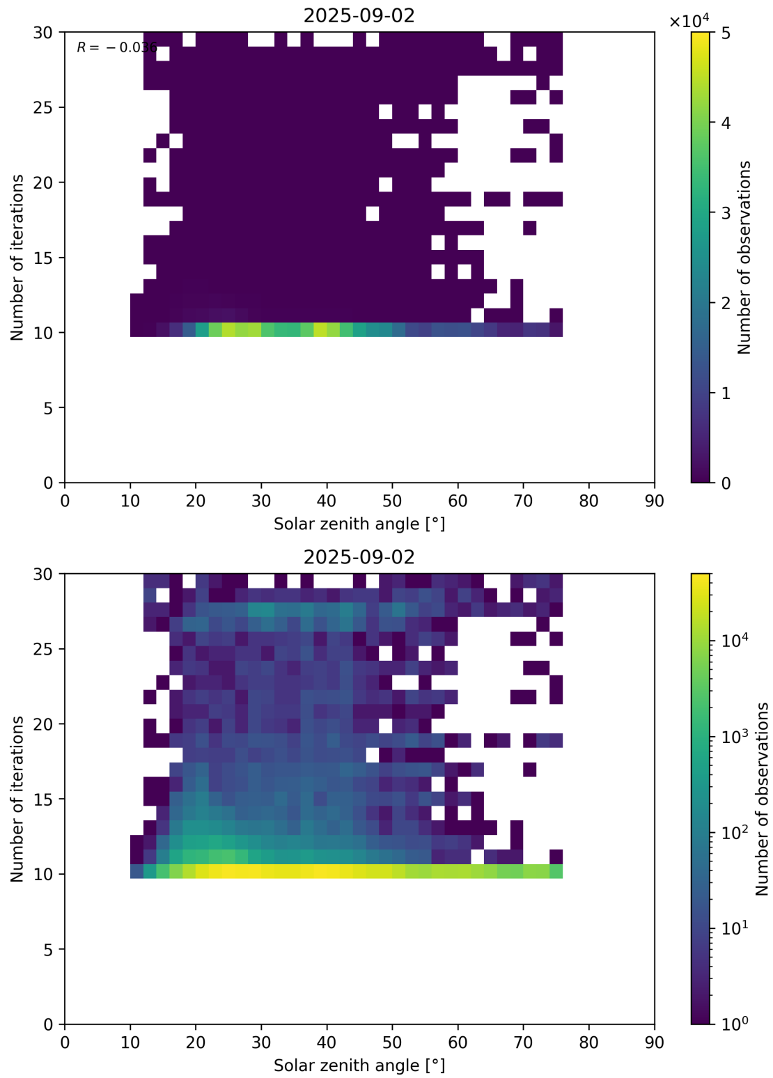
Figure 102: Scatter density plot of “Solar zenith angle” against “Number of iterations” for 2025-09-01 to 2025-09-03.
