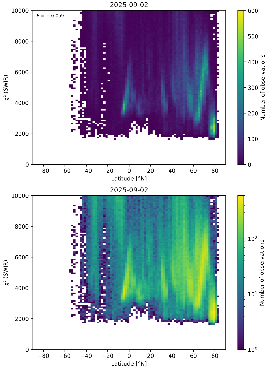
Figure 54: Scatter density plot of “Latitude” against “ \chi^2 (SWIR)” for 2025-09-01 to 2025-09-03.
