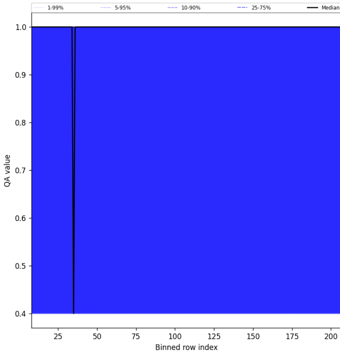
Figure 33: Along track statistics of “QA value” for 2025-09-01 to 2025-09-03
