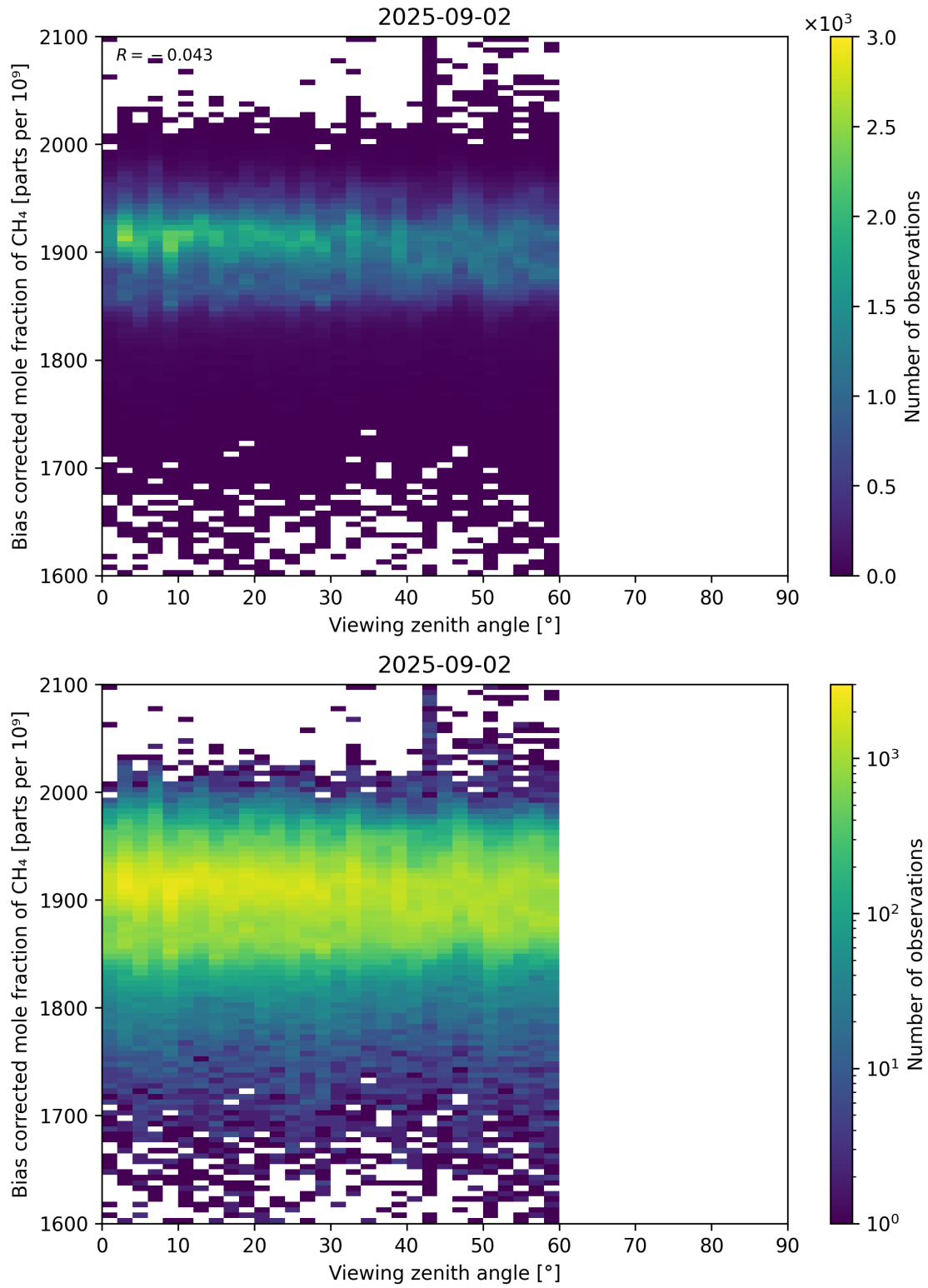
Figure 111: Scatter density plot of “Viewing zenith angle” against “Bias corrected mole fraction of CH 4 ” for 2025-09-01 to 2025-09-03.
