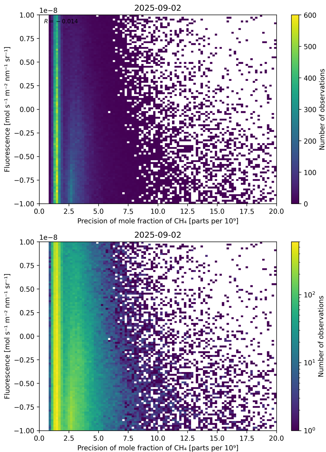
Figure 81: Scatter density plot of “Precision of mole fraction of \text{CH}_4 ” against “Fluorescence” for 2025-09-01 to 2025-09-03.
