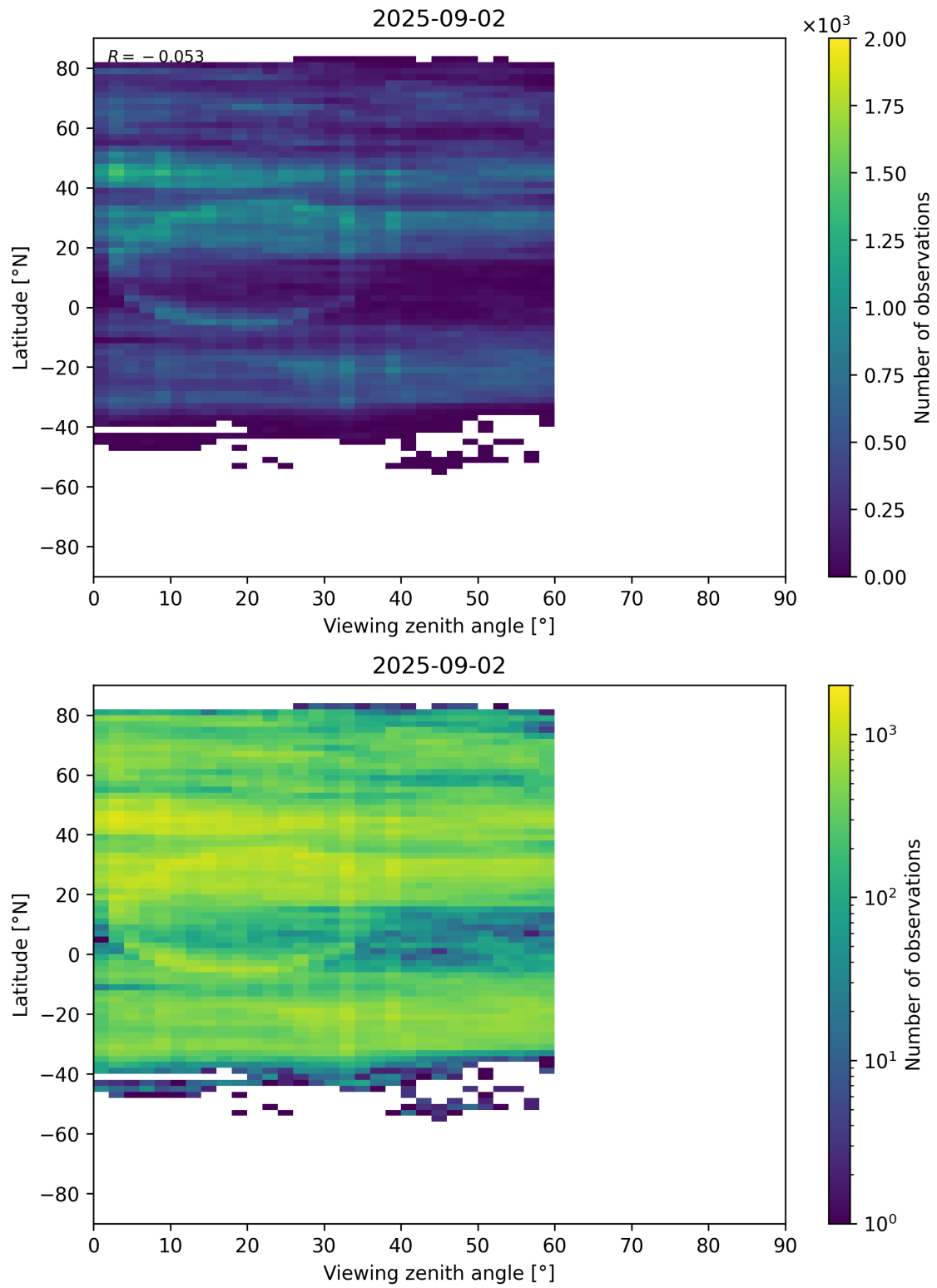
Figure 109: Scatter density plot of “Viewing zenith angle” against “Latitude” for 2025-09-01 to 2025-09-03.
