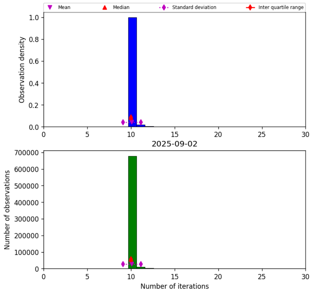
Figure 31: Histogram of “Number of iterations” for 2025-09-01 to 2025-09-03
