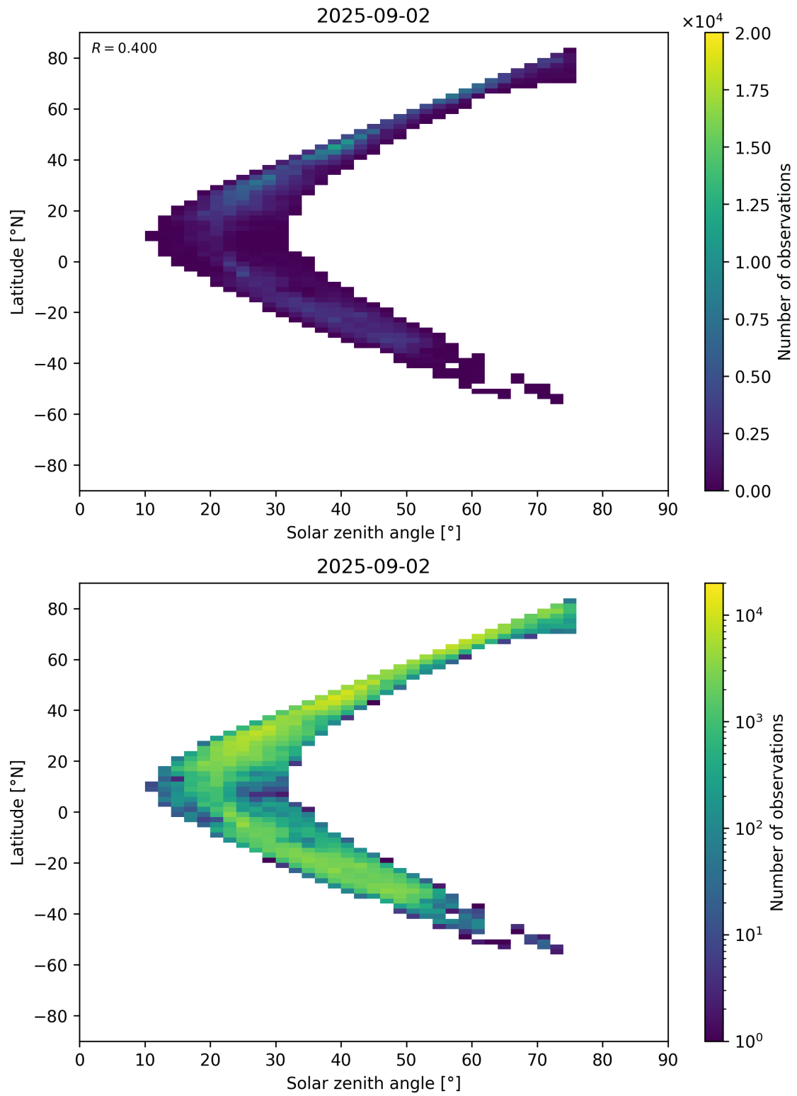
Figure 98: Scatter density plot of “Solar zenith angle” against “Latitude” for 2025-09-01 to 2025-09-03.
