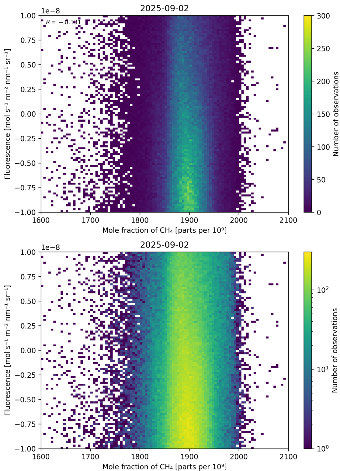
Figure 73: Scatter density plot of “Mole fraction of \text{CH}_4 ” against “Fluorescence” for 2025-09-01 to 2025-09-03.
