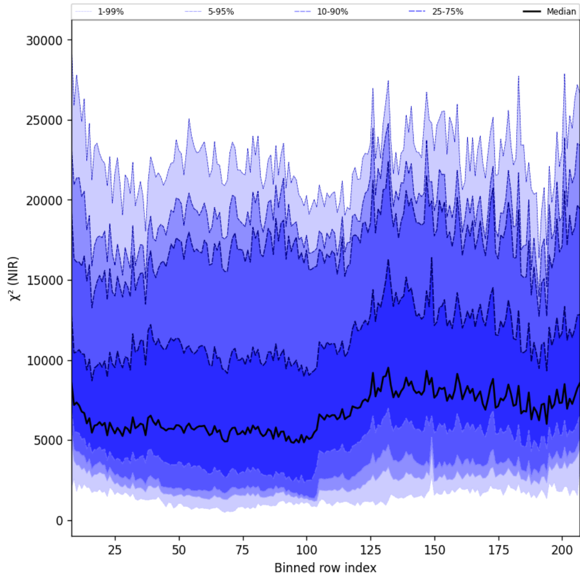
Figure 40: Along track statistics of “ \chi^2 (NIR)” for 2025-09-01 to 2025-09-03
