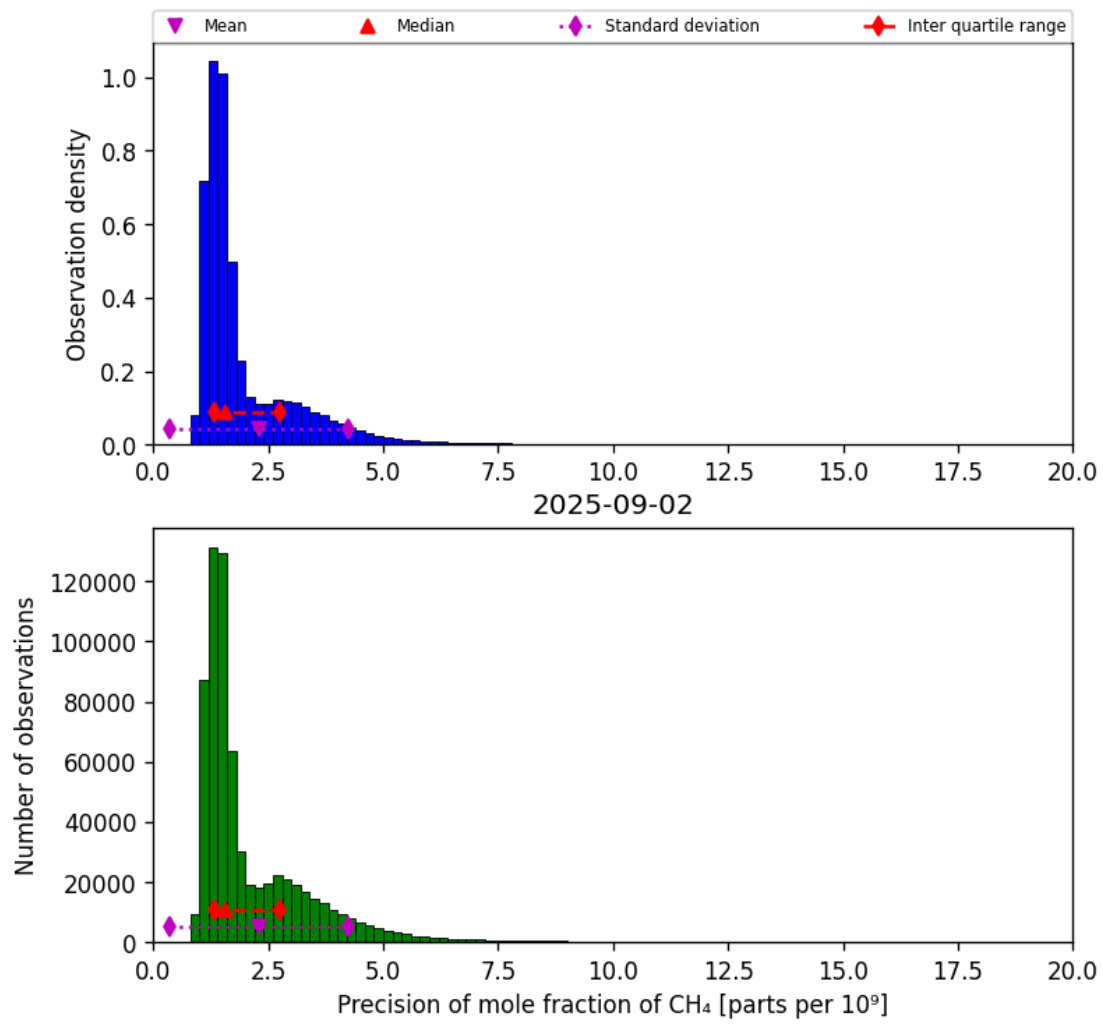
Figure 24: Histogram of “Precision of mole fraction of CH 4 ” for 2025-09-01 to 2025-09-03
