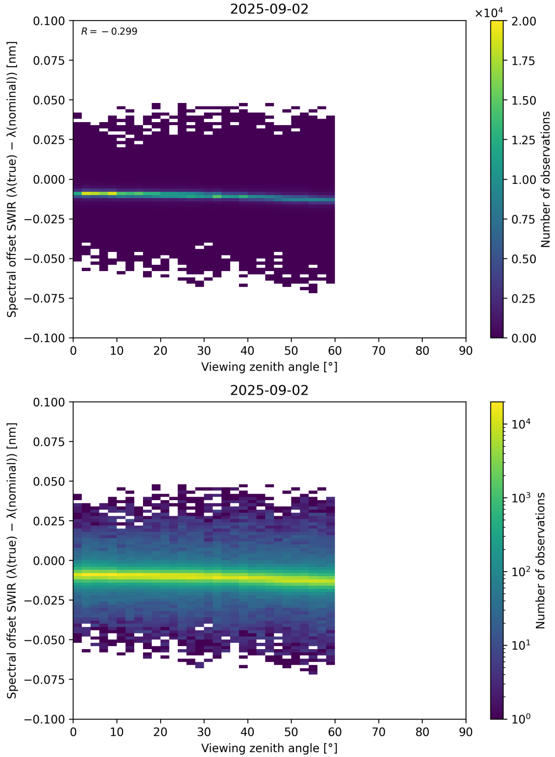
Figure 116: Scatter density plot of “Viewing zenith angle” against “Spectral offset SWIR ( \lambda_{\text{true}} - \lambda_{\text{nominal}} )” for 2025-09-01 to 2025-09-03.
