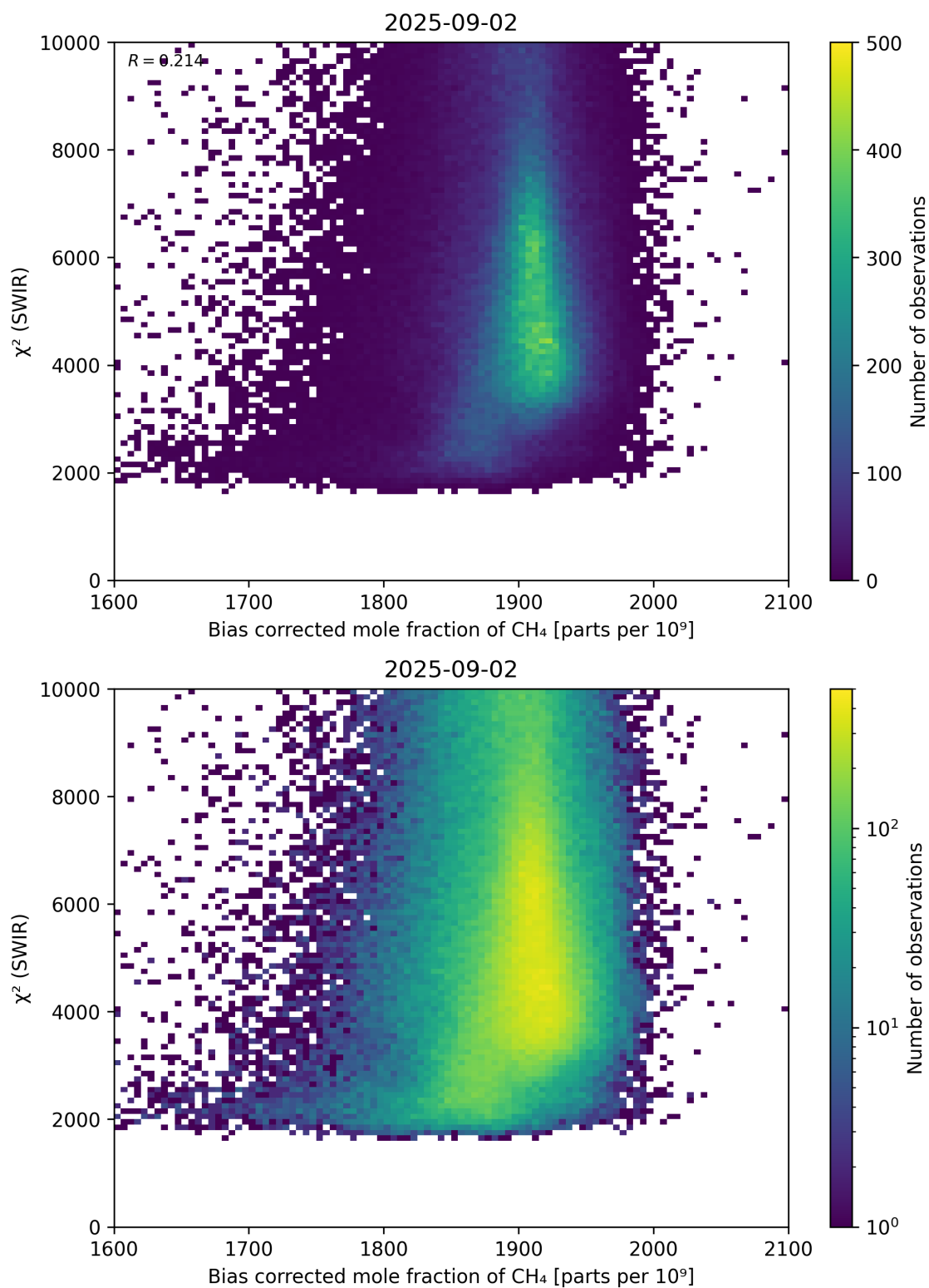
Figure 64: Scatter density plot of “Bias corrected mole fraction of \text{CH}_4 ” against “ \chi^2 (SWIR)” for 2025-09-01 to 2025-09-03.
