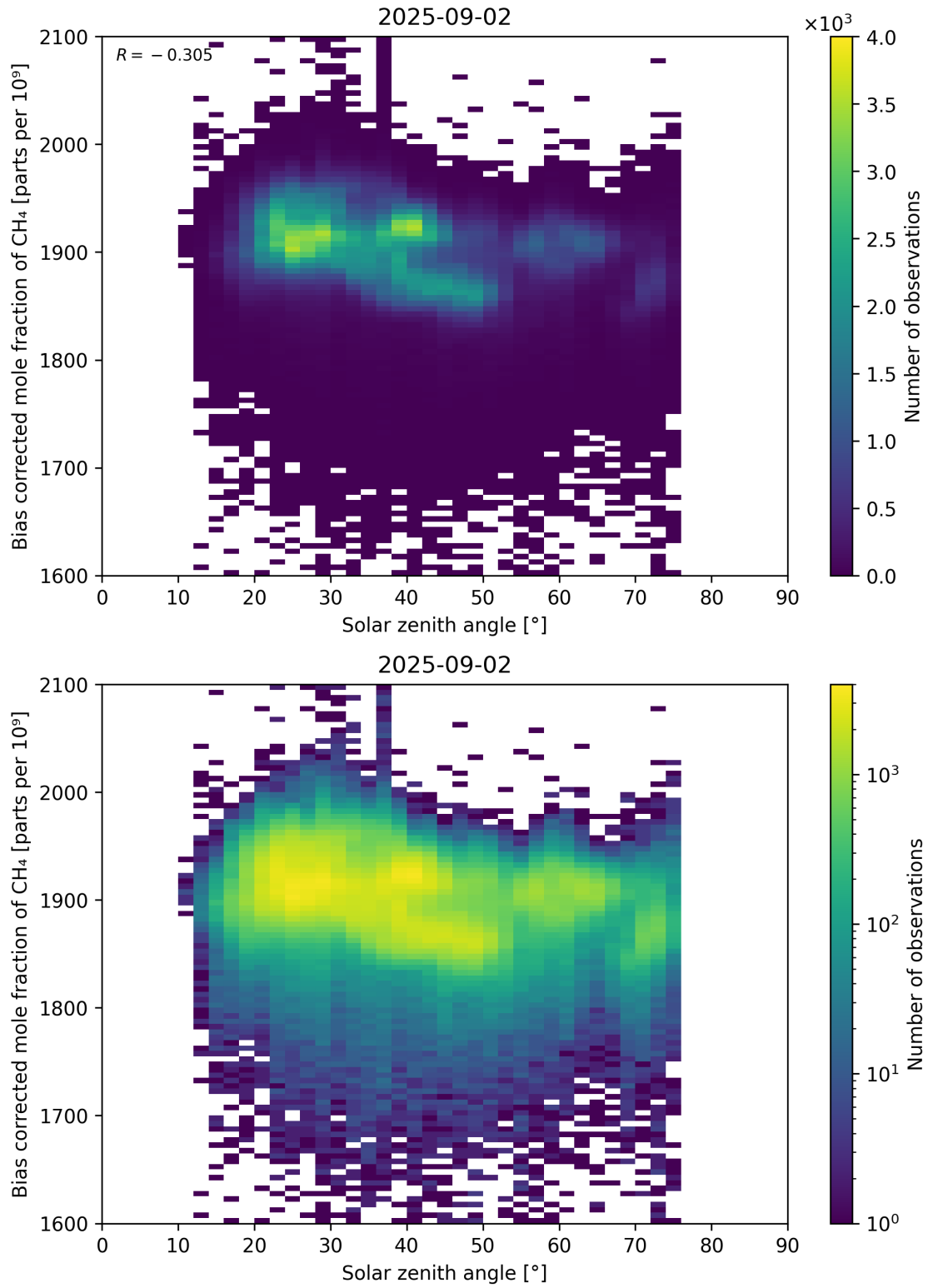
Figure 100: Scatter density plot of “Solar zenith angle” against “Bias corrected mole fraction of \text{CH}_4 ” for 2025-09-01 to 2025-09-03.
