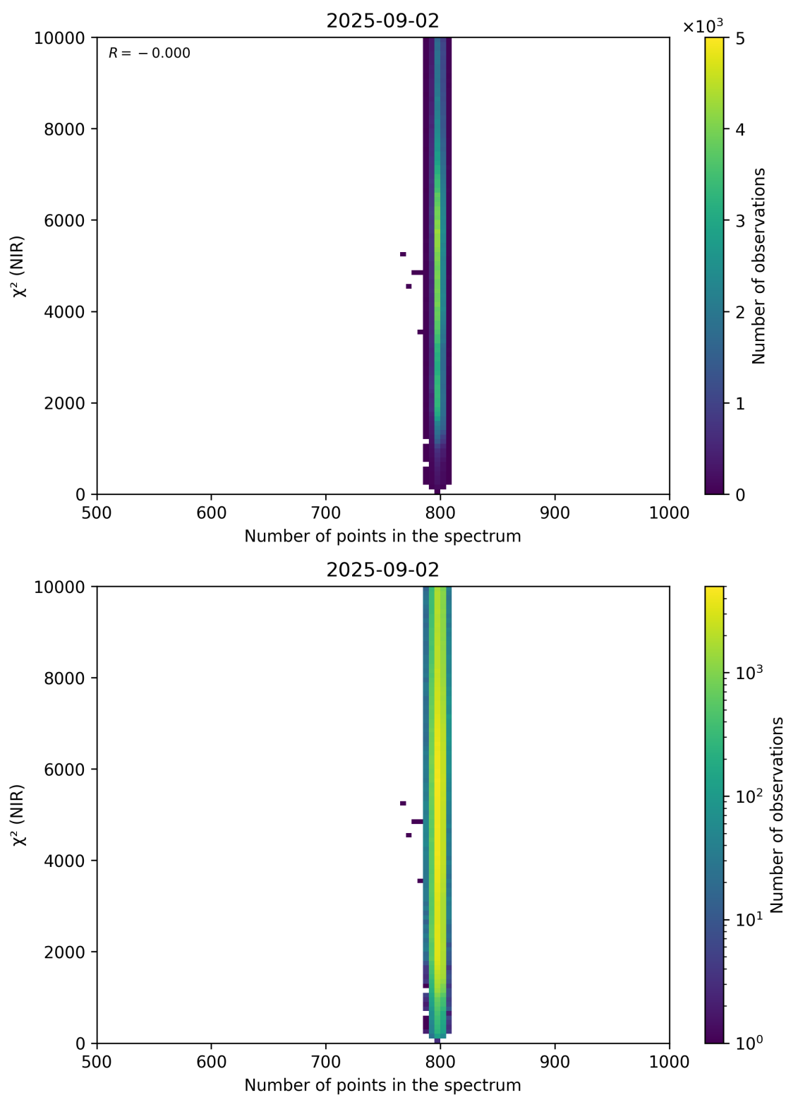
Figure 88: Scatter density plot of “Number of points in the spectrum” against “ \chi^2 (NIR)” for 2025-09-01 to 2025-09-03.
