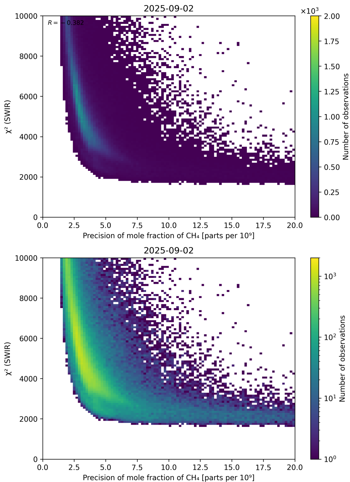
Figure 79: Scatter density plot of “Precision of mole fraction of \text{CH}_4 ” against “ \chi^2 (SWIR)” for 2025-09-01 to 2025-09-03.
