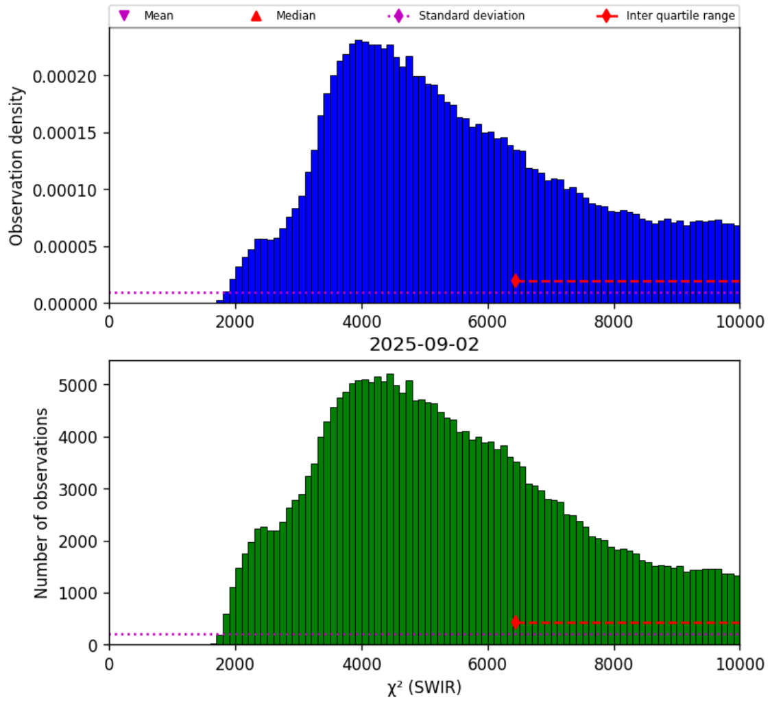
Figure 28: Histogram of “ \chi^2 (SWIR)” for 2025-09-01 to 2025-09-03
