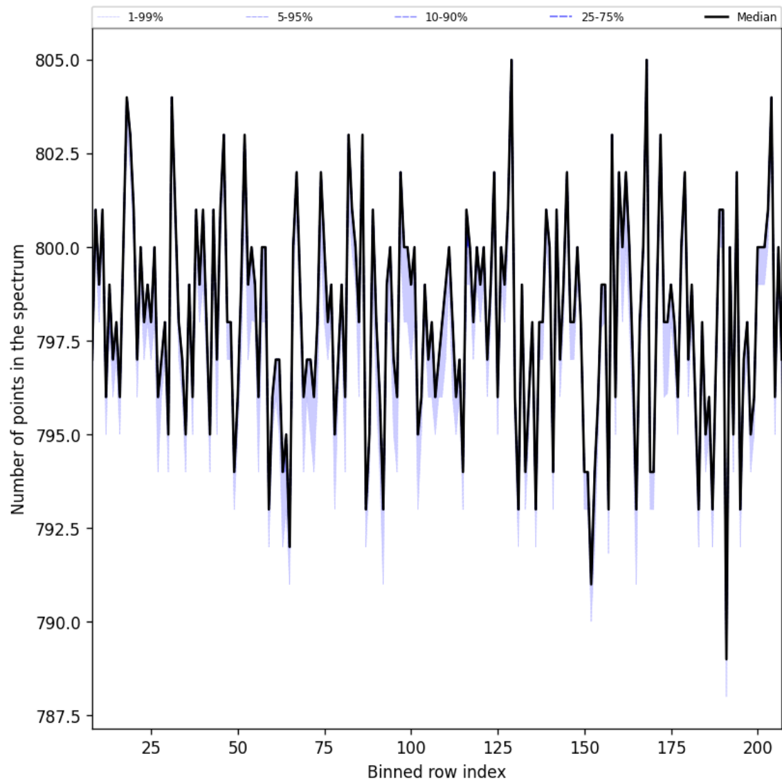
Figure 37: Along track statistics of “Number of points in the spectrum” for 2025-09-01 to 2025-09-03
