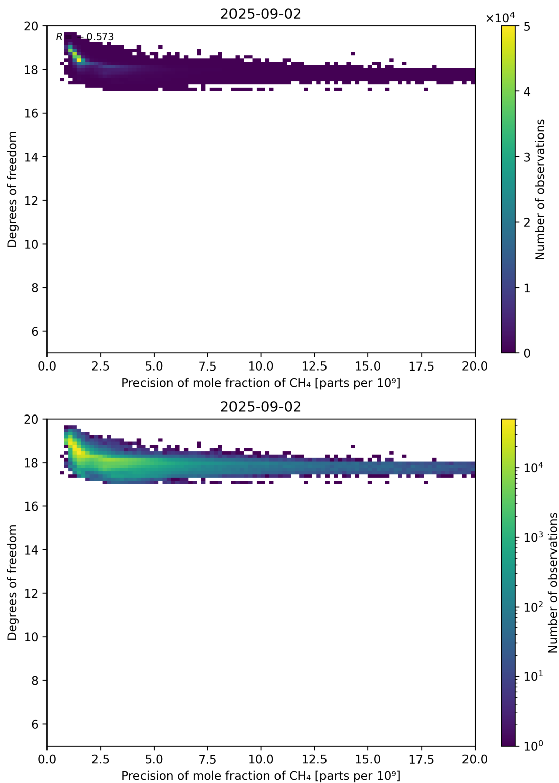
Figure 80: Scatter density plot of “Precision of mole fraction of CH 4 ” against “Degrees of freedom” for 2025-09-01 to 2025-09-03.
