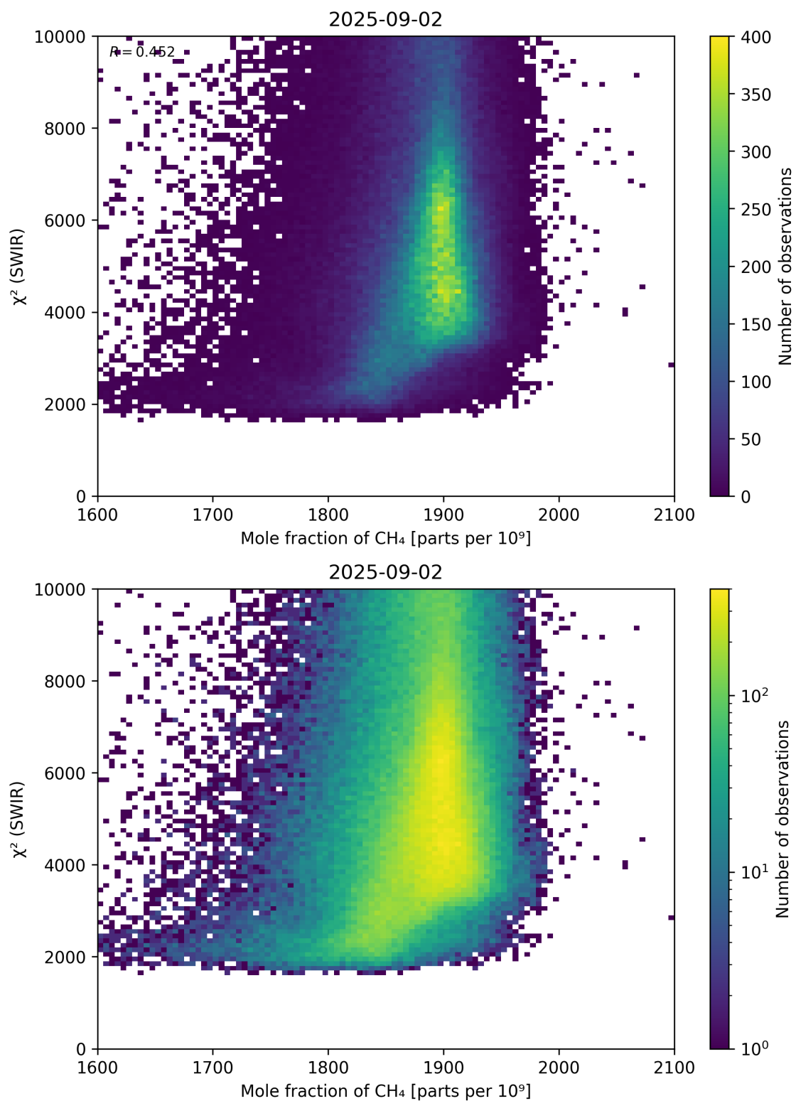
Figure 71: Scatter density plot of “Mole fraction of \text{CH}_4 ” against “ \chi^2 (SWIR)” for 2025-09-01 to 2025-09-03.
