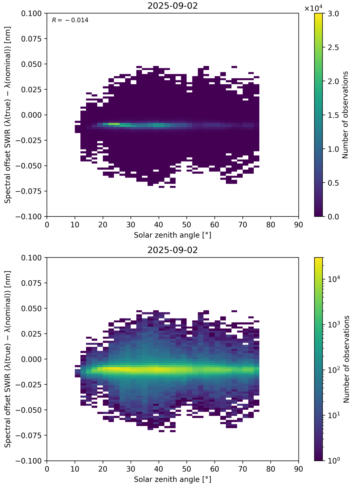
Figure 104: Scatter density plot of “Solar zenith angle” against “Spectral offset SWIR ( \lambda_{\text{true}} - \lambda_{\text{nominal}} )” for 2025-09-01 to 2025-09-03.
