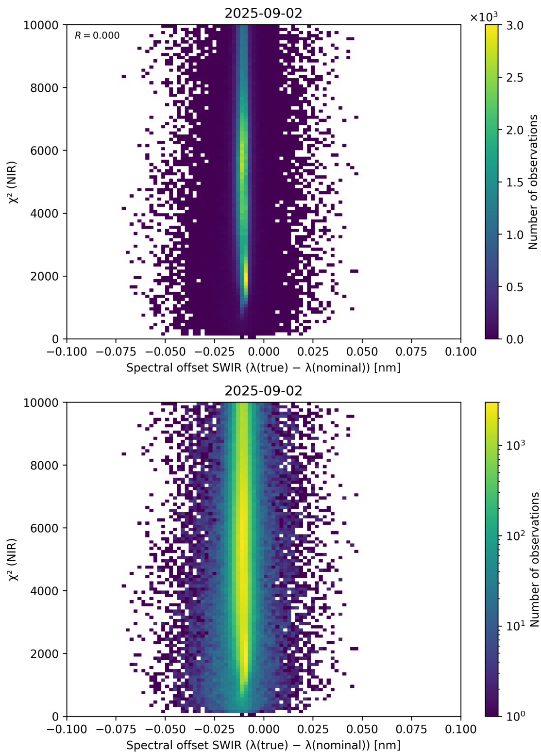
Figure 117: Scatter density plot of “Spectral offset SWIR ( \lambda_{\text{true}} - \lambda_{\text{nominal}} )” against “ \chi^2 (NIR)” for 2025-09-01 to 2025-09-03.
