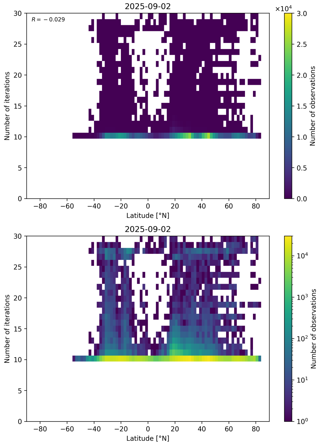
Figure 60: Scatter density plot of “Latitude” against “Number of iterations” for 2025-09-01 to 2025-09-03.
