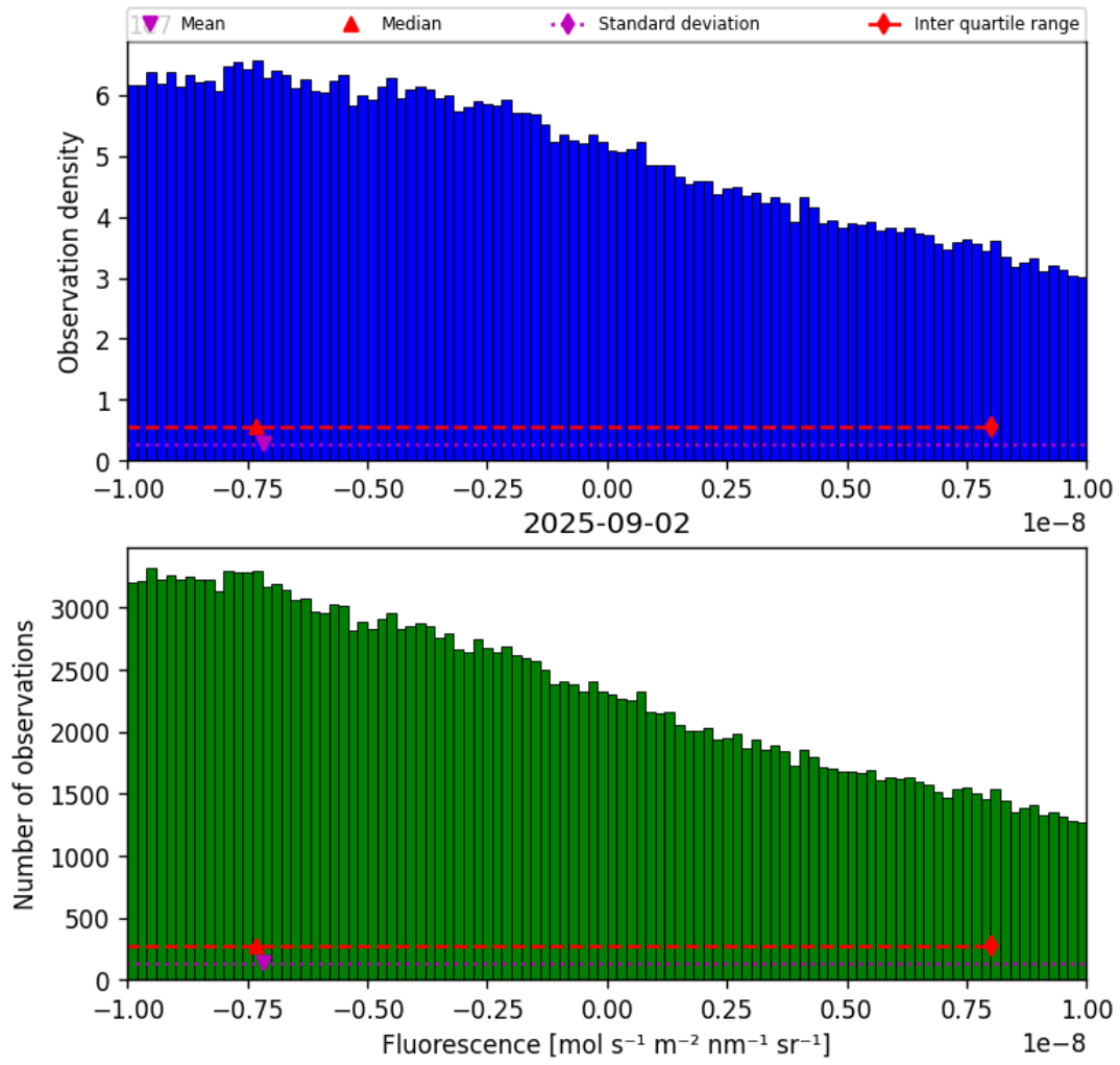
Figure 32: Histogram of “Fluorescence” for 2025-09-01 to 2025-09-03
