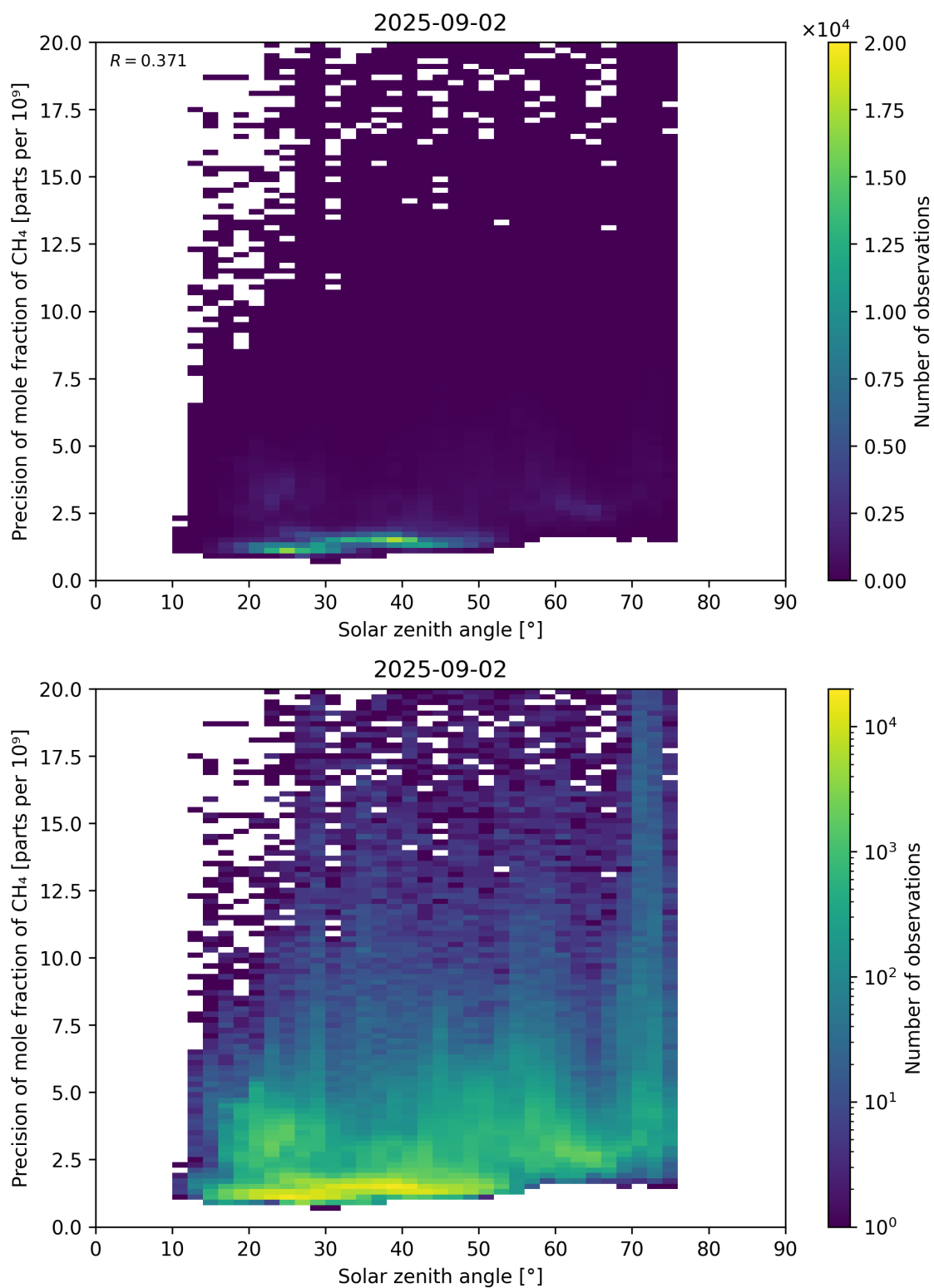
Figure 101: Scatter density plot of “Solar zenith angle” against “Precision of mole fraction of \text{CH}_4 ” for 2025-09-01 to 2025-09-03.
