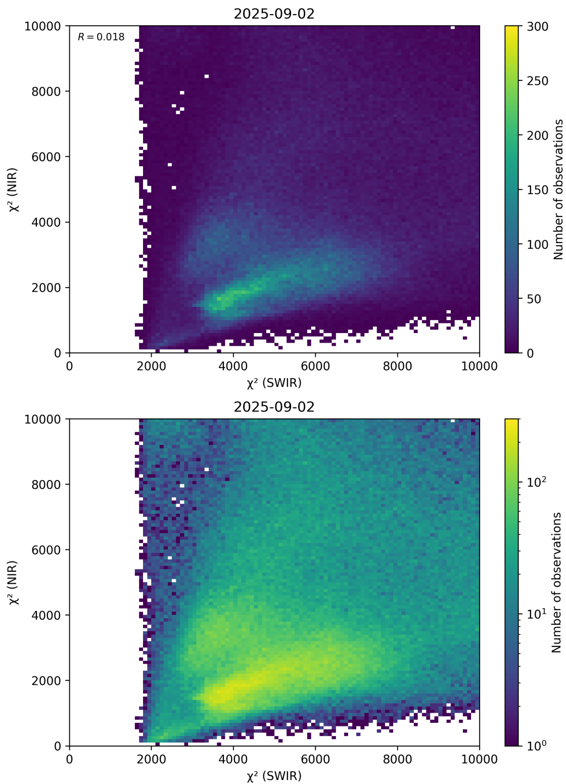
Figure 47: Scatter density plot of “ \chi^2 (SWIR)” against “ \chi^2 (NIR)” for 2025-09-01 to 2025-09-03.
