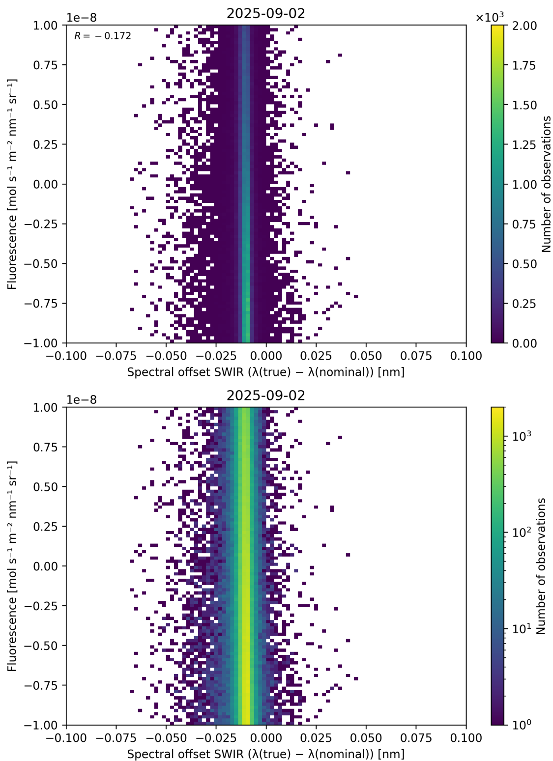
Figure 120: Scatter density plot of “Spectral offset SWIR ( \lambda_{\text{true}} - \lambda_{\text{nominal}} )” against “Fluorescence” for 2025-09-01 to 2025-09-03.
