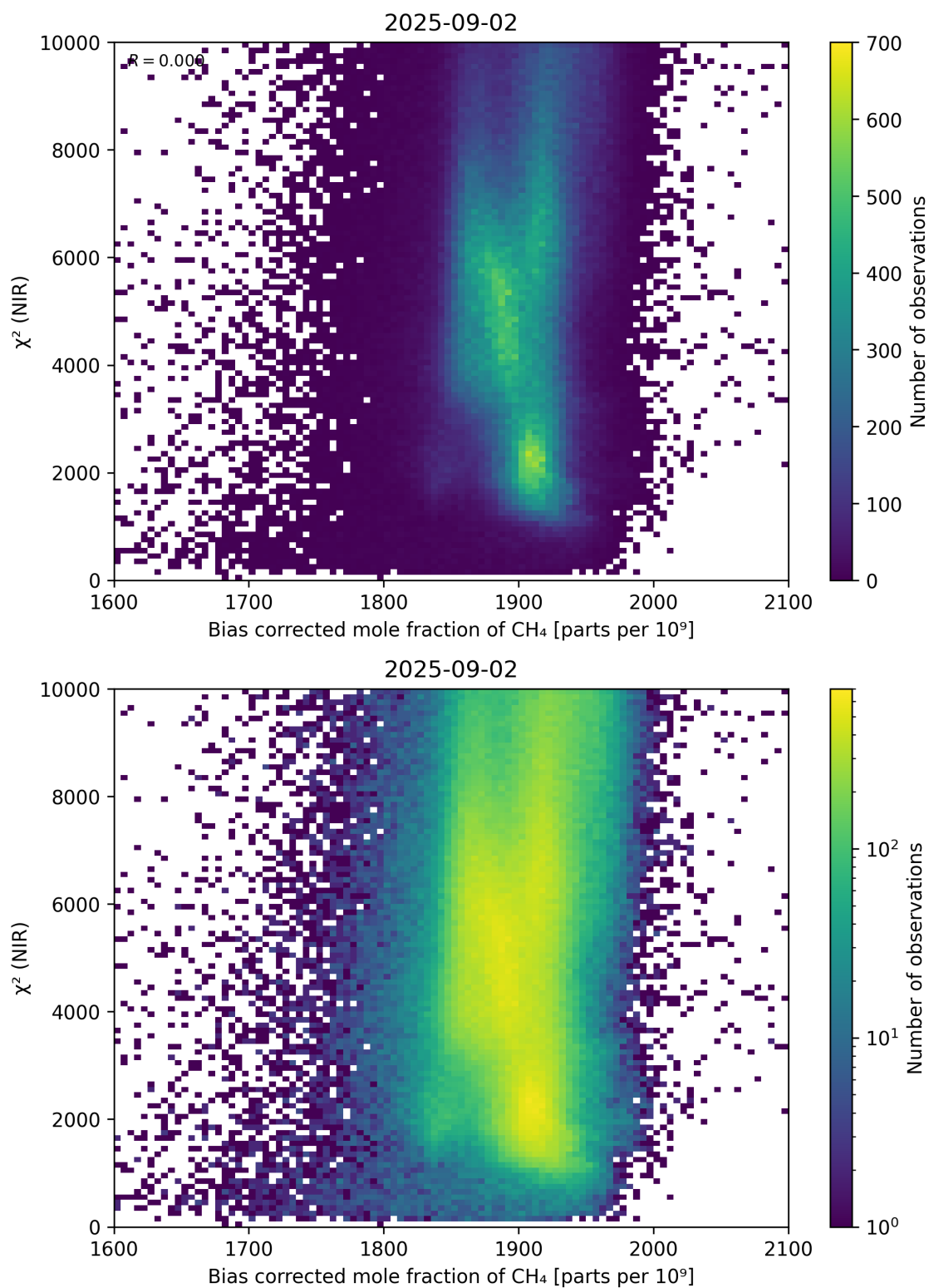
Figure 63: Scatter density plot of “Bias corrected mole fraction of \text{CH}_4 ” against “ \chi^2 (NIR)” for 2025-09-01 to 2025-09-03.
