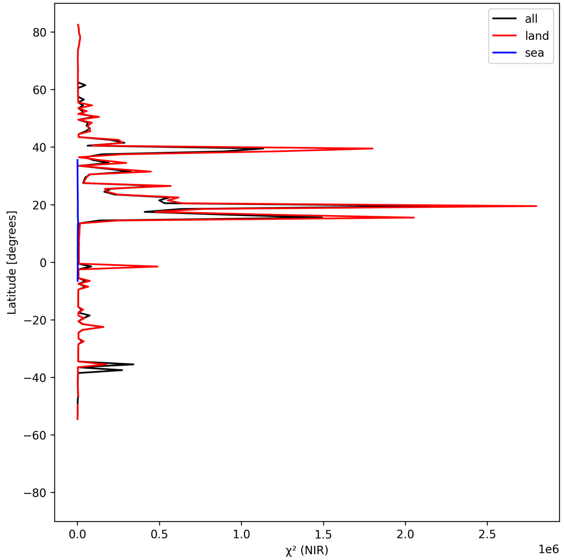
Figure 18: Zonal average of “ \chi^2 (NIR)” for 2025-09-01 to 2025-09-03.
