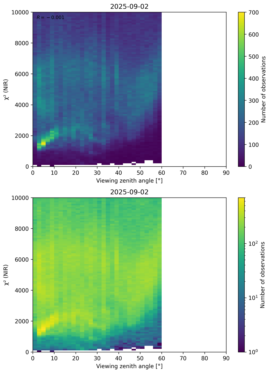
Figure 105: Scatter density plot of “Viewing zenith angle” against “ \chi^2 (NIR)” for 2025-09-01 to 2025-09-03.
