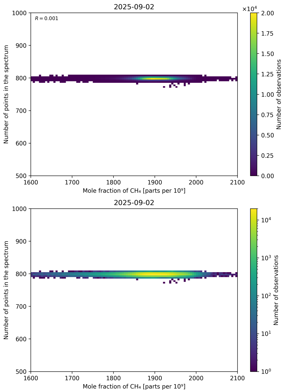
Figure 77: Scatter density plot of “Mole fraction of CH 4 ” against “Number of points in the spectrum” for 2025-09-01 to 2025-09-03.
