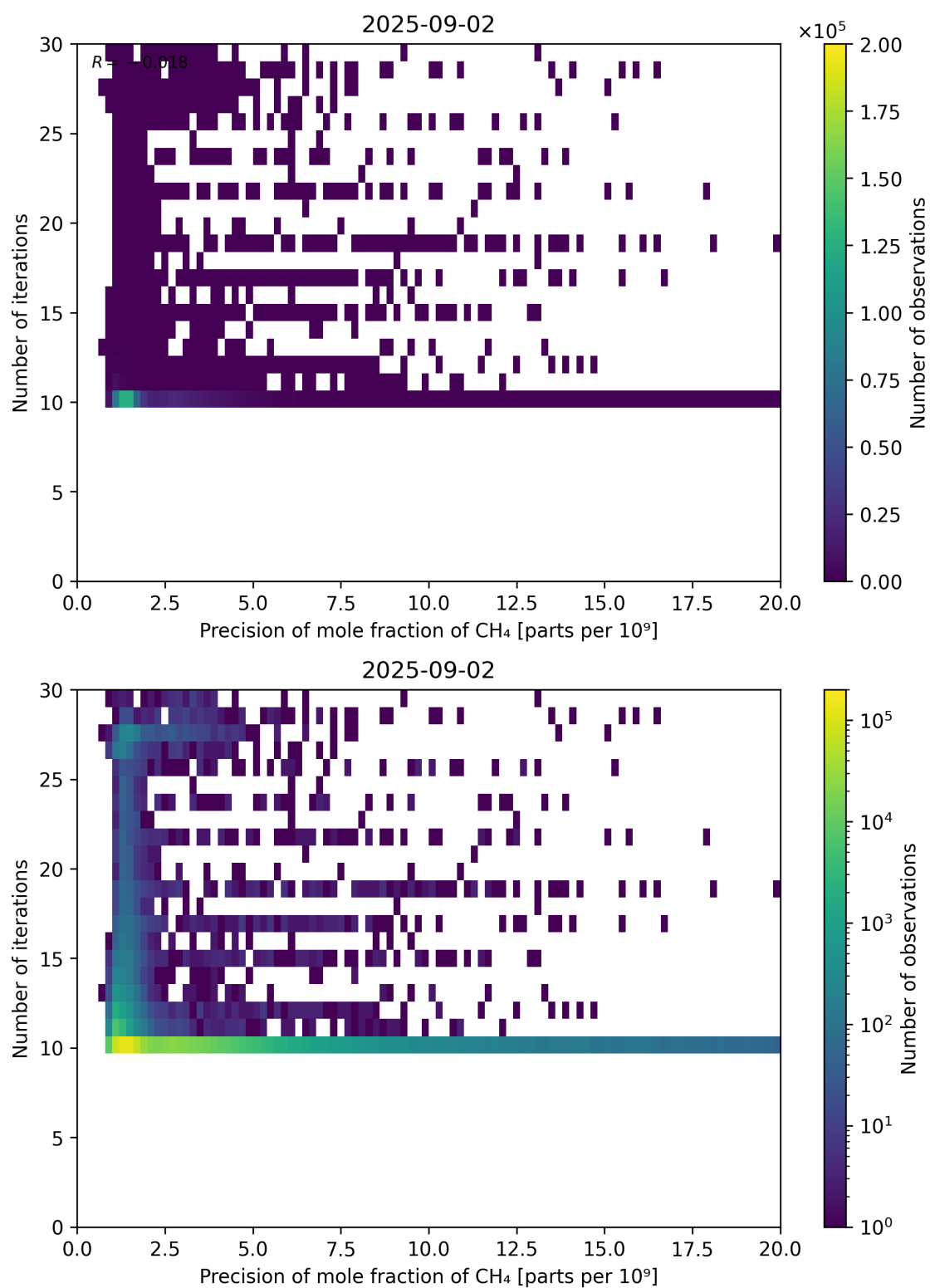
Figure 83: Scatter density plot of “Precision of mole fraction of CH 4 ” against “Number of iterations” for 2025-09-01 to 2025-09-03.
