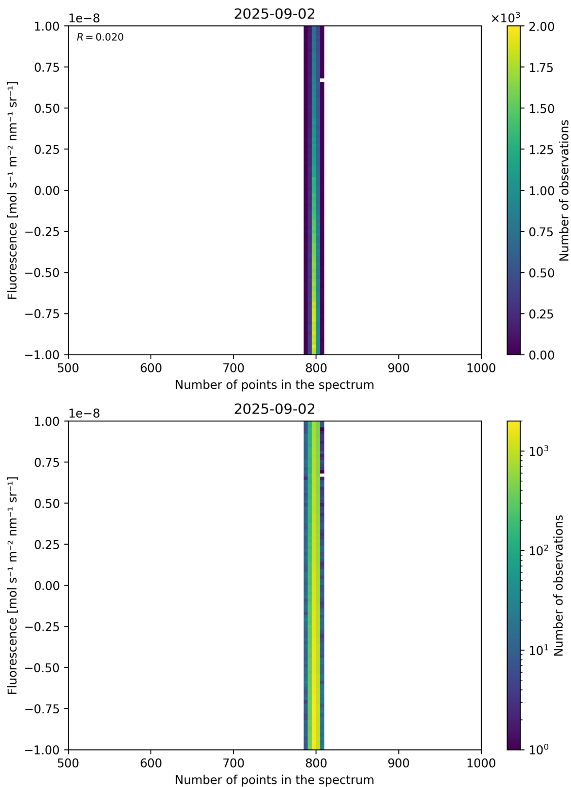
Figure 91: Scatter density plot of “Number of points in the spectrum” against “Fluorescence” for 2025-09-01 to 2025-09-03.
