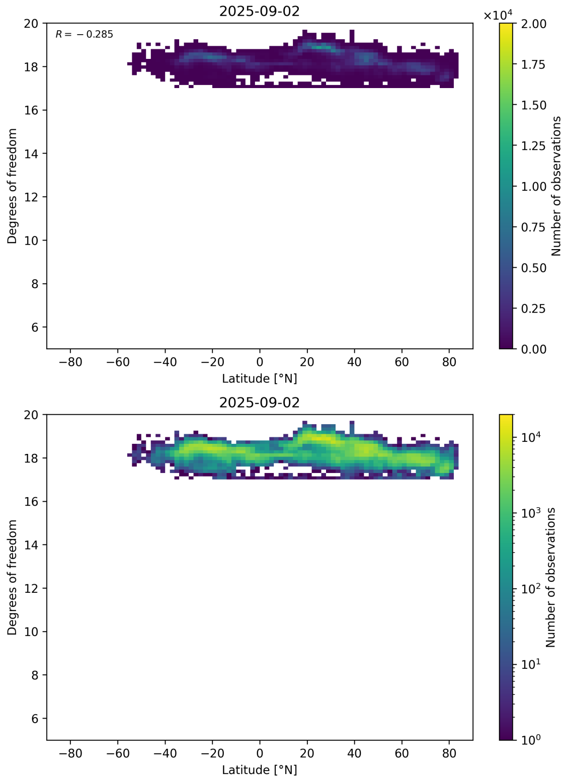
Figure 55: Scatter density plot of “Latitude” against “Degrees of freedom” for 2025-09-01 to 2025-09-03.
