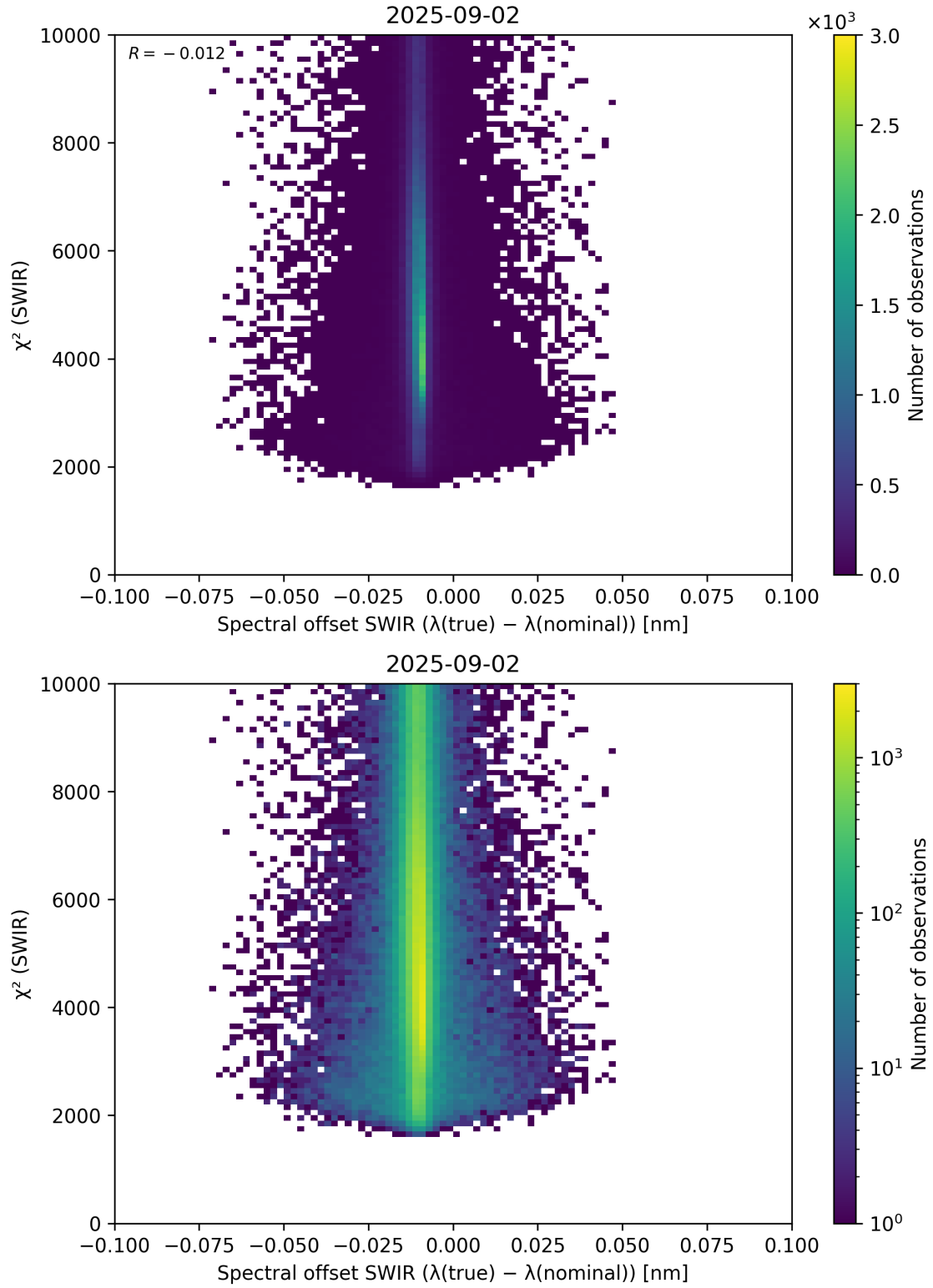
Figure 118: Scatter density plot of “Spectral offset SWIR ( \lambda_{\text{true}} - \lambda_{\text{nominal}} )” against “ \chi^2 (SWIR)” for 2025-09-01 to 2025-09-03.
