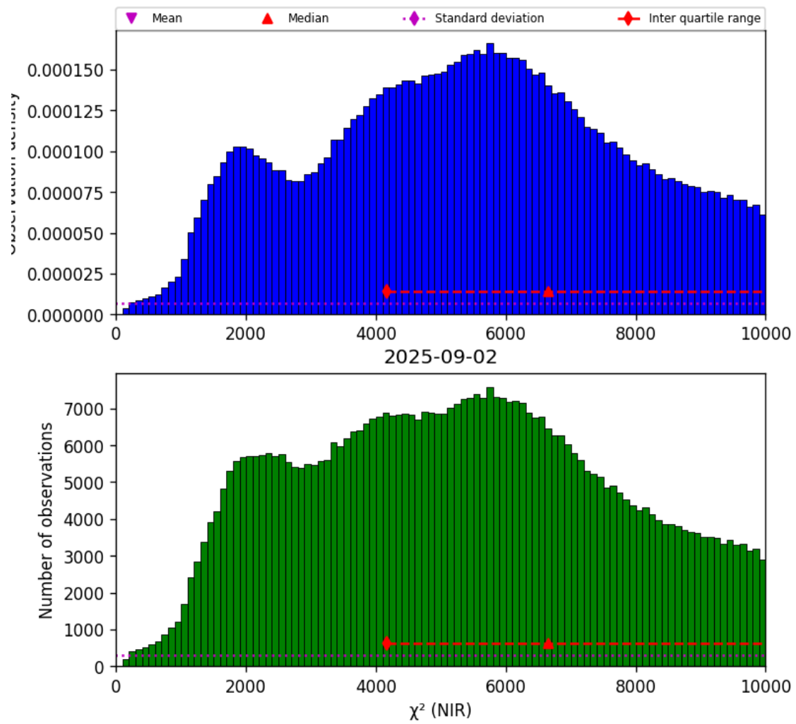
Figure 29: Histogram of “ \chi^2 (NIR)” for 2025-09-01 to 2025-09-03
