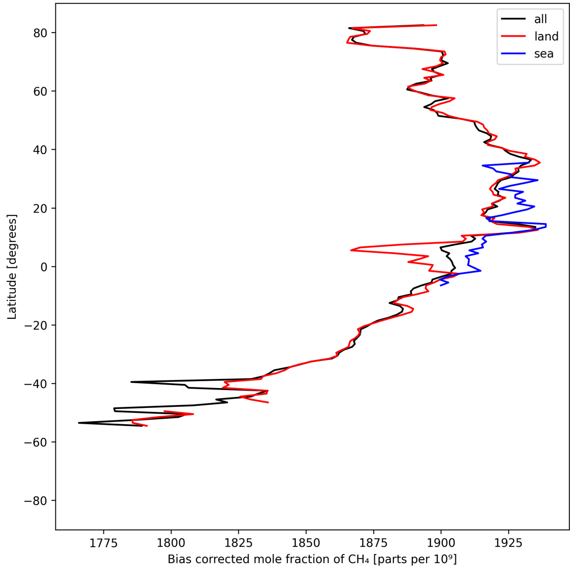
Figure 14: Zonal average of “Bias corrected mole fraction of CH 4 ” for 2025-09-01 to 2025-09-03.
