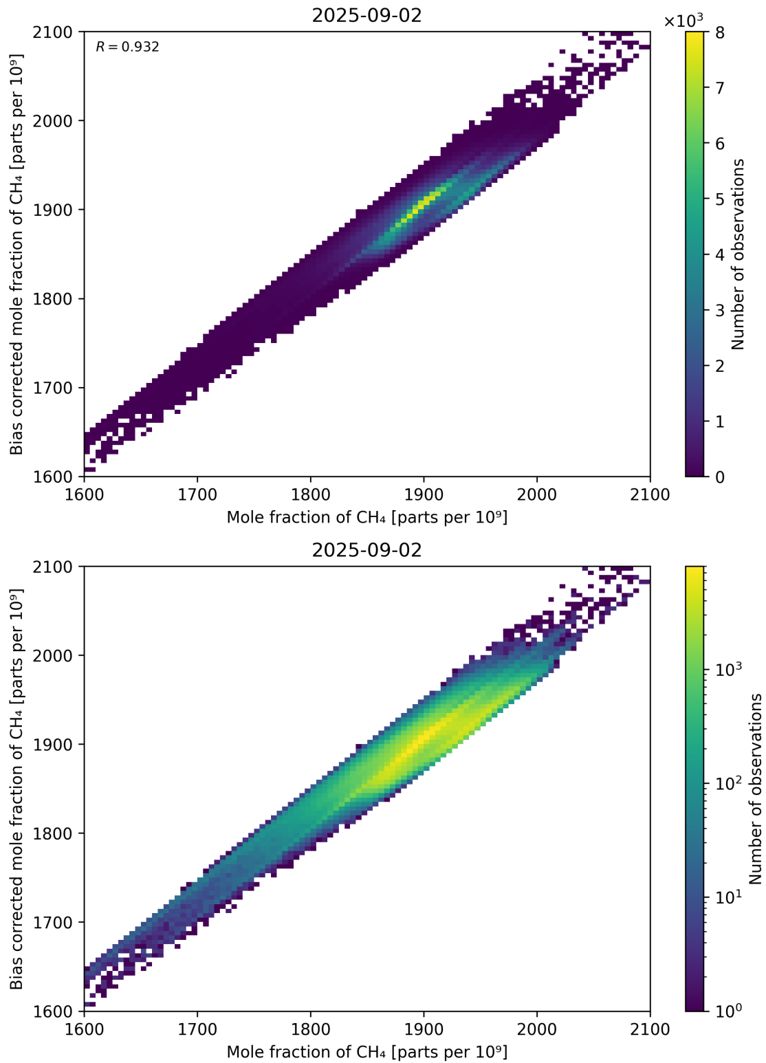
Figure 74: Scatter density plot of “Mole fraction of CH 4 ” against “Bias corrected mole fraction of CH 4 ” for 2025-09-01 to 2025-09-03.
