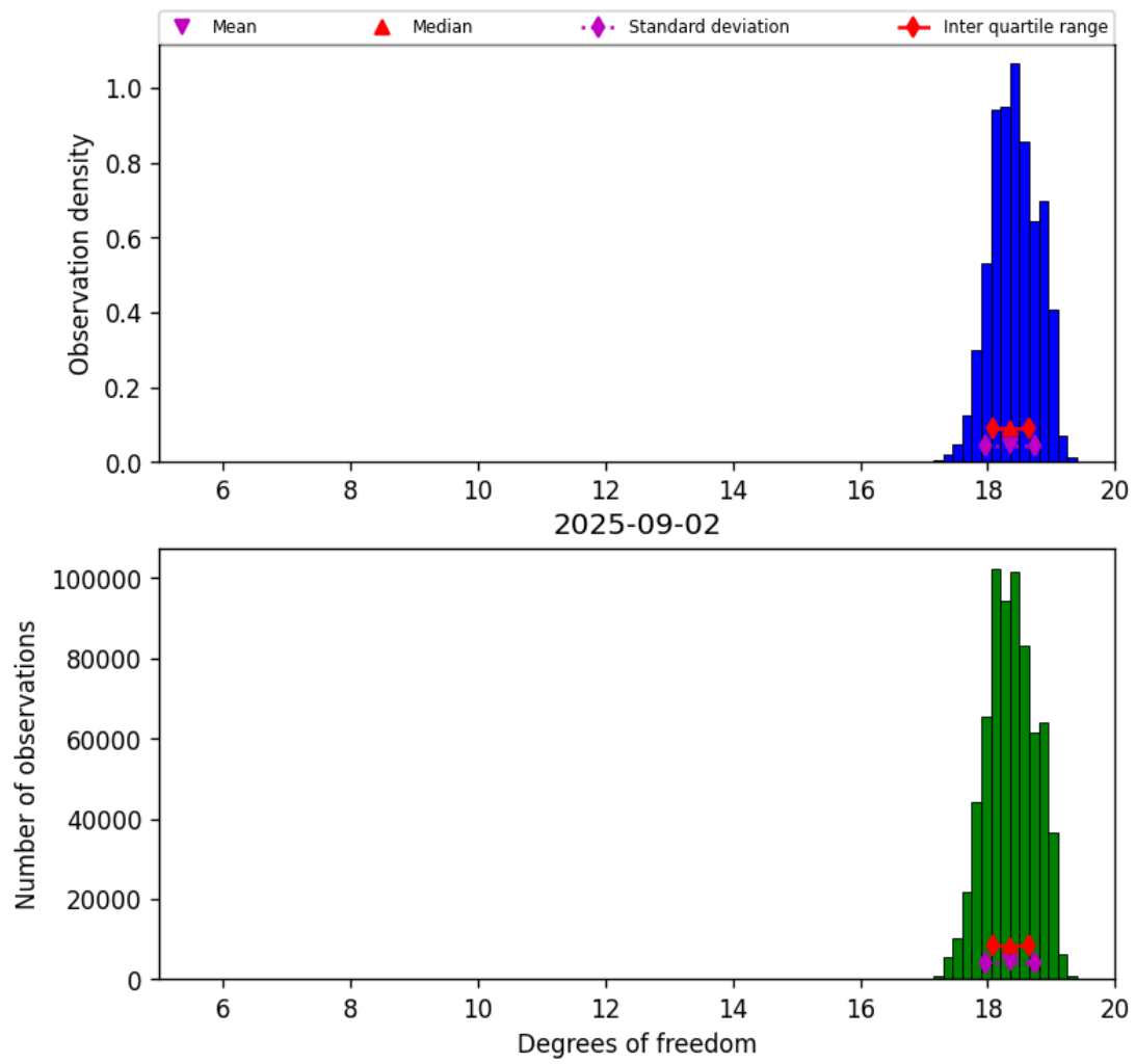
Figure 30: Histogram of “Degrees of freedom” for 2025-09-01 to 2025-09-03
