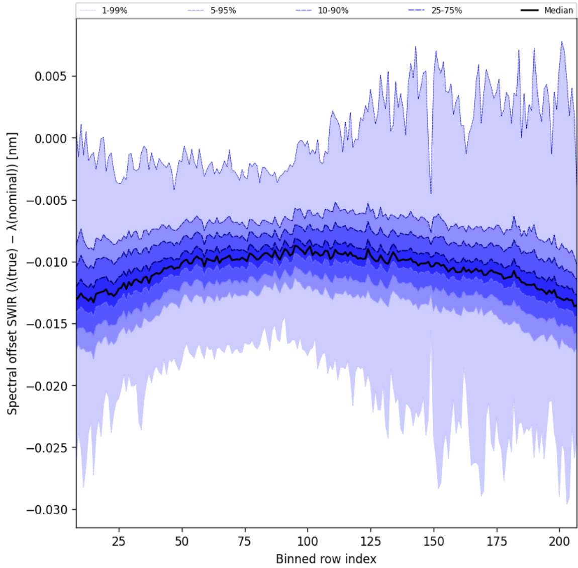
Figure 38: Along track statistics of “Spectral offset SWIR ( \lambda_{\text{true}} - \lambda_{\text{nominal}} )” for 2025-09-01 to 2025-09-03
