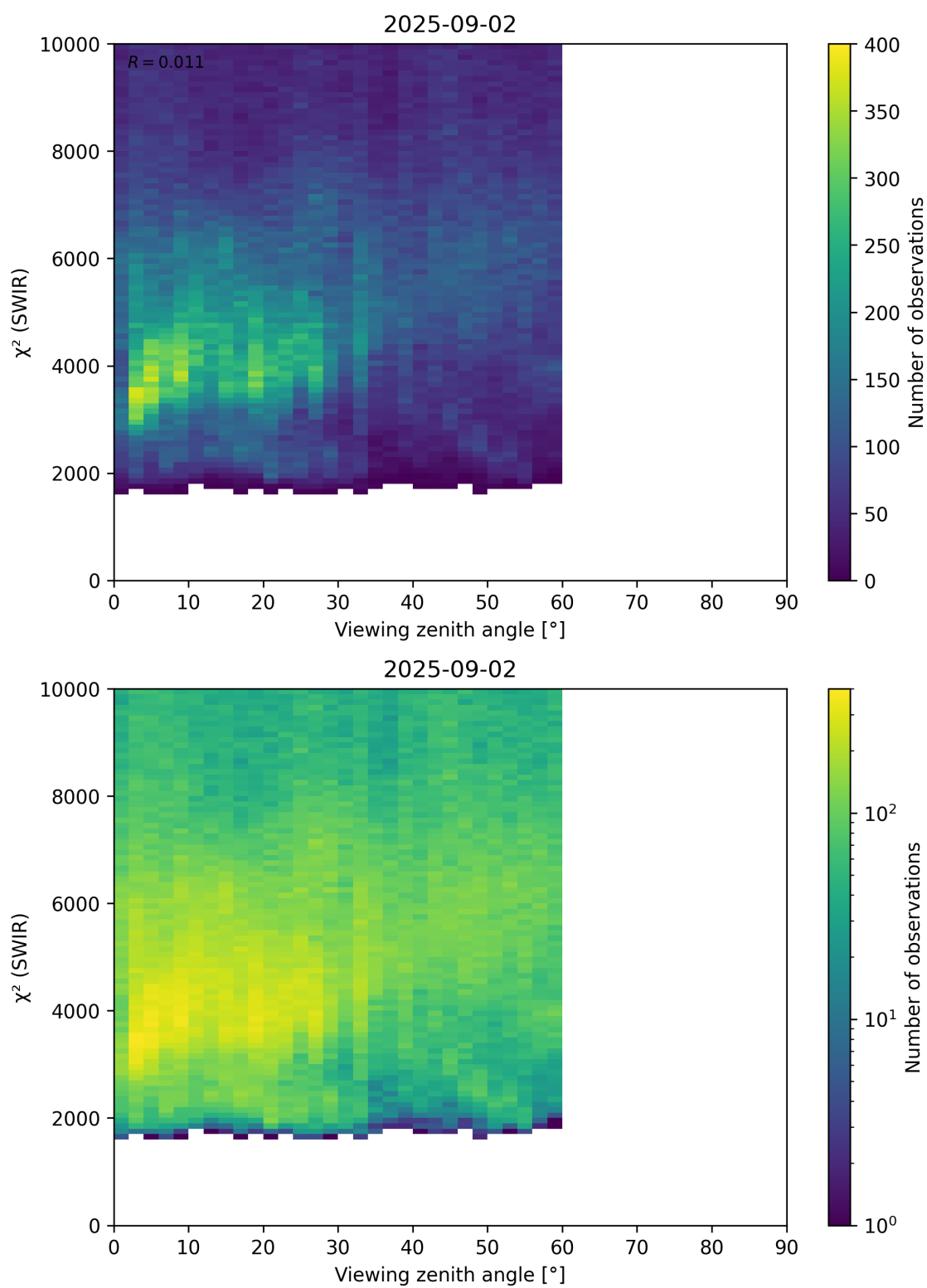
Figure 106: Scatter density plot of “Viewing zenith angle” against “ \chi^2 (SWIR)” for 2025-09-01 to 2025-09-03.
