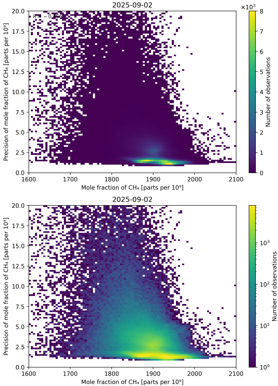
Figure 75: Scatter density plot of “Mole fraction of CH 4 ” against “Precision of mole fraction of CH 4 ” for 2025-09-01 to 2025-09-03.
