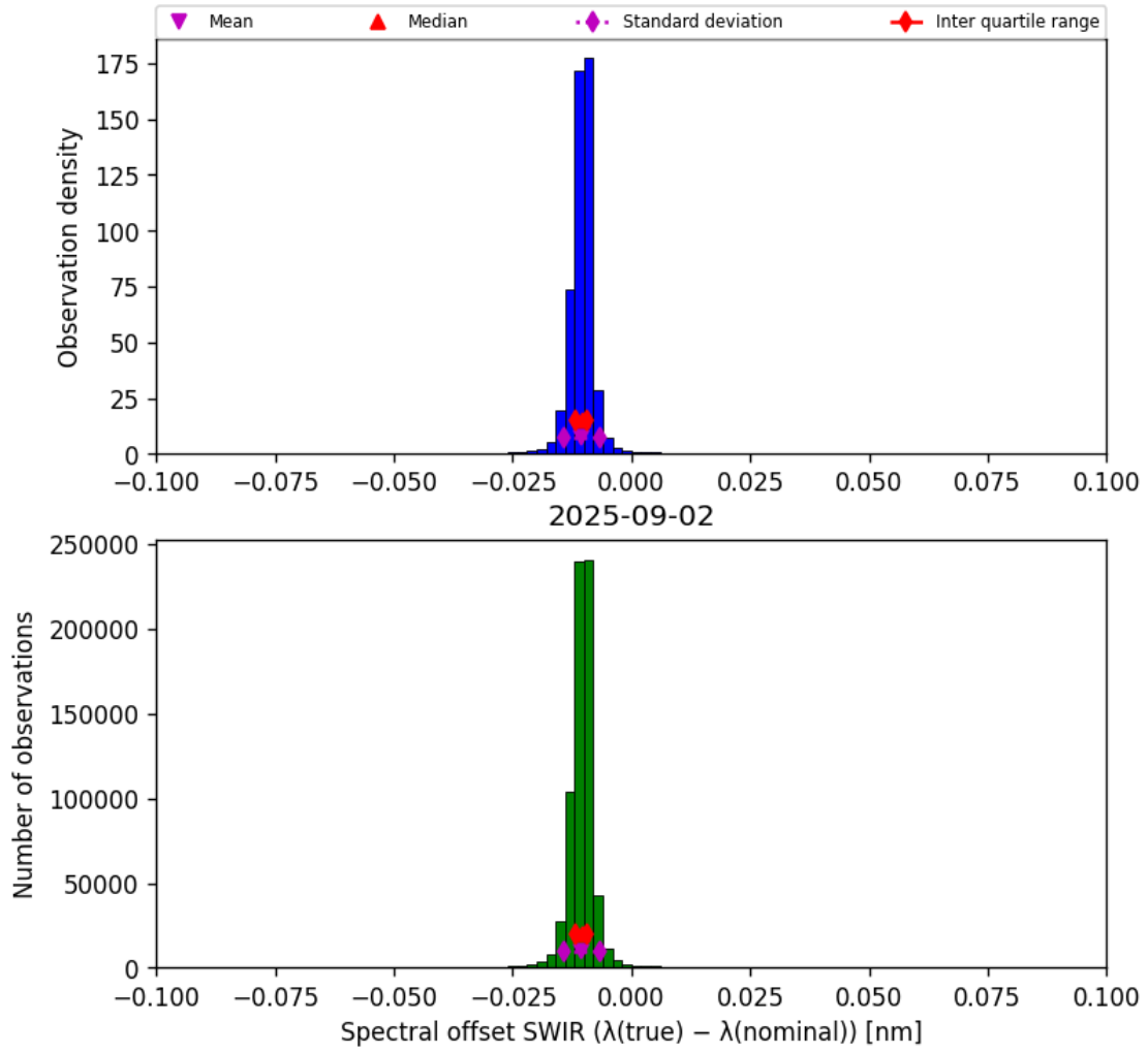
Figure 27: Histogram of “Spectral offset SWIR ( \lambda_{\text{true}} - \lambda_{\text{nominal}} )” for 2025-09-01 to 2025-09-03
