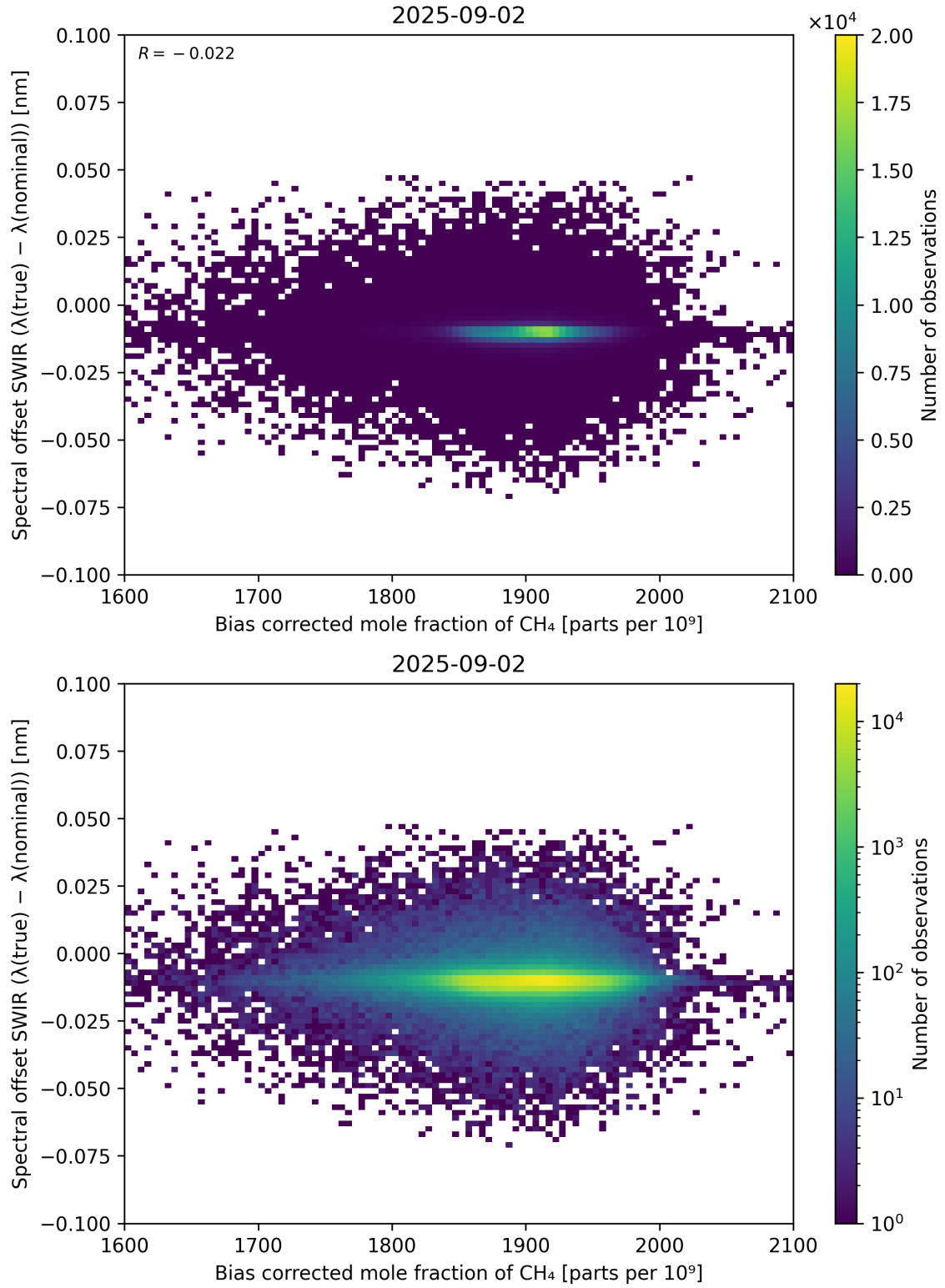
Figure 69: Scatter density plot of “Bias corrected mole fraction of \text{CH}_4 ” against “Spectral offset SWIR ( \lambda_{\text{true}} - \lambda_{\text{nominal}} )” for 2025-09-01 to 2025-09-03.
