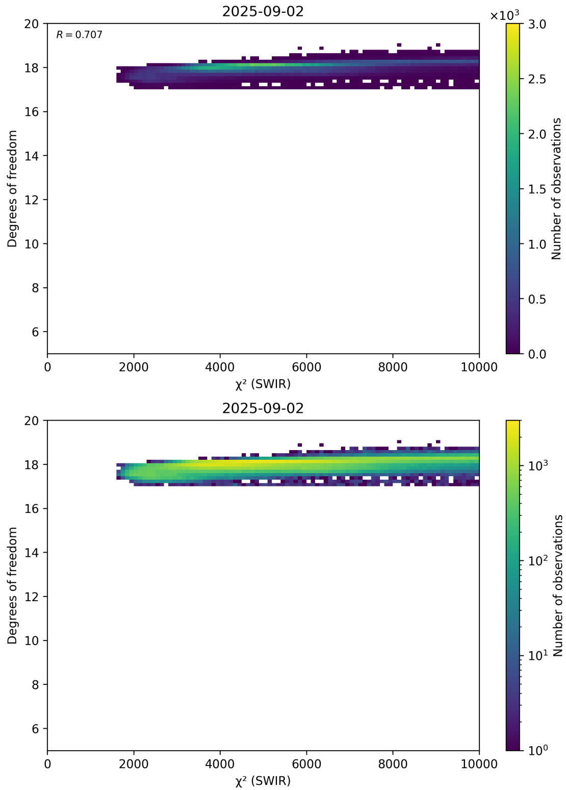
Figure 48: Scatter density plot of “ \chi^2 (SWIR)” against “Degrees of freedom” for 2025-09-01 to 2025-09-03.
