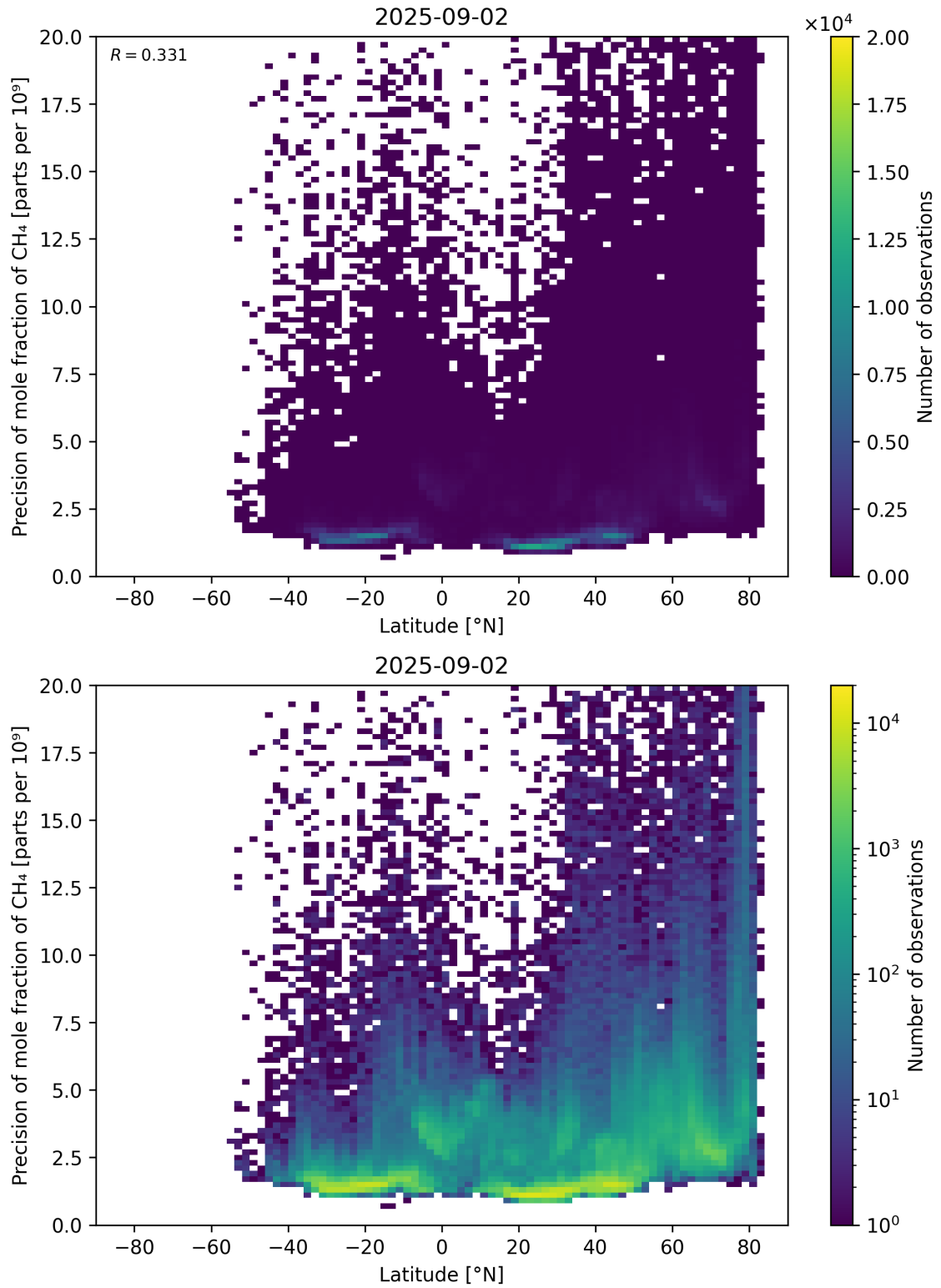
Figure 59: Scatter density plot of “Latitude” against “Precision of mole fraction of \text{CH}_4 ” for 2025-09-01 to 2025-09-03.
