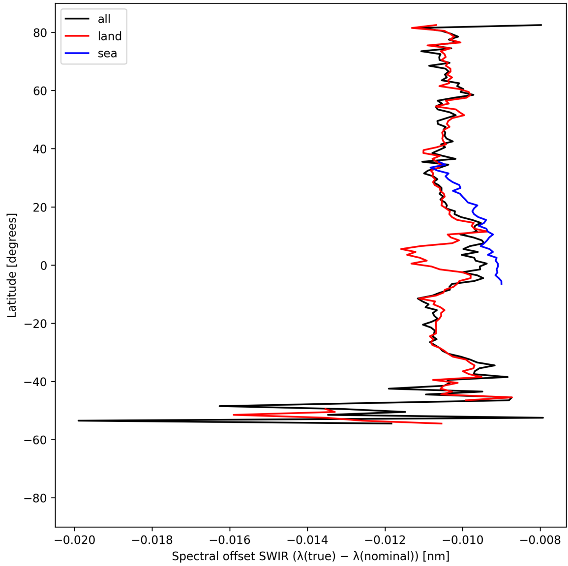
Figure 16: Zonal average of “Spectral offset SWIR ( \lambda_{\text{true}} - \lambda_{\text{nominal}} )” for 2025-09-01 to 2025-09-03.
