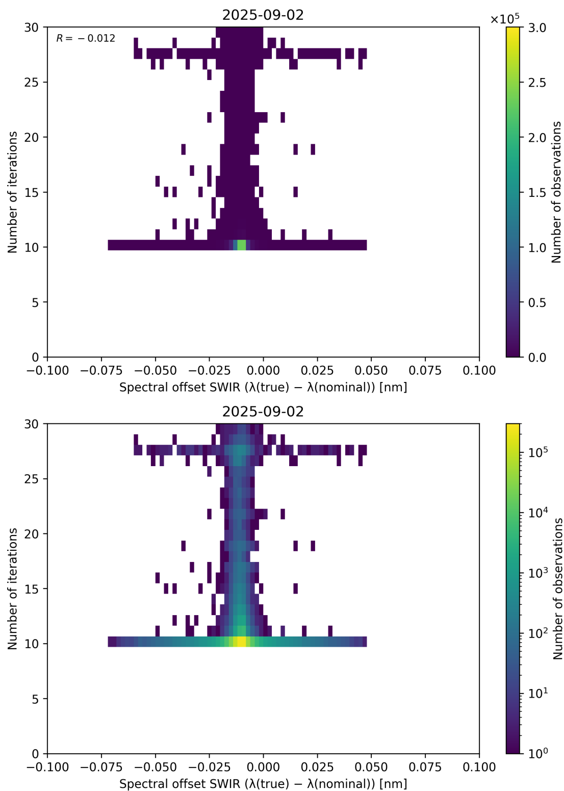
Figure 121: Scatter density plot of “Spectral offset SWIR ( \lambda_{\text{true}} - \lambda_{\text{nominal}} )” against “Number of iterations” for 2025-09-01 to 2025-09-03.
