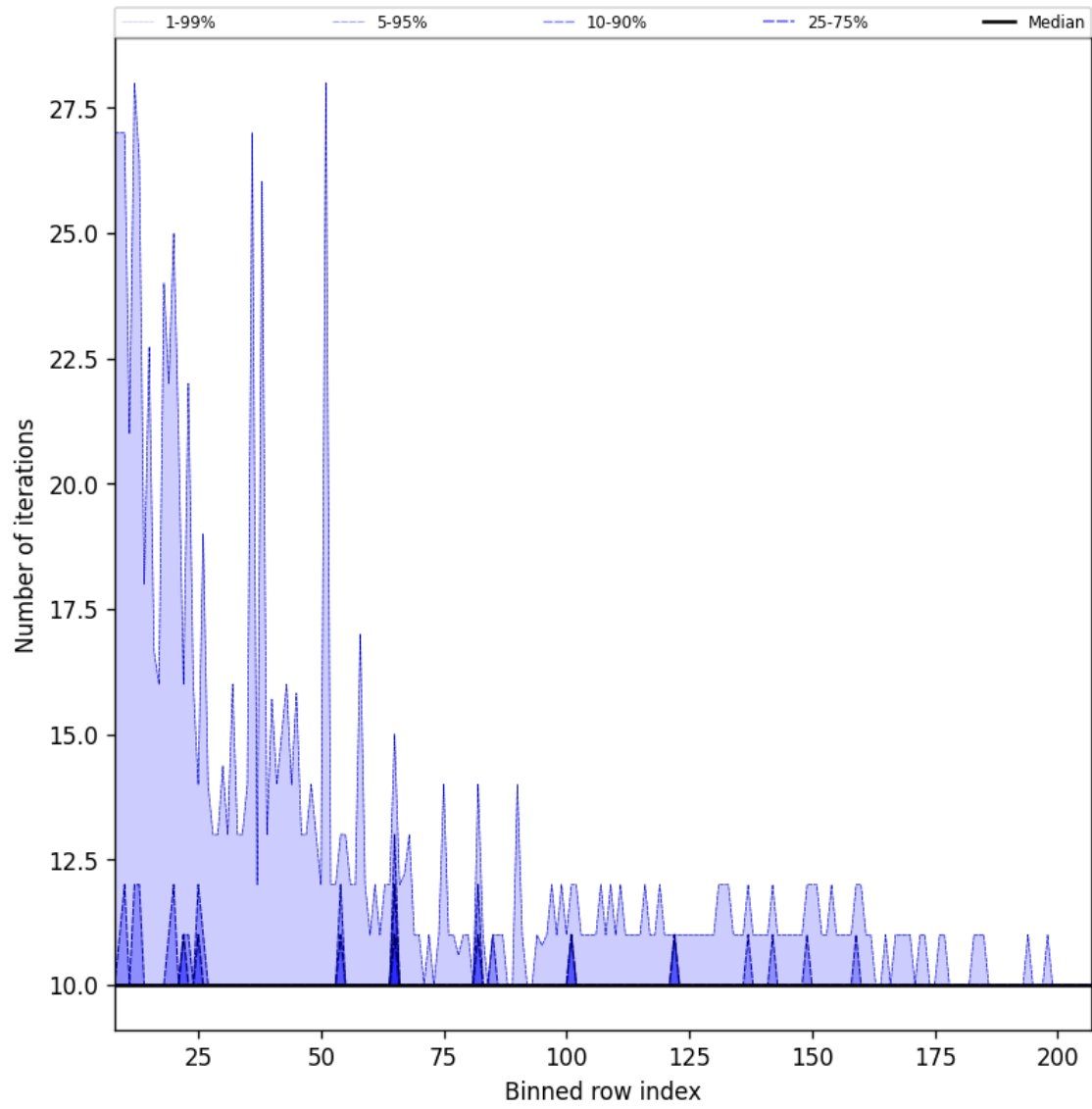
Figure 42: Along track statistics of “Number of iterations” for 2025-09-01 to 2025-09-03
