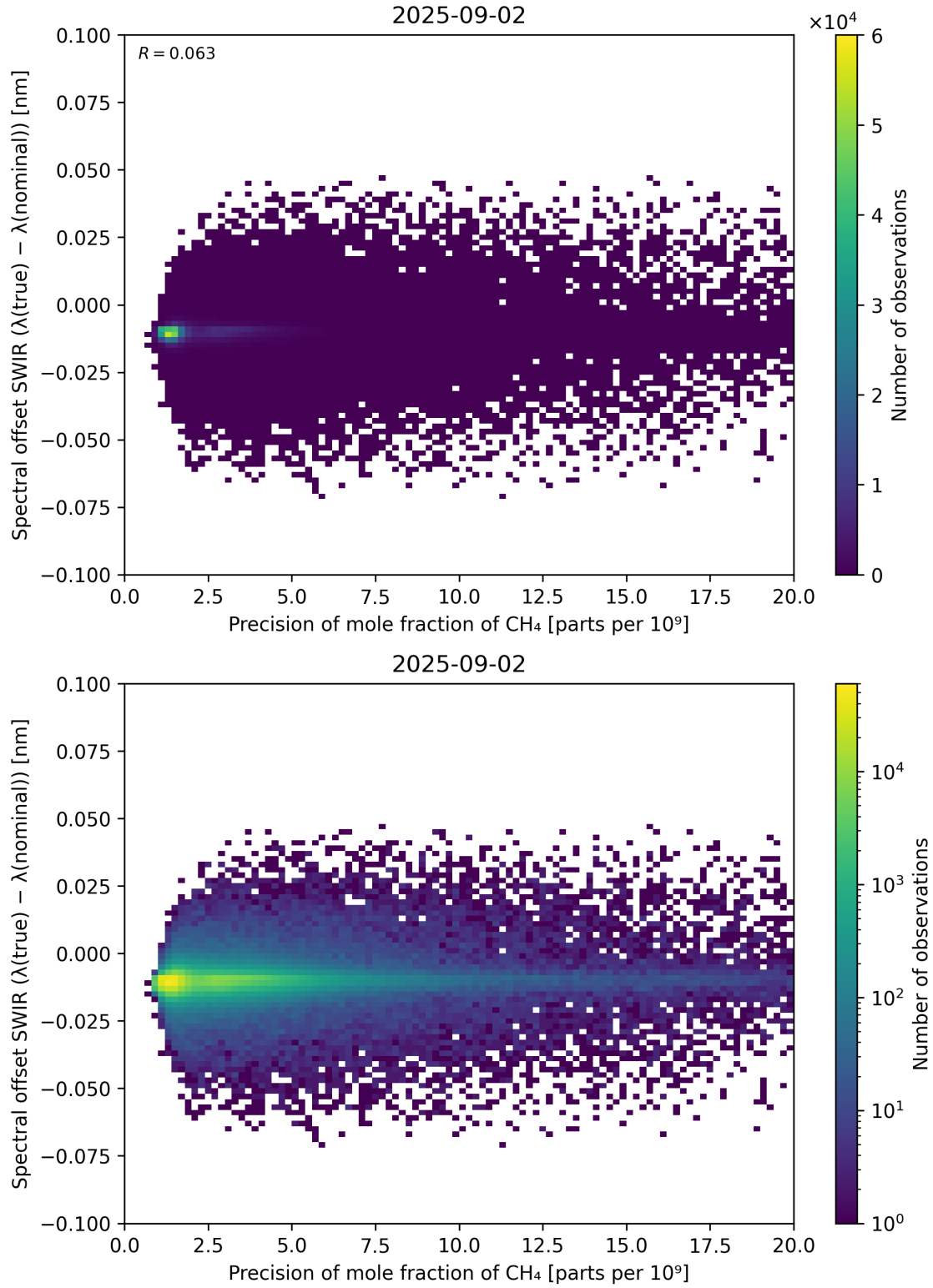
Figure 85: Scatter density plot of “Precision of mole fraction of \text{CH}_4 ” against “Spectral offset SWIR ( \lambda_{\text{true}} - \lambda_{\text{nominal}} )” for 2025-09-01 to 2025-09-03.
