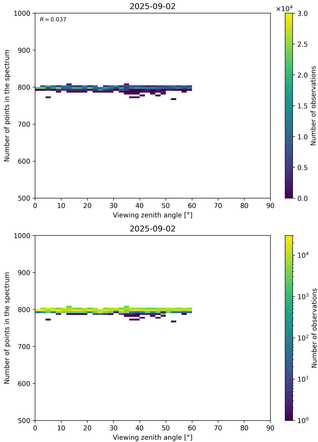
Figure 114: Scatter density plot of “Viewing zenith angle” against “Number of points in the spectrum” for 2025-09-01 to 2025-09-03.
