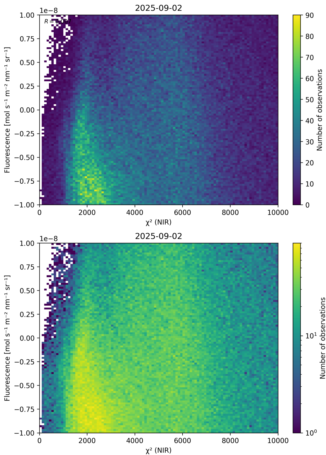
Figure 45: Scatter density plot of “ \chi^2 (NIR)” against “Fluorescence” for 2025-09-01 to 2025-09-03.
