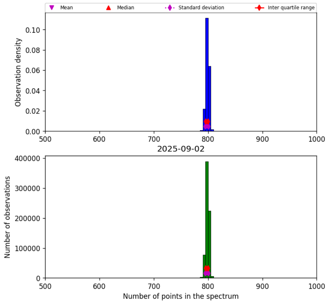
Figure 26: Histogram of “Number of points in the spectrum” for 2025-09-01 to 2025-09-03
