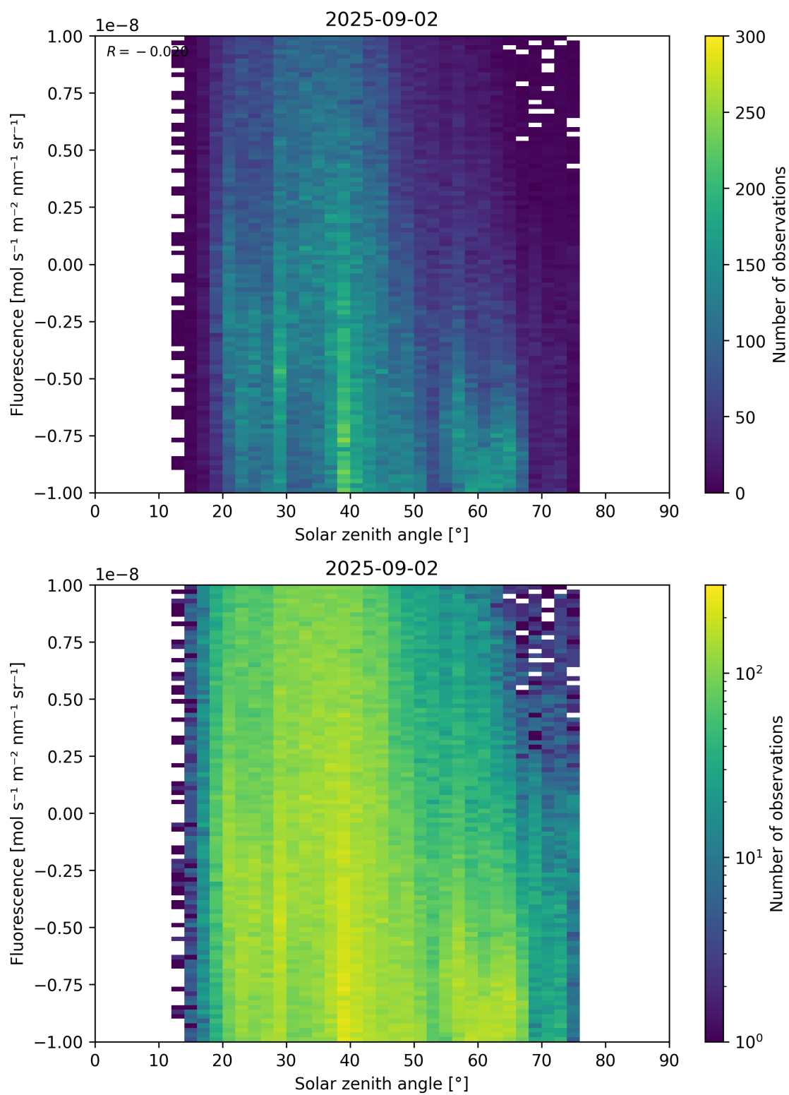
Figure 97: Scatter density plot of “Solar zenith angle” against “Fluorescence” for 2025-09-01 to 2025-09-03.
