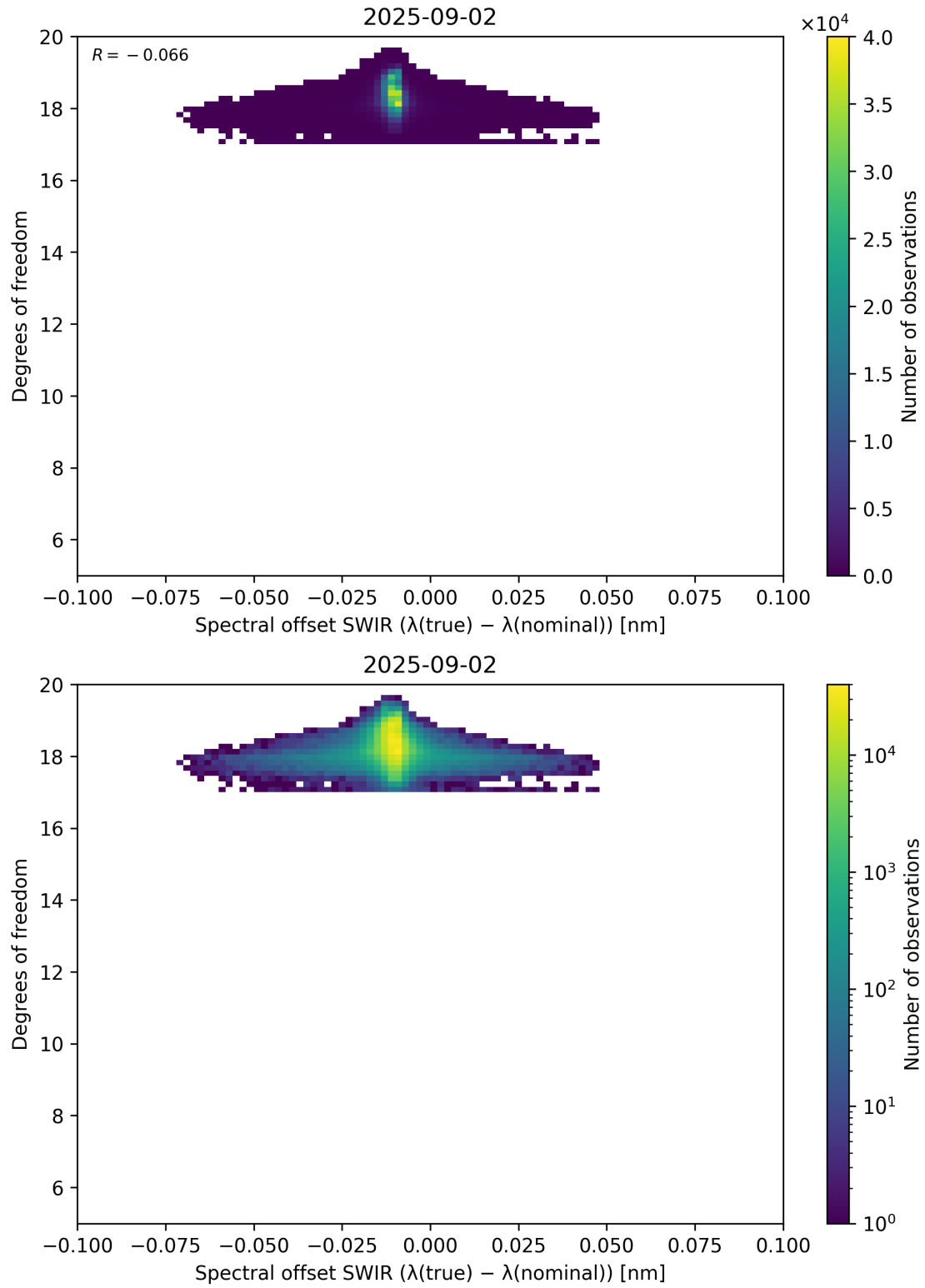
Figure 119: Scatter density plot of “Spectral offset SWIR ( \lambda_{\text{true}} - \lambda_{\text{nominal}} )” against “Degrees of freedom” for 2025-09-01 to 2025-09-03.
