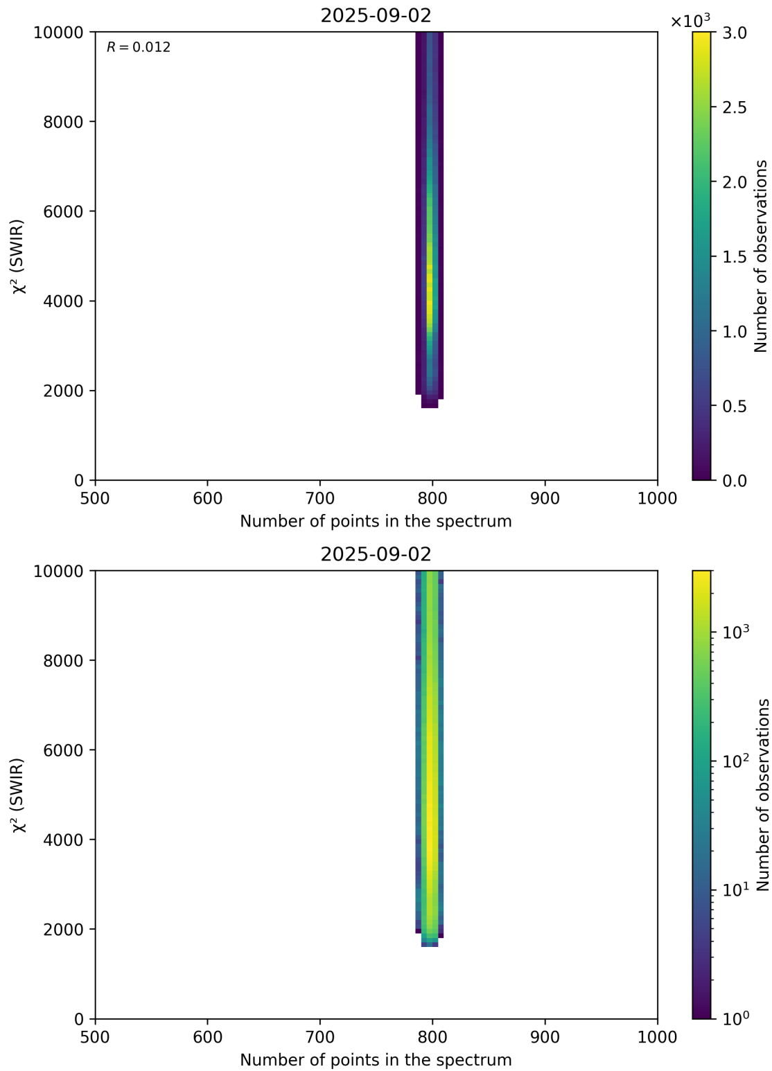
Figure 89: Scatter density plot of “Number of points in the spectrum” against “ \chi^2 (SWIR)” for 2025-09-01 to 2025-09-03.
