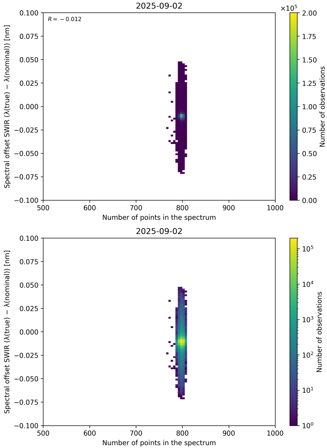
Figure 93: Scatter density plot of “Number of points in the spectrum” against “Spectral offset SWIR ( \lambda_{\text{true}} - \lambda_{\text{nominal}} )” for 2025-09-01 to 2025-09-03.
