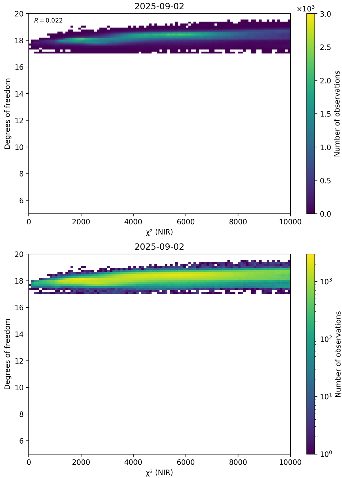
Figure 44: Scatter density plot of “ \chi^2 (NIR)” against “Degrees of freedom” for 2025-09-01 to 2025-09-03.
