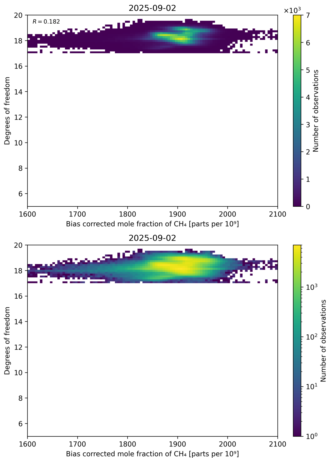
Figure 65: Scatter density plot of “Bias corrected mole fraction of CH 4 ” against “Degrees of freedom” for 2025-09-01 to 2025-09-03.
