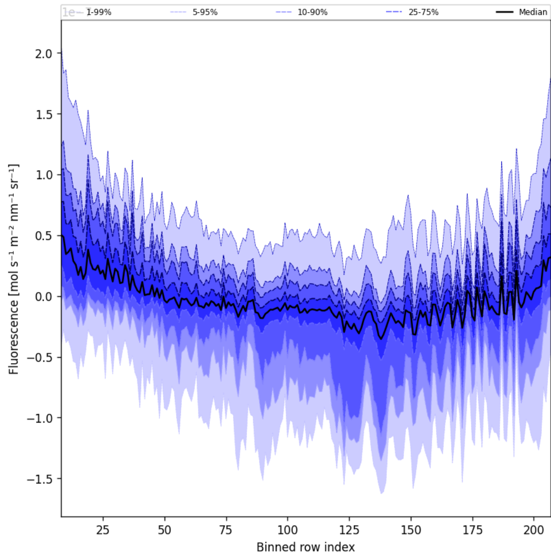
Figure 43: Along track statistics of “Fluorescence” for 2025-09-01 to 2025-09-03
