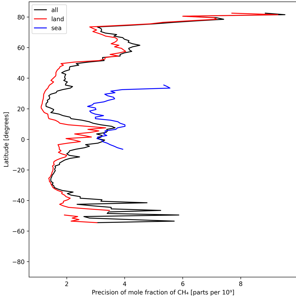
Figure 13: Zonal average of “Precision of mole fraction of CH 4 ” for 2025-09-01 to 2025-09-03.
