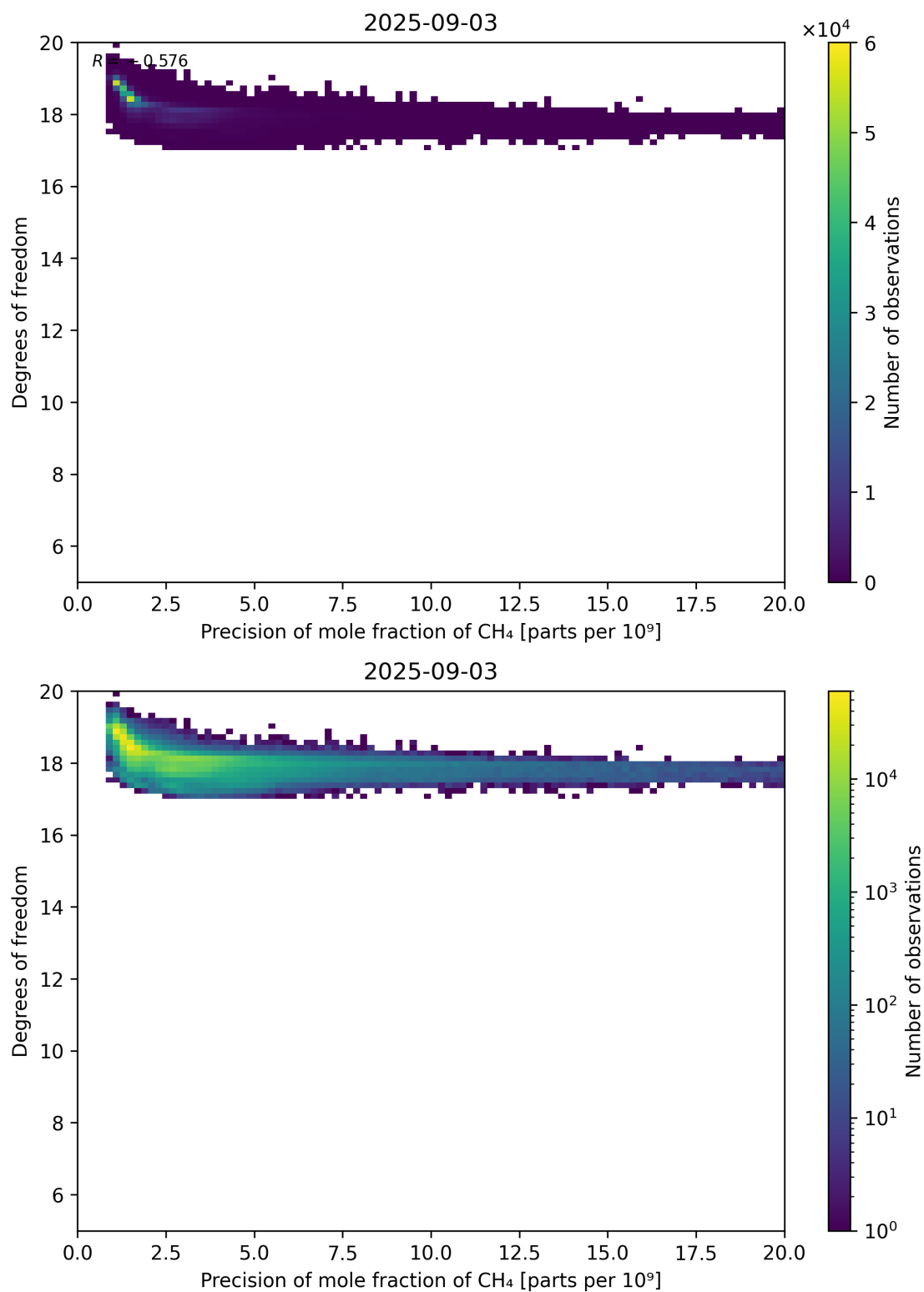
Figure 80: Scatter density plot of “Precision of mole fraction of CH 4 ” against “Degrees of freedom” for 2025-09-02 to 2025-09-04.
