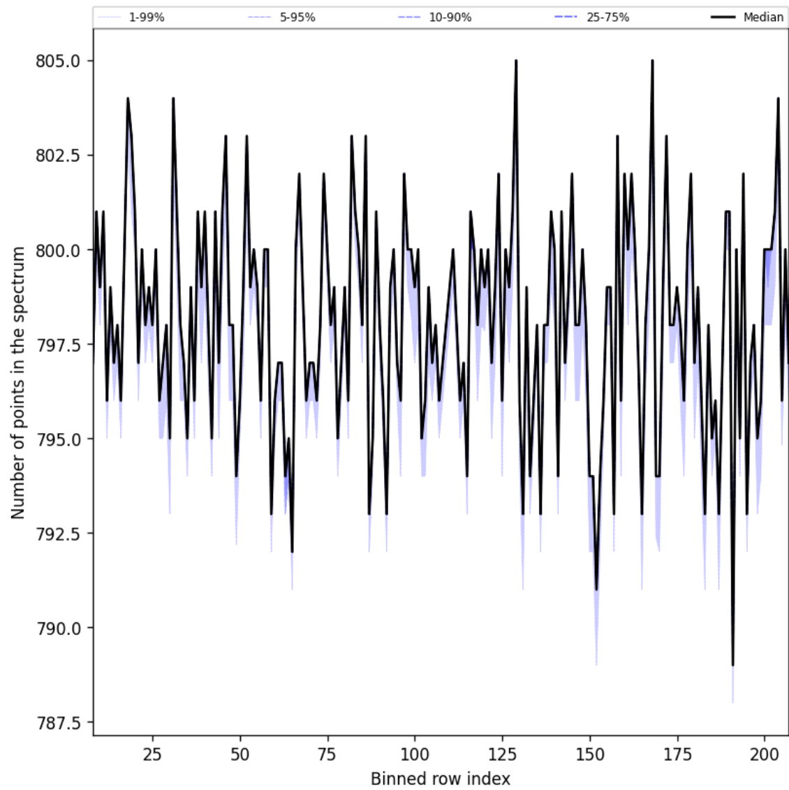
Figure 37: Along track statistics of “Number of points in the spectrum” for 2025-09-02 to 2025-09-04
