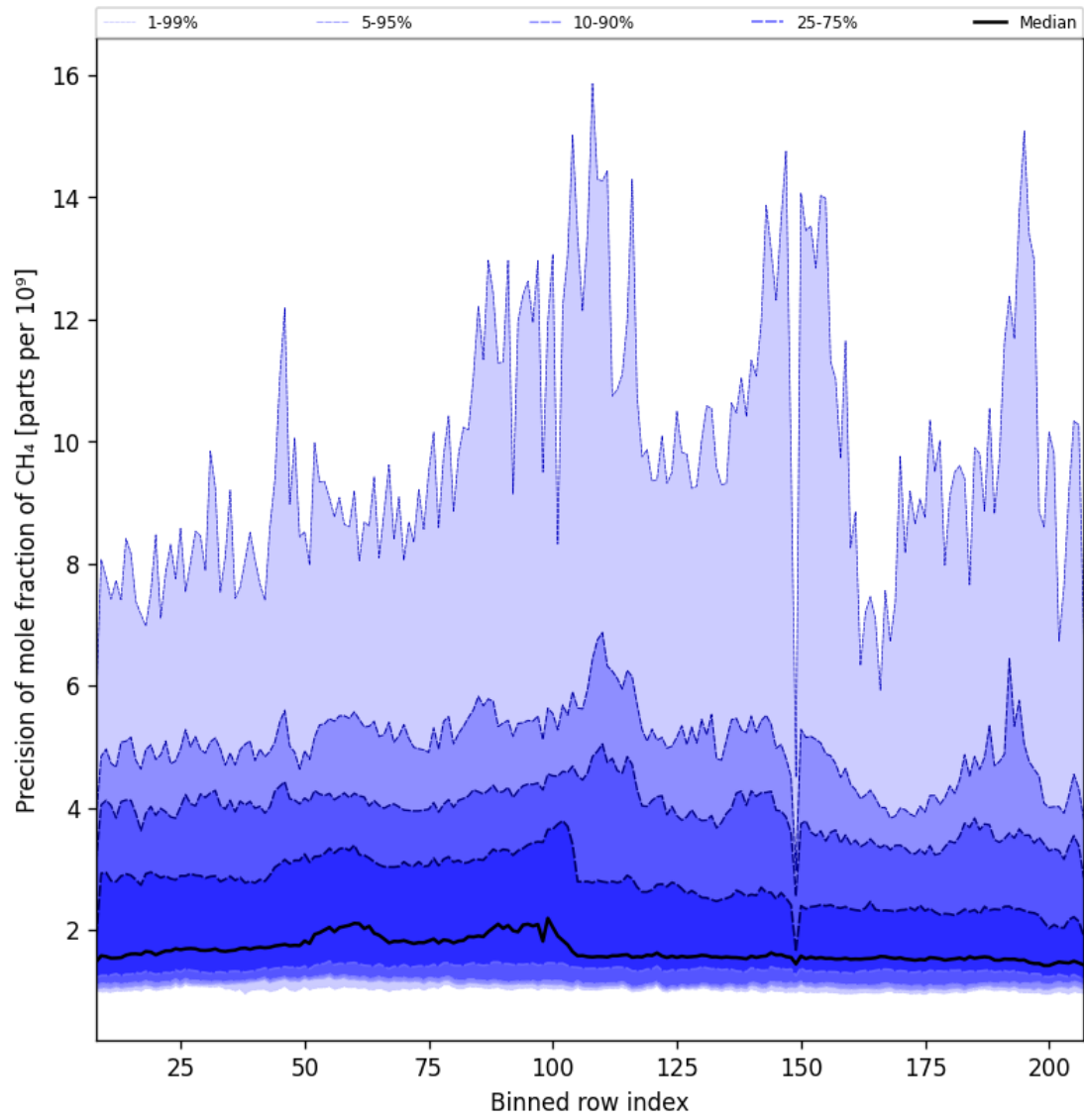
Figure 35: Along track statistics of “Precision of mole fraction of CH 4 ” for 2025-09-02 to 2025-09-04
