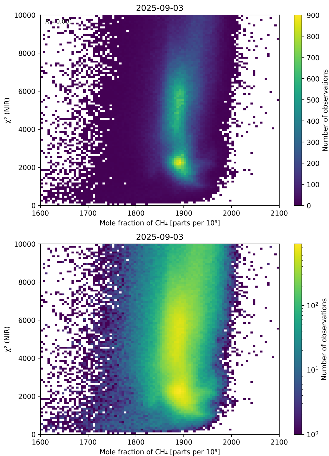
Figure 70: Scatter density plot of “Mole fraction of \text{CH}_4 ” against “ \chi^2 (NIR)” for 2025-09-02 to 2025-09-04.
