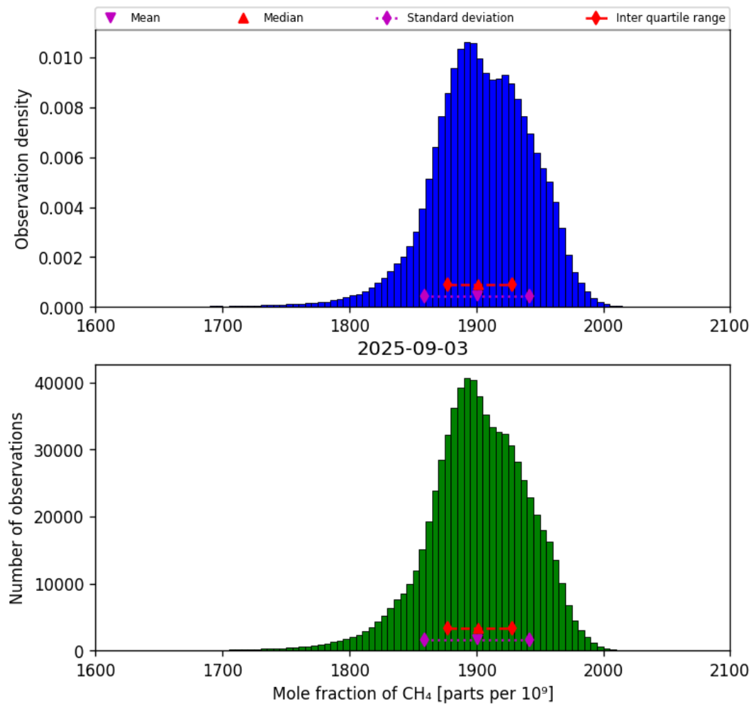
Figure 23: Histogram of “Mole fraction of CH 4 ” for 2025-09-02 to 2025-09-04
