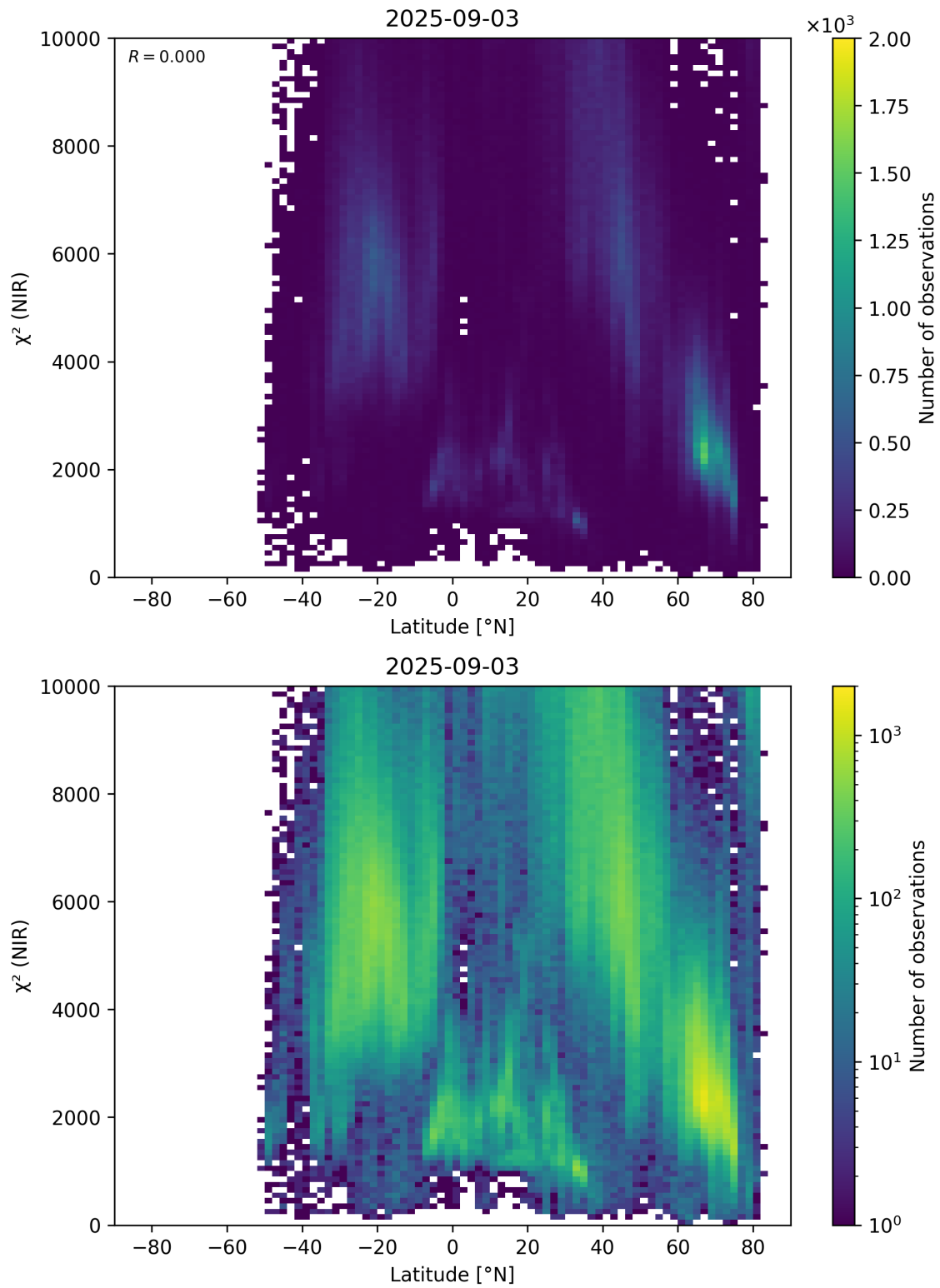
Figure 53: Scatter density plot of “Latitude” against “ \chi^2 (NIR)” for 2025-09-02 to 2025-09-04.
