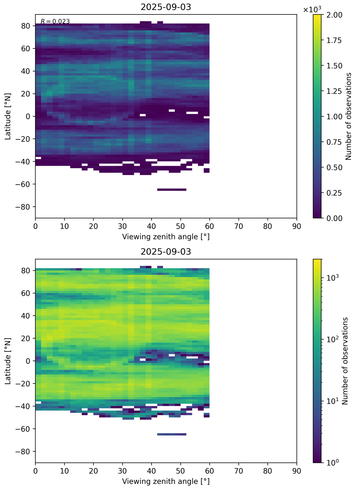
Figure 109: Scatter density plot of “Viewing zenith angle” against “Latitude” for 2025-09-02 to 2025-09-04.
