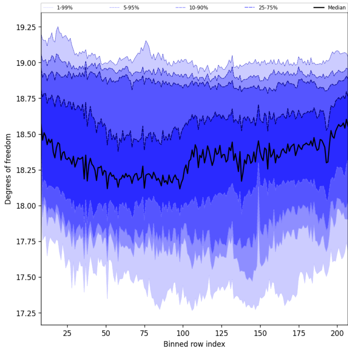
Figure 41: Along track statistics of “Degrees of freedom” for 2025-09-02 to 2025-09-04
