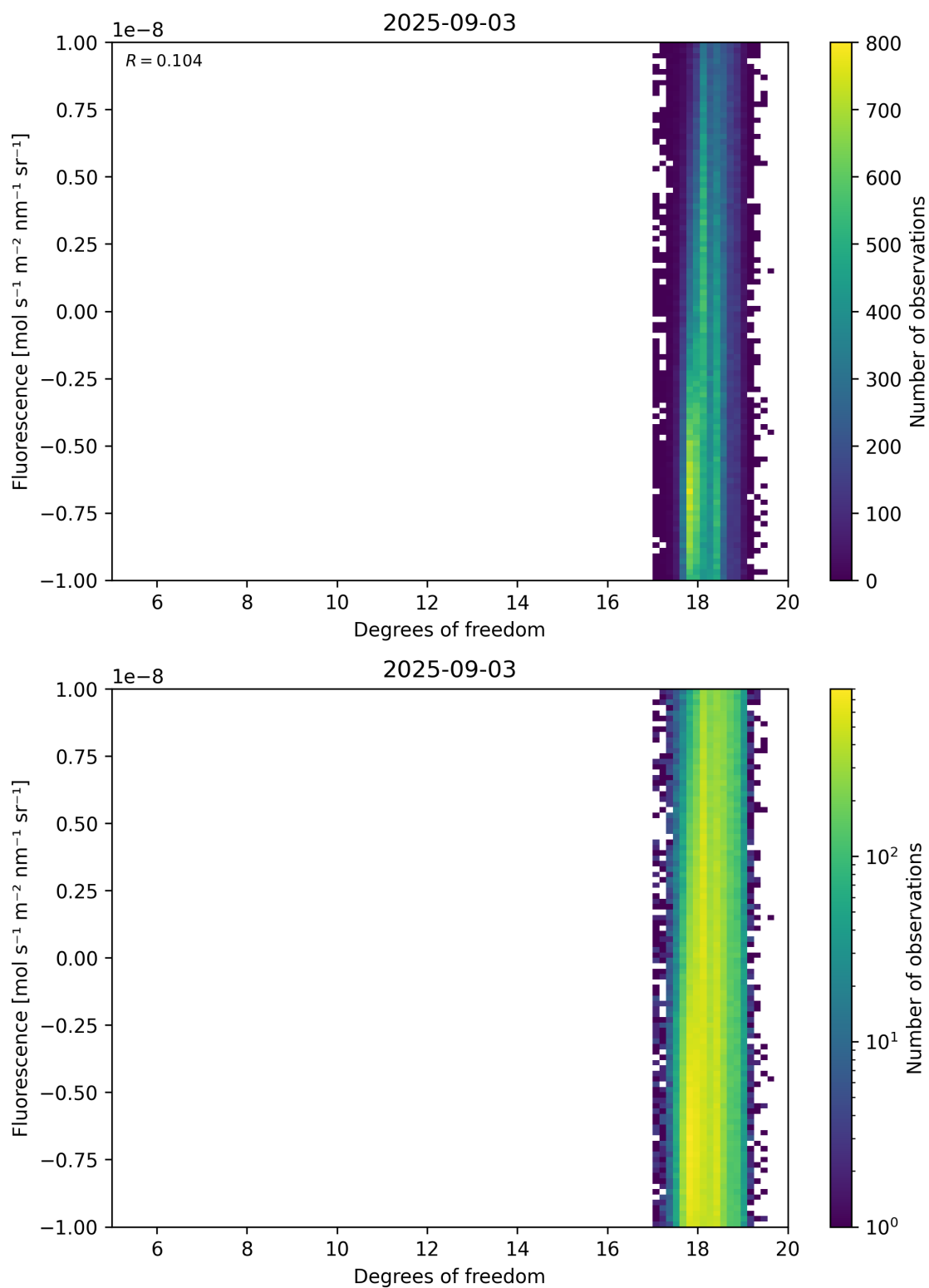
Figure 51: Scatter density plot of “Degrees of freedom” against “Fluorescence” for 2025-09-02 to 2025-09-04.
