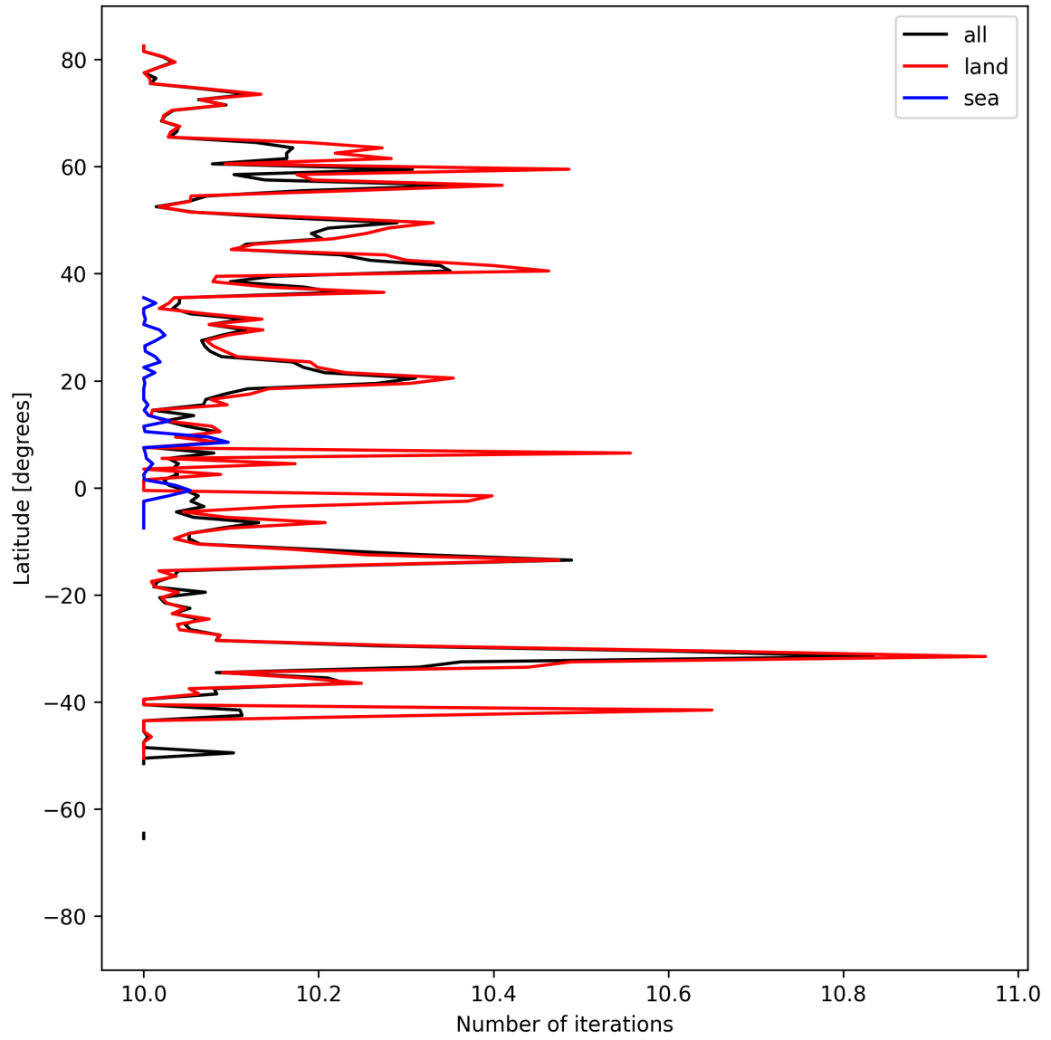
Figure 20: Zonal average of “Number of iterations” for 2025-09-02 to 2025-09-04.
