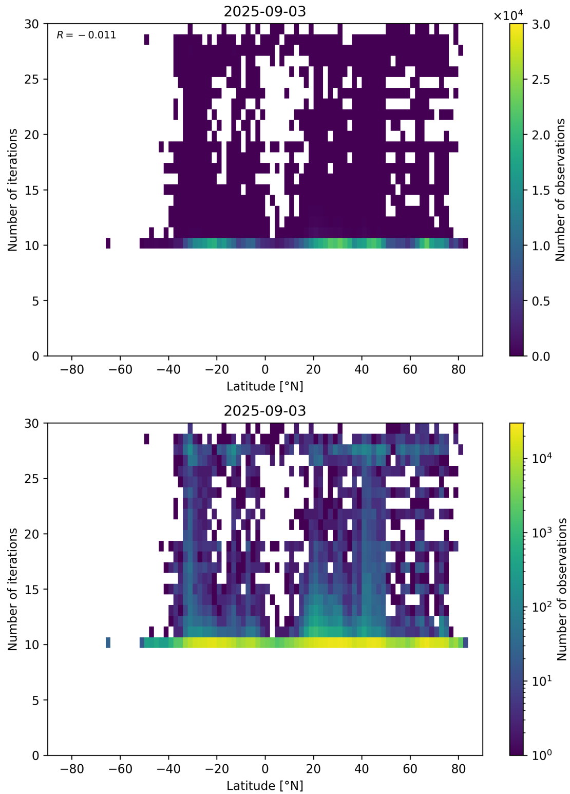
Figure 60: Scatter density plot of “Latitude” against “Number of iterations” for 2025-09-02 to 2025-09-04.
