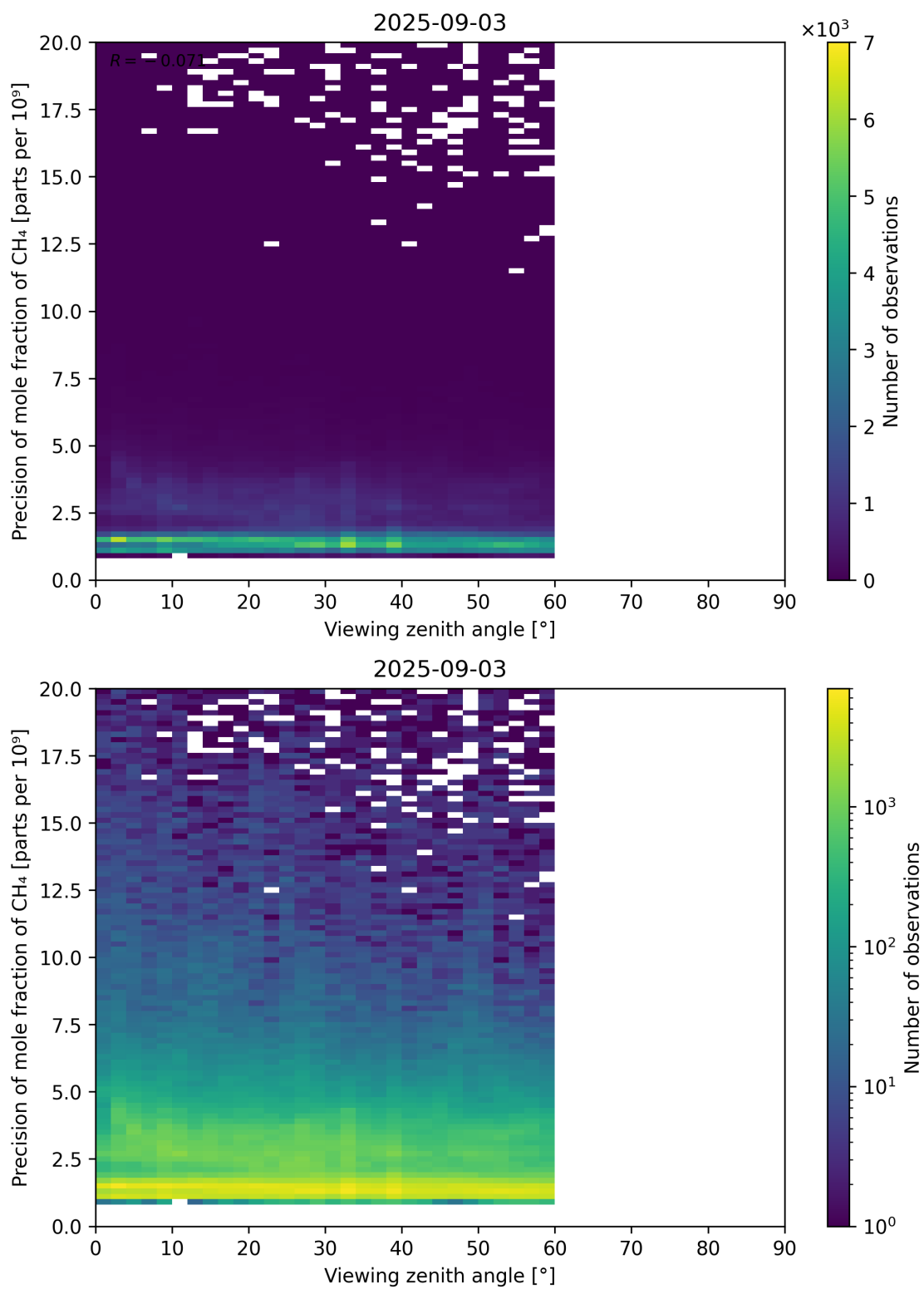
Figure 112: Scatter density plot of “Viewing zenith angle” against “Precision of mole fraction of CH 4 ” for 2025-09-02 to 2025-09-04.
