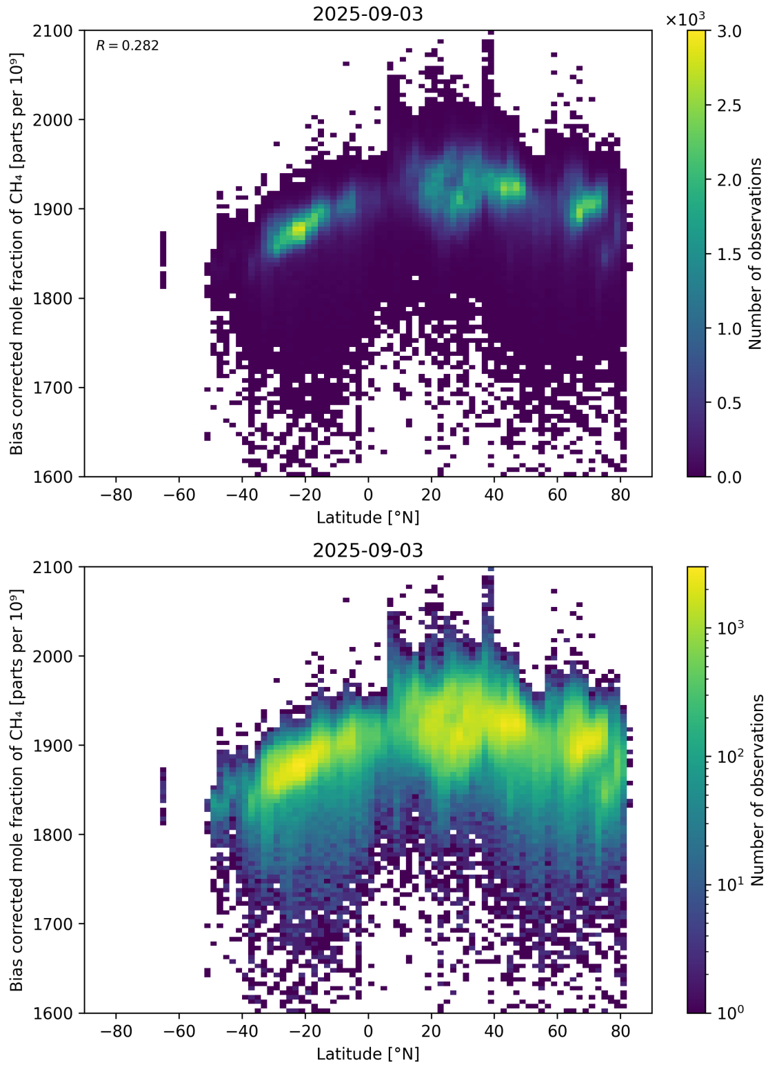
Figure 58: Scatter density plot of “Latitude” against “Bias corrected mole fraction of CH 4 ” for 2025-09-02 to 2025-09-04.
