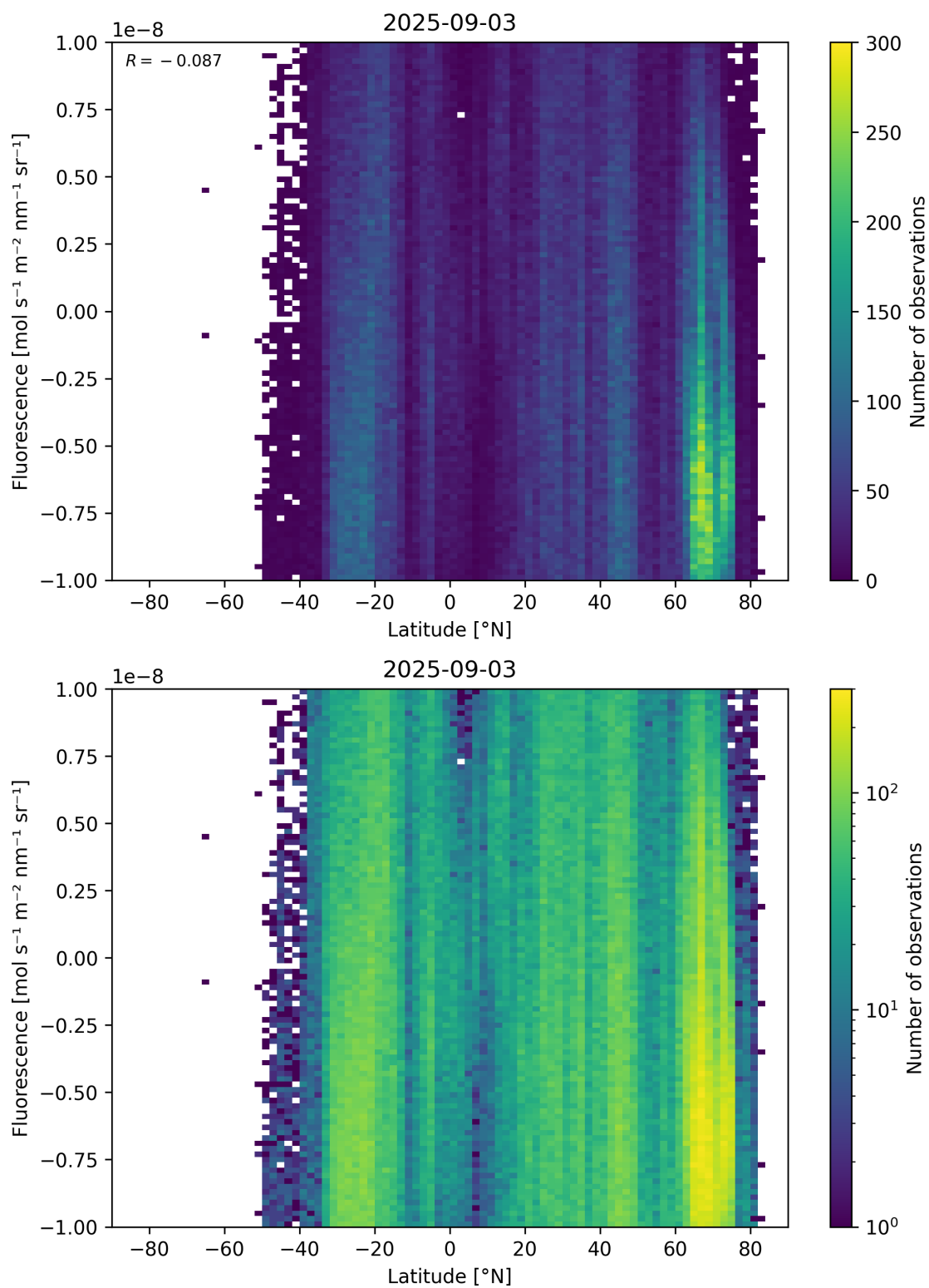
Figure 56: Scatter density plot of “Latitude” against “Fluorescence” for 2025-09-02 to 2025-09-04.
