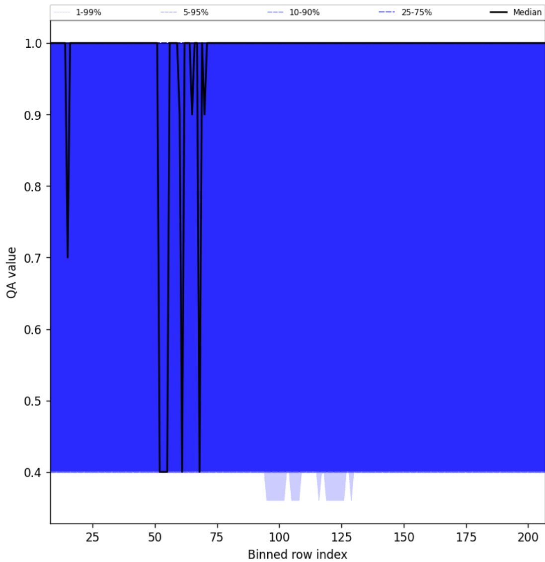
Figure 33: Along track statistics of “QA value” for 2025-09-02 to 2025-09-04
