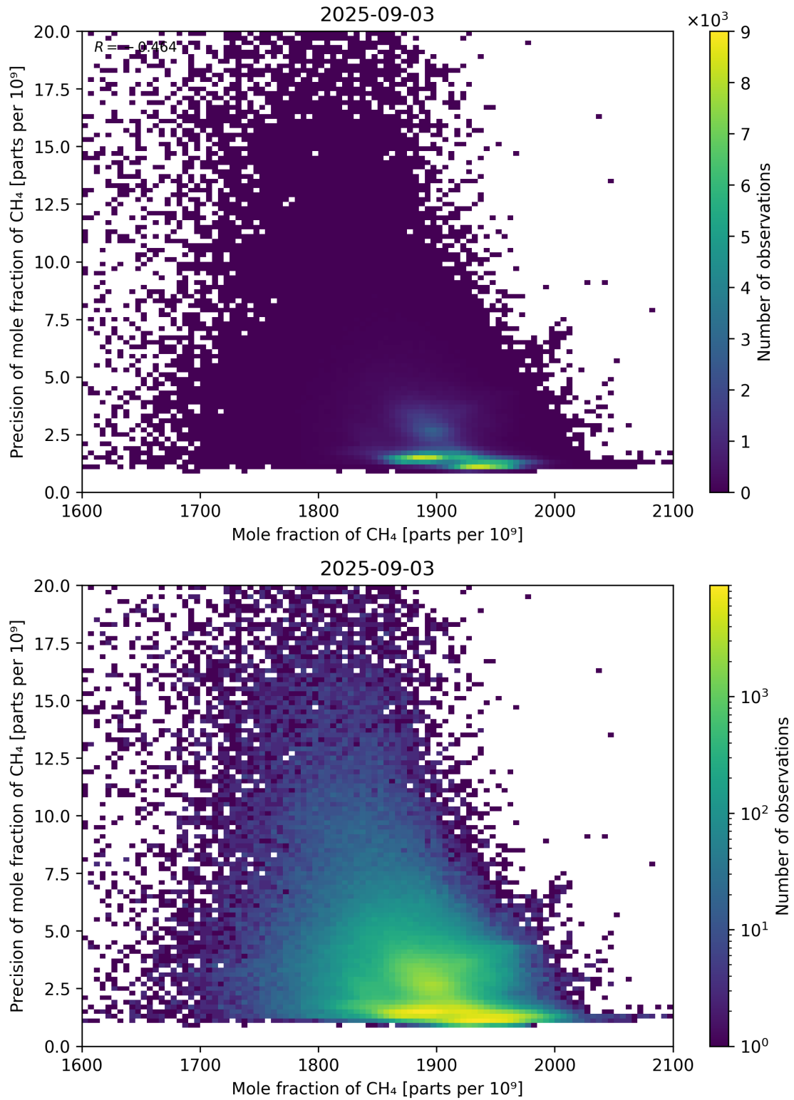
Figure 75: Scatter density plot of “Mole fraction of CH 4 ” against “Precision of mole fraction of CH 4 ” for 2025-09-02 to 2025-09-04.
