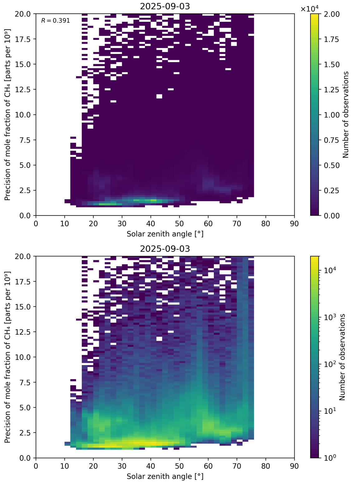
Figure 101: Scatter density plot of “Solar zenith angle” against “Precision of mole fraction of CH 4 ” for 2025-09-02 to 2025-09-04.
