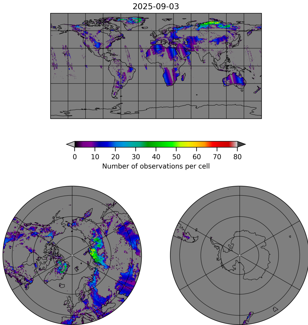
Figure 10: Map of the number of observations for 2025-09-02 to 2025-09-04
