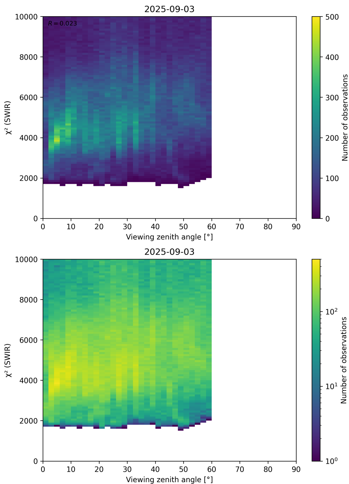
Figure 106: Scatter density plot of “Viewing zenith angle” against “ \chi^2 (SWIR)” for 2025-09-02 to 2025-09-04.
