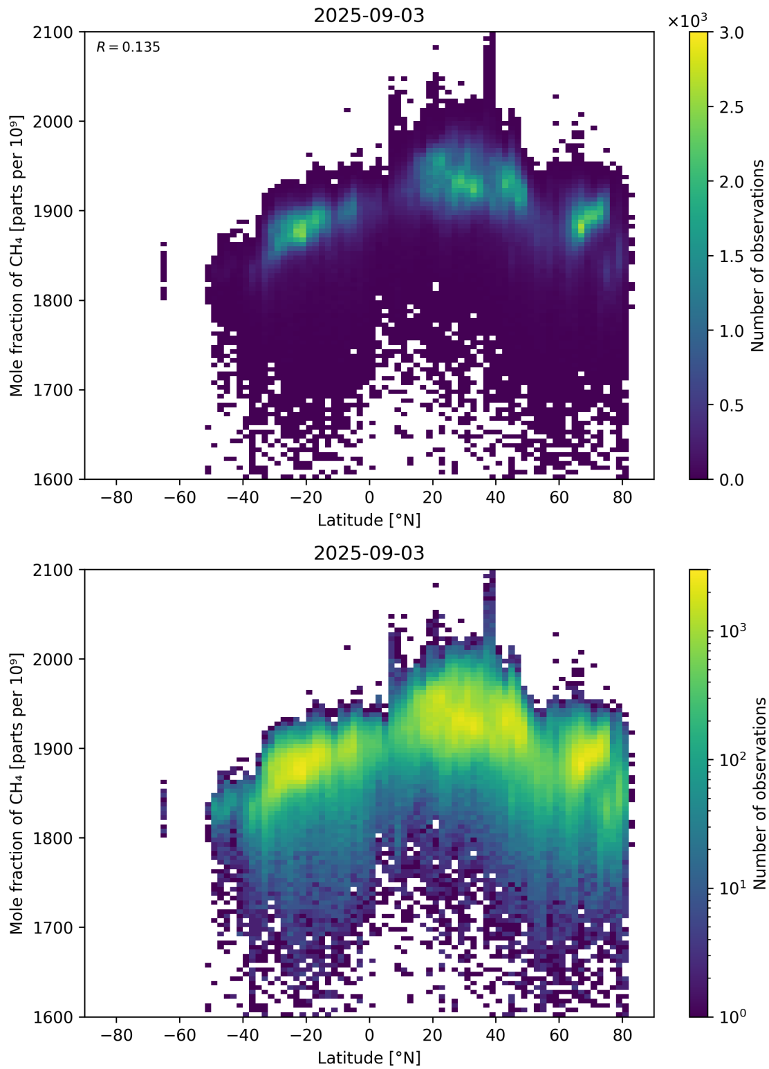
Figure 57: Scatter density plot of “Latitude” against “Mole fraction of \text{CH}_4 ” for 2025-09-02 to 2025-09-04.
