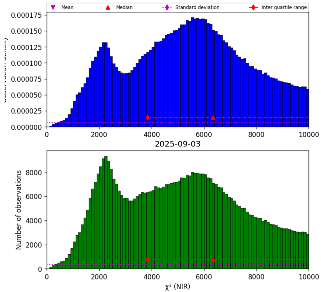
Figure 29: Histogram of “ \chi^2 (NIR)” for 2025-09-02 to 2025-09-04
