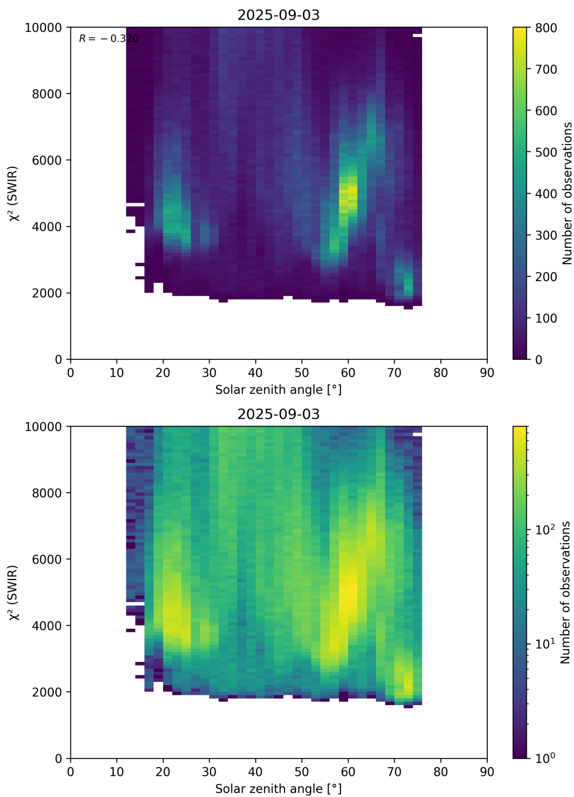
Figure 95: Scatter density plot of “Solar zenith angle” against “ \chi^2 (SWIR)” for 2025-09-02 to 2025-09-04.
