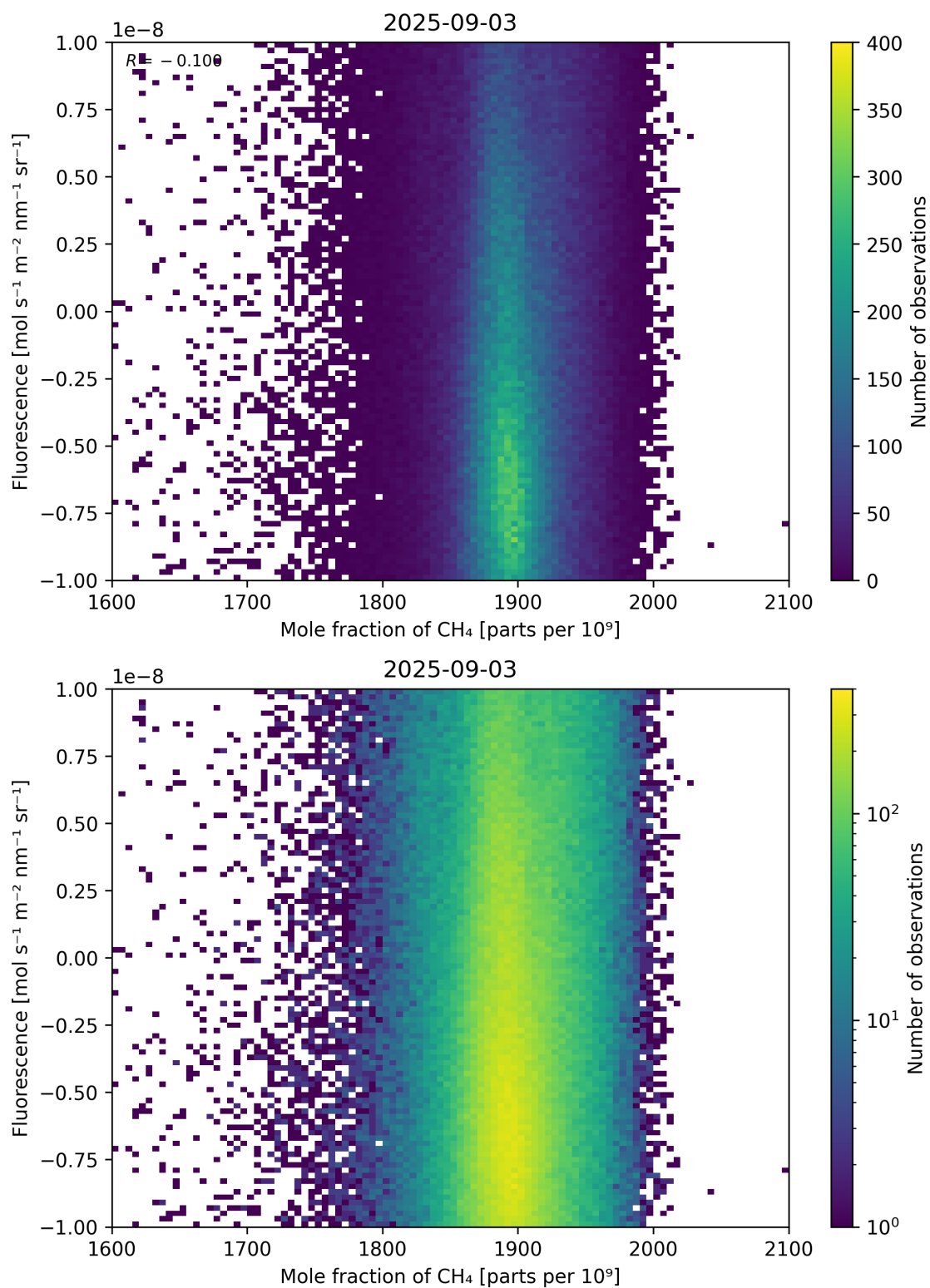
Figure 73: Scatter density plot of “Mole fraction of \text{CH}_4 ” against “Fluorescence” for 2025-09-02 to 2025-09-04.
