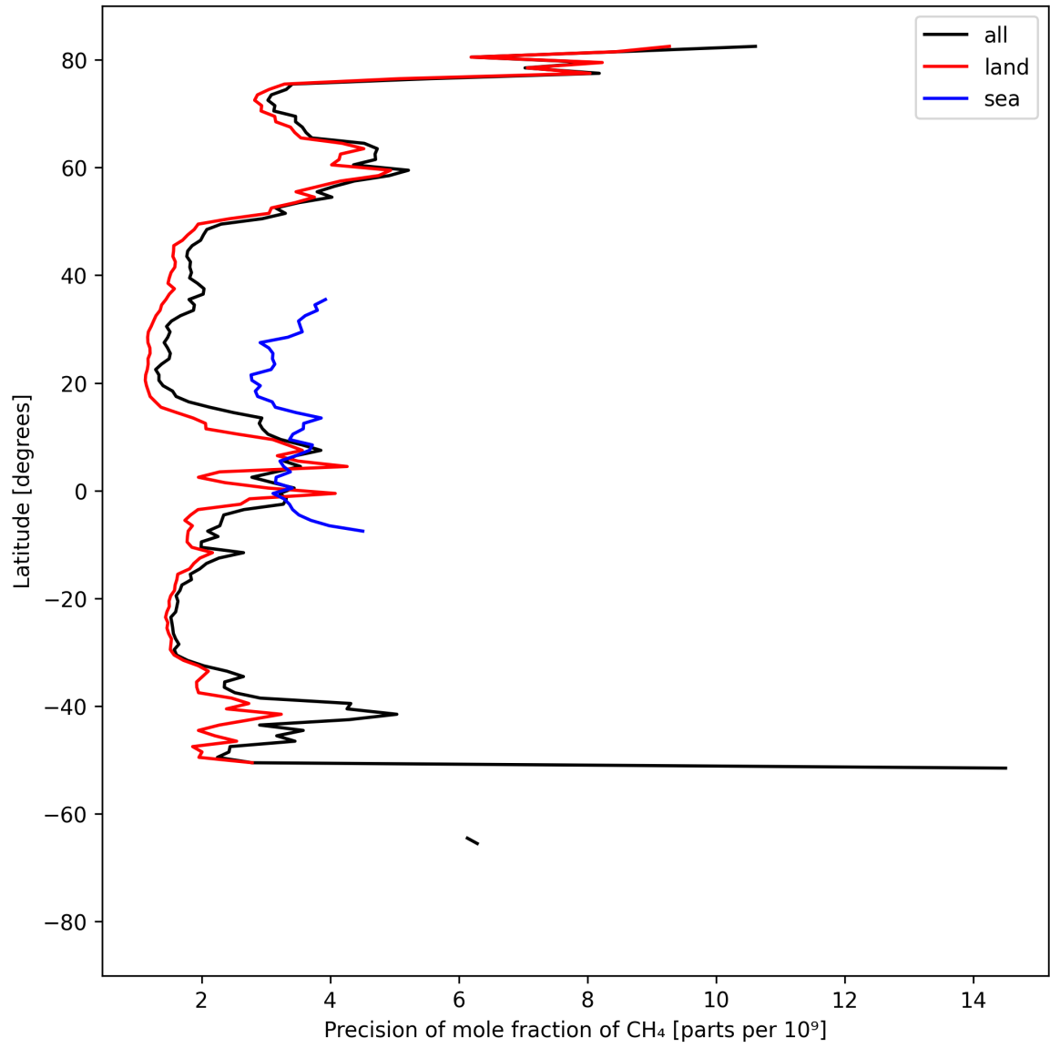
Figure 13: Zonal average of “Precision of mole fraction of CH 4 ” for 2025-09-02 to 2025-09-04.
