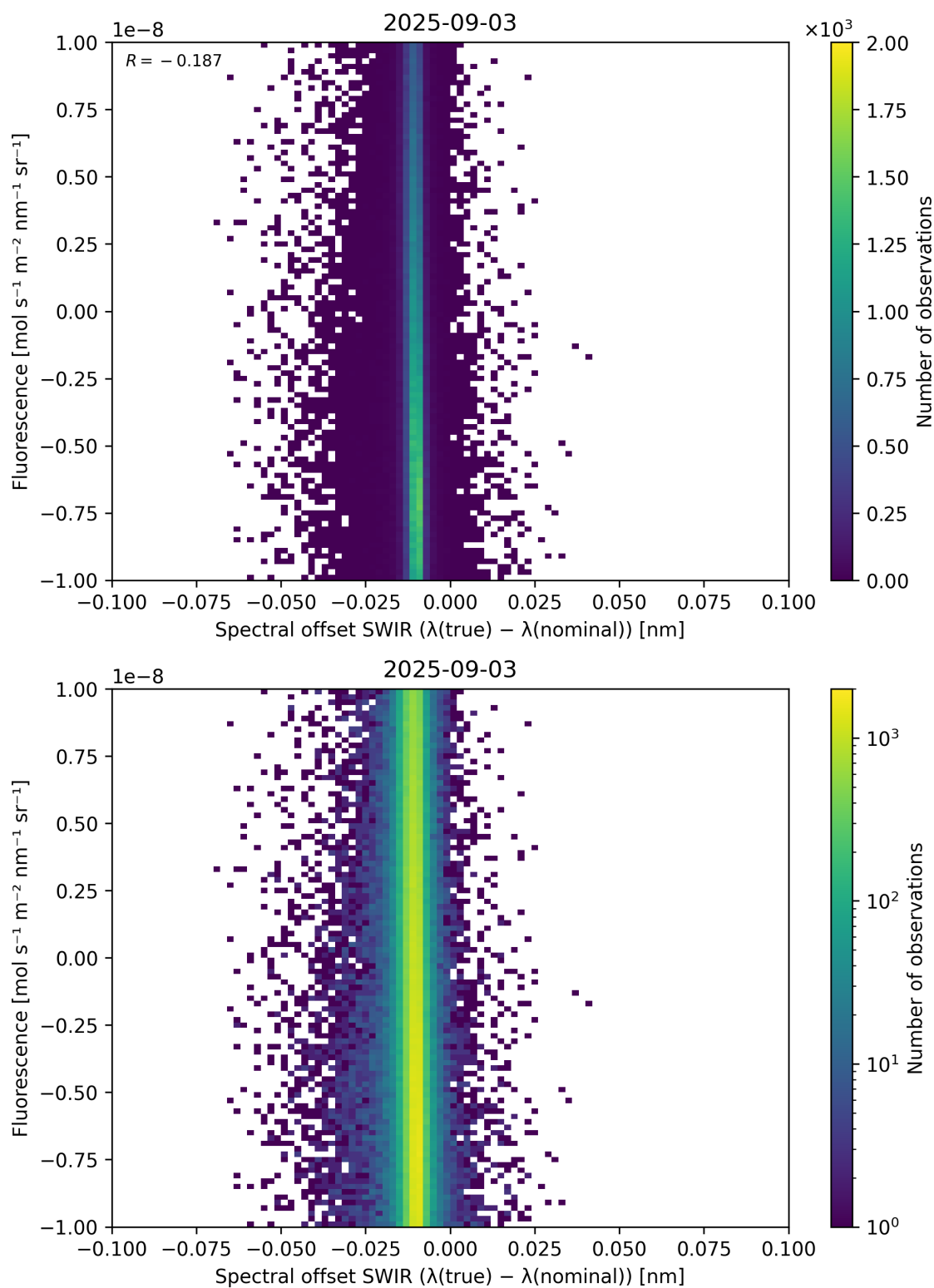
Figure 120: Scatter density plot of “Spectral offset SWIR ( \lambda_{\text{true}} - \lambda_{\text{nominal}} )” against “Fluorescence” for 2025-09-02 to 2025-09-04.
