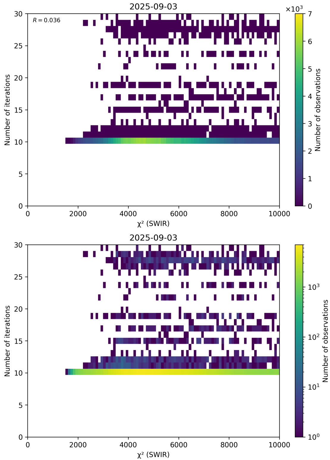
Figure 50: Scatter density plot of “ \chi^2 (SWIR)” against “Number of iterations” for 2025-09-02 to 2025-09-04.
