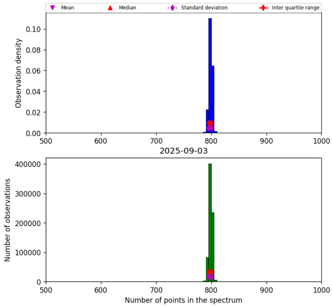
Figure 26: Histogram of “Number of points in the spectrum” for 2025-09-02 to 2025-09-04
