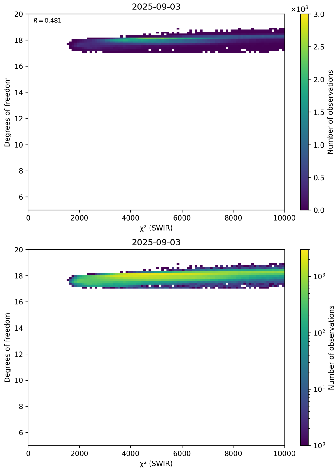
Figure 48: Scatter density plot of “ \chi^2 (SWIR)” against “Degrees of freedom” for 2025-09-02 to 2025-09-04.
