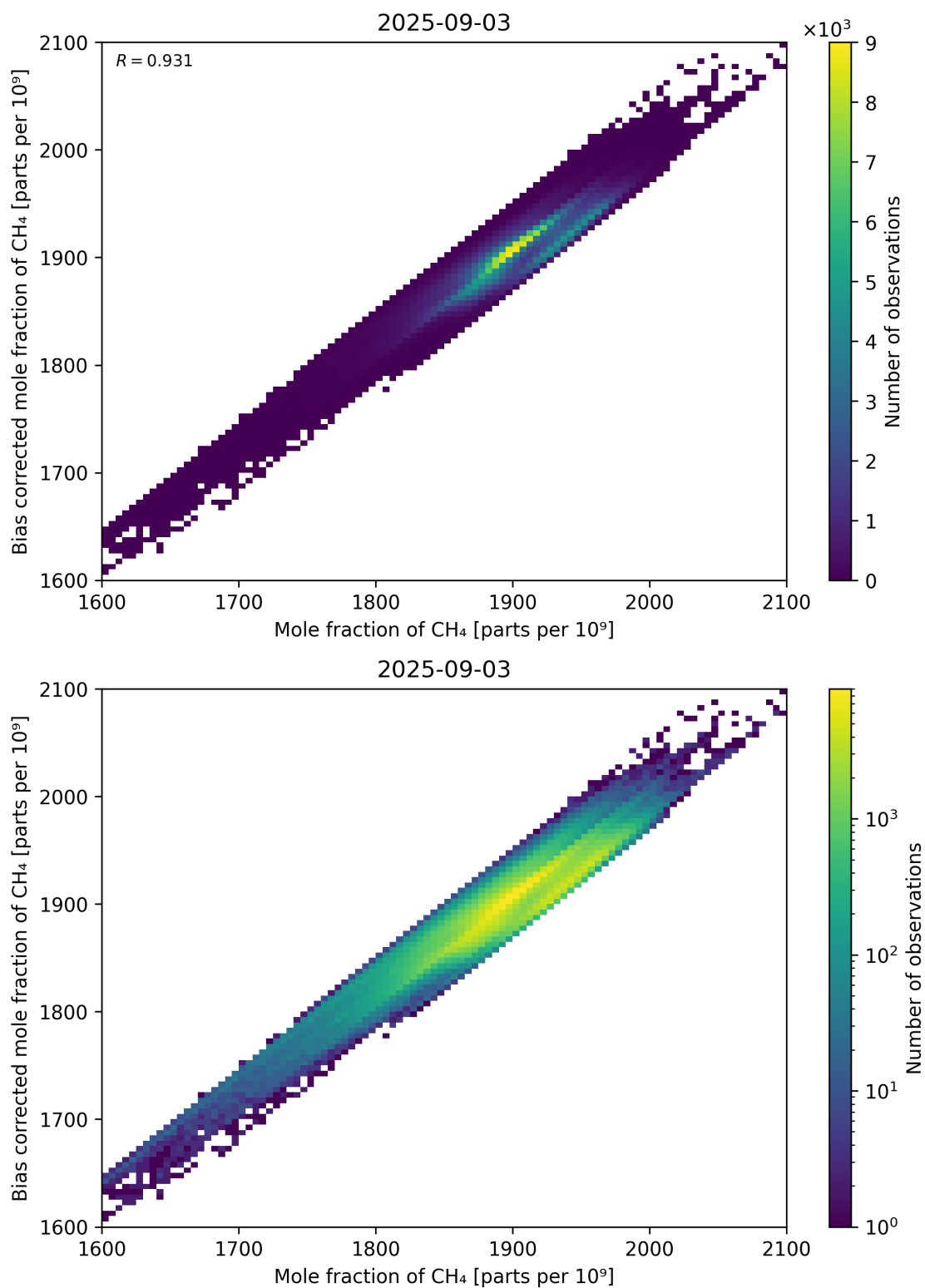
Figure 74: Scatter density plot of “Mole fraction of CH 4 ” against “Bias corrected mole fraction of CH 4 ” for 2025-09-02 to 2025-09-04.
