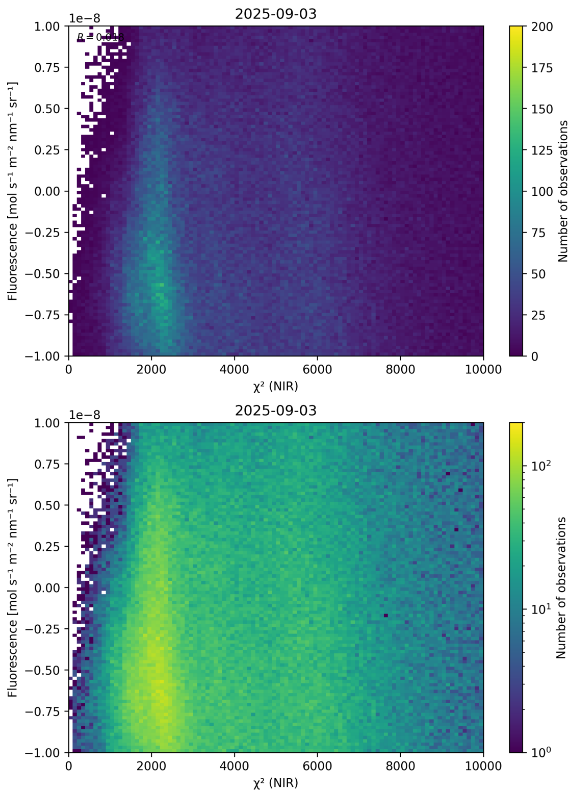
Figure 45: Scatter density plot of “ \chi^2 (NIR)” against “Fluorescence” for 2025-09-02 to 2025-09-04.
