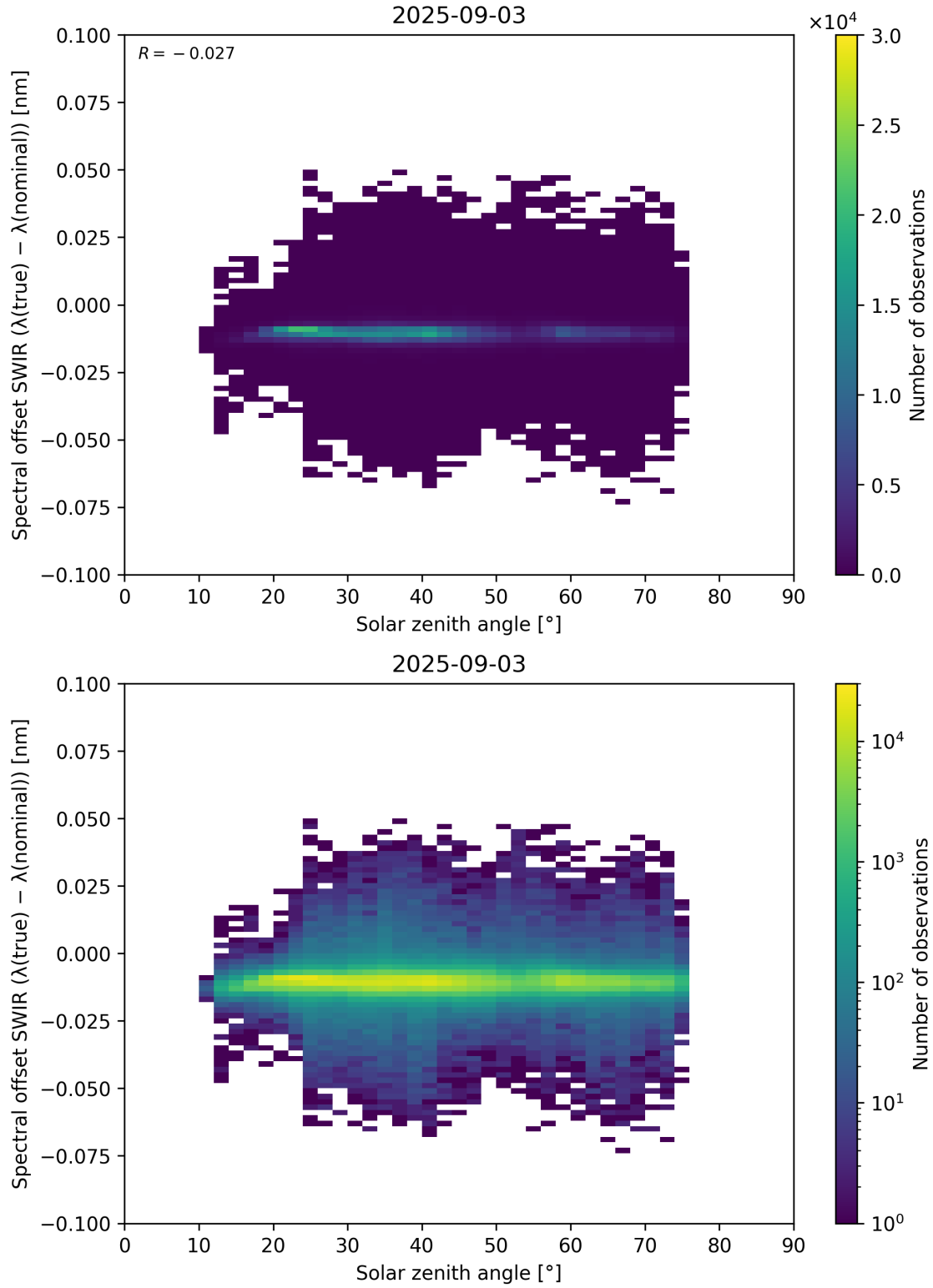
Figure 104: Scatter density plot of “Solar zenith angle” against “Spectral offset SWIR ( \lambda_{\text{true}} - \lambda_{\text{nominal}} )” for 2025-09-02 to 2025-09-04.
