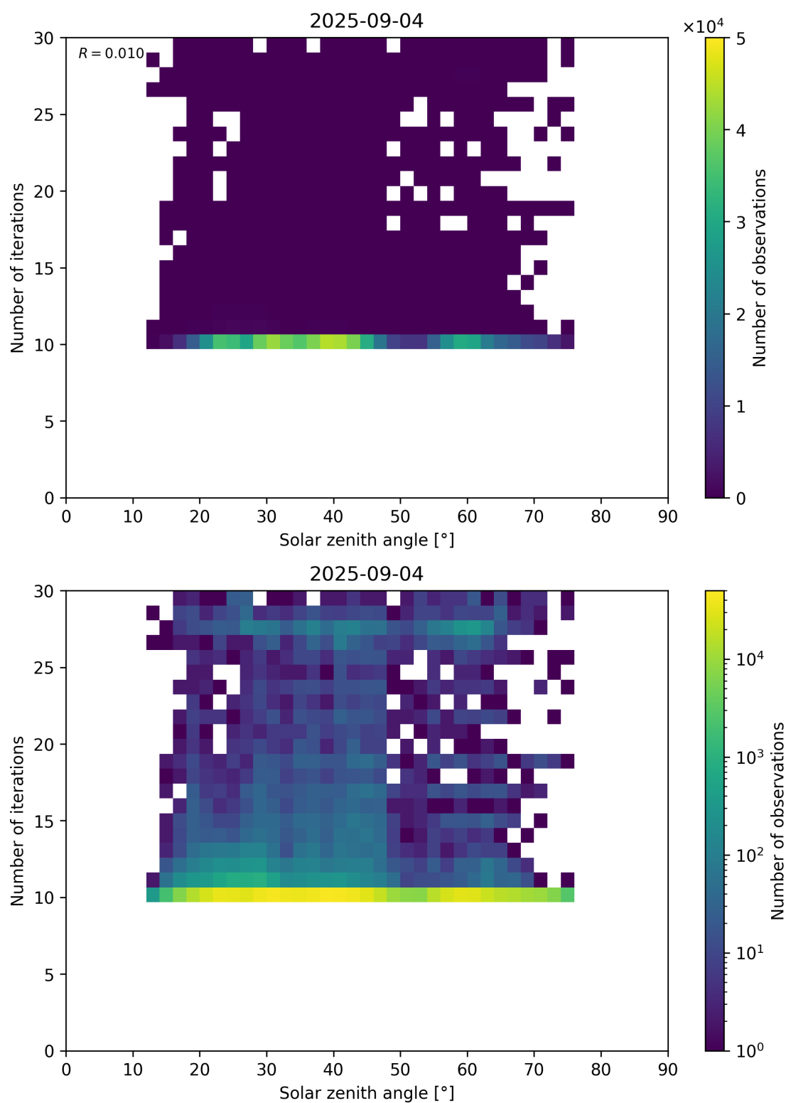
Figure 102: Scatter density plot of “Solar zenith angle” against “Number of iterations” for 2025-09-04 to 2025-09-05.
