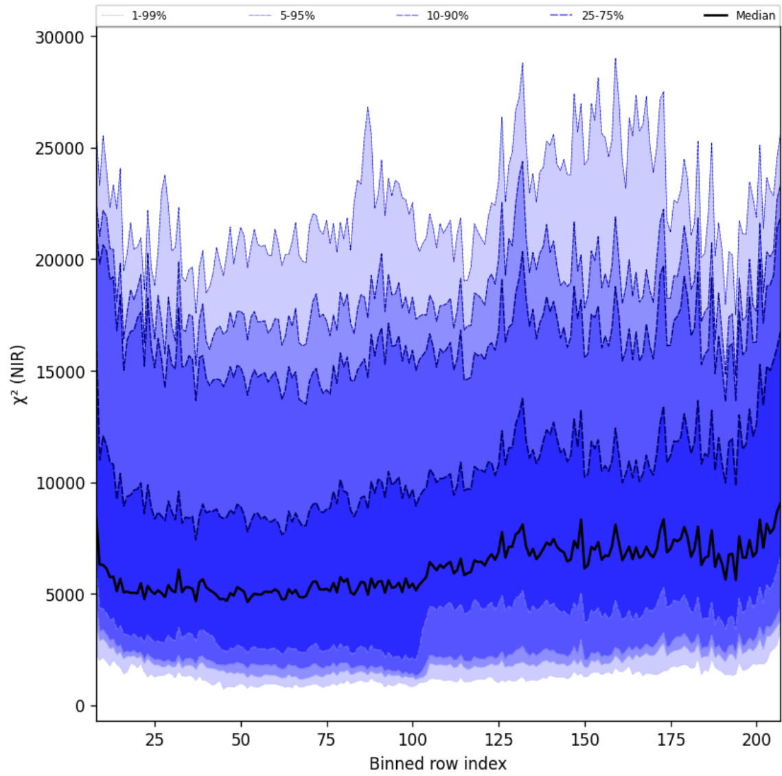
Figure 40: Along track statistics of " \chi^2 (NIR)" for 2025-09-04 to 2025-09-05
