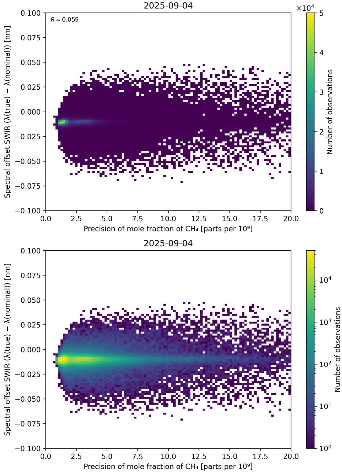
Figure 85: Scatter density plot of “Precision of mole fraction of \text{CH}_4 ” against “Spectral offset SWIR ( \lambda_{\text{true}} - \lambda_{\text{nominal}} )” for 2025-09-04 to 2025-09-05.
