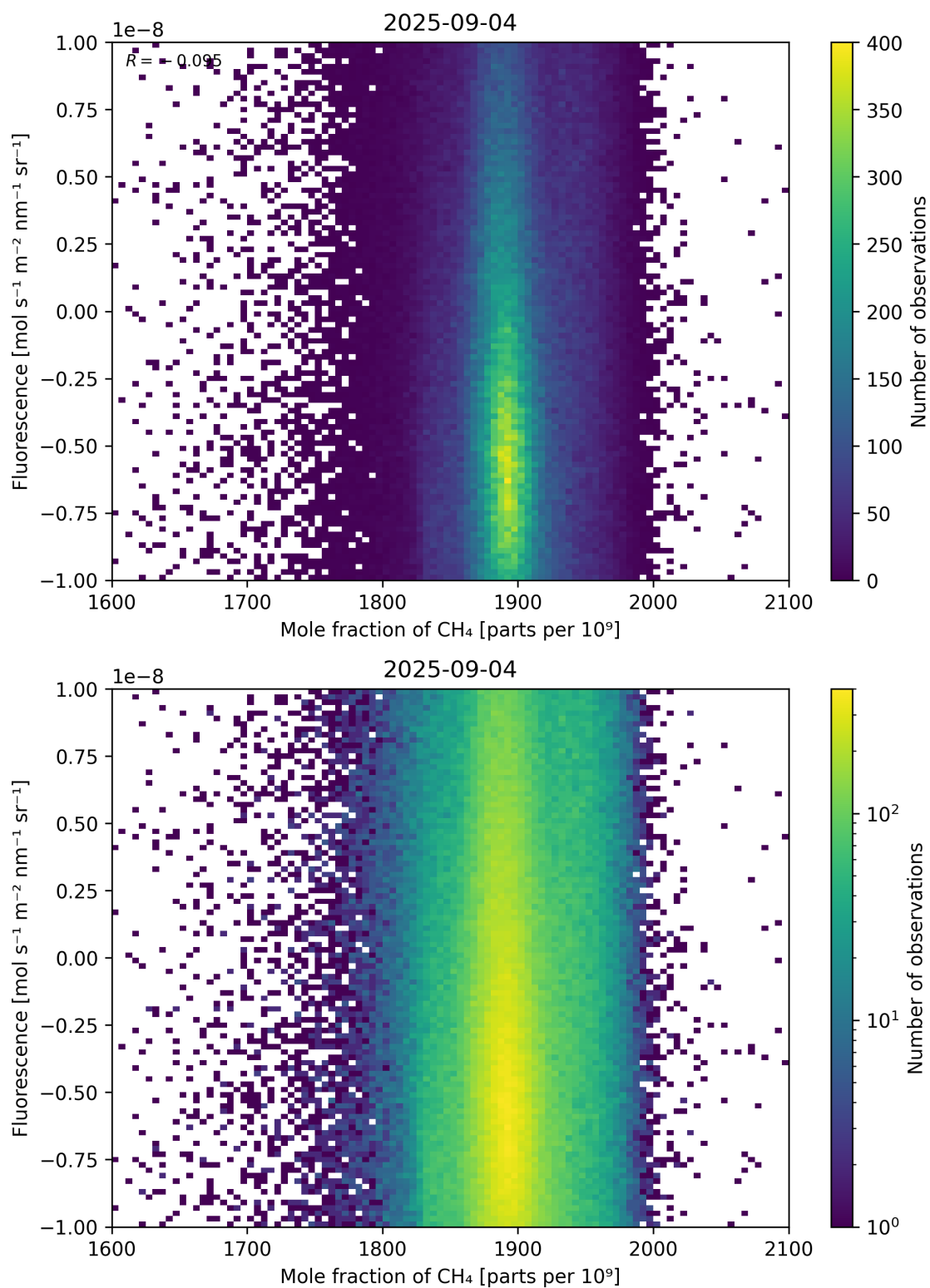
Figure 73: Scatter density plot of “Mole fraction of \text{CH}_4 ” against “Fluorescence” for 2025-09-04 to 2025-09-05.
