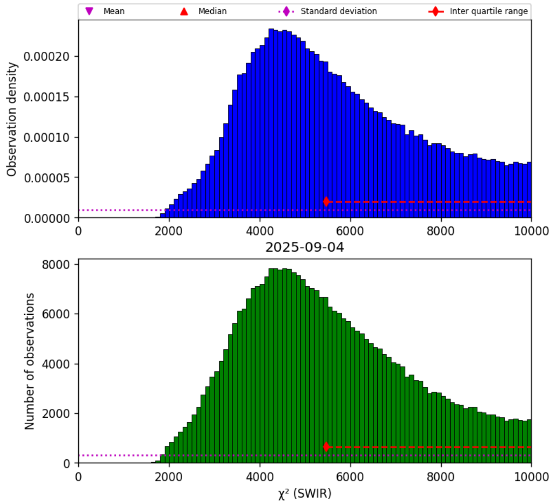
Figure 28: Histogram of “ \chi^2 (SWIR)” for 2025-09-04 to 2025-09-05
