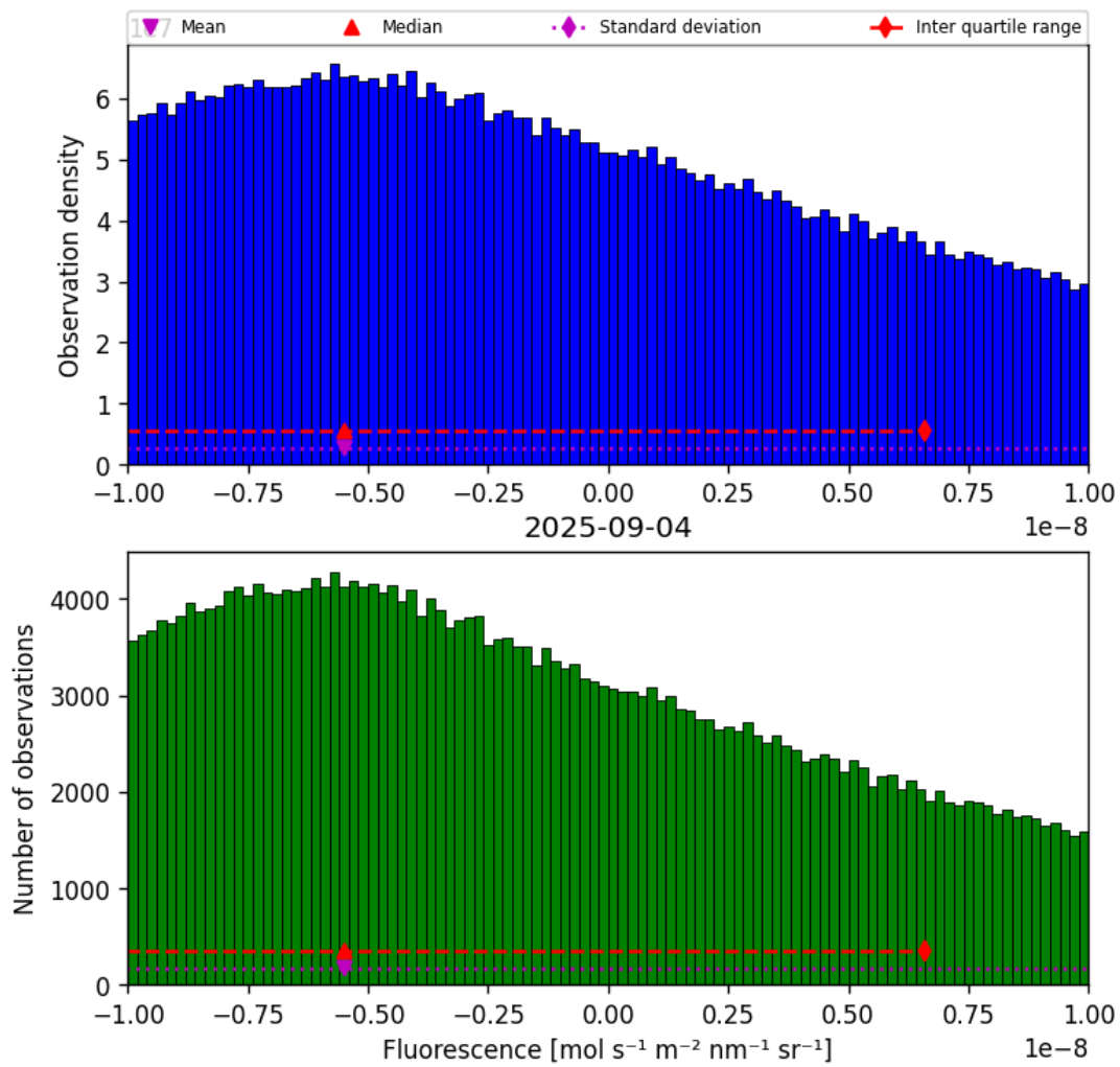
Figure 32: Histogram of “Fluorescence” for 2025-09-04 to 2025-09-05
