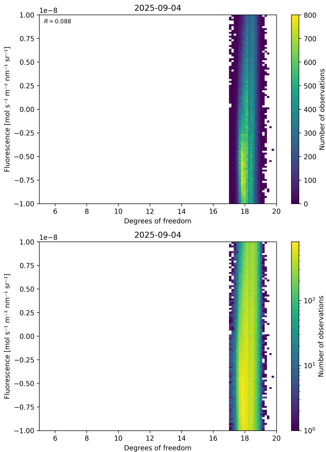
Figure 51: Scatter density plot of “Degrees of freedom” against “Fluorescence” for 2025-09-04 to 2025-09-05.
