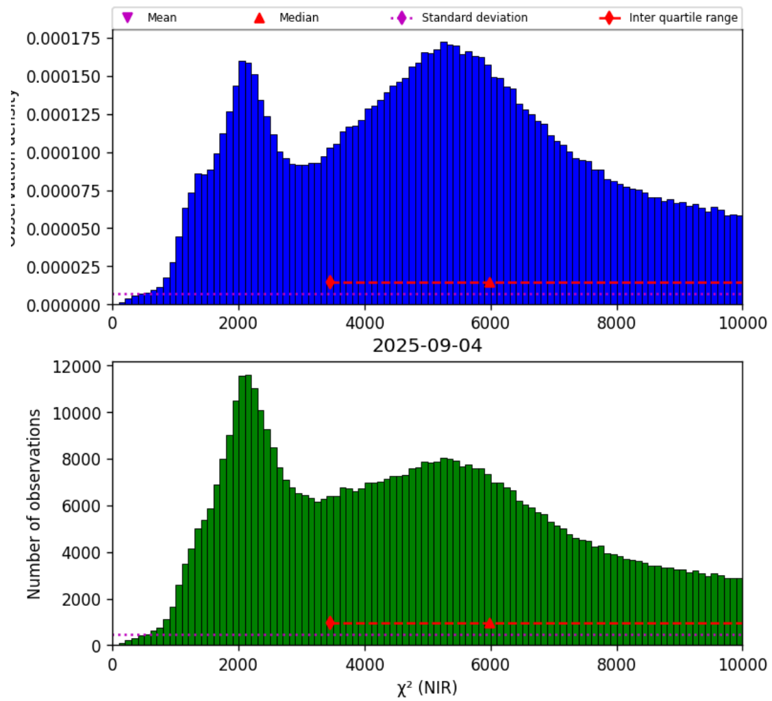
Figure 29: Histogram of “ \chi^2 (NIR)” for 2025-09-04 to 2025-09-05
