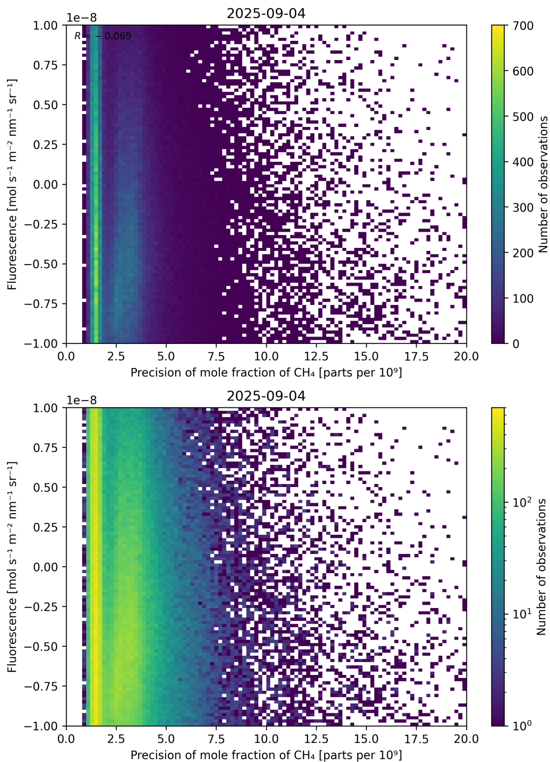
Figure 81: Scatter density plot of “Precision of mole fraction of \text{CH}_4 ” against “Fluorescence” for 2025-09-04 to 2025-09-05.
