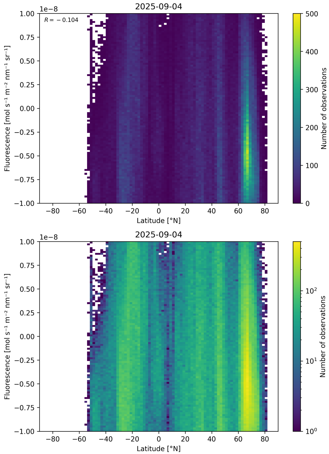
Figure 56: Scatter density plot of “Latitude” against “Fluorescence” for 2025-09-04 to 2025-09-05.
