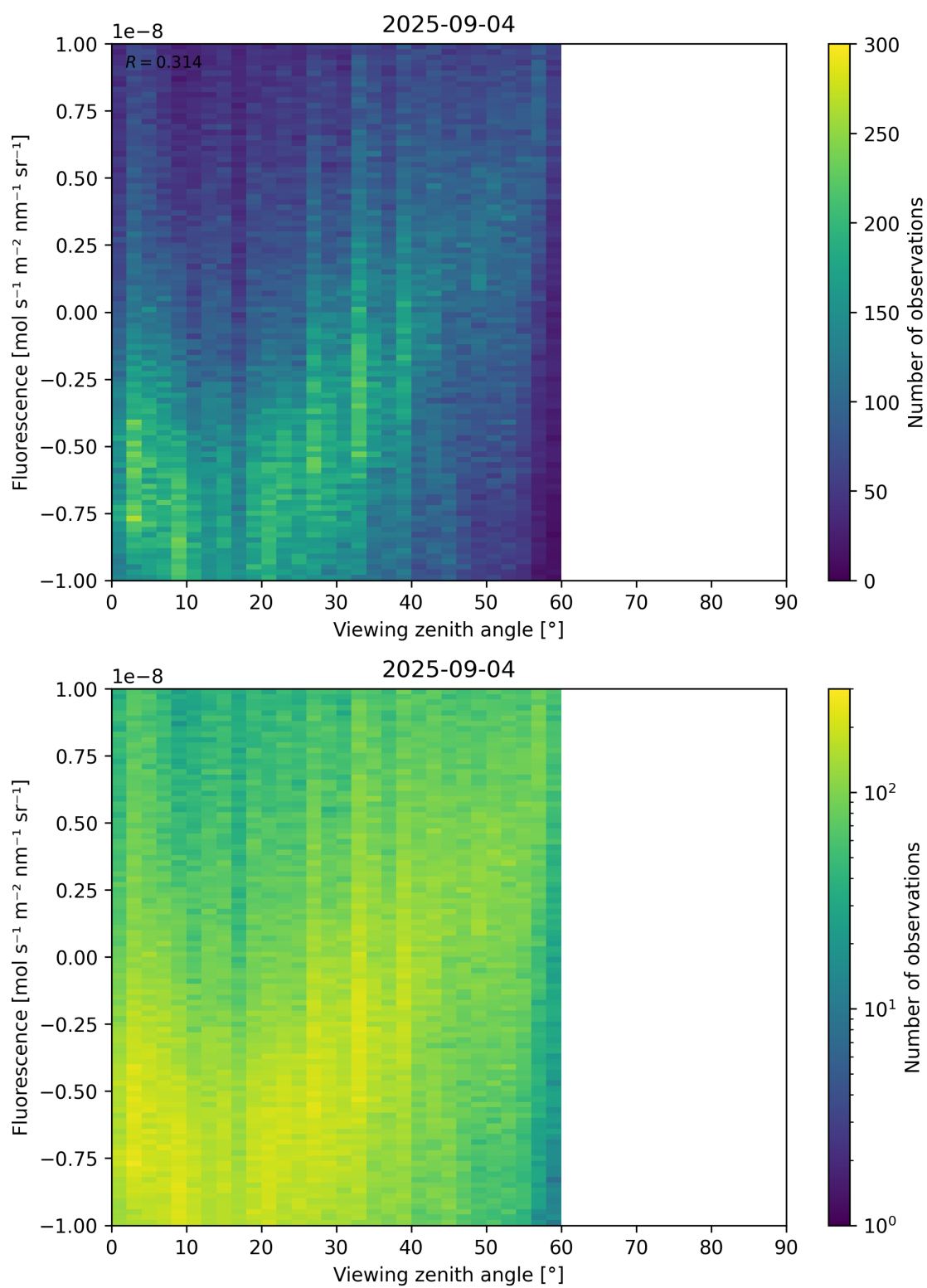
Figure 108: Scatter density plot of “Viewing zenith angle” against “Fluorescence” for 2025-09-04 to 2025-09-05.
