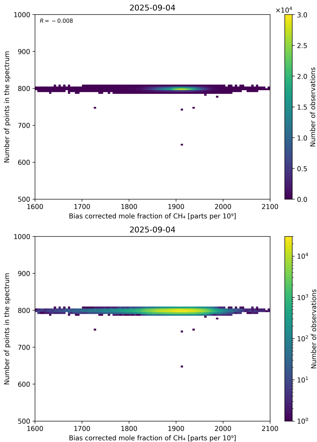
Figure 68: Scatter density plot of “Bias corrected mole fraction of CH 4 ” against “Number of points in the spectrum” for 2025-09-04 to 2025-09-05.
