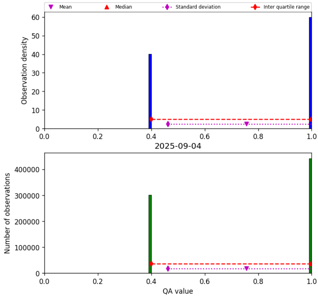
Figure 22: Histogram of “QA value” for 2025-09-04 to 2025-09-05
