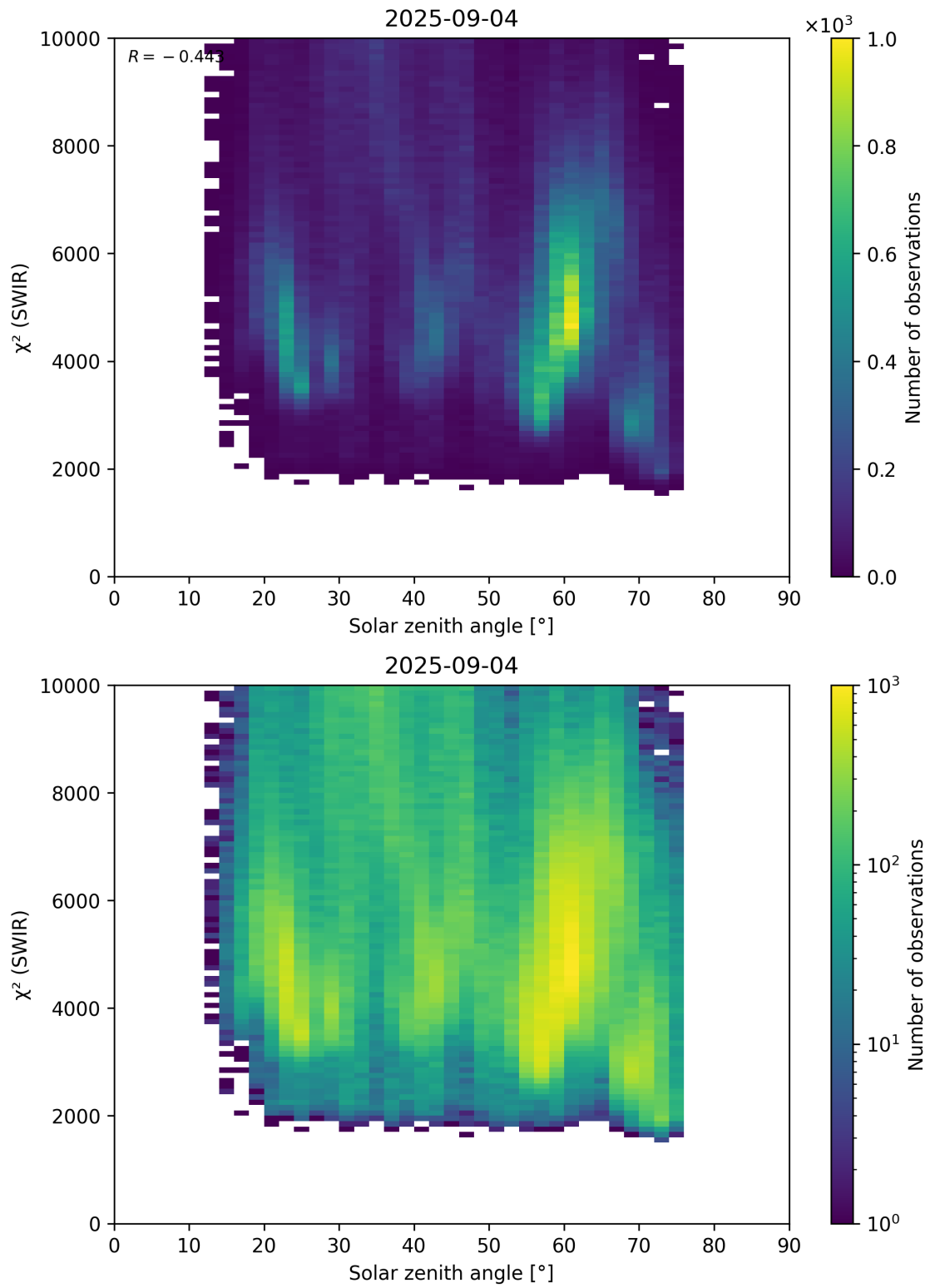
Figure 95: Scatter density plot of “Solar zenith angle” against “ \chi^2 (SWIR)” for 2025-09-04 to 2025-09-05.
