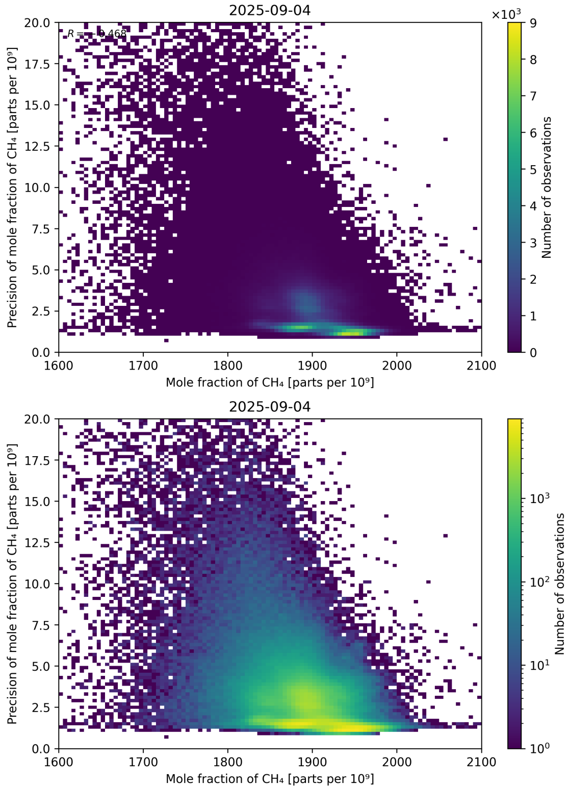
Figure 75: Scatter density plot of “Mole fraction of CH 4 ” against “Precision of mole fraction of CH 4 ” for 2025-09-04 to 2025-09-05.
