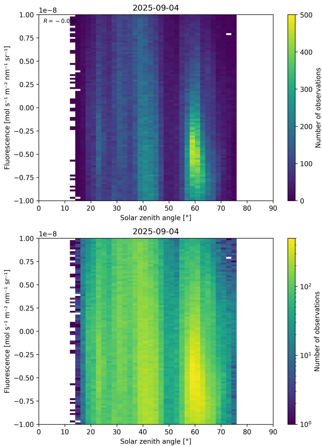
Figure 97: Scatter density plot of “Solar zenith angle” against “Fluorescence” for 2025-09-04 to 2025-09-05.
