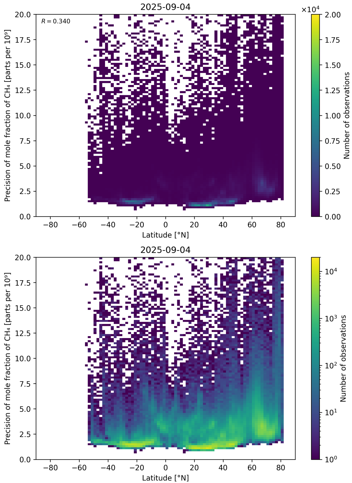
Figure 59: Scatter density plot of “Latitude” against “Precision of mole fraction of \text{CH}_4 ” for 2025-09-04 to 2025-09-05.
