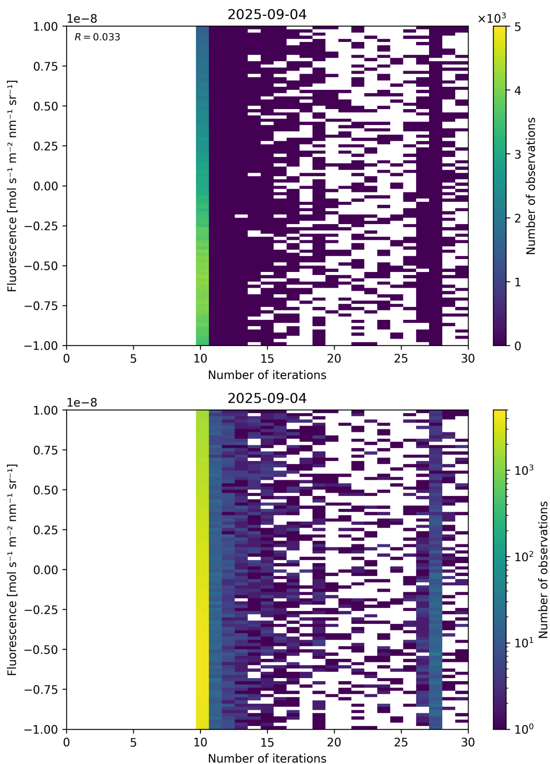
Figure 87: Scatter density plot of "Number of iterations" against "Fluorescence" for 2025-09-04 to 2025-09-05.
