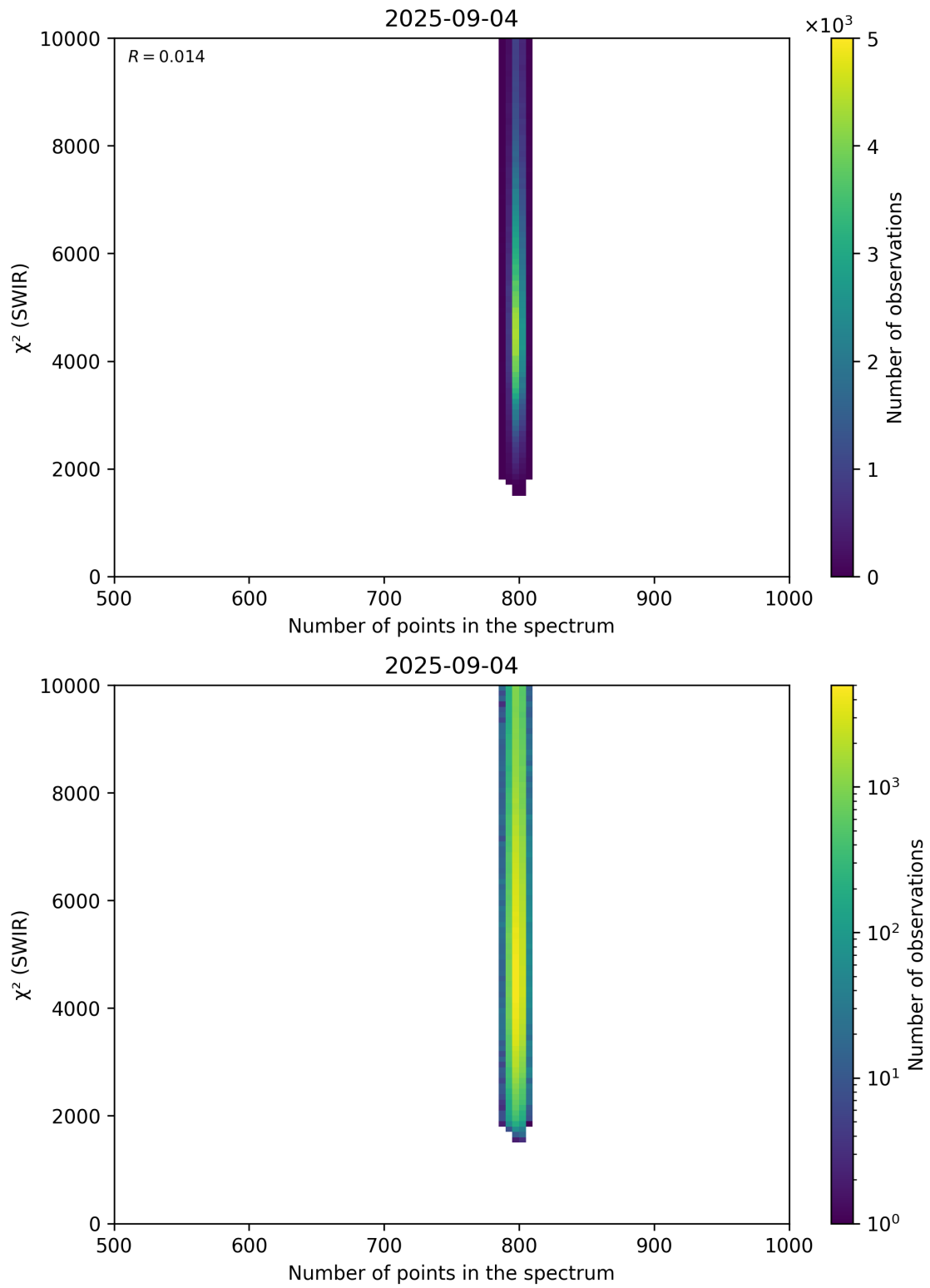
Figure 89: Scatter density plot of “Number of points in the spectrum” against “ \chi^2 (SWIR)” for 2025-09-04 to 2025-09-05.
