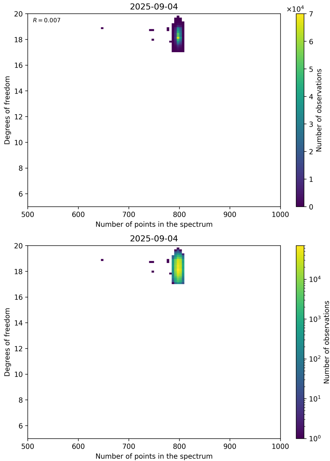
Figure 90: Scatter density plot of “Number of points in the spectrum” against “Degrees of freedom” for 2025-09-04 to 2025-09-05.
