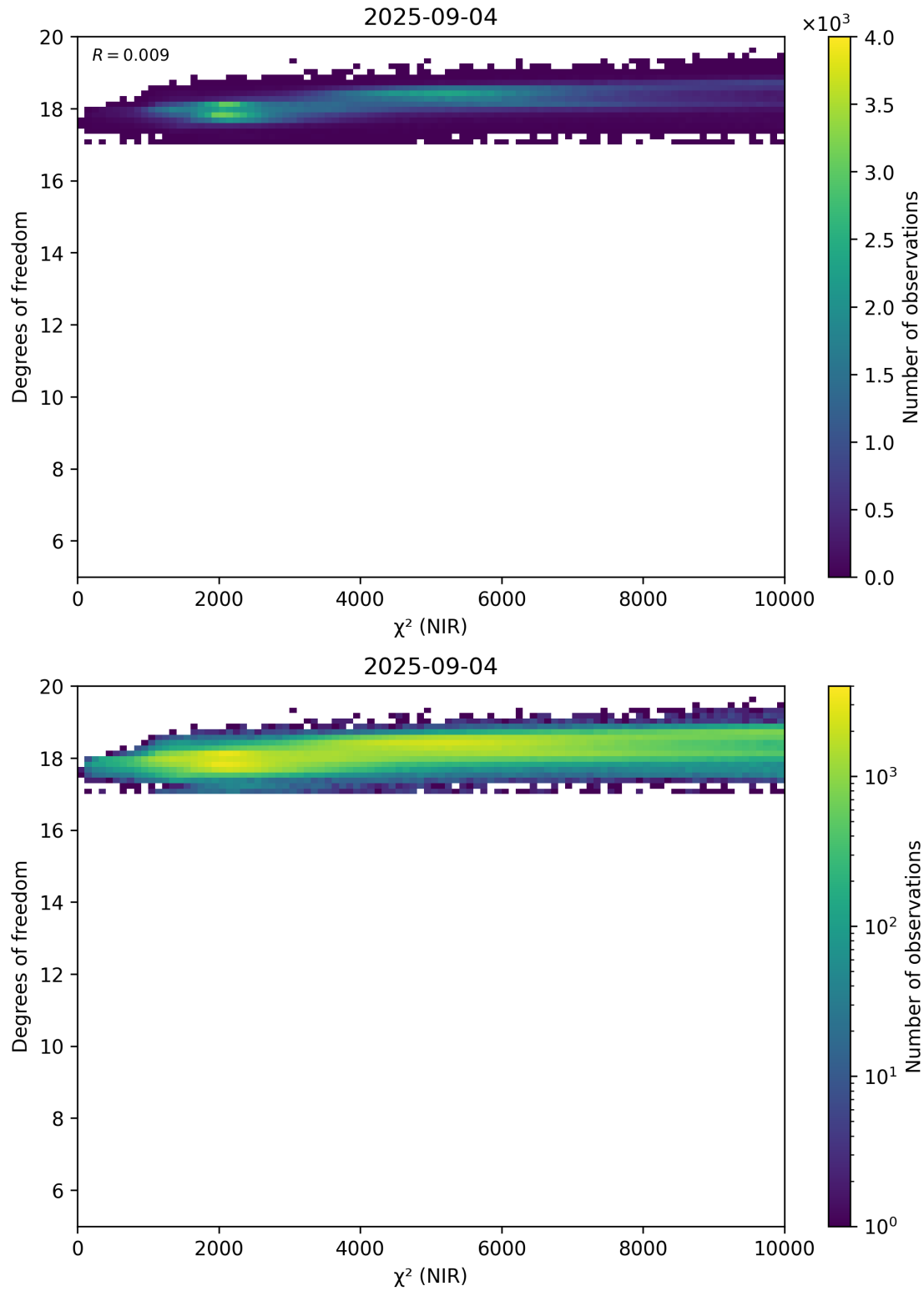
Figure 44: Scatter density plot of “ \chi^2 (NIR)” against “Degrees of freedom” for 2025-09-04 to 2025-09-05.
