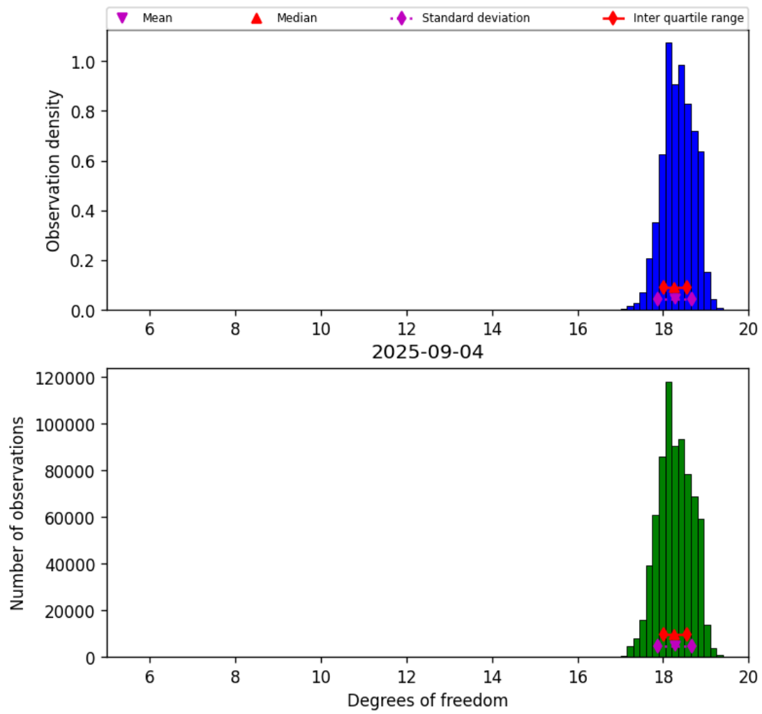
Figure 30: Histogram of “Degrees of freedom” for 2025-09-04 to 2025-09-05
