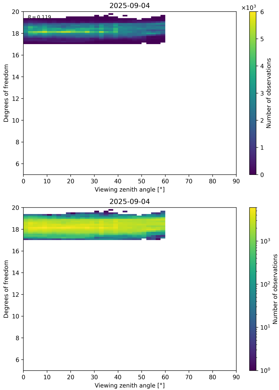
Figure 107: Scatter density plot of “Viewing zenith angle” against “Degrees of freedom” for 2025-09-04 to 2025-09-05.
