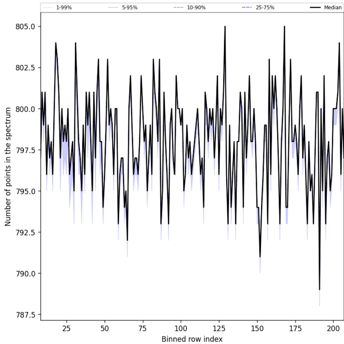
Figure 37: Along track statistics of “Number of points in the spectrum” for 2025-09-04 to 2025-09-05
