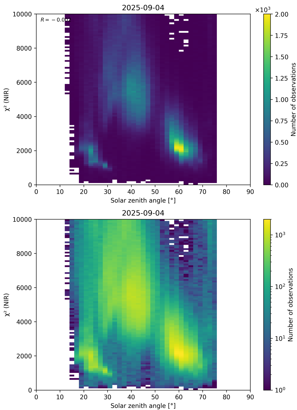
Figure 94: Scatter density plot of “Solar zenith angle” against “ \chi^2 (NIR)” for 2025-09-04 to 2025-09-05.
