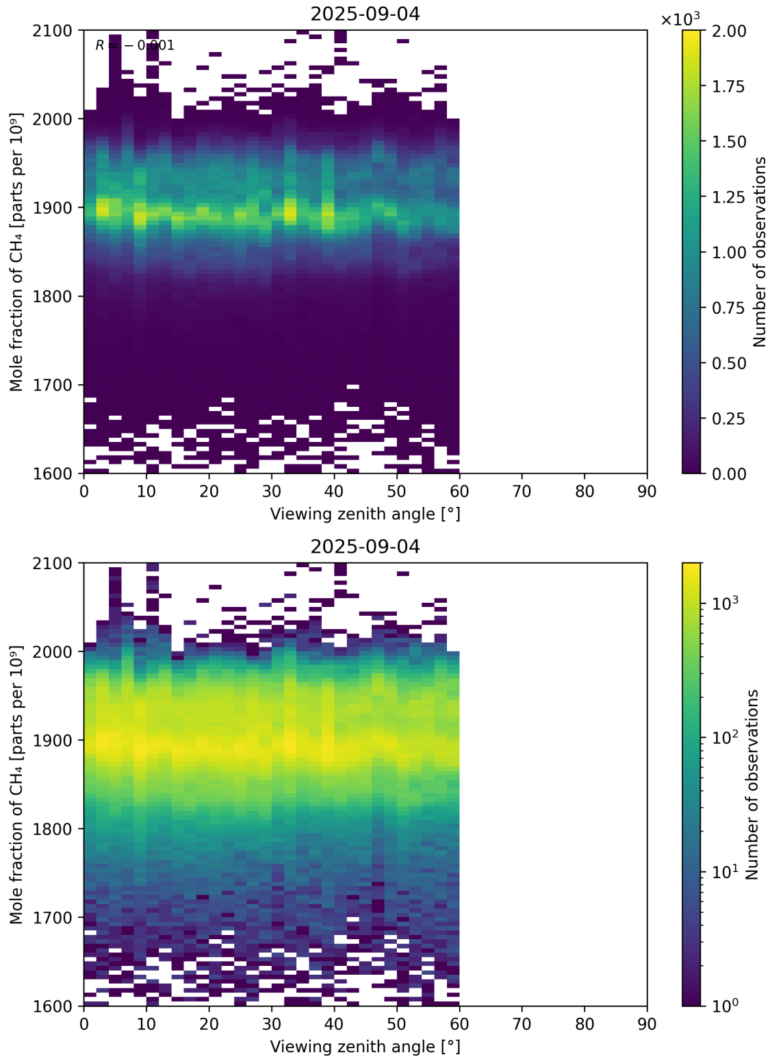
Figure 110: Scatter density plot of “Viewing zenith angle” against “Mole fraction of CH 4 ” for 2025-09-04 to 2025-09-05.
