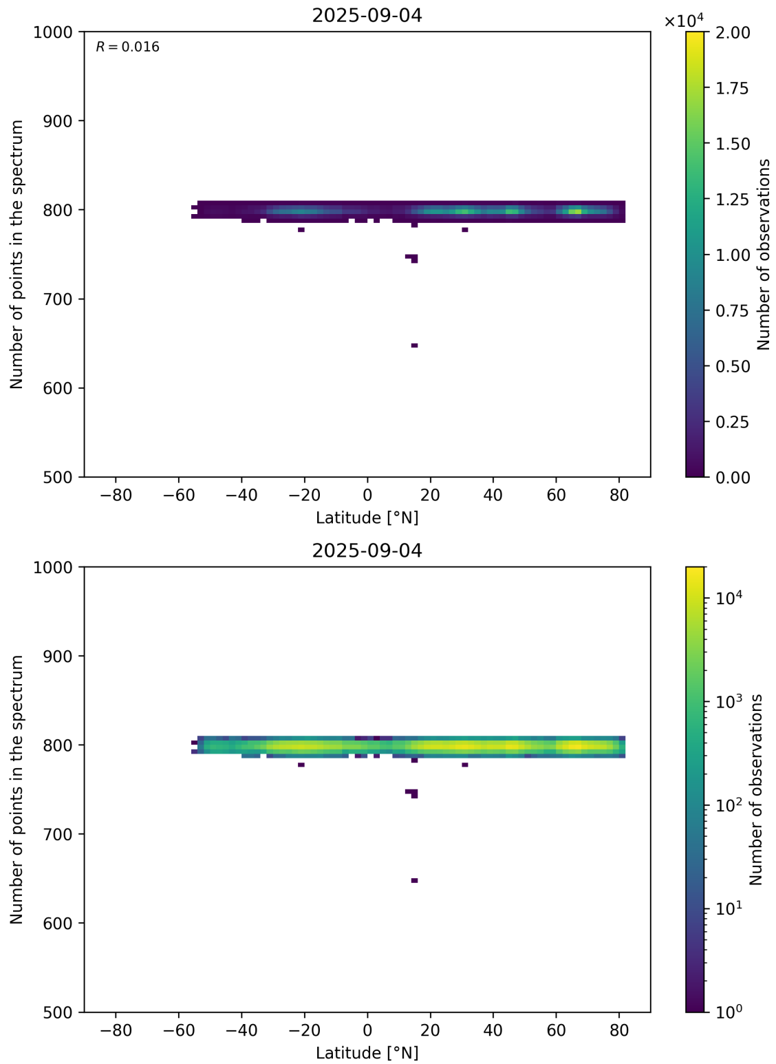
Figure 61: Scatter density plot of “Latitude” against “Number of points in the spectrum” for 2025-09-04 to 2025-09-05.
