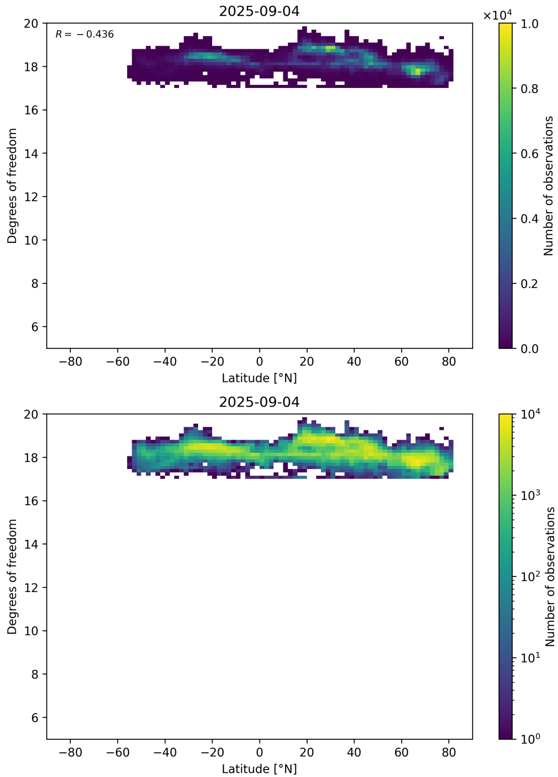
Figure 55: Scatter density plot of “Latitude” against “Degrees of freedom” for 2025-09-04 to 2025-09-05.
