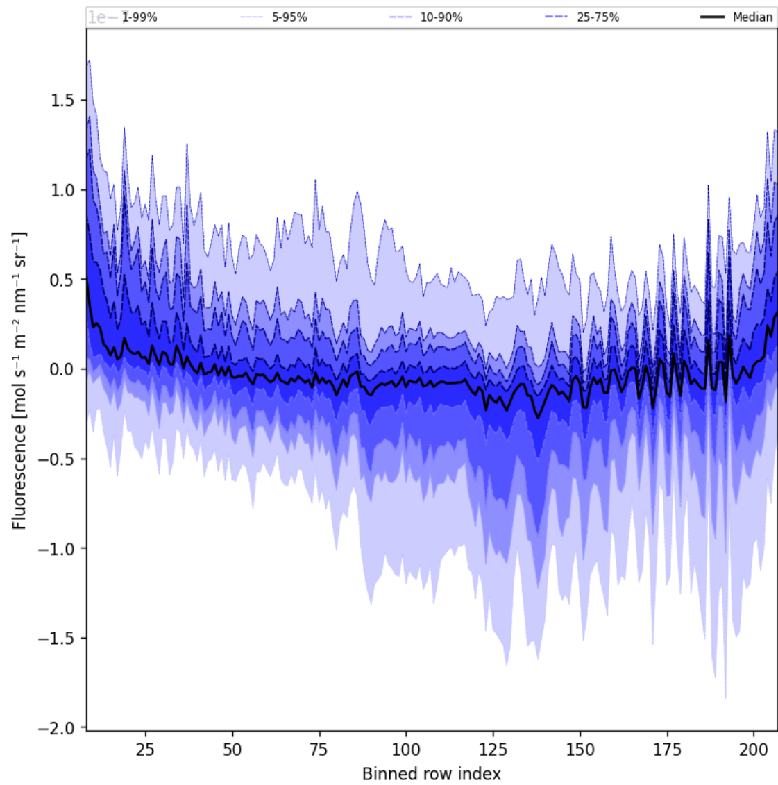
Figure 43: Along track statistics of “Fluorescence” for 2025-09-04 to 2025-09-05
