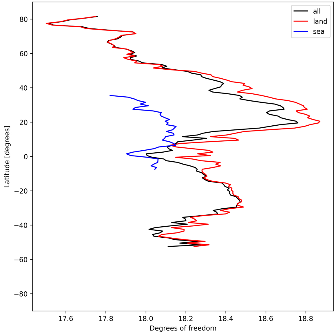
Figure 19: Zonal average of “Degrees of freedom” for 2025-09-04 to 2025-09-05.
