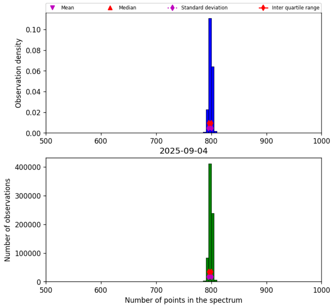
Figure 26: Histogram of “Number of points in the spectrum” for 2025-09-04 to 2025-09-05
