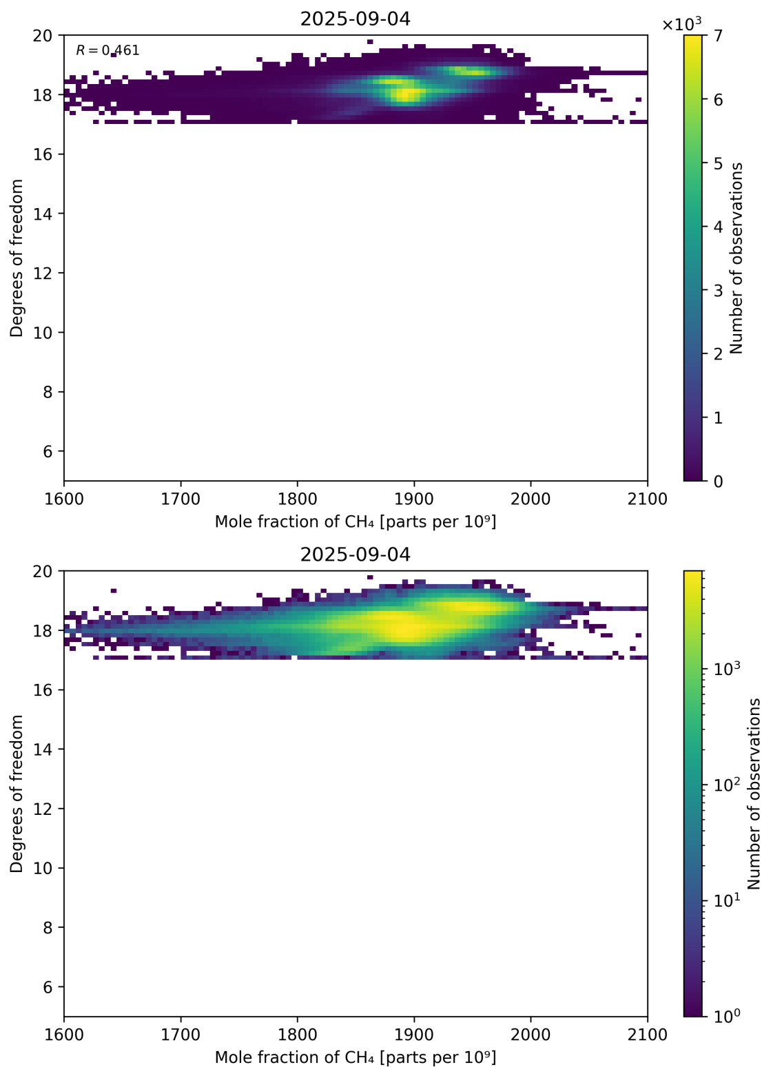
Figure 72: Scatter density plot of “Mole fraction of CH 4 ” against “Degrees of freedom” for 2025-09-04 to 2025-09-05.
