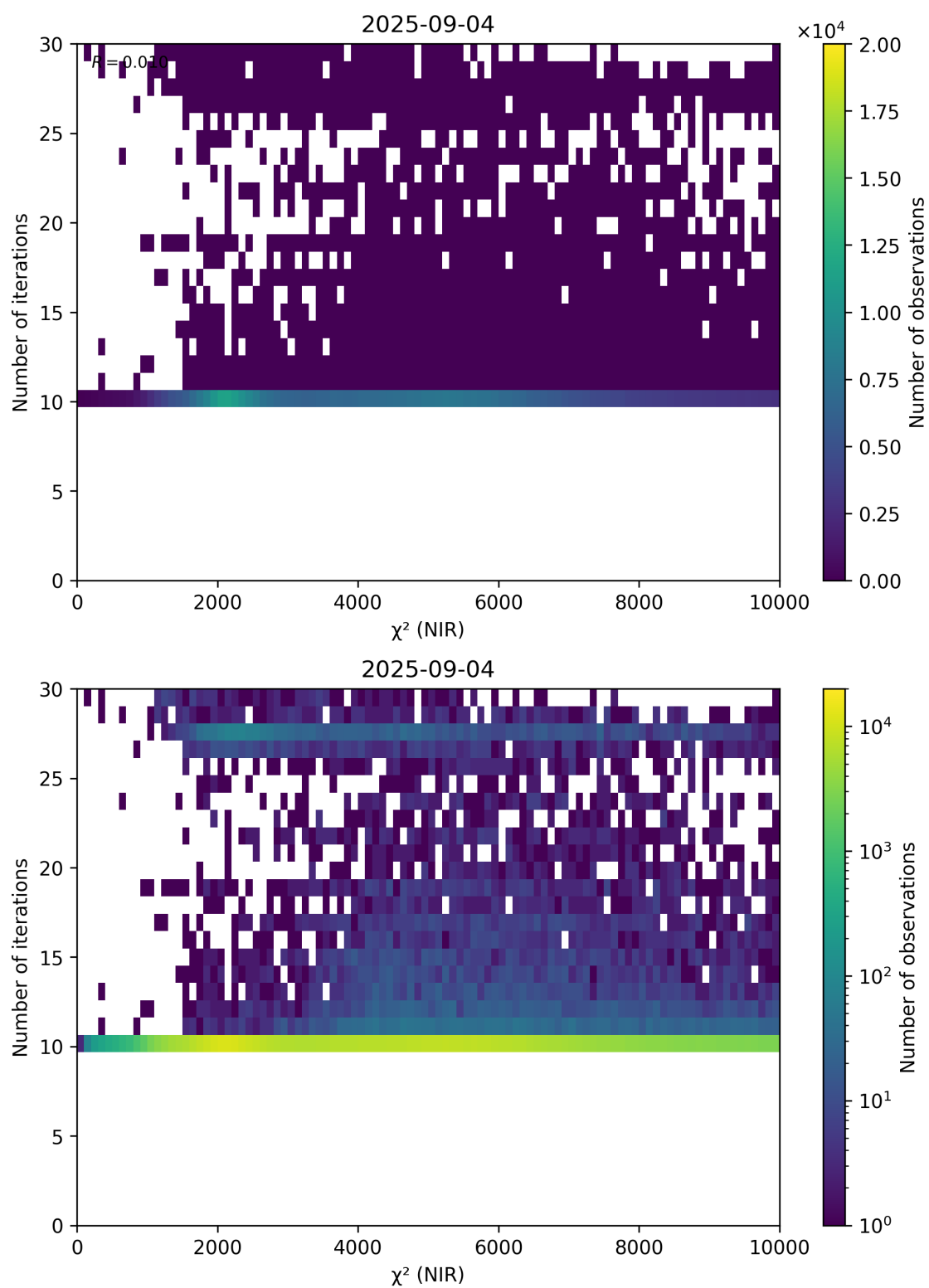
Figure 46: Scatter density plot of “ \chi^2 (NIR)” against “Number of iterations” for 2025-09-04 to 2025-09-05.
