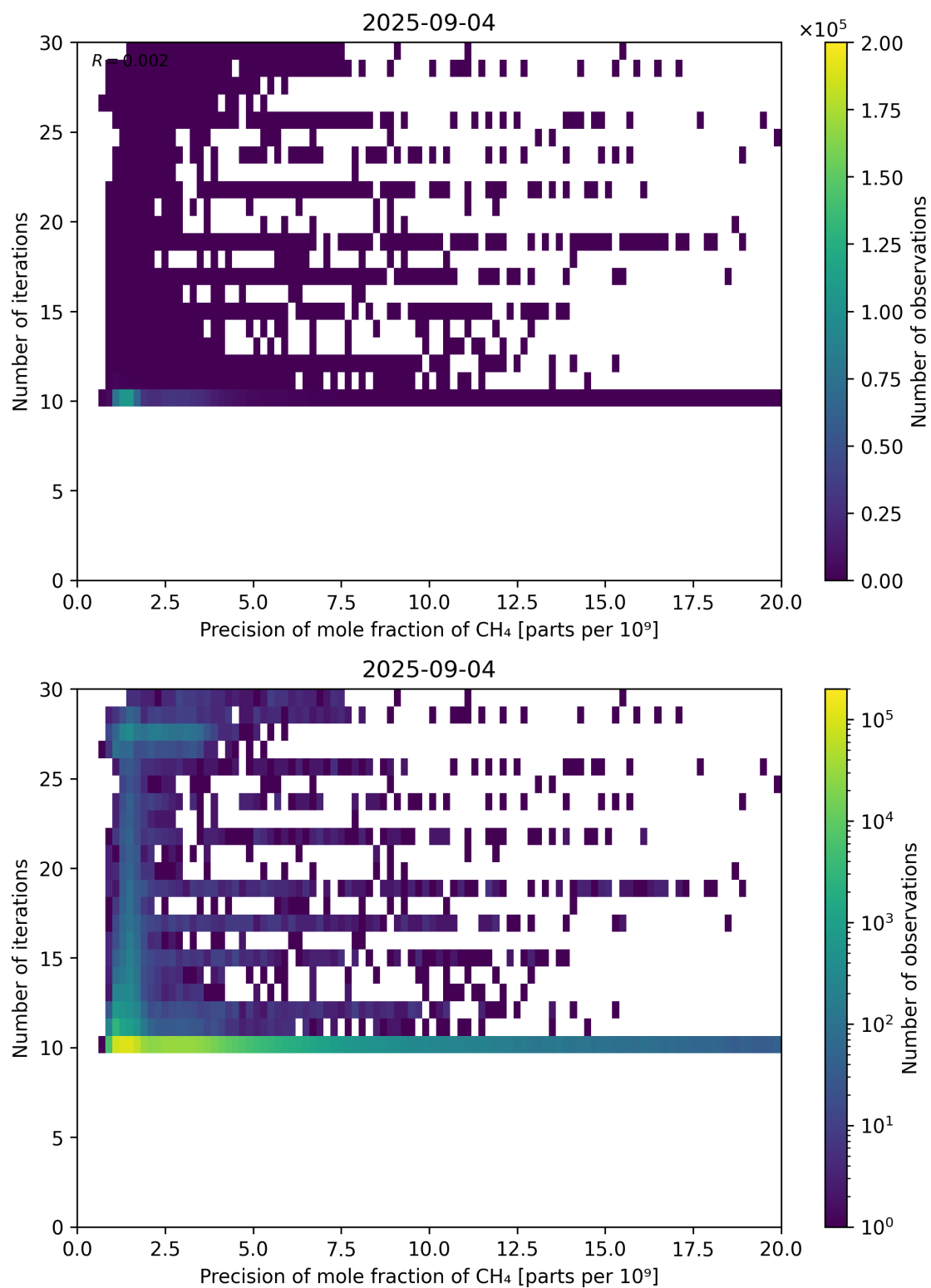
Figure 83: Scatter density plot of “Precision of mole fraction of CH 4 ” against “Number of iterations” for 2025-09-04 to 2025-09-05.
