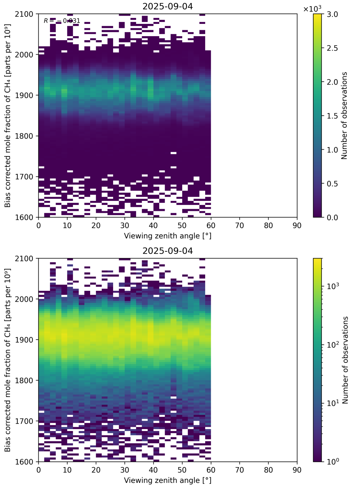
Figure 111: Scatter density plot of “Viewing zenith angle” against “Bias corrected mole fraction of CH 4 ” for 2025-09-04 to 2025-09-05.
