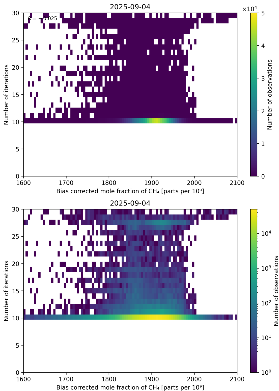
Figure 67: Scatter density plot of “Bias corrected mole fraction of CH 4 ” against “Number of iterations” for 2025-09-04 to 2025-09-05.
