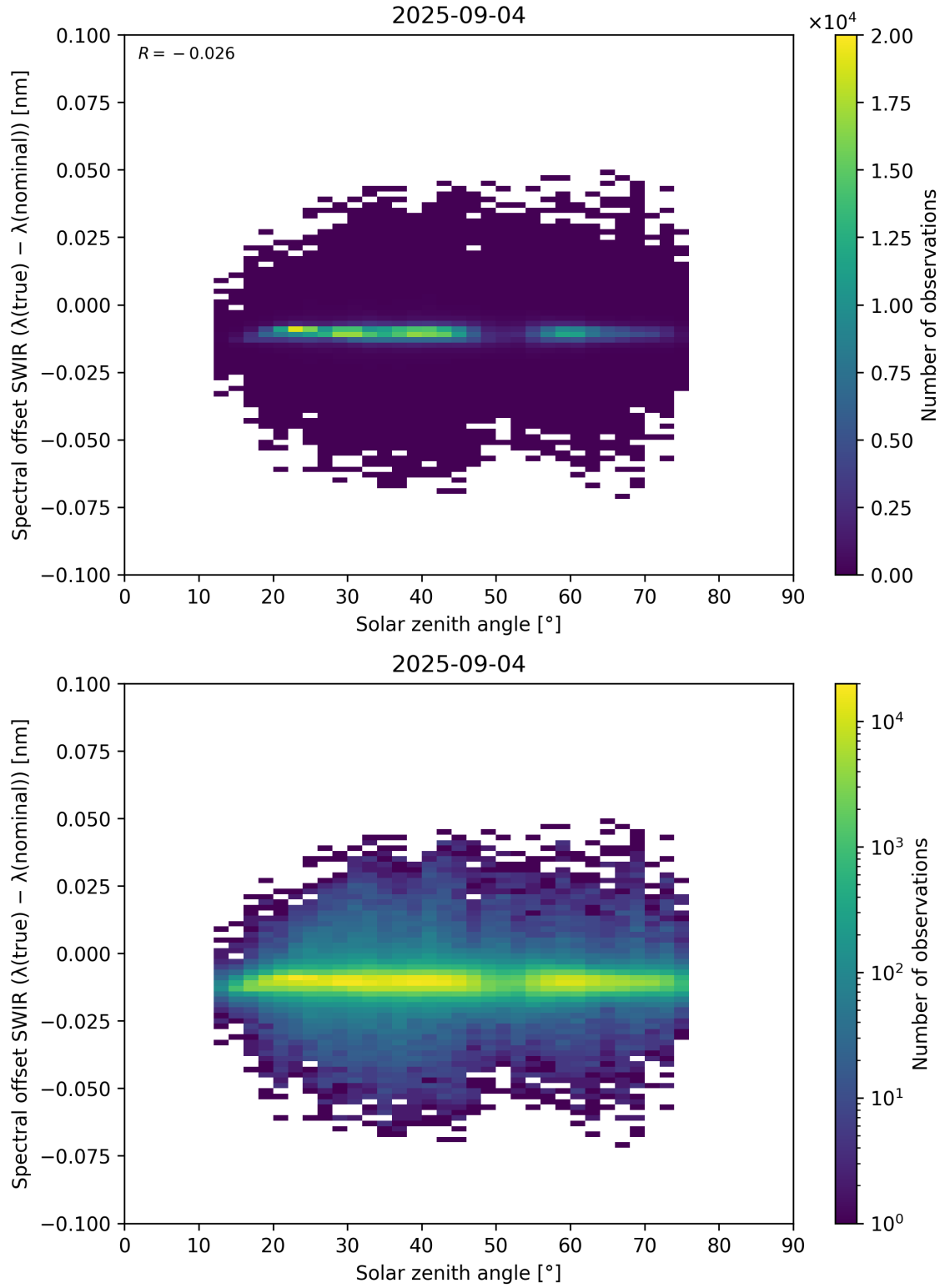
Figure 104: Scatter density plot of “Solar zenith angle” against “Spectral offset SWIR ( \lambda_{\text{true}} - \lambda_{\text{nominal}} )” for 2025-09-04 to 2025-09-05.
