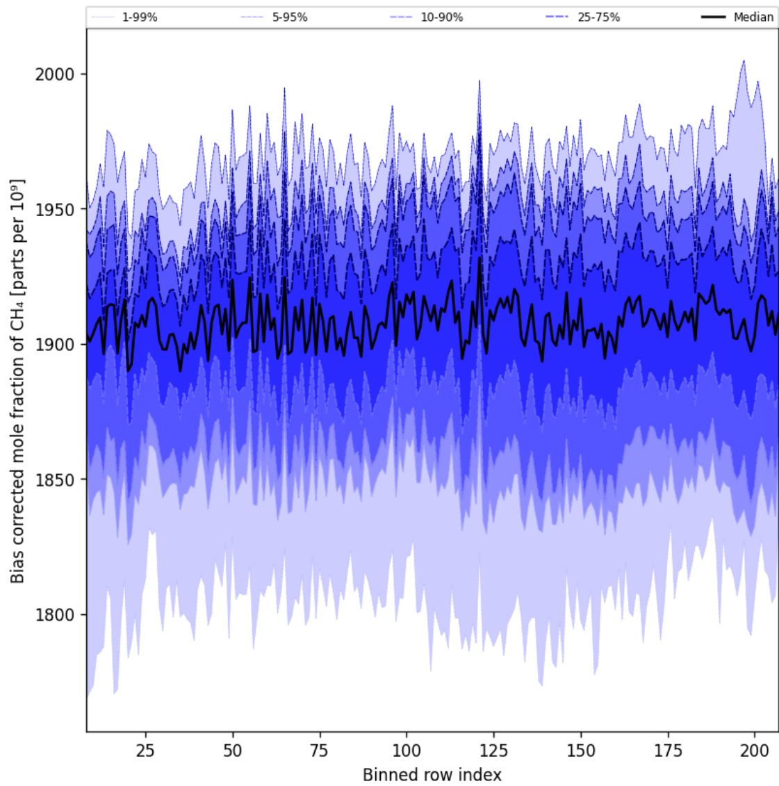
Figure 36: Along track statistics of “Bias corrected mole fraction of CH 4 ” for 2025-09-04 to 2025-09-05
