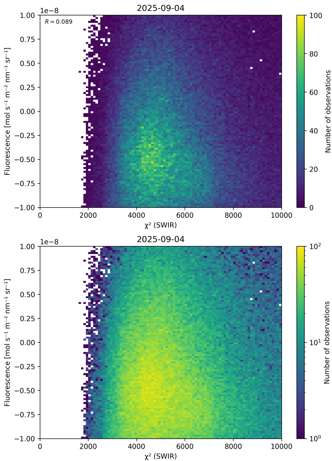
Figure 49: Scatter density plot of “ \chi^2 (SWIR)” against “Fluorescence” for 2025-09-04 to 2025-09-05.
