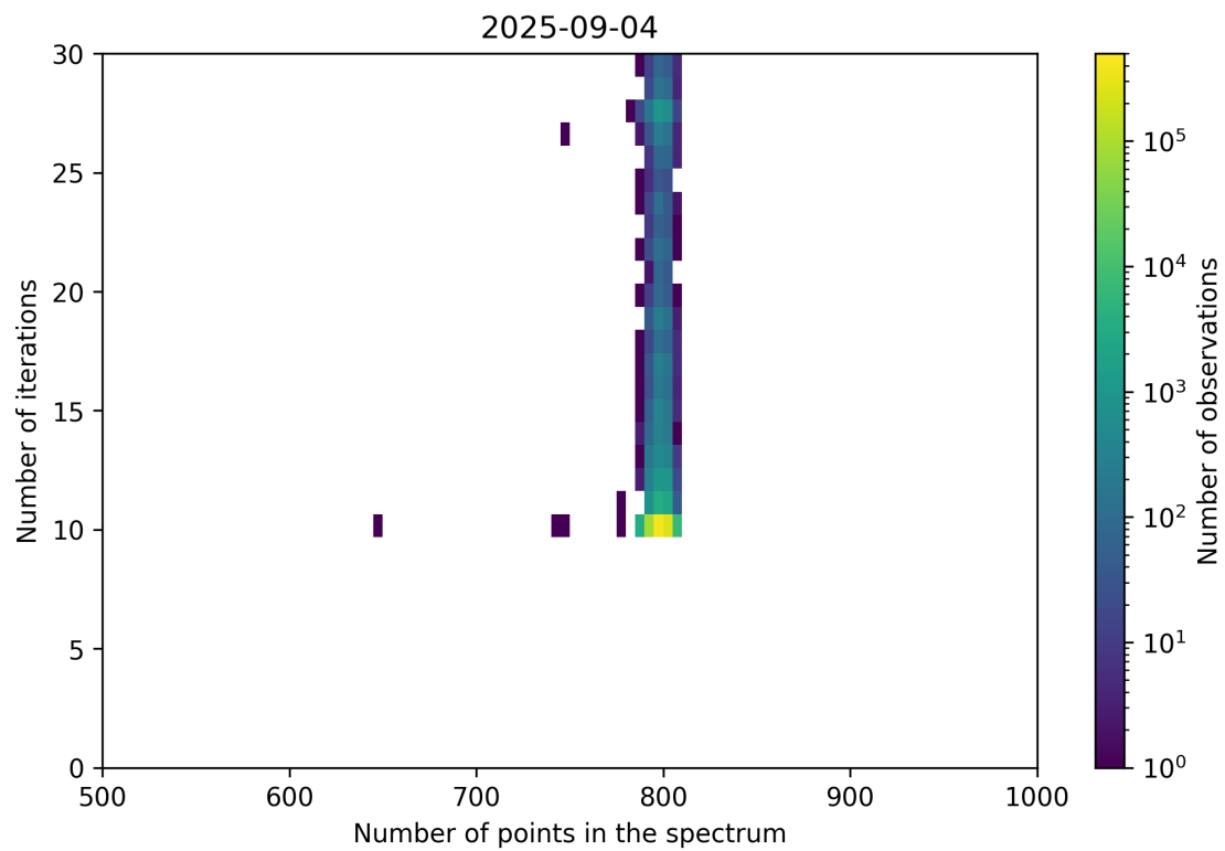
Figure 92: Scatter density plot of “Number of points in the spectrum” against “Number of iterations” for 2025-09-04 to 2025-09-05.
