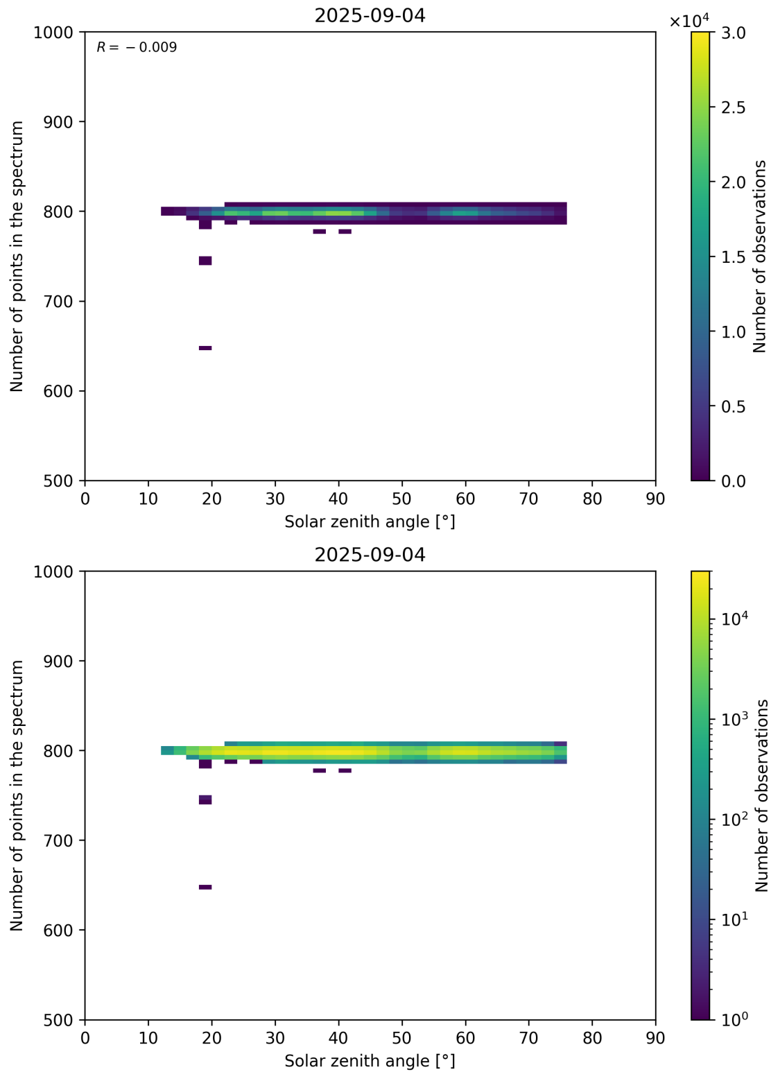
Figure 103: Scatter density plot of “Solar zenith angle” against “Number of points in the spectrum” for 2025-09-04 to 2025-09-05.
