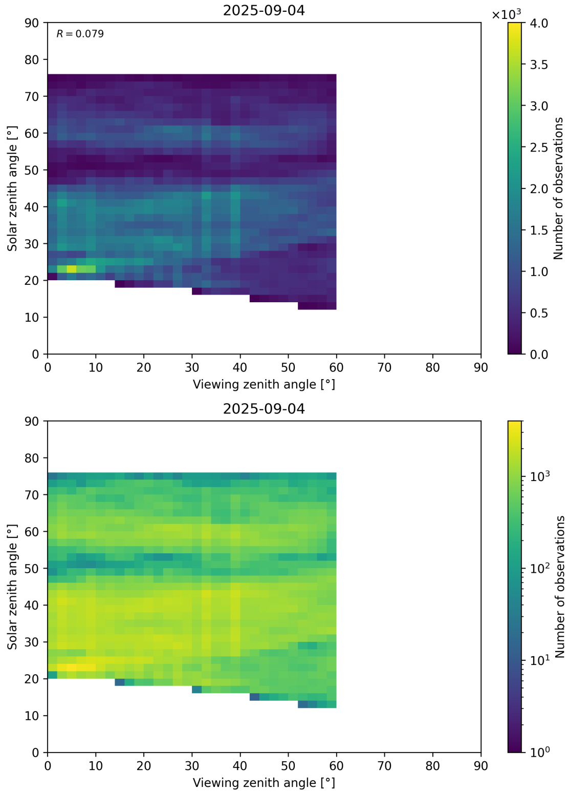
Figure 115: Scatter density plot of “Viewing zenith angle” against “Solar zenith angle” for 2025-09-04 to 2025-09-05.
