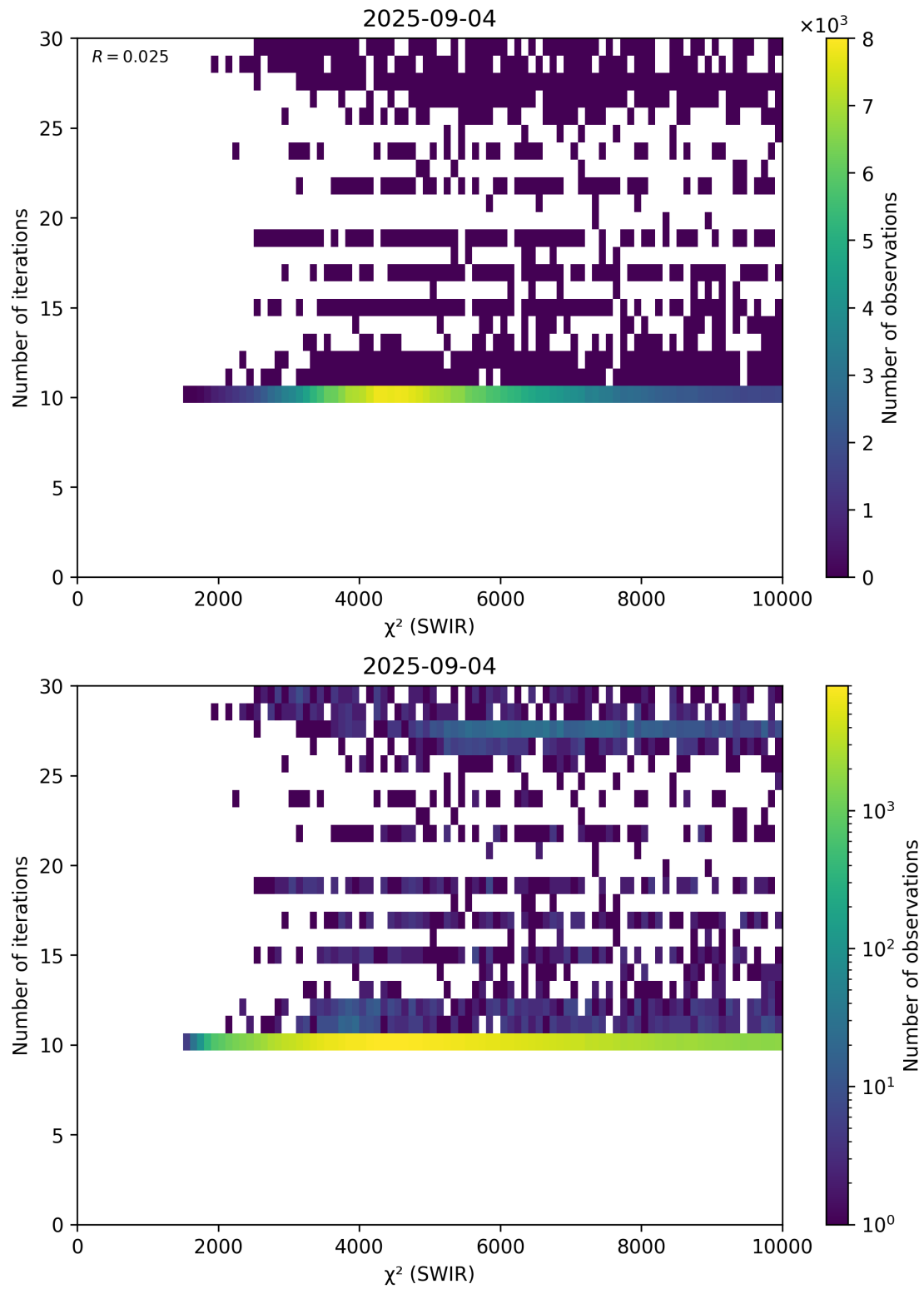
Figure 50: Scatter density plot of “ \chi^2 (SWIR)” against “Number of iterations” for 2025-09-04 to 2025-09-05.
