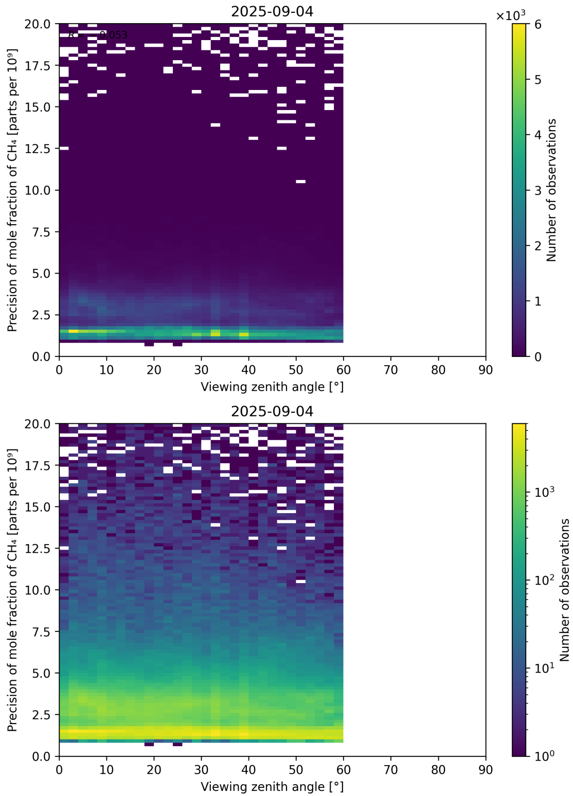
Figure 112: Scatter density plot of “Viewing zenith angle” against “Precision of mole fraction of CH 4 ” for 2025-09-04 to 2025-09-05.
