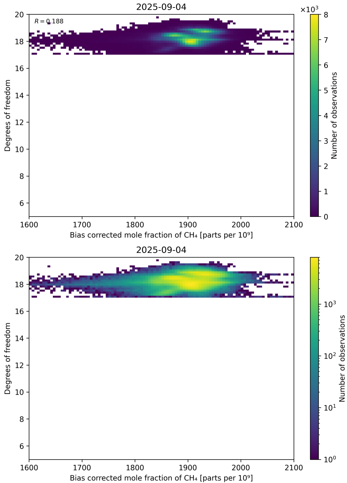
Figure 65: Scatter density plot of “Bias corrected mole fraction of CH 4 ” against “Degrees of freedom” for 2025-09-04 to 2025-09-05.
