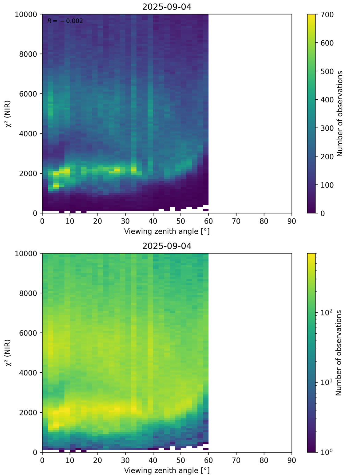
Figure 105: Scatter density plot of “Viewing zenith angle” against “ \chi^2 (NIR)” for 2025-09-04 to 2025-09-05.
