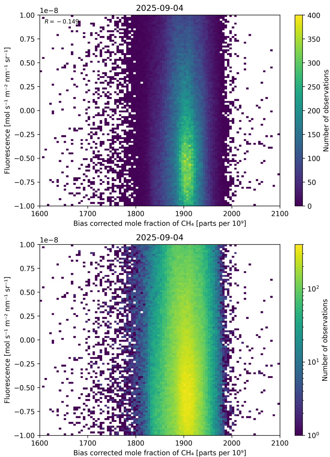
Figure 66: Scatter density plot of “Bias corrected mole fraction of \text{CH}_4 ” against “Fluorescence” for 2025-09-04 to 2025-09-05.
