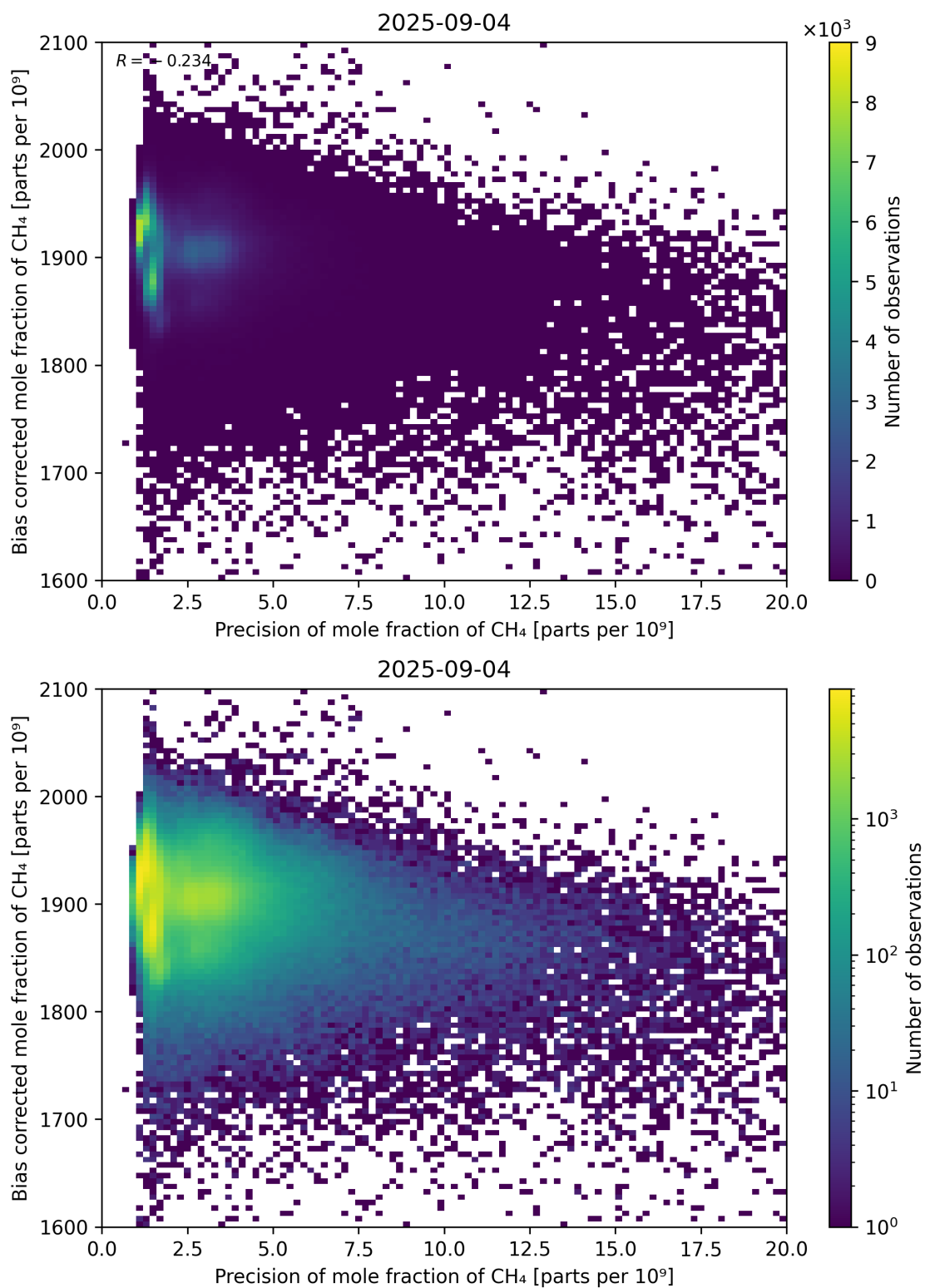
Figure 82: Scatter density plot of “Precision of mole fraction of CH 4 ” against “Bias corrected mole fraction of CH 4 ” for 2025-09-04 to 2025-09-05.
