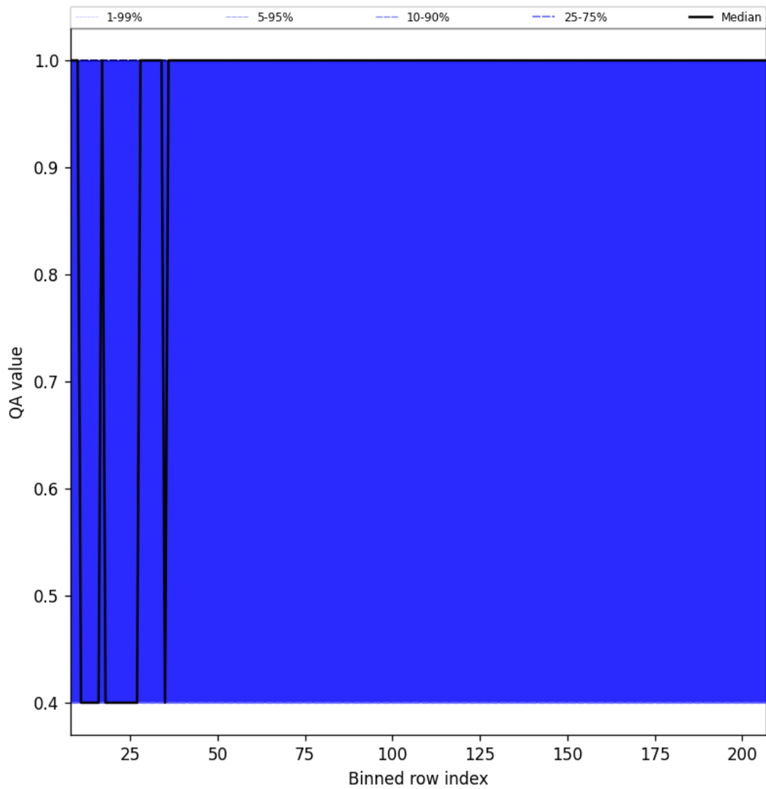
Figure 33: Along track statistics of “QA value” for 2025-09-04 to 2025-09-05
