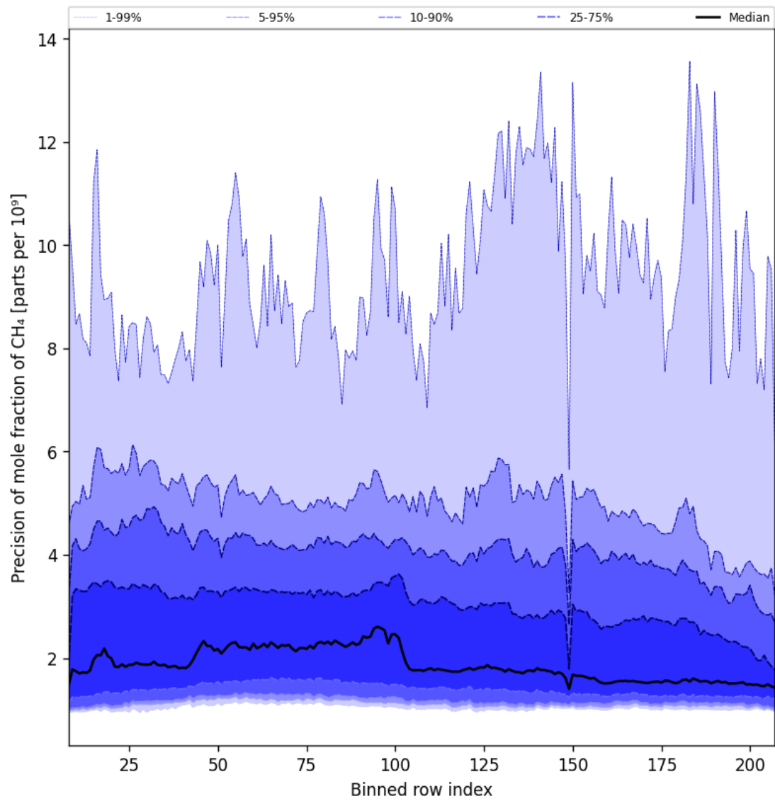
Figure 35: Along track statistics of “Precision of mole fraction of CH 4 ” for 2025-09-04 to 2025-09-05
