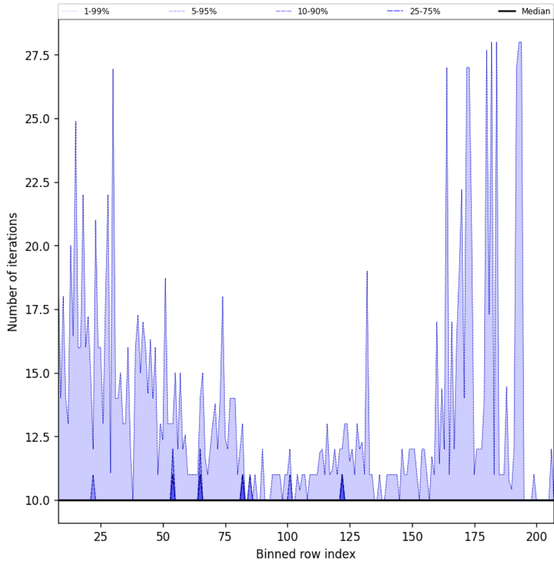
Figure 42: Along track statistics of “Number of iterations” for 2025-09-04 to 2025-09-05
