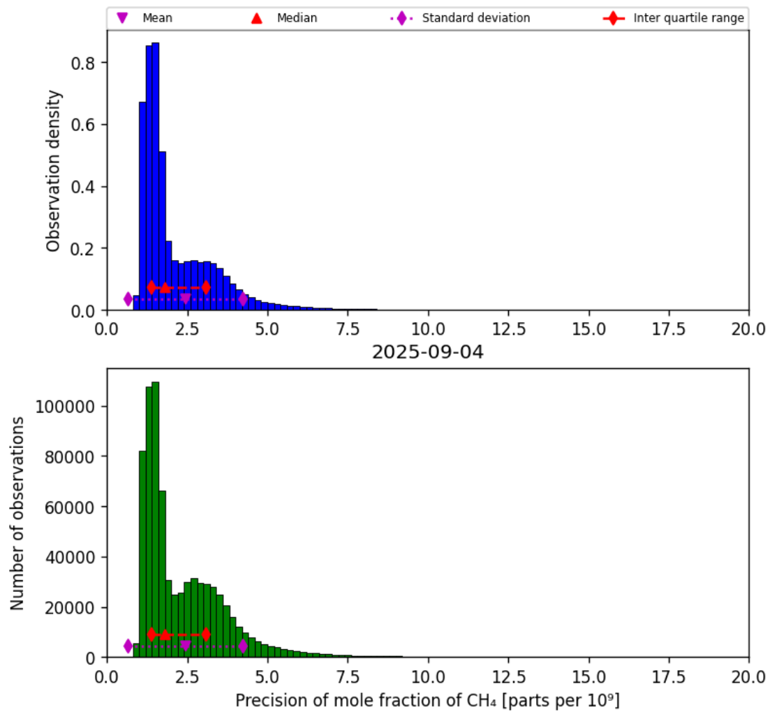
Figure 24: Histogram of “Precision of mole fraction of CH 4 ” for 2025-09-04 to 2025-09-05
