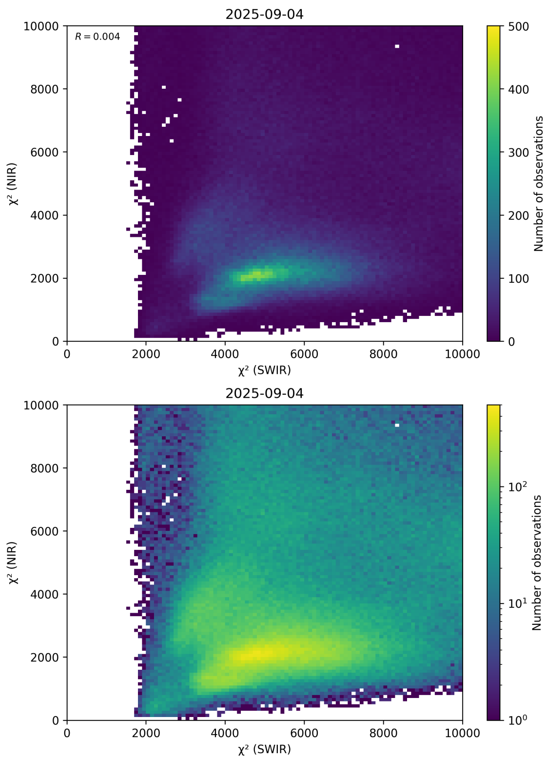
Figure 47: Scatter density plot of “ \chi^2 (SWIR)” against “ \chi^2 (NIR)” for 2025-09-04 to 2025-09-05.
