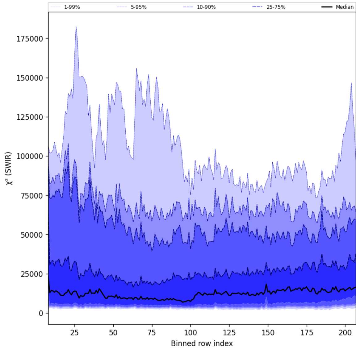
Figure 39: Along track statistics of “ \chi^2 (SWIR)” for 2025-09-04 to 2025-09-05
