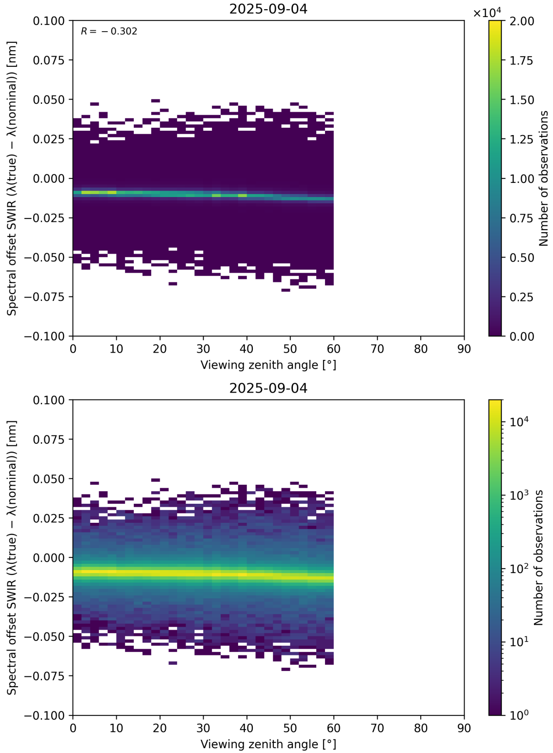
Figure 116: Scatter density plot of “Viewing zenith angle” against “Spectral offset SWIR ( \lambda_{\text{true}} - \lambda_{\text{nominal}} )” for 2025-09-04 to 2025-09-05.
