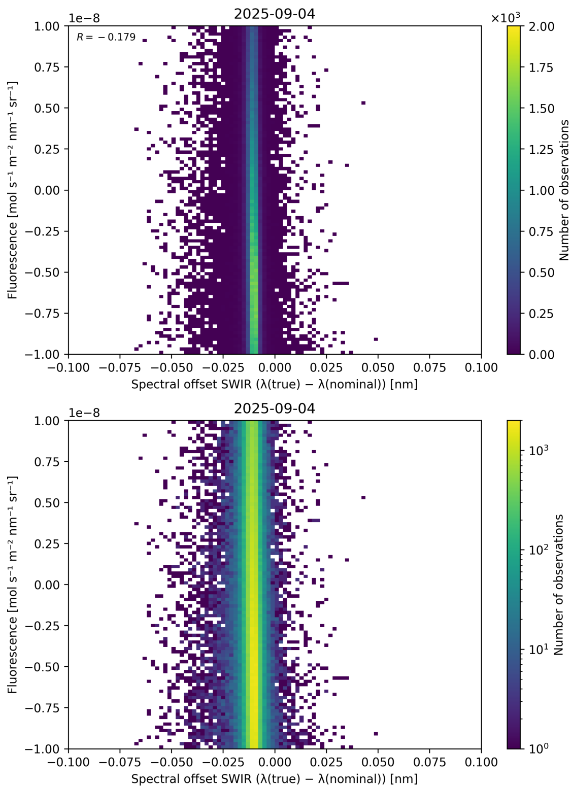
Figure 120: Scatter density plot of “Spectral offset SWIR ( \lambda_{\text{true}} - \lambda_{\text{nominal}} )” against “Fluorescence” for 2025-09-04 to 2025-09-05.
