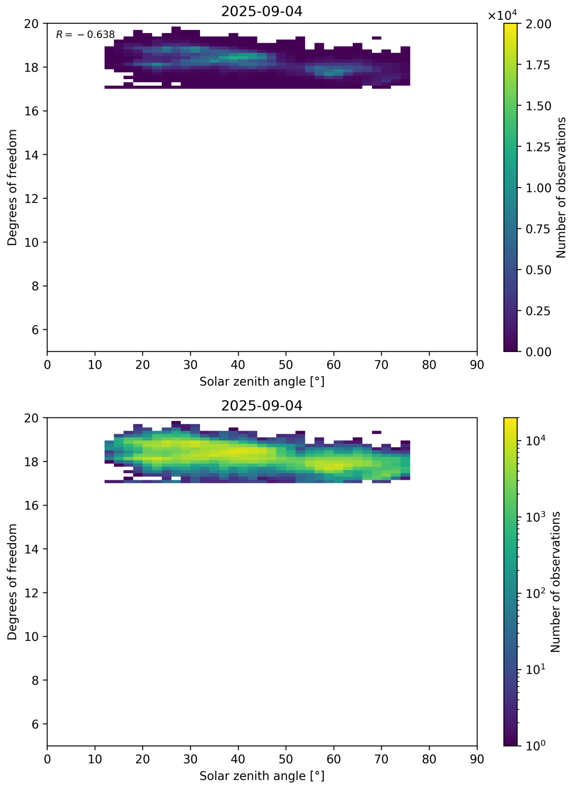
Figure 96: Scatter density plot of “Solar zenith angle” against “Degrees of freedom” for 2025-09-04 to 2025-09-05.
