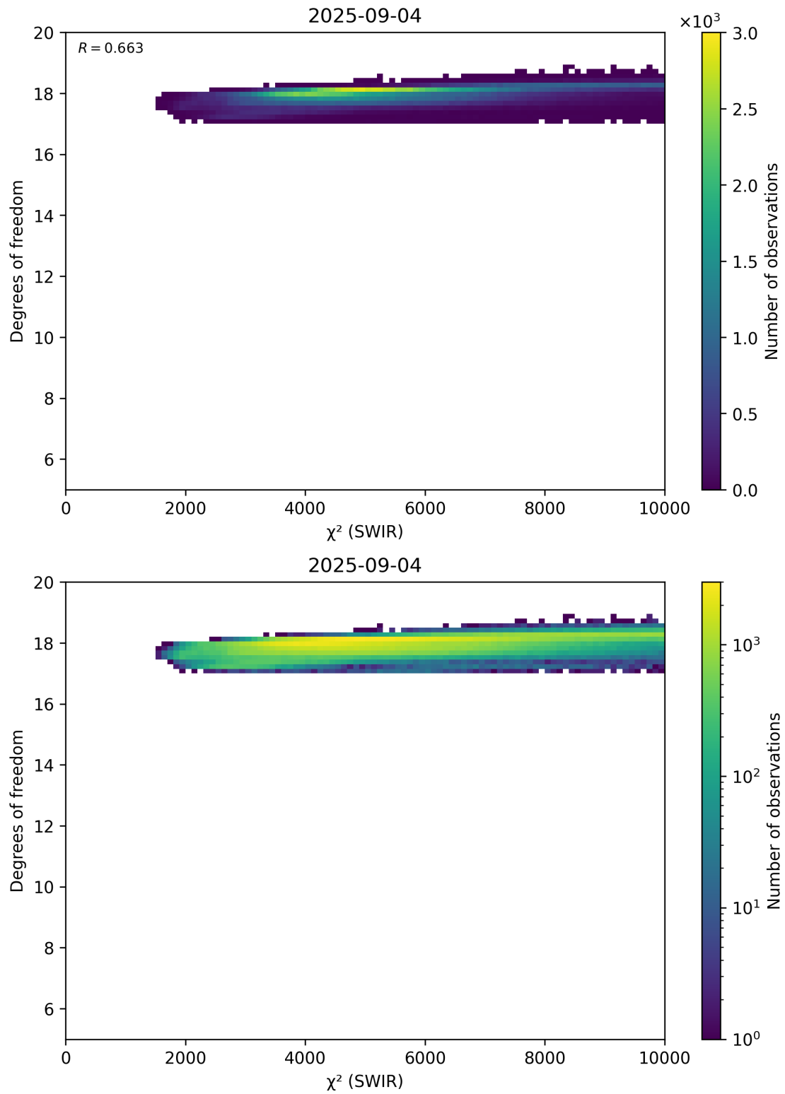
Figure 48: Scatter density plot of “ \chi^2 (SWIR)” against “Degrees of freedom” for 2025-09-04 to 2025-09-05.
