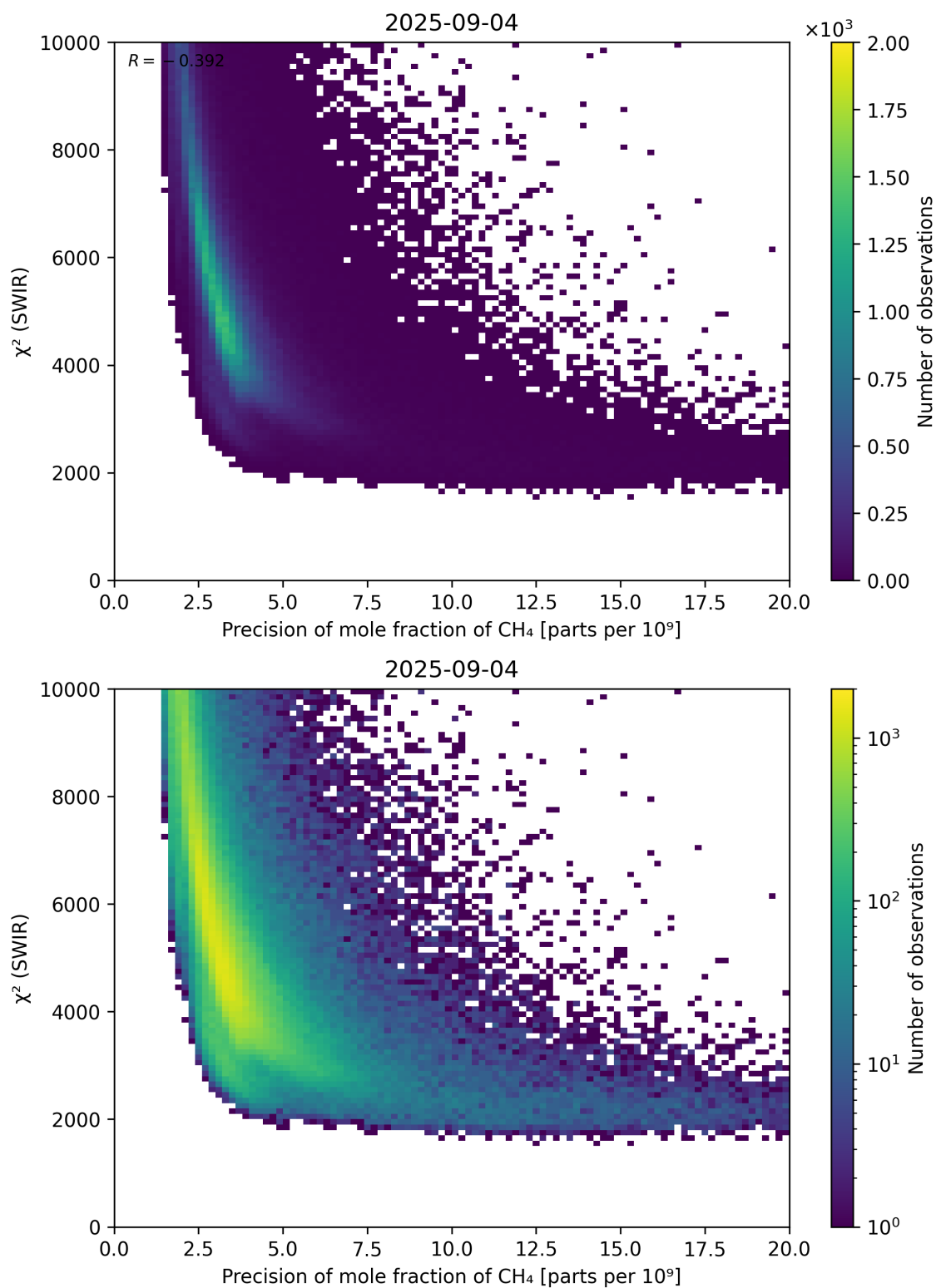
Figure 79: Scatter density plot of “Precision of mole fraction of CH 4 ” against “ \chi^2 (SWIR)” for 2025-09-04 to 2025-09-05.
