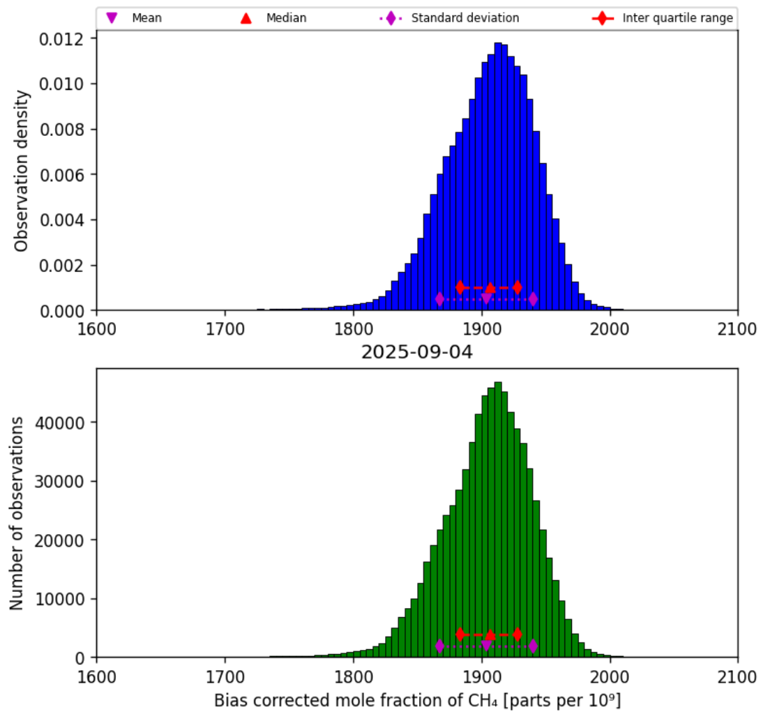
Figure 25: Histogram of “Bias corrected mole fraction of CH 4 ” for 2025-09-04 to 2025-09-05
