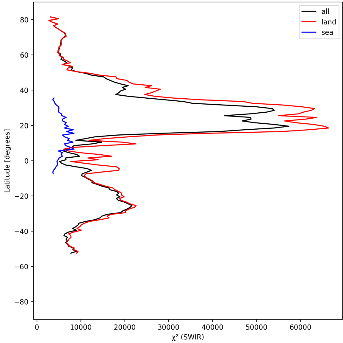
Figure 17: Zonal average of “ \chi^2 (SWIR)” for 2025-09-04 to 2025-09-05.
