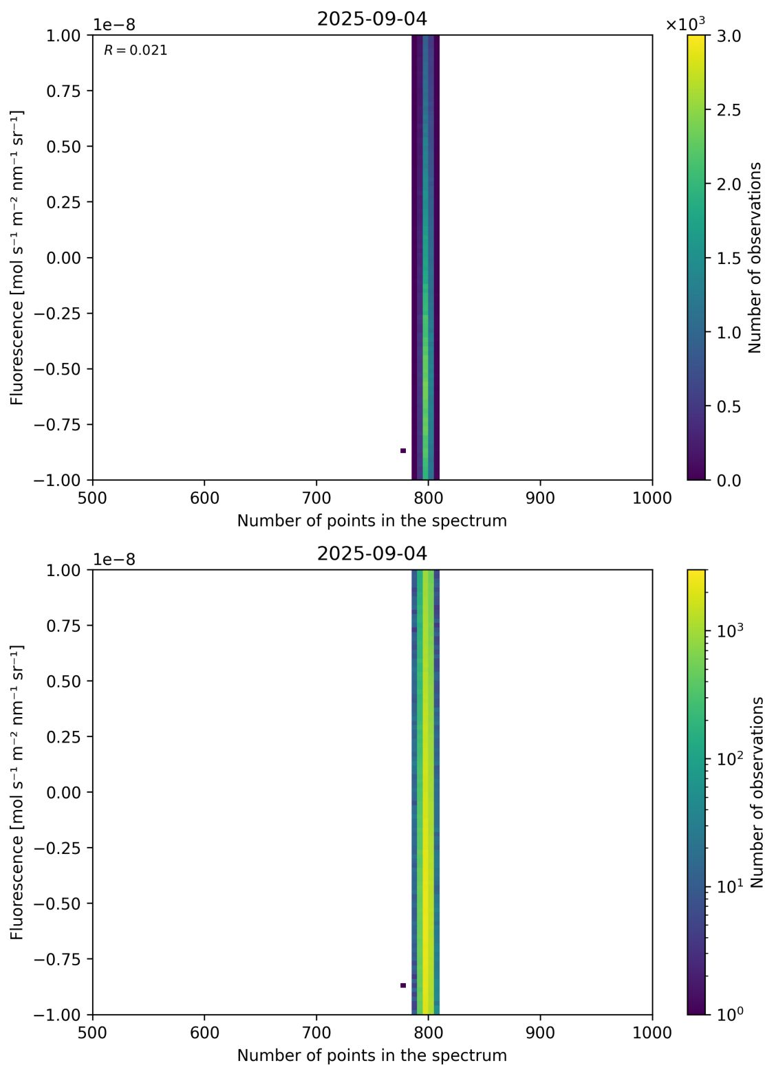
Figure 91: Scatter density plot of “Number of points in the spectrum” against “Fluorescence” for 2025-09-04 to 2025-09-05.
