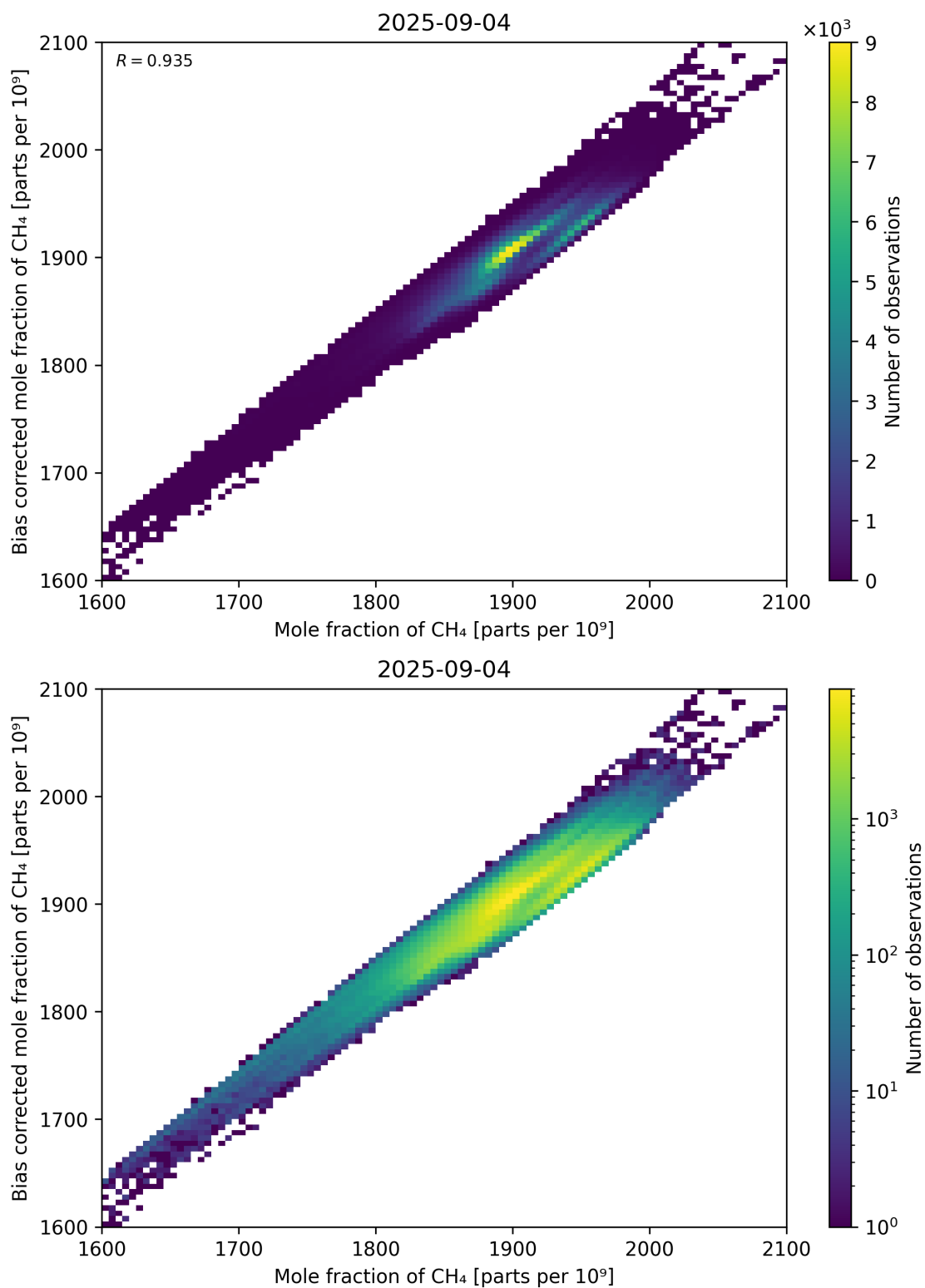
Figure 74: Scatter density plot of “Mole fraction of CH 4 ” against “Bias corrected mole fraction of CH 4 ” for 2025-09-04 to 2025-09-05.
