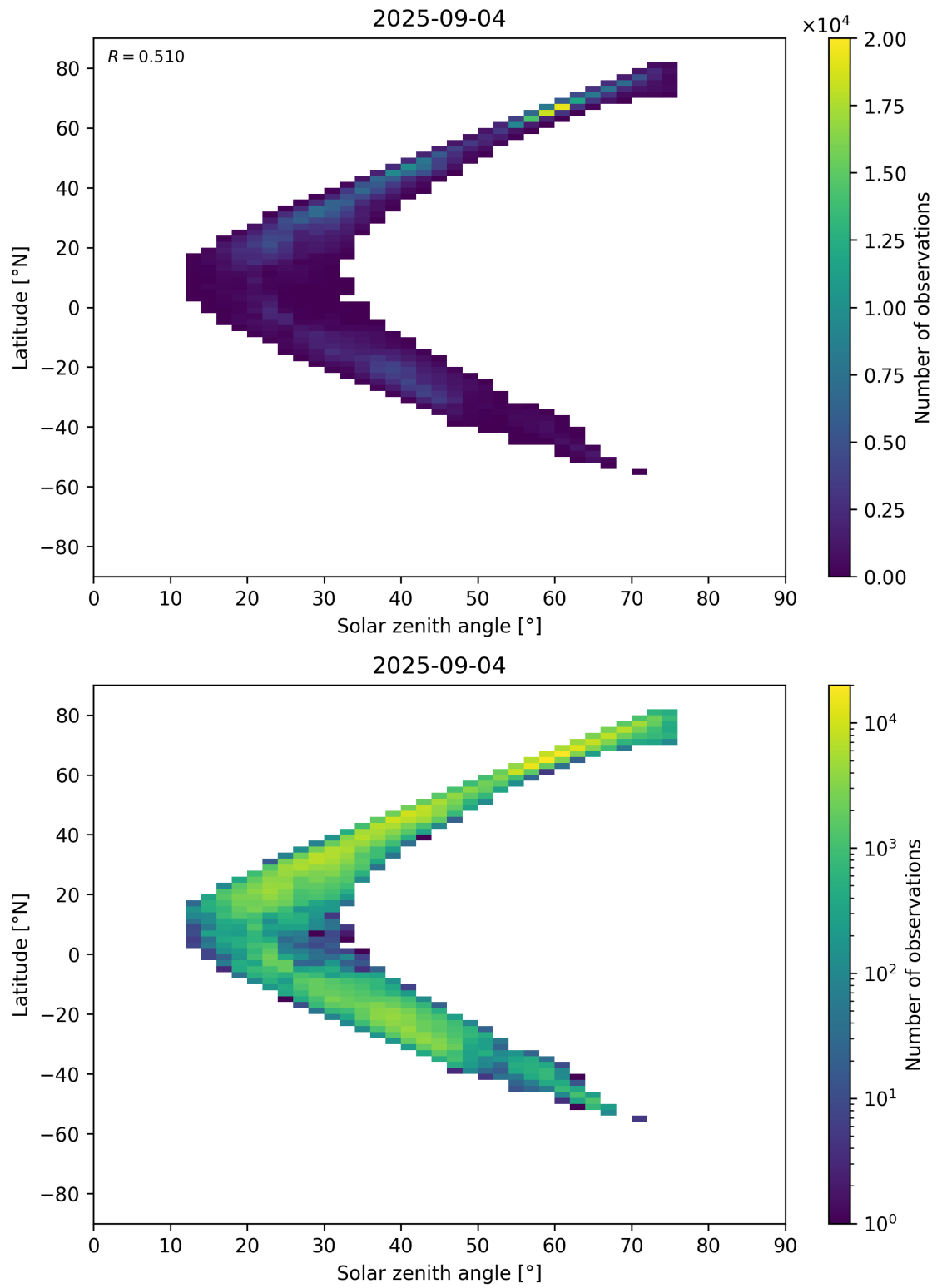
Figure 98: Scatter density plot of “Solar zenith angle” against “Latitude” for 2025-09-04 to 2025-09-05.
