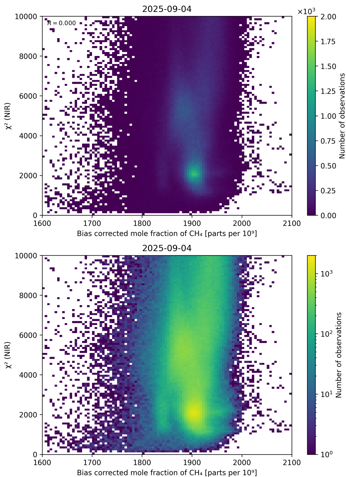
Figure 63: Scatter density plot of “Bias corrected mole fraction of \text{CH}_4 ” against “ \chi^2 (NIR)” for 2025-09-04 to 2025-09-05.
