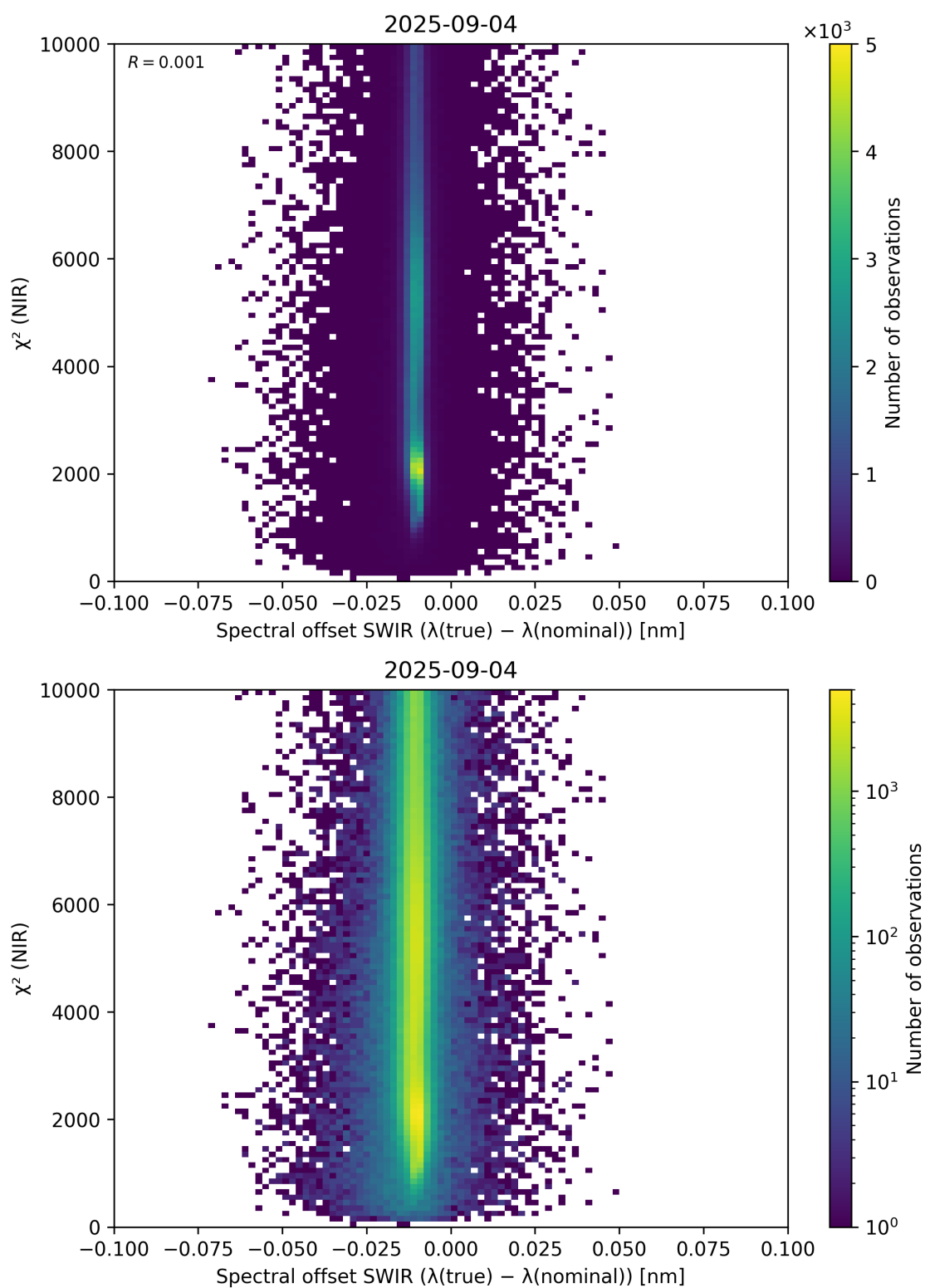
Figure 117: Scatter density plot of “Spectral offset SWIR ( \lambda_{\text{true}} - \lambda_{\text{nominal}} )” against “ \chi^2 (NIR)” for 2025-09-04 to 2025-09-05.
