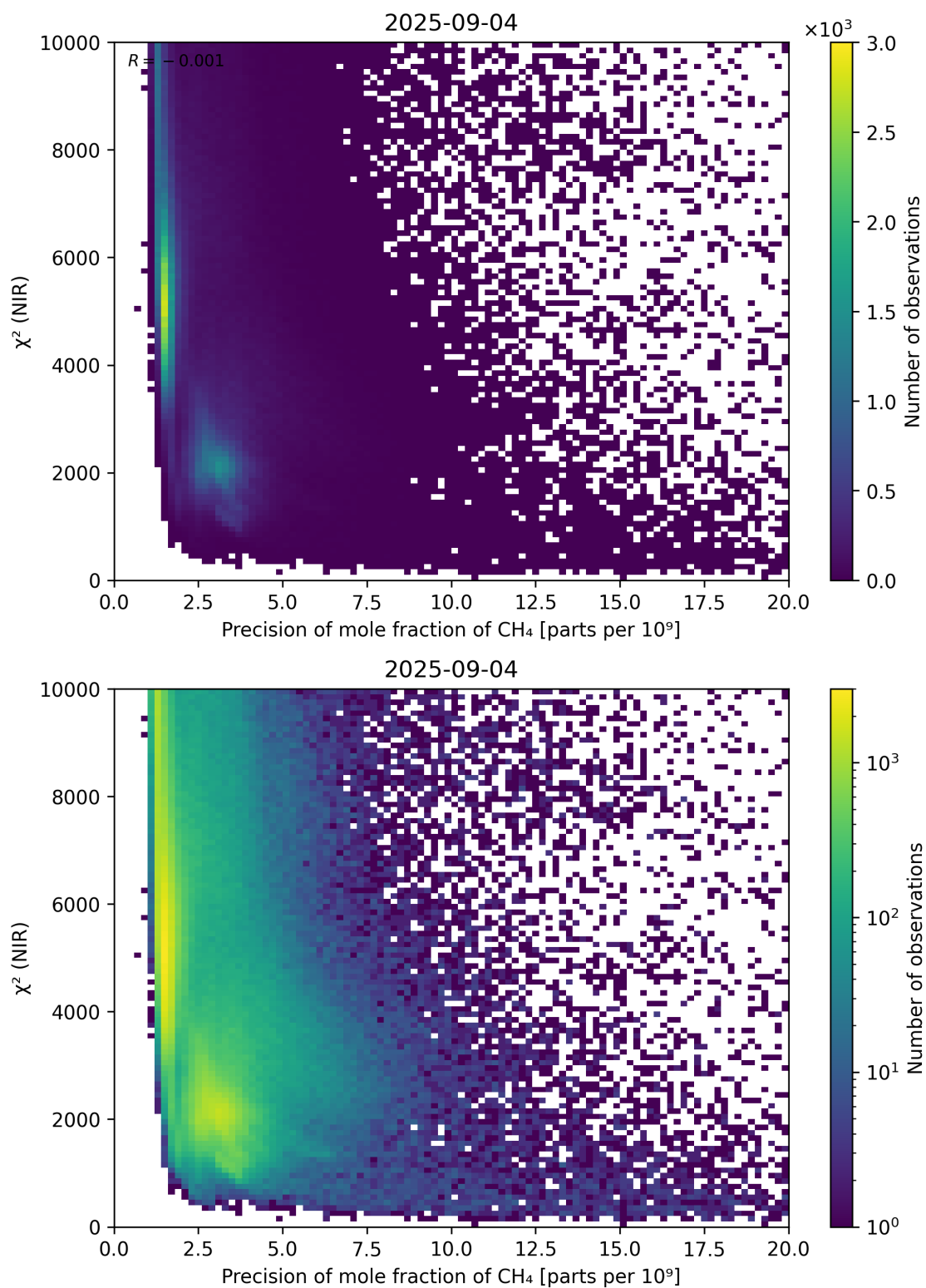
Figure 78: Scatter density plot of “Precision of mole fraction of \text{CH}_4 ” against “ \chi^2 (NIR)” for 2025-09-04 to 2025-09-05.
