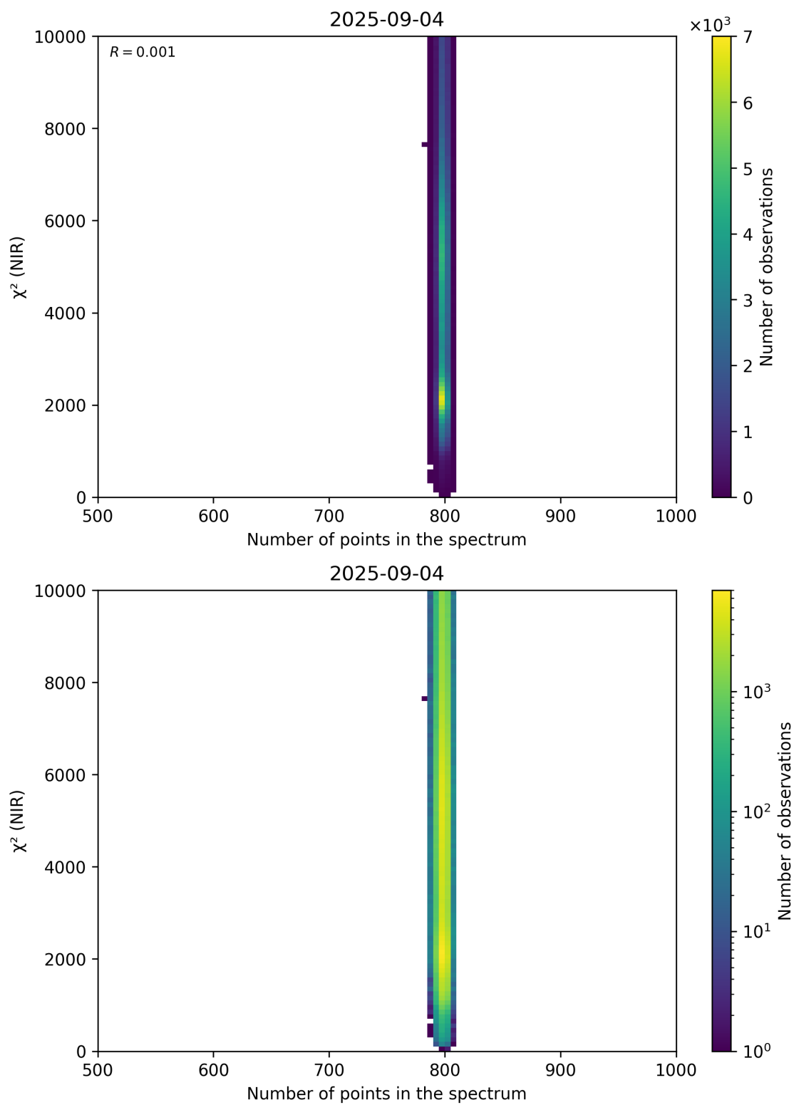
Figure 88: Scatter density plot of “Number of points in the spectrum” against “ \chi^2 (NIR)” for 2025-09-04 to 2025-09-05.
