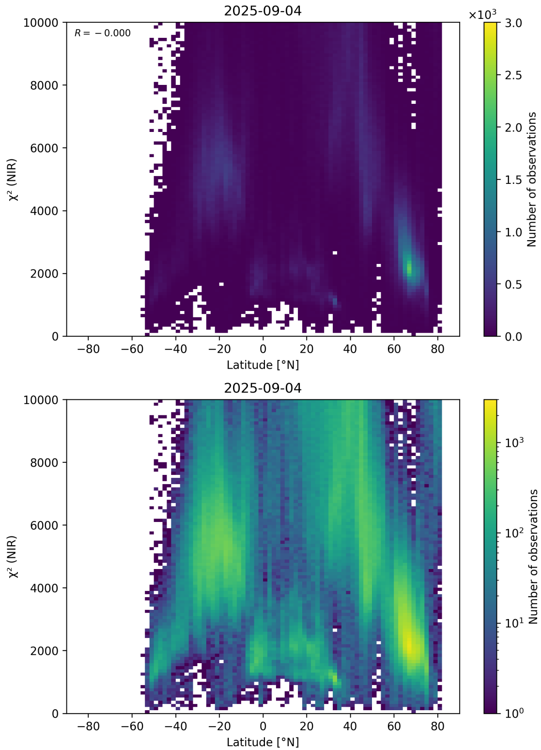
Figure 53: Scatter density plot of “Latitude” against “ \chi^2 (NIR)” for 2025-09-04 to 2025-09-05.
