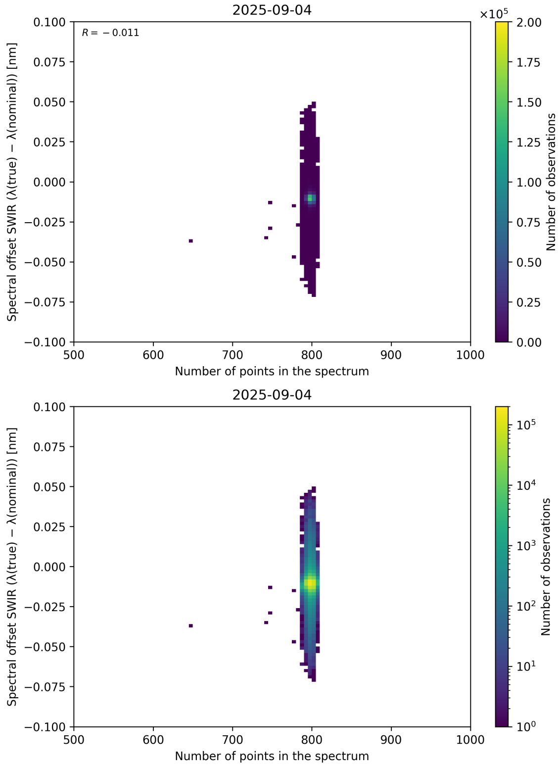
Figure 93: Scatter density plot of “Number of points in the spectrum” against “Spectral offset SWIR ( \lambda_{\text{true}} - \lambda_{\text{nominal}} )” for 2025-09-04 to 2025-09-05.
