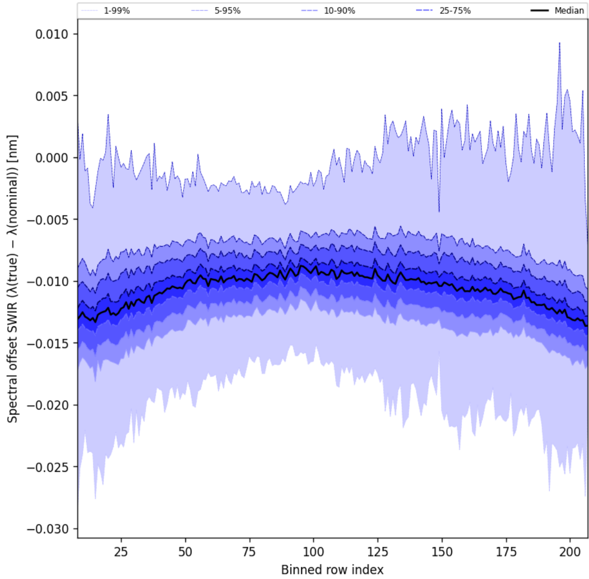
Figure 38: Along track statistics of “Spectral offset SWIR ( \lambda_{\text{true}} - \lambda_{\text{nominal}} )” for 2025-09-04 to 2025-09-05
