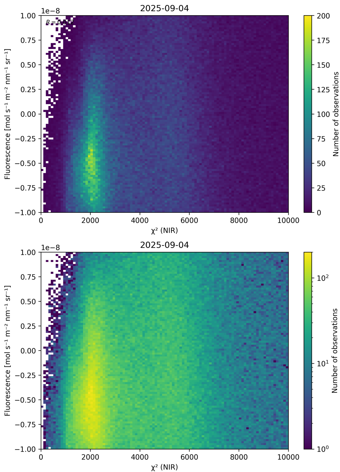
Figure 45: Scatter density plot of “ \chi^2 (NIR)” against “Fluorescence” for 2025-09-04 to 2025-09-05.
