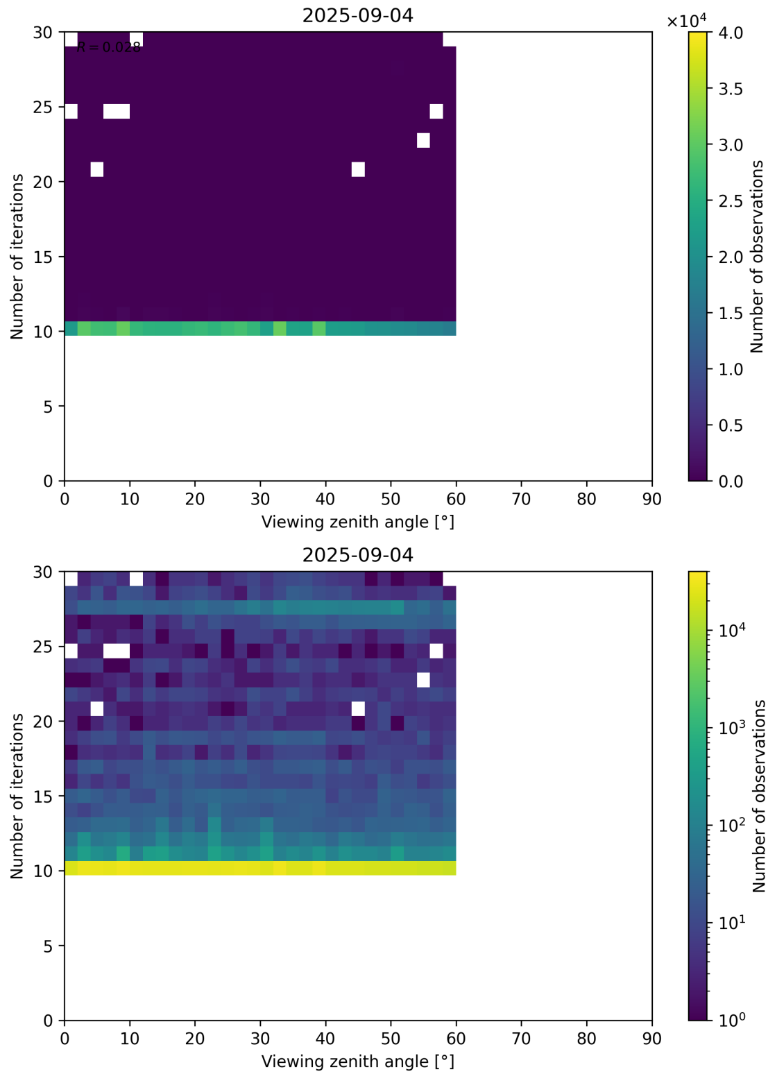
Figure 113: Scatter density plot of “Viewing zenith angle” against “Number of iterations” for 2025-09-04 to 2025-09-05.
