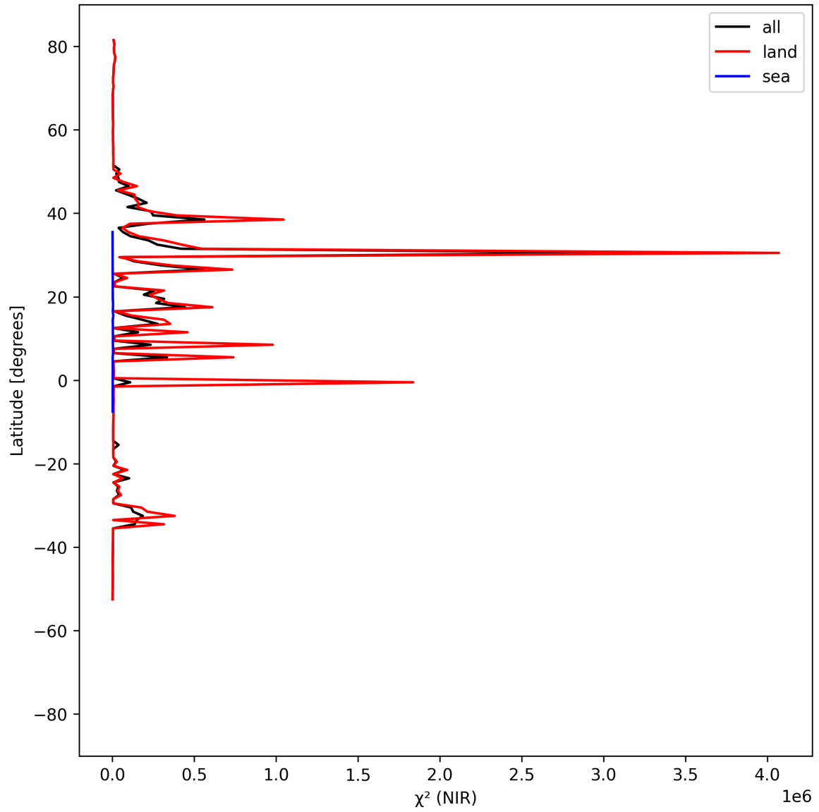
Figure 18: Zonal average of “ \chi^2 (NIR)” for 2025-09-04 to 2025-09-05.
