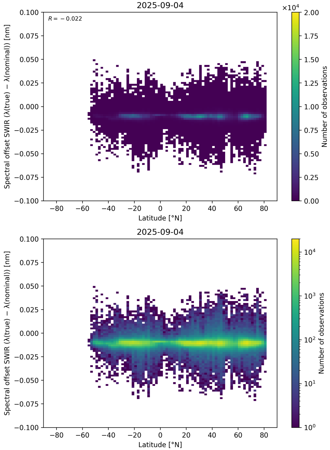
Figure 62: Scatter density plot of “Latitude” against “Spectral offset SWIR ( \lambda_{\text{true}} - \lambda_{\text{nominal}} )” for 2025-09-04 to 2025-09-05.
