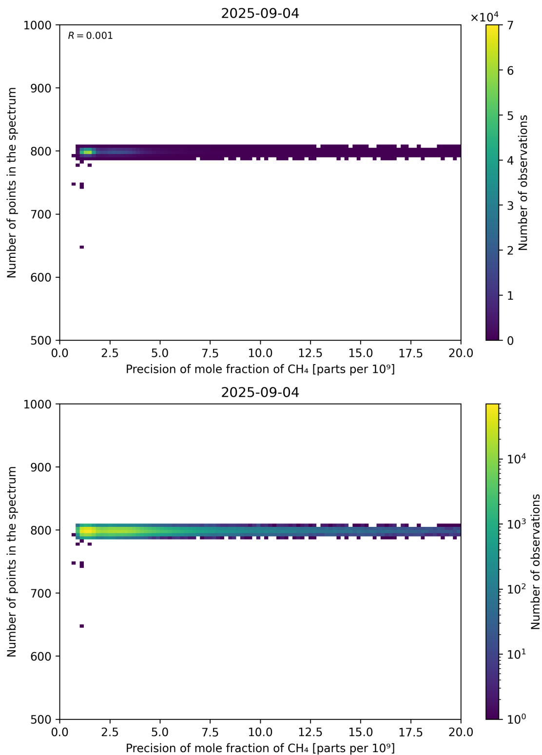
Figure 84: Scatter density plot of “Precision of mole fraction of CH 4 ” against “Number of points in the spectrum” for 2025-09-04 to 2025-09-05.
