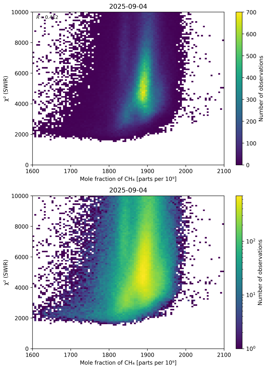
Figure 71: Scatter density plot of “Mole fraction of CH 4 ” against “ \chi^2 (SWIR)” for 2025-09-04 to 2025-09-05.
