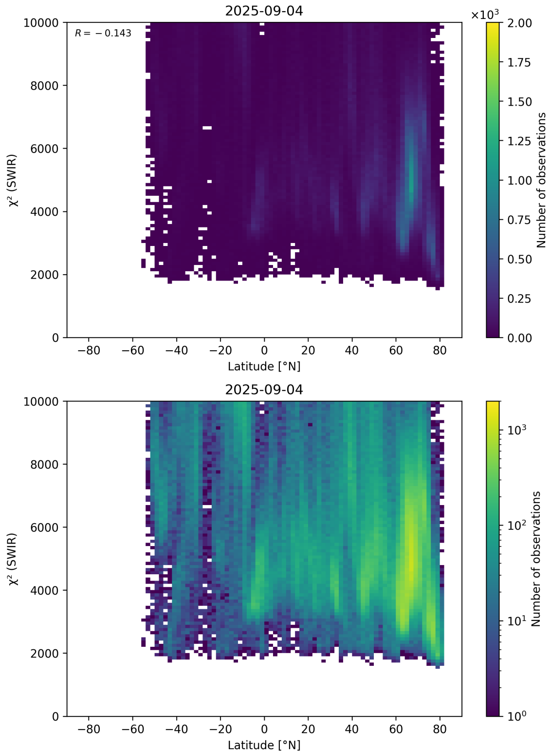
Figure 54: Scatter density plot of “Latitude” against “ \chi^2 (SWIR)” for 2025-09-04 to 2025-09-05.
