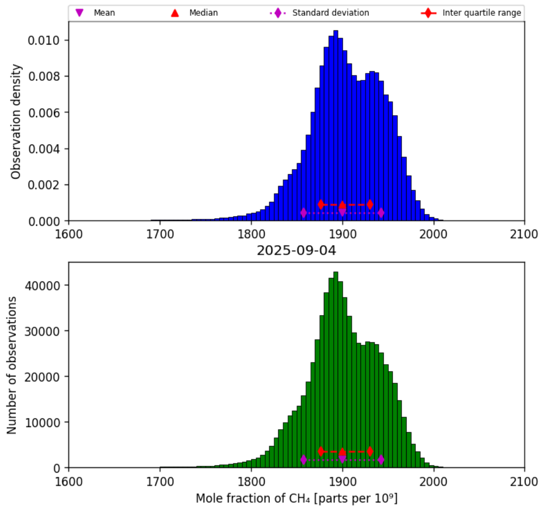
Figure 23: Histogram of “Mole fraction of CH 4 ” for 2025-09-04 to 2025-09-05
