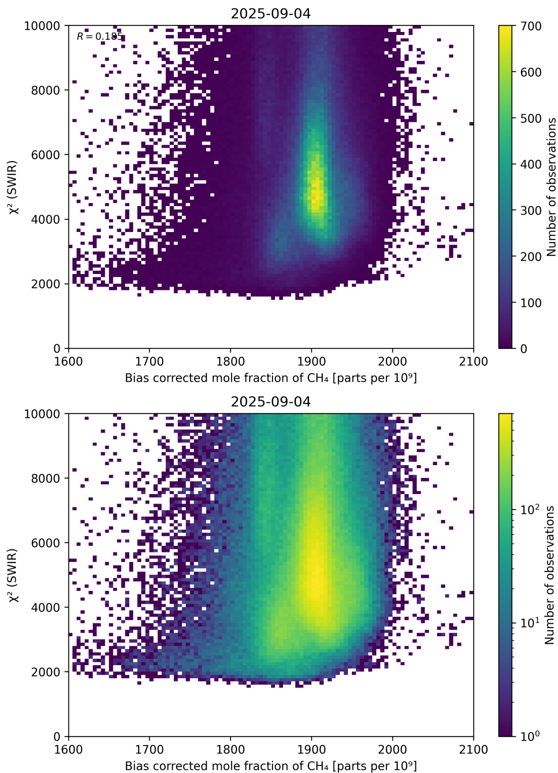
Figure 64: Scatter density plot of “Bias corrected mole fraction of \text{CH}_4 ” against “ \chi^2 (SWIR)” for 2025-09-04 to 2025-09-05.
