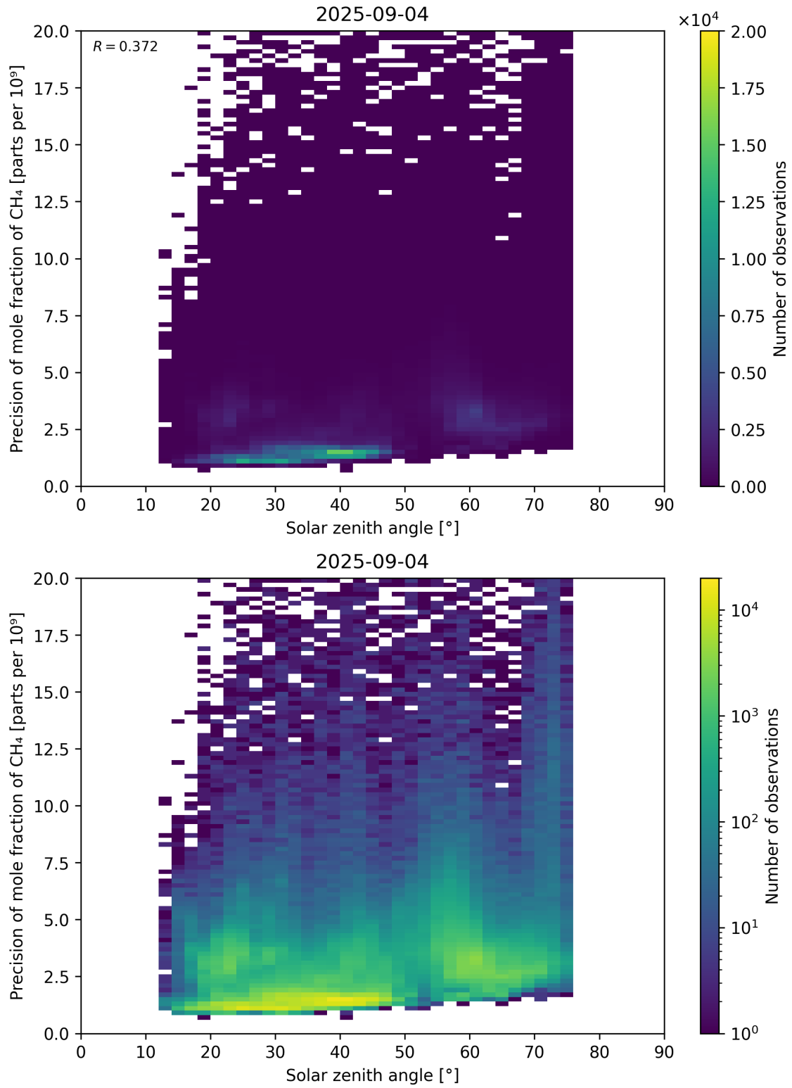
Figure 101: Scatter density plot of “Solar zenith angle” against “Precision of mole fraction of CH 4 ” for 2025-09-04 to 2025-09-05.
