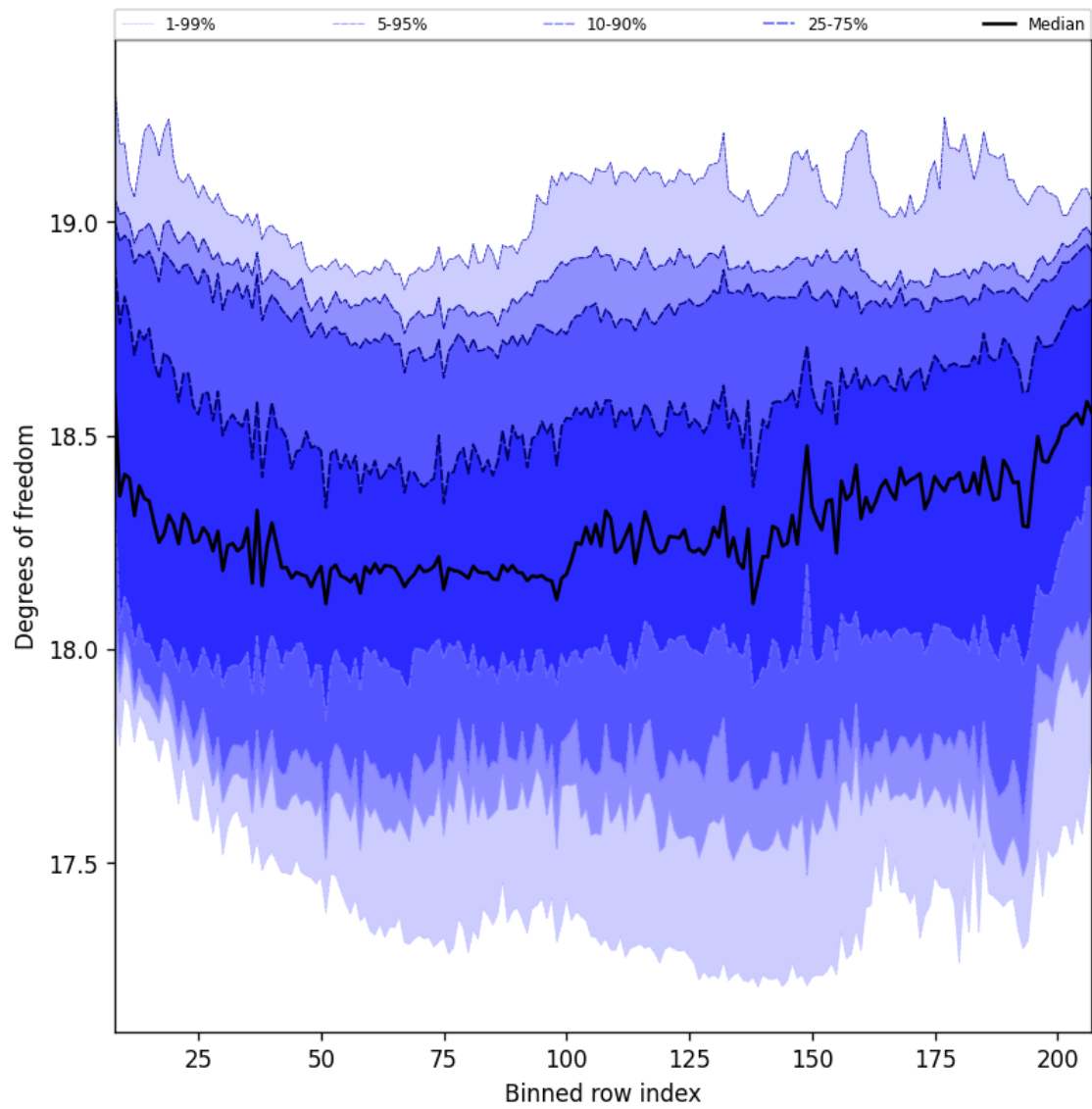
Figure 41: Along track statistics of “Degrees of freedom” for 2025-09-04 to 2025-09-05
