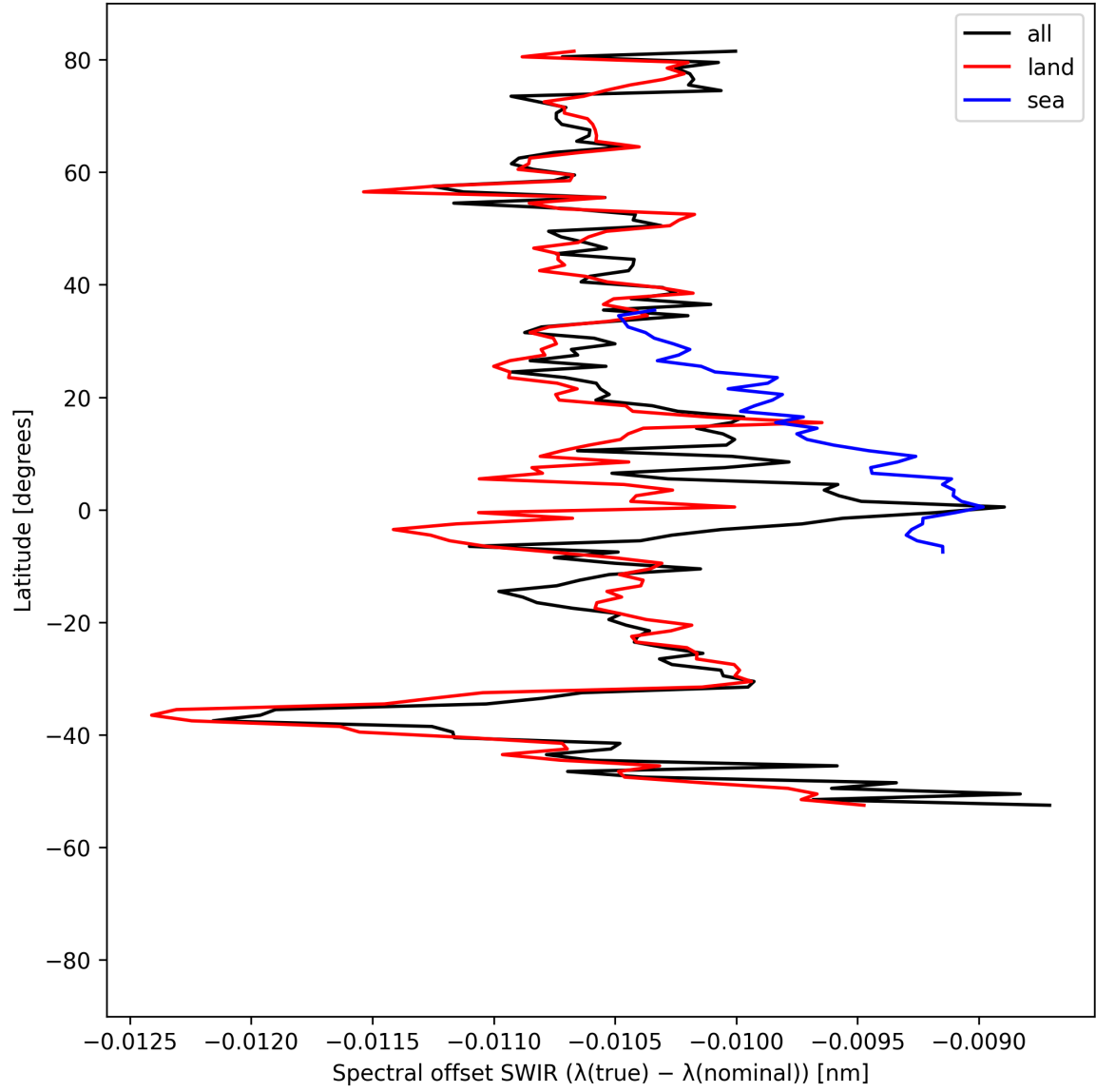
Figure 16: Zonal average of “Spectral offset SWIR ( \lambda_{\text{true}} - \lambda_{\text{nominal}} )” for 2025-09-04 to 2025-09-05.
