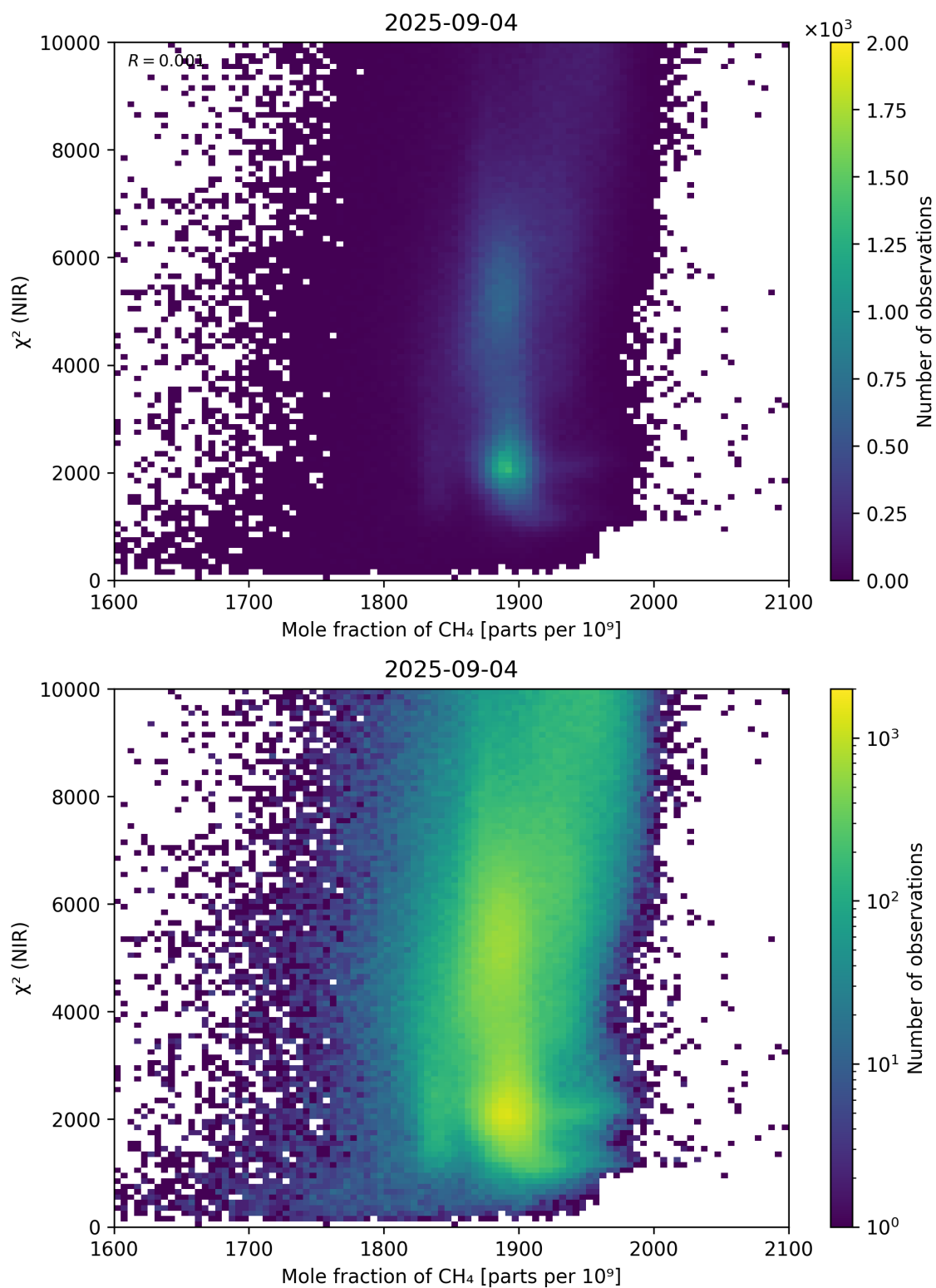
Figure 70: Scatter density plot of “Mole fraction of \text{CH}_4 ” against “ \chi^2 (NIR)” for 2025-09-04 to 2025-09-05.
