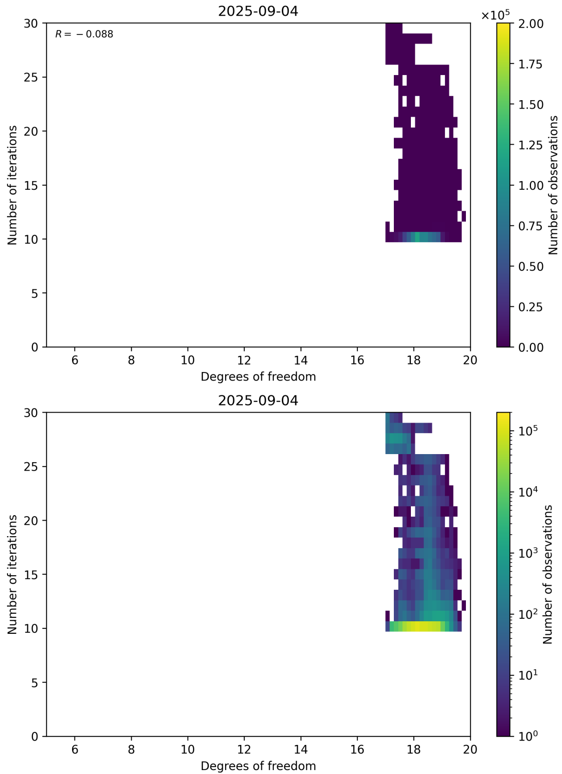
Figure 52: Scatter density plot of “Degrees of freedom” against “Number of iterations” for 2025-09-04 to 2025-09-05.
