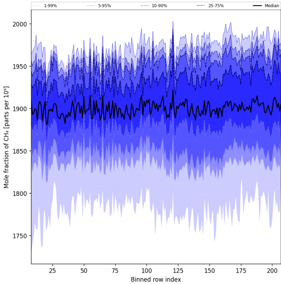
Figure 34: Along track statistics of “Mole fraction of CH 4 ” for 2025-09-04 to 2025-09-05
