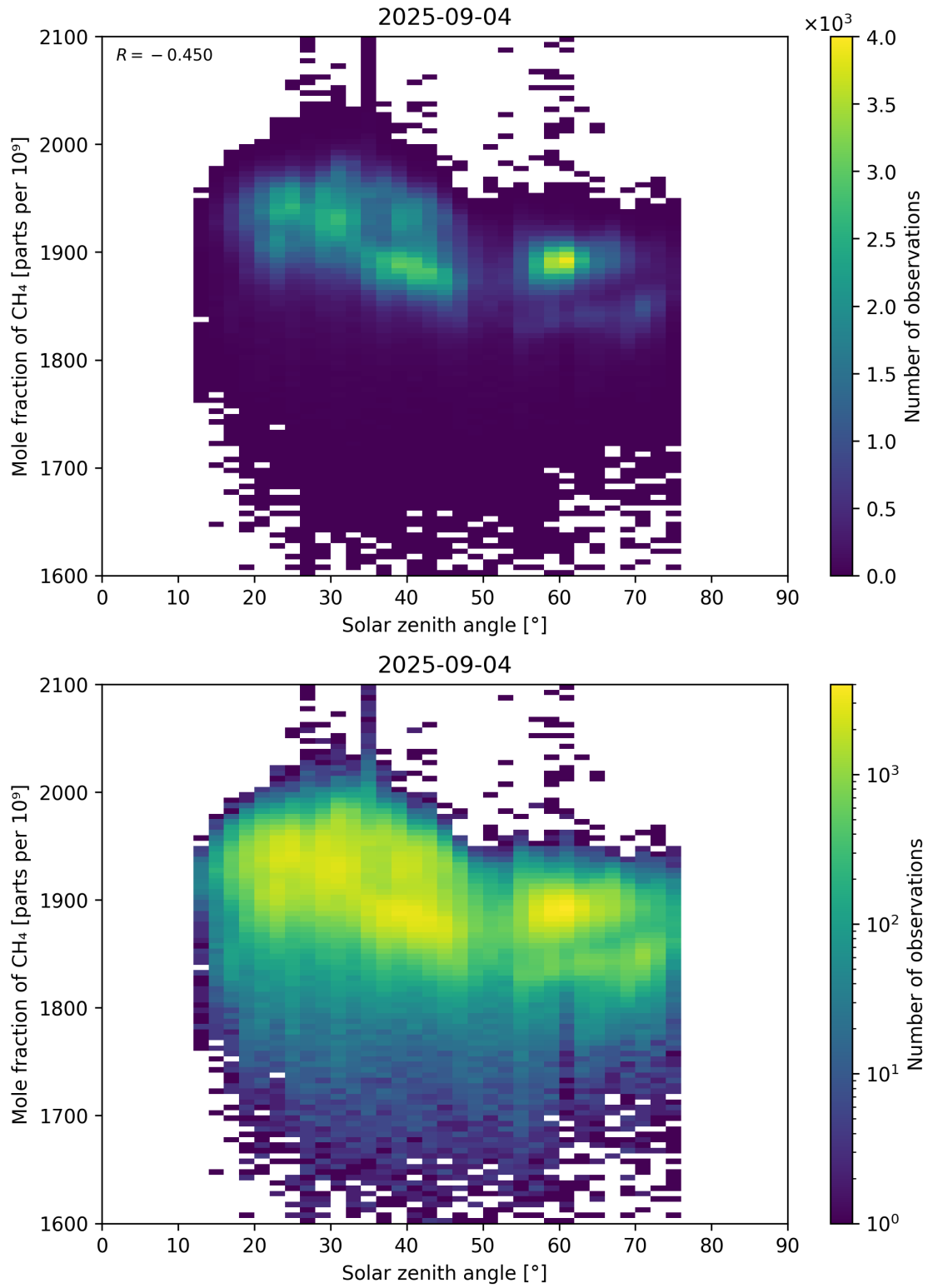
Figure 99: Scatter density plot of “Solar zenith angle” against “Mole fraction of CH 4 ” for 2025-09-04 to 2025-09-05.
