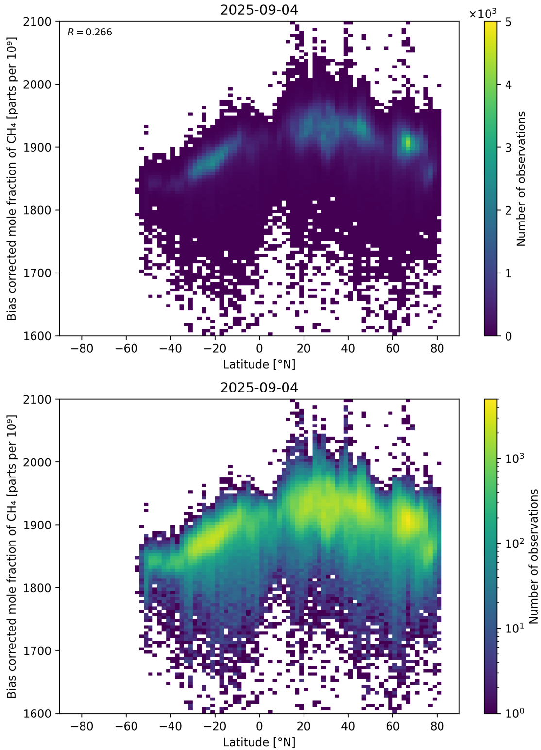
Figure 58: Scatter density plot of “Latitude” against “Bias corrected mole fraction of CH 4 ” for 2025-09-04 to 2025-09-05.
