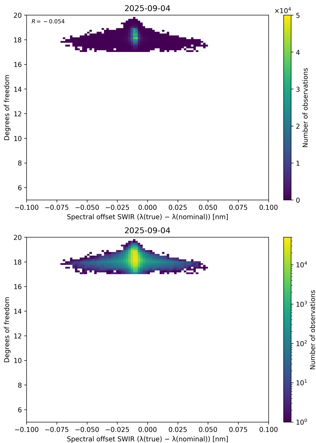
Figure 119: Scatter density plot of “Spectral offset SWIR ( \lambda_{\text{true}} - \lambda_{\text{nominal}} )” against “Degrees of freedom” for 2025-09-04 to 2025-09-05.
