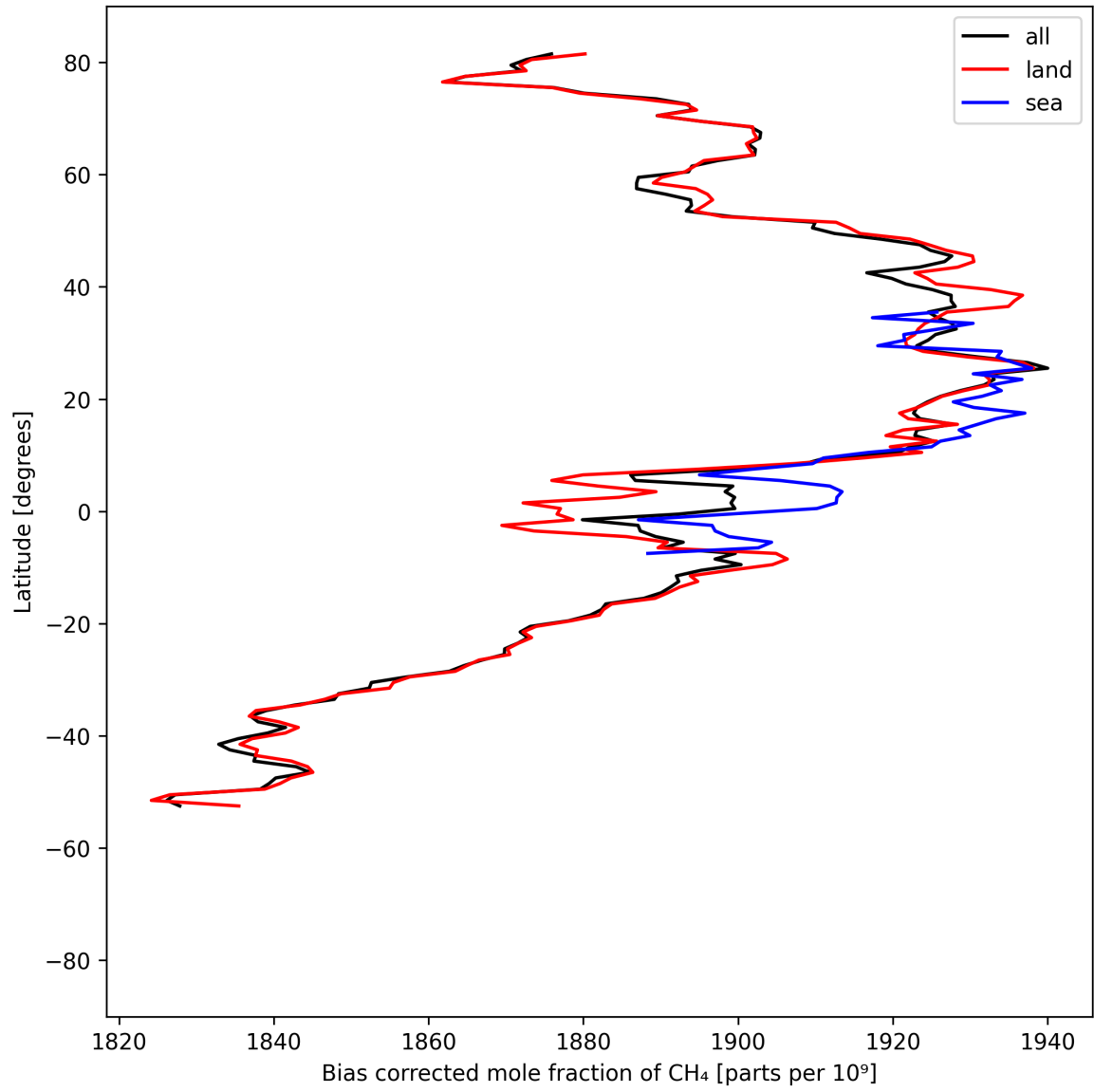
Figure 14: Zonal average of “Bias corrected mole fraction of CH 4 ” for 2025-09-04 to 2025-09-05.
