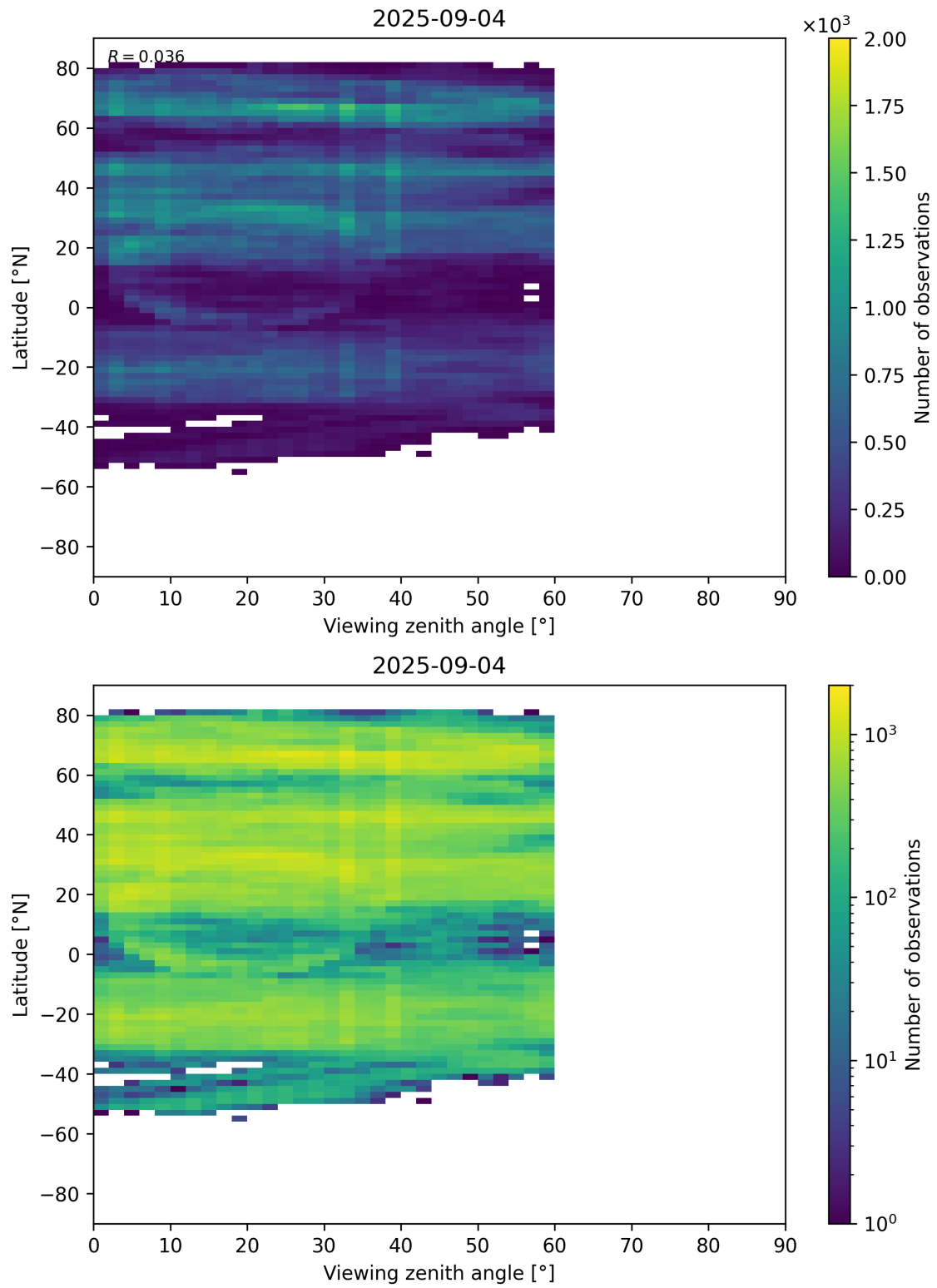
Figure 109: Scatter density plot of “Viewing zenith angle” against “Latitude” for 2025-09-04 to 2025-09-05.
