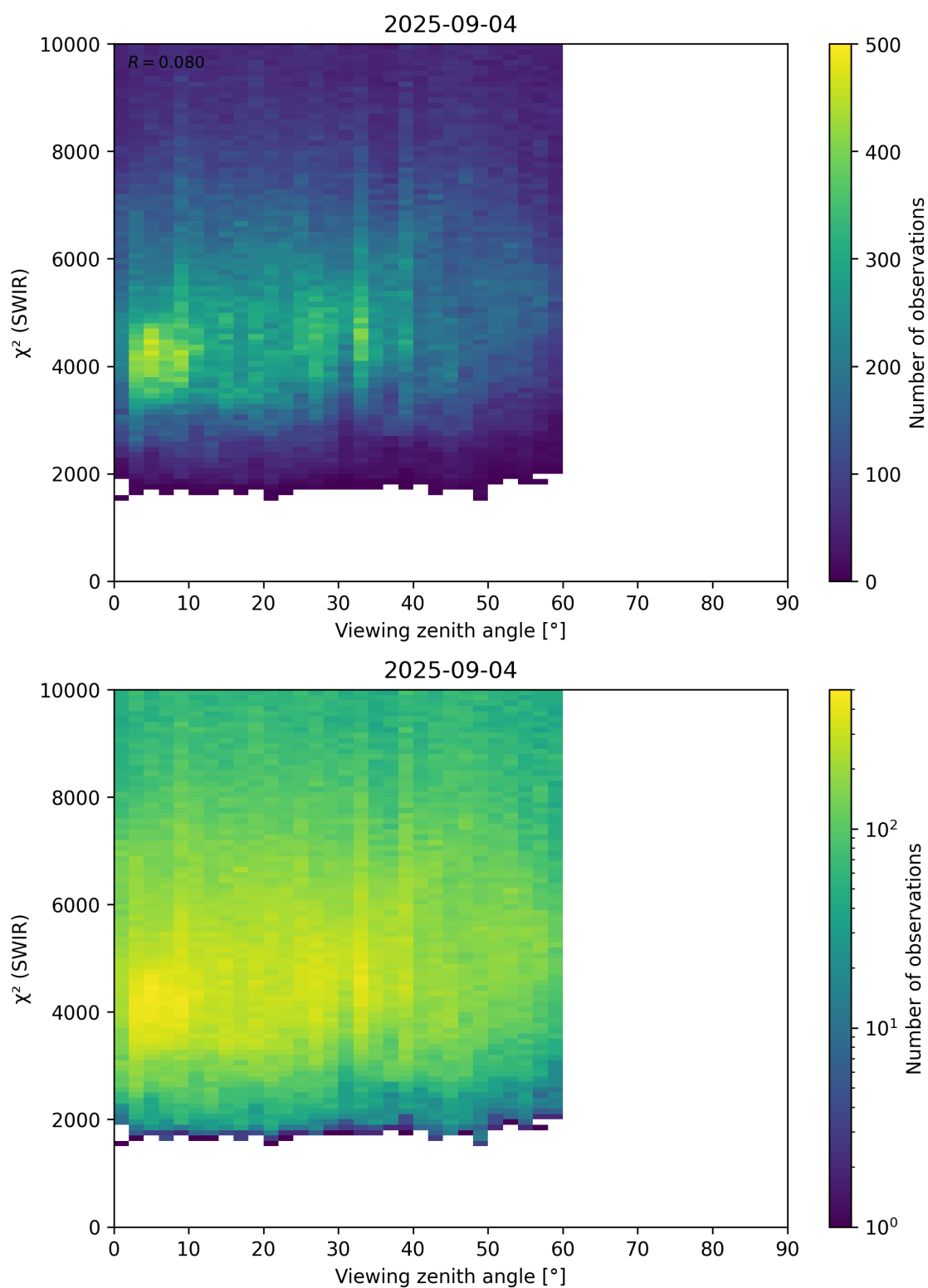
Figure 106: Scatter density plot of “Viewing zenith angle” against “ \chi^2 (SWIR)” for 2025-09-04 to 2025-09-05.
