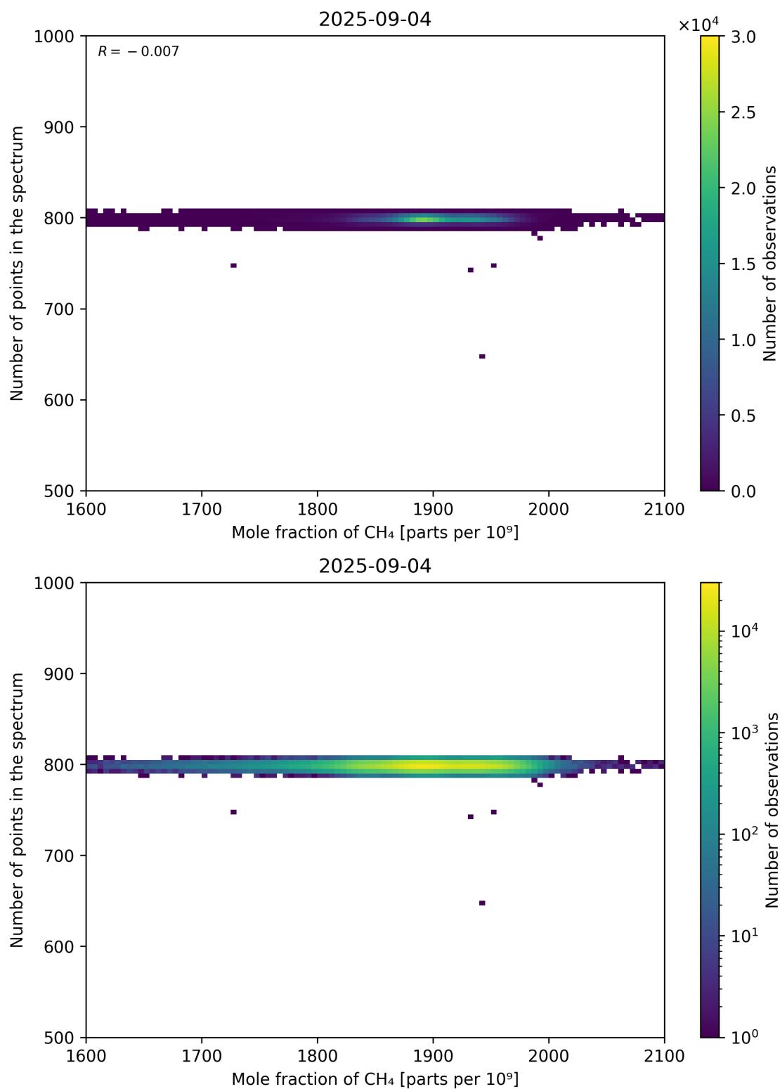
Figure 77: Scatter density plot of “Mole fraction of CH 4 ” against “Number of points in the spectrum” for 2025-09-04 to 2025-09-05.
