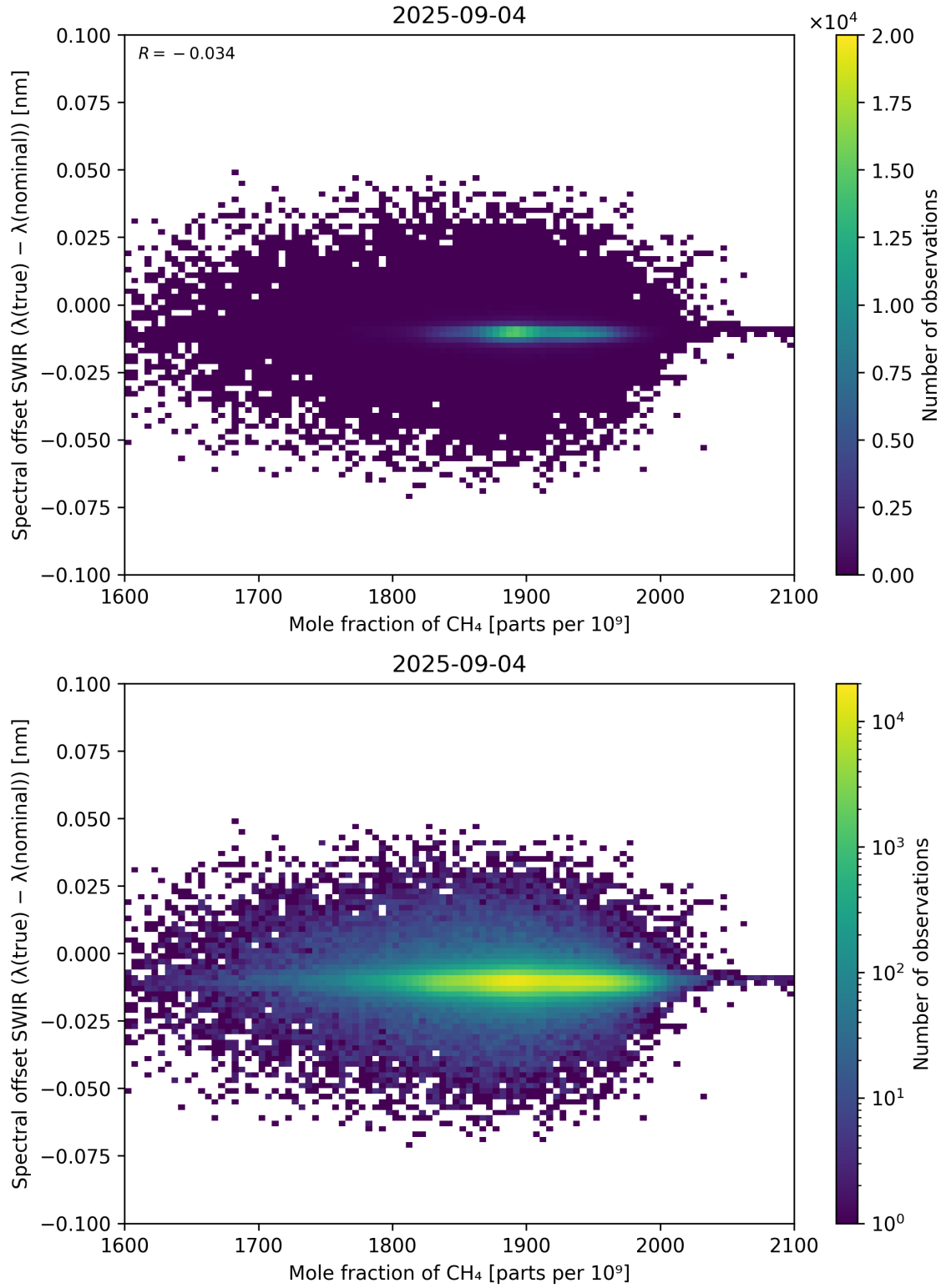
Figure 86: Scatter density plot of “Mole fraction of CH 4 ” against “Spectral offset SWIR ( \lambda_{\text{true}} - \lambda_{\text{nominal}} )” for 2025-09-04 to 2025-09-05.
