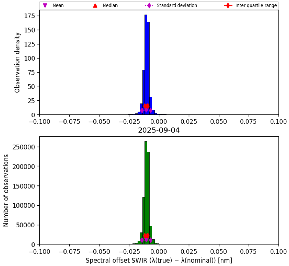
Figure 27: Histogram of “Spectral offset SWIR ( \lambda_{\text{true}} - \lambda_{\text{nominal}} )” for 2025-09-04 to 2025-09-05
