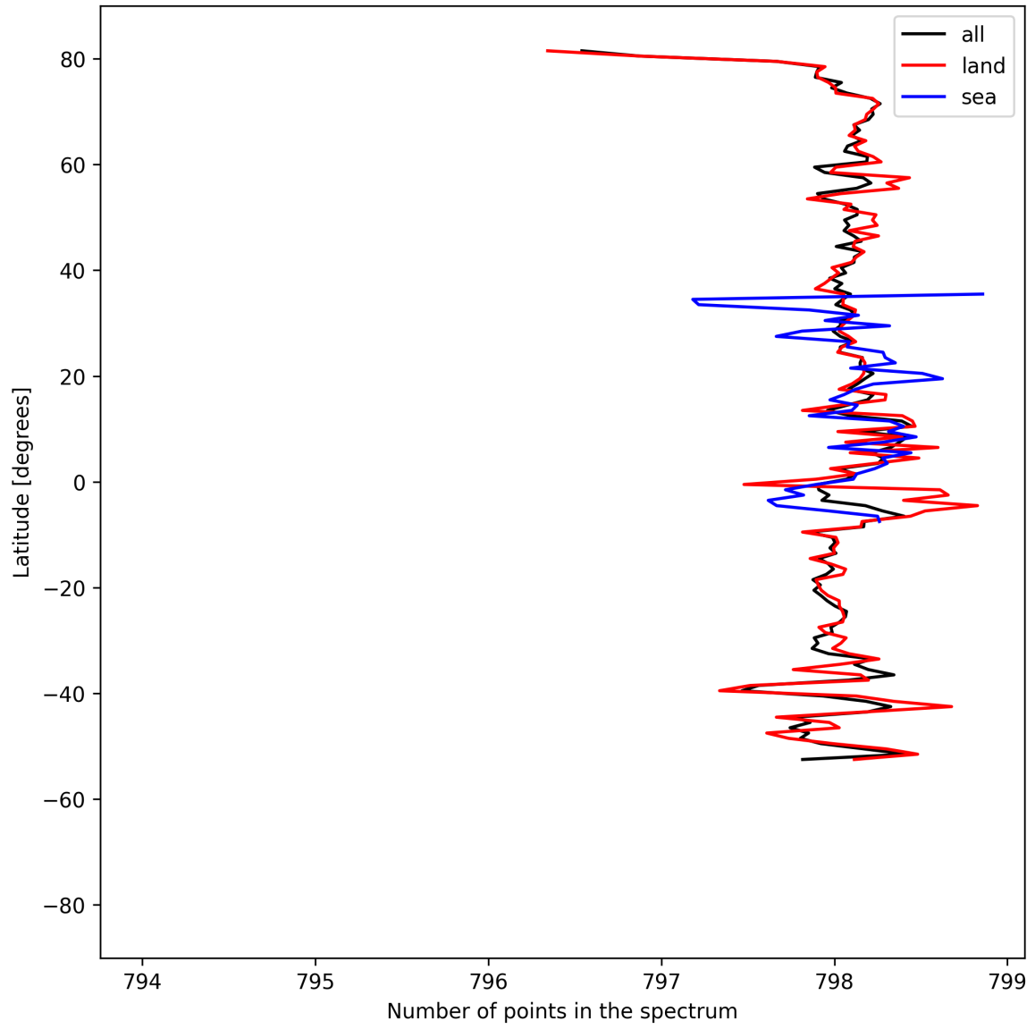
Figure 15: Zonal average of “Number of points in the spectrum” for 2025-09-04 to 2025-09-05.
