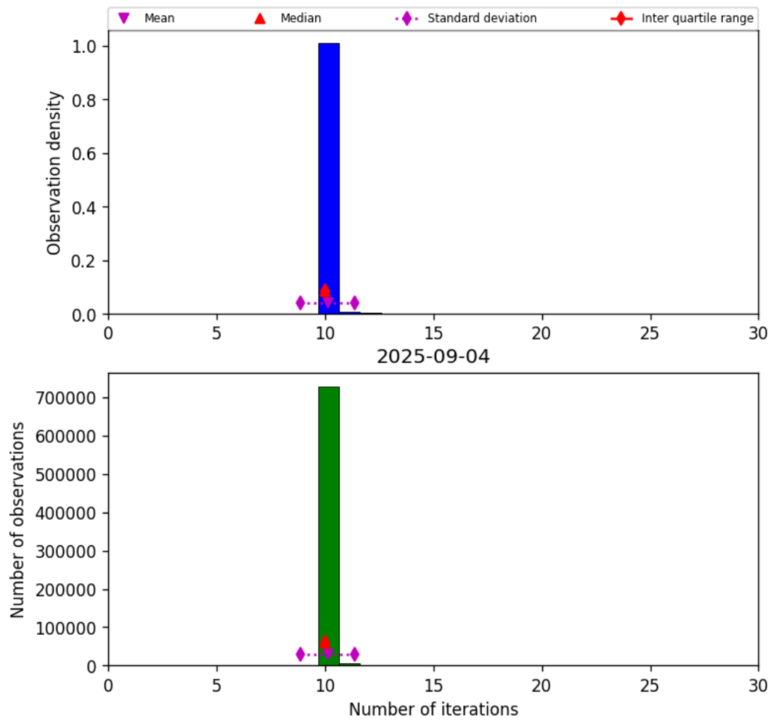
Figure 31: Histogram of “Number of iterations” for 2025-09-04 to 2025-09-05
