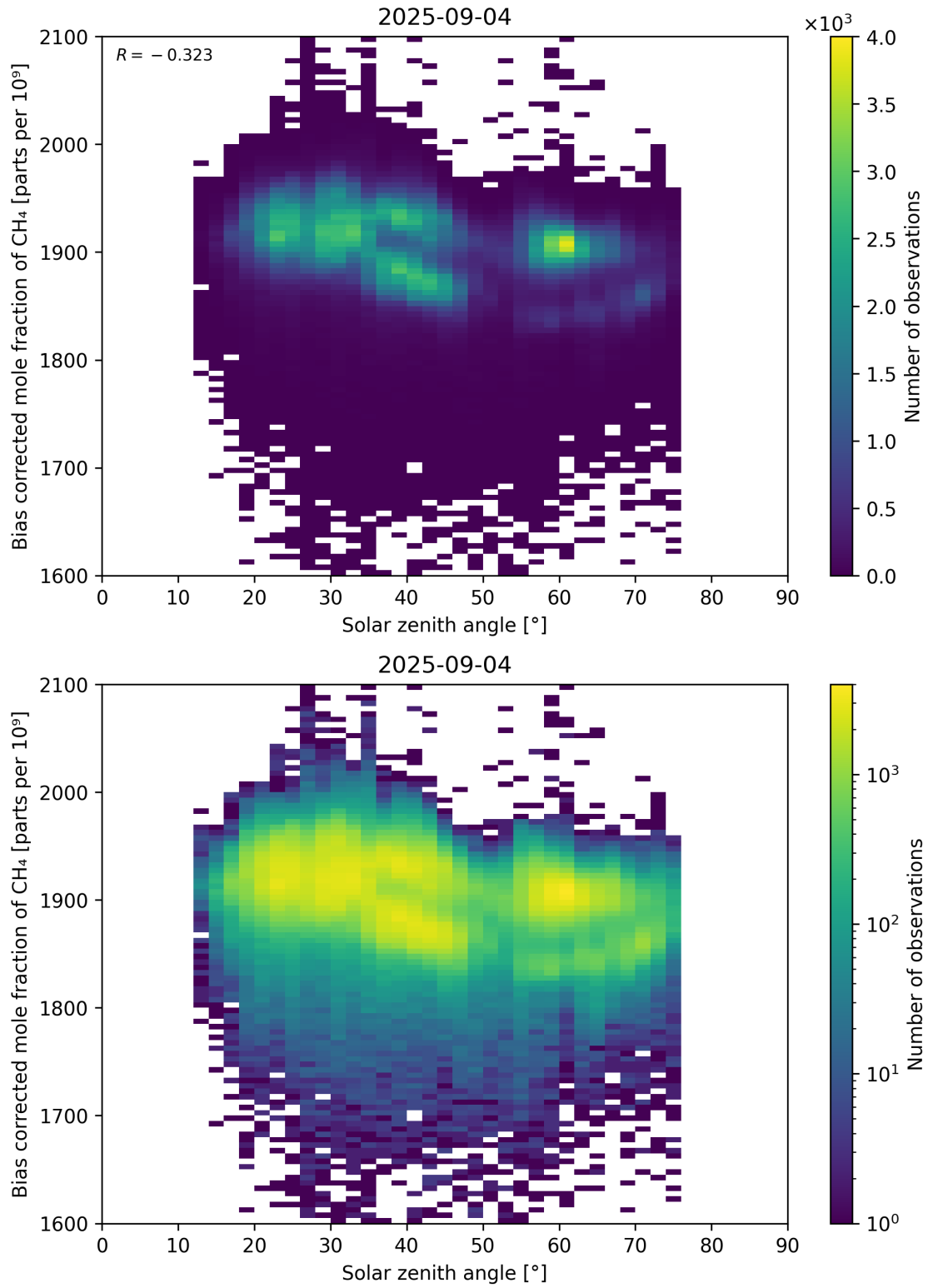
Figure 100: Scatter density plot of “Solar zenith angle” against “Bias corrected mole fraction of CH 4 ” for 2025-09-04 to 2025-09-05.
