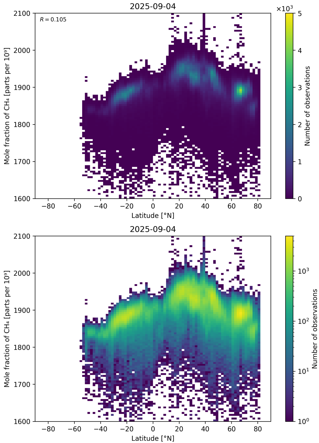
Figure 57: Scatter density plot of “Latitude” against “Mole fraction of CH 4 ” for 2025-09-04 to 2025-09-05.
