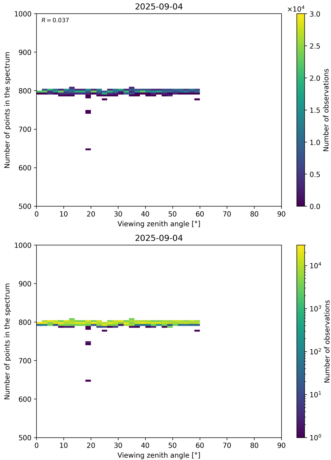
Figure 114: Scatter density plot of “Viewing zenith angle” against “Number of points in the spectrum” for 2025-09-04 to 2025-09-05.
