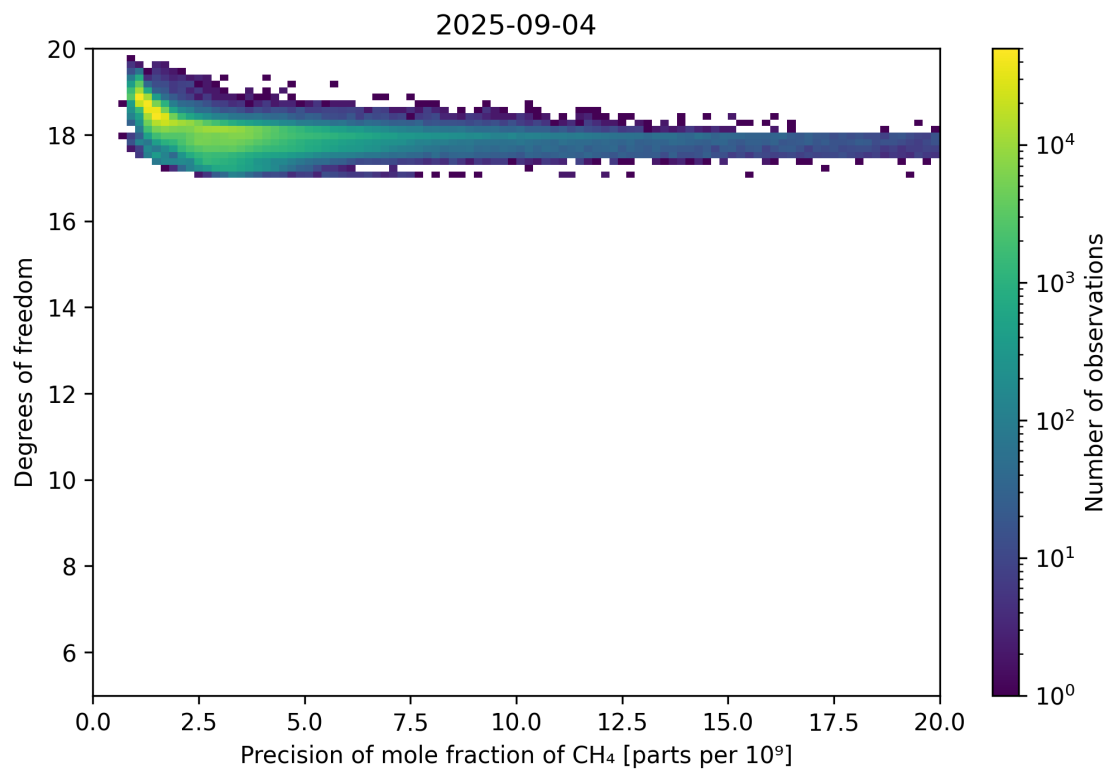
Figure 80: Scatter density plot of “Precision of mole fraction of CH 4 ” against “Degrees of freedom” for 2025-09-04 to 2025-09-05.
