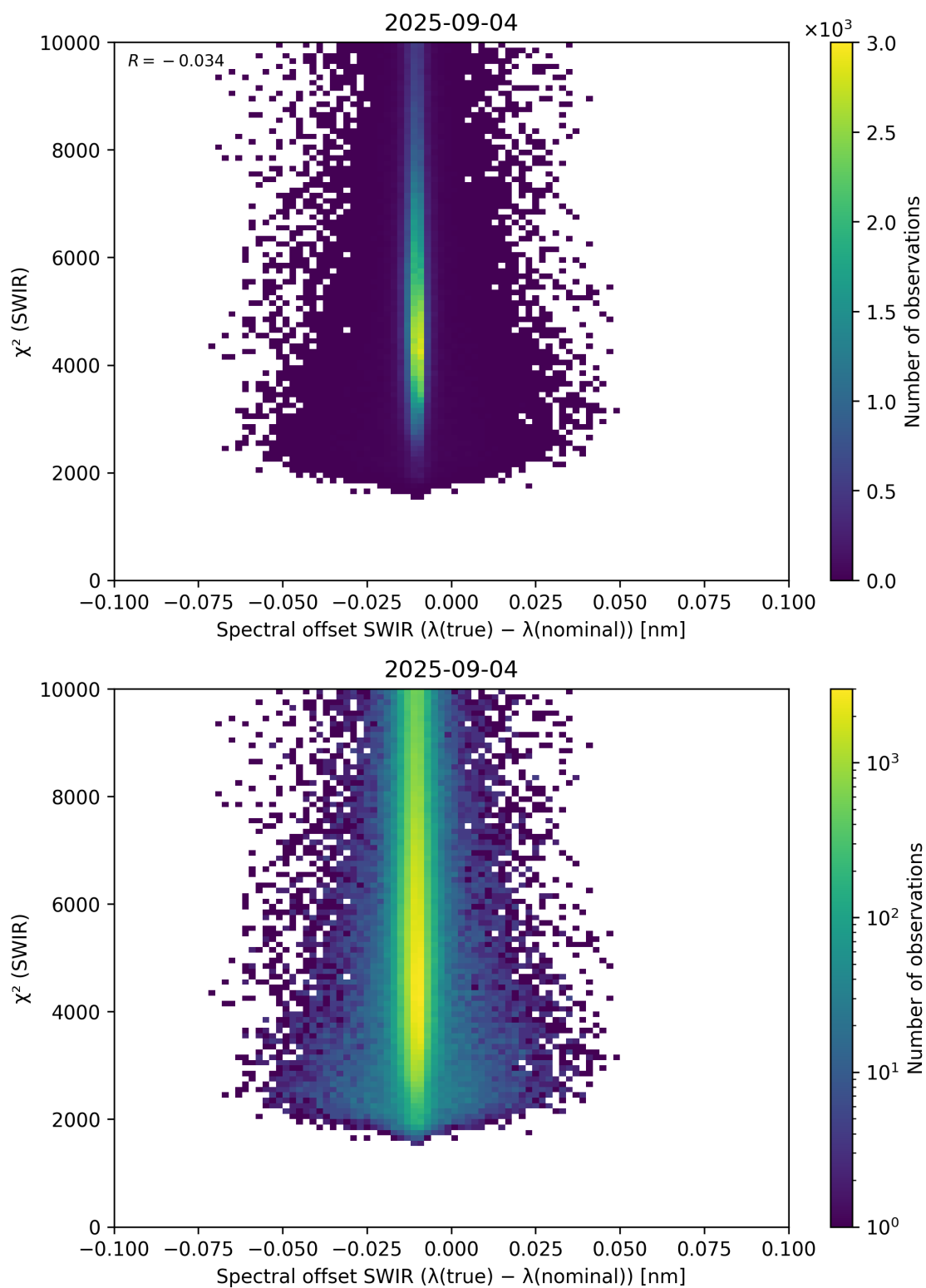
Figure 118: Scatter density plot of “Spectral offset SWIR ( \lambda_{\text{true}} - \lambda_{\text{nominal}} )” against “ \chi^2 (SWIR)” for 2025-09-04 to 2025-09-05.
