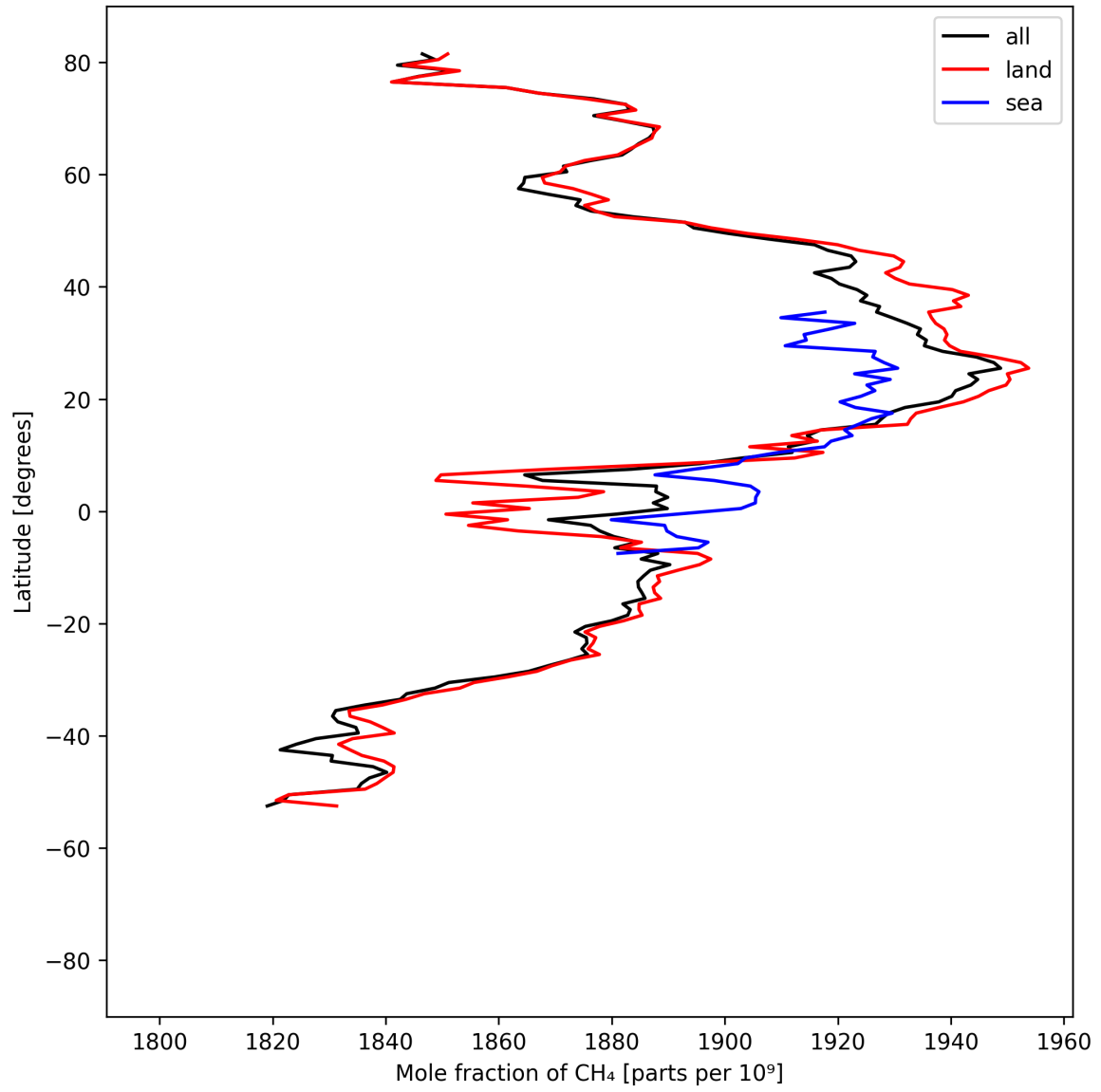
Figure 12: Zonal average of “Mole fraction of \text{CH}_4 ” for 2025-09-04 to 2025-09-05.
