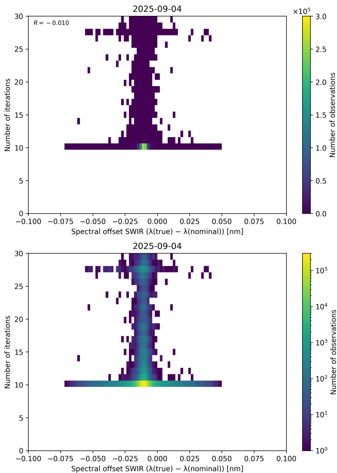
Figure 121: Scatter density plot of “Spectral offset SWIR ( \lambda_{\text{true}} - \lambda_{\text{nominal}} )” against “Number of iterations” for 2025-09-04 to 2025-09-05.
