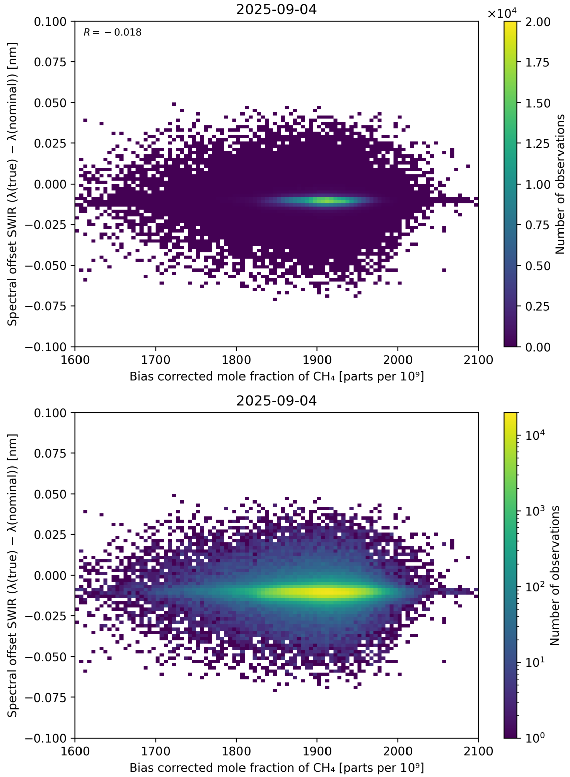
Figure 69: Scatter density plot of “Bias corrected mole fraction of \text{CH}_4 ” against “Spectral offset SWIR ( \lambda_{\text{true}} - \lambda_{\text{nominal}} )” for 2025-09-04 to 2025-09-05.
