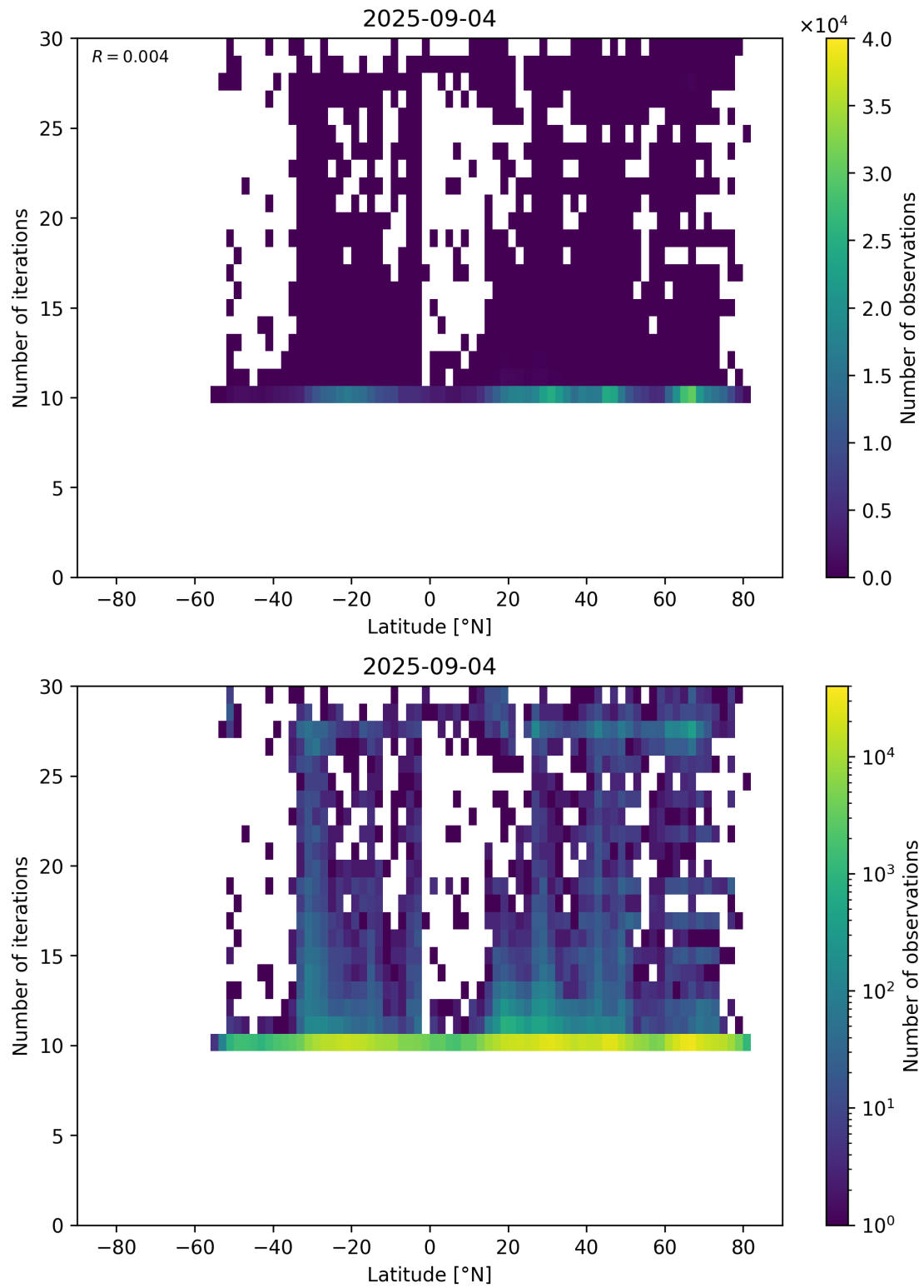
Figure 60: Scatter density plot of “Latitude” against “Number of iterations” for 2025-09-04 to 2025-09-05.
