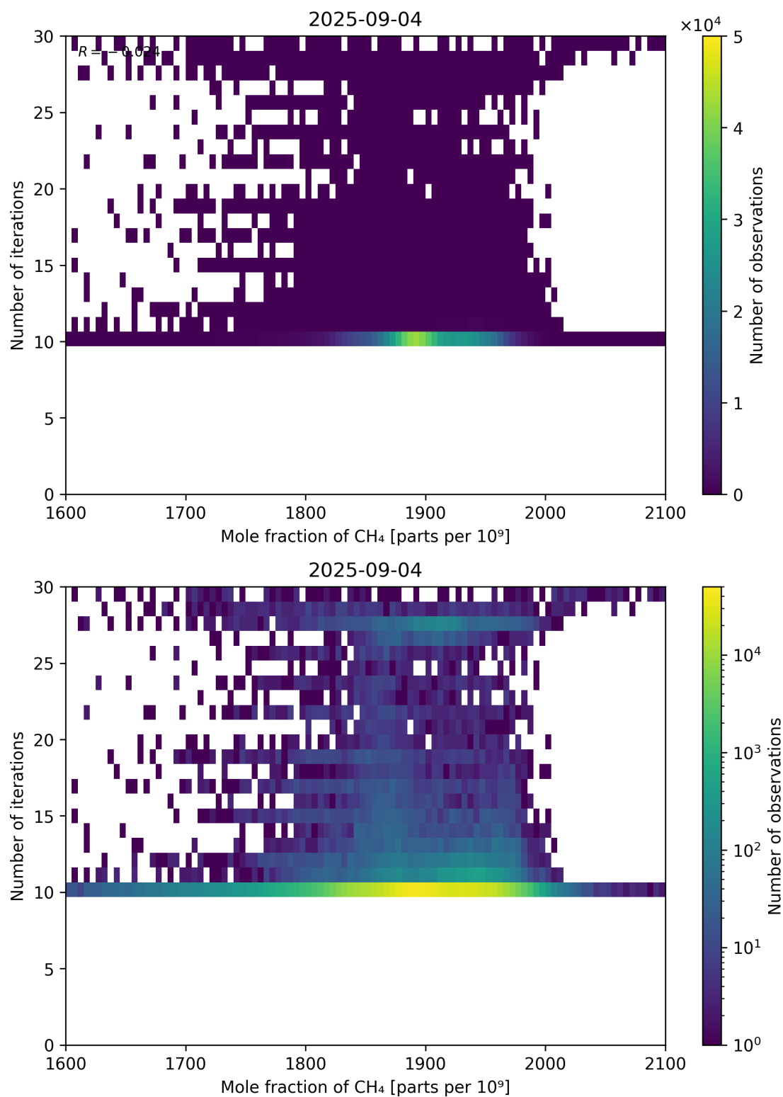
Figure 76: Scatter density plot of “Mole fraction of CH 4 ” against “Number of iterations” for 2025-09-04 to 2025-09-05.
