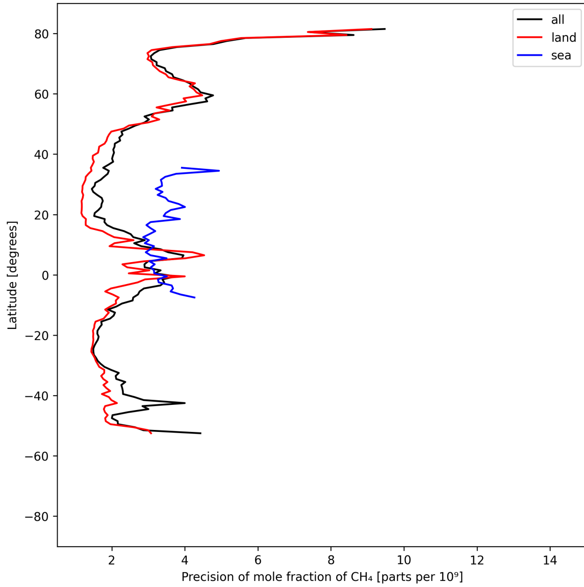
Figure 13: Zonal average of “Precision of mole fraction of CH 4 ” for 2025-09-04 to 2025-09-05.
