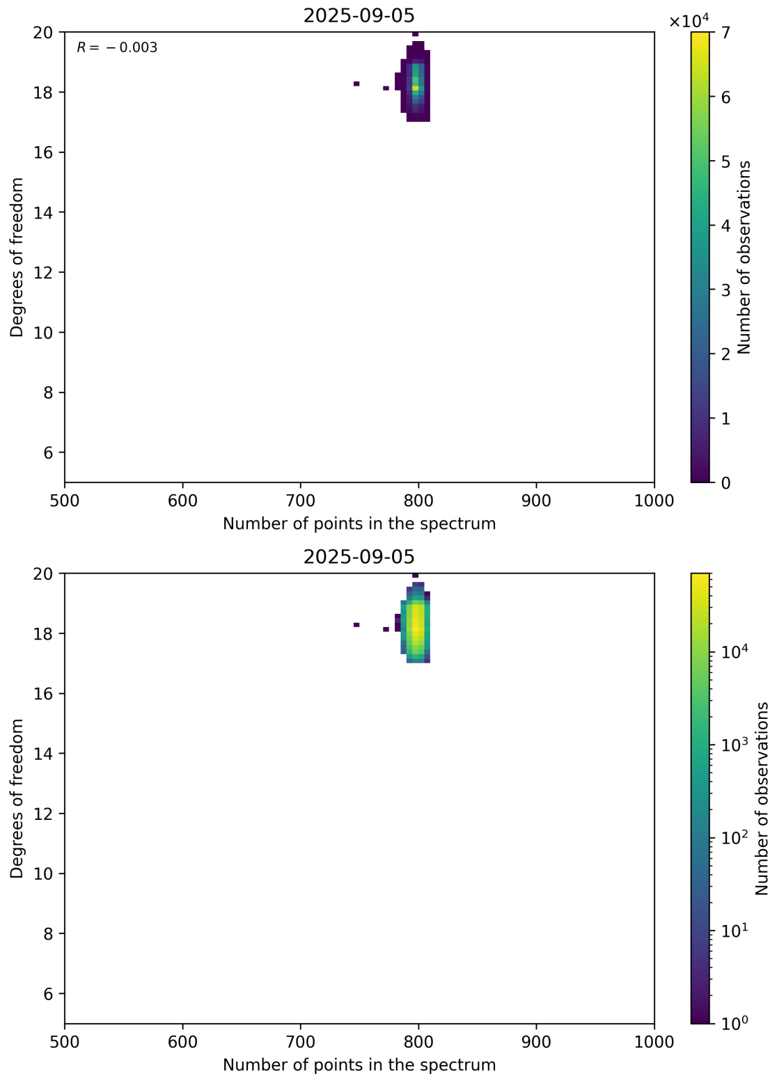
Figure 90: Scatter density plot of “Number of points in the spectrum” against “Degrees of freedom” for 2025-09-04 to 2025-09-06.
