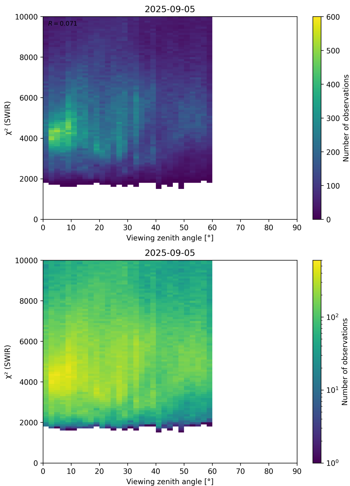
Figure 106: Scatter density plot of “Viewing zenith angle” against “ \chi^2 (SWIR)” for 2025-09-04 to 2025-09-06.
