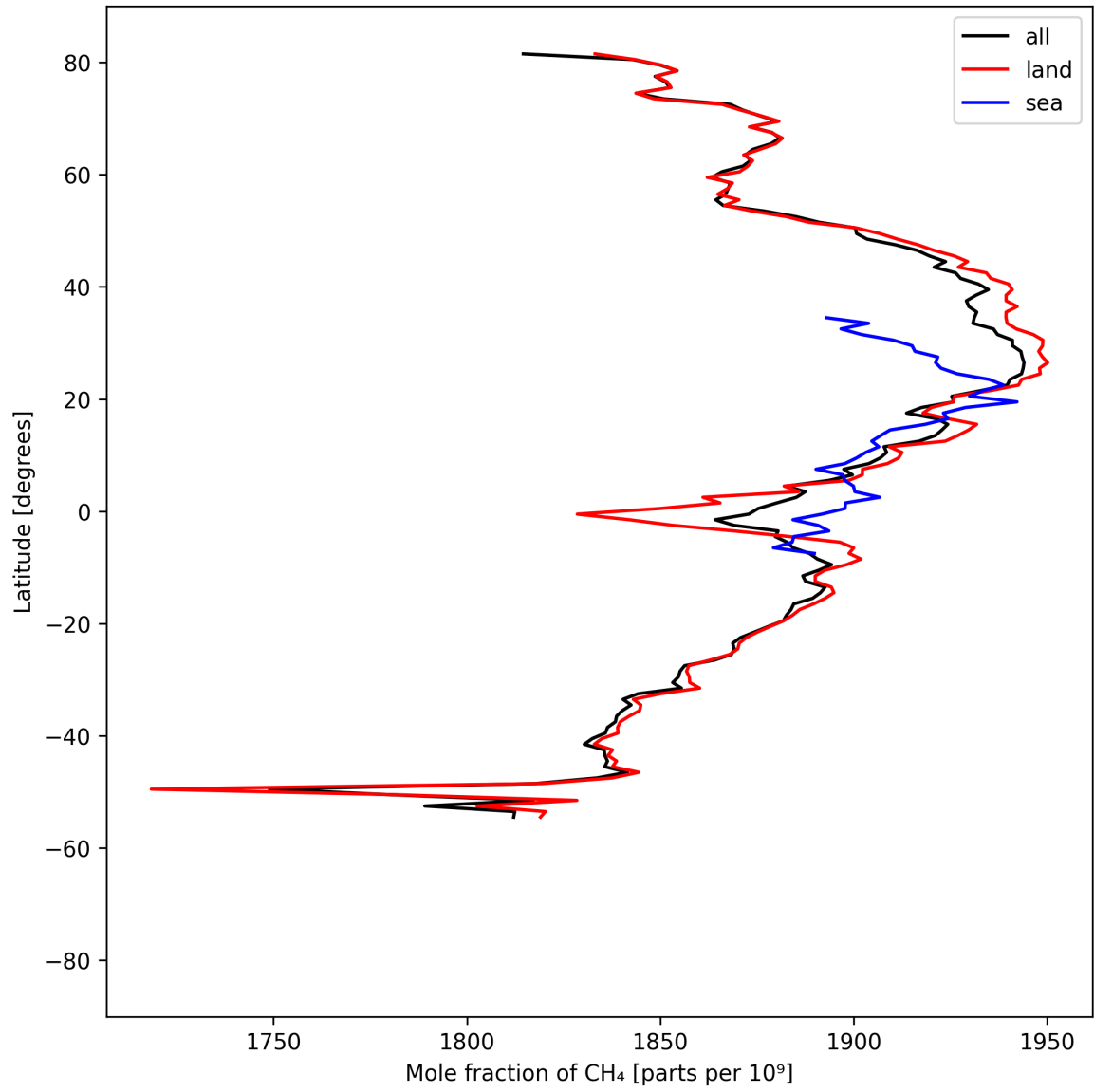
Figure 12: Zonal average of “Mole fraction of \text{CH}_4 ” for 2025-09-04 to 2025-09-06.
