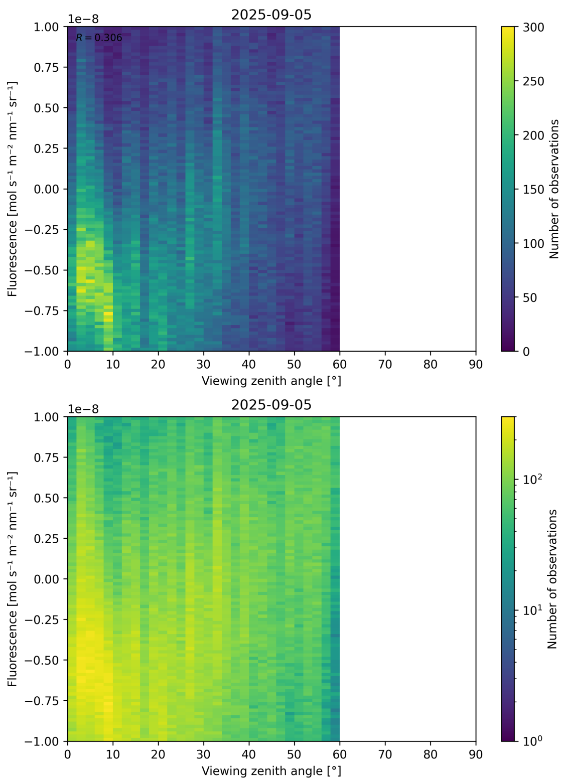
Figure 108: Scatter density plot of “Viewing zenith angle” against “Fluorescence” for 2025-09-04 to 2025-09-06.
