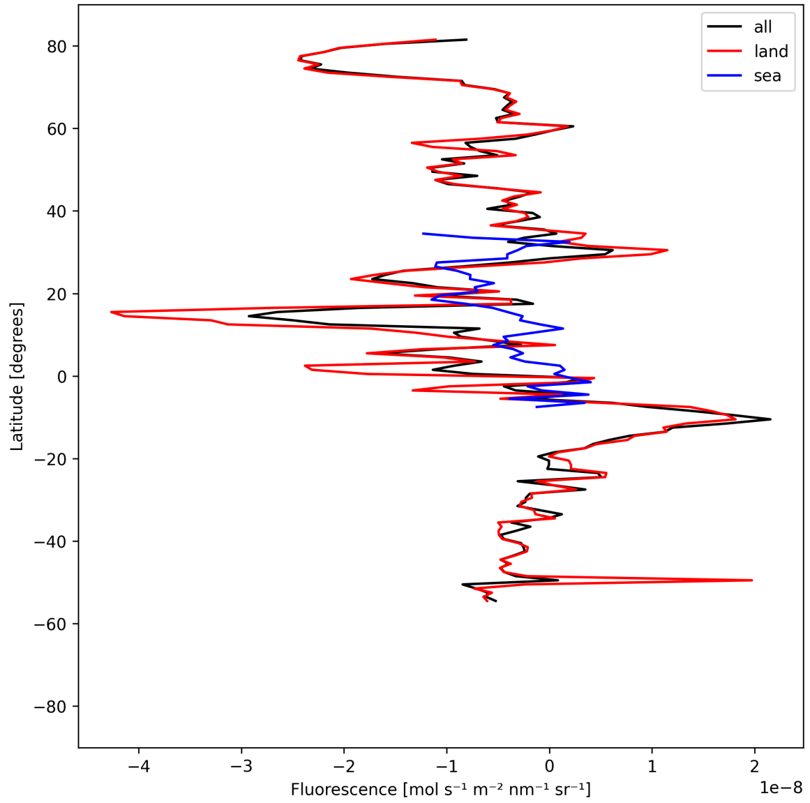
Figure 21: Zonal average of “Fluorescence” for 2025-09-04 to 2025-09-06.
