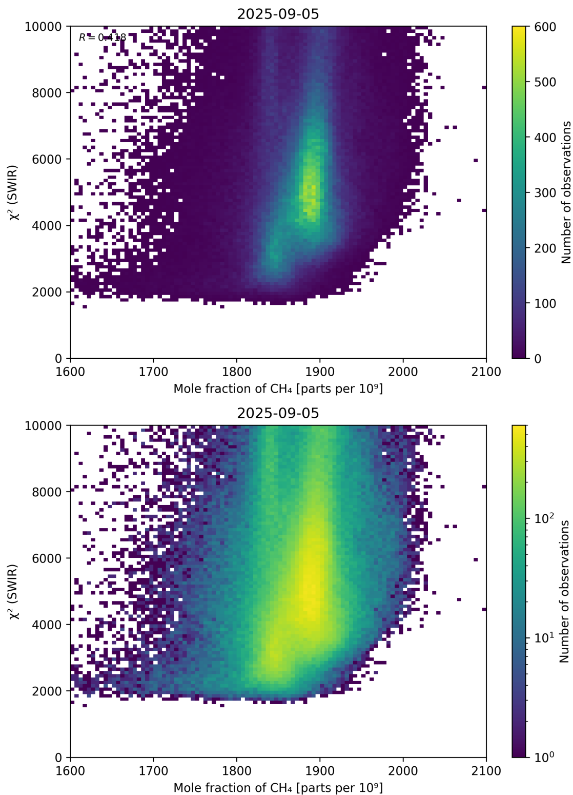
Figure 71: Scatter density plot of “Mole fraction of \text{CH}_4 ” against “ \chi^2 (SWIR)” for 2025-09-04 to 2025-09-06.
