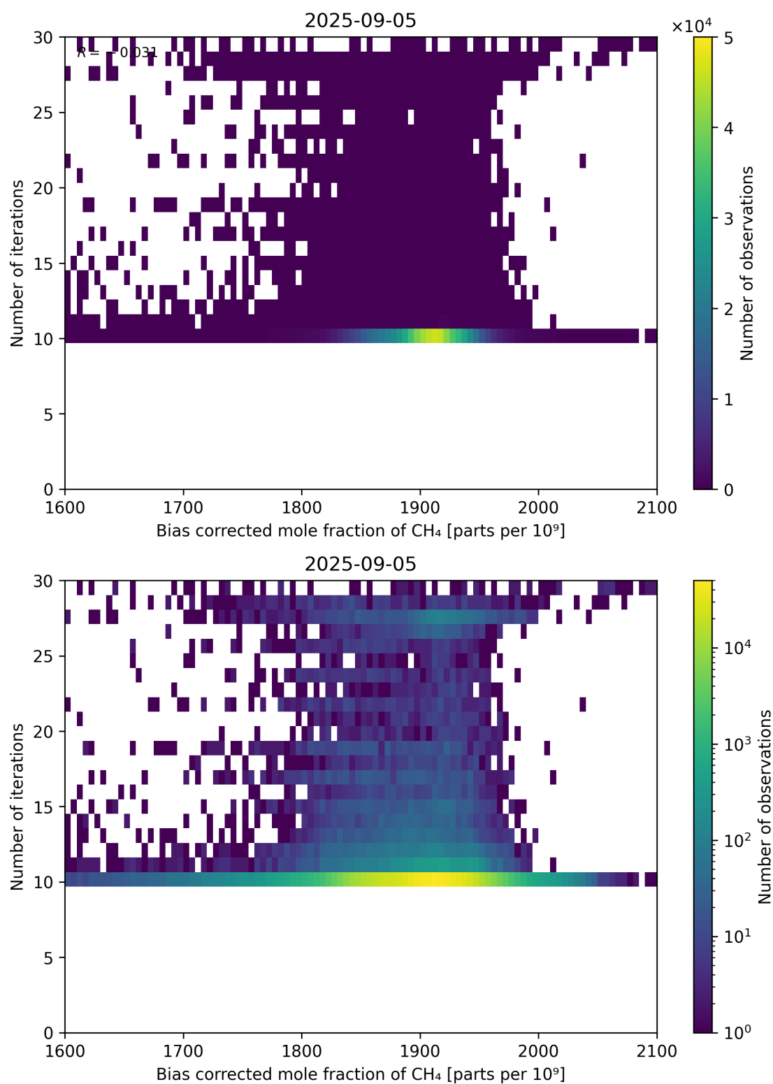
Figure 67: Scatter density plot of “Bias corrected mole fraction of CH 4 ” against “Number of iterations” for 2025-09-04 to 2025-09-06.
