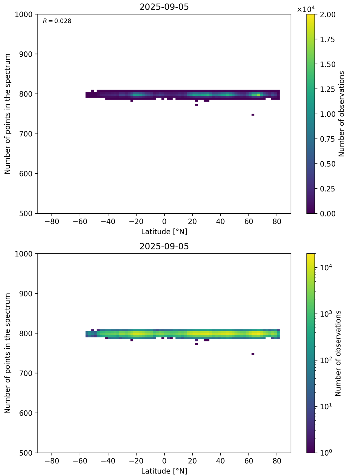
Figure 61: Scatter density plot of “Latitude” against “Number of points in the spectrum” for 2025-09-04 to 2025-09-06.
