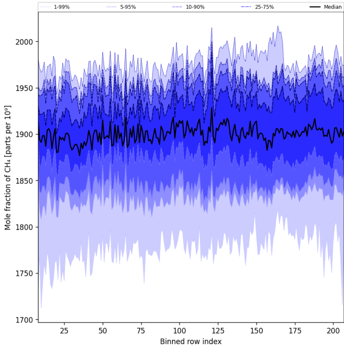
Figure 34: Along track statistics of “Mole fraction of CH 4 ” for 2025-09-04 to 2025-09-06
