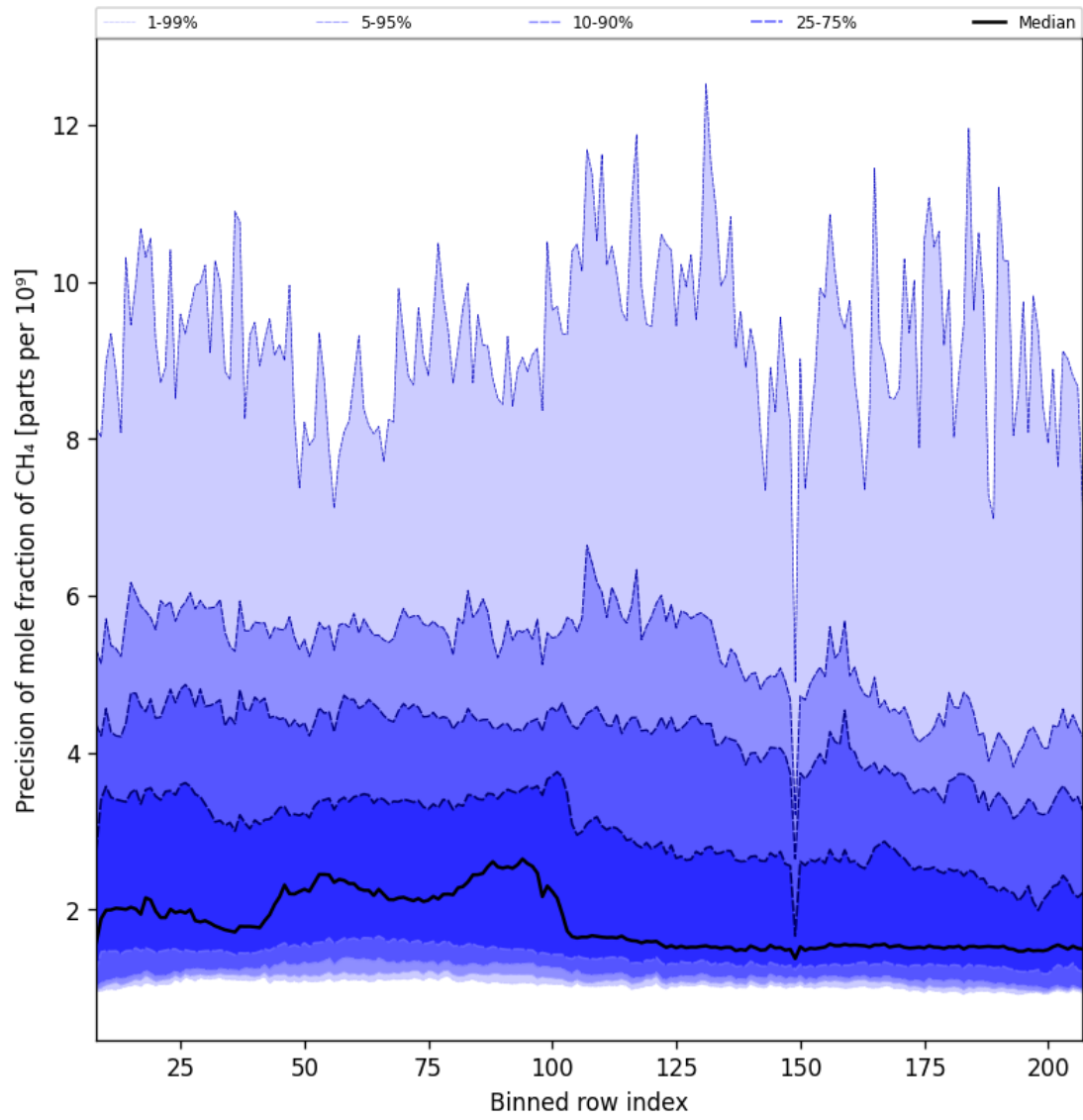
Figure 35: Along track statistics of “Precision of mole fraction of CH 4 ” for 2025-09-04 to 2025-09-06
