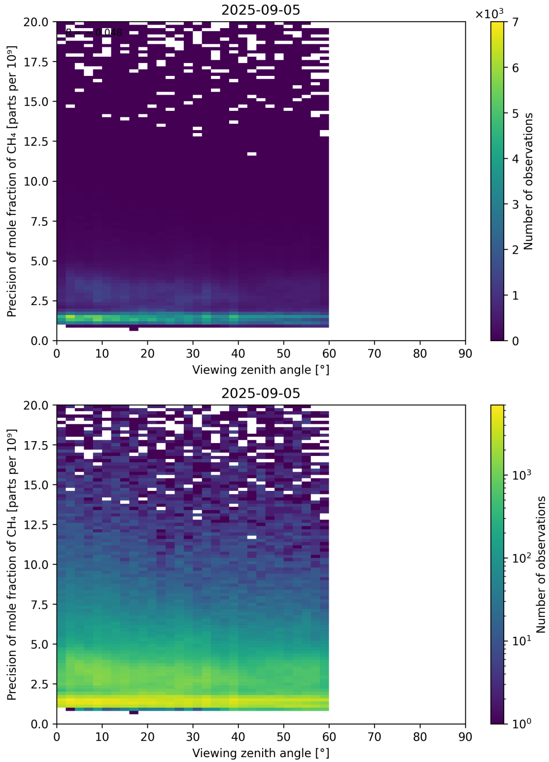
Figure 112: Scatter density plot of “Viewing zenith angle” against “Precision of mole fraction of CH 4 ” for 2025-09-04 to 2025-09-06.
