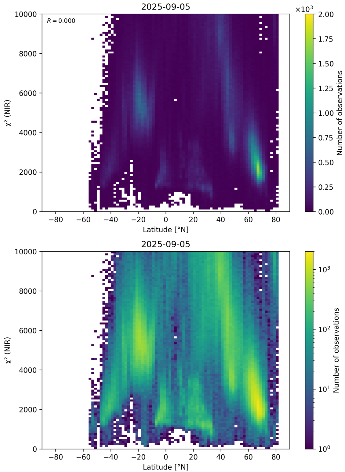
Figure 53: Scatter density plot of “Latitude” against “ \chi^2 (NIR)” for 2025-09-04 to 2025-09-06.
