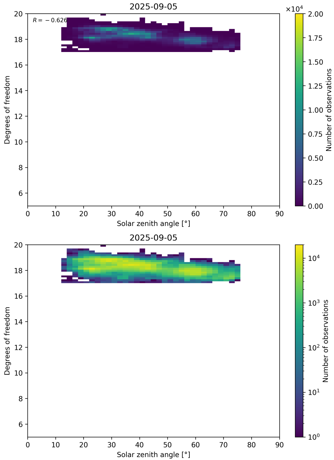
Figure 96: Scatter density plot of “Solar zenith angle” against “Degrees of freedom” for 2025-09-04 to 2025-09-06.
