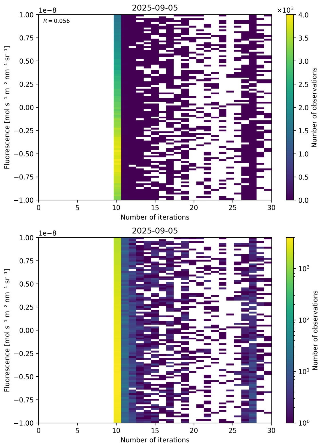
Figure 87: Scatter density plot of “Number of iterations” against “Fluorescence” for 2025-09-04 to 2025-09-06.
