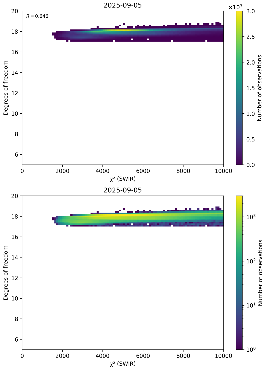
Figure 48: Scatter density plot of “ \chi^2 (SWIR)” against “Degrees of freedom” for 2025-09-04 to 2025-09-06.
