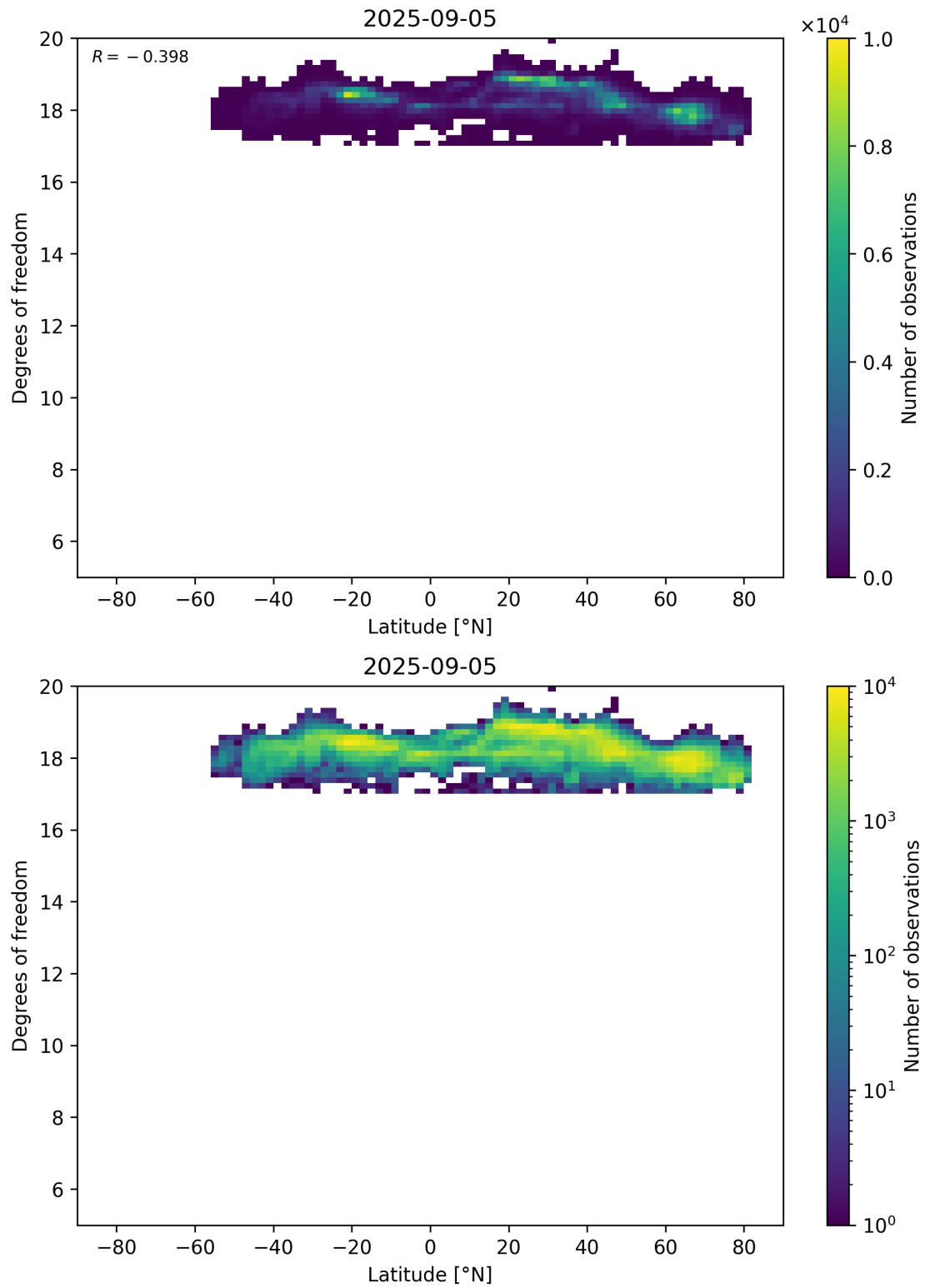
Figure 55: Scatter density plot of “Latitude” against “Degrees of freedom” for 2025-09-04 to 2025-09-06.
