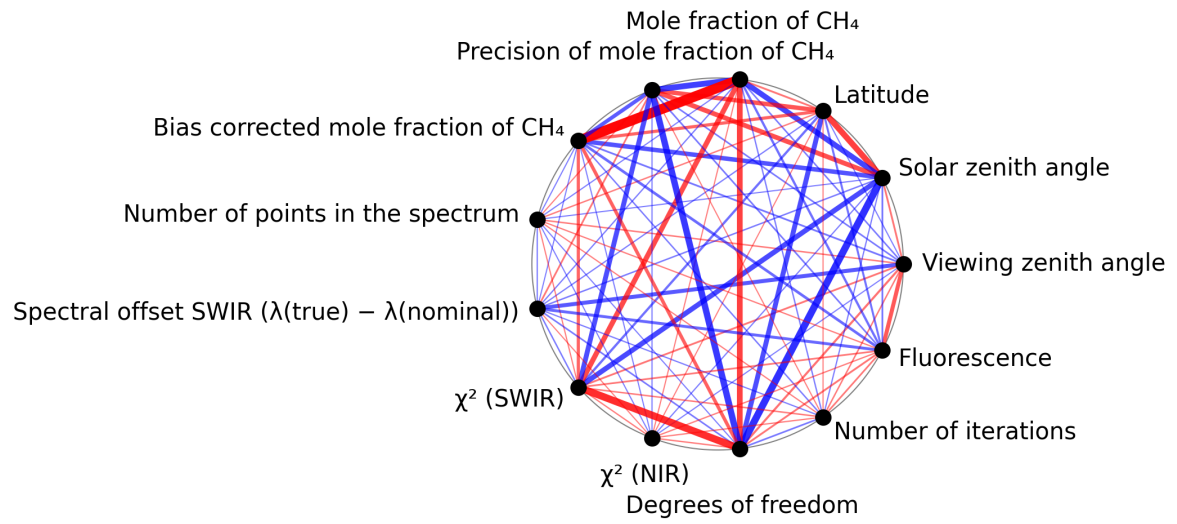
Figure 1: Map of correlation graph for 2025-09-04 to 2025-09-06.
