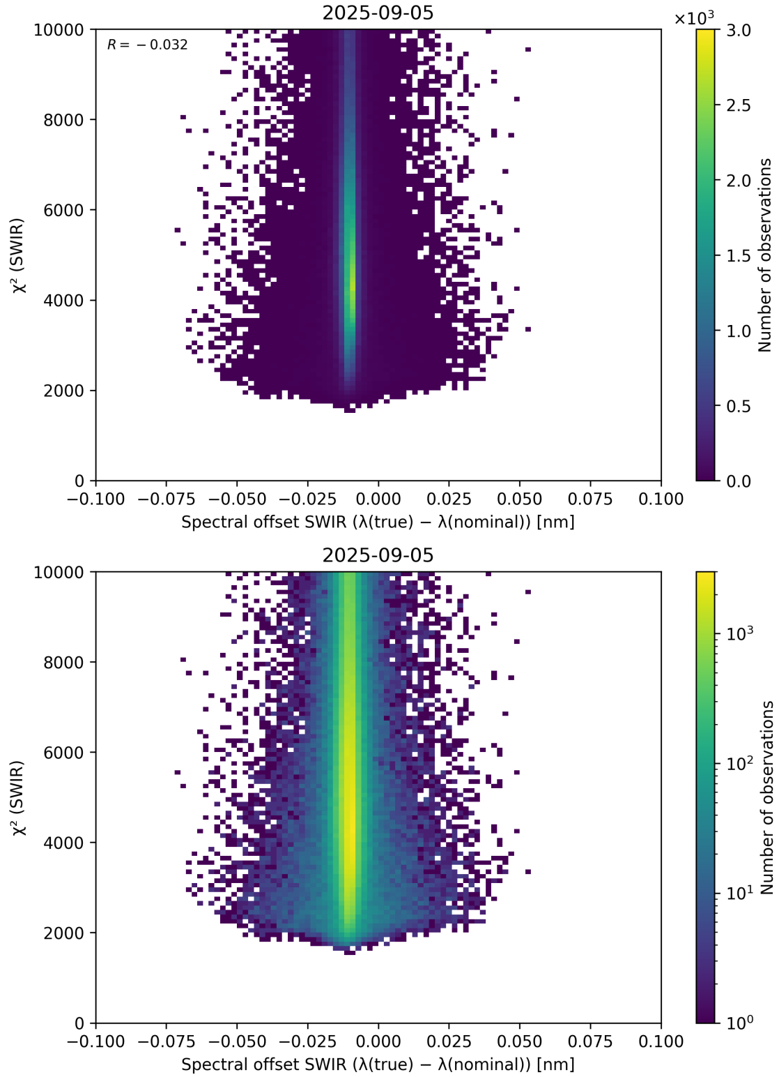
Figure 118: Scatter density plot of “Spectral offset SWIR ( \lambda_{\text{true}} - \lambda_{\text{nominal}} )” against “ \chi^2 (SWIR)” for 2025-09-04 to 2025-09-06.
