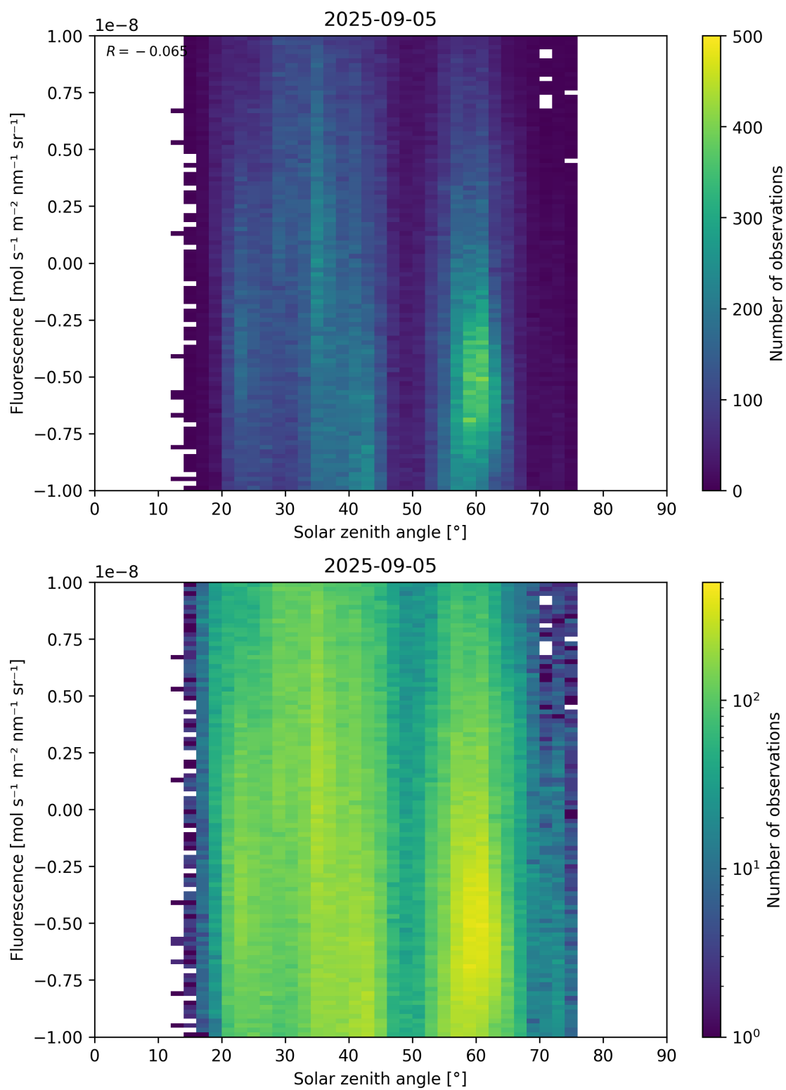
Figure 97: Scatter density plot of “Solar zenith angle” against “Fluorescence” for 2025-09-04 to 2025-09-06.
