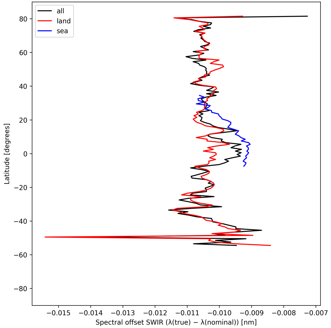
Figure 16: Zonal average of “Spectral offset SWIR ( \lambda_{\text{true}} - \lambda_{\text{nominal}} )” for 2025-09-04 to 2025-09-06.
