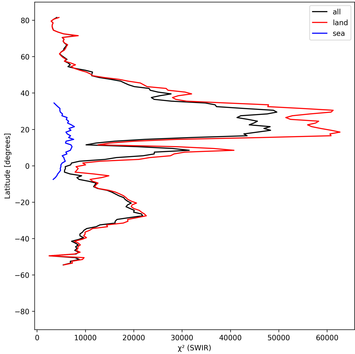
Figure 17: Zonal average of “ \chi^2 (SWIR)” for 2025-09-04 to 2025-09-06.
