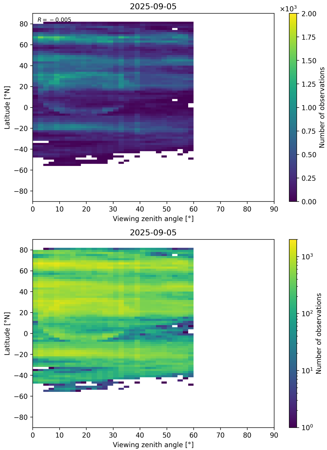
Figure 109: Scatter density plot of “Viewing zenith angle” against “Latitude” for 2025-09-04 to 2025-09-06.
