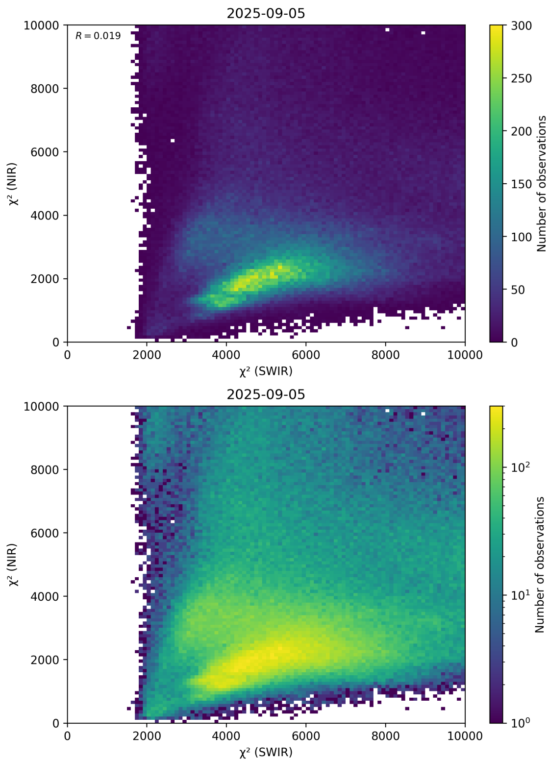
Figure 47: Scatter density plot of “ \chi^2 (SWIR)” against “ \chi^2 (NIR)” for 2025-09-04 to 2025-09-06.
