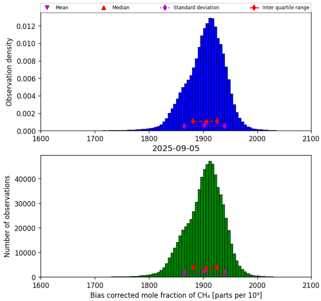
Figure 25: Histogram of “Bias corrected mole fraction of CH 4 ” for 2025-09-04 to 2025-09-06
