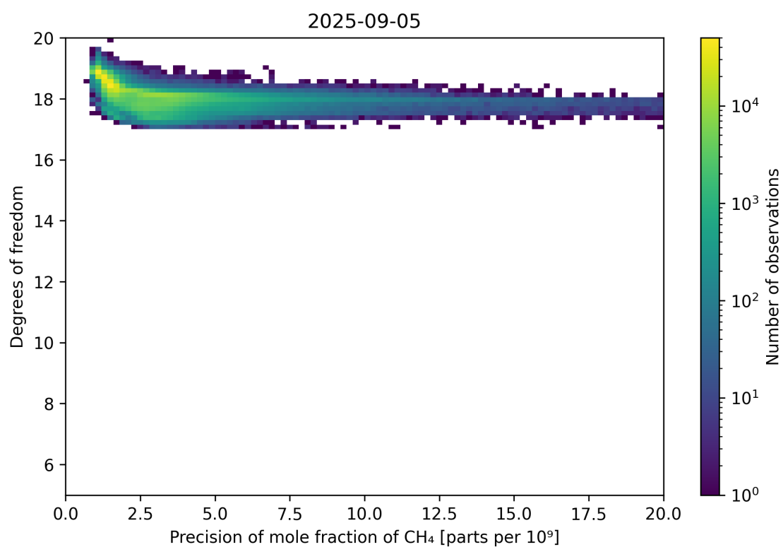
Figure 80: Scatter density plot of “Precision of mole fraction of CH 4 ” against “Degrees of freedom” for 2025-09-04 to 2025-09-06.
