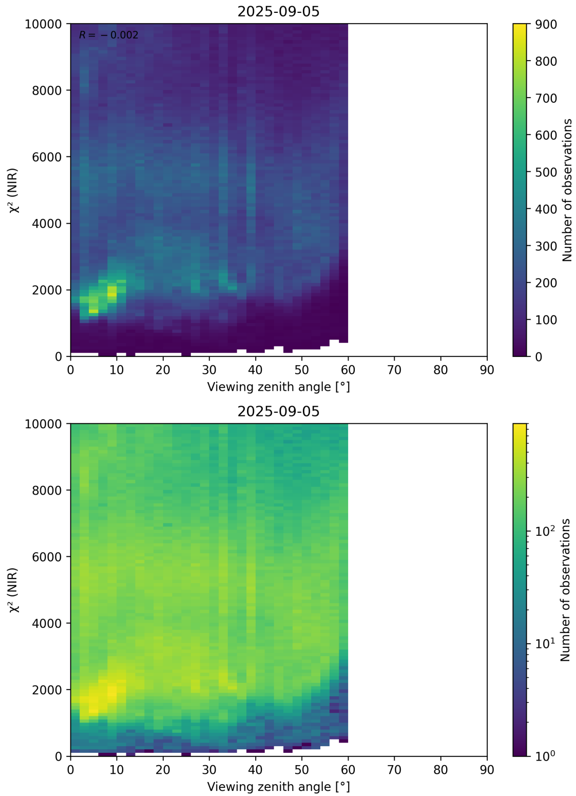
Figure 105: Scatter density plot of “Viewing zenith angle” against “ \chi^2 (NIR)” for 2025-09-04 to 2025-09-06.
