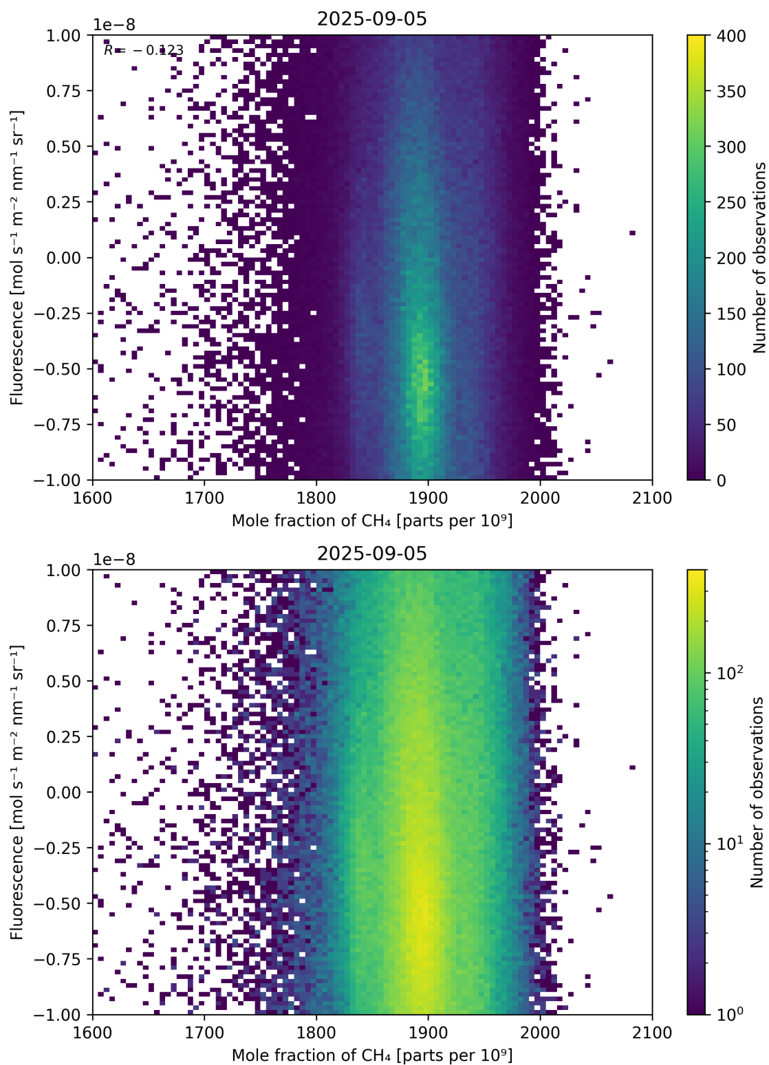
Figure 73: Scatter density plot of “Mole fraction of \text{CH}_4 ” against “Fluorescence” for 2025-09-04 to 2025-09-06.
