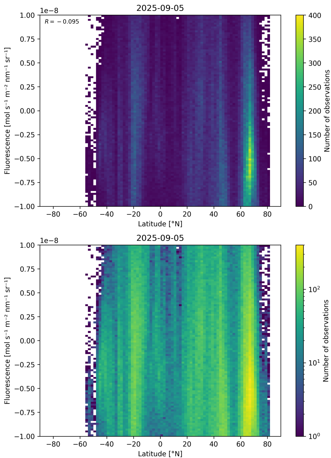
Figure 56: Scatter density plot of “Latitude” against “Fluorescence” for 2025-09-04 to 2025-09-06.
