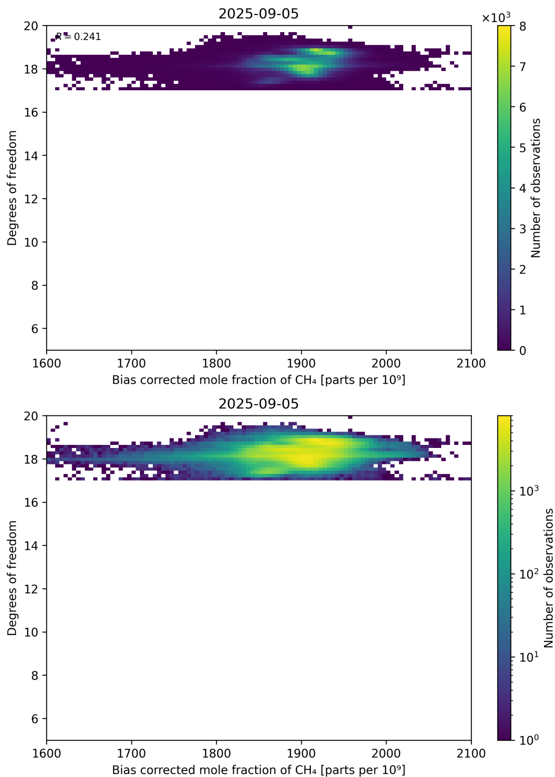
Figure 65: Scatter density plot of “Bias corrected mole fraction of CH 4 ” against “Degrees of freedom” for 2025-09-04 to 2025-09-06.
