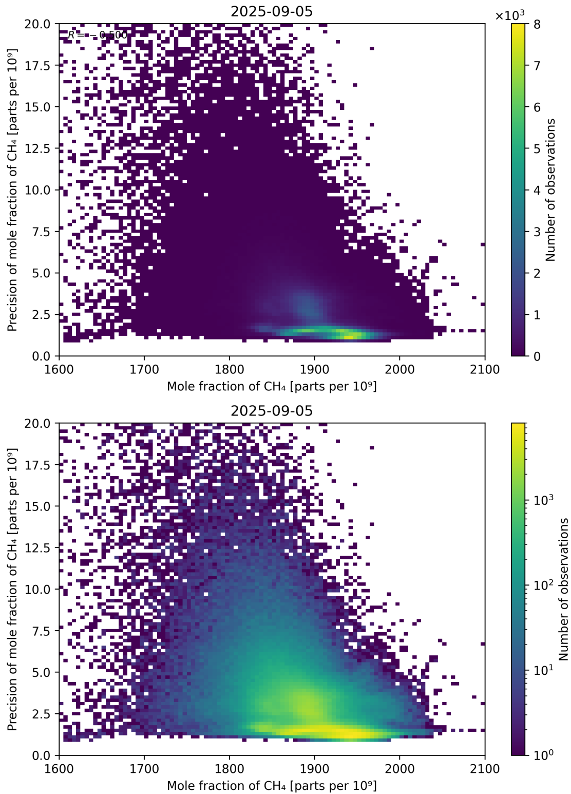
Figure 75: Scatter density plot of “Mole fraction of CH 4 ” against “Precision of mole fraction of CH 4 ” for 2025-09-04 to 2025-09-06.
