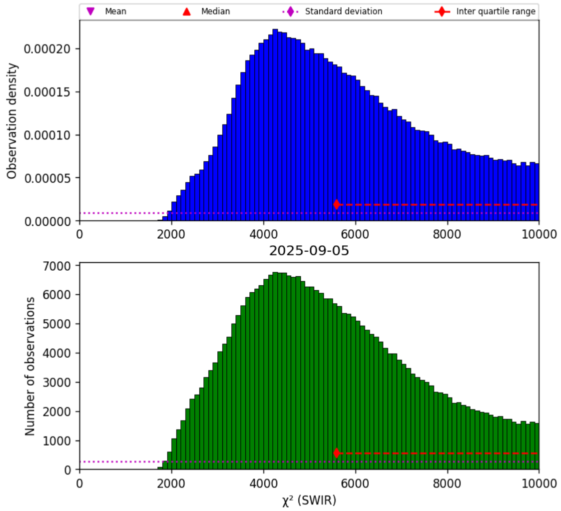
Figure 28: Histogram of " \chi^2 (SWIR)" for 2025-09-04 to 2025-09-06
