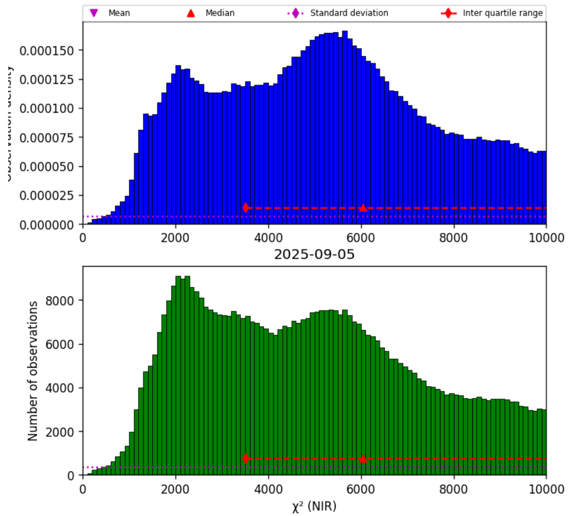
Figure 29: Histogram of “ \chi^2 (NIR)” for 2025-09-04 to 2025-09-06
