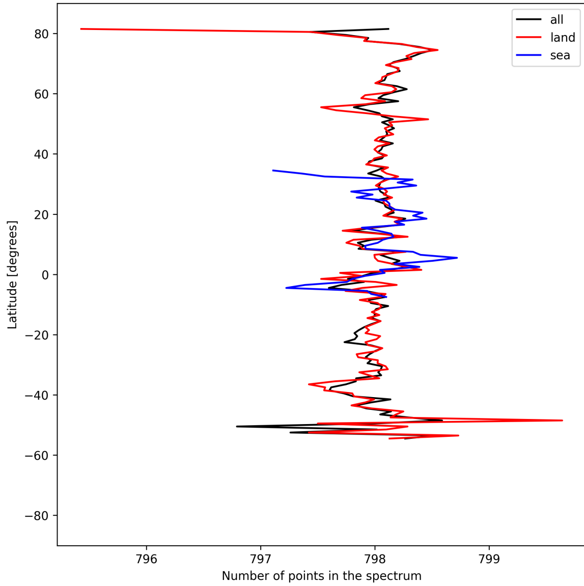
Figure 15: Zonal average of “Number of points in the spectrum” for 2025-09-04 to 2025-09-06.
