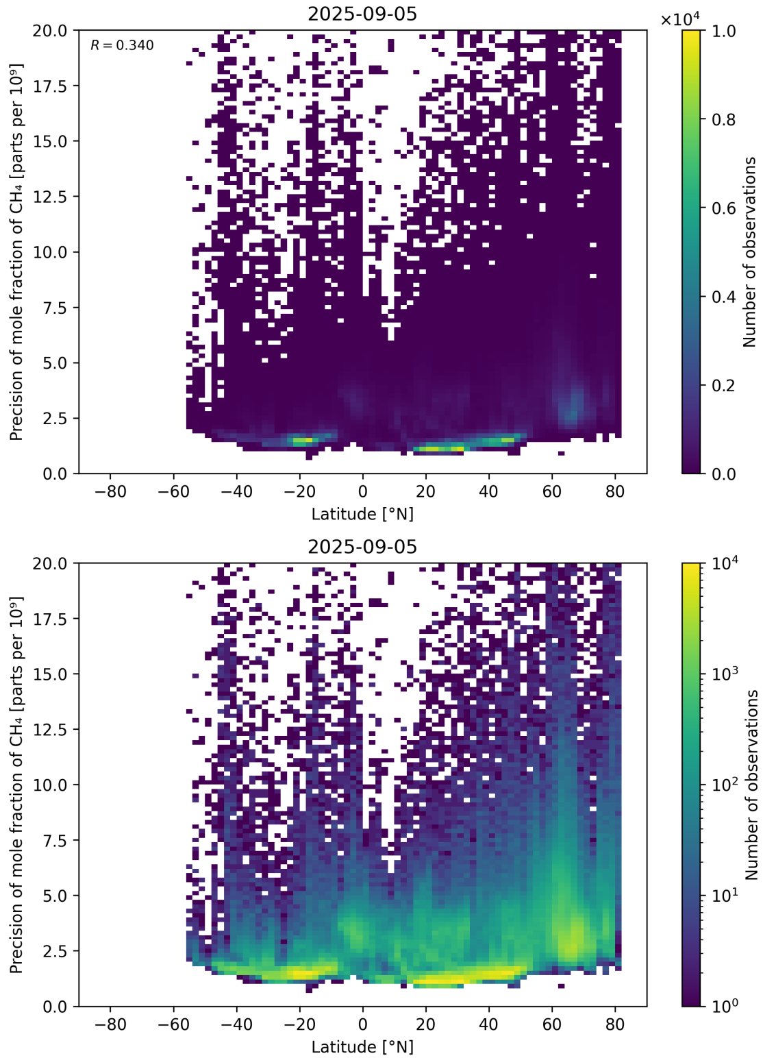
Figure 59: Scatter density plot of “Latitude” against “Precision of mole fraction of \text{CH}_4 ” for 2025-09-04 to 2025-09-06.
