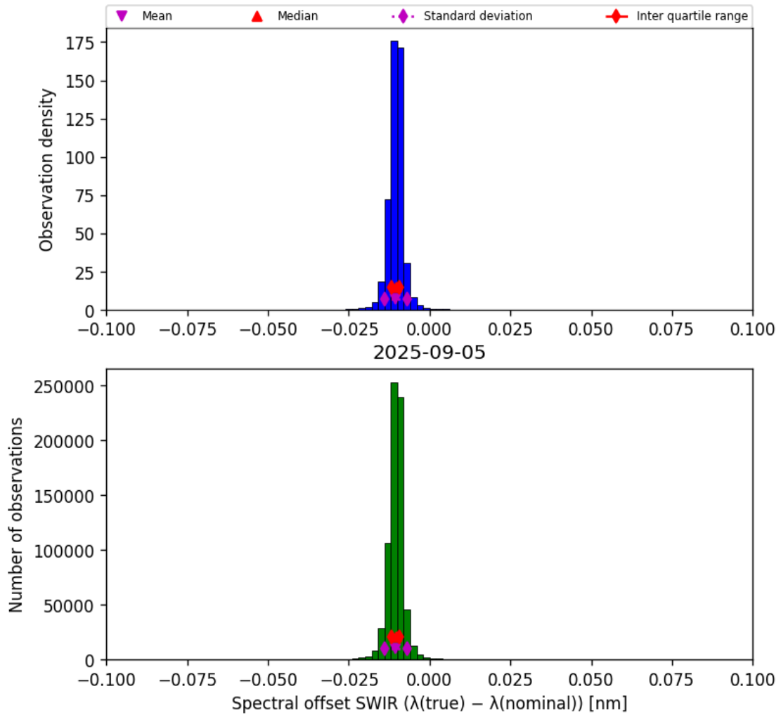
Figure 27: Histogram of “Spectral offset SWIR ( \lambda_{\text{true}} - \lambda_{\text{nominal}} )” for 2025-09-04 to 2025-09-06
