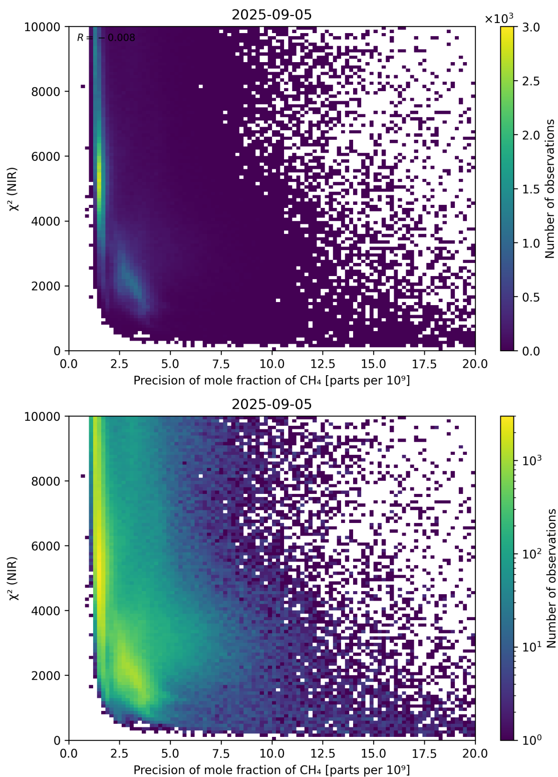
Figure 78: Scatter density plot of “Precision of mole fraction of CH 4 ” against “ \chi^2 (NIR)” for 2025-09-04 to 2025-09-06.
