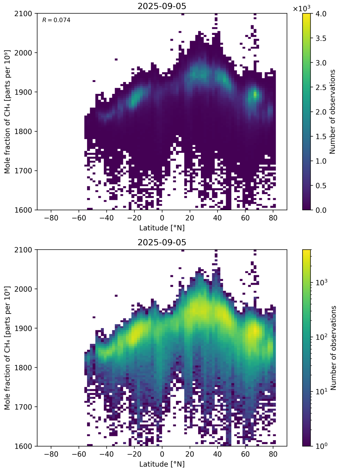
Figure 57: Scatter density plot of “Latitude” against “Mole fraction of CH 4 ” for 2025-09-04 to 2025-09-06.
