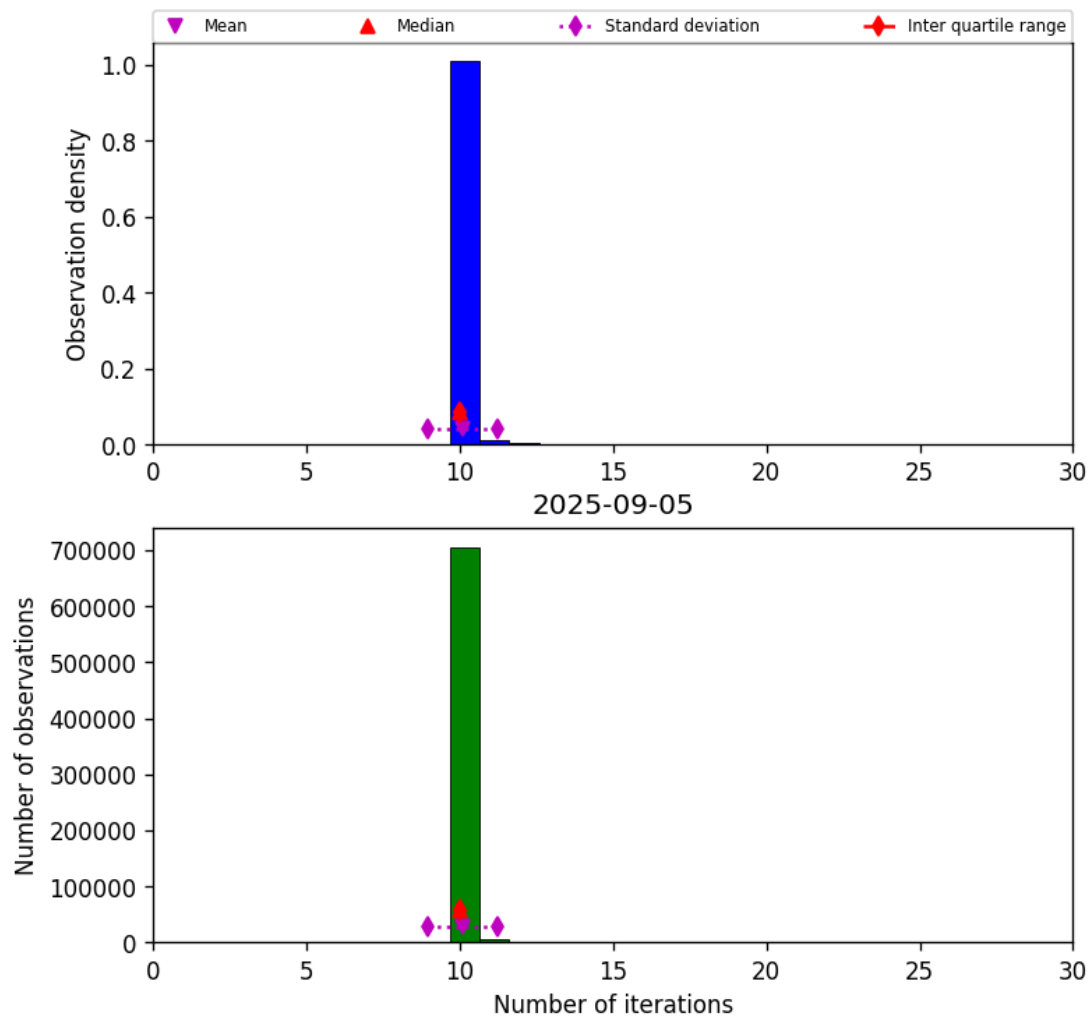
Figure 31: Histogram of “Number of iterations” for 2025-09-04 to 2025-09-06
