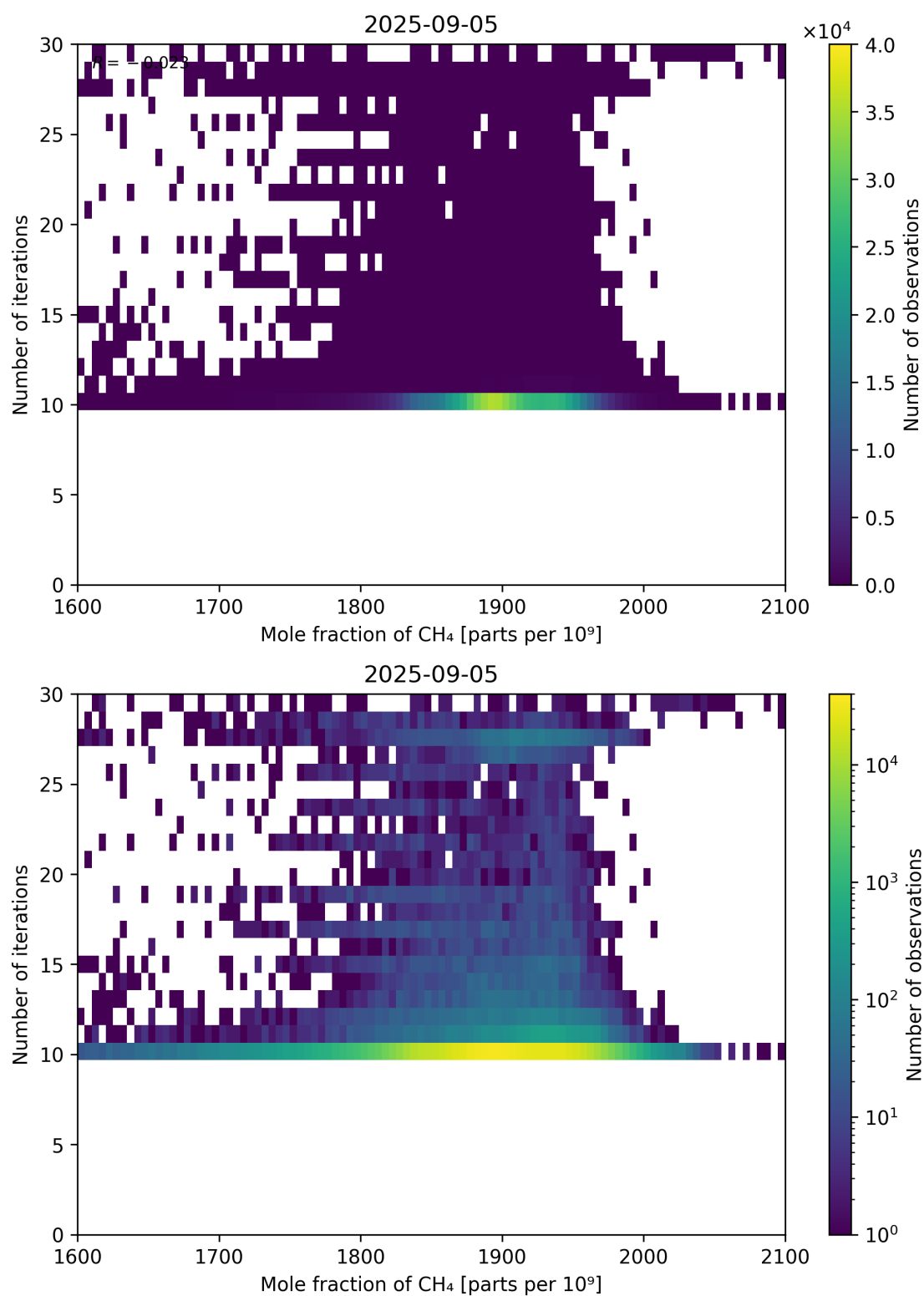
Figure 76: Scatter density plot of “Mole fraction of CH 4 ” against “Number of iterations” for 2025-09-04 to 2025-09-06.
