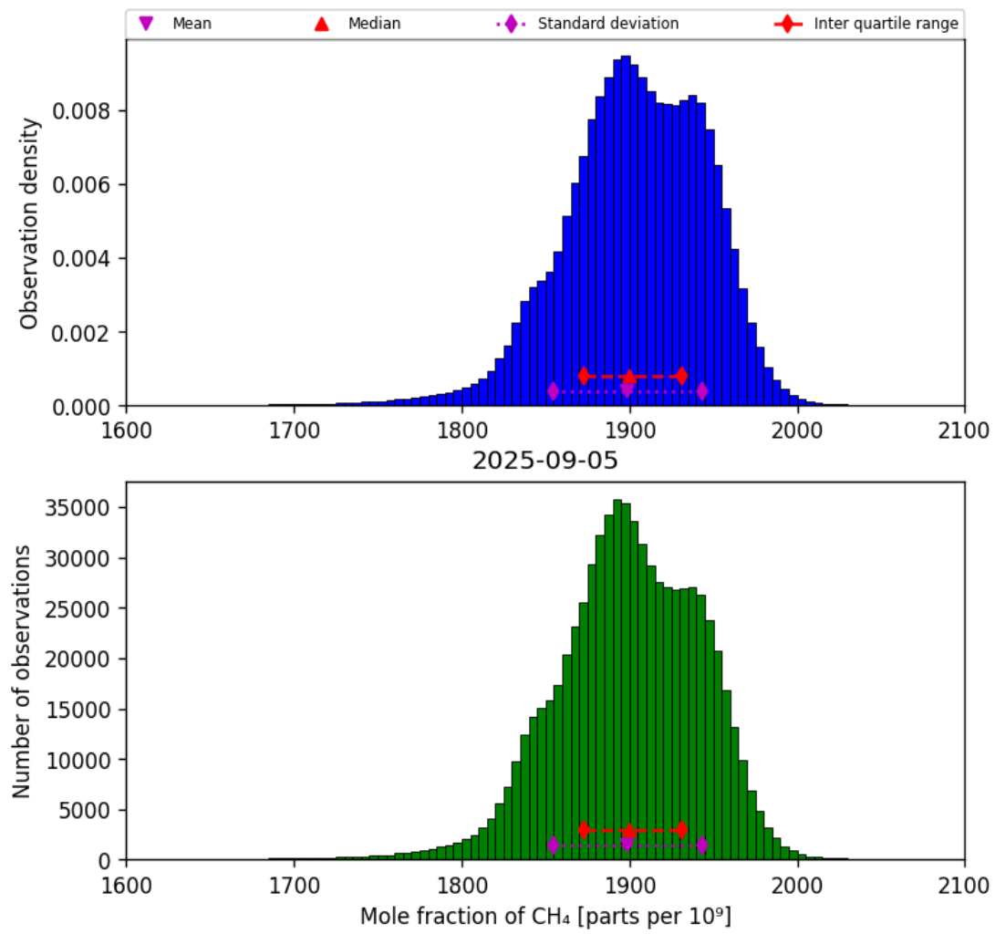
Figure 23: Histogram of “Mole fraction of CH 4 ” for 2025-09-04 to 2025-09-06
