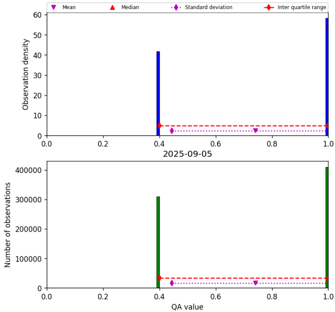
Figure 22: Histogram of “QA value” for 2025-09-04 to 2025-09-06
