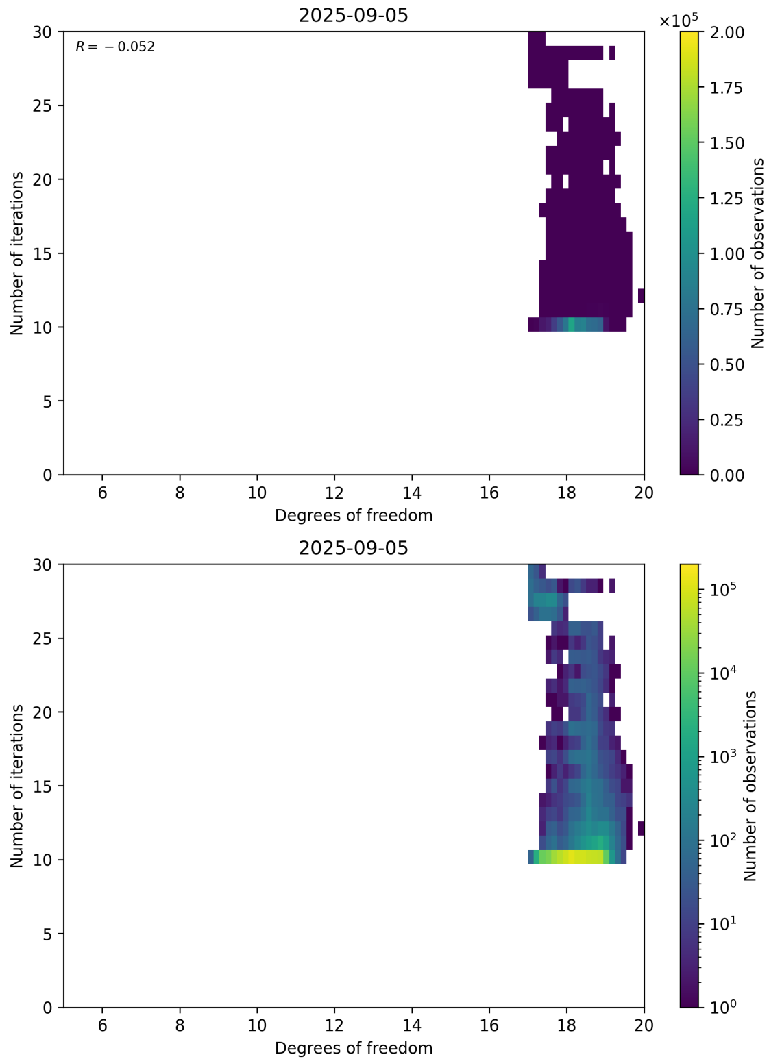
Figure 52: Scatter density plot of “Degrees of freedom” against “Number of iterations” for 2025-09-04 to 2025-09-06.
