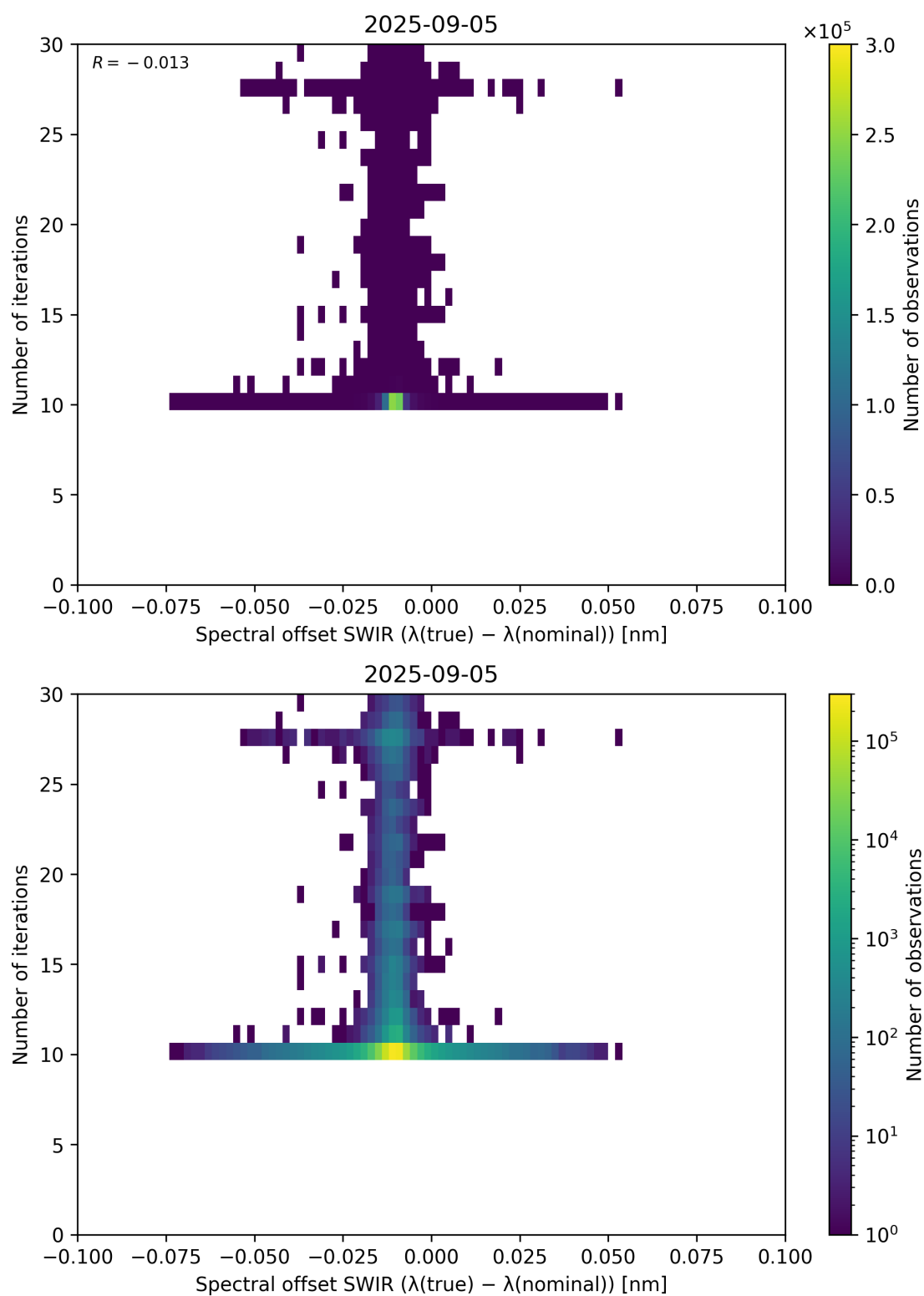
Figure 121: Scatter density plot of “Spectral offset SWIR ( \lambda_{\text{true}} - \lambda_{\text{nominal}} )” against “Number of iterations” for 2025-09-04 to 2025-09-06.
