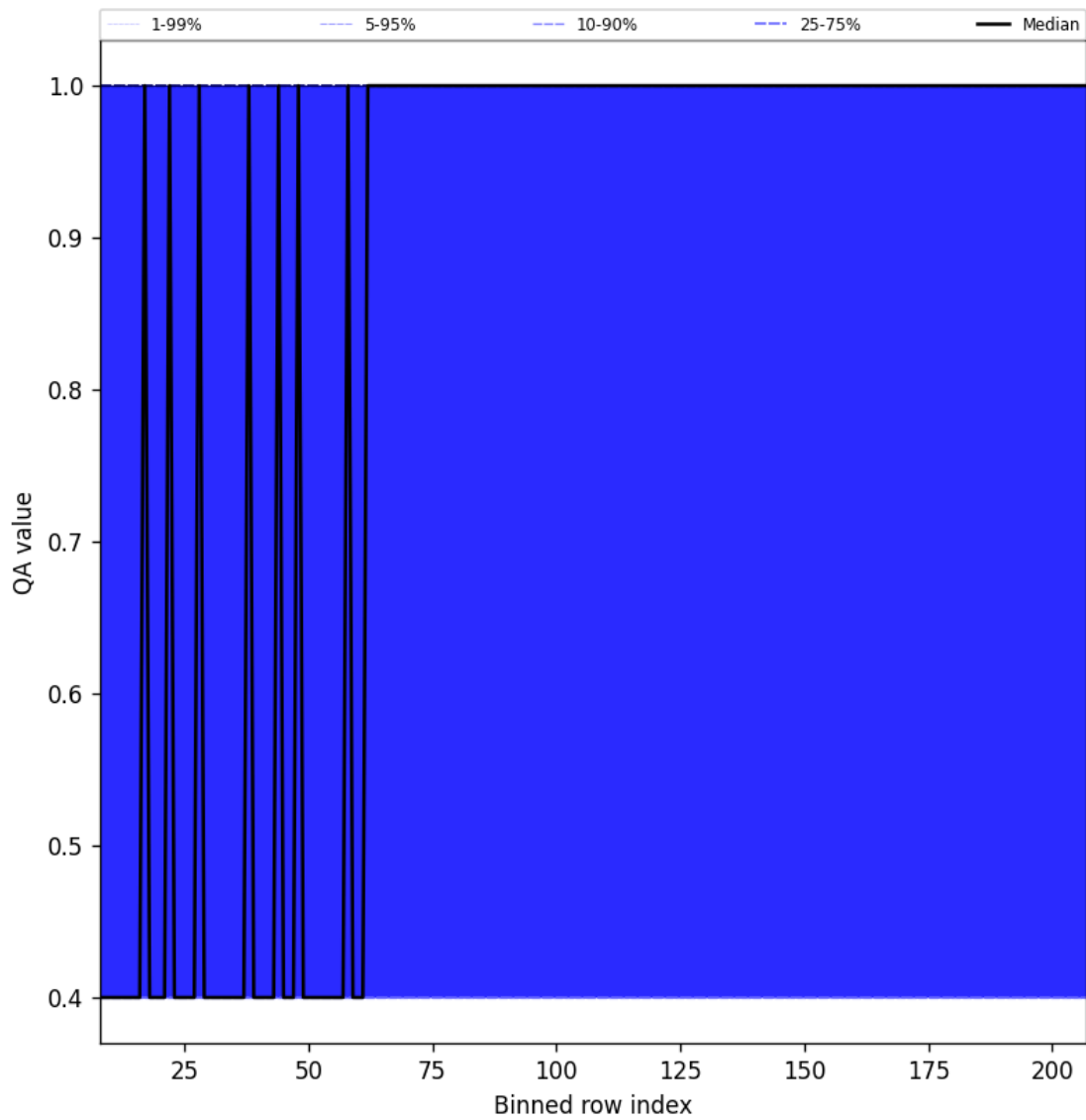
Figure 33: Along track statistics of “QA value” for 2025-09-04 to 2025-09-06
