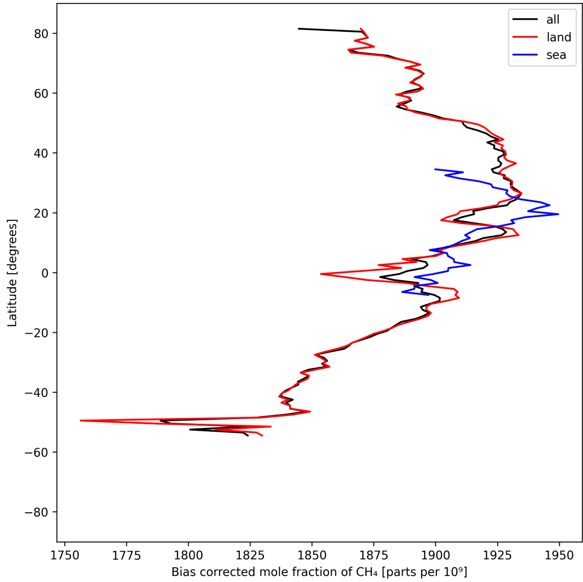
Figure 14: Zonal average of “Bias corrected mole fraction of \text{CH}_4 ” for 2025-09-04 to 2025-09-06.
