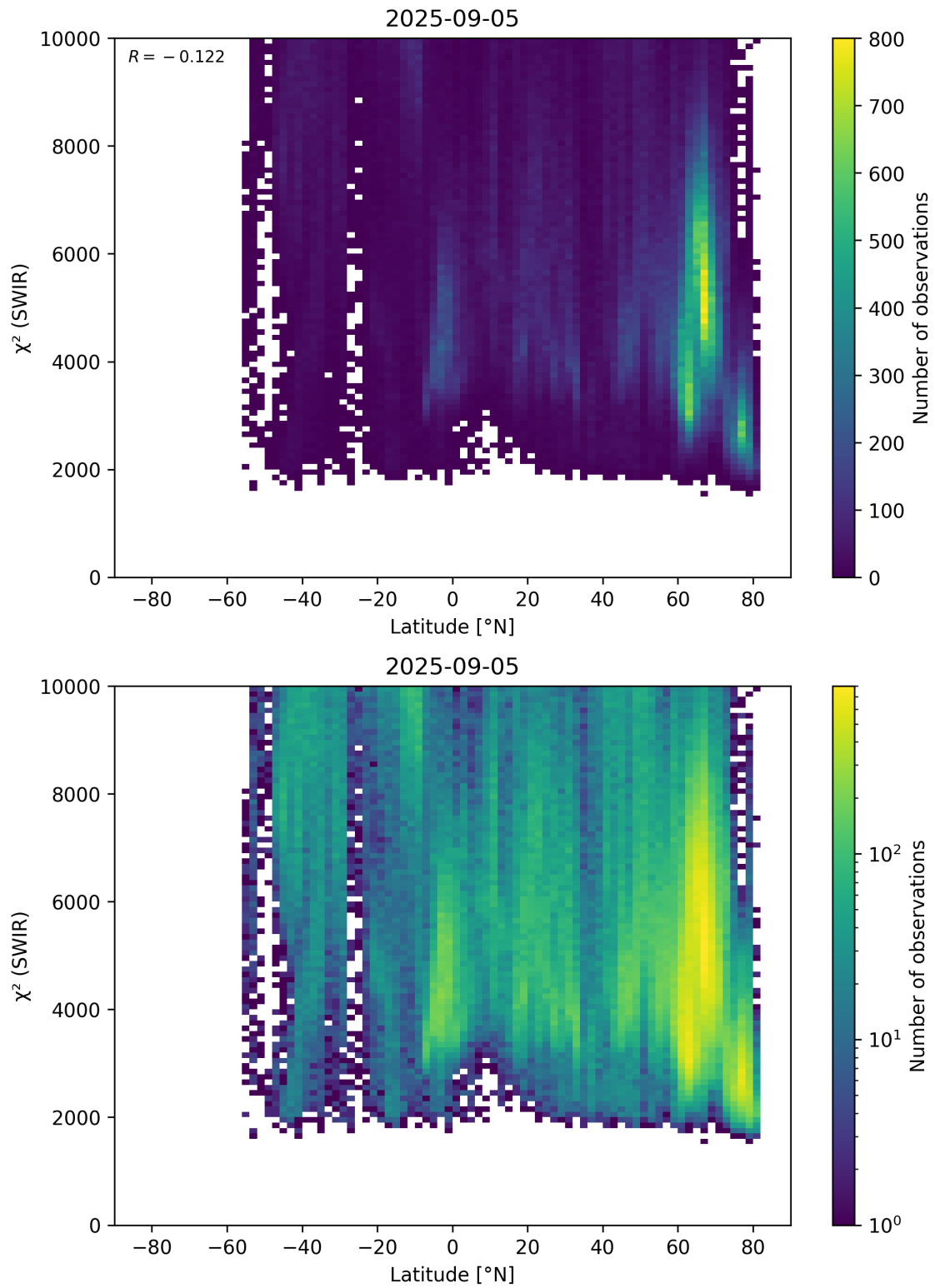
Figure 54: Scatter density plot of “Latitude” against “ \chi^2 (SWIR)” for 2025-09-04 to 2025-09-06.
