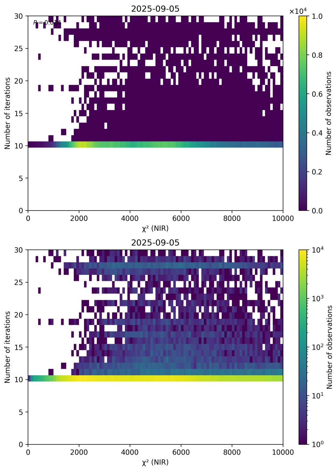
Figure 46: Scatter density plot of “ \chi^2 (NIR)” against “Number of iterations” for 2025-09-04 to 2025-09-06.
