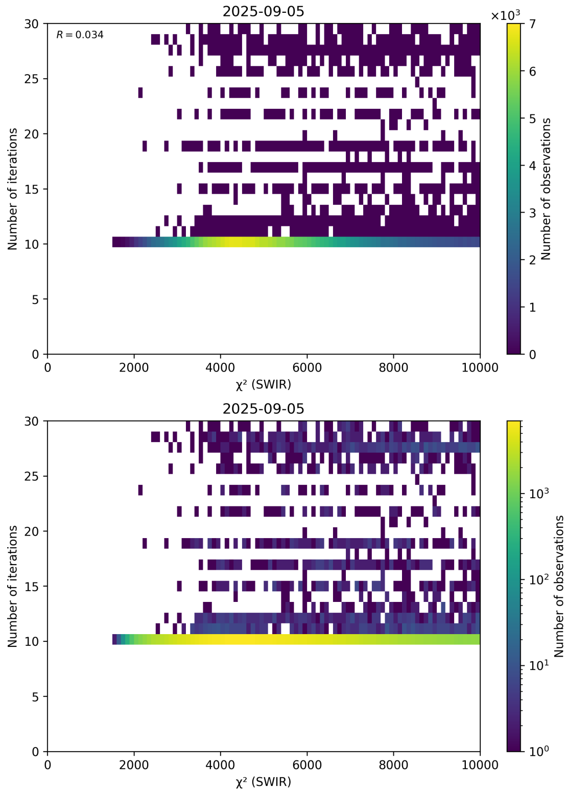
Figure 50: Scatter density plot of “ \chi^2 (SWIR)” against “Number of iterations” for 2025-09-04 to 2025-09-06.
