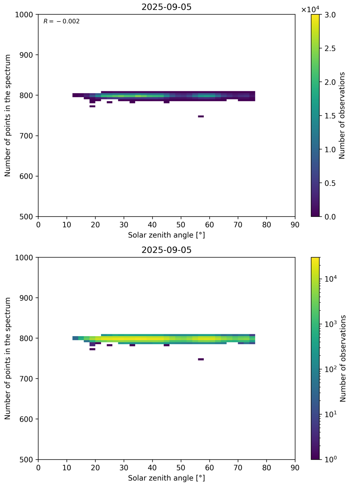
Figure 103: Scatter density plot of “Solar zenith angle” against “Number of points in the spectrum” for 2025-09-04 to 2025-09-06.
