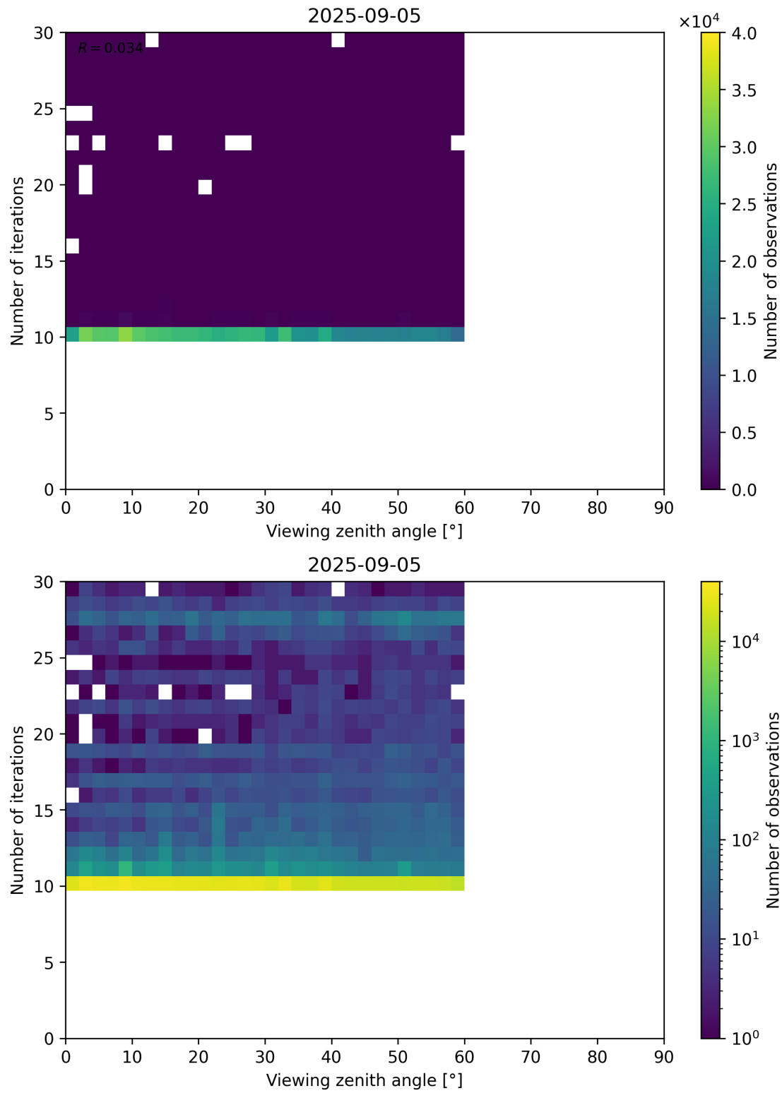
Figure 113: Scatter density plot of “Viewing zenith angle” against “Number of iterations” for 2025-09-04 to 2025-09-06.
