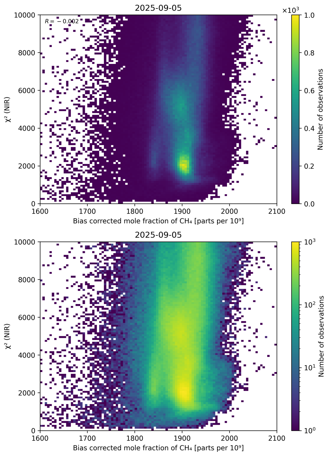
Figure 63: Scatter density plot of “Bias corrected mole fraction of \text{CH}_4 ” against “ \chi^2 (NIR)” for 2025-09-04 to 2025-09-06.
