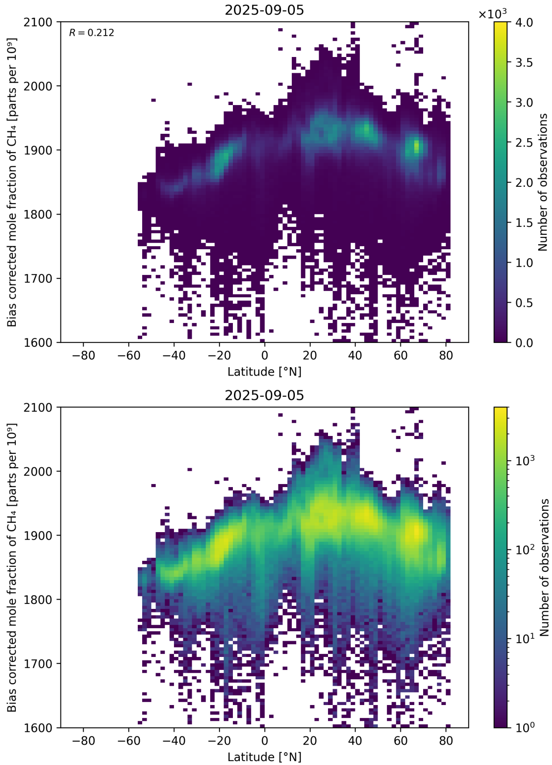
Figure 58: Scatter density plot of “Latitude” against “Bias corrected mole fraction of \text{CH}_4 ” for 2025-09-04 to 2025-09-06.
