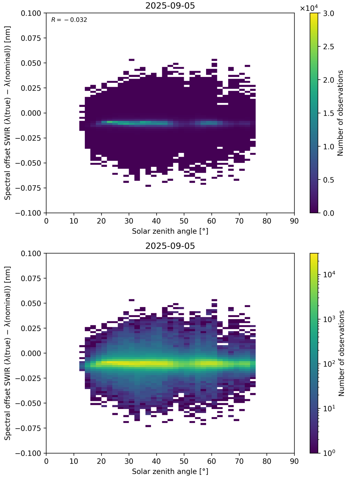
Figure 104: Scatter density plot of “Solar zenith angle” against “Spectral offset SWIR ( \lambda_{\text{true}} - \lambda_{\text{nominal}} )” for 2025-09-04 to 2025-09-06.
