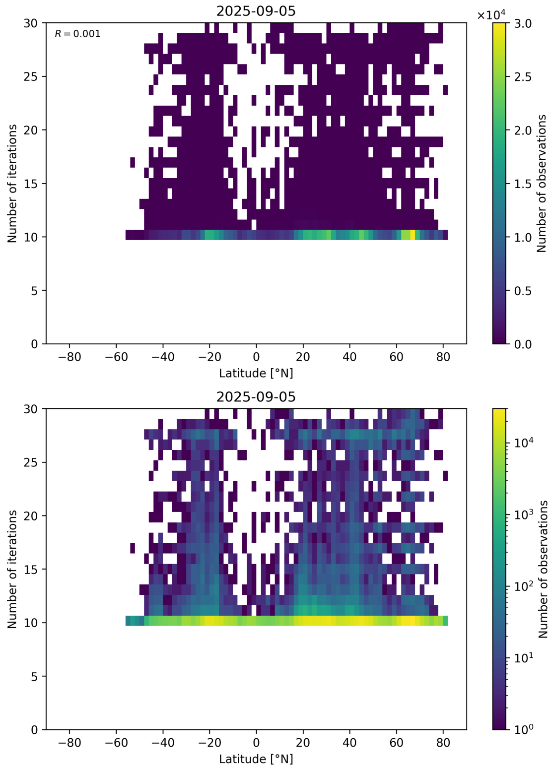
Figure 60: Scatter density plot of “Latitude” against “Number of iterations” for 2025-09-04 to 2025-09-06.
