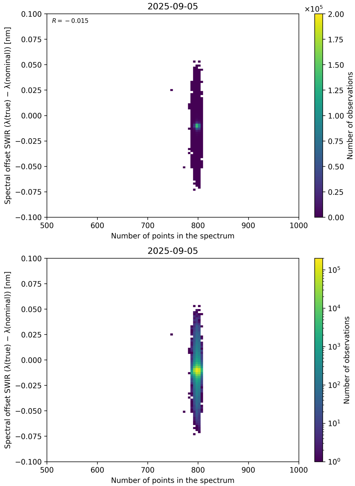
Figure 93: Scatter density plot of “Number of points in the spectrum” against “Spectral offset SWIR ( \lambda_{\text{true}} - \lambda_{\text{nominal}} )” for 2025-09-04 to 2025-09-06.
