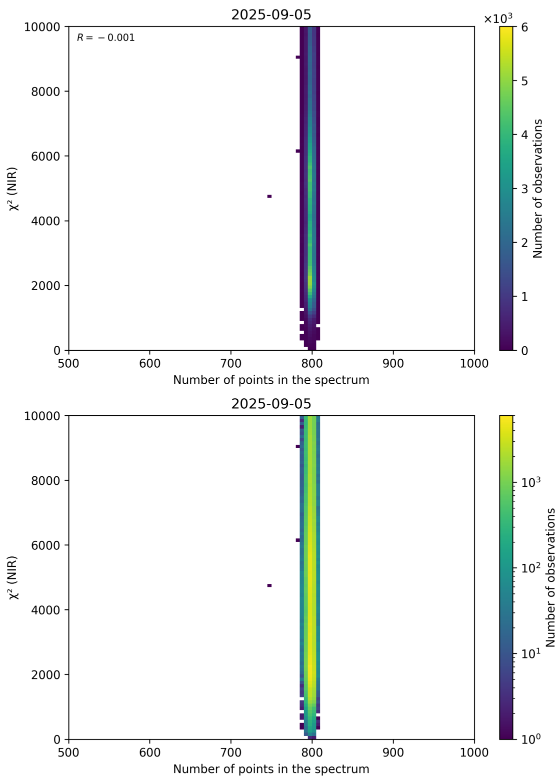
Figure 88: Scatter density plot of “Number of points in the spectrum” against “ \chi^2 (NIR)” for 2025-09-04 to 2025-09-06.
