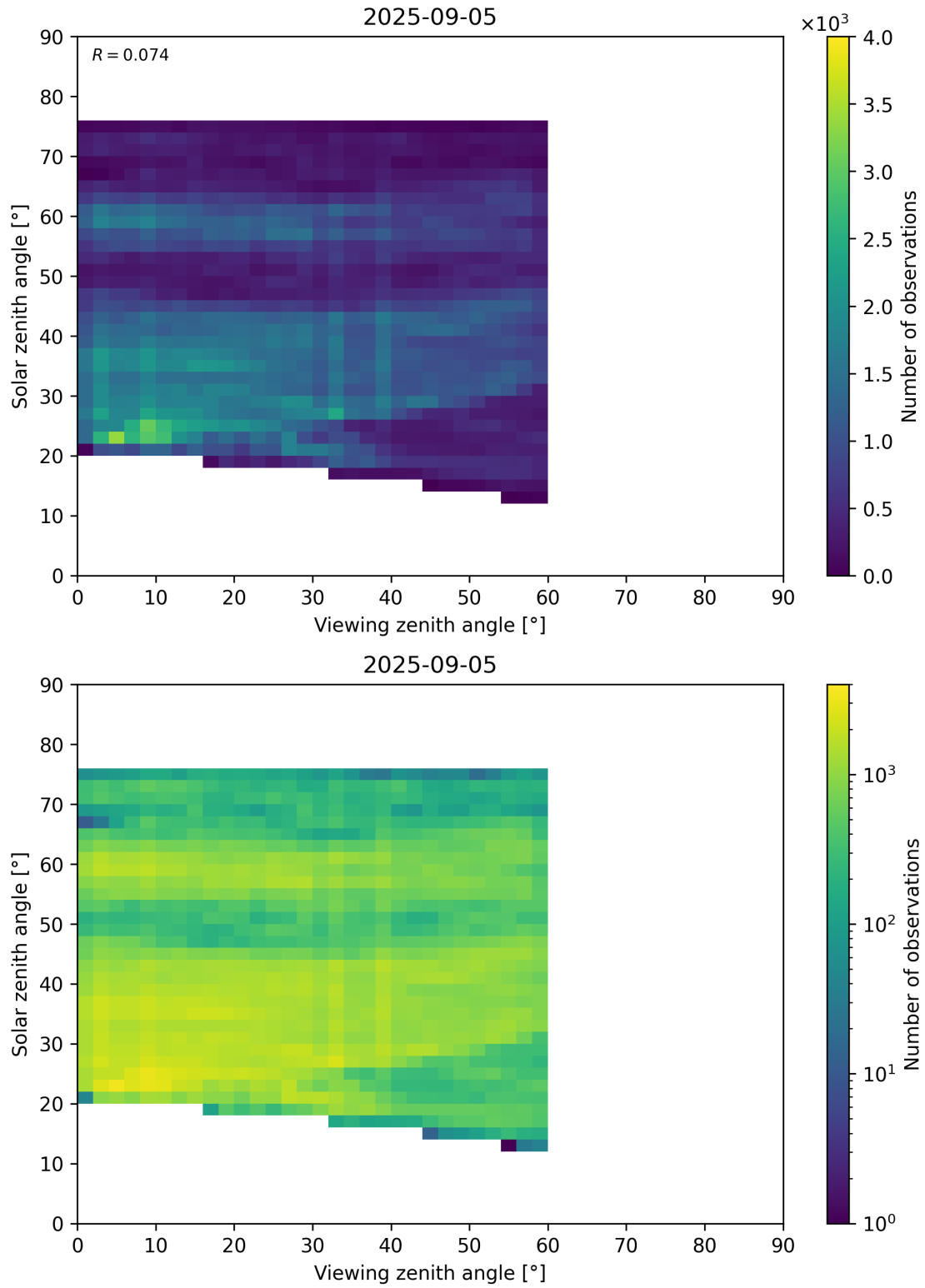
Figure 115: Scatter density plot of “Viewing zenith angle” against “Solar zenith angle” for 2025-09-04 to 2025-09-06.
