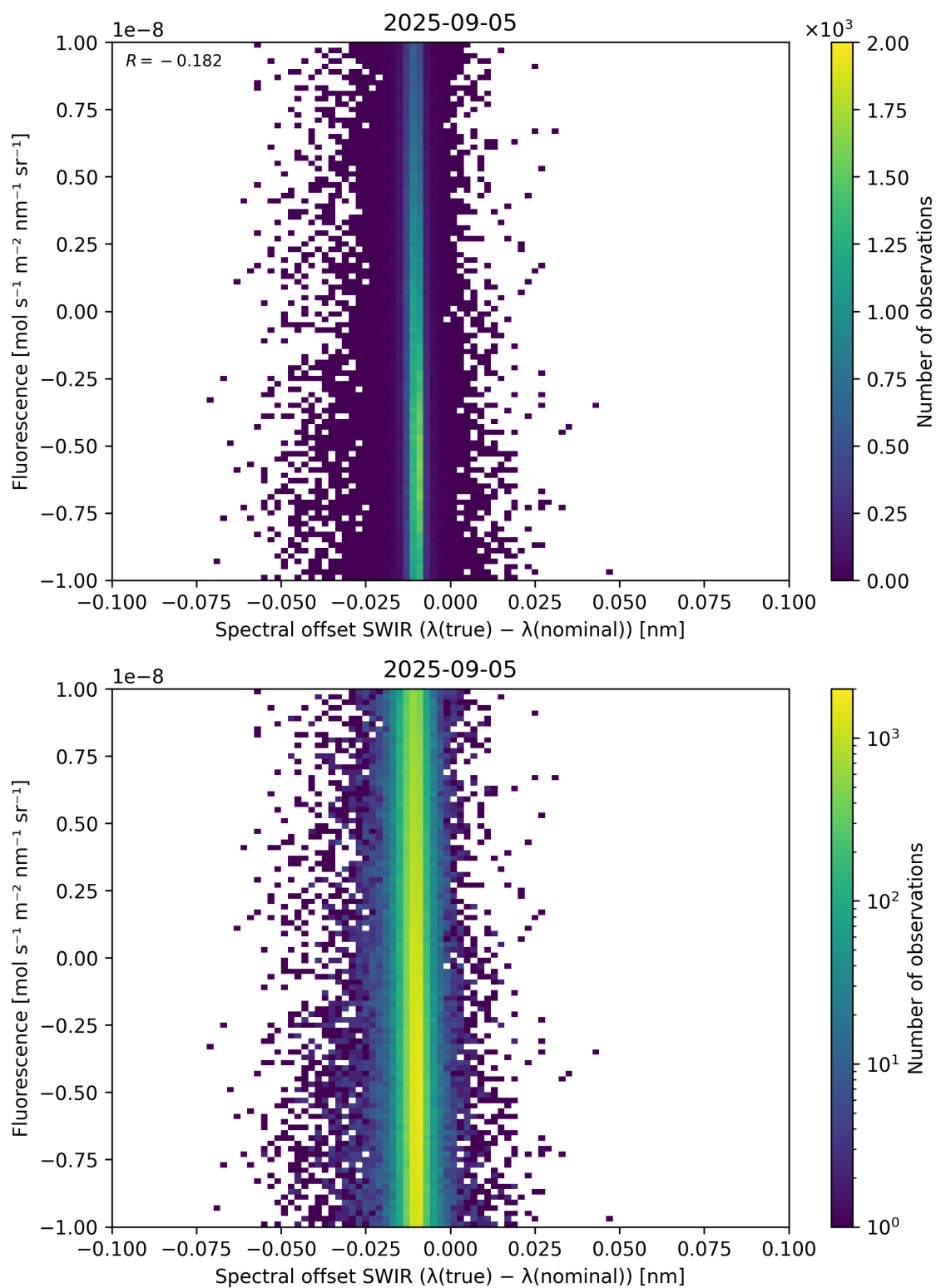
Figure 120: Scatter density plot of “Spectral offset SWIR ( \lambda_{\text{true}} - \lambda_{\text{nominal}} )” against “Fluorescence” for 2025-09-04 to 2025-09-06.
