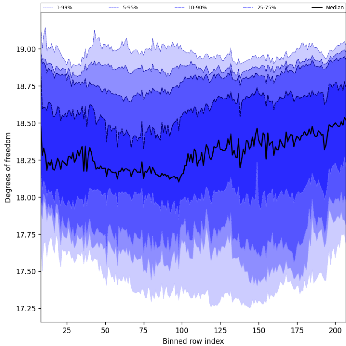
Figure 41: Along track statistics of “Degrees of freedom” for 2025-09-04 to 2025-09-06
