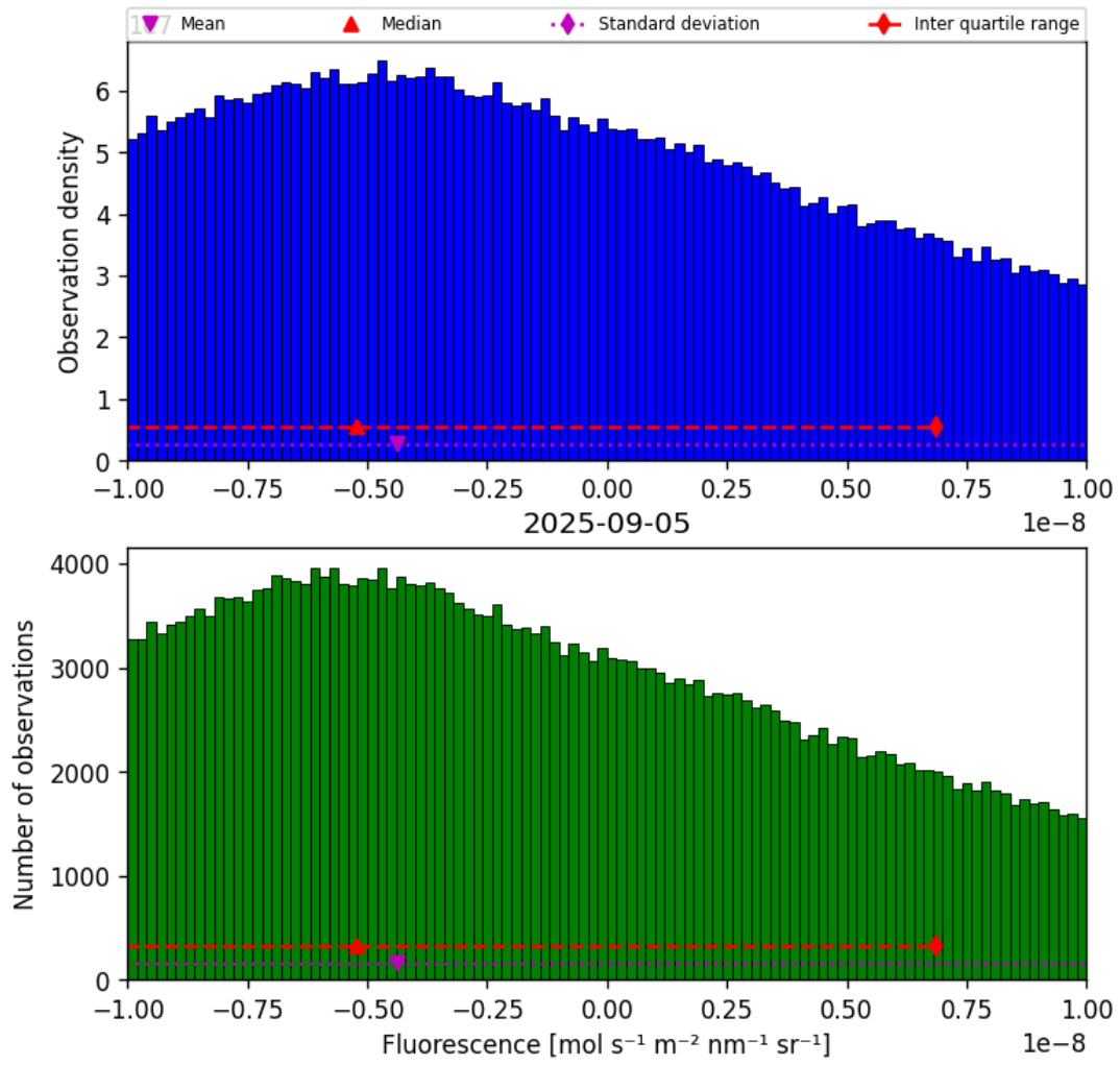
Figure 32: Histogram of “Fluorescence” for 2025-09-04 to 2025-09-06
