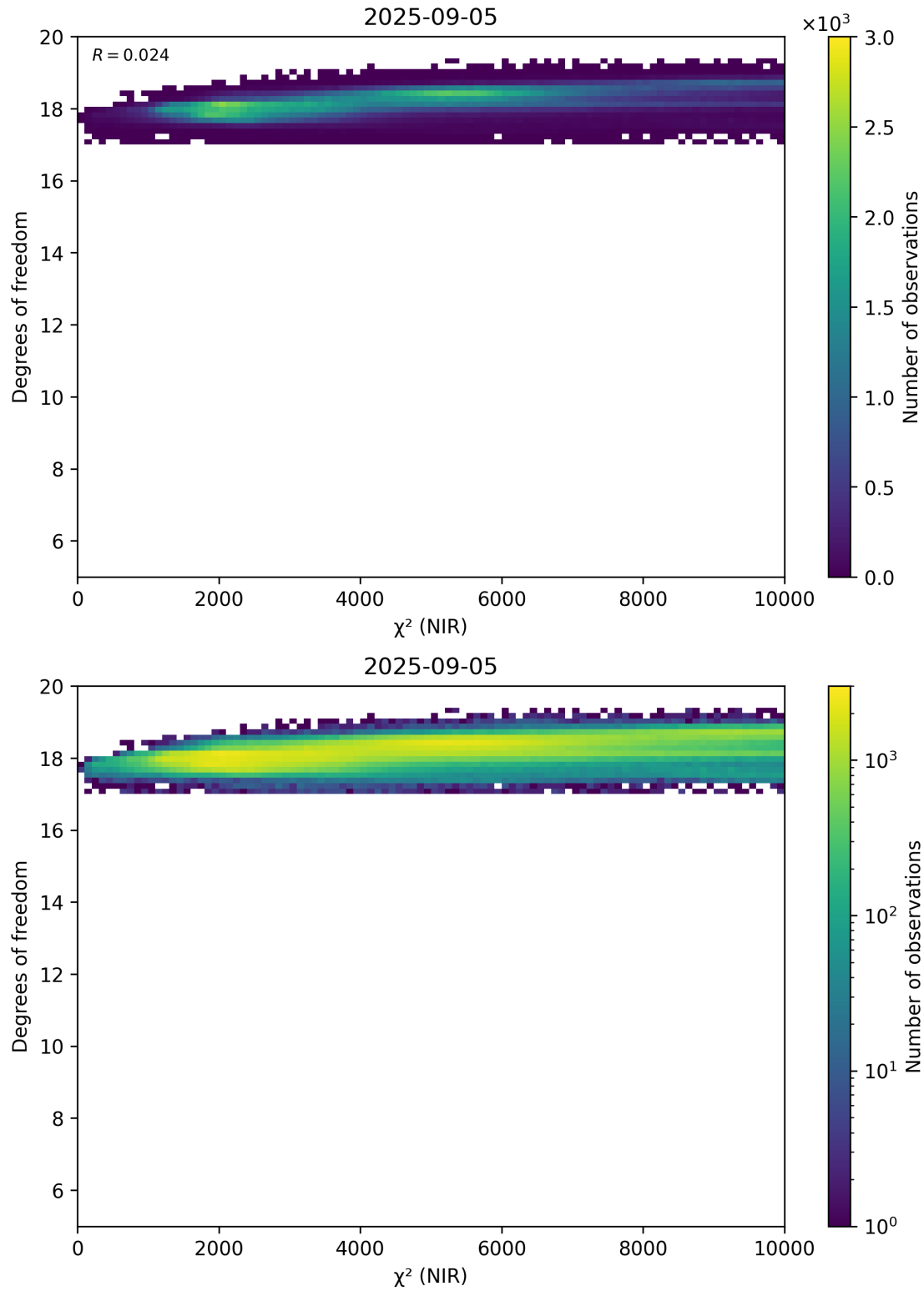
Figure 44: Scatter density plot of “ \chi^2 (NIR)” against “Degrees of freedom” for 2025-09-04 to 2025-09-06.
