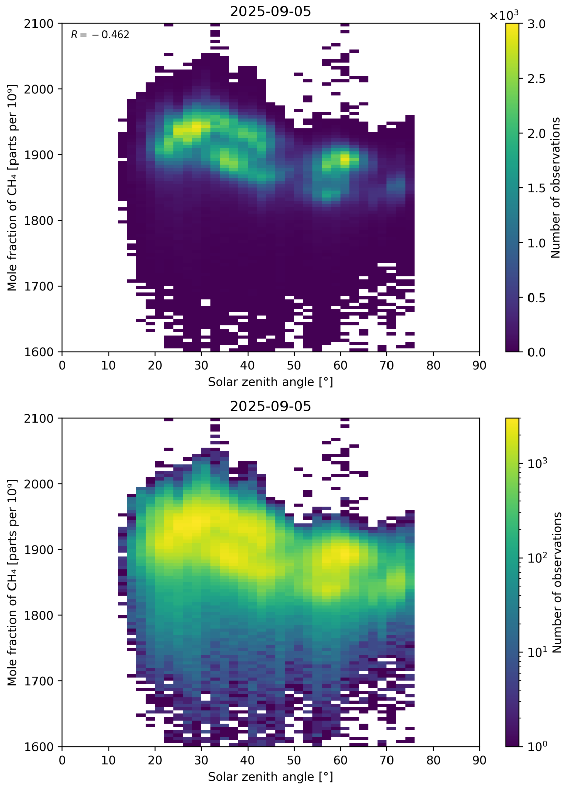
Figure 99: Scatter density plot of “Solar zenith angle” against “Mole fraction of CH 4 ” for 2025-09-04 to 2025-09-06.
