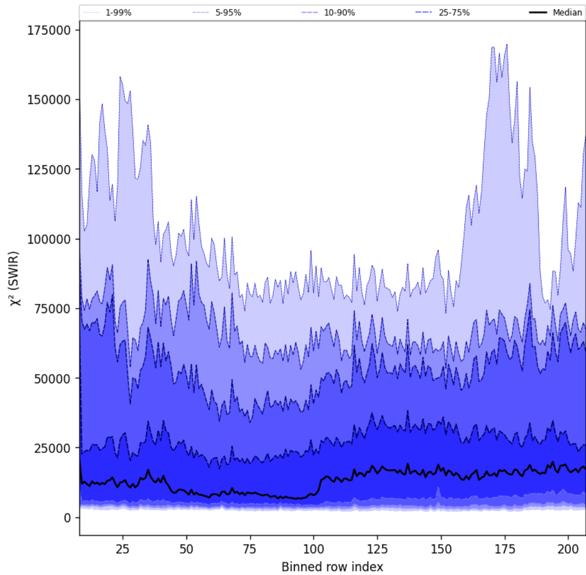
Figure 39: Along track statistics of " \chi^2 (SWIR)" for 2025-09-04 to 2025-09-06
