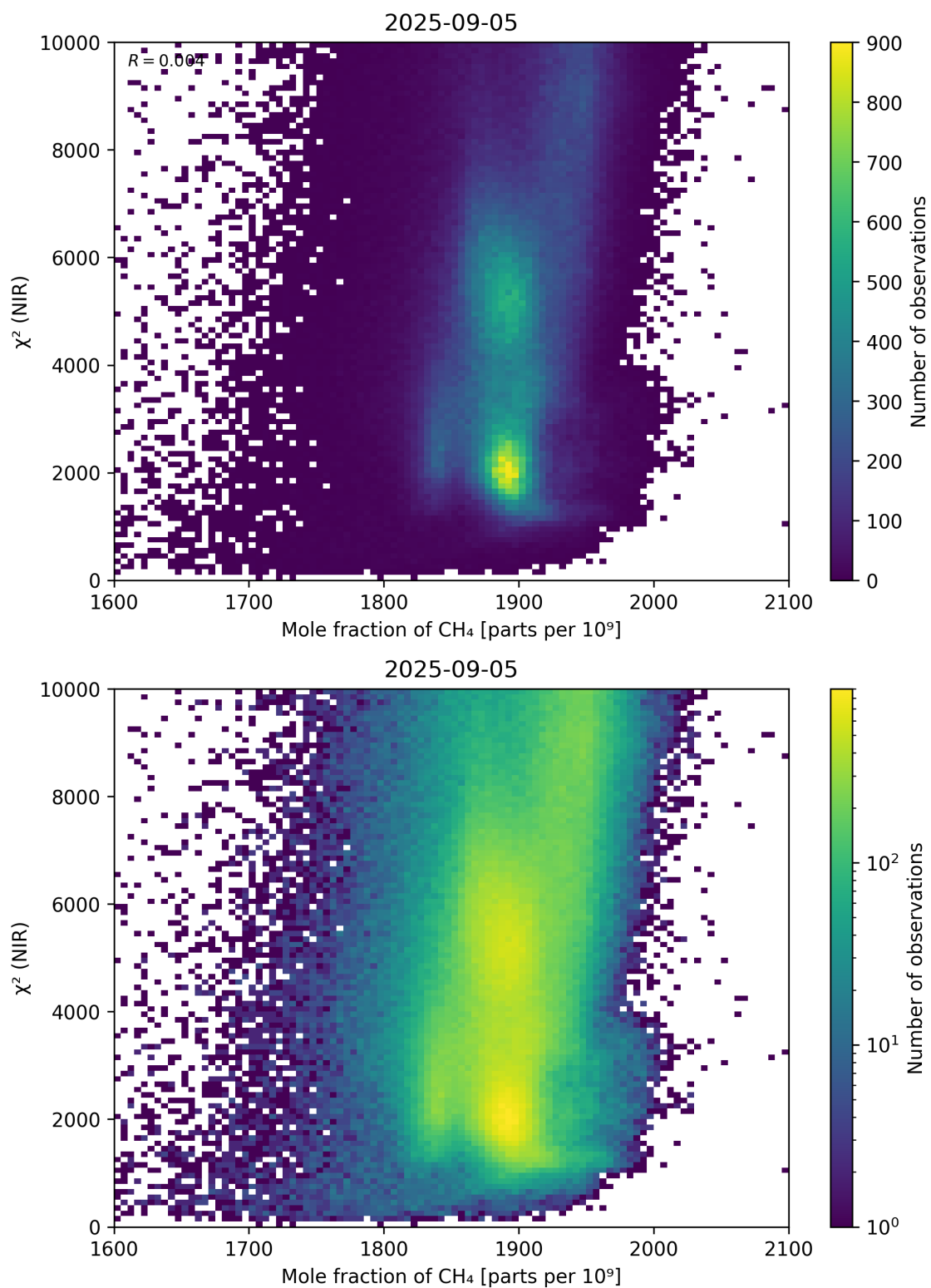
Figure 70: Scatter density plot of “Mole fraction of \text{CH}_4 ” against “ \chi^2 (NIR)” for 2025-09-04 to 2025-09-06.
