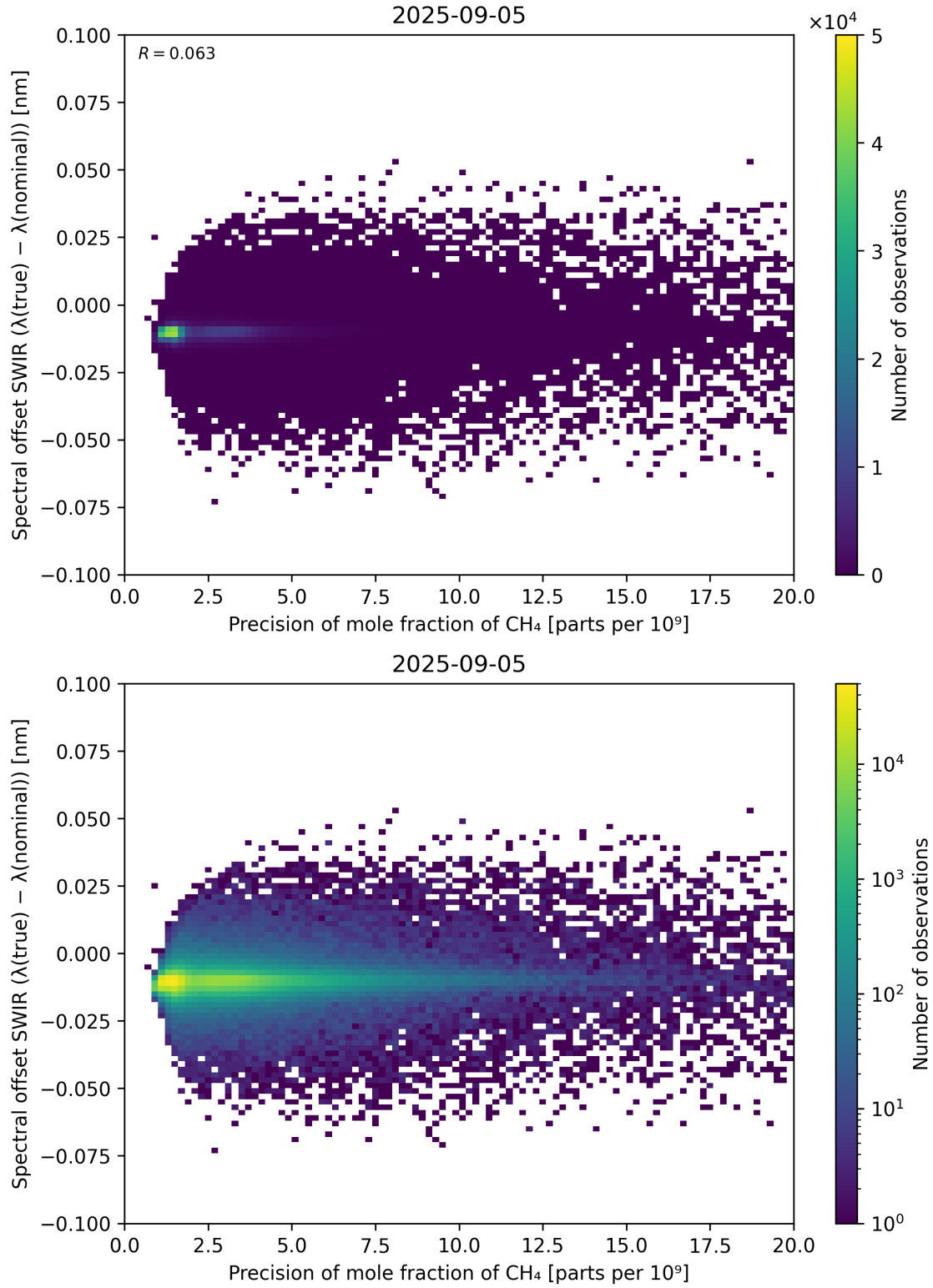
Figure 85: Scatter density plot of “Precision of mole fraction of \text{CH}_4 ” against “Spectral offset SWIR ( \lambda_{\text{true}} - \lambda_{\text{nominal}} )” for 2025-09-04 to 2025-09-06.
