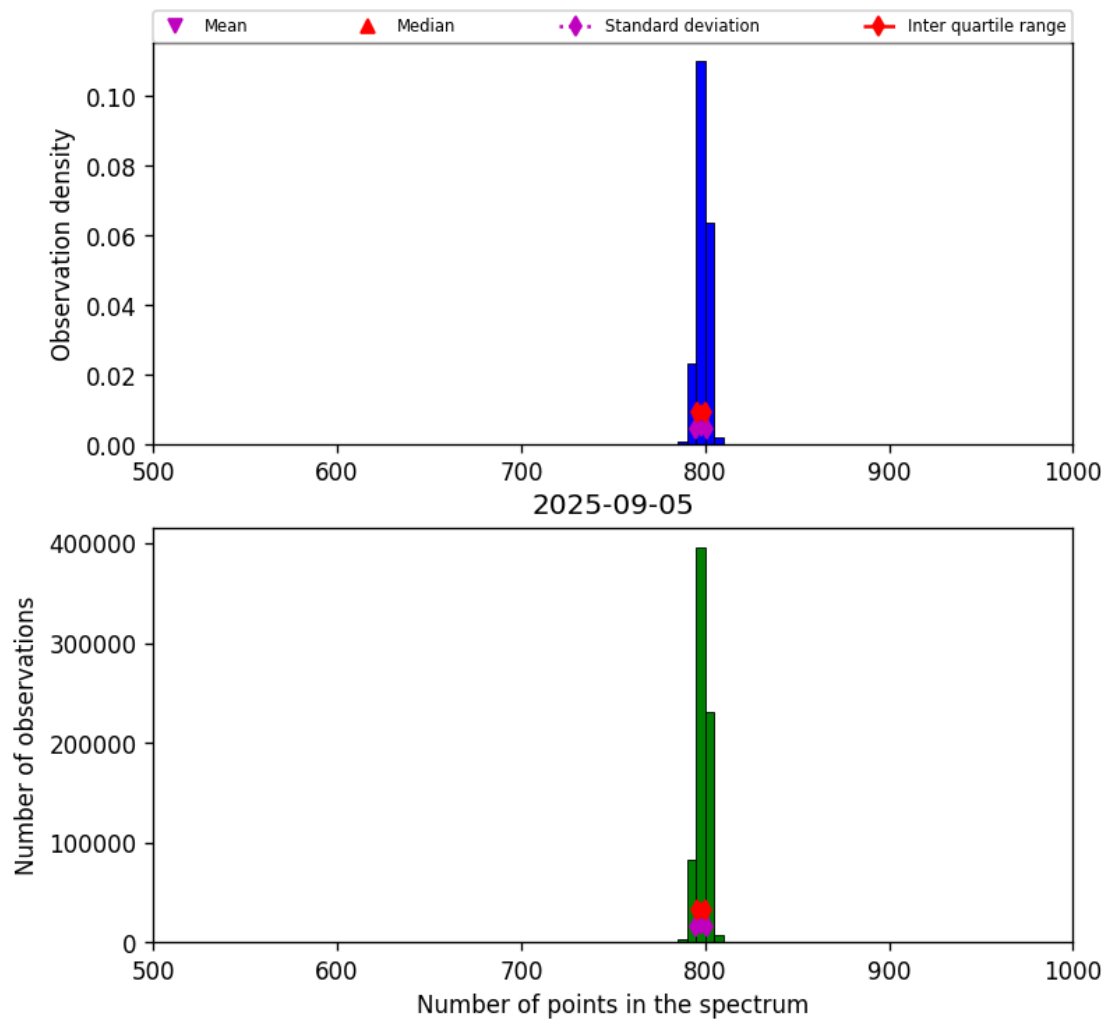
Figure 26: Histogram of “Number of points in the spectrum” for 2025-09-04 to 2025-09-06
