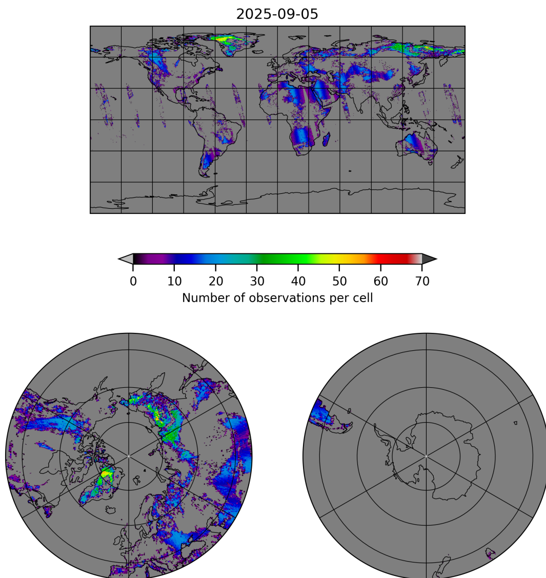
Figure 10: Map of the number of observations for 2025-09-04 to 2025-09-06
