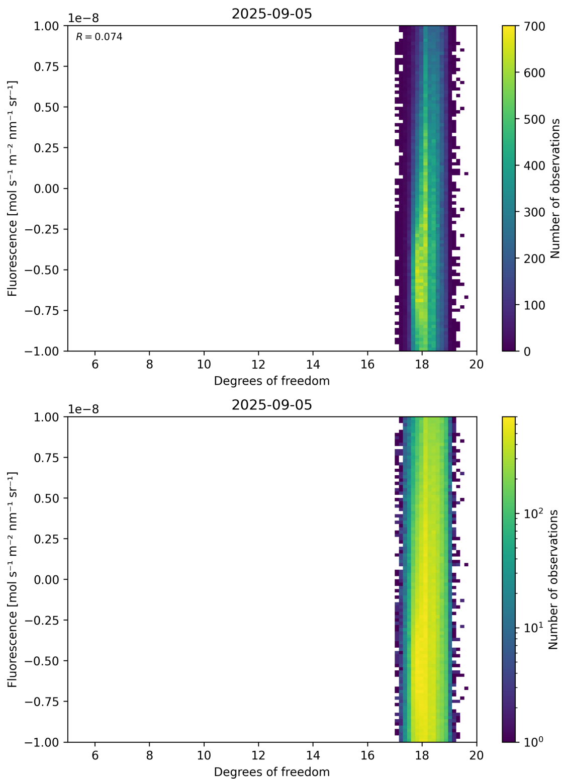
Figure 51: Scatter density plot of “Degrees of freedom” against “Fluorescence” for 2025-09-04 to 2025-09-06.
