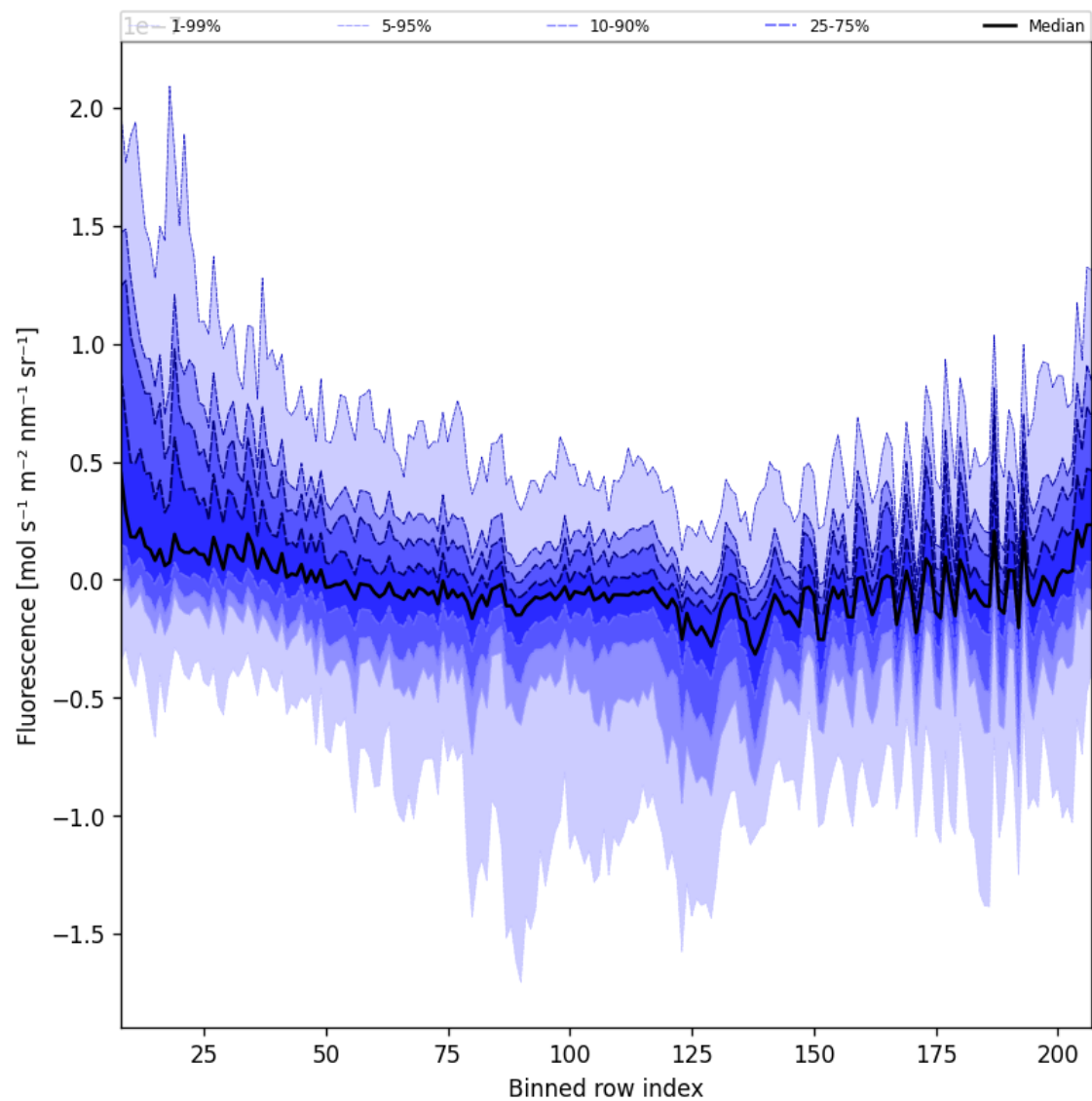
Figure 43: Along track statistics of “Fluorescence” for 2025-09-04 to 2025-09-06
