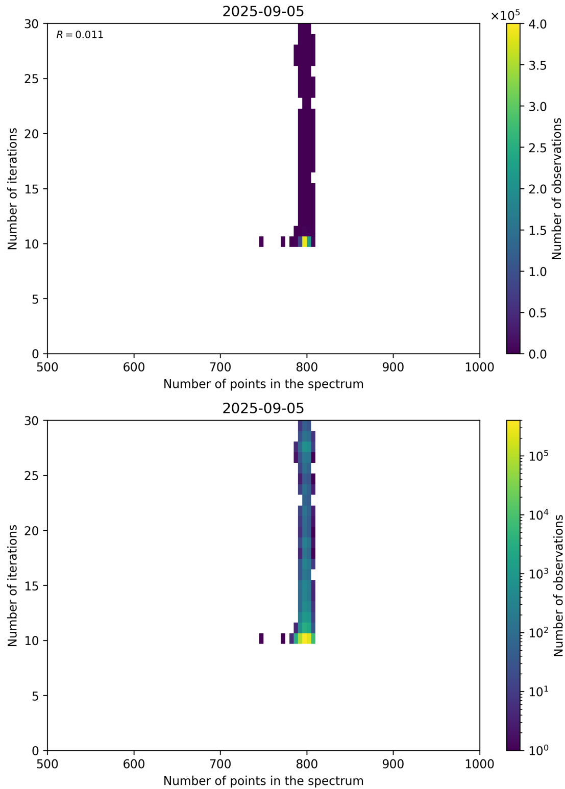
Figure 92: Scatter density plot of “Number of points in the spectrum” against “Number of iterations” for 2025-09-04 to 2025-09-06.
