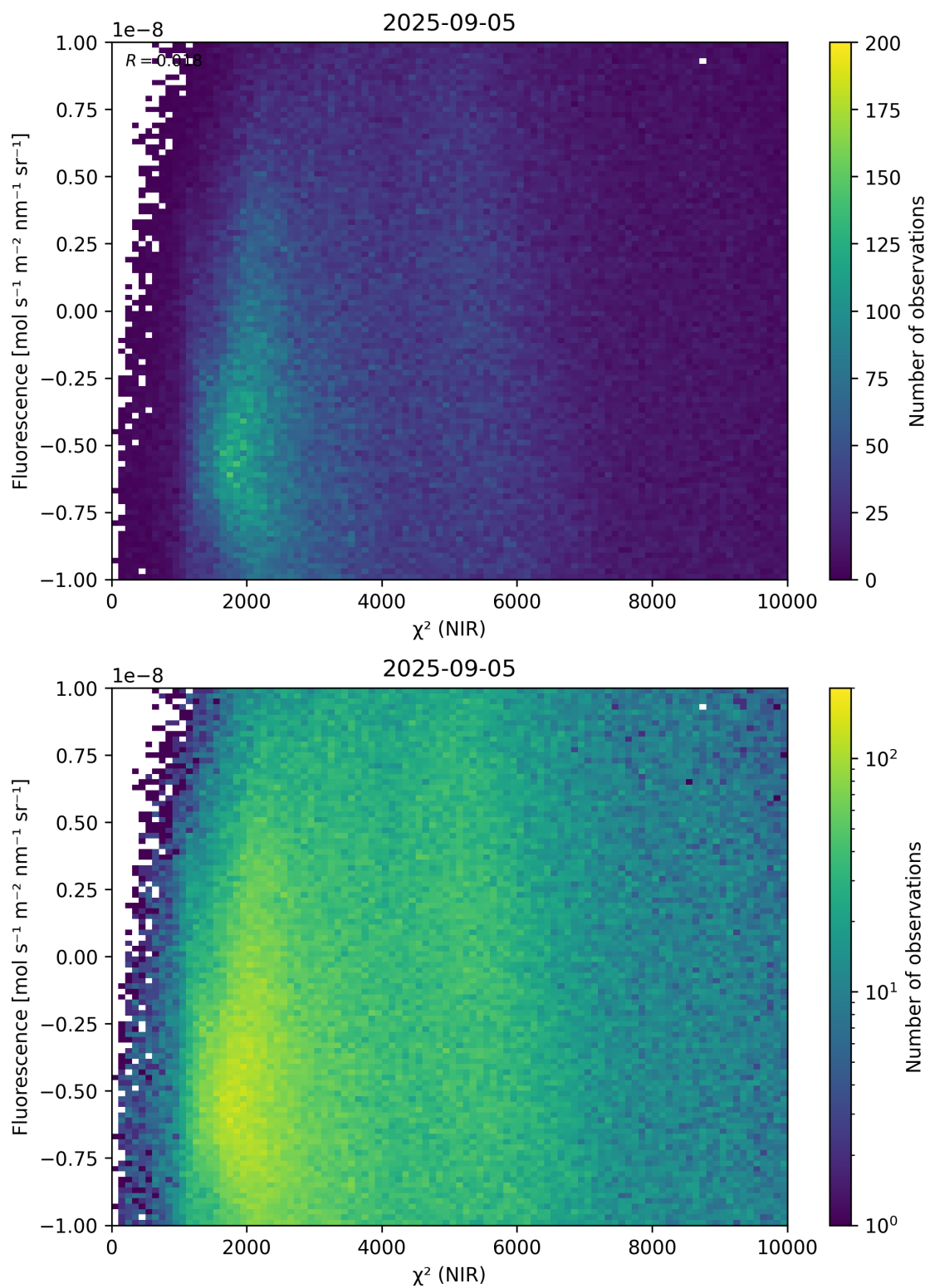
Figure 45: Scatter density plot of “ \chi^2 (NIR)” against “Fluorescence” for 2025-09-04 to 2025-09-06.
