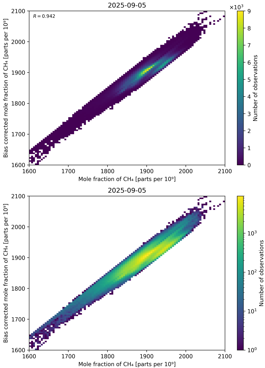
Figure 74: Scatter density plot of “Mole fraction of CH 4 ” against “Bias corrected mole fraction of CH 4 ” for 2025-09-04 to 2025-09-06.
