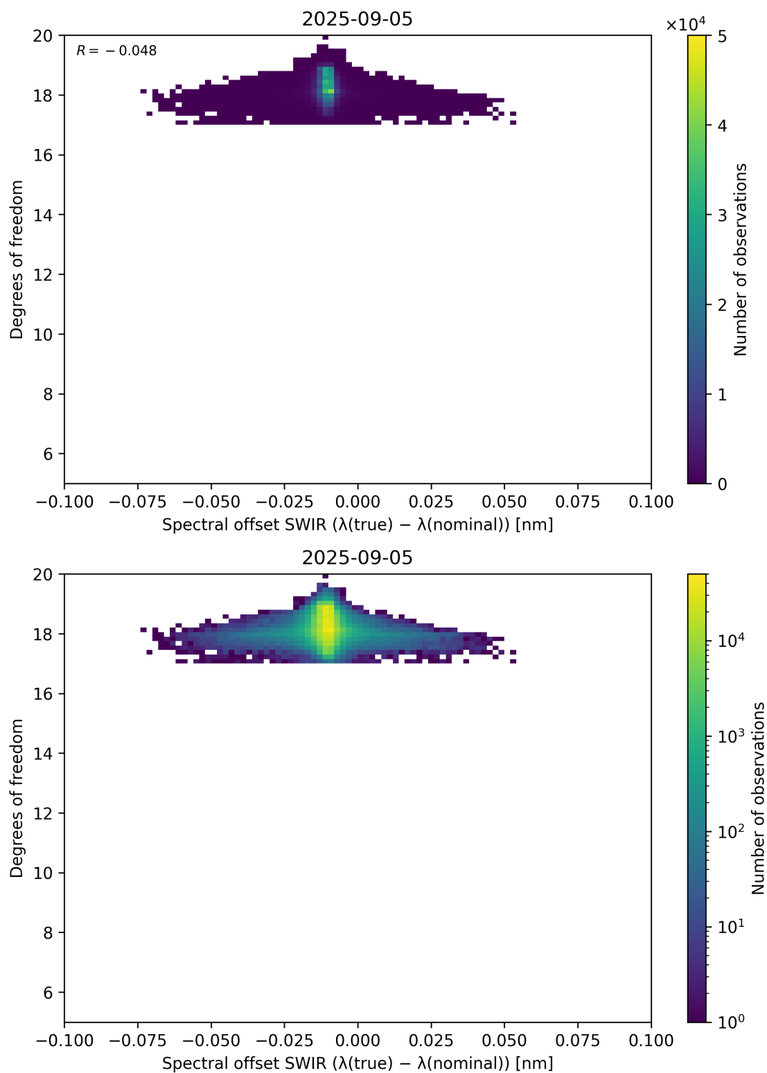
Figure 119: Scatter density plot of “Spectral offset SWIR ( \lambda_{\text{true}} - \lambda_{\text{nominal}} )” against “Degrees of freedom” for 2025-09-04 to 2025-09-06.
