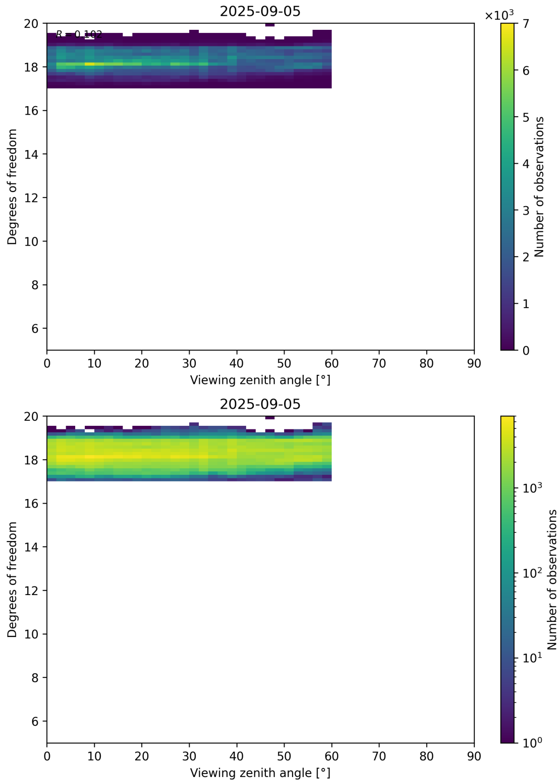
Figure 107: Scatter density plot of “Viewing zenith angle” against “Degrees of freedom” for 2025-09-04 to 2025-09-06.
