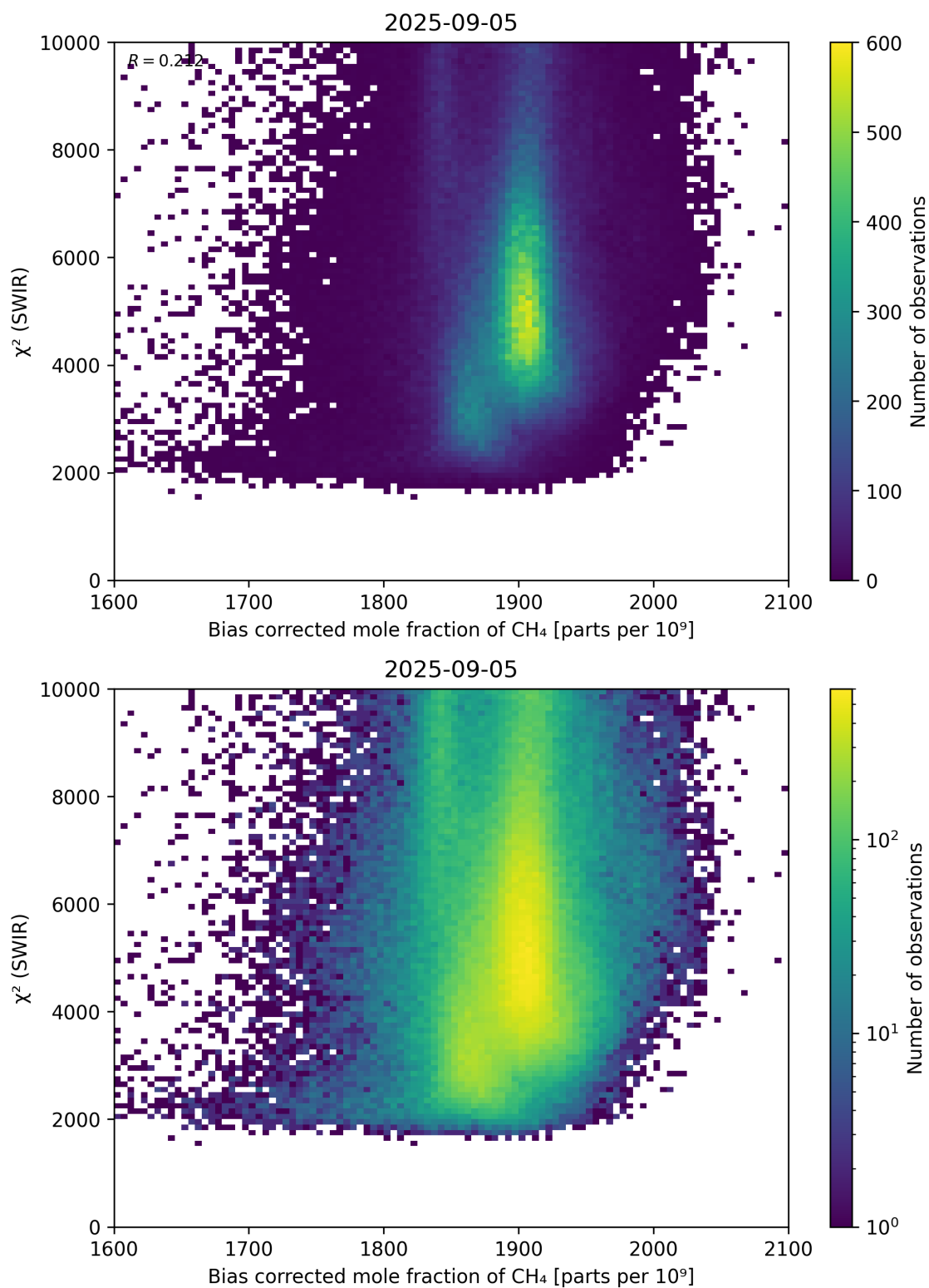
Figure 64: Scatter density plot of “Bias corrected mole fraction of \text{CH}_4 ” against “ \chi^2 (SWIR)” for 2025-09-04 to 2025-09-06.
