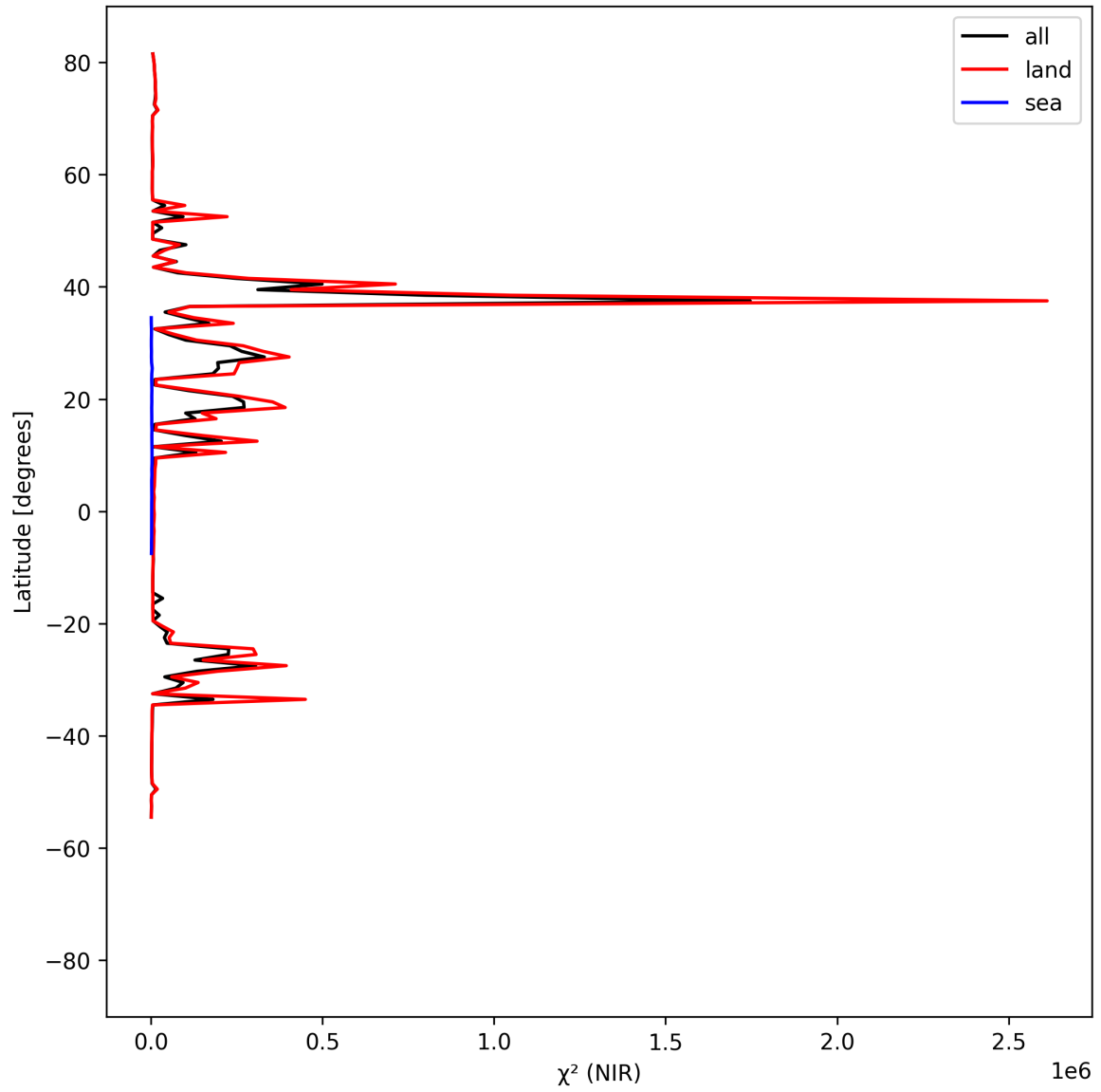
Figure 18: Zonal average of “ \chi^2 (NIR)” for 2025-09-04 to 2025-09-06.
