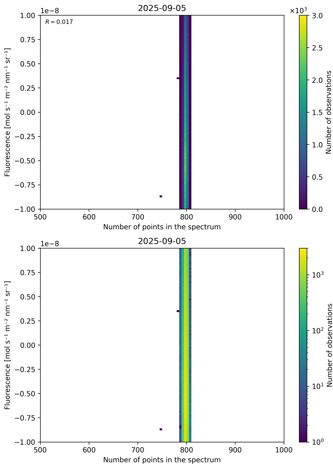
Figure 91: Scatter density plot of “Number of points in the spectrum” against “Fluorescence” for 2025-09-04 to 2025-09-06.
