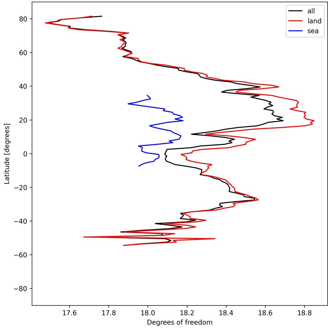
Figure 19: Zonal average of “Degrees of freedom” for 2025-09-04 to 2025-09-06.
