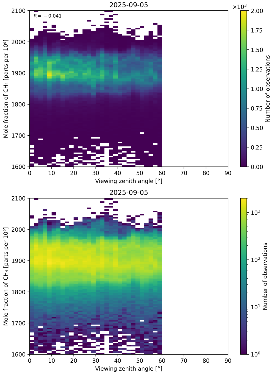
Figure 110: Scatter density plot of “Viewing zenith angle” against “Mole fraction of CH 4 ” for 2025-09-04 to 2025-09-06.
