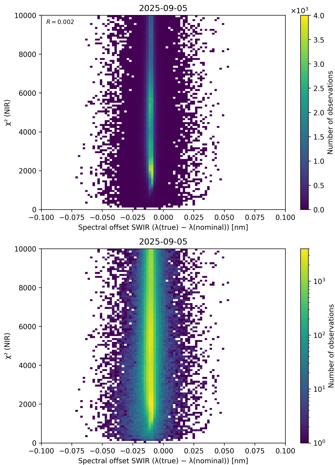
Figure 117: Scatter density plot of “Spectral offset SWIR ( \lambda_{\text{true}} - \lambda_{\text{nominal}} )” against “ \chi^2 (NIR)” for 2025-09-04 to 2025-09-06.
