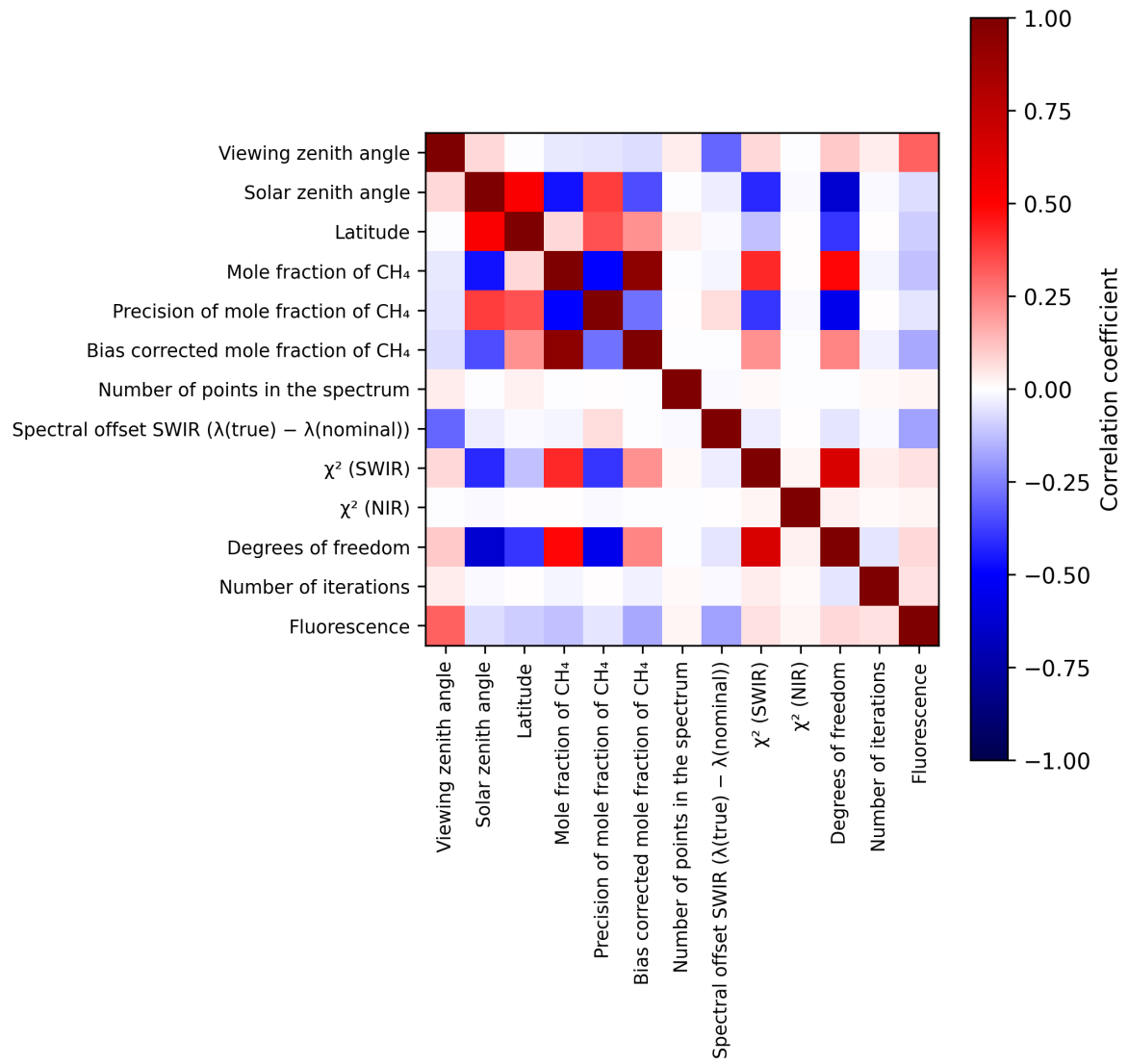
Figure 2: Map of correlation matrix for 2025-09-04 to 2025-09-06.
