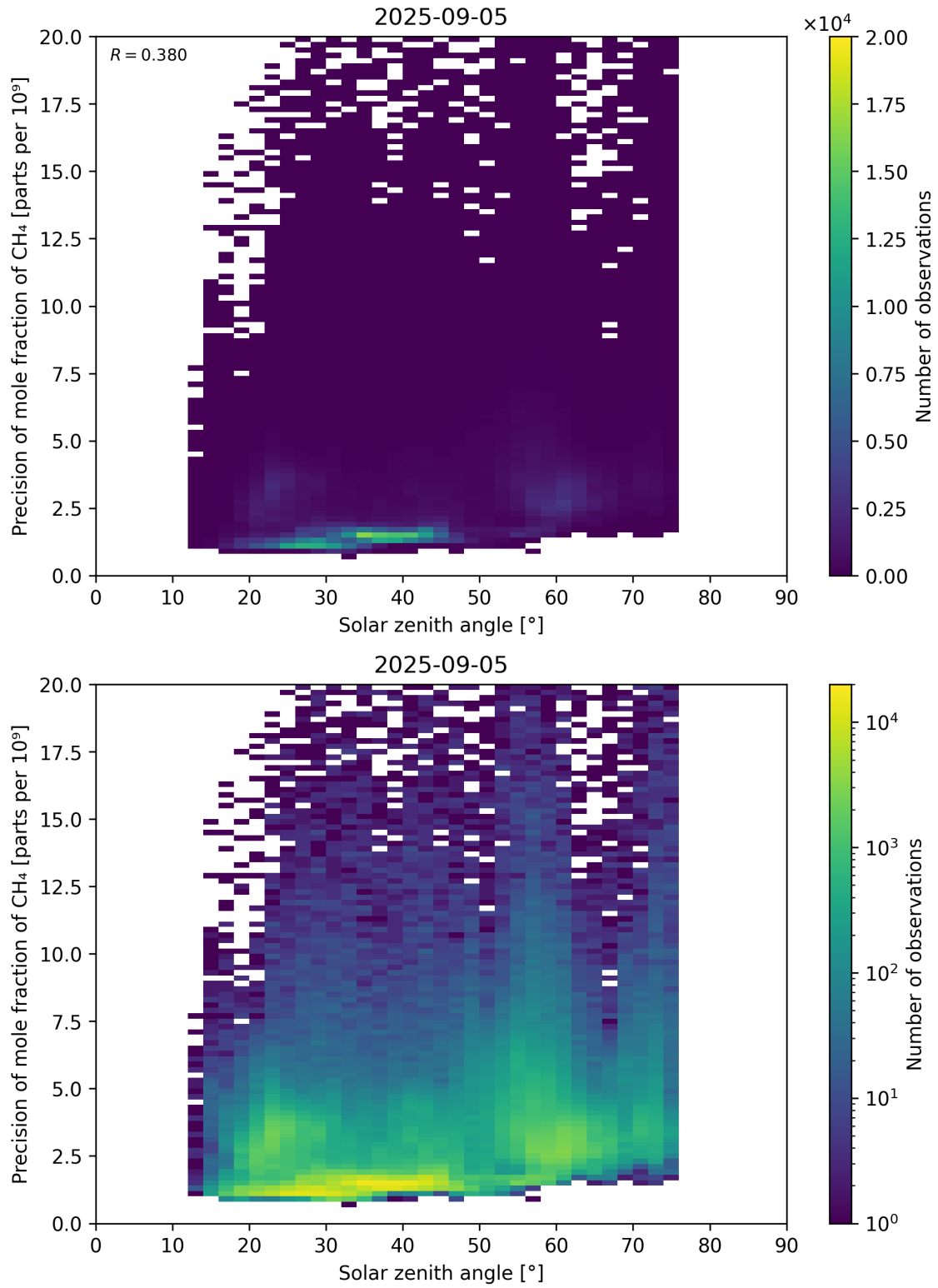
Figure 101: Scatter density plot of “Solar zenith angle” against “Precision of mole fraction of CH 4 ” for 2025-09-04 to 2025-09-06.
