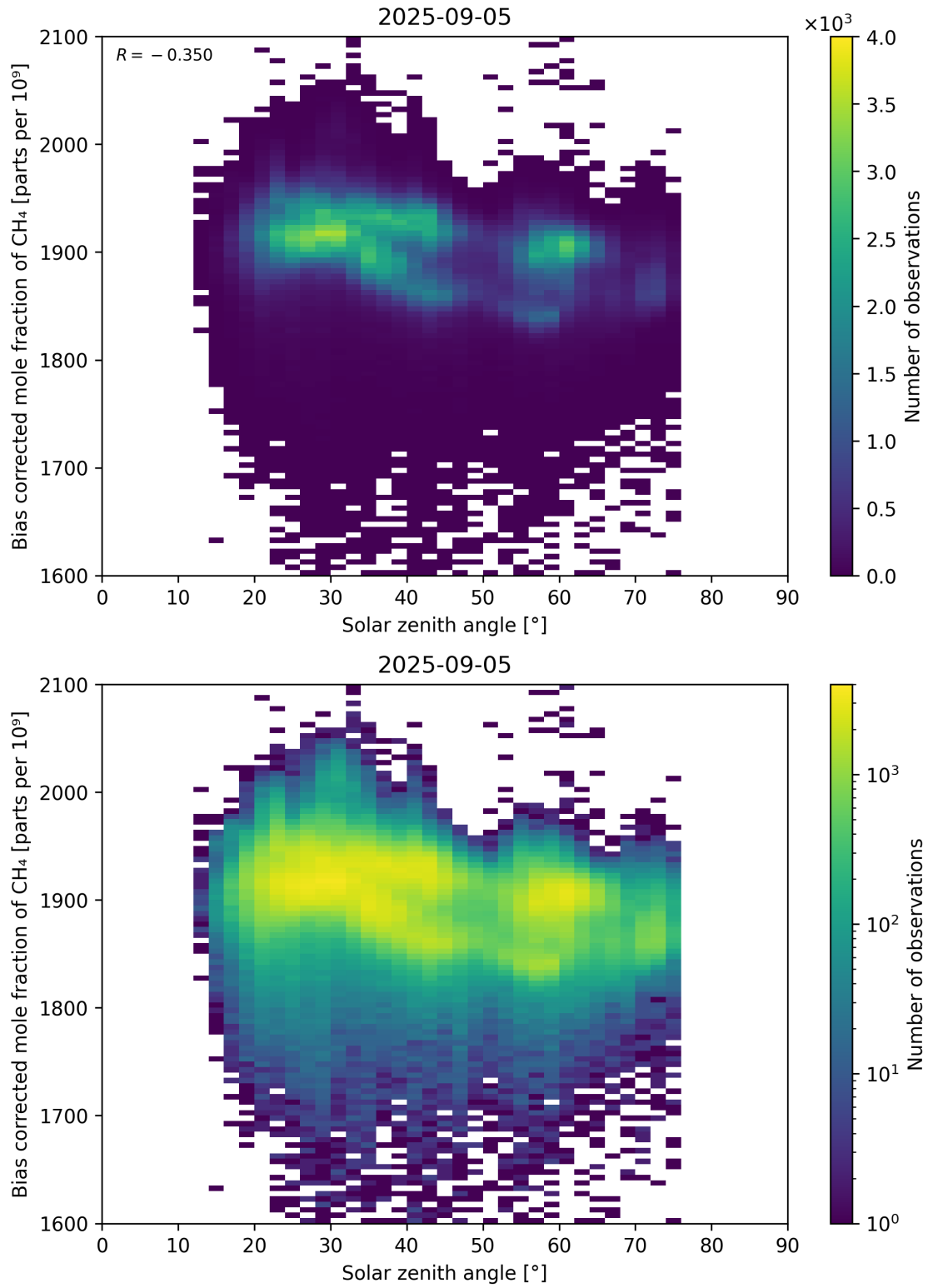
Figure 100: Scatter density plot of “Solar zenith angle” against “Bias corrected mole fraction of CH 4 ” for 2025-09-04 to 2025-09-06.
