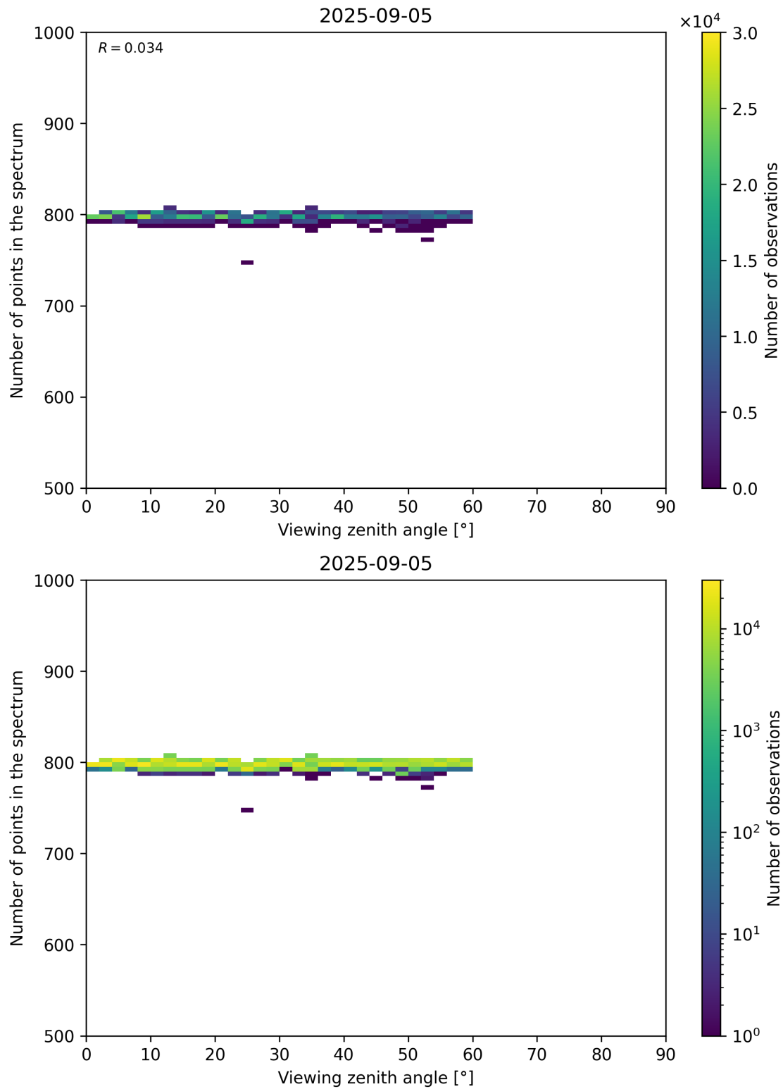
Figure 114: Scatter density plot of “Viewing zenith angle” against “Number of points in the spectrum” for 2025-09-04 to 2025-09-06.
