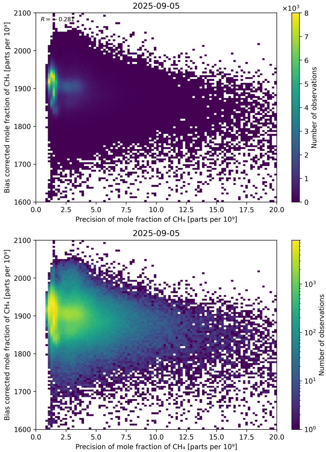
Figure 82: Scatter density plot of “Precision of mole fraction of CH 4 ” against “Bias corrected mole fraction of CH 4 ” for 2025-09-04 to 2025-09-06.
