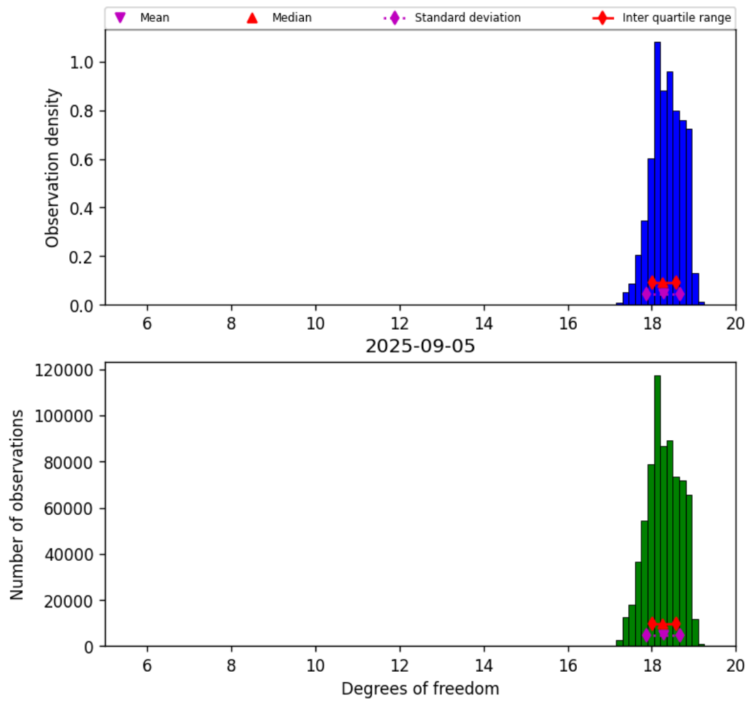
Figure 30: Histogram of “Degrees of freedom” for 2025-09-04 to 2025-09-06
