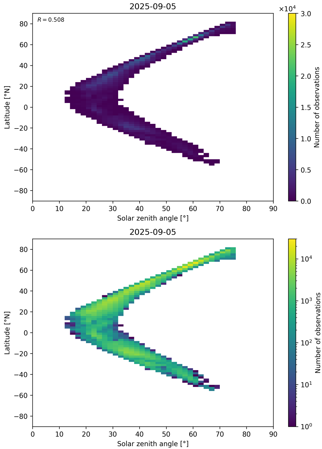
Figure 98: Scatter density plot of “Solar zenith angle” against “Latitude” for 2025-09-04 to 2025-09-06.
