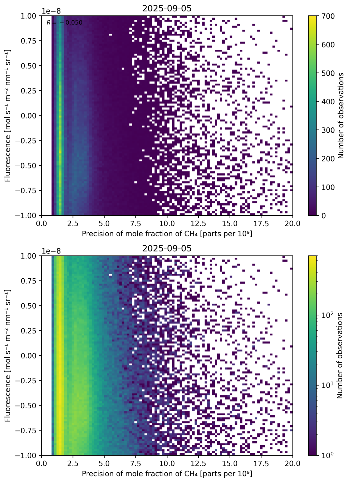
Figure 81: Scatter density plot of “Precision of mole fraction of \text{CH}_4 ” against “Fluorescence” for 2025-09-04 to 2025-09-06.
