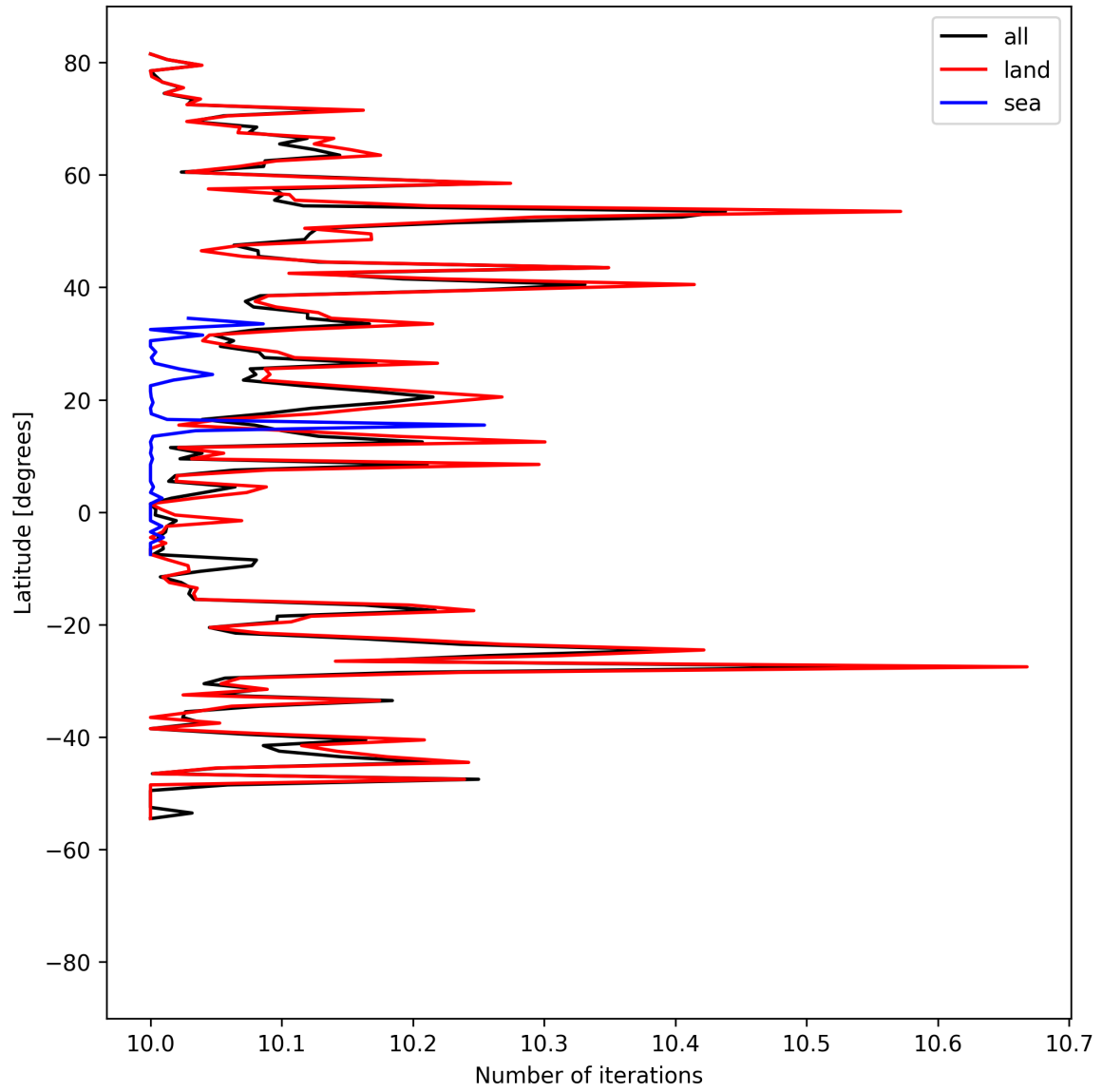
Figure 20: Zonal average of “Number of iterations” for 2025-09-04 to 2025-09-06.
