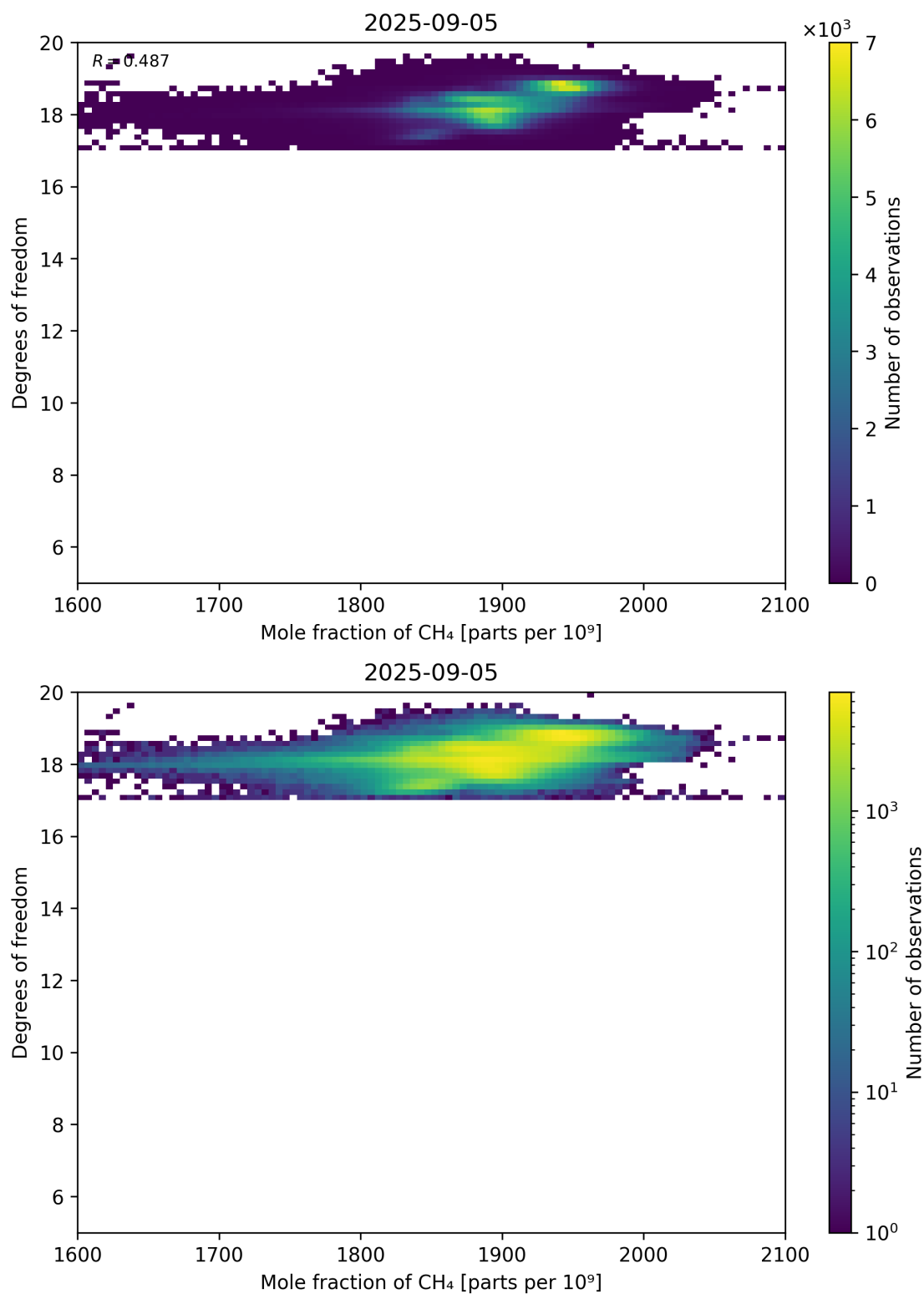
Figure 72: Scatter density plot of “Mole fraction of CH 4 ” against “Degrees of freedom” for 2025-09-04 to 2025-09-06.
