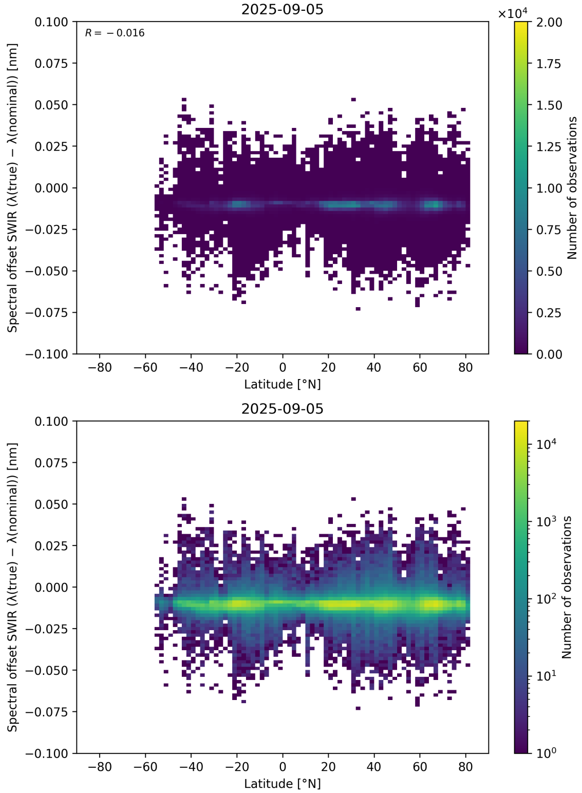
Figure 62: Scatter density plot of “Latitude” against “Spectral offset SWIR ( \lambda_{\text{true}} - \lambda_{\text{nominal}} )” for 2025-09-04 to 2025-09-06.
