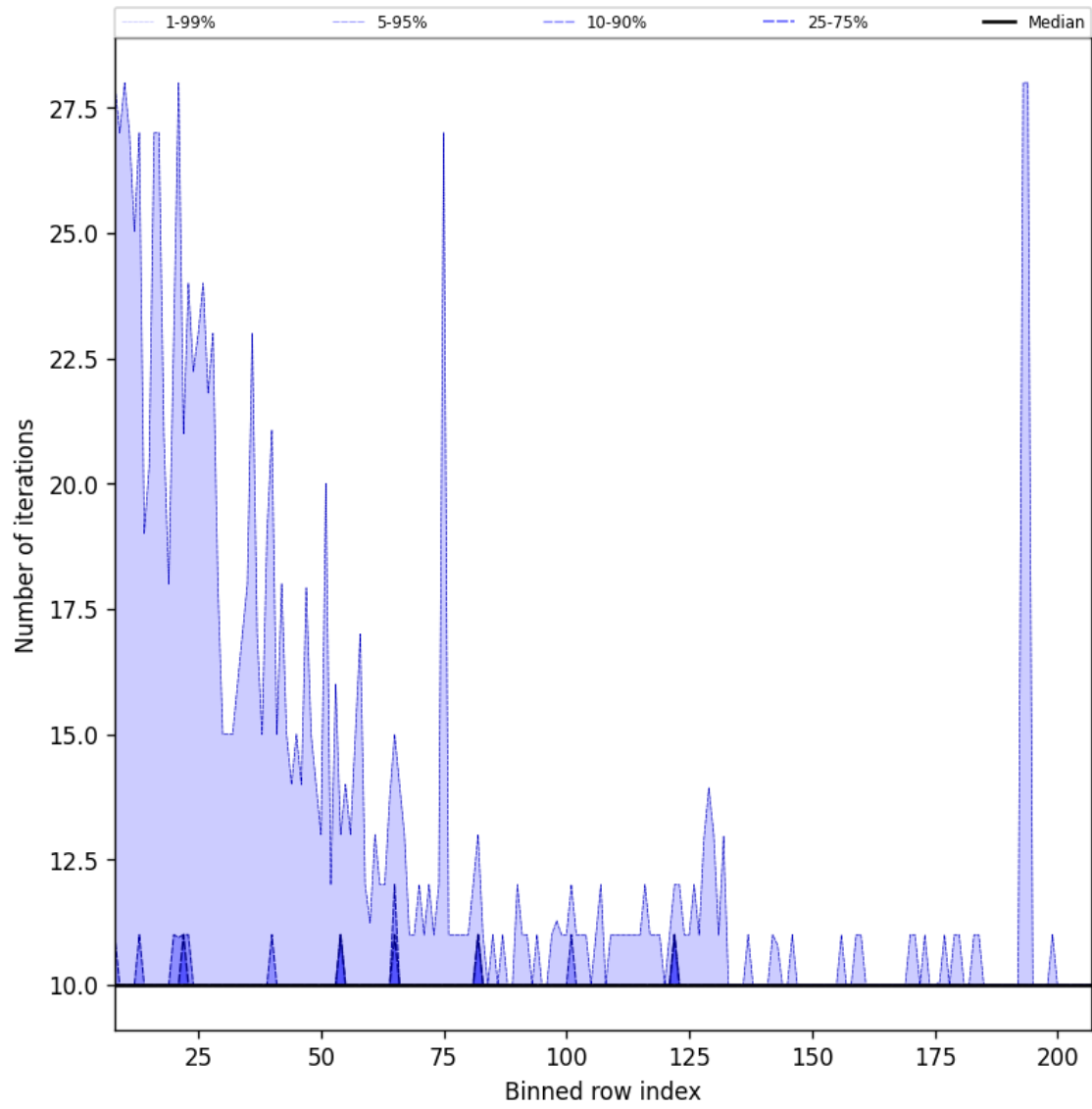
Figure 42: Along track statistics of “Number of iterations” for 2025-09-04 to 2025-09-06
