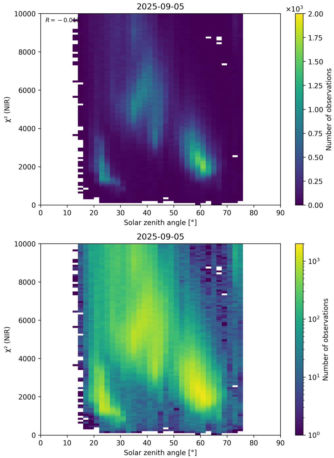
Figure 94: Scatter density plot of “Solar zenith angle” against “ \chi^2 (NIR)” for 2025-09-04 to 2025-09-06.
