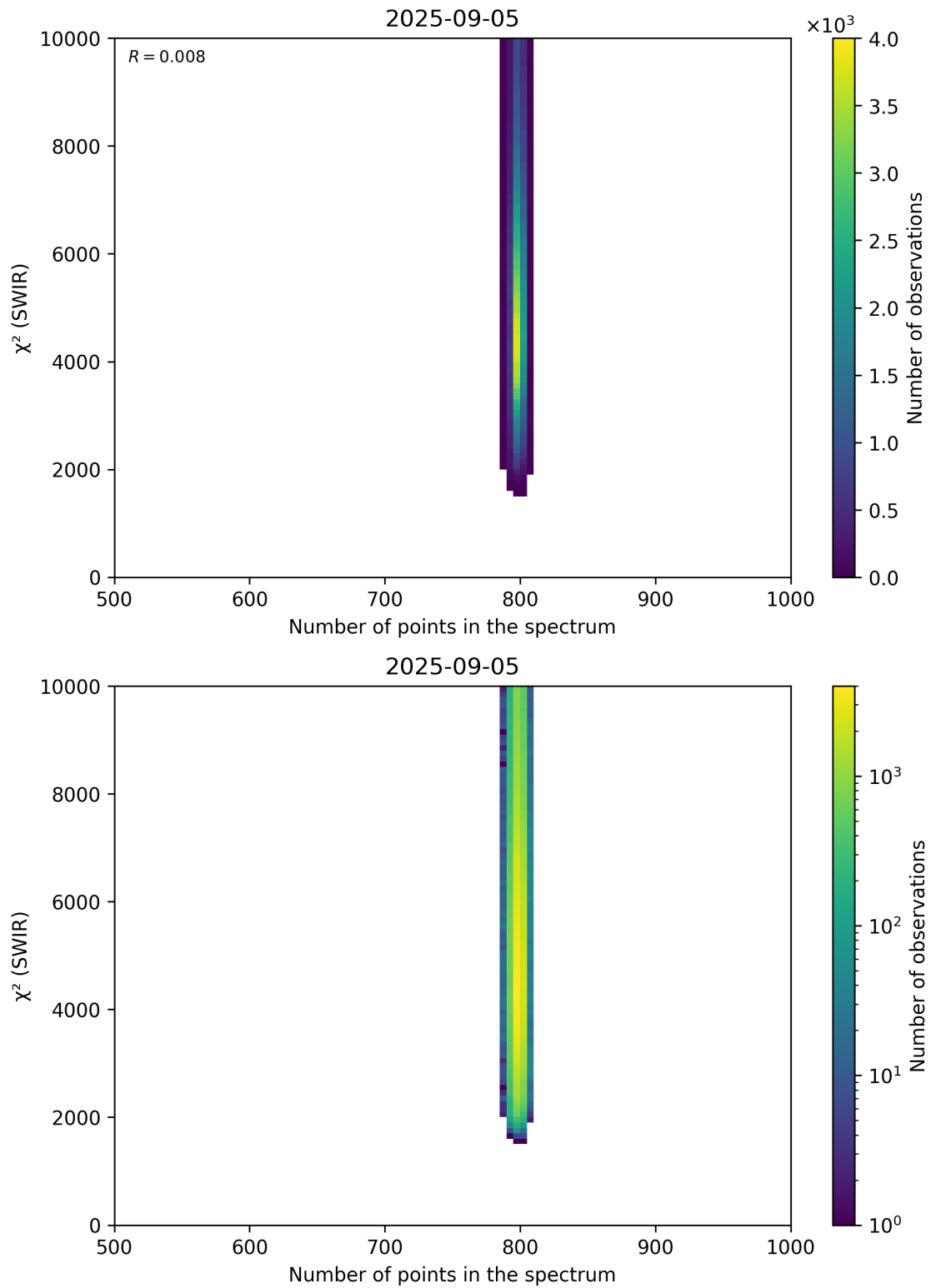
Figure 89: Scatter density plot of “Number of points in the spectrum” against “ \chi^2 (SWIR)” for 2025-09-04 to 2025-09-06.
