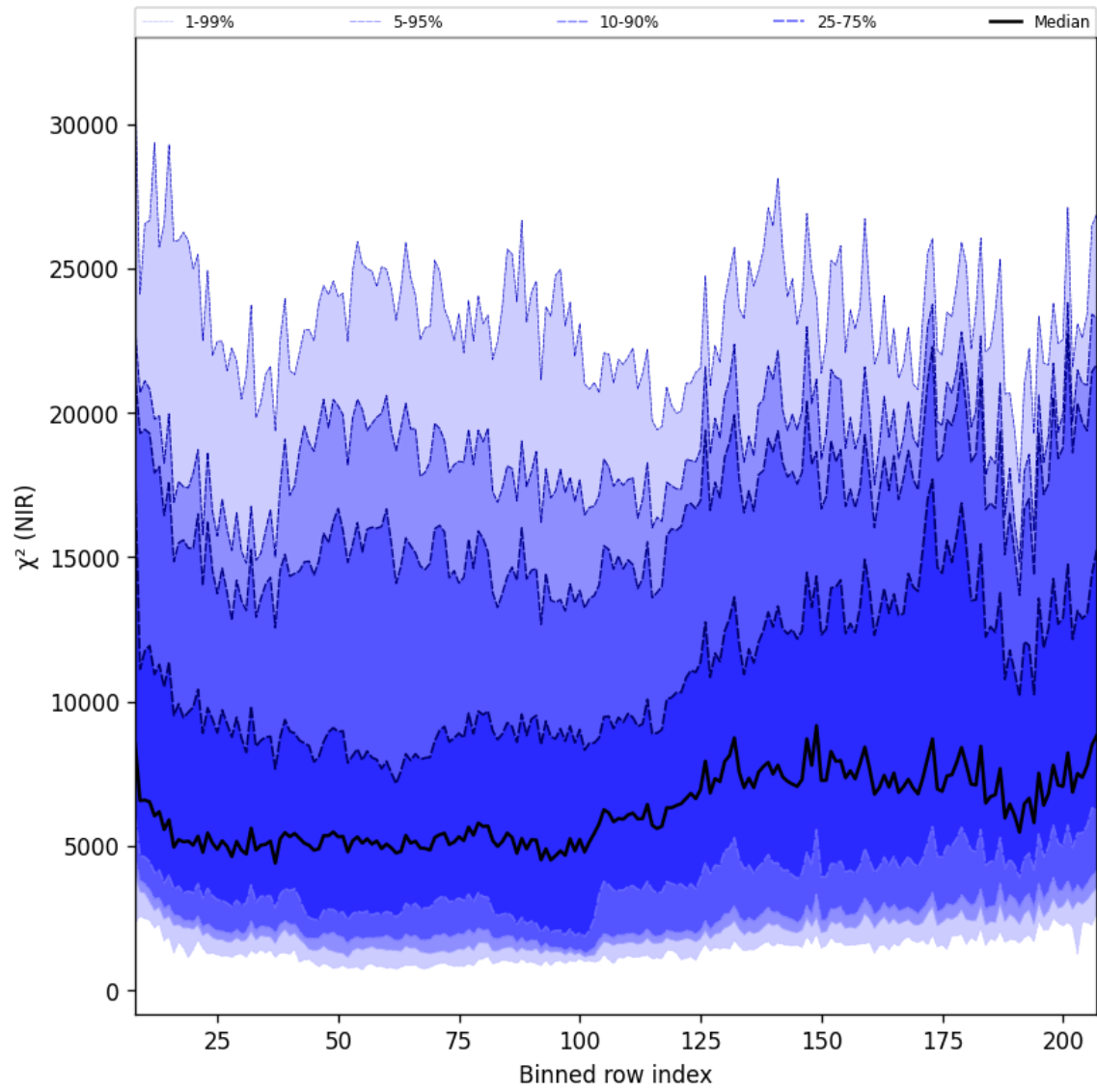
Figure 40: Along track statistics of “ \chi^2 (NIR)” for 2025-09-04 to 2025-09-06
