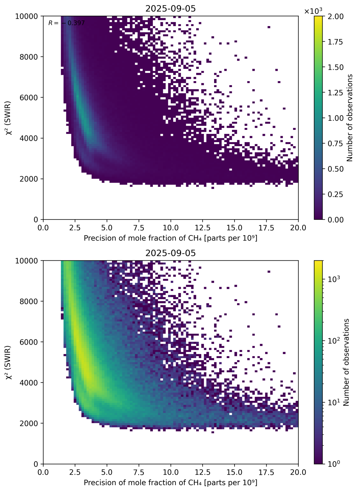
Figure 79: Scatter density plot of “Precision of mole fraction of \text{CH}_4 ” against “ \chi^2 (SWIR)” for 2025-09-04 to 2025-09-06.
