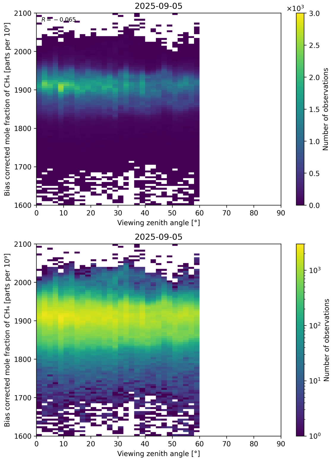
Figure 111: Scatter density plot of “Viewing zenith angle” against “Bias corrected mole fraction of CH 4 ” for 2025-09-04 to 2025-09-06.
