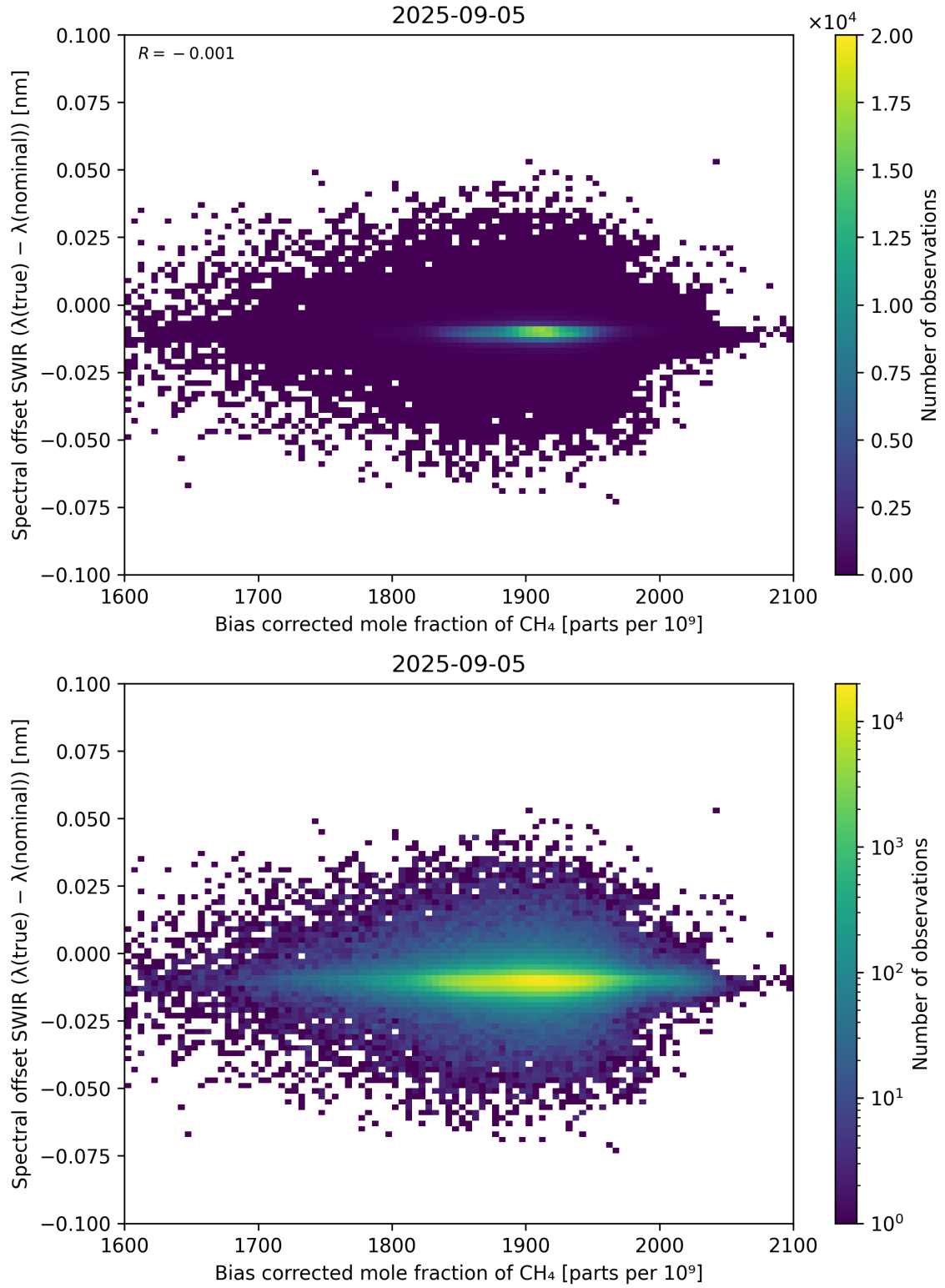
Figure 69: Scatter density plot of “Bias corrected mole fraction of \text{CH}_4 ” against “Spectral offset SWIR ( \lambda_{\text{true}} - \lambda_{\text{nominal}} )” for 2025-09-04 to 2025-09-06.
