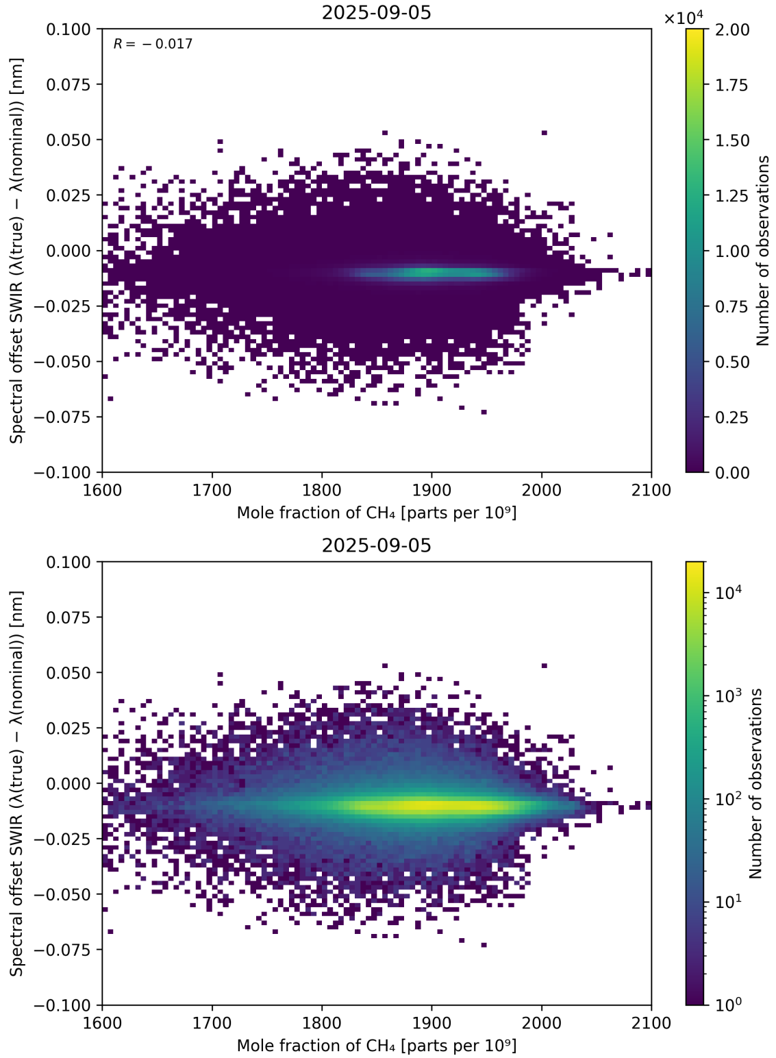
Figure 86: Scatter density plot of “Mole fraction of CH 4 ” against “Spectral offset SWIR ( \lambda_{\text{true}} - \lambda_{\text{nominal}} )” for 2025-09-04 to 2025-09-06.
