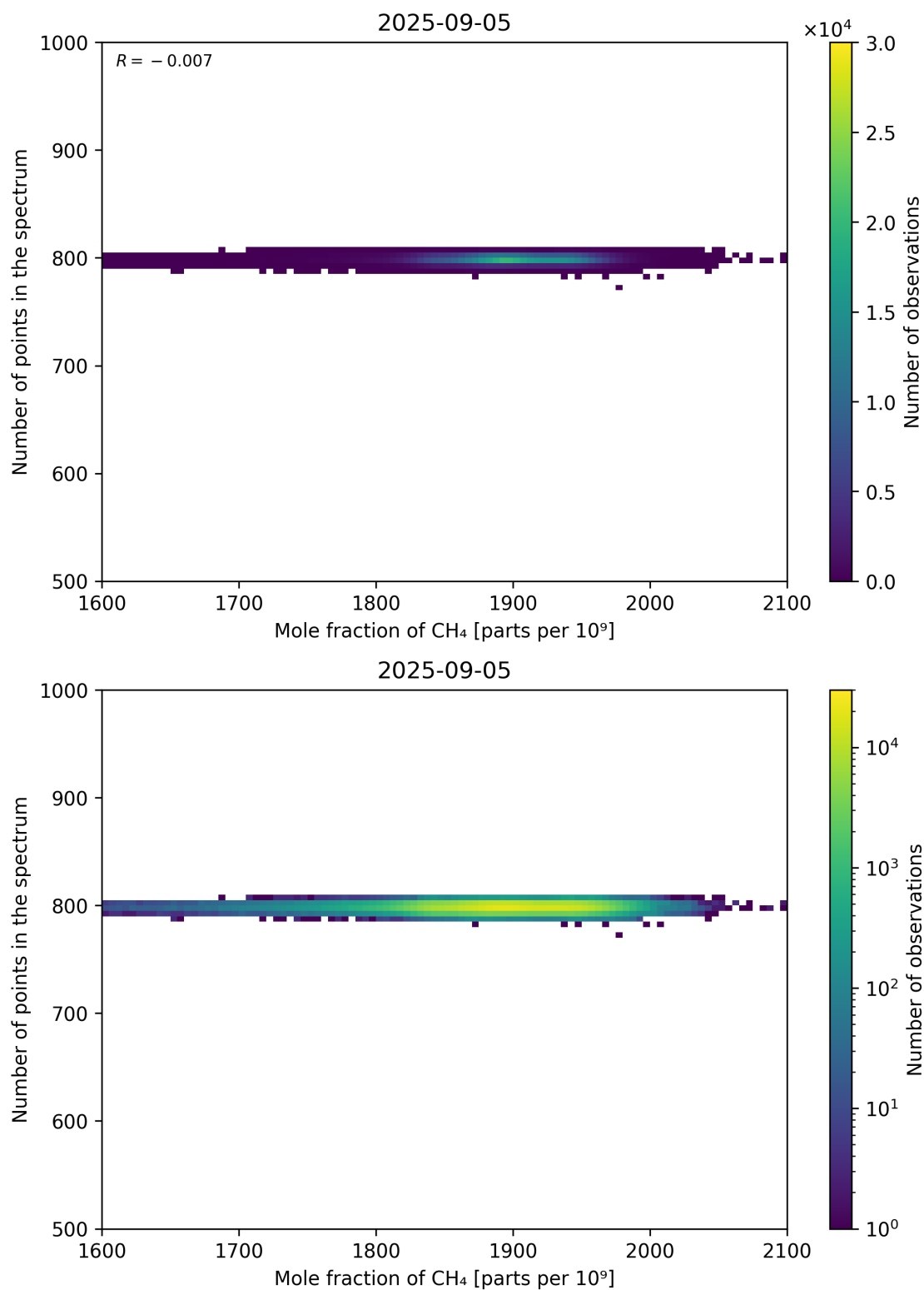
Figure 77: Scatter density plot of “Mole fraction of CH 4 ” against “Number of points in the spectrum” for 2025-09-04 to 2025-09-06.
