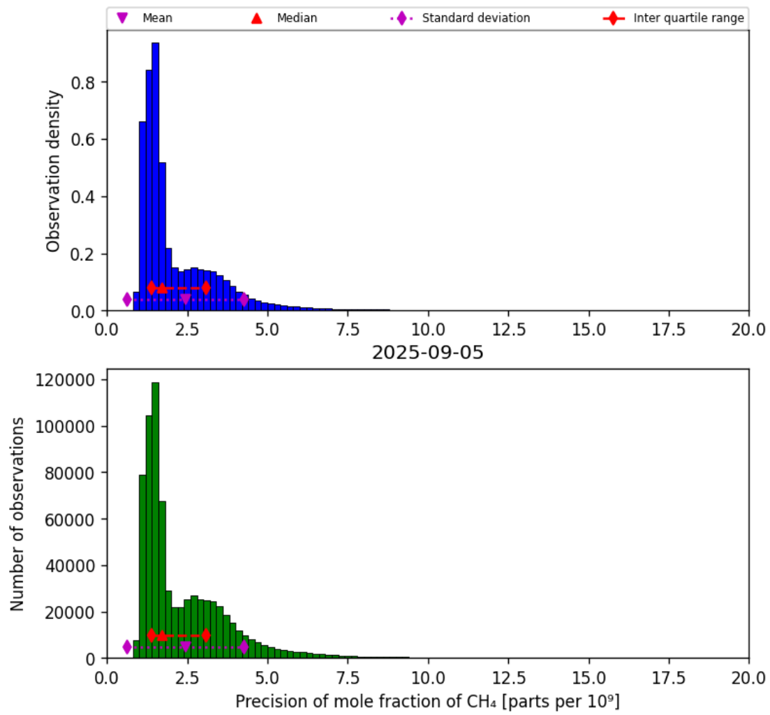
Figure 24: Histogram of “Precision of mole fraction of CH 4 ” for 2025-09-04 to 2025-09-06
