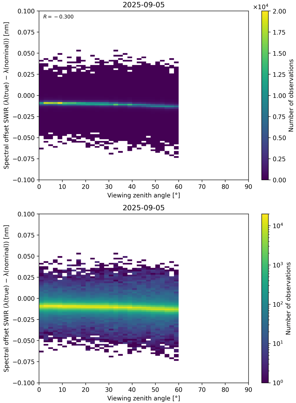
Figure 116: Scatter density plot of “Viewing zenith angle” against “Spectral offset SWIR ( \lambda_{\text{true}} - \lambda_{\text{nominal}} )” for 2025-09-04 to 2025-09-06.
