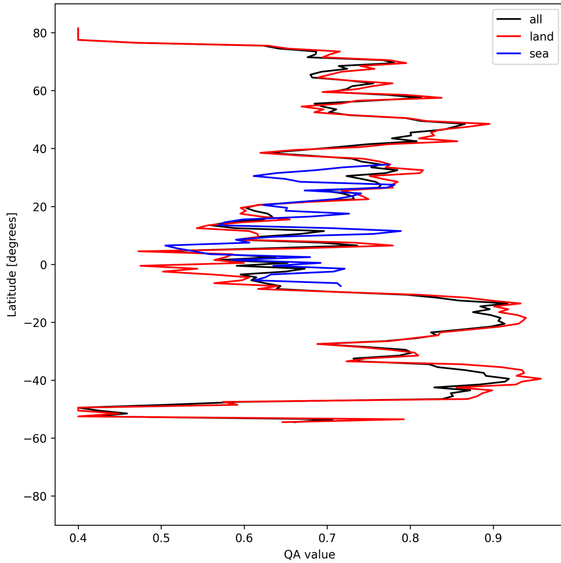
Figure 11: Zonal average of “QA value” for 2025-09-04 to 2025-09-06.
