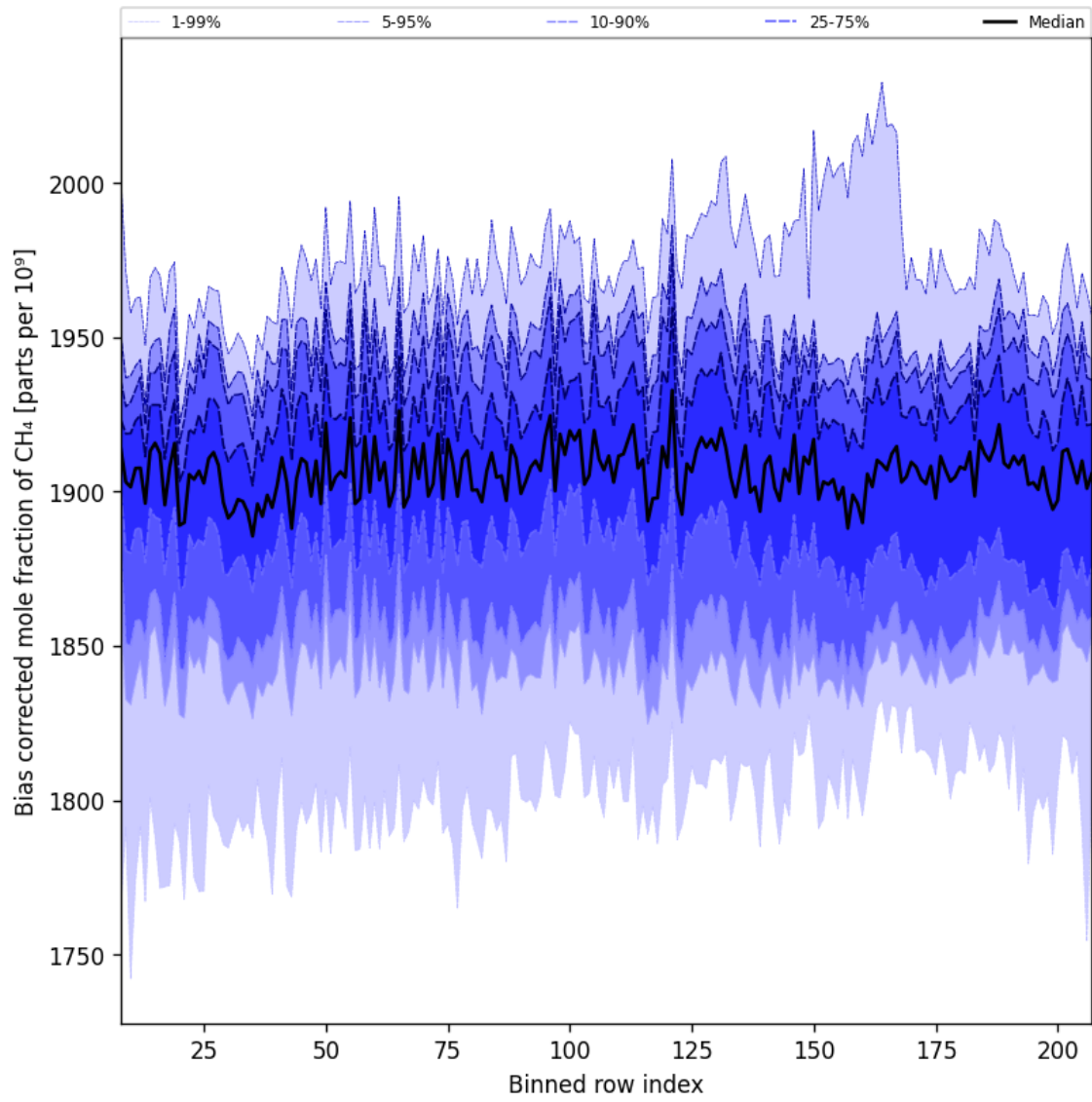
Figure 36: Along track statistics of “Bias corrected mole fraction of CH 4 ” for 2025-09-04 to 2025-09-06
