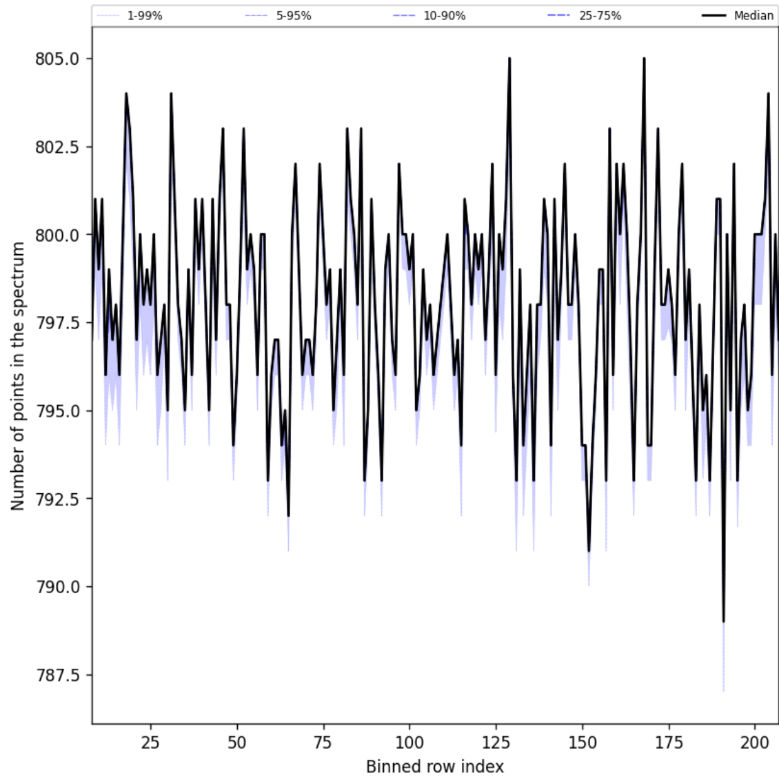
Figure 37: Along track statistics of “Number of points in the spectrum” for 2025-09-04 to 2025-09-06
