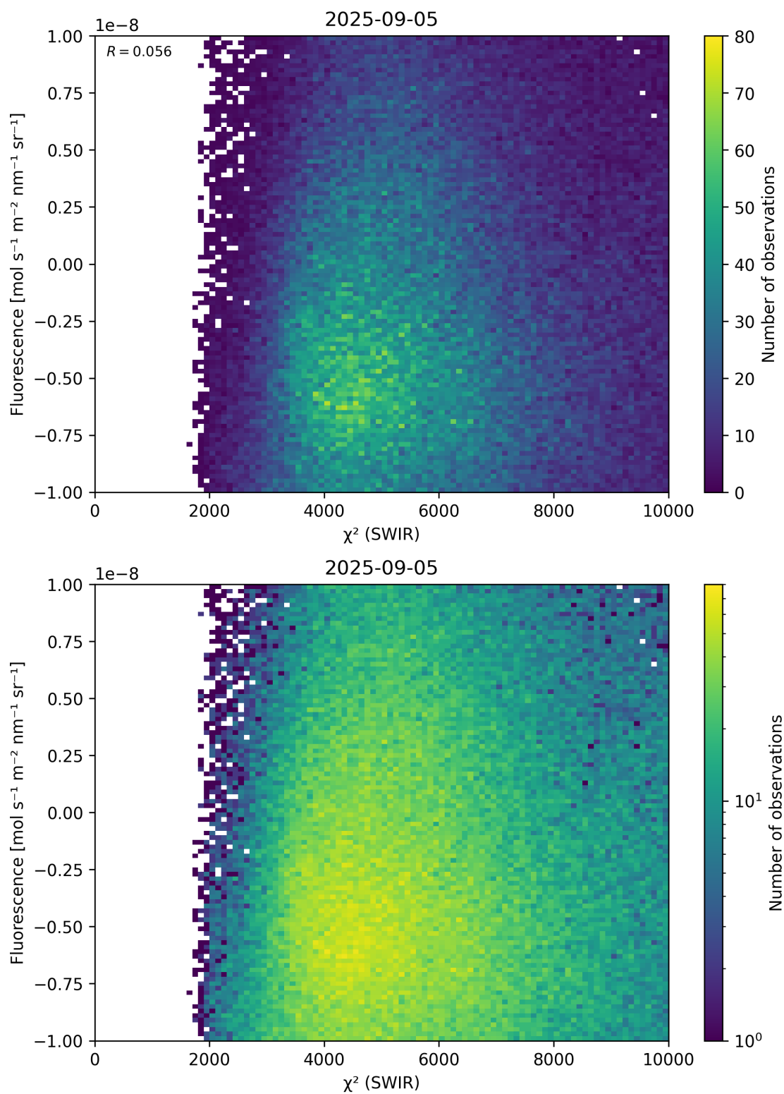
Figure 49: Scatter density plot of “ \chi^2 (SWIR)” against “Fluorescence” for 2025-09-04 to 2025-09-06.
