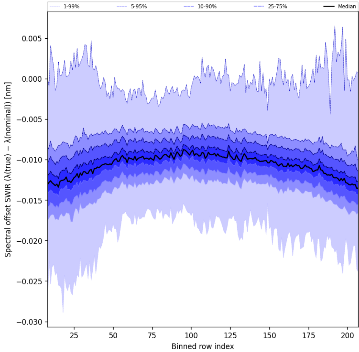
Figure 38: Along track statistics of “Spectral offset SWIR ( \lambda_{\text{true}} - \lambda_{\text{nominal}} )” for 2025-09-04 to 2025-09-06
