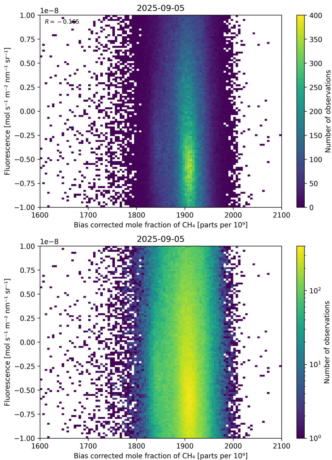
Figure 66: Scatter density plot of “Bias corrected mole fraction of \text{CH}_4 ” against “Fluorescence” for 2025-09-04 to 2025-09-06.
