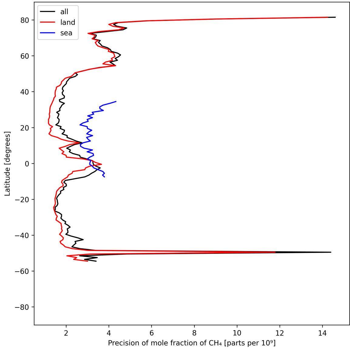
Figure 13: Zonal average of “Precision of mole fraction of CH 4 ” for 2025-09-04 to 2025-09-06.
