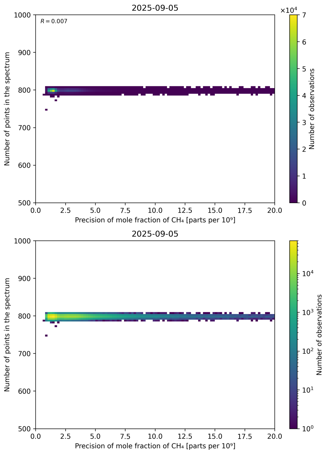
Figure 84: Scatter density plot of “Precision of mole fraction of CH 4 ” against “Number of points in the spectrum” for 2025-09-04 to 2025-09-06.
