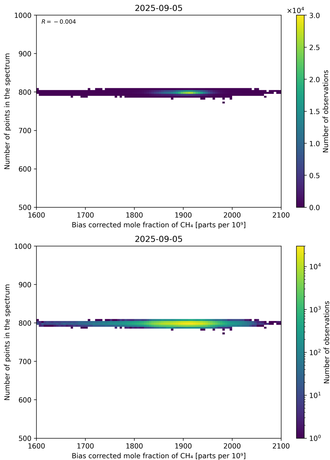
Figure 68: Scatter density plot of “Bias corrected mole fraction of CH 4 ” against “Number of points in the spectrum” for 2025-09-04 to 2025-09-06.
