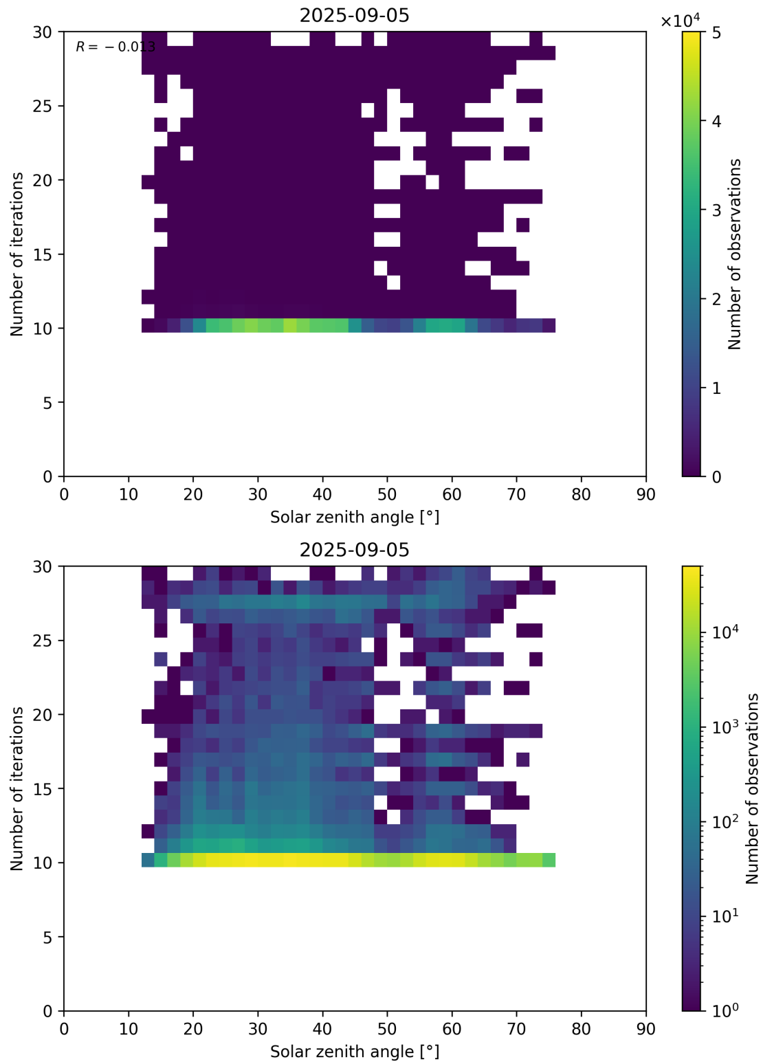
Figure 102: Scatter density plot of “Solar zenith angle” against “Number of iterations” for 2025-09-04 to 2025-09-06.
