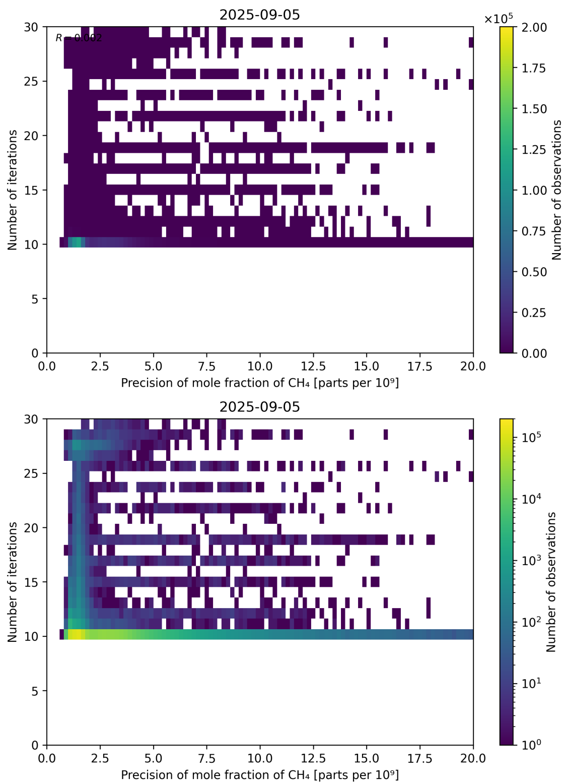
Figure 83: Scatter density plot of “Precision of mole fraction of CH 4 ” against “Number of iterations” for 2025-09-04 to 2025-09-06.
