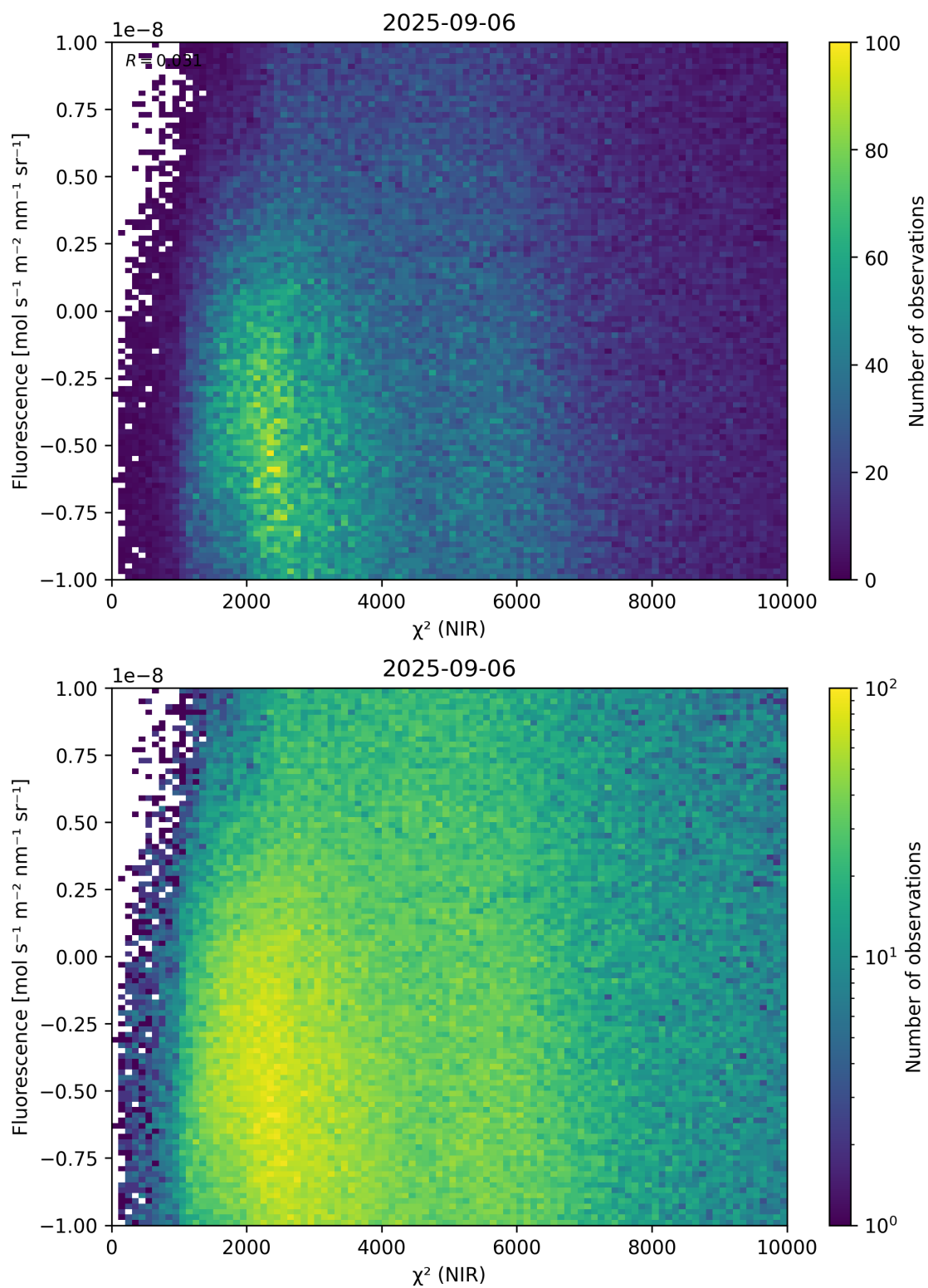
Figure 45: Scatter density plot of “ \chi^2 (NIR)” against “Fluorescence” for 2025-09-05 to 2025-09-07.
