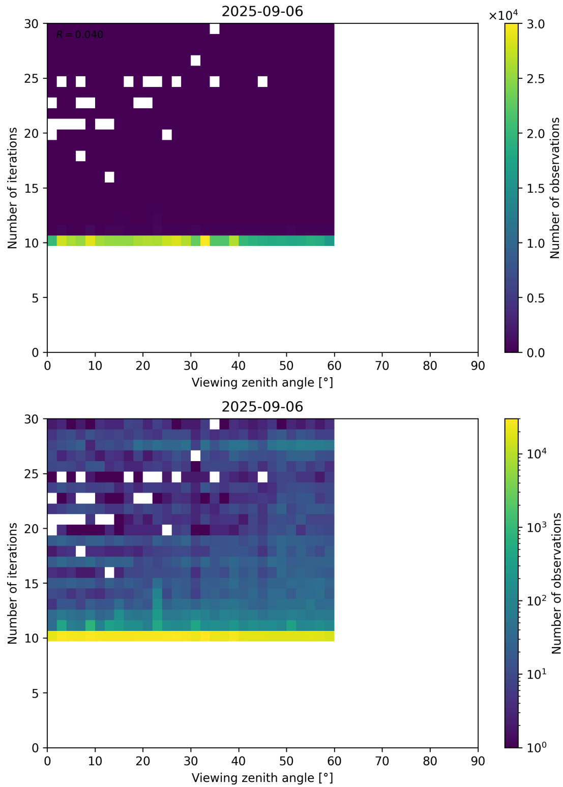
Figure 113: Scatter density plot of “Viewing zenith angle” against “Number of iterations” for 2025-09-05 to 2025-09-07.
