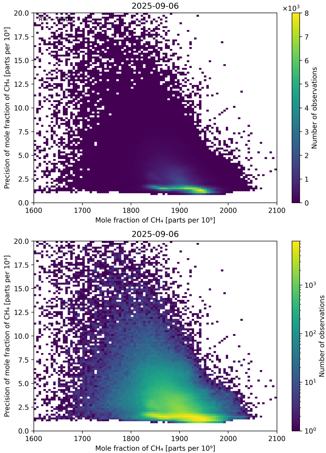
Figure 75: Scatter density plot of “Mole fraction of CH 4 ” against “Precision of mole fraction of CH 4 ” for 2025-09-05 to 2025-09-07.
