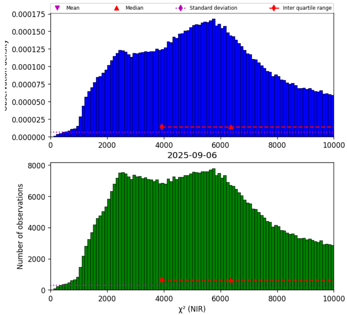
Figure 29: Histogram of “ \chi^2 (NIR)” for 2025-09-05 to 2025-09-07
