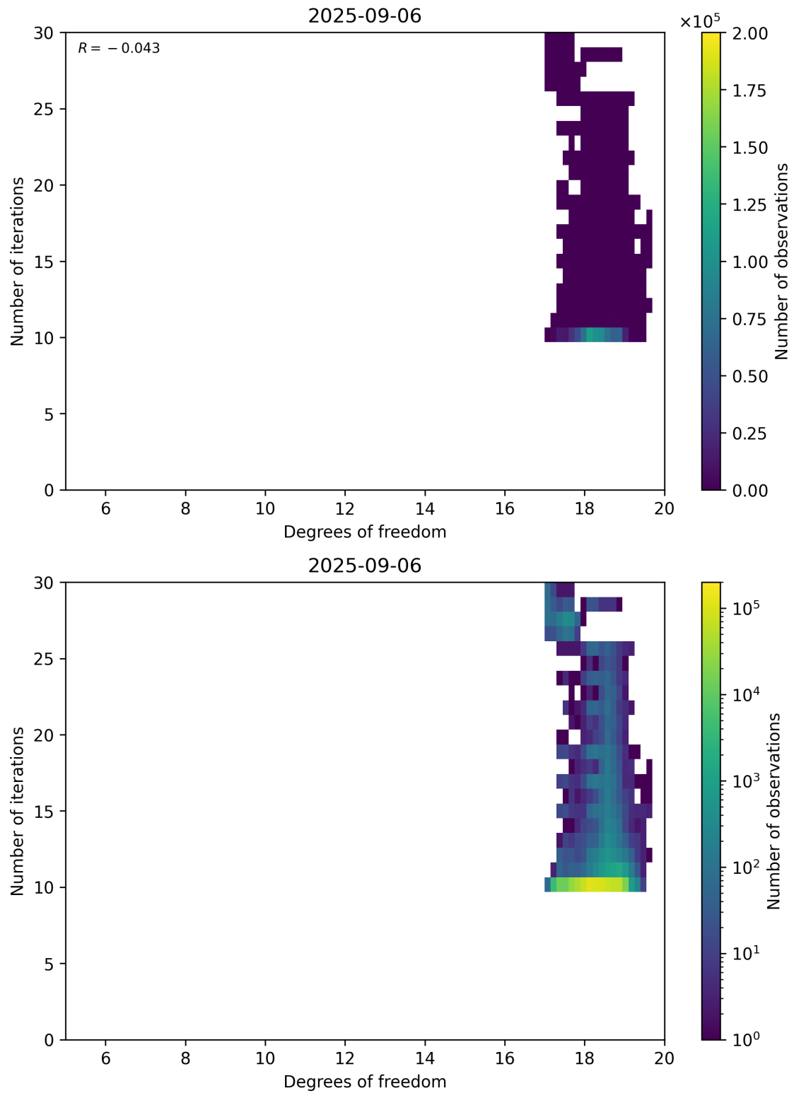
Figure 52: Scatter density plot of “Degrees of freedom” against “Number of iterations” for 2025-09-05 to 2025-09-07.
