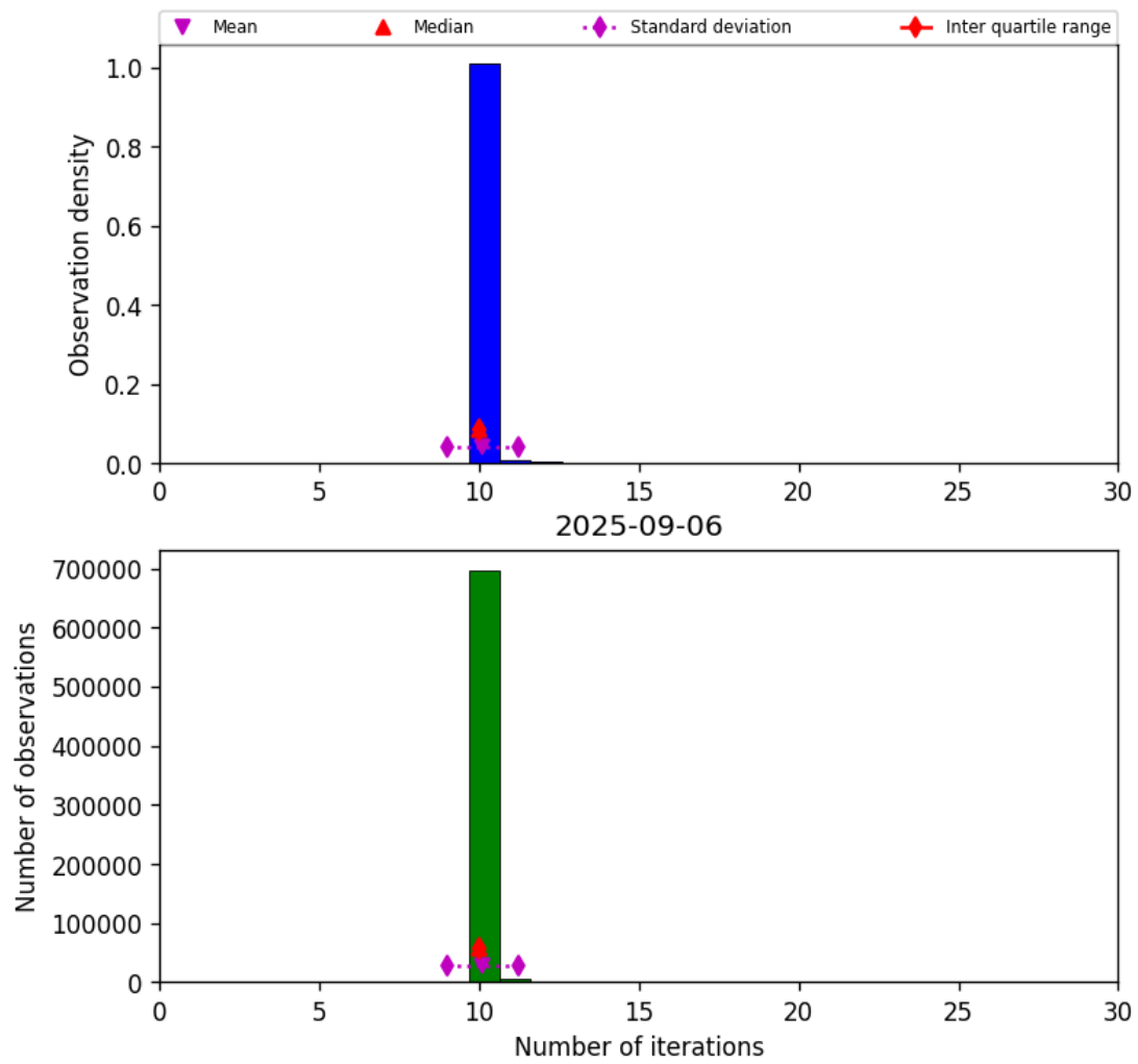
Figure 31: Histogram of “Number of iterations” for 2025-09-05 to 2025-09-07
