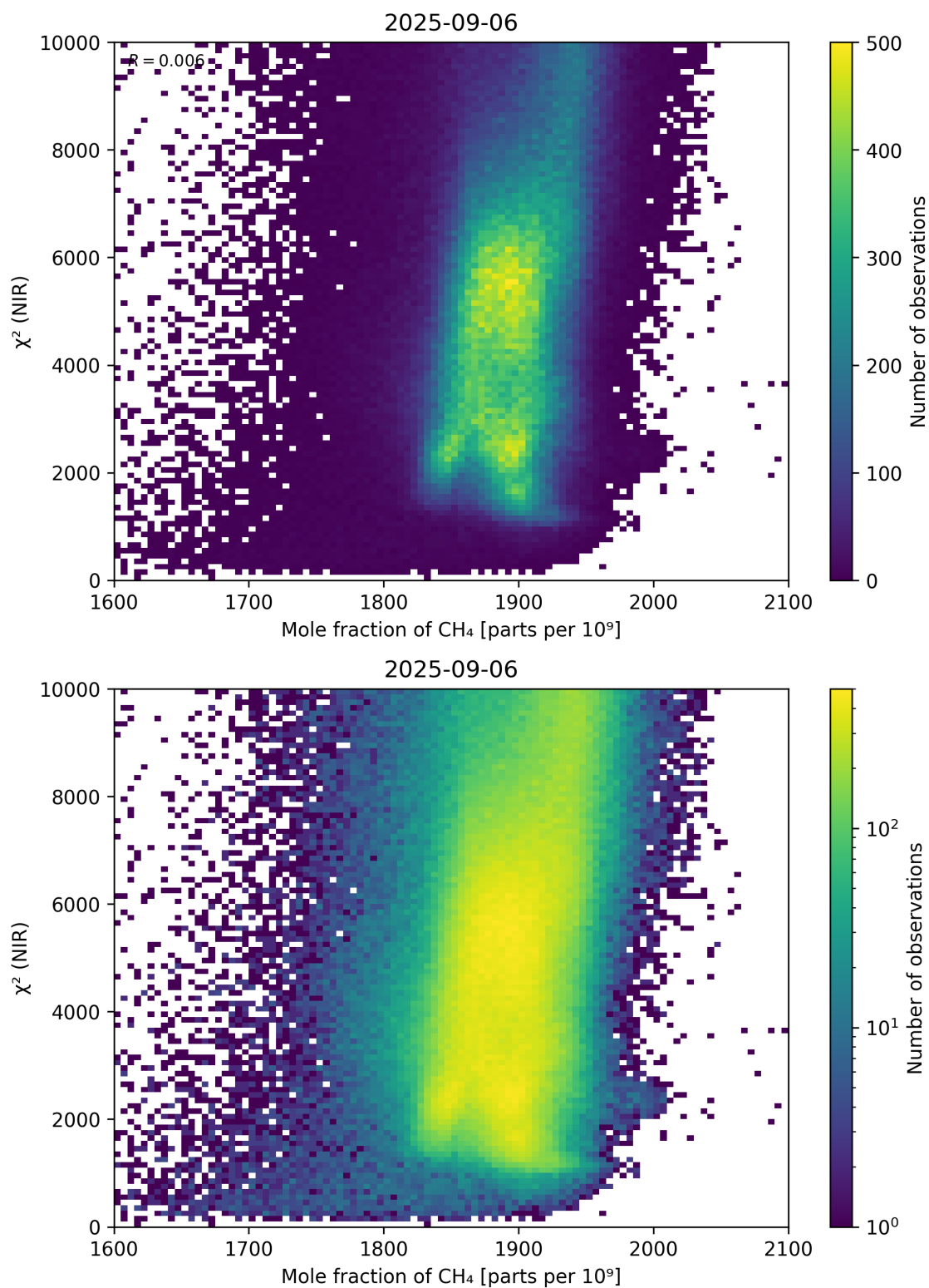
Figure 70: Scatter density plot of “Mole fraction of \text{CH}_4 ” against “ \chi^2 (NIR)” for 2025-09-05 to 2025-09-07.
