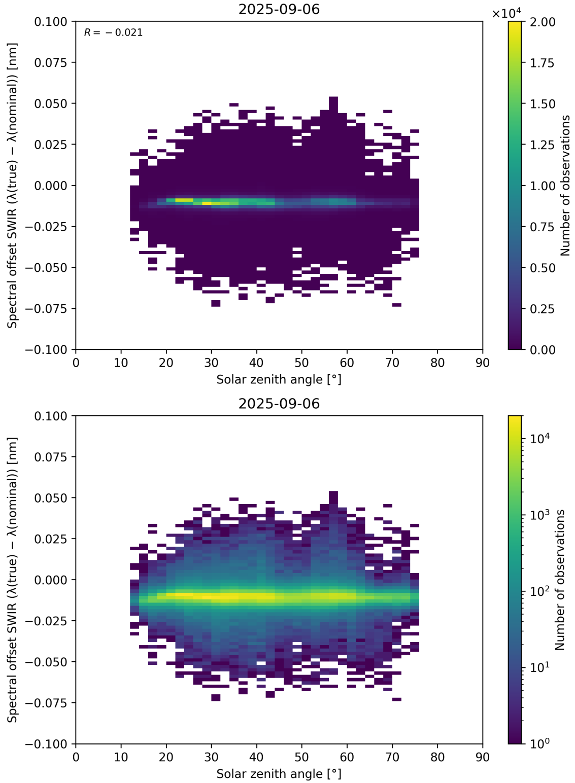
Figure 104: Scatter density plot of “Solar zenith angle” against “Spectral offset SWIR ( \lambda_{\text{true}} - \lambda_{\text{nominal}} )” for 2025-09-05 to 2025-09-07.
