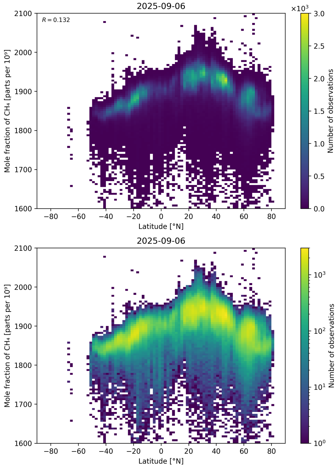
Figure 57: Scatter density plot of “Latitude” against “Mole fraction of \text{CH}_4 ” for 2025-09-05 to 2025-09-07.
