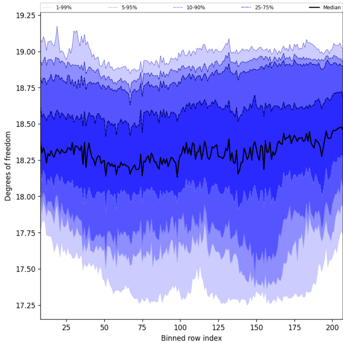
Figure 41: Along track statistics of “Degrees of freedom” for 2025-09-05 to 2025-09-07
