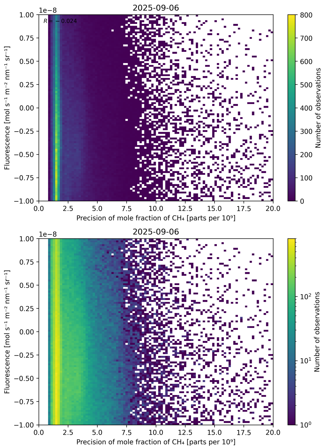
Figure 81: Scatter density plot of “Precision of mole fraction of \text{CH}_4 ” against “Fluorescence” for 2025-09-05 to 2025-09-07.
