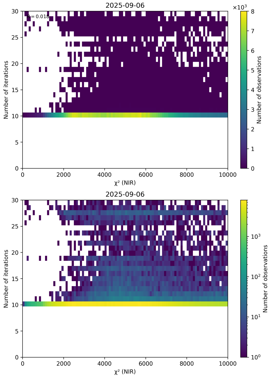
Figure 46: Scatter density plot of “ \chi^2 (NIR)” against “Number of iterations” for 2025-09-05 to 2025-09-07.
