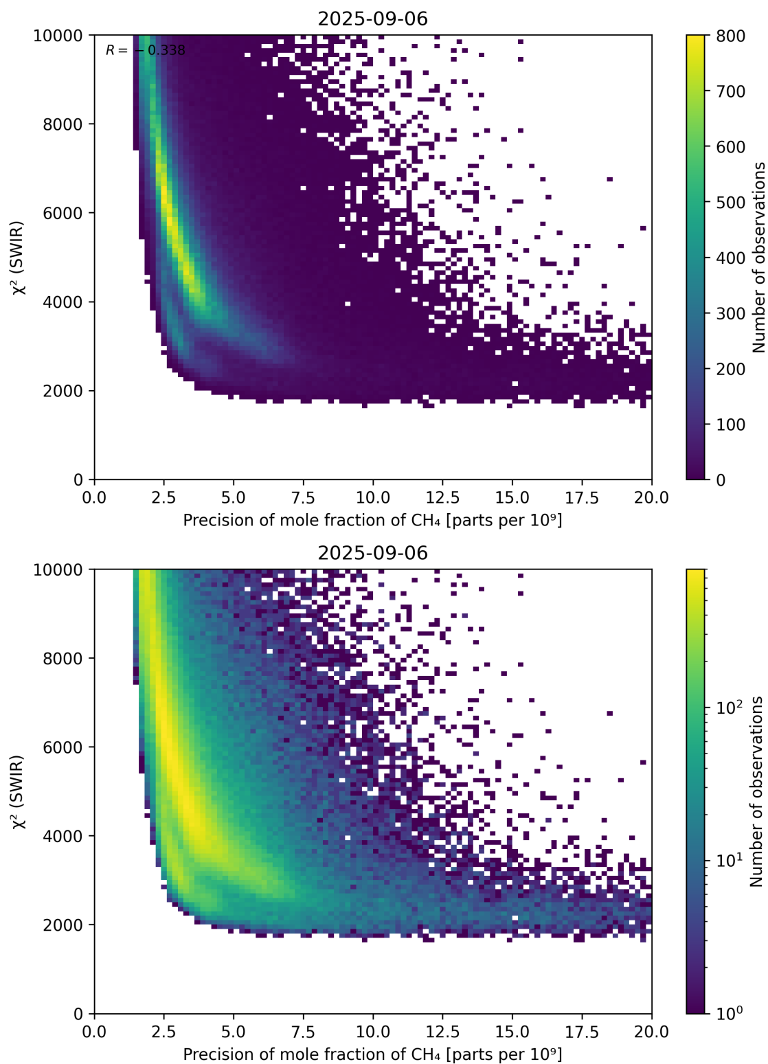
Figure 79: Scatter density plot of “Precision of mole fraction of CH 4 ” against “ \chi^2 (SWIR)” for 2025-09-05 to 2025-09-07.
