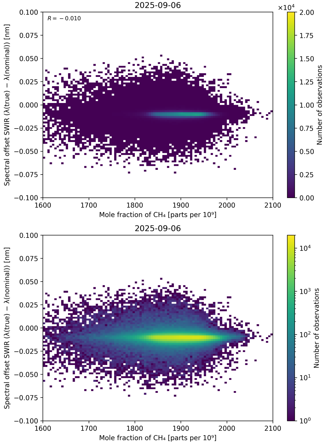
Figure 86: Scatter density plot of “Mole fraction of CH 4 ” against “Spectral offset SWIR ( \lambda_{\text{true}} - \lambda_{\text{nominal}} )” for 2025-09-05 to 2025-09-07.
