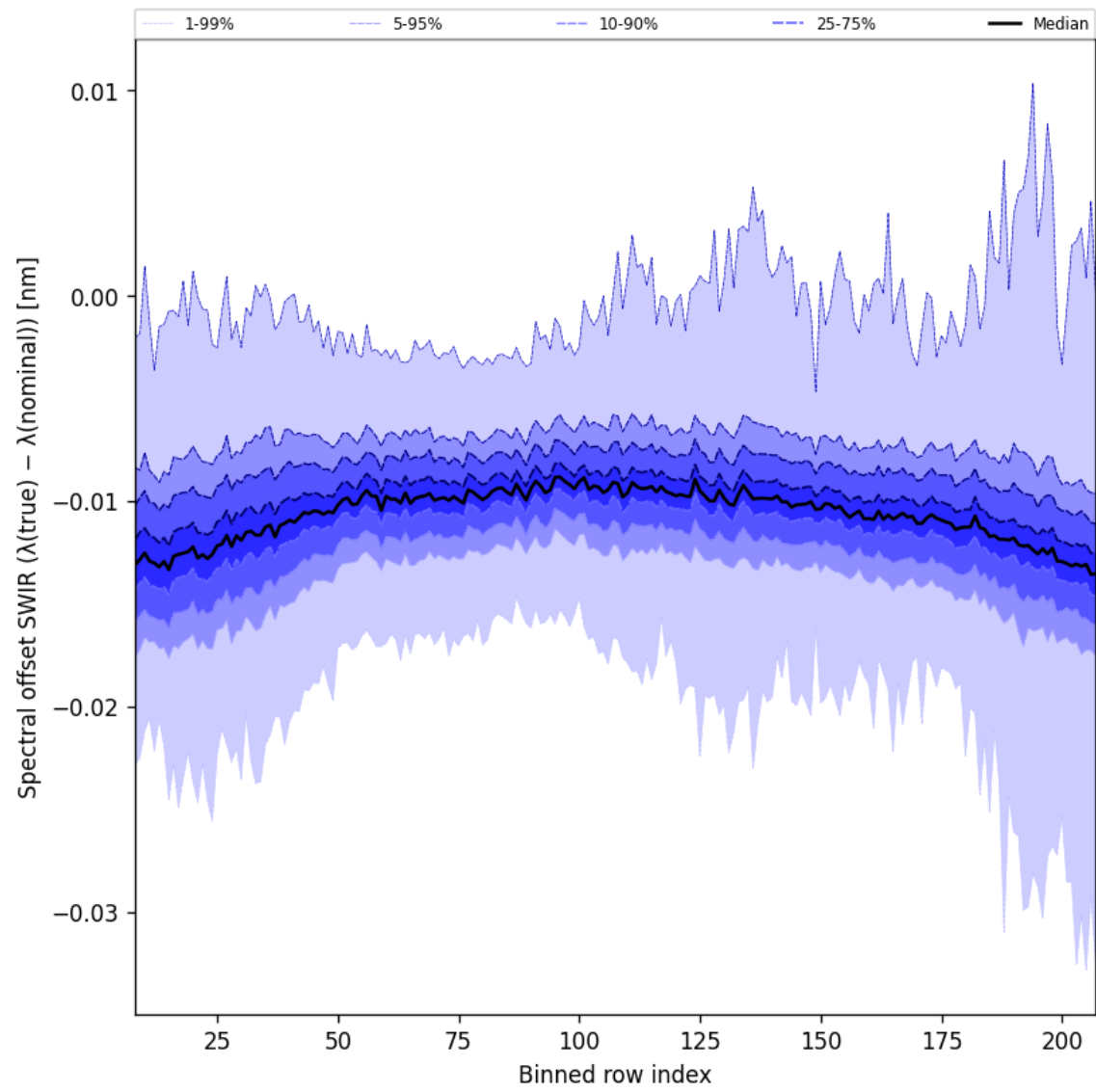
Figure 38: Along track statistics of “Spectral offset SWIR ( \lambda_{\text{true}} - \lambda_{\text{nominal}} )” for 2025-09-05 to 2025-09-07
