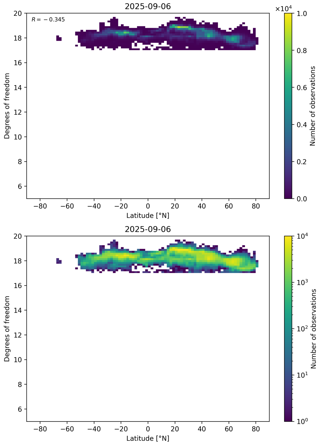
Figure 55: Scatter density plot of “Latitude” against “Degrees of freedom” for 2025-09-05 to 2025-09-07.
