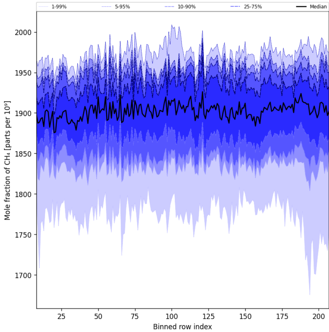
Figure 34: Along track statistics of “Mole fraction of CH 4 ” for 2025-09-05 to 2025-09-07
