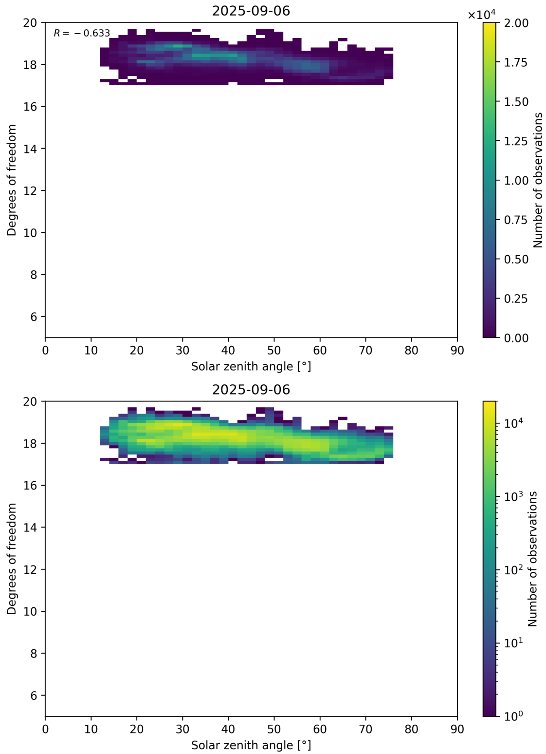
Figure 96: Scatter density plot of “Solar zenith angle” against “Degrees of freedom” for 2025-09-05 to 2025-09-07.
