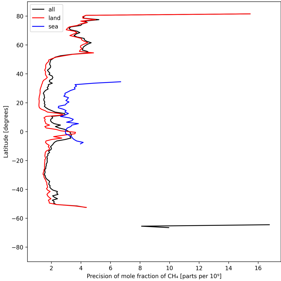
Figure 13: Zonal average of “Precision of mole fraction of CH 4 ” for 2025-09-05 to 2025-09-07.
