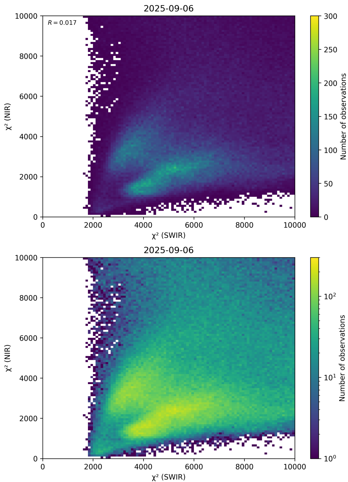
Figure 47: Scatter density plot of “ \chi^2 (SWIR)” against “ \chi^2 (NIR)” for 2025-09-05 to 2025-09-07.
