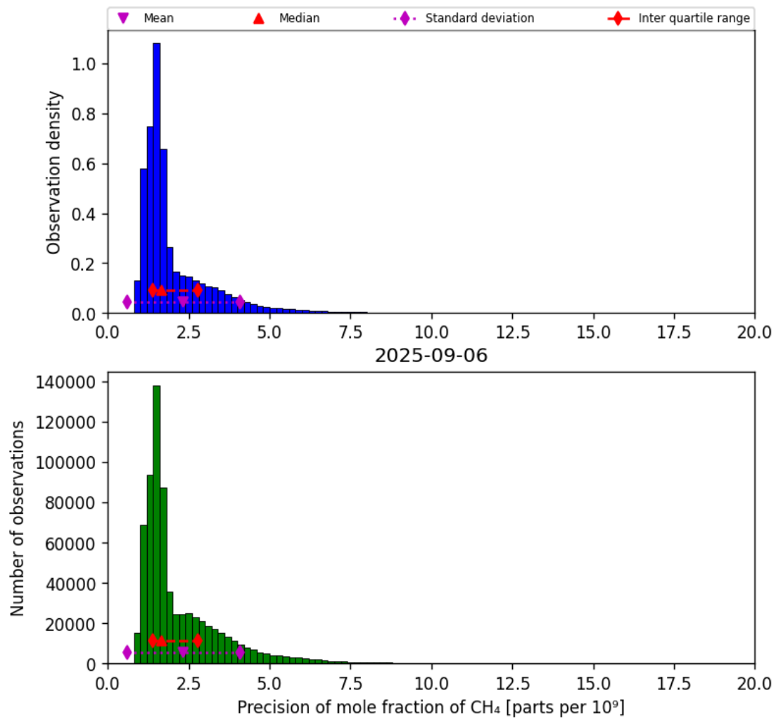
Figure 24: Histogram of “Precision of mole fraction of CH 4 ” for 2025-09-05 to 2025-09-07
