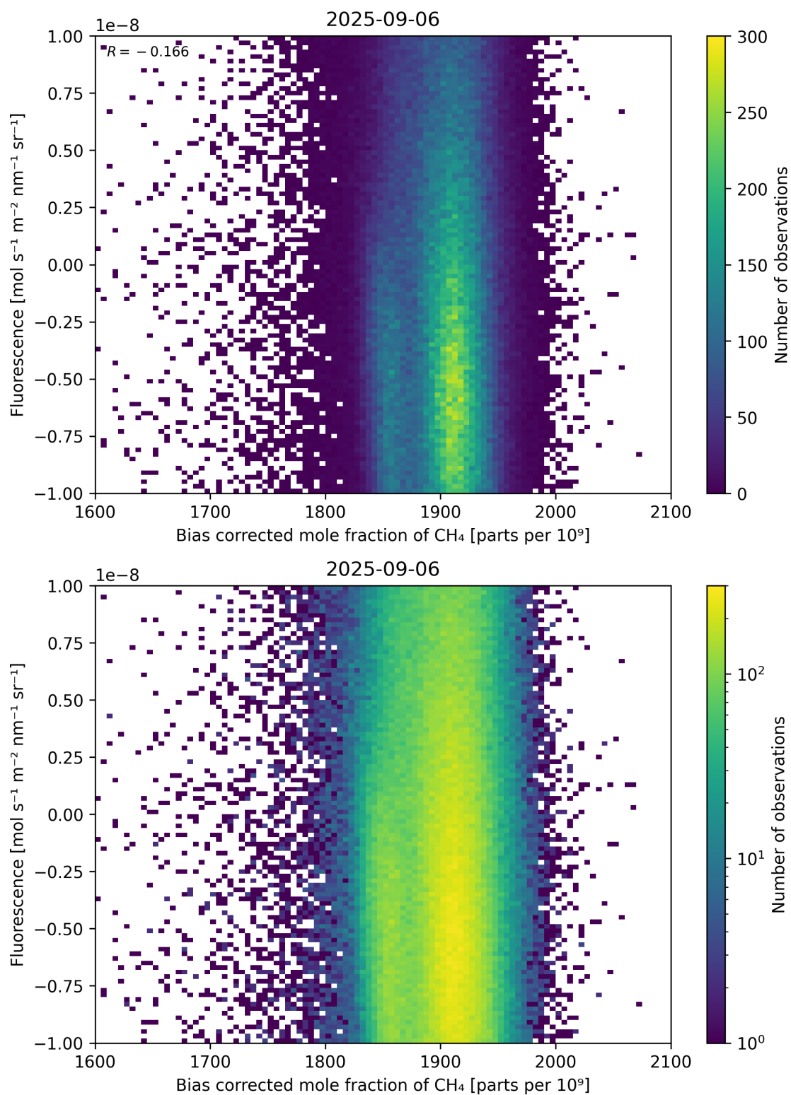
Figure 66: Scatter density plot of “Bias corrected mole fraction of \text{CH}_4 ” against “Fluorescence” for 2025-09-05 to 2025-09-07.
