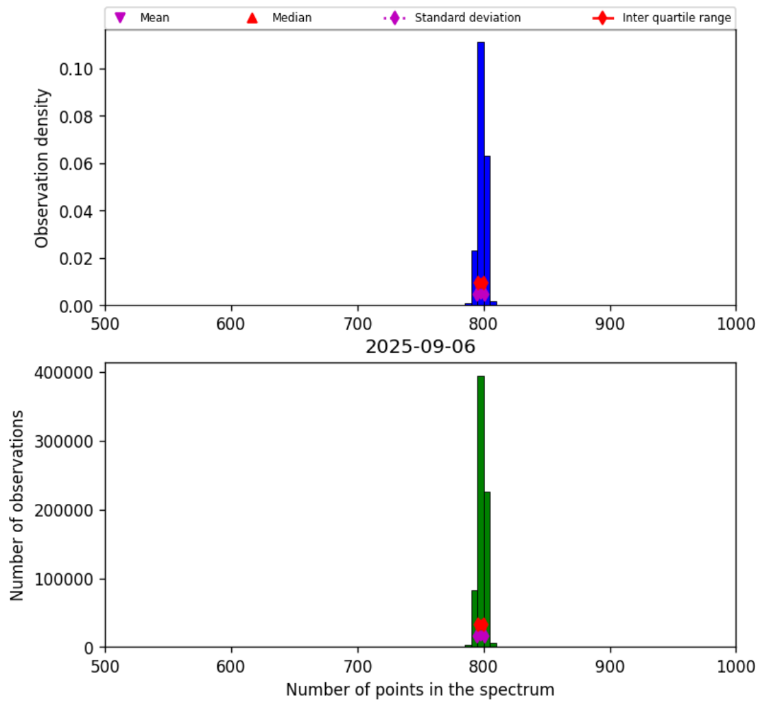
Figure 26: Histogram of “Number of points in the spectrum” for 2025-09-05 to 2025-09-07
