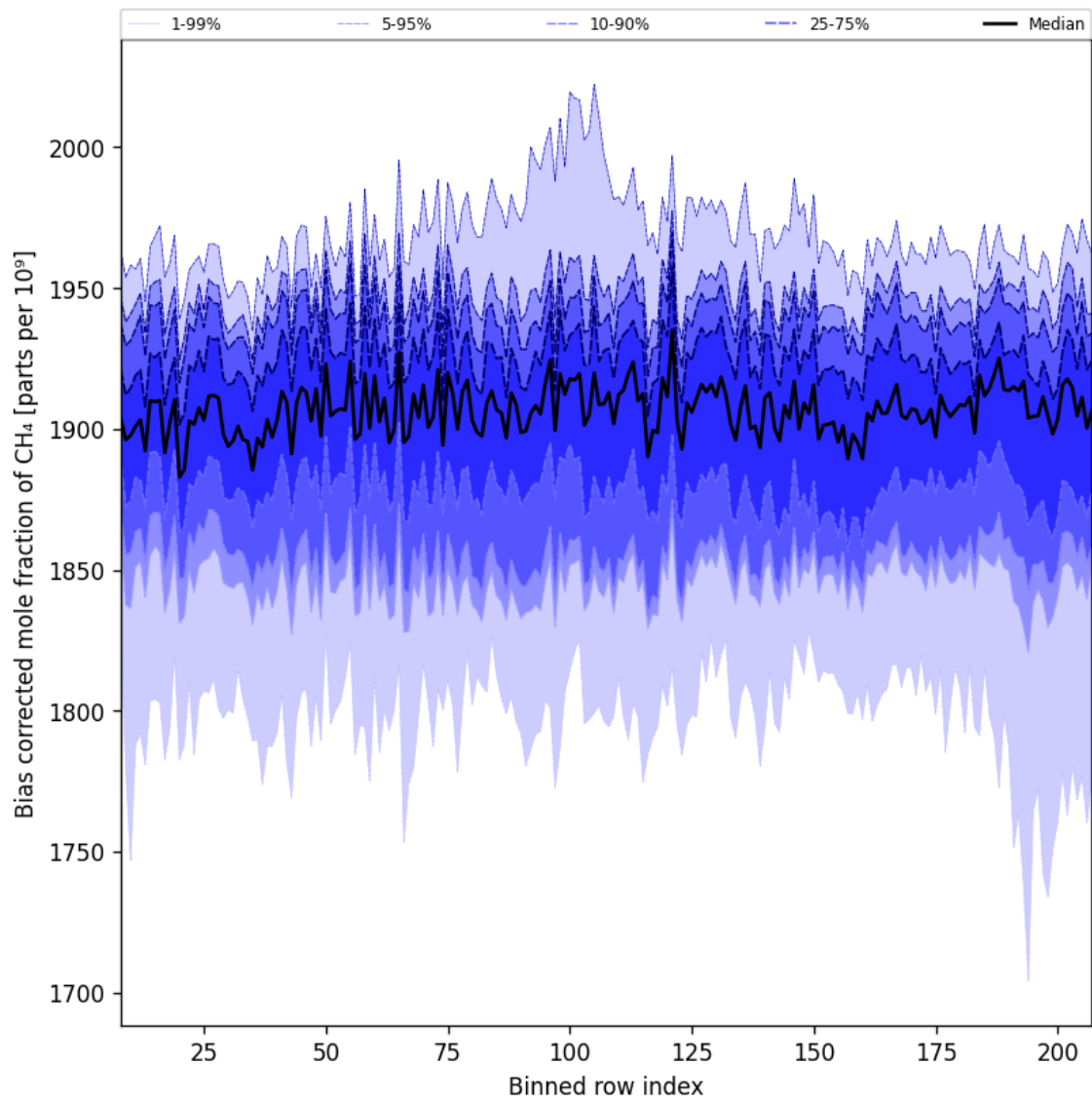
Figure 36: Along track statistics of “Bias corrected mole fraction of CH 4 ” for 2025-09-05 to 2025-09-07
