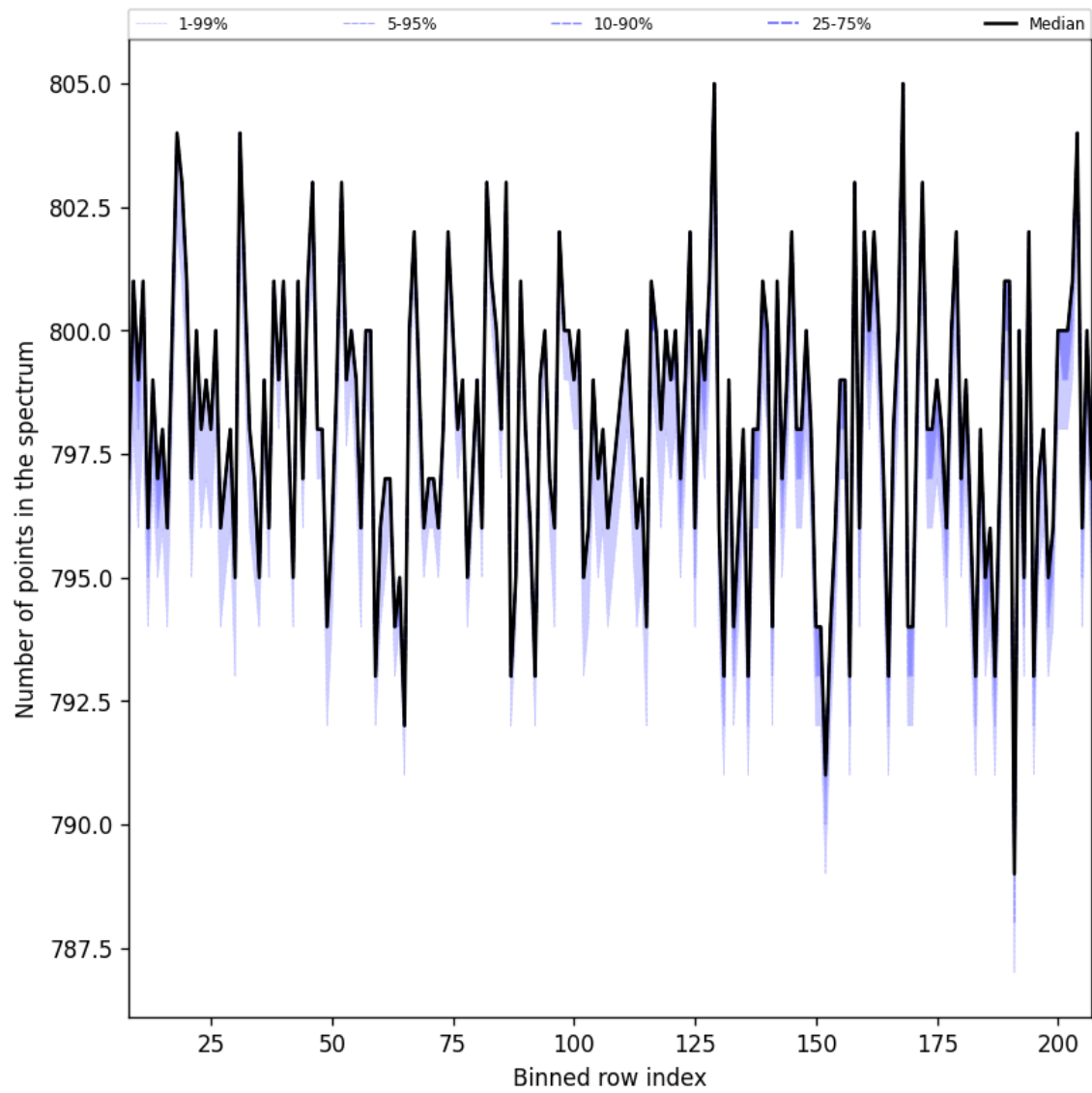
Figure 37: Along track statistics of “Number of points in the spectrum” for 2025-09-05 to 2025-09-07
