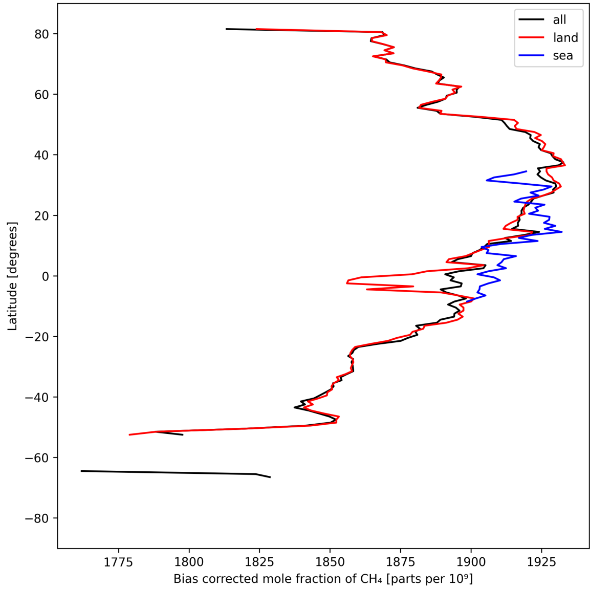
Figure 14: Zonal average of “Bias corrected mole fraction of CH 4 ” for 2025-09-05 to 2025-09-07.
