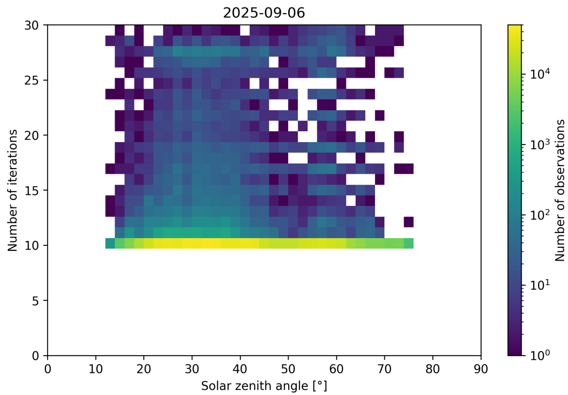
Figure 102: Scatter density plot of “Solar zenith angle” against “Number of iterations” for 2025-09-05 to 2025-09-07.
