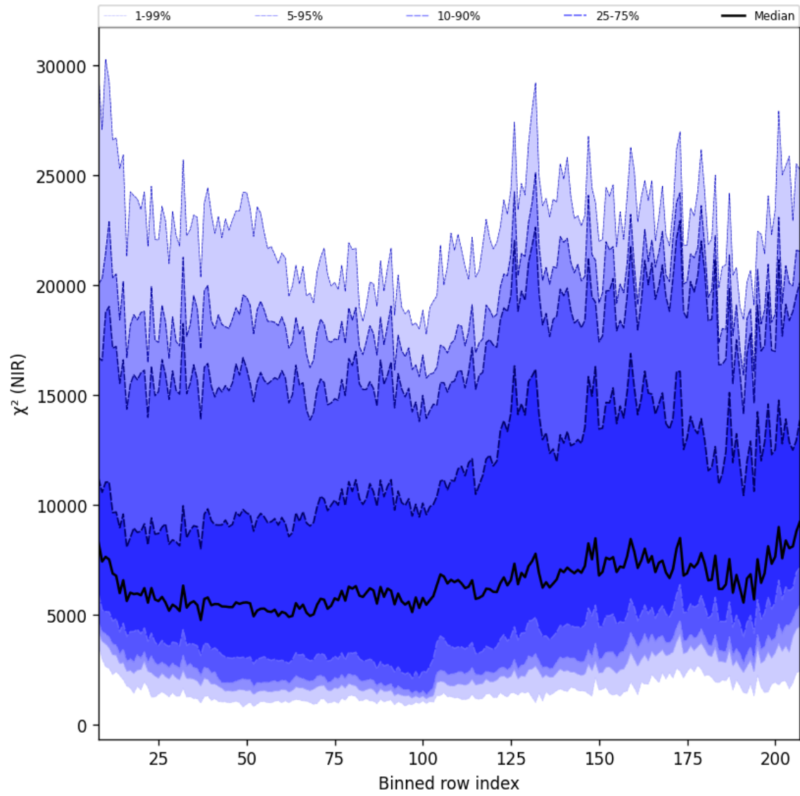
Figure 40: Along track statistics of " \chi^2 (NIR)" for 2025-09-05 to 2025-09-07
