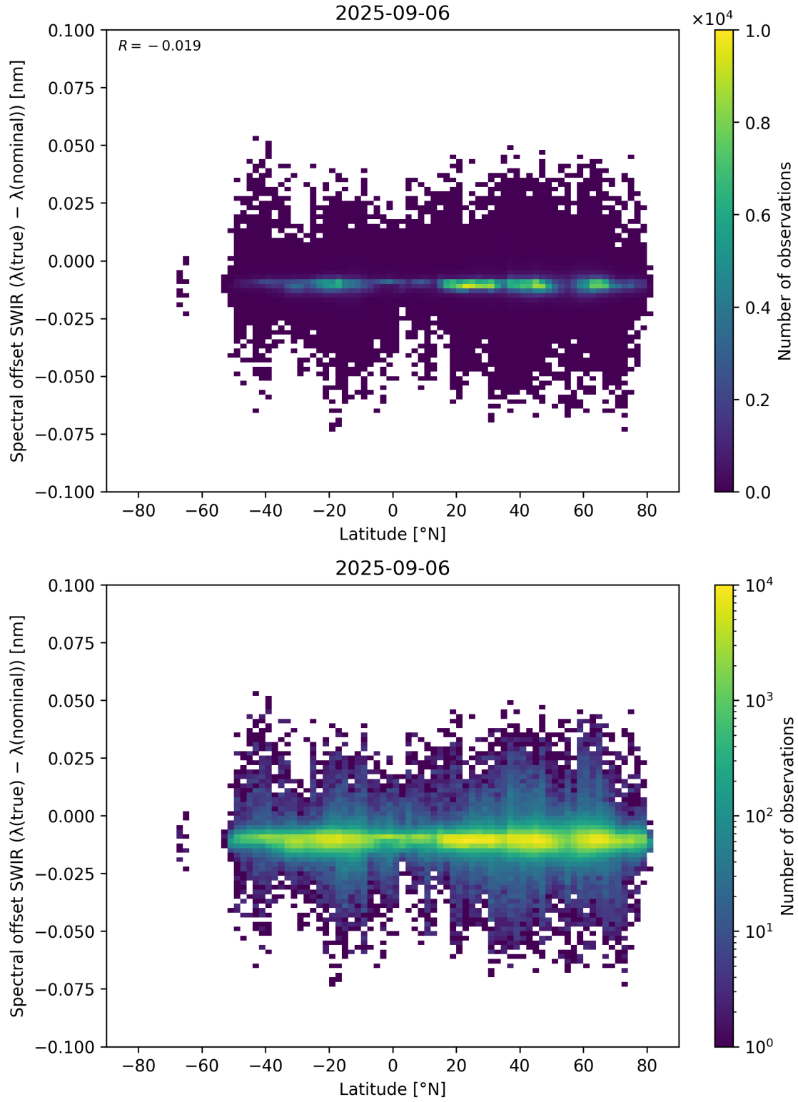
Figure 62: Scatter density plot of “Latitude” against “Spectral offset SWIR ( \lambda_{\text{true}} - \lambda_{\text{nominal}} )” for 2025-09-05 to 2025-09-07.
