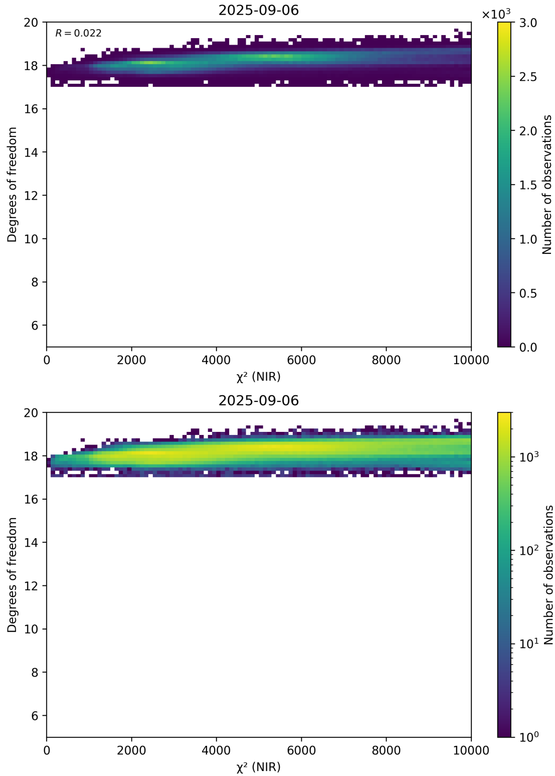
Figure 44: Scatter density plot of “ \chi^2 (NIR)” against “Degrees of freedom” for 2025-09-05 to 2025-09-07.
