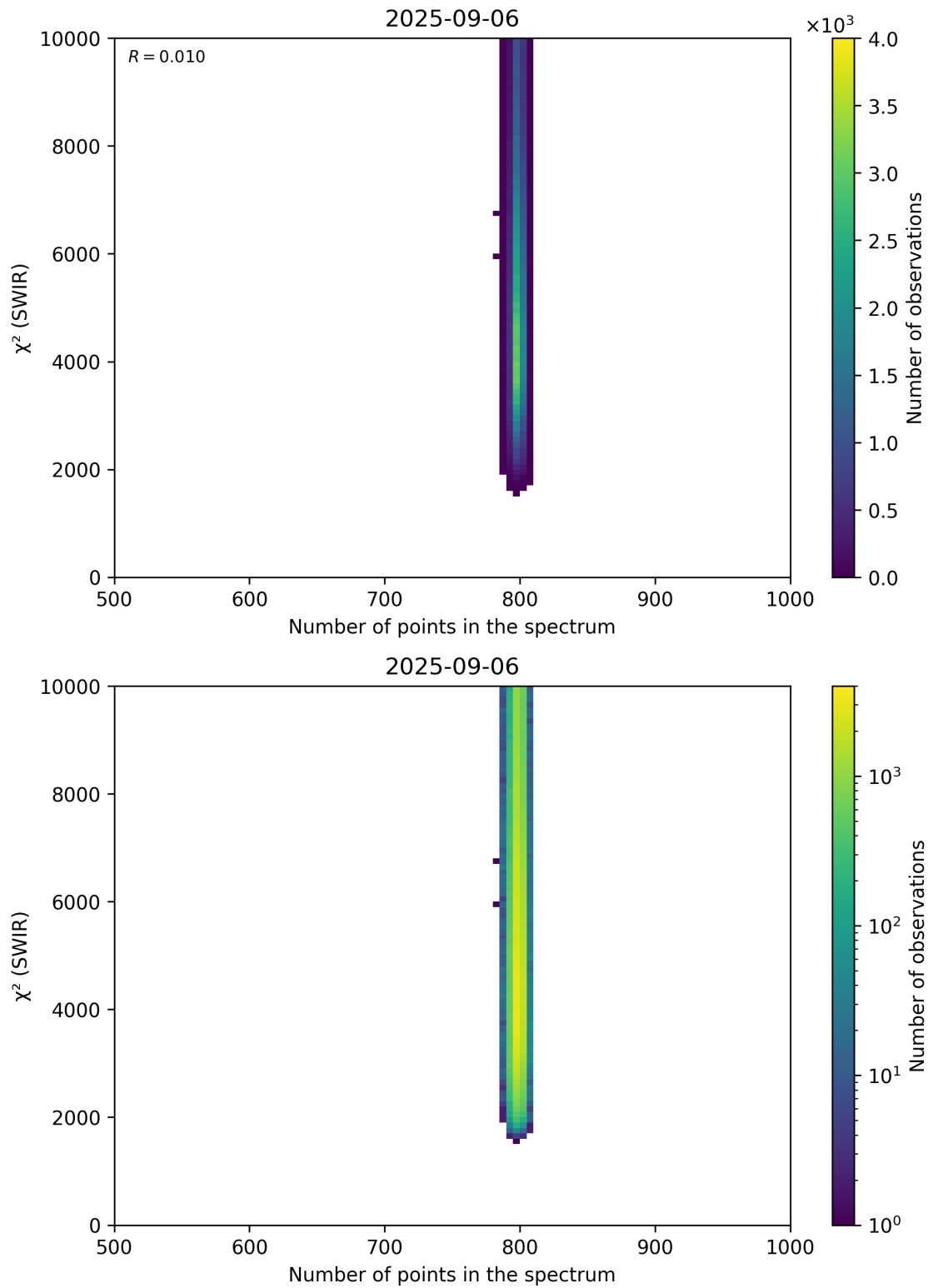
Figure 89: Scatter density plot of “Number of points in the spectrum” against “ \chi^2 (SWIR)” for 2025-09-05 to 2025-09-07.
