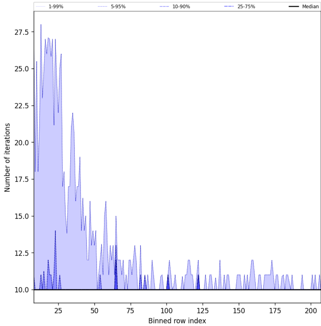
Figure 42: Along track statistics of “Number of iterations” for 2025-09-05 to 2025-09-07
