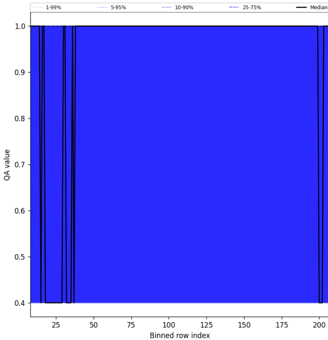
Figure 33: Along track statistics of “QA value” for 2025-09-05 to 2025-09-07
