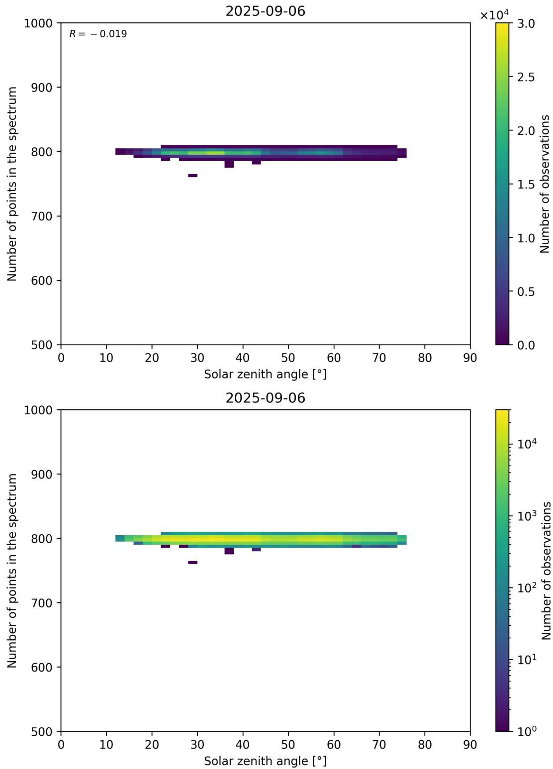
Figure 103: Scatter density plot of “Solar zenith angle” against “Number of points in the spectrum” for 2025-09-05 to 2025-09-07.
