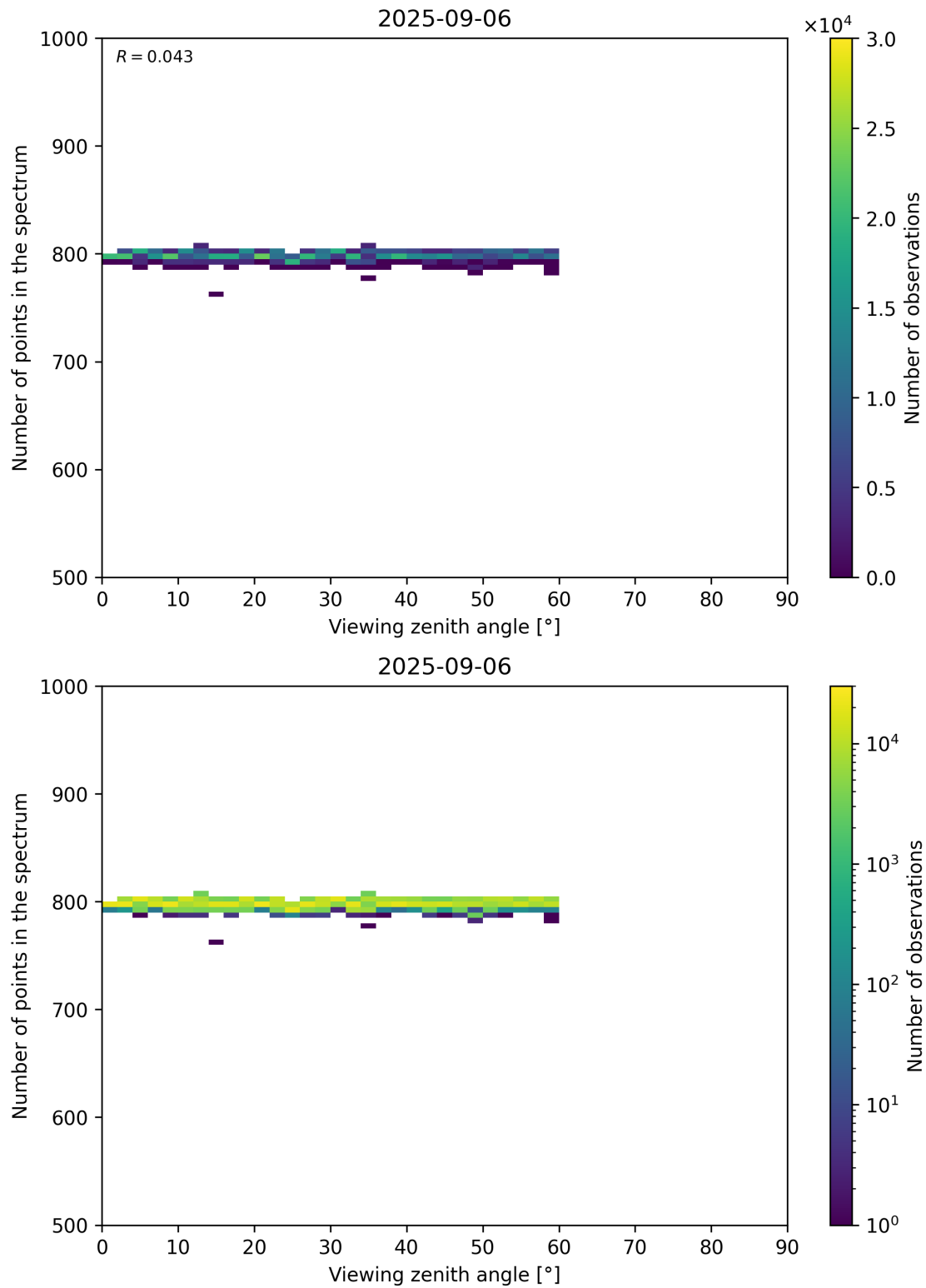
Figure 114: Scatter density plot of “Viewing zenith angle” against “Number of points in the spectrum” for 2025-09-05 to 2025-09-07.
