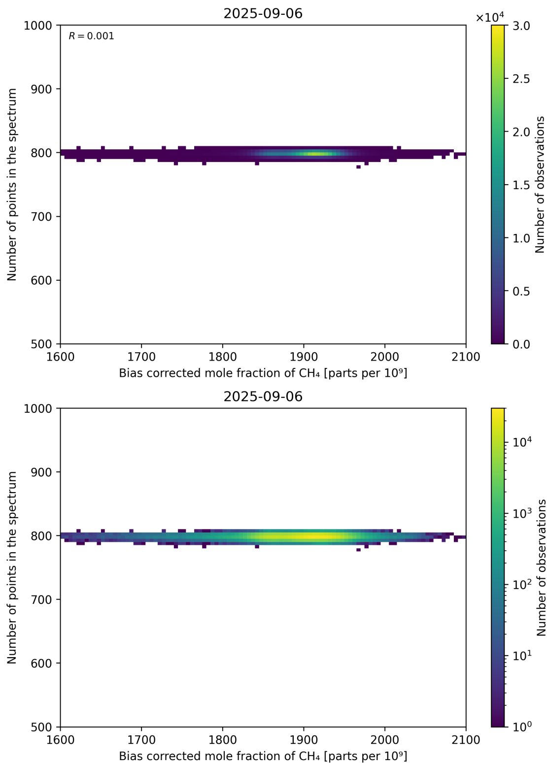
Figure 68: Scatter density plot of “Bias corrected mole fraction of CH 4 ” against “Number of points in the spectrum” for 2025-09-05 to 2025-09-07.
