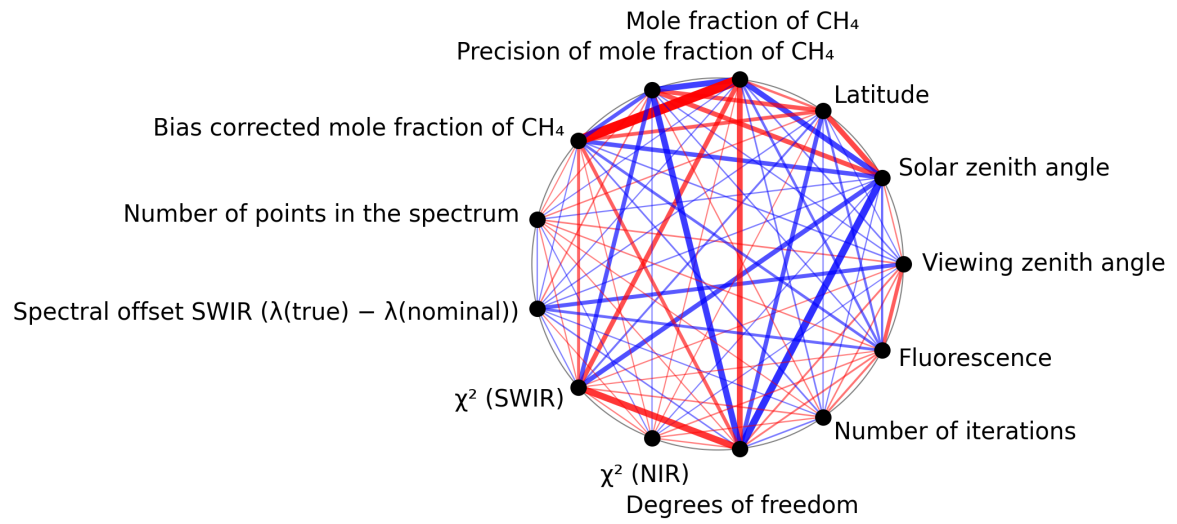
Figure 1: Map of correlation graph for 2025-09-05 to 2025-09-07.
