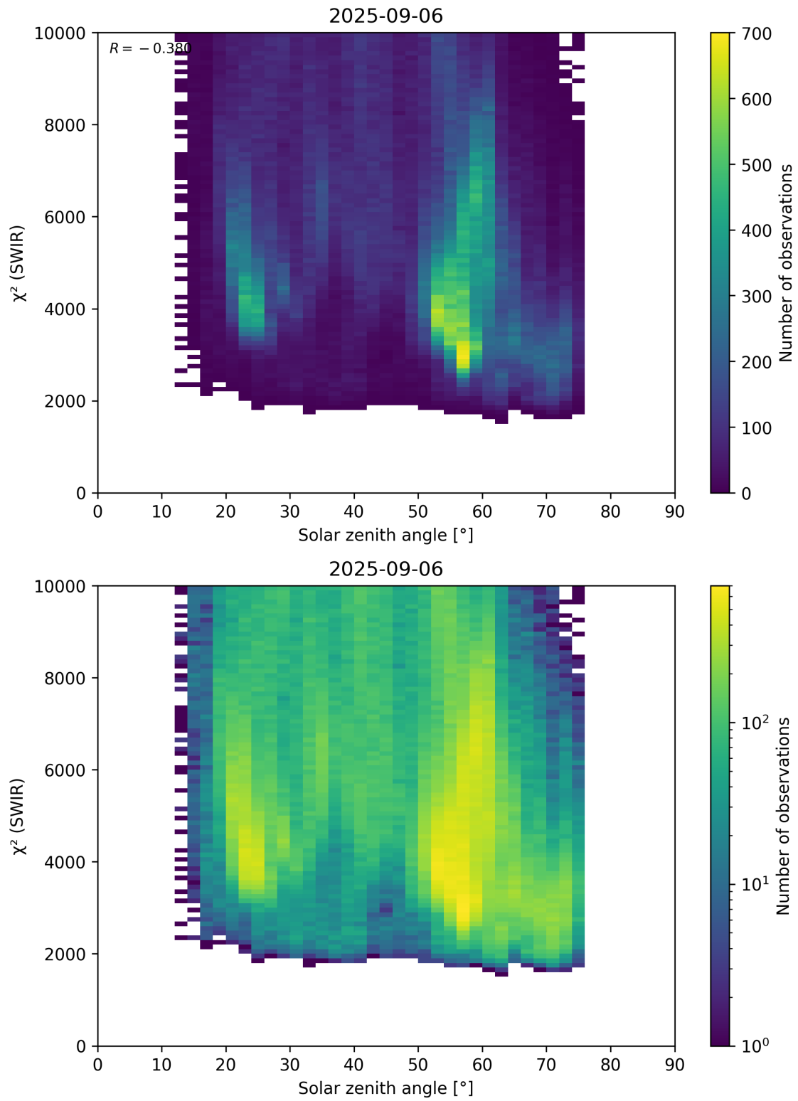
Figure 95: Scatter density plot of “Solar zenith angle” against “ \chi^2 (SWIR)” for 2025-09-05 to 2025-09-07.
