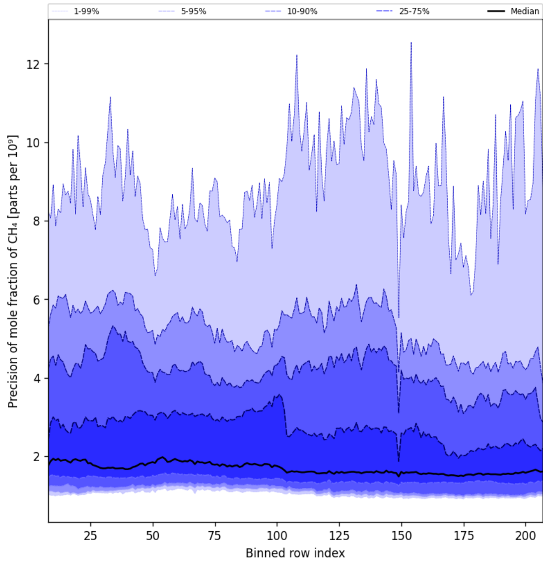
Figure 35: Along track statistics of “Precision of mole fraction of CH 4 ” for 2025-09-05 to 2025-09-07
