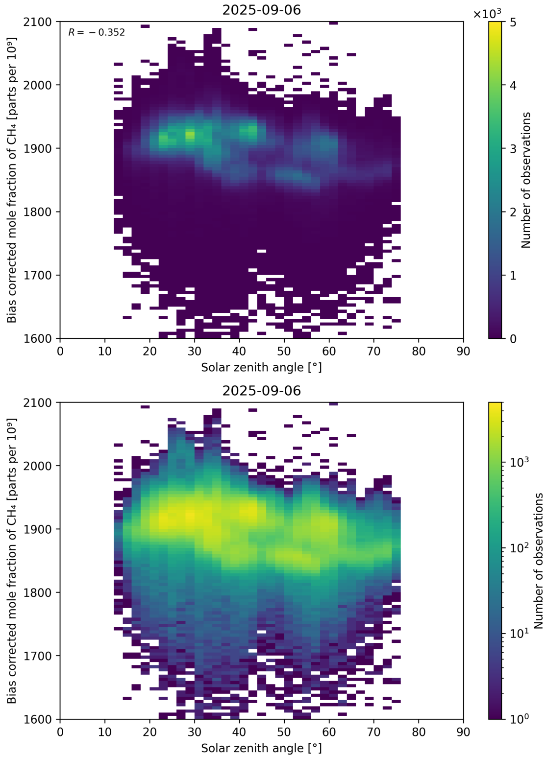
Figure 100: Scatter density plot of “Solar zenith angle” against “Bias corrected mole fraction of CH 4 ” for 2025-09-05 to 2025-09-07.
