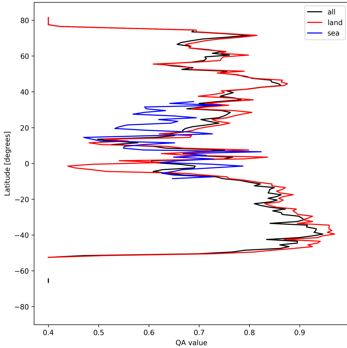
Figure 11: Zonal average of “QA value” for 2025-09-05 to 2025-09-07.
