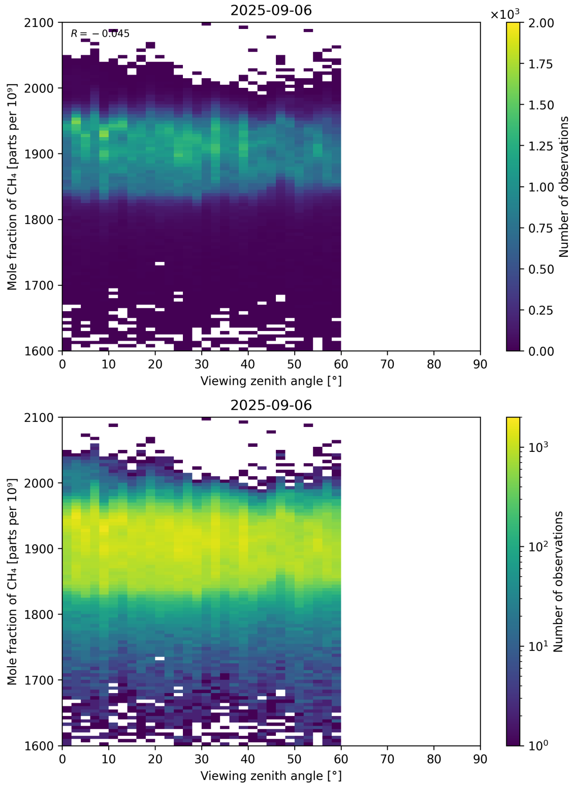
Figure 110: Scatter density plot of “Viewing zenith angle” against “Mole fraction of CH 4 ” for 2025-09-05 to 2025-09-07.
