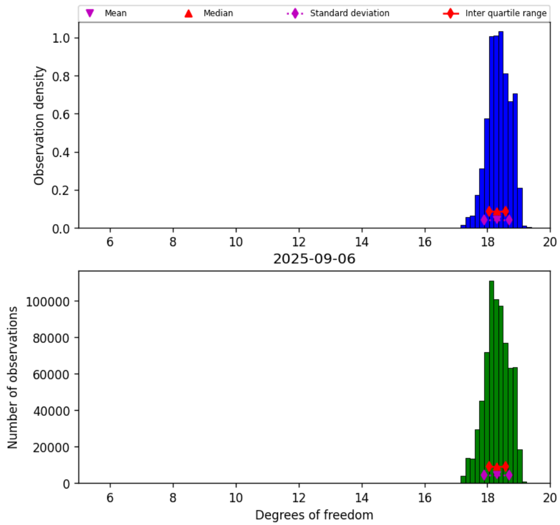
Figure 30: Histogram of “Degrees of freedom” for 2025-09-05 to 2025-09-07
