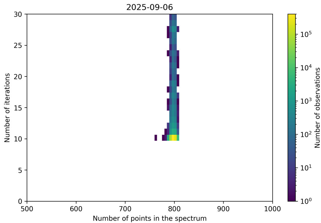
Figure 92: Scatter density plot of “Number of points in the spectrum” against “Number of iterations” for 2025-09-05 to 2025-09-07.
