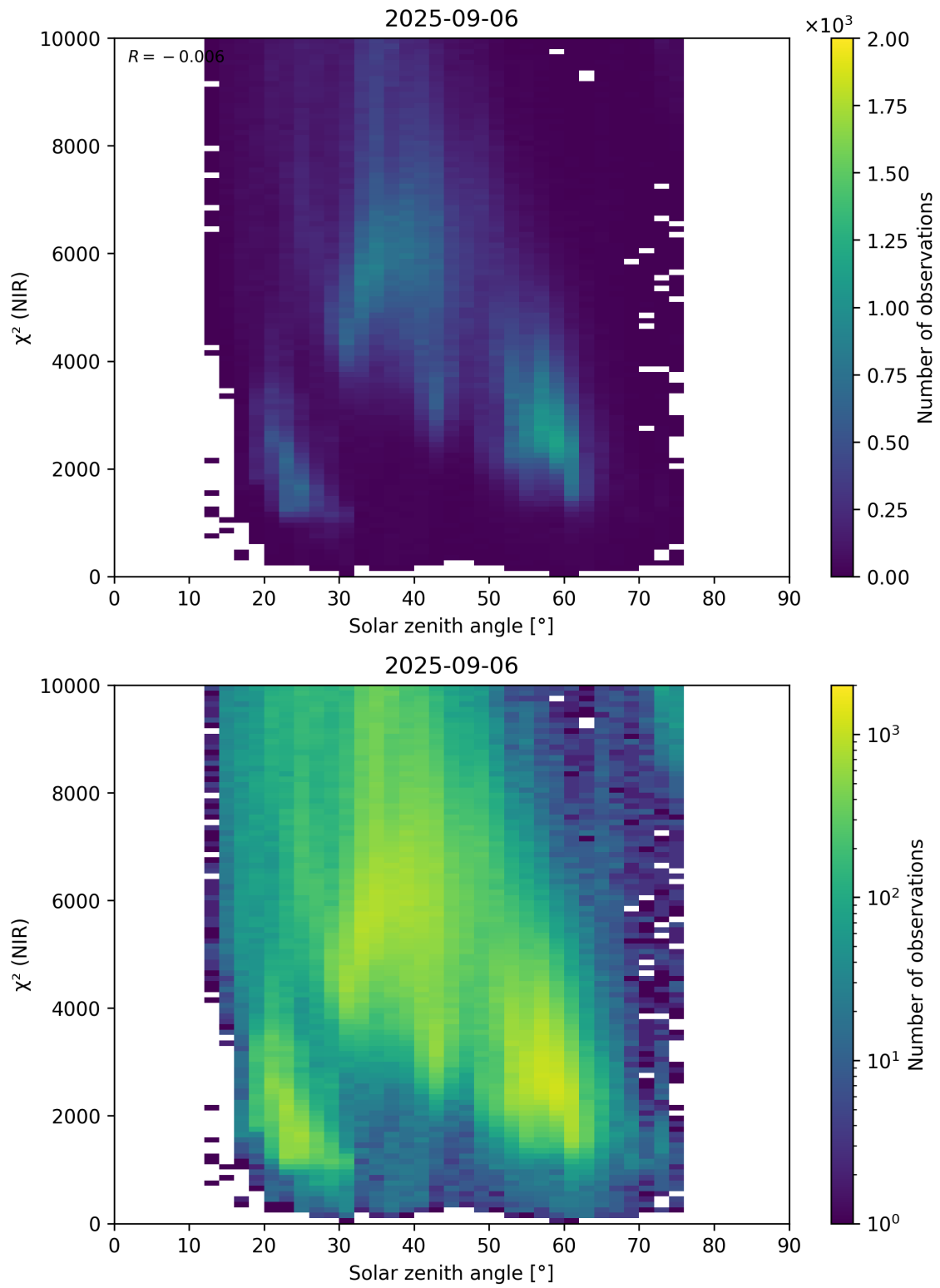
Figure 94: Scatter density plot of “Solar zenith angle” against “ \chi^2 (NIR)” for 2025-09-05 to 2025-09-07.
