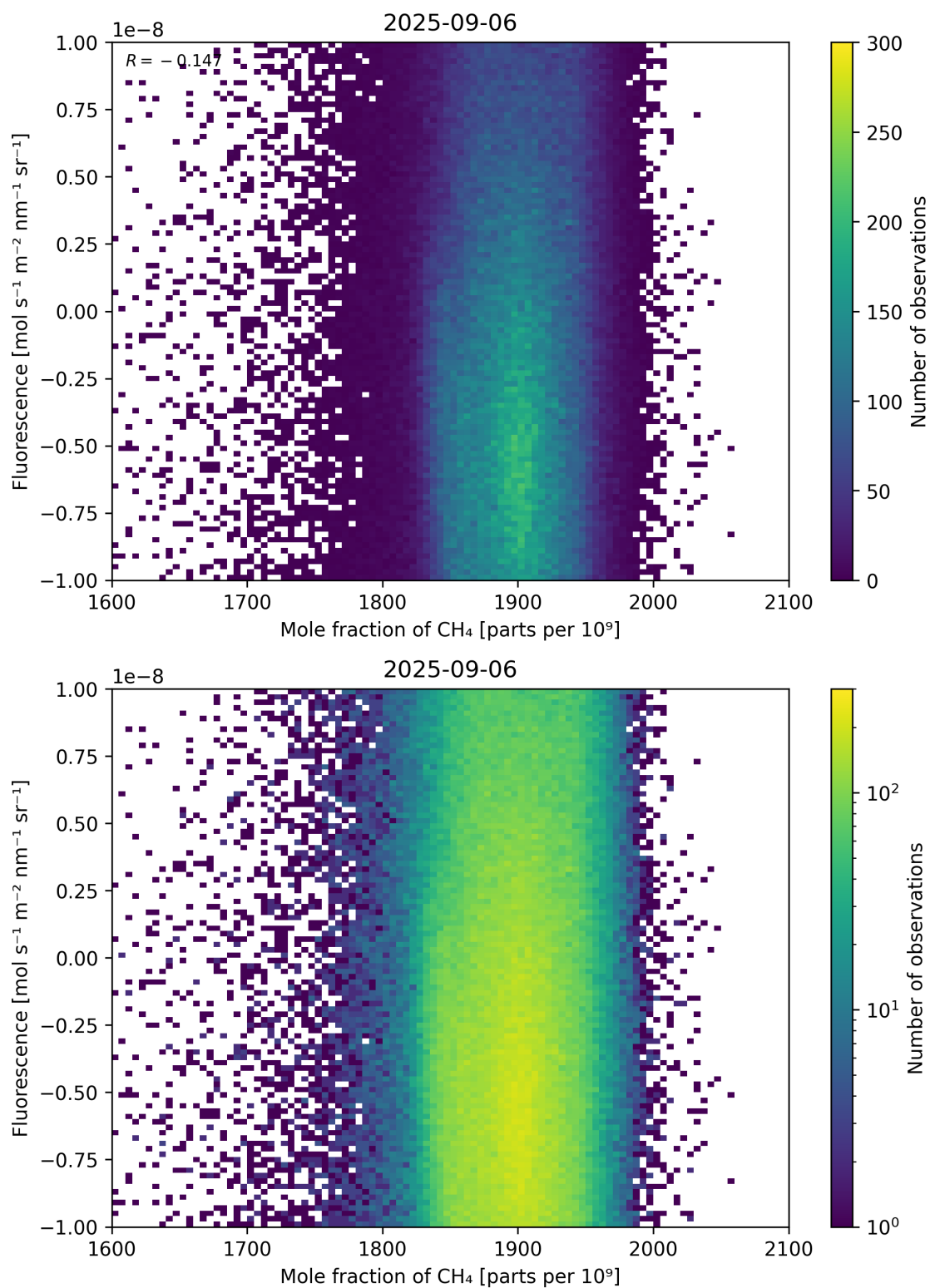
Figure 73: Scatter density plot of “Mole fraction of CH 4 ” against “Fluorescence” for 2025-09-05 to 2025-09-07.
