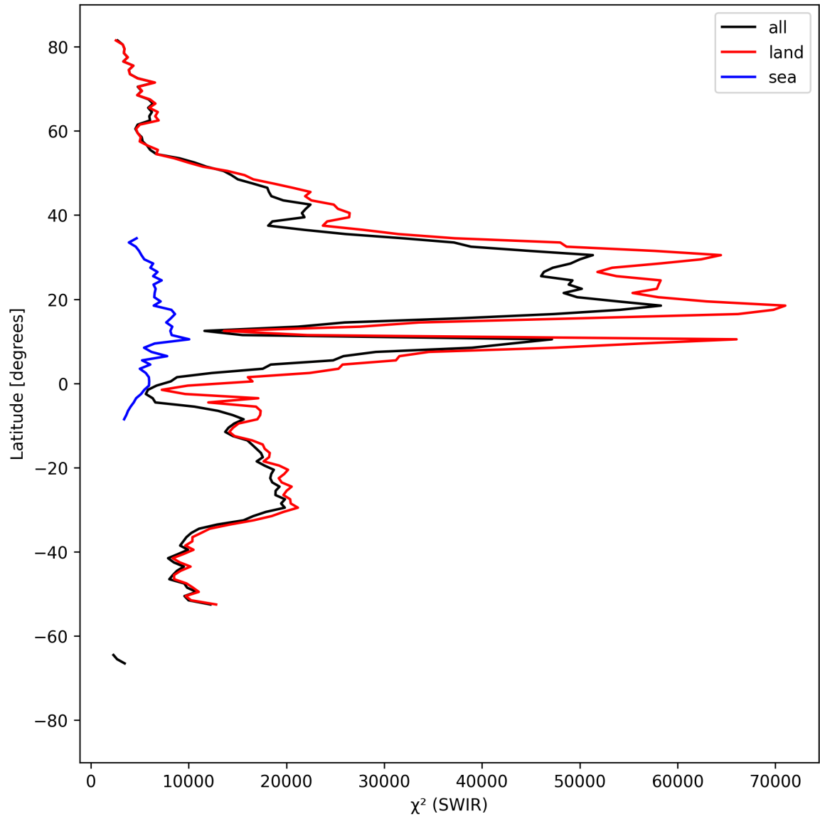
Figure 17: Zonal average of “ \chi^2 (SWIR)” for 2025-09-05 to 2025-09-07.
