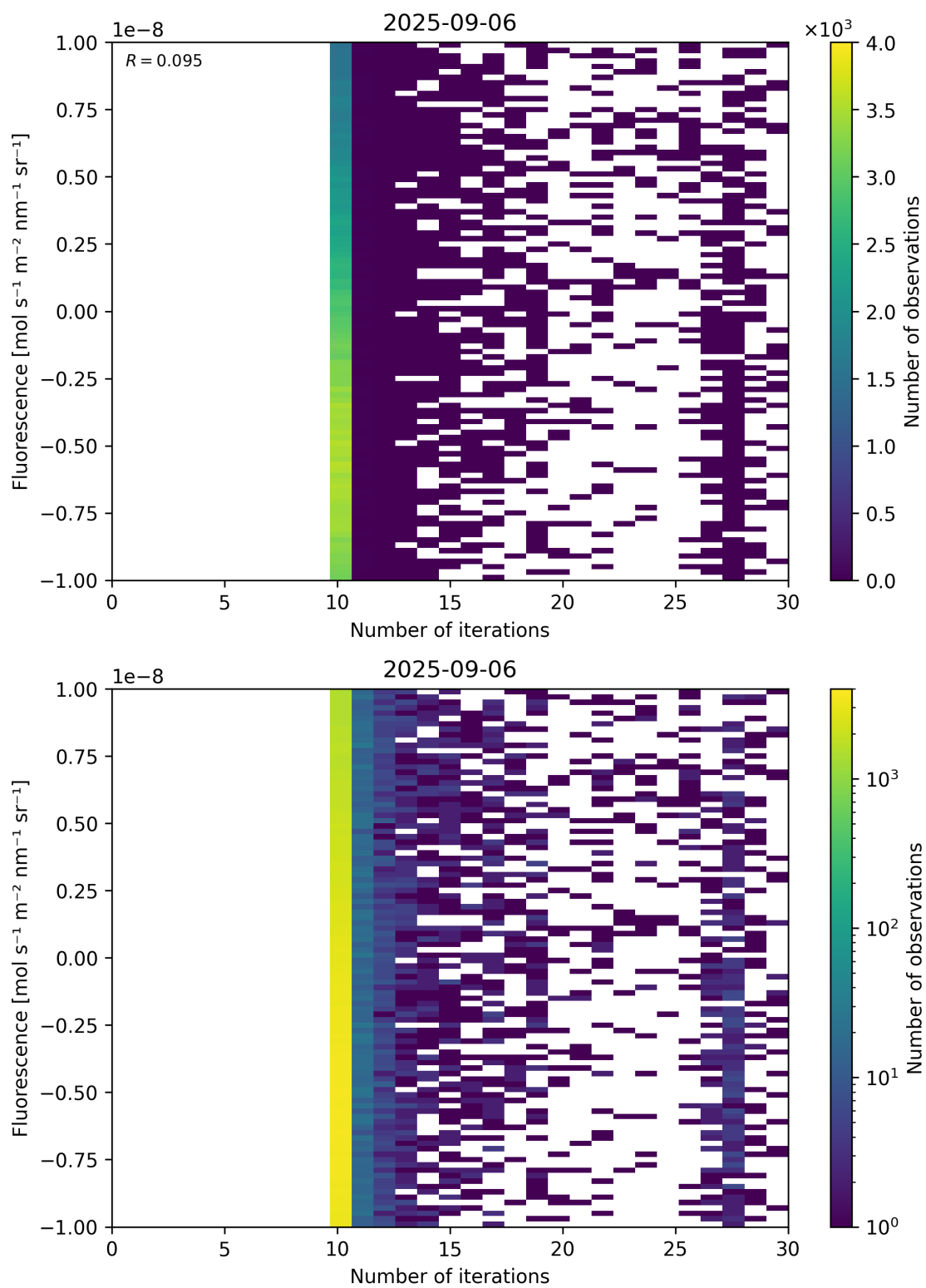
Figure 87: Scatter density plot of “Number of iterations” against “Fluorescence” for 2025-09-05 to 2025-09-07.
