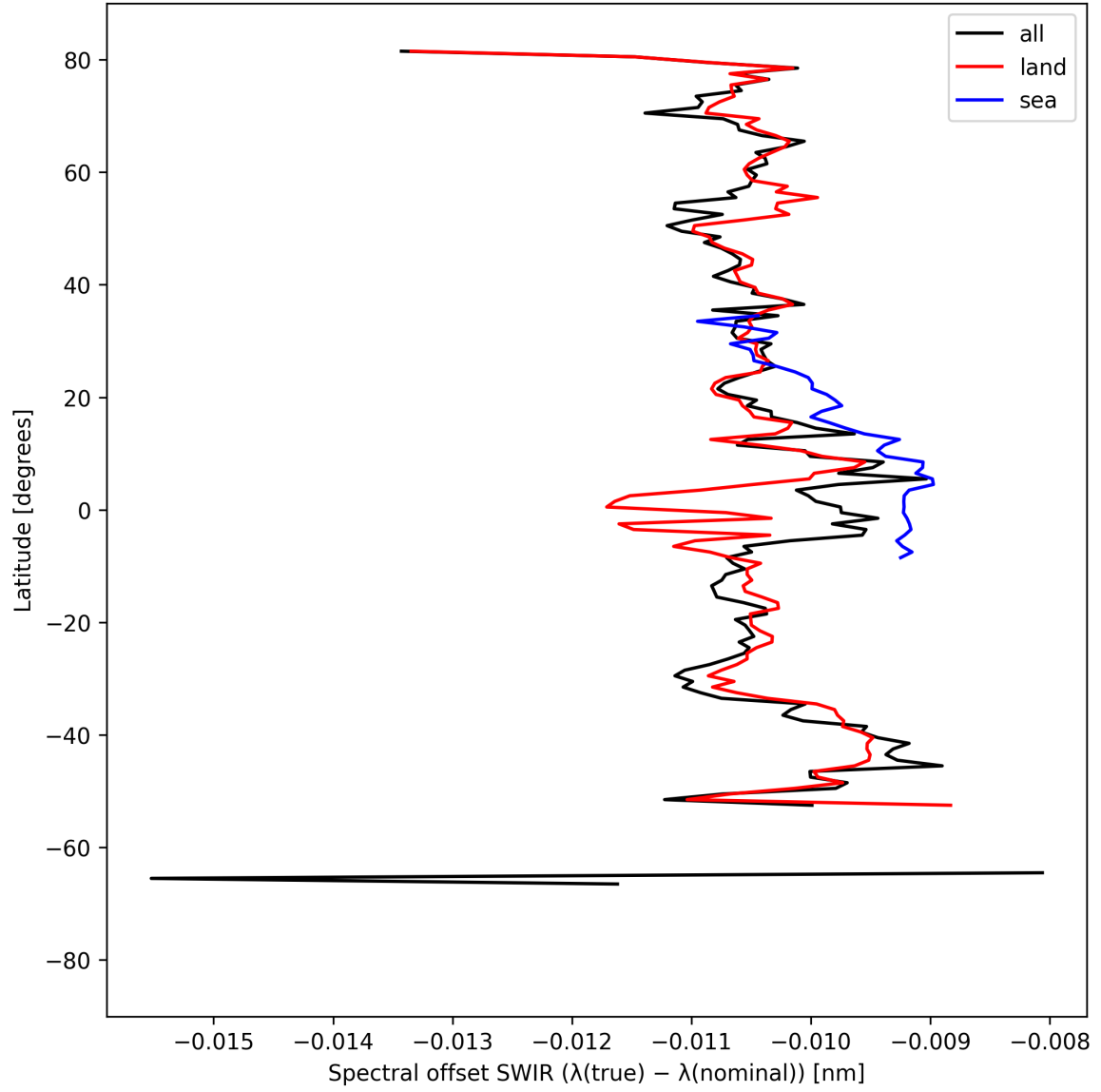
Figure 16: Zonal average of “Spectral offset SWIR ( \lambda_{\text{true}} - \lambda_{\text{nominal}} )” for 2025-09-05 to 2025-09-07.
