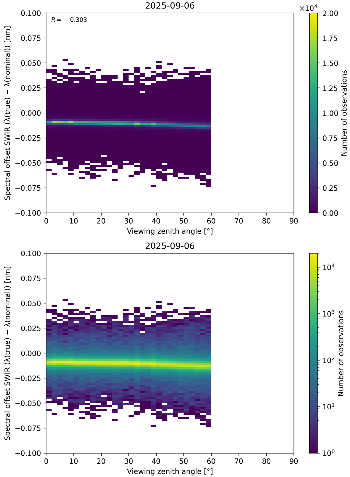
Figure 116: Scatter density plot of “Viewing zenith angle” against “Spectral offset SWIR ( \lambda_{\text{true}} - \lambda_{\text{nominal}} )” for 2025-09-05 to 2025-09-07.
