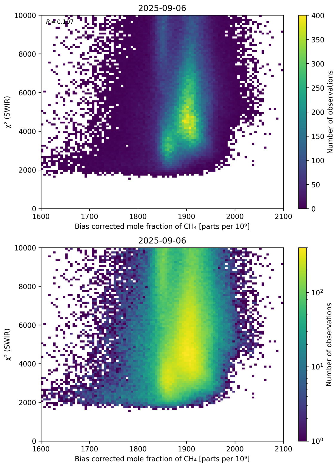
Figure 64: Scatter density plot of “Bias corrected mole fraction of \text{CH}_4 ” against “ \chi^2 (SWIR)” for 2025-09-05 to 2025-09-07.
