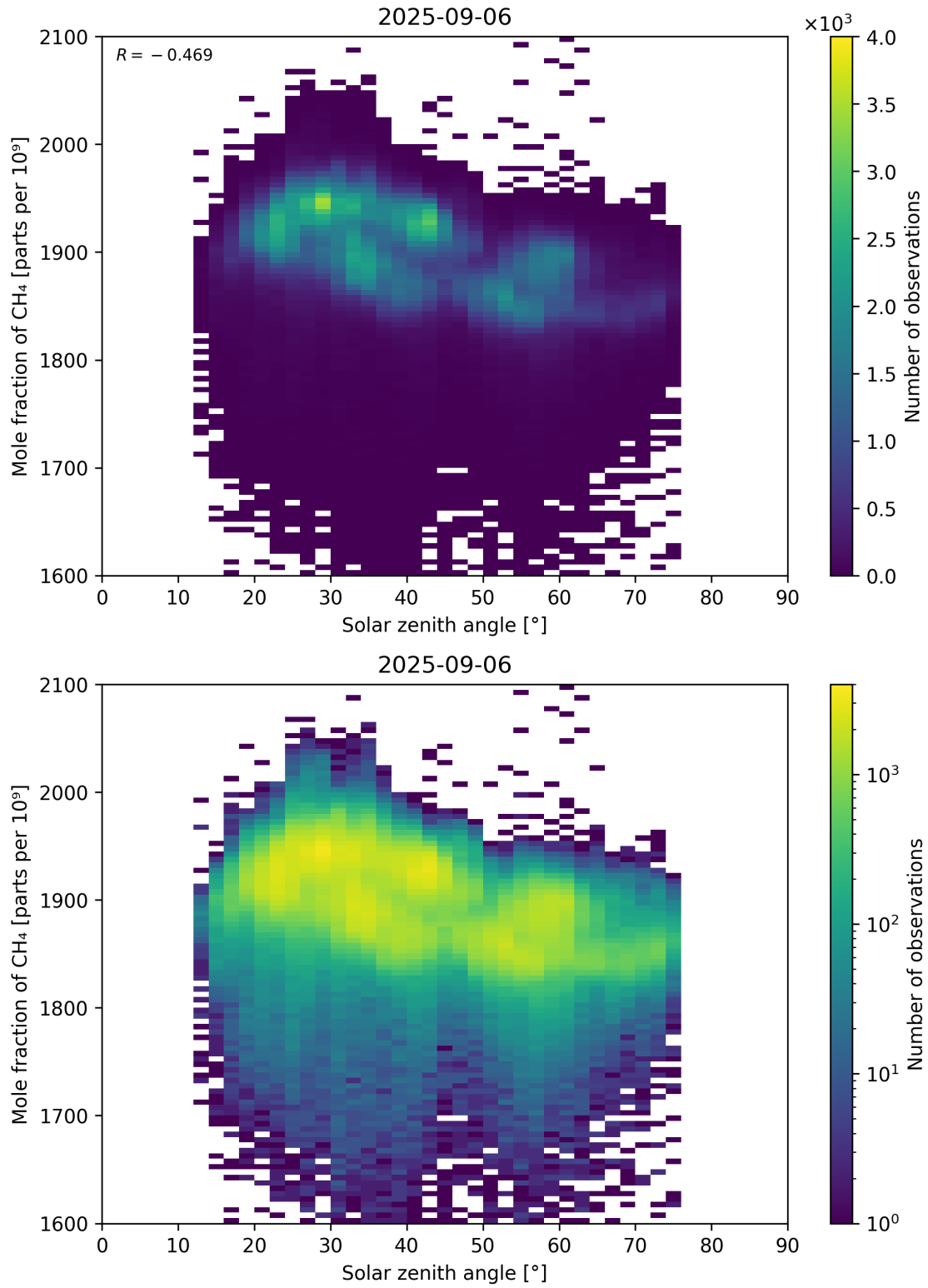
Figure 99: Scatter density plot of “Solar zenith angle” against “Mole fraction of CH 4 ” for 2025-09-05 to 2025-09-07.
