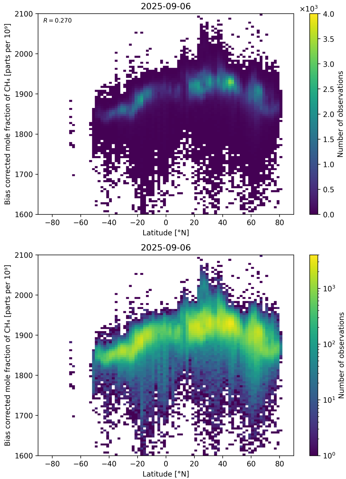
Figure 58: Scatter density plot of “Latitude” against “Bias corrected mole fraction of CH 4 ” for 2025-09-05 to 2025-09-07.
