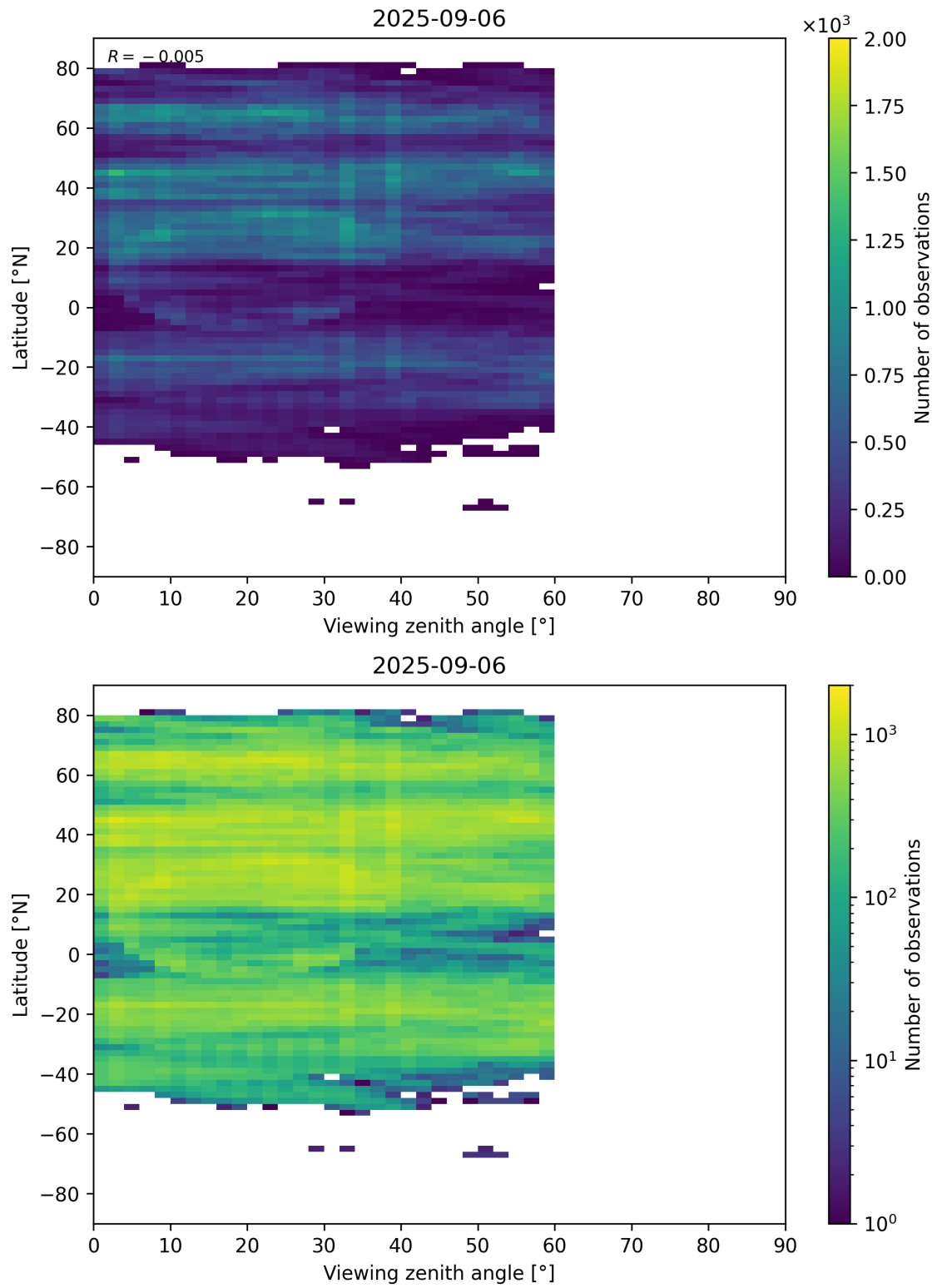
Figure 109: Scatter density plot of “Viewing zenith angle” against “Latitude” for 2025-09-05 to 2025-09-07.
