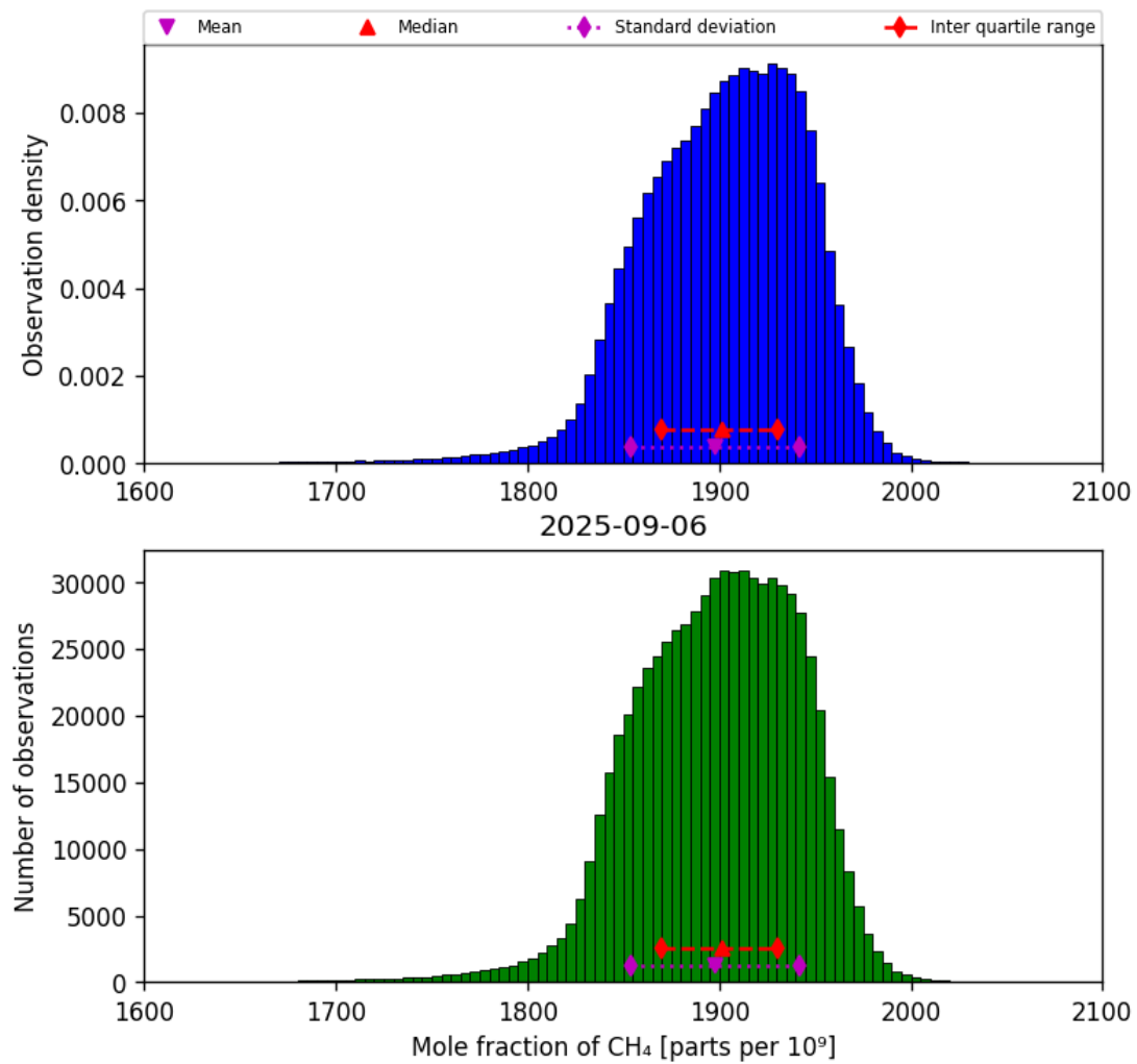
Figure 23: Histogram of “Mole fraction of CH 4 ” for 2025-09-05 to 2025-09-07
