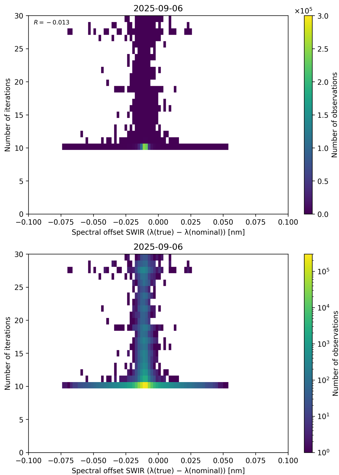
Figure 121: Scatter density plot of “Spectral offset SWIR ( \lambda_{\text{true}} - \lambda_{\text{nominal}} )” against “Number of iterations” for 2025-09-05 to 2025-09-07.
