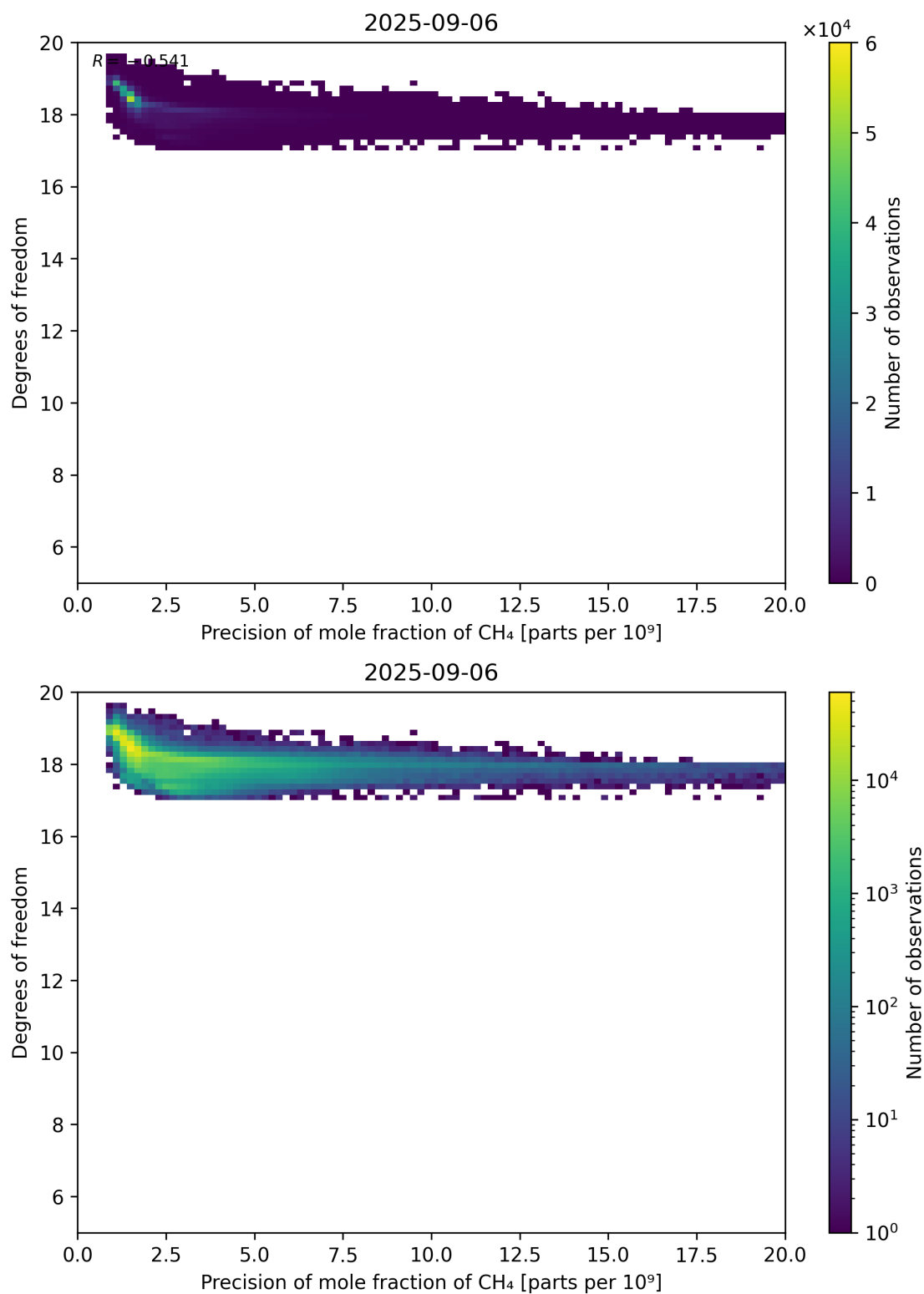
Figure 80: Scatter density plot of “Precision of mole fraction of CH 4 ” against “Degrees of freedom” for 2025-09-05 to 2025-09-07.
