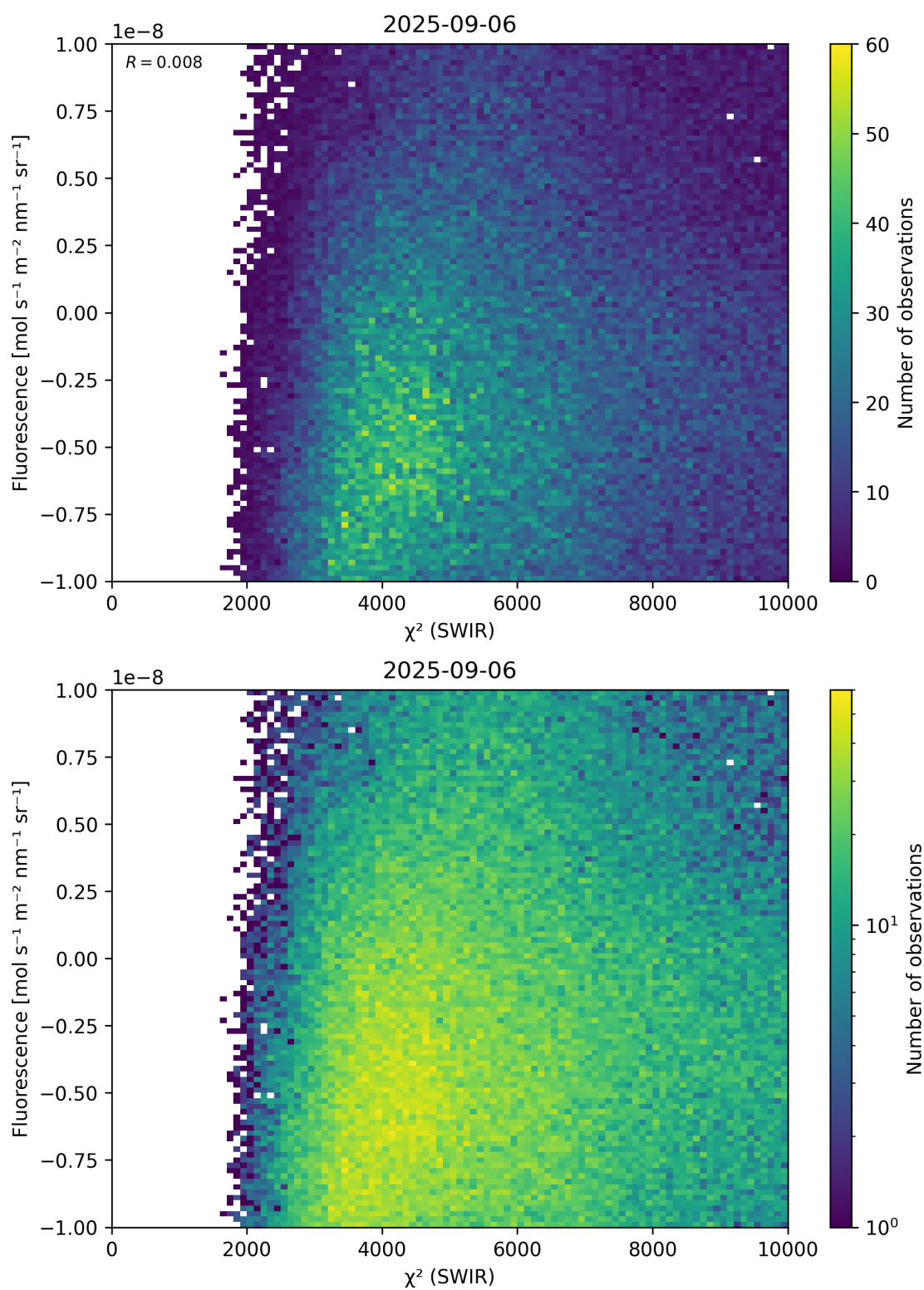
Figure 49: Scatter density plot of “ \chi^2 (SWIR)” against “Fluorescence” for 2025-09-05 to 2025-09-07.
