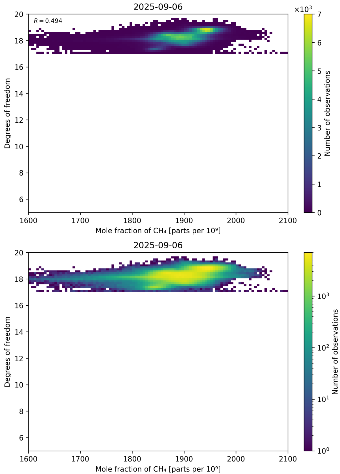
Figure 72: Scatter density plot of “Mole fraction of CH 4 ” against “Degrees of freedom” for 2025-09-05 to 2025-09-07.
