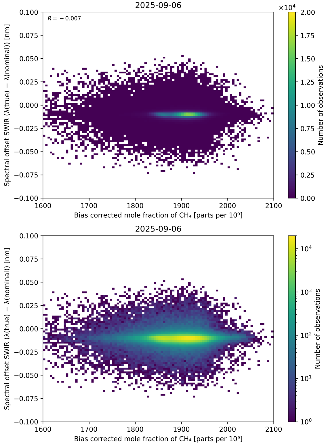
Figure 69: Scatter density plot of “Bias corrected mole fraction of \text{CH}_4 ” against “Spectral offset SWIR ( \lambda_{\text{true}} - \lambda_{\text{nominal}} )” for 2025-09-05 to 2025-09-07.
