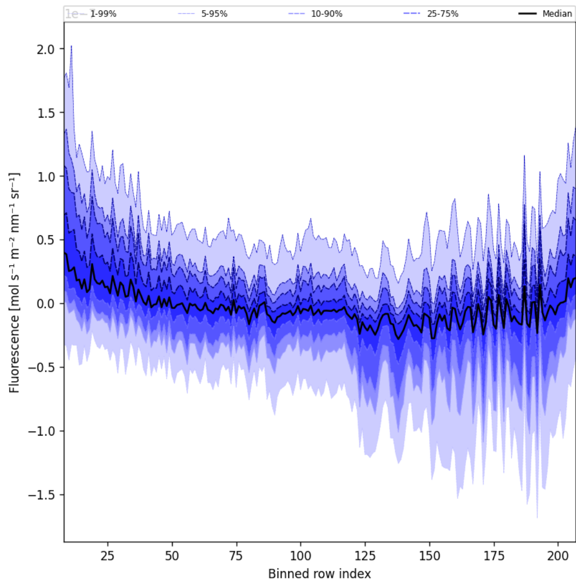
Figure 43: Along track statistics of "Fluorescence" for 2025-09-05 to 2025-09-07
