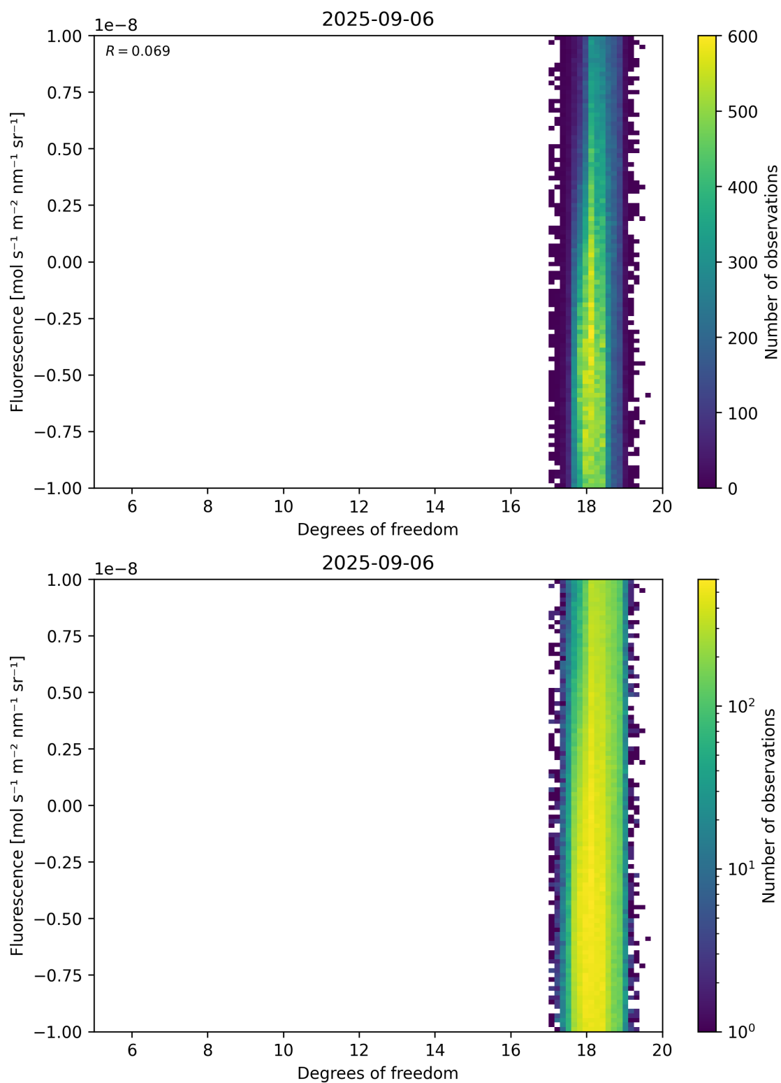
Figure 51: Scatter density plot of “Degrees of freedom” against “Fluorescence” for 2025-09-05 to 2025-09-07.
