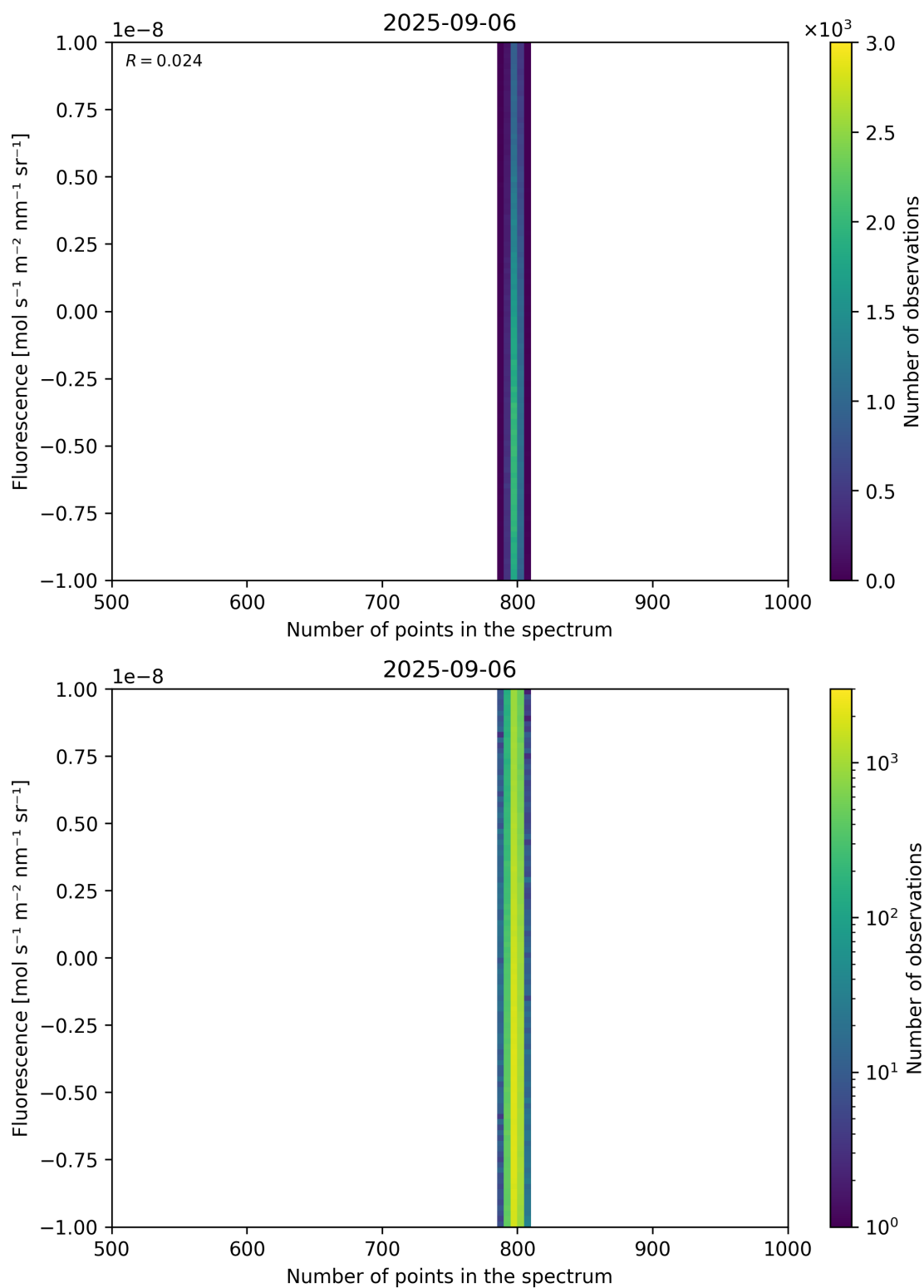
Figure 91: Scatter density plot of “Number of points in the spectrum” against “Fluorescence” for 2025-09-05 to 2025-09-07.
