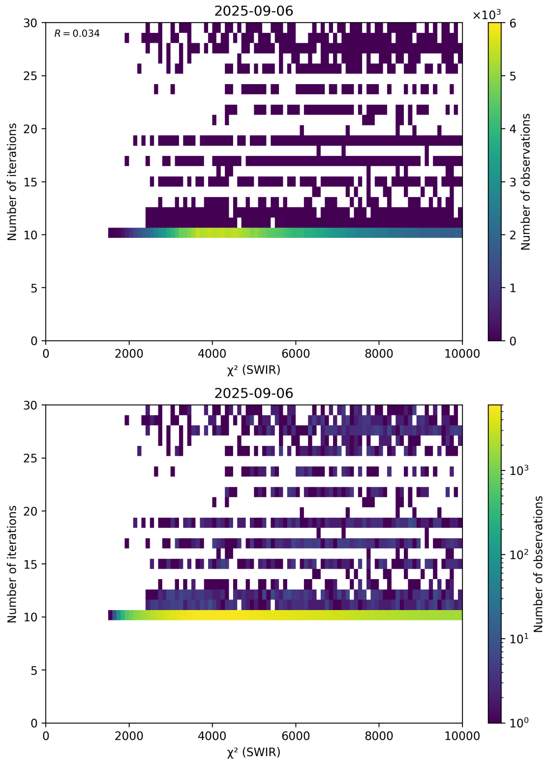
Figure 50: Scatter density plot of “ \chi^2 (SWIR)” against “Number of iterations” for 2025-09-05 to 2025-09-07.
