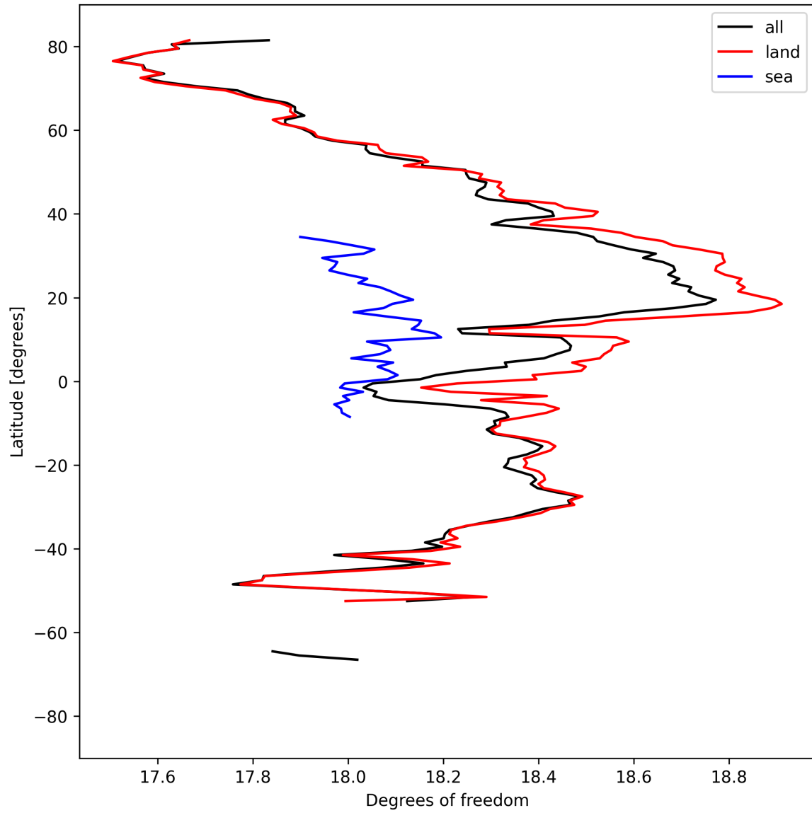
Figure 19: Zonal average of “Degrees of freedom” for 2025-09-05 to 2025-09-07.
