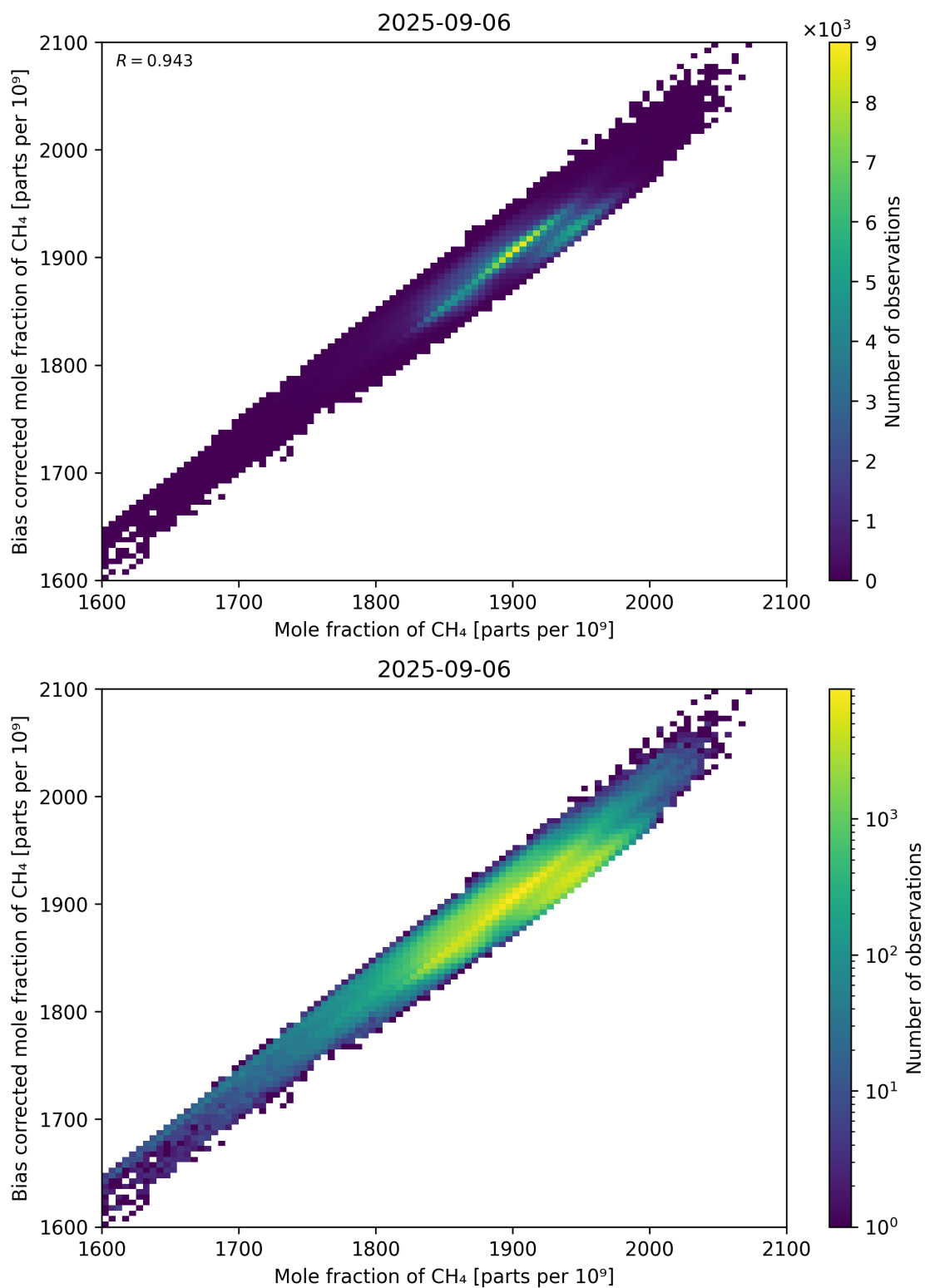
Figure 74: Scatter density plot of “Mole fraction of CH 4 ” against “Bias corrected mole fraction of CH 4 ” for 2025-09-05 to 2025-09-07.
