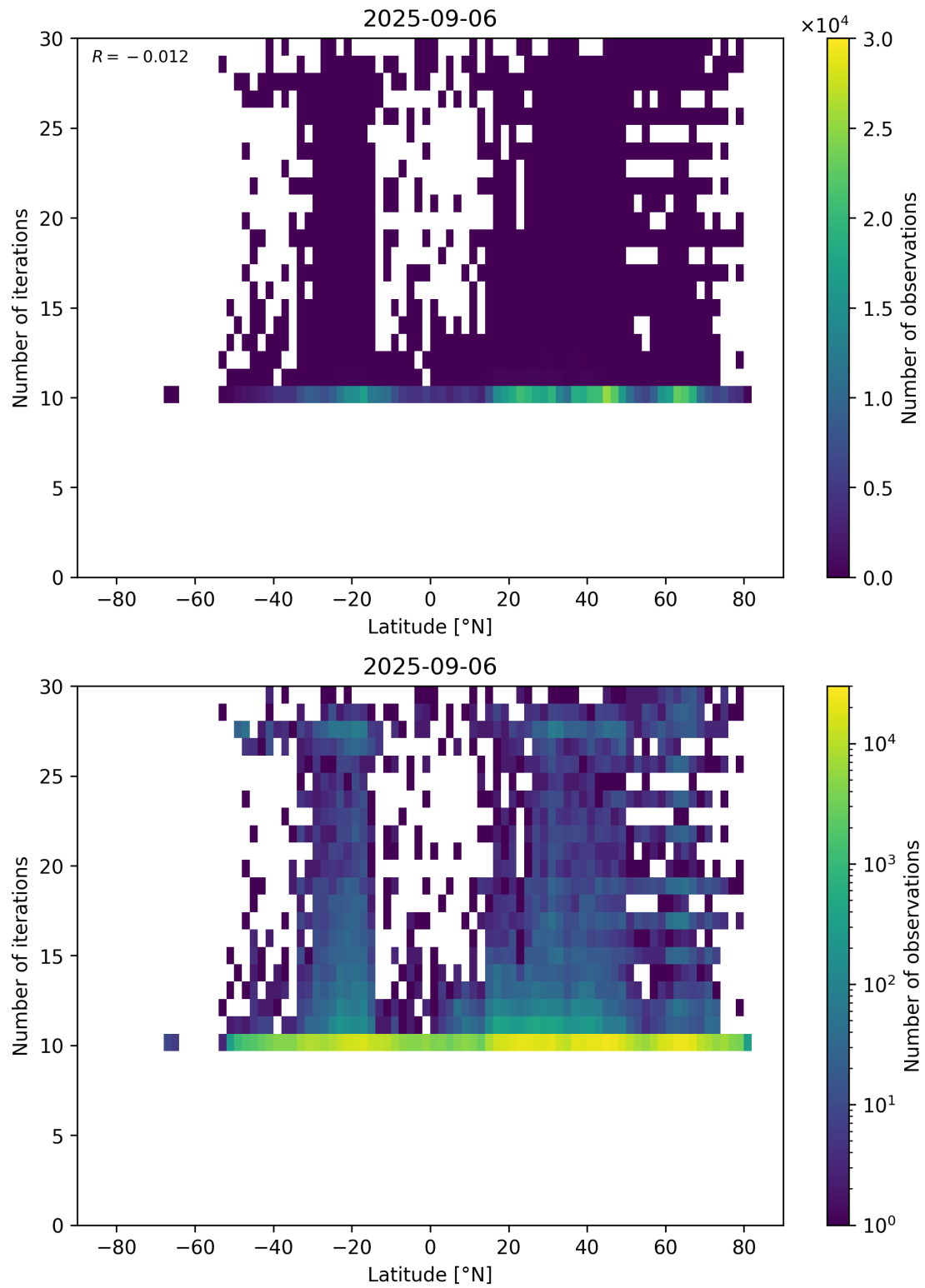
Figure 60: Scatter density plot of “Latitude” against “Number of iterations” for 2025-09-05 to 2025-09-07.
