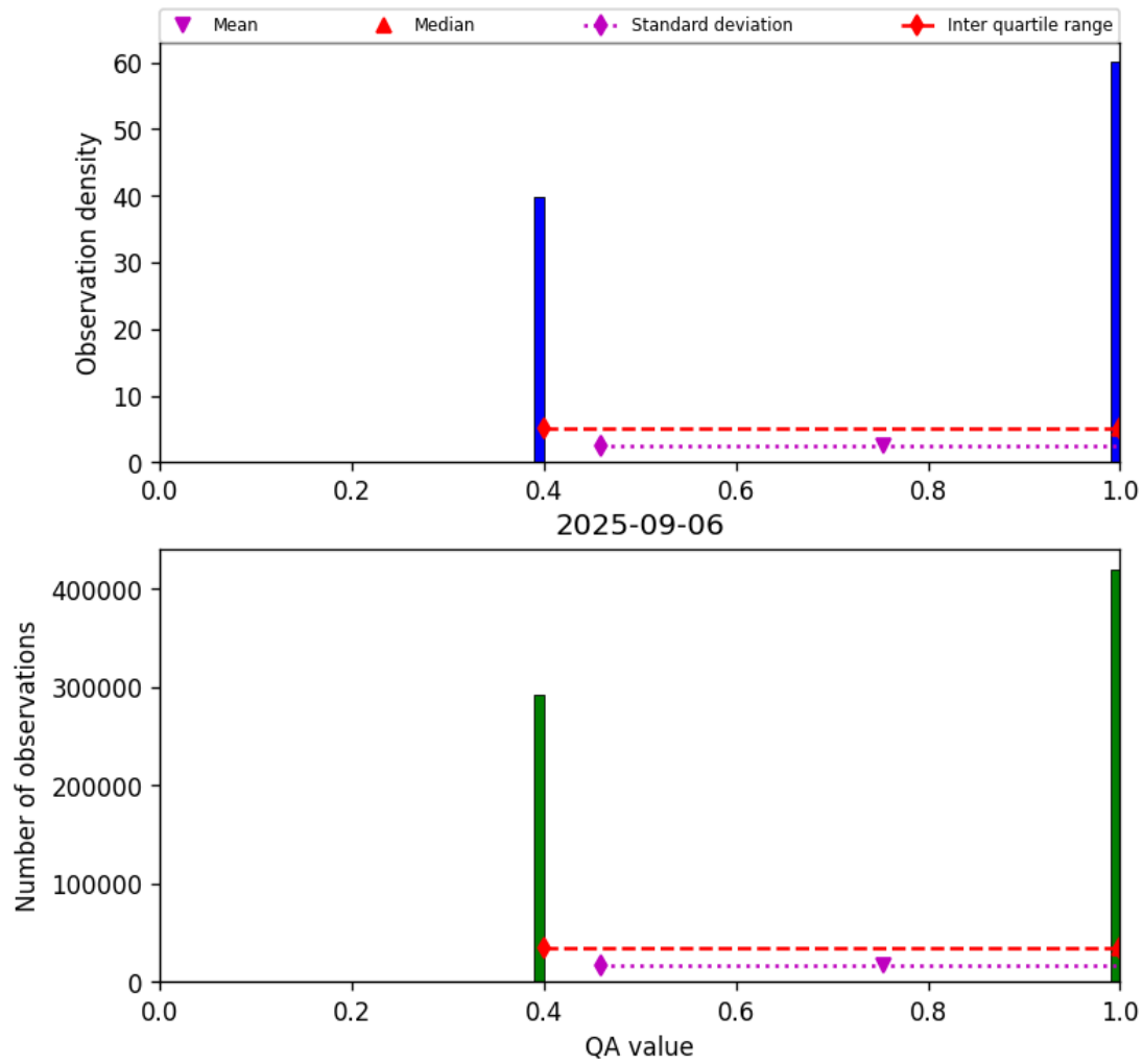
Figure 22: Histogram of “QA value” for 2025-09-05 to 2025-09-07
