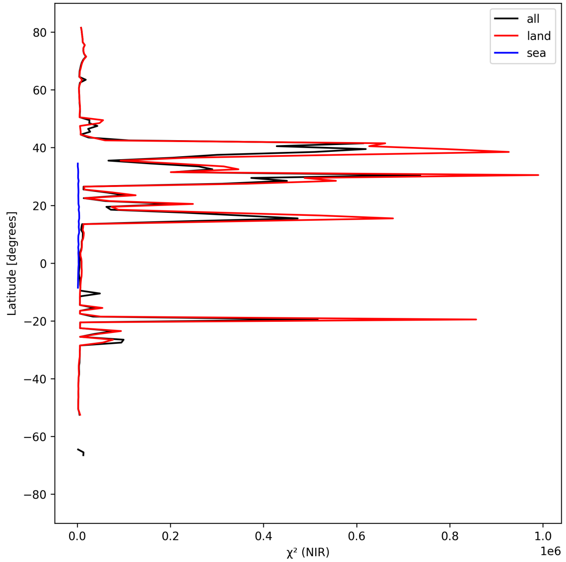
Figure 18: Zonal average of “ \chi^2 (NIR)” for 2025-09-05 to 2025-09-07.
