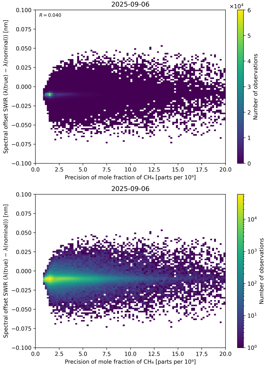
Figure 85: Scatter density plot of “Precision of mole fraction of \text{CH}_4 ” against “Spectral offset SWIR ( \lambda_{\text{true}} - \lambda_{\text{nominal}} )” for 2025-09-05 to 2025-09-07.
