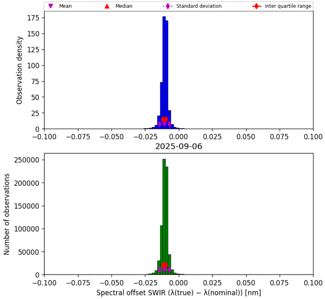
Figure 27: Histogram of “Spectral offset SWIR ( \lambda_{\text{true}} - \lambda_{\text{nominal}} )” for 2025-09-05 to 2025-09-07
