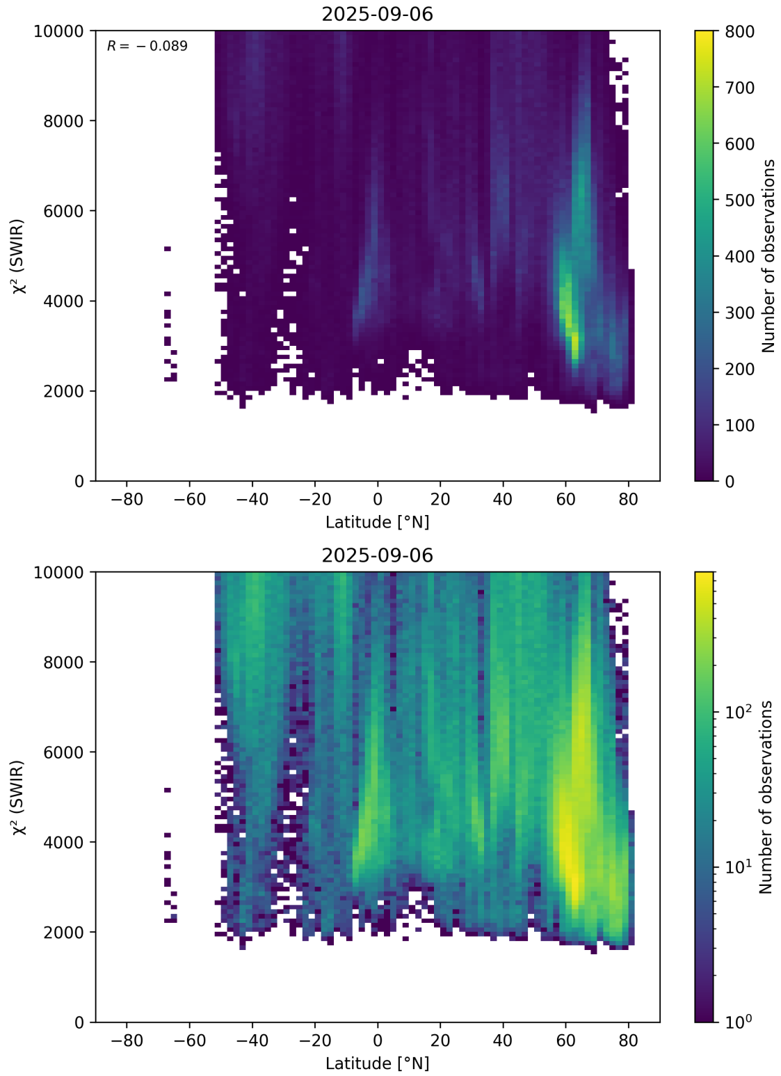
Figure 54: Scatter density plot of “Latitude” against “ \chi^2 (SWIR)” for 2025-09-05 to 2025-09-07.
