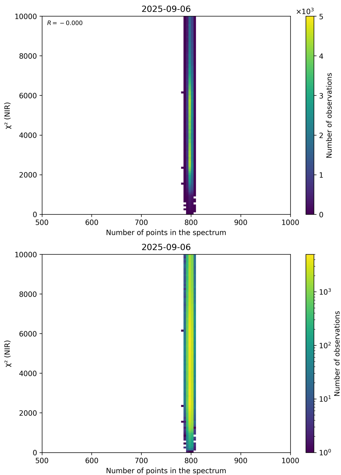
Figure 88: Scatter density plot of “Number of points in the spectrum” against “ \chi^2 (NIR)” for 2025-09-05 to 2025-09-07.
