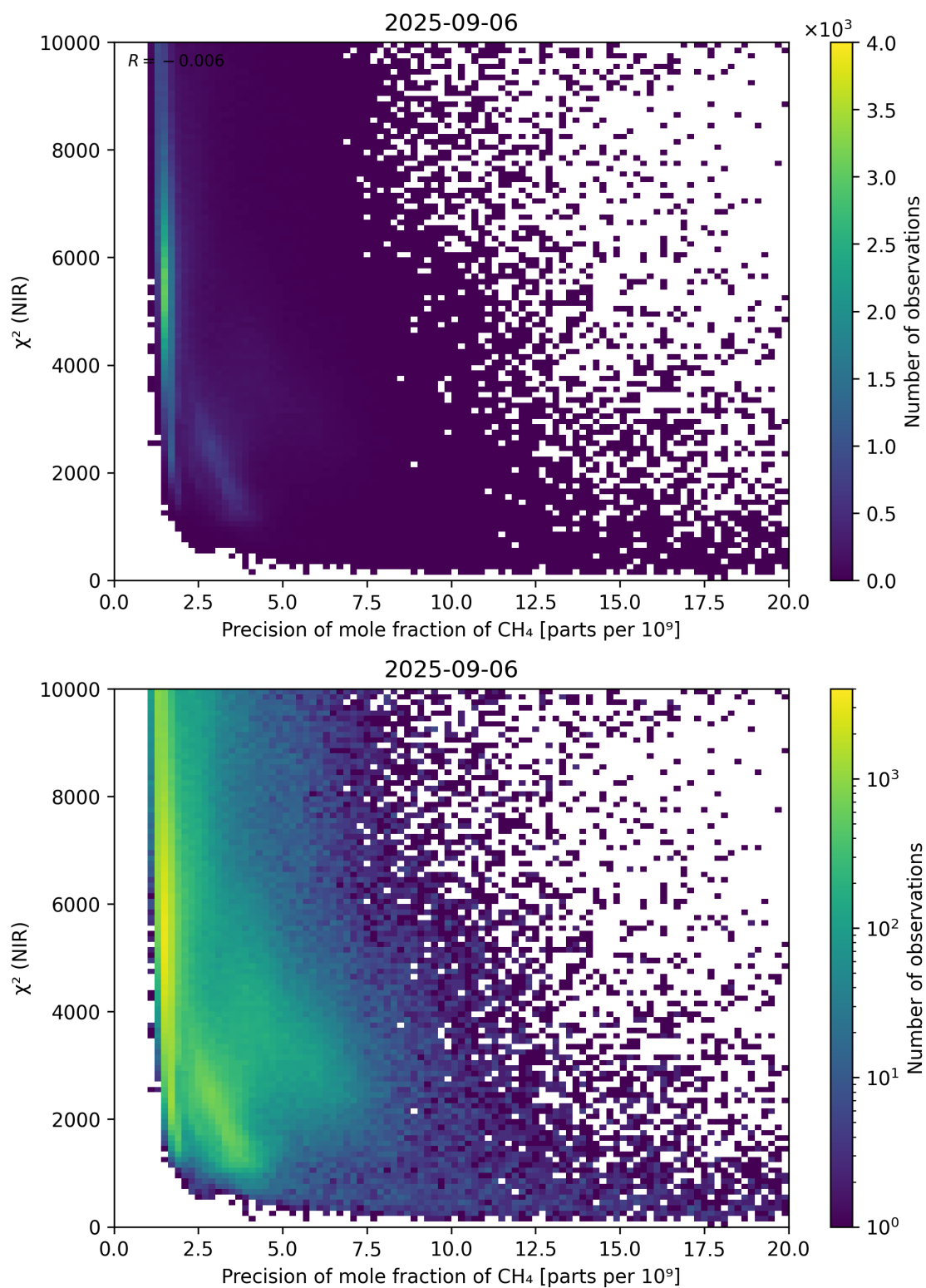
Figure 78: Scatter density plot of “Precision of mole fraction of CH 4 ” against “ \chi^2 (NIR)” for 2025-09-05 to 2025-09-07.
