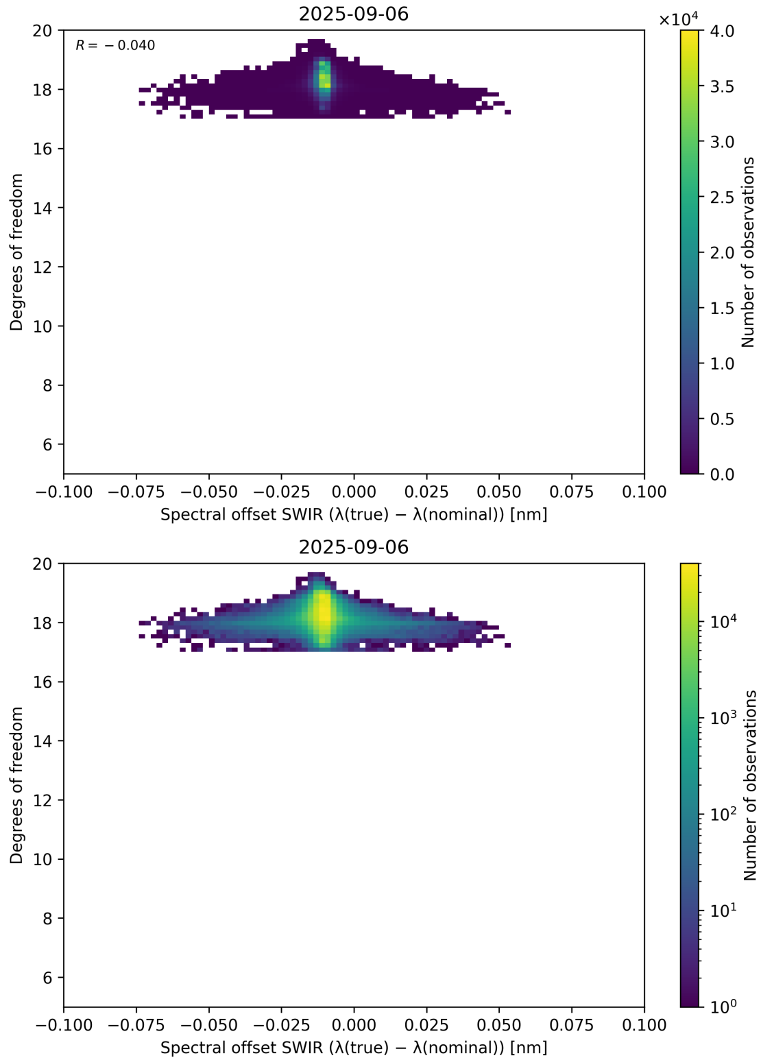
Figure 119: Scatter density plot of “Spectral offset SWIR ( \lambda_{\text{true}} - \lambda_{\text{nominal}} )” against “Degrees of freedom” for 2025-09-05 to 2025-09-07.
