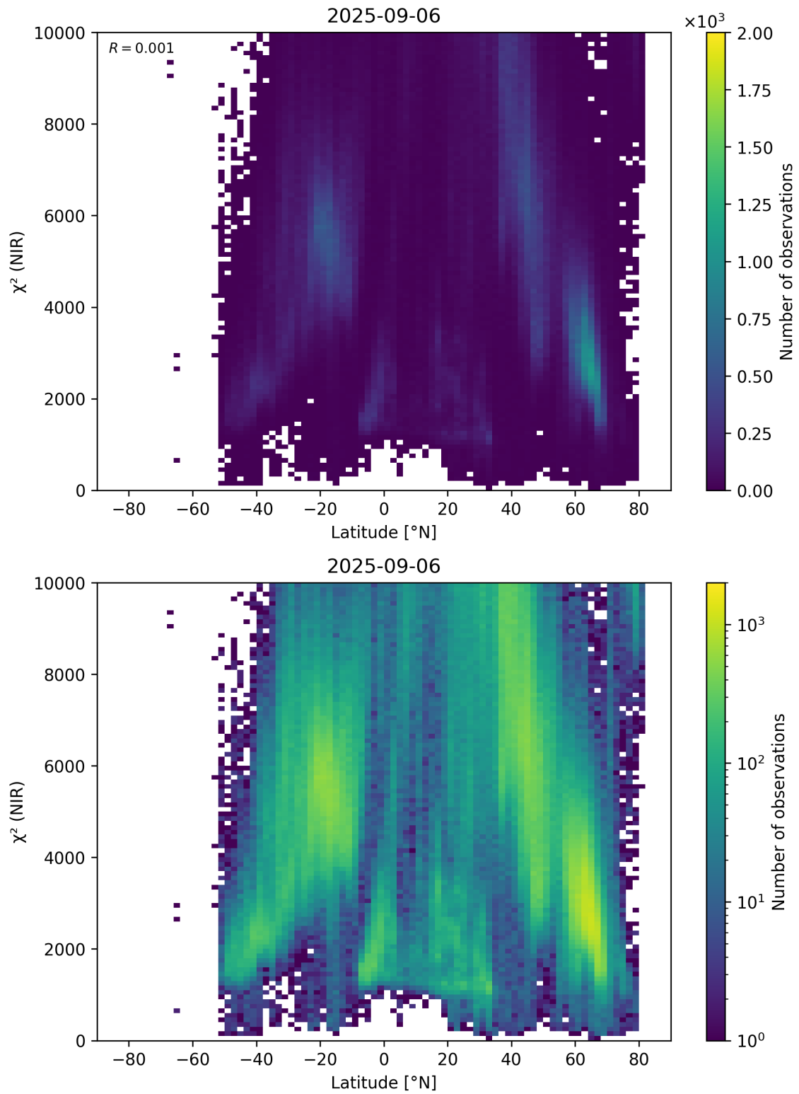
Figure 53: Scatter density plot of “Latitude” against “ \chi^2 (NIR)” for 2025-09-05 to 2025-09-07.
