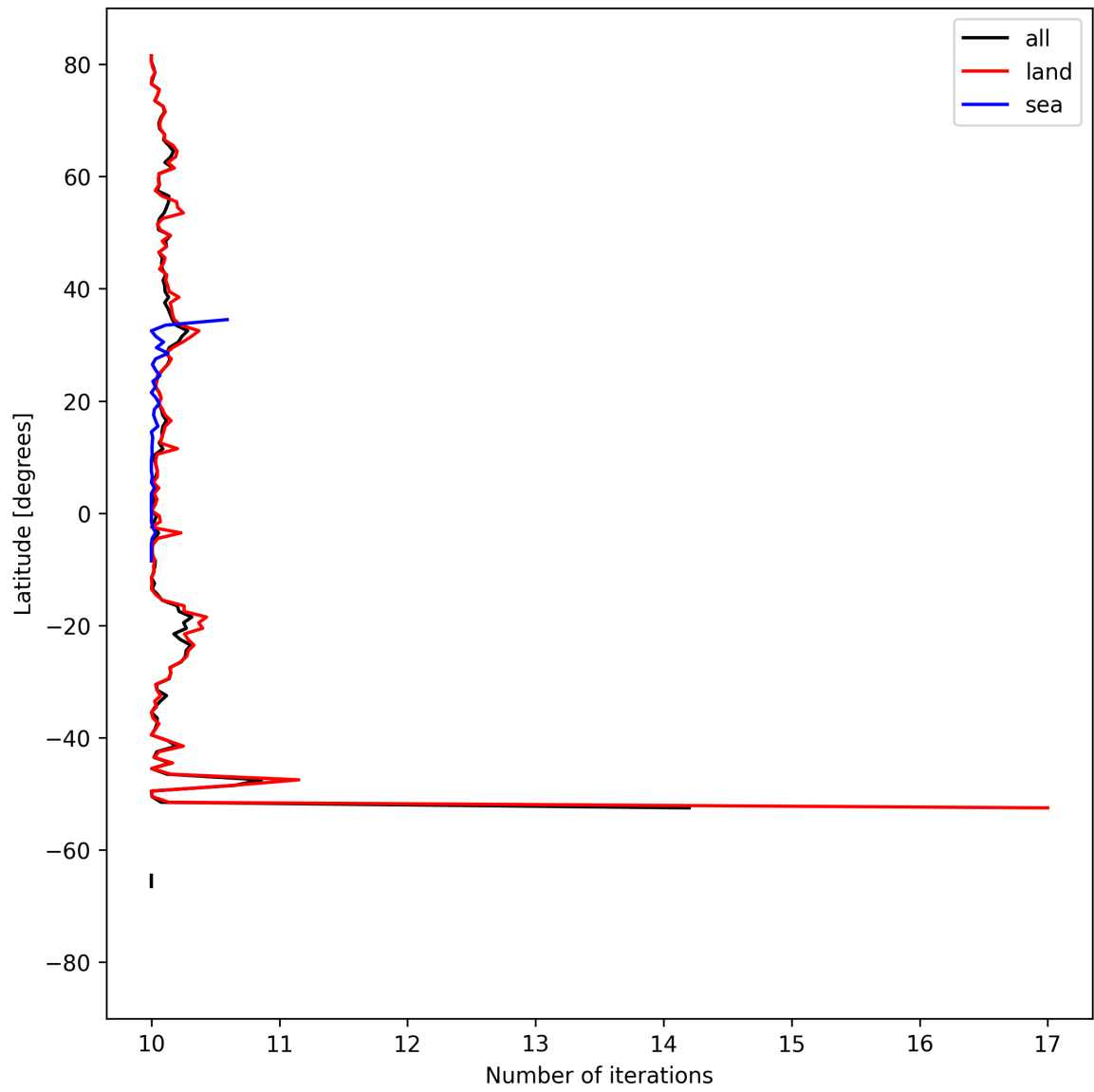
Figure 20: Zonal average of “Number of iterations” for 2025-09-05 to 2025-09-07.
