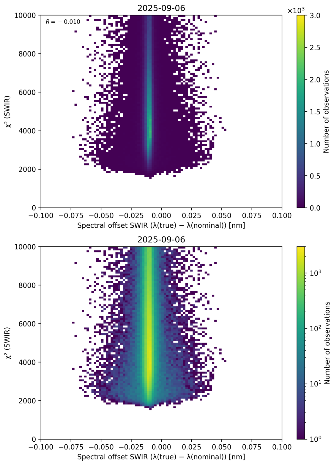
Figure 118: Scatter density plot of “Spectral offset SWIR ( \lambda_{\text{true}} - \lambda_{\text{nominal}} )” against “ \chi^2 (SWIR)” for 2025-09-05 to 2025-09-07.
