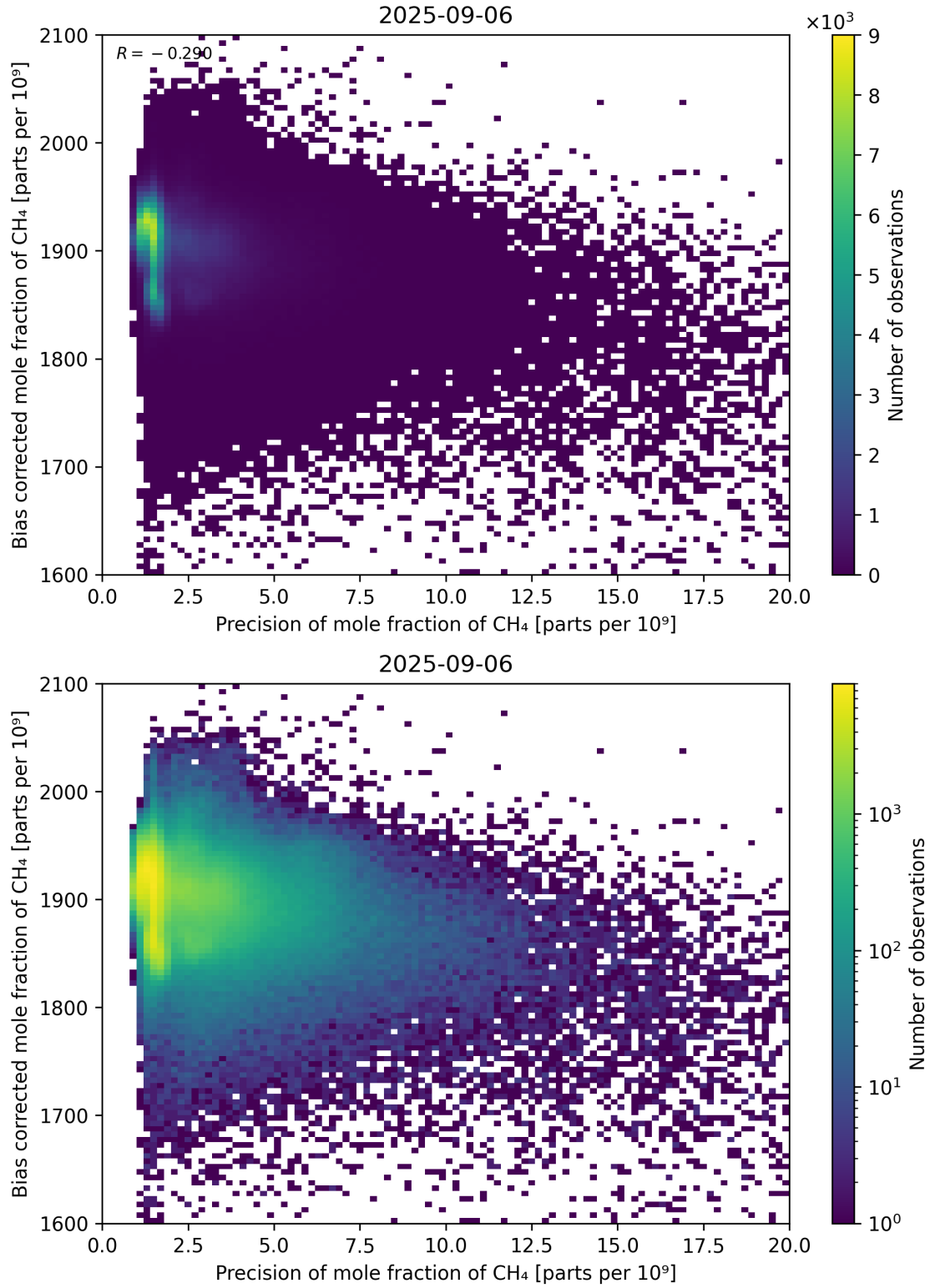
Figure 82: Scatter density plot of “Precision of mole fraction of CH 4 ” against “Bias corrected mole fraction of CH 4 ” for 2025-09-05 to 2025-09-07.
