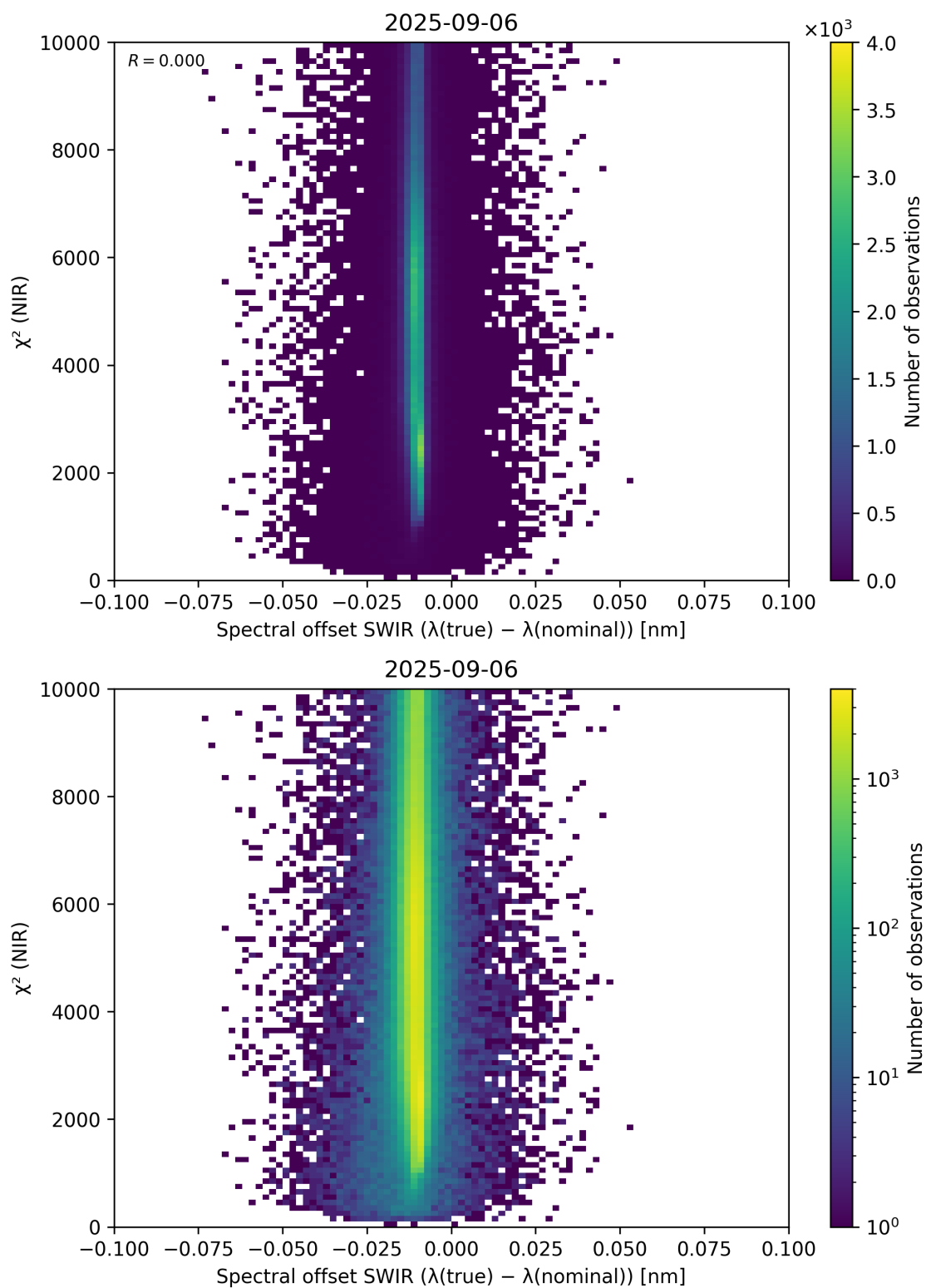
Figure 117: Scatter density plot of “Spectral offset SWIR ( \lambda_{\text{true}} - \lambda_{\text{nominal}} )” against “ \chi^2 (NIR)” for 2025-09-05 to 2025-09-07.
