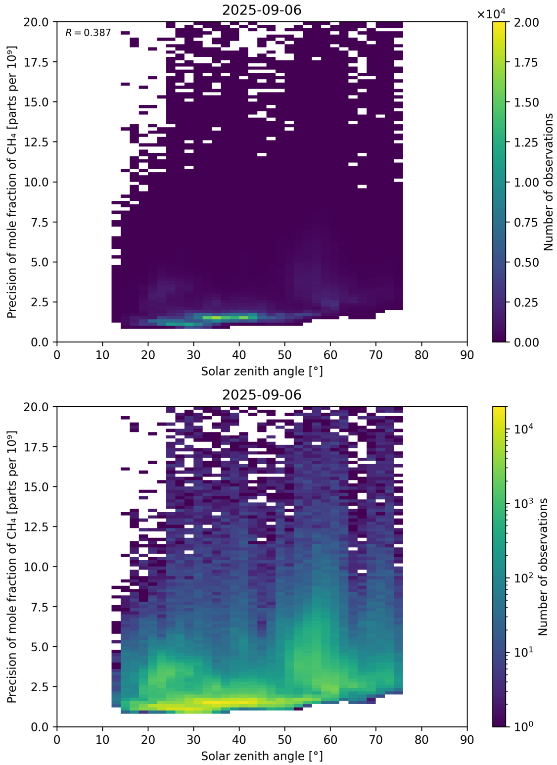
Figure 101: Scatter density plot of “Solar zenith angle” against “Precision of mole fraction of \text{CH}_4 ” for 2025-09-05 to 2025-09-07.
