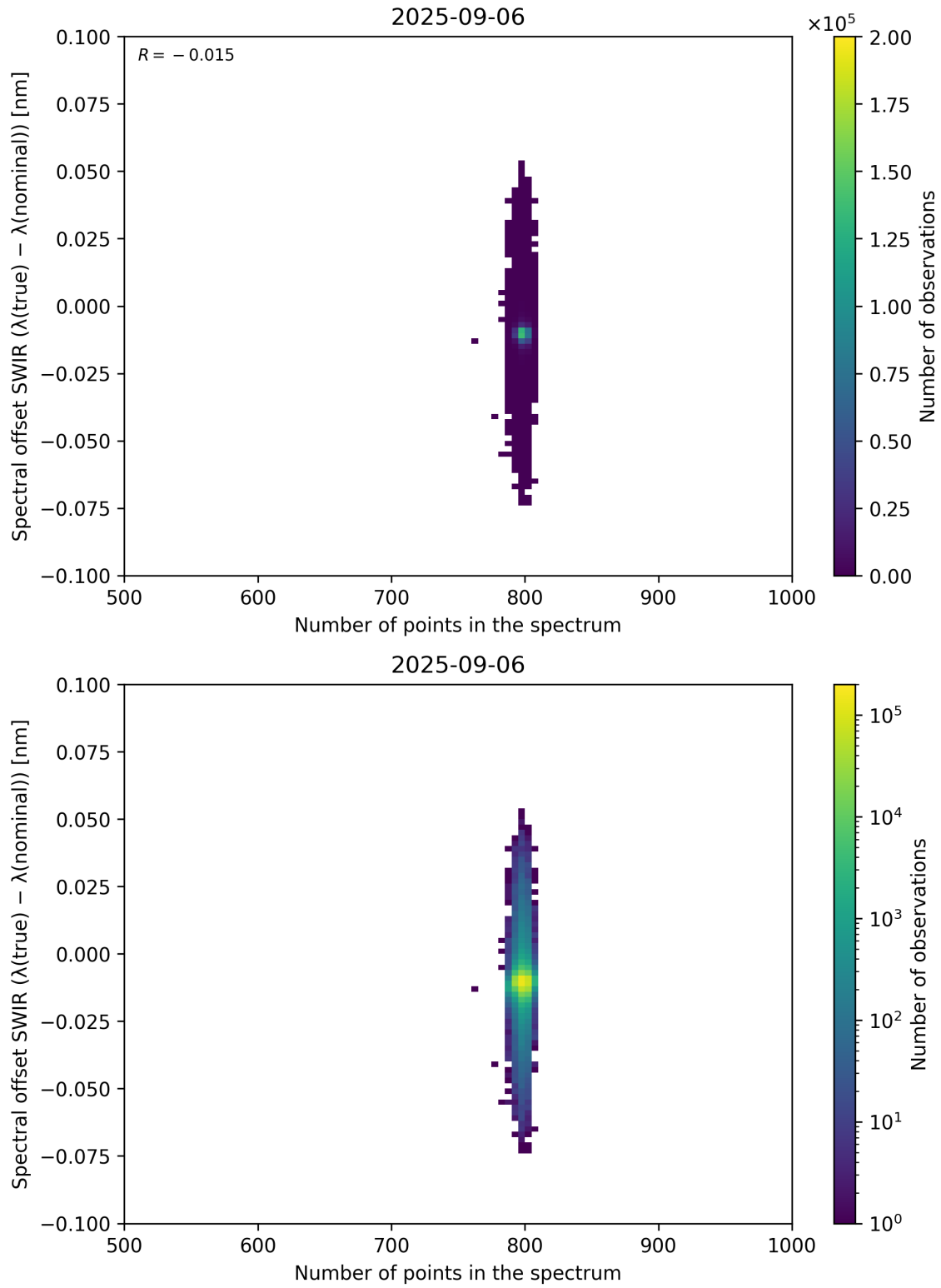
Figure 93: Scatter density plot of “Number of points in the spectrum” against “Spectral offset SWIR ( \lambda_{\text{true}} - \lambda_{\text{nominal}} )” for 2025-09-05 to 2025-09-07.
