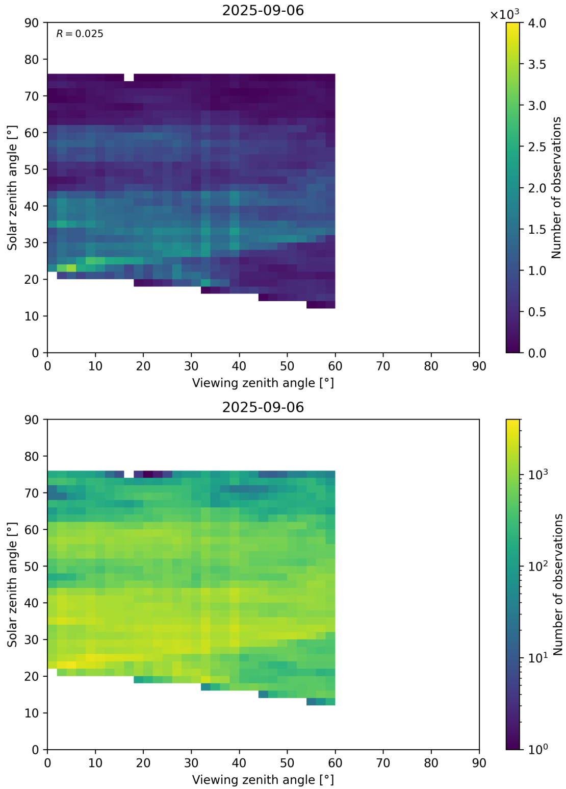
Figure 115: Scatter density plot of “Viewing zenith angle” against “Solar zenith angle” for 2025-09-05 to 2025-09-07.
