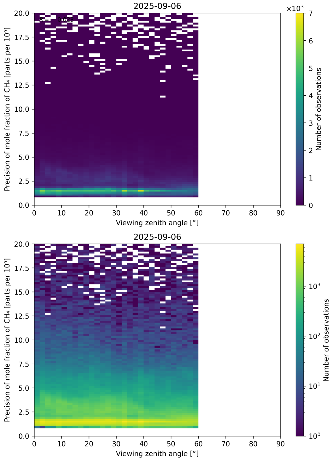
Figure 112: Scatter density plot of “Viewing zenith angle” against “Precision of mole fraction of CH 4 ” for 2025-09-05 to 2025-09-07.
