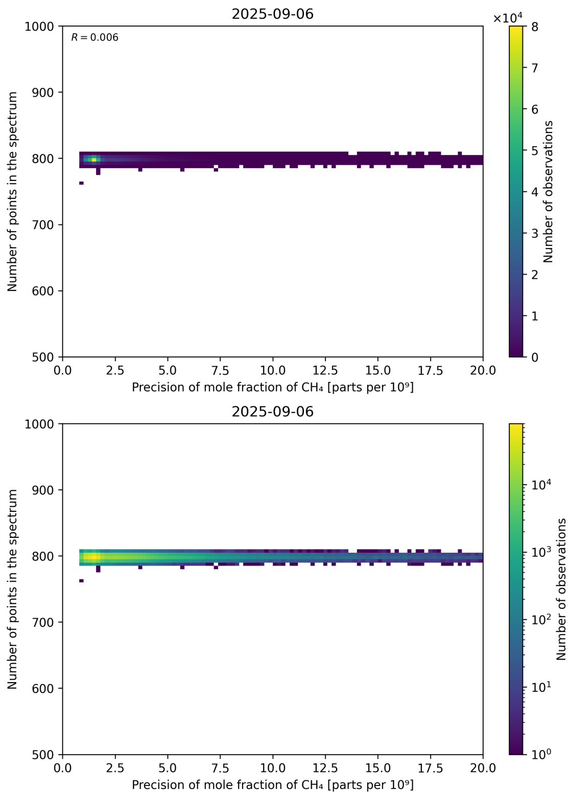
Figure 84: Scatter density plot of “Precision of mole fraction of CH 4 ” against “Number of points in the spectrum” for 2025-09-05 to 2025-09-07.
