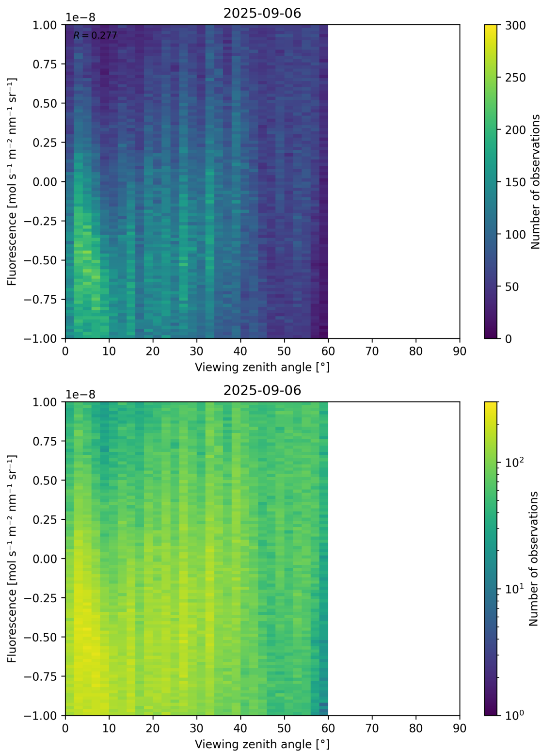
Figure 108: Scatter density plot of “Viewing zenith angle” against “Fluorescence” for 2025-09-05 to 2025-09-07.
