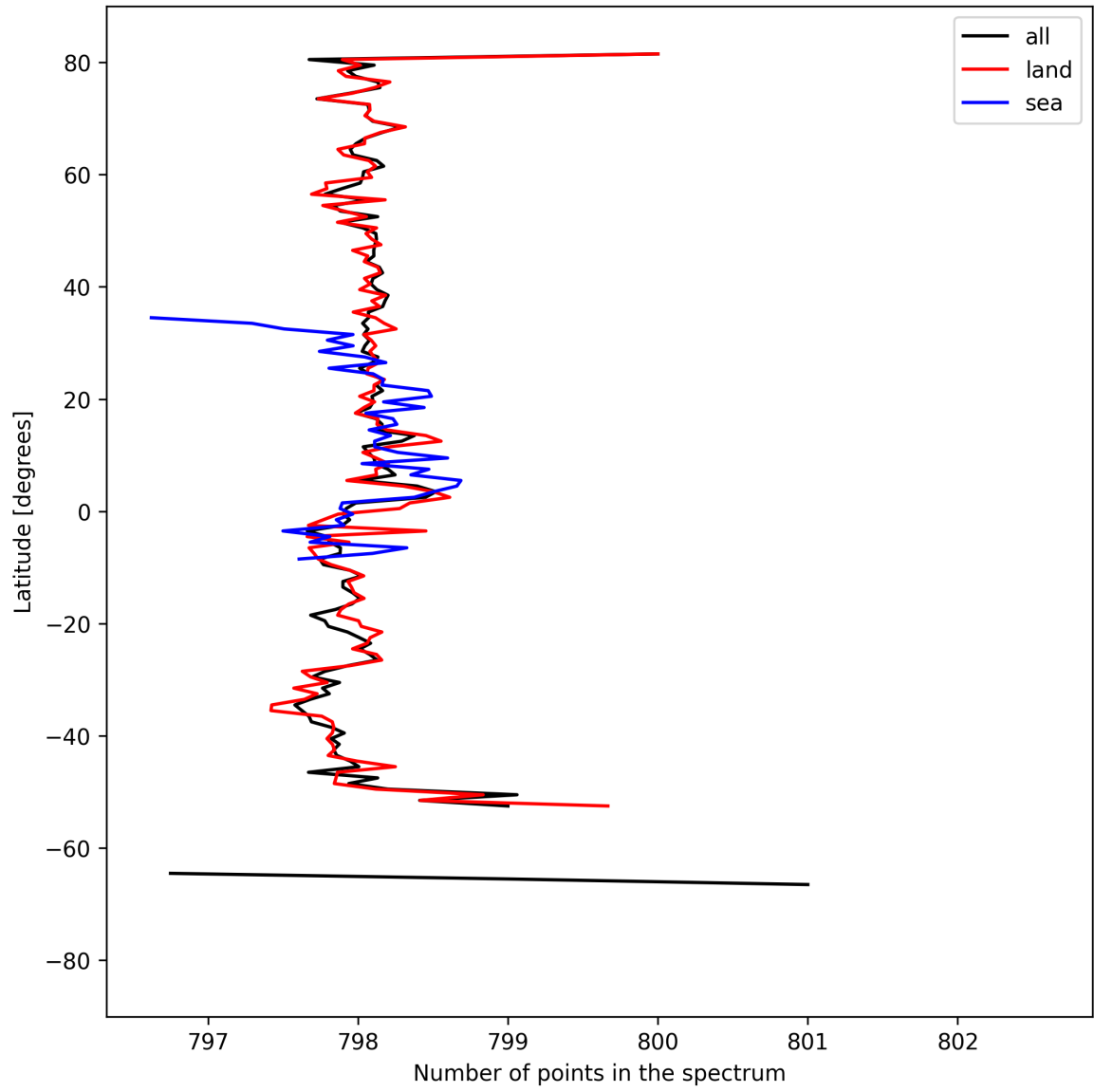
Figure 15: Zonal average of “Number of points in the spectrum” for 2025-09-05 to 2025-09-07.
