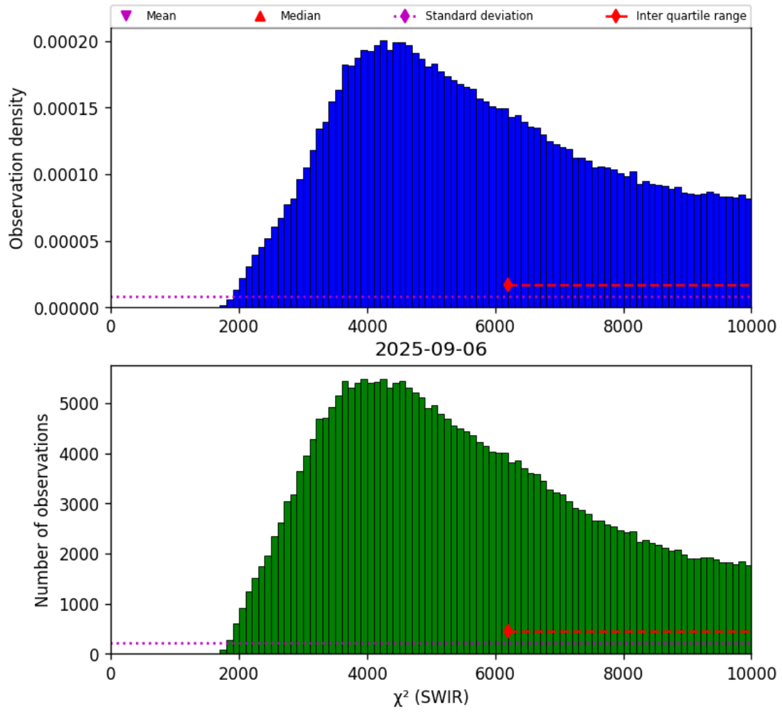
Figure 28: Histogram of " \chi^2 (SWIR)" for 2025-09-05 to 2025-09-07
