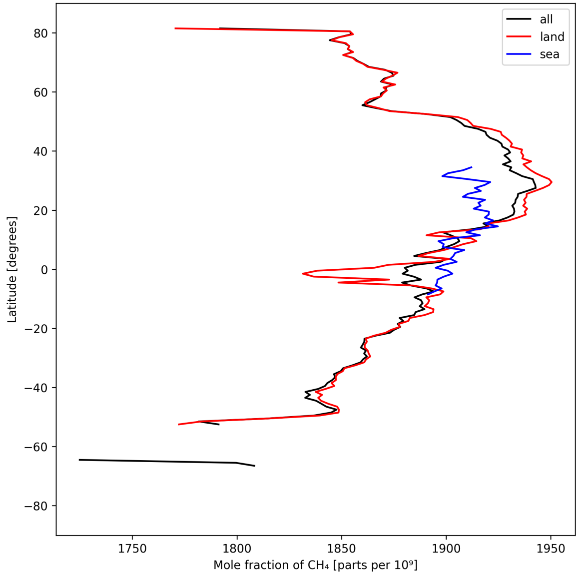
Figure 12: Zonal average of “Mole fraction of \text{CH}_4 ” for 2025-09-05 to 2025-09-07.
