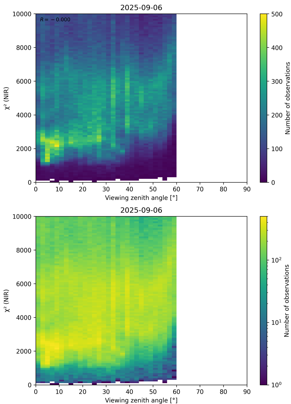
Figure 105: Scatter density plot of “Viewing zenith angle” against “ \chi^2 (NIR)” for 2025-09-05 to 2025-09-07.
