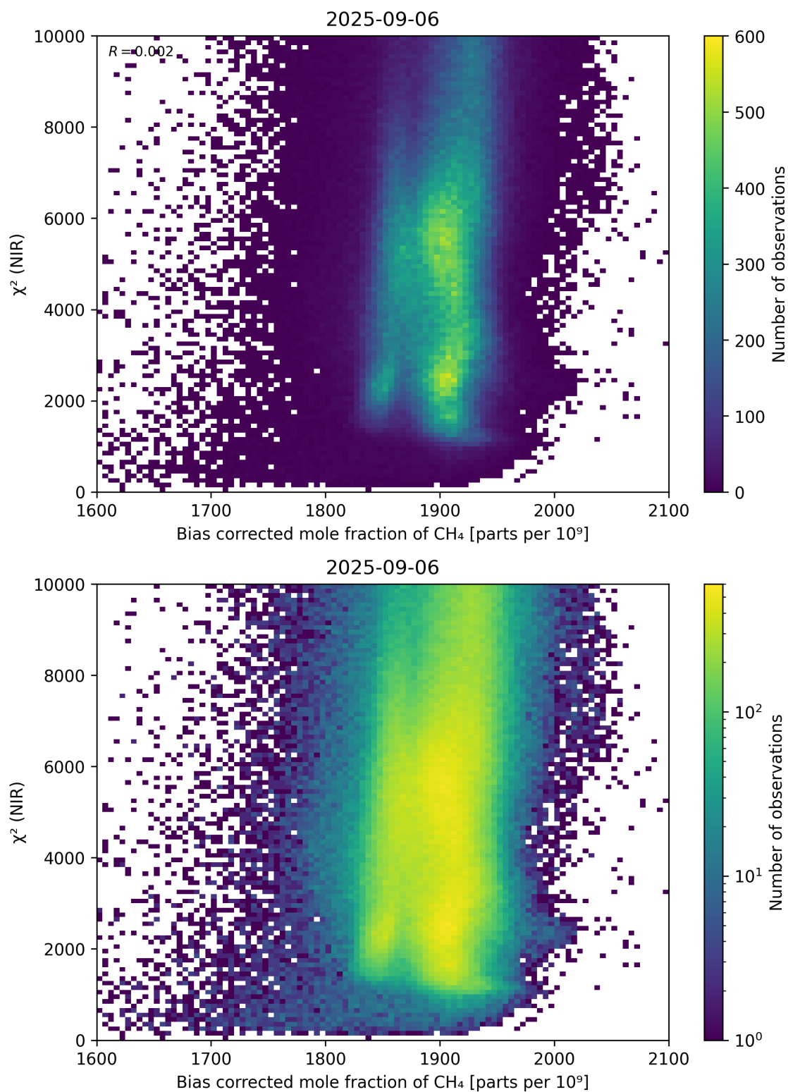
Figure 63: Scatter density plot of “Bias corrected mole fraction of \text{CH}_4 ” against “ \chi^2 (NIR)” for 2025-09-05 to 2025-09-07.
