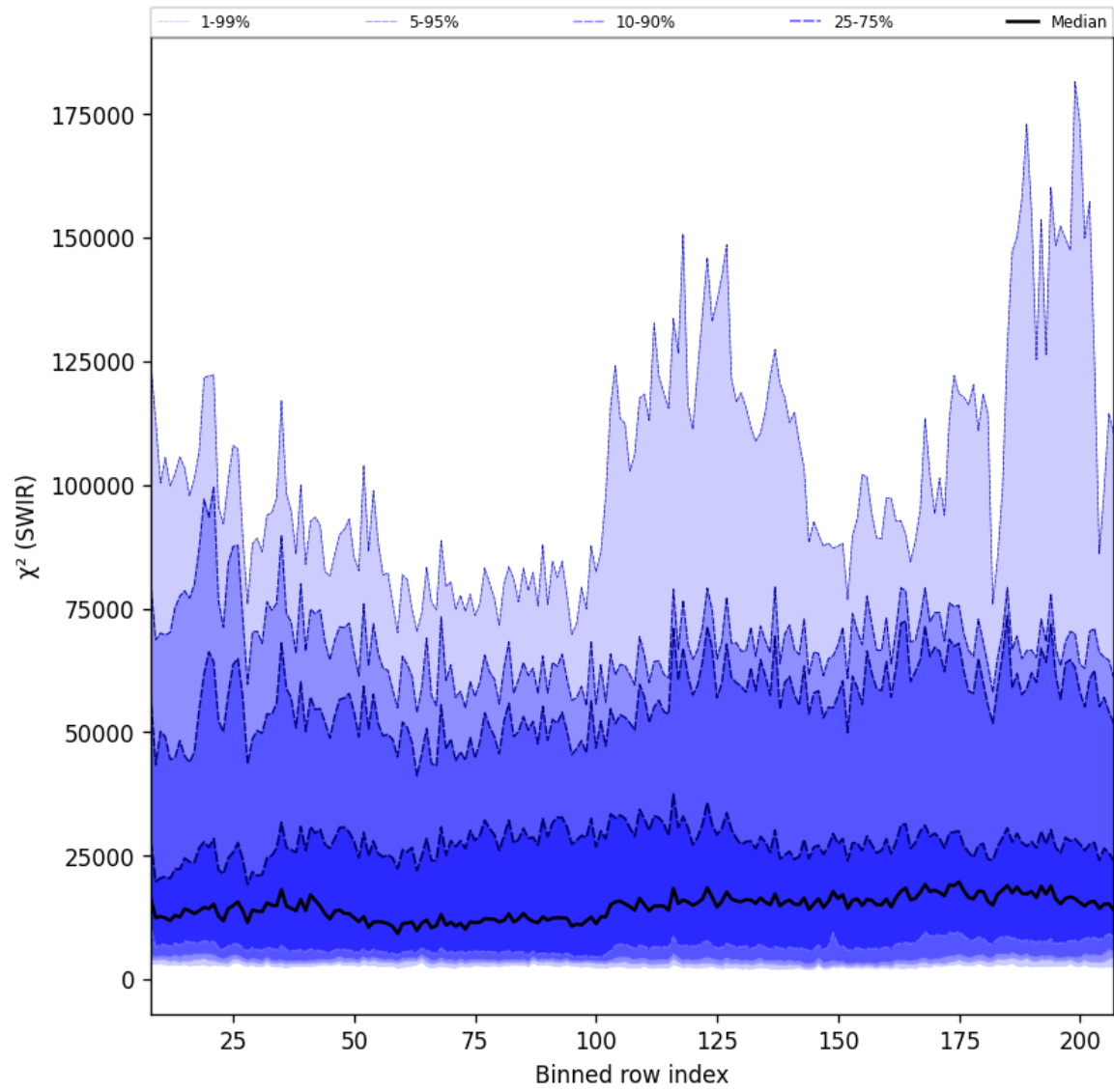
Figure 39: Along track statistics of “ \chi^2 (SWIR)” for 2025-09-05 to 2025-09-07
