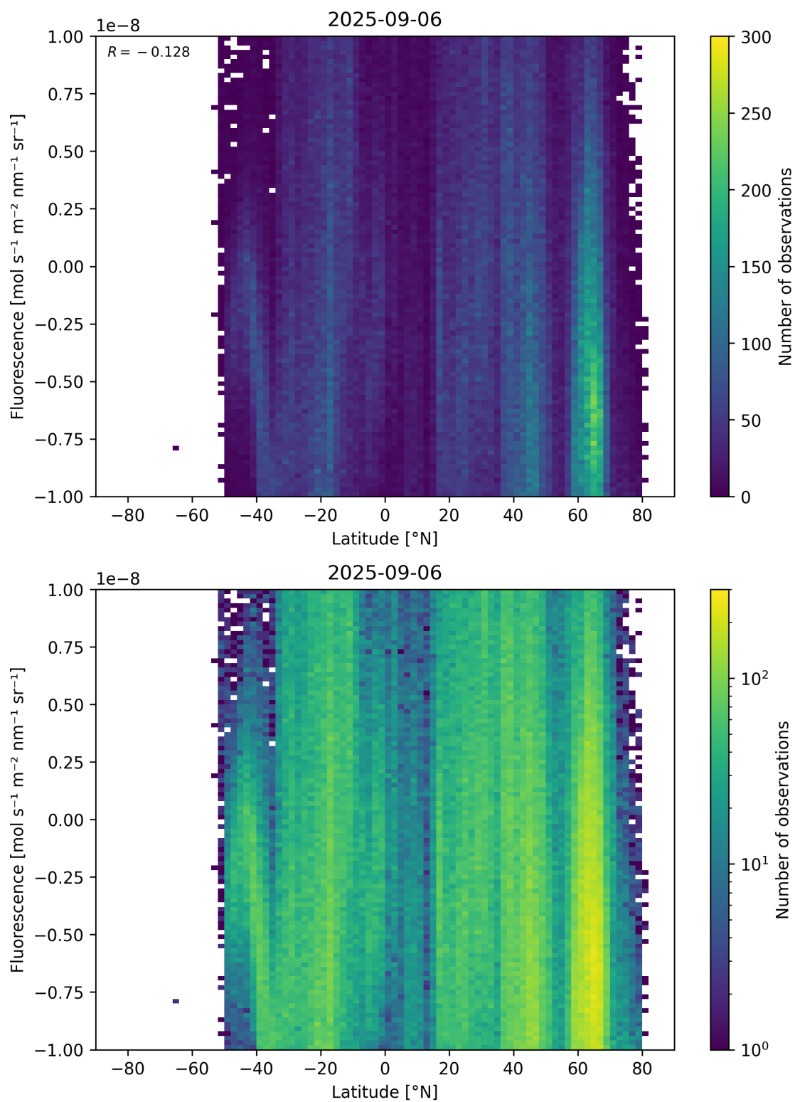
Figure 56: Scatter density plot of “Latitude” against “Fluorescence” for 2025-09-05 to 2025-09-07.
