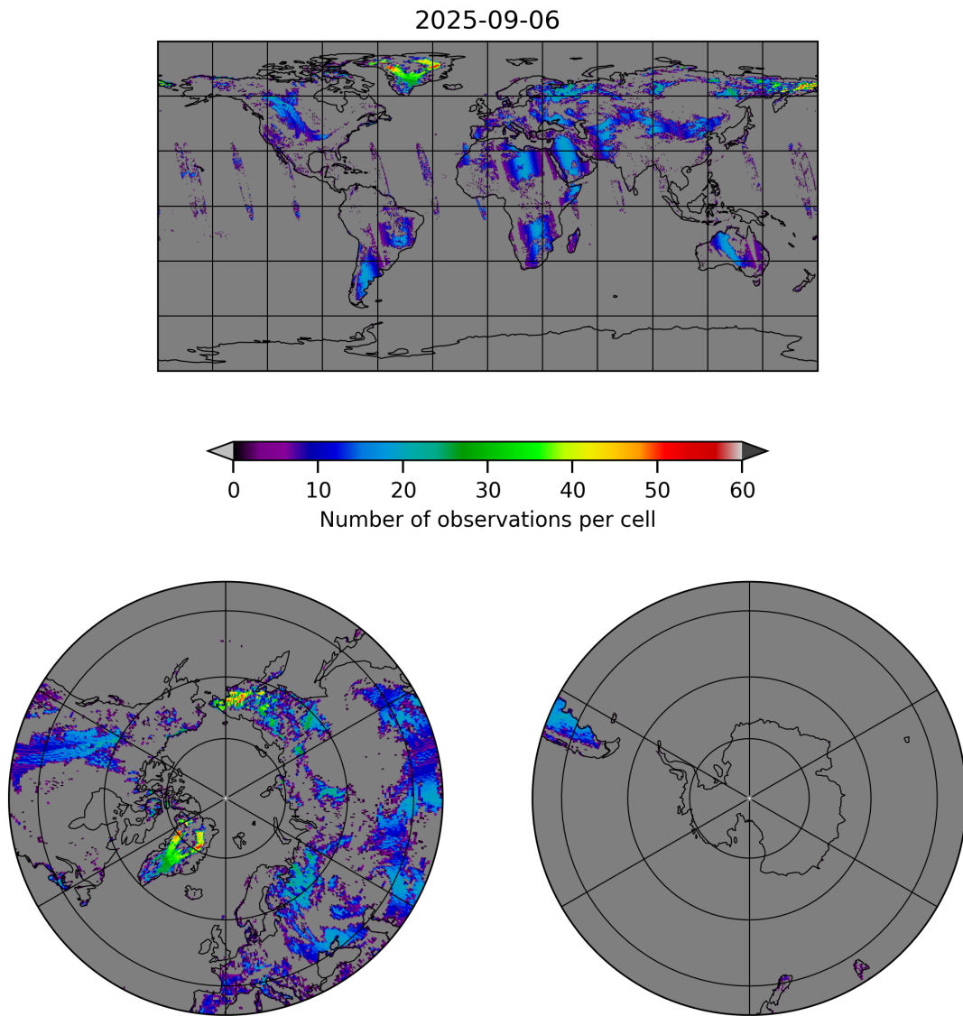
Figure 10: Map of the number of observations for 2025-09-05 to 2025-09-07
