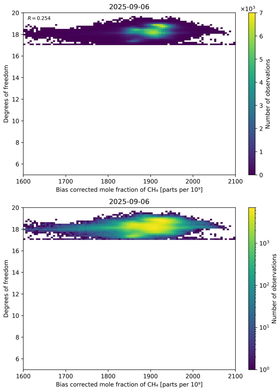
Figure 65: Scatter density plot of “Bias corrected mole fraction of CH 4 ” against “Degrees of freedom” for 2025-09-05 to 2025-09-07.
