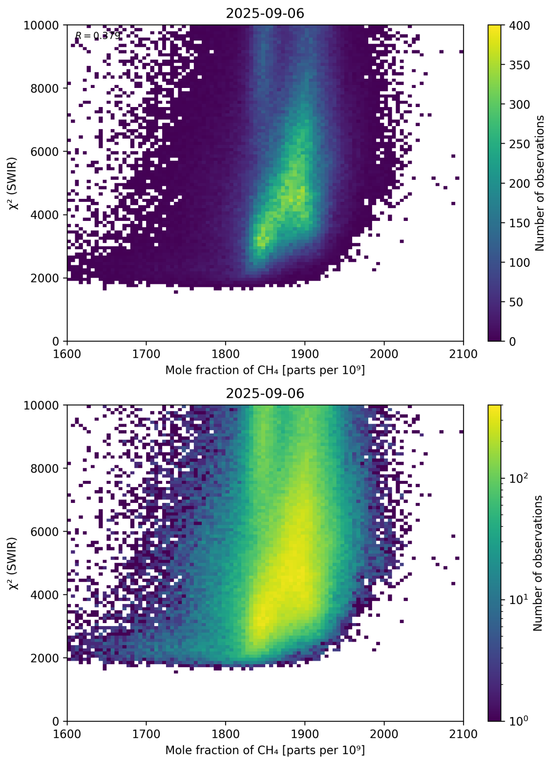
Figure 71: Scatter density plot of “Mole fraction of \text{CH}_4 ” against “ \chi^2 (SWIR)” for 2025-09-05 to 2025-09-07.
