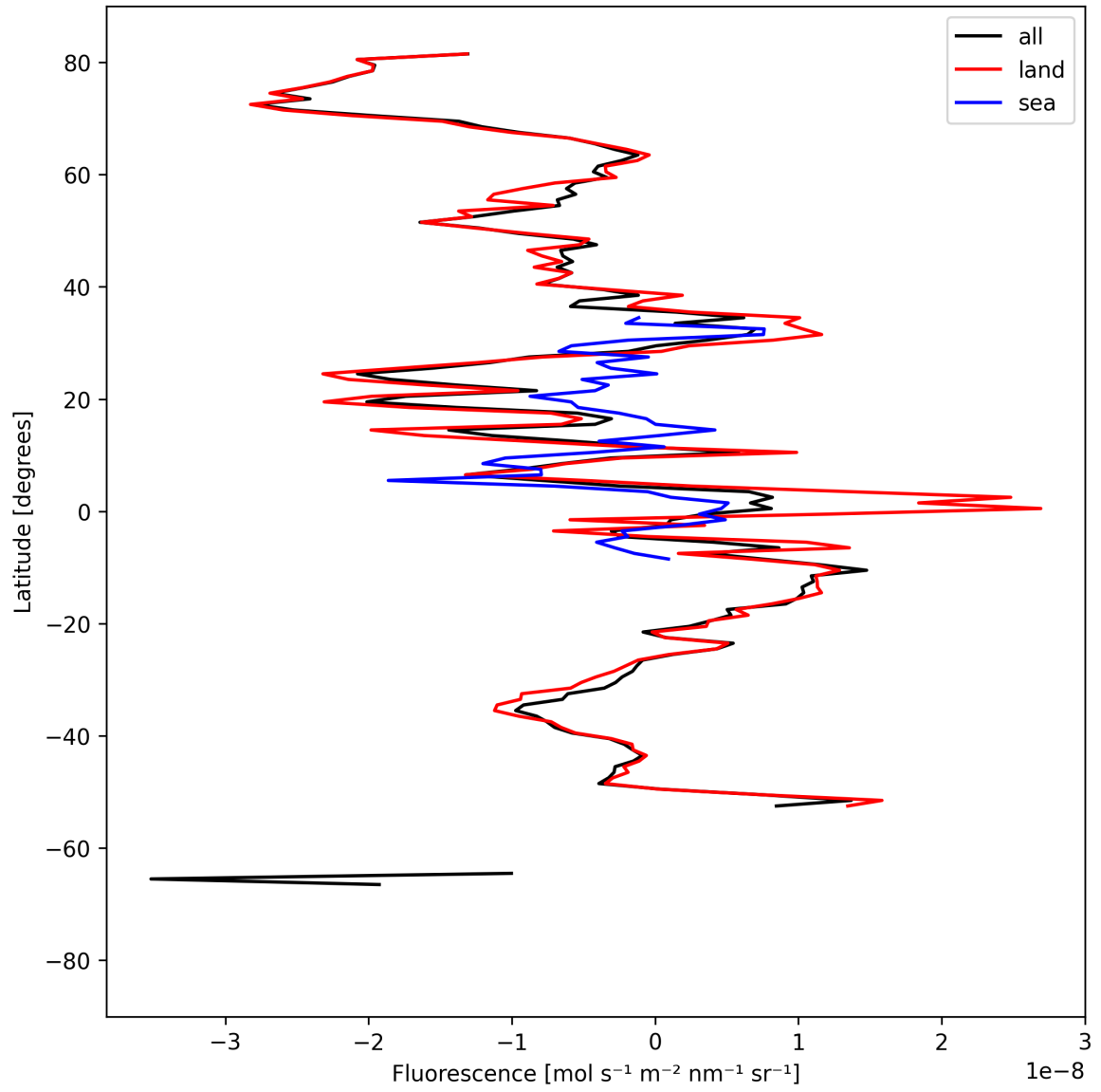
Figure 21: Zonal average of “Fluorescence” for 2025-09-05 to 2025-09-07.
