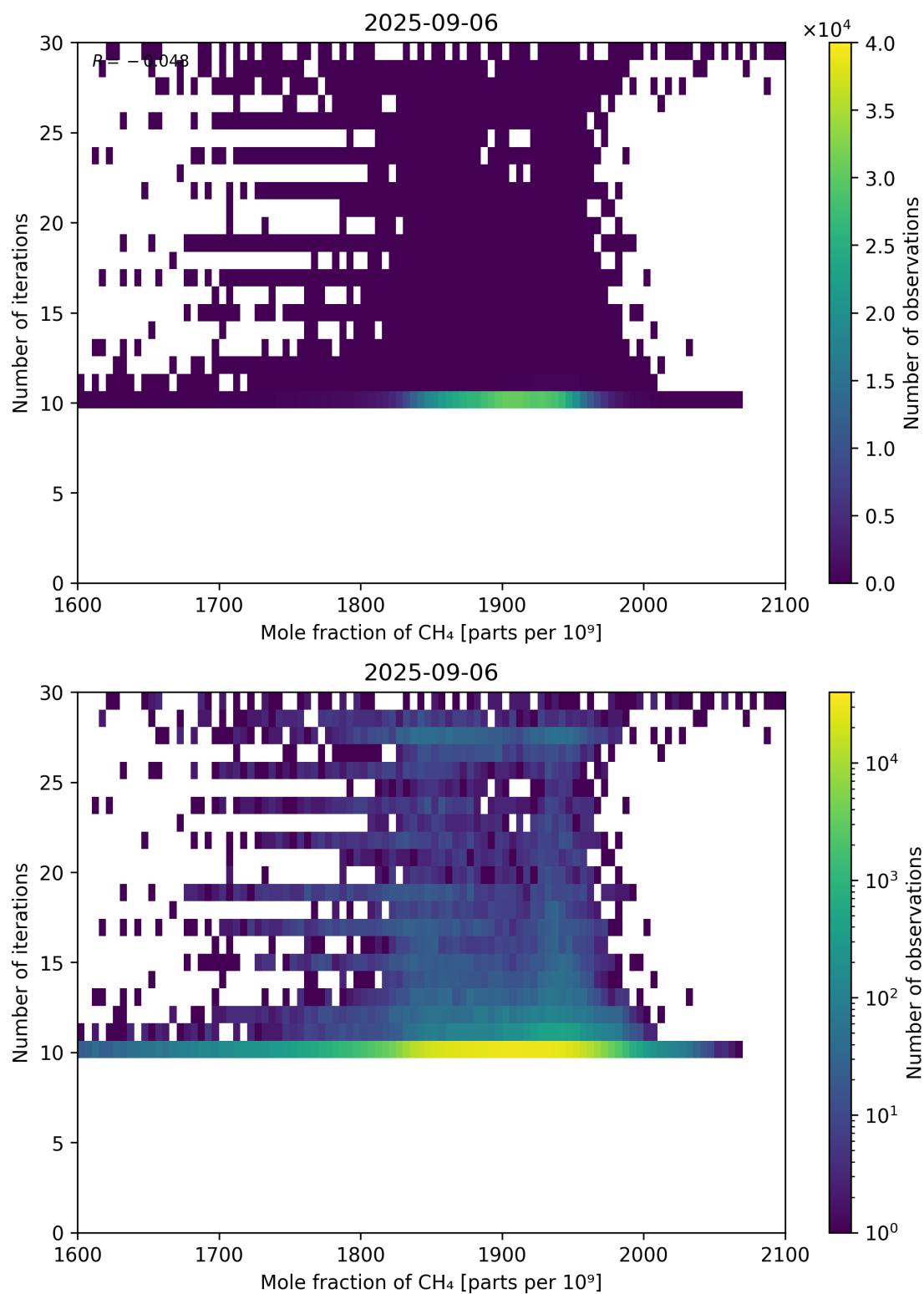
Figure 76: Scatter density plot of “Mole fraction of CH 4 ” against “Number of iterations” for 2025-09-05 to 2025-09-07.
