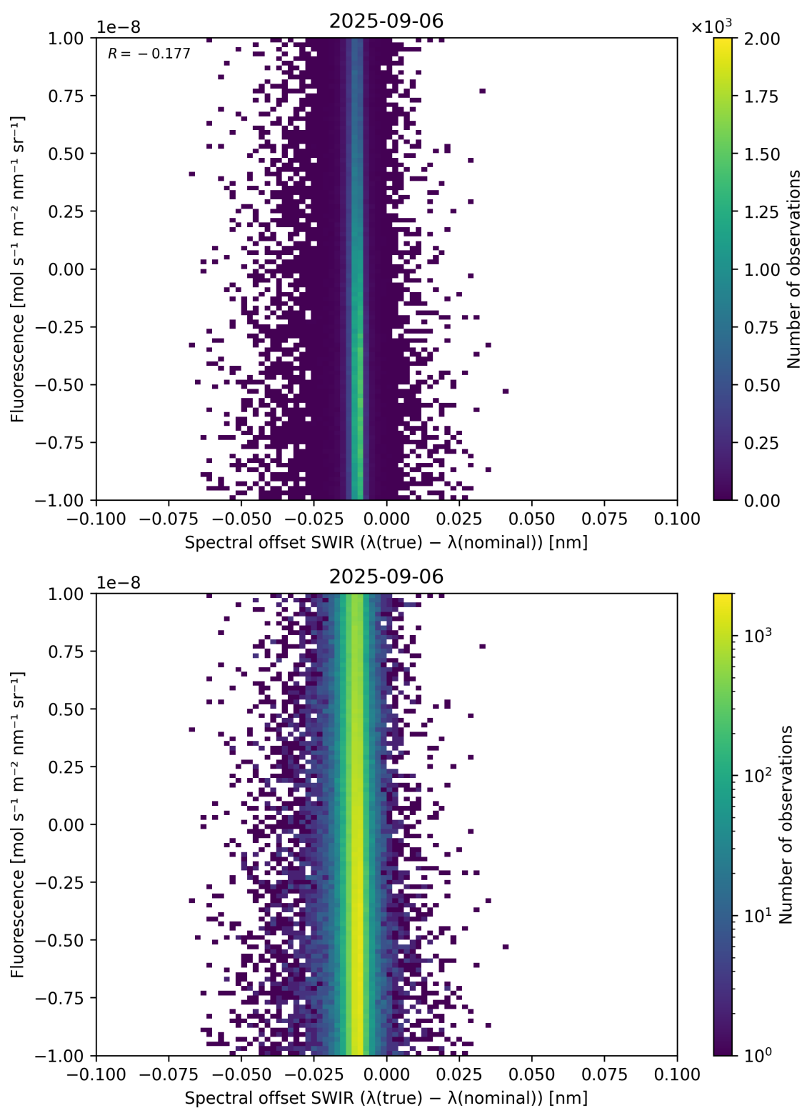
Figure 120: Scatter density plot of “Spectral offset SWIR ( \lambda_{\text{true}} - \lambda_{\text{nominal}} )” against “Fluorescence” for 2025-09-05 to 2025-09-07.
