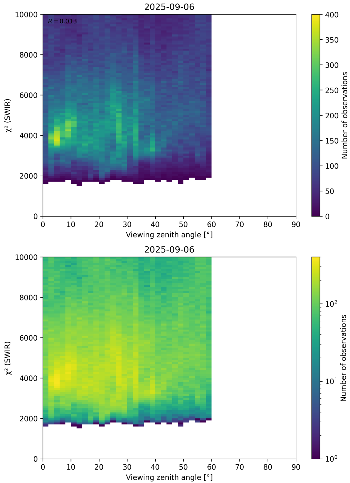
Figure 106: Scatter density plot of “Viewing zenith angle” against “ \chi^2 (SWIR)” for 2025-09-05 to 2025-09-07.
