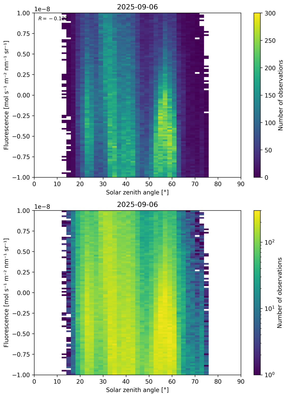
Figure 97: Scatter density plot of “Solar zenith angle” against “Fluorescence” for 2025-09-05 to 2025-09-07.
