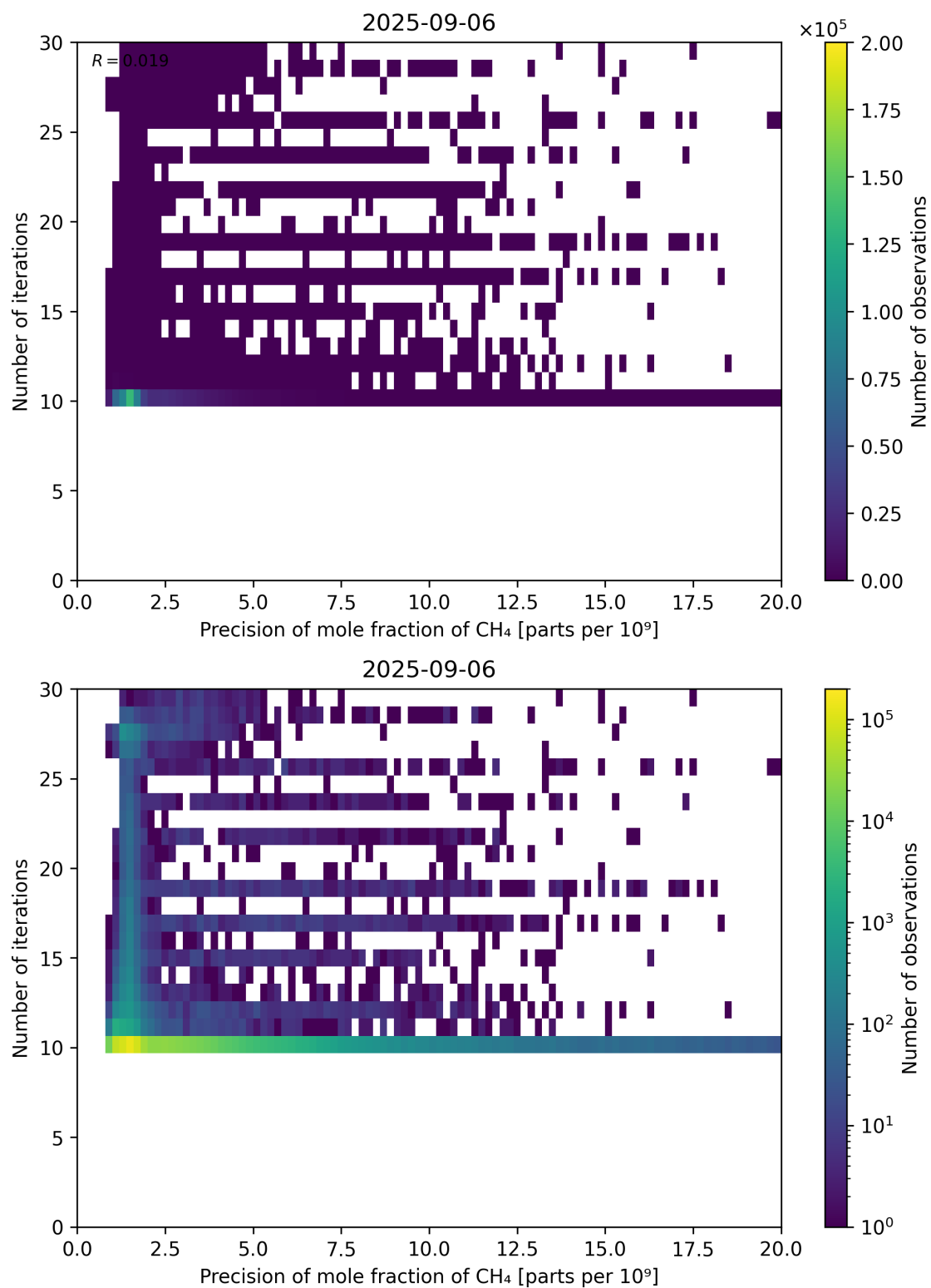
Figure 83: Scatter density plot of “Precision of mole fraction of CH 4 ” against “Number of iterations” for 2025-09-05 to 2025-09-07.
