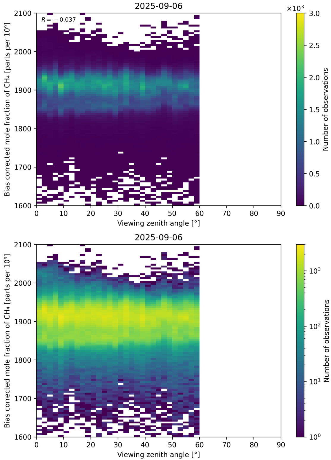
Figure 111: Scatter density plot of “Viewing zenith angle” against “Bias corrected mole fraction of CH 4 ” for 2025-09-05 to 2025-09-07.
