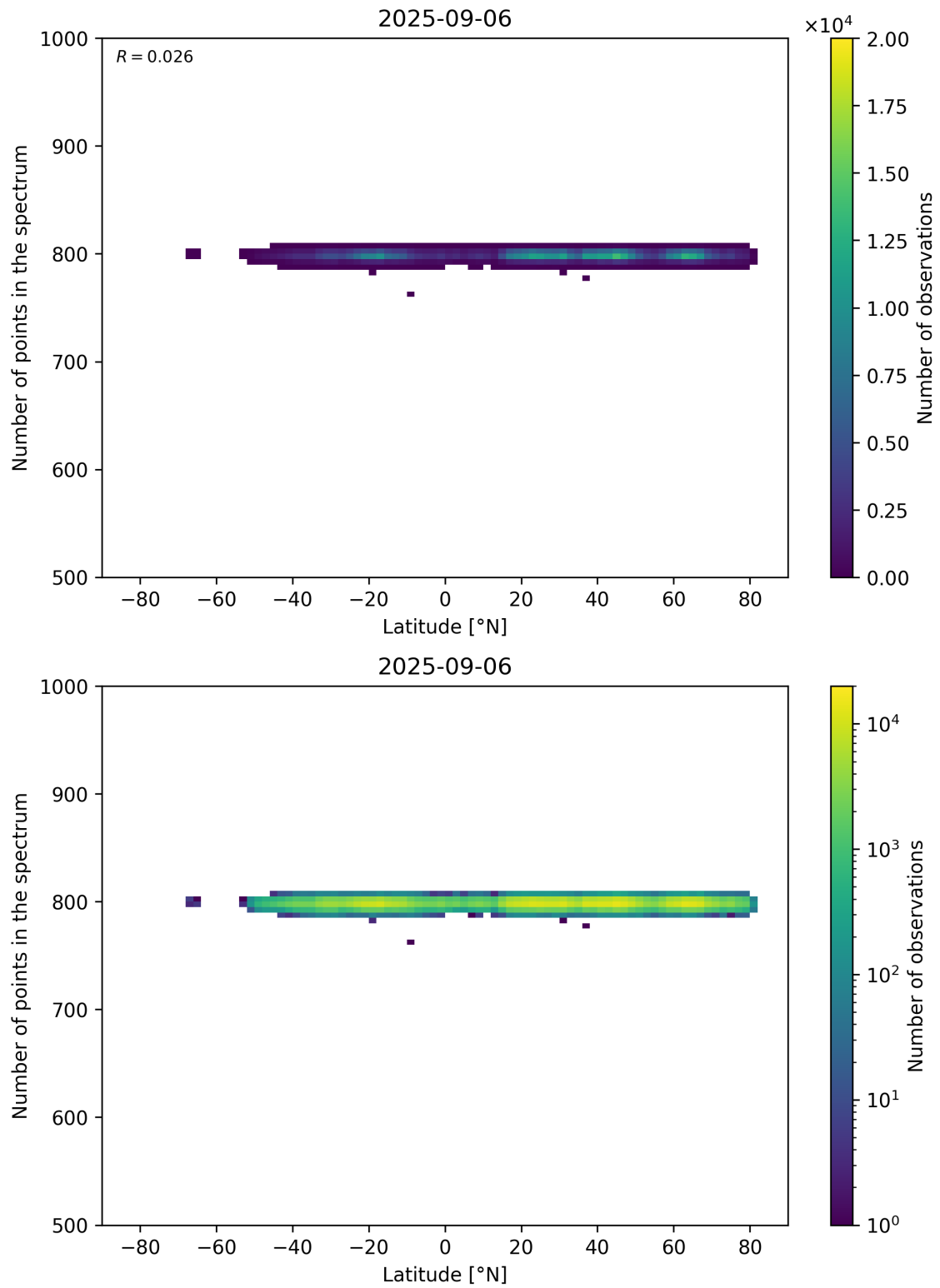
Figure 61: Scatter density plot of “Latitude” against “Number of points in the spectrum” for 2025-09-05 to 2025-09-07.
