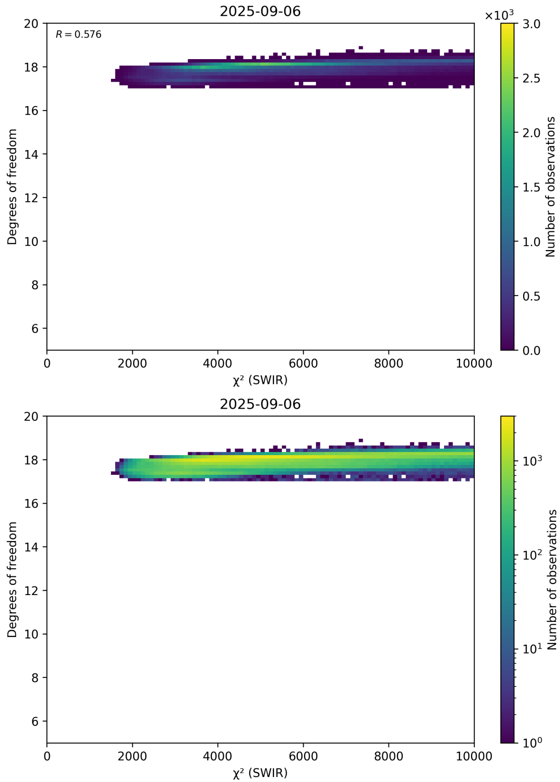
Figure 48: Scatter density plot of “ \chi^2 (SWIR)” against “Degrees of freedom” for 2025-09-05 to 2025-09-07.
