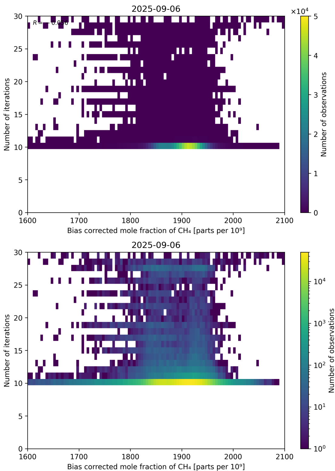
Figure 67: Scatter density plot of “Bias corrected mole fraction of \text{CH}_4 ” against “Number of iterations” for 2025-09-05 to 2025-09-07.
