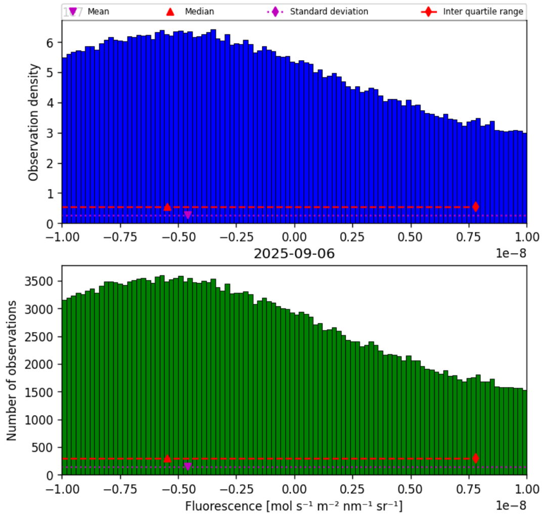
Figure 32: Histogram of “Fluorescence” for 2025-09-05 to 2025-09-07
