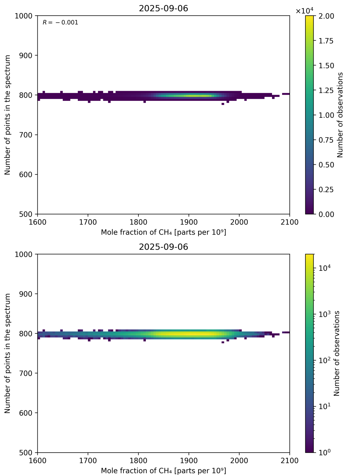
Figure 77: Scatter density plot of “Mole fraction of CH 4 ” against “Number of points in the spectrum” for 2025-09-05 to 2025-09-07.
