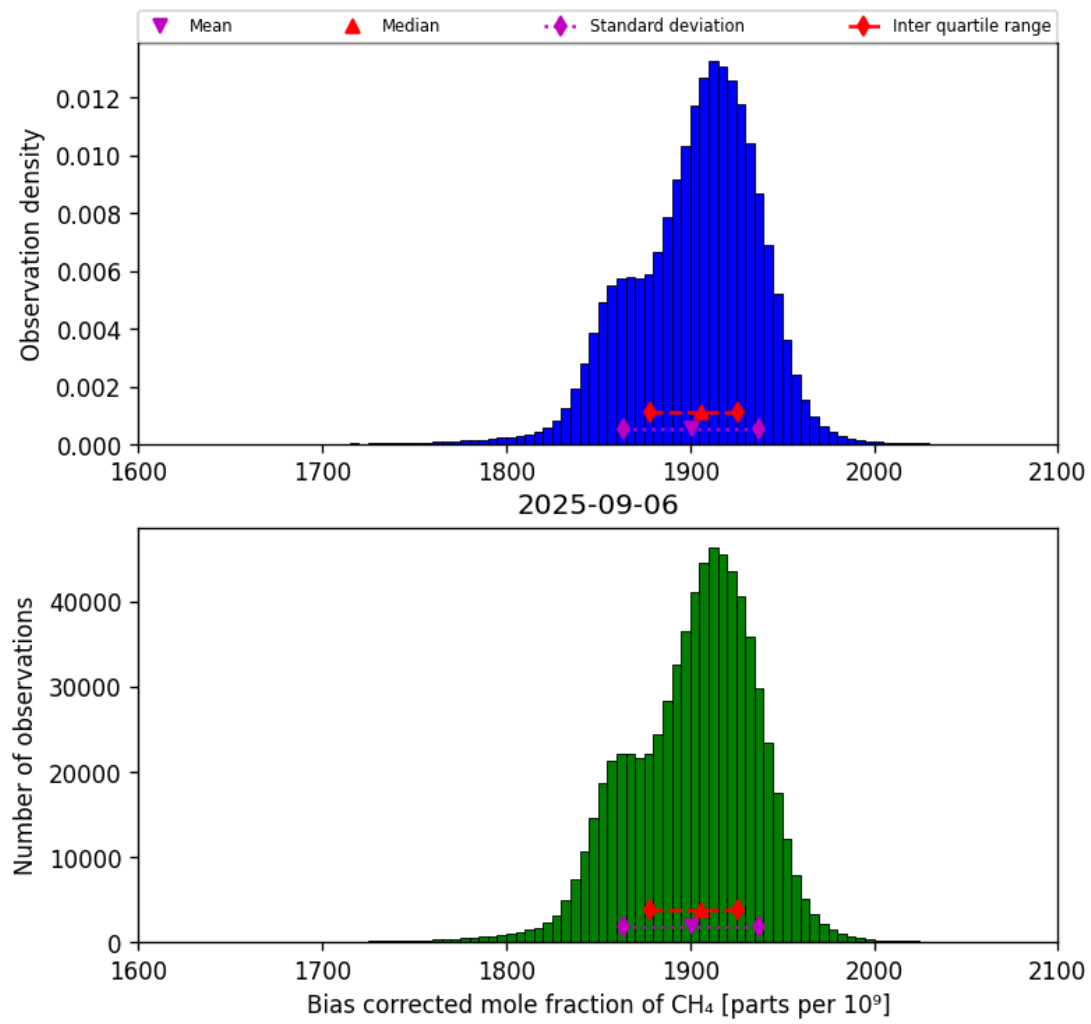
Figure 25: Histogram of “Bias corrected mole fraction of CH 4 ” for 2025-09-05 to 2025-09-07
