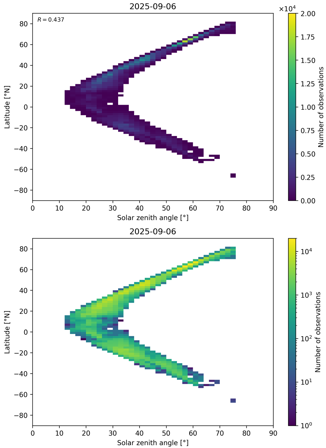
Figure 98: Scatter density plot of “Solar zenith angle” against “Latitude” for 2025-09-05 to 2025-09-07.
