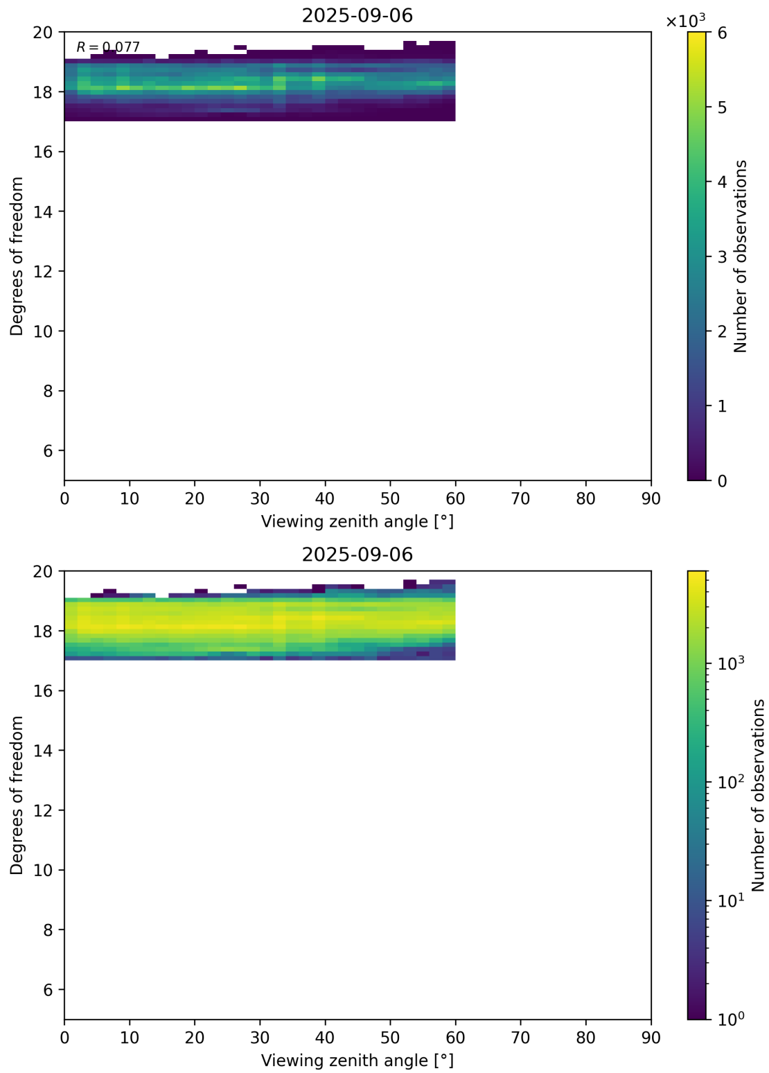
Figure 107: Scatter density plot of “Viewing zenith angle” against “Degrees of freedom” for 2025-09-05 to 2025-09-07.
