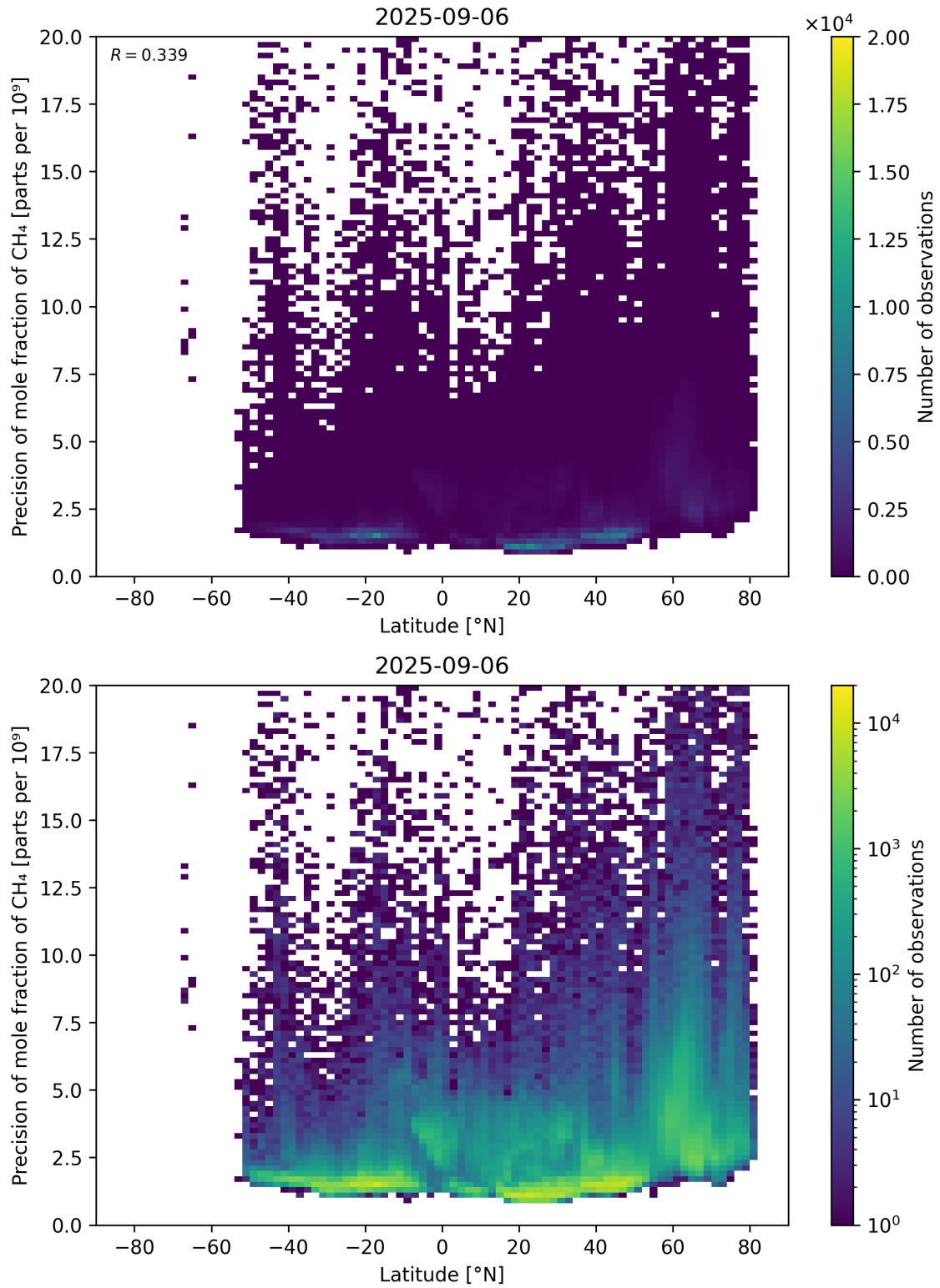
Figure 59: Scatter density plot of “Latitude” against “Precision of mole fraction of CH 4 ” for 2025-09-05 to 2025-09-07.
