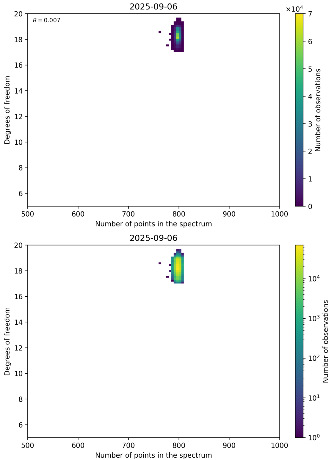
Figure 90: Scatter density plot of “Number of points in the spectrum” against “Degrees of freedom” for 2025-09-05 to 2025-09-07.
