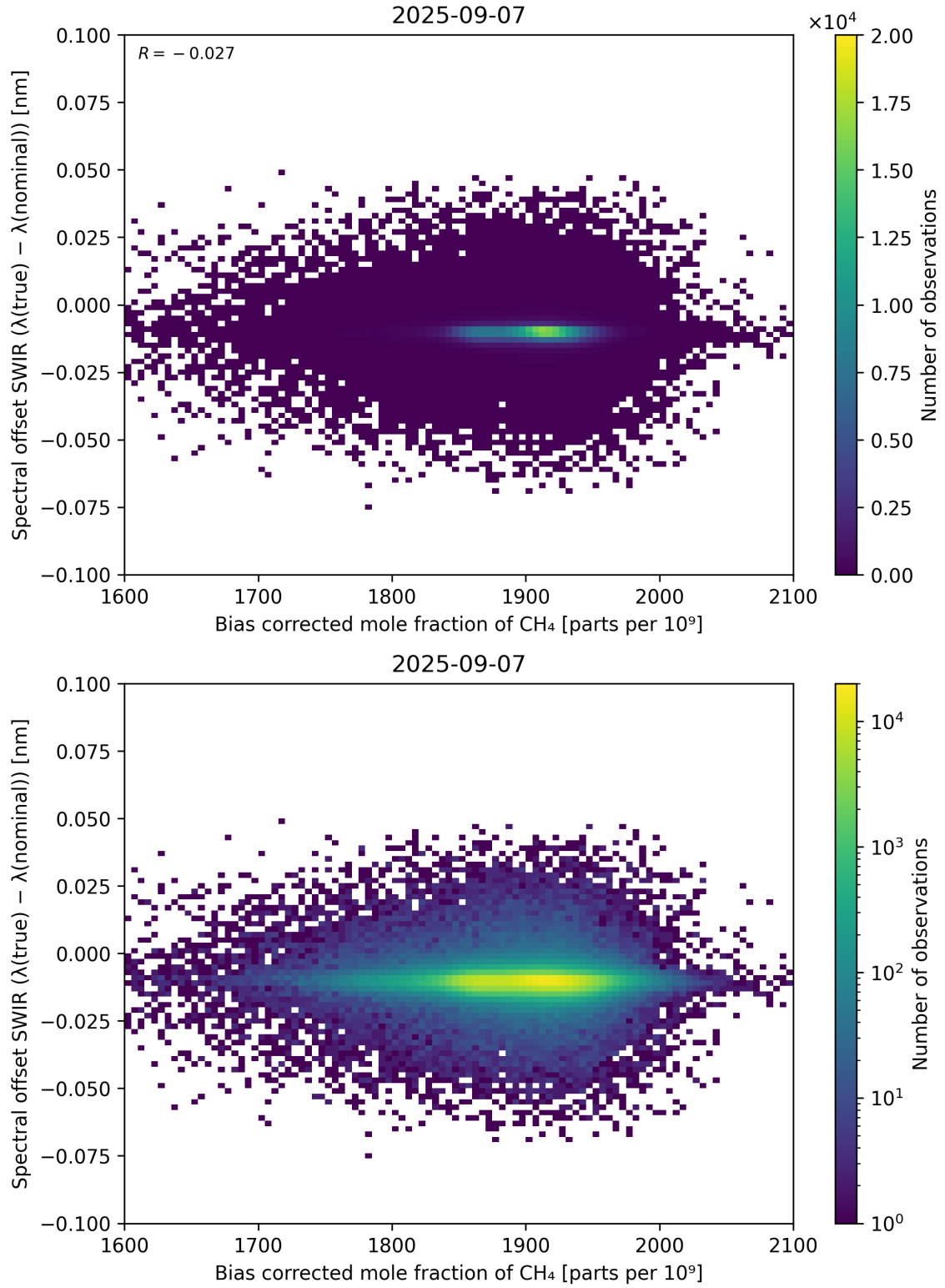
Figure 69: Scatter density plot of “Bias corrected mole fraction of \text{CH}_4 ” against “Spectral offset SWIR ( \lambda_{\text{true}} - \lambda_{\text{nominal}} )” for 2025-09-06 to 2025-09-08.
