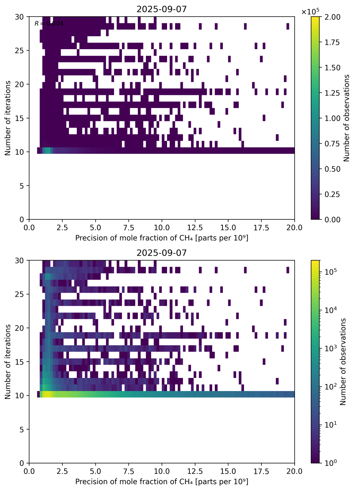
Figure 83: Scatter density plot of “Precision of mole fraction of CH 4 ” against “Number of iterations” for 2025-09-06 to 2025-09-08.
