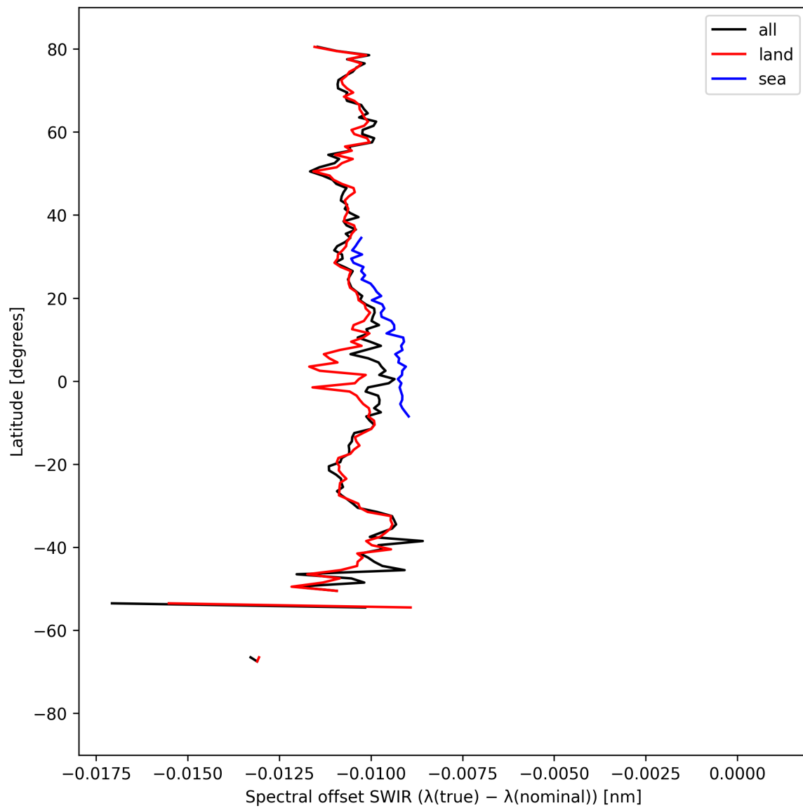
Figure 16: Zonal average of “Spectral offset SWIR ( \lambda_{\text{true}} - \lambda_{\text{nominal}} )” for 2025-09-06 to 2025-09-08.
