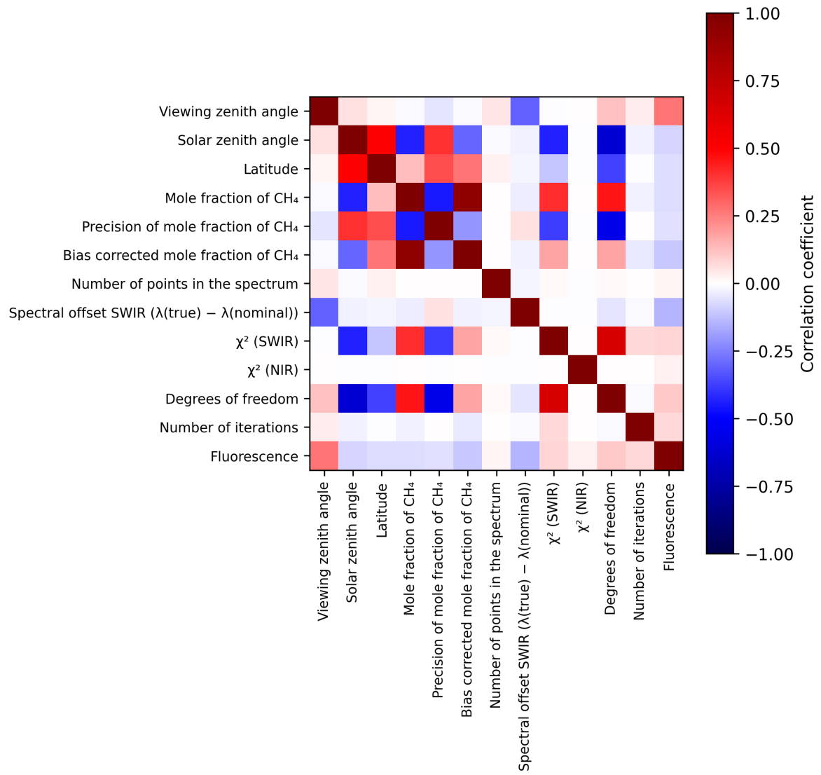
Figure 2: Map of correlation matrix for 2025-09-06 to 2025-09-08.
