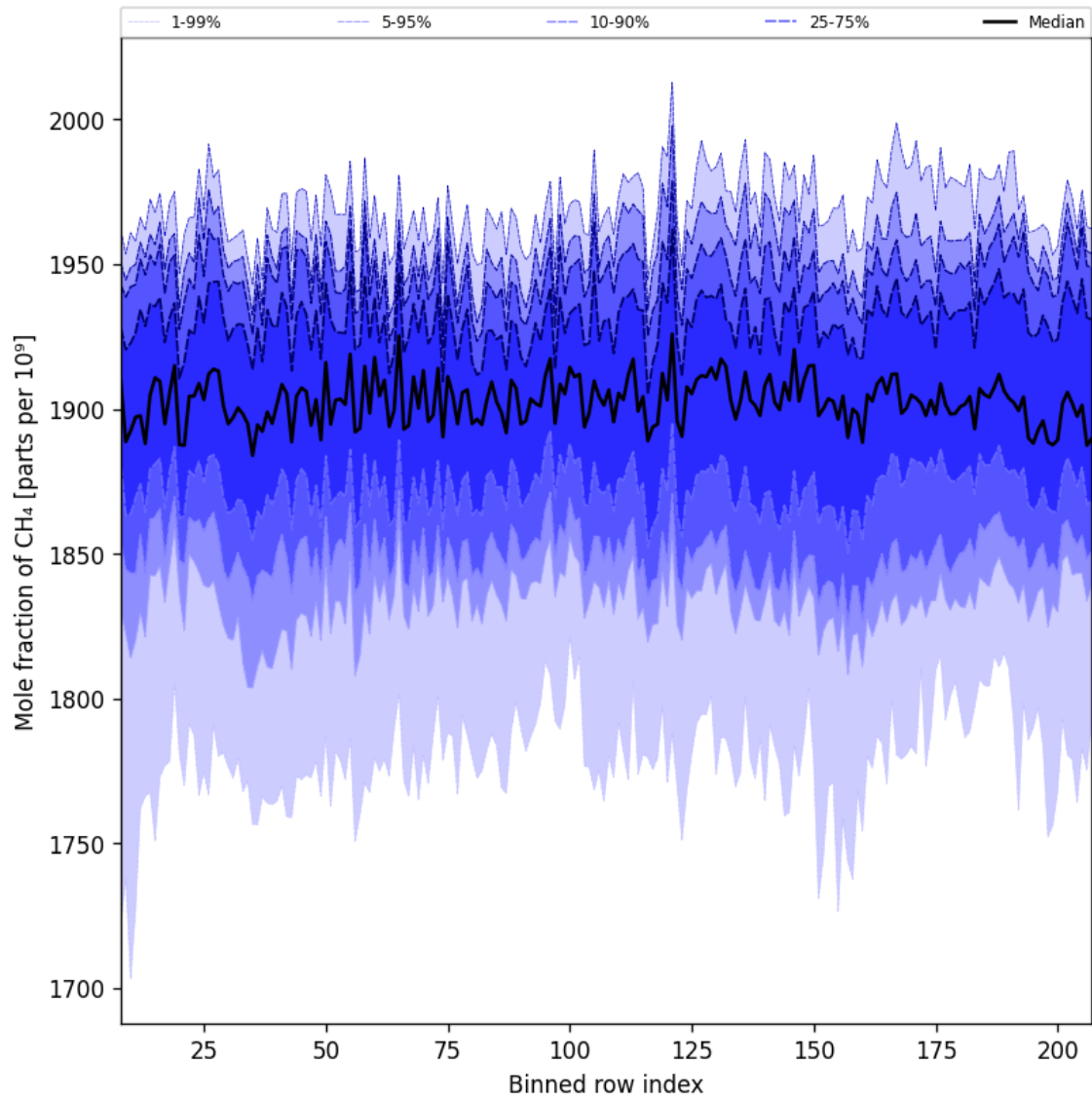
Figure 34: Along track statistics of “Mole fraction of CH 4 ” for 2025-09-06 to 2025-09-08
