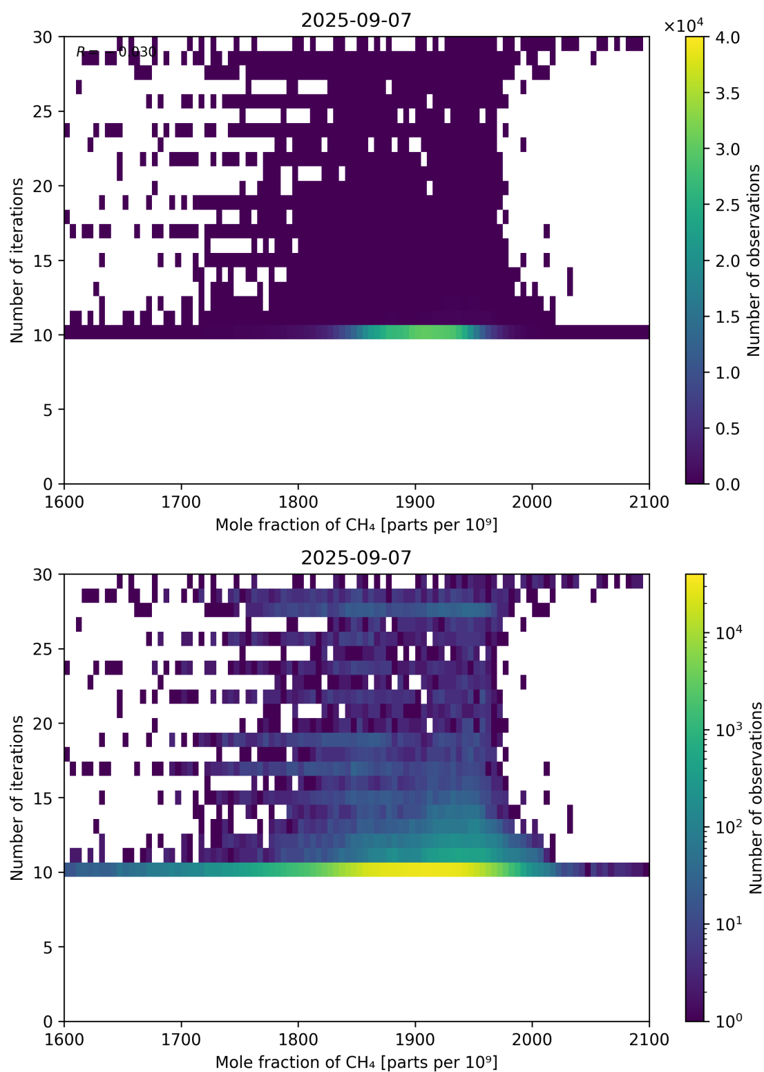
Figure 76: Scatter density plot of “Mole fraction of CH 4 ” against “Number of iterations” for 2025-09-06 to 2025-09-08.
