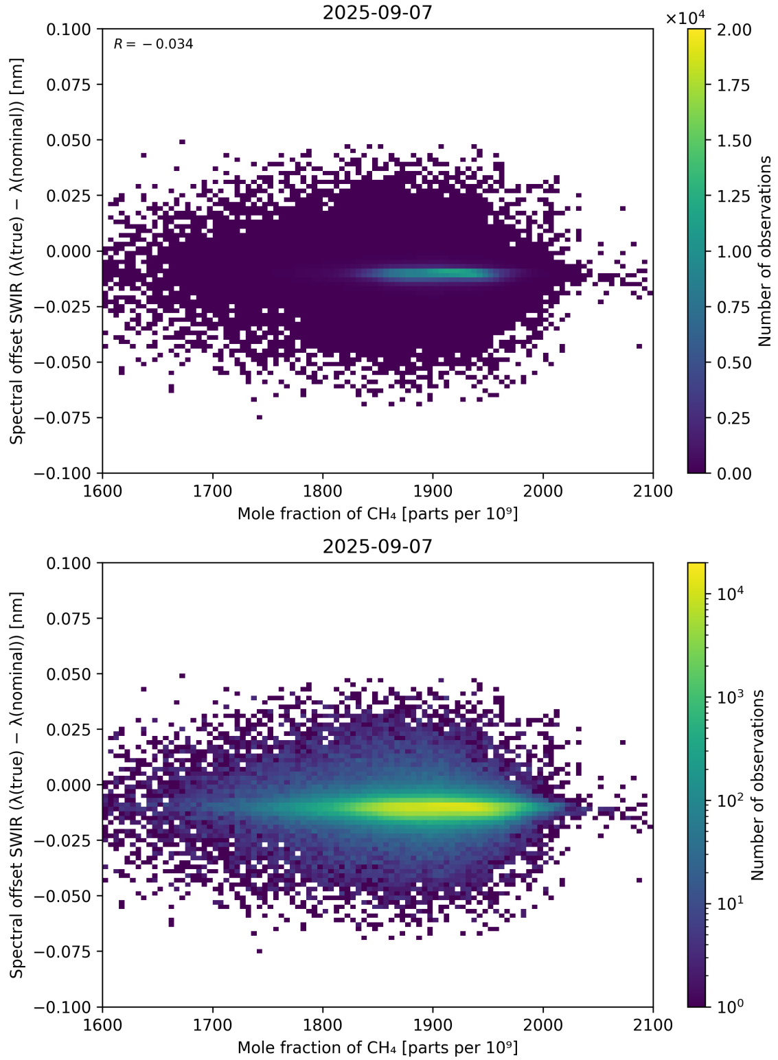
Figure 86: Scatter density plot of “Mole fraction of CH 4 ” against “Spectral offset SWIR ( \lambda_{\text{true}} - \lambda_{\text{nominal}} )” for 2025-09-06 to 2025-09-08.
