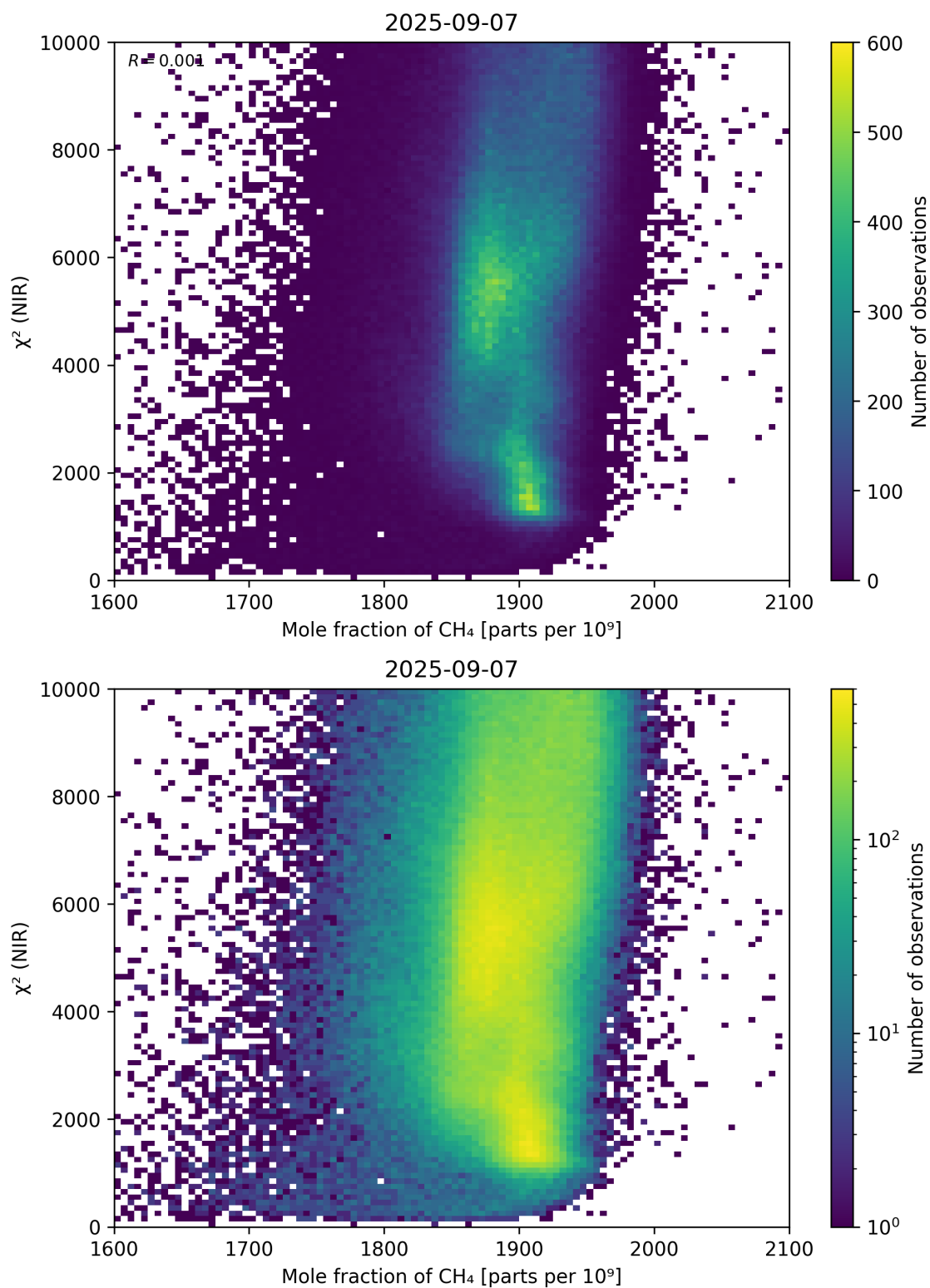
Figure 70: Scatter density plot of “Mole fraction of \text{CH}_4 ” against “ \chi^2 (NIR)” for 2025-09-06 to 2025-09-08.
