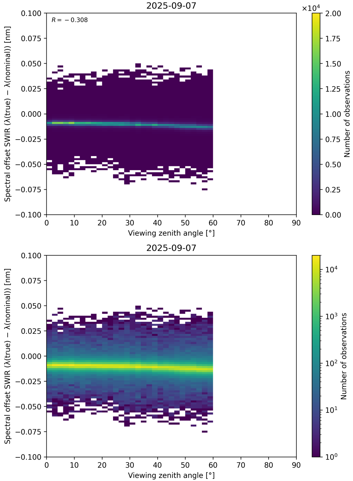
Figure 116: Scatter density plot of “Viewing zenith angle” against “Spectral offset SWIR ( \lambda_{\text{true}} - \lambda_{\text{nominal}} )” for 2025-09-06 to 2025-09-08.
