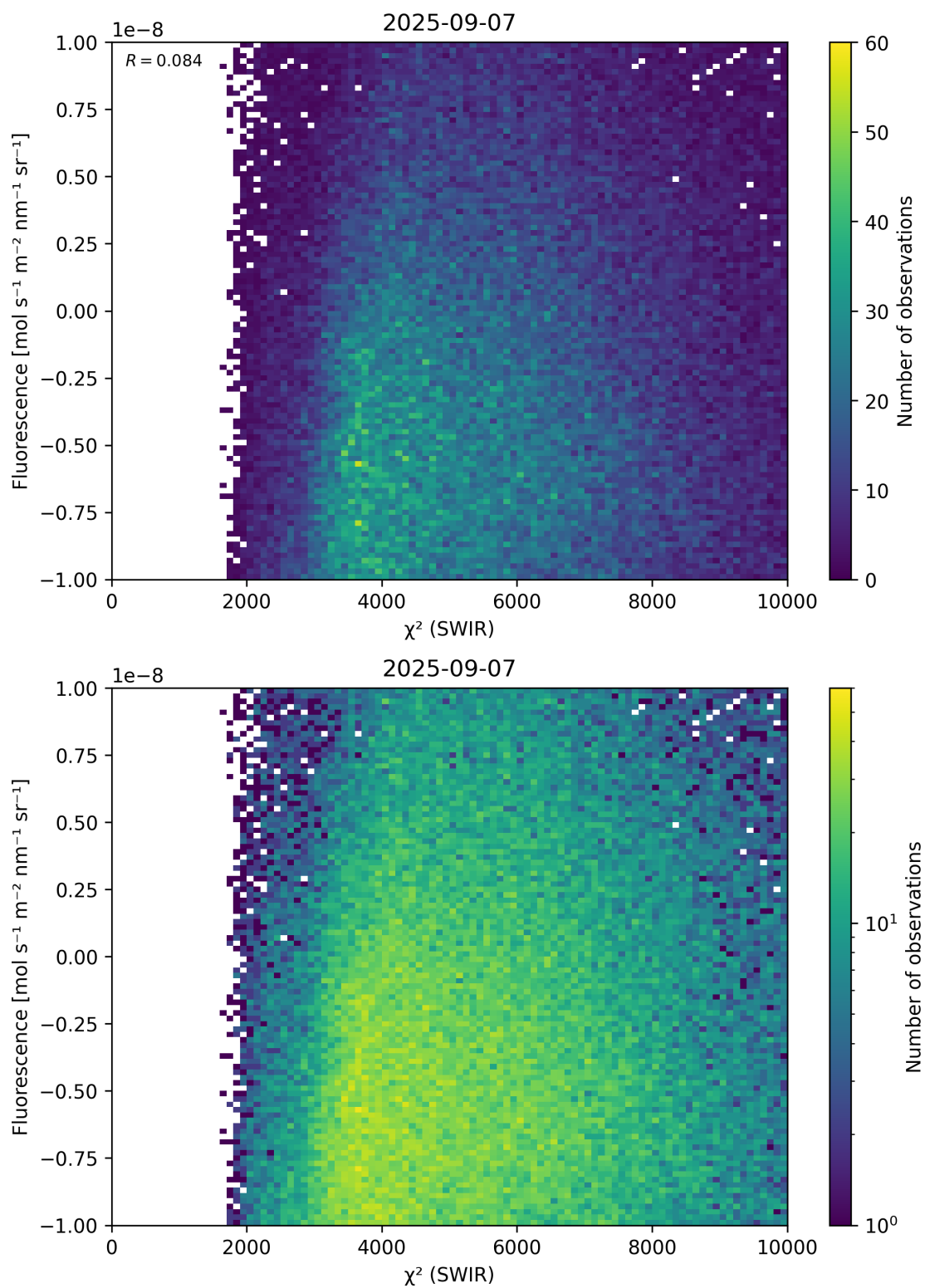
Figure 49: Scatter density plot of “ \chi^2 (SWIR)” against “Fluorescence” for 2025-09-06 to 2025-09-08.
