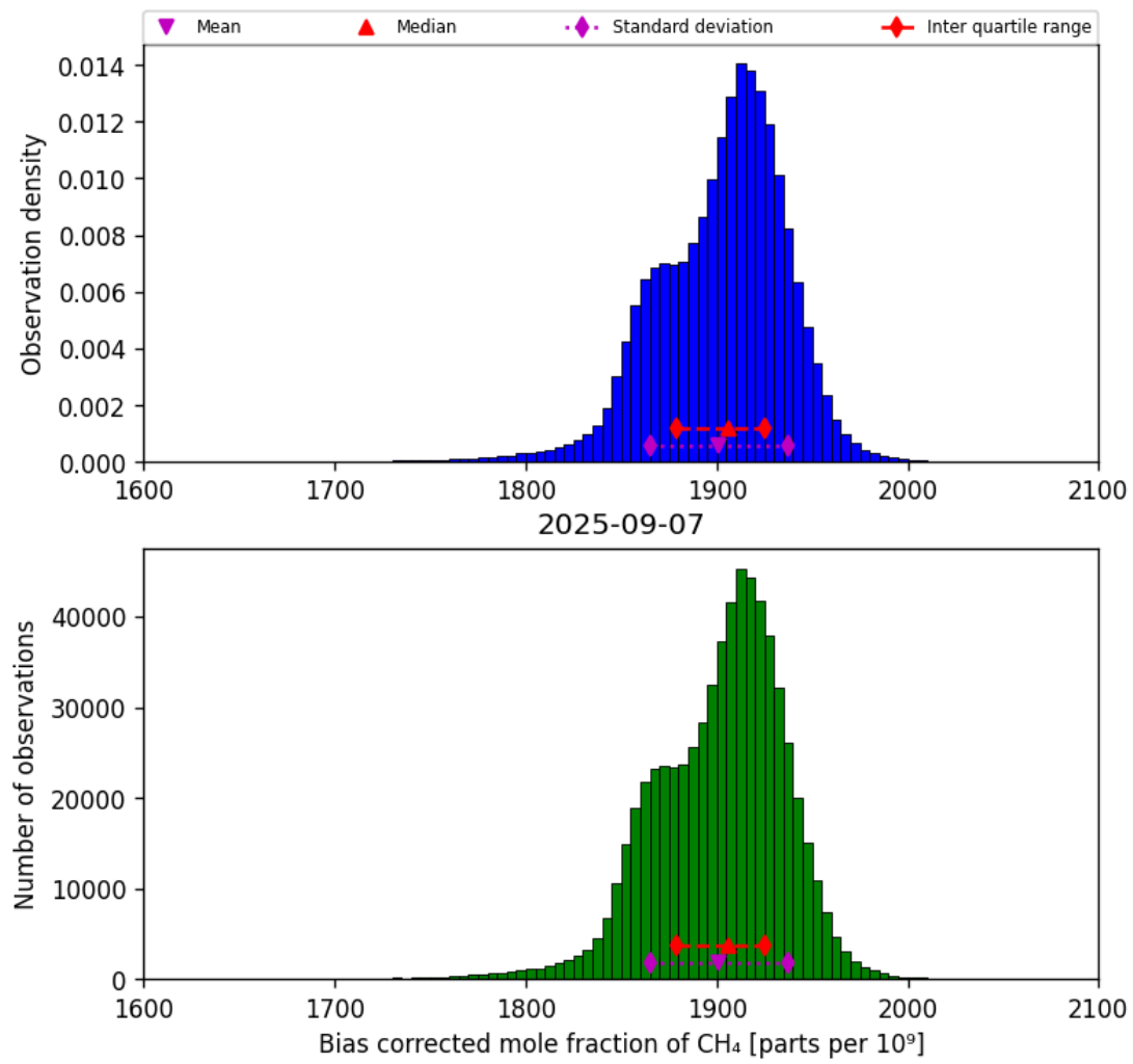
Figure 25: Histogram of “Bias corrected mole fraction of CH 4 ” for 2025-09-06 to 2025-09-08
