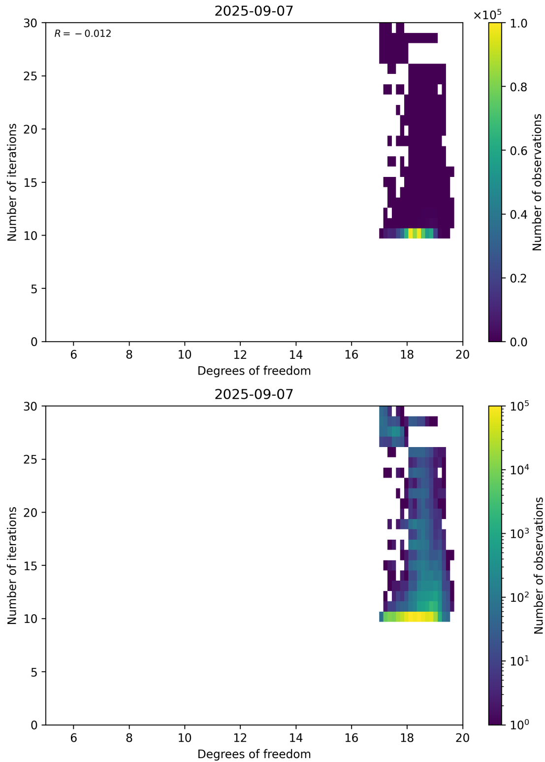
Figure 52: Scatter density plot of “Degrees of freedom” against “Number of iterations” for 2025-09-06 to 2025-09-08.
