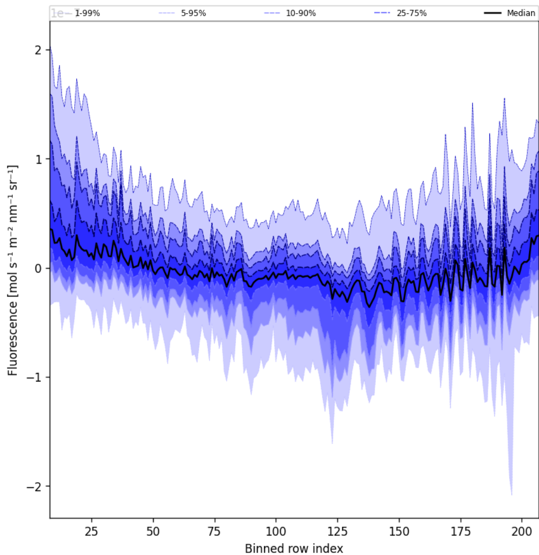
Figure 43: Along track statistics of “Fluorescence” for 2025-09-06 to 2025-09-08
