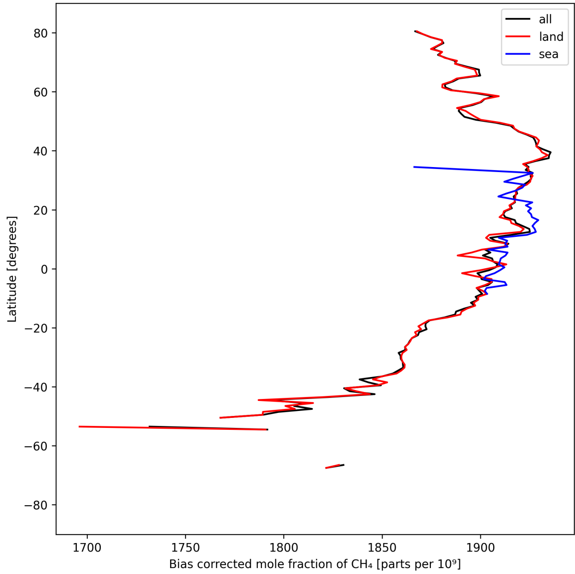
Figure 14: Zonal average of “Bias corrected mole fraction of CH 4 ” for 2025-09-06 to 2025-09-08.
