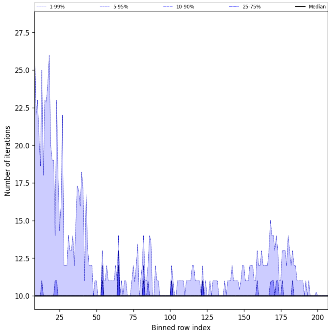
Figure 42: Along track statistics of “Number of iterations” for 2025-09-06 to 2025-09-08
