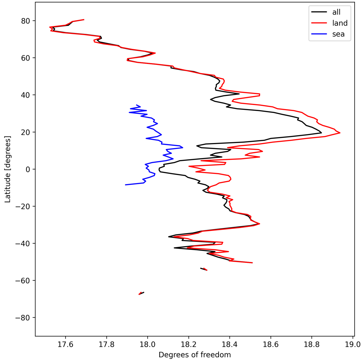
Figure 19: Zonal average of “Degrees of freedom” for 2025-09-06 to 2025-09-08.
