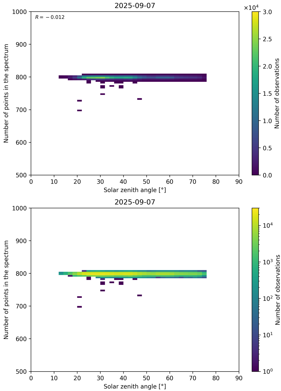
Figure 103: Scatter density plot of “Solar zenith angle” against “Number of points in the spectrum” for 2025-09-06 to 2025-09-08.
