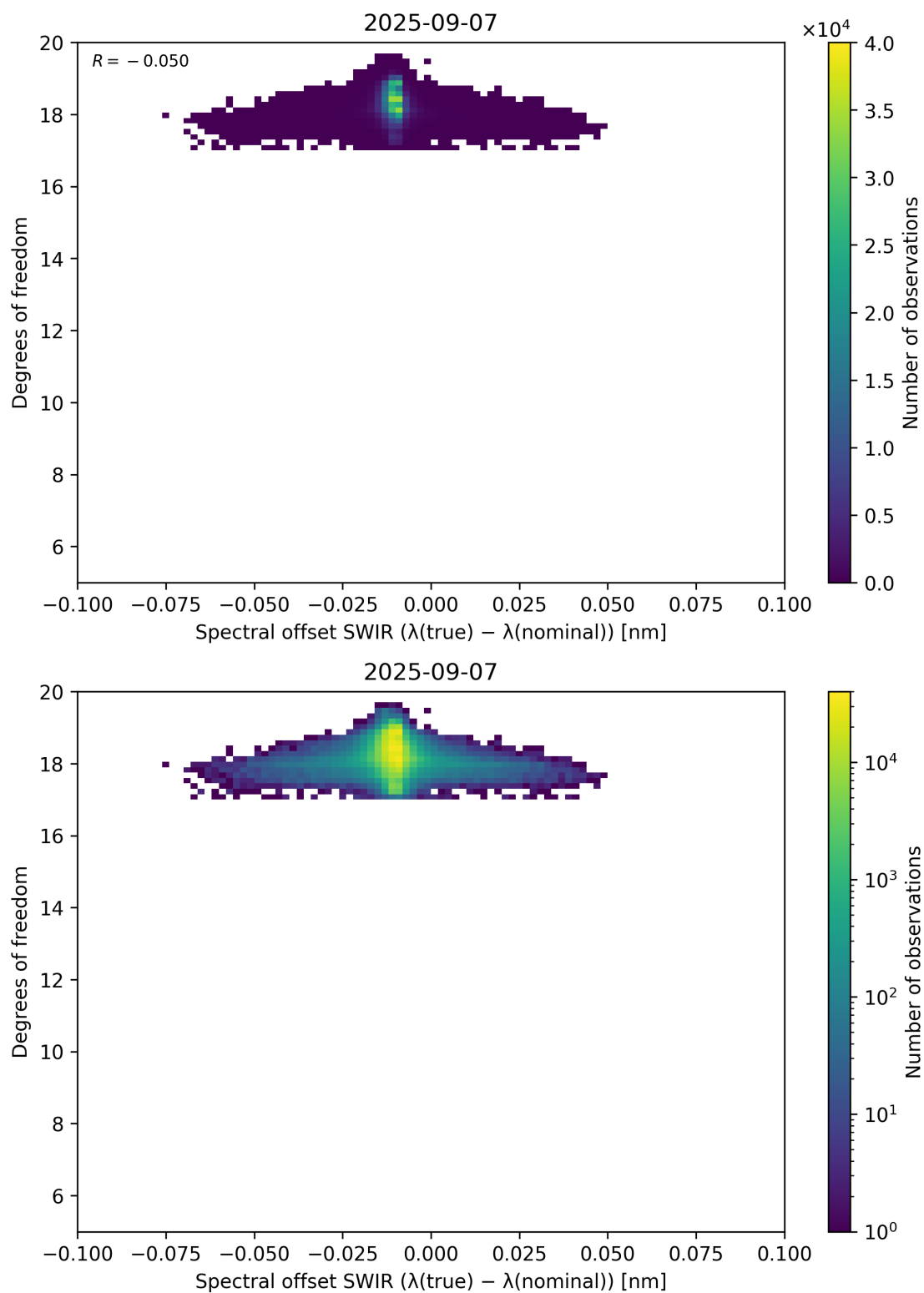
Figure 119: Scatter density plot of “Spectral offset SWIR ( \lambda_{\text{true}} - \lambda_{\text{nominal}} )” against “Degrees of freedom” for 2025-09-06 to 2025-09-08.
