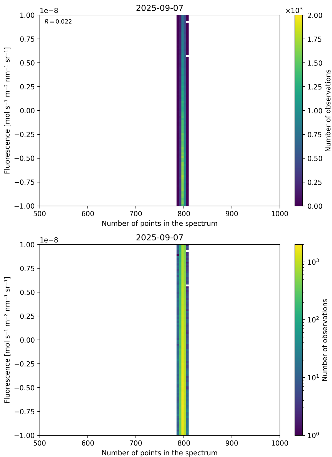
Figure 91: Scatter density plot of “Number of points in the spectrum” against “Fluorescence” for 2025-09-06 to 2025-09-08.
