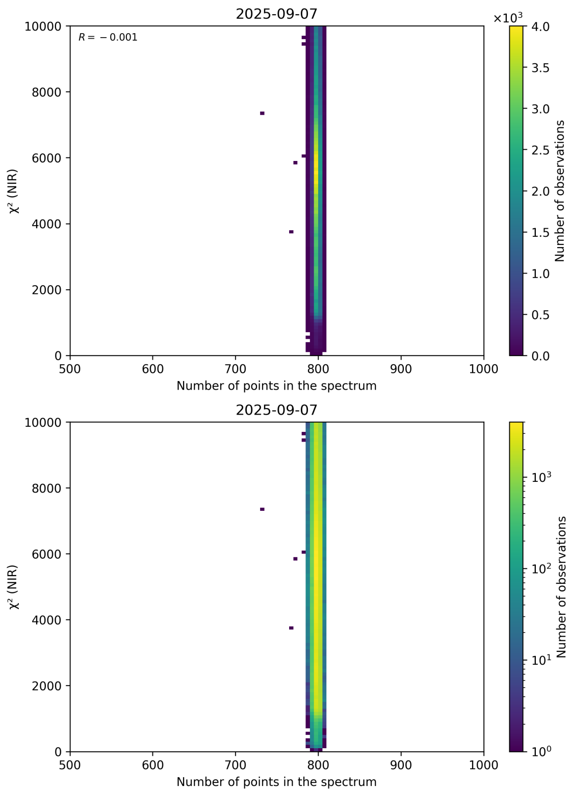
Figure 88: Scatter density plot of “Number of points in the spectrum” against “ \chi^2 (NIR)” for 2025-09-06 to 2025-09-08.
