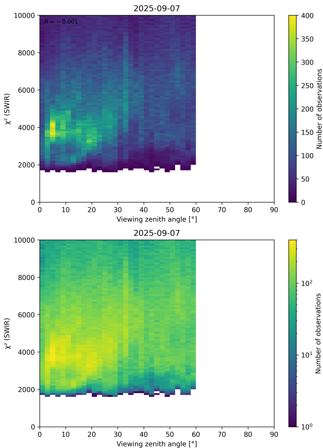
Figure 106: Scatter density plot of “Viewing zenith angle” against “ \chi^2 (SWIR)” for 2025-09-06 to 2025-09-08.
