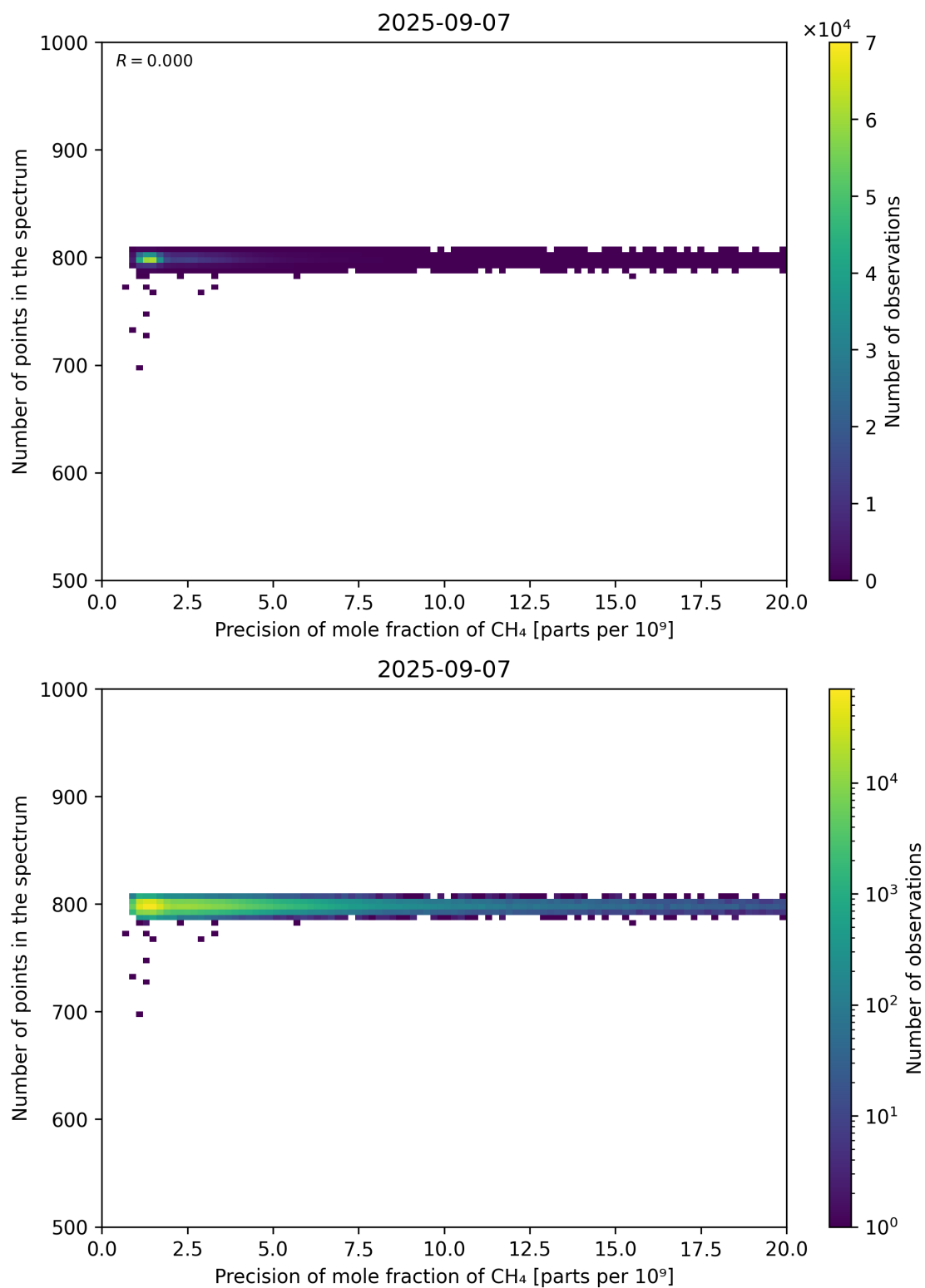
Figure 84: Scatter density plot of “Precision of mole fraction of CH 4 ” against “Number of points in the spectrum” for 2025-09-06 to 2025-09-08.
