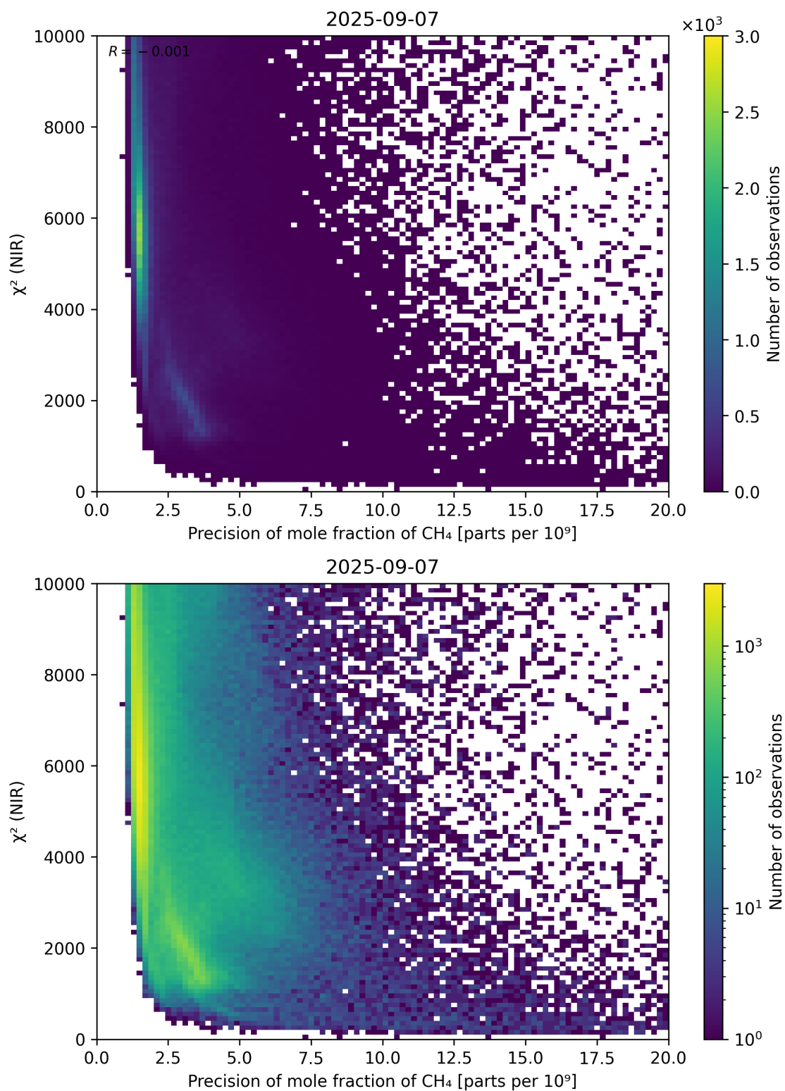
Figure 78: Scatter density plot of “Precision of mole fraction of CH 4 ” against “ \chi^2 (NIR)” for 2025-09-06 to 2025-09-08.
