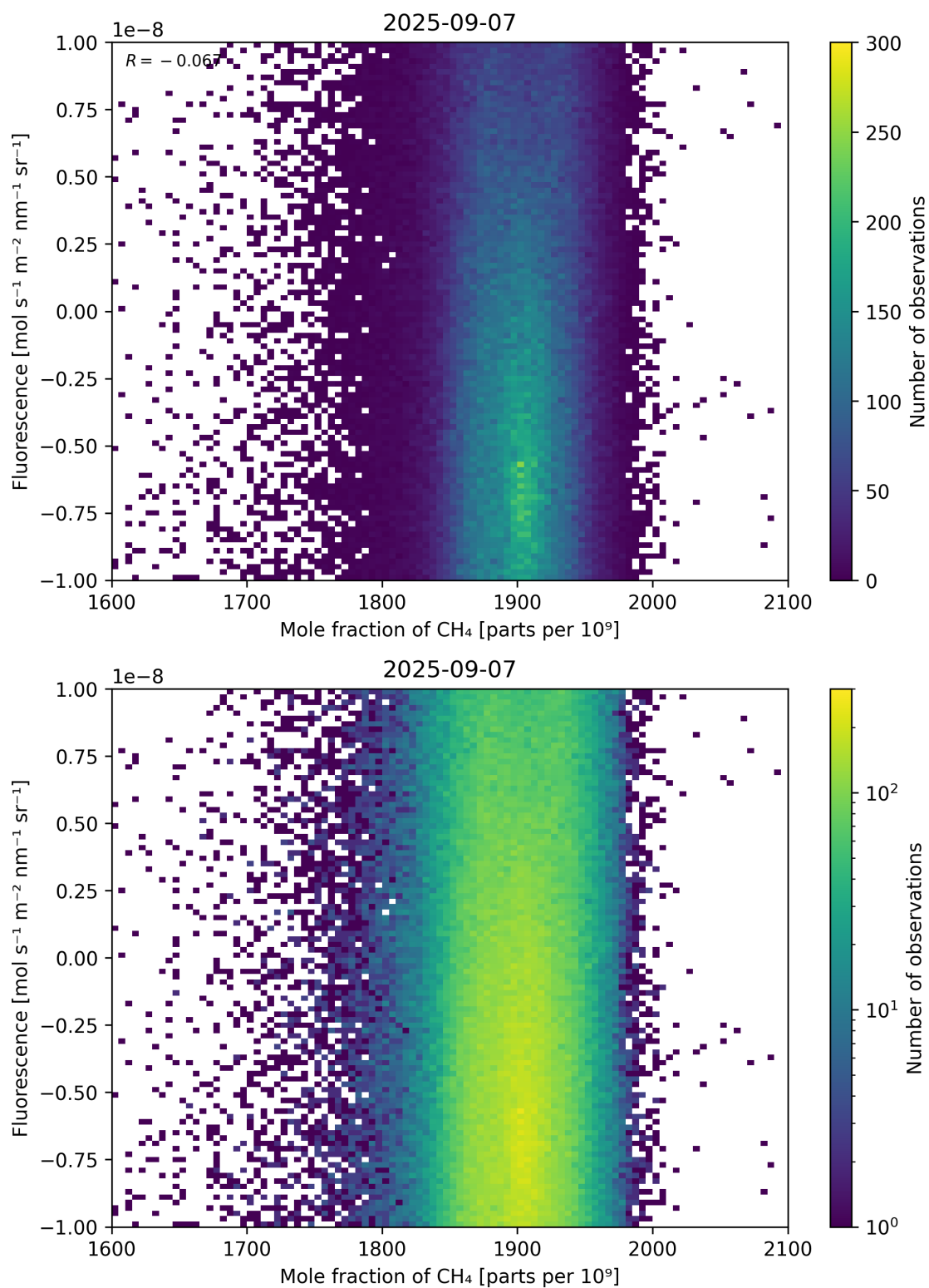
Figure 73: Scatter density plot of “Mole fraction of \text{CH}_4 ” against “Fluorescence” for 2025-09-06 to 2025-09-08.
