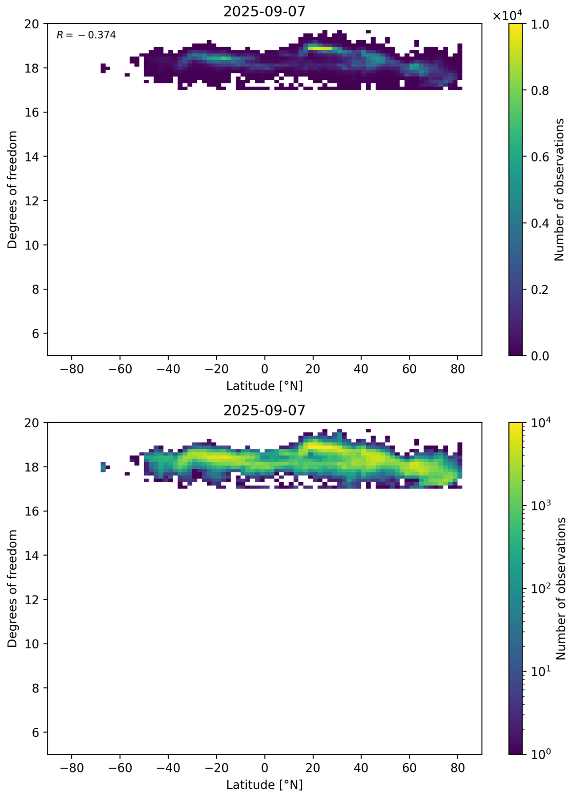
Figure 55: Scatter density plot of “Latitude” against “Degrees of freedom” for 2025-09-06 to 2025-09-08.
