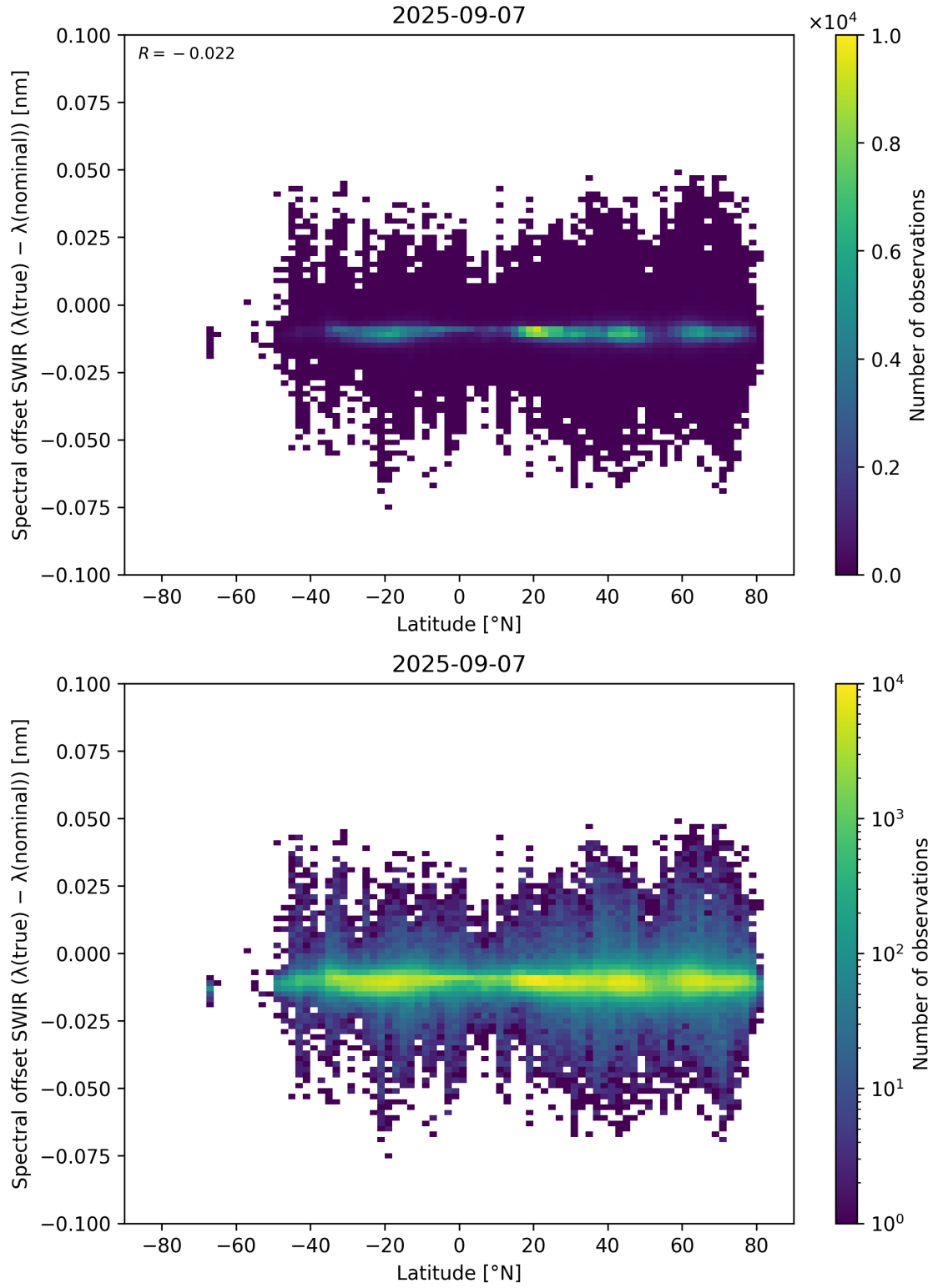
Figure 62: Scatter density plot of “Latitude” against “Spectral offset SWIR ( \lambda_{\text{true}} - \lambda_{\text{nominal}} )” for 2025-09-06 to 2025-09-08.
