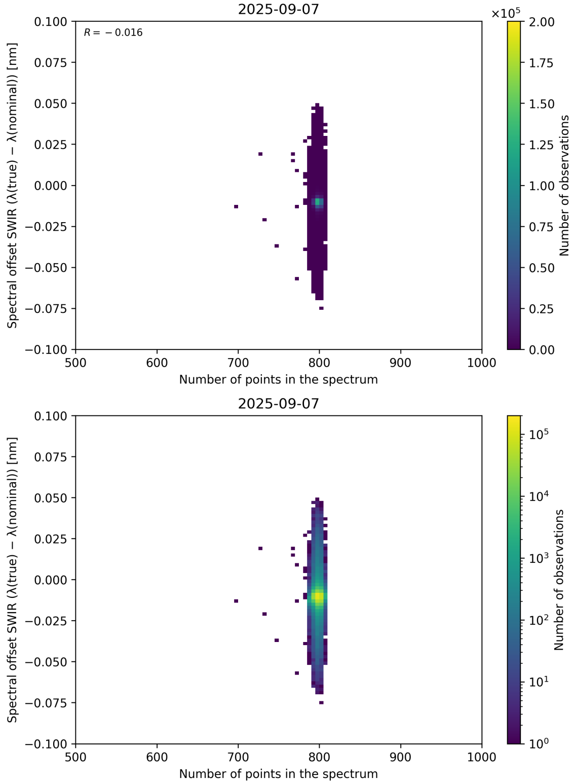
Figure 93: Scatter density plot of “Number of points in the spectrum” against “Spectral offset SWIR ( \lambda_{\text{true}} - \lambda_{\text{nominal}} )” for 2025-09-06 to 2025-09-08.
