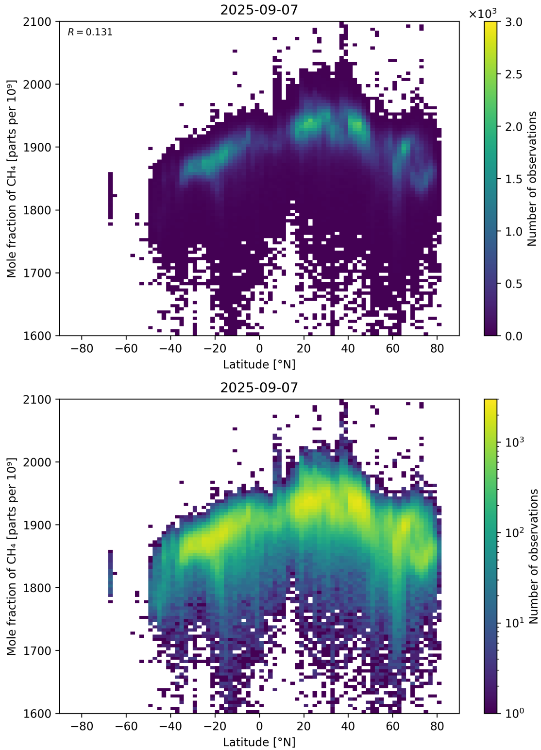
Figure 57: Scatter density plot of “Latitude” against “Mole fraction of \text{CH}_4 ” for 2025-09-06 to 2025-09-08.
