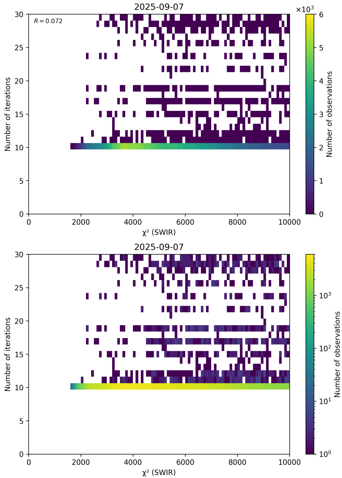
Figure 50: Scatter density plot of “ \chi^2 (SWIR)” against “Number of iterations” for 2025-09-06 to 2025-09-08.
