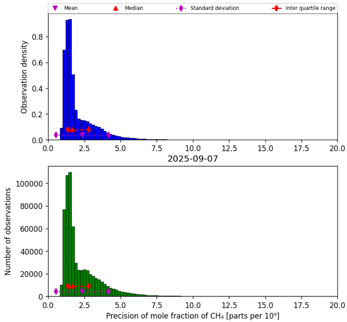
Figure 24: Histogram of “Precision of mole fraction of CH 4 ” for 2025-09-06 to 2025-09-08
