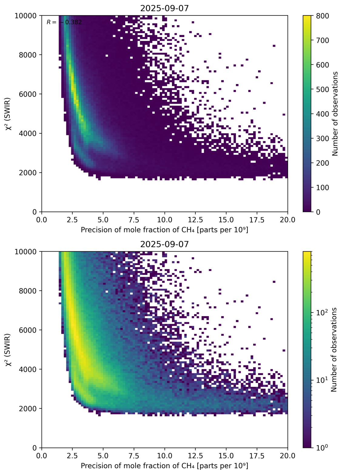
Figure 79: Scatter density plot of “Precision of mole fraction of CH 4 ” against “ \chi^2 (SWIR)” for 2025-09-06 to 2025-09-08.
