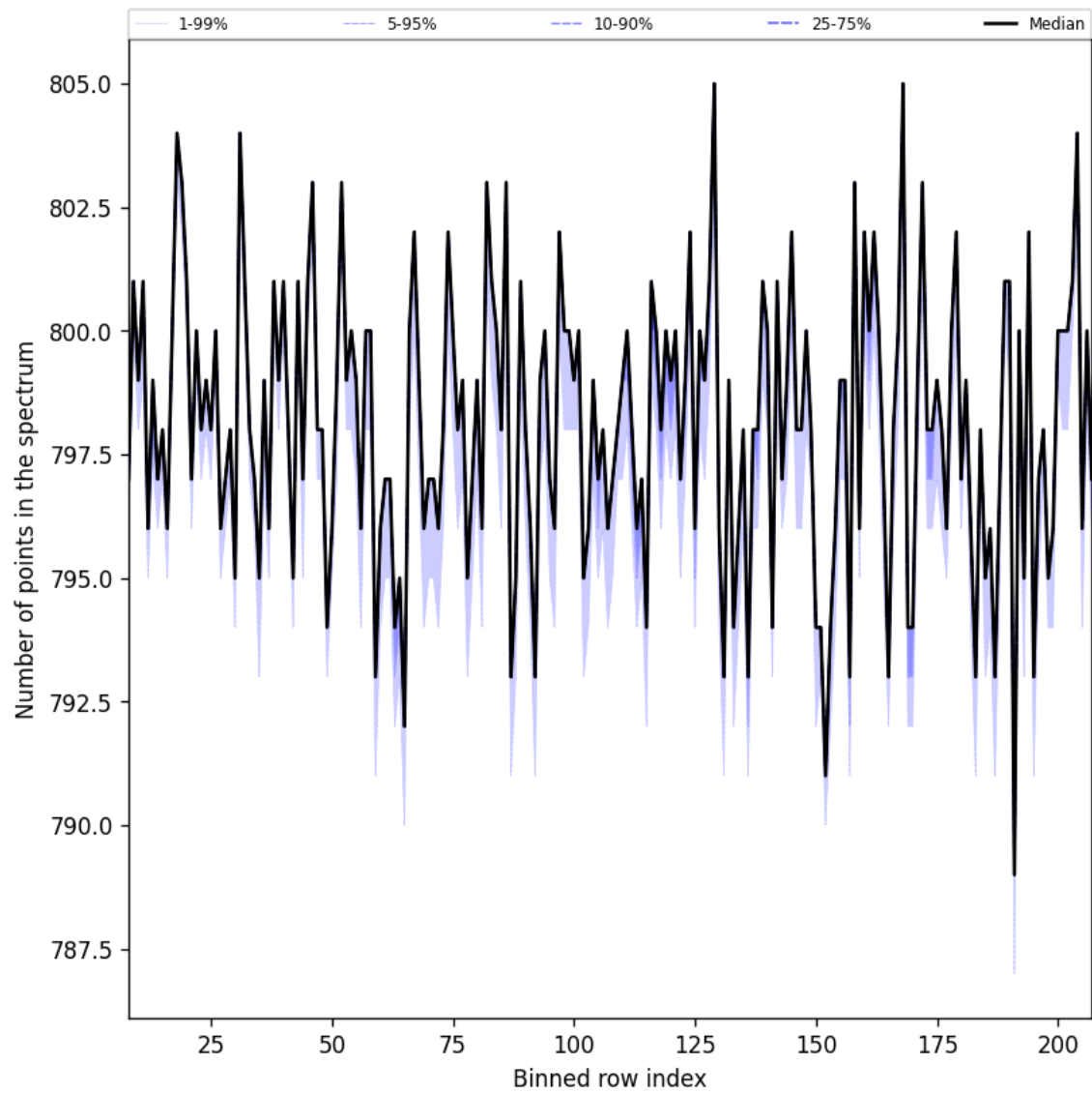
Figure 37: Along track statistics of “Number of points in the spectrum” for 2025-09-06 to 2025-09-08
