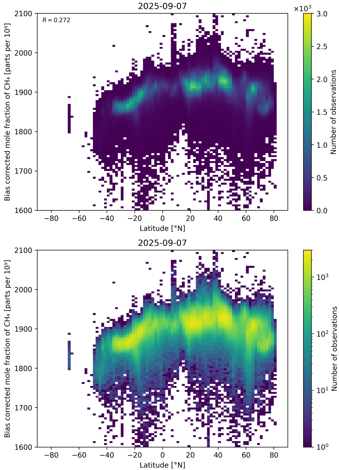
Figure 58: Scatter density plot of “Latitude” against “Bias corrected mole fraction of \text{CH}_4 ” for 2025-09-06 to 2025-09-08.
