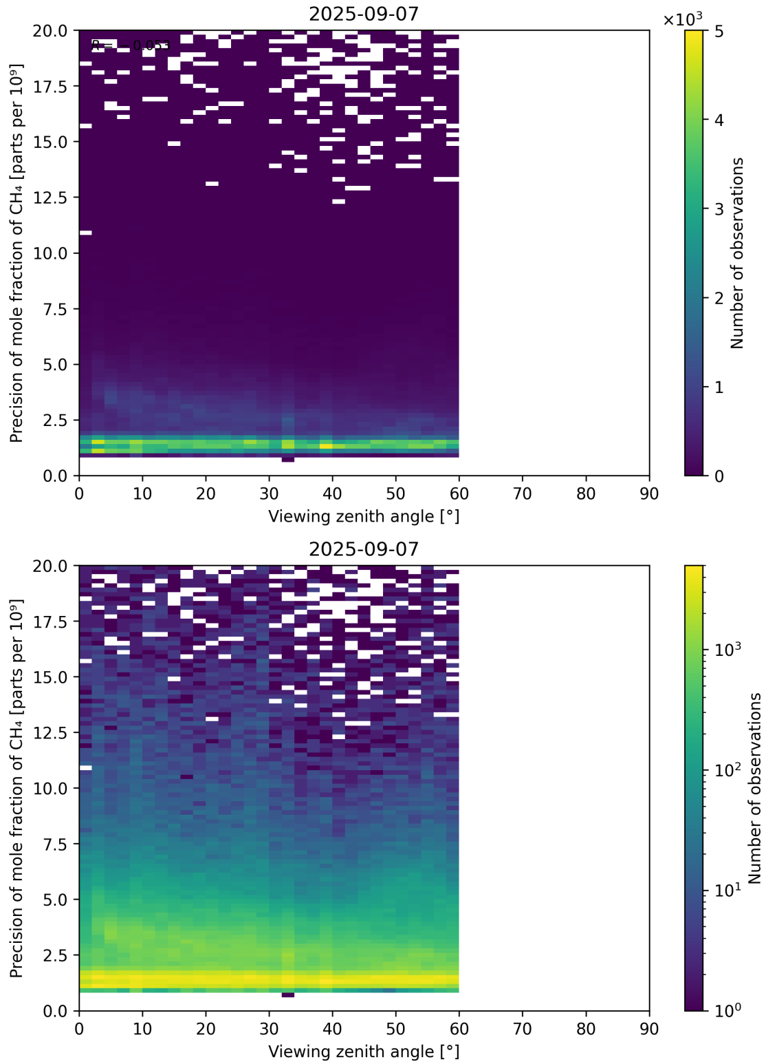
Figure 112: Scatter density plot of “Viewing zenith angle” against “Precision of mole fraction of CH 4 ” for 2025-09-06 to 2025-09-08.
