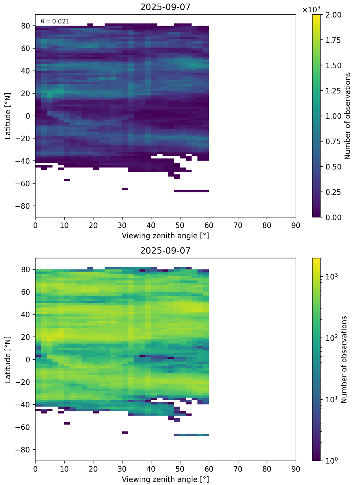
Figure 109: Scatter density plot of “Viewing zenith angle” against “Latitude” for 2025-09-06 to 2025-09-08.
