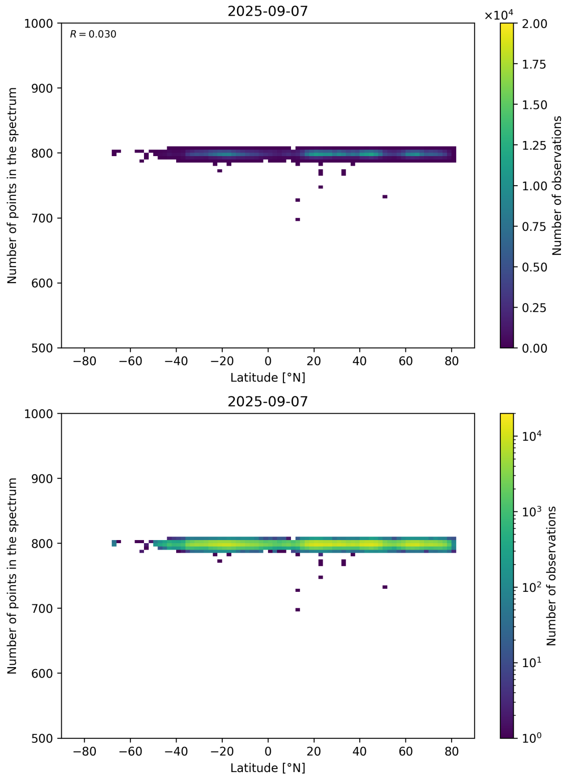
Figure 61: Scatter density plot of “Latitude” against “Number of points in the spectrum” for 2025-09-06 to 2025-09-08.
