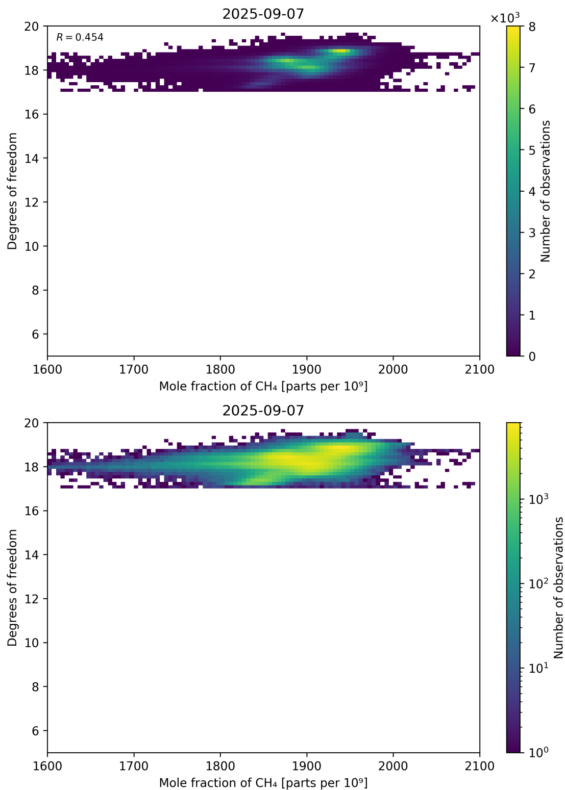
Figure 72: Scatter density plot of “Mole fraction of CH 4 ” against “Degrees of freedom” for 2025-09-06 to 2025-09-08.
