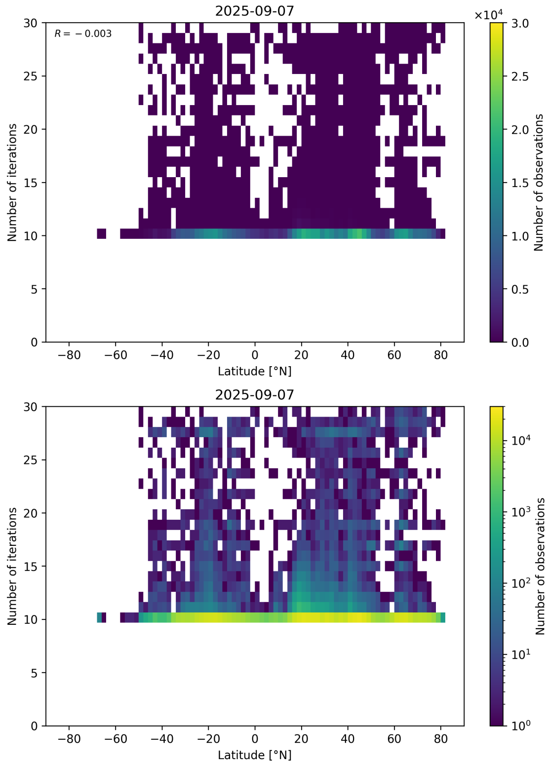
Figure 60: Scatter density plot of “Latitude” against “Number of iterations” for 2025-09-06 to 2025-09-08.
