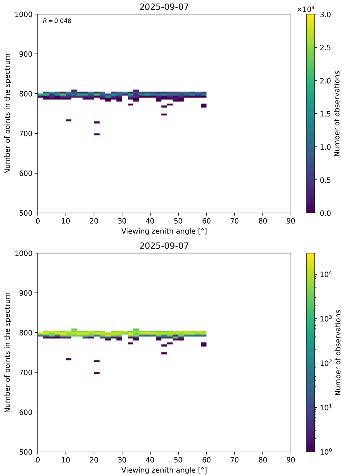
Figure 114: Scatter density plot of “Viewing zenith angle” against “Number of points in the spectrum” for 2025-09-06 to 2025-09-08.
