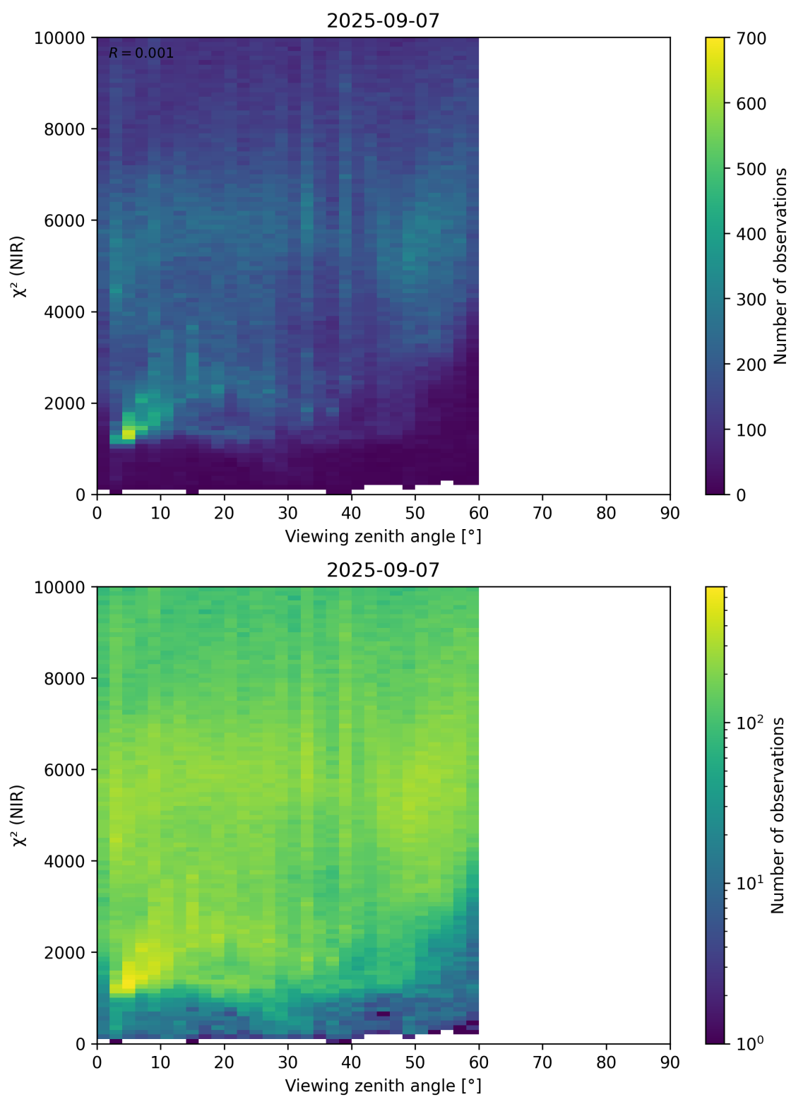
Figure 105: Scatter density plot of “Viewing zenith angle” against “ \chi^2 (NIR)” for 2025-09-06 to 2025-09-08.
