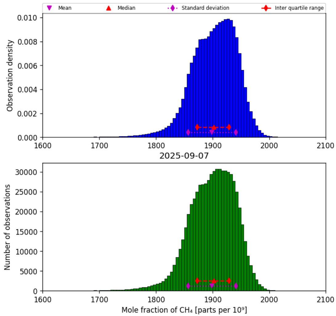
Figure 23: Histogram of “Mole fraction of CH 4 ” for 2025-09-06 to 2025-09-08
