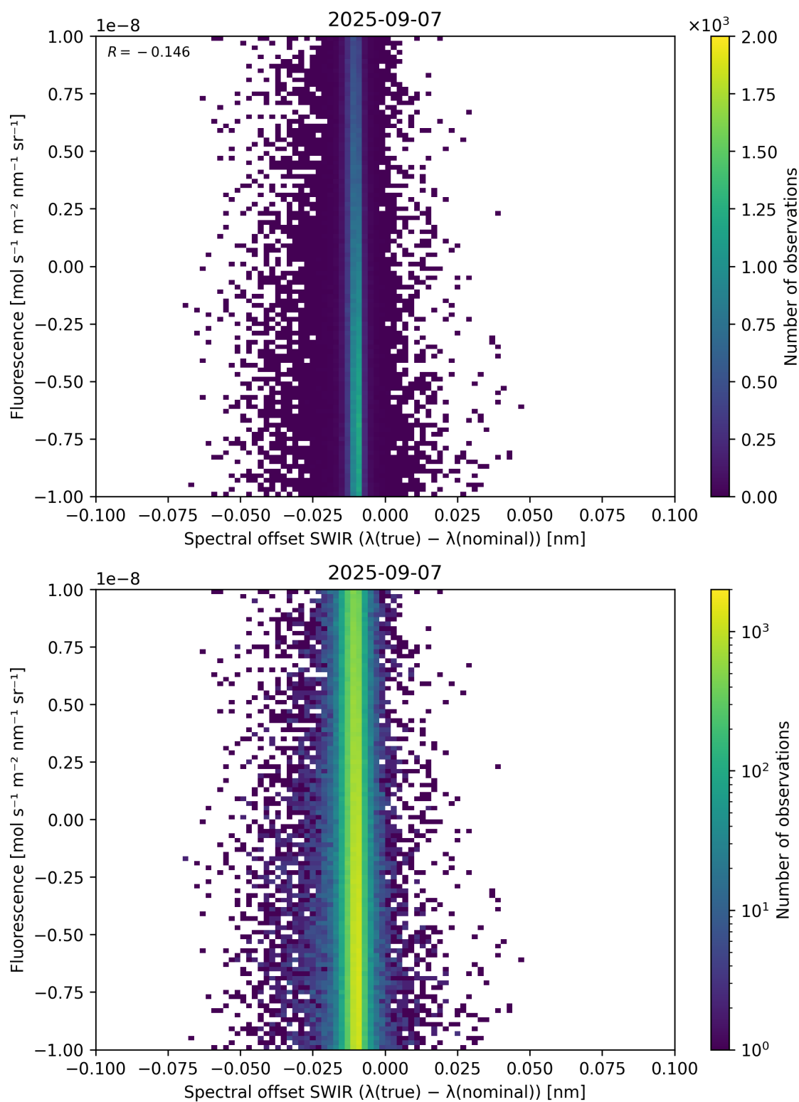
Figure 120: Scatter density plot of “Spectral offset SWIR ( \lambda_{\text{true}} - \lambda_{\text{nominal}} )” against “Fluorescence” for 2025-09-06 to 2025-09-08.
