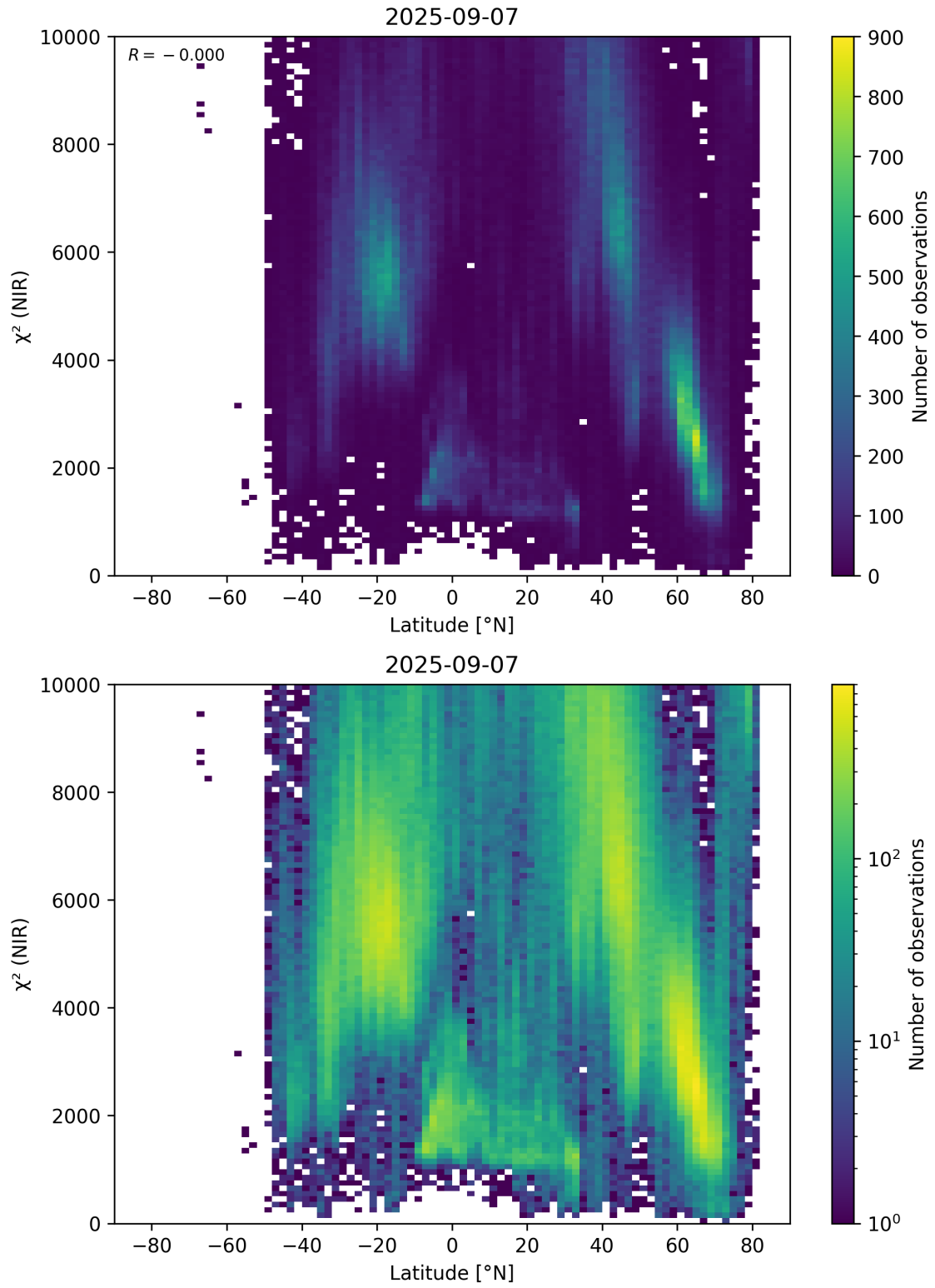
Figure 53: Scatter density plot of “Latitude” against “ \chi^2 (NIR)” for 2025-09-06 to 2025-09-08.
