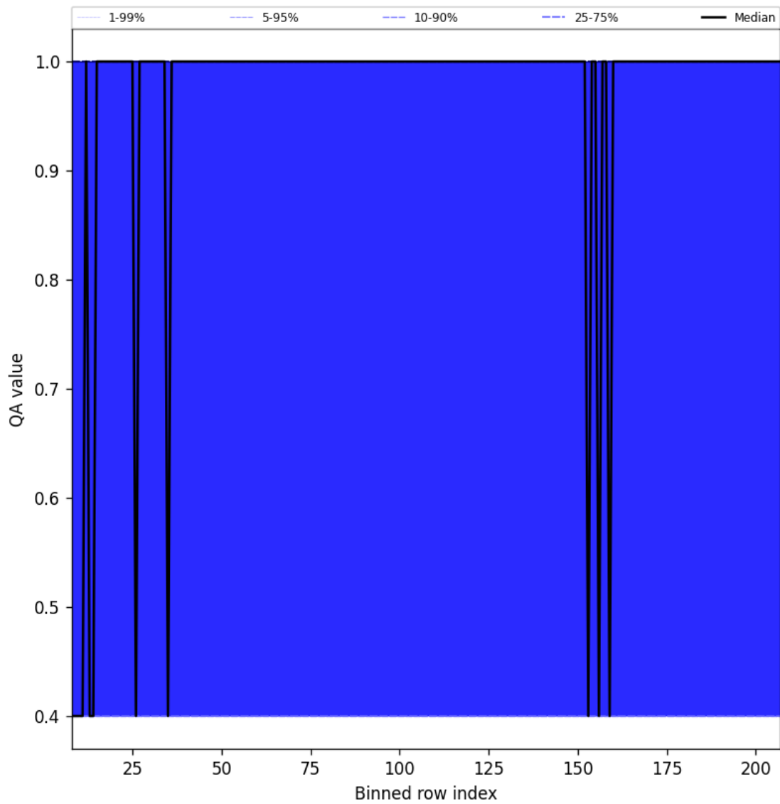
Figure 33: Along track statistics of “QA value” for 2025-09-06 to 2025-09-08
