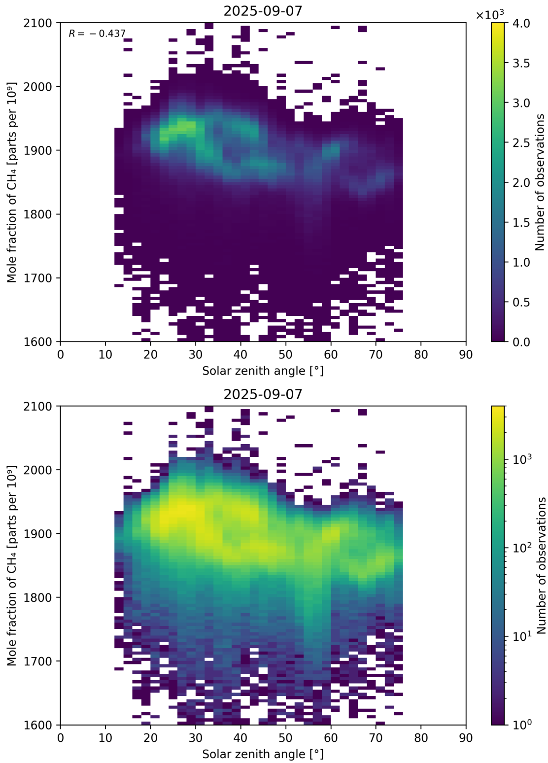
Figure 99: Scatter density plot of “Solar zenith angle” against “Mole fraction of CH 4 ” for 2025-09-06 to 2025-09-08.
