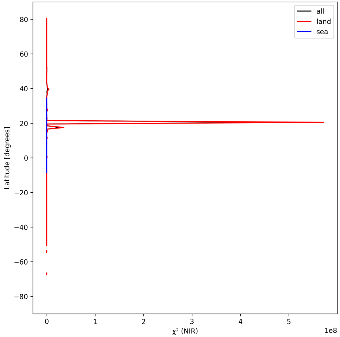
Figure 18: Zonal average of “ \chi^2 (NIR)” for 2025-09-06 to 2025-09-08.
