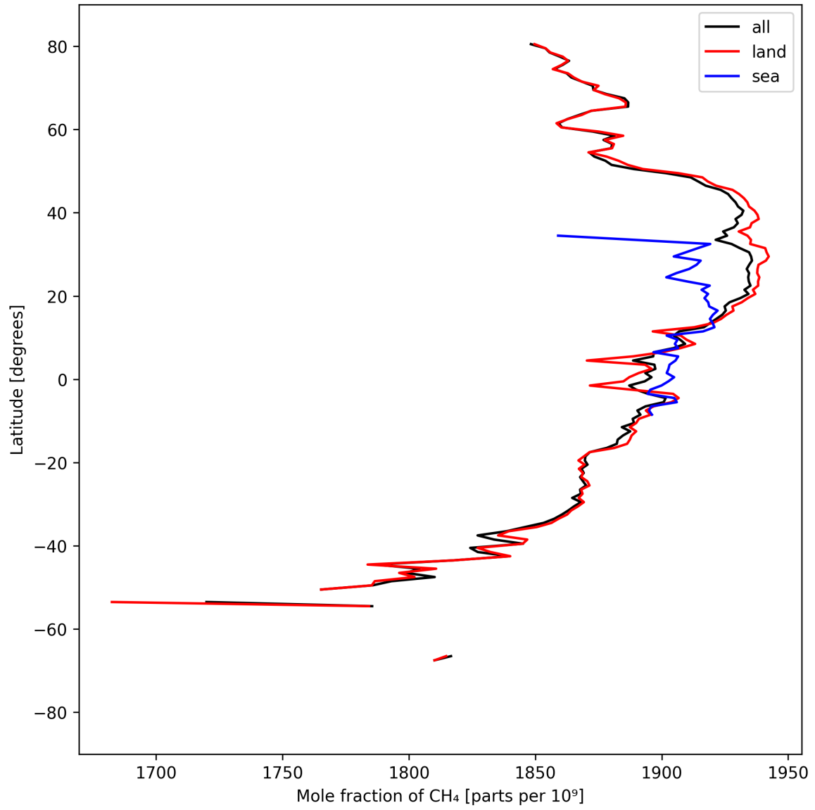
Figure 12: Zonal average of “Mole fraction of \text{CH}_4 ” for 2025-09-06 to 2025-09-08.
