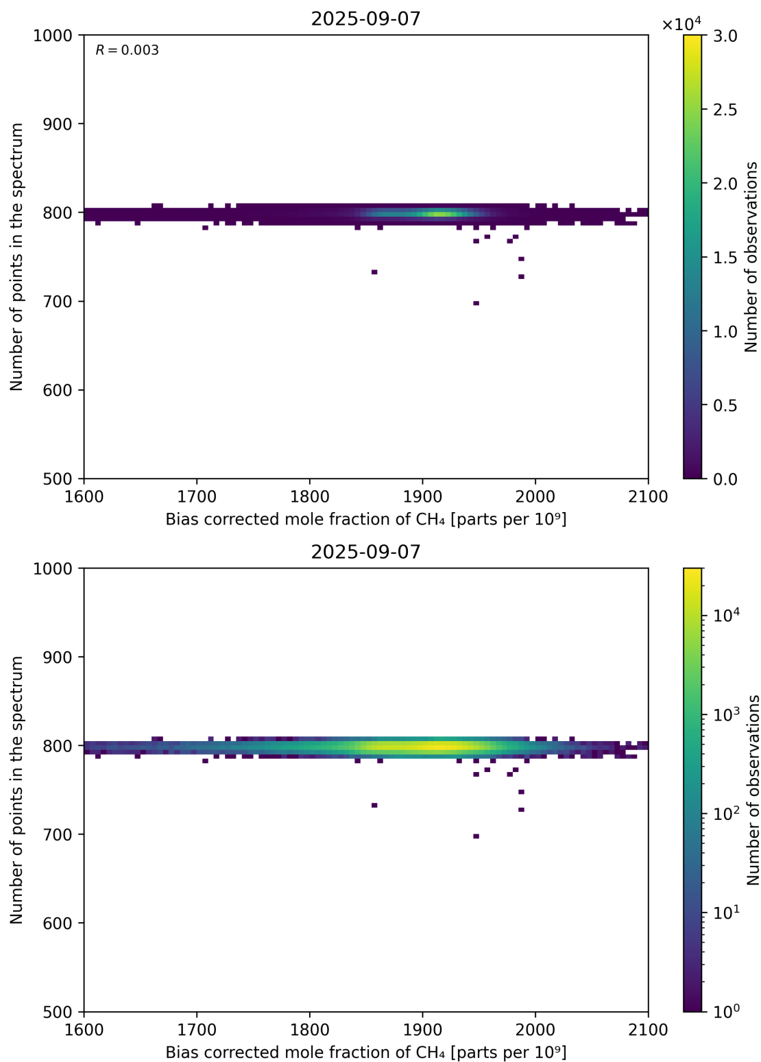
Figure 68: Scatter density plot of “Bias corrected mole fraction of CH 4 ” against “Number of points in the spectrum” for 2025-09-06 to 2025-09-08.
