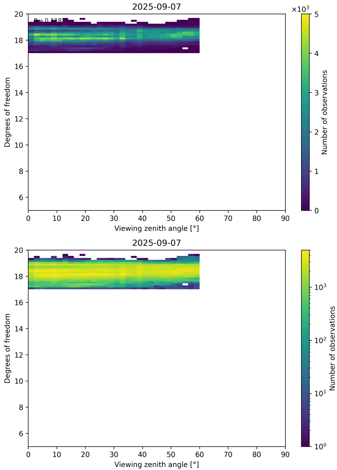
Figure 107: Scatter density plot of “Viewing zenith angle” against “Degrees of freedom” for 2025-09-06 to 2025-09-08.
