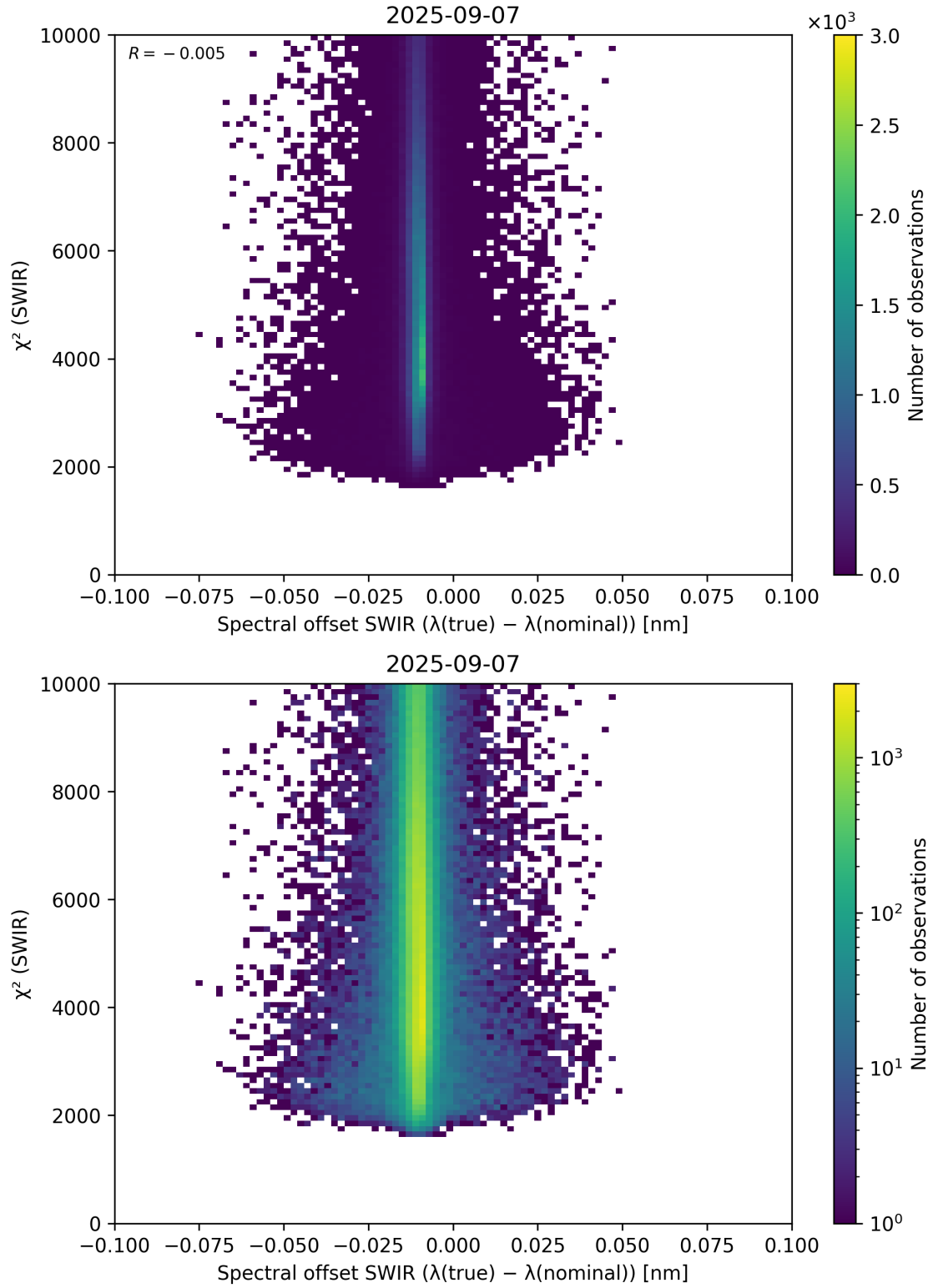
Figure 118: Scatter density plot of “Spectral offset SWIR ( \lambda_{\text{true}} - \lambda_{\text{nominal}} )” against “ \chi^2 (SWIR)” for 2025-09-06 to 2025-09-08.
