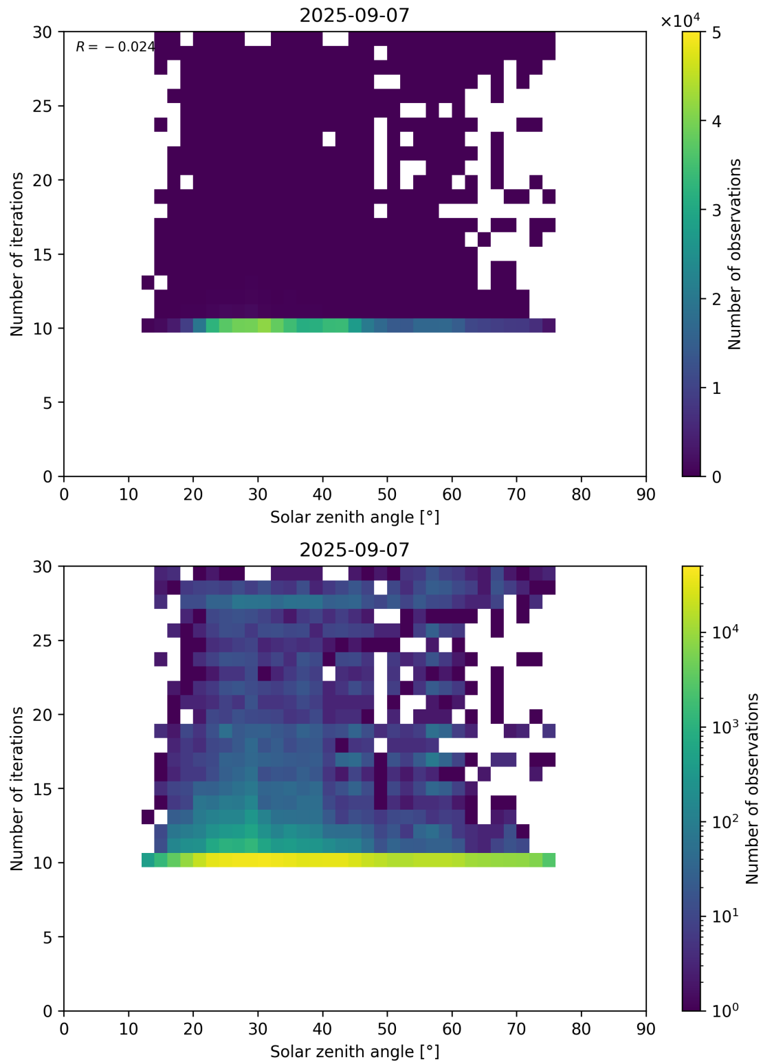
Figure 102: Scatter density plot of “Solar zenith angle” against “Number of iterations” for 2025-09-06 to 2025-09-08.
