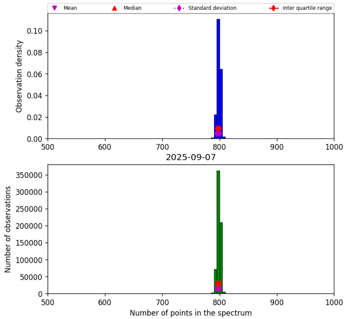
Figure 26: Histogram of “Number of points in the spectrum” for 2025-09-06 to 2025-09-08
