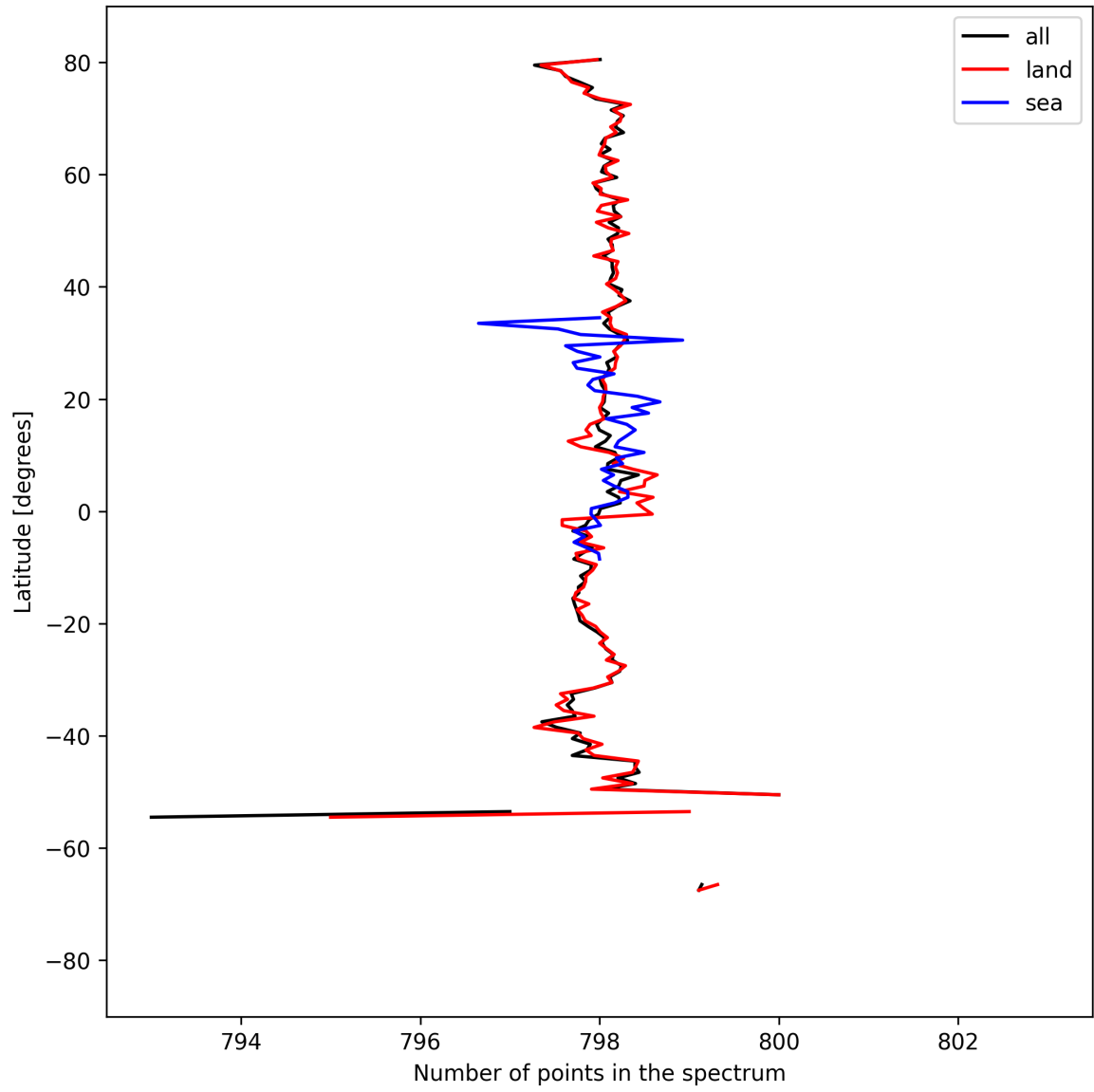
Figure 15: Zonal average of “Number of points in the spectrum” for 2025-09-06 to 2025-09-08.
