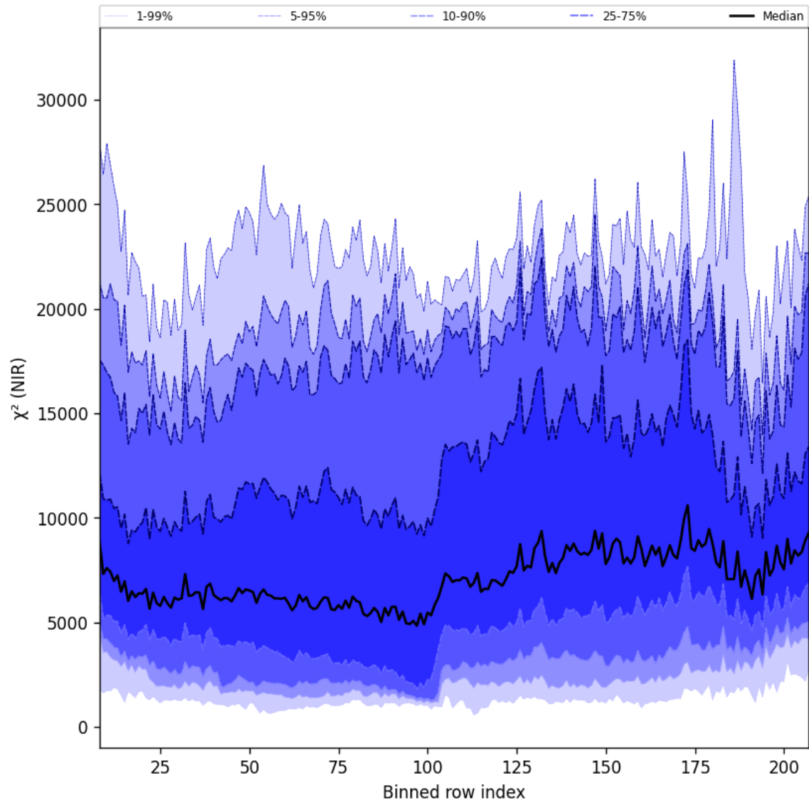
Figure 40: Along track statistics of “ \chi^2 (NIR)” for 2025-09-06 to 2025-09-08
