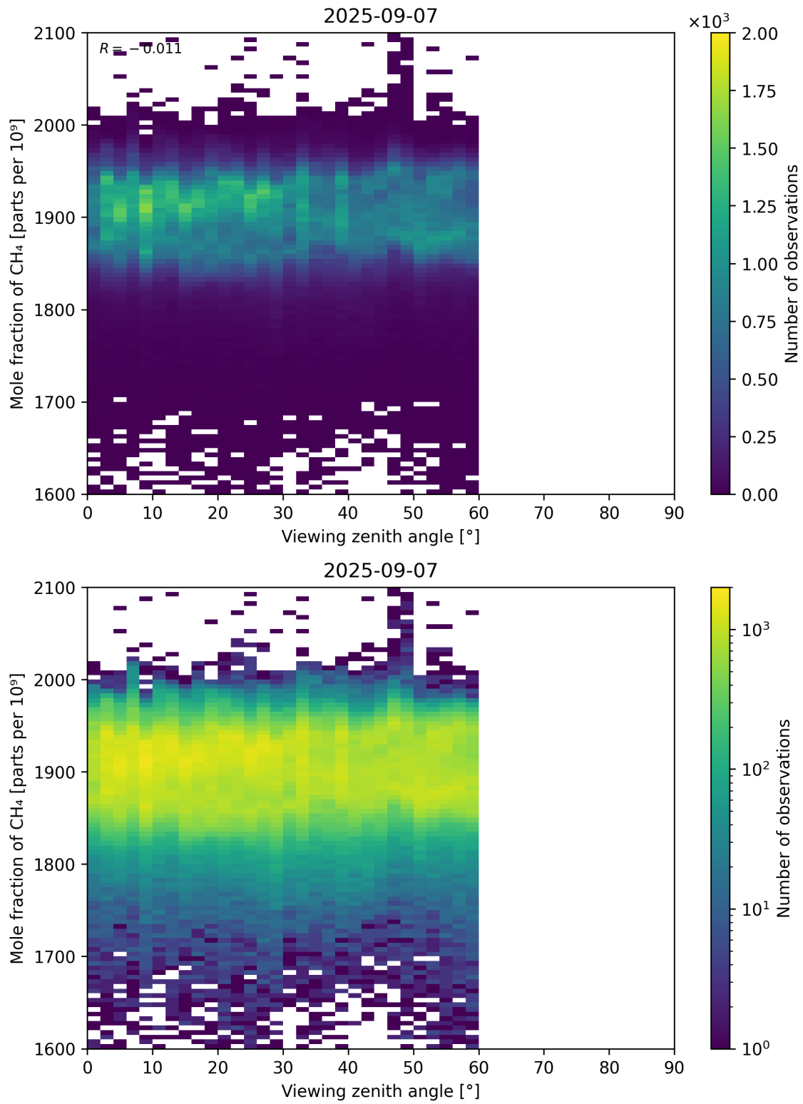
Figure 110: Scatter density plot of “Viewing zenith angle” against “Mole fraction of CH 4 ” for 2025-09-06 to 2025-09-08.
