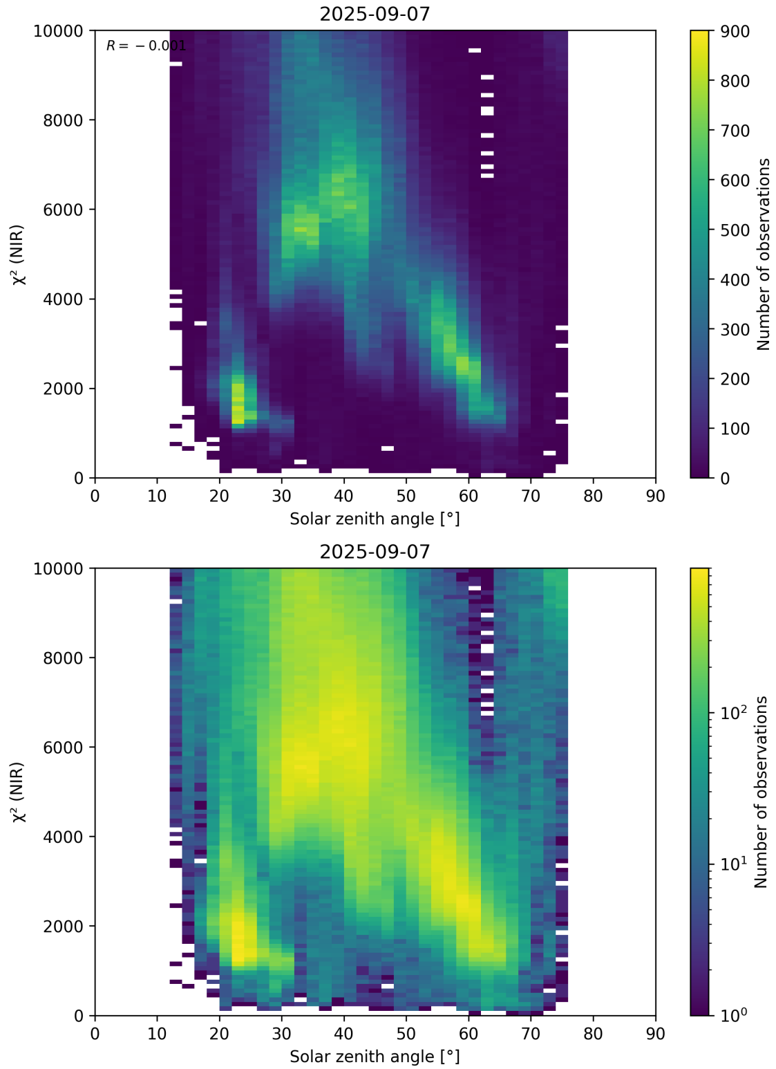
Figure 94: Scatter density plot of “Solar zenith angle” against “ \chi^2 (NIR)” for 2025-09-06 to 2025-09-08.
