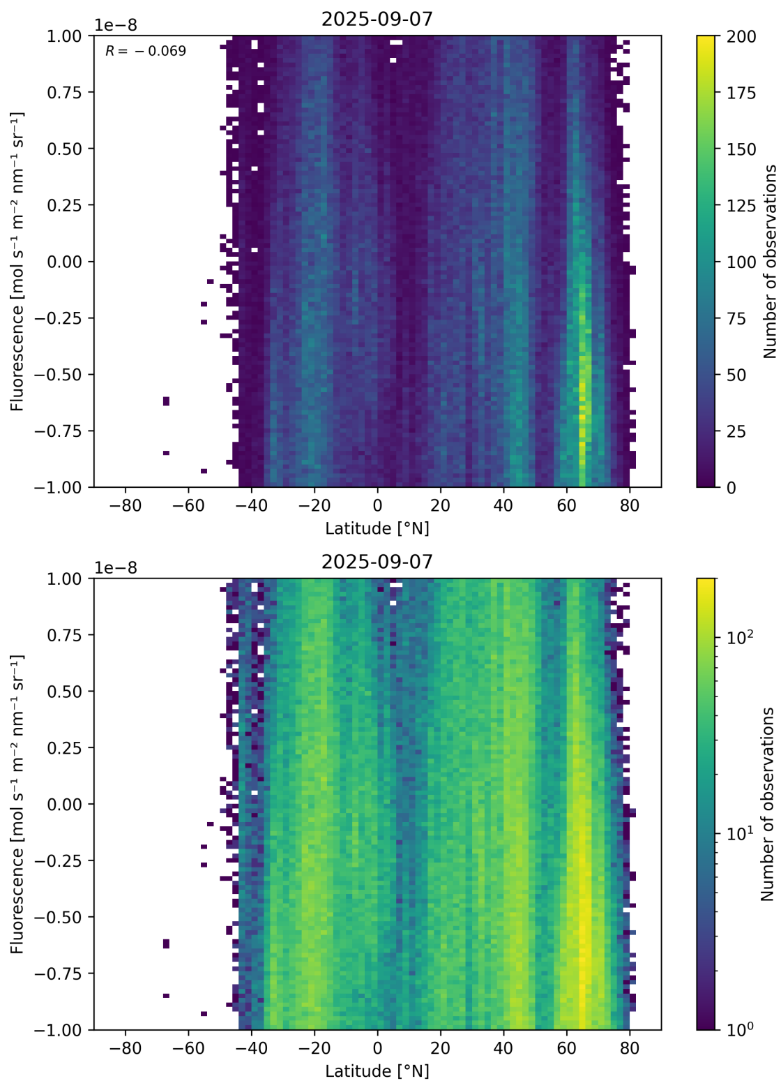
Figure 56: Scatter density plot of “Latitude” against “Fluorescence” for 2025-09-06 to 2025-09-08.
