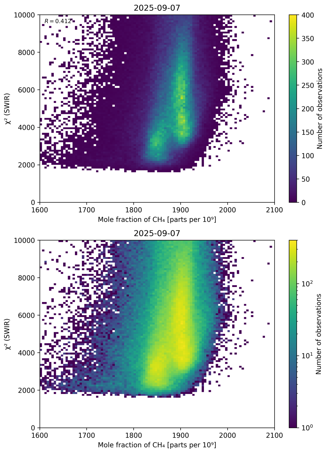
Figure 71: Scatter density plot of “Mole fraction of CH 4 ” against “ \chi^2 (SWIR)” for 2025-09-06 to 2025-09-08.
