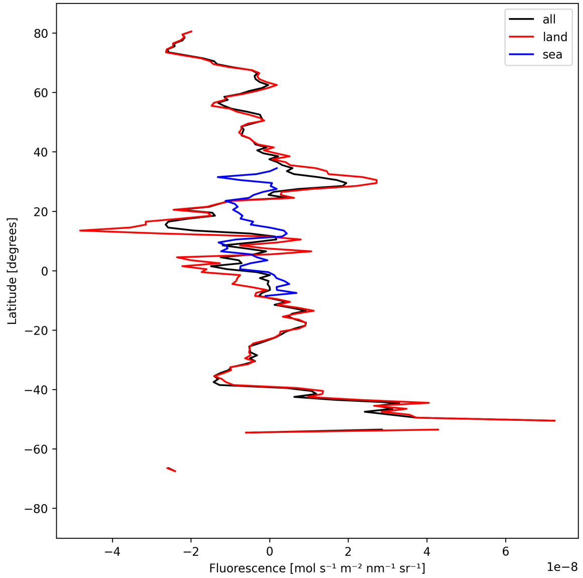
Figure 21: Zonal average of “Fluorescence” for 2025-09-06 to 2025-09-08.
