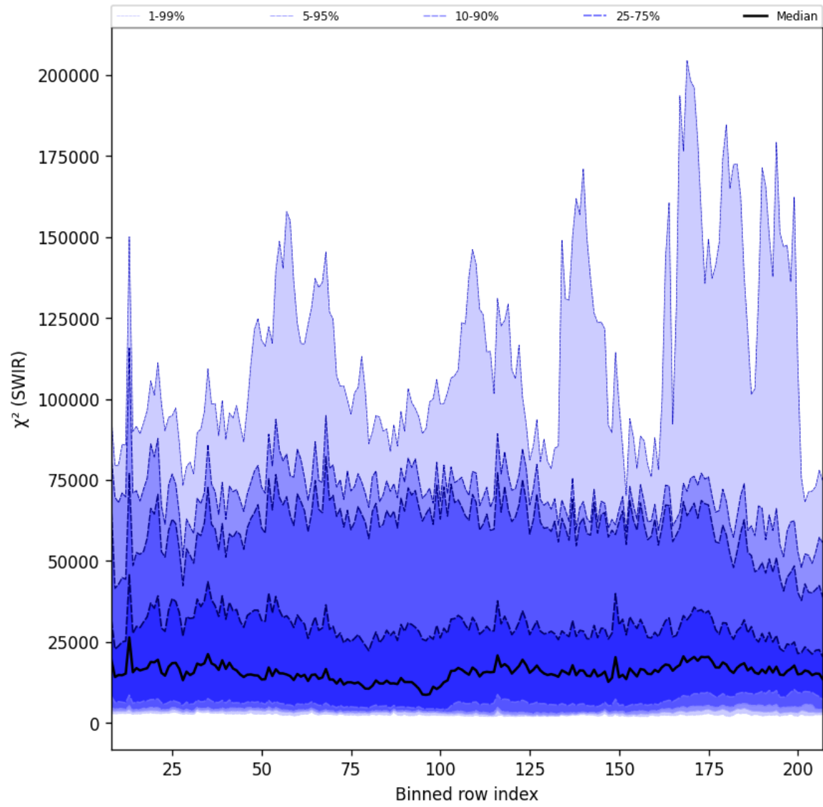
Figure 39: Along track statistics of “ \chi^2 (SWIR)” for 2025-09-06 to 2025-09-08
