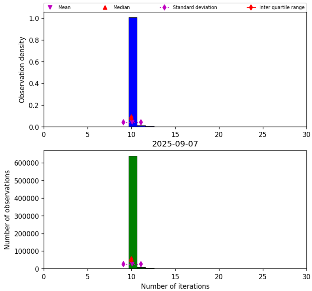
Figure 31: Histogram of “Number of iterations” for 2025-09-06 to 2025-09-08
