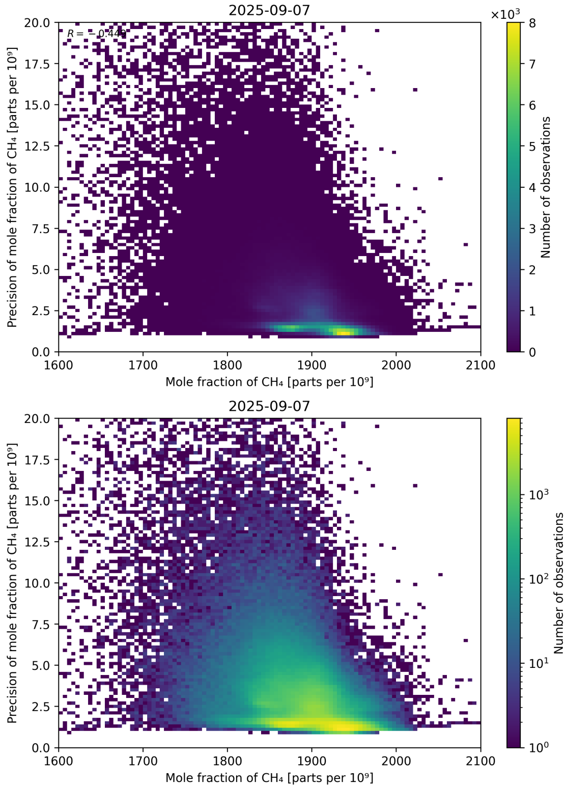
Figure 75: Scatter density plot of “Mole fraction of CH 4 ” against “Precision of mole fraction of CH 4 ” for 2025-09-06 to 2025-09-08.
