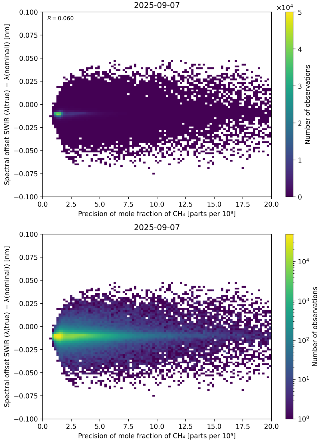
Figure 85: Scatter density plot of “Precision of mole fraction of CH 4 ” against “Spectral offset SWIR ( \lambda_{\text{true}} - \lambda_{\text{nominal}} )” for 2025-09-06 to 2025-09-08.
