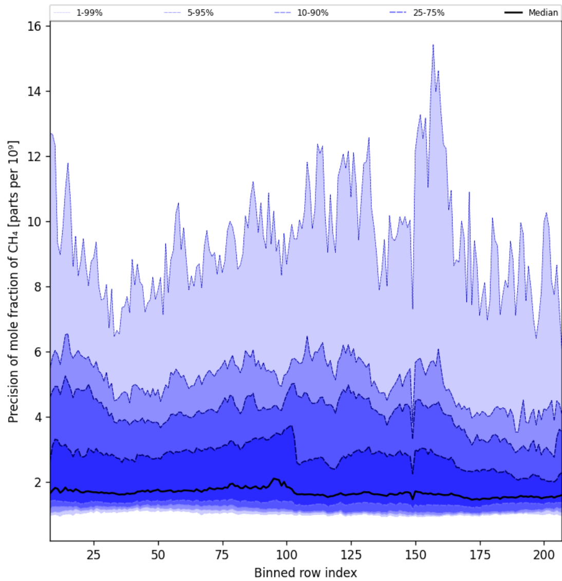
Figure 35: Along track statistics of “Precision of mole fraction of CH 4 ” for 2025-09-06 to 2025-09-08
