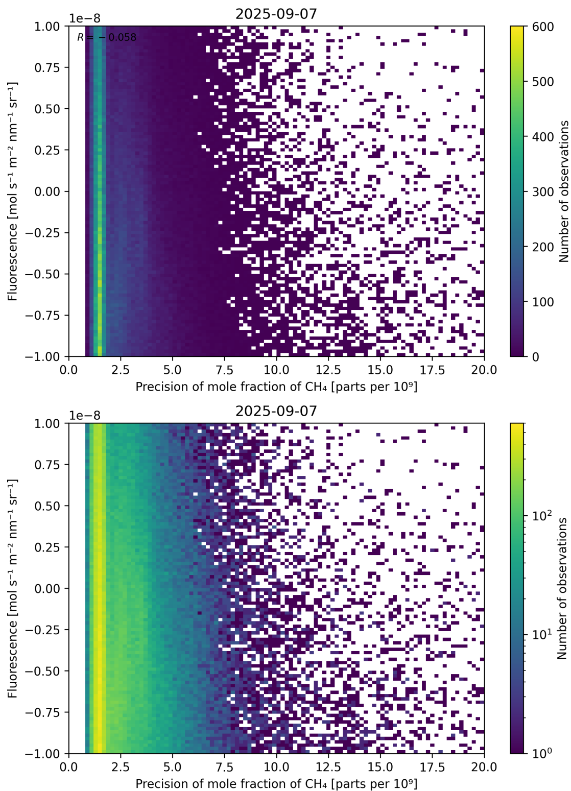
Figure 81: Scatter density plot of “Precision of mole fraction of CH 4 ” against “Fluorescence” for 2025-09-06 to 2025-09-08.
