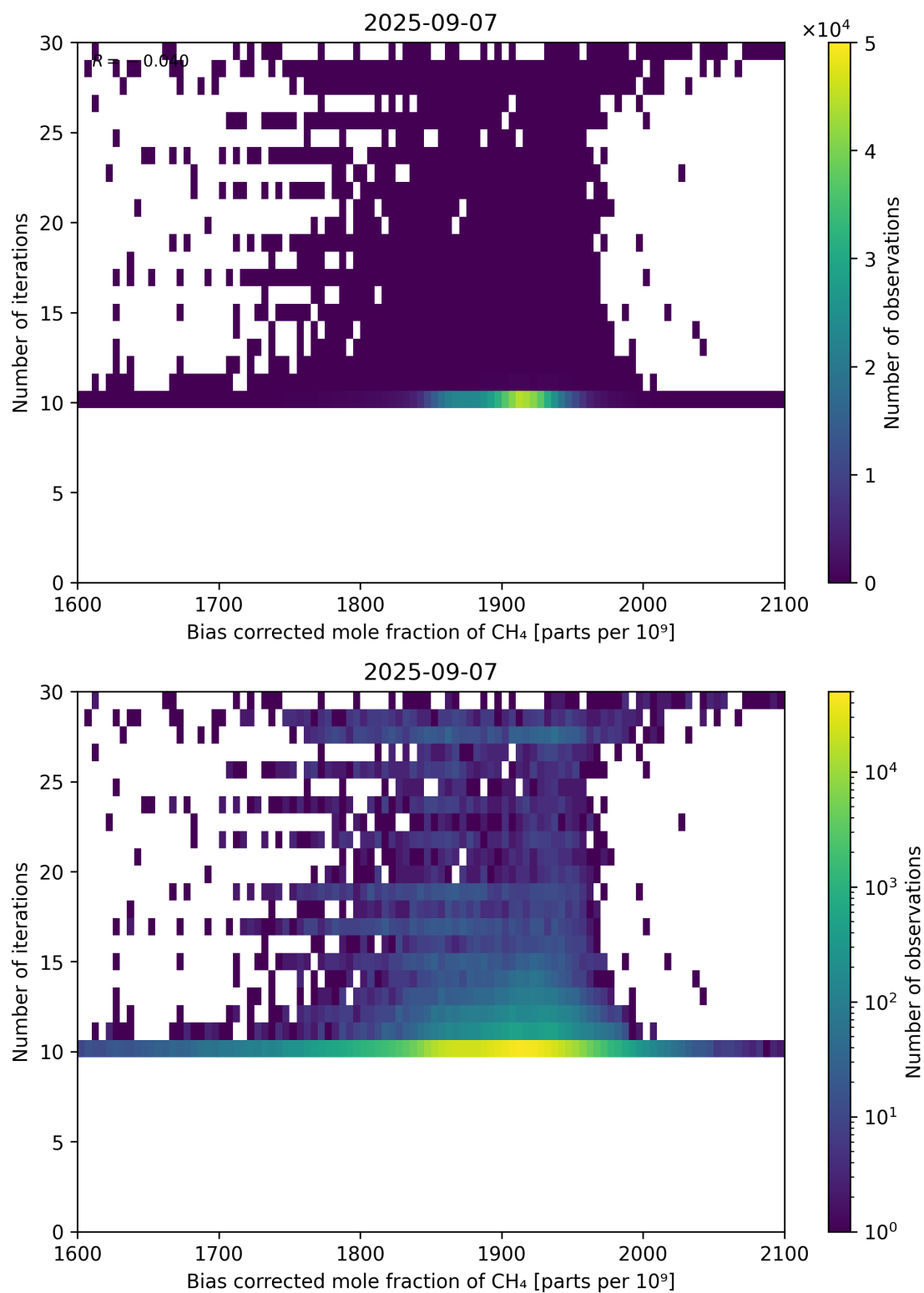
Figure 67: Scatter density plot of “Bias corrected mole fraction of CH 4 ” against “Number of iterations” for 2025-09-06 to 2025-09-08.
