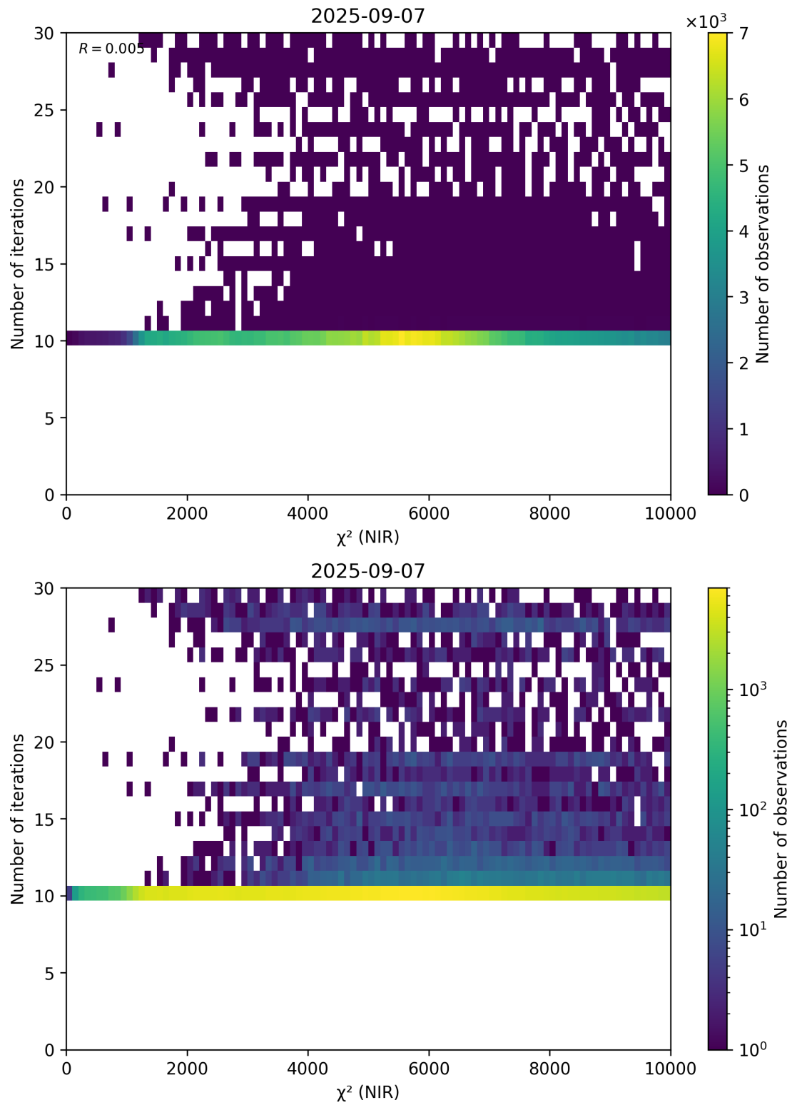
Figure 46: Scatter density plot of “ \chi^2 (NIR)” against “Number of iterations” for 2025-09-06 to 2025-09-08.
