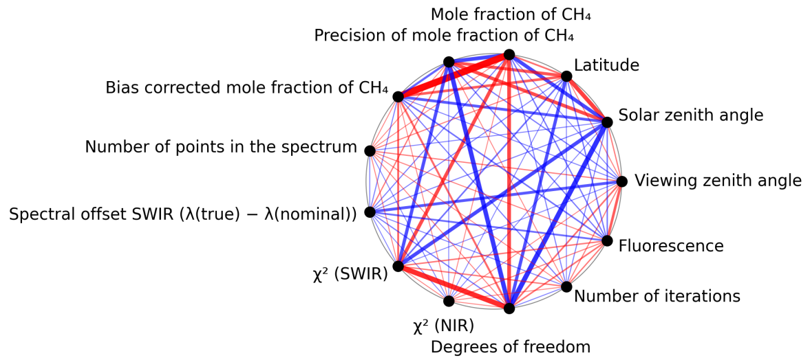
Figure 1: Map of correlation graph for 2025-09-06 to 2025-09-08.
