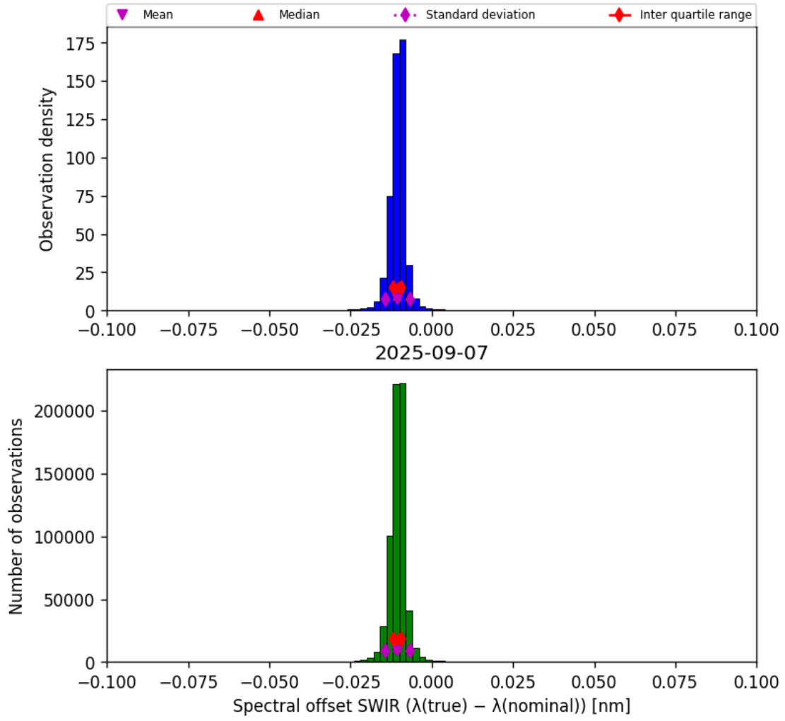
Figure 27: Histogram of “Spectral offset SWIR ( \lambda_{\text{true}} - \lambda_{\text{nominal}} )” for 2025-09-06 to 2025-09-08
