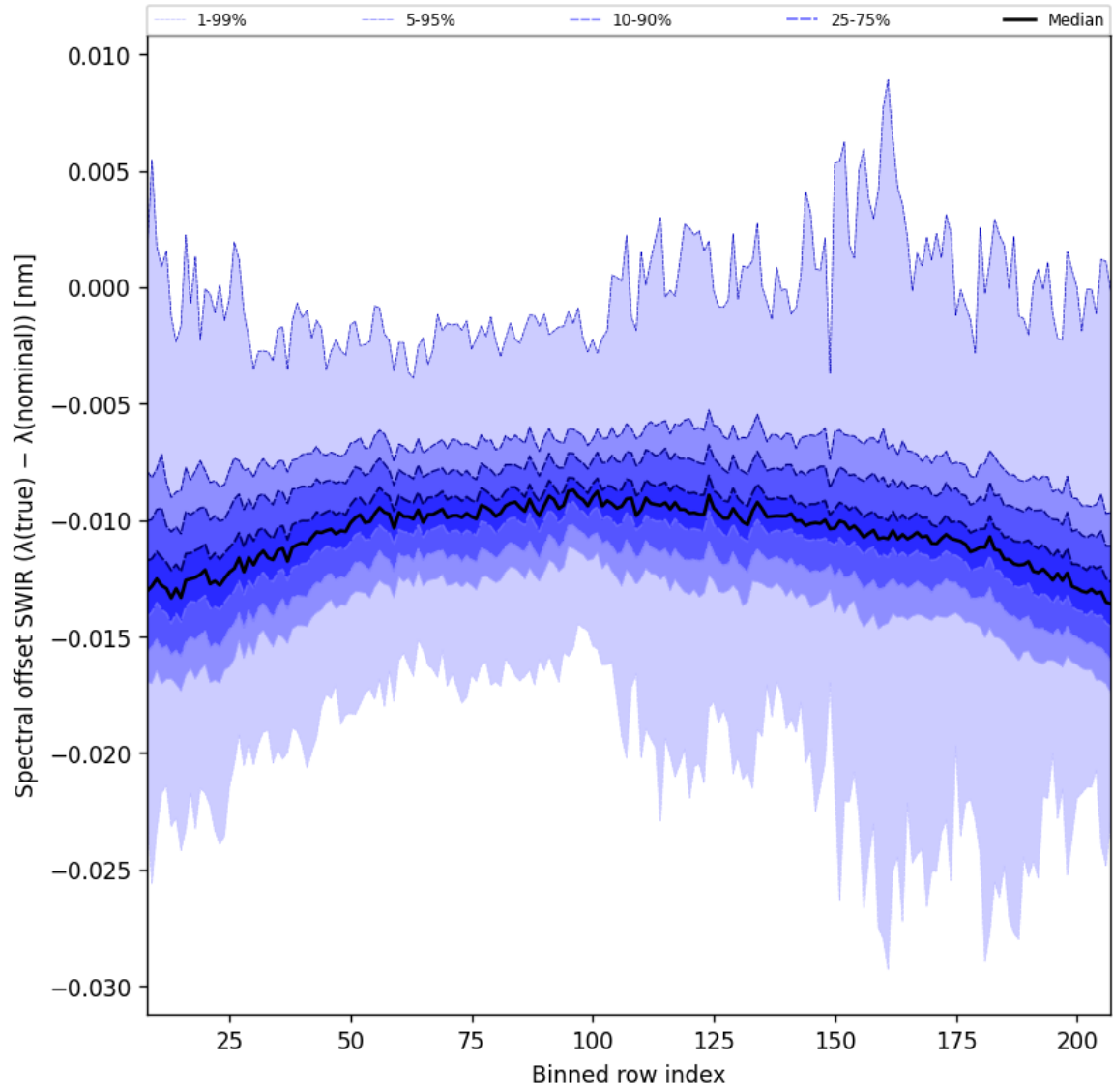
Figure 38: Along track statistics of “Spectral offset SWIR ( \lambda_{\text{true}} - \lambda_{\text{nominal}} )” for 2025-09-06 to 2025-09-08
