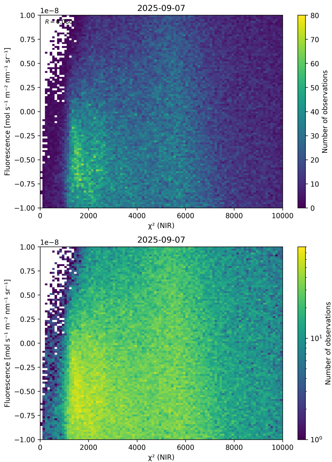
Figure 45: Scatter density plot of “ \chi^2 (NIR)” against “Fluorescence” for 2025-09-06 to 2025-09-08.
