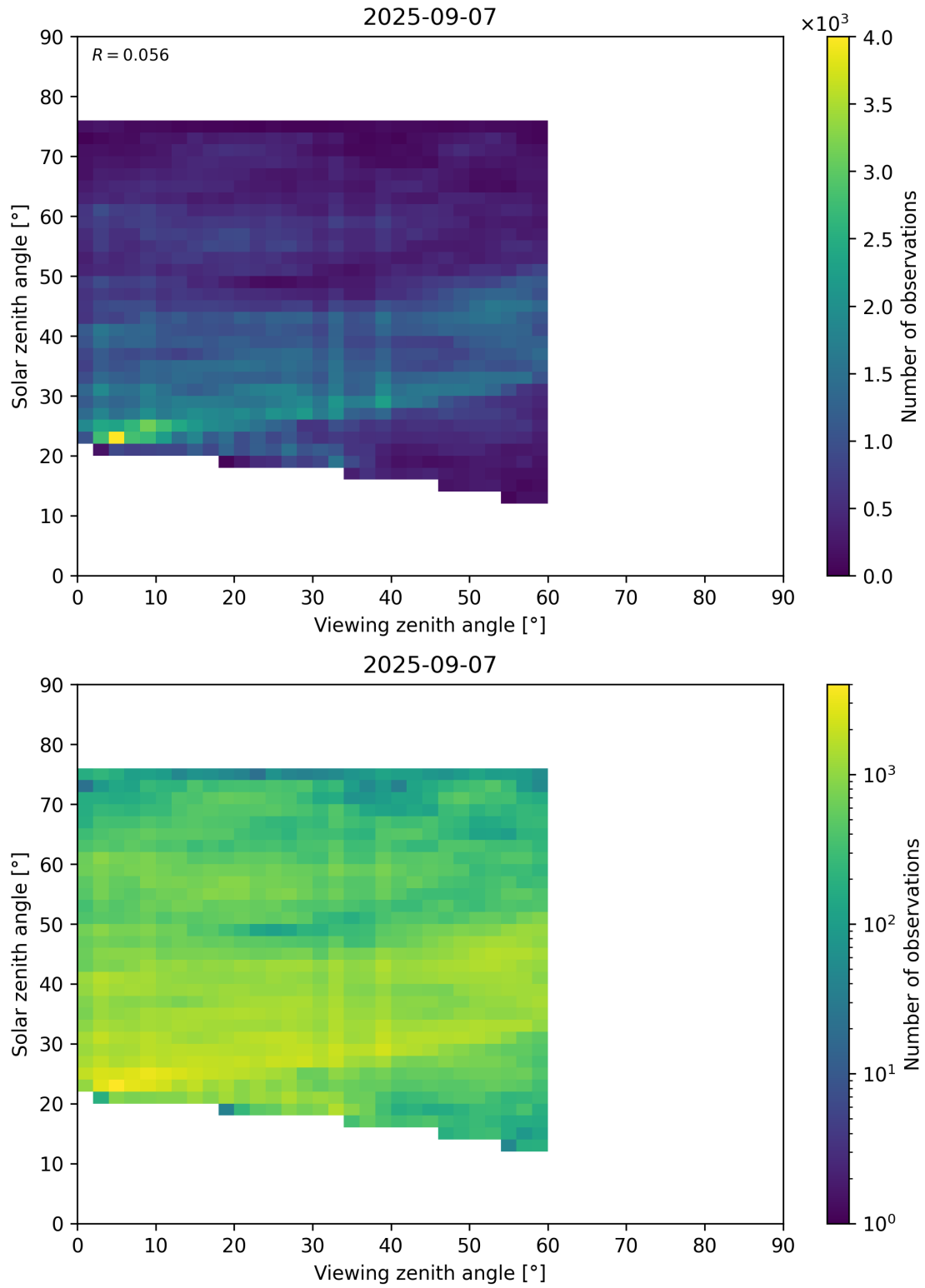
Figure 115: Scatter density plot of “Viewing zenith angle” against “Solar zenith angle” for 2025-09-06 to 2025-09-08.
