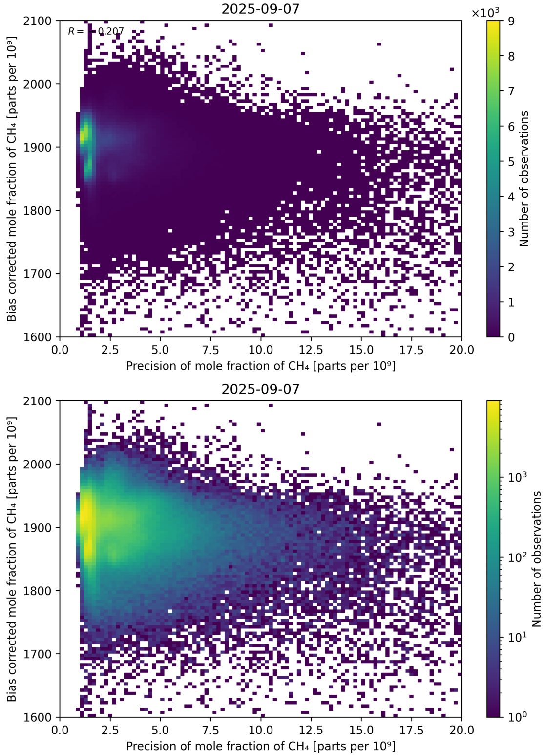
Figure 82: Scatter density plot of “Precision of mole fraction of CH 4 ” against “Bias corrected mole fraction of CH 4 ” for 2025-09-06 to 2025-09-08.
