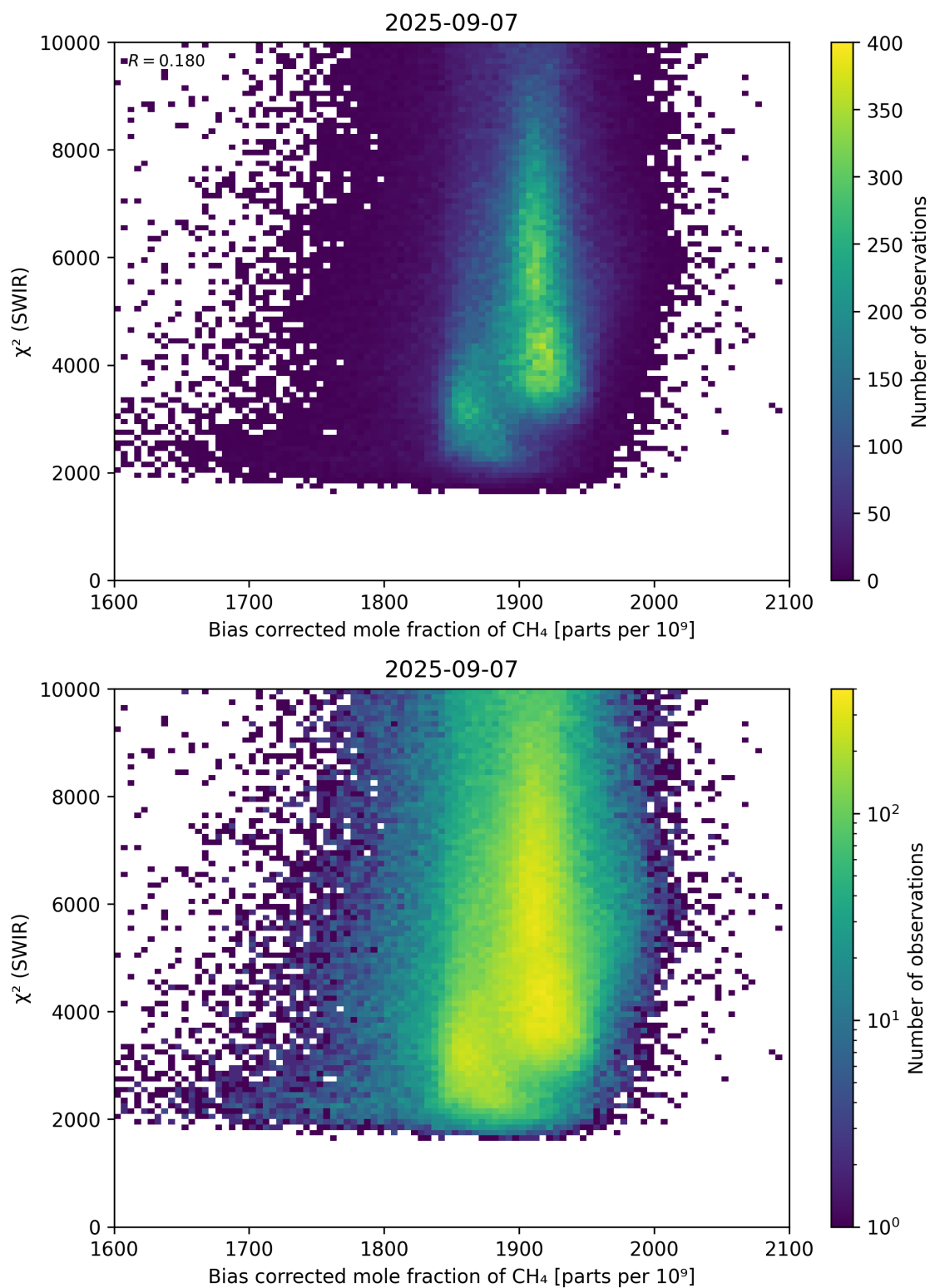
Figure 64: Scatter density plot of “Bias corrected mole fraction of CH 4 ” against “ \chi^2 (SWIR)” for 2025-09-06 to 2025-09-08.
