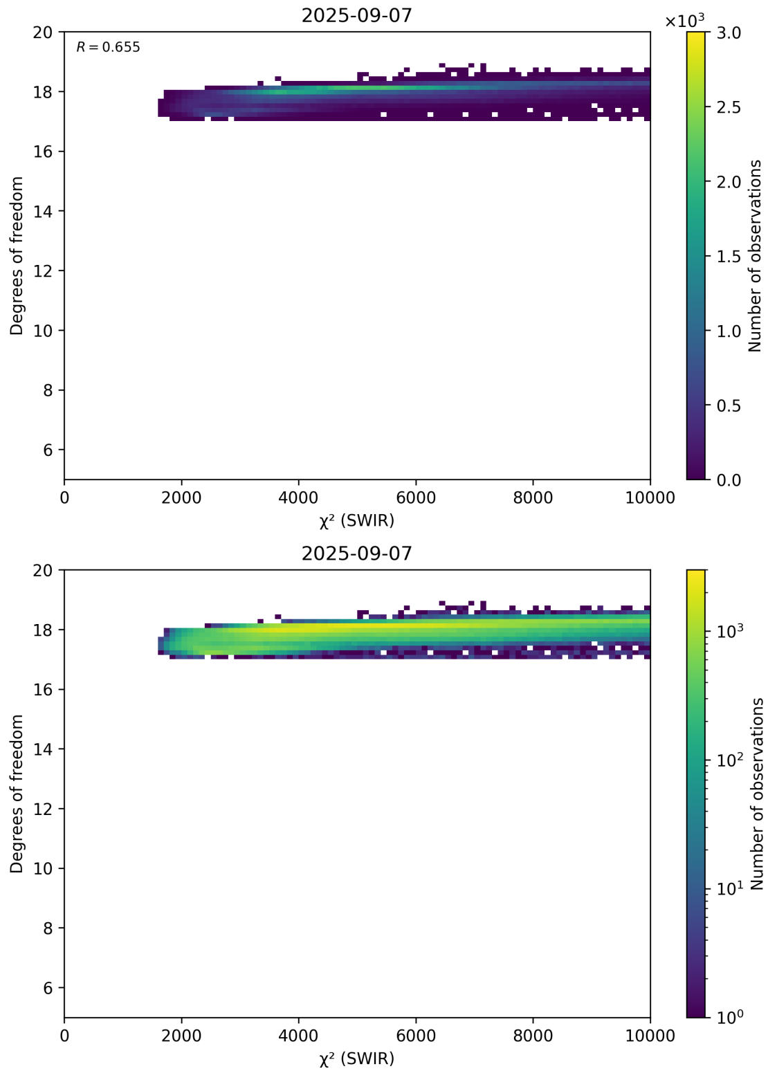
Figure 48: Scatter density plot of “ \chi^2 (SWIR)” against “Degrees of freedom” for 2025-09-06 to 2025-09-08.
