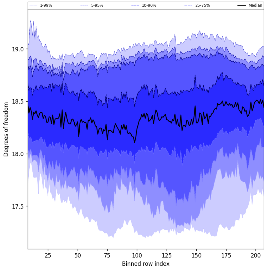
Figure 41: Along track statistics of “Degrees of freedom” for 2025-09-06 to 2025-09-08
