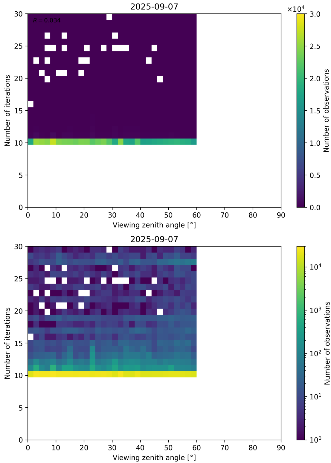
Figure 113: Scatter density plot of “Viewing zenith angle” against “Number of iterations” for 2025-09-06 to 2025-09-08.
