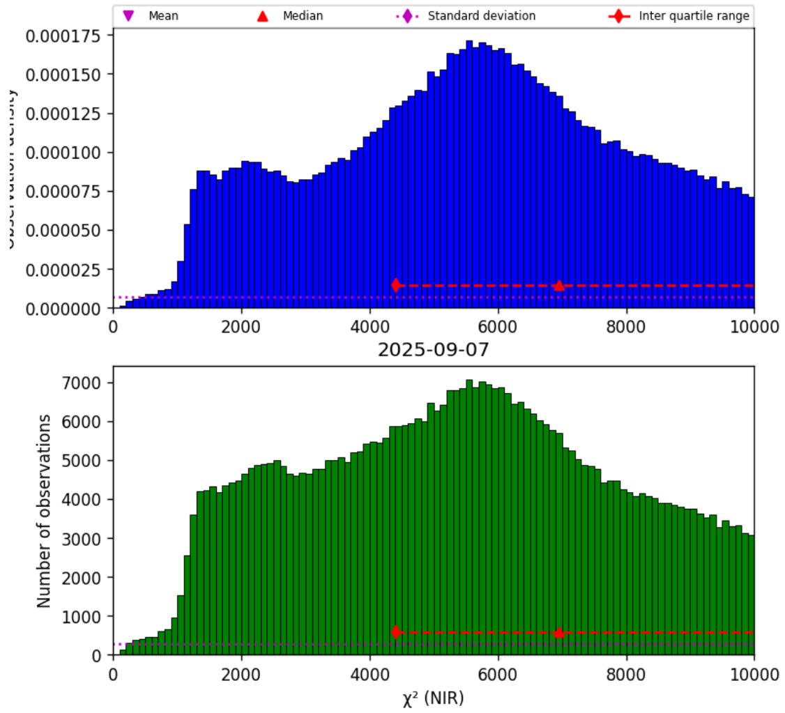
Figure 29: Histogram of “ \chi^2 (NIR)” for 2025-09-06 to 2025-09-08
