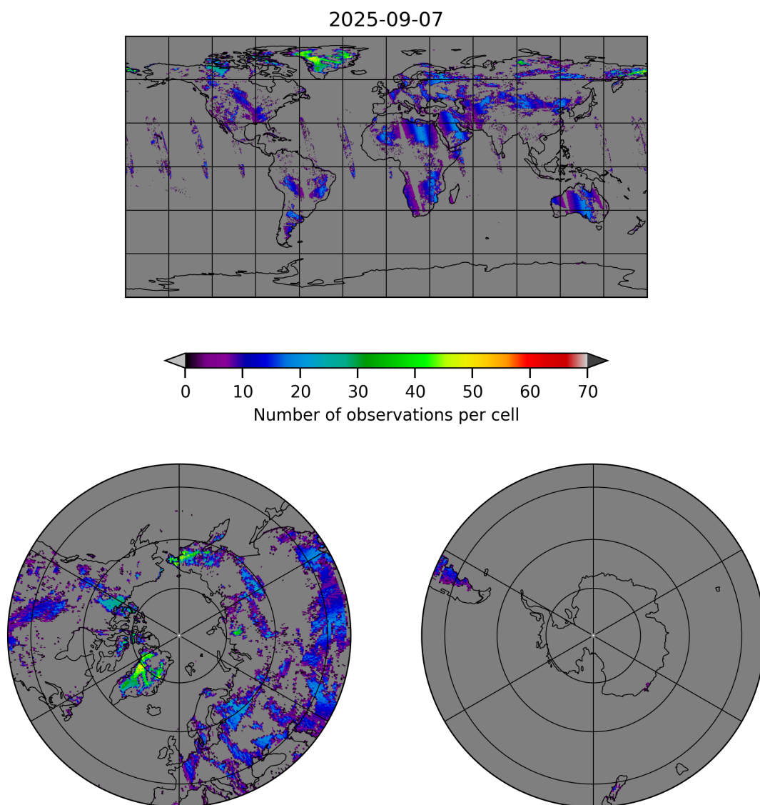
Figure 10: Map of the number of observations for 2025-09-06 to 2025-09-08
