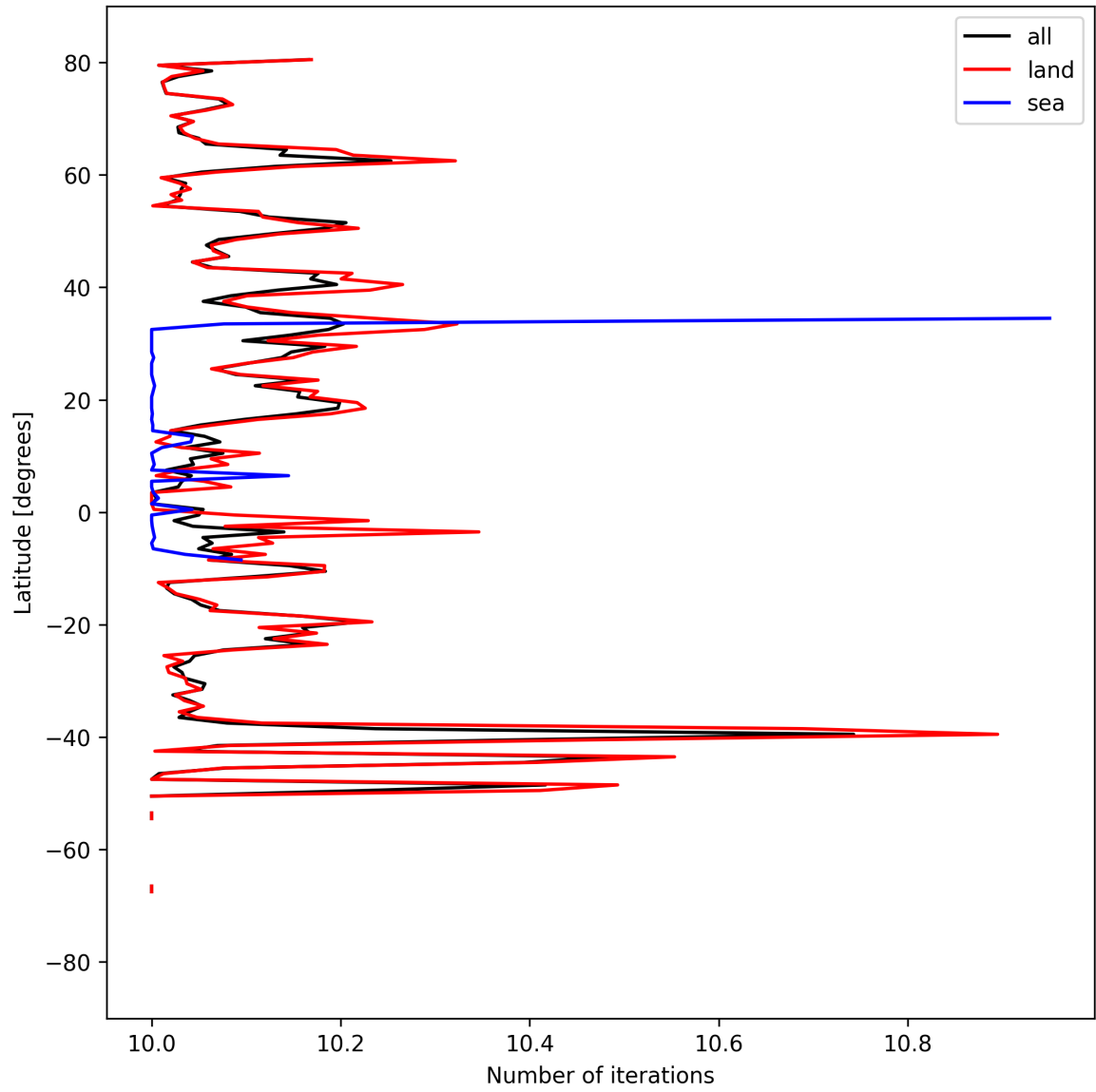
Figure 20: Zonal average of “Number of iterations” for 2025-09-06 to 2025-09-08.
