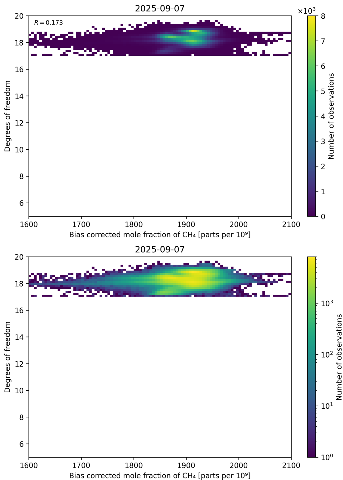
Figure 65: Scatter density plot of “Bias corrected mole fraction of CH 4 ” against “Degrees of freedom” for 2025-09-06 to 2025-09-08.
