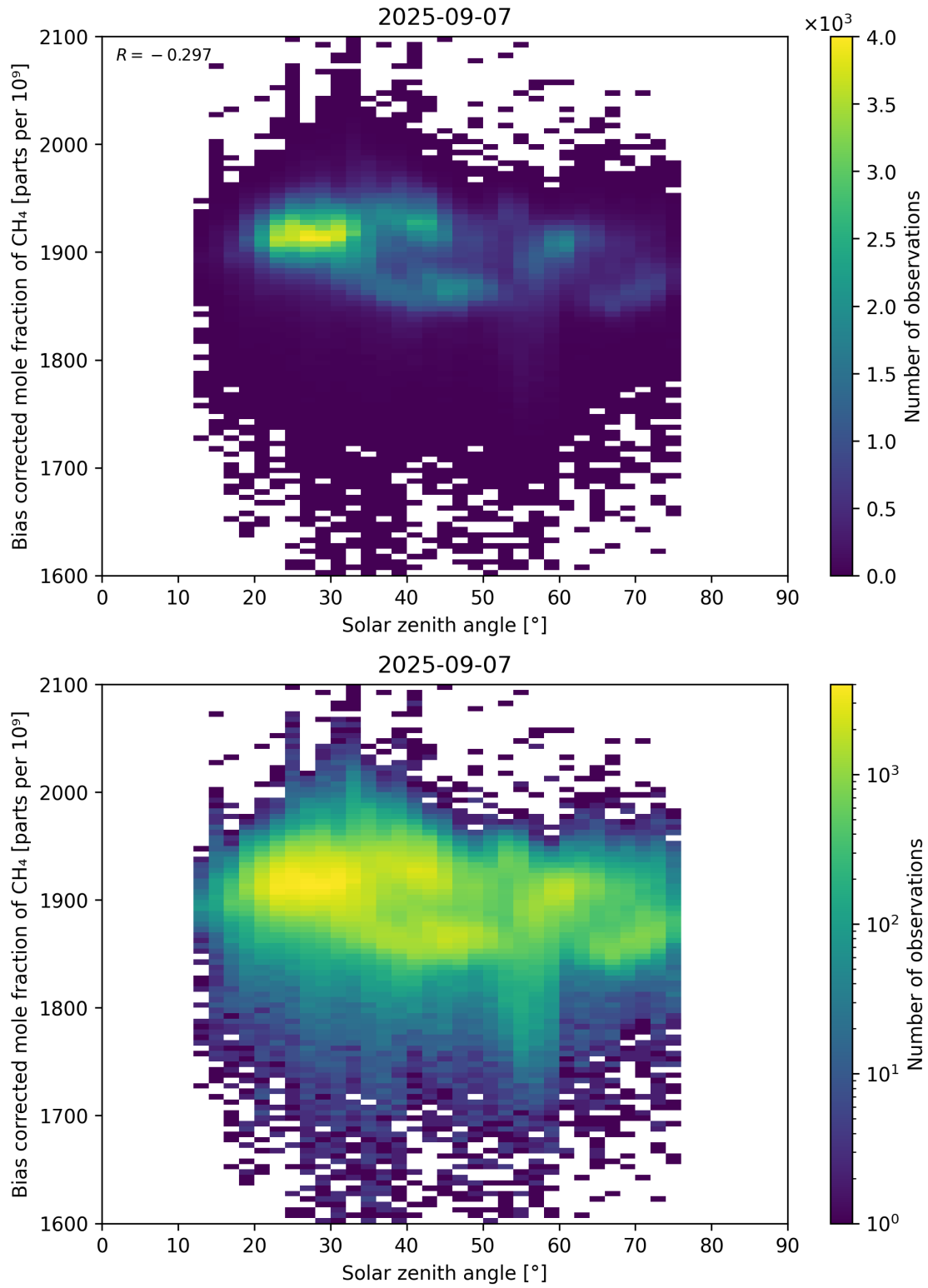
Figure 100: Scatter density plot of “Solar zenith angle” against “Bias corrected mole fraction of CH 4 ” for 2025-09-06 to 2025-09-08.
