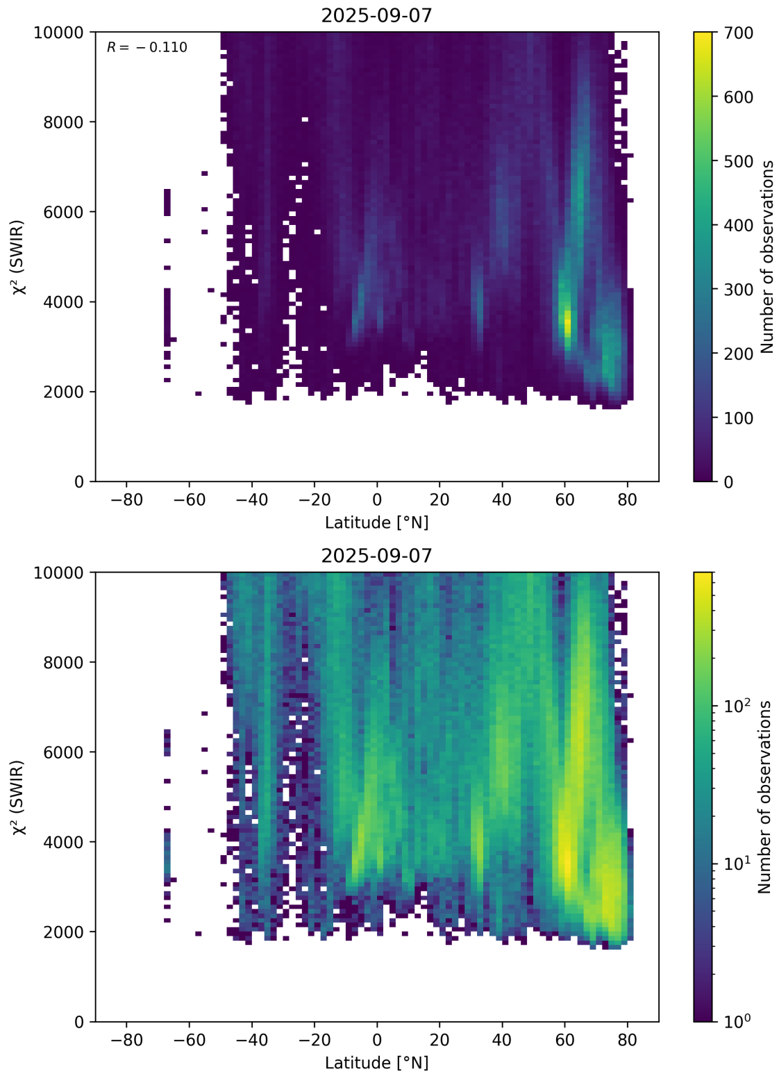
Figure 54: Scatter density plot of “Latitude” against “ \chi^2 (SWIR)” for 2025-09-06 to 2025-09-08.
