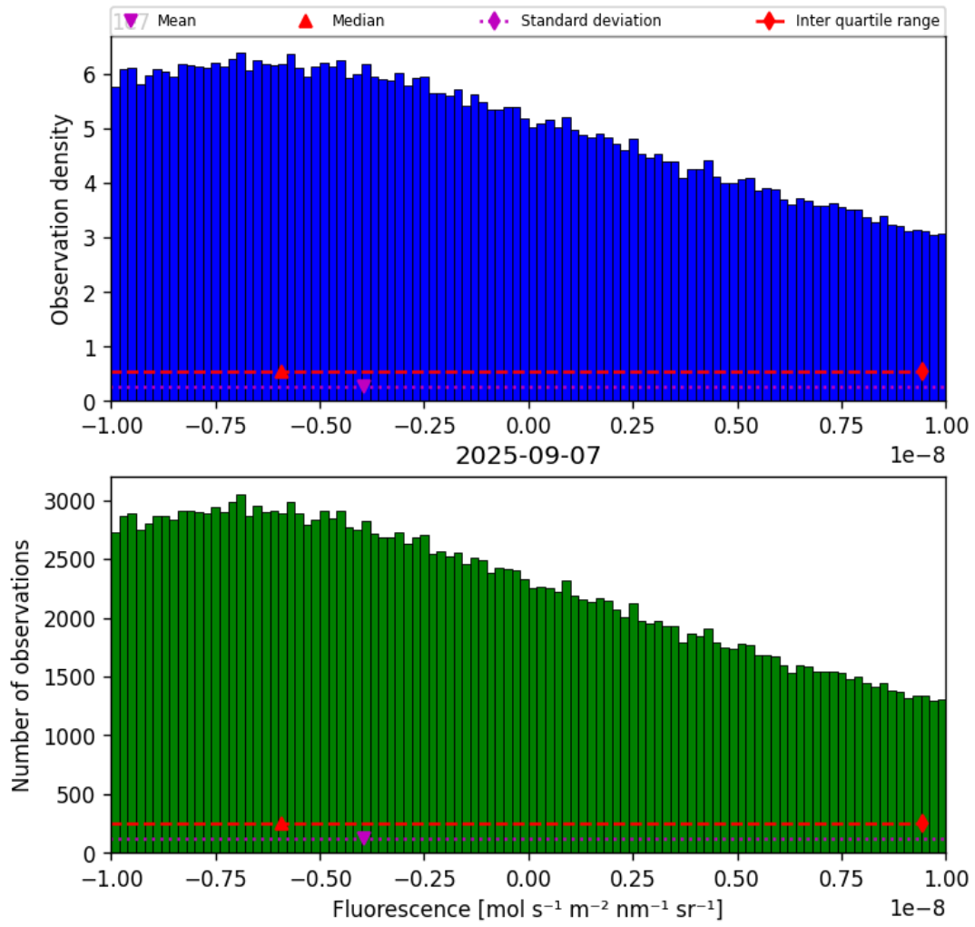
Figure 32: Histogram of “Fluorescence” for 2025-09-06 to 2025-09-08
