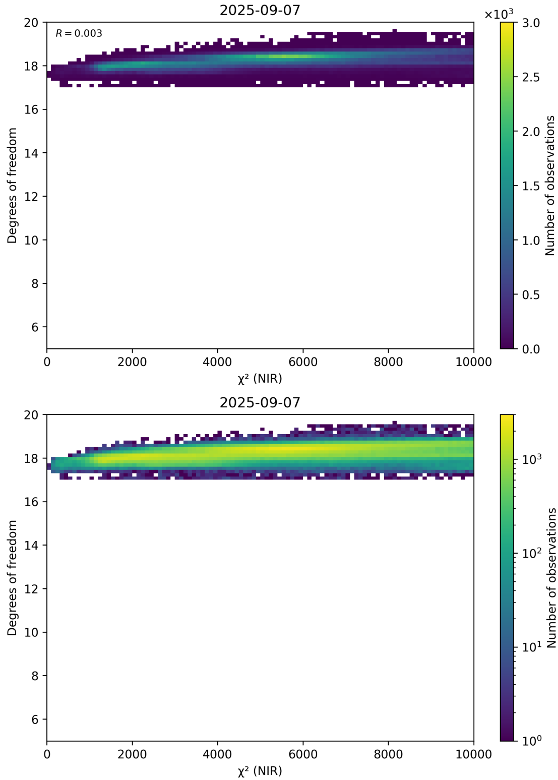
Figure 44: Scatter density plot of “ \chi^2 (NIR)” against “Degrees of freedom” for 2025-09-06 to 2025-09-08.
