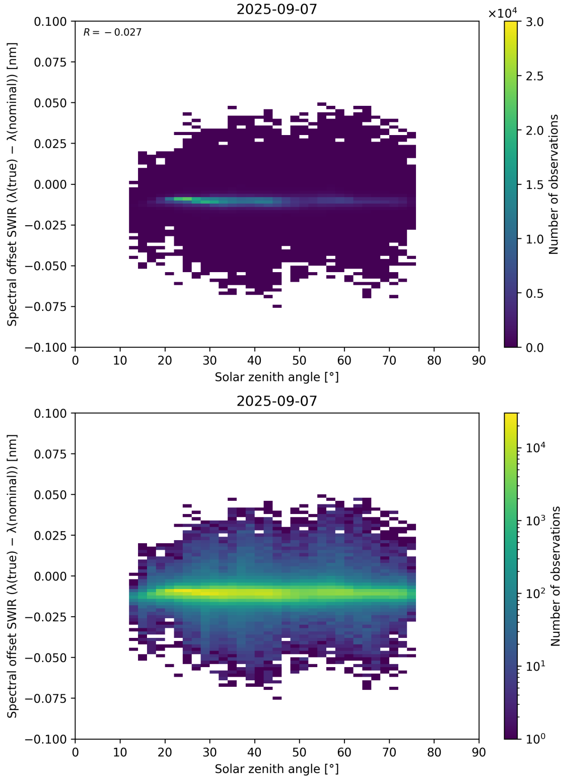
Figure 104: Scatter density plot of “Solar zenith angle” against “Spectral offset SWIR ( \lambda_{\text{true}} - \lambda_{\text{nominal}} )” for 2025-09-06 to 2025-09-08.
