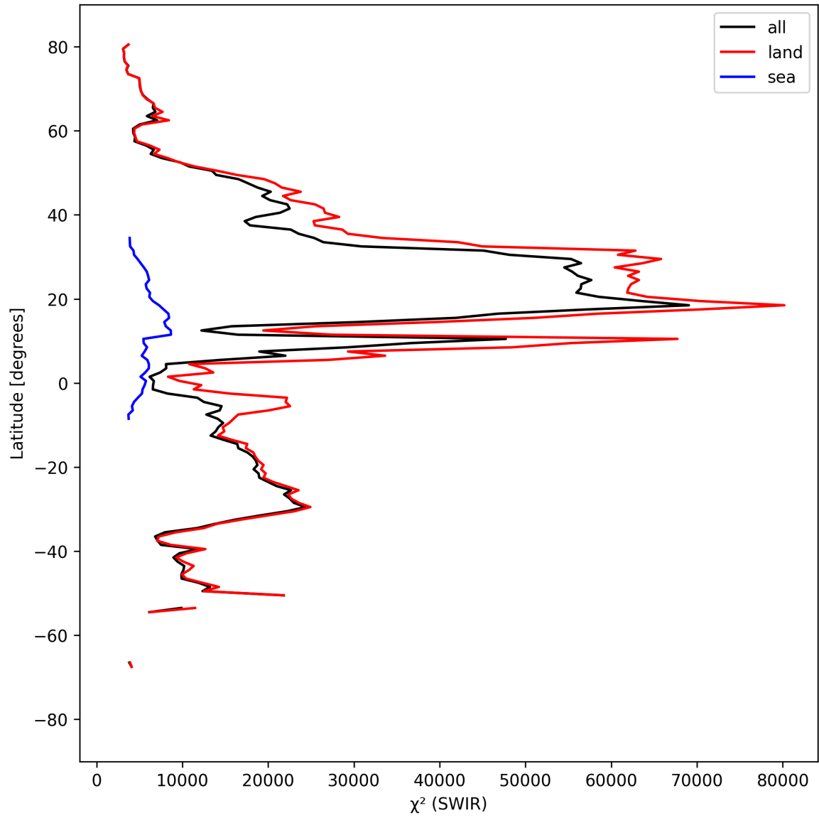
Figure 17: Zonal average of “ \chi^2 (SWIR)” for 2025-09-06 to 2025-09-08.
