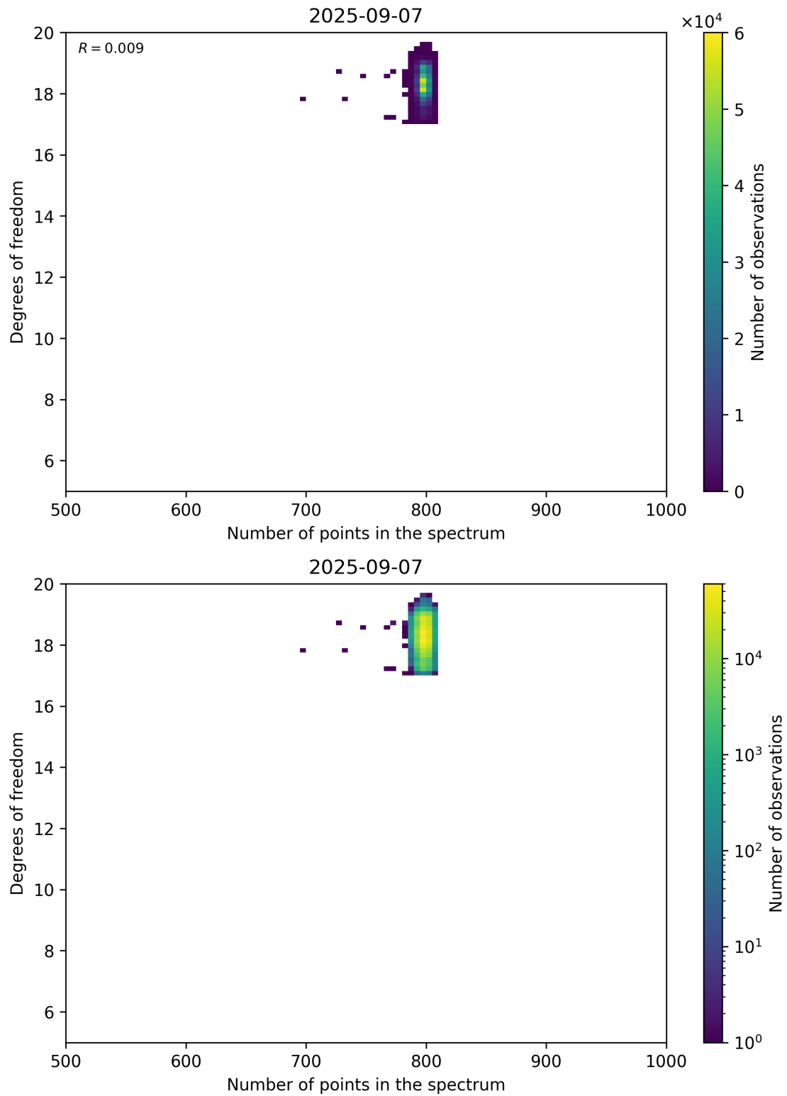
Figure 90: Scatter density plot of “Number of points in the spectrum” against “Degrees of freedom” for 2025-09-06 to 2025-09-08.
