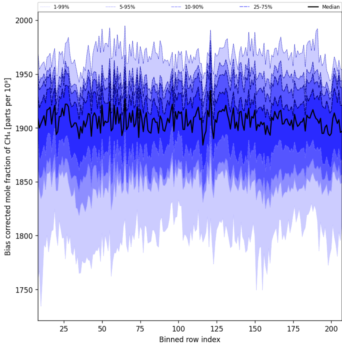
Figure 36: Along track statistics of “Bias corrected mole fraction of CH 4 ” for 2025-09-06 to 2025-09-08
