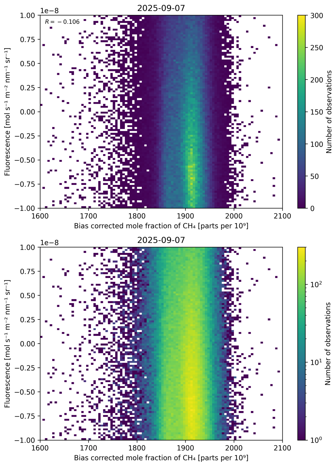
Figure 66: Scatter density plot of “Bias corrected mole fraction of \text{CH}_4 ” against “Fluorescence” for 2025-09-06 to 2025-09-08.
