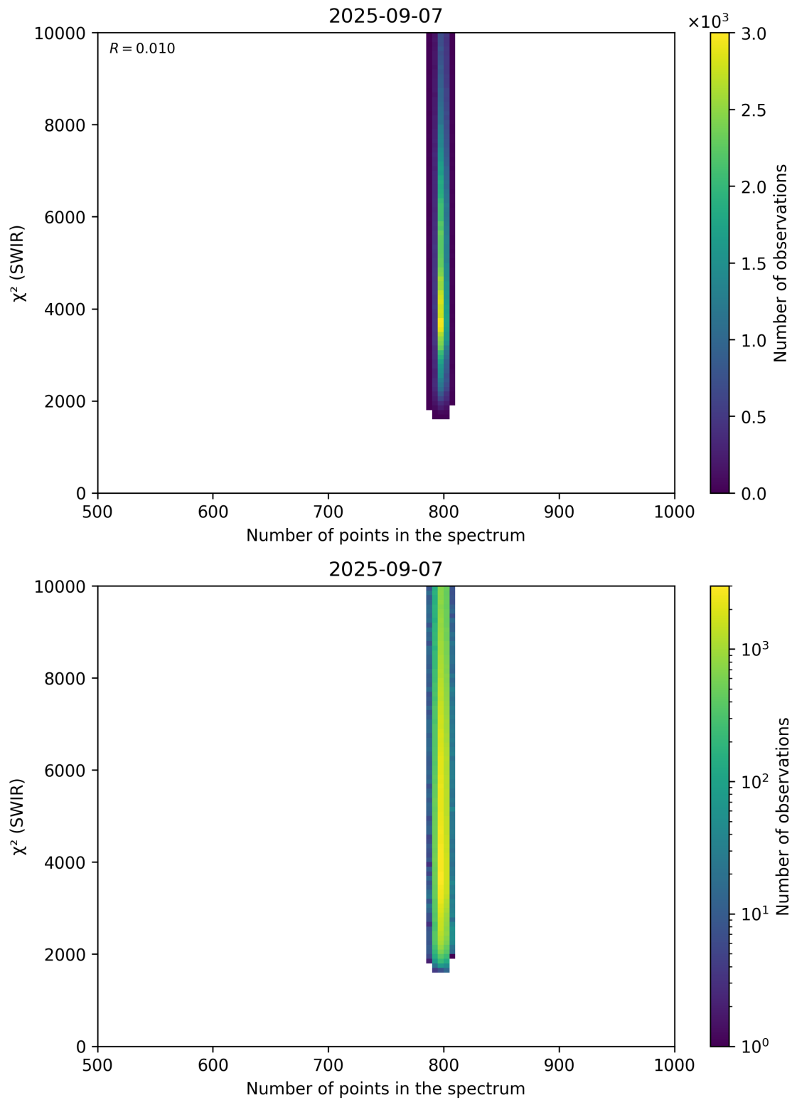
Figure 89: Scatter density plot of “Number of points in the spectrum” against “ \chi^2 (SWIR)” for 2025-09-06 to 2025-09-08.
