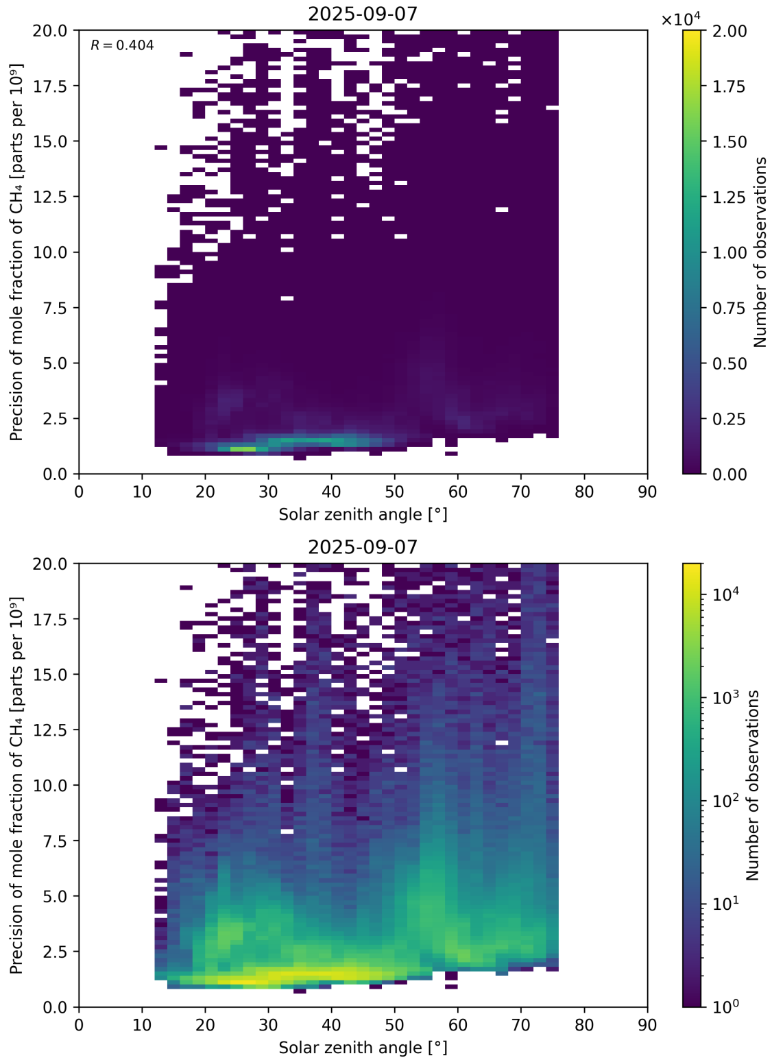
Figure 101: Scatter density plot of “Solar zenith angle” against “Precision of mole fraction of \text{CH}_4 ” for 2025-09-06 to 2025-09-08.
