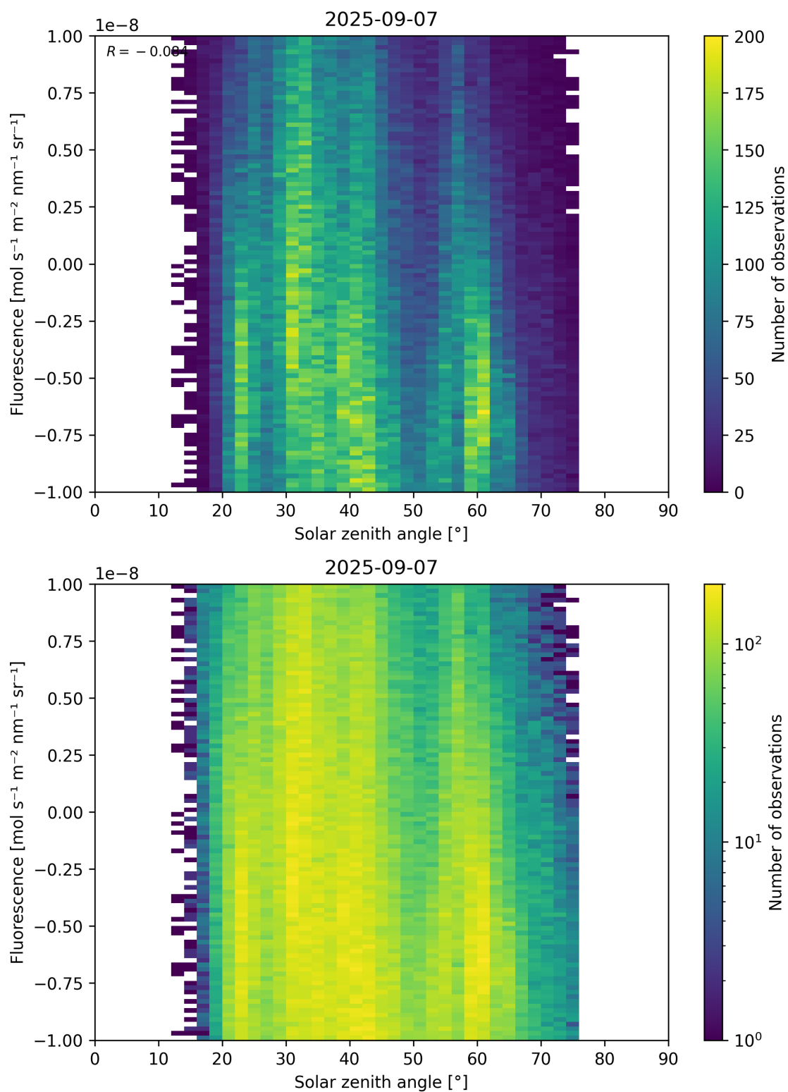
Figure 97: Scatter density plot of “Solar zenith angle” against “Fluorescence” for 2025-09-06 to 2025-09-08.
