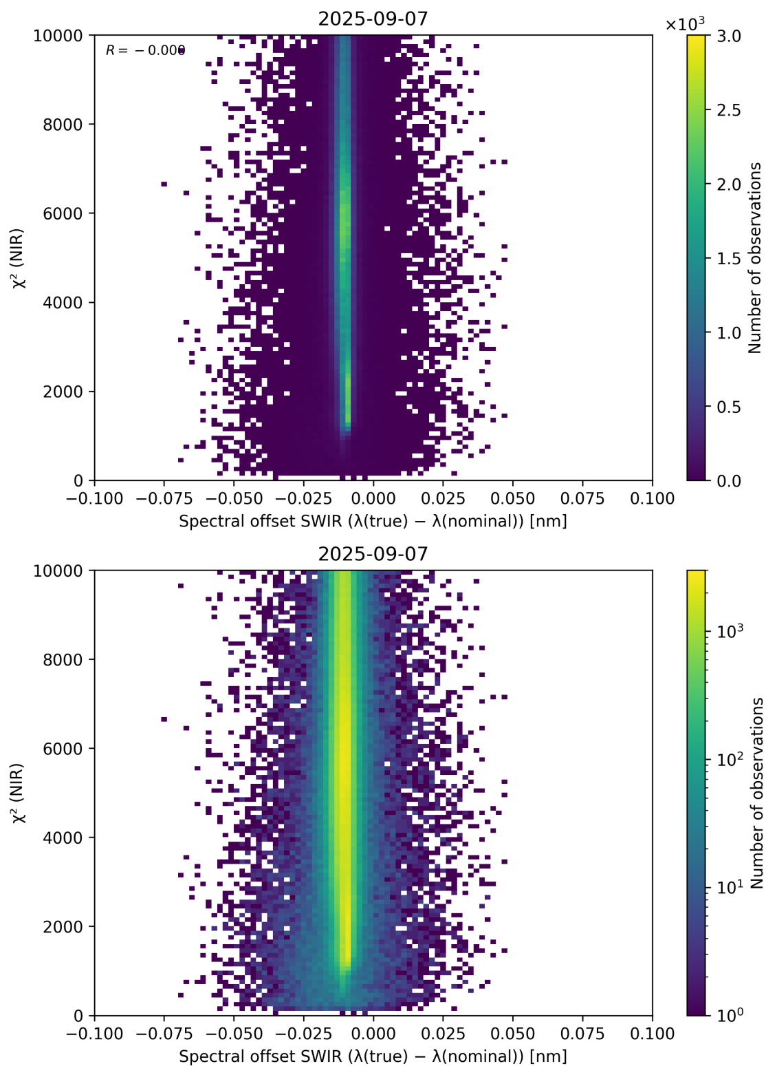
Figure 117: Scatter density plot of “Spectral offset SWIR ( \lambda_{\text{true}} - \lambda_{\text{nominal}} )” against “ \chi^2 (NIR)” for 2025-09-06 to 2025-09-08.
