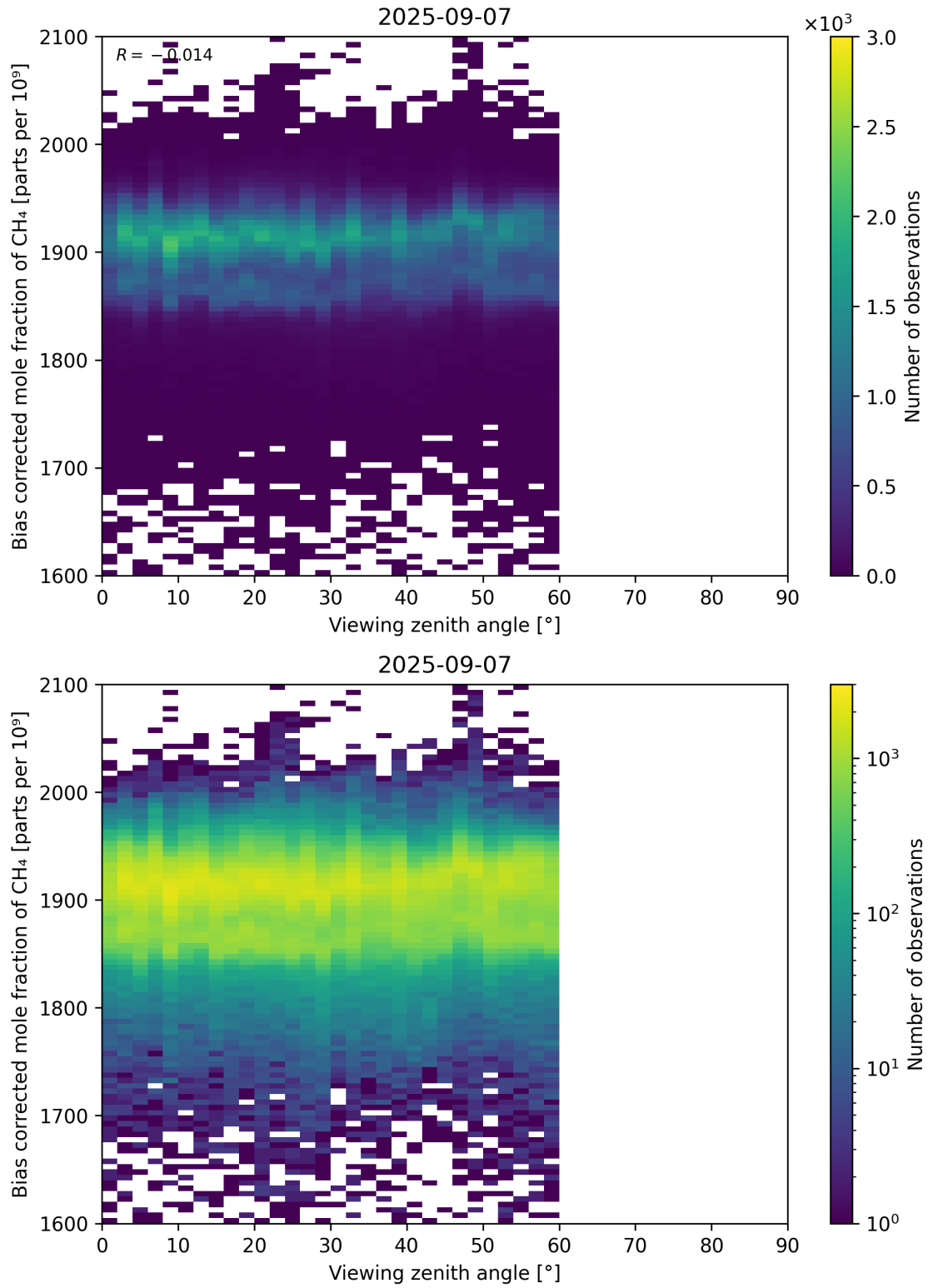
Figure 111: Scatter density plot of “Viewing zenith angle” against “Bias corrected mole fraction of CH 4 ” for 2025-09-06 to 2025-09-08.
