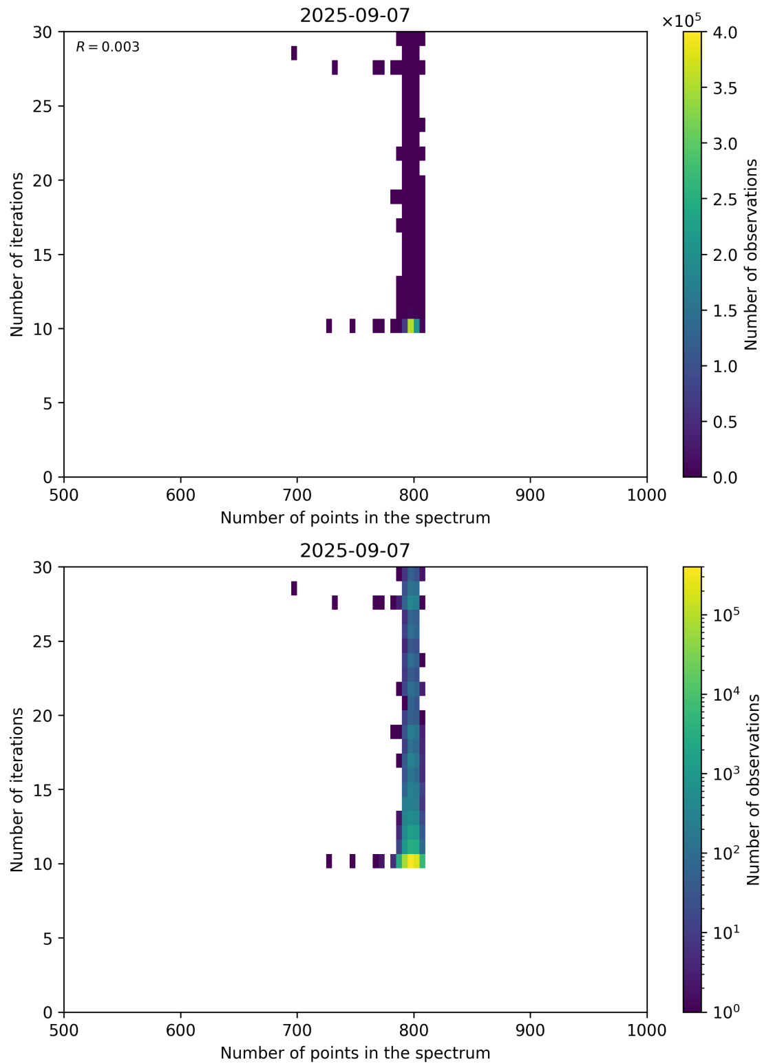
Figure 92: Scatter density plot of “Number of points in the spectrum” against “Number of iterations” for 2025-09-06 to 2025-09-08.
