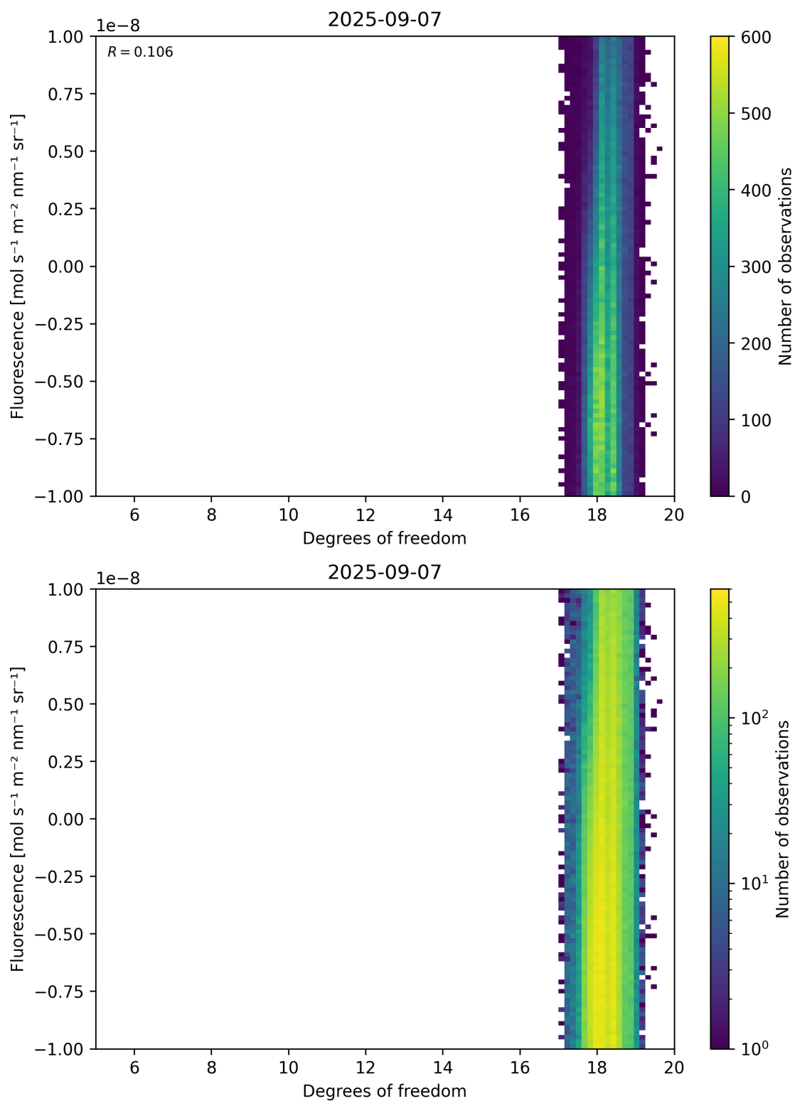
Figure 51: Scatter density plot of “Degrees of freedom” against “Fluorescence” for 2025-09-06 to 2025-09-08.
