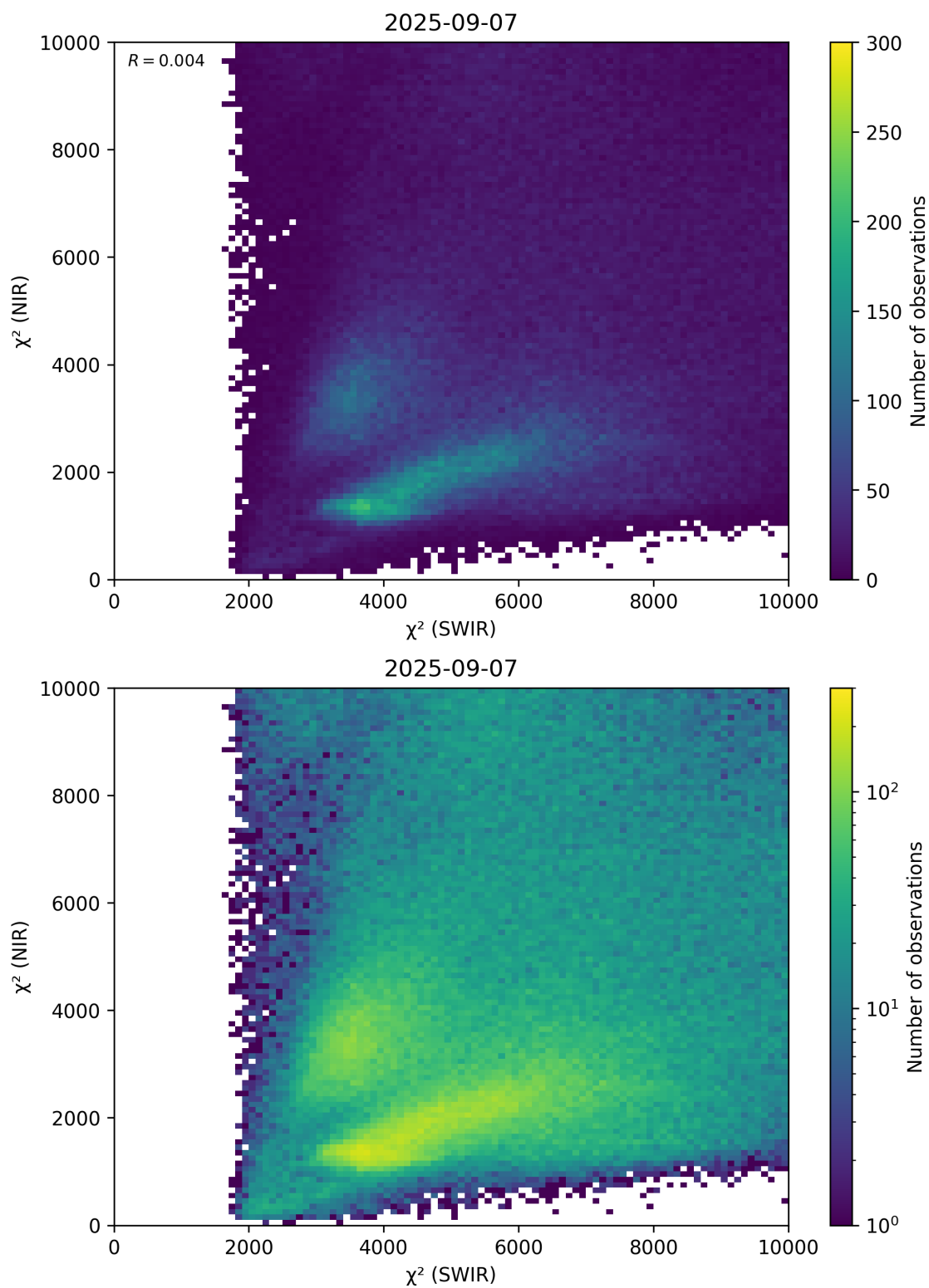
Figure 47: Scatter density plot of “ \chi^2 (SWIR)” against “ \chi^2 (NIR)” for 2025-09-06 to 2025-09-08.
