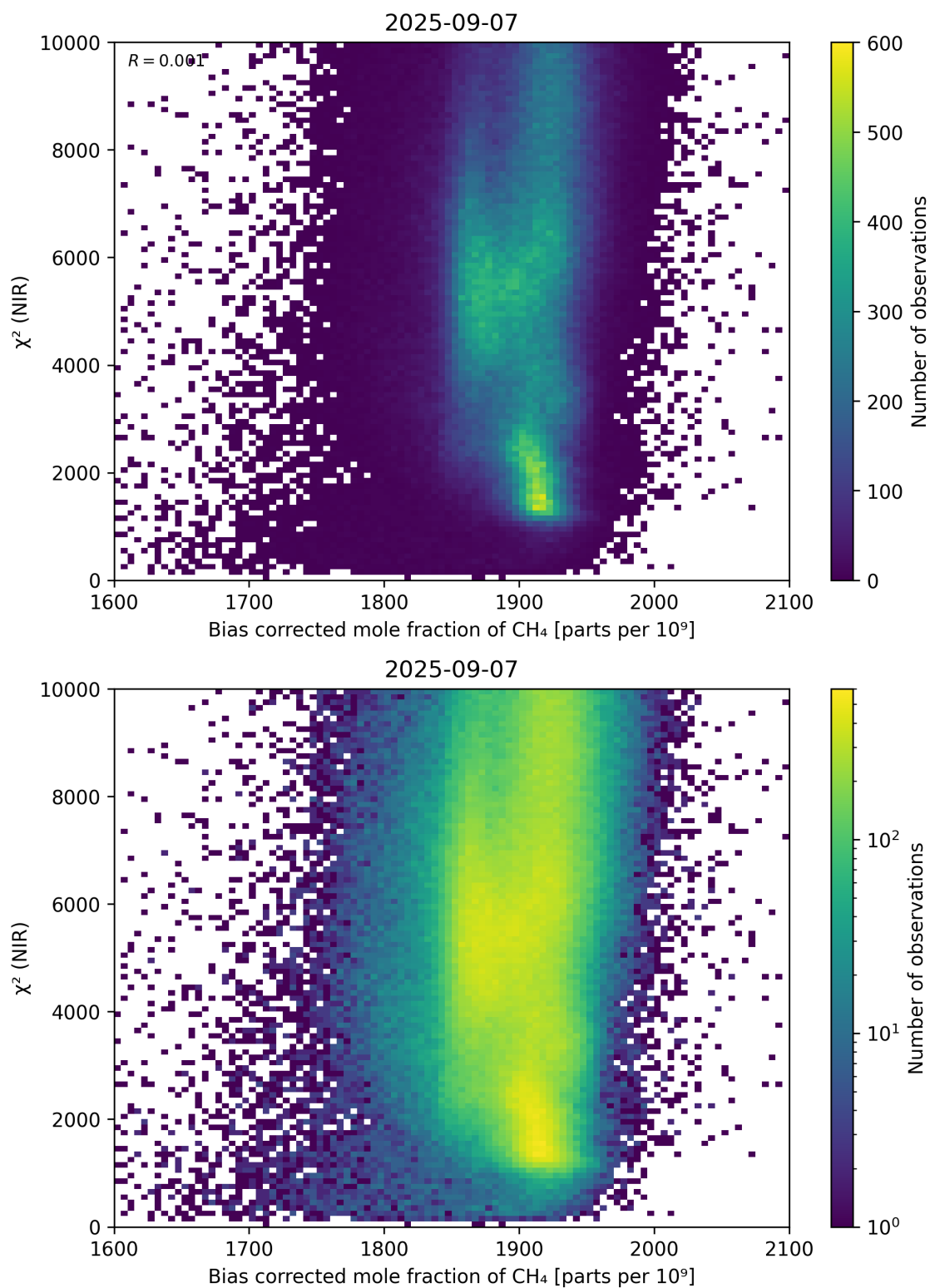
Figure 63: Scatter density plot of “Bias corrected mole fraction of \text{CH}_4 ” against “ \chi^2 (NIR)” for 2025-09-06 to 2025-09-08.
