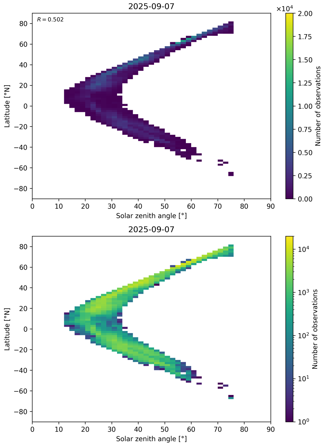
Figure 98: Scatter density plot of “Solar zenith angle” against “Latitude” for 2025-09-06 to 2025-09-08.
