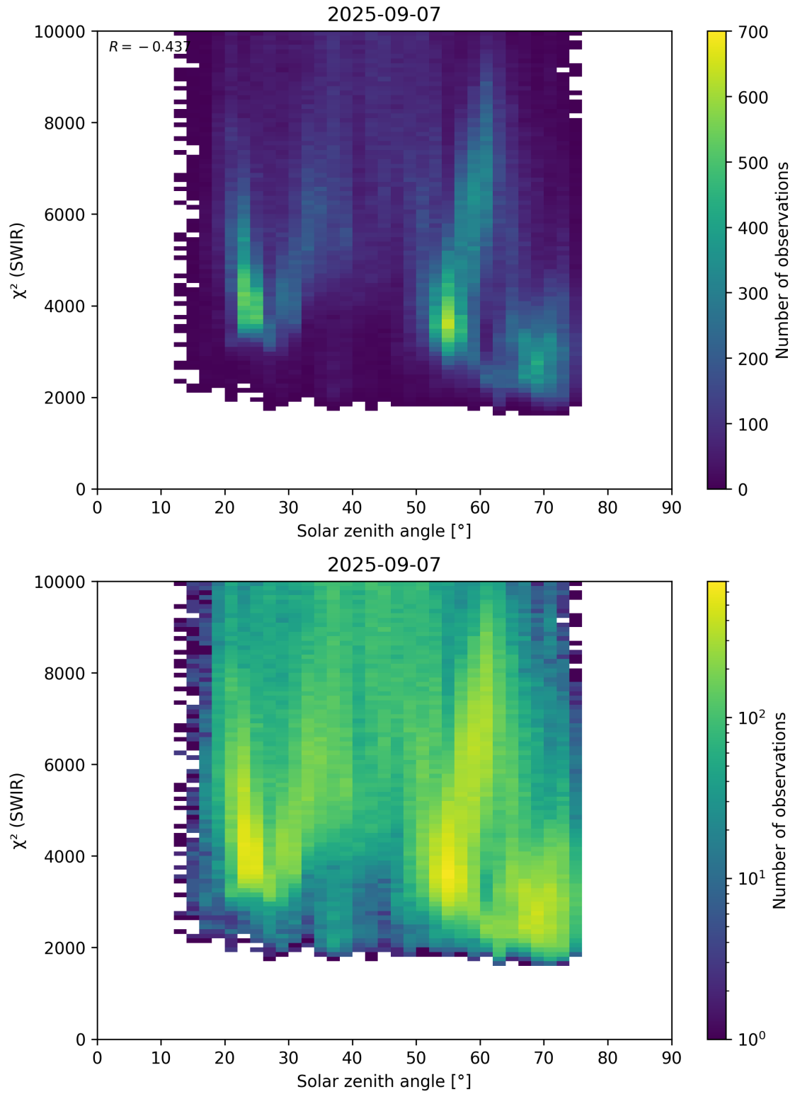
Figure 95: Scatter density plot of “Solar zenith angle” against “ \chi^2 (SWIR)” for 2025-09-06 to 2025-09-08.
