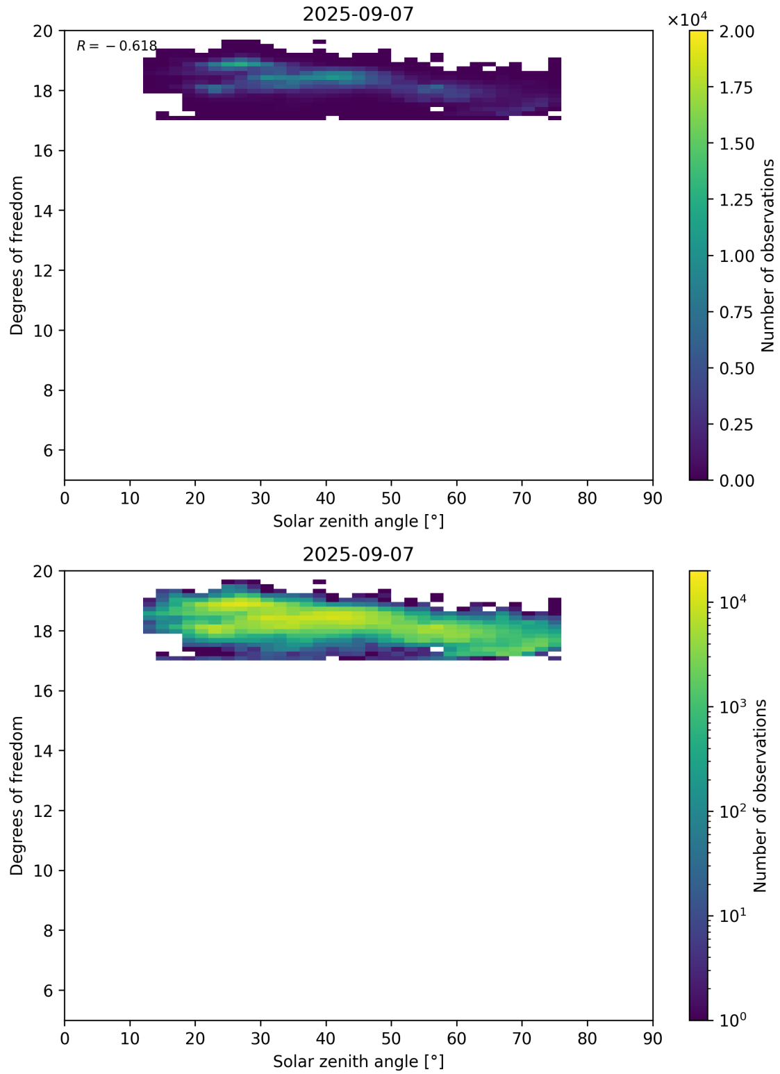
Figure 96: Scatter density plot of “Solar zenith angle” against “Degrees of freedom” for 2025-09-06 to 2025-09-08.
