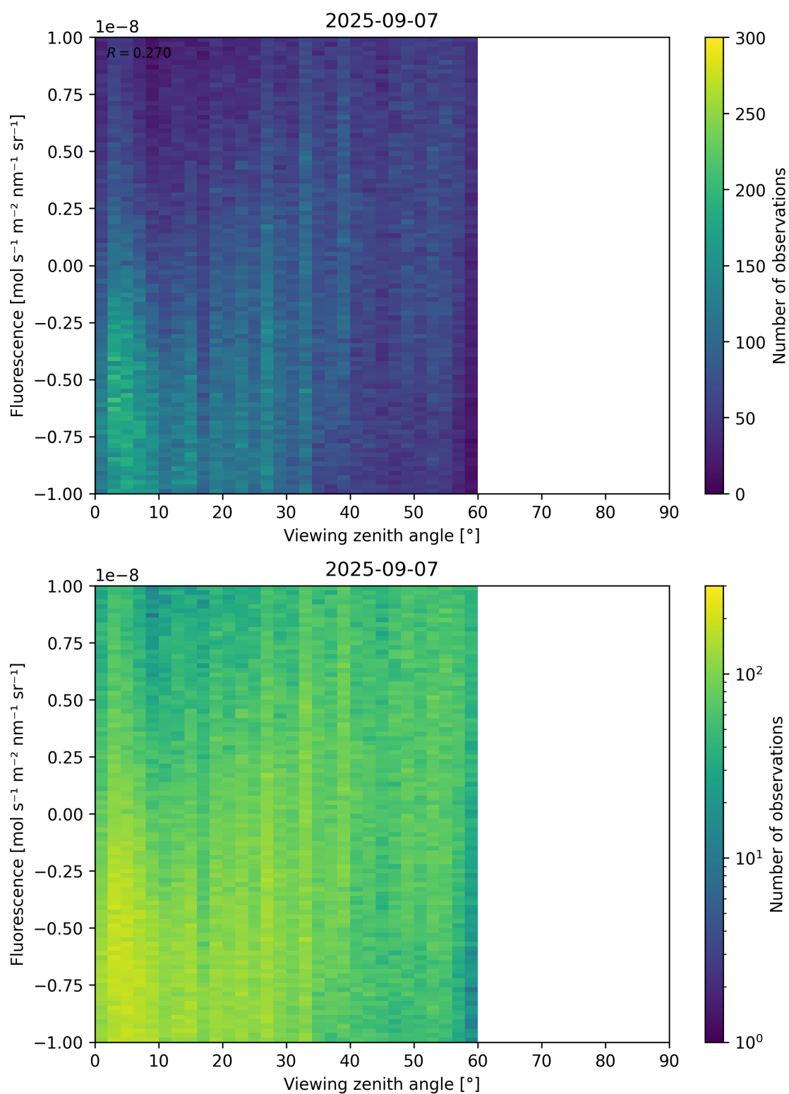
Figure 108: Scatter density plot of “Viewing zenith angle” against “Fluorescence” for 2025-09-06 to 2025-09-08.
