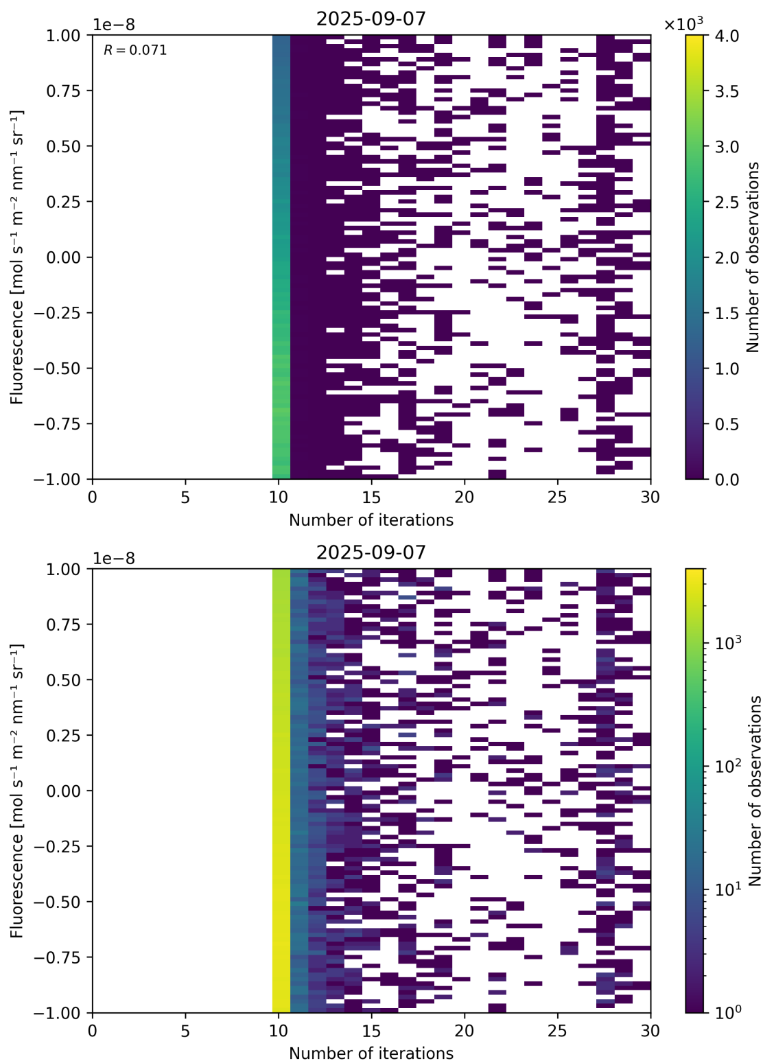
Figure 87: Scatter density plot of “Number of iterations” against “Fluorescence” for 2025-09-06 to 2025-09-08.
