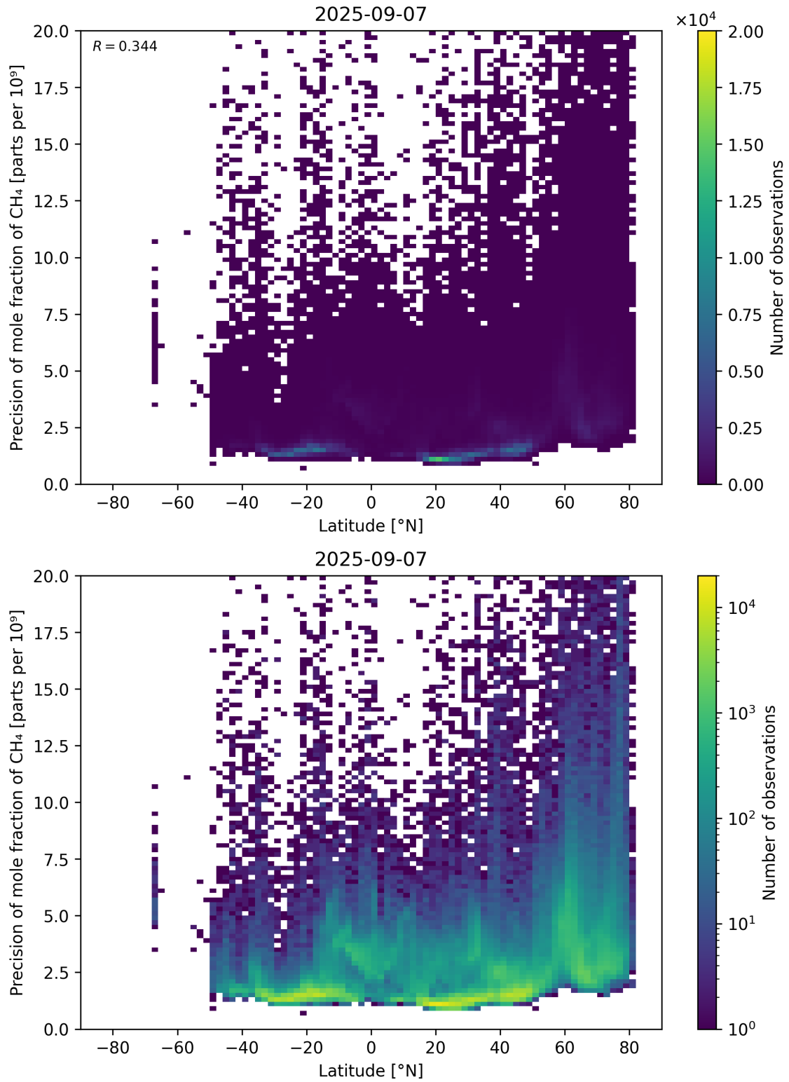
Figure 59: Scatter density plot of “Latitude” against “Precision of mole fraction of \text{CH}_4 ” for 2025-09-06 to 2025-09-08.
