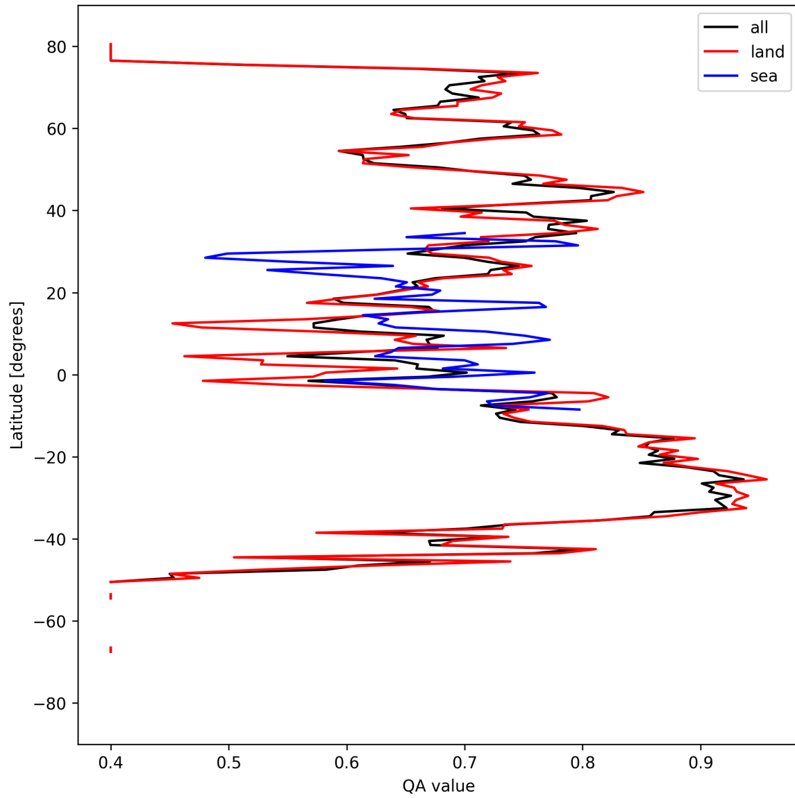
Figure 11: Zonal average of “QA value” for 2025-09-06 to 2025-09-08.
