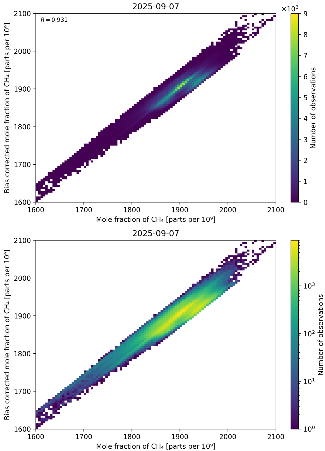
Figure 74: Scatter density plot of “Mole fraction of CH 4 ” against “Bias corrected mole fraction of CH 4 ” for 2025-09-06 to 2025-09-08.
