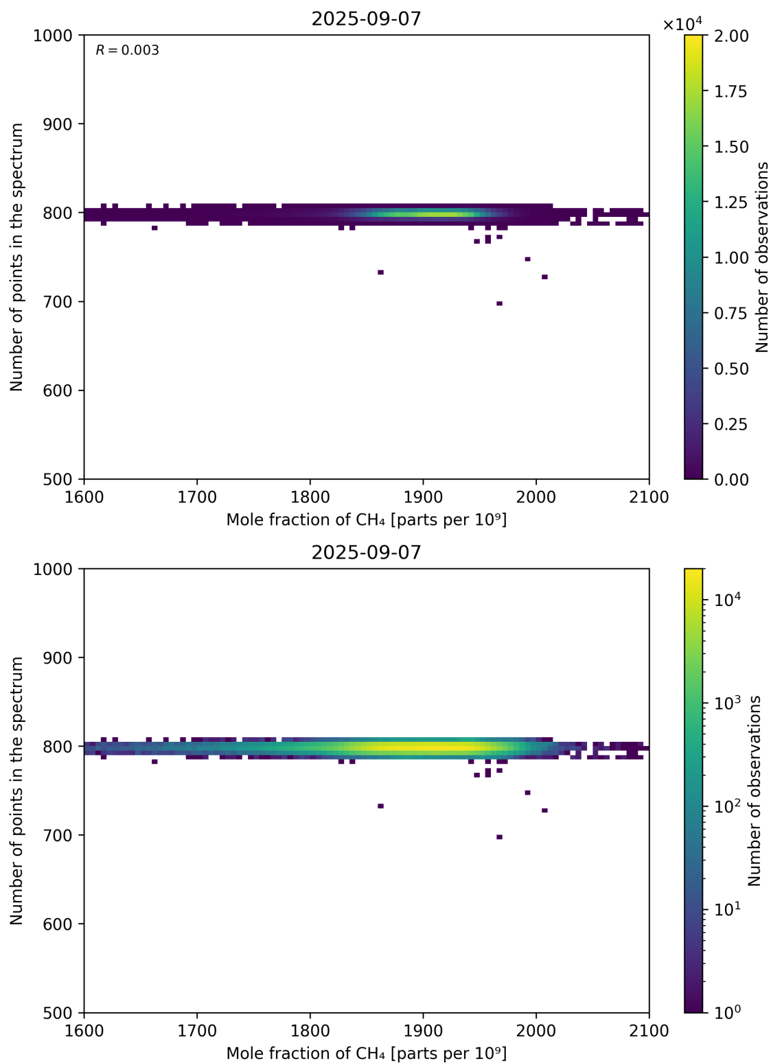
Figure 77: Scatter density plot of “Mole fraction of CH 4 ” against “Number of points in the spectrum” for 2025-09-06 to 2025-09-08.
