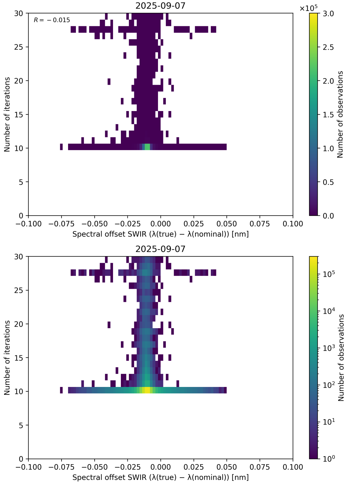
Figure 121: Scatter density plot of “Spectral offset SWIR ( \lambda_{\text{true}} - \lambda_{\text{nominal}} )” against “Number of iterations” for 2025-09-06 to 2025-09-08.
