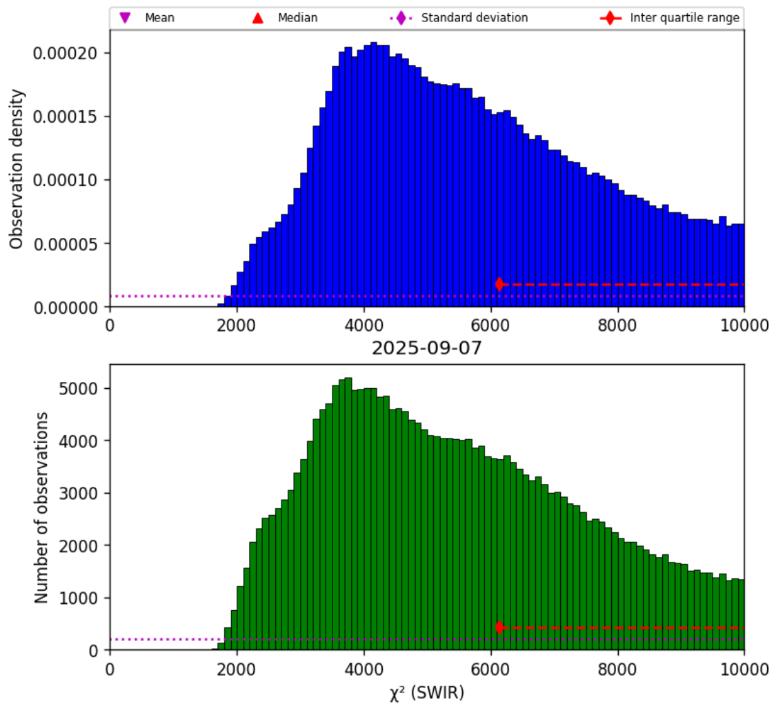
Figure 28: Histogram of “ \chi^2 (SWIR)” for 2025-09-06 to 2025-09-08
