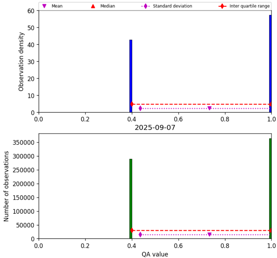
Figure 22: Histogram of “QA value” for 2025-09-06 to 2025-09-08
