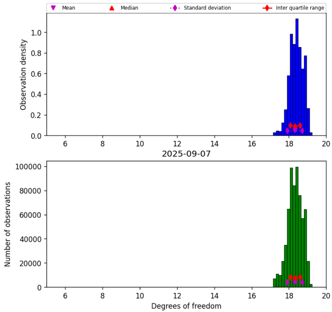
Figure 30: Histogram of “Degrees of freedom” for 2025-09-06 to 2025-09-08
