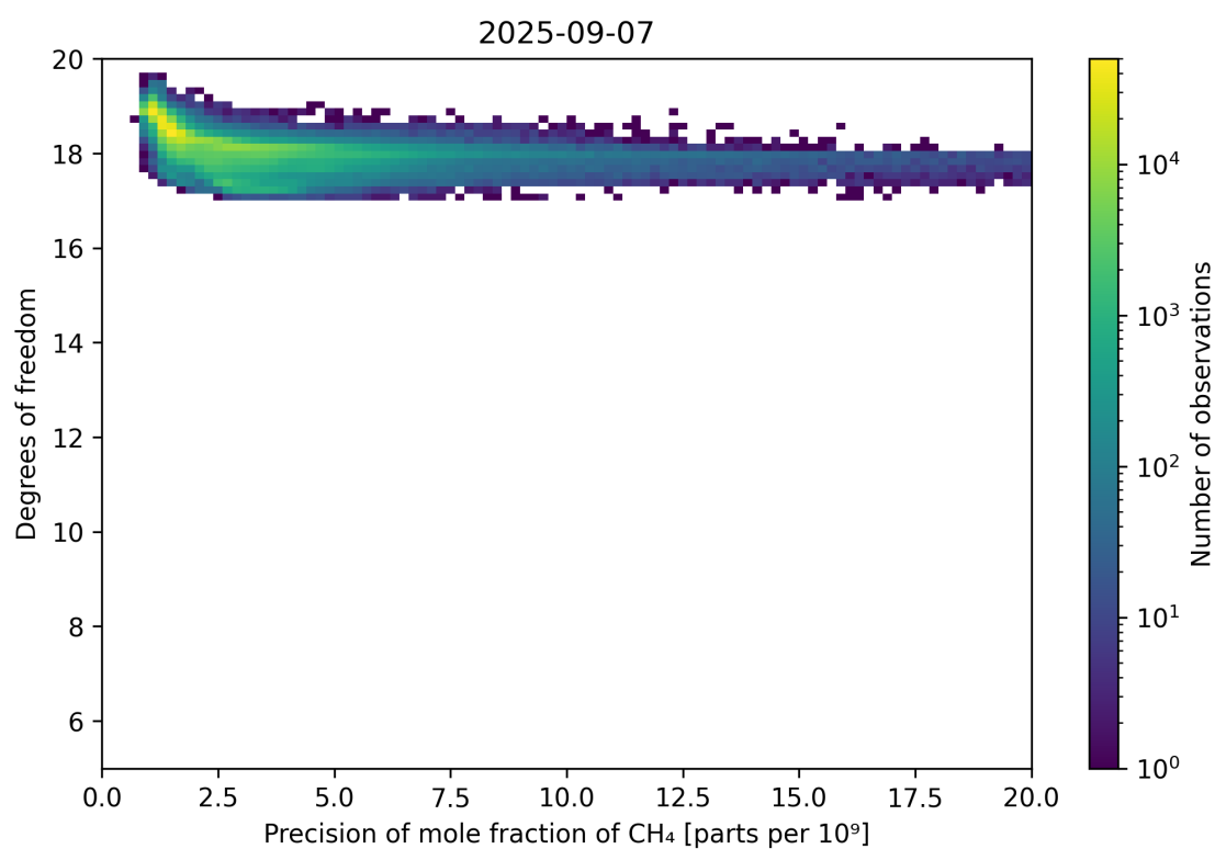
Figure 80: Scatter density plot of “Precision of mole fraction of CH 4 ” against “Degrees of freedom” for 2025-09-06 to 2025-09-08.
