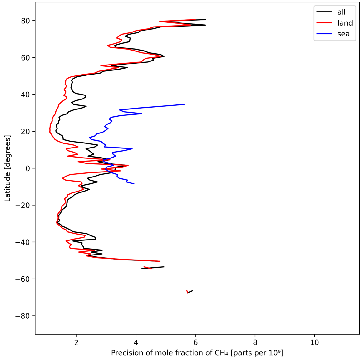
Figure 13: Zonal average of “Precision of mole fraction of CH 4 ” for 2025-09-06 to 2025-09-08.
