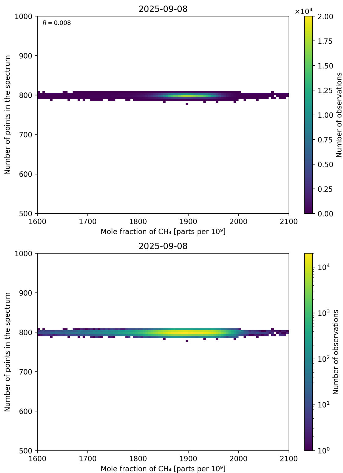
Figure 77: Scatter density plot of “Mole fraction of CH 4 ” against “Number of points in the spectrum” for 2025-09-07 to 2025-09-09.
