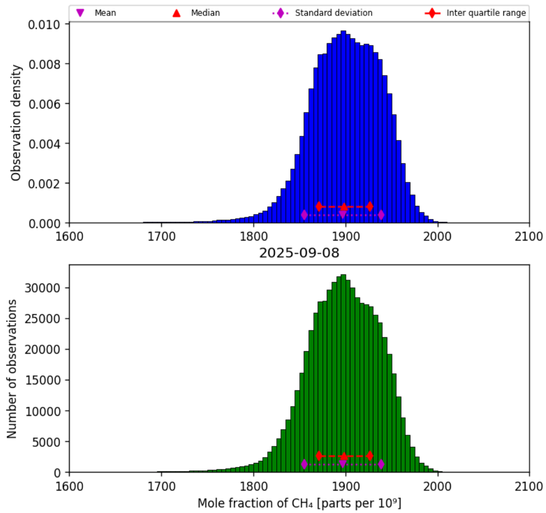
Figure 23: Histogram of “Mole fraction of CH 4 ” for 2025-09-07 to 2025-09-09
