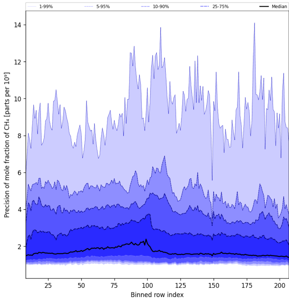
Figure 35: Along track statistics of “Precision of mole fraction of CH 4 ” for 2025-09-07 to 2025-09-09
