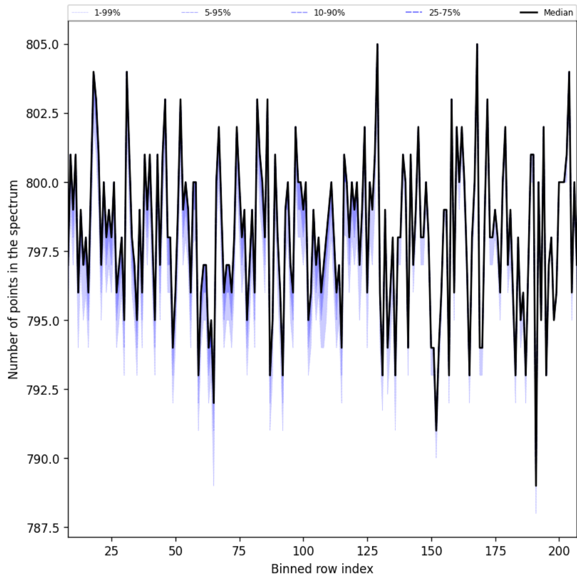
Figure 37: Along track statistics of “Number of points in the spectrum” for 2025-09-07 to 2025-09-09
