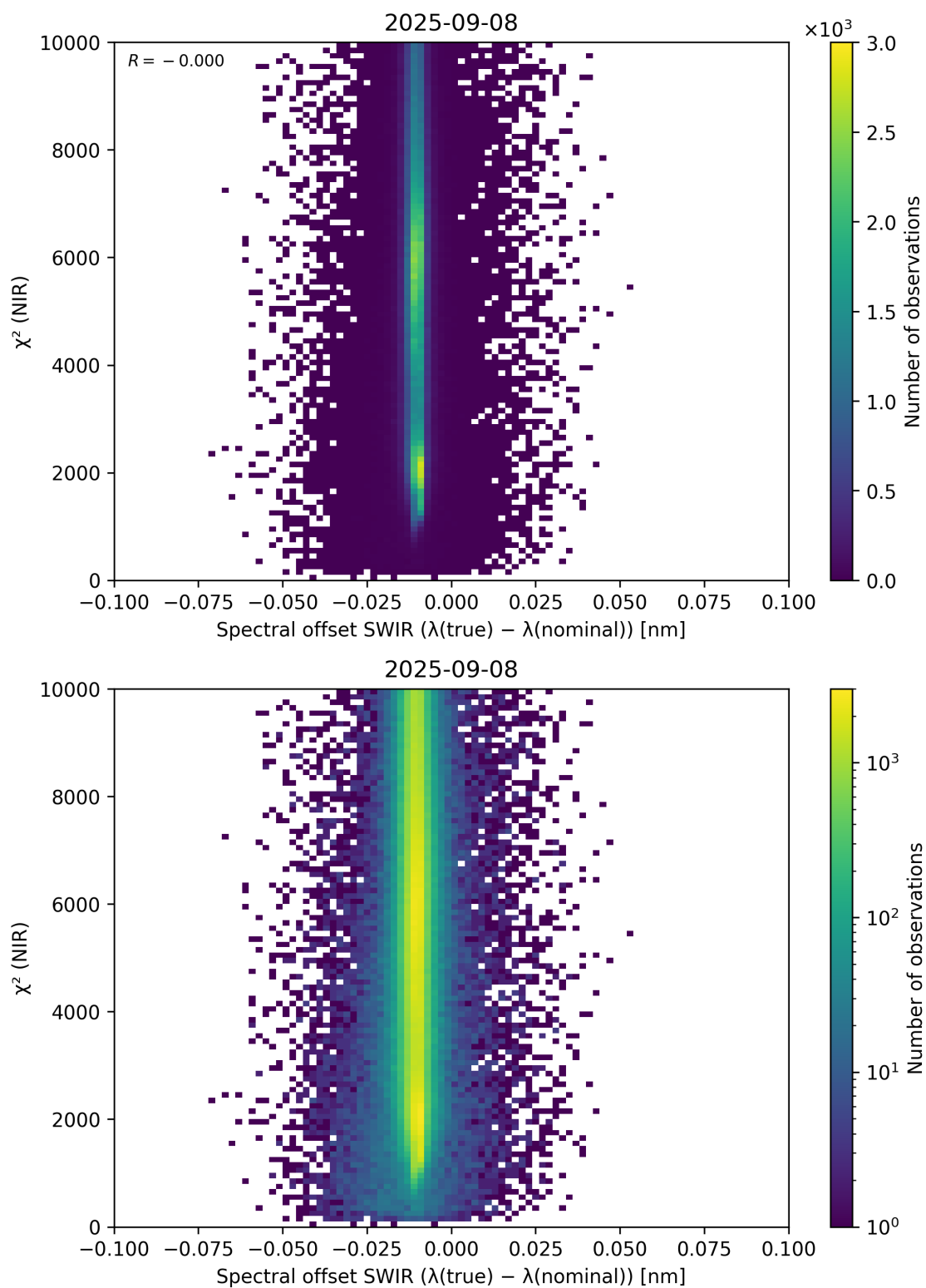
Figure 117: Scatter density plot of “Spectral offset SWIR ( \lambda_{\text{true}} - \lambda_{\text{nominal}} )” against “ \chi^2 (NIR)” for 2025-09-07 to 2025-09-09.
