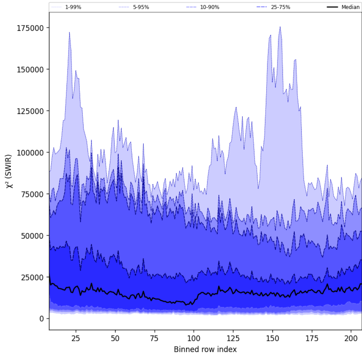
Figure 39: Along track statistics of “ \chi^2 (SWIR)” for 2025-09-07 to 2025-09-09
