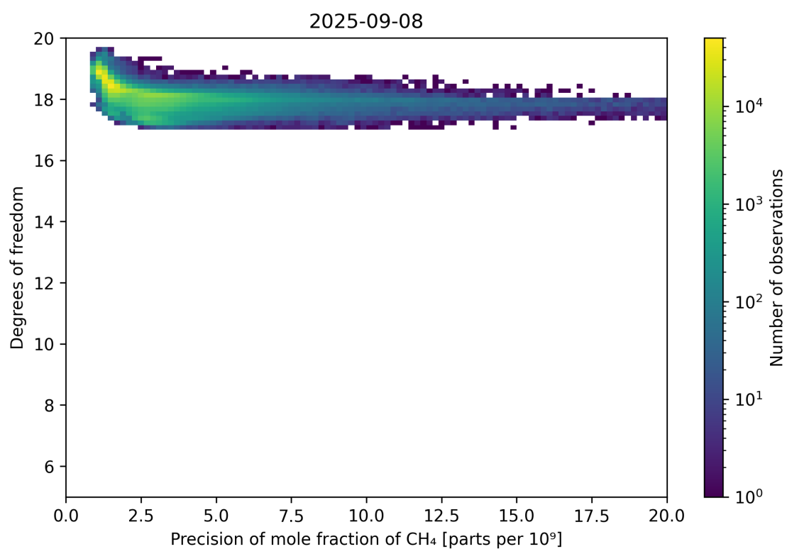
Figure 80: Scatter density plot of “Precision of mole fraction of CH 4 ” against “Degrees of freedom” for 2025-09-07 to 2025-09-09.
