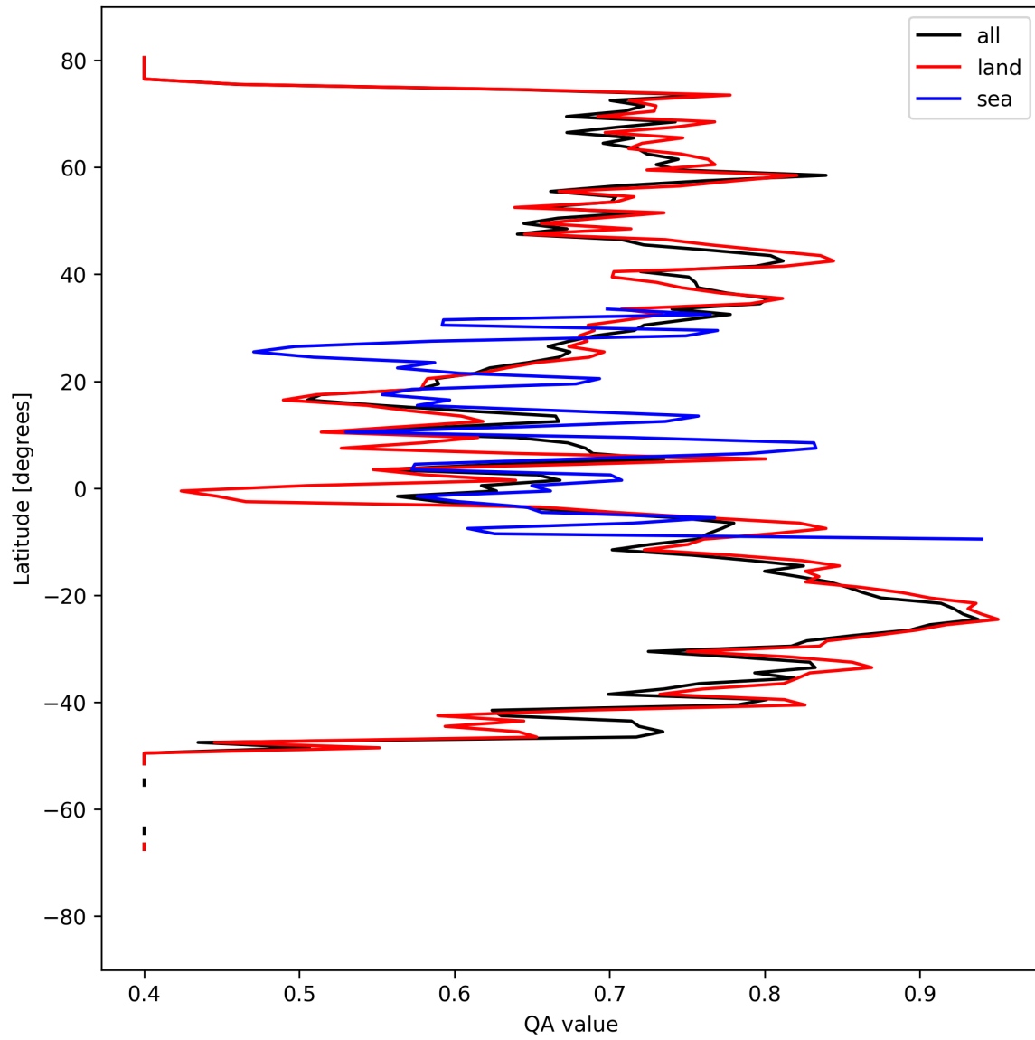
Figure 11: Zonal average of “QA value” for 2025-09-07 to 2025-09-09.
