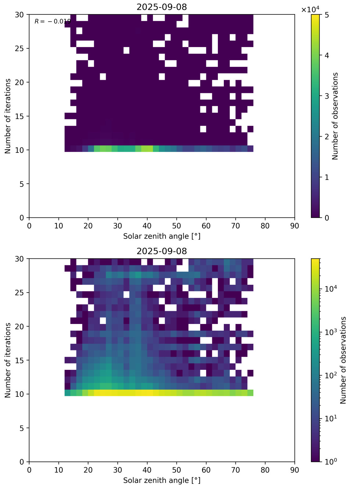
Figure 102: Scatter density plot of “Solar zenith angle” against “Number of iterations” for 2025-09-07 to 2025-09-09.
