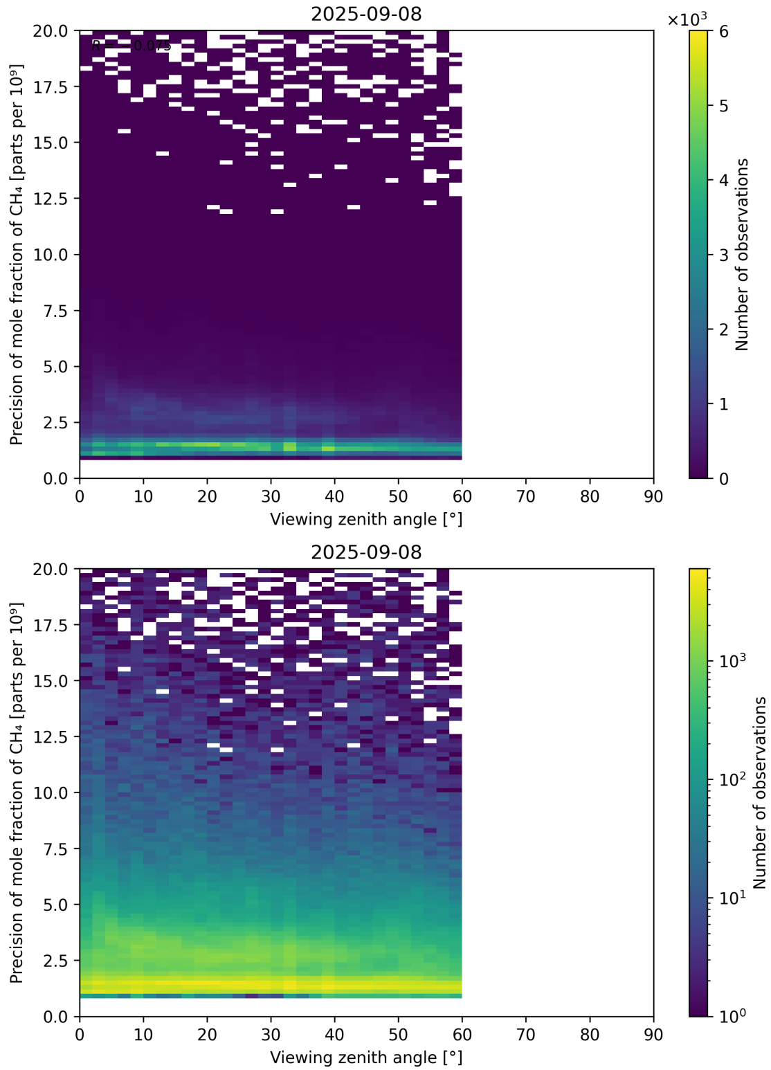
Figure 112: Scatter density plot of “Viewing zenith angle” against “Precision of mole fraction of CH 4 ” for 2025-09-07 to 2025-09-09.
