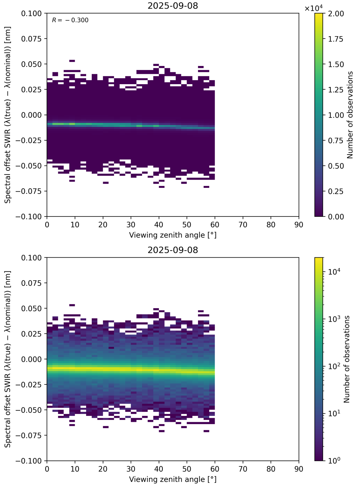
Figure 116: Scatter density plot of “Viewing zenith angle” against “Spectral offset SWIR ( \lambda_{\text{true}} - \lambda_{\text{nominal}} )” for 2025-09-07 to 2025-09-09.
