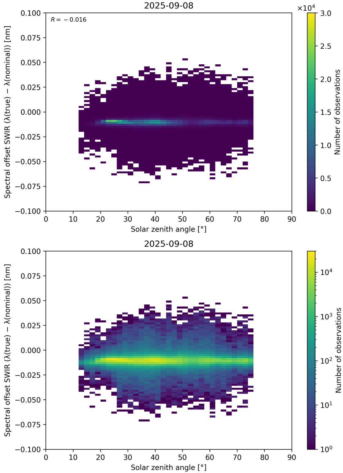
Figure 104: Scatter density plot of “Solar zenith angle” against “Spectral offset SWIR ( \lambda_{\text{true}} - \lambda_{\text{nominal}} )” for 2025-09-07 to 2025-09-09.
