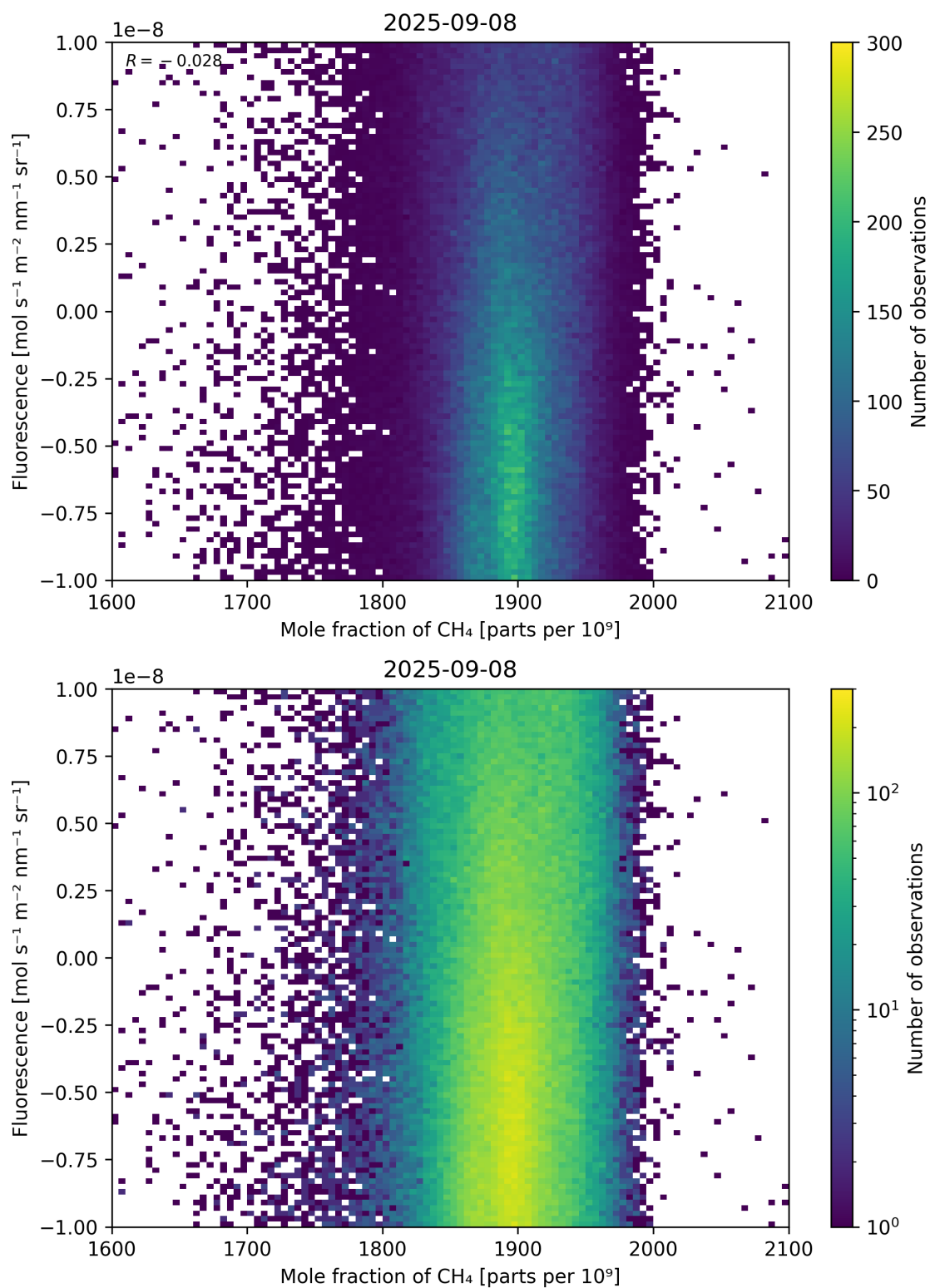
Figure 73: Scatter density plot of “Mole fraction of \text{CH}_4 ” against “Fluorescence” for 2025-09-07 to 2025-09-09.
