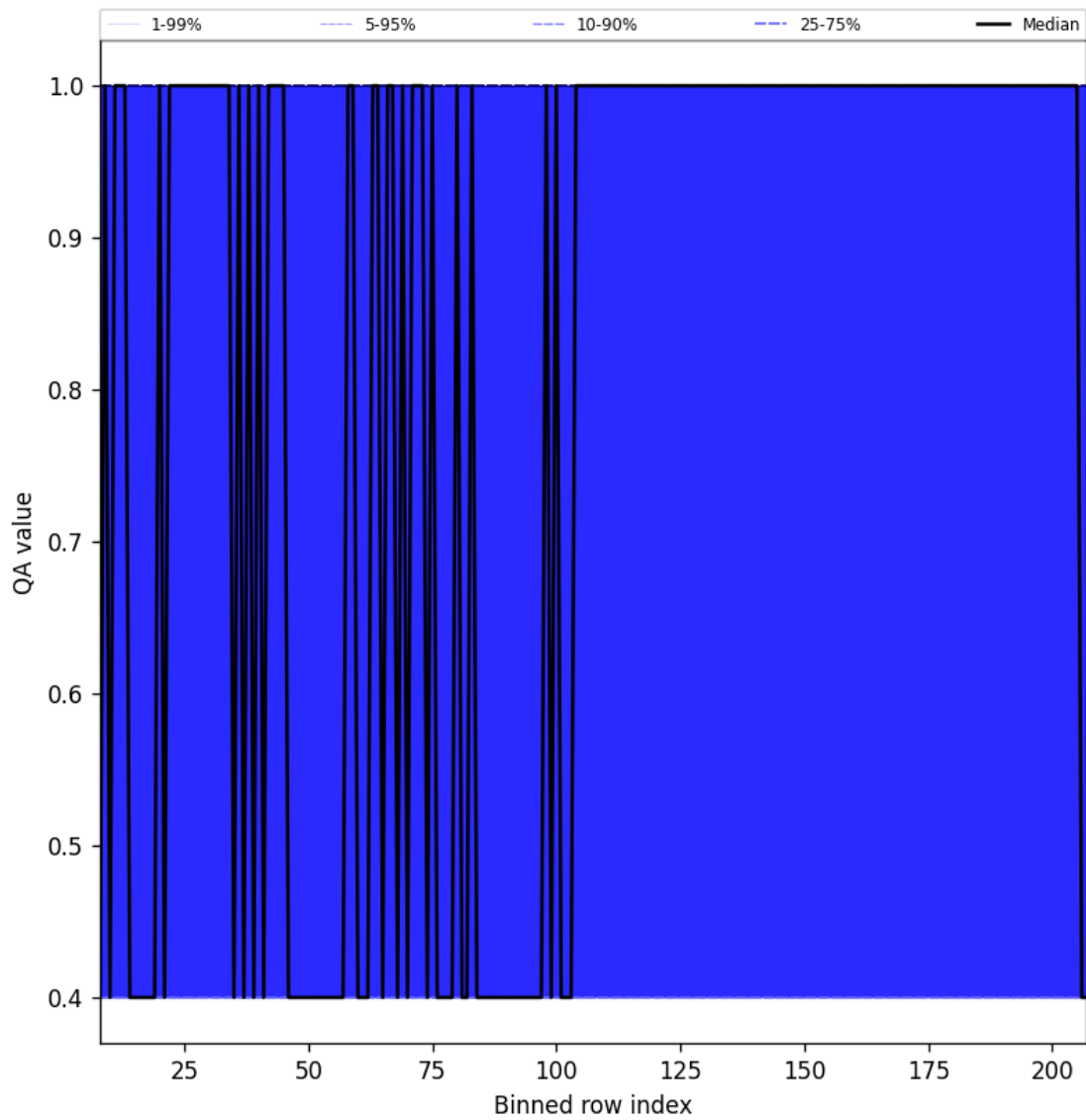
Figure 33: Along track statistics of “QA value” for 2025-09-07 to 2025-09-09
