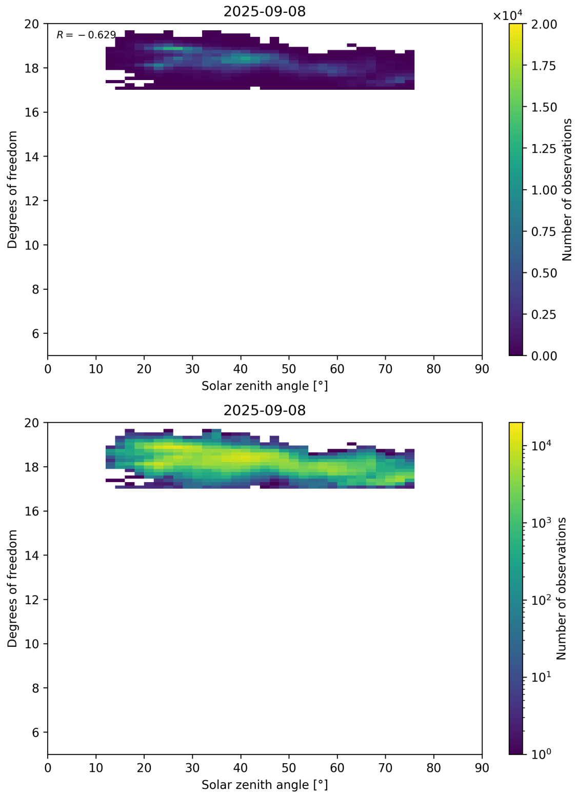
Figure 96: Scatter density plot of “Solar zenith angle” against “Degrees of freedom” for 2025-09-07 to 2025-09-09.
