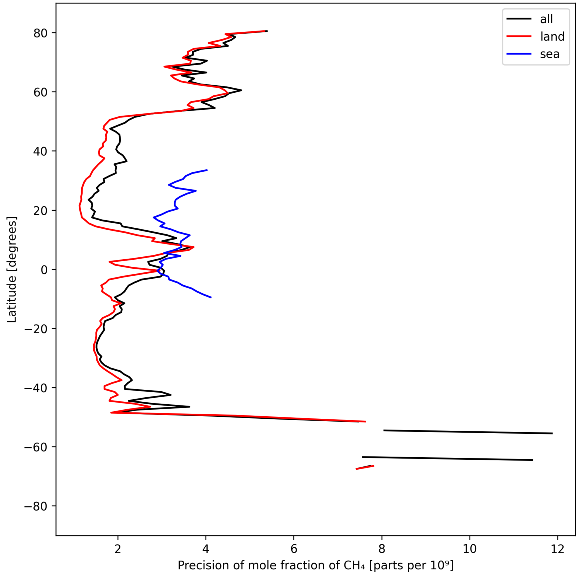
Figure 13: Zonal average of “Precision of mole fraction of CH 4 ” for 2025-09-07 to 2025-09-09.
