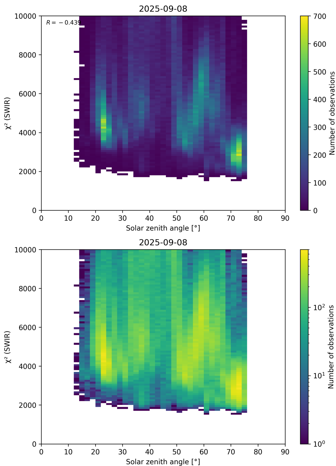
Figure 95: Scatter density plot of “Solar zenith angle” against “ \chi^2 (SWIR)” for 2025-09-07 to 2025-09-09.
