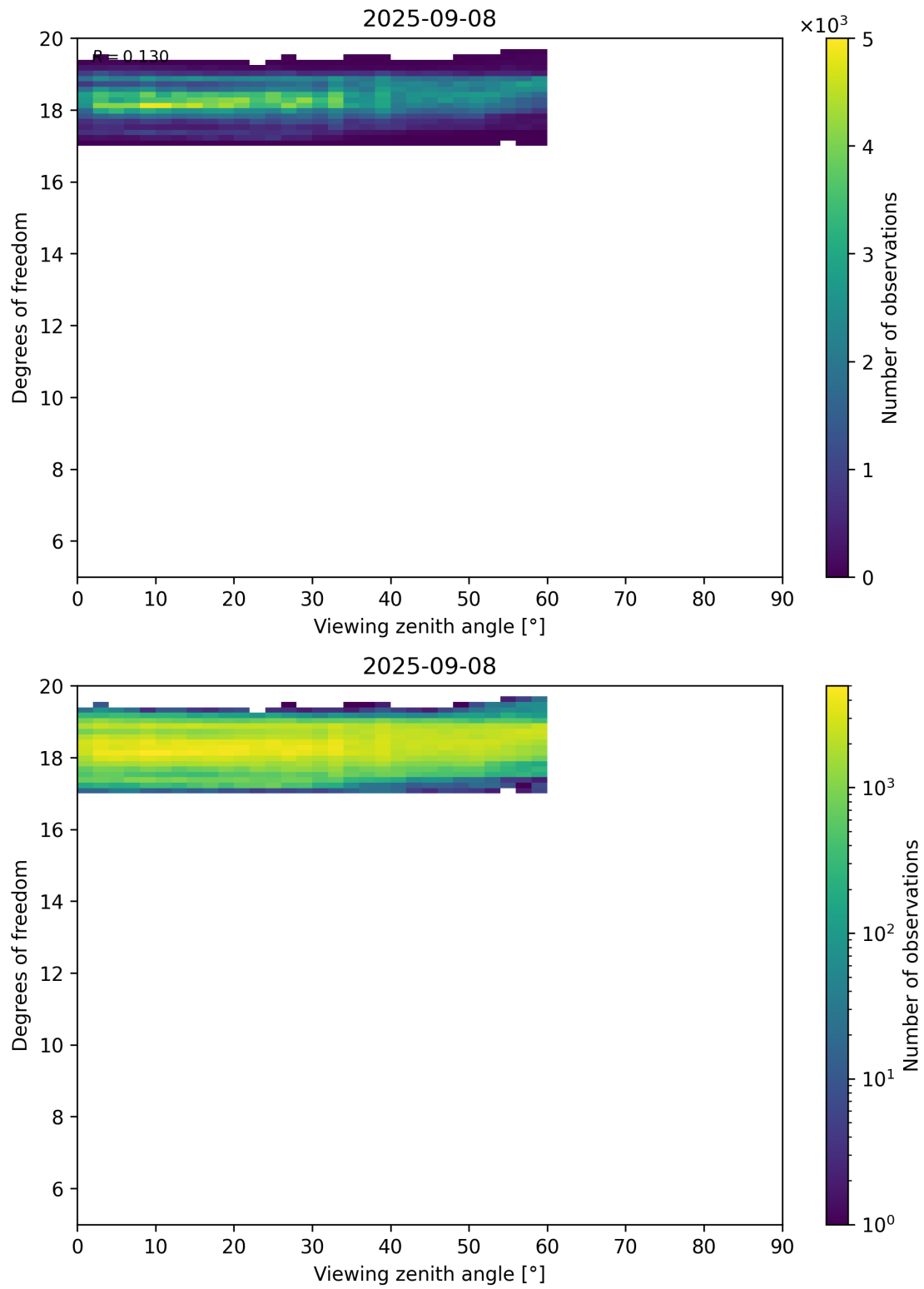
Figure 107: Scatter density plot of “Viewing zenith angle” against “Degrees of freedom” for 2025-09-07 to 2025-09-09.
