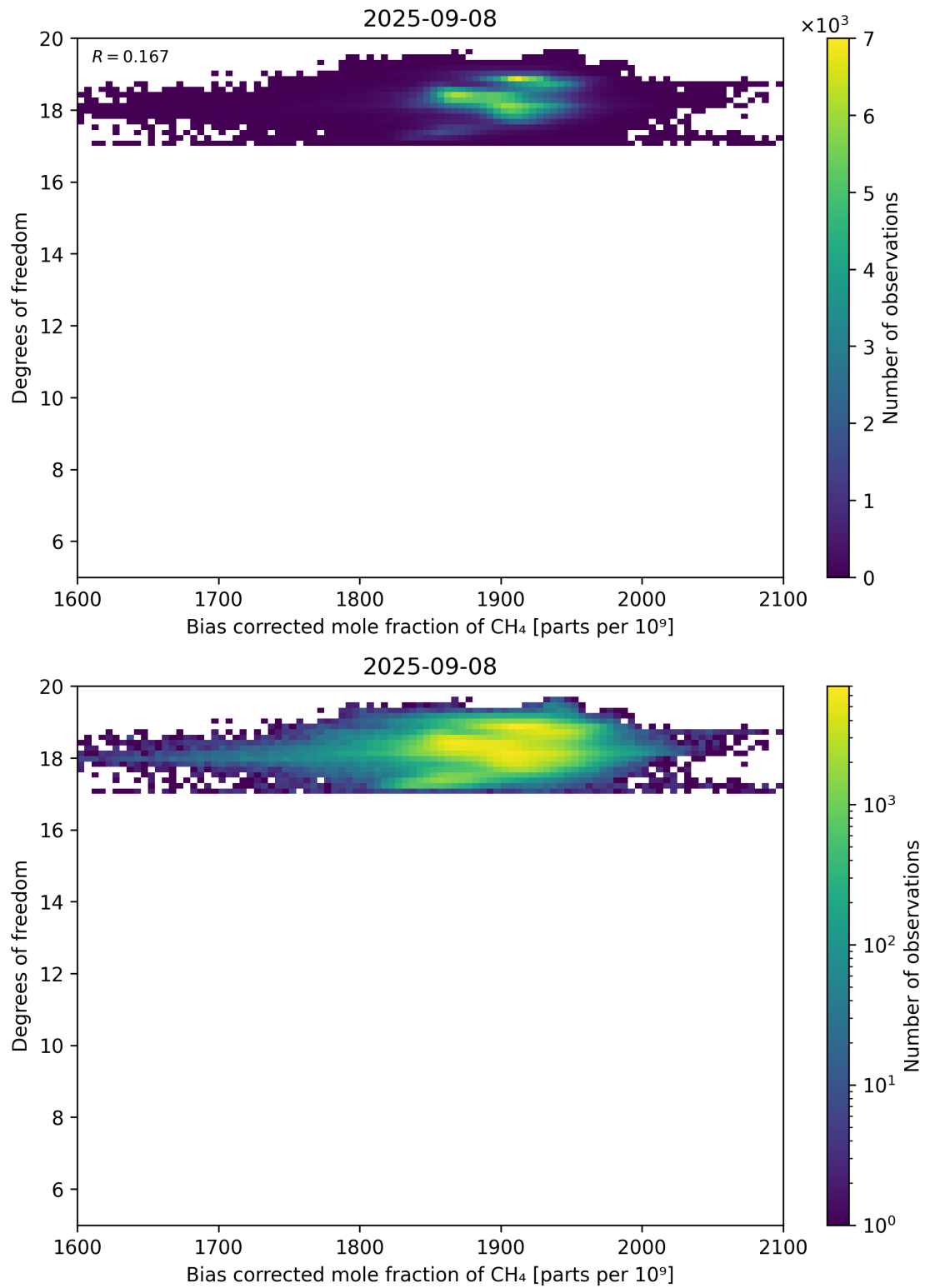
Figure 65: Scatter density plot of “Bias corrected mole fraction of CH 4 ” against “Degrees of freedom” for 2025-09-07 to 2025-09-09.
