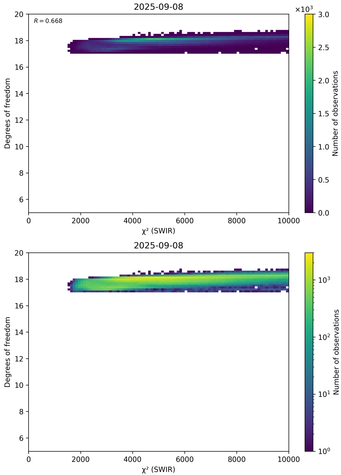
Figure 48: Scatter density plot of “ \chi^2 (SWIR)” against “Degrees of freedom” for 2025-09-07 to 2025-09-09.
