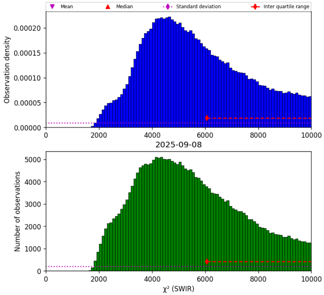
Figure 28: Histogram of “ \chi^2 (SWIR)” for 2025-09-07 to 2025-09-09
