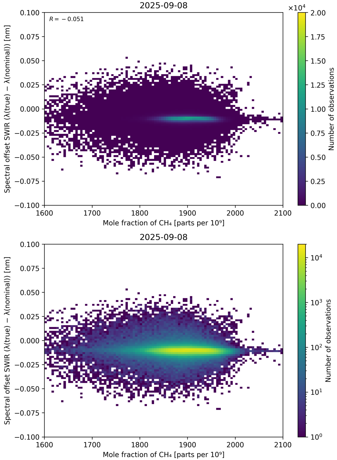
Figure 86: Scatter density plot of “Mole fraction of CH 4 ” against “Spectral offset SWIR ( \lambda_{\text{true}} - \lambda_{\text{nominal}} )” for 2025-09-07 to 2025-09-09.
