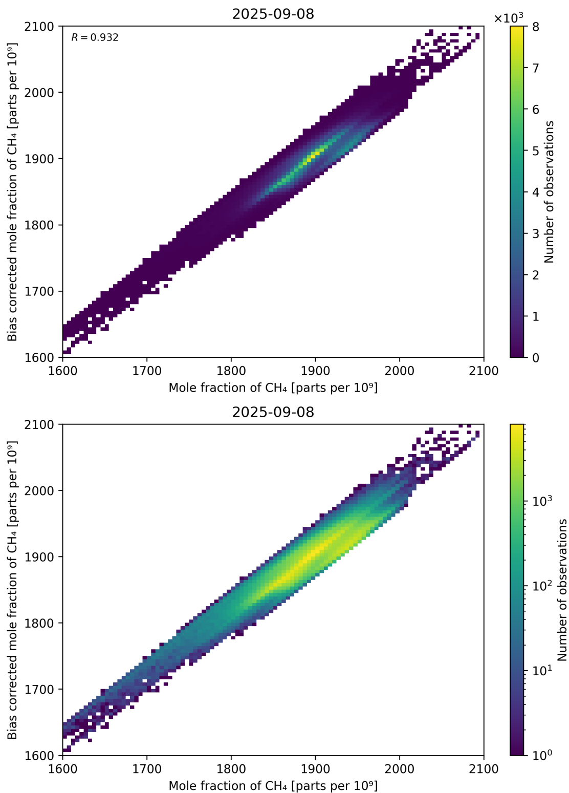
Figure 74: Scatter density plot of “Mole fraction of CH 4 ” against “Bias corrected mole fraction of CH 4 ” for 2025-09-07 to 2025-09-09.
