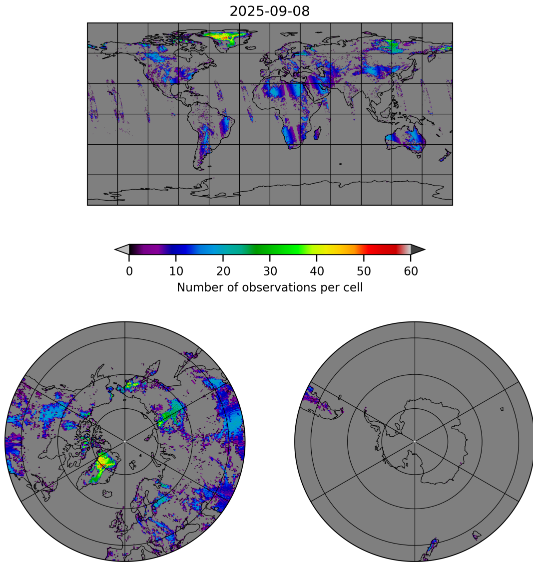
Figure 10: Map of the number of observations for 2025-09-07 to 2025-09-09
