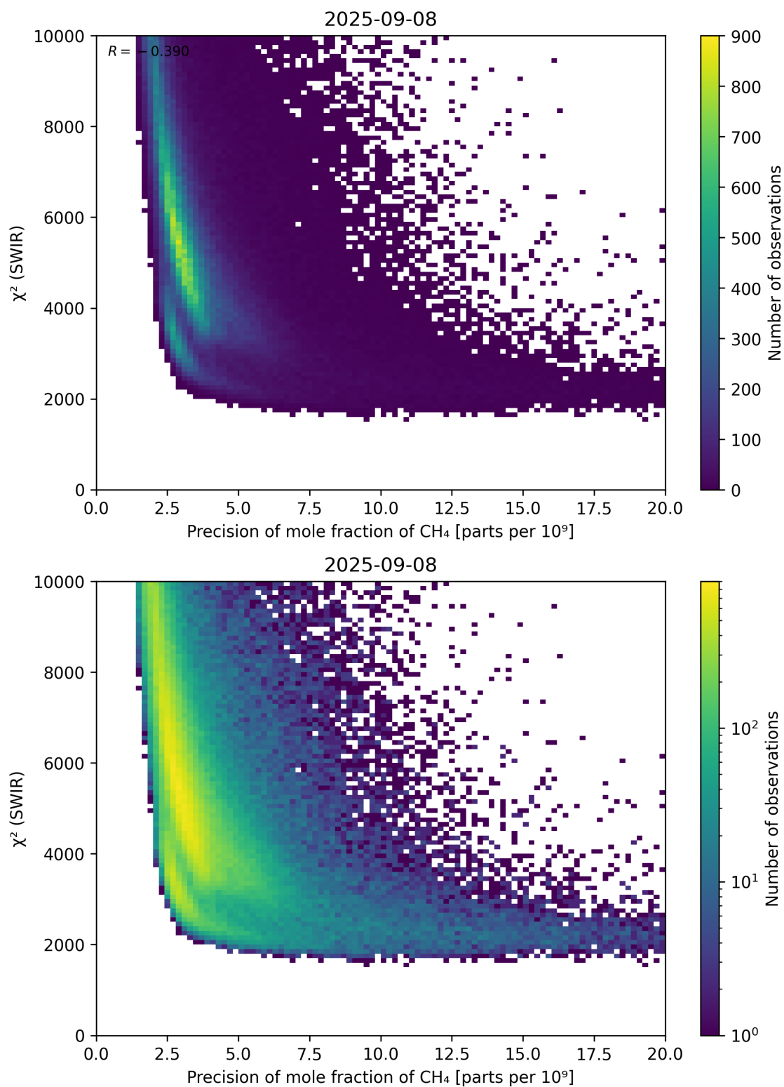
Figure 79: Scatter density plot of “Precision of mole fraction of \text{CH}_4 ” against “ \chi^2 (SWIR)” for 2025-09-07 to 2025-09-09.
