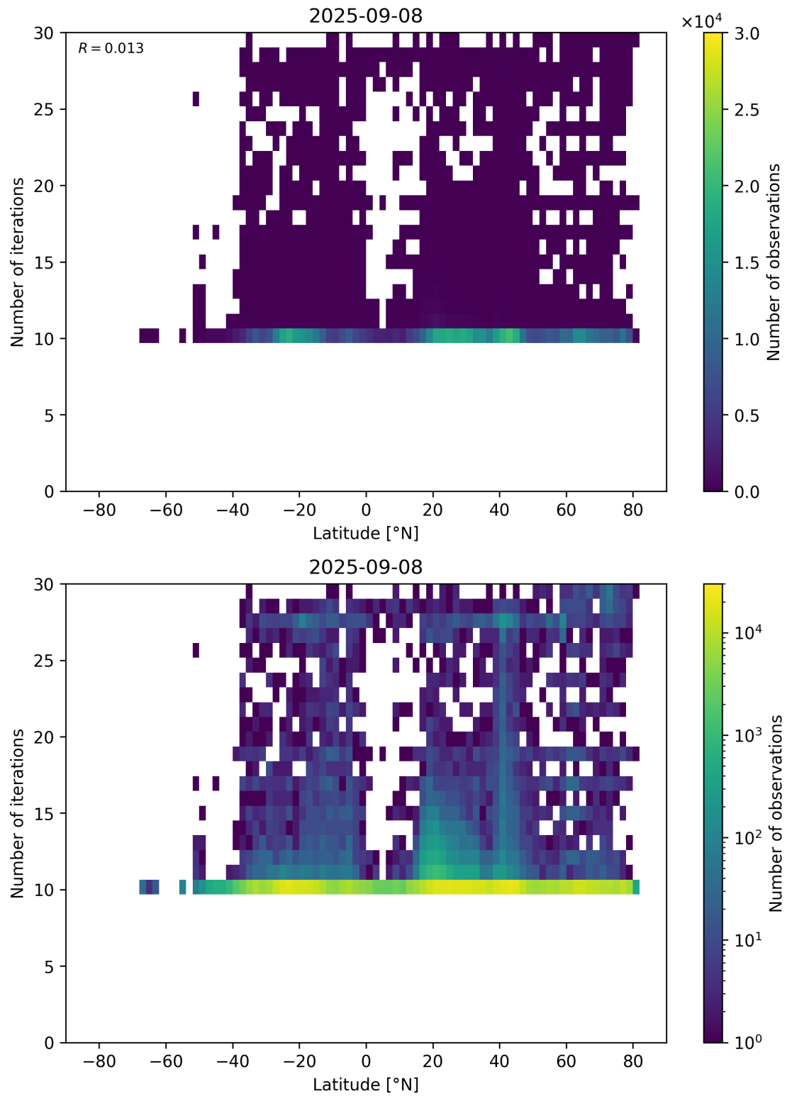
Figure 60: Scatter density plot of “Latitude” against “Number of iterations” for 2025-09-07 to 2025-09-09.
