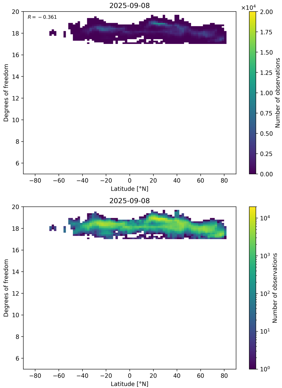
Figure 55: Scatter density plot of “Latitude” against “Degrees of freedom” for 2025-09-07 to 2025-09-09.
