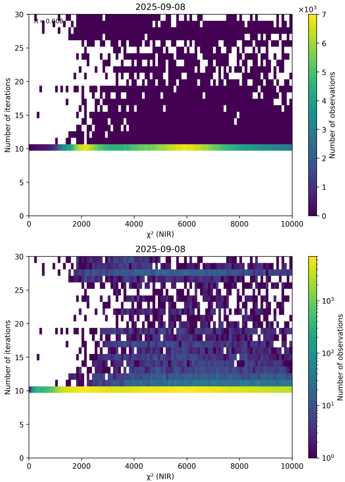
Figure 46: Scatter density plot of “ \chi^2 (NIR)” against “Number of iterations” for 2025-09-07 to 2025-09-09.
