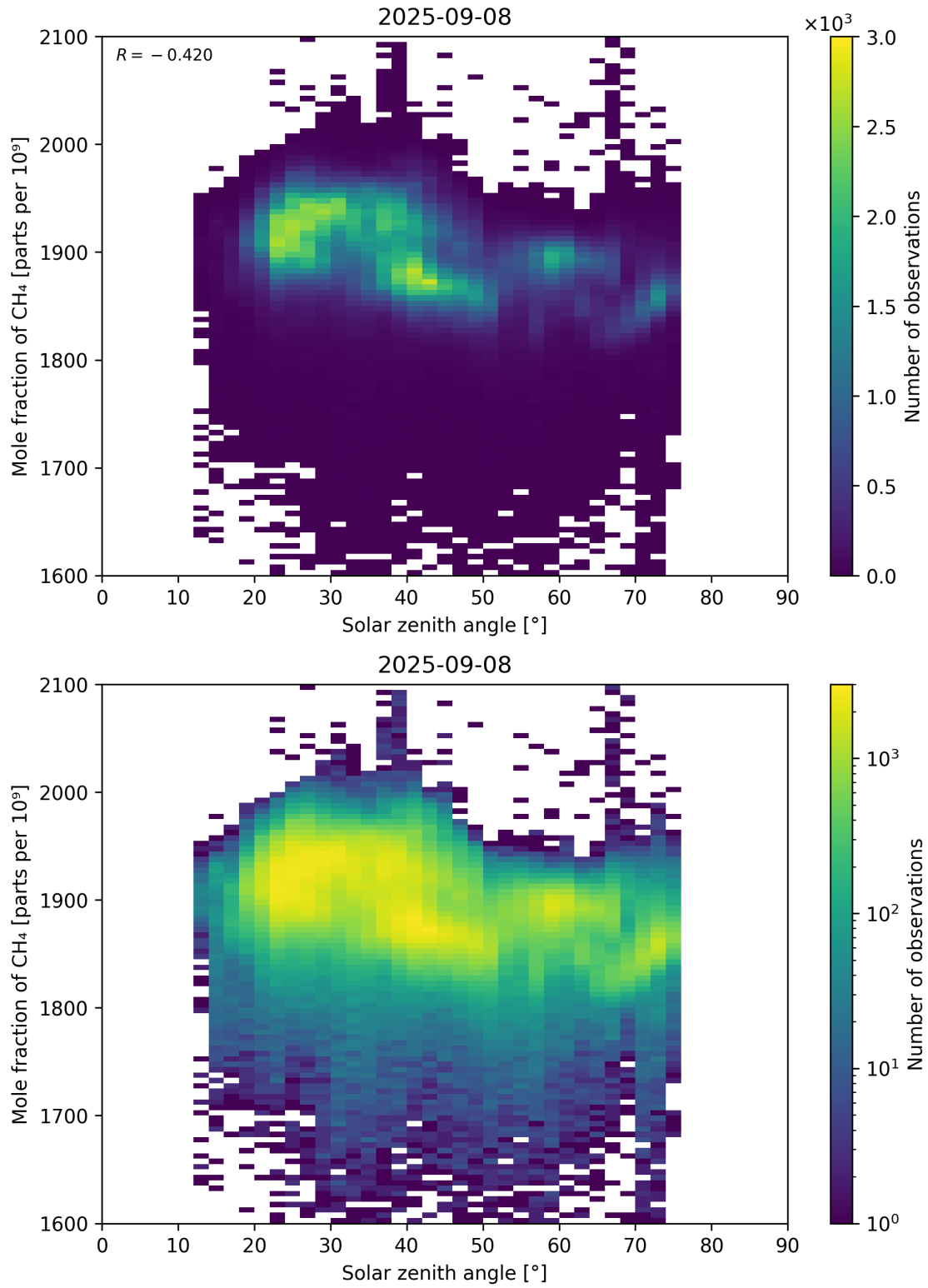
Figure 99: Scatter density plot of “Solar zenith angle” against “Mole fraction of \text{CH}_4 ” for 2025-09-07 to 2025-09-09.
