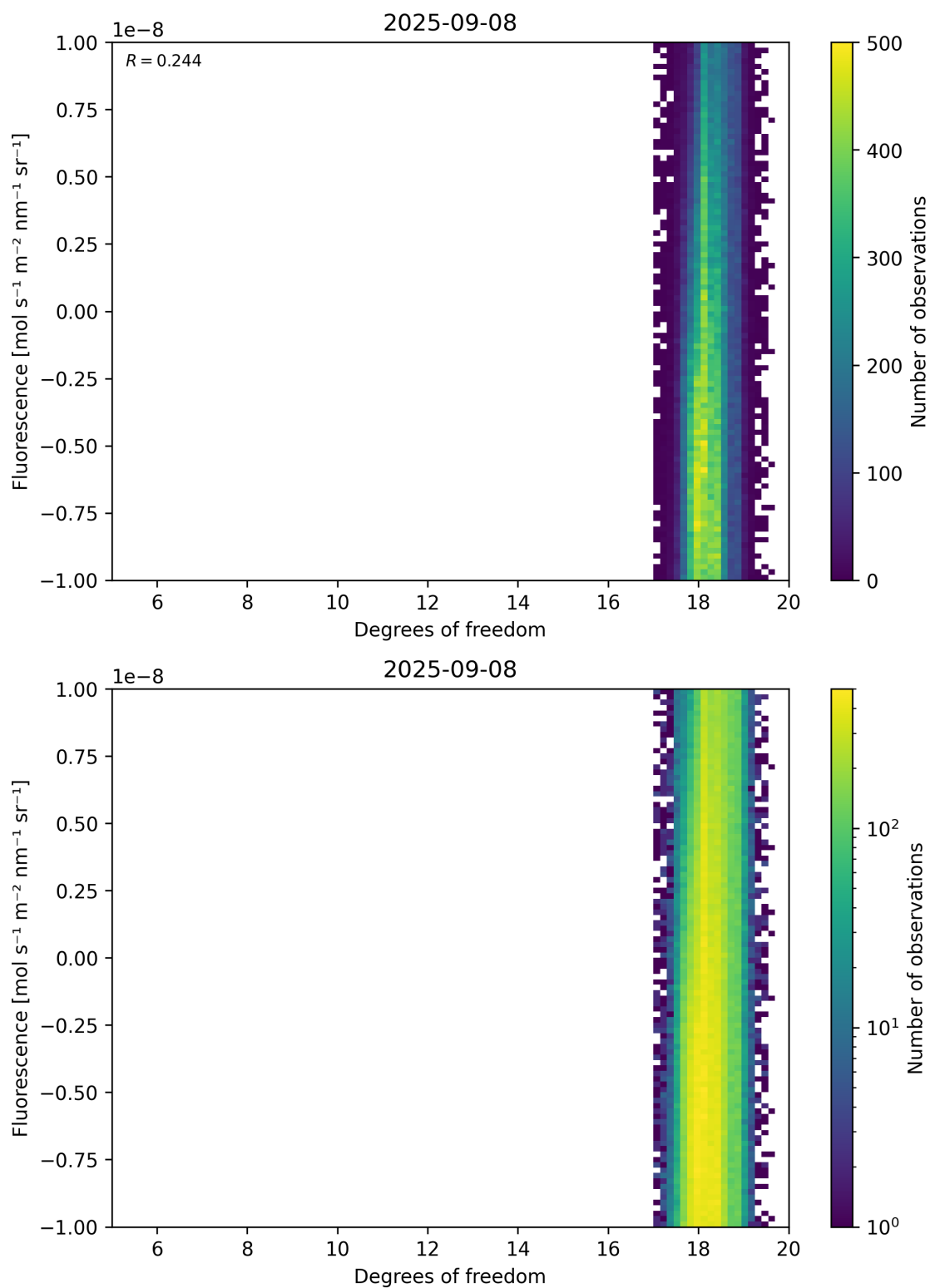
Figure 51: Scatter density plot of “Degrees of freedom” against “Fluorescence” for 2025-09-07 to 2025-09-09.
