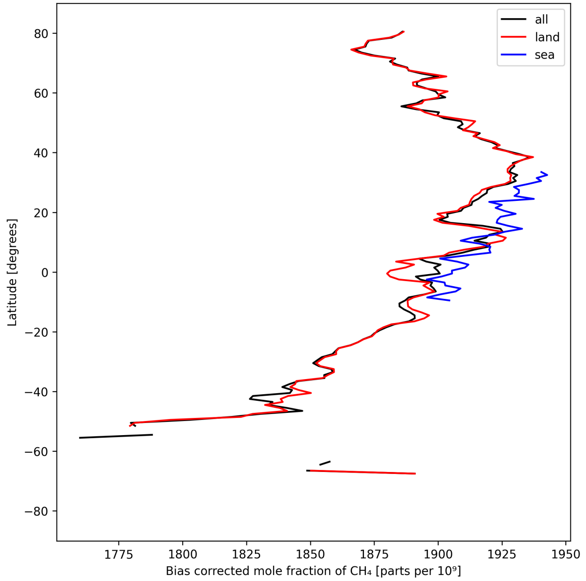
Figure 14: Zonal average of “Bias corrected mole fraction of CH 4 ” for 2025-09-07 to 2025-09-09.
