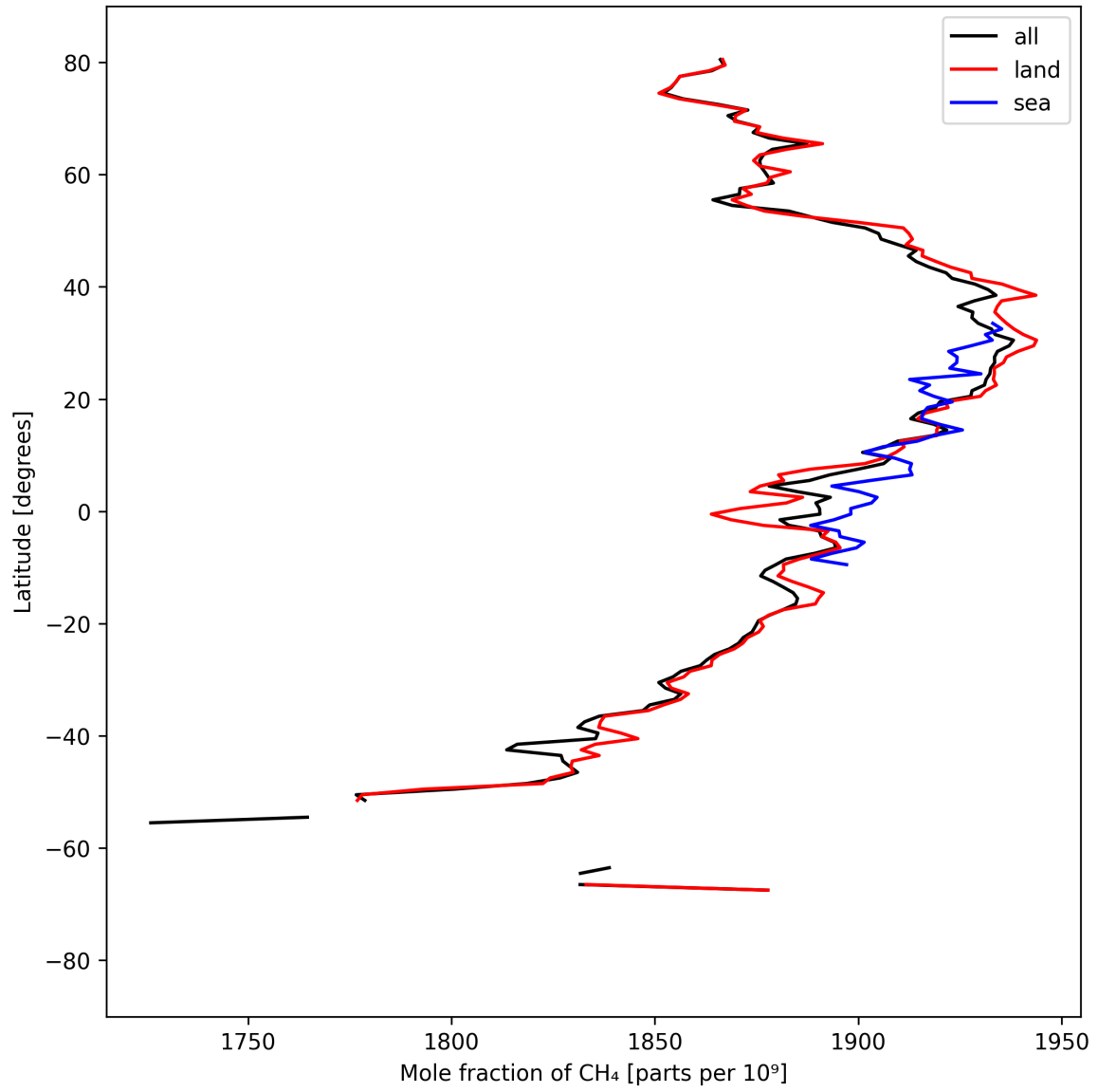
Figure 12: Zonal average of “Mole fraction of CH 4 ” for 2025-09-07 to 2025-09-09.
