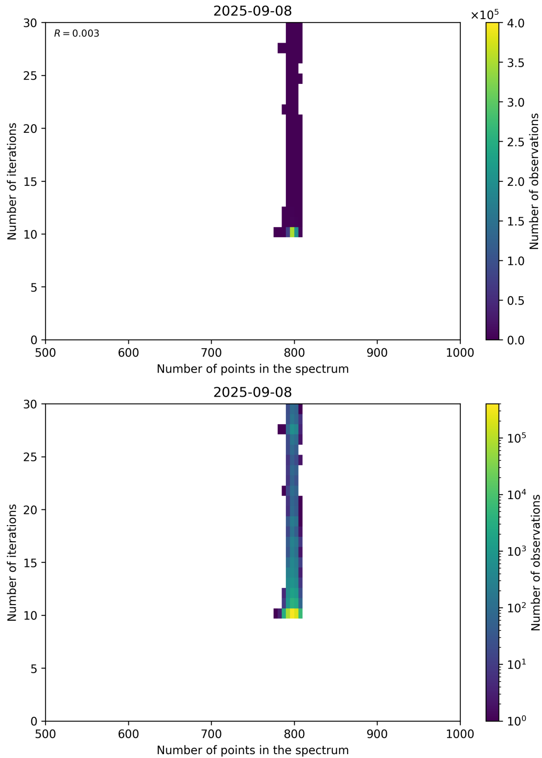
Figure 92: Scatter density plot of “Number of points in the spectrum” against “Number of iterations” for 2025-09-07 to 2025-09-09.
