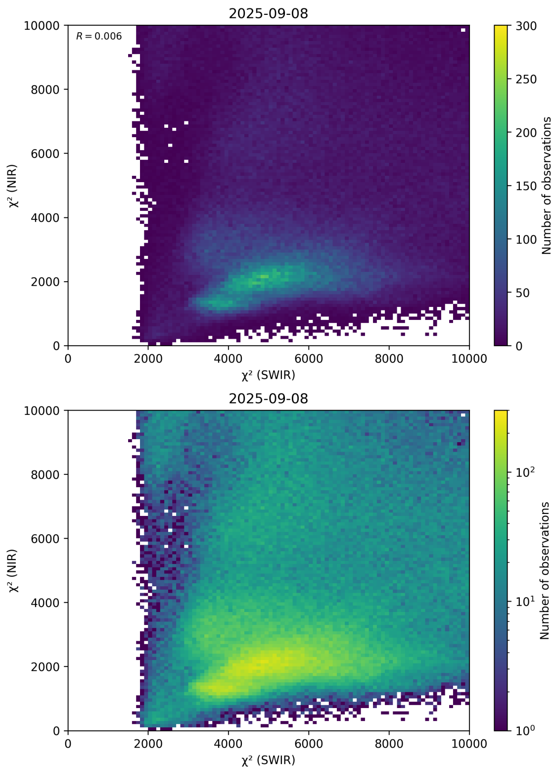
Figure 47: Scatter density plot of “ \chi^2 (SWIR)” against “ \chi^2 (NIR)” for 2025-09-07 to 2025-09-09.
