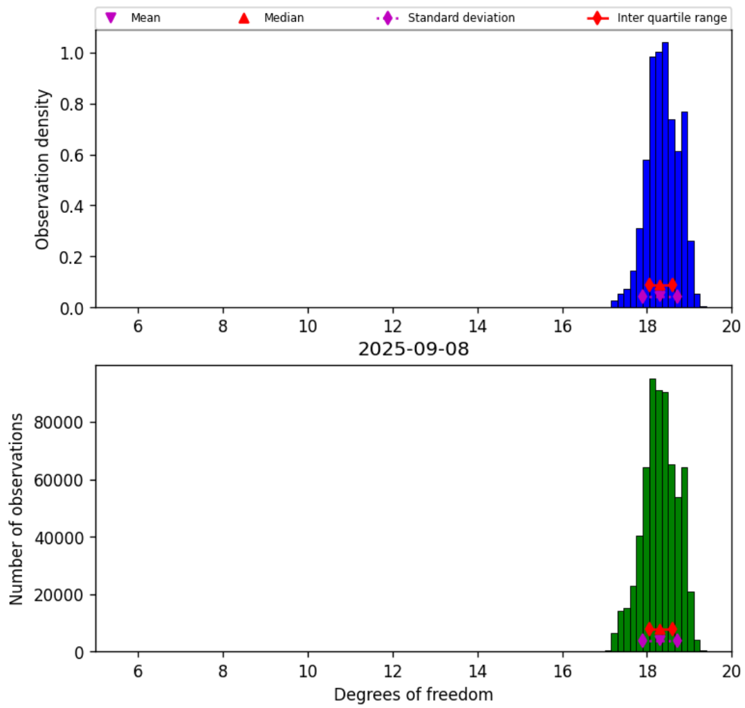
Figure 30: Histogram of “Degrees of freedom” for 2025-09-07 to 2025-09-09
