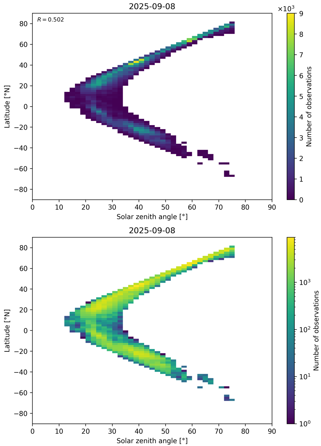
Figure 98: Scatter density plot of “Solar zenith angle” against “Latitude” for 2025-09-07 to 2025-09-09.
