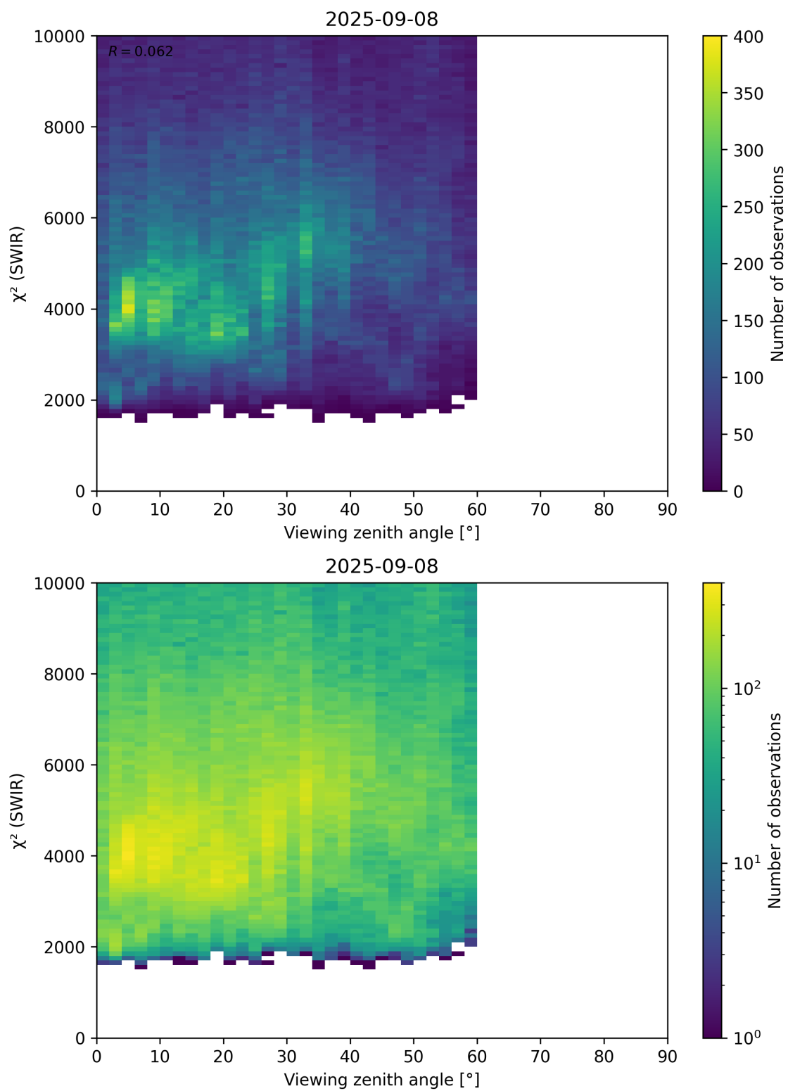
Figure 106: Scatter density plot of “Viewing zenith angle” against “ \chi^2 (SWIR)” for 2025-09-07 to 2025-09-09.
