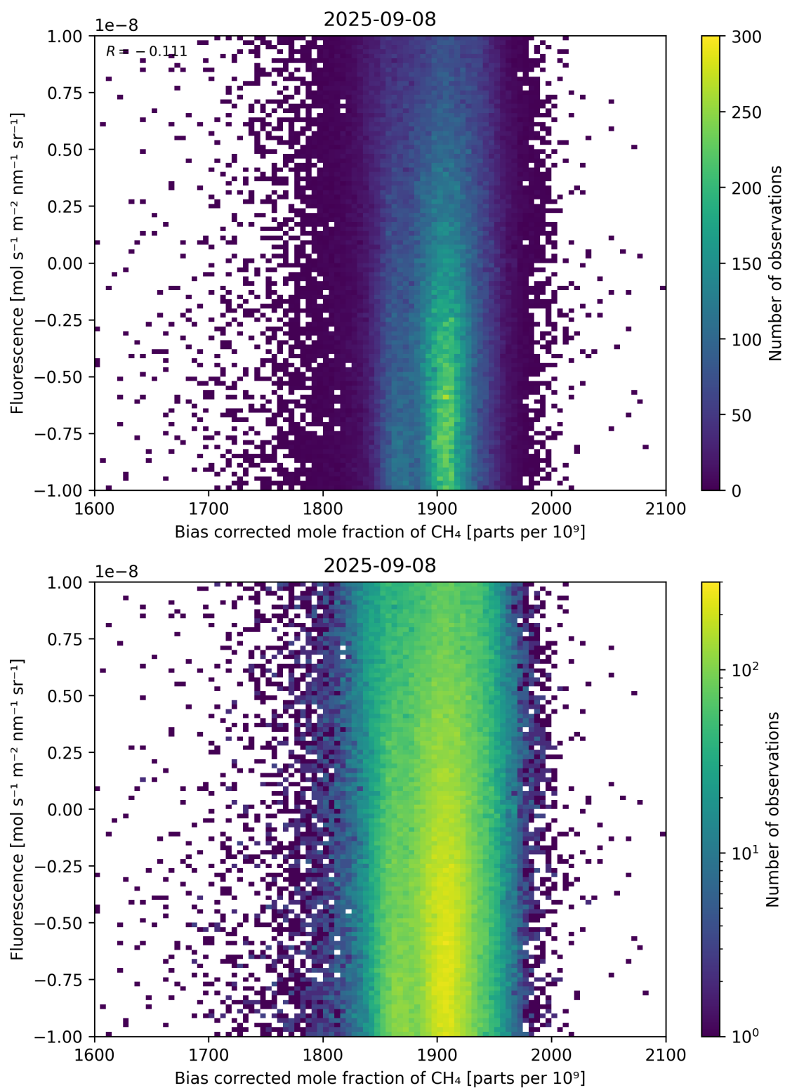
Figure 66: Scatter density plot of “Bias corrected mole fraction of \text{CH}_4 ” against “Fluorescence” for 2025-09-07 to 2025-09-09.
