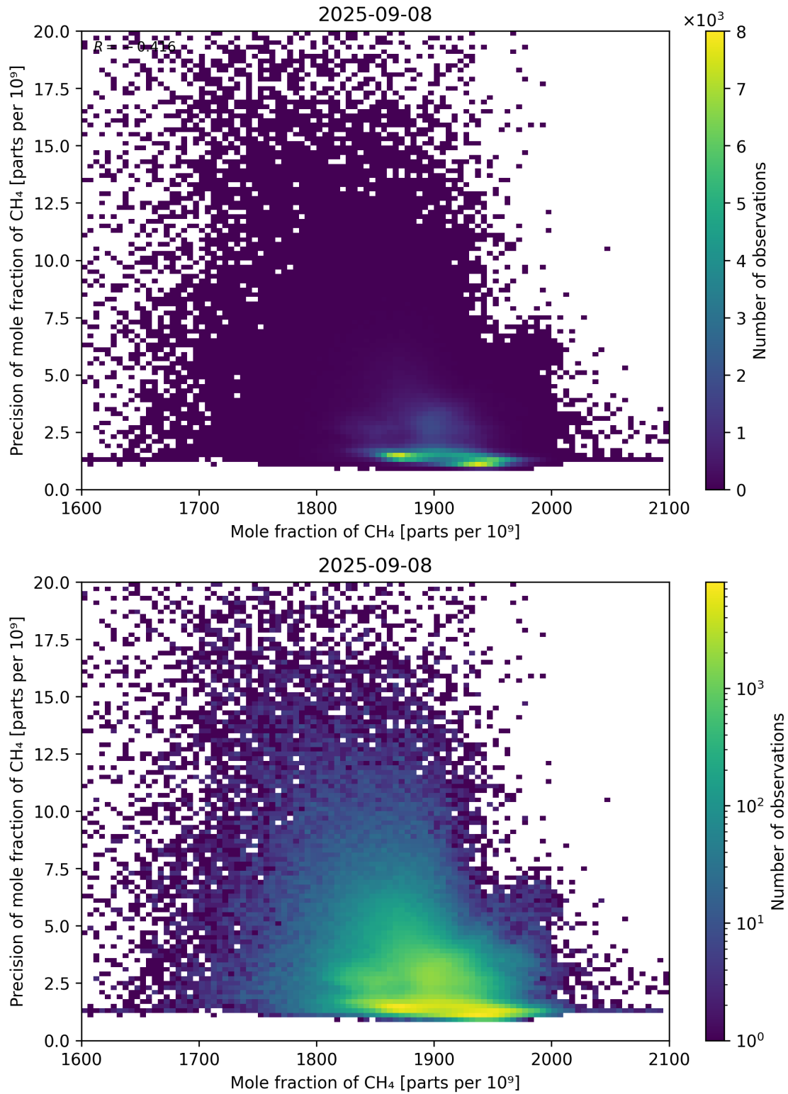
Figure 75: Scatter density plot of “Mole fraction of CH 4 ” against “Precision of mole fraction of CH 4 ” for 2025-09-07 to 2025-09-09.
