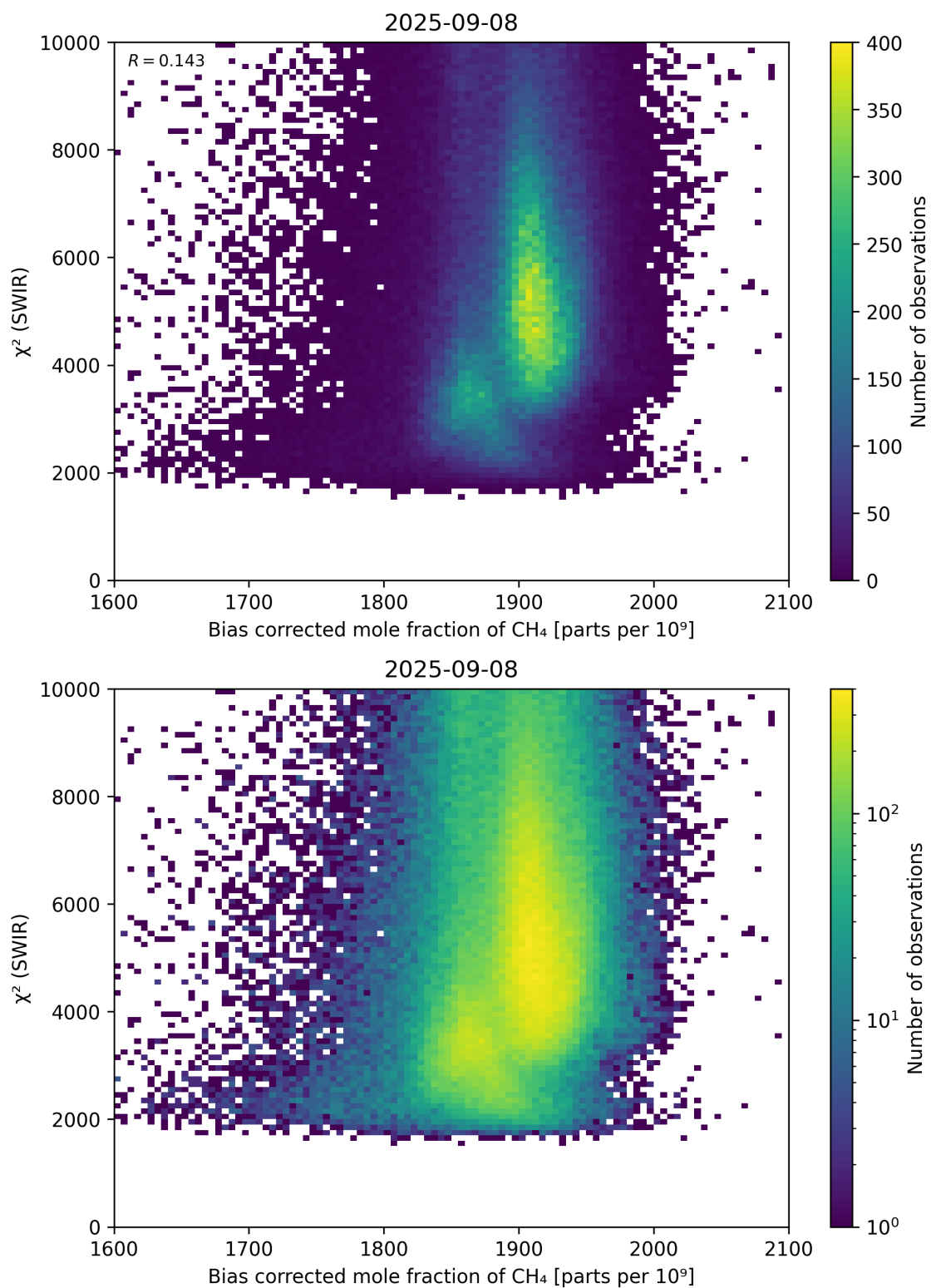
Figure 64: Scatter density plot of “Bias corrected mole fraction of \text{CH}_4 ” against “ \chi^2 (SWIR)” for 2025-09-07 to 2025-09-09.
