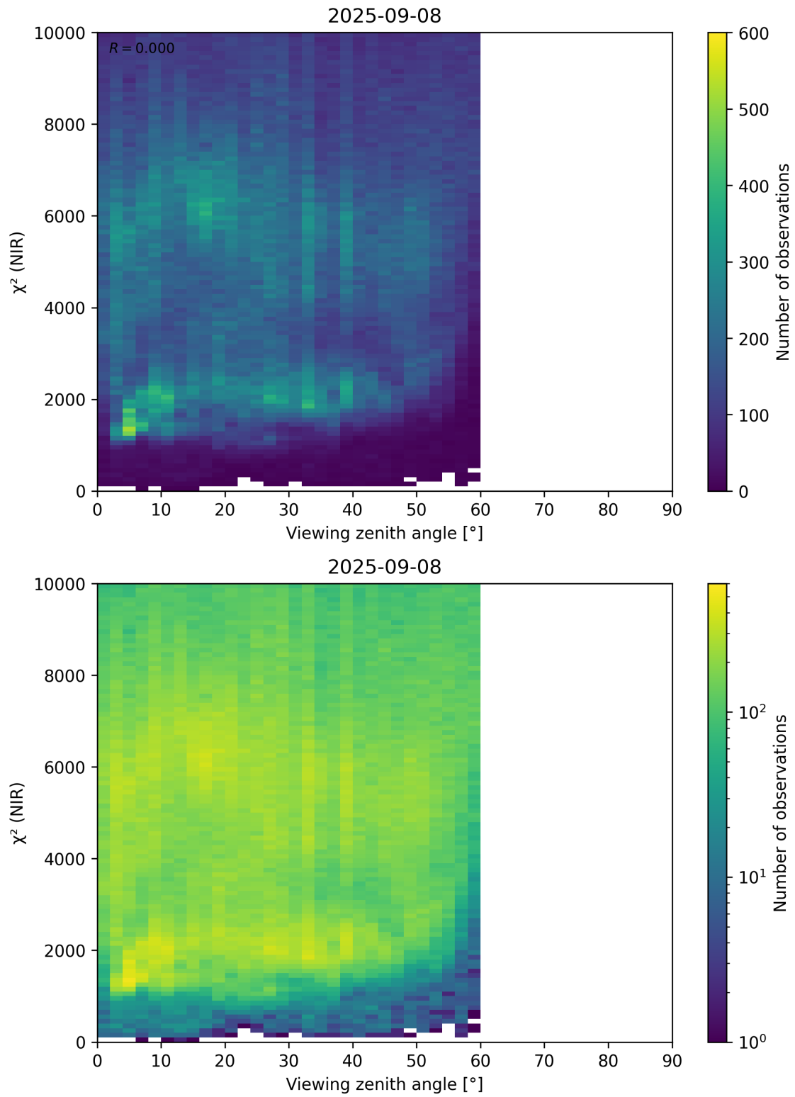
Figure 105: Scatter density plot of “Viewing zenith angle” against “ \chi^2 (NIR)” for 2025-09-07 to 2025-09-09.
