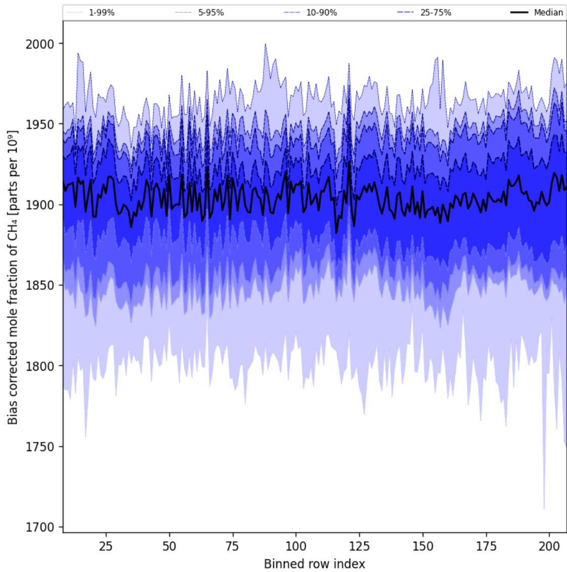
Figure 36: Along track statistics of “Bias corrected mole fraction of CH 4 ” for 2025-09-07 to 2025-09-09
