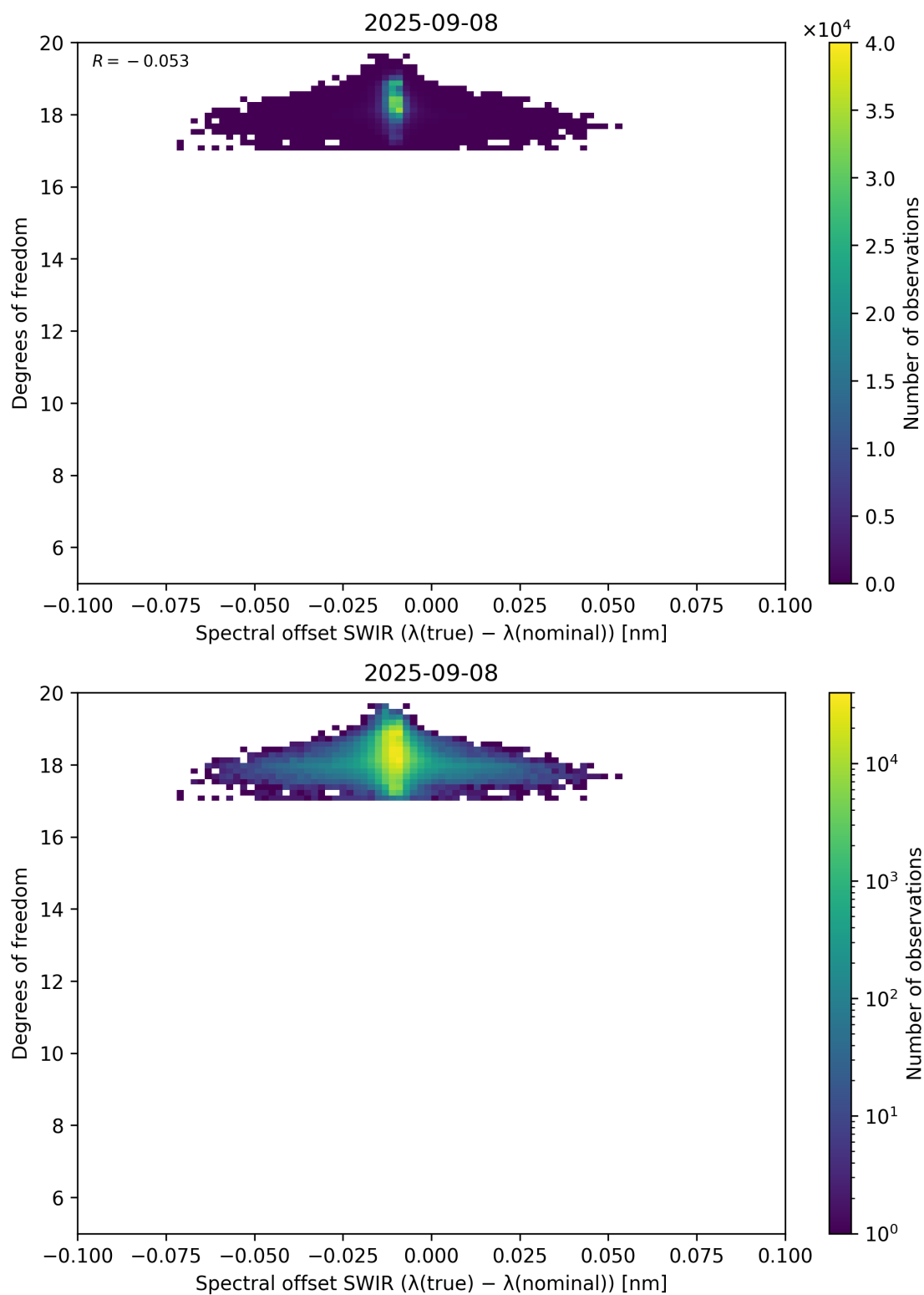
Figure 119: Scatter density plot of “Spectral offset SWIR ( \lambda_{\text{true}} - \lambda_{\text{nominal}} )” against “Degrees of freedom” for 2025-09-07 to 2025-09-09.
