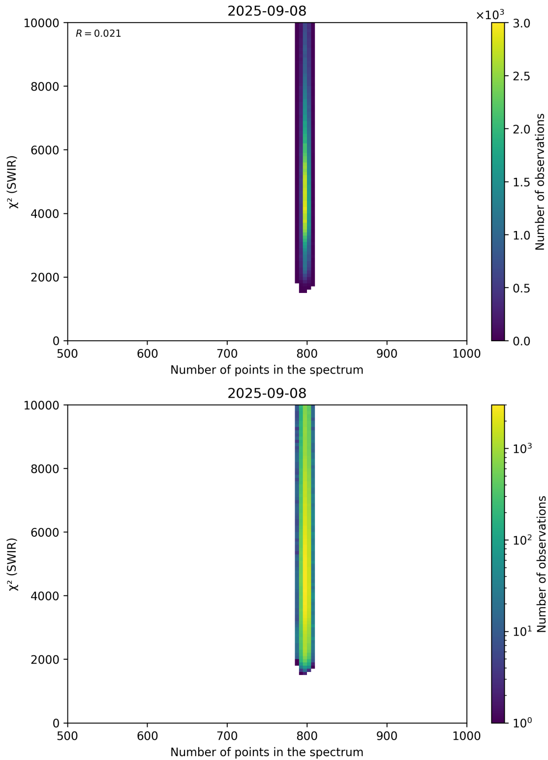
Figure 89: Scatter density plot of “Number of points in the spectrum” against “ \chi^2 (SWIR)” for 2025-09-07 to 2025-09-09.
