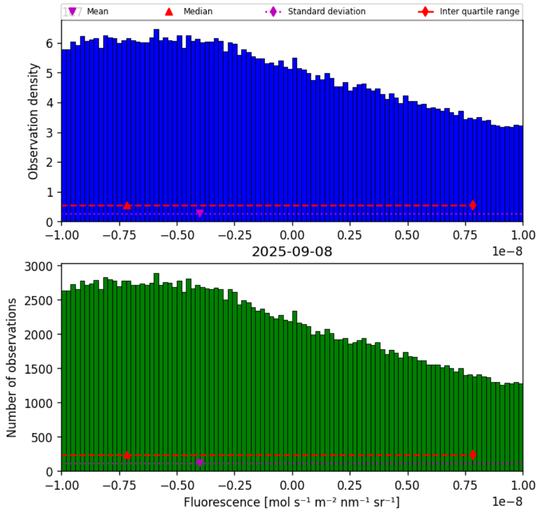
Figure 32: Histogram of “Fluorescence” for 2025-09-07 to 2025-09-09
