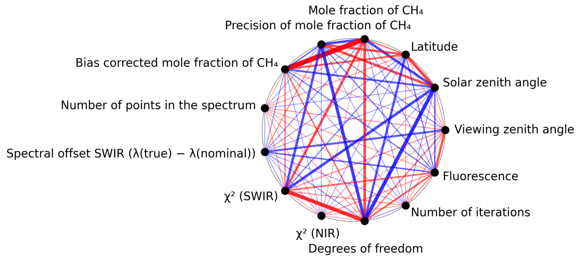
Figure 1: Map of correlation graph for 2025-09-07 to 2025-09-09.
