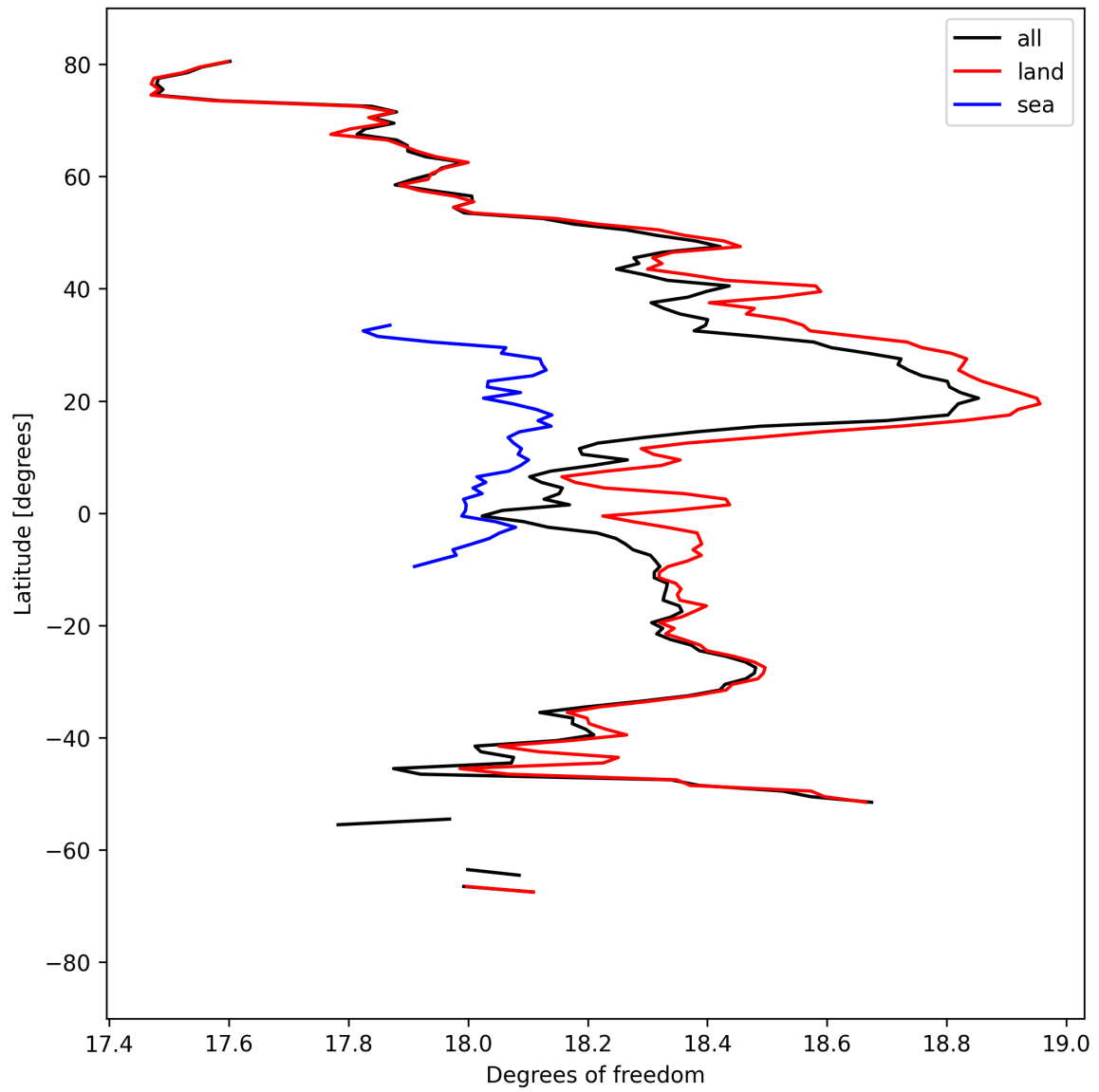
Figure 19: Zonal average of “Degrees of freedom” for 2025-09-07 to 2025-09-09.
