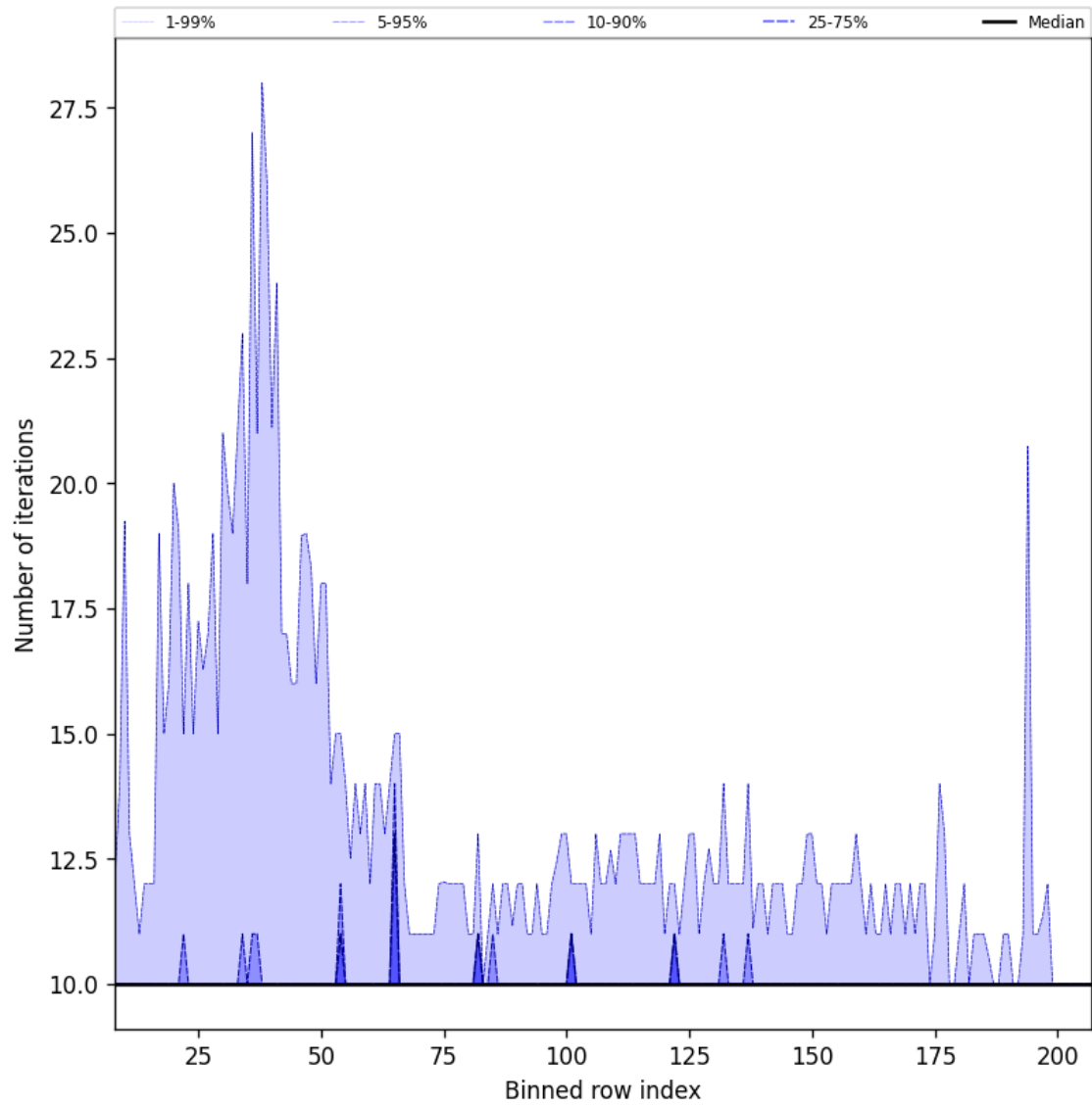
Figure 42: Along track statistics of “Number of iterations” for 2025-09-07 to 2025-09-09
