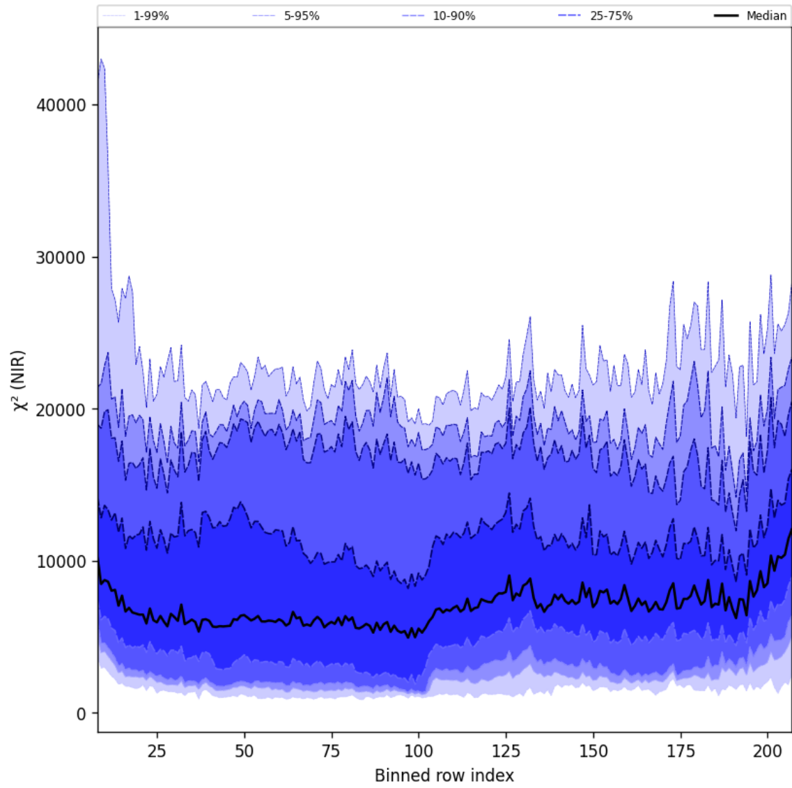
Figure 40: Along track statistics of “ \chi^2 (NIR)” for 2025-09-07 to 2025-09-09
