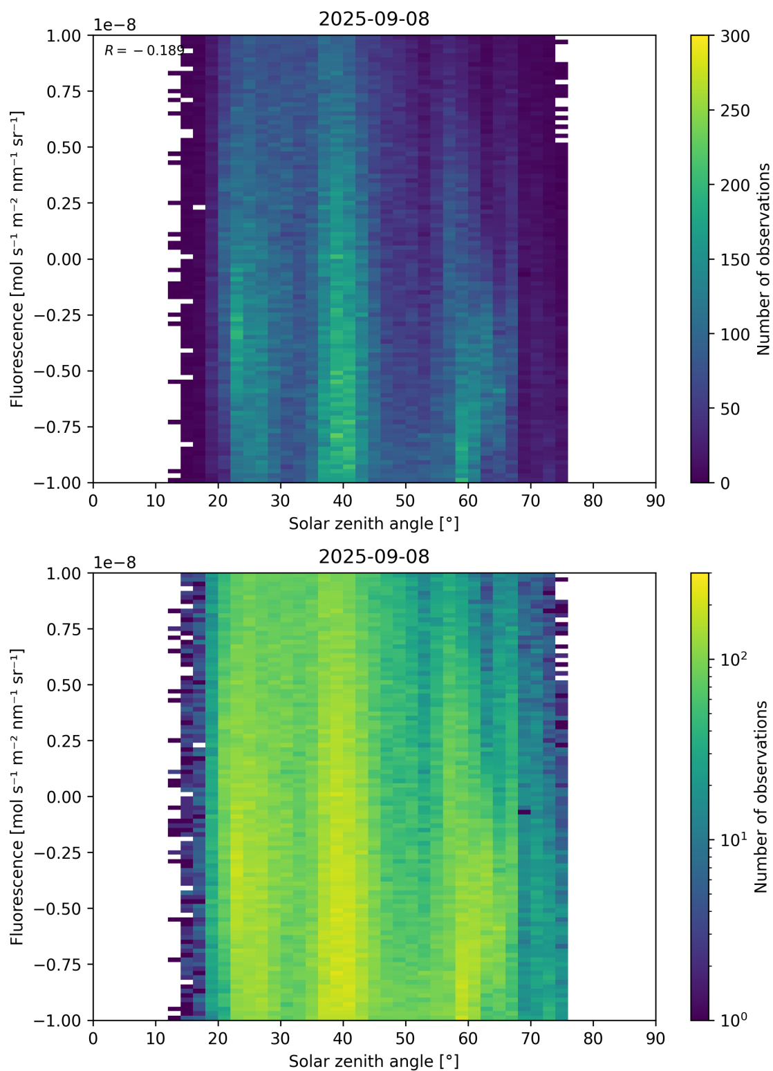
Figure 97: Scatter density plot of “Solar zenith angle” against “Fluorescence” for 2025-09-07 to 2025-09-09.
