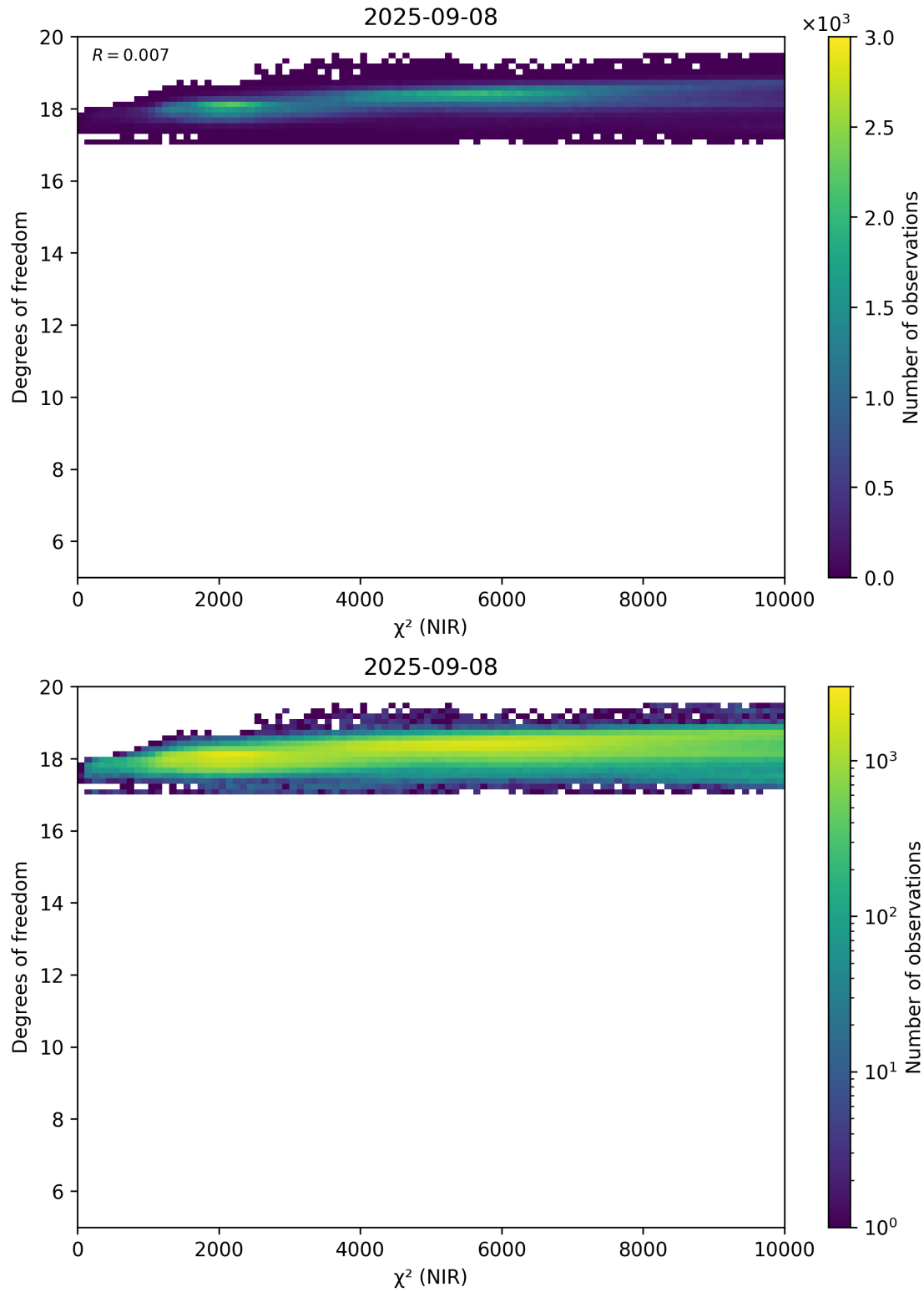
Figure 44: Scatter density plot of “ \chi^2 (NIR)” against “Degrees of freedom” for 2025-09-07 to 2025-09-09.
