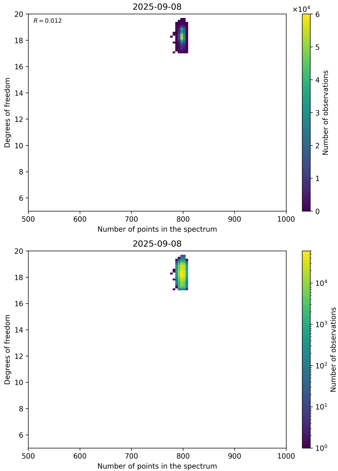
Figure 90: Scatter density plot of “Number of points in the spectrum” against “Degrees of freedom” for 2025-09-07 to 2025-09-09.
