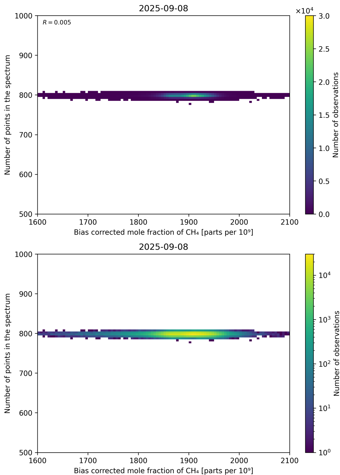
Figure 68: Scatter density plot of “Bias corrected mole fraction of CH 4 ” against “Number of points in the spectrum” for 2025-09-07 to 2025-09-09.
