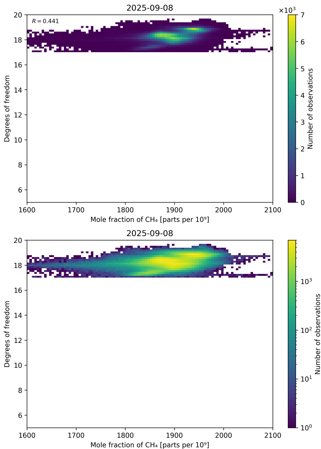
Figure 72: Scatter density plot of “Mole fraction of CH 4 ” against “Degrees of freedom” for 2025-09-07 to 2025-09-09.
