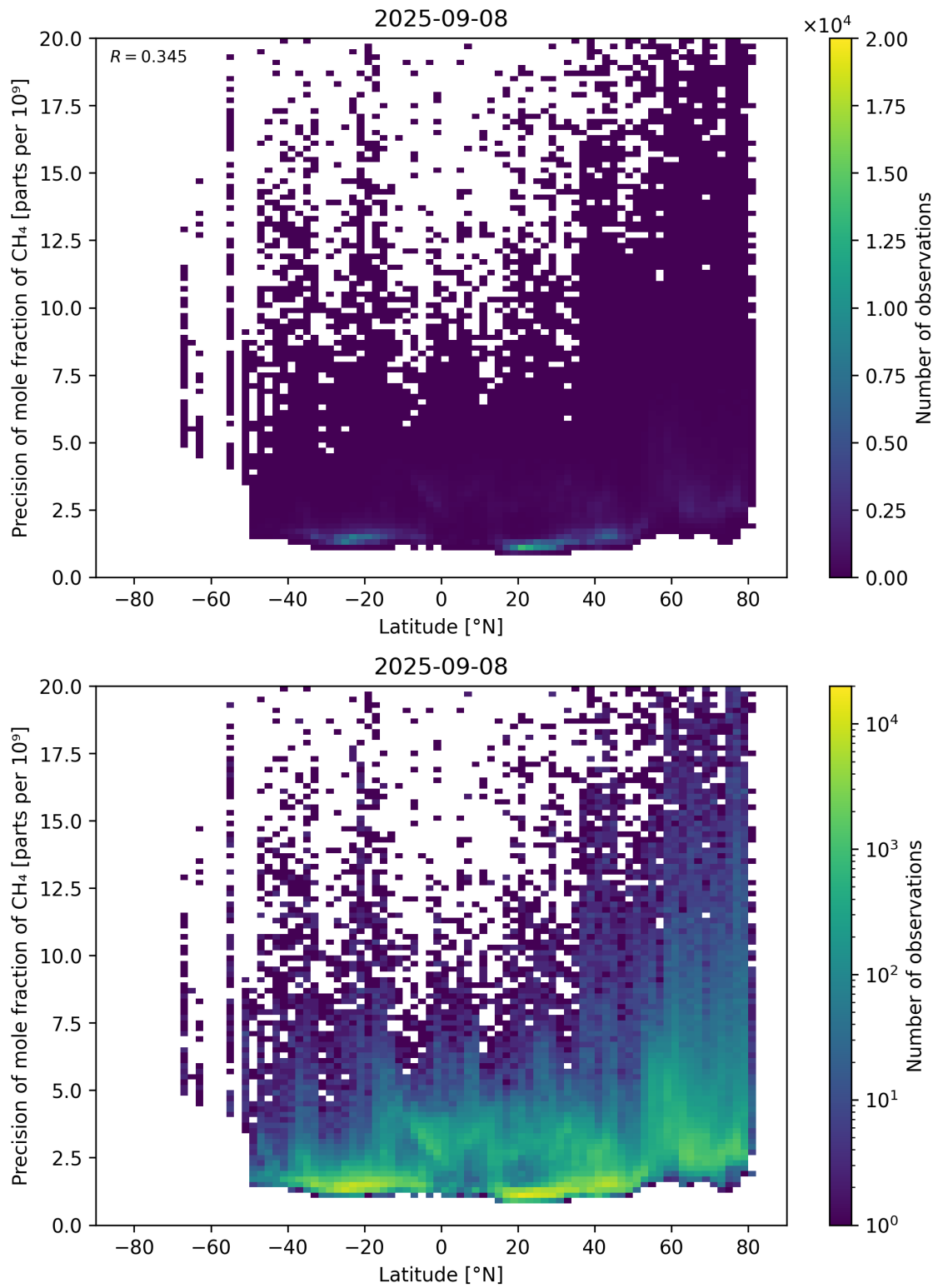
Figure 59: Scatter density plot of “Latitude” against “Precision of mole fraction of \text{CH}_4 ” for 2025-09-07 to 2025-09-09.
