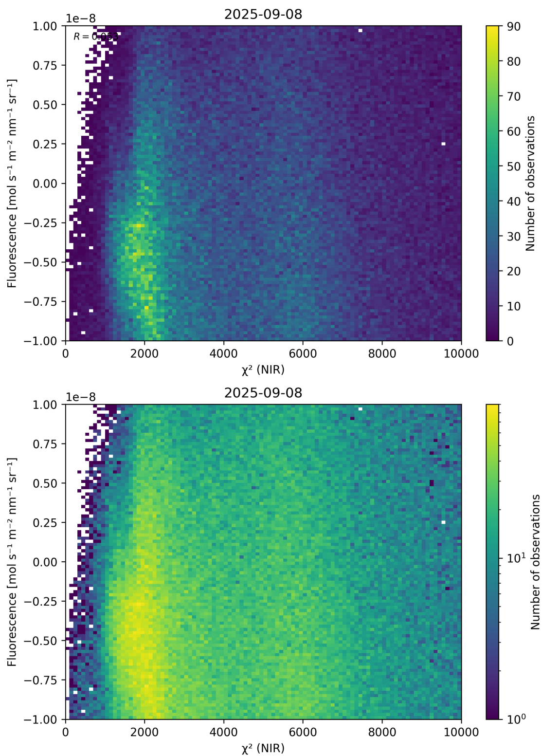
Figure 45: Scatter density plot of “ \chi^2 (NIR)” against “Fluorescence” for 2025-09-07 to 2025-09-09.
