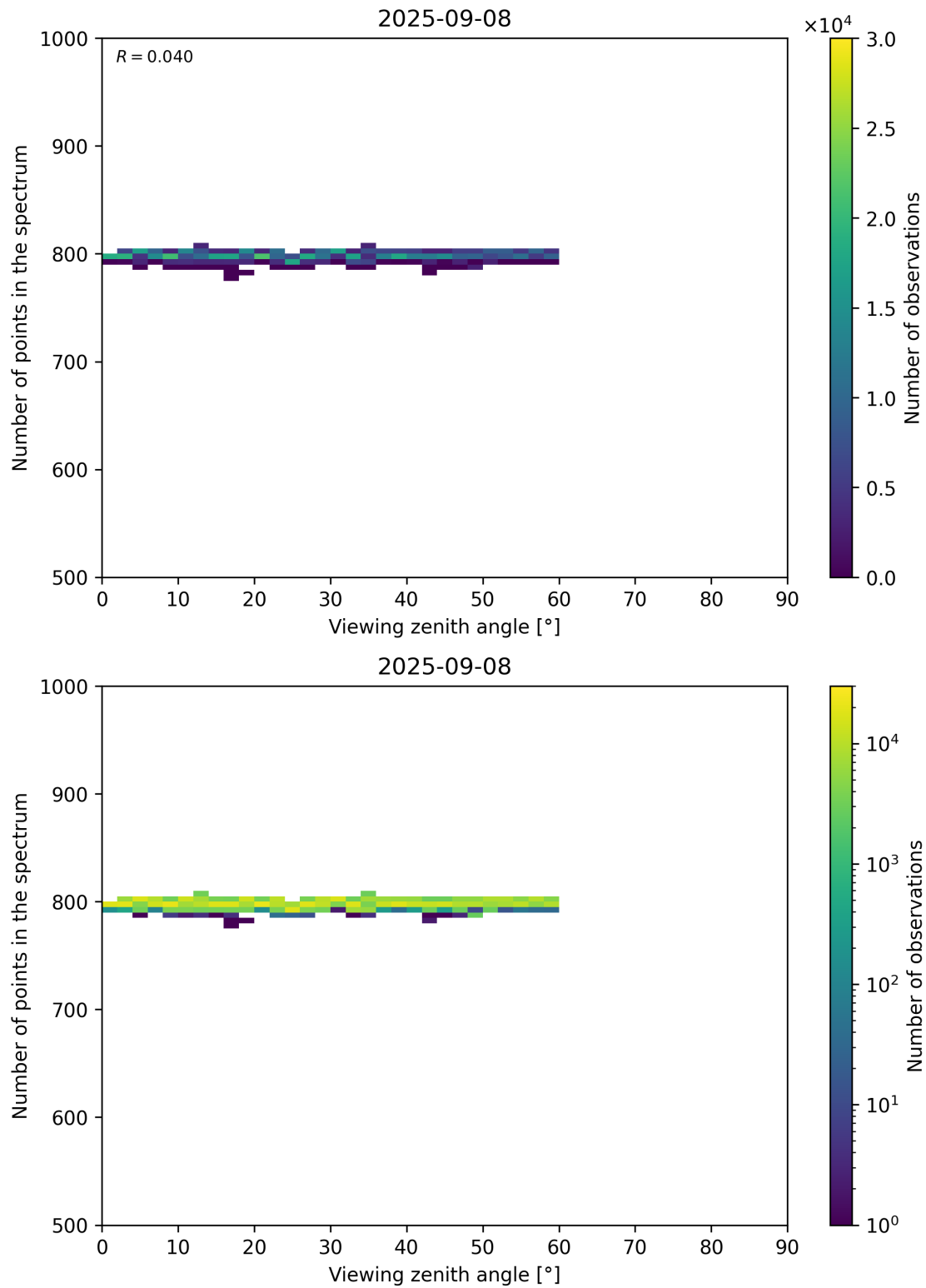
Figure 114: Scatter density plot of “Viewing zenith angle” against “Number of points in the spectrum” for 2025-09-07 to 2025-09-09.
