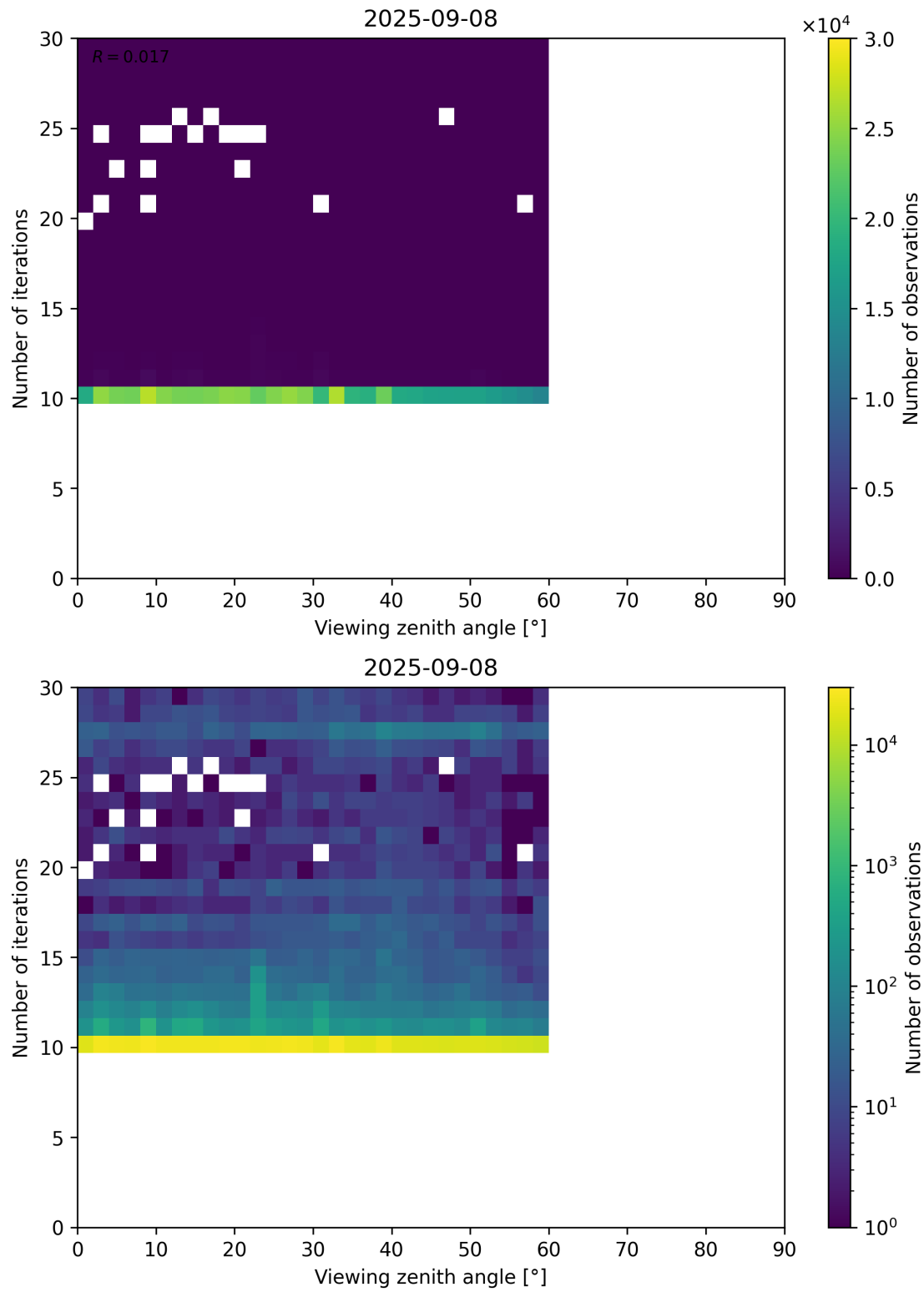
Figure 113: Scatter density plot of “Viewing zenith angle” against “Number of iterations” for 2025-09-07 to 2025-09-09.
