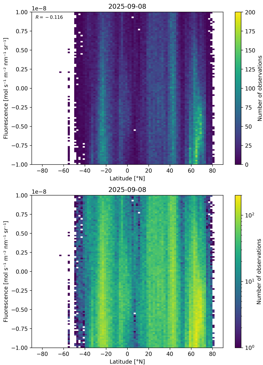
Figure 56: Scatter density plot of “Latitude” against “Fluorescence” for 2025-09-07 to 2025-09-09.
