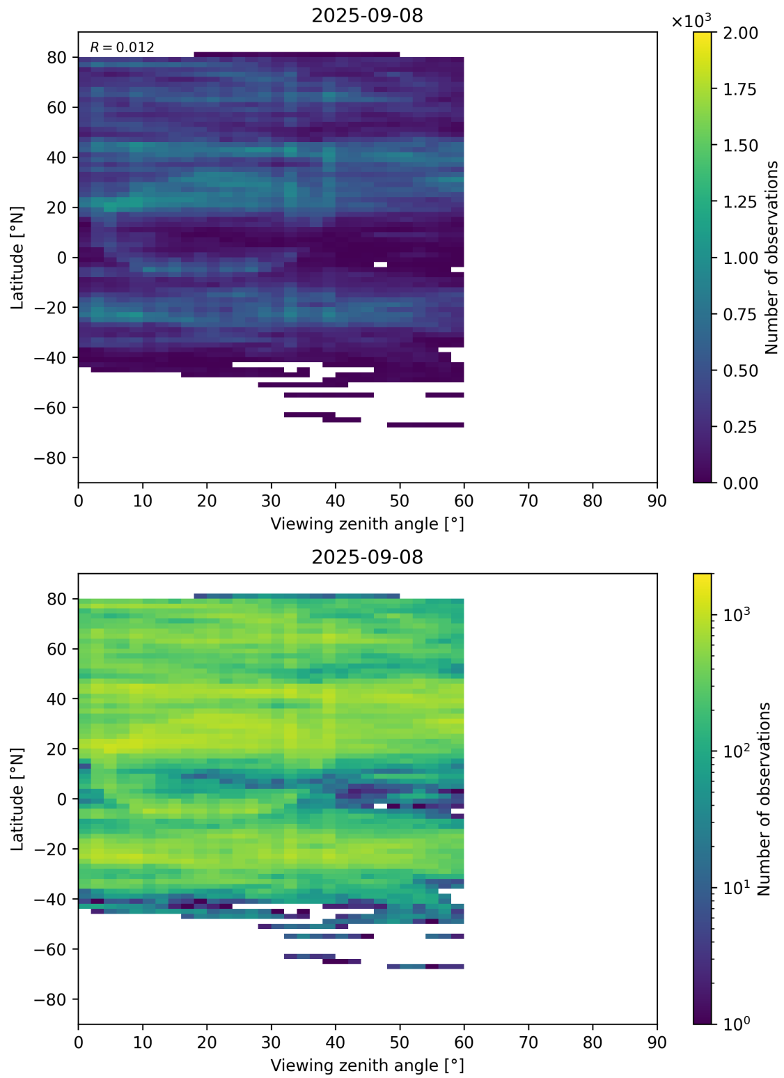
Figure 109: Scatter density plot of “Viewing zenith angle” against “Latitude” for 2025-09-07 to 2025-09-09.
