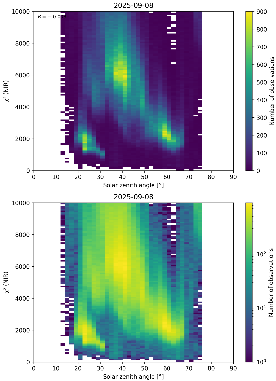
Figure 94: Scatter density plot of “Solar zenith angle” against “ \chi^2 (NIR)” for 2025-09-07 to 2025-09-09.
