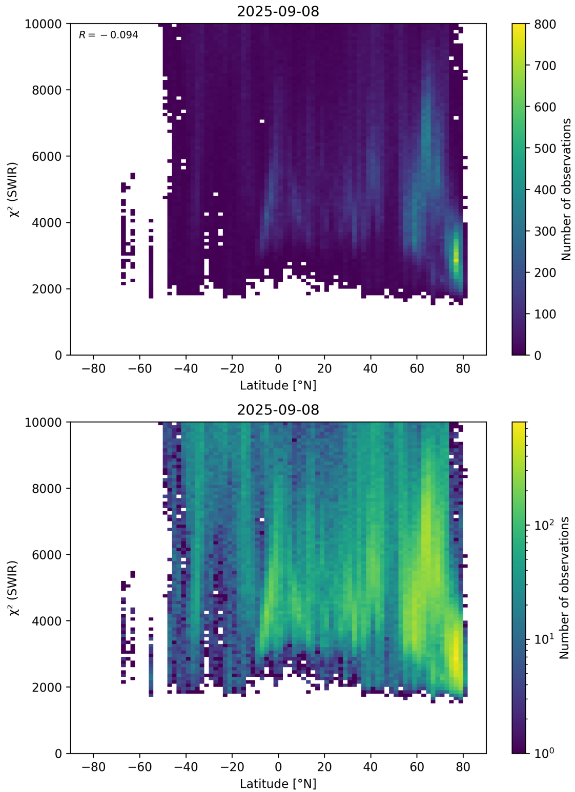
Figure 54: Scatter density plot of “Latitude” against “ \chi^2 (SWIR)” for 2025-09-07 to 2025-09-09.
