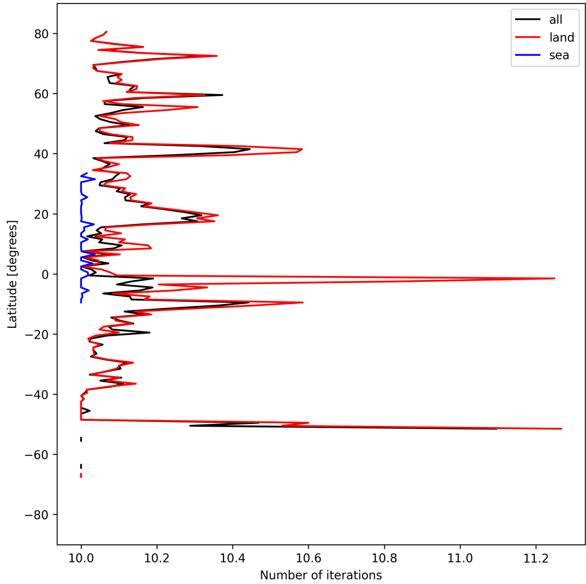
Figure 20: Zonal average of “Number of iterations” for 2025-09-07 to 2025-09-09.
