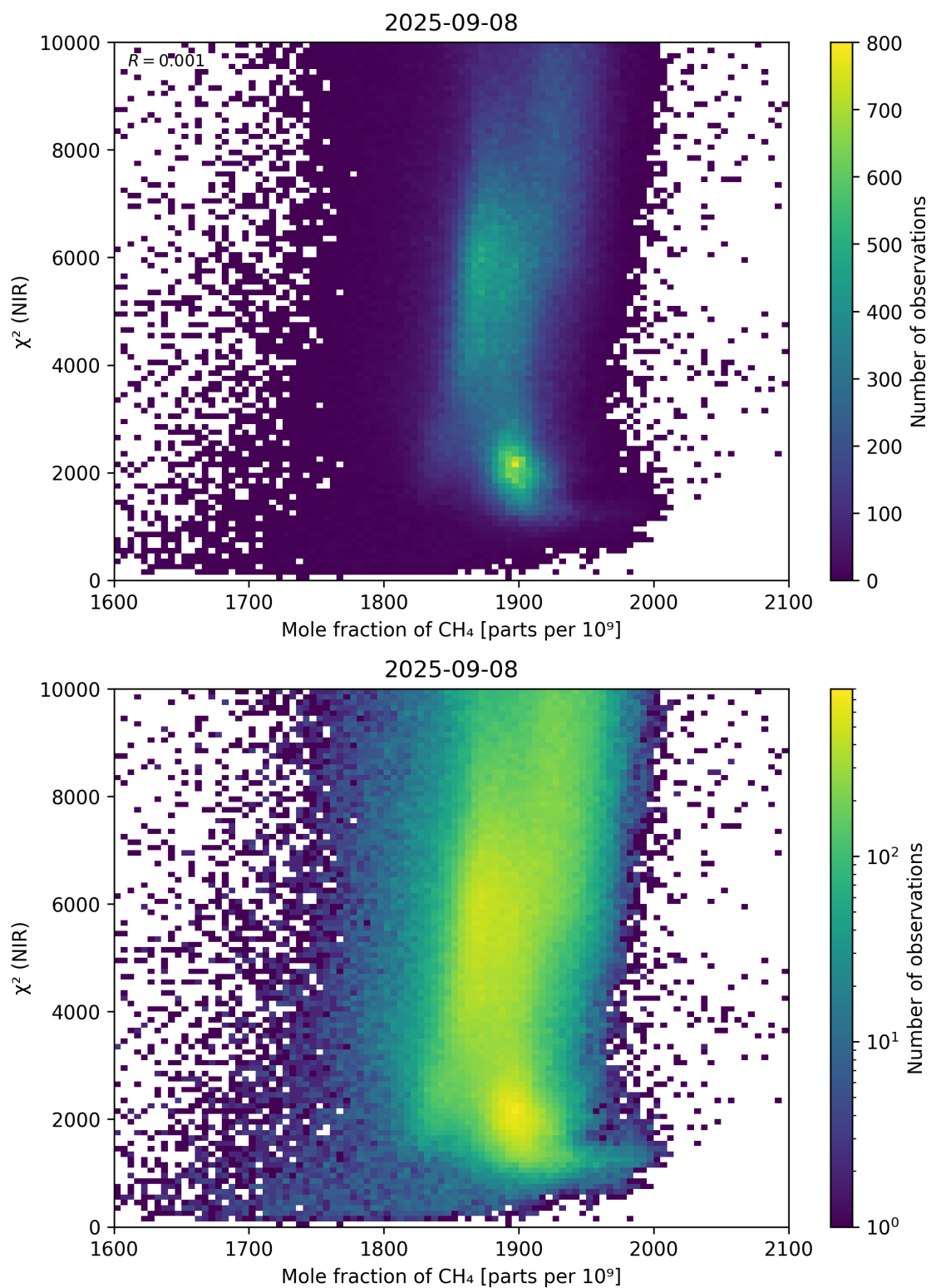
Figure 70: Scatter density plot of “Mole fraction of CH 4 ” against “ \chi^2 (NIR)” for 2025-09-07 to 2025-09-09.
