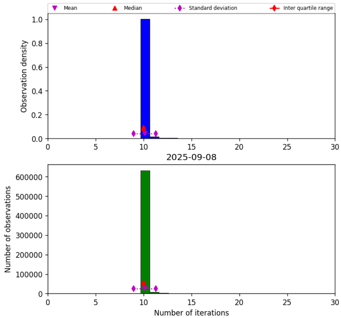
Figure 31: Histogram of “Number of iterations” for 2025-09-07 to 2025-09-09
