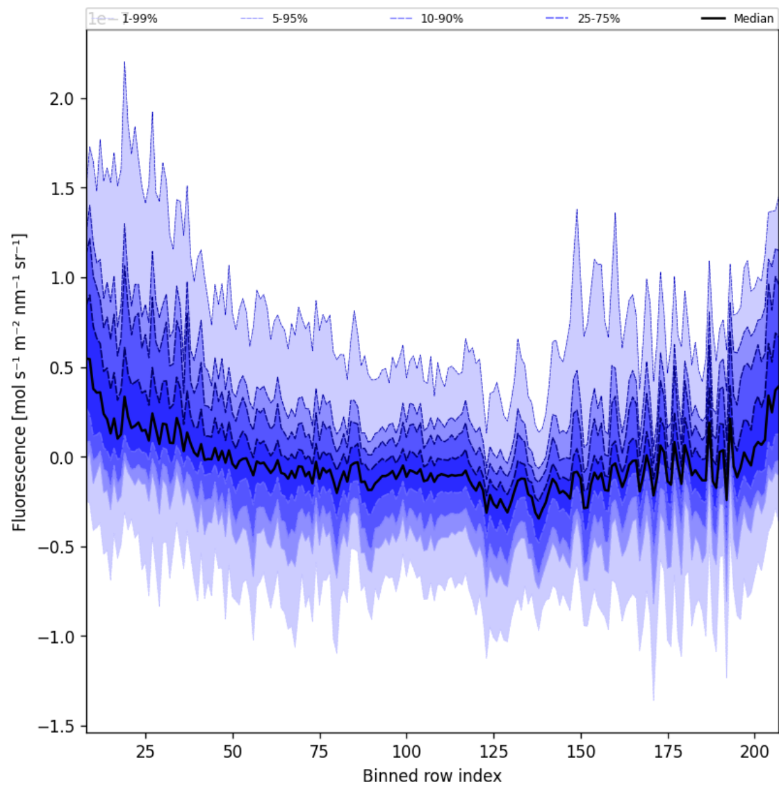
Figure 43: Along track statistics of “Fluorescence” for 2025-09-07 to 2025-09-09
