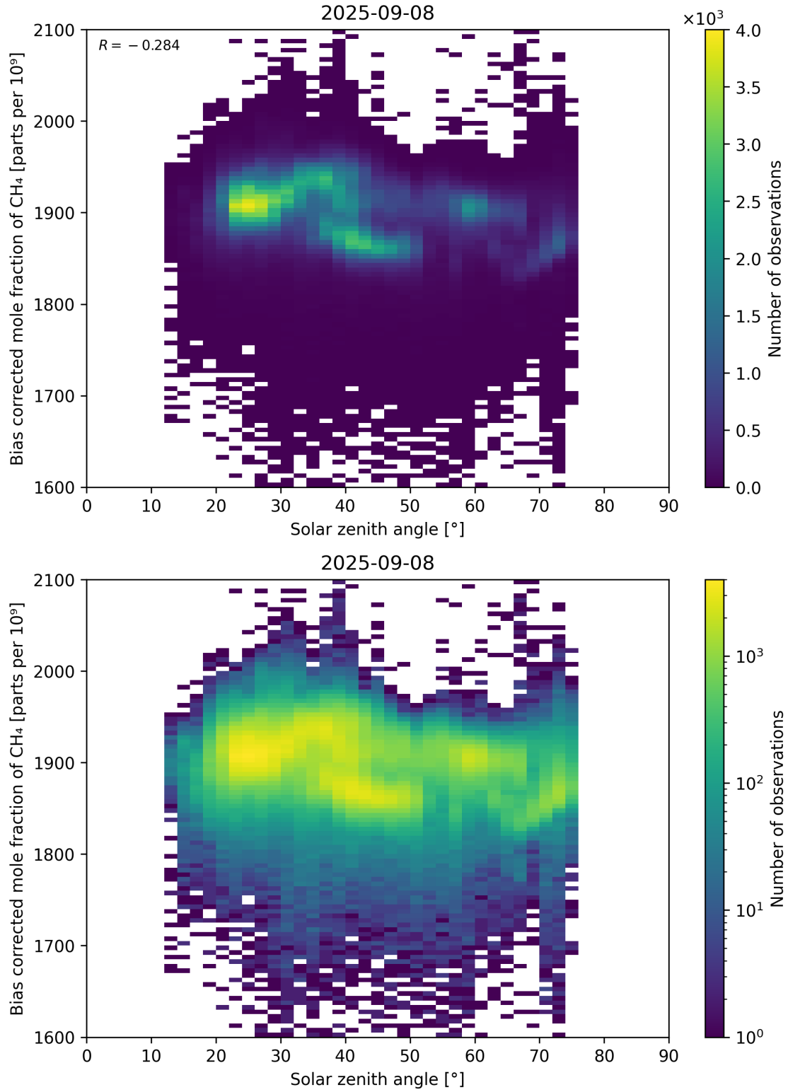
Figure 100: Scatter density plot of “Solar zenith angle” against “Bias corrected mole fraction of CH 4 ” for 2025-09-07 to 2025-09-09.
