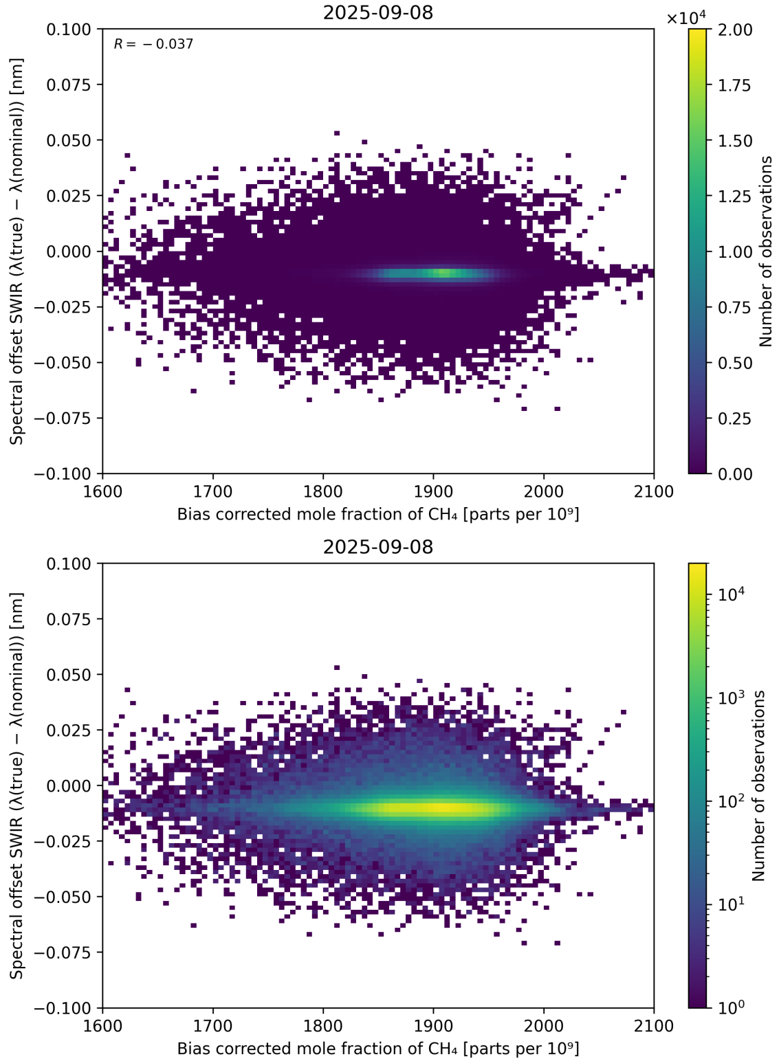
Figure 69: Scatter density plot of “Bias corrected mole fraction of \text{CH}_4 ” against “Spectral offset SWIR ( \lambda_{\text{true}} - \lambda_{\text{nominal}} )” for 2025-09-07 to 2025-09-09.
