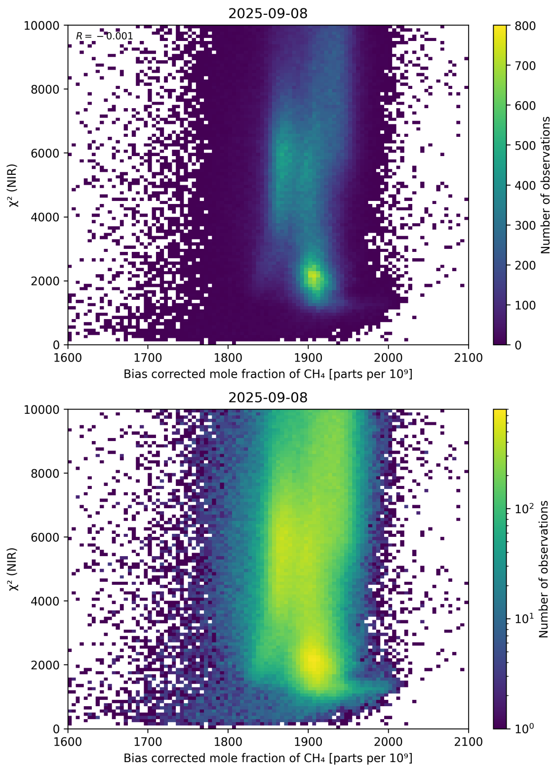
Figure 63: Scatter density plot of “Bias corrected mole fraction of CH 4 ” against “ \chi^2 (NIR)” for 2025-09-07 to 2025-09-09.
