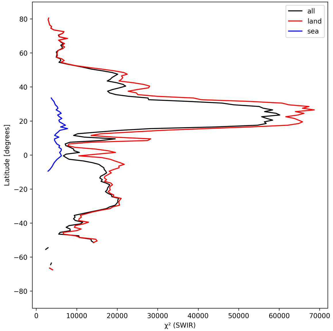
Figure 17: Zonal average of “ \chi^2 (SWIR)” for 2025-09-07 to 2025-09-09.
