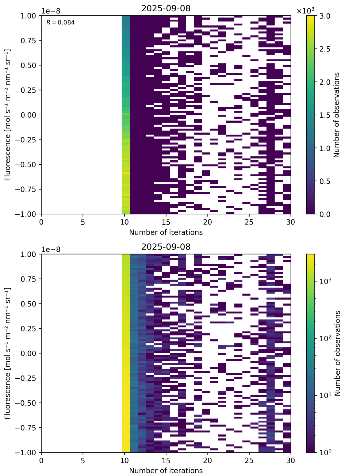
Figure 87: Scatter density plot of “Number of iterations” against “Fluorescence” for 2025-09-07 to 2025-09-09.
