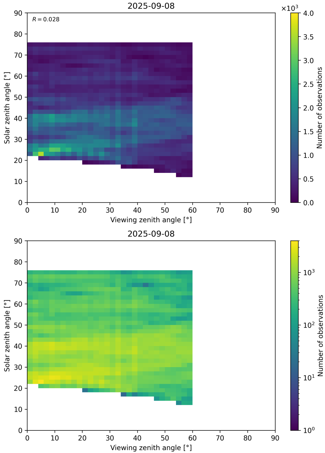
Figure 115: Scatter density plot of “Viewing zenith angle” against “Solar zenith angle” for 2025-09-07 to 2025-09-09.
