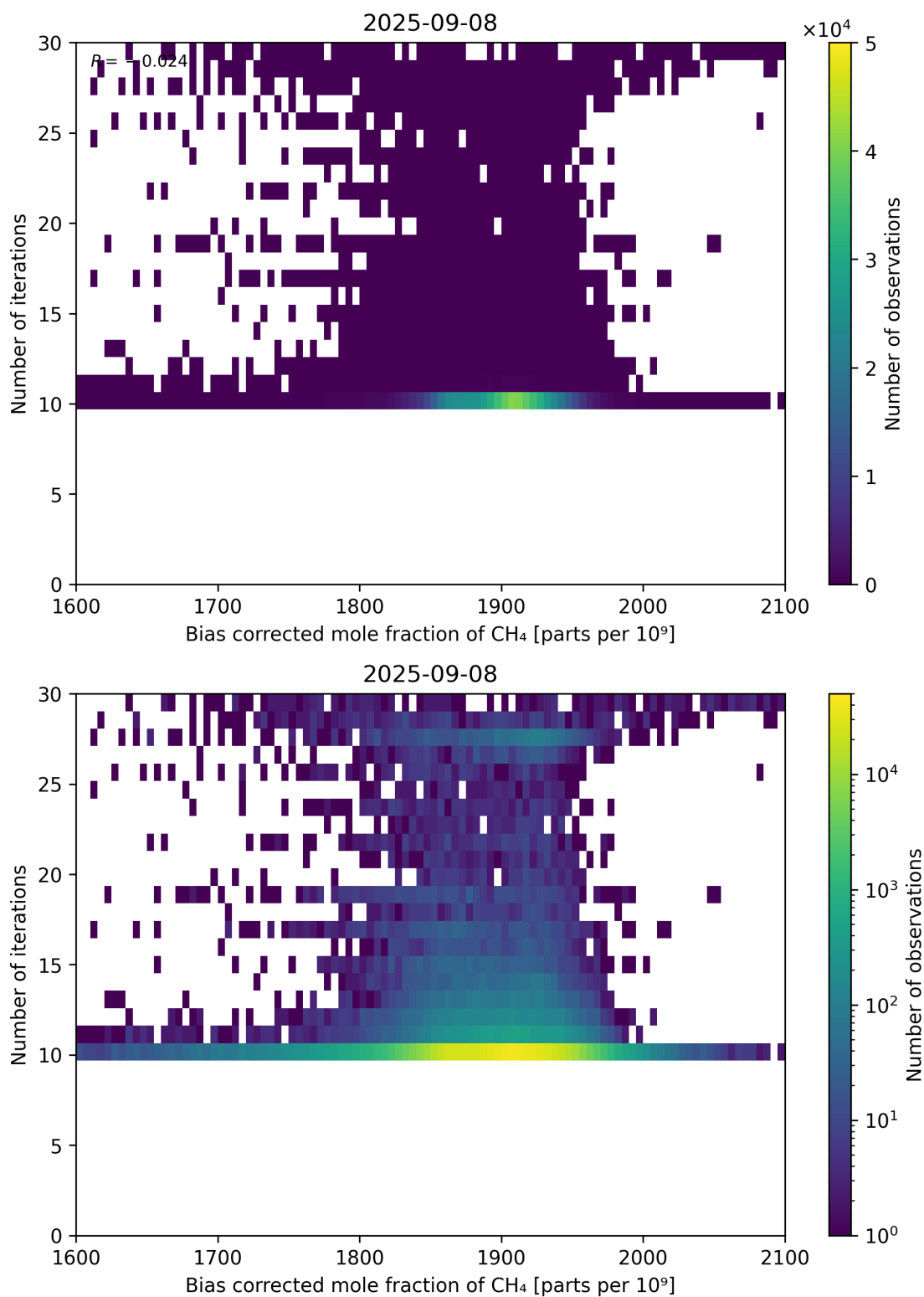
Figure 67: Scatter density plot of “Bias corrected mole fraction of CH 4 ” against “Number of iterations” for 2025-09-07 to 2025-09-09.
