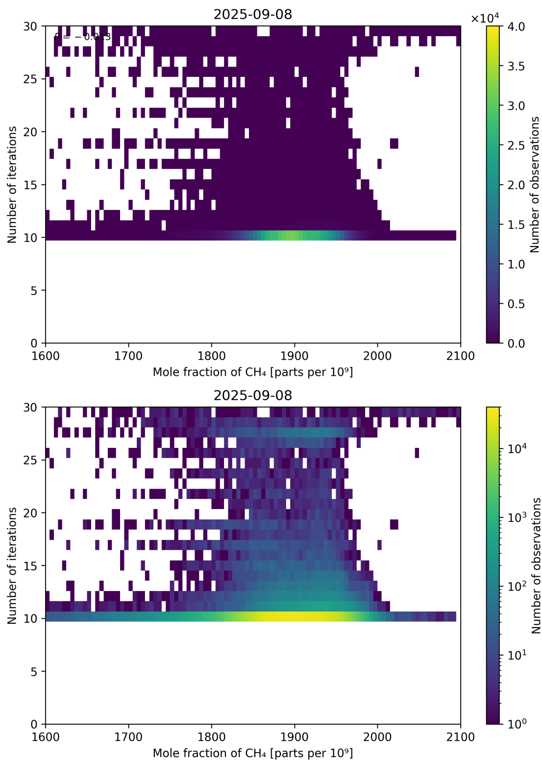
Figure 76: Scatter density plot of “Mole fraction of CH 4 ” against “Number of iterations” for 2025-09-07 to 2025-09-09.
