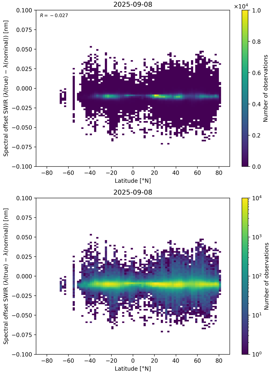
Figure 62: Scatter density plot of “Latitude” against “Spectral offset SWIR ( \lambda_{\text{true}} - \lambda_{\text{nominal}} )” for 2025-09-07 to 2025-09-09.
