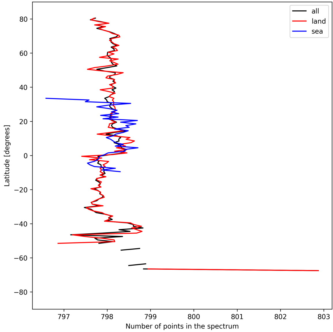
Figure 15: Zonal average of “Number of points in the spectrum” for 2025-09-07 to 2025-09-09.
