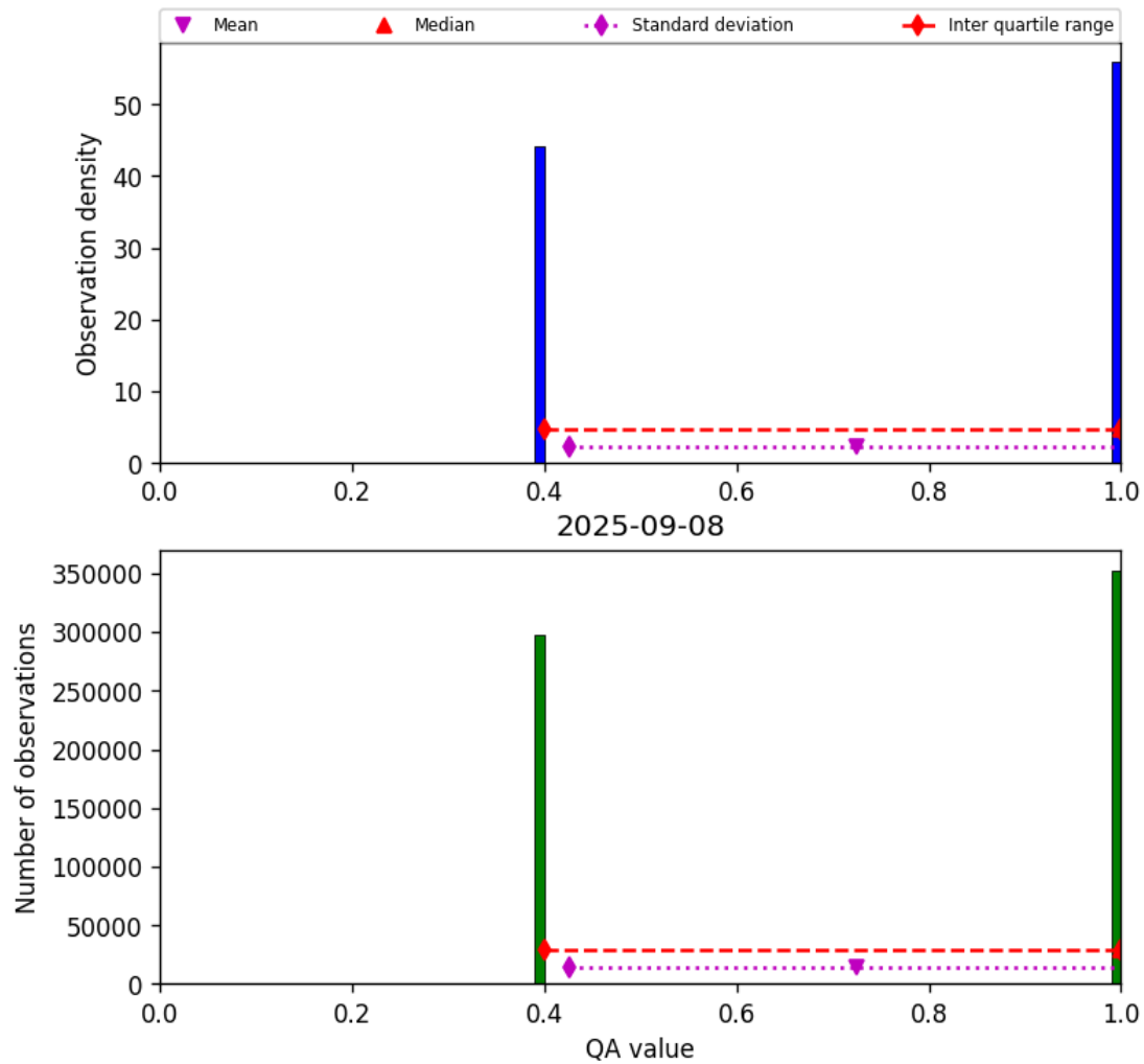
Figure 22: Histogram of “QA value” for 2025-09-07 to 2025-09-09
