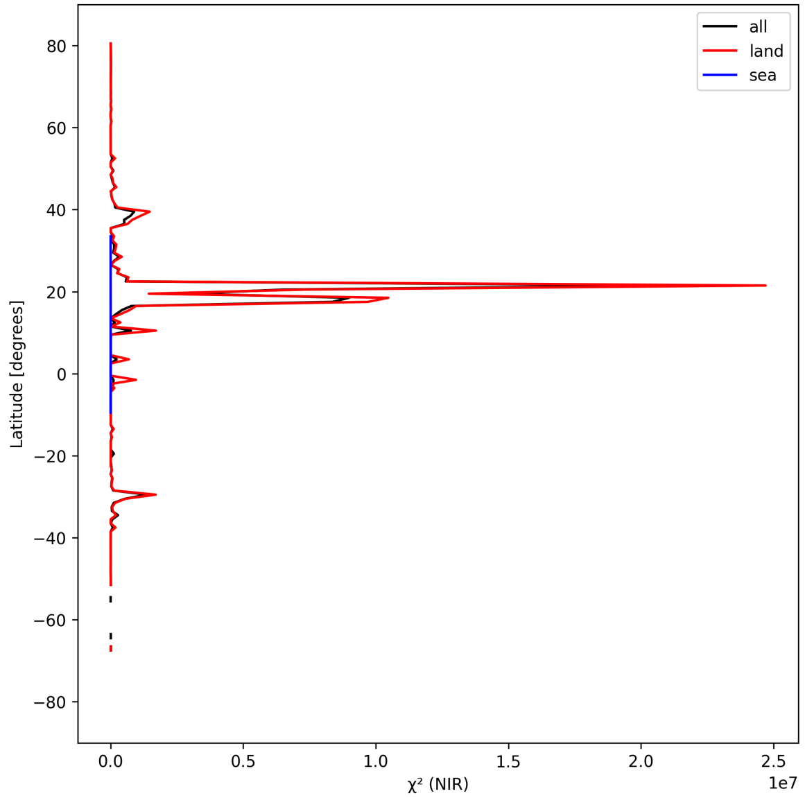
Figure 18: Zonal average of “ \chi^2 (NIR)” for 2025-09-07 to 2025-09-09.
