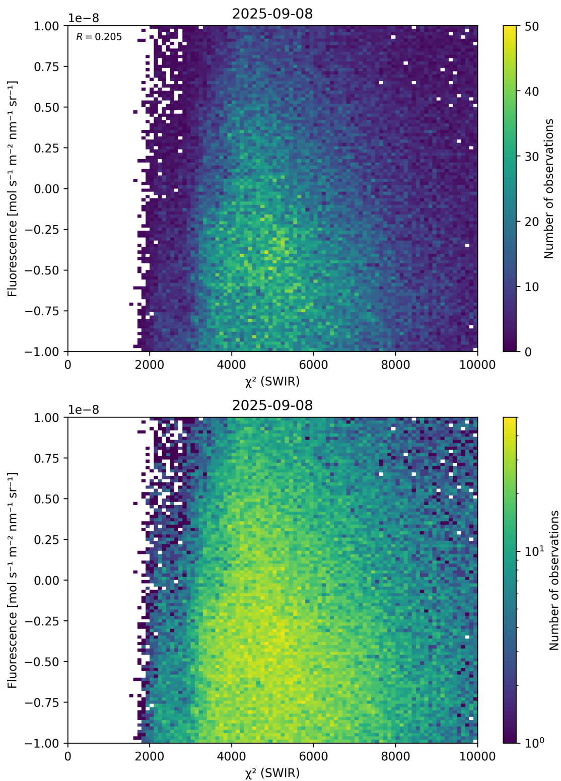
Figure 49: Scatter density plot of “ \chi^2 (SWIR)” against “Fluorescence” for 2025-09-07 to 2025-09-09.
