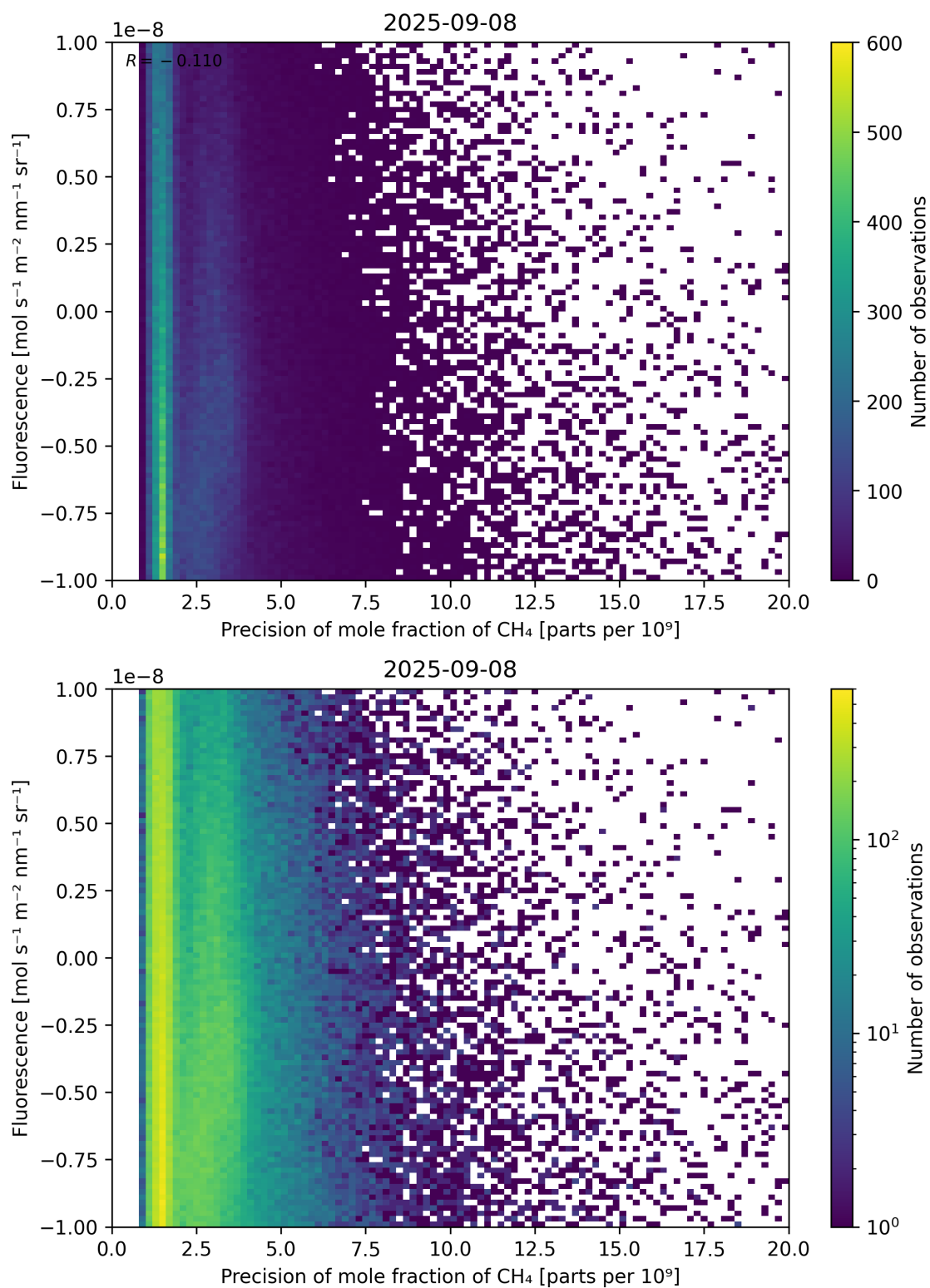
Figure 81: Scatter density plot of “Precision of mole fraction of \text{CH}_4 ” against “Fluorescence” for 2025-09-07 to 2025-09-09.
