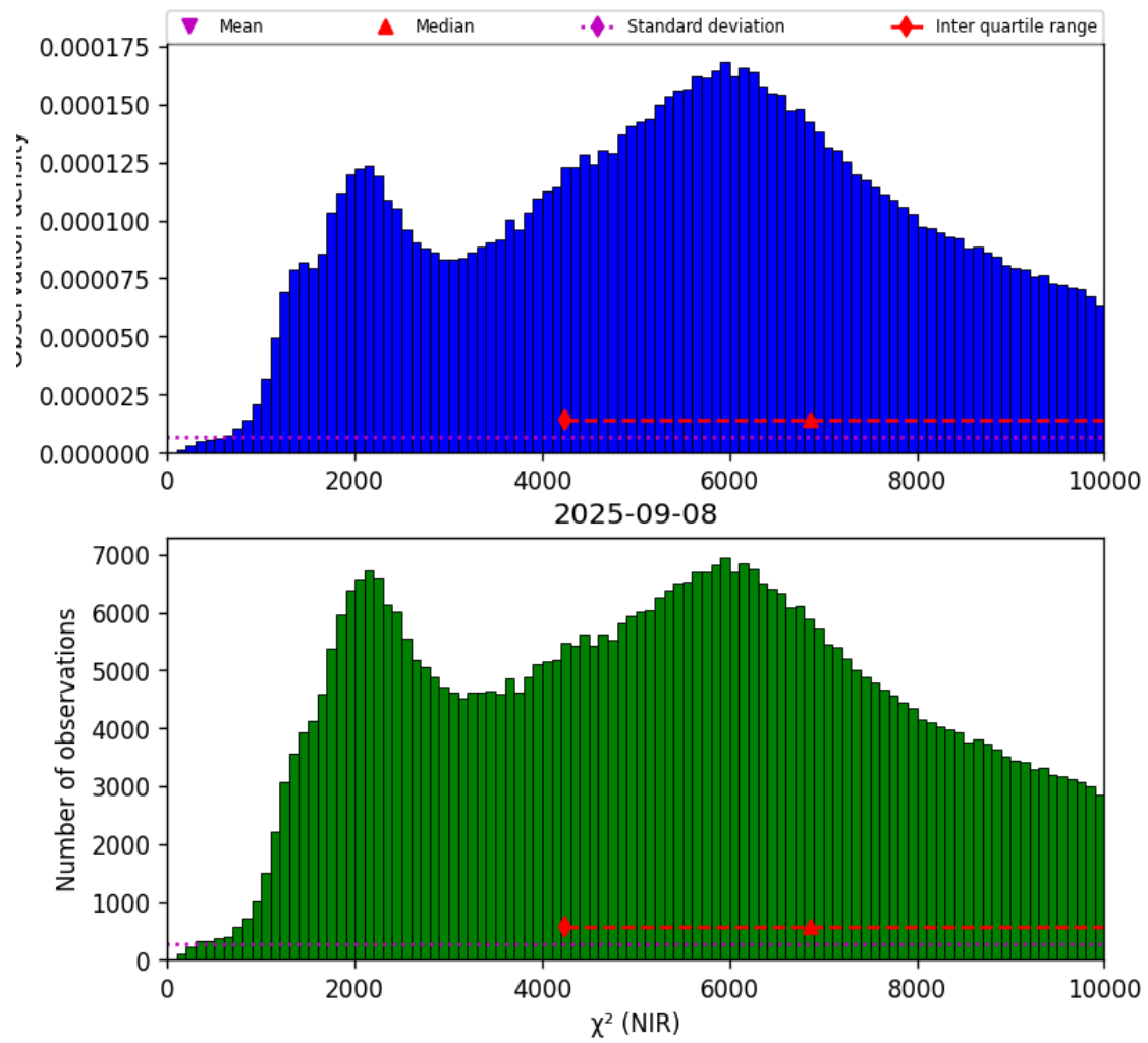
Figure 29: Histogram of “ \chi^2 (NIR)” for 2025-09-07 to 2025-09-09
