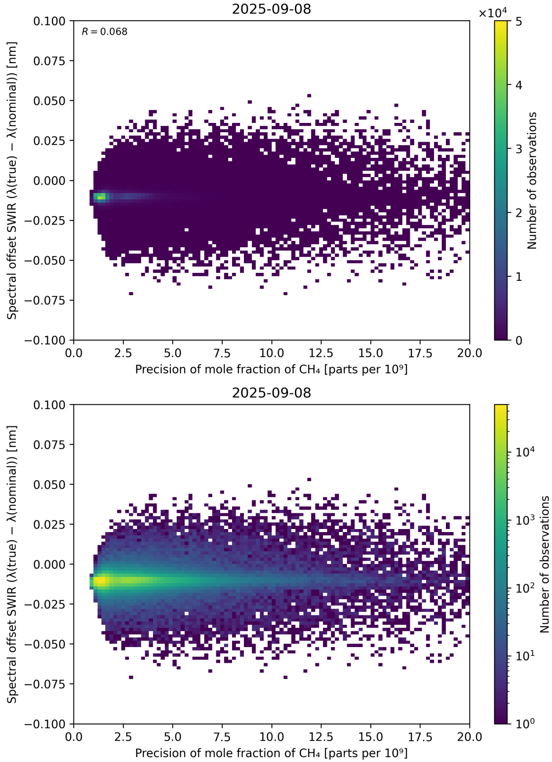
Figure 85: Scatter density plot of “Precision of mole fraction of \text{CH}_4 ” against “Spectral offset SWIR ( \lambda_{\text{true}} - \lambda_{\text{nominal}} )” for 2025-09-07 to 2025-09-09.
