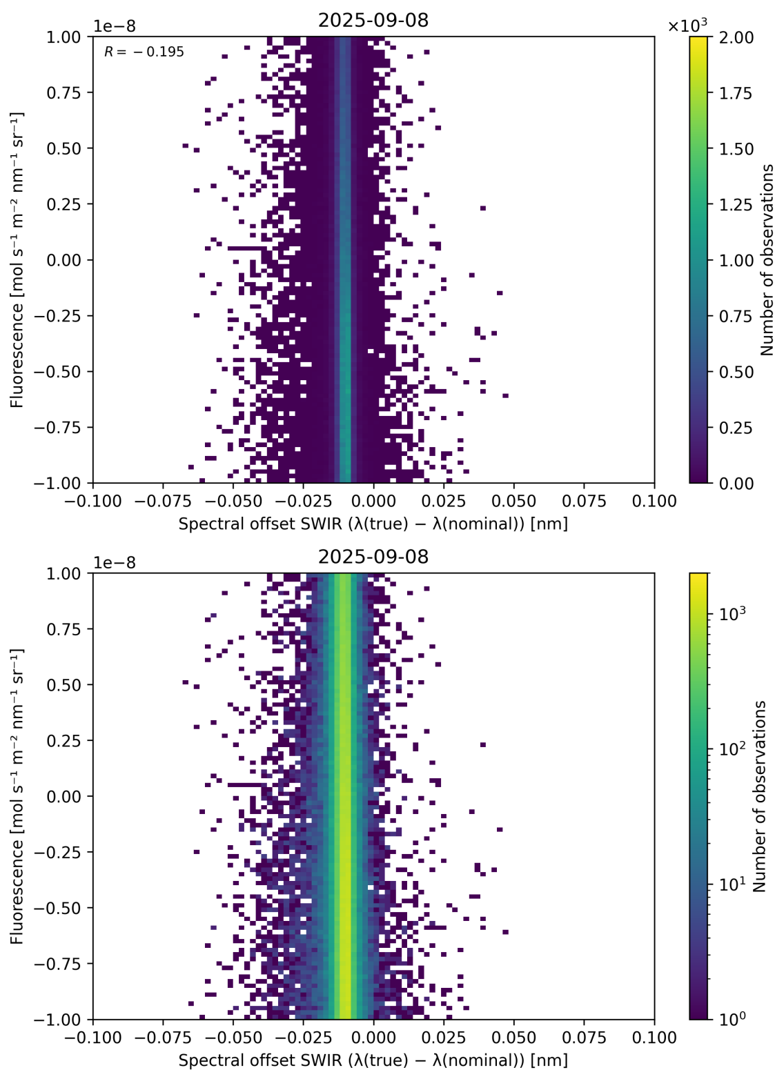
Figure 120: Scatter density plot of “Spectral offset SWIR ( \lambda_{\text{true}} - \lambda_{\text{nominal}} )” against “Fluorescence” for 2025-09-07 to 2025-09-09.
