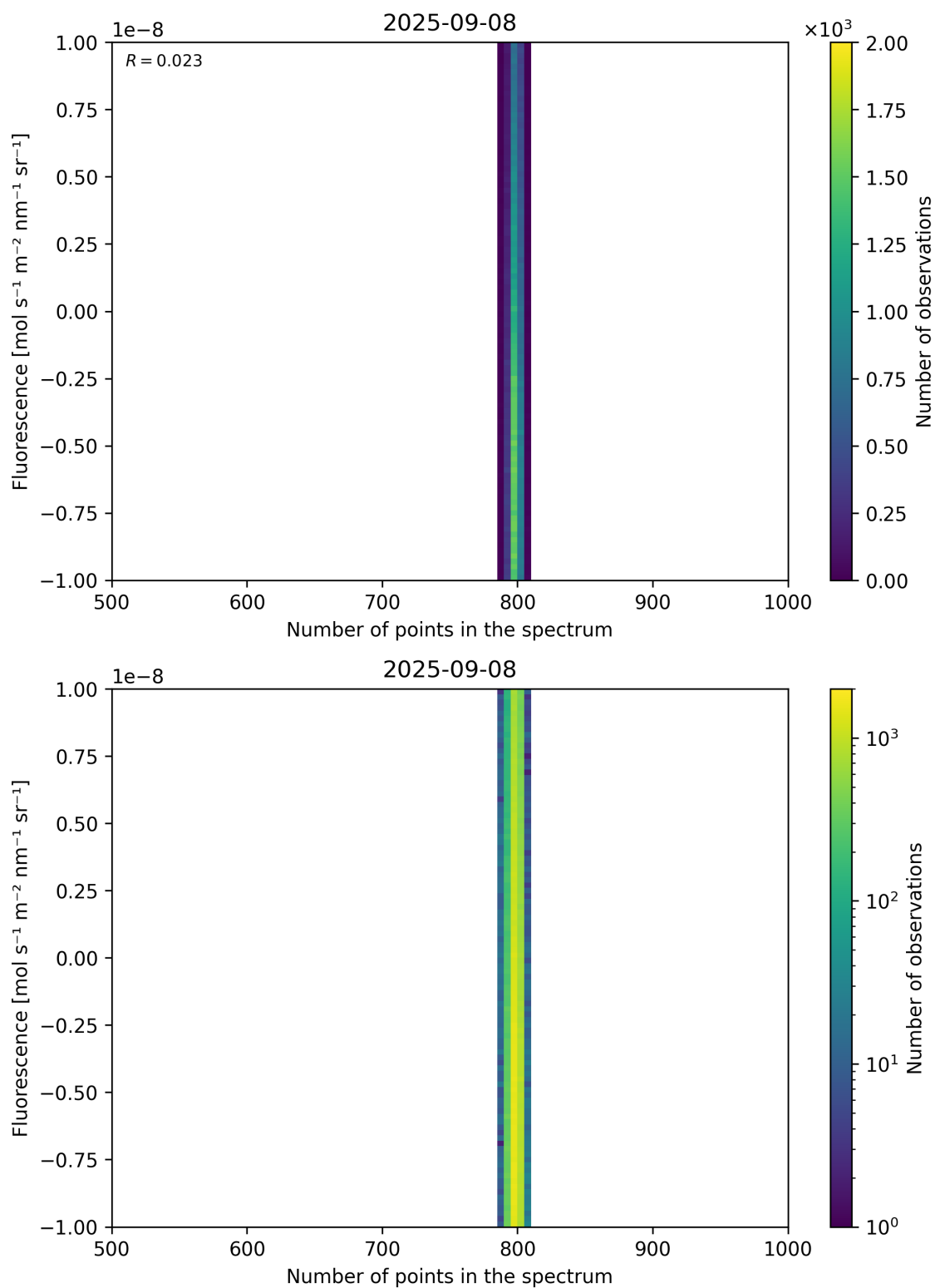
Figure 91: Scatter density plot of “Number of points in the spectrum” against “Fluorescence” for 2025-09-07 to 2025-09-09.
