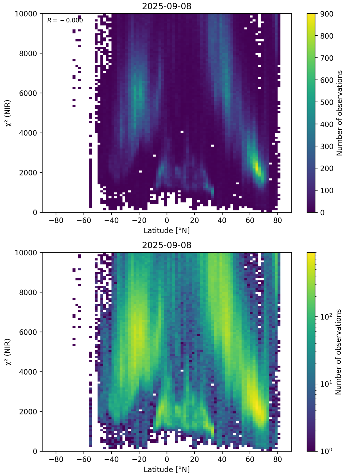
Figure 53: Scatter density plot of “Latitude” against “ \chi^2 (NIR)” for 2025-09-07 to 2025-09-09.
