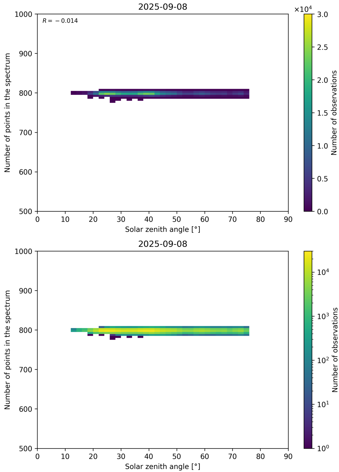
Figure 103: Scatter density plot of “Solar zenith angle” against “Number of points in the spectrum” for 2025-09-07 to 2025-09-09.
