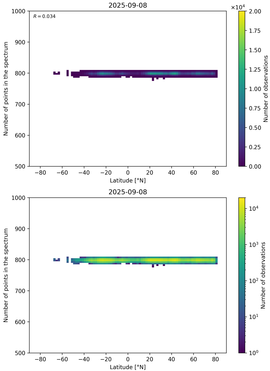
Figure 61: Scatter density plot of “Latitude” against “Number of points in the spectrum” for 2025-09-07 to 2025-09-09.
