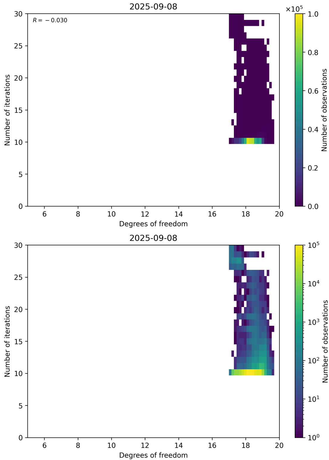
Figure 52: Scatter density plot of “Degrees of freedom” against “Number of iterations” for 2025-09-07 to 2025-09-09.
