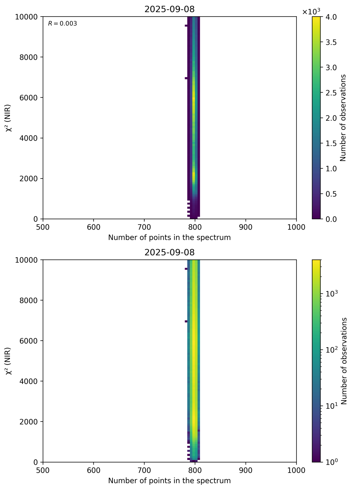
Figure 88: Scatter density plot of “Number of points in the spectrum” against “ \chi^2 (NIR)” for 2025-09-07 to 2025-09-09.
