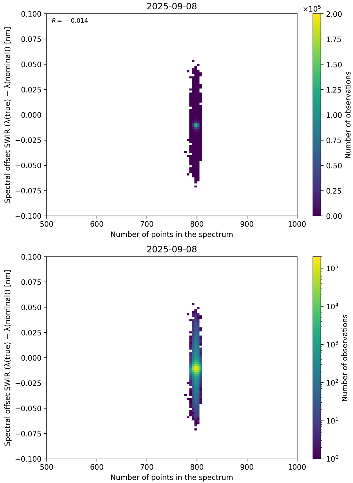
Figure 93: Scatter density plot of “Number of points in the spectrum” against “Spectral offset SWIR ( \lambda_{\text{true}} - \lambda_{\text{nominal}} )” for 2025-09-07 to 2025-09-09.
