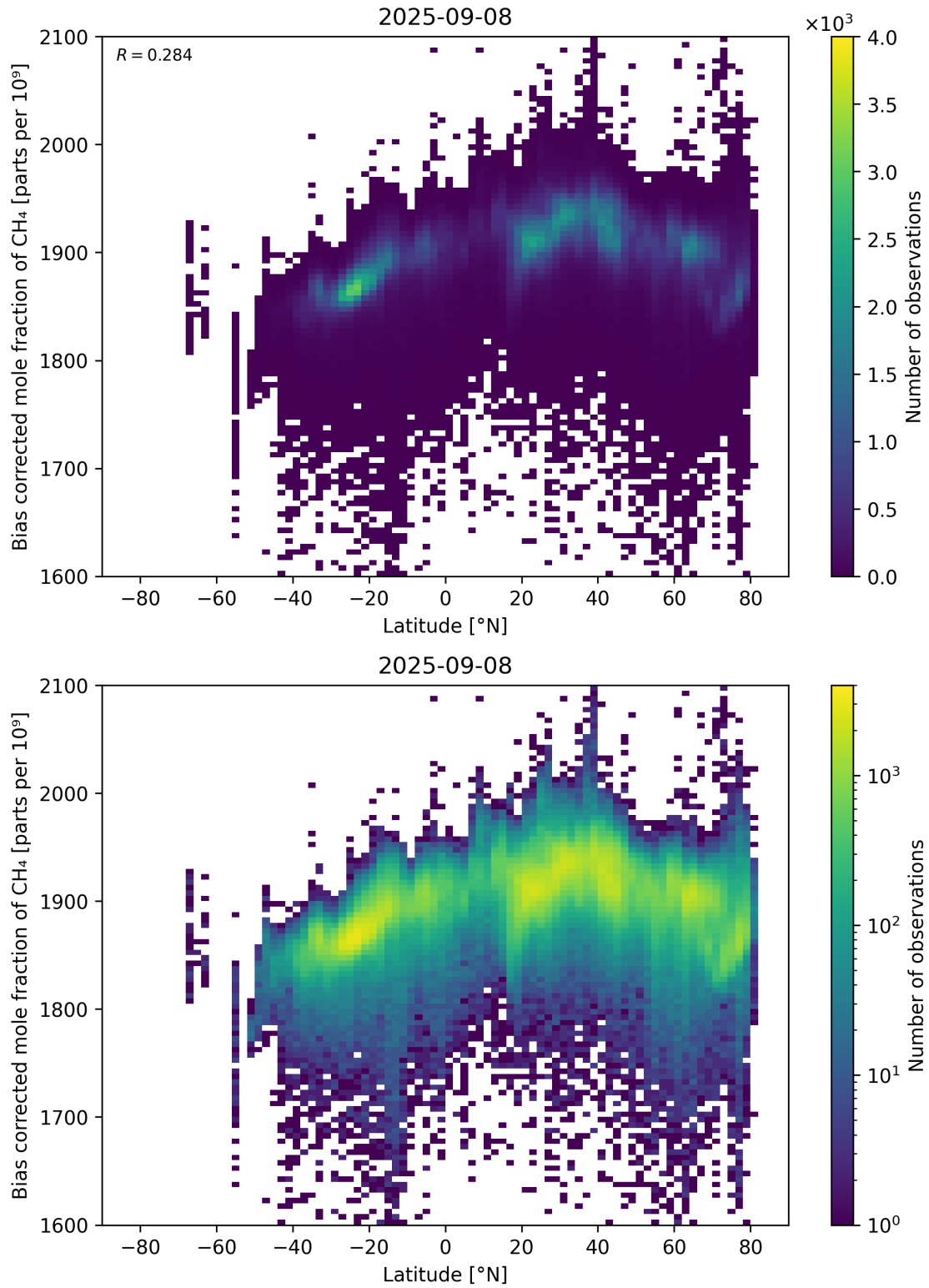
Figure 58: Scatter density plot of “Latitude” against “Bias corrected mole fraction of CH 4 ” for 2025-09-07 to 2025-09-09.
