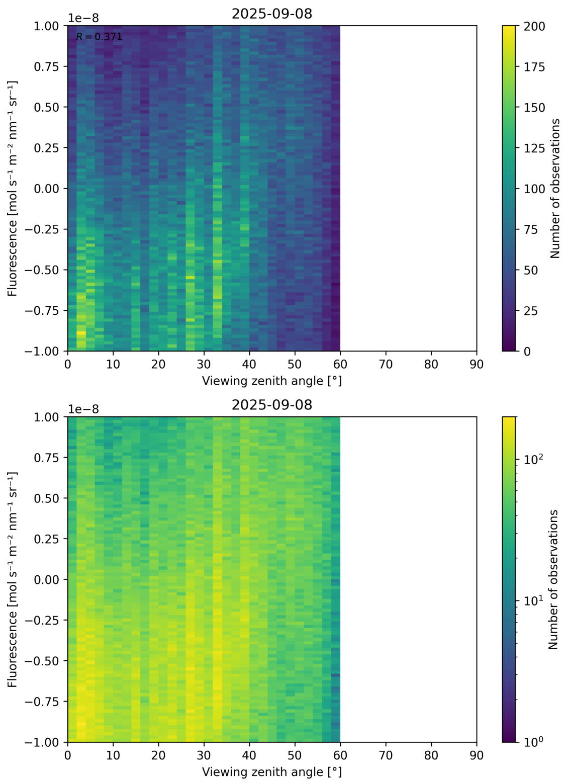
Figure 108: Scatter density plot of “Viewing zenith angle” against “Fluorescence” for 2025-09-07 to 2025-09-09.
