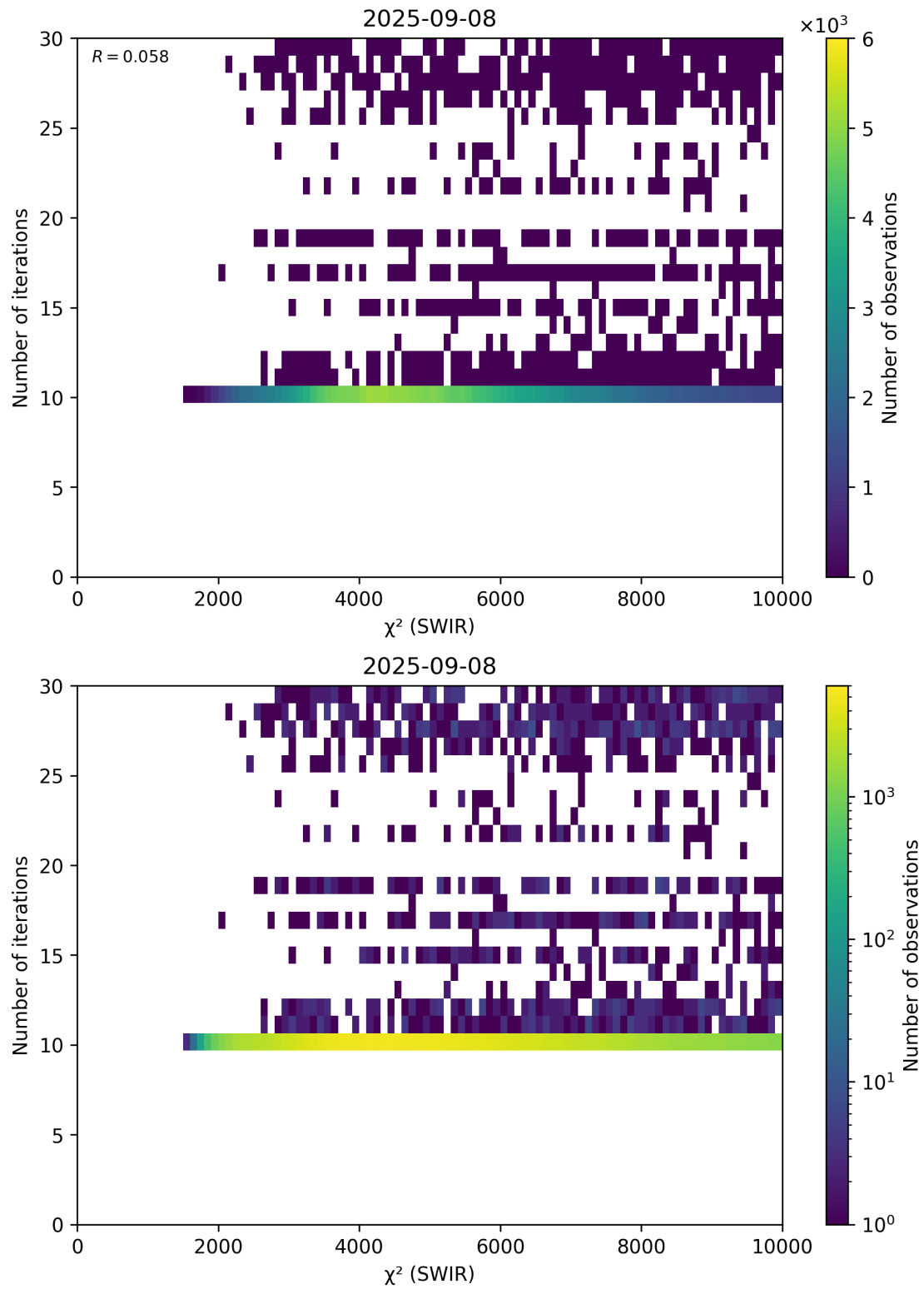
Figure 50: Scatter density plot of “ \chi^2 (SWIR)” against “Number of iterations” for 2025-09-07 to 2025-09-09.
