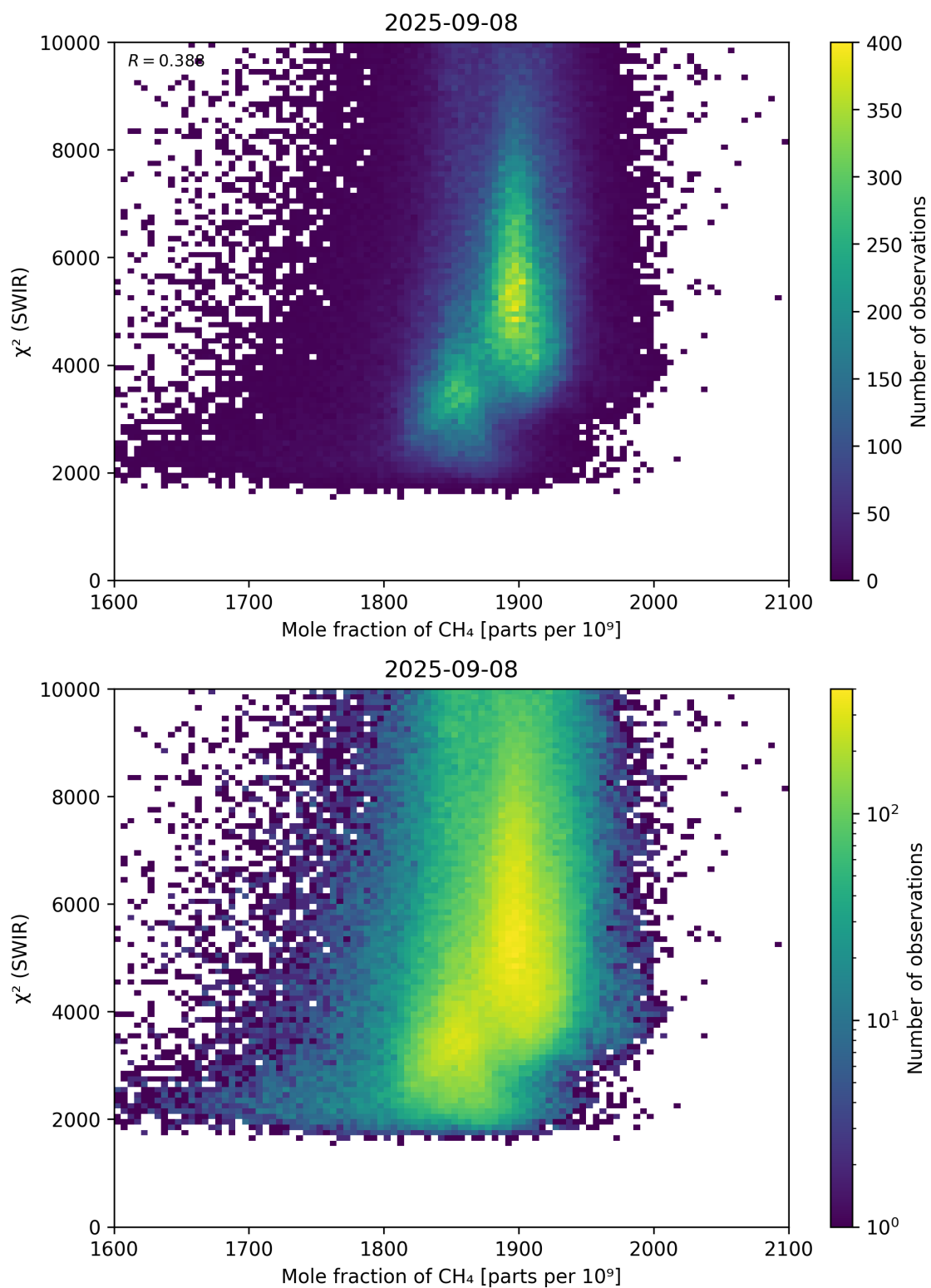
Figure 71: Scatter density plot of “Mole fraction of \text{CH}_4 ” against “ \chi^2 (SWIR)” for 2025-09-07 to 2025-09-09.
