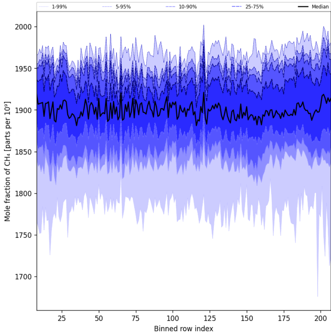
Figure 34: Along track statistics of “Mole fraction of CH 4 ” for 2025-09-07 to 2025-09-09
