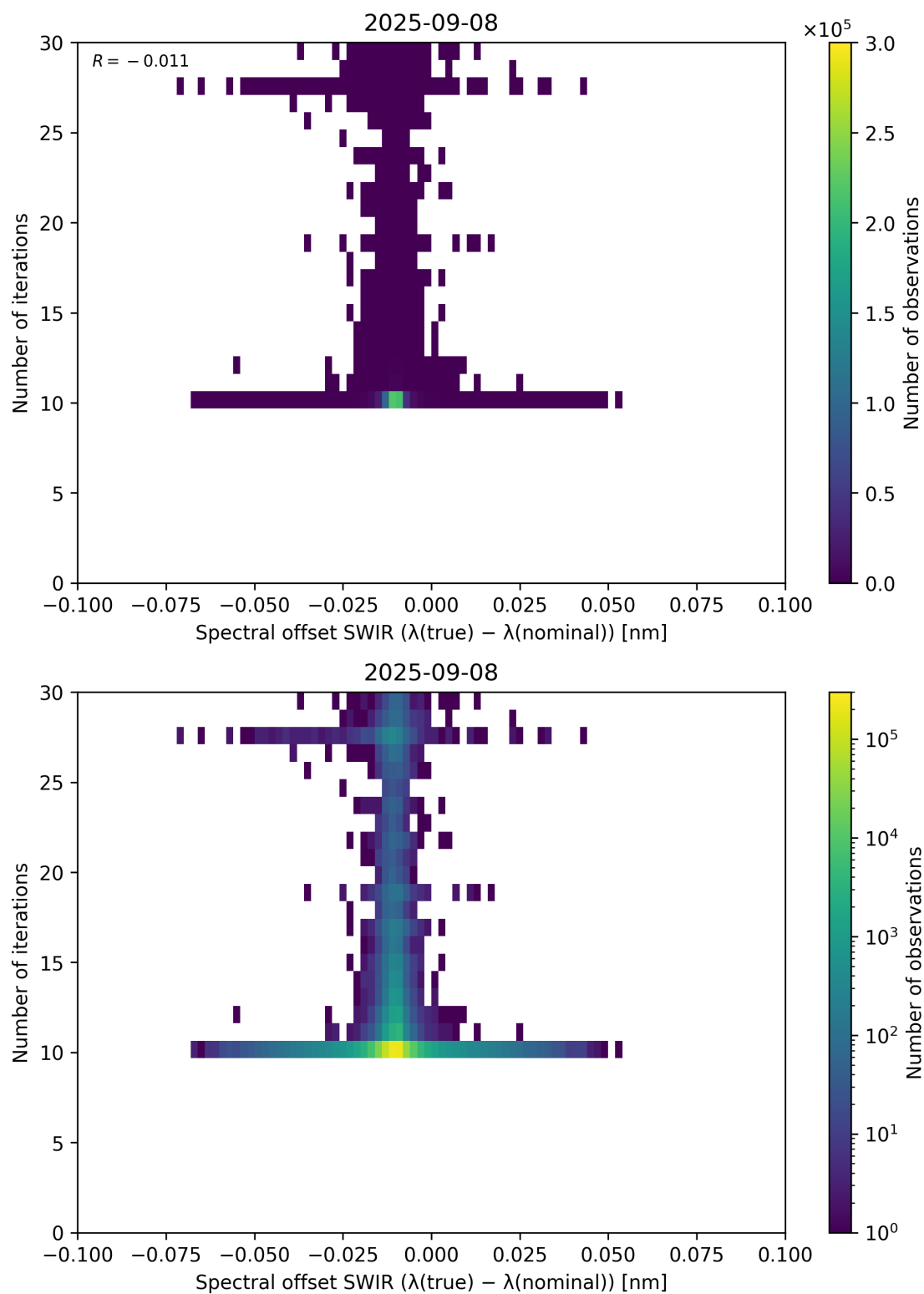
Figure 121: Scatter density plot of “Spectral offset SWIR ( \lambda_{\text{true}} - \lambda_{\text{nominal}} )” against “Number of iterations” for 2025-09-07 to 2025-09-09.
