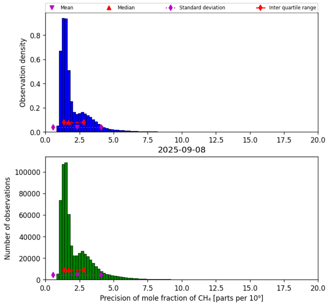
Figure 24: Histogram of “Precision of mole fraction of CH 4 ” for 2025-09-07 to 2025-09-09
