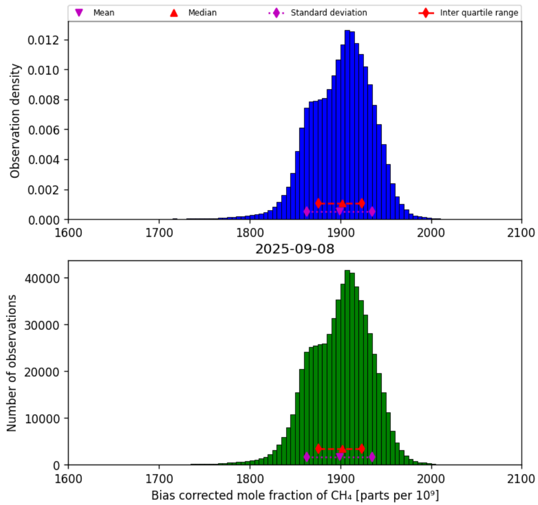
Figure 25: Histogram of “Bias corrected mole fraction of CH 4 ” for 2025-09-07 to 2025-09-09
