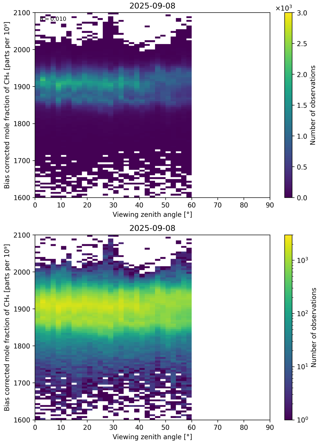
Figure 111: Scatter density plot of “Viewing zenith angle” against “Bias corrected mole fraction of CH 4 ” for 2025-09-07 to 2025-09-09.
