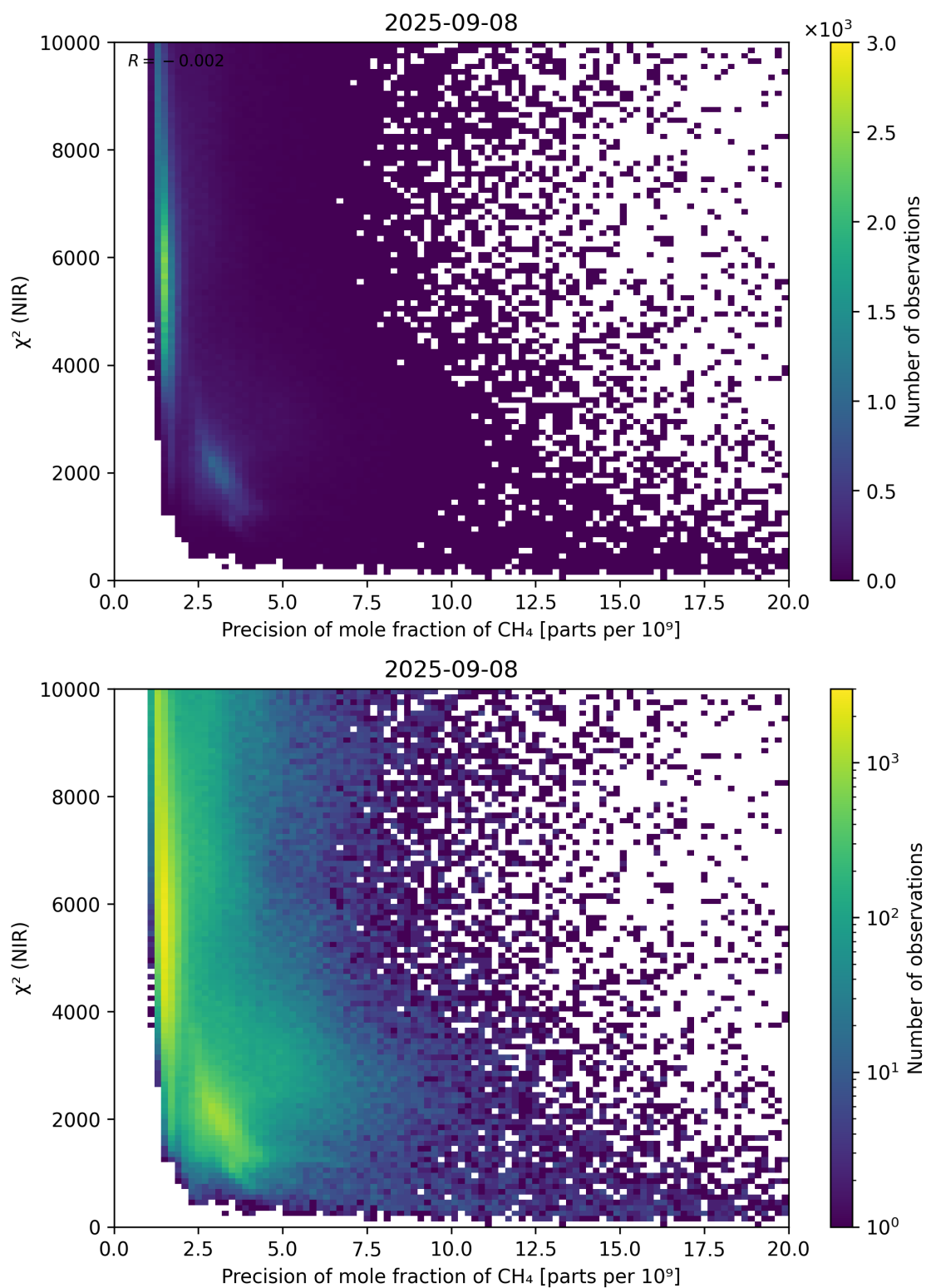
Figure 78: Scatter density plot of “Precision of mole fraction of CH 4 ” against “ \chi^2 (NIR)” for 2025-09-07 to 2025-09-09.
