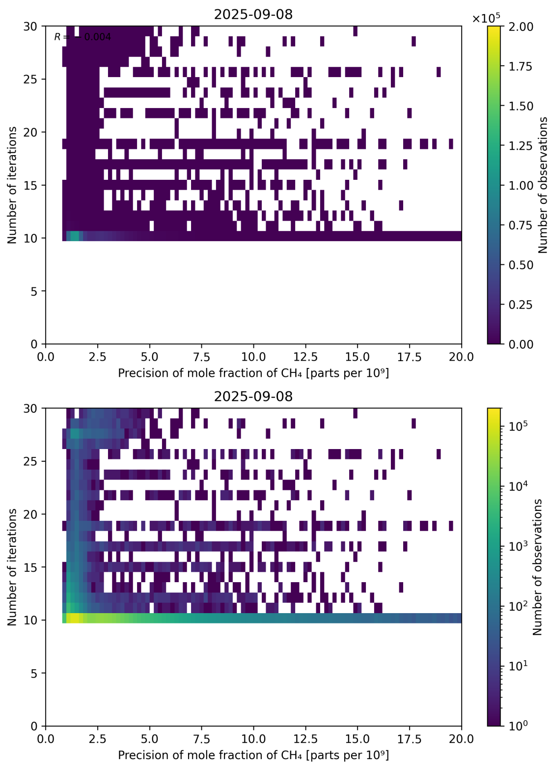
Figure 83: Scatter density plot of “Precision of mole fraction of CH 4 ” against “Number of iterations” for 2025-09-07 to 2025-09-09.
