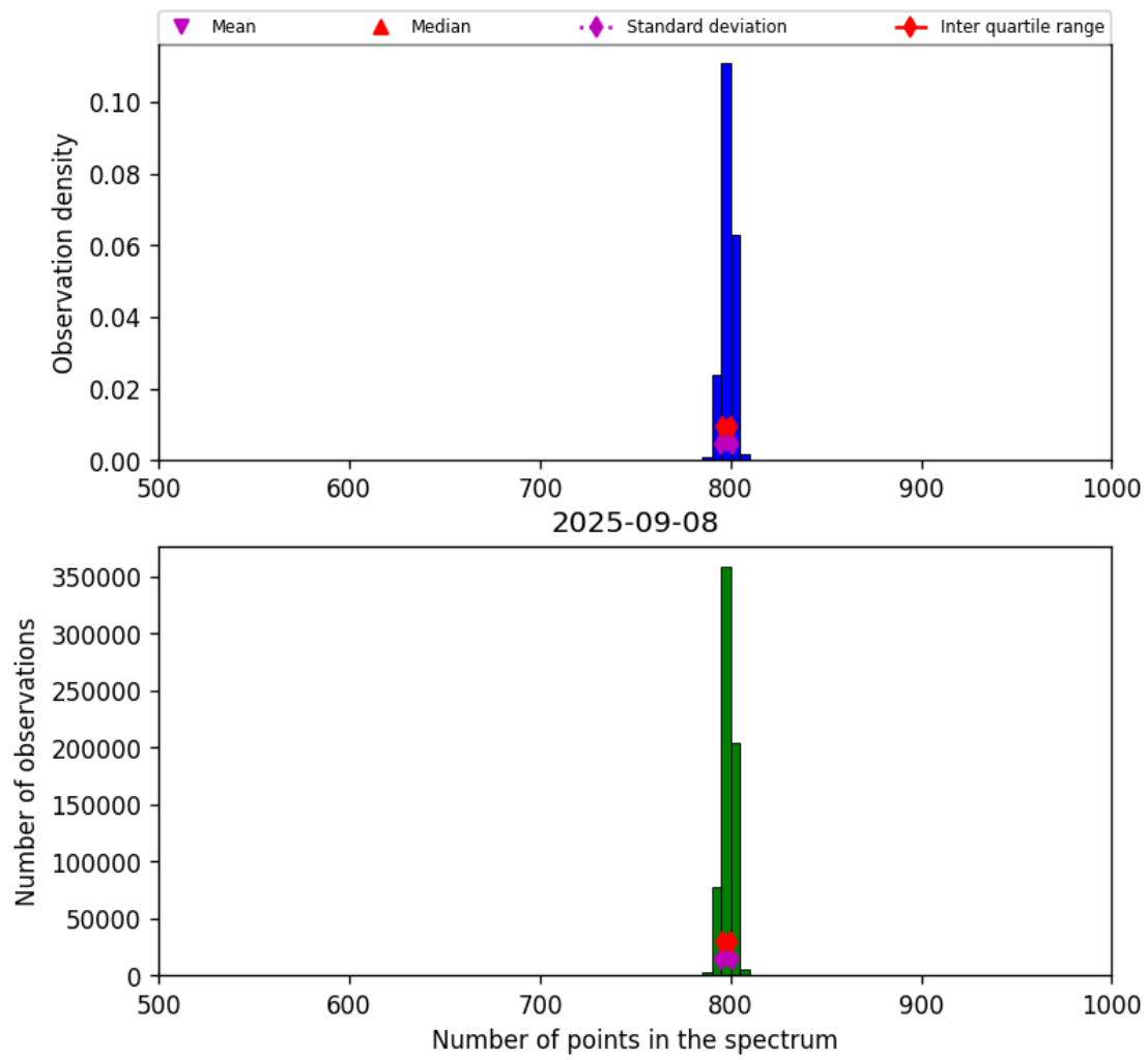
Figure 26: Histogram of “Number of points in the spectrum” for 2025-09-07 to 2025-09-09
