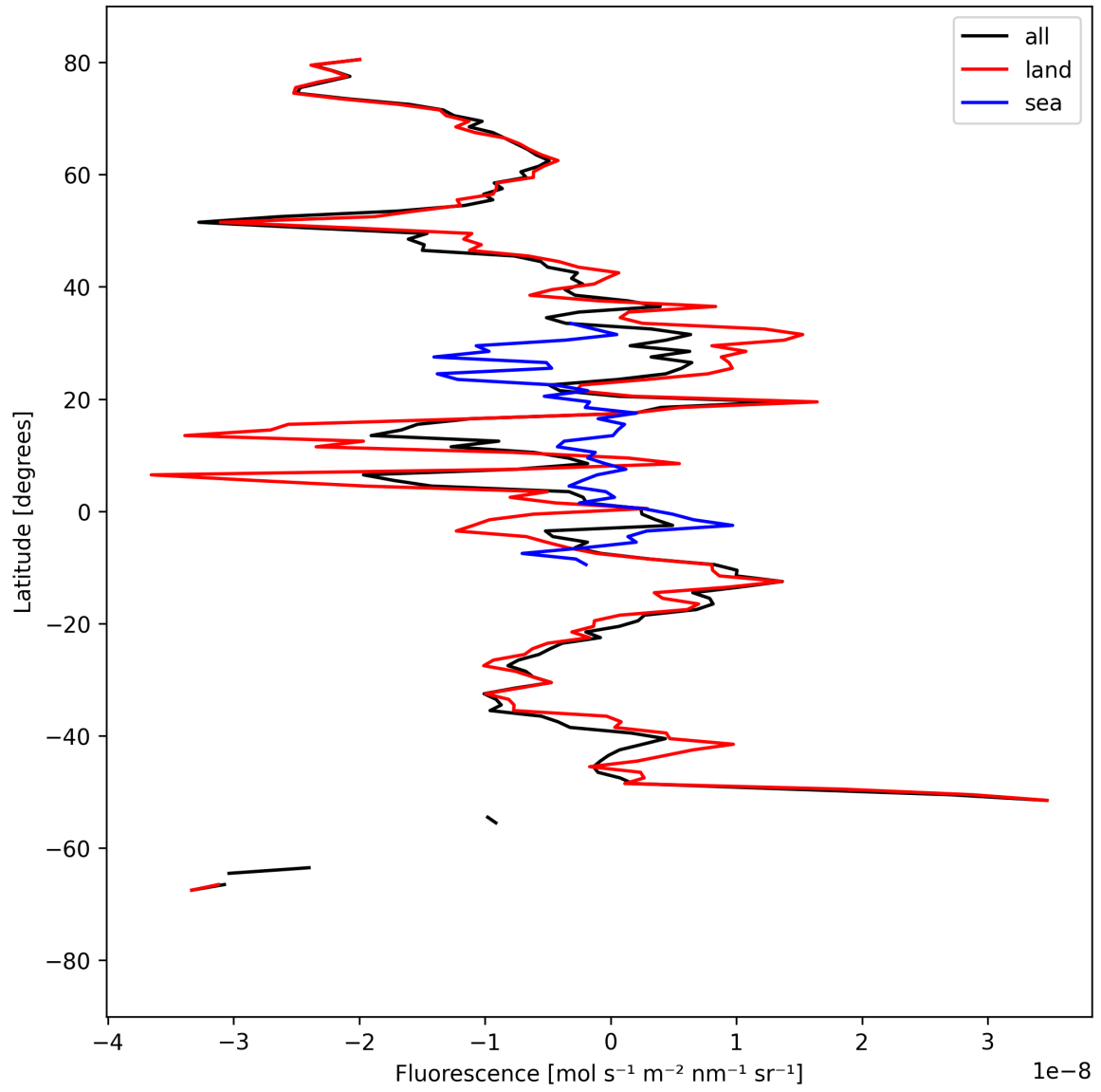
Figure 21: Zonal average of “Fluorescence” for 2025-09-07 to 2025-09-09.
