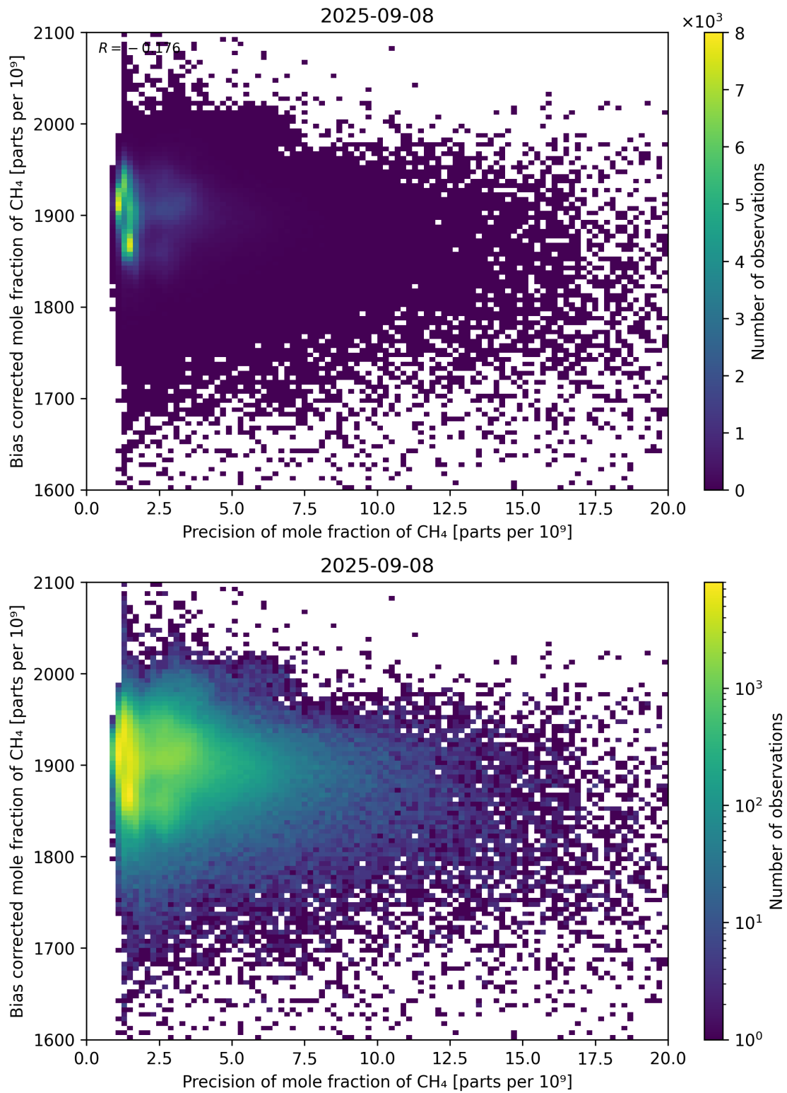
Figure 82: Scatter density plot of “Precision of mole fraction of CH 4 ” against “Bias corrected mole fraction of CH 4 ” for 2025-09-07 to 2025-09-09.
