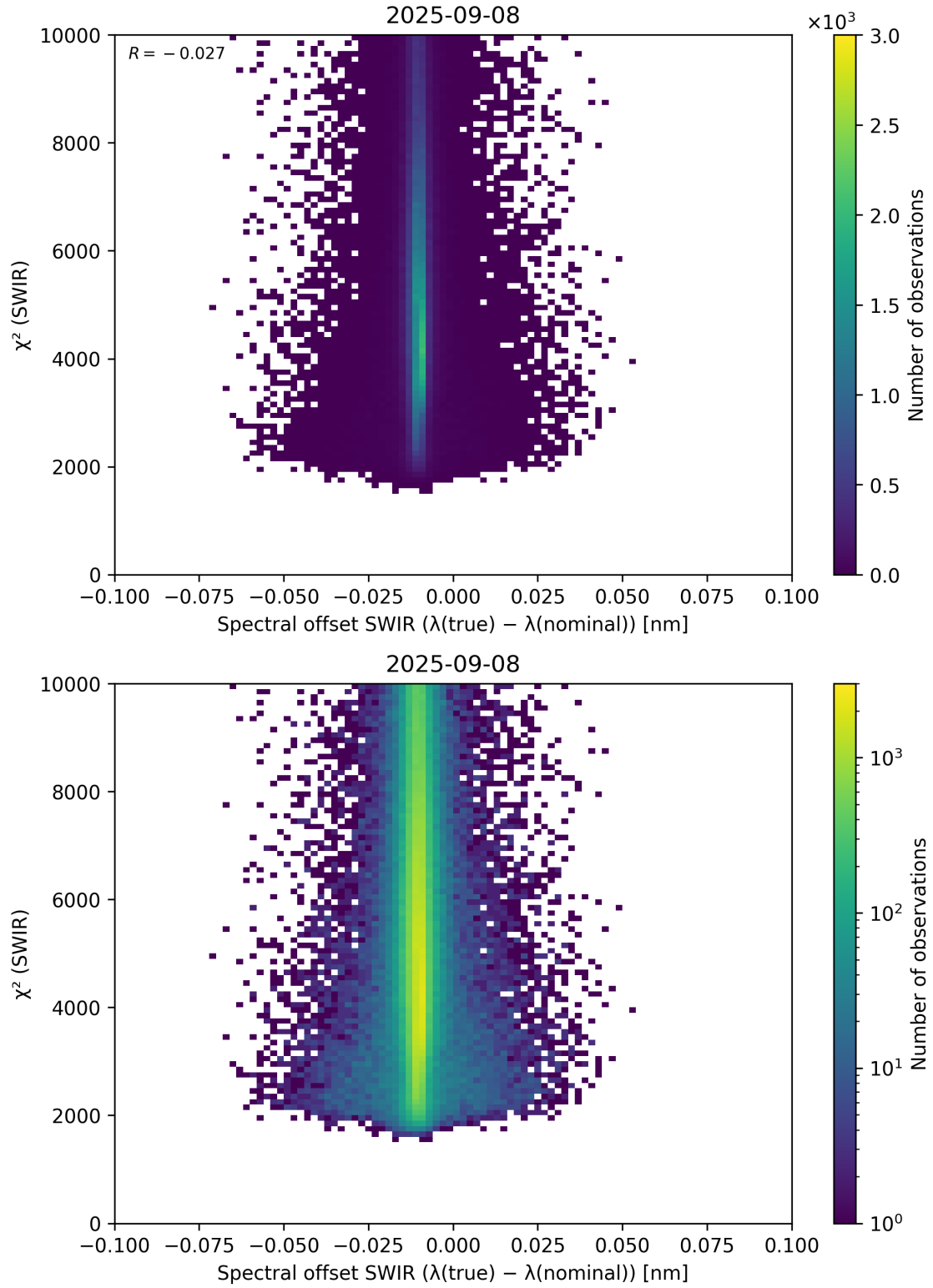
Figure 118: Scatter density plot of “Spectral offset SWIR ( \lambda_{\text{true}} - \lambda_{\text{nominal}} )” against “ \chi^2 (SWIR)” for 2025-09-07 to 2025-09-09.
