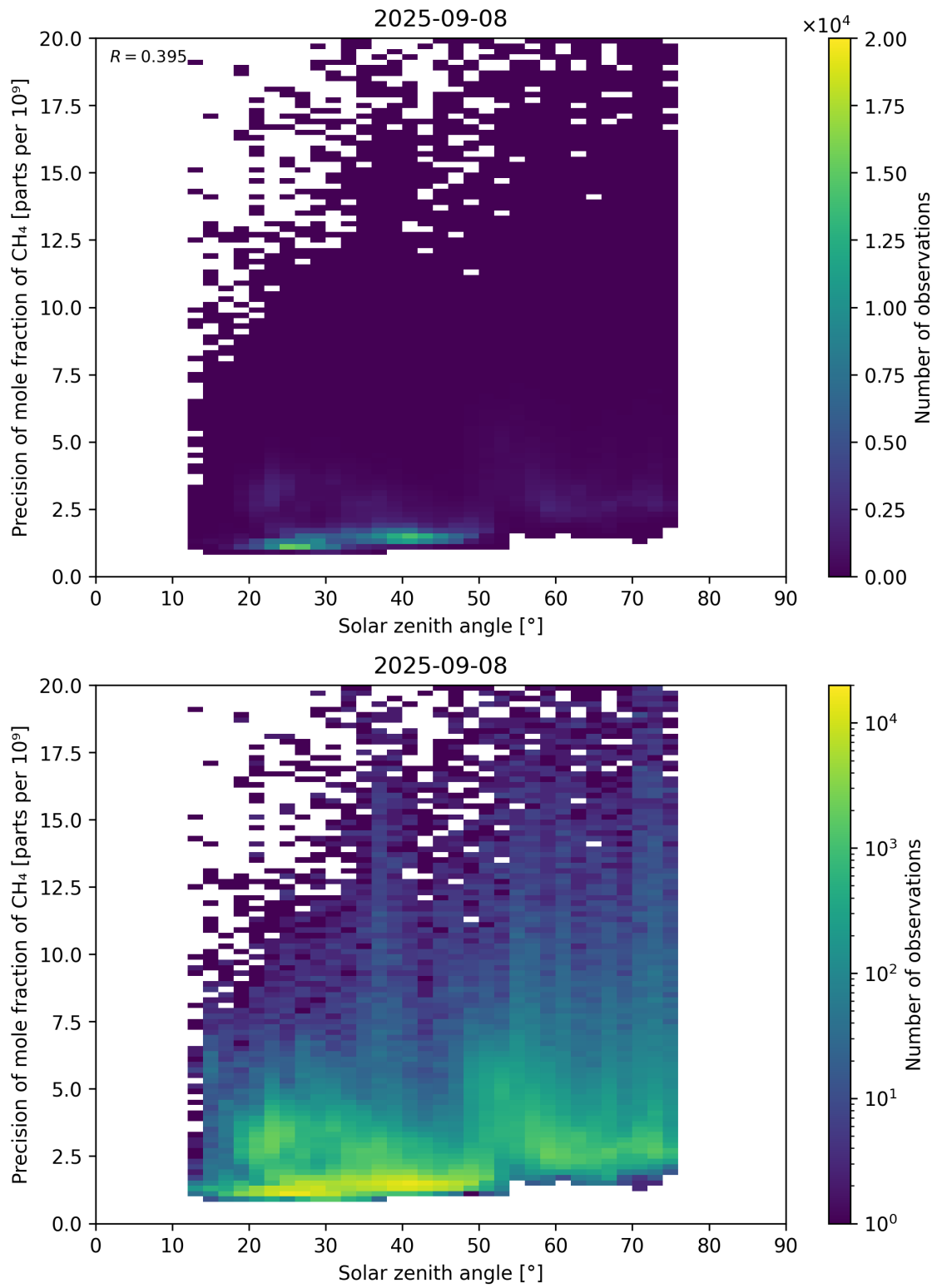
Figure 101: Scatter density plot of “Solar zenith angle” against “Precision of mole fraction of CH 4 ” for 2025-09-07 to 2025-09-09.
