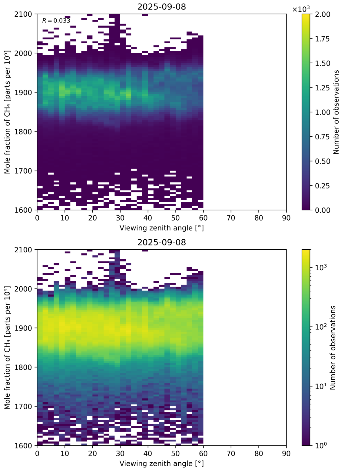
Figure 110: Scatter density plot of “Viewing zenith angle” against “Mole fraction of CH 4 ” for 2025-09-07 to 2025-09-09.
