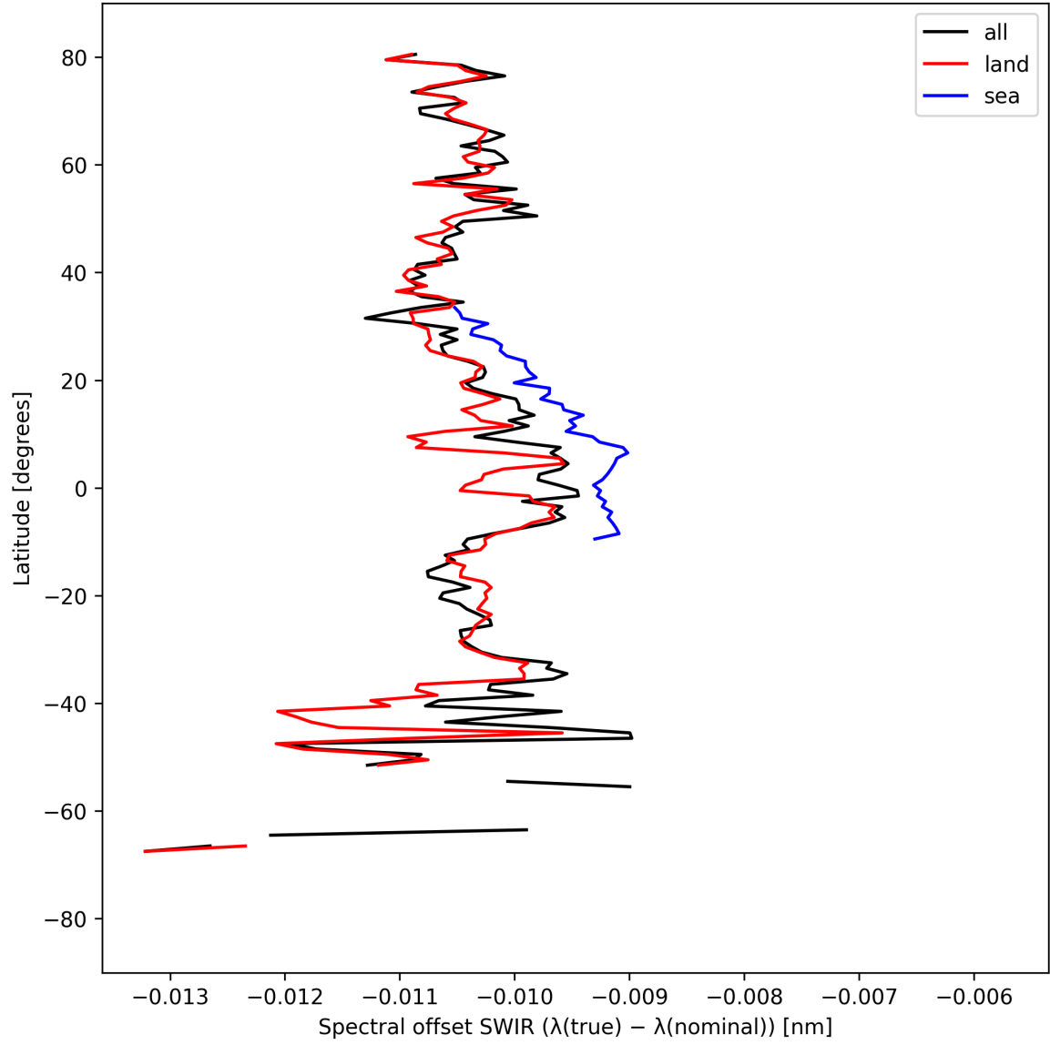
Figure 16: Zonal average of “Spectral offset SWIR ( \lambda_{\text{true}} - \lambda_{\text{nominal}} )” for 2025-09-07 to 2025-09-09.
