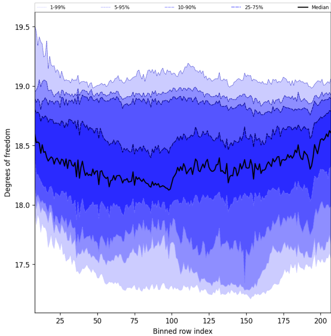
Figure 41: Along track statistics of “Degrees of freedom” for 2025-09-07 to 2025-09-09
