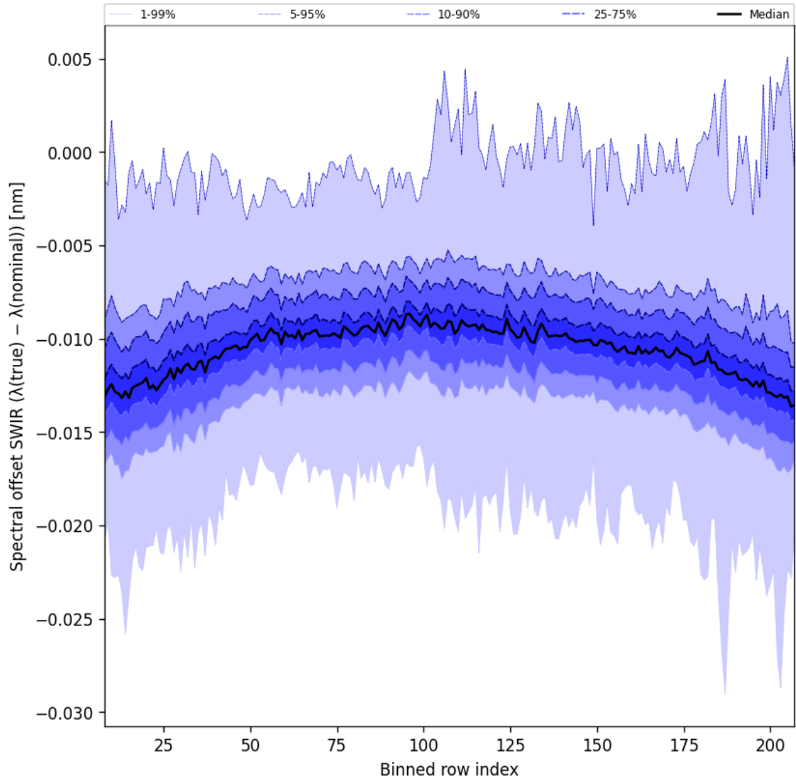
Figure 38: Along track statistics of “Spectral offset SWIR ( \lambda_{\text{true}} - \lambda_{\text{nominal}} )” for 2025-09-07 to 2025-09-09
