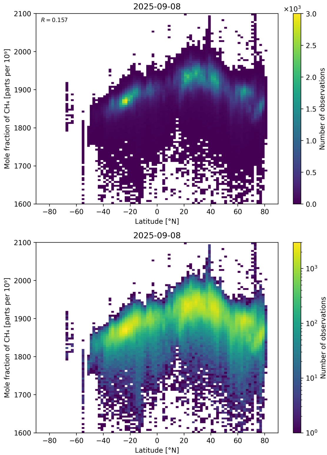
Figure 57: Scatter density plot of “Latitude” against “Mole fraction of CH 4 ” for 2025-09-07 to 2025-09-09.
