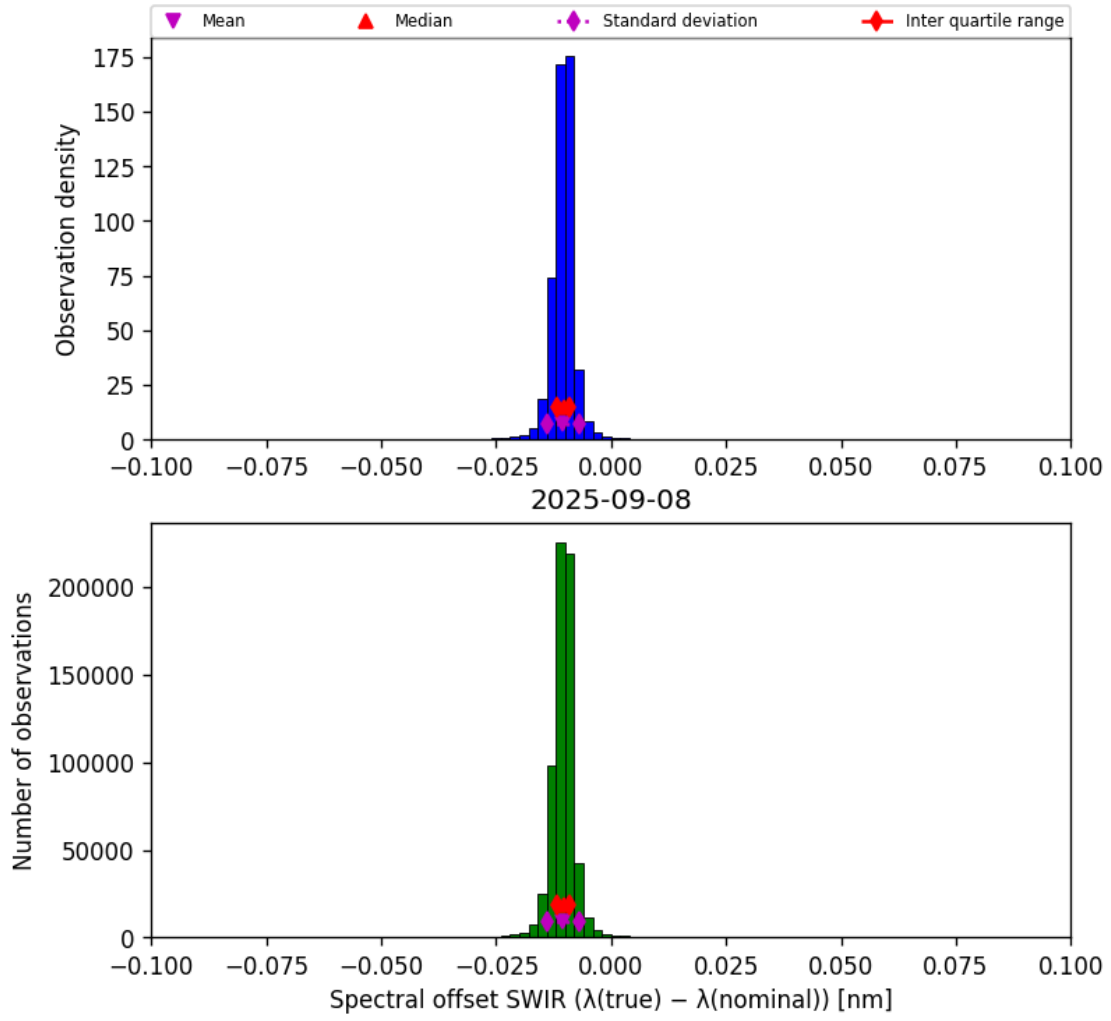
Figure 27: Histogram of “Spectral offset SWIR ( \lambda_{\text{true}} - \lambda_{\text{nominal}} )” for 2025-09-07 to 2025-09-09
