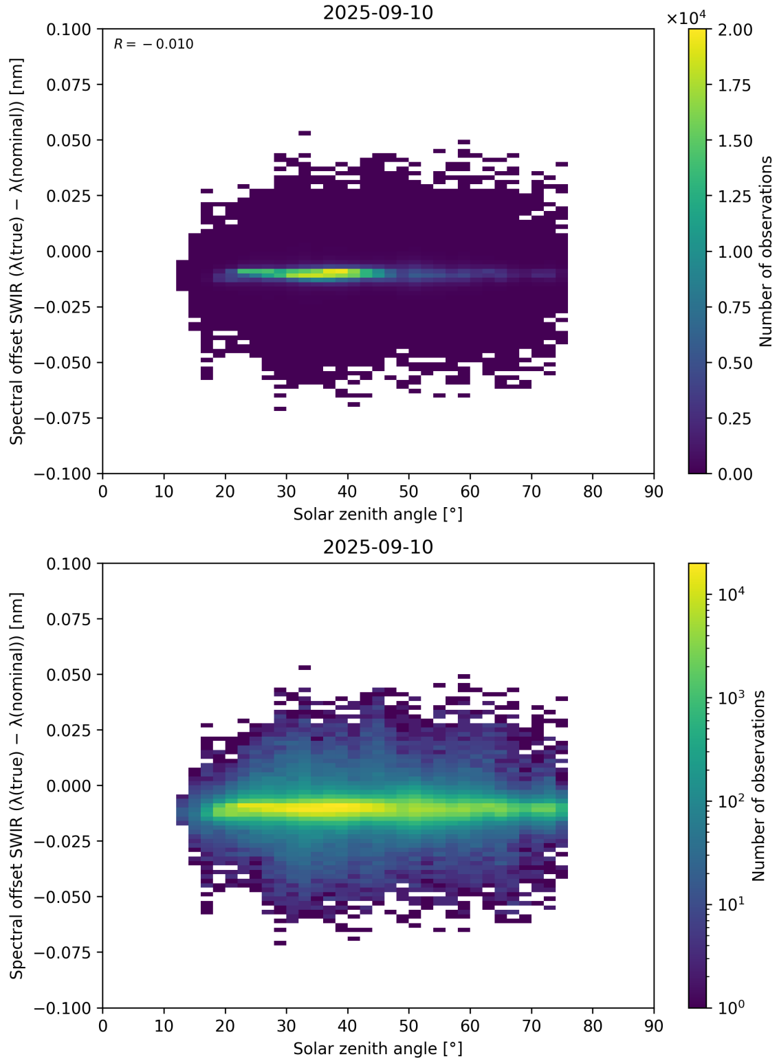
Figure 104: Scatter density plot of “Solar zenith angle” against “Spectral offset SWIR ( \lambda_{\text{true}} - \lambda_{\text{nominal}} )” for 2025-09-10 to 2025-09-11.
