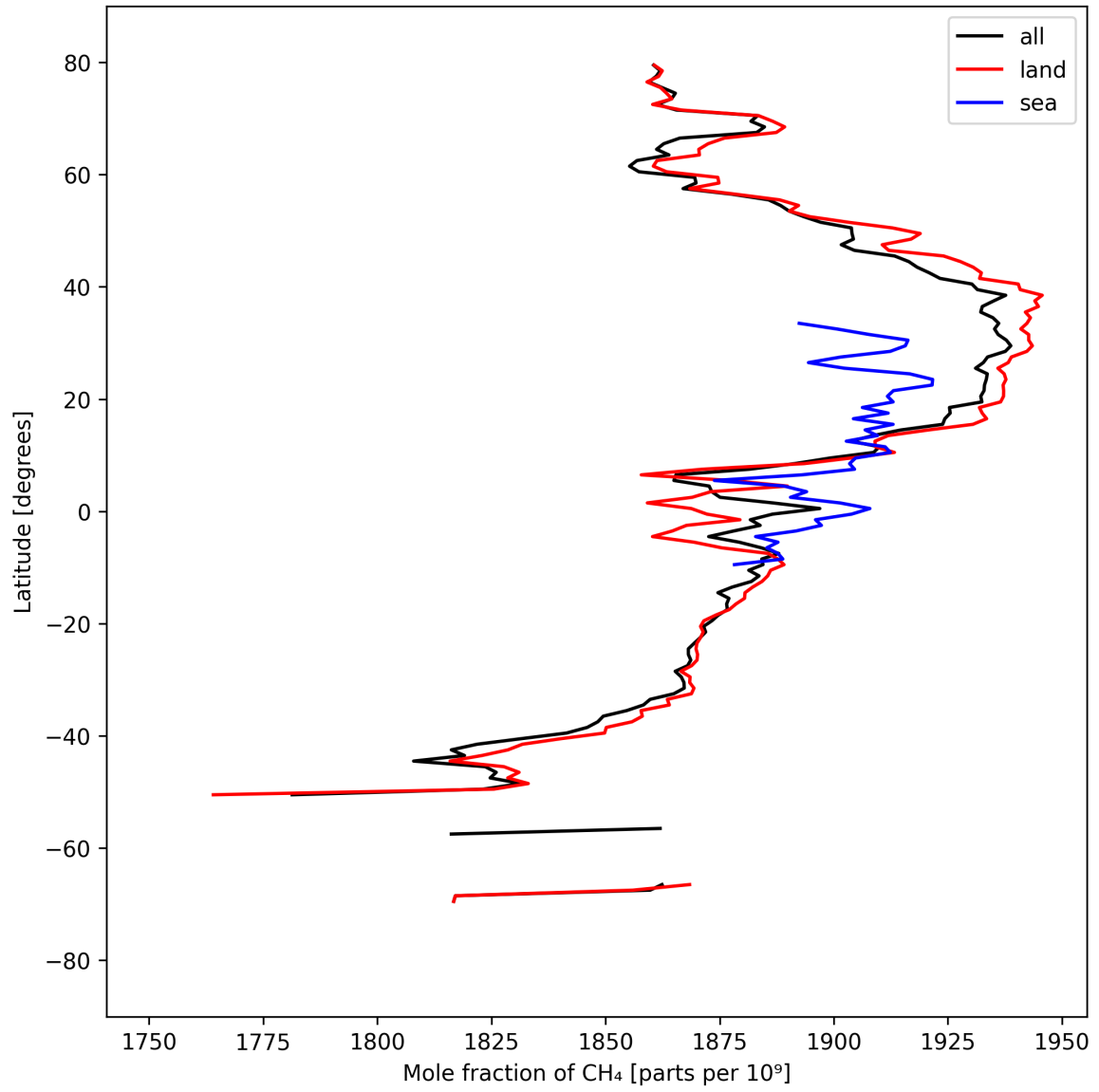
Figure 12: Zonal average of “Mole fraction of \text{CH}_4 ” for 2025-09-10 to 2025-09-11.
