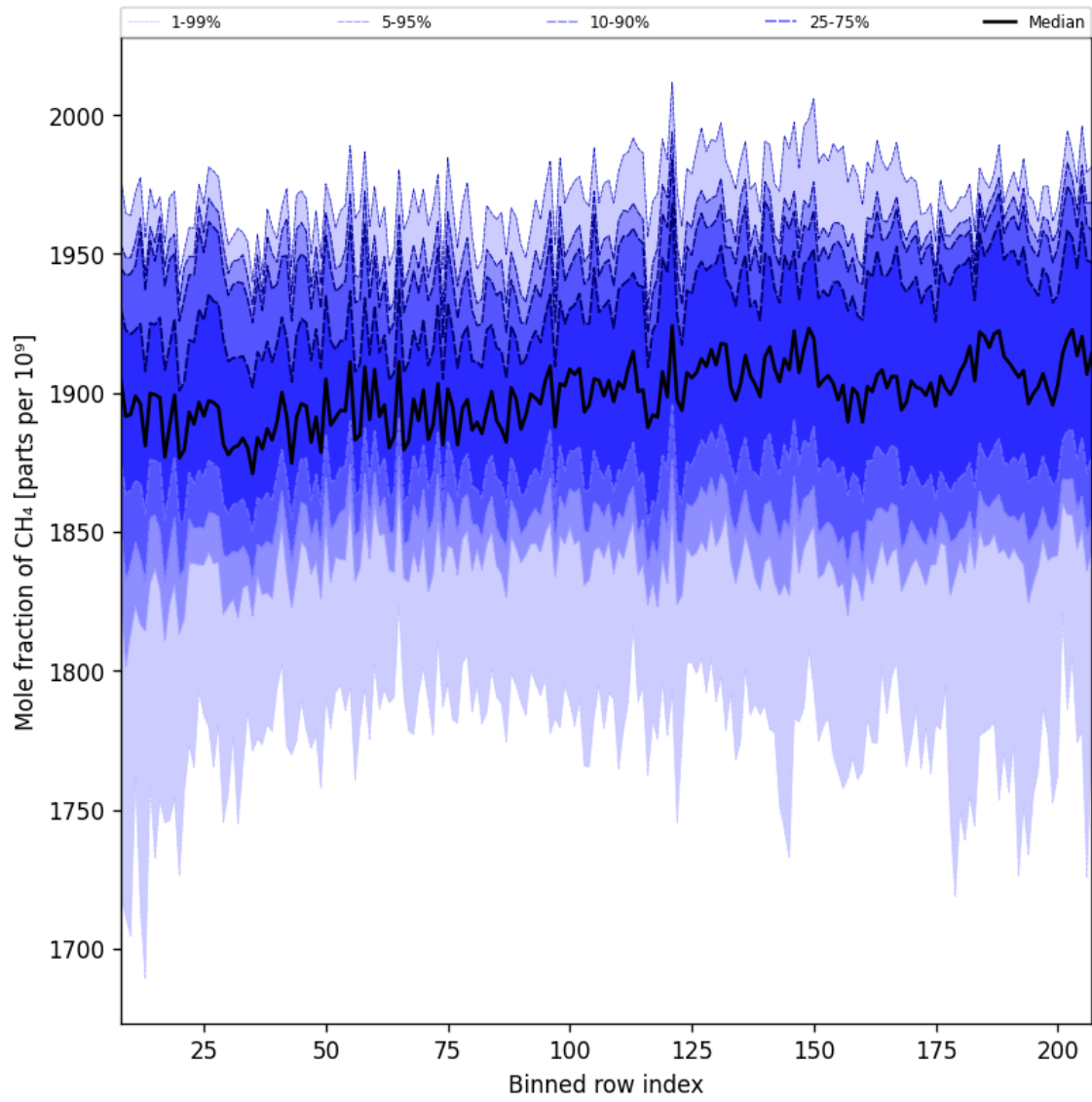
Figure 34: Along track statistics of “Mole fraction of CH 4 ” for 2025-09-10 to 2025-09-11
