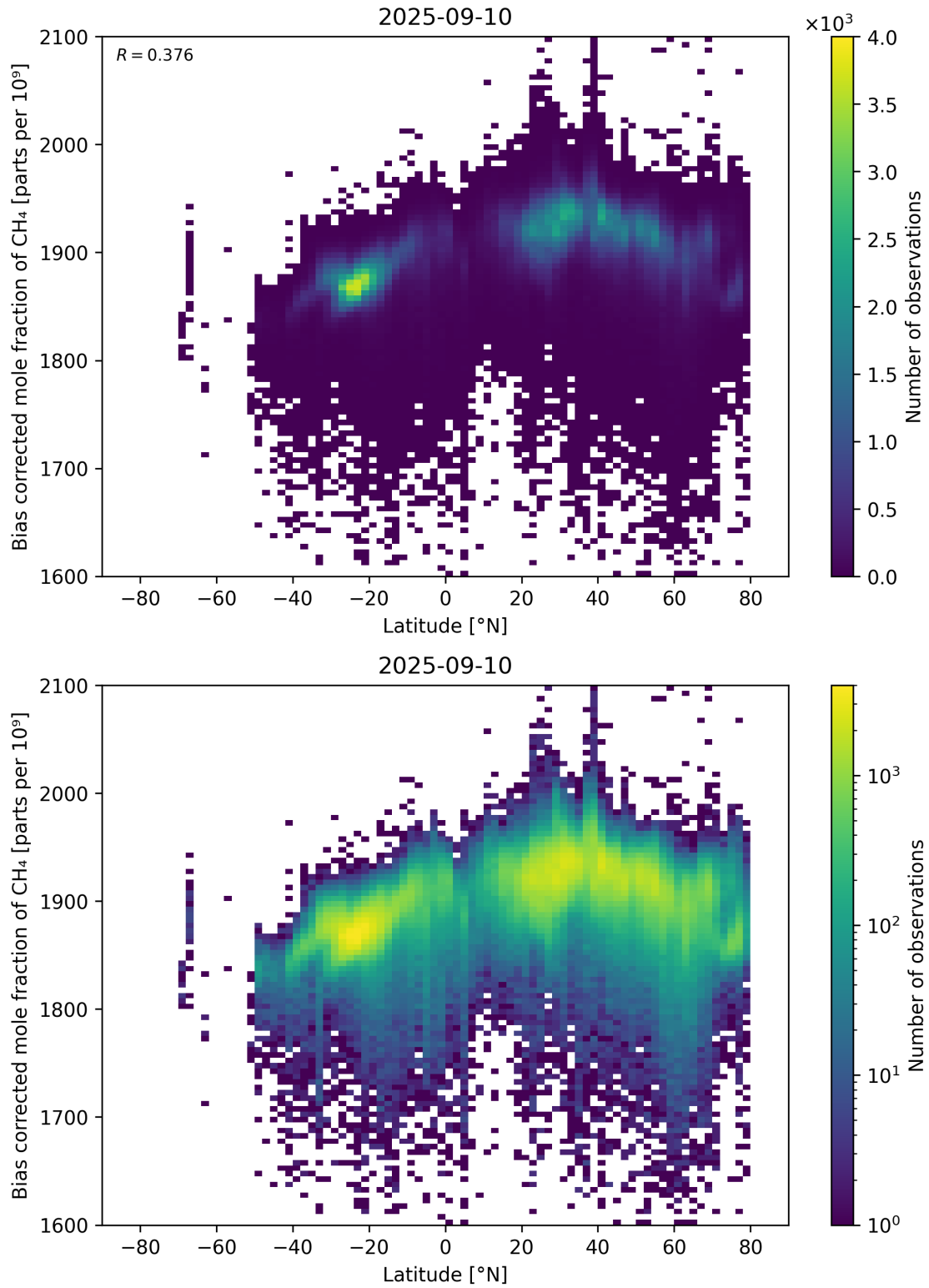
Figure 58: Scatter density plot of “Latitude” against “Bias corrected mole fraction of CH 4 ” for 2025-09-10 to 2025-09-11.
