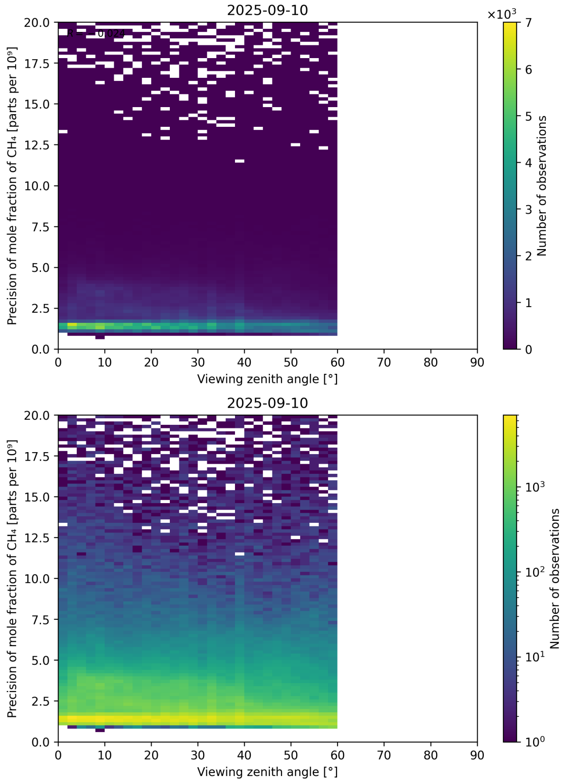
Figure 112: Scatter density plot of “Viewing zenith angle” against “Precision of mole fraction of CH 4 ” for 2025-09-10 to 2025-09-11.
