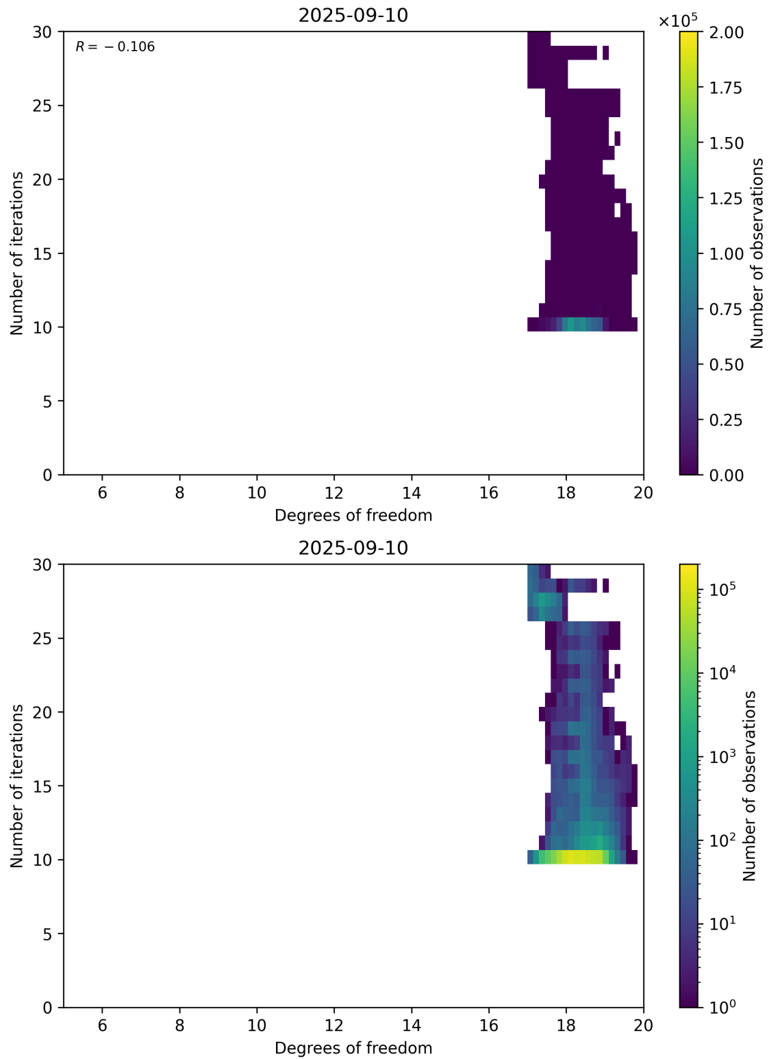
Figure 52: Scatter density plot of “Degrees of freedom” against “Number of iterations” for 2025-09-10 to 2025-09-11.
