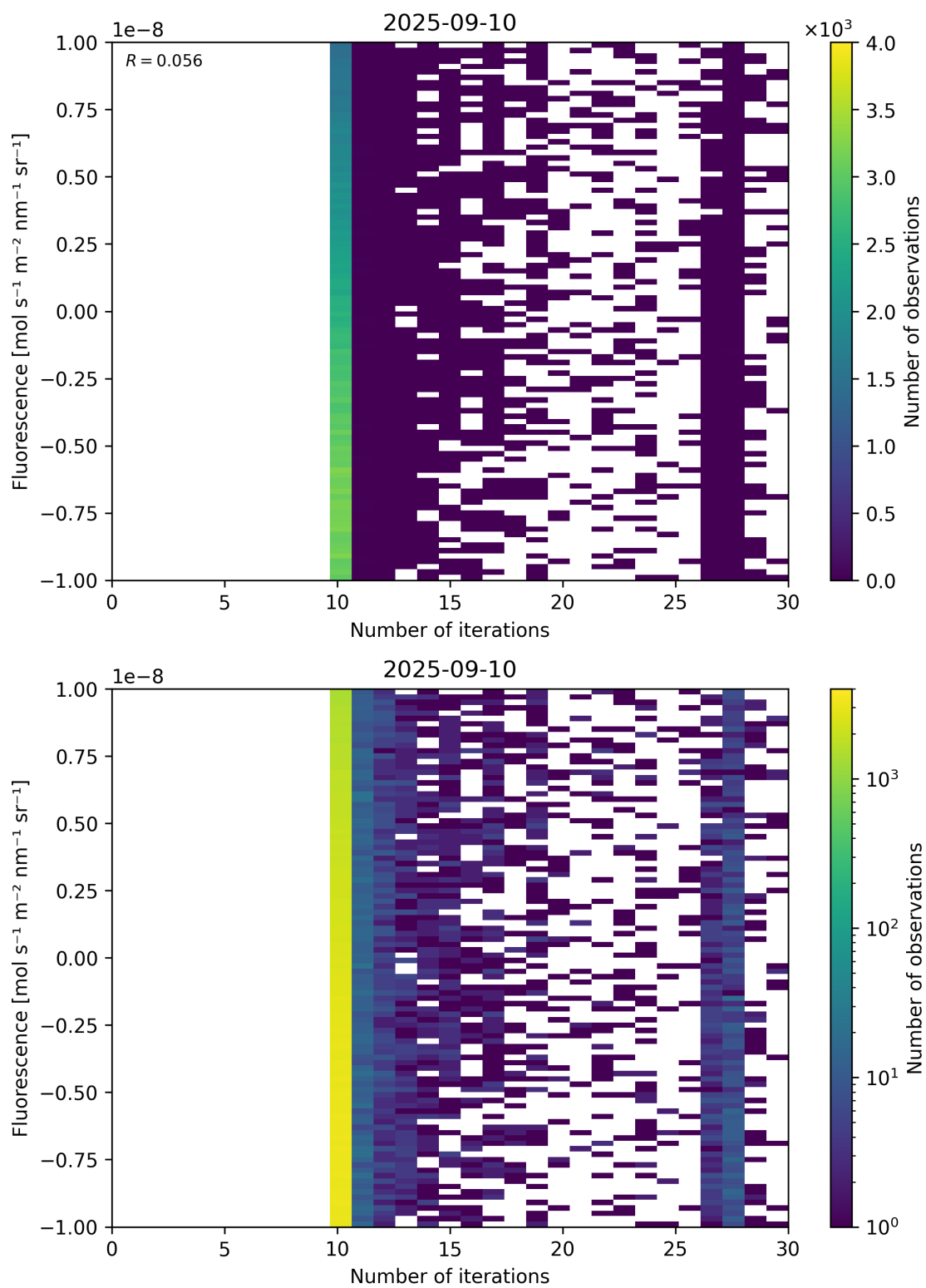
Figure 87: Scatter density plot of “Number of iterations” against “Fluorescence” for 2025-09-10 to 2025-09-11.
