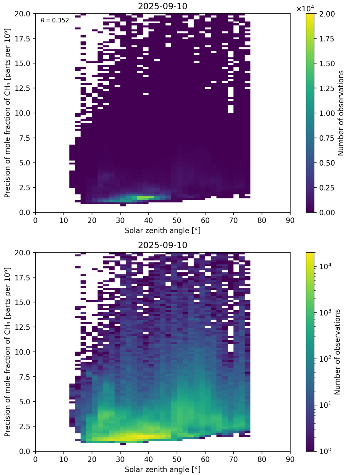
Figure 101: Scatter density plot of “Solar zenith angle” against “Precision of mole fraction of CH 4 ” for 2025-09-10 to 2025-09-11.
