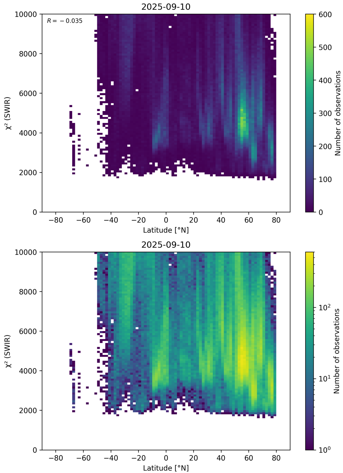
Figure 54: Scatter density plot of “Latitude” against “ \chi^2 (SWIR)” for 2025-09-10 to 2025-09-11.
