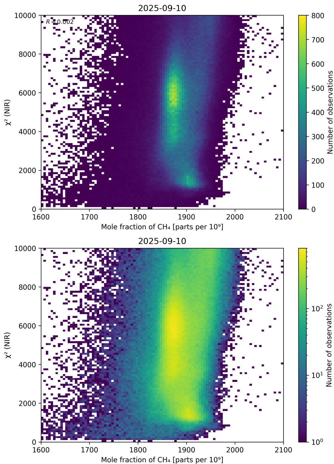
Figure 70: Scatter density plot of “Mole fraction of CH 4 ” against “ \chi^2 (NIR)” for 2025-09-10 to 2025-09-11.
