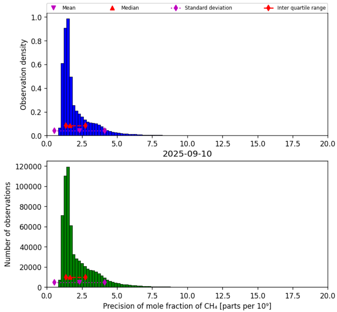
Figure 24: Histogram of “Precision of mole fraction of CH 4 ” for 2025-09-10 to 2025-09-11
