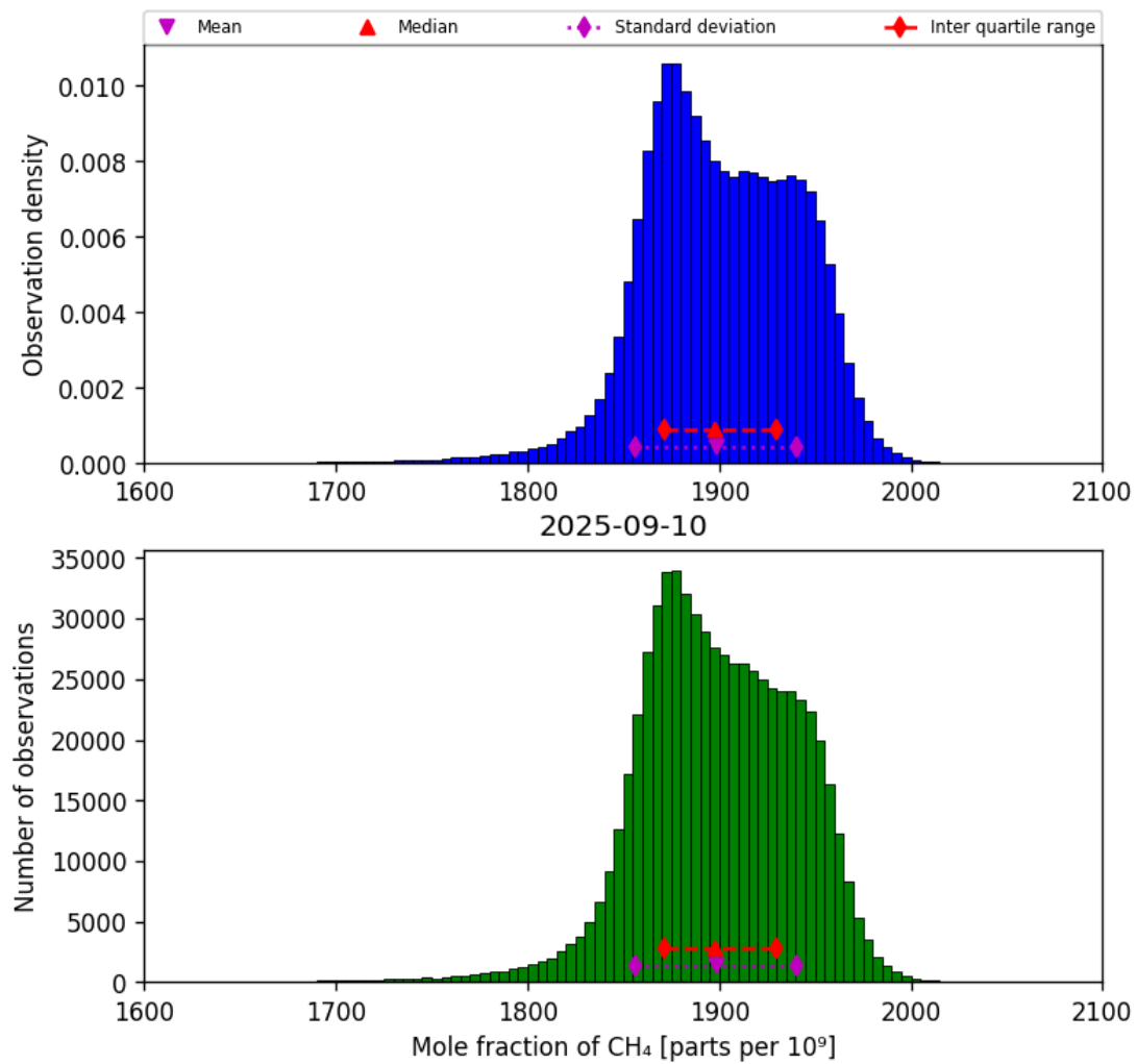
Figure 23: Histogram of “Mole fraction of CH 4 ” for 2025-09-10 to 2025-09-11
