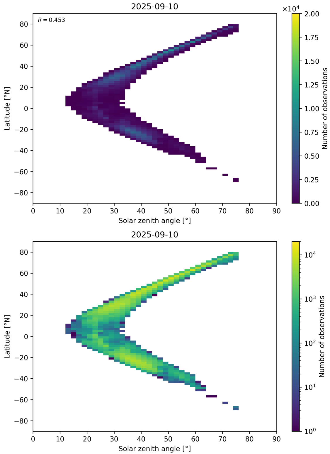
Figure 98: Scatter density plot of “Solar zenith angle” against “Latitude” for 2025-09-10 to 2025-09-11.
