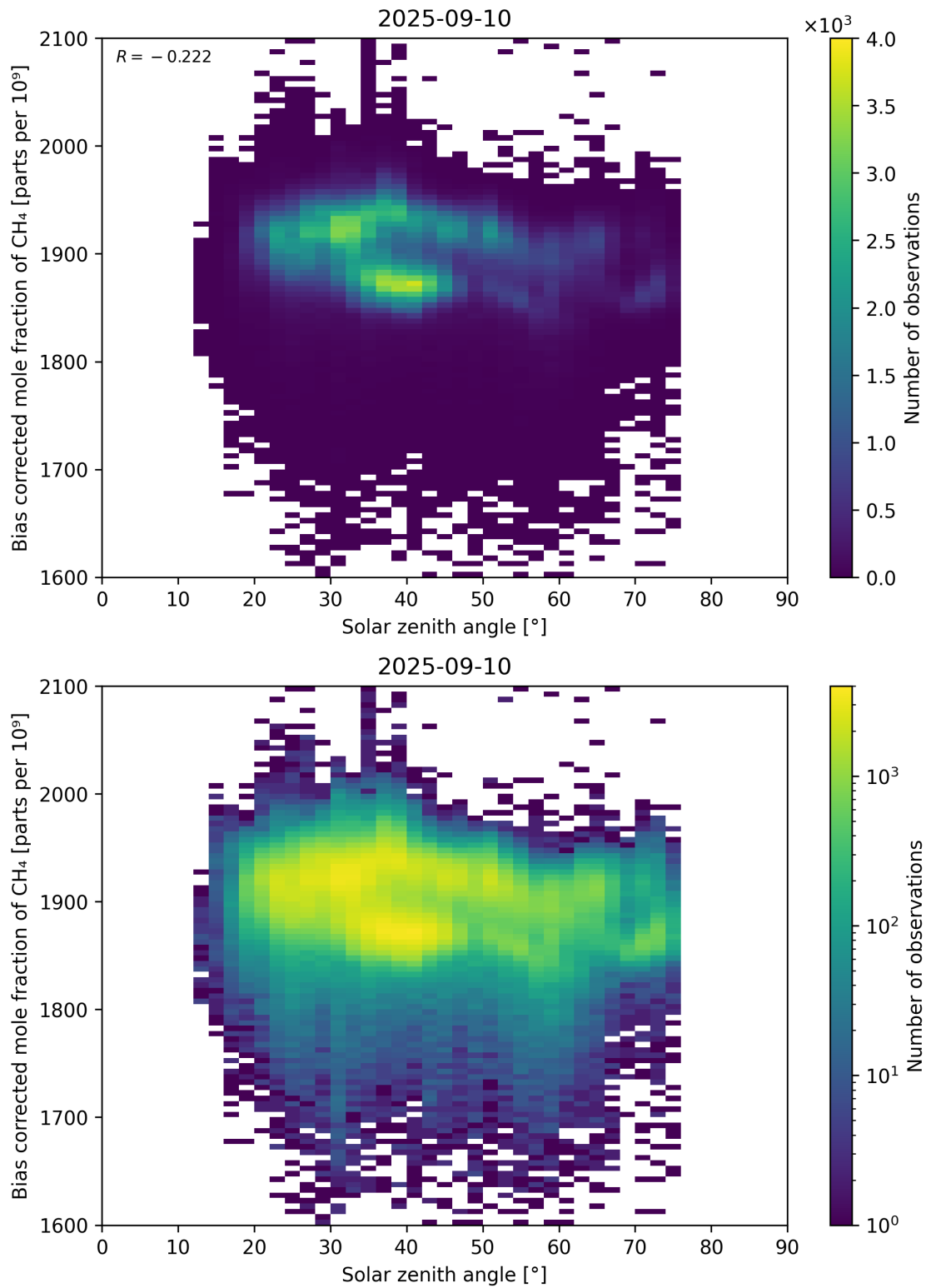
Figure 100: Scatter density plot of “Solar zenith angle” against “Bias corrected mole fraction of CH 4 ” for 2025-09-10 to 2025-09-11.
