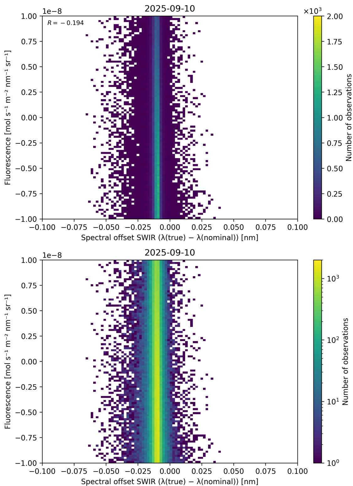
Figure 120: Scatter density plot of “Spectral offset SWIR ( \lambda_{\text{true}} - \lambda_{\text{nominal}} )” against “Fluorescence” for 2025-09-10 to 2025-09-11.
