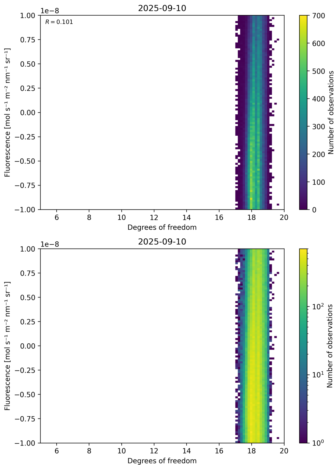
Figure 51: Scatter density plot of “Degrees of freedom” against “Fluorescence” for 2025-09-10 to 2025-09-11.
