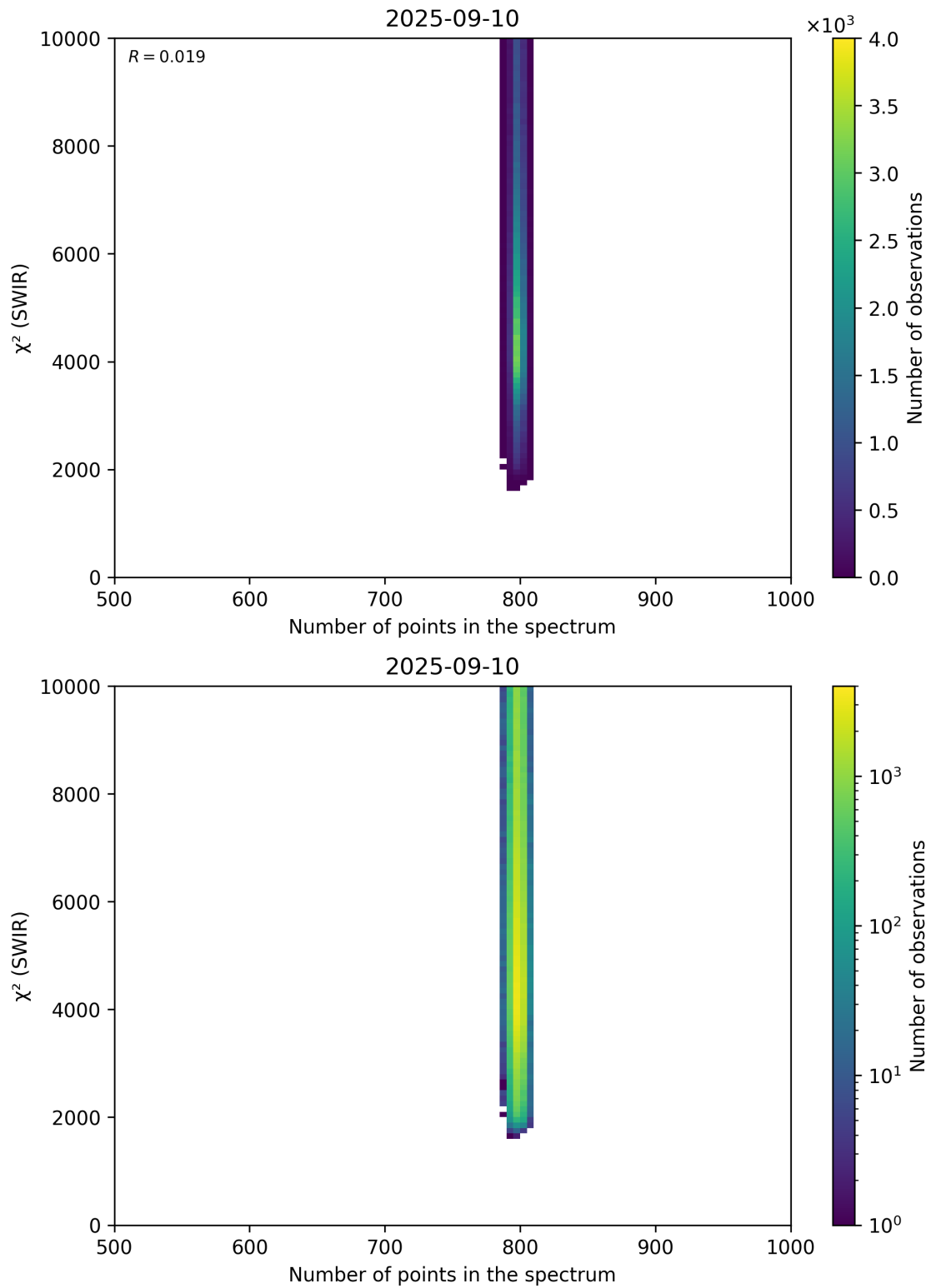
Figure 89: Scatter density plot of “Number of points in the spectrum” against “ \chi^2 (SWIR)” for 2025-09-10 to 2025-09-11.
