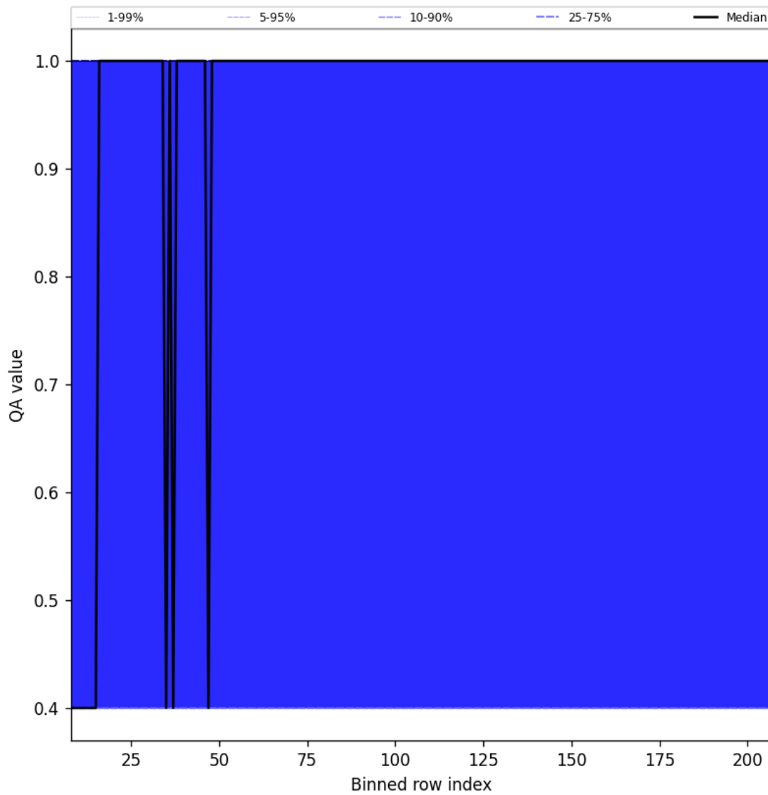
Figure 33: Along track statistics of “QA value” for 2025-09-10 to 2025-09-11
