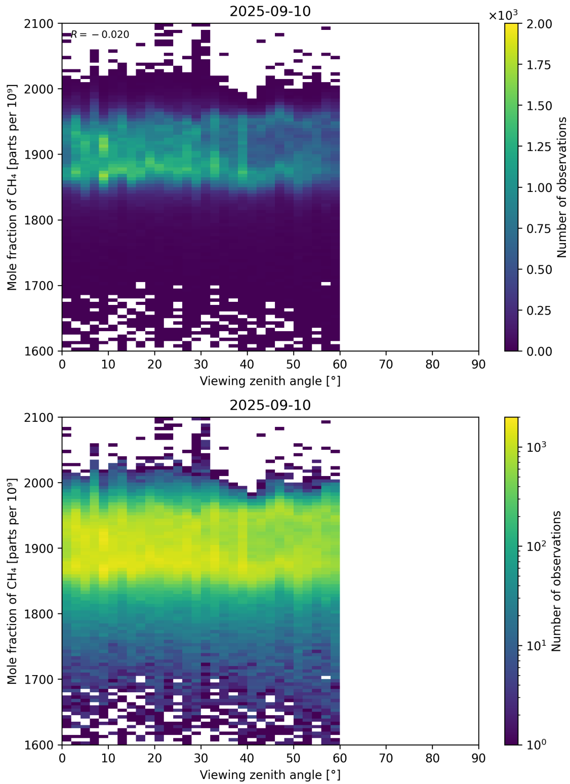
Figure 110: Scatter density plot of “Viewing zenith angle” against “Mole fraction of CH 4 ” for 2025-09-10 to 2025-09-11.
