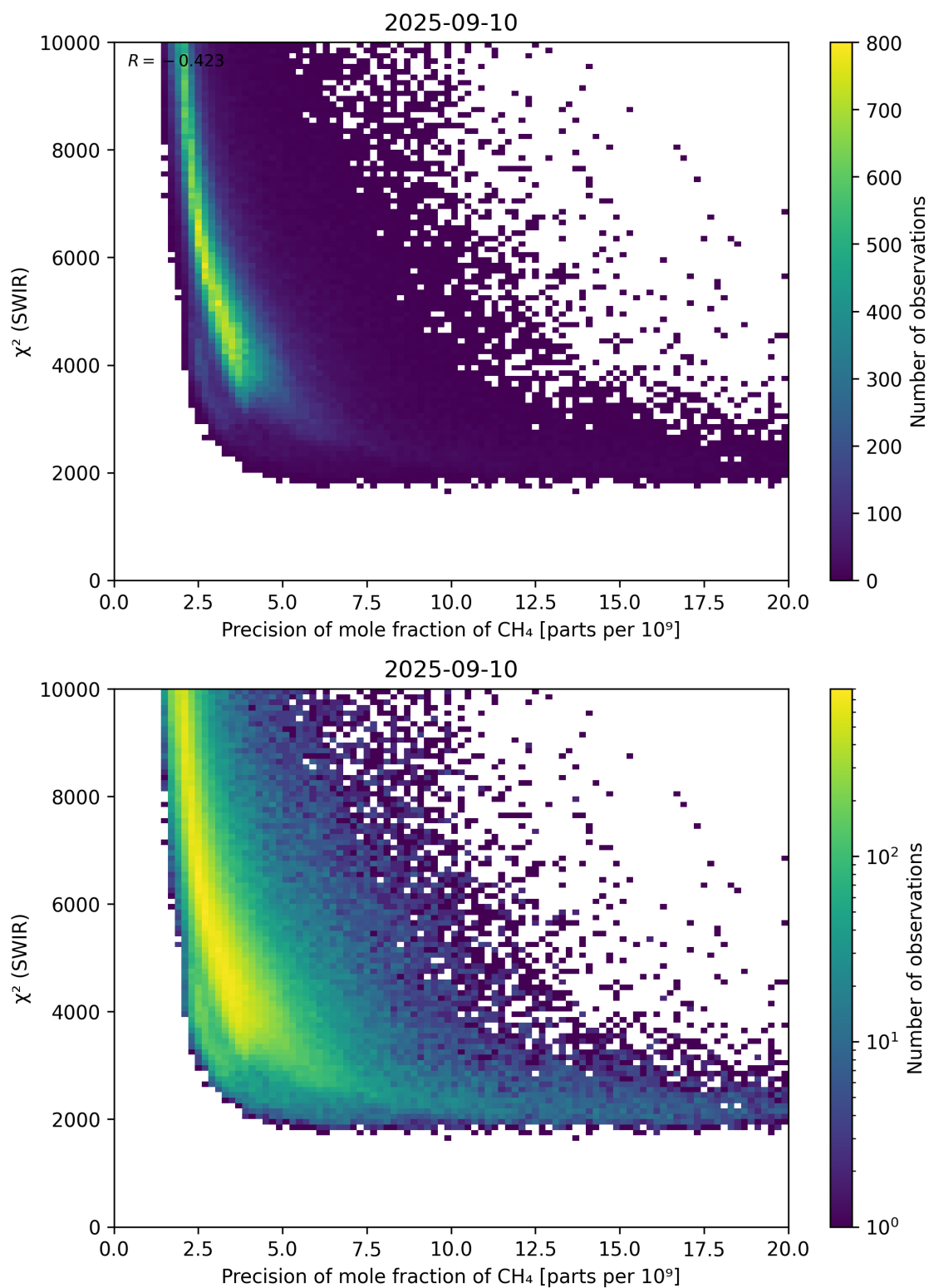
Figure 79: Scatter density plot of “Precision of mole fraction of \text{CH}_4 ” against “ \chi^2 (SWIR)” for 2025-09-10 to 2025-09-11.
