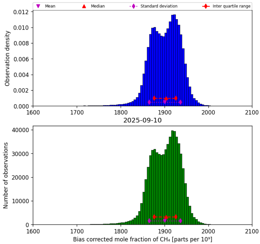
Figure 25: Histogram of “Bias corrected mole fraction of CH 4 ” for 2025-09-10 to 2025-09-11
