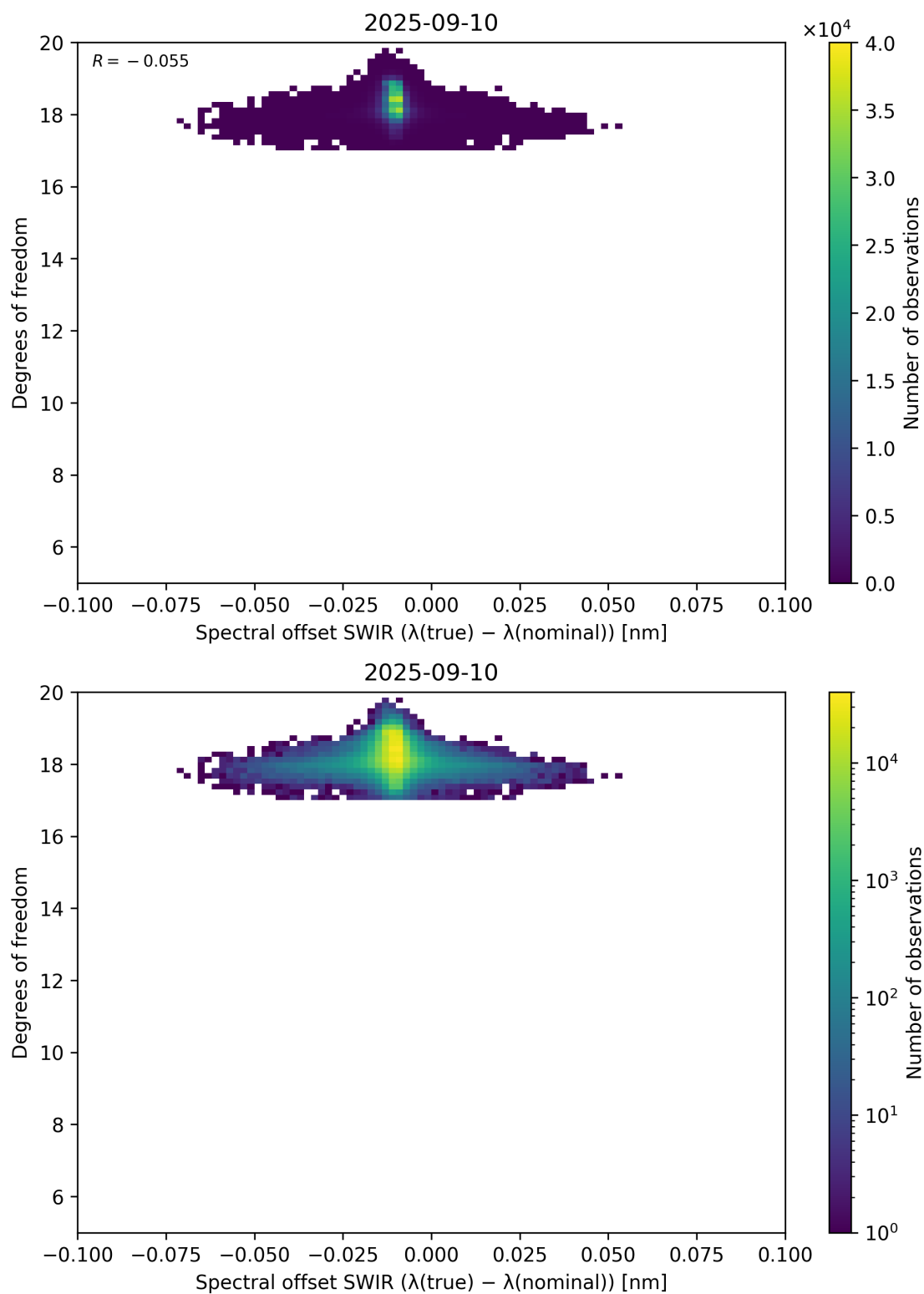
Figure 119: Scatter density plot of “Spectral offset SWIR ( \lambda_{\text{true}} - \lambda_{\text{nominal}} )” against “Degrees of freedom” for 2025-09-10 to 2025-09-11.
