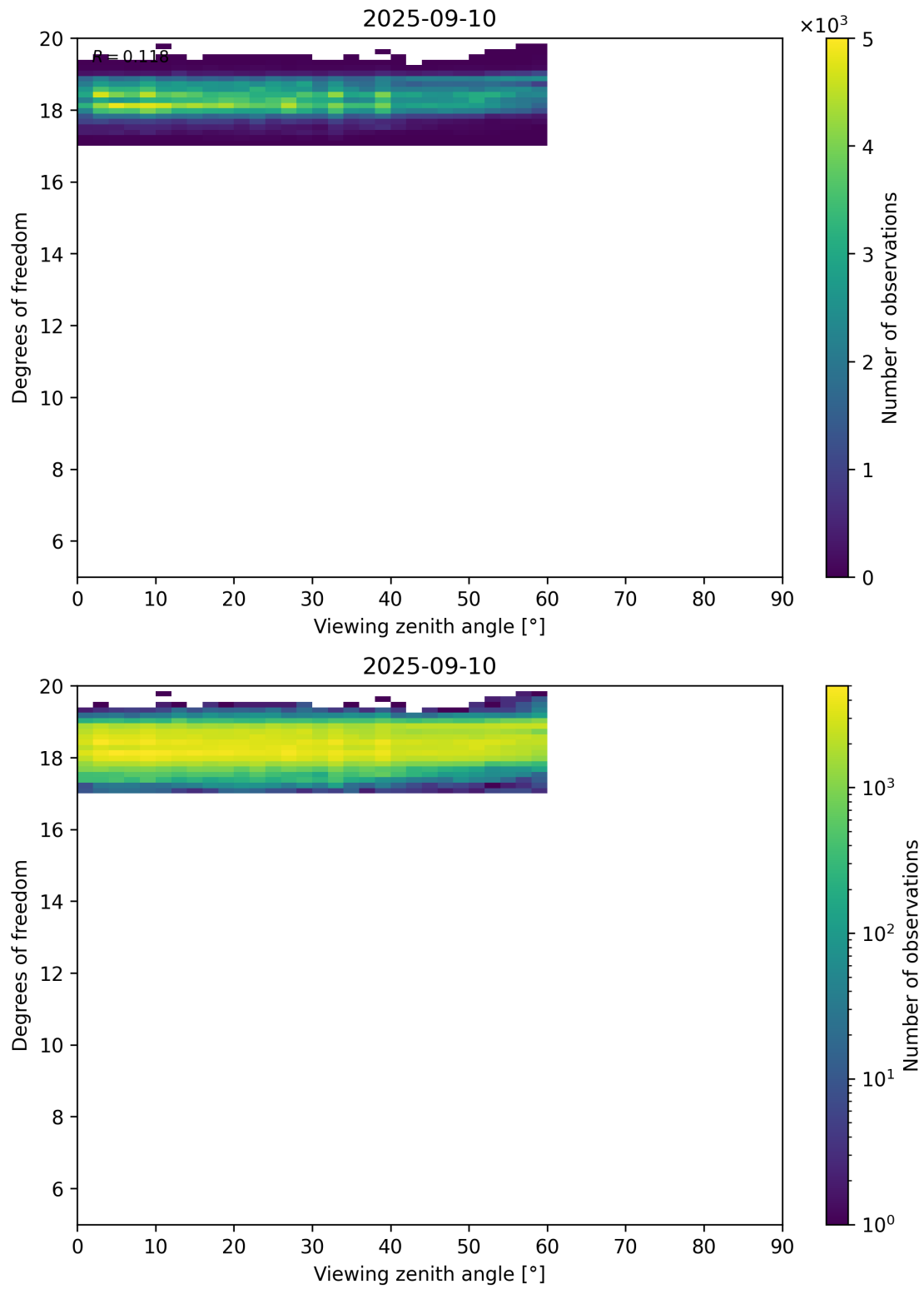
Figure 107: Scatter density plot of “Viewing zenith angle” against “Degrees of freedom” for 2025-09-10 to 2025-09-11.
