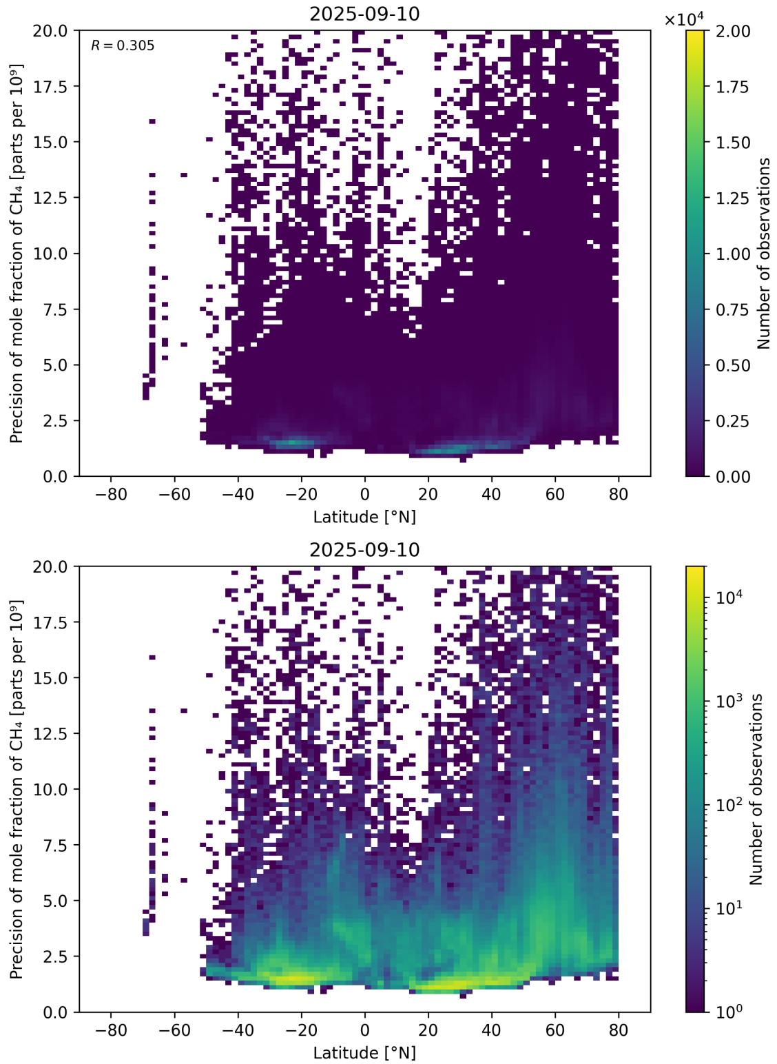
Figure 59: Scatter density plot of “Latitude” against “Precision of mole fraction of \text{CH}_4 ” for 2025-09-10 to 2025-09-11.
