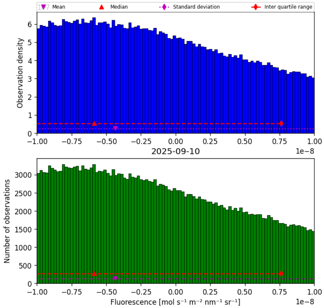
Figure 32: Histogram of “Fluorescence” for 2025-09-10 to 2025-09-11
