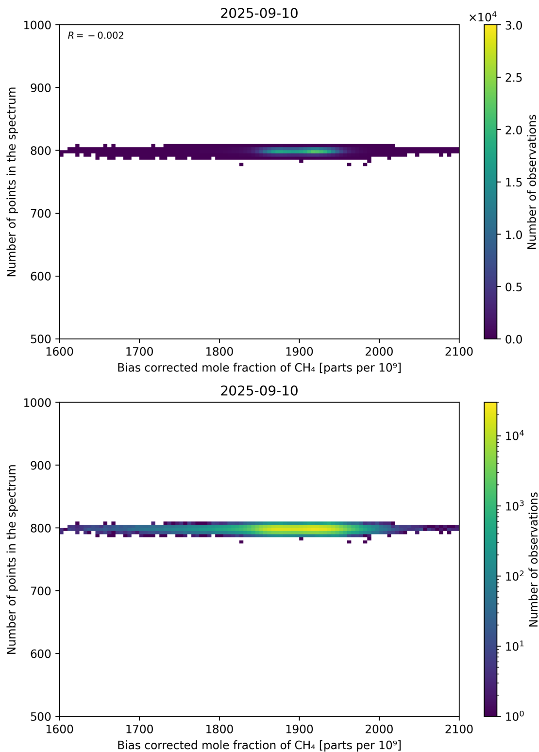
Figure 68: Scatter density plot of “Bias corrected mole fraction of CH 4 ” against “Number of points in the spectrum” for 2025-09-10 to 2025-09-11.
