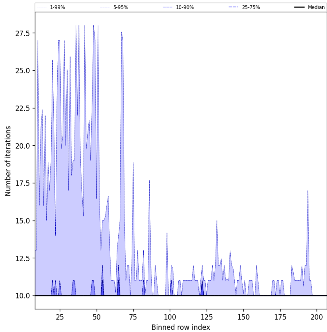
Figure 42: Along track statistics of “Number of iterations” for 2025-09-10 to 2025-09-11
