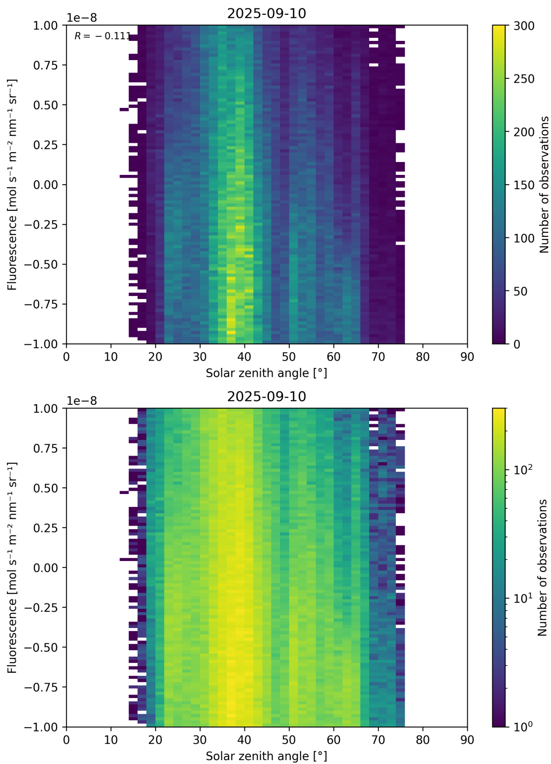
Figure 97: Scatter density plot of “Solar zenith angle” against “Fluorescence” for 2025-09-10 to 2025-09-11.
