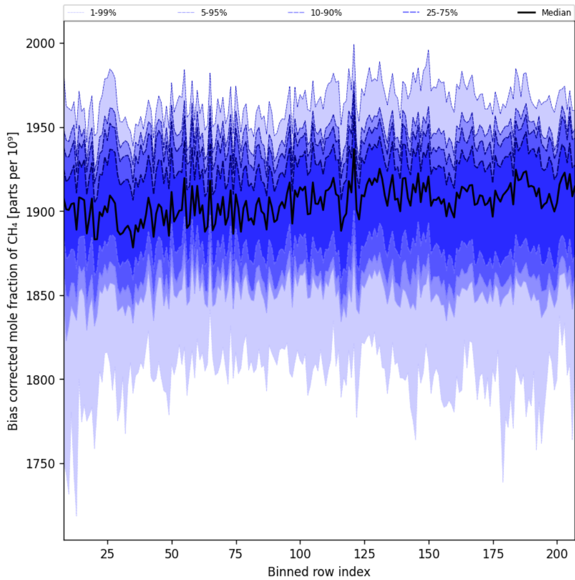
Figure 36: Along track statistics of “Bias corrected mole fraction of CH 4 ” for 2025-09-10 to 2025-09-11
