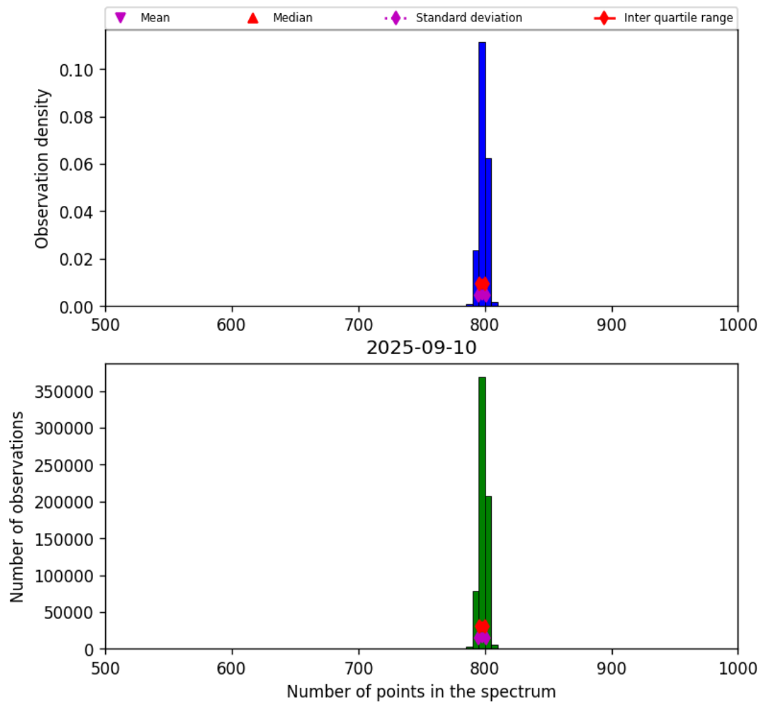
Figure 26: Histogram of “Number of points in the spectrum” for 2025-09-10 to 2025-09-11
