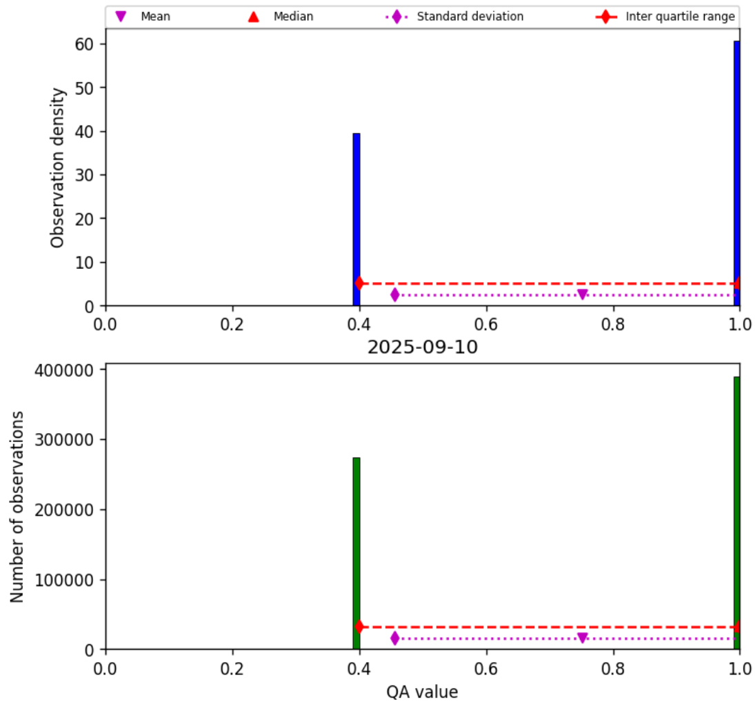
Figure 22: Histogram of “QA value” for 2025-09-10 to 2025-09-11
