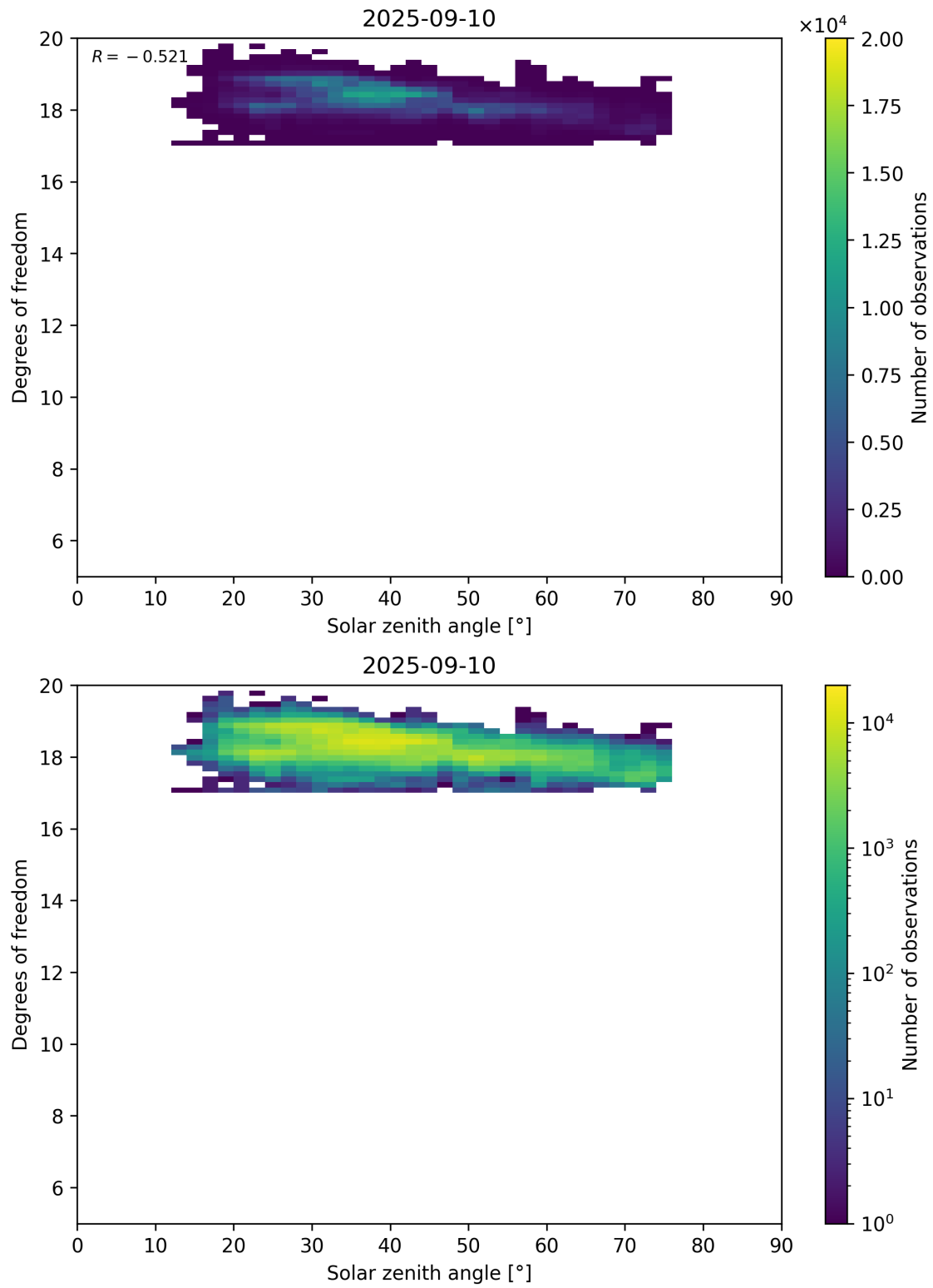
Figure 96: Scatter density plot of “Solar zenith angle” against “Degrees of freedom” for 2025-09-10 to 2025-09-11.
