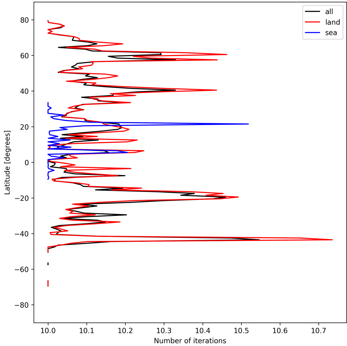
Figure 20: Zonal average of “Number of iterations” for 2025-09-10 to 2025-09-11.
