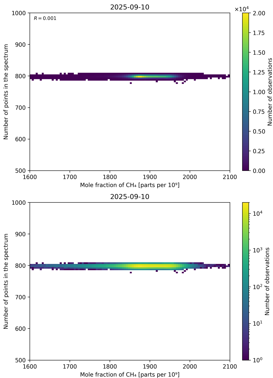
Figure 77: Scatter density plot of “Mole fraction of CH 4 ” against “Number of points in the spectrum” for 2025-09-10 to 2025-09-11.
