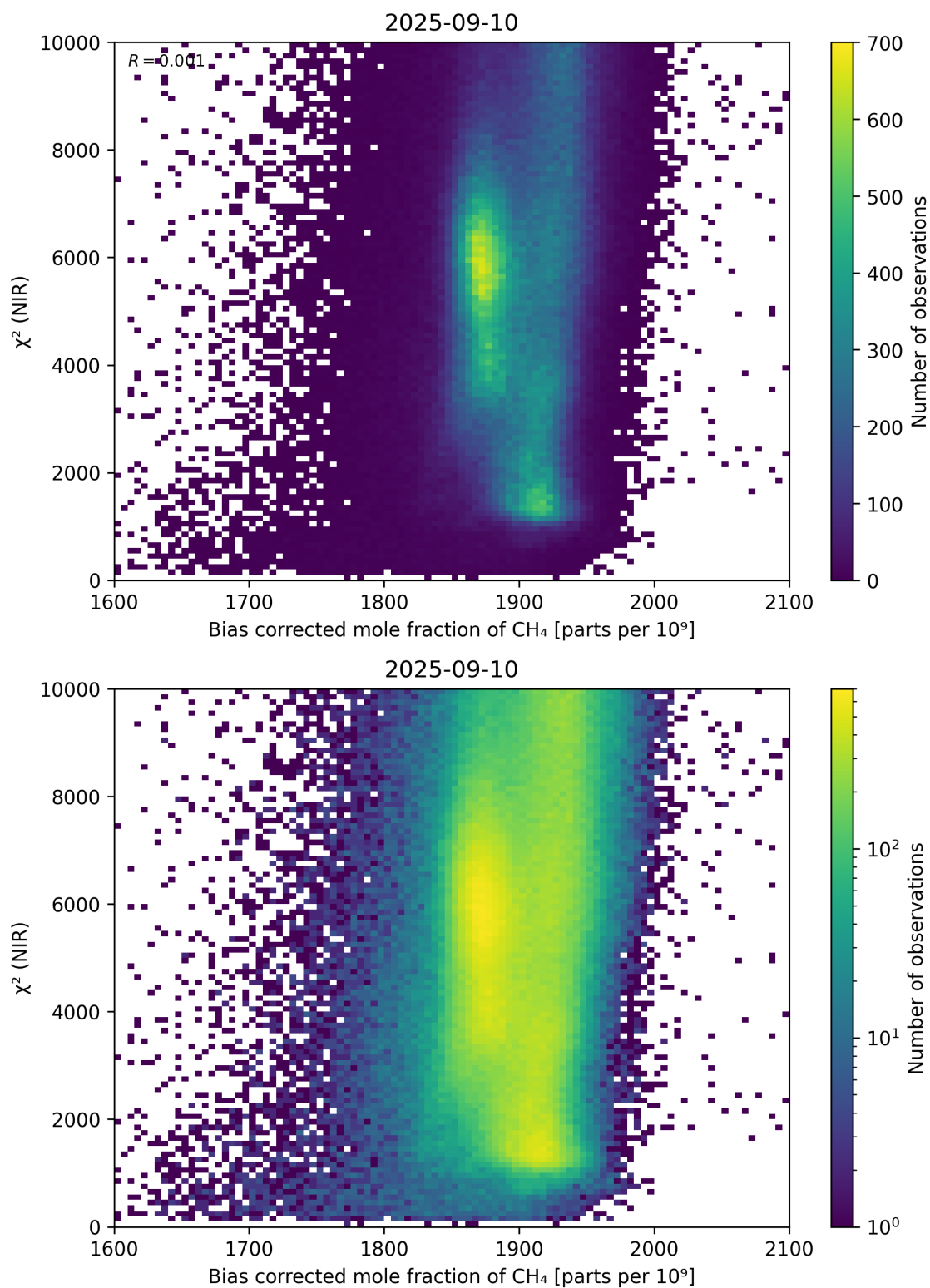
Figure 63: Scatter density plot of “Bias corrected mole fraction of \text{CH}_4 ” against “ \chi^2 (NIR)” for 2025-09-10 to 2025-09-11.
