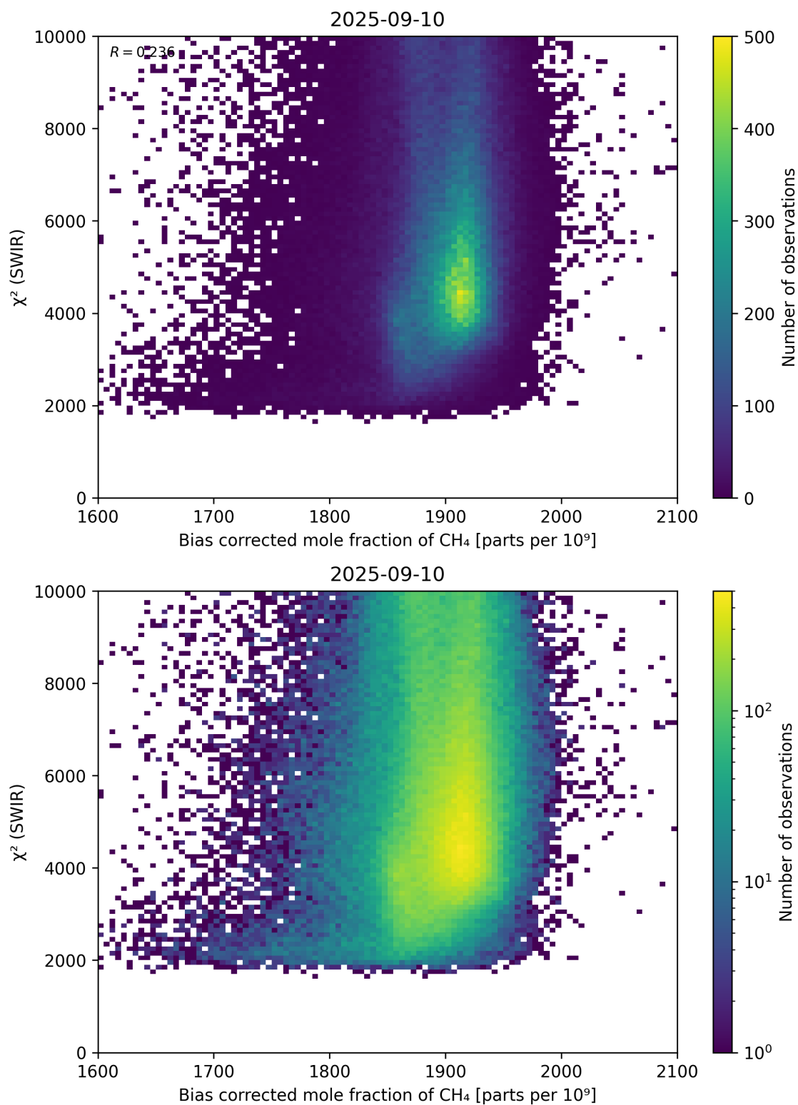
Figure 64: Scatter density plot of “Bias corrected mole fraction of \text{CH}_4 ” against “ \chi^2 (SWIR)” for 2025-09-10 to 2025-09-11.
