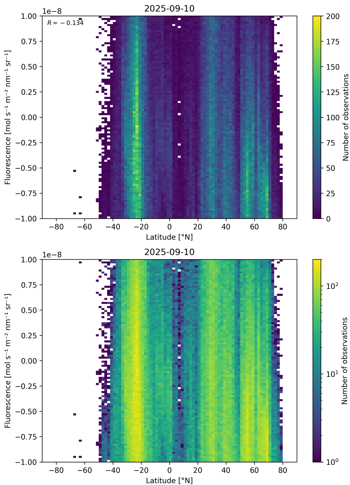
Figure 56: Scatter density plot of “Latitude” against “Fluorescence” for 2025-09-10 to 2025-09-11.
