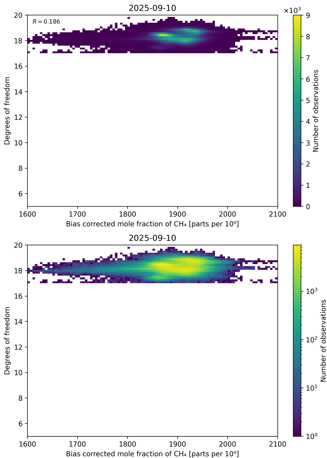
Figure 65: Scatter density plot of “Bias corrected mole fraction of CH 4 ” against “Degrees of freedom” for 2025-09-10 to 2025-09-11.
