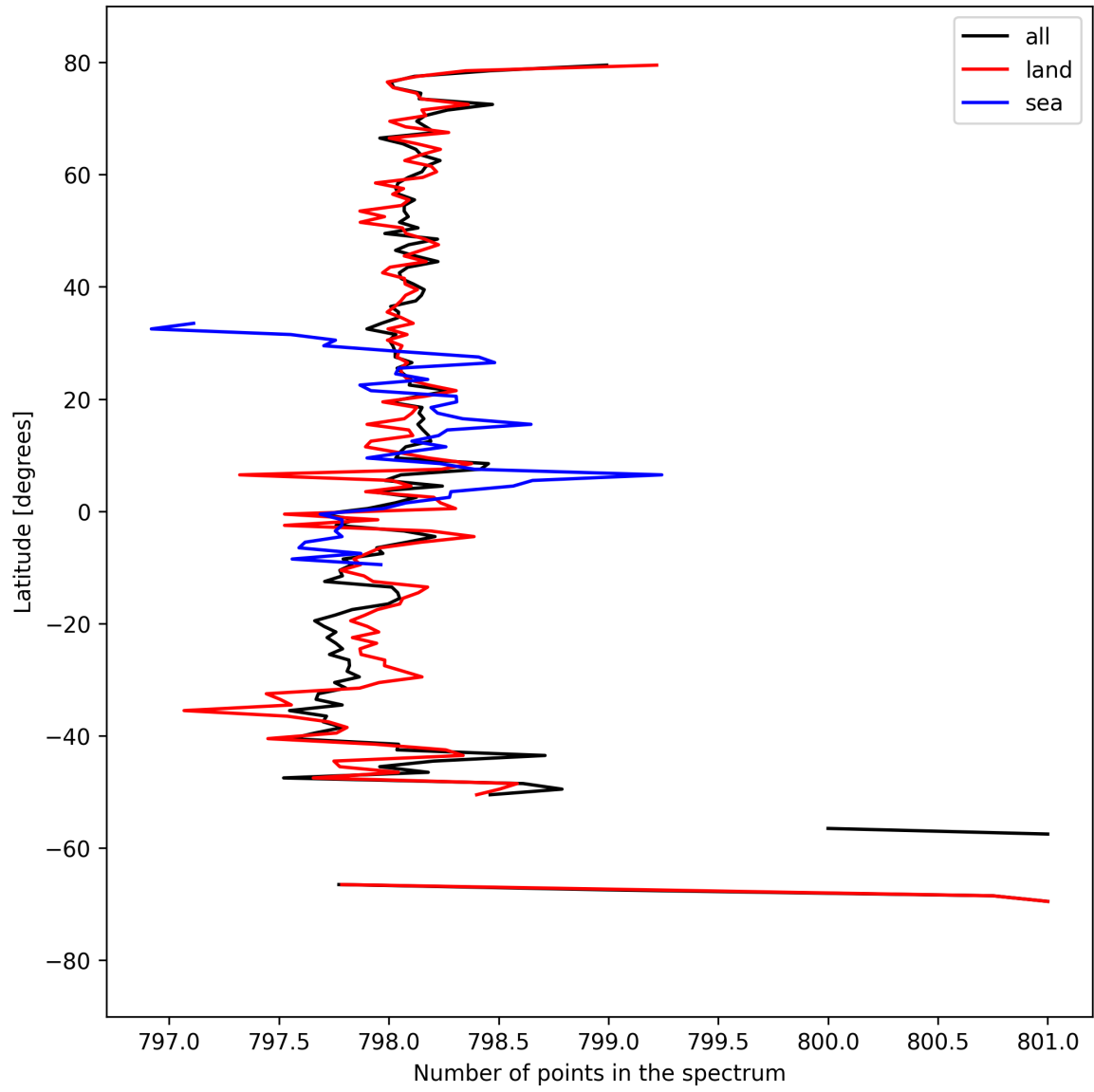
Figure 15: Zonal average of “Number of points in the spectrum” for 2025-09-10 to 2025-09-11.
