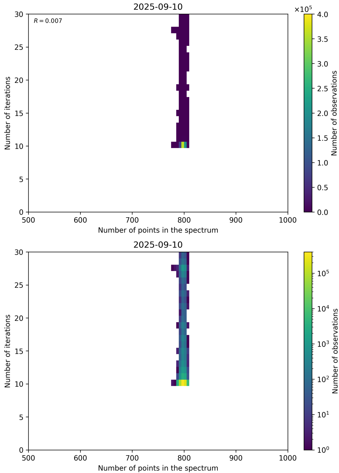
Figure 92: Scatter density plot of “Number of points in the spectrum” against “Number of iterations” for 2025-09-10 to 2025-09-11.
