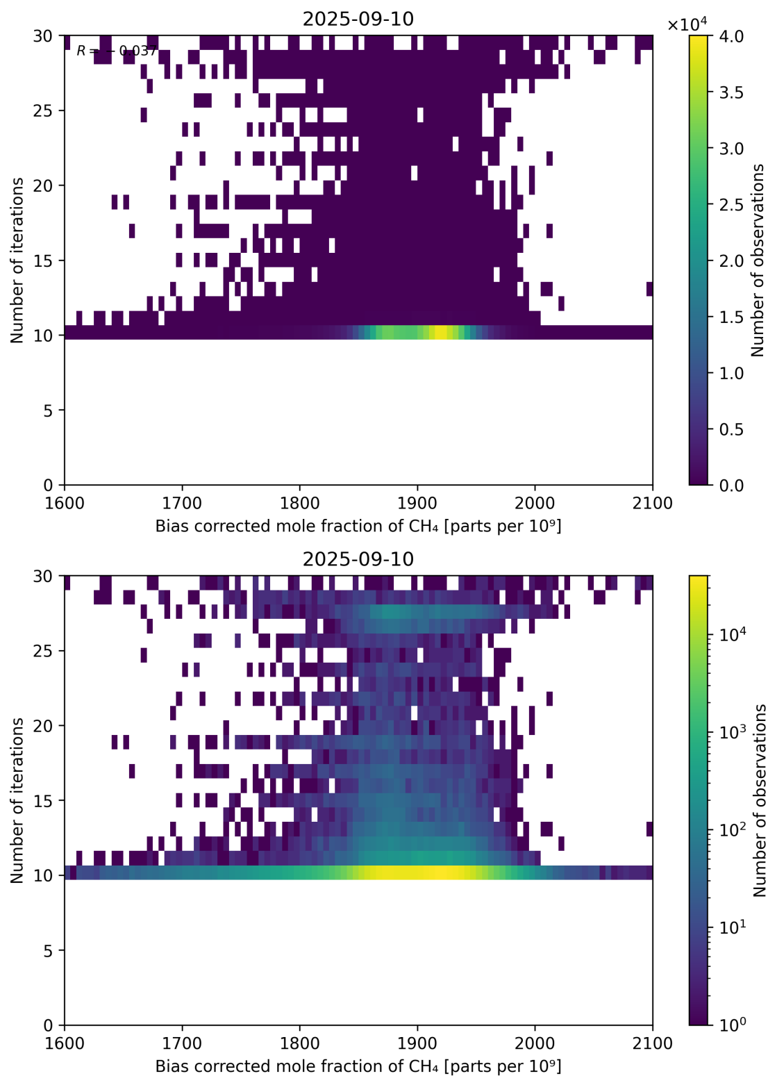
Figure 67: Scatter density plot of “Bias corrected mole fraction of CH 4 ” against “Number of iterations” for 2025-09-10 to 2025-09-11.
