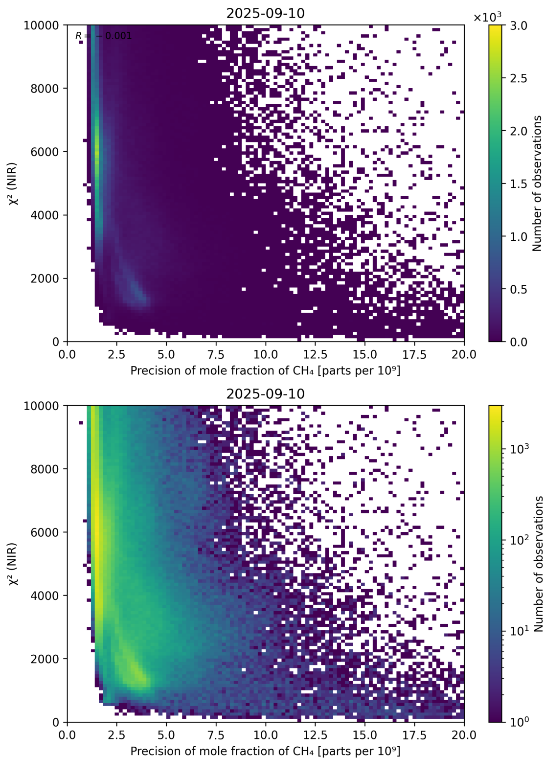
Figure 78: Scatter density plot of “Precision of mole fraction of CH 4 ” against “ \chi^2 (NIR)” for 2025-09-10 to 2025-09-11.
