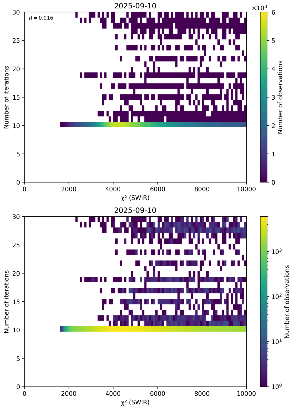
Figure 50: Scatter density plot of “ \chi^2 (SWIR)” against “Number of iterations” for 2025-09-10 to 2025-09-11.
