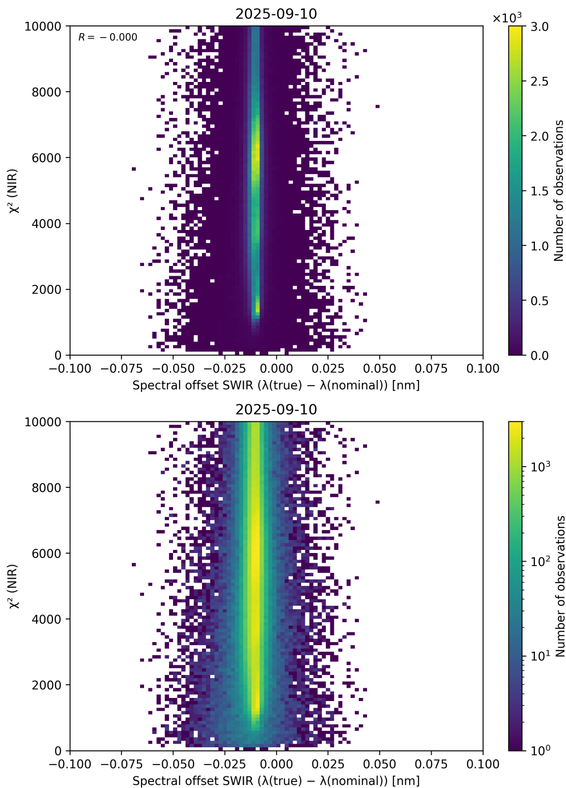
Figure 117: Scatter density plot of “Spectral offset SWIR ( \lambda_{\text{true}} - \lambda_{\text{nominal}} )” against “ \chi^2 (NIR)” for 2025-09-10 to 2025-09-11.
