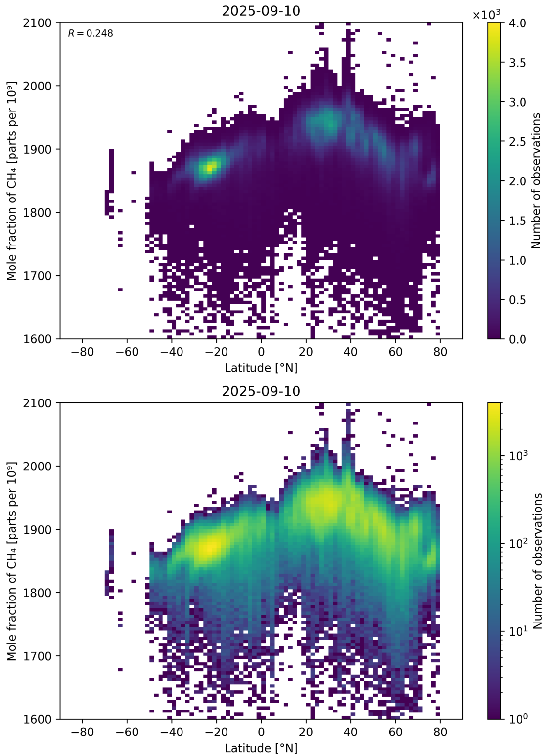
Figure 57: Scatter density plot of “Latitude” against “Mole fraction of \text{CH}_4 ” for 2025-09-10 to 2025-09-11.
