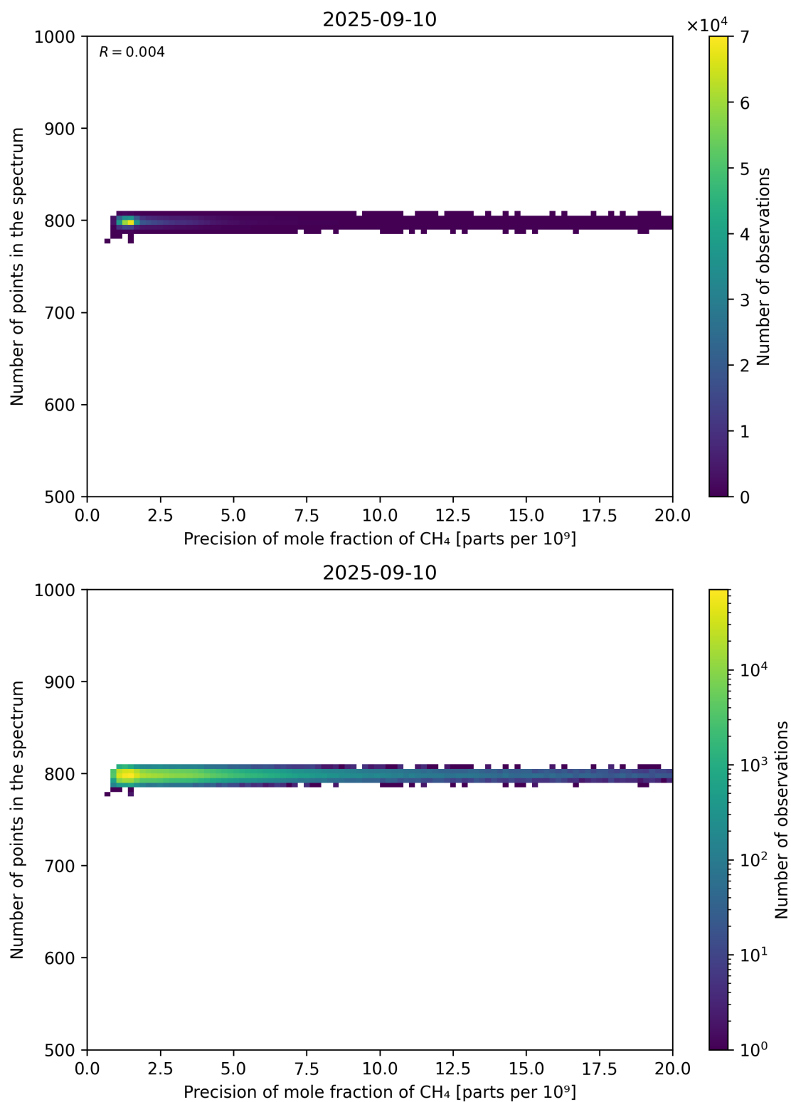
Figure 84: Scatter density plot of “Precision of mole fraction of CH 4 ” against “Number of points in the spectrum” for 2025-09-10 to 2025-09-11.
