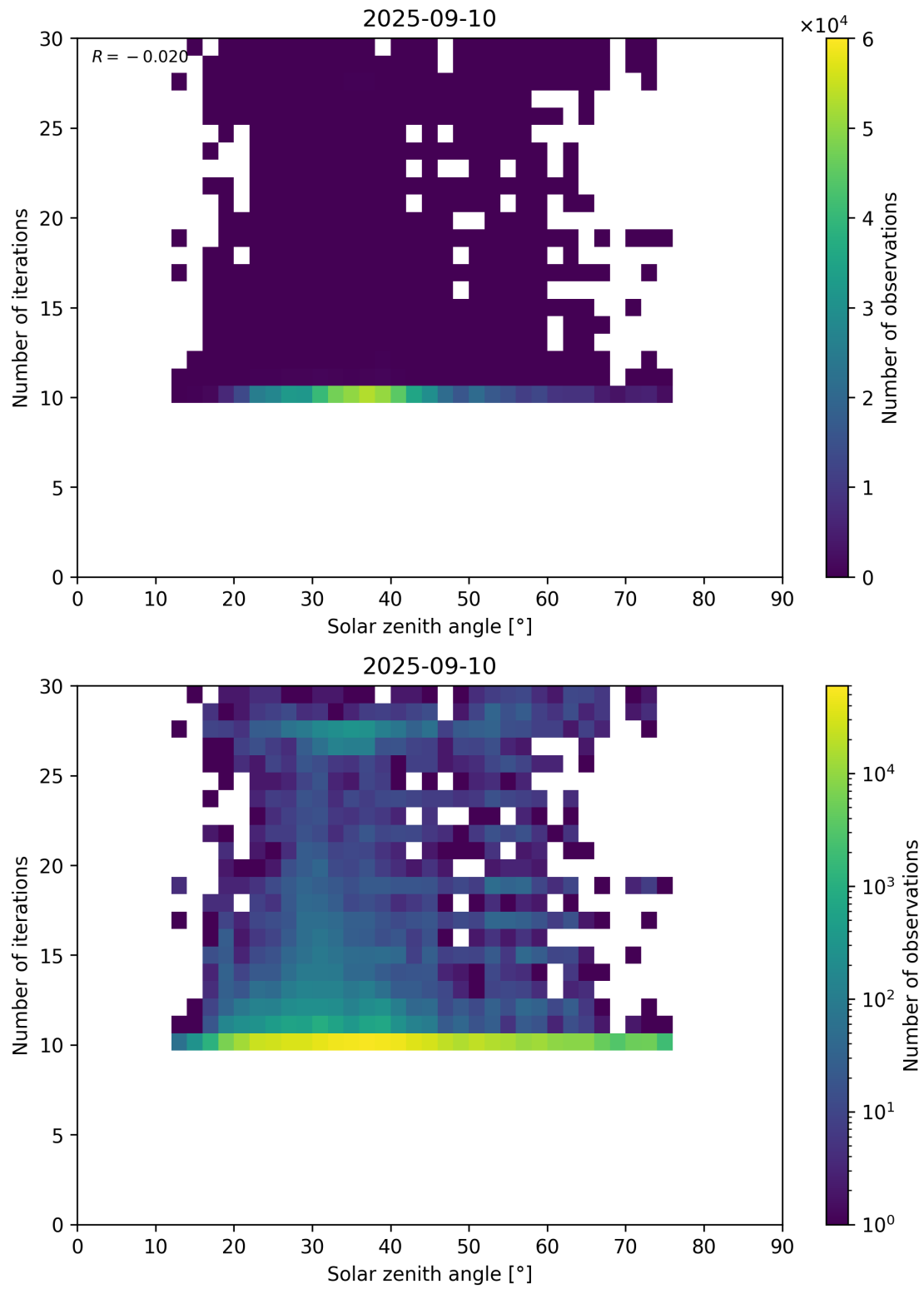
Figure 102: Scatter density plot of “Solar zenith angle” against “Number of iterations” for 2025-09-10 to 2025-09-11.
