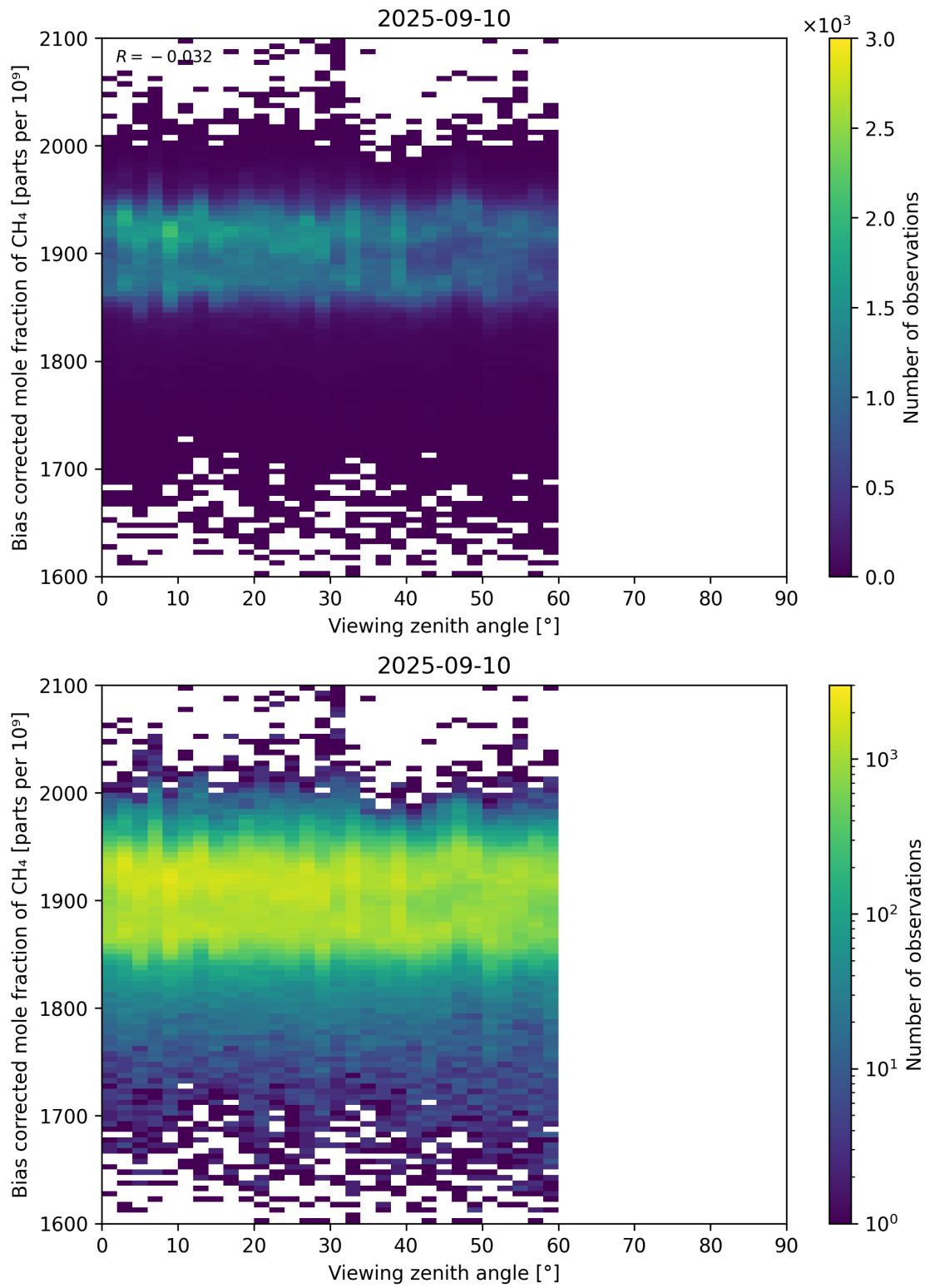
Figure 111: Scatter density plot of “Viewing zenith angle” against “Bias corrected mole fraction of CH 4 ” for 2025-09-10 to 2025-09-11.
