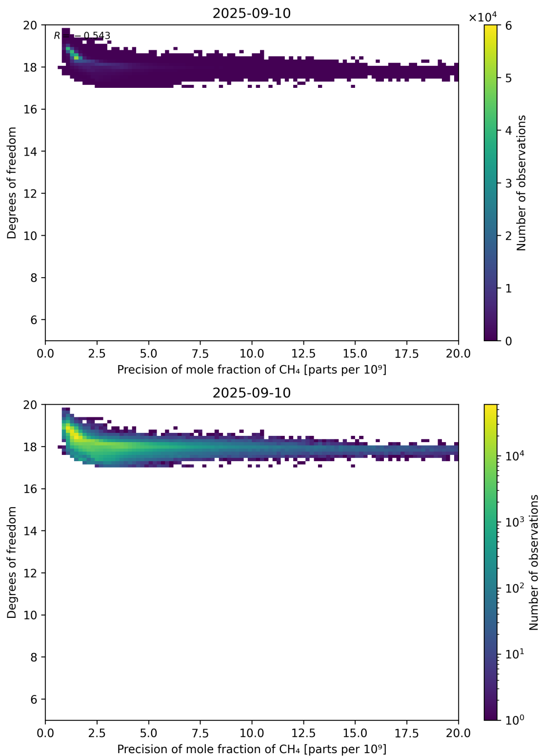
Figure 80: Scatter density plot of “Precision of mole fraction of CH 4 ” against “Degrees of freedom” for 2025-09-10 to 2025-09-11.
