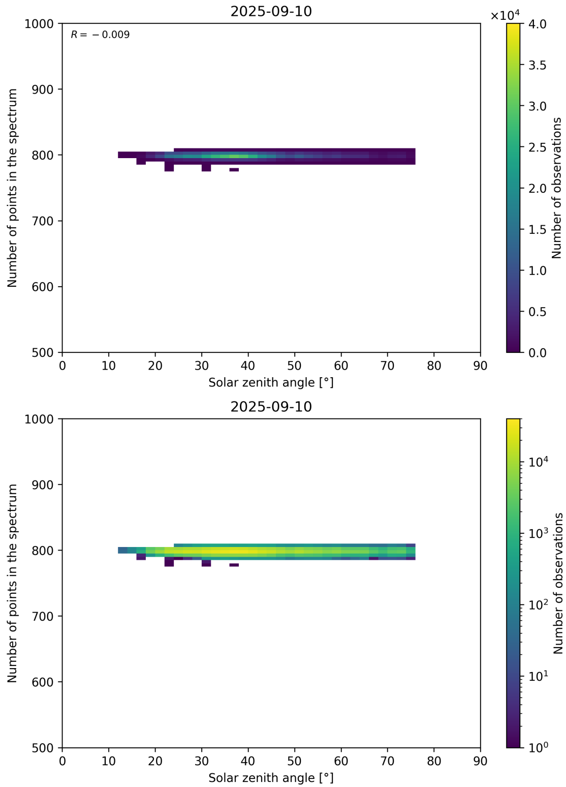
Figure 103: Scatter density plot of “Solar zenith angle” against “Number of points in the spectrum” for 2025-09-10 to 2025-09-11.
