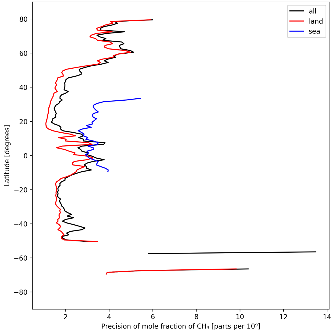
Figure 13: Zonal average of “Precision of mole fraction of CH 4 ” for 2025-09-10 to 2025-09-11.
