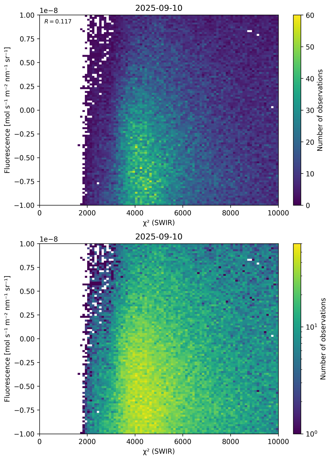
Figure 49: Scatter density plot of “ \chi^2 (SWIR)” against “Fluorescence” for 2025-09-10 to 2025-09-11.
