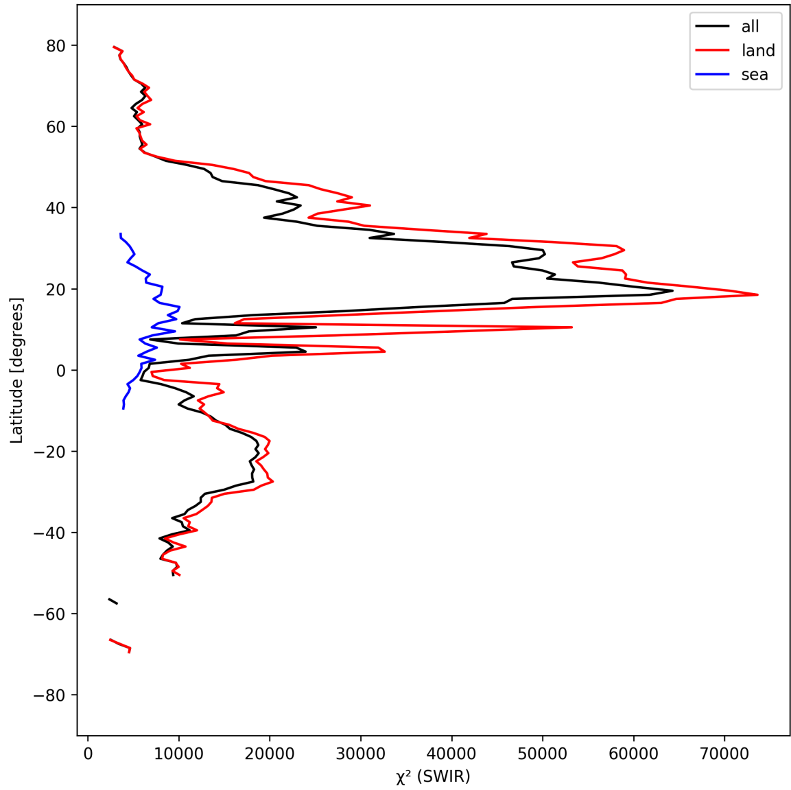
Figure 17: Zonal average of “ \chi^2 (SWIR)” for 2025-09-10 to 2025-09-11.
