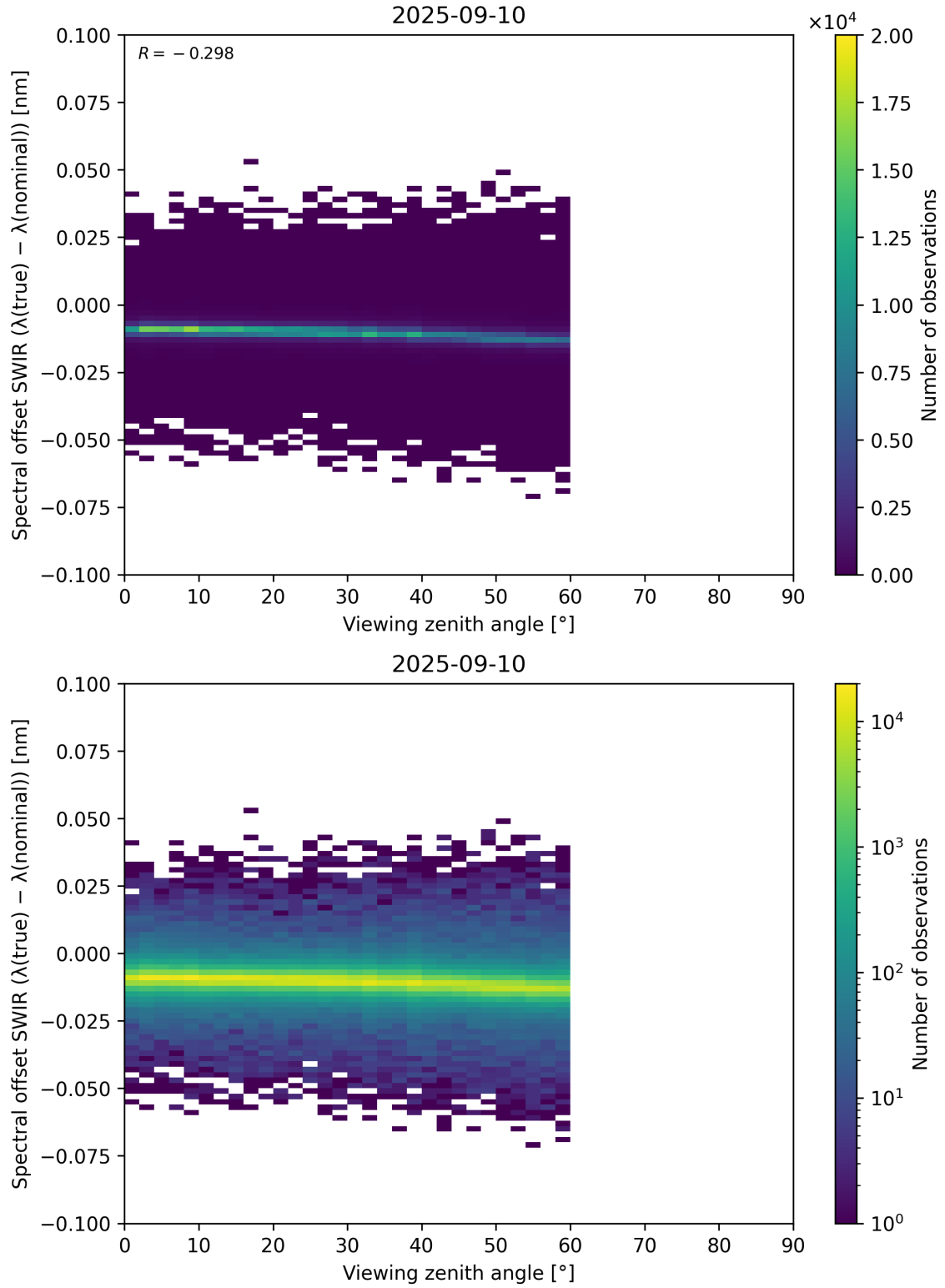
Figure 116: Scatter density plot of “Viewing zenith angle” against “Spectral offset SWIR ( \lambda_{\text{true}} - \lambda_{\text{nominal}} )” for 2025-09-10 to 2025-09-11.
