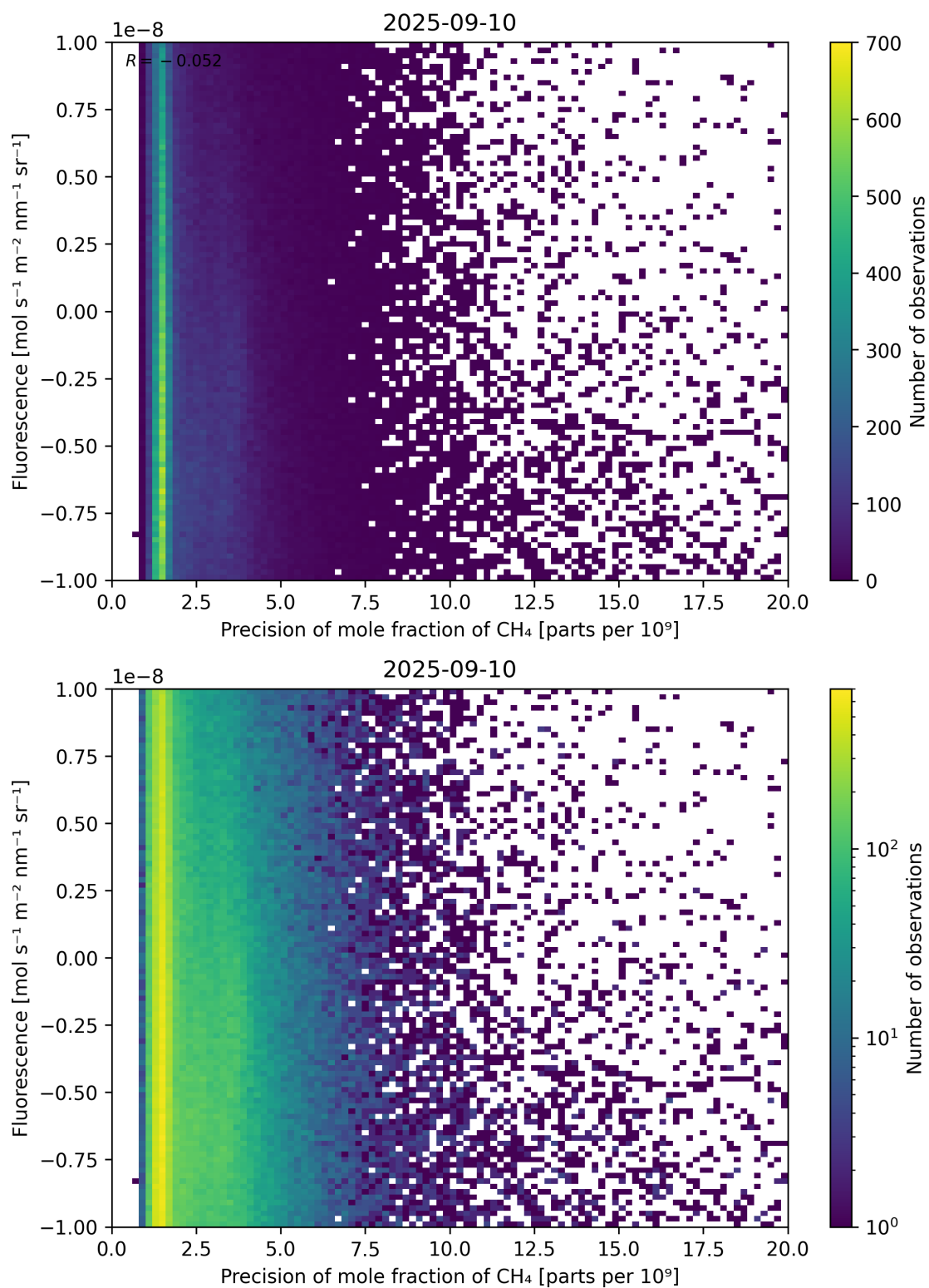
Figure 81: Scatter density plot of “Precision of mole fraction of \text{CH}_4 ” against “Fluorescence” for 2025-09-10 to 2025-09-11.
