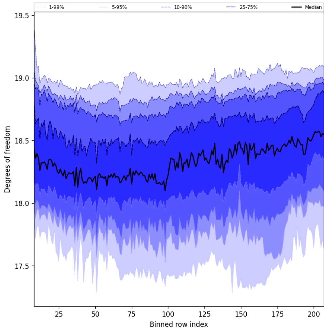
Figure 41: Along track statistics of “Degrees of freedom” for 2025-09-10 to 2025-09-11
