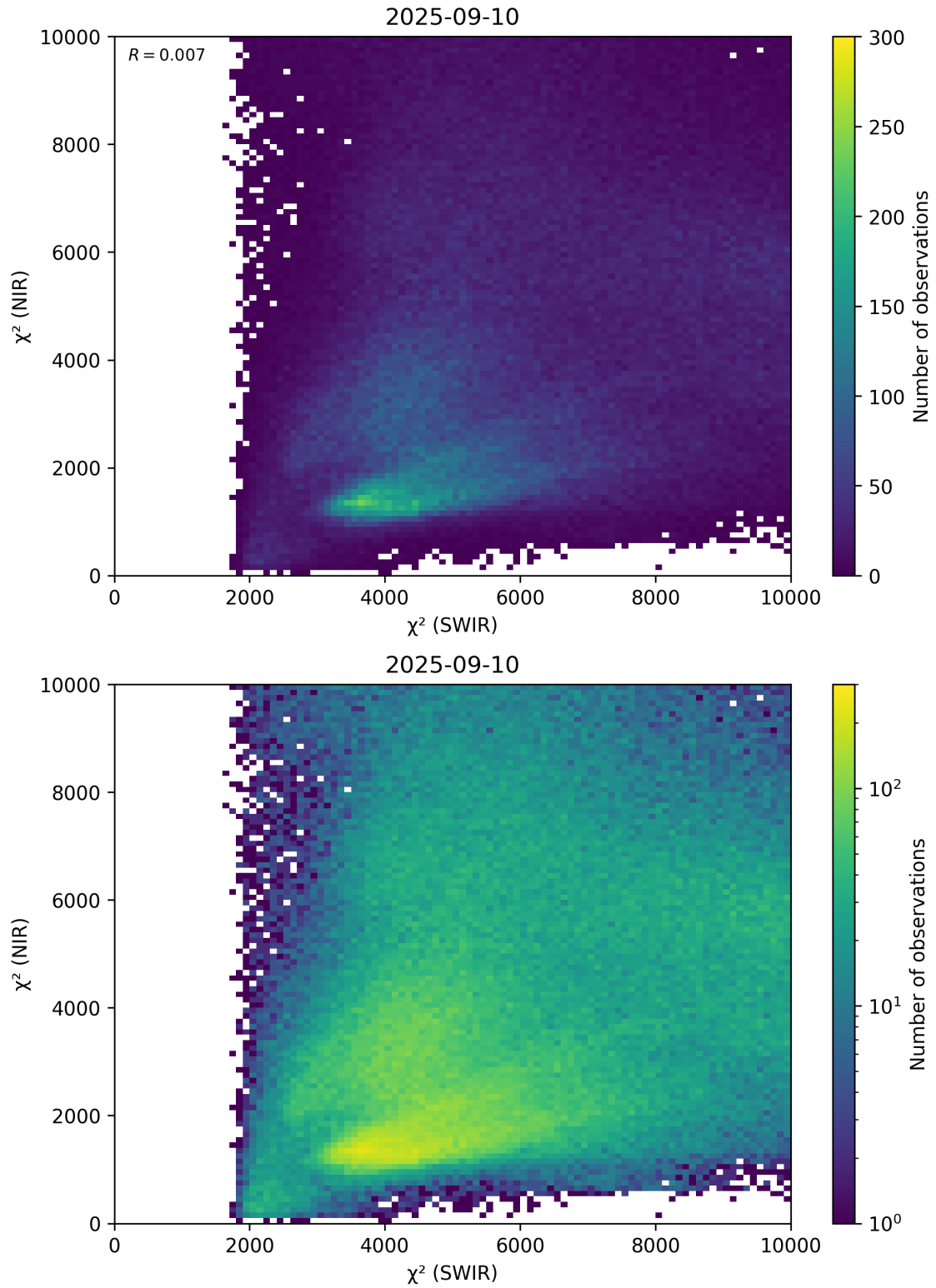
Figure 47: Scatter density plot of “ \chi^2 (SWIR)” against “ \chi^2 (NIR)” for 2025-09-10 to 2025-09-11.
