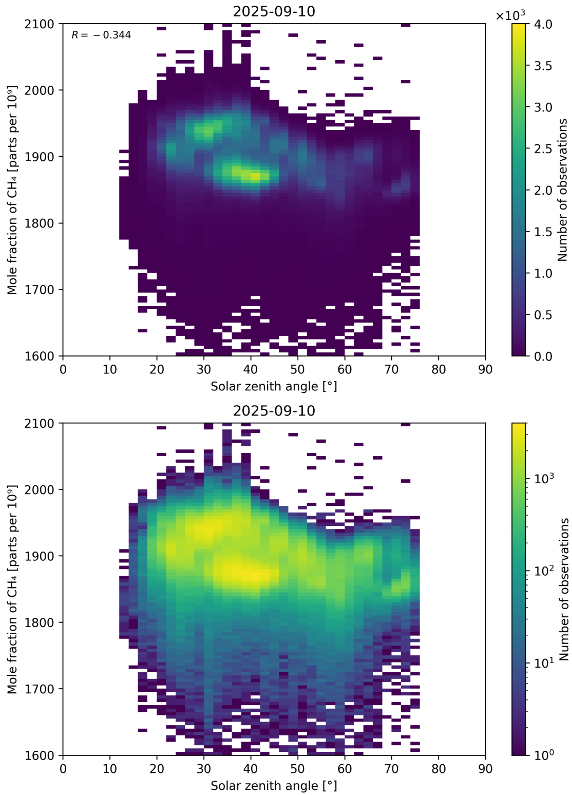
Figure 99: Scatter density plot of “Solar zenith angle” against “Mole fraction of CH 4 ” for 2025-09-10 to 2025-09-11.
