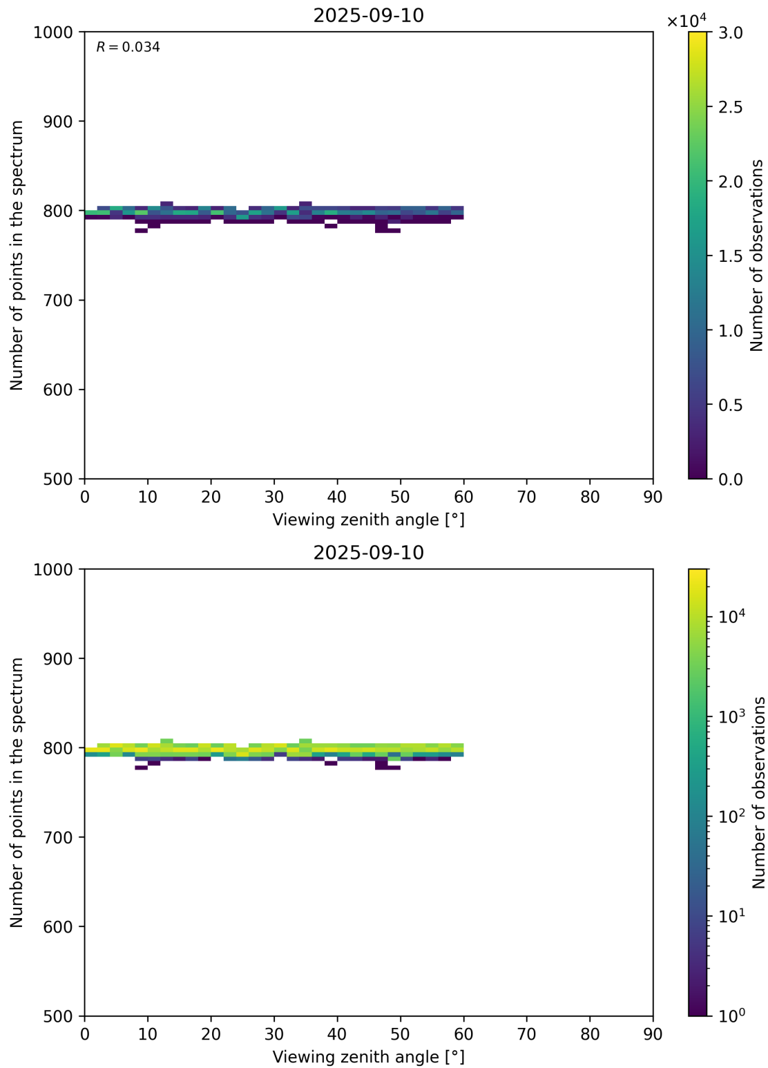
Figure 114: Scatter density plot of “Viewing zenith angle” against “Number of points in the spectrum” for 2025-09-10 to 2025-09-11.
