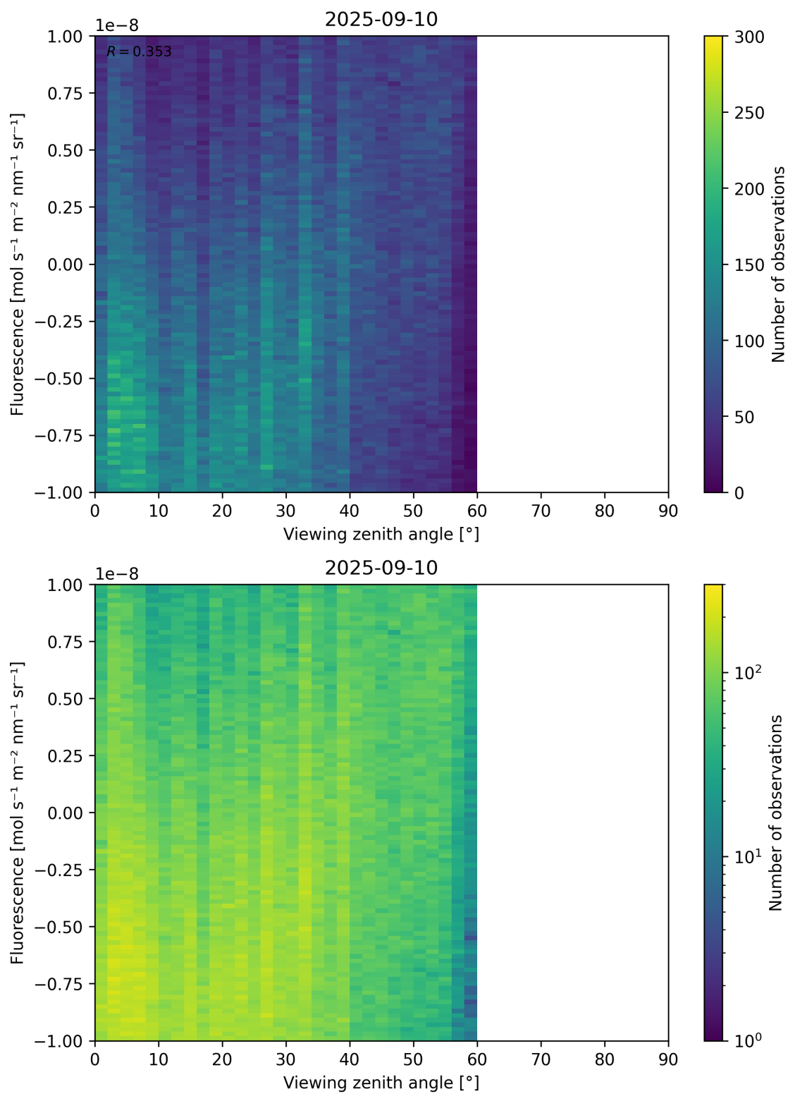
Figure 108: Scatter density plot of “Viewing zenith angle” against “Fluorescence” for 2025-09-10 to 2025-09-11.
