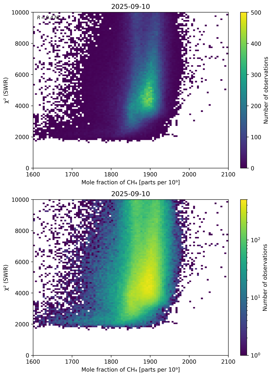
Figure 71: Scatter density plot of “Mole fraction of \text{CH}_4 ” against “ \chi^2 (SWIR)” for 2025-09-10 to 2025-09-11.
