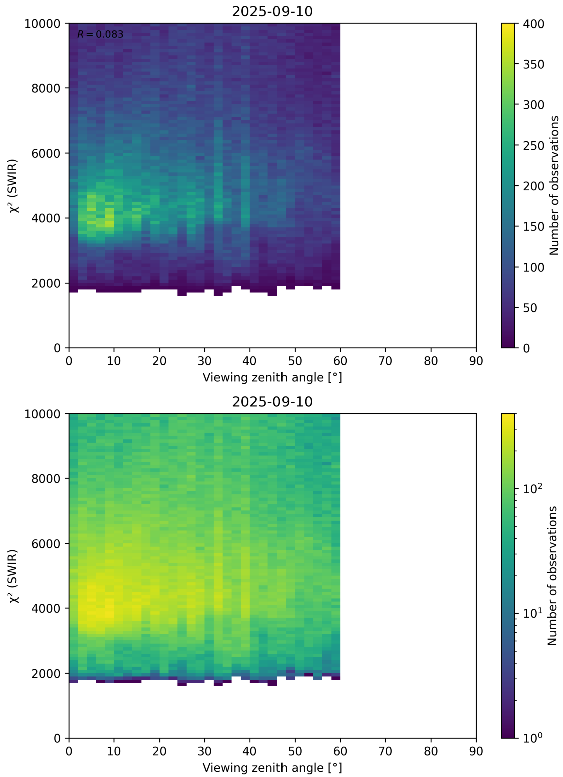
Figure 106: Scatter density plot of “Viewing zenith angle” against “ \chi^2 (SWIR)” for 2025-09-10 to 2025-09-11.
