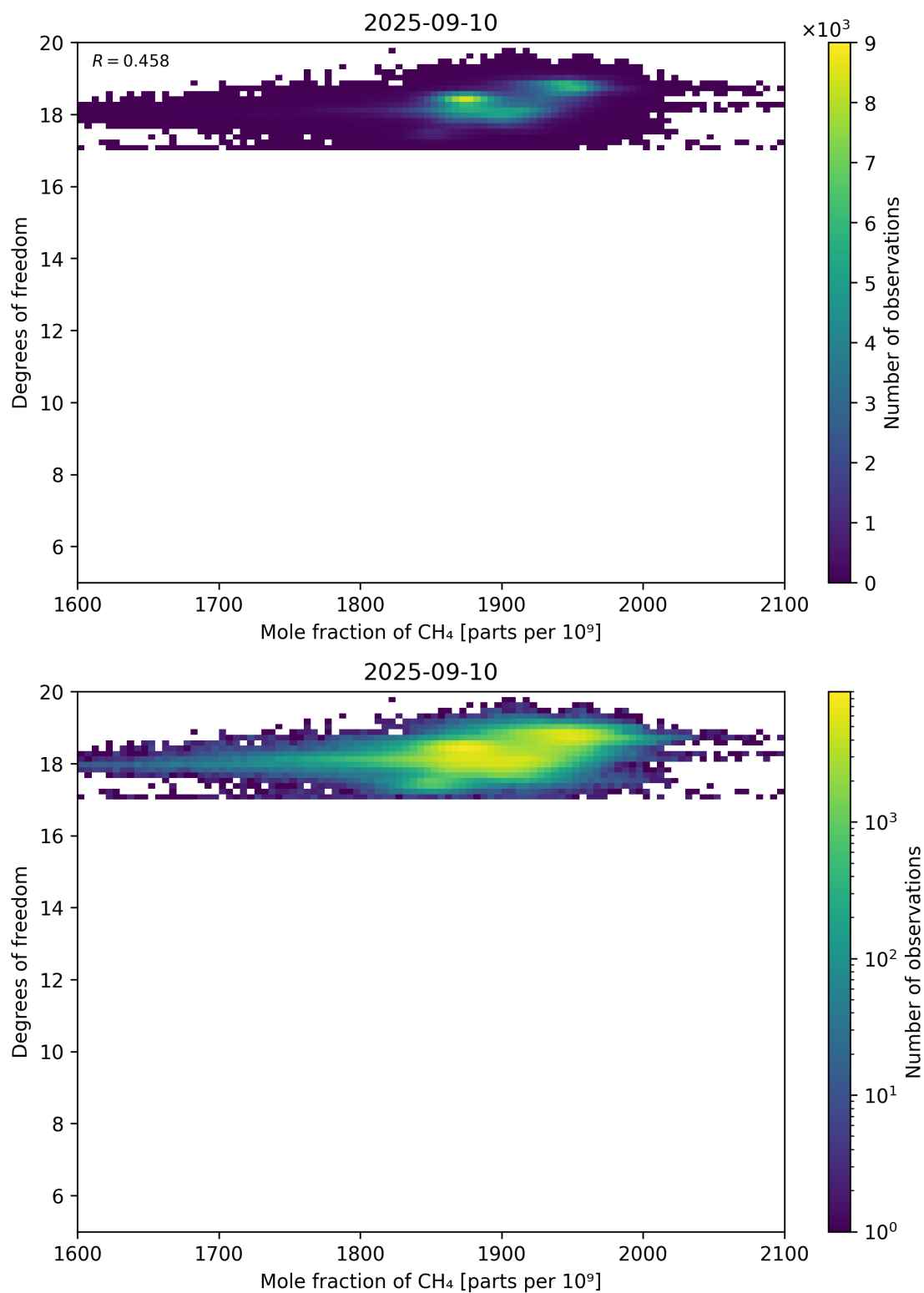
Figure 72: Scatter density plot of “Mole fraction of CH 4 ” against “Degrees of freedom” for 2025-09-10 to 2025-09-11.
