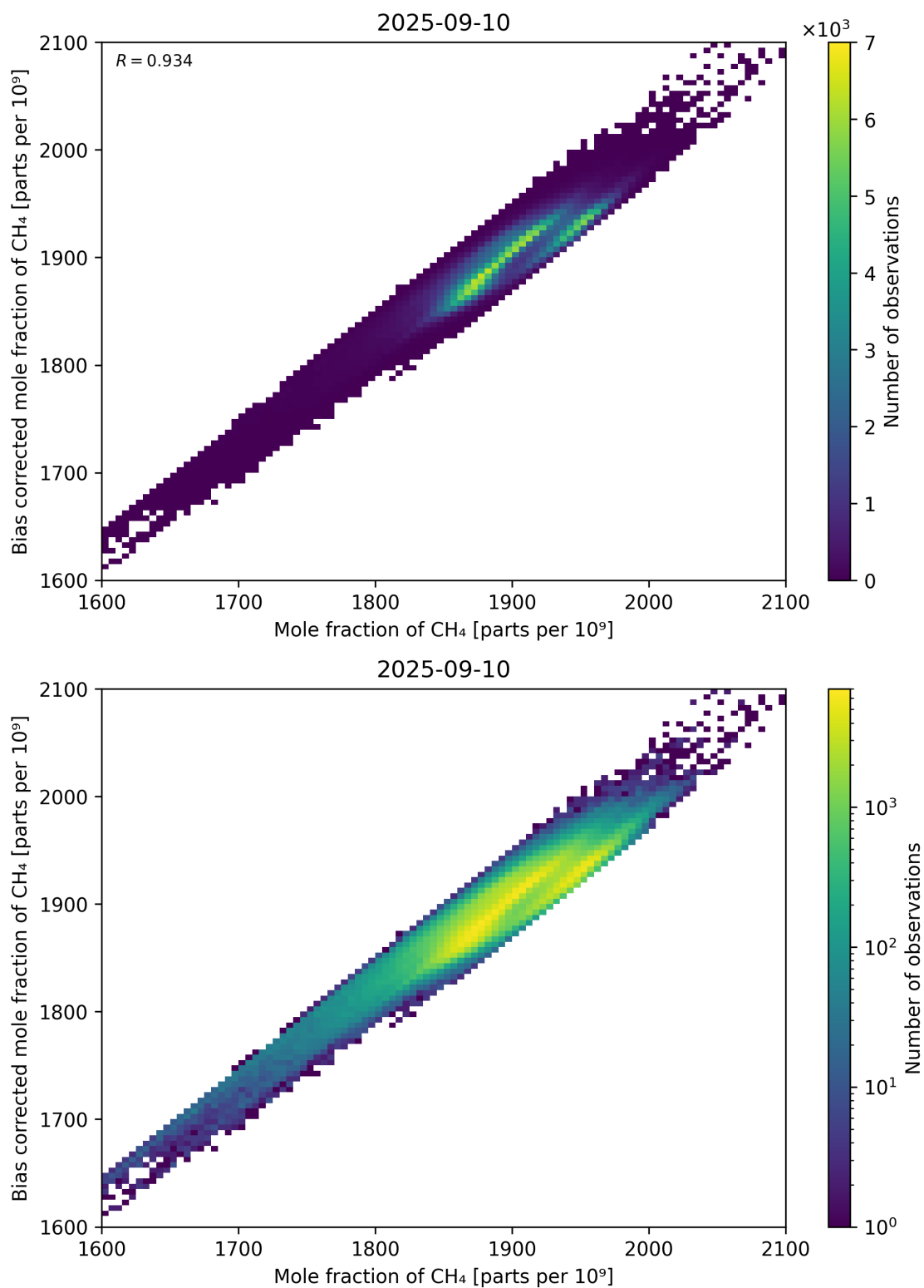
Figure 74: Scatter density plot of “Mole fraction of CH 4 ” against “Bias corrected mole fraction of CH 4 ” for 2025-09-10 to 2025-09-11.
