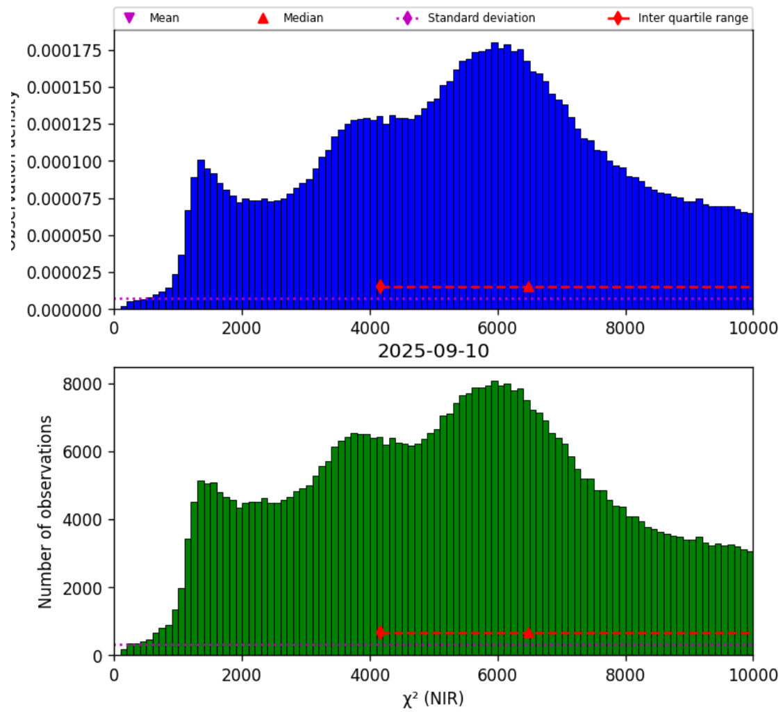
Figure 29: Histogram of “ \chi^2 (NIR)” for 2025-09-10 to 2025-09-11
