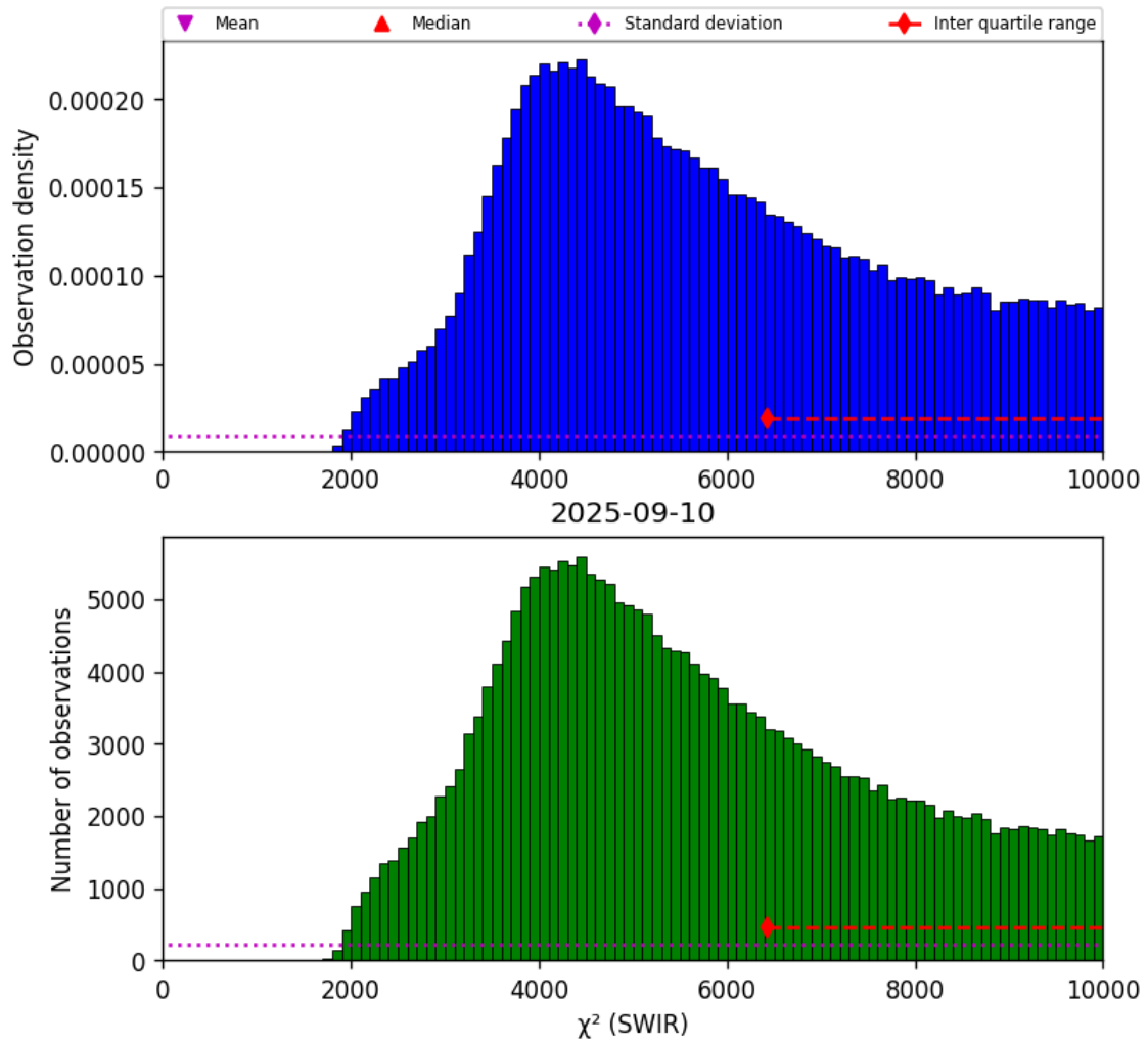
Figure 28: Histogram of “ \chi^2 (SWIR)” for 2025-09-10 to 2025-09-11
