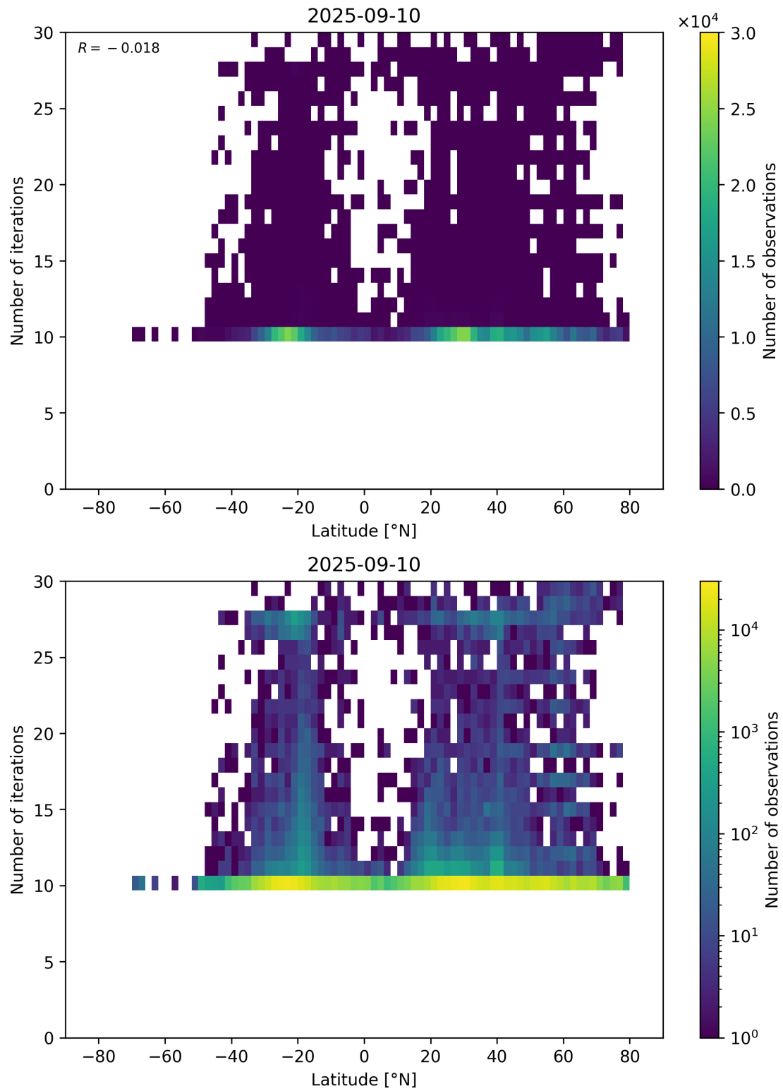
Figure 60: Scatter density plot of “Latitude” against “Number of iterations” for 2025-09-10 to 2025-09-11.
