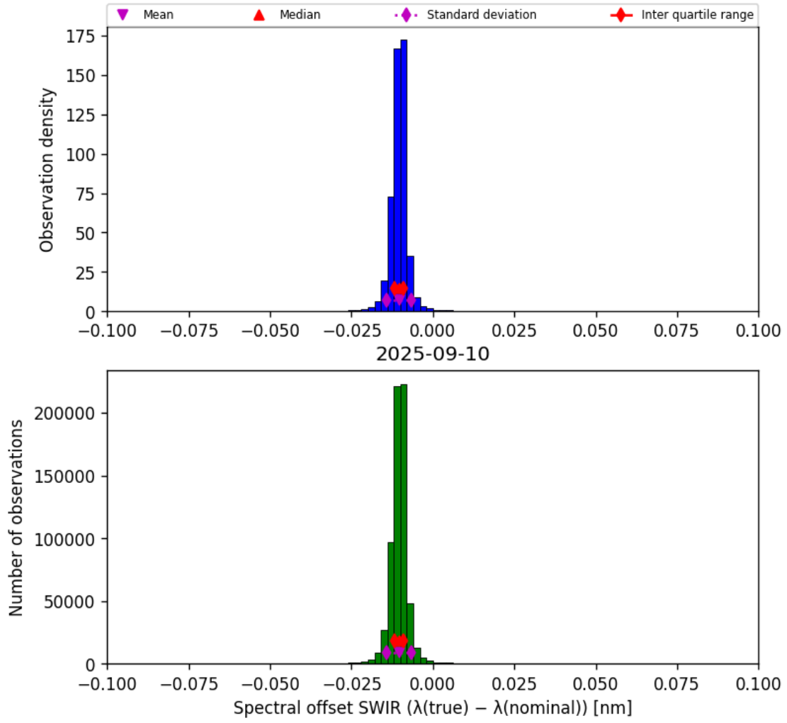
Figure 27: Histogram of “Spectral offset SWIR ( \lambda_{\text{true}} - \lambda_{\text{nominal}} )” for 2025-09-10 to 2025-09-11
