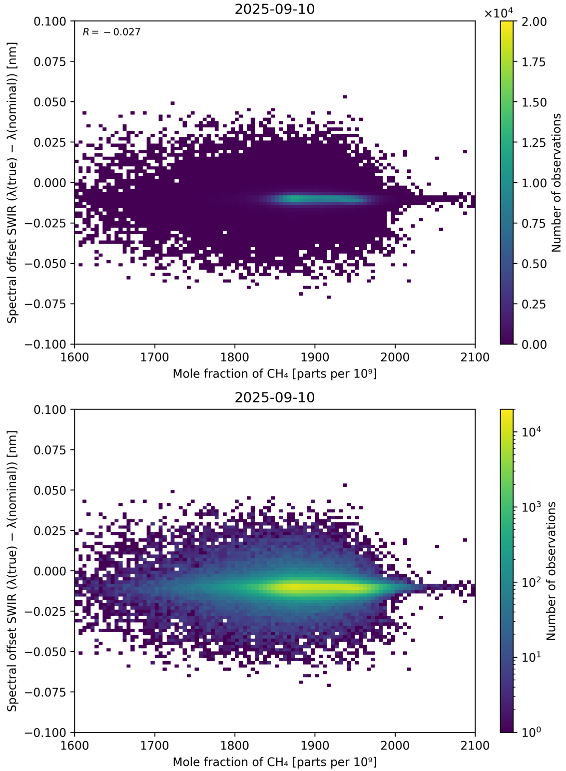
Figure 86: Scatter density plot of “Mole fraction of CH 4 ” against “Spectral offset SWIR ( \lambda_{\text{true}} - \lambda_{\text{nominal}} )” for 2025-09-10 to 2025-09-11.
