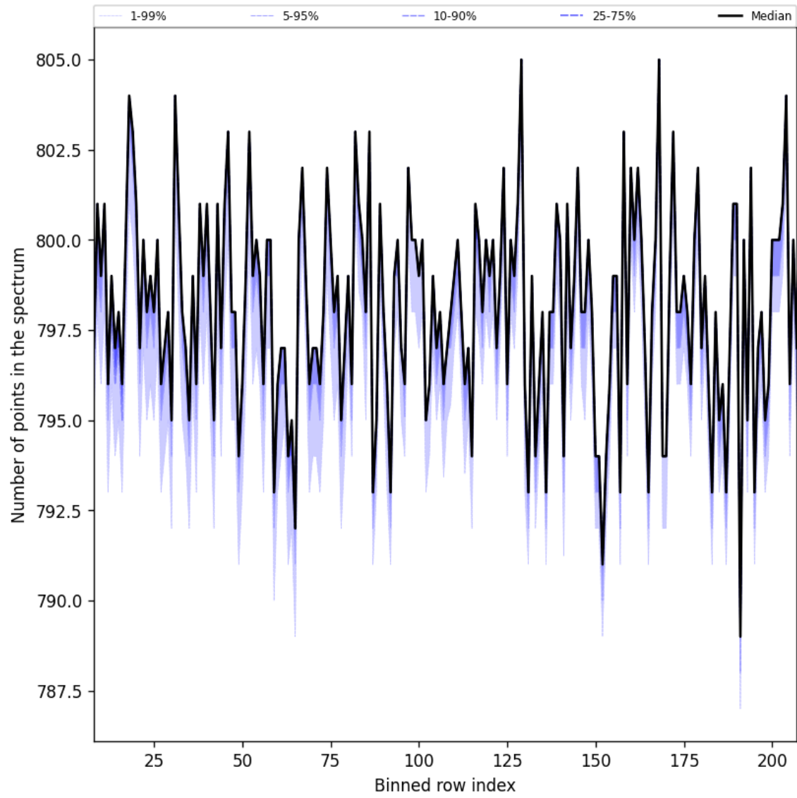
Figure 37: Along track statistics of “Number of points in the spectrum” for 2025-09-10 to 2025-09-11
