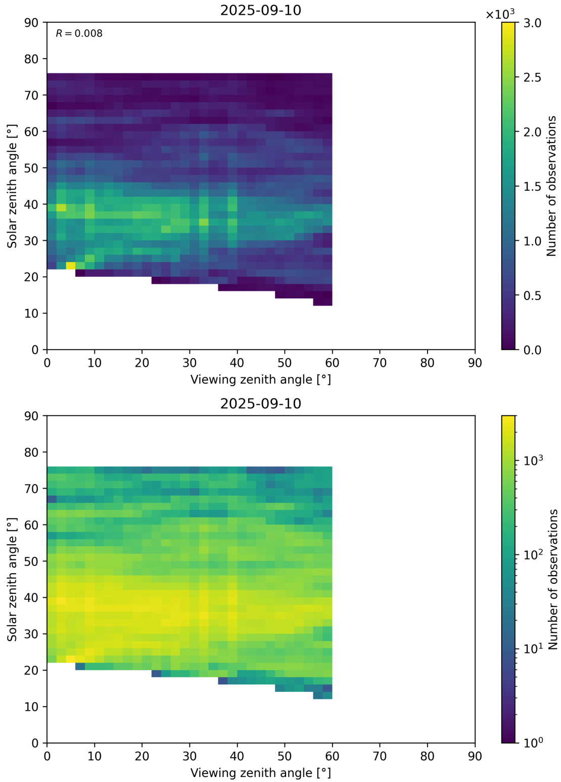
Figure 115: Scatter density plot of “Viewing zenith angle” against “Solar zenith angle” for 2025-09-10 to 2025-09-11.
