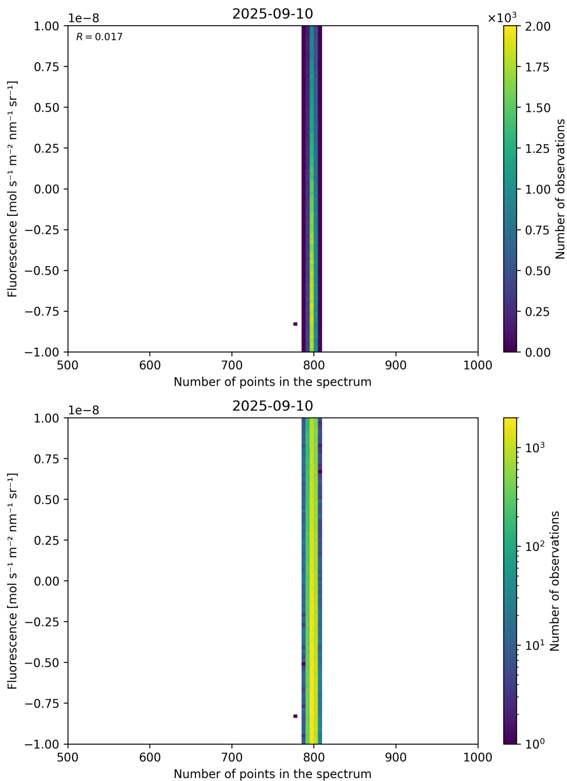
Figure 91: Scatter density plot of “Number of points in the spectrum” against “Fluorescence” for 2025-09-10 to 2025-09-11.
