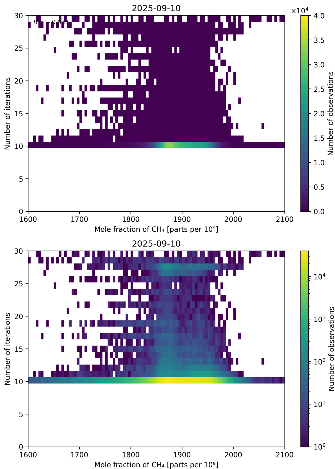
Figure 76: Scatter density plot of “Mole fraction of CH 4 ” against “Number of iterations” for 2025-09-10 to 2025-09-11.
