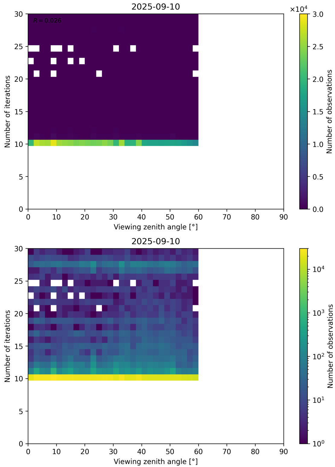
Figure 113: Scatter density plot of “Viewing zenith angle” against “Number of iterations” for 2025-09-10 to 2025-09-11.
