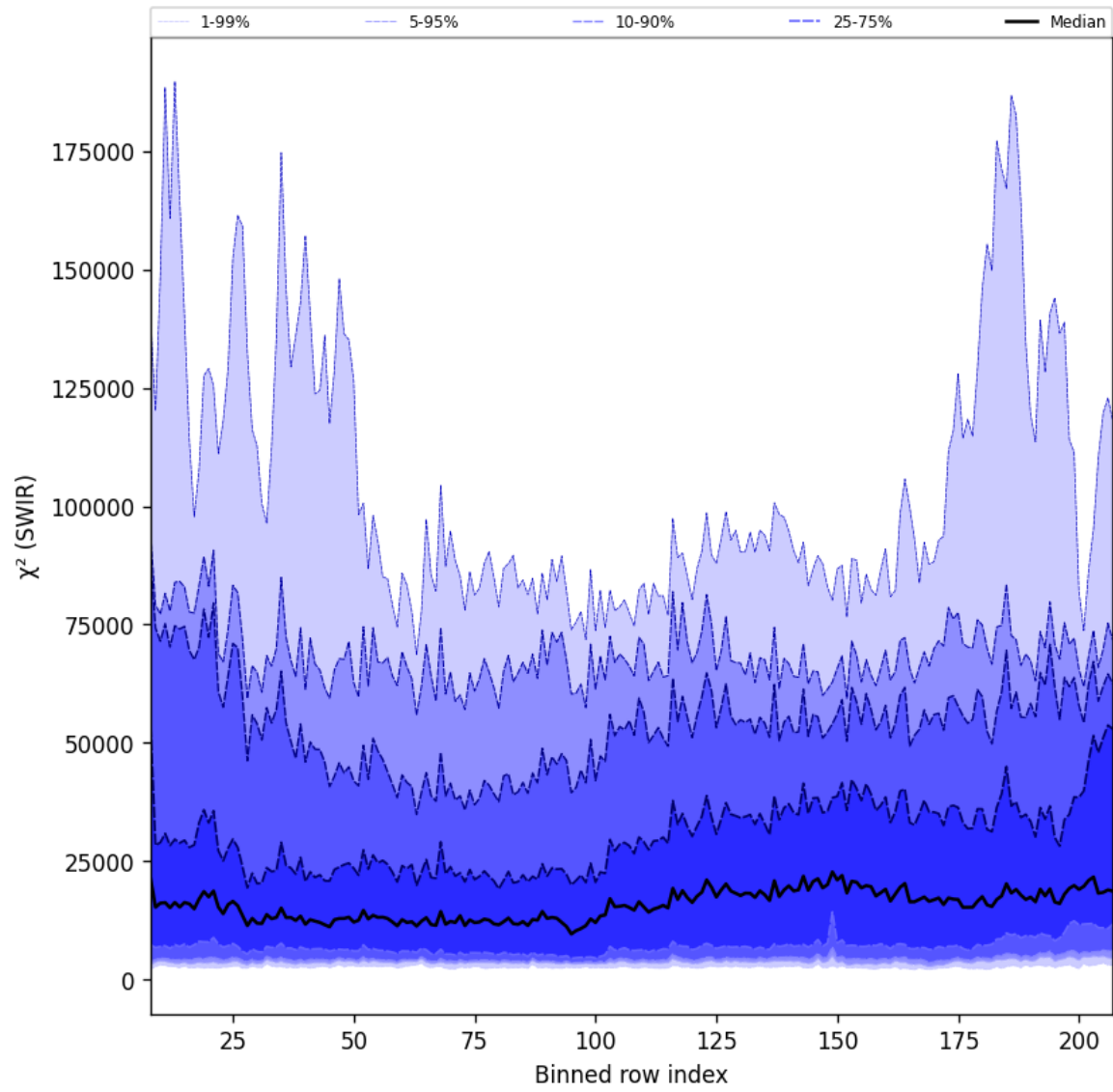
Figure 39: Along track statistics of “ \chi^2 (SWIR)” for 2025-09-10 to 2025-09-11
