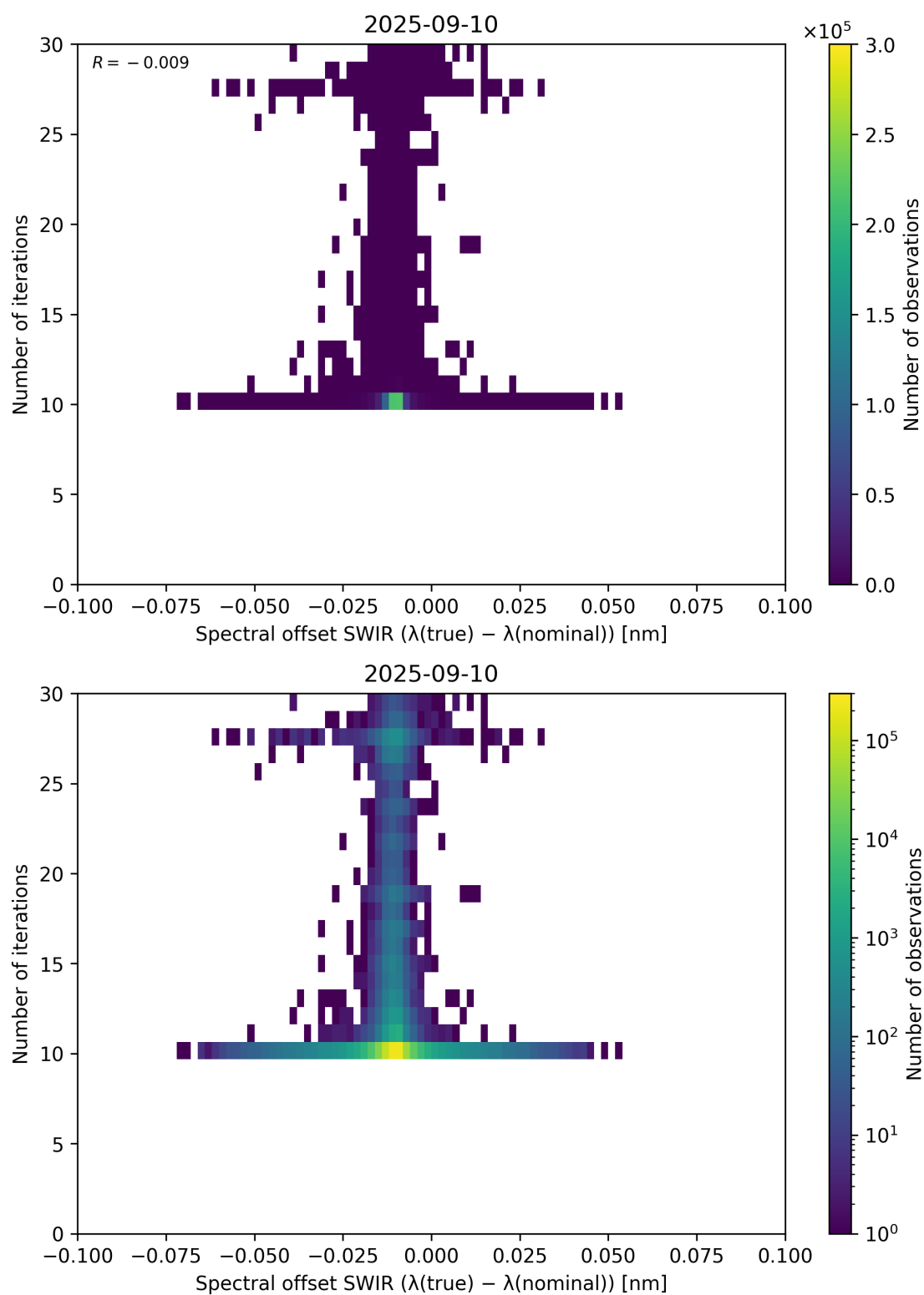
Figure 121: Scatter density plot of “Spectral offset SWIR ( \lambda_{\text{true}} - \lambda_{\text{nominal}} )” against “Number of iterations” for 2025-09-10 to 2025-09-11.
