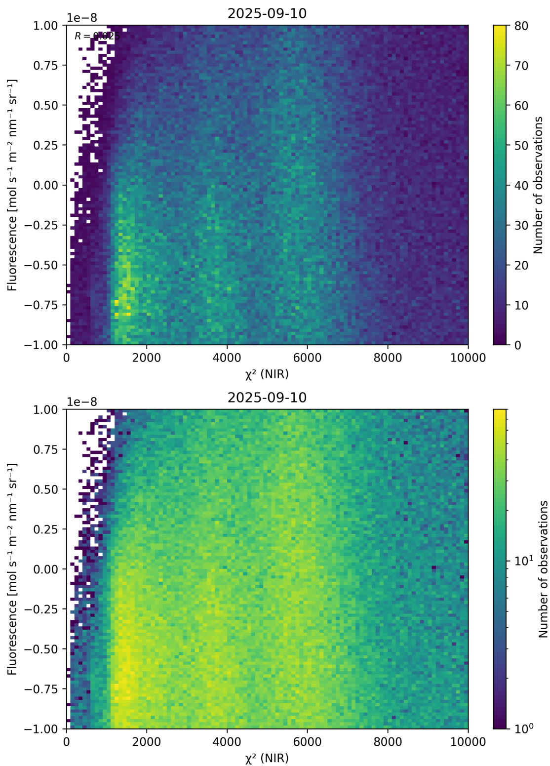
Figure 45: Scatter density plot of “ \chi^2 (NIR)” against “Fluorescence” for 2025-09-10 to 2025-09-11.
