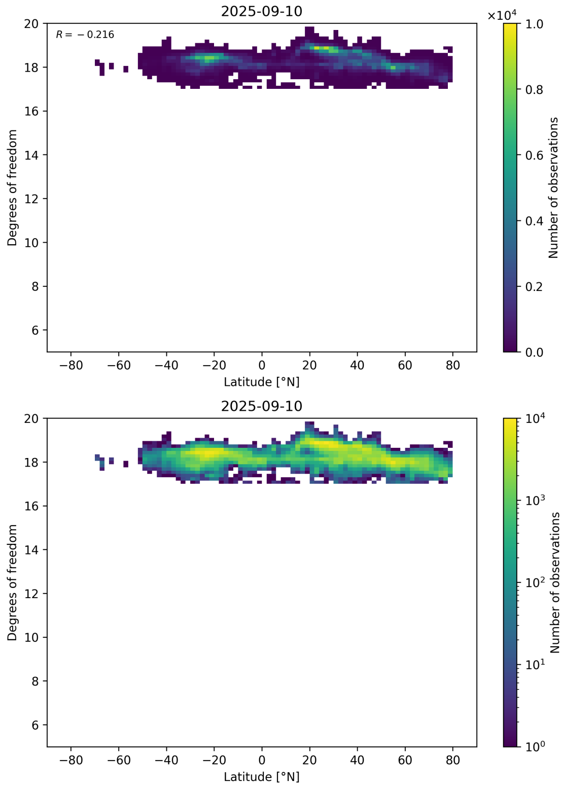
Figure 55: Scatter density plot of “Latitude” against “Degrees of freedom” for 2025-09-10 to 2025-09-11.
