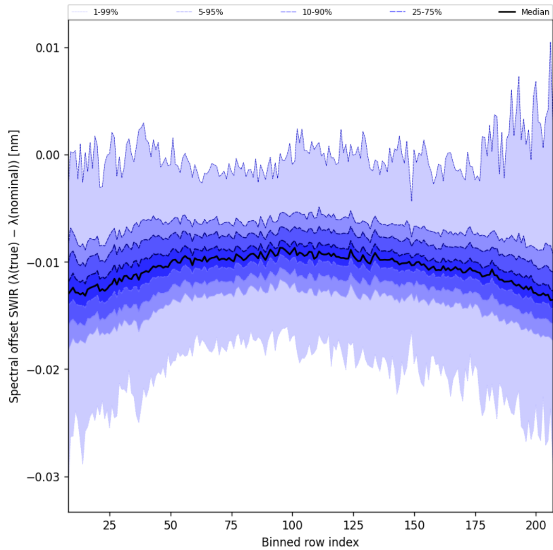
Figure 38: Along track statistics of “Spectral offset SWIR ( \lambda_{\text{true}} - \lambda_{\text{nominal}} )” for 2025-09-10 to 2025-09-11
