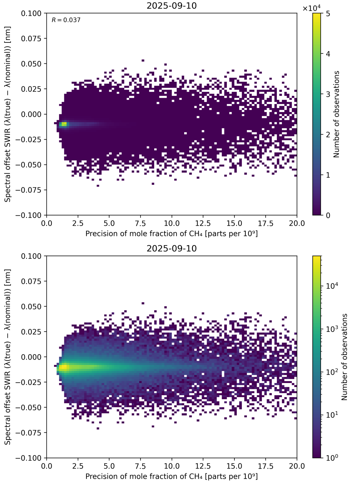
Figure 85: Scatter density plot of “Precision of mole fraction of CH 4 ” against “Spectral offset SWIR ( \lambda_{\text{true}} - \lambda_{\text{nominal}} )” for 2025-09-10 to 2025-09-11.
