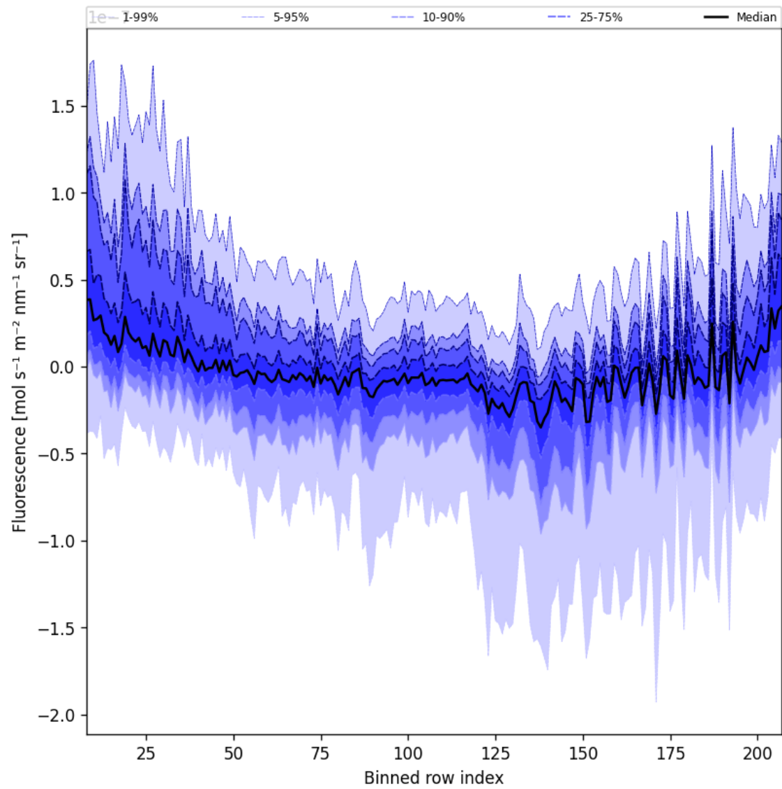
Figure 43: Along track statistics of “Fluorescence” for 2025-09-10 to 2025-09-11
