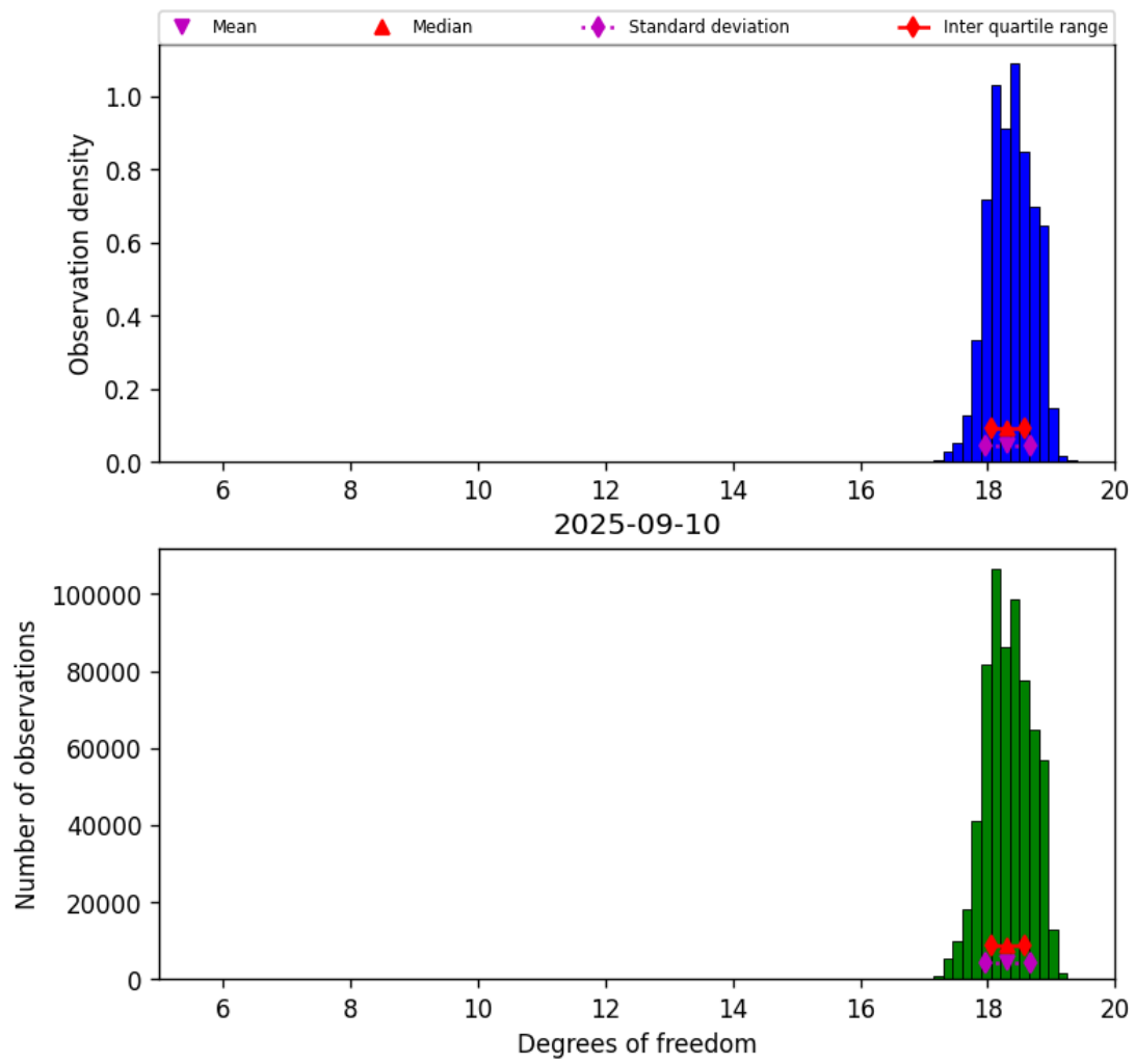
Figure 30: Histogram of “Degrees of freedom” for 2025-09-10 to 2025-09-11
