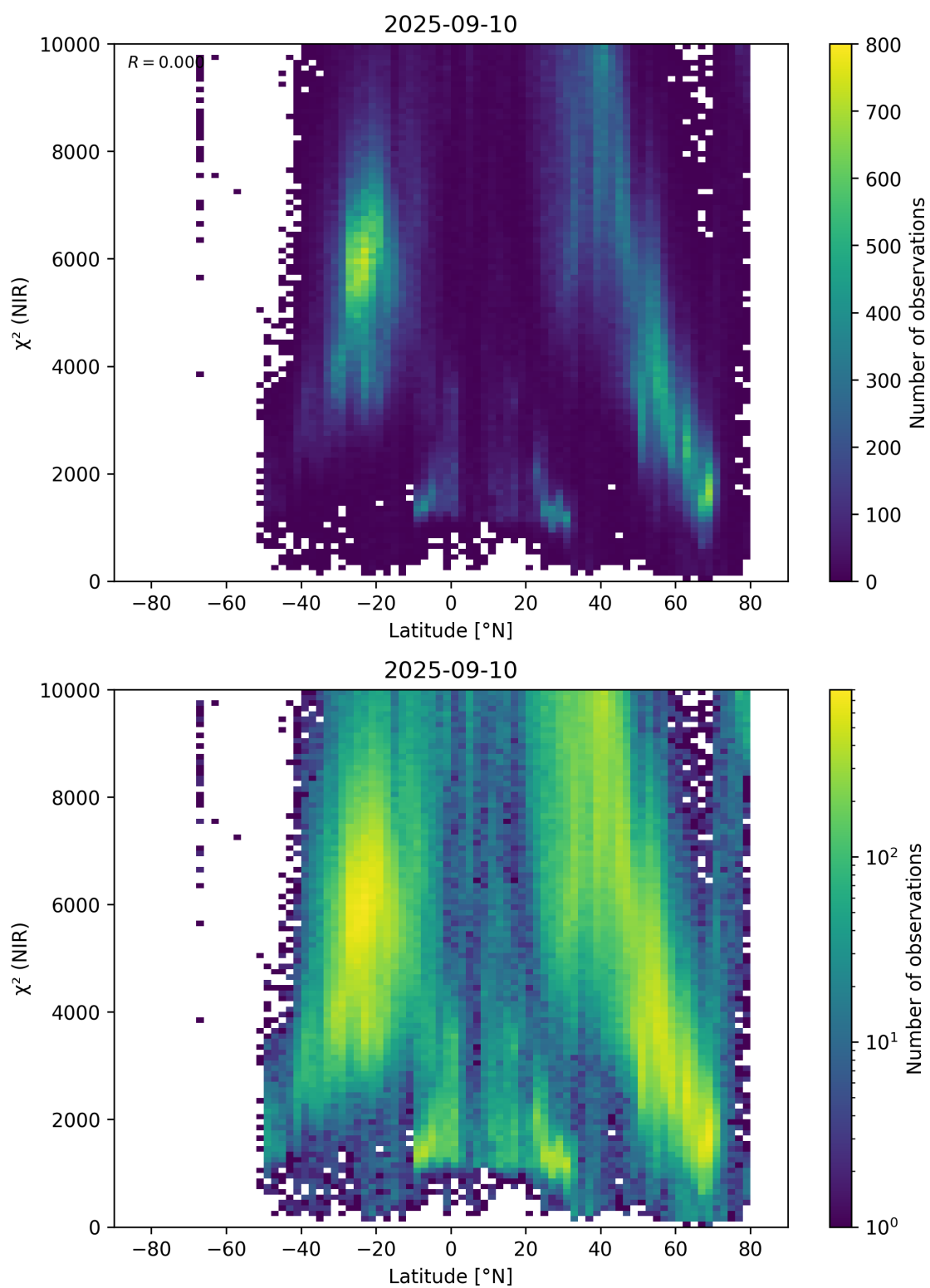
Figure 53: Scatter density plot of “Latitude” against “ \chi^2 (NIR)” for 2025-09-10 to 2025-09-11.
