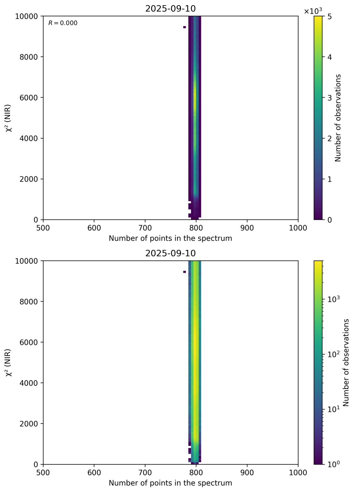
Figure 88: Scatter density plot of “Number of points in the spectrum” against “ \chi^2 (NIR)” for 2025-09-10 to 2025-09-11.
