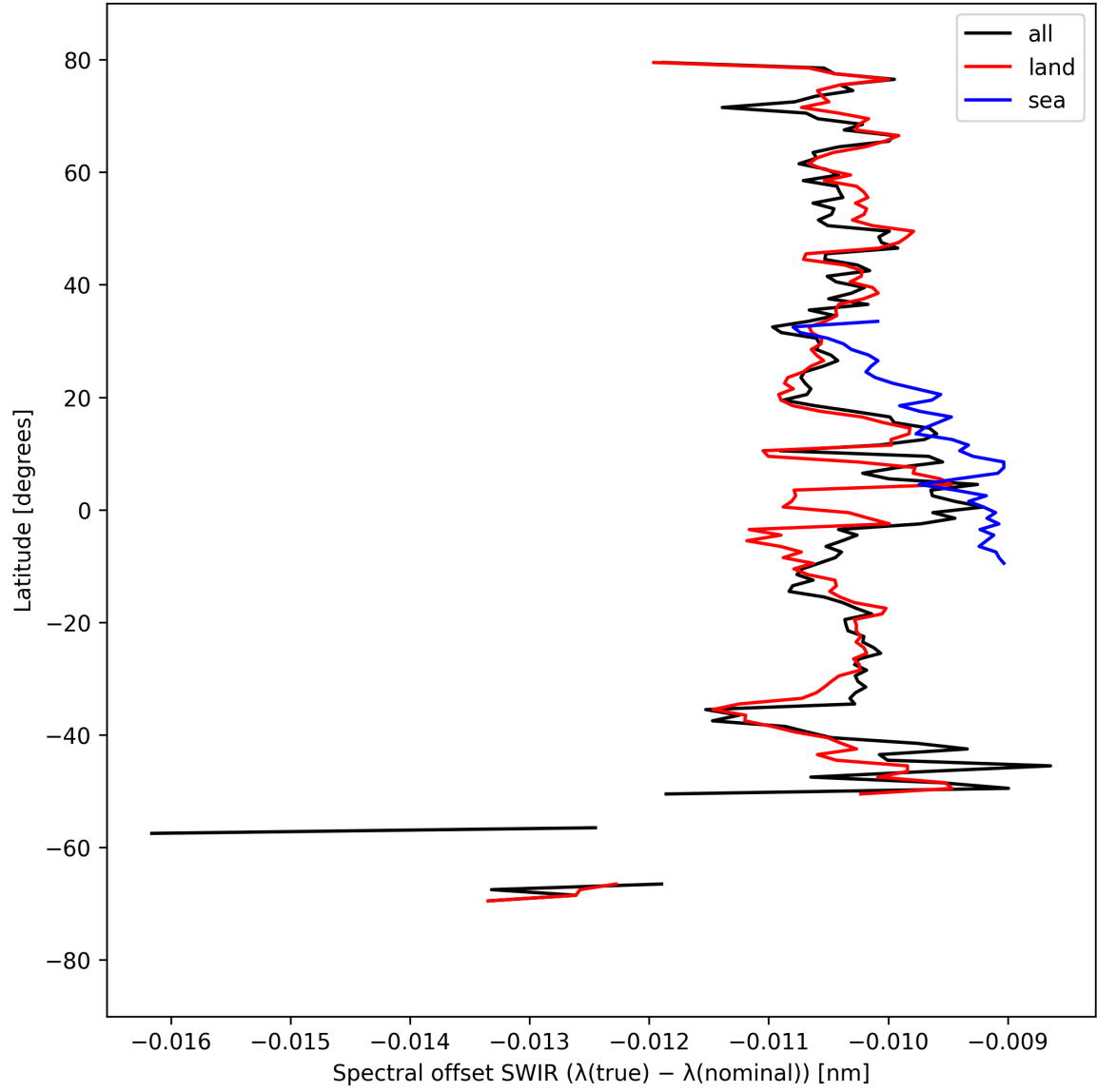
Figure 16: Zonal average of “Spectral offset SWIR ( \lambda_{\text{true}} - \lambda_{\text{nominal}} )” for 2025-09-10 to 2025-09-11.
