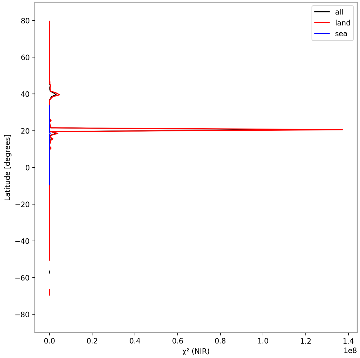
Figure 18: Zonal average of “ \chi^2 (NIR)” for 2025-09-10 to 2025-09-11.
