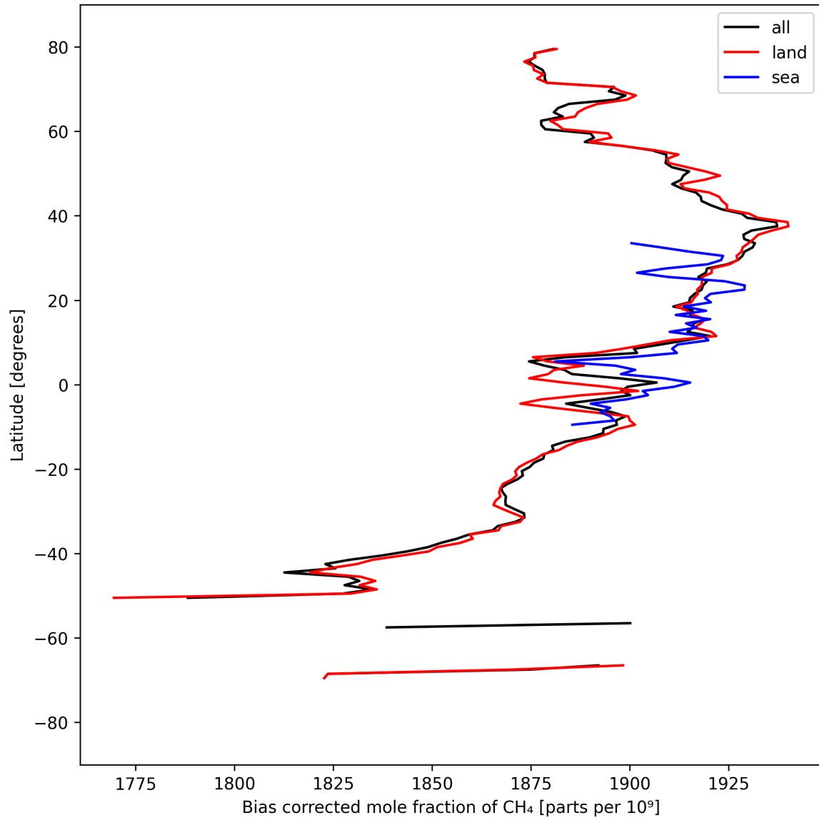
Figure 14: Zonal average of “Bias corrected mole fraction of CH 4 ” for 2025-09-10 to 2025-09-11.
