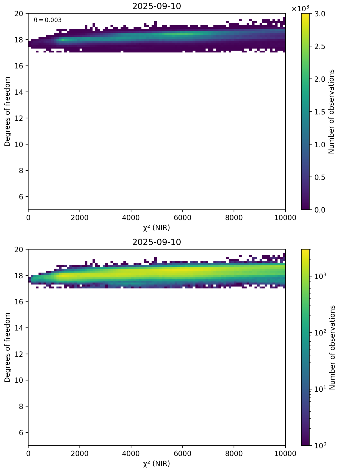
Figure 44: Scatter density plot of “ \chi^2 (NIR)” against “Degrees of freedom” for 2025-09-10 to 2025-09-11.
