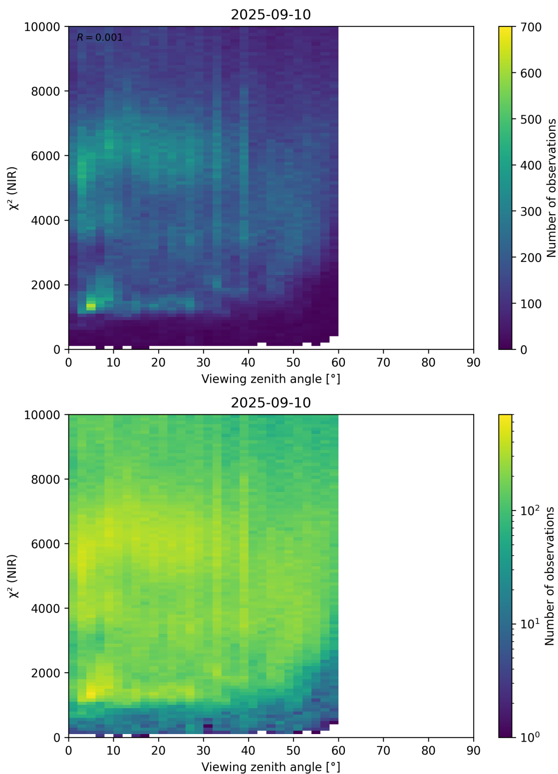
Figure 105: Scatter density plot of “Viewing zenith angle” against “ \chi^2 (NIR)” for 2025-09-10 to 2025-09-11.
