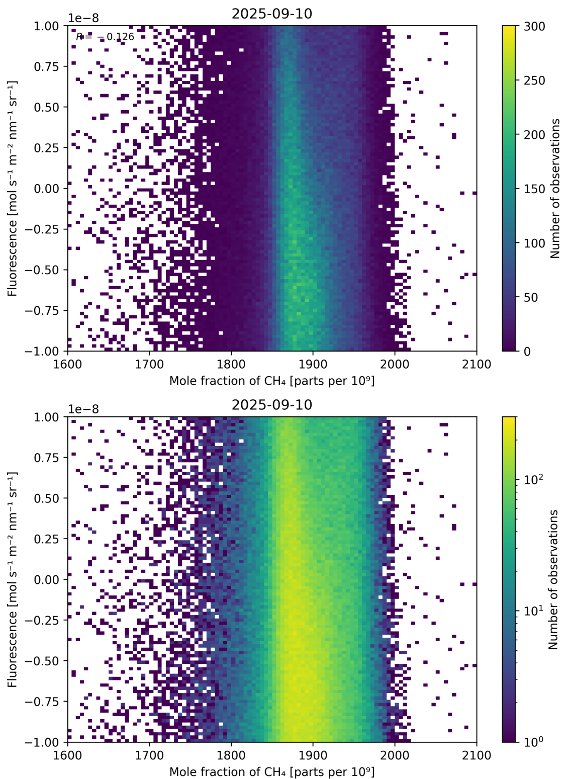
Figure 73: Scatter density plot of “Mole fraction of \text{CH}_4 ” against “Fluorescence” for 2025-09-10 to 2025-09-11.
