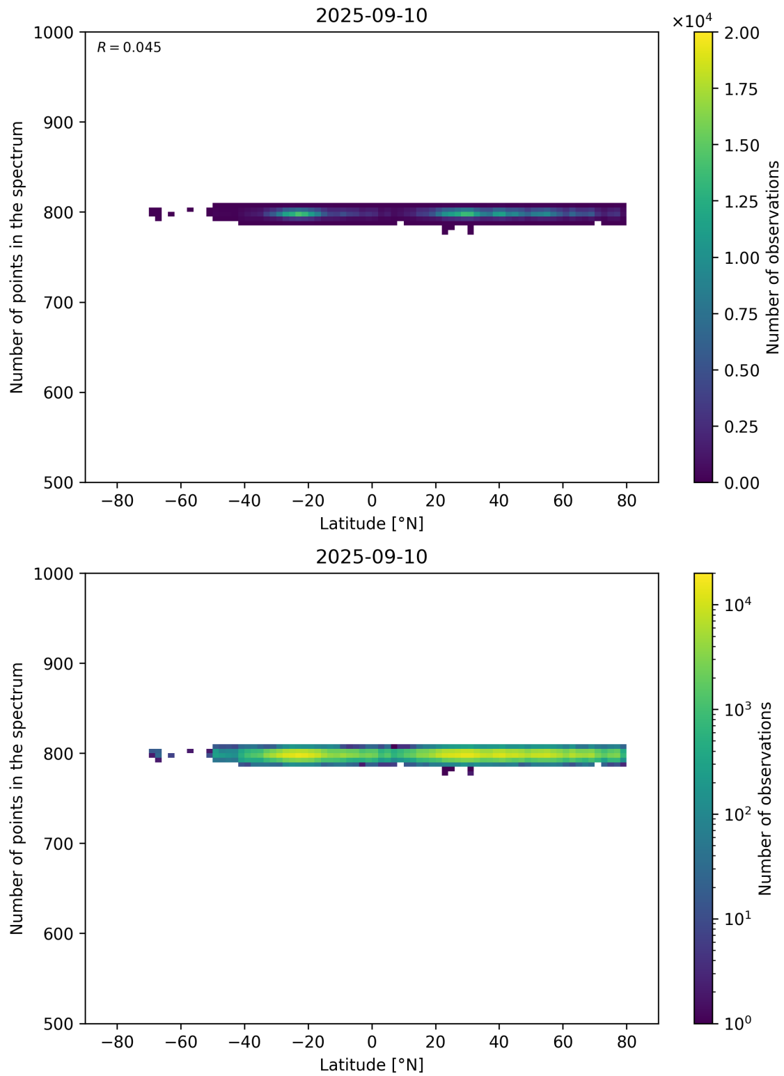
Figure 61: Scatter density plot of “Latitude” against “Number of points in the spectrum” for 2025-09-10 to 2025-09-11.
