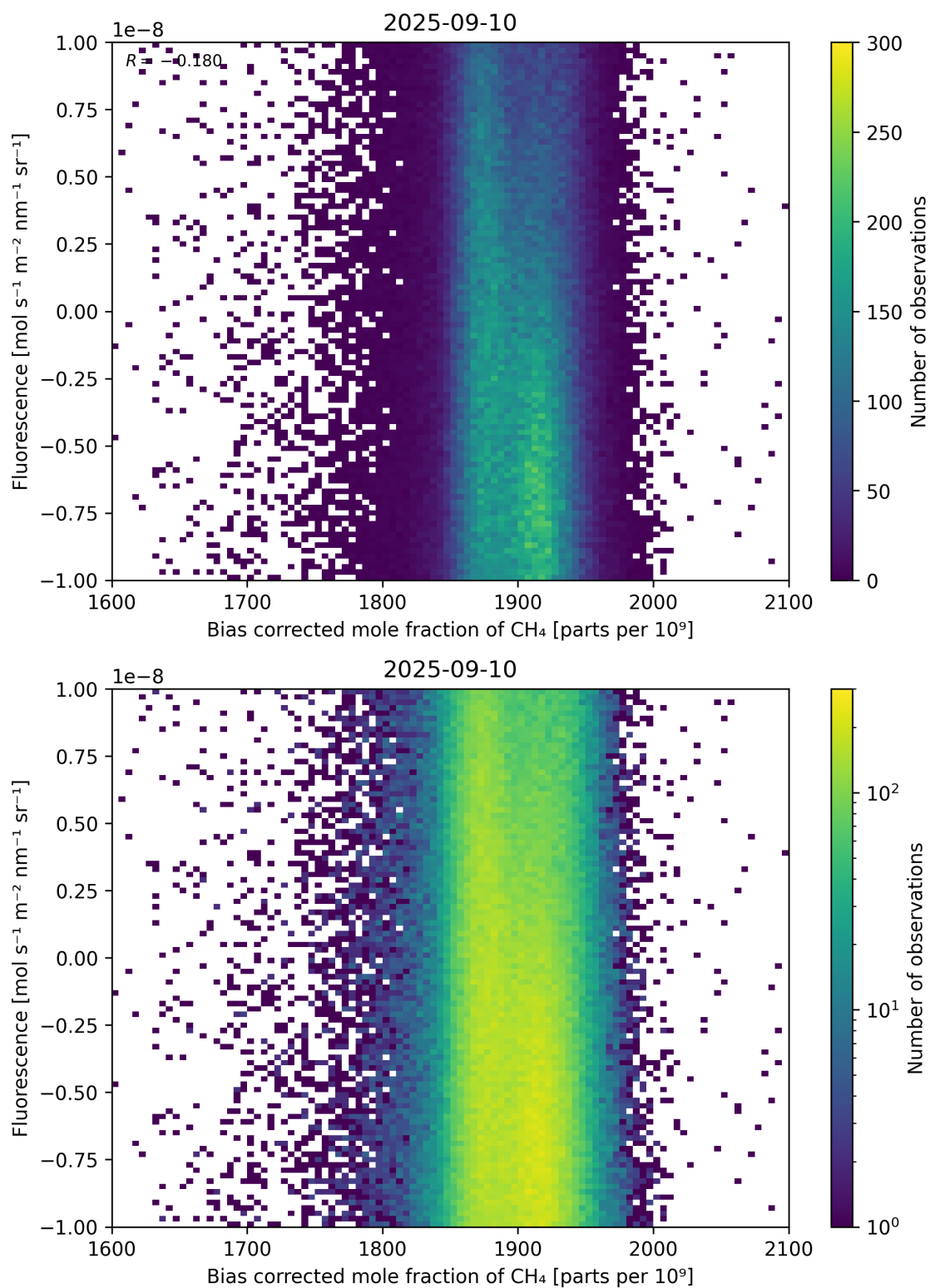
Figure 66: Scatter density plot of “Bias corrected mole fraction of \text{CH}_4 ” against “Fluorescence” for 2025-09-10 to 2025-09-11.
