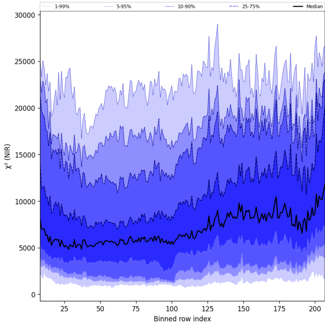
Figure 40: Along track statistics of “ \chi^2 (NIR)” for 2025-09-10 to 2025-09-11
