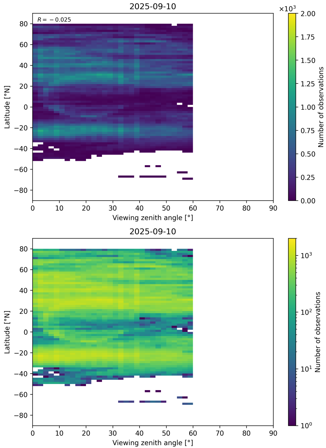
Figure 109: Scatter density plot of “Viewing zenith angle” against “Latitude” for 2025-09-10 to 2025-09-11.
