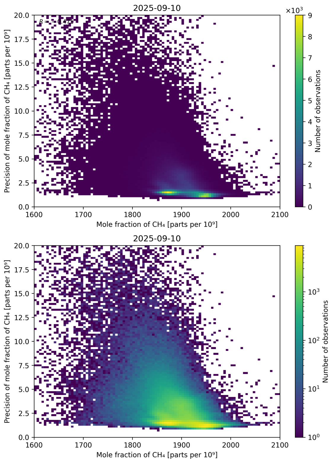
Figure 75: Scatter density plot of “Mole fraction of CH 4 ” against “Precision of mole fraction of CH 4 ” for 2025-09-10 to 2025-09-11.
