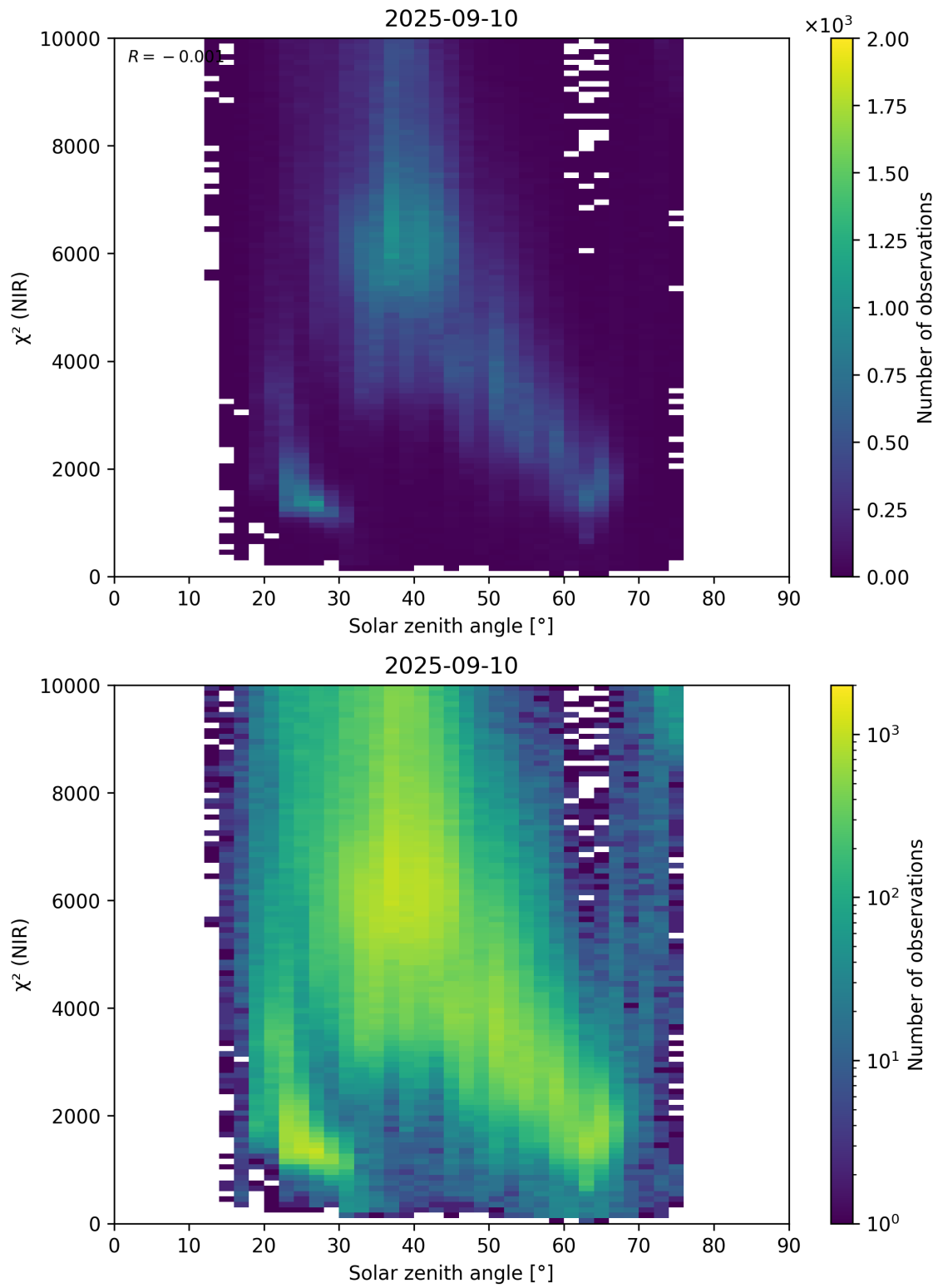
Figure 94: Scatter density plot of “Solar zenith angle” against “ \chi^2 (NIR)” for 2025-09-10 to 2025-09-11.
