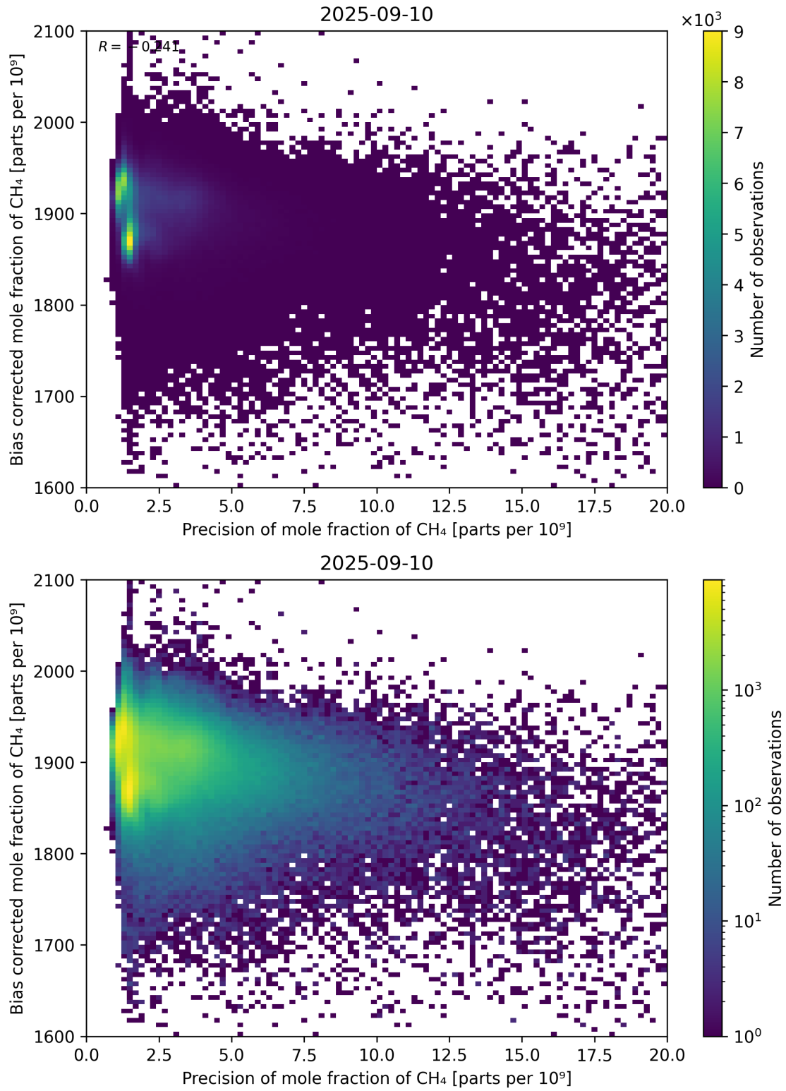
Figure 82: Scatter density plot of “Precision of mole fraction of CH 4 ” against “Bias corrected mole fraction of CH 4 ” for 2025-09-10 to 2025-09-11.
