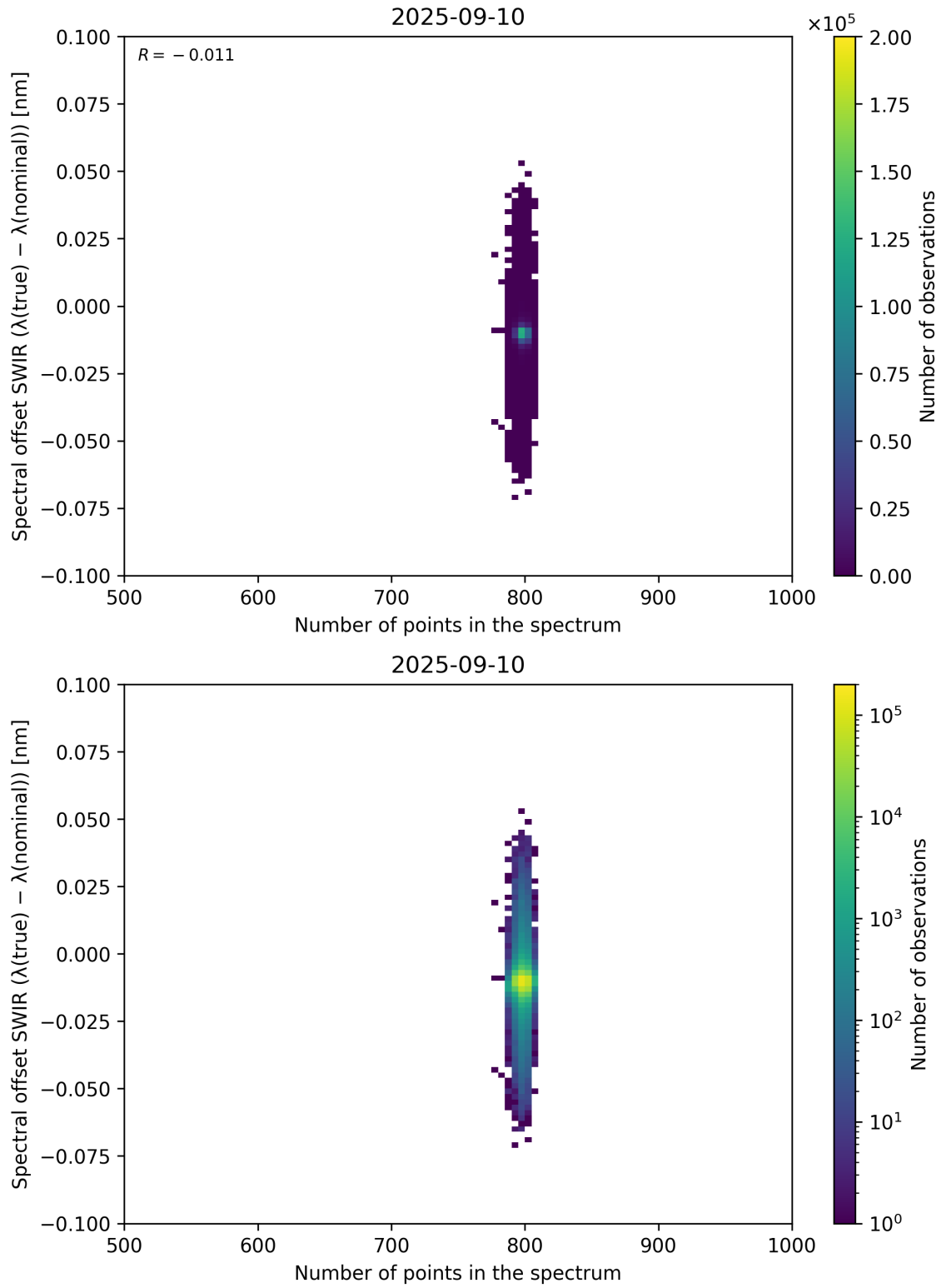
Figure 93: Scatter density plot of “Number of points in the spectrum” against “Spectral offset SWIR ( \lambda_{\text{true}} - \lambda_{\text{nominal}} )” for 2025-09-10 to 2025-09-11.
