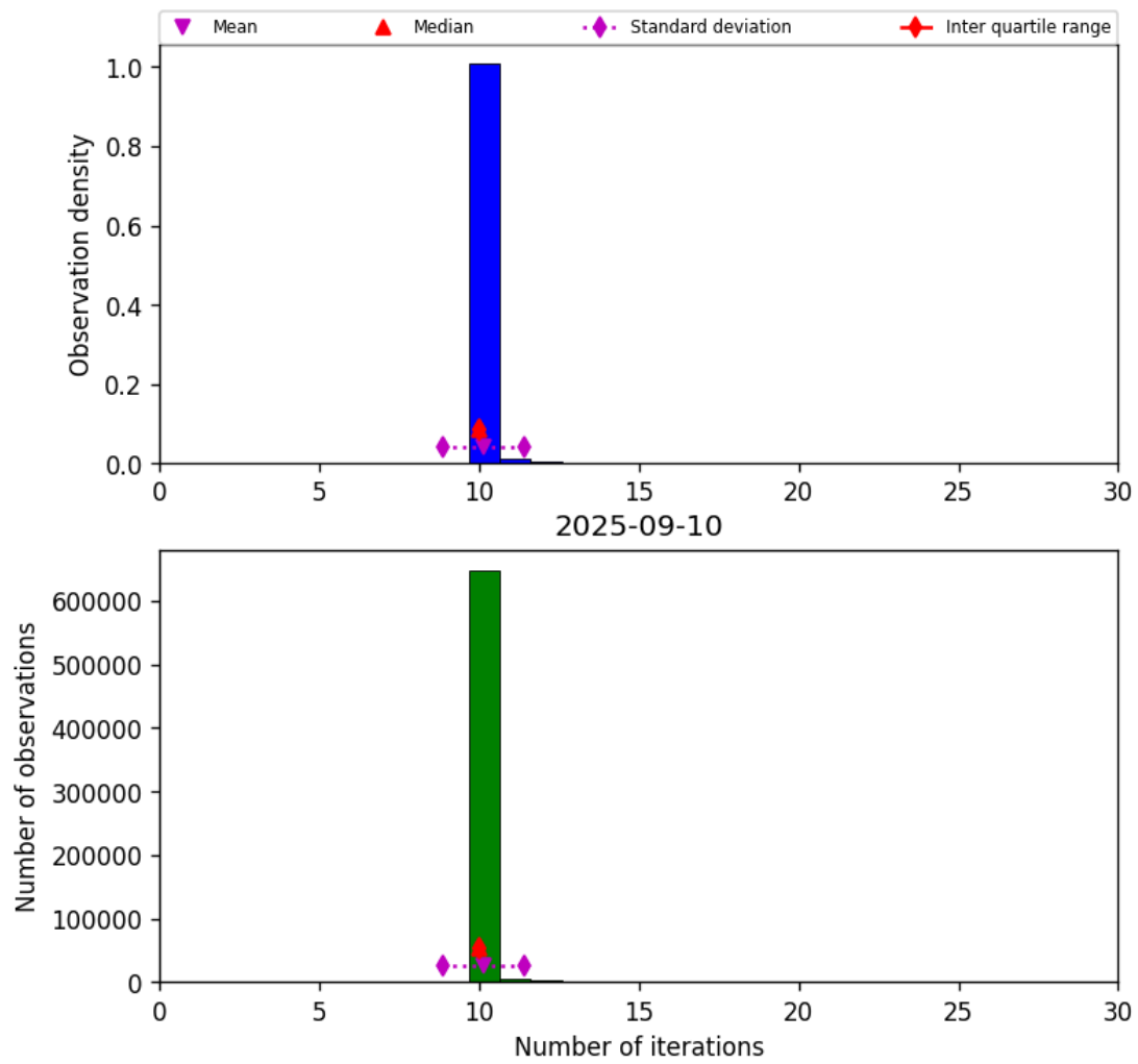
Figure 31: Histogram of “Number of iterations” for 2025-09-10 to 2025-09-11
