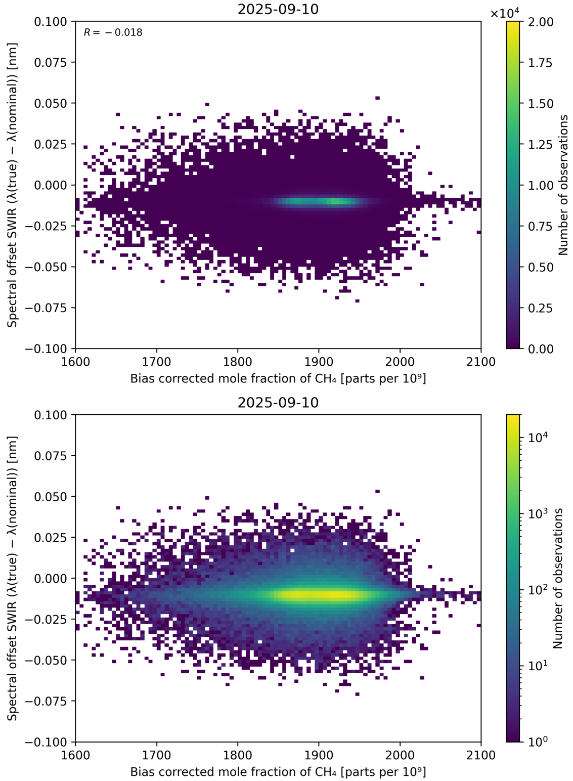
Figure 69: Scatter density plot of “Bias corrected mole fraction of CH 4 ” against “Spectral offset SWIR ( \lambda_{\text{true}} - \lambda_{\text{nominal}} )” for 2025-09-10 to 2025-09-11.
