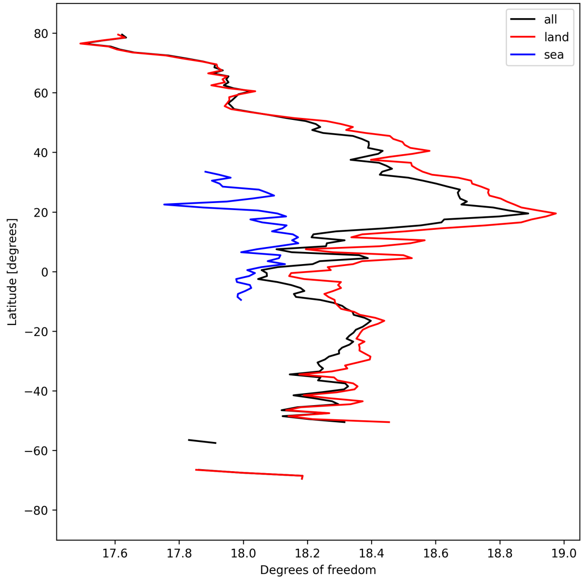
Figure 19: Zonal average of “Degrees of freedom” for 2025-09-10 to 2025-09-11.
