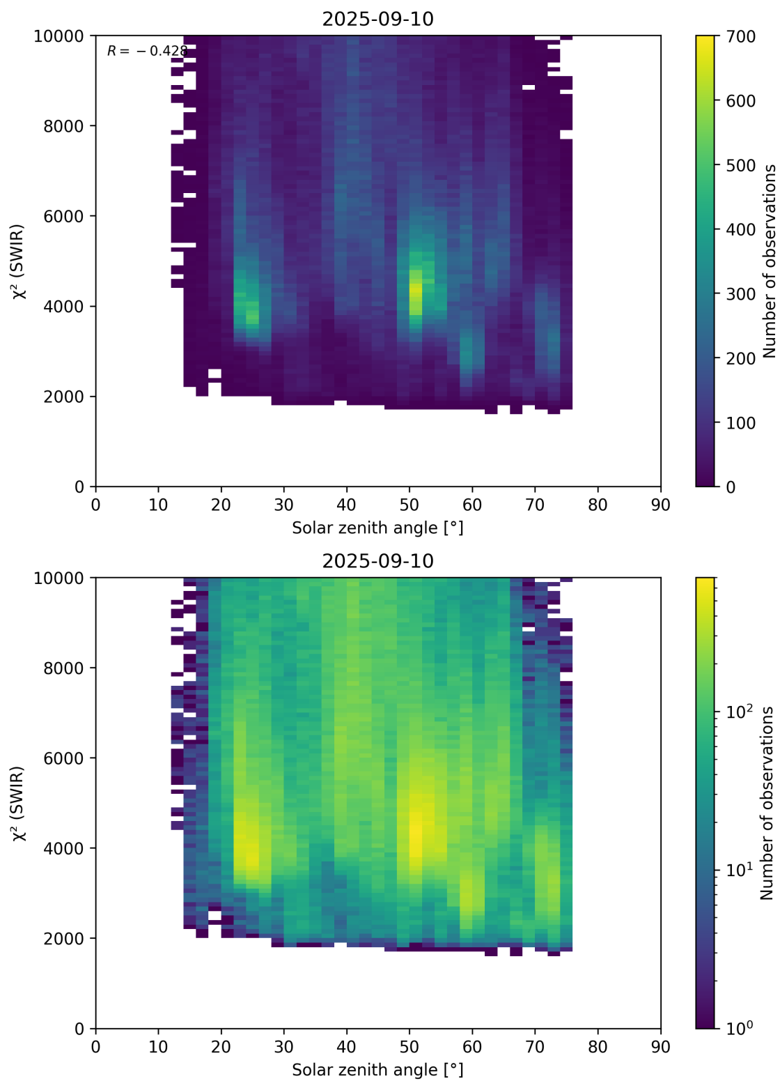
Figure 95: Scatter density plot of “Solar zenith angle” against “ \chi^2 (SWIR)” for 2025-09-10 to 2025-09-11.
