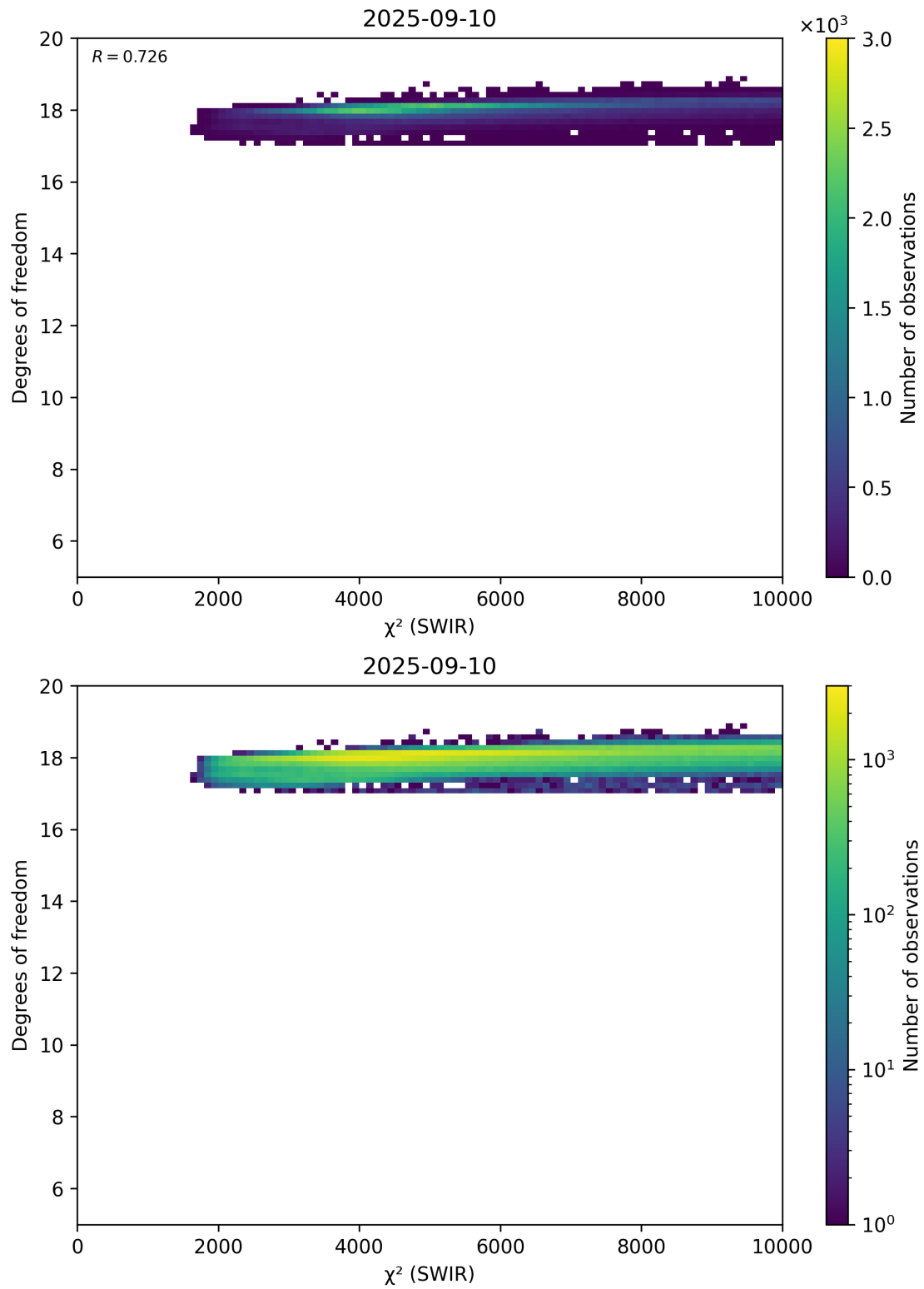
Figure 48: Scatter density plot of “ \chi^2 (SWIR)” against “Degrees of freedom” for 2025-09-10 to 2025-09-11.
