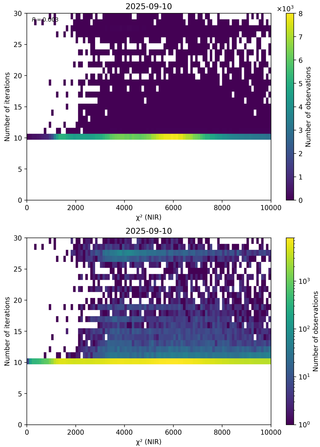
Figure 46: Scatter density plot of “ \chi^2 (NIR)” against “Number of iterations” for 2025-09-10 to 2025-09-11.
