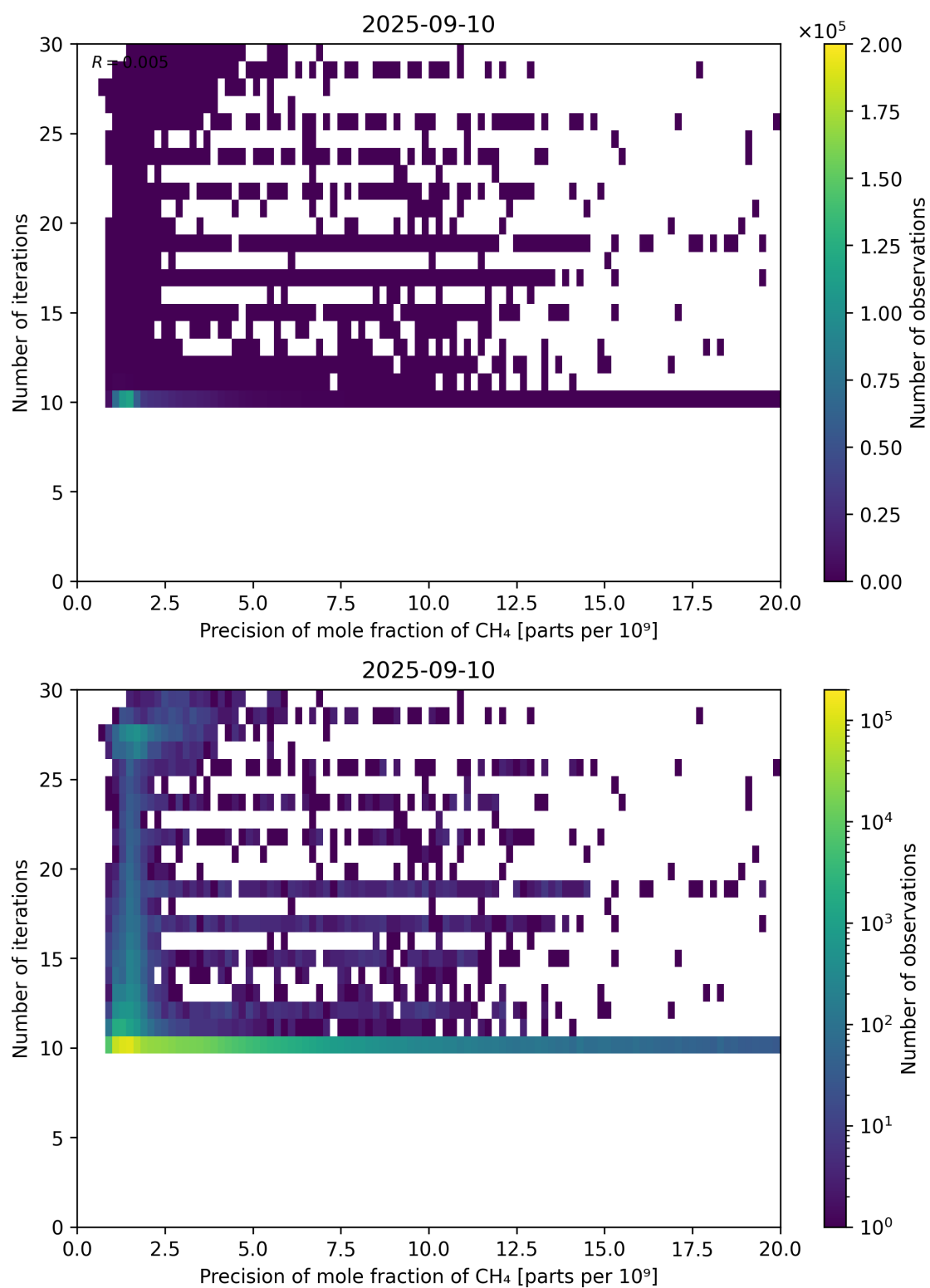
Figure 83: Scatter density plot of “Precision of mole fraction of CH 4 ” against “Number of iterations” for 2025-09-10 to 2025-09-11.
