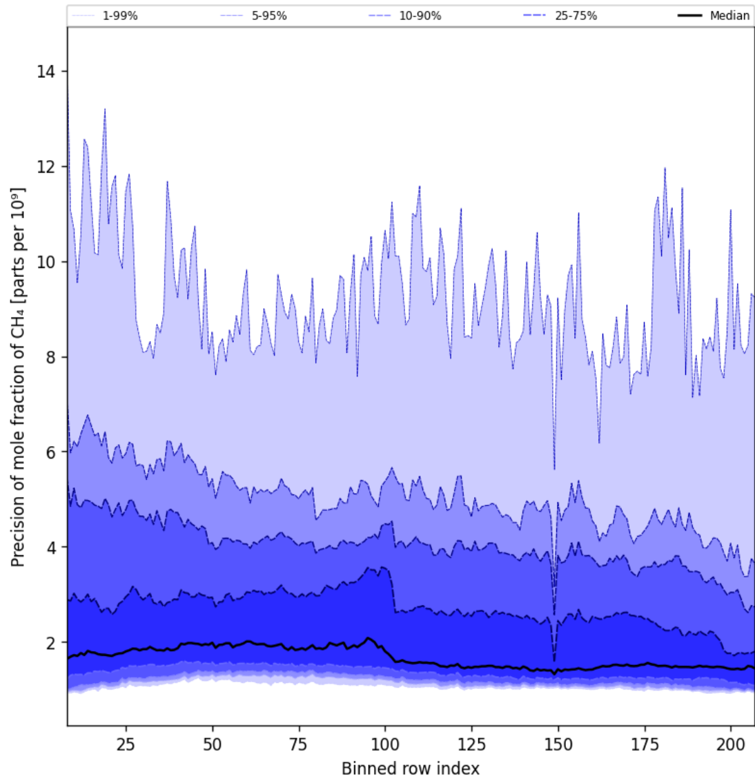
Figure 35: Along track statistics of “Precision of mole fraction of CH 4 ” for 2025-09-10 to 2025-09-11
