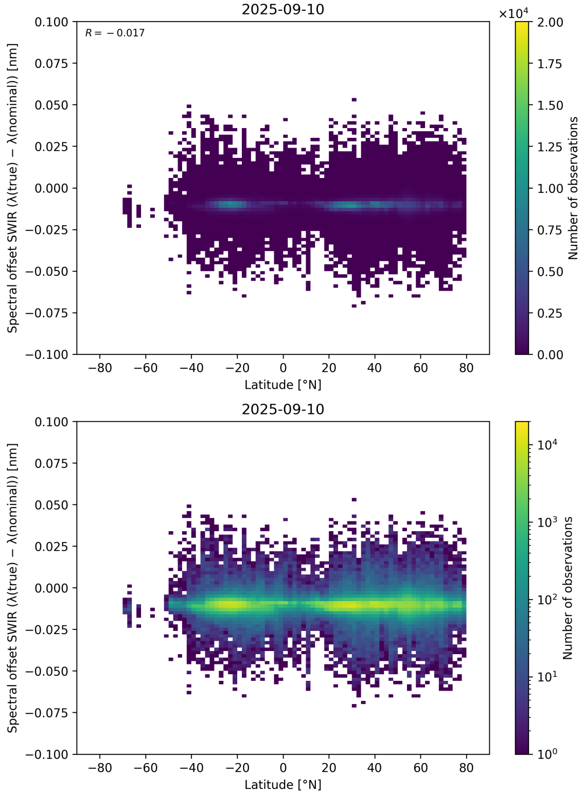
Figure 62: Scatter density plot of “Latitude” against “Spectral offset SWIR ( \lambda_{\text{true}} - \lambda_{\text{nominal}} )” for 2025-09-10 to 2025-09-11.
