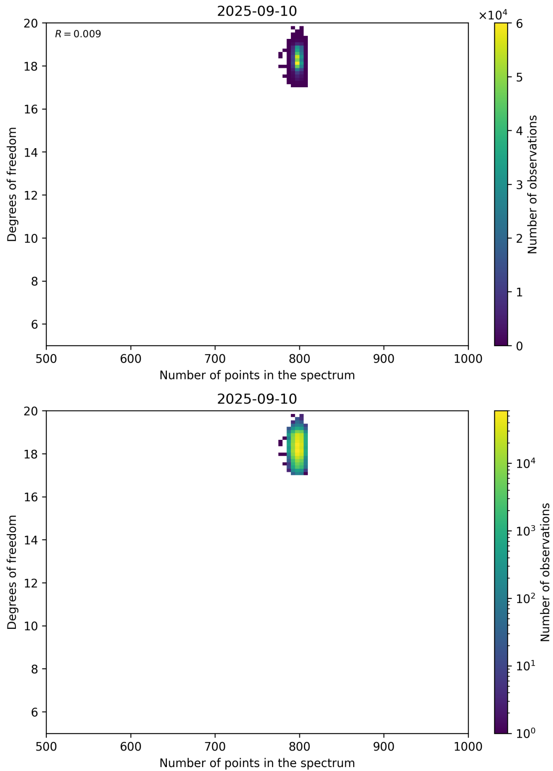
Figure 90: Scatter density plot of “Number of points in the spectrum” against “Degrees of freedom” for 2025-09-10 to 2025-09-11.
