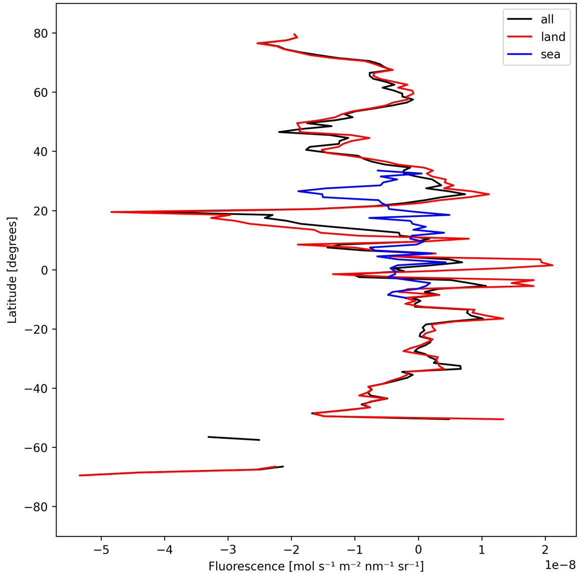
Figure 21: Zonal average of “Fluorescence” for 2025-09-10 to 2025-09-11.
