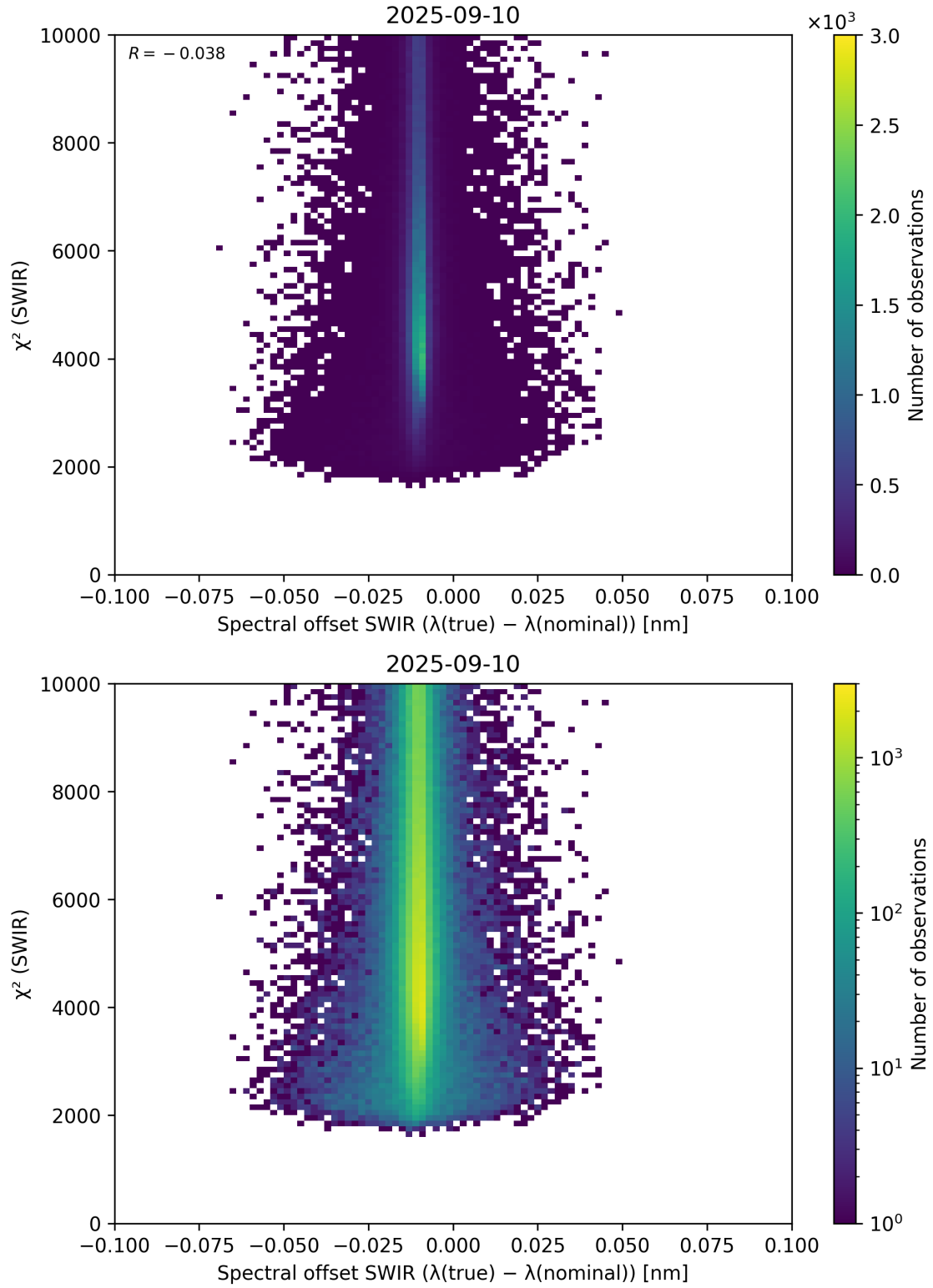
Figure 118: Scatter density plot of “Spectral offset SWIR ( \lambda_{\text{true}} - \lambda_{\text{nominal}} )” against “ \chi^2 (SWIR)” for 2025-09-10 to 2025-09-11.
