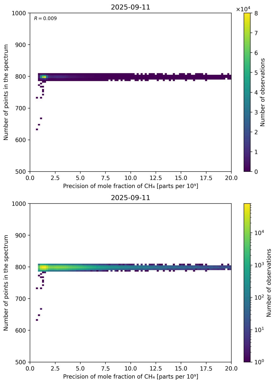
Figure 84: Scatter density plot of “Precision of mole fraction of CH 4 ” against “Number of points in the spectrum” for 2025-09-10 to 2025-09-12.
