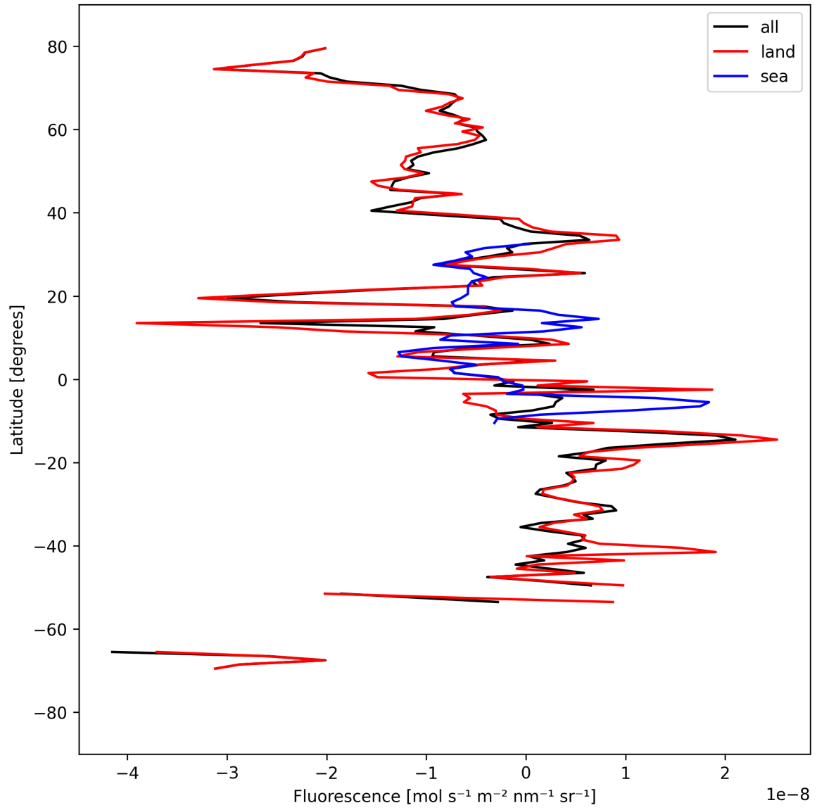
Figure 21: Zonal average of “Fluorescence” for 2025-09-10 to 2025-09-12.
