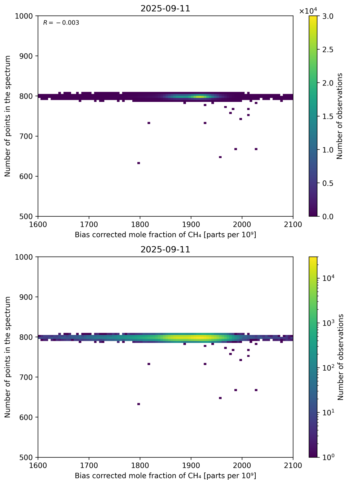
Figure 68: Scatter density plot of “Bias corrected mole fraction of CH 4 ” against “Number of points in the spectrum” for 2025-09-10 to 2025-09-12.
