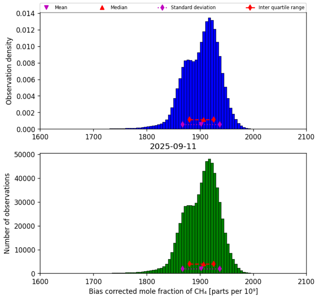
Figure 25: Histogram of “Bias corrected mole fraction of CH 4 ” for 2025-09-10 to 2025-09-12
