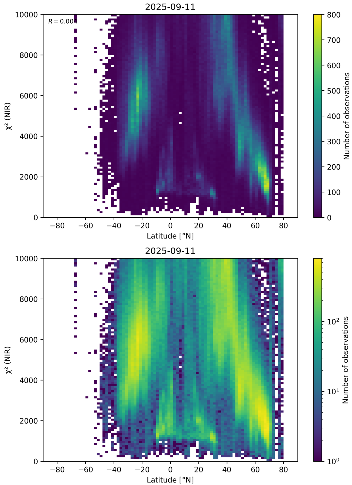
Figure 53: Scatter density plot of “Latitude” against “ \chi^2 (NIR)” for 2025-09-10 to 2025-09-12.
