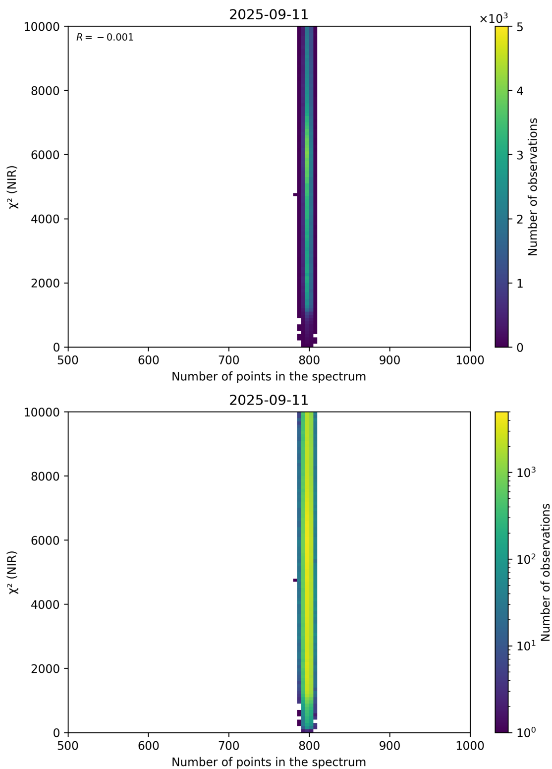
Figure 88: Scatter density plot of “Number of points in the spectrum” against “ \chi^2 (NIR)” for 2025-09-10 to 2025-09-12.
