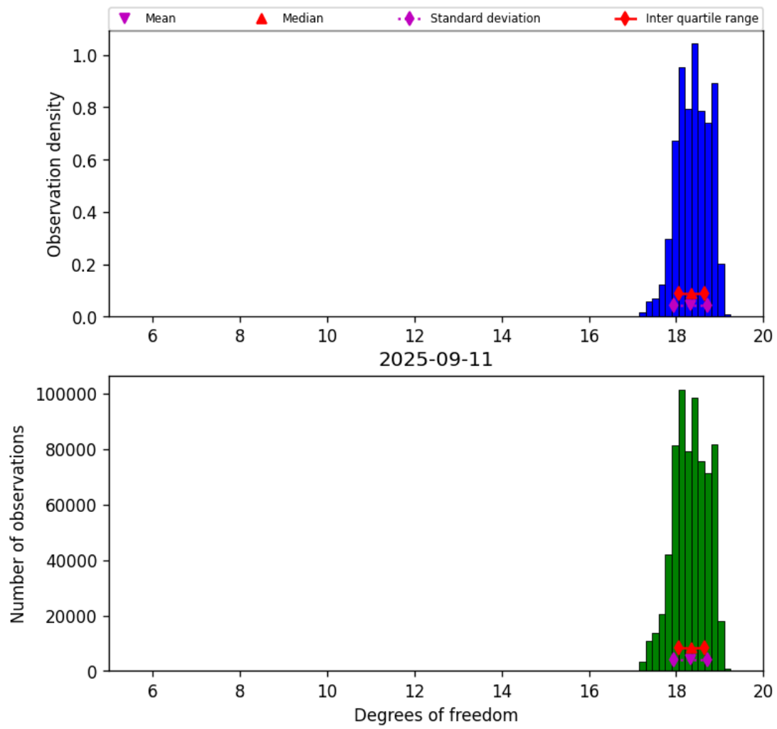
Figure 30: Histogram of “Degrees of freedom” for 2025-09-10 to 2025-09-12
