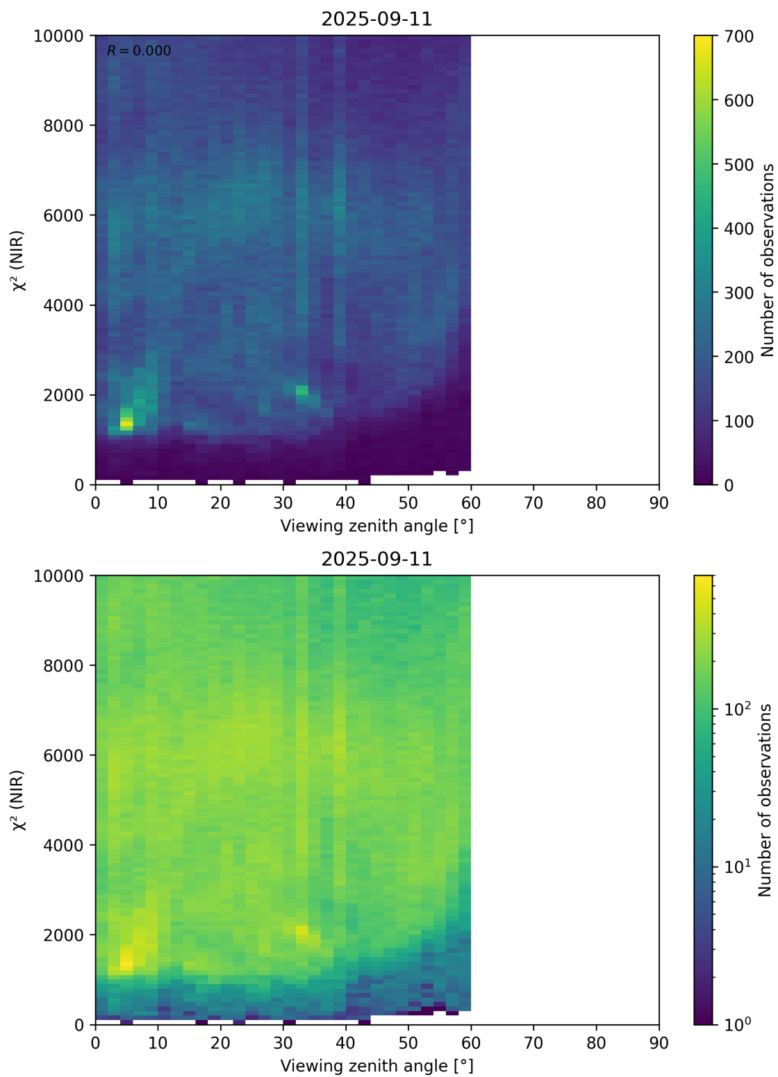
Figure 105: Scatter density plot of “Viewing zenith angle” against “ \chi^2 (NIR)” for 2025-09-10 to 2025-09-12.
