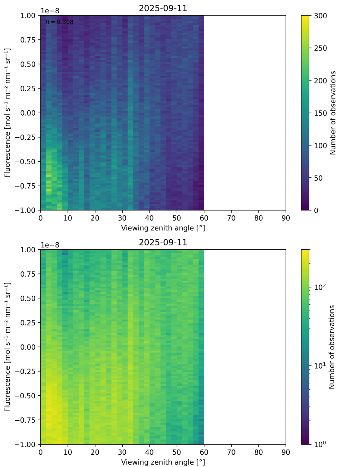
Figure 108: Scatter density plot of “Viewing zenith angle” against “Fluorescence” for 2025-09-10 to 2025-09-12.
