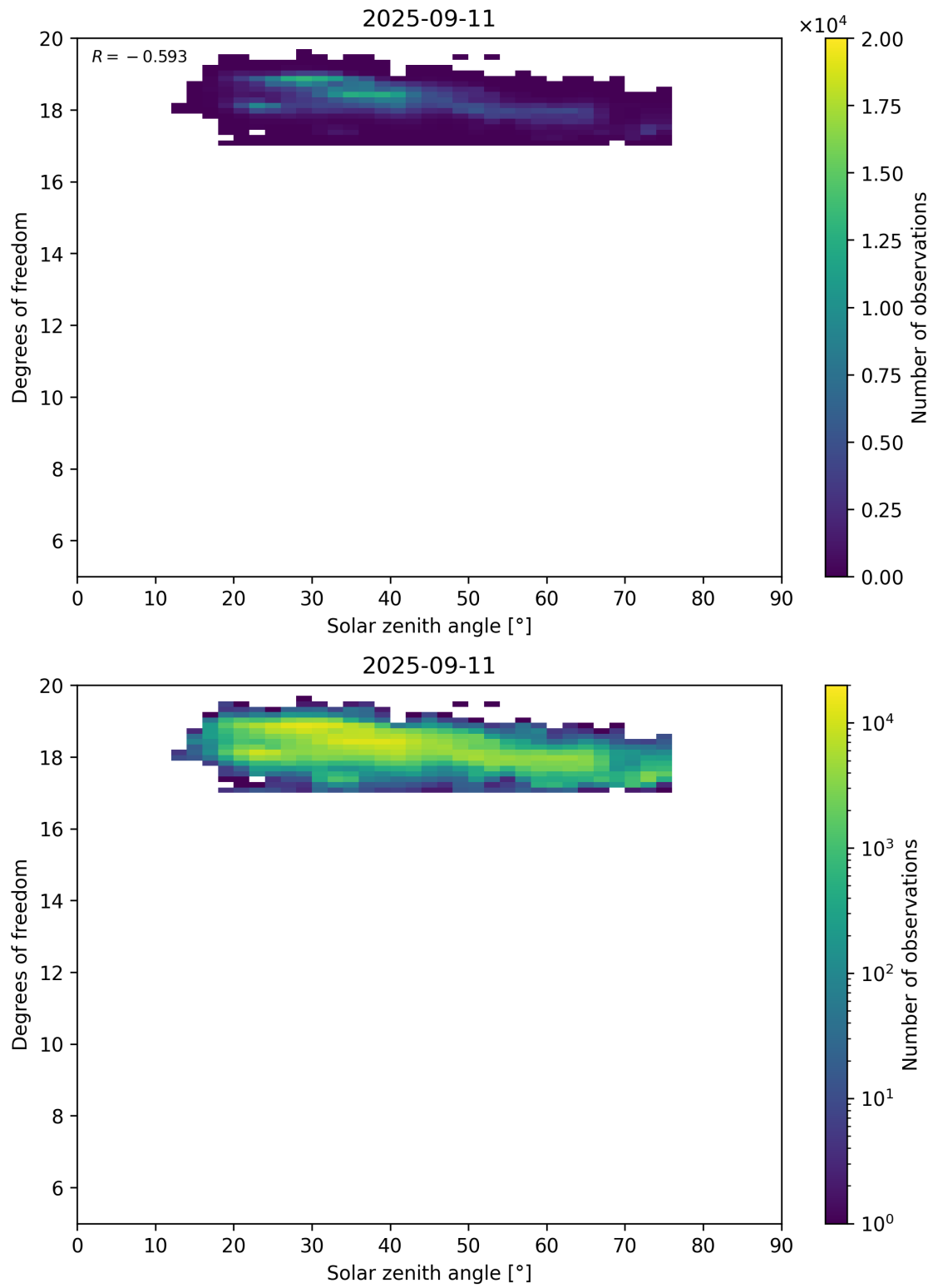
Figure 96: Scatter density plot of “Solar zenith angle” against “Degrees of freedom” for 2025-09-10 to 2025-09-12.
