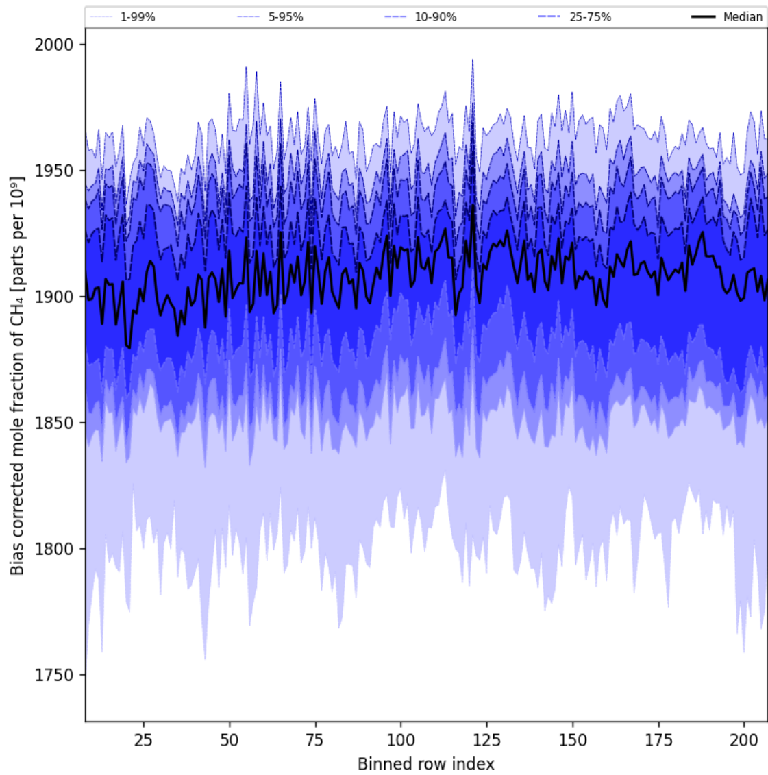
Figure 36: Along track statistics of “Bias corrected mole fraction of CH 4 ” for 2025-09-10 to 2025-09-12
