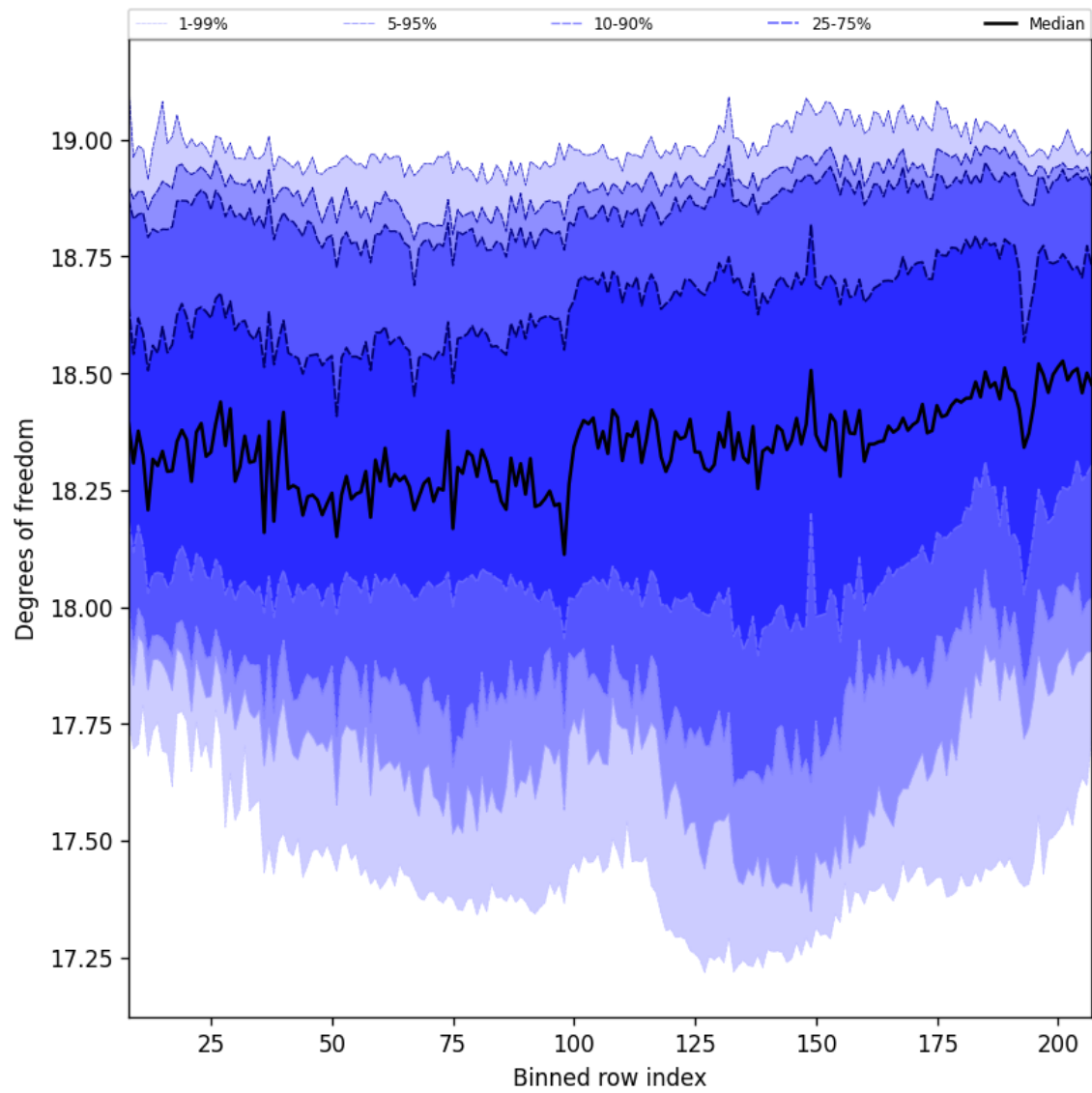
Figure 41: Along track statistics of “Degrees of freedom” for 2025-09-10 to 2025-09-12
