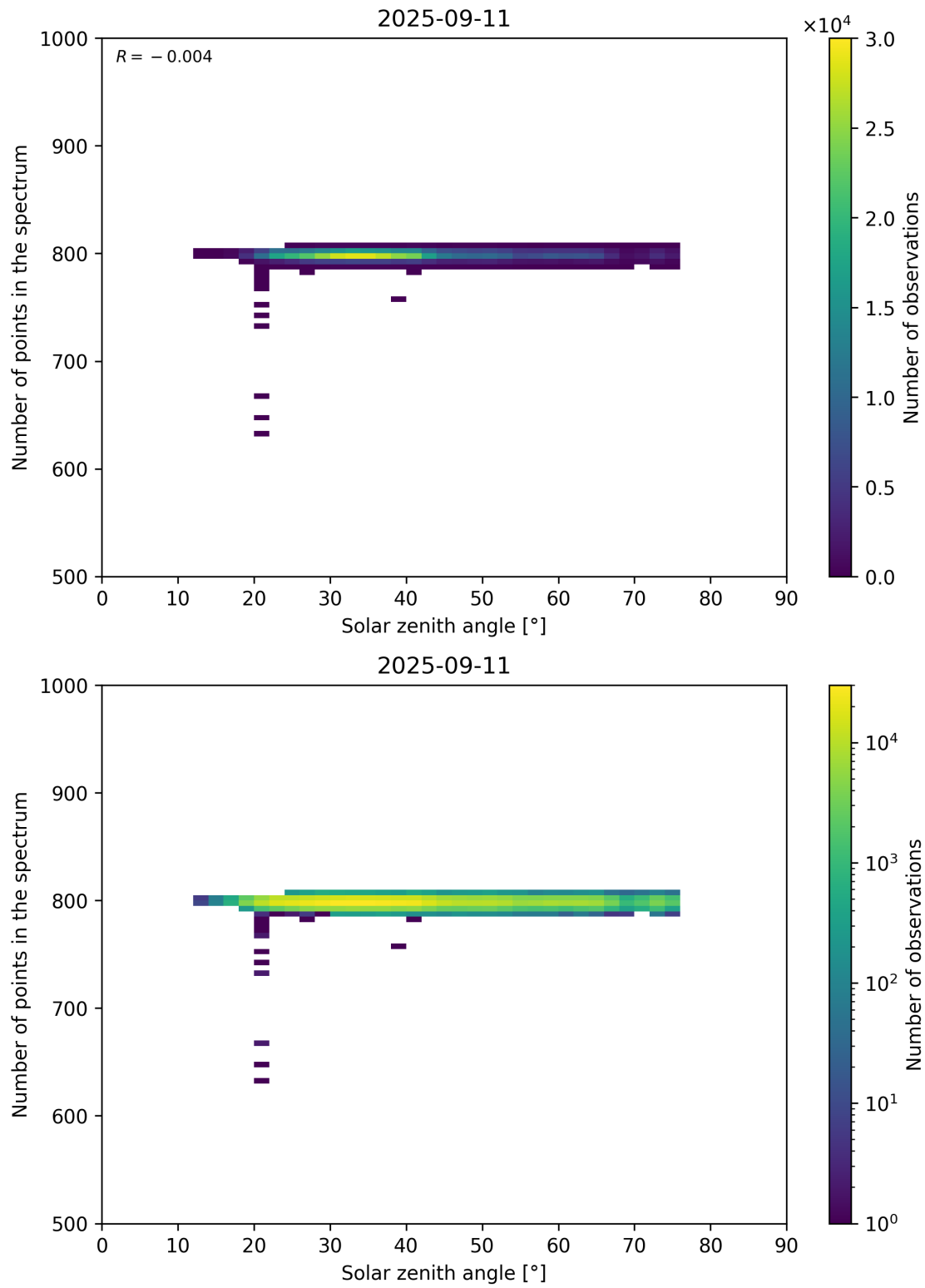
Figure 103: Scatter density plot of “Solar zenith angle” against “Number of points in the spectrum” for 2025-09-10 to 2025-09-12.
