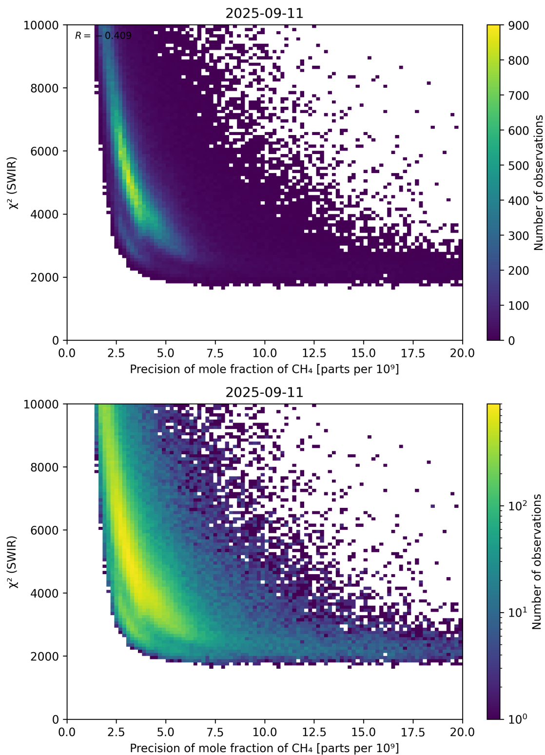
Figure 79: Scatter density plot of “Precision of mole fraction of \text{CH}_4 ” against “ \chi^2 (SWIR)” for 2025-09-10 to 2025-09-12.
