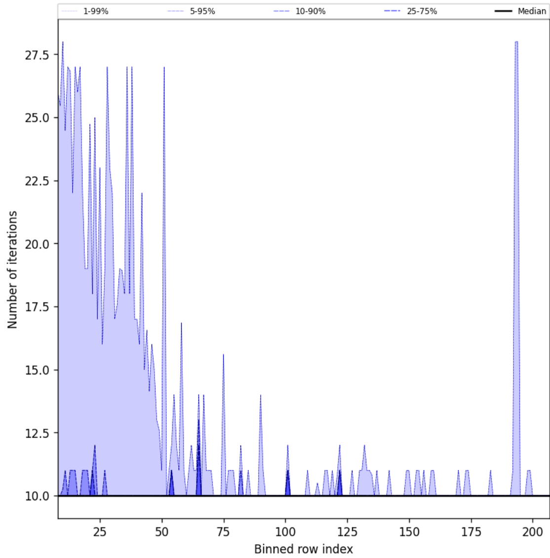
Figure 42: Along track statistics of “Number of iterations” for 2025-09-10 to 2025-09-12
