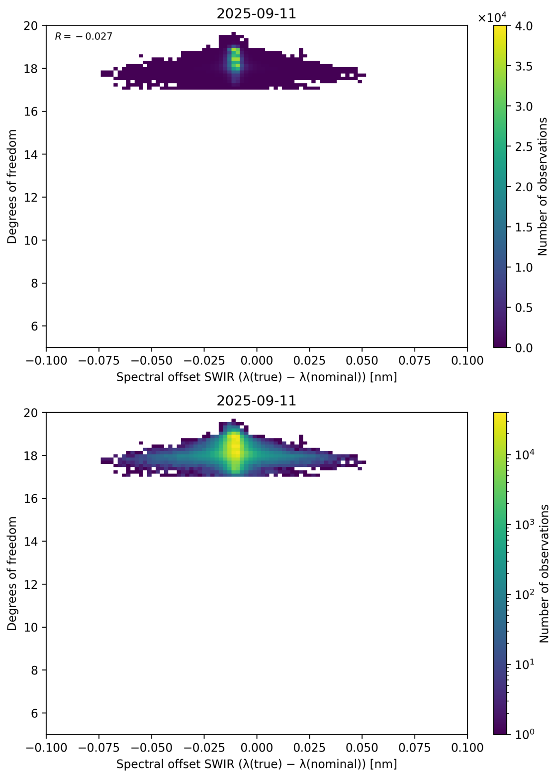
Figure 119: Scatter density plot of “Spectral offset SWIR ( \lambda_{\text{true}} - \lambda_{\text{nominal}} )” against “Degrees of freedom” for 2025-09-10 to 2025-09-12.
