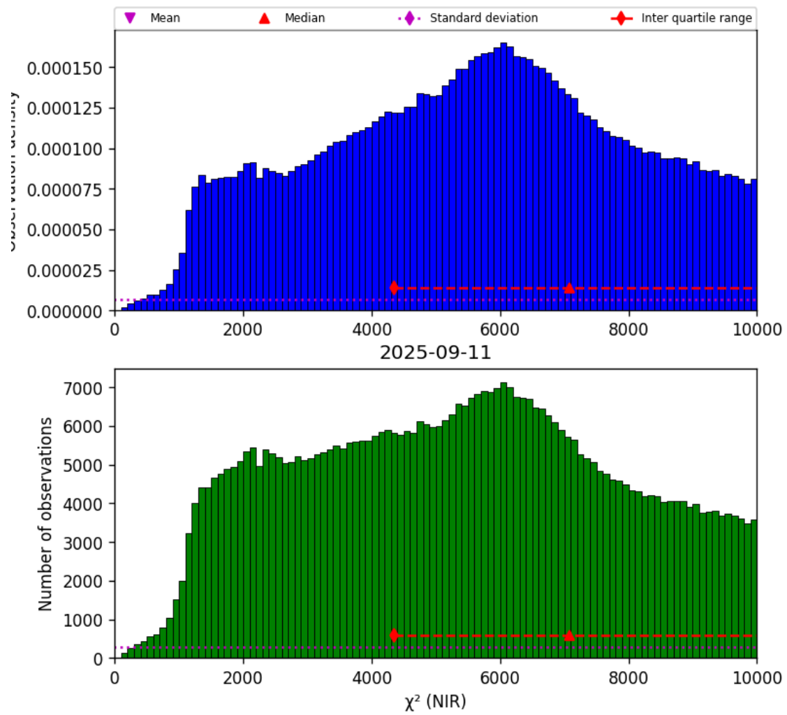
Figure 29: Histogram of “ \chi^2 (NIR)” for 2025-09-10 to 2025-09-12
