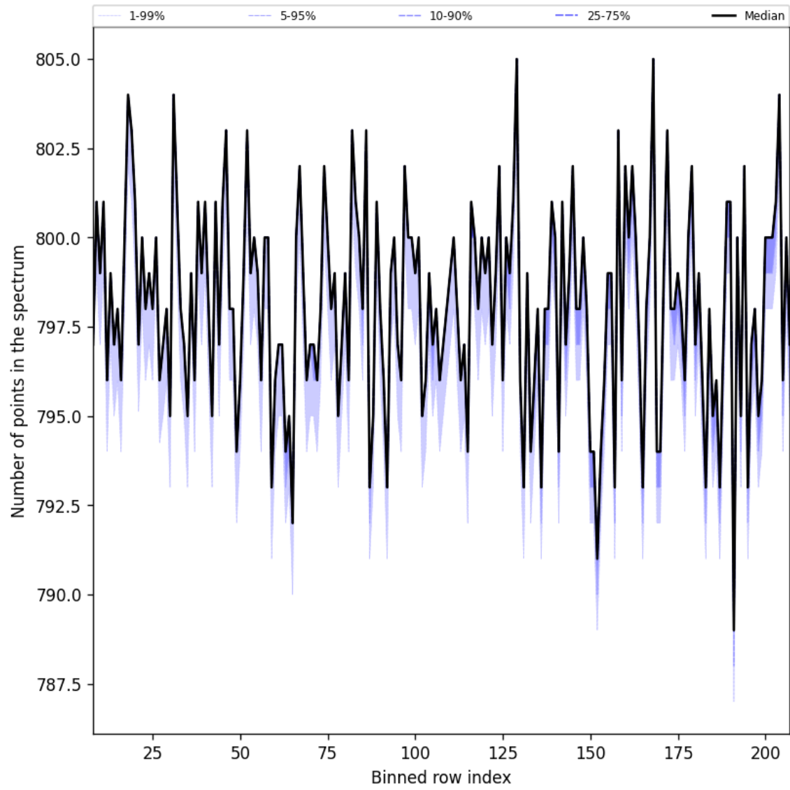
Figure 37: Along track statistics of “Number of points in the spectrum” for 2025-09-10 to 2025-09-12
