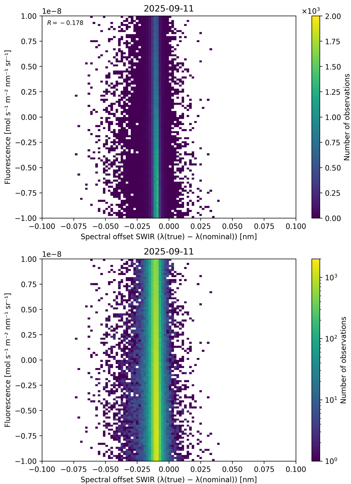
Figure 120: Scatter density plot of “Spectral offset SWIR ( \lambda_{\text{true}} - \lambda_{\text{nominal}} )” against “Fluorescence” for 2025-09-10 to 2025-09-12.
