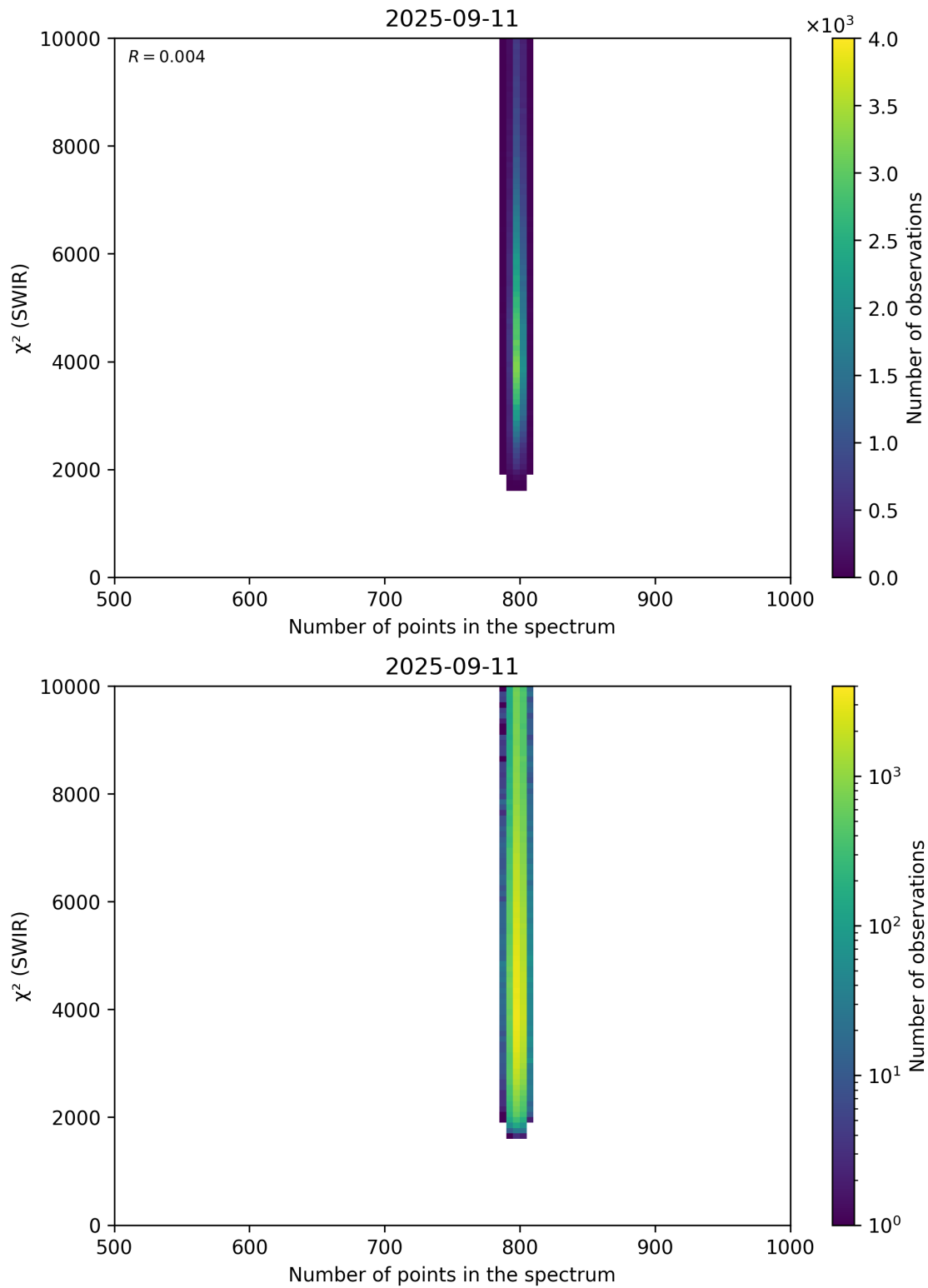
Figure 89: Scatter density plot of “Number of points in the spectrum” against “ \chi^2 (SWIR)” for 2025-09-10 to 2025-09-12.
