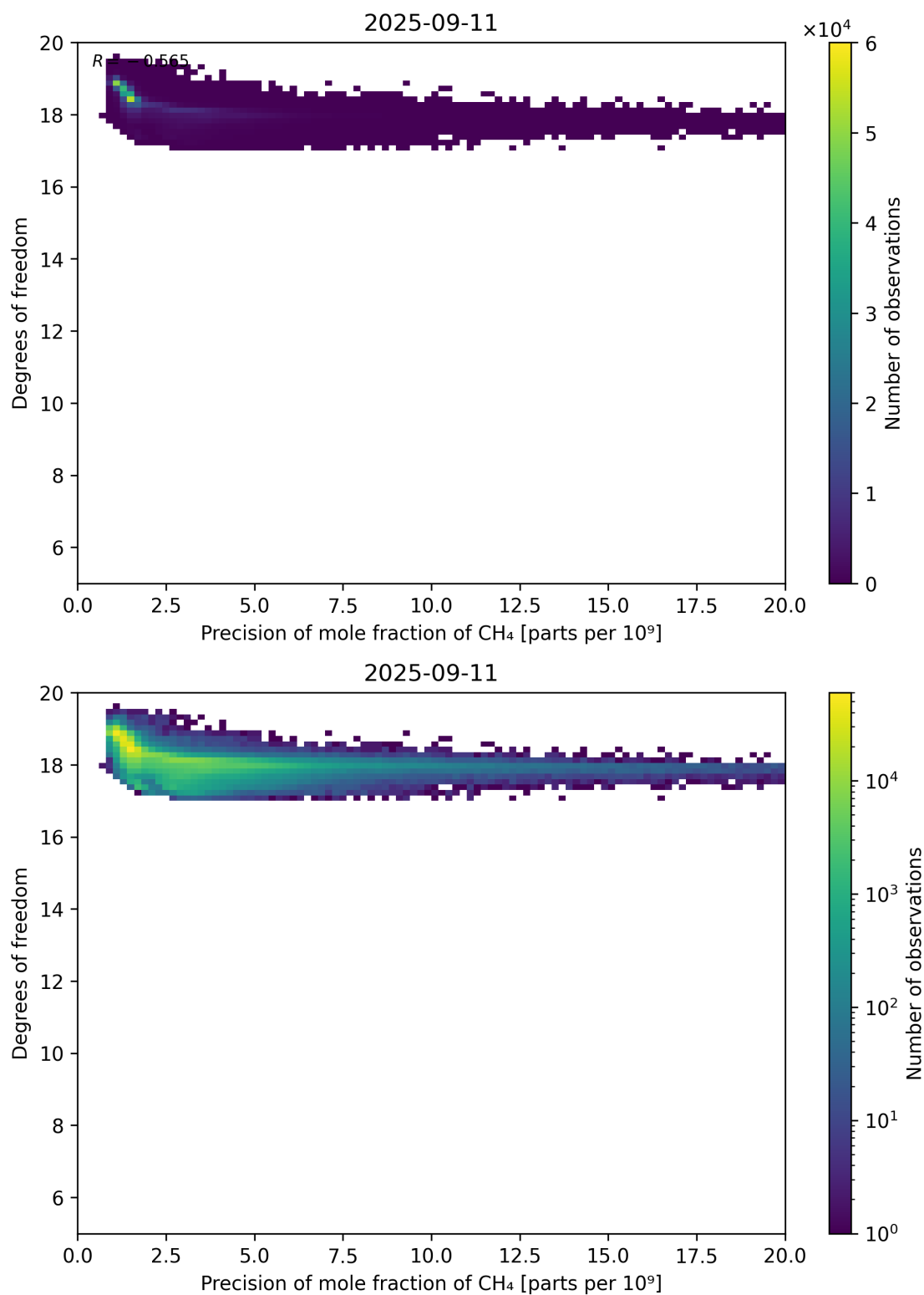
Figure 80: Scatter density plot of “Precision of mole fraction of CH 4 ” against “Degrees of freedom” for 2025-09-10 to 2025-09-12.
