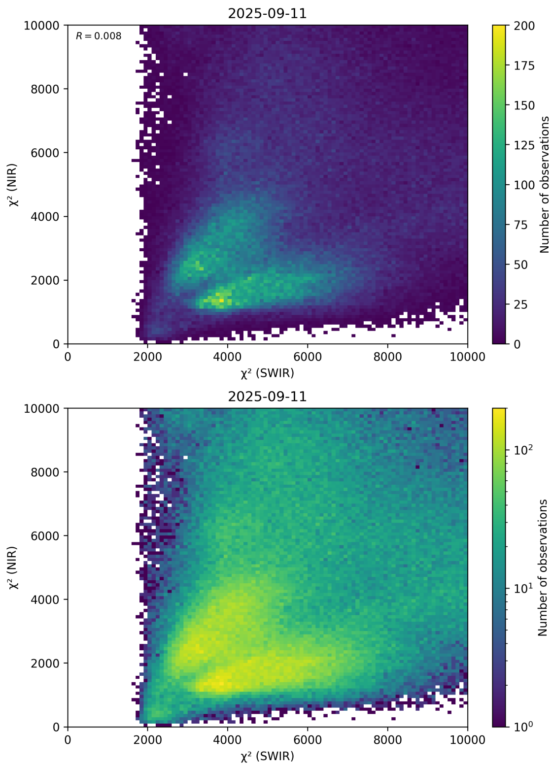
Figure 47: Scatter density plot of “ \chi^2 (SWIR)” against “ \chi^2 (NIR)” for 2025-09-10 to 2025-09-12.
