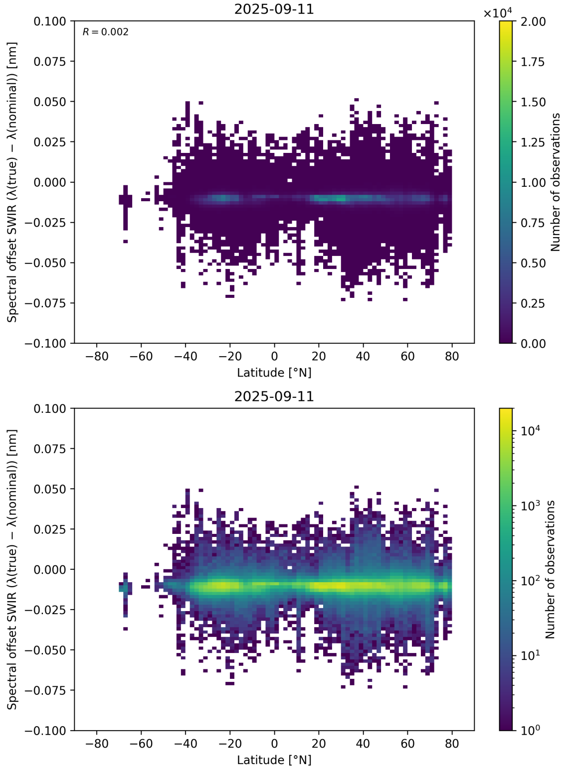
Figure 62: Scatter density plot of “Latitude” against “Spectral offset SWIR ( \lambda_{\text{true}} - \lambda_{\text{nominal}} )” for 2025-09-10 to 2025-09-12.
