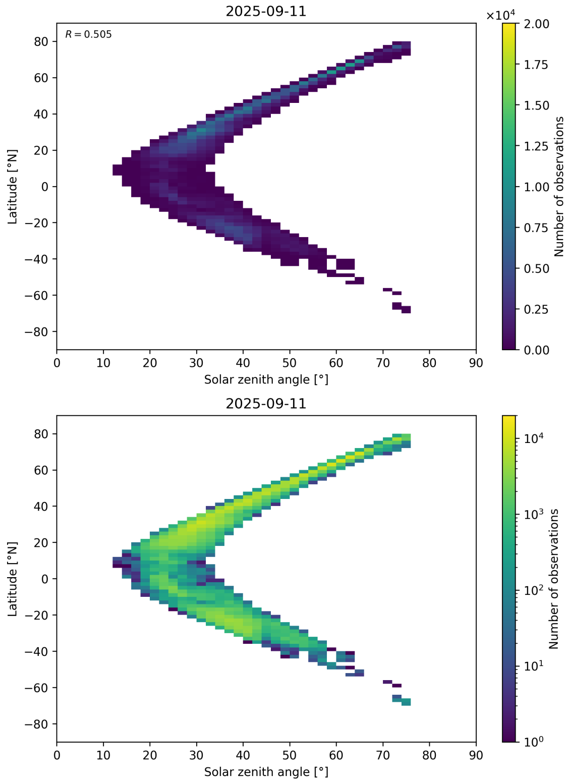
Figure 98: Scatter density plot of “Solar zenith angle” against “Latitude” for 2025-09-10 to 2025-09-12.
