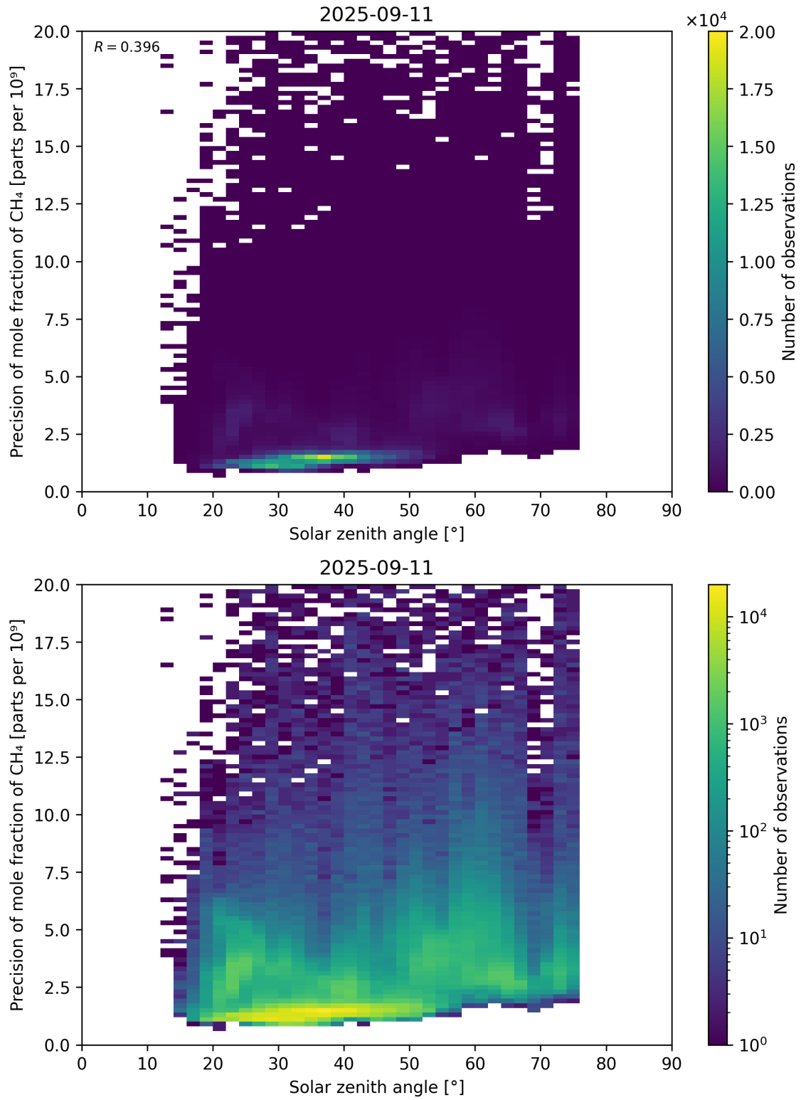
Figure 101: Scatter density plot of “Solar zenith angle” against “Precision of mole fraction of CH 4 ” for 2025-09-10 to 2025-09-12.
