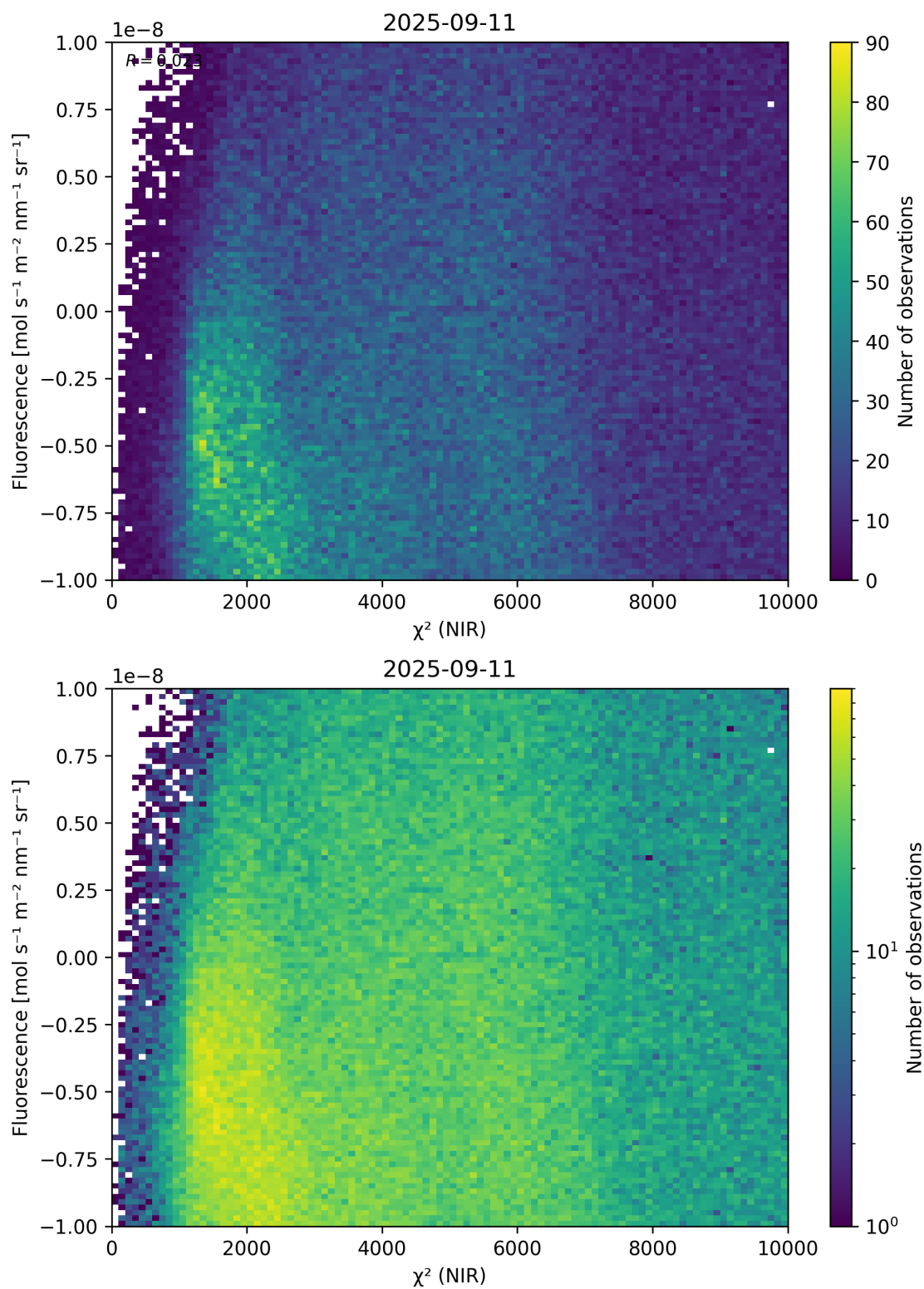
Figure 45: Scatter density plot of “ \chi^2 (NIR)” against “Fluorescence” for 2025-09-10 to 2025-09-12.
