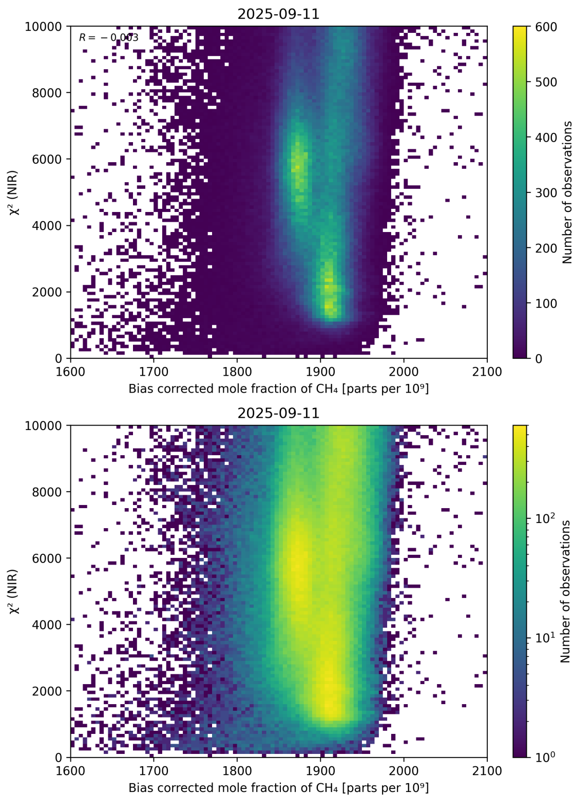
Figure 63: Scatter density plot of “Bias corrected mole fraction of \text{CH}_4 ” against “ \chi^2 (NIR)” for 2025-09-10 to 2025-09-12.
