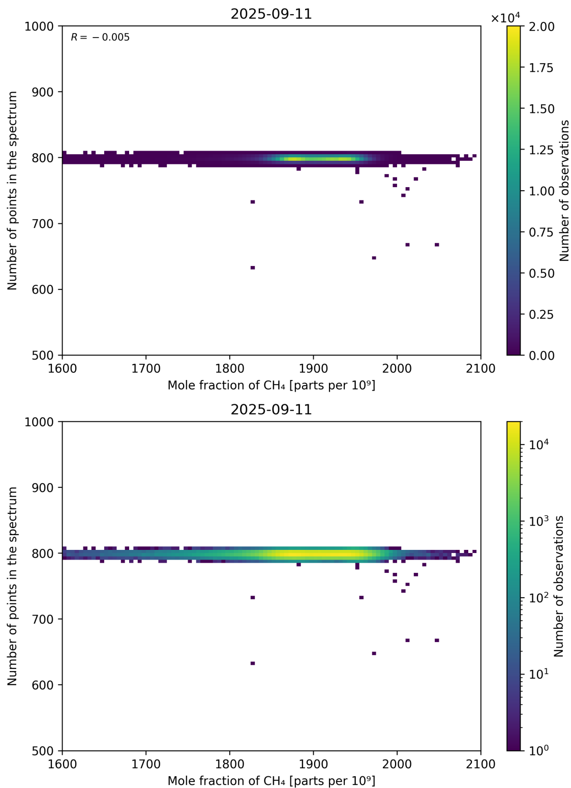
Figure 77: Scatter density plot of “Mole fraction of CH 4 ” against “Number of points in the spectrum” for 2025-09-10 to 2025-09-12.
