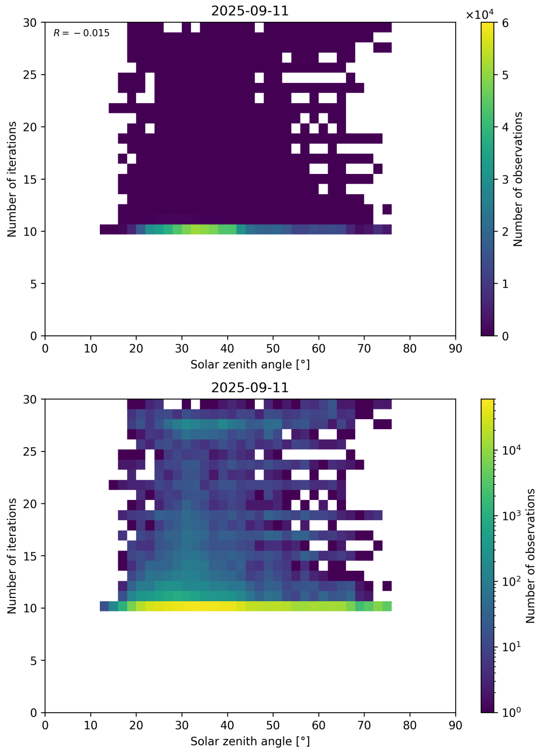
Figure 102: Scatter density plot of “Solar zenith angle” against “Number of iterations” for 2025-09-10 to 2025-09-12.
