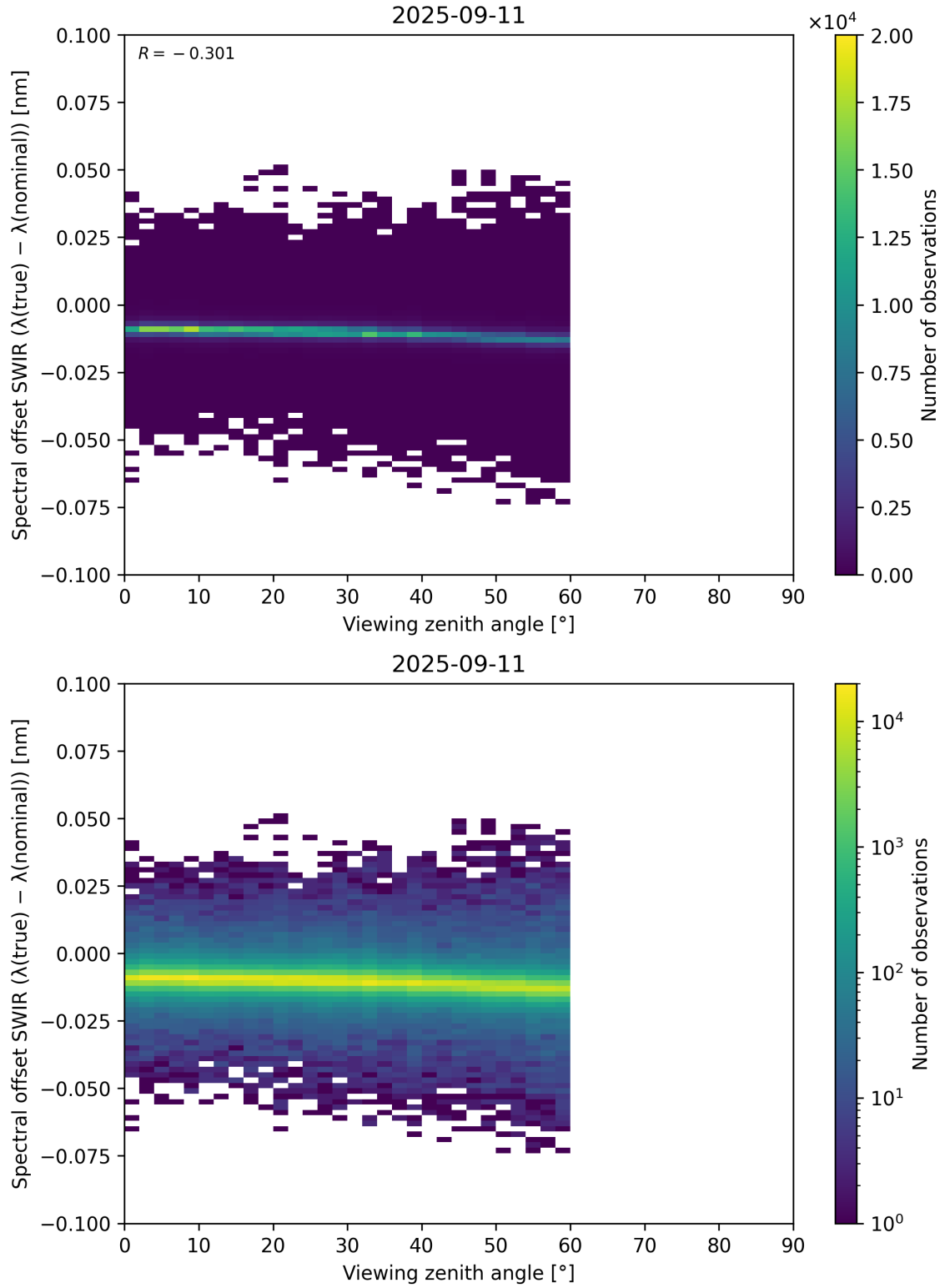
Figure 116: Scatter density plot of “Viewing zenith angle” against “Spectral offset SWIR ( \lambda_{\text{true}} - \lambda_{\text{nominal}} )” for 2025-09-10 to 2025-09-12.
