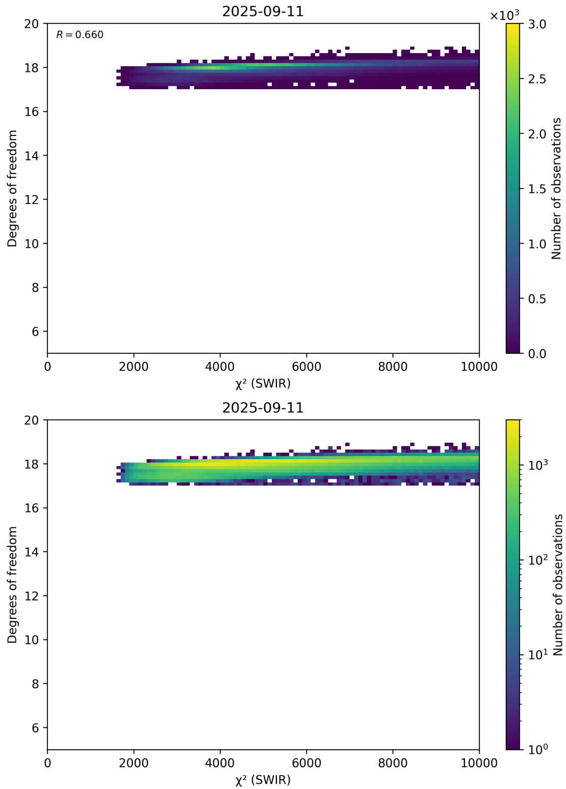
Figure 48: Scatter density plot of “ \chi^2 (SWIR)” against “Degrees of freedom” for 2025-09-10 to 2025-09-12.
