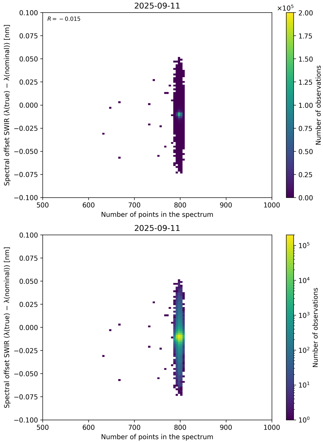
Figure 93: Scatter density plot of “Number of points in the spectrum” against “Spectral offset SWIR ( \lambda_{\text{true}} - \lambda_{\text{nominal}} )” for 2025-09-10 to 2025-09-12.
