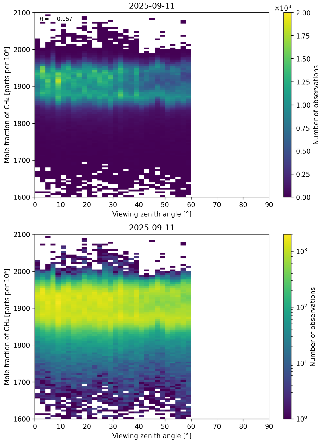
Figure 110: Scatter density plot of “Viewing zenith angle” against “Mole fraction of CH 4 ” for 2025-09-10 to 2025-09-12.
