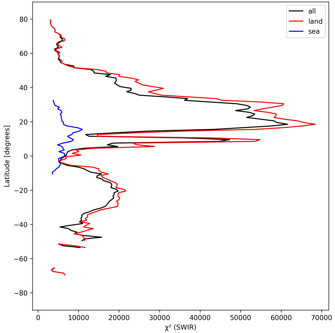
Figure 17: Zonal average of “ \chi^2 (SWIR)” for 2025-09-10 to 2025-09-12.
