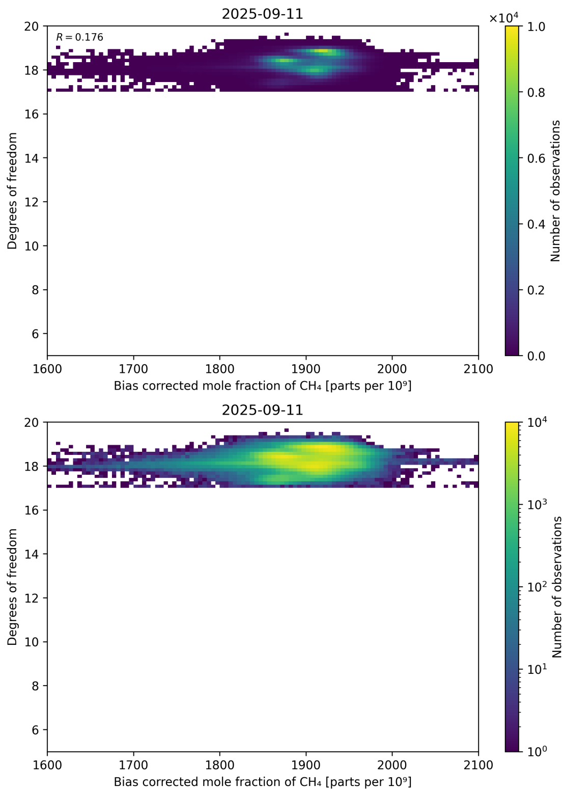
Figure 65: Scatter density plot of “Bias corrected mole fraction of CH 4 ” against “Degrees of freedom” for 2025-09-10 to 2025-09-12.
