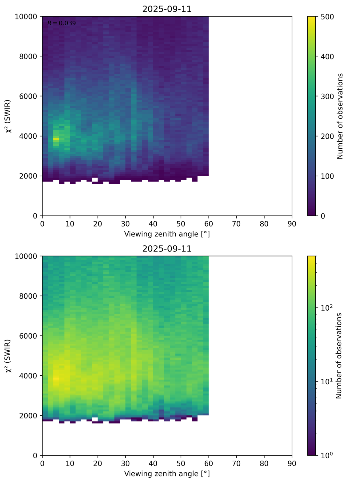
Figure 106: Scatter density plot of “Viewing zenith angle” against “ \chi^2 (SWIR)” for 2025-09-10 to 2025-09-12.
