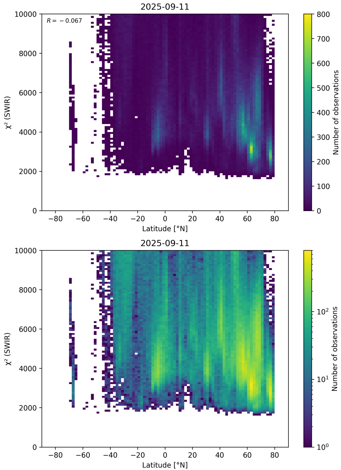
Figure 54: Scatter density plot of “Latitude” against “ \chi^2 (SWIR)” for 2025-09-10 to 2025-09-12.
