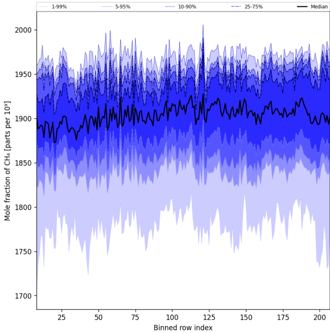
Figure 34: Along track statistics of “Mole fraction of CH 4 ” for 2025-09-10 to 2025-09-12
