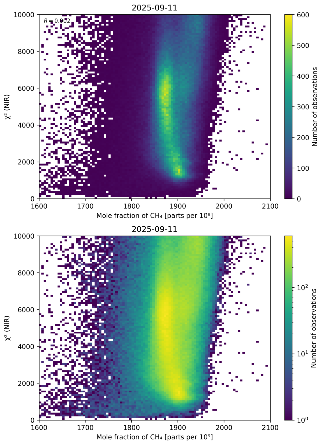
Figure 70: Scatter density plot of “Mole fraction of \text{CH}_4 ” against “ \chi^2 (NIR)” for 2025-09-10 to 2025-09-12.
