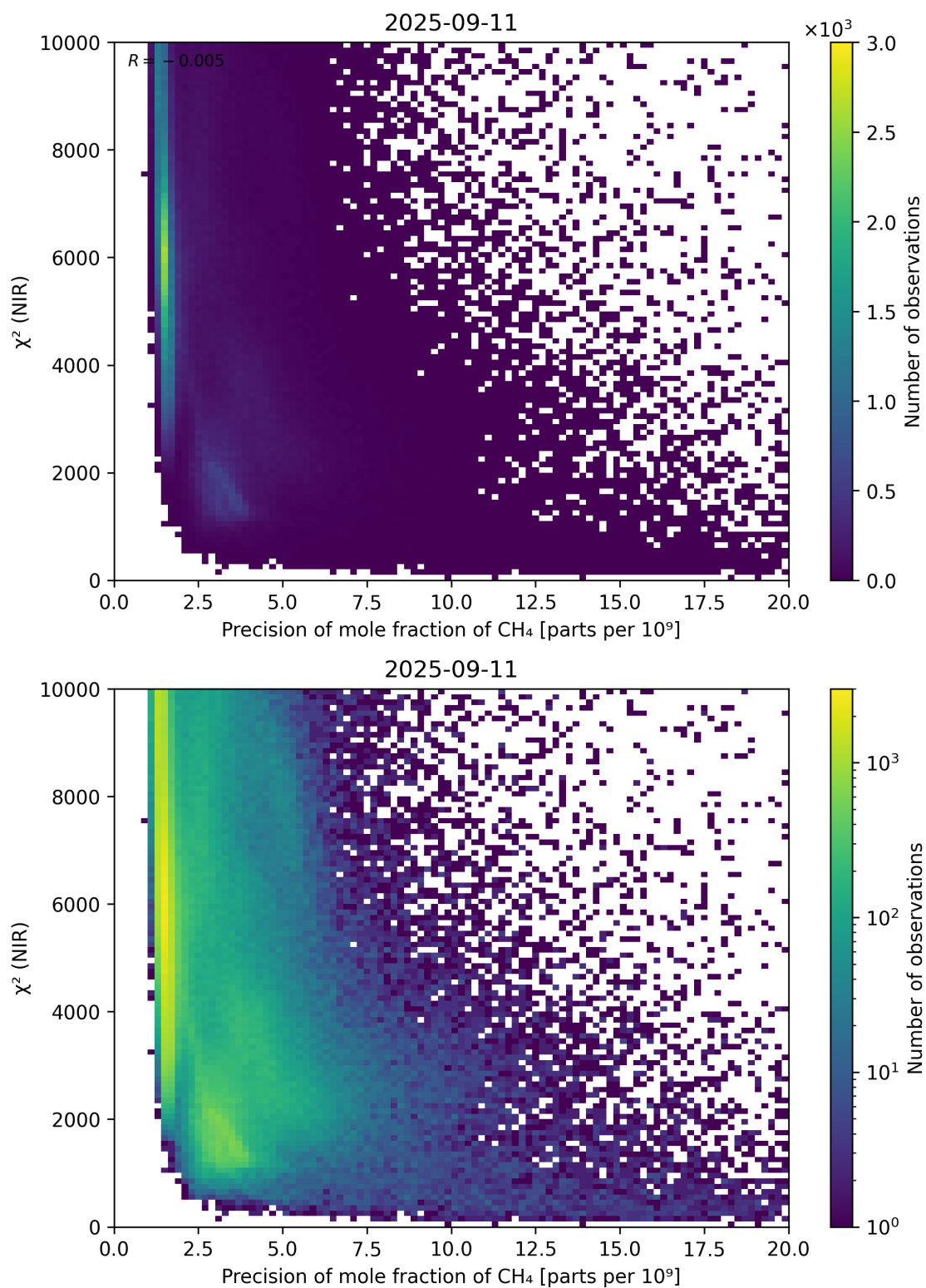
Figure 78: Scatter density plot of “Precision of mole fraction of \text{CH}_4 ” against “ \chi^2 (NIR)” for 2025-09-10 to 2025-09-12.
