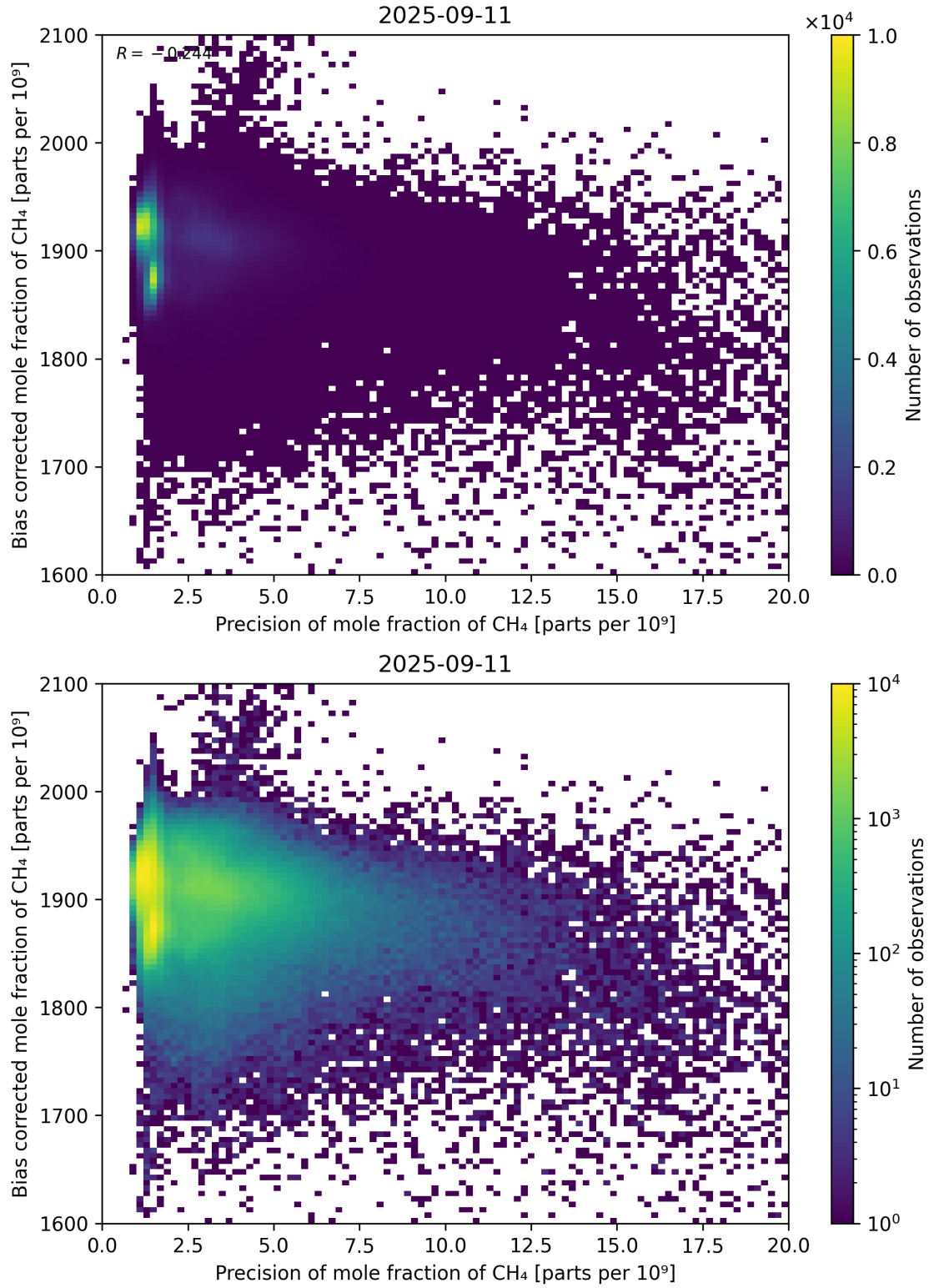
Figure 82: Scatter density plot of “Precision of mole fraction of \text{CH}_4 ” against “Bias corrected mole fraction of \text{CH}_4 ” for 2025-09-10 to 2025-09-12.
