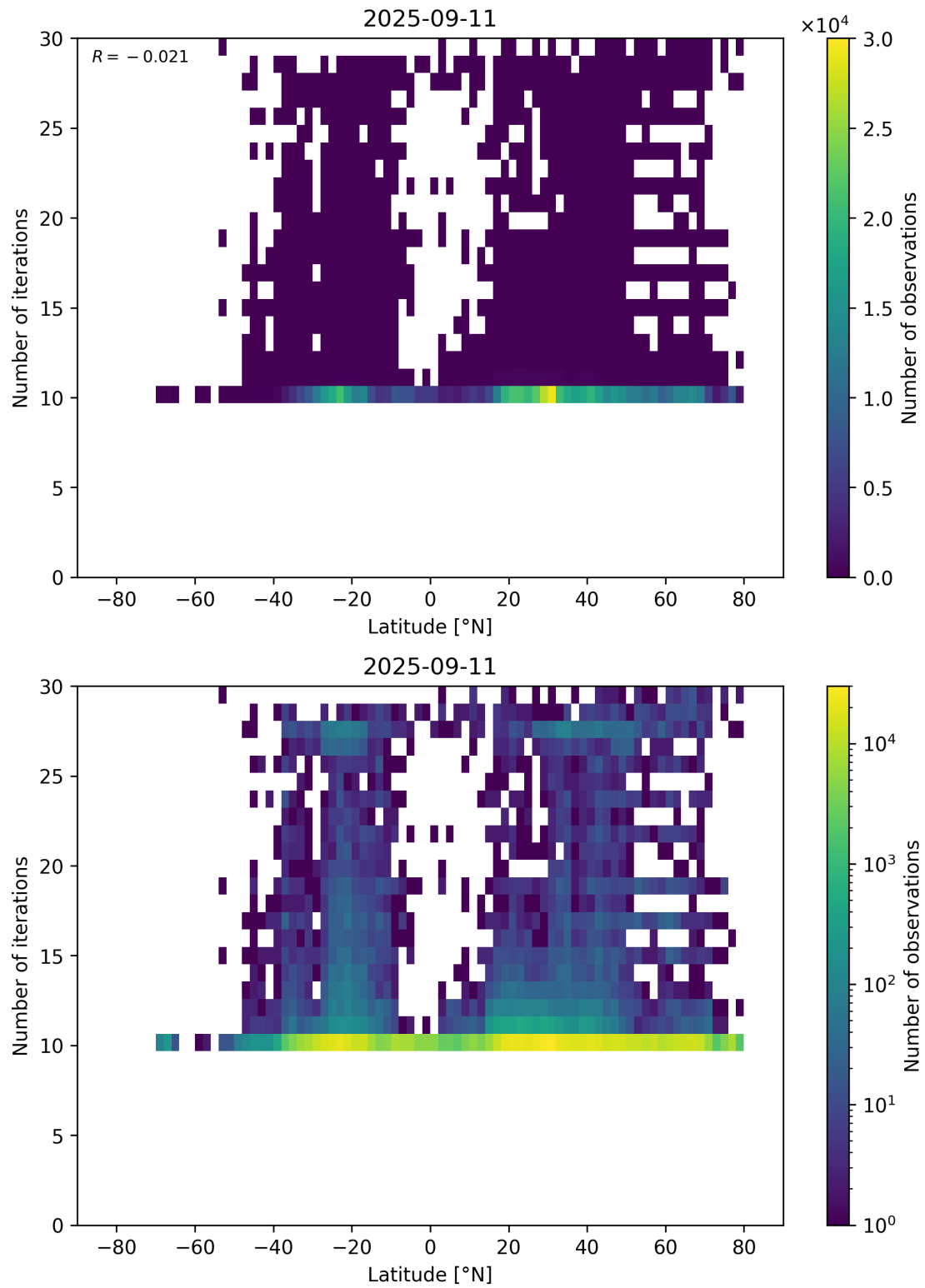
Figure 60: Scatter density plot of “Latitude” against “Number of iterations” for 2025-09-10 to 2025-09-12.
