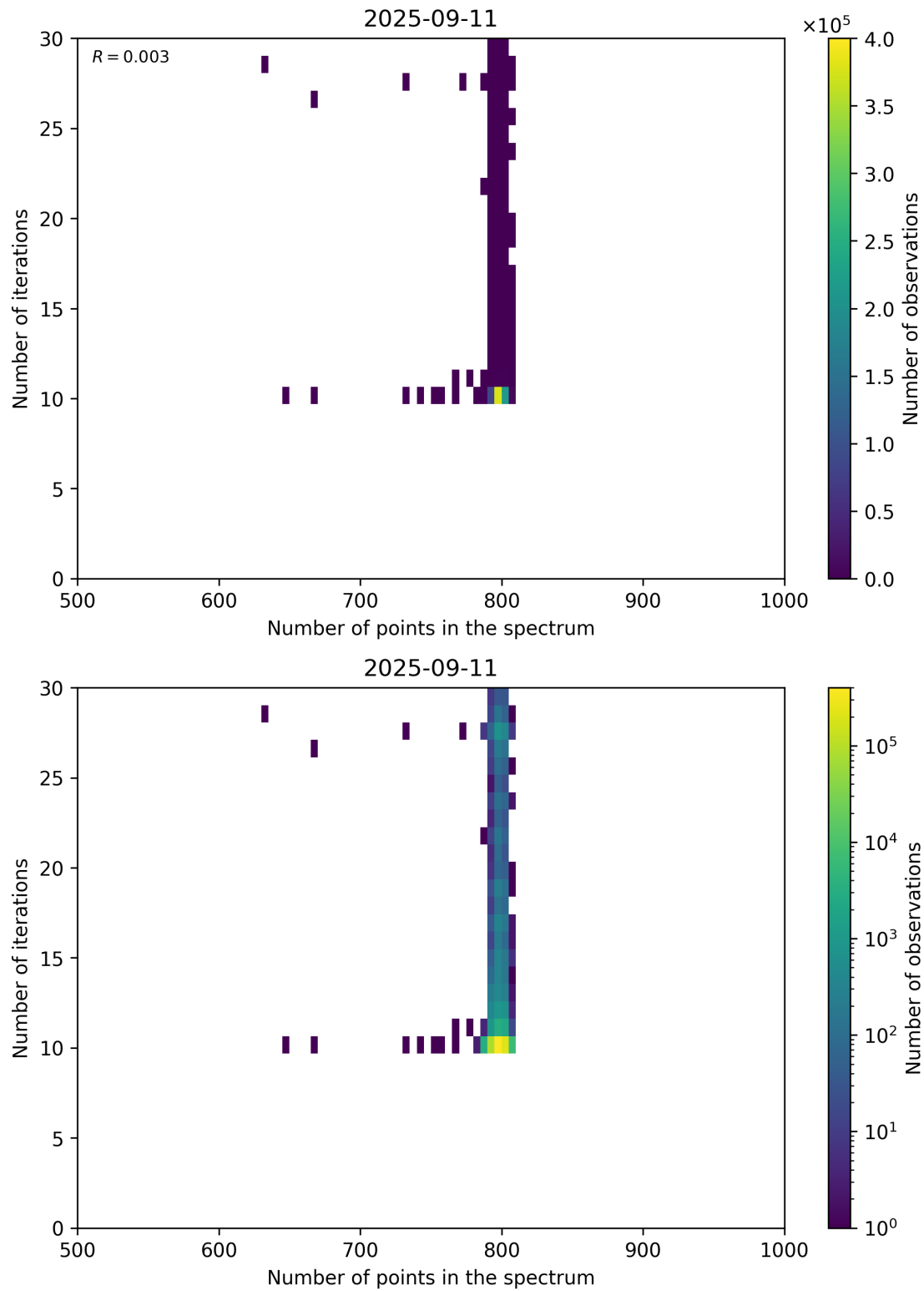
Figure 92: Scatter density plot of “Number of points in the spectrum” against “Number of iterations” for 2025-09-10 to 2025-09-12.
