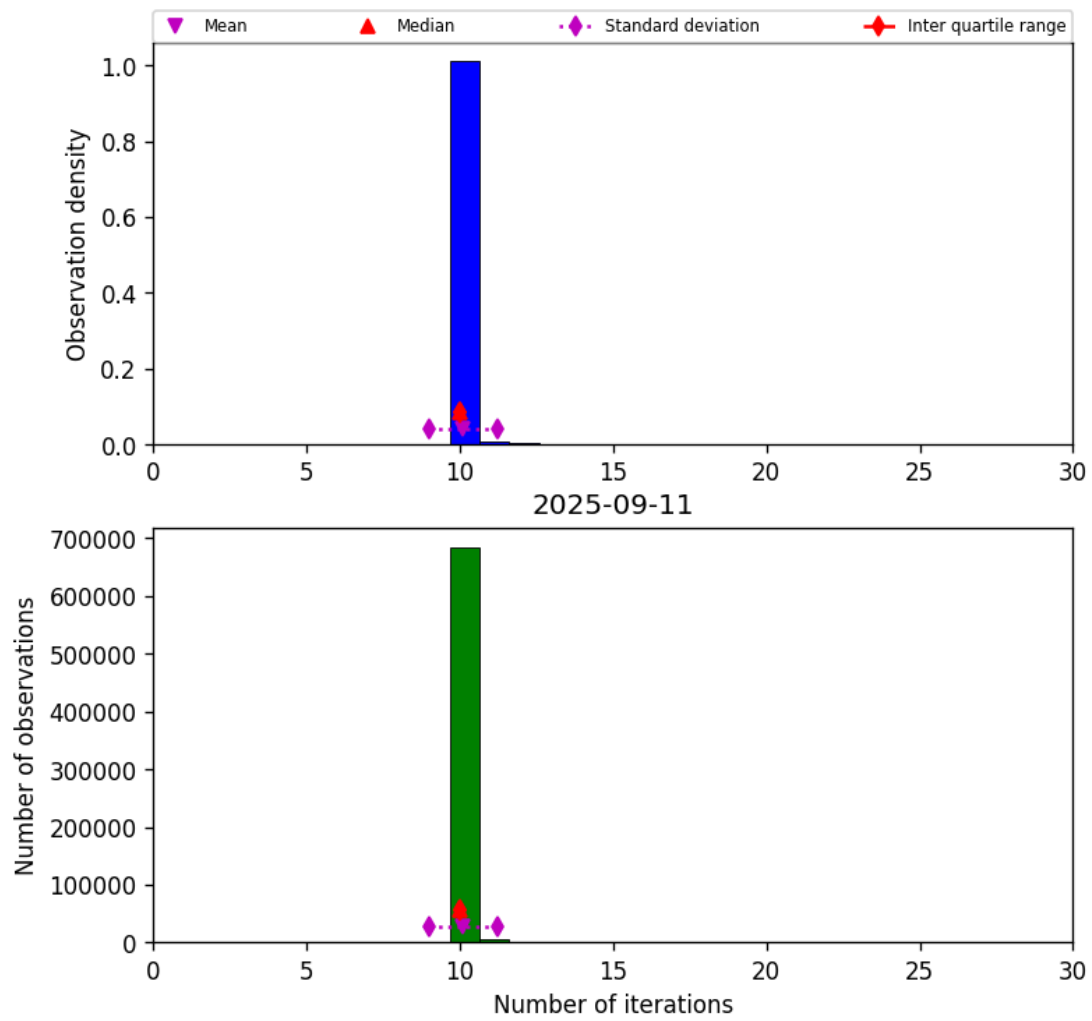
Figure 31: Histogram of “Number of iterations” for 2025-09-10 to 2025-09-12
