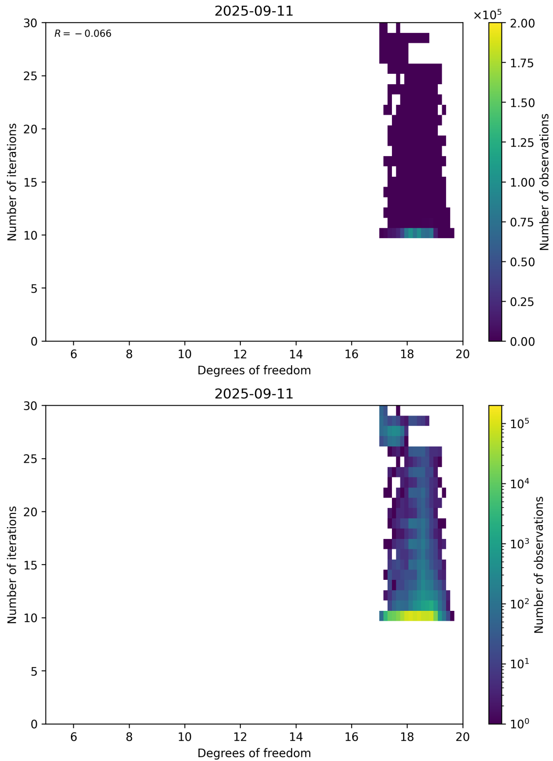
Figure 52: Scatter density plot of “Degrees of freedom” against “Number of iterations” for 2025-09-10 to 2025-09-12.
