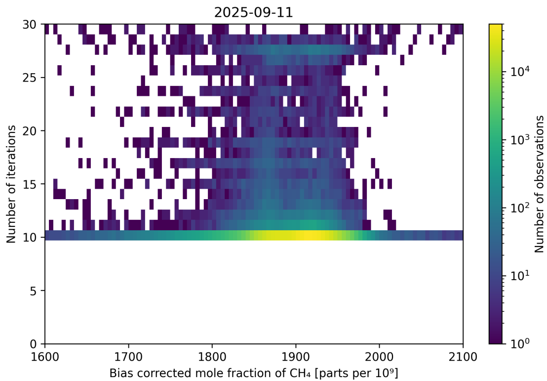
Figure 67: Scatter density plot of “Bias corrected mole fraction of CH 4 ” against “Number of iterations” for 2025-09-10 to 2025-09-12.
