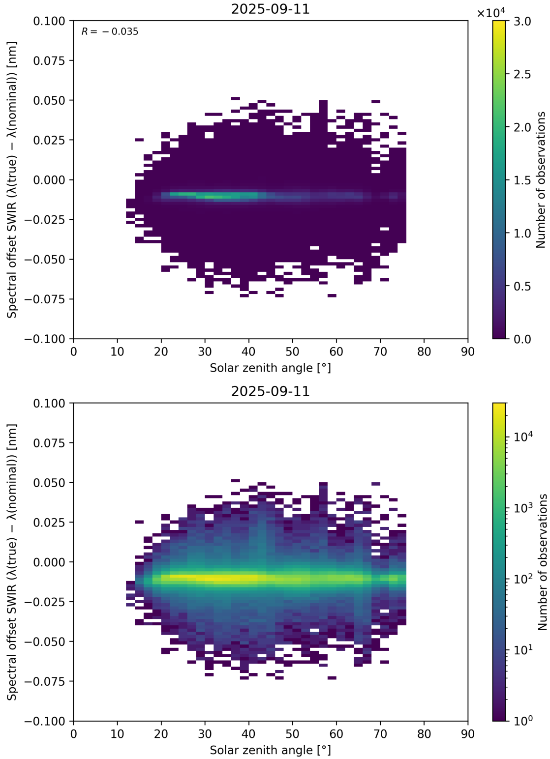
Figure 104: Scatter density plot of “Solar zenith angle” against “Spectral offset SWIR ( \lambda_{\text{true}} - \lambda_{\text{nominal}} )” for 2025-09-10 to 2025-09-12.
