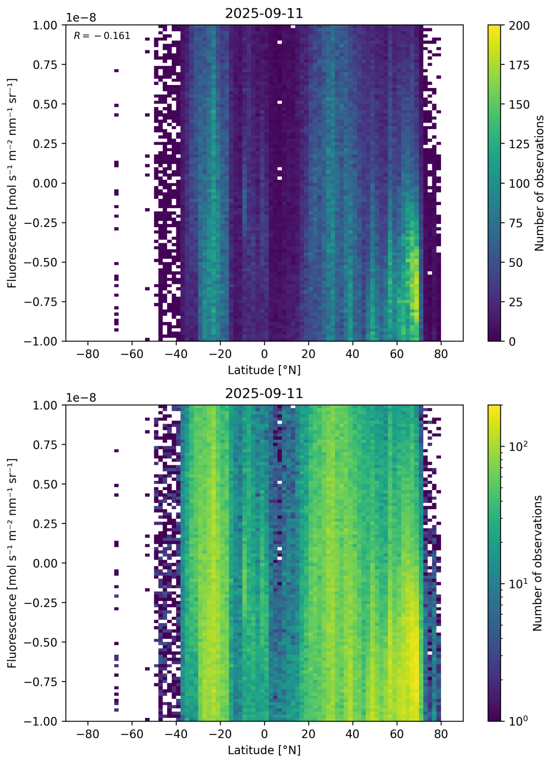
Figure 56: Scatter density plot of “Latitude” against “Fluorescence” for 2025-09-10 to 2025-09-12.
