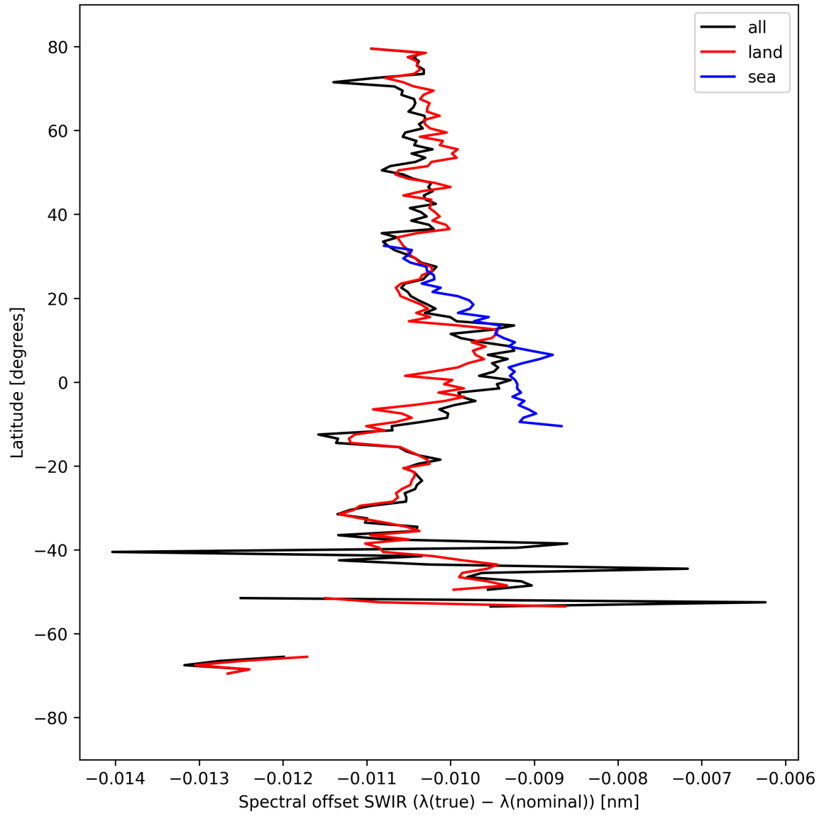
Figure 16: Zonal average of “Spectral offset SWIR ( \lambda_{\text{true}} - \lambda_{\text{nominal}} )” for 2025-09-10 to 2025-09-12.
