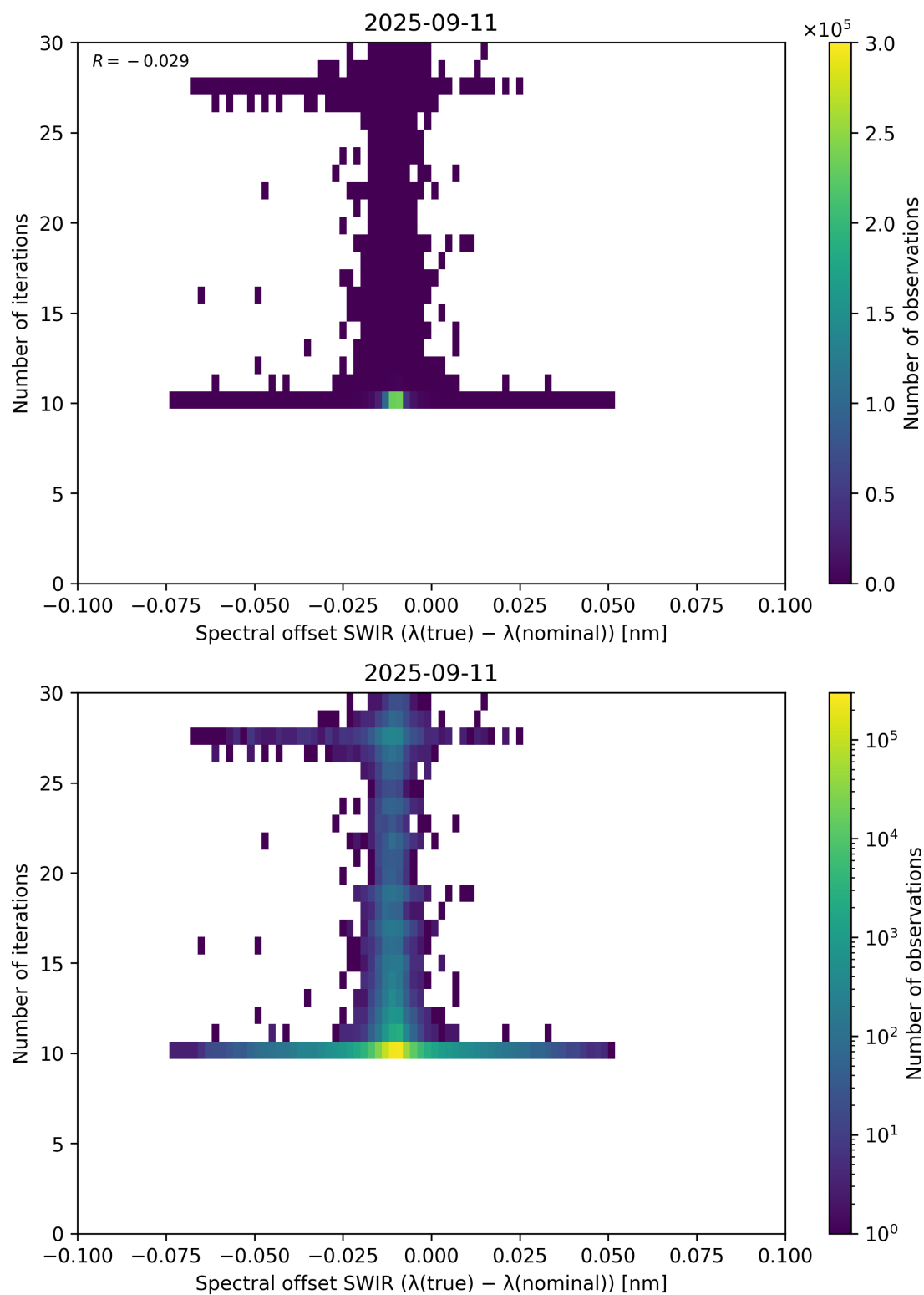
Figure 121: Scatter density plot of “Spectral offset SWIR ( \lambda_{\text{true}} - \lambda_{\text{nominal}} )” against “Number of iterations” for 2025-09-10 to 2025-09-12.
