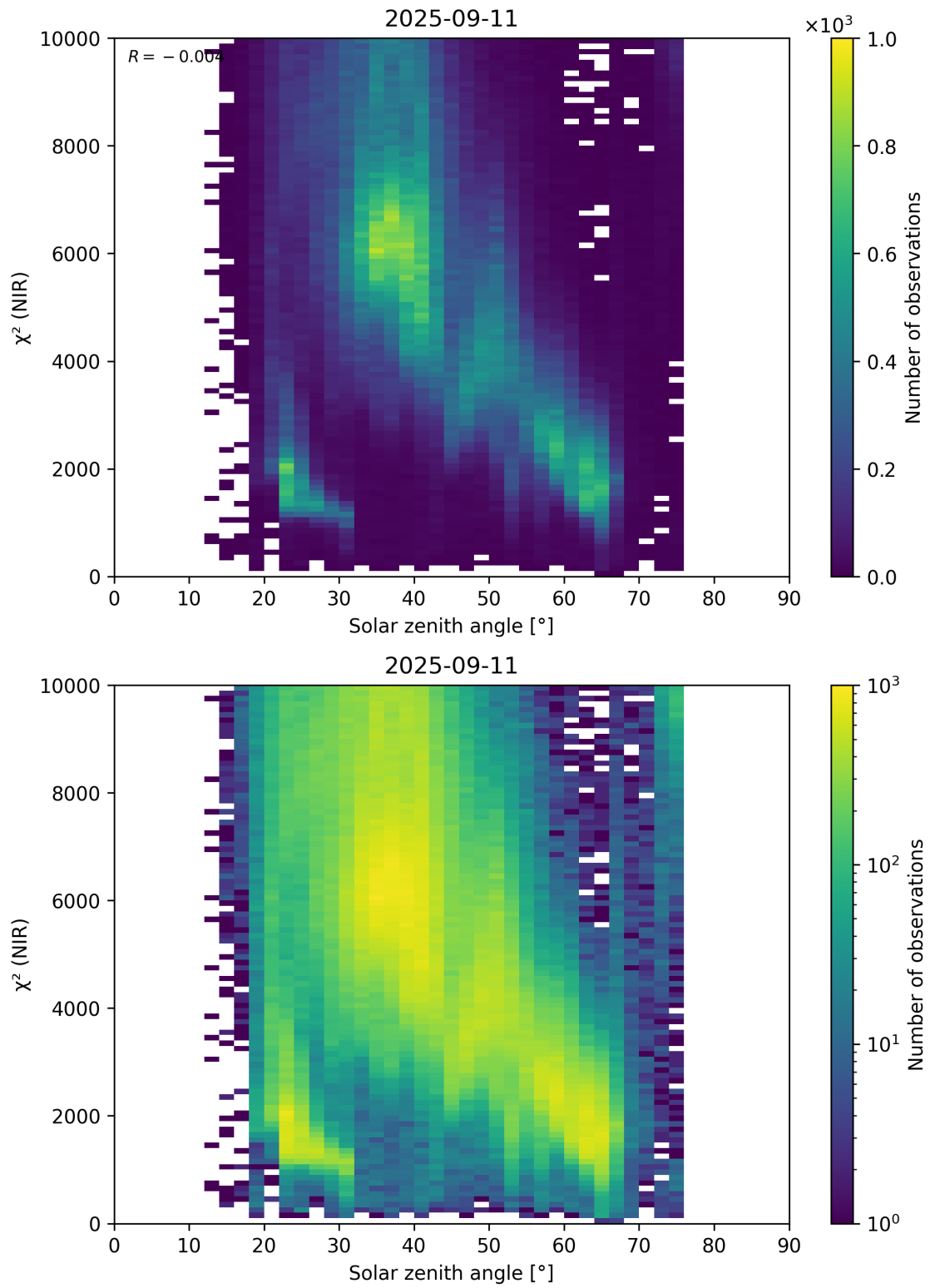
Figure 94: Scatter density plot of “Solar zenith angle” against “ \chi^2 (NIR)” for 2025-09-10 to 2025-09-12.
