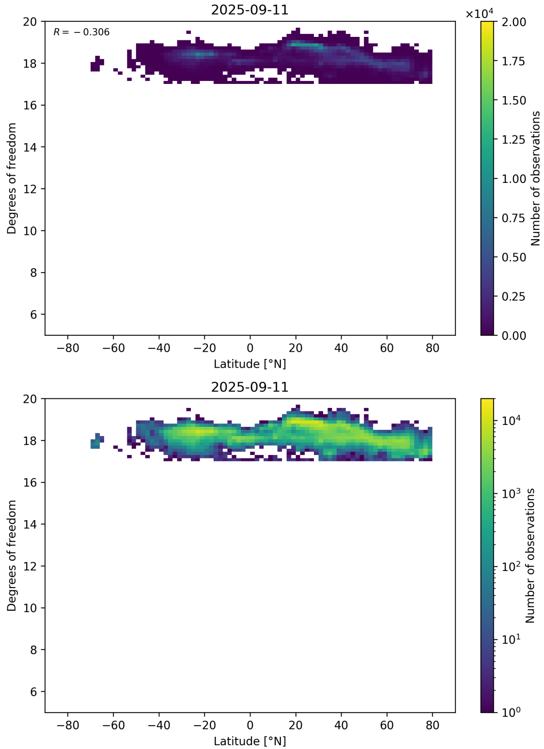
Figure 55: Scatter density plot of “Latitude” against “Degrees of freedom” for 2025-09-10 to 2025-09-12.
