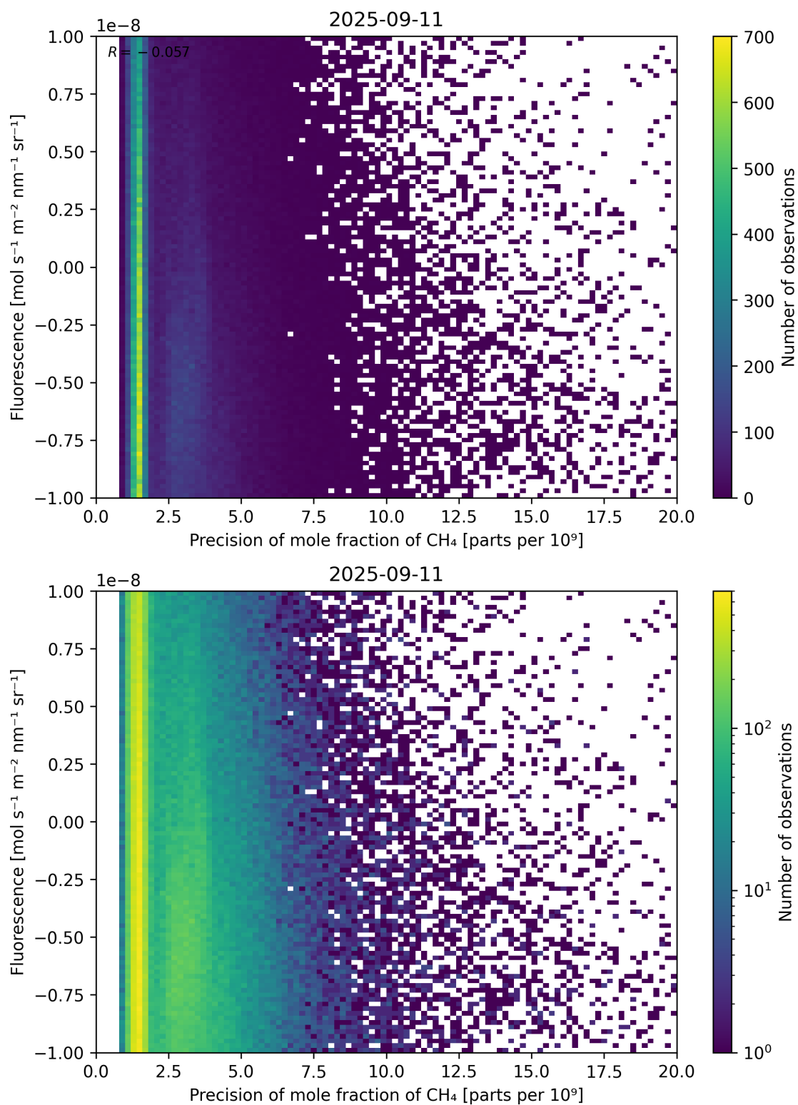
Figure 81: Scatter density plot of “Precision of mole fraction of \text{CH}_4 ” against “Fluorescence” for 2025-09-10 to 2025-09-12.
