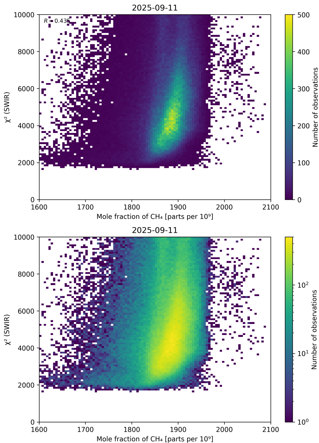
Figure 71: Scatter density plot of “Mole fraction of \text{CH}_4 ” against “ \chi^2 (SWIR)” for 2025-09-10 to 2025-09-12.
