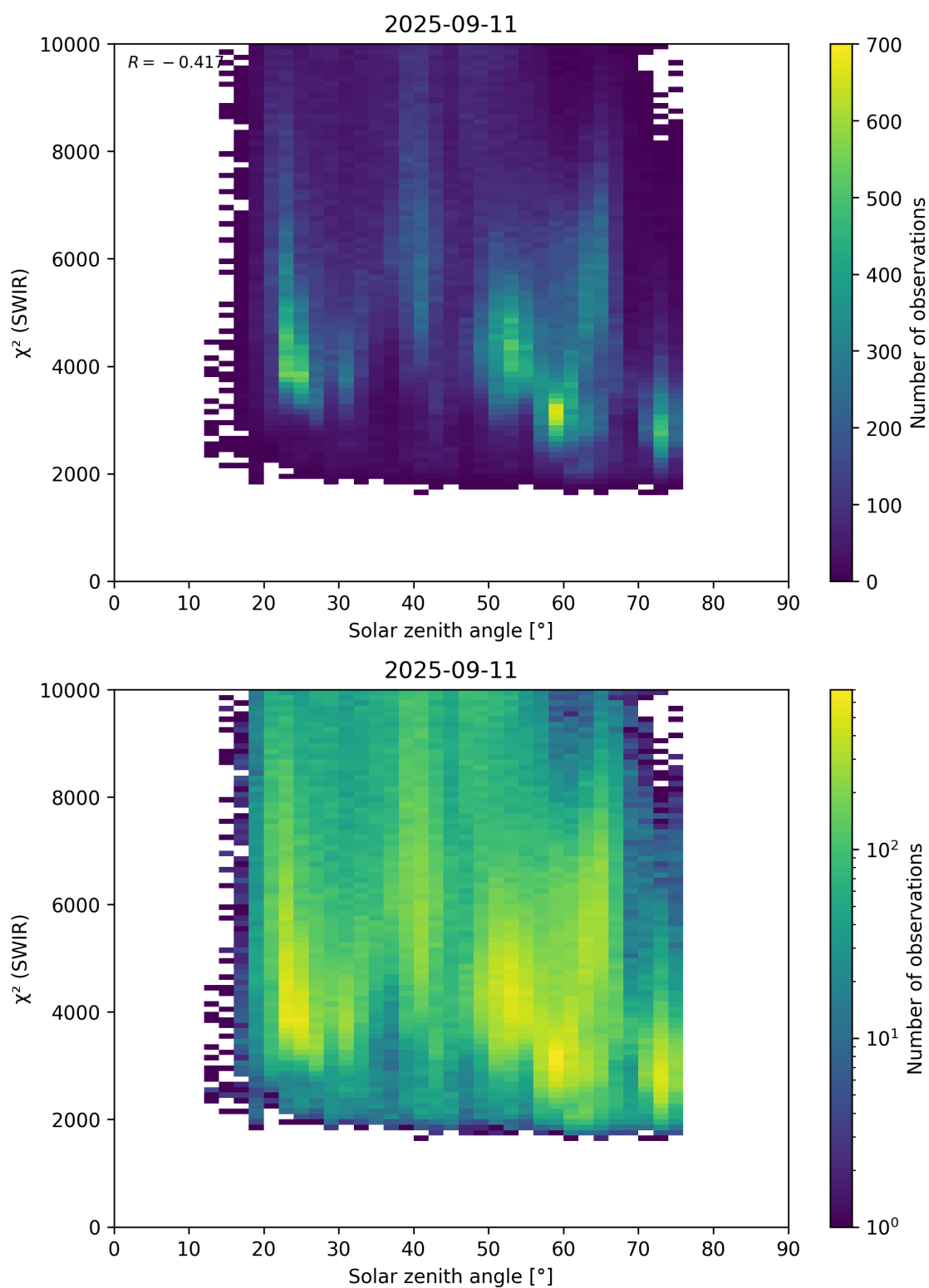
Figure 95: Scatter density plot of “Solar zenith angle” against “ \chi^2 (SWIR)” for 2025-09-10 to 2025-09-12.
