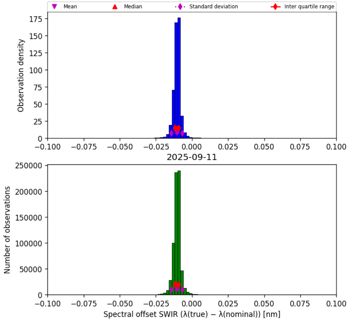
Figure 27: Histogram of “Spectral offset SWIR ( \lambda_{\text{true}} - \lambda_{\text{nominal}} )” for 2025-09-10 to 2025-09-12
