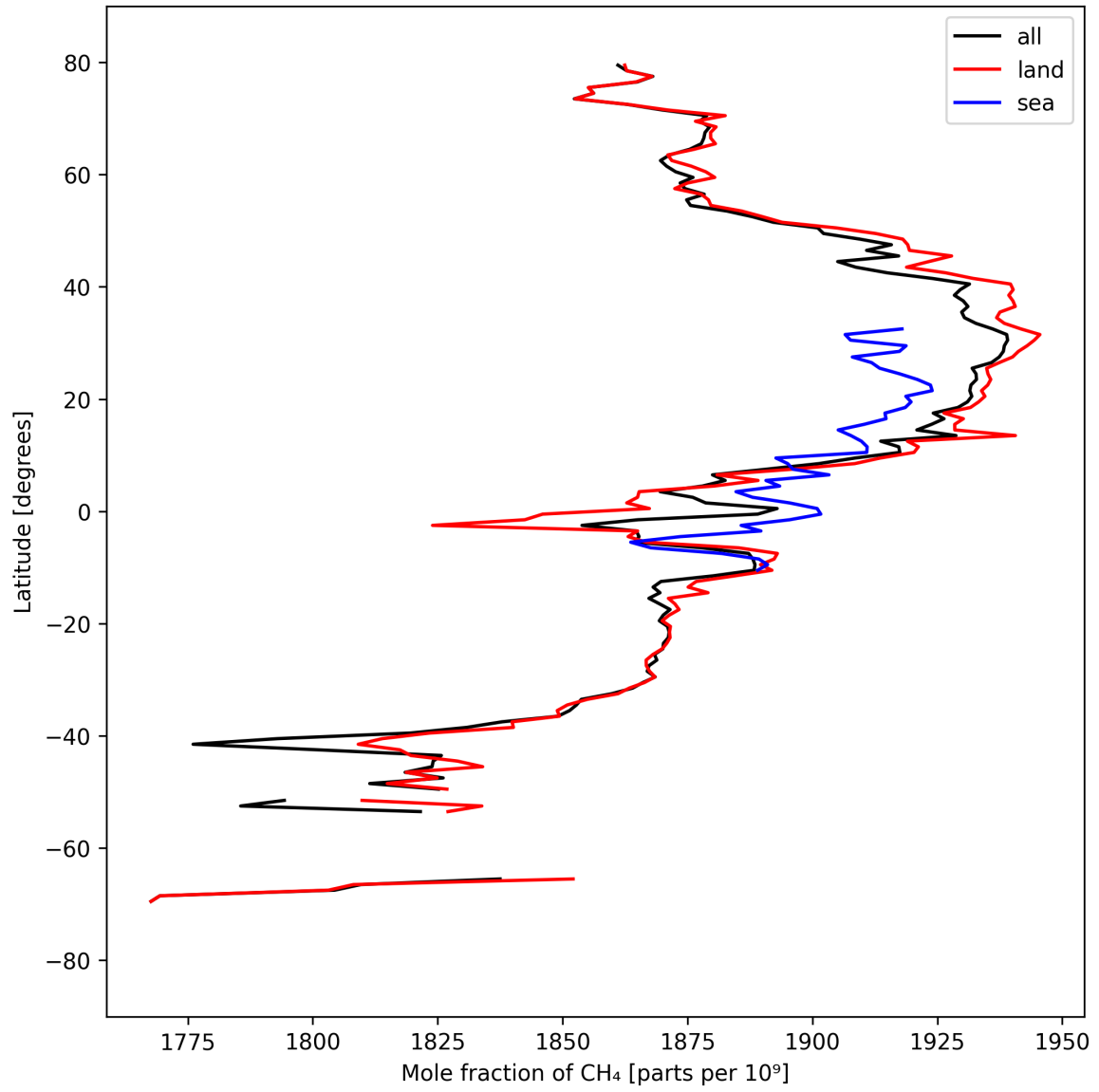
Figure 12: Zonal average of “Mole fraction of \text{CH}_4 ” for 2025-09-10 to 2025-09-12.
