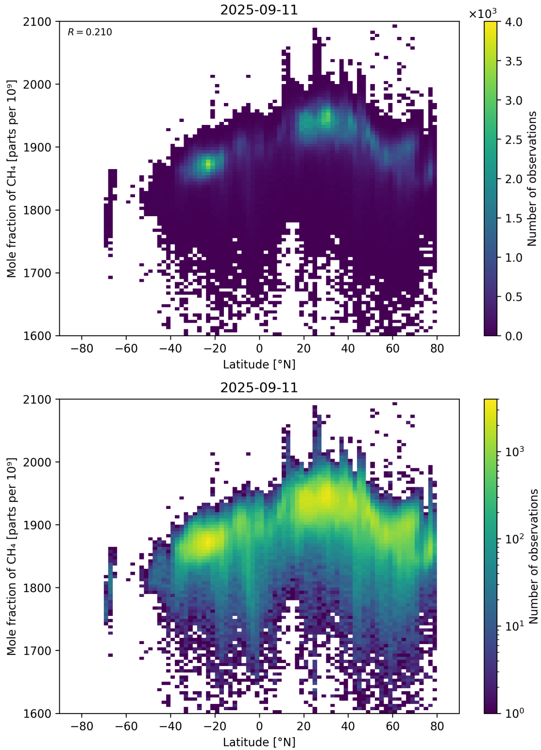
Figure 57: Scatter density plot of “Latitude” against “Mole fraction of CH 4 ” for 2025-09-10 to 2025-09-12.
