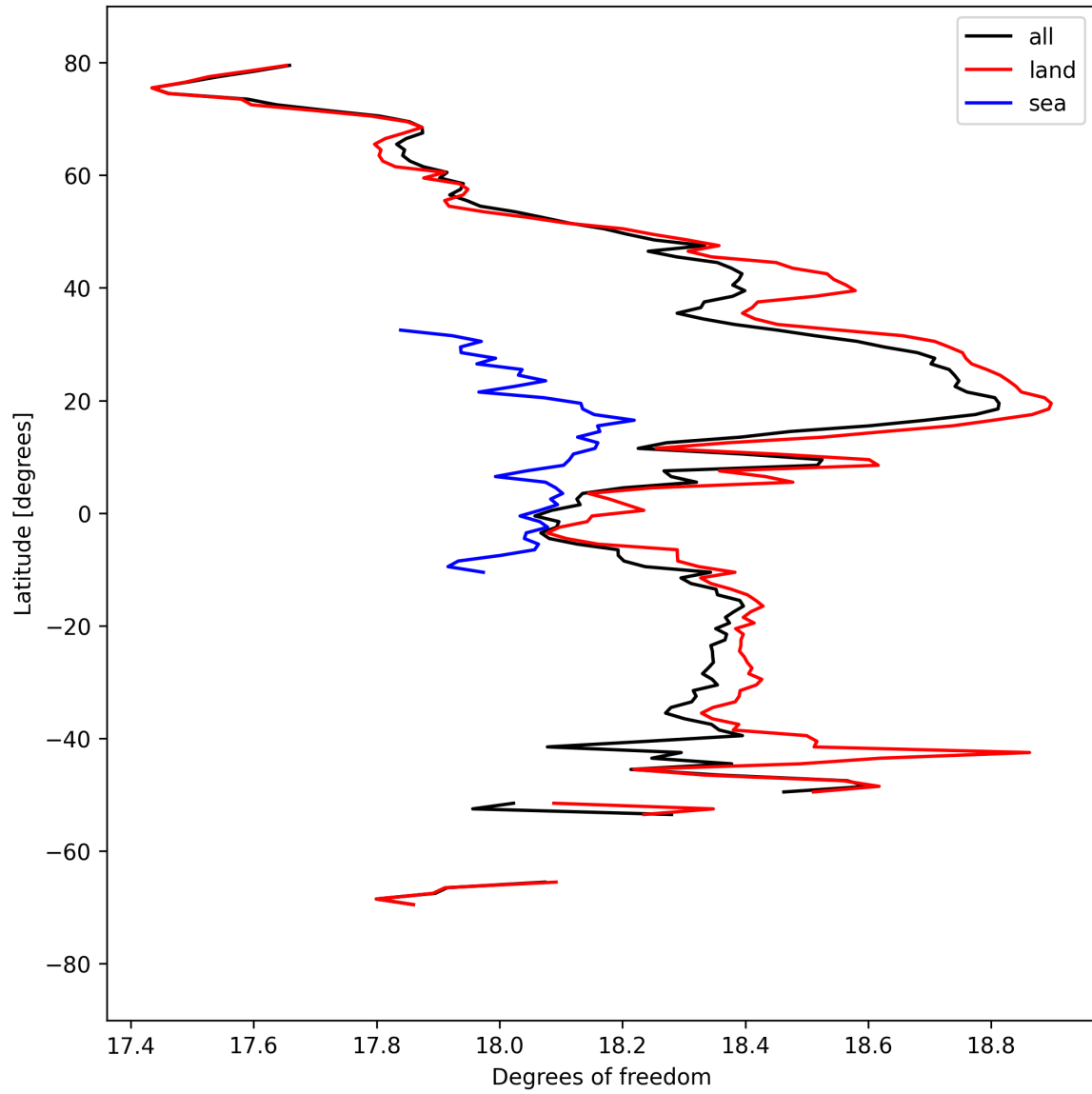
Figure 19: Zonal average of “Degrees of freedom” for 2025-09-10 to 2025-09-12.
