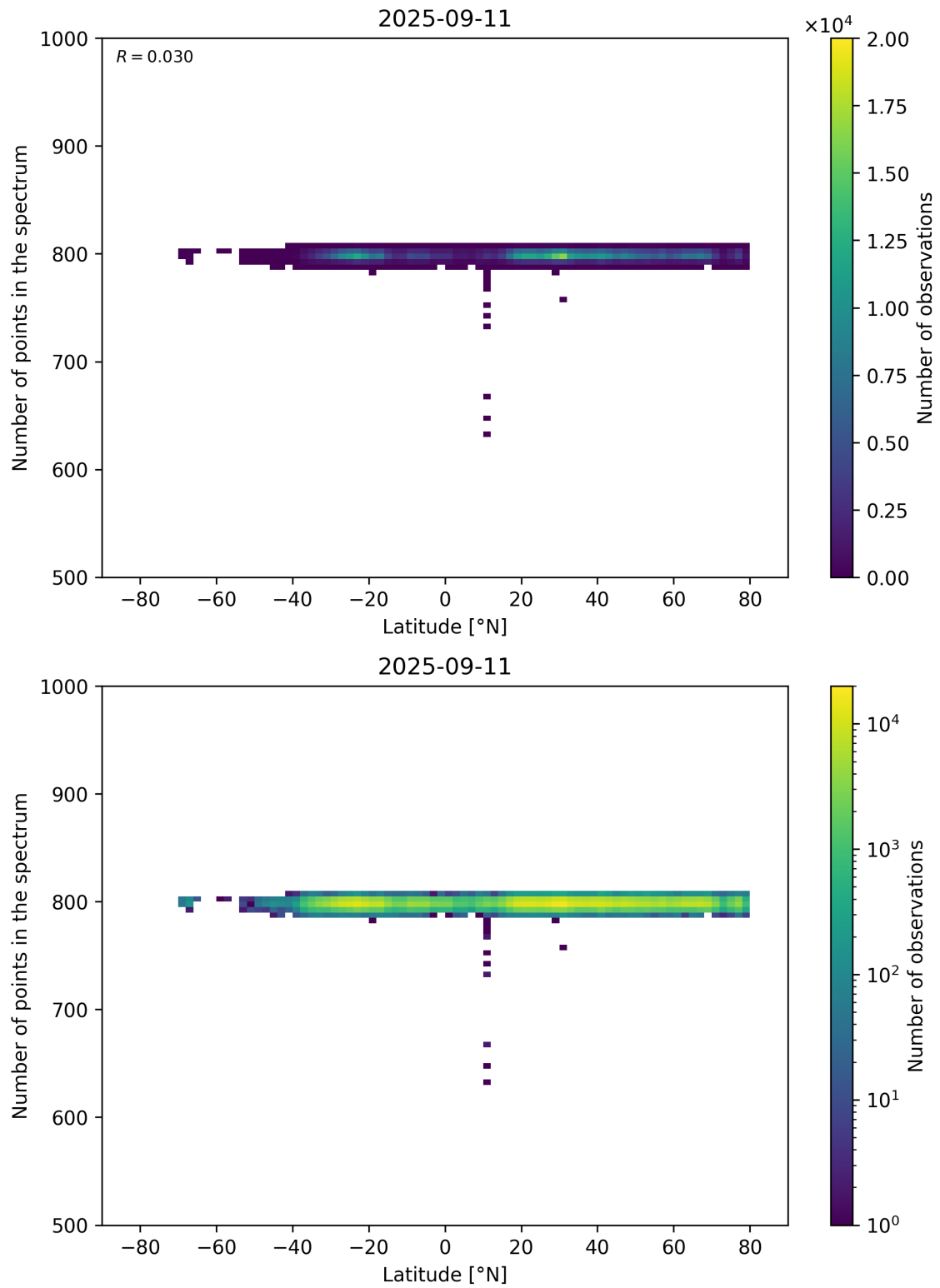
Figure 61: Scatter density plot of “Latitude” against “Number of points in the spectrum” for 2025-09-10 to 2025-09-12.
