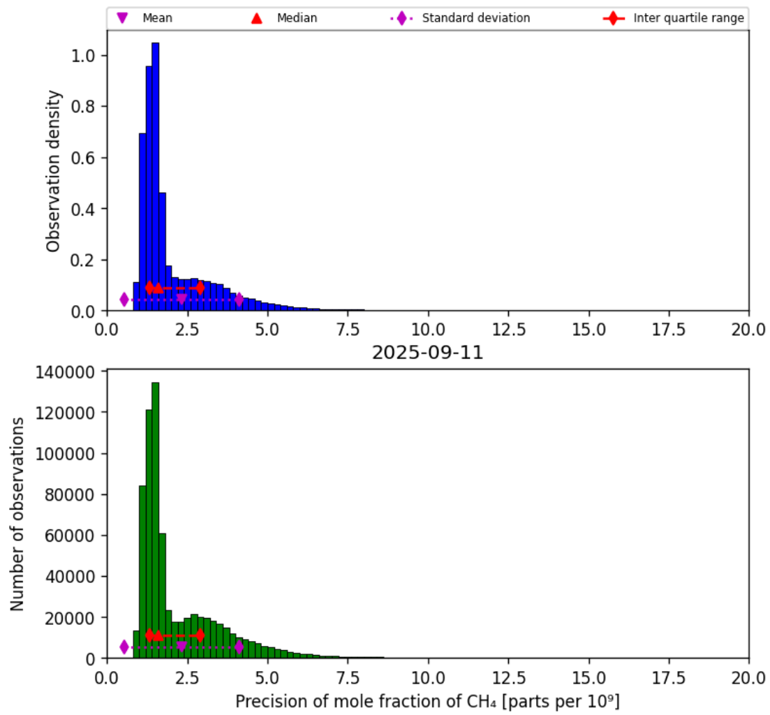
Figure 24: Histogram of “Precision of mole fraction of CH 4 ” for 2025-09-10 to 2025-09-12
