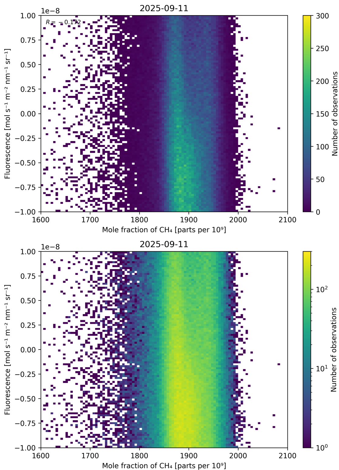
Figure 73: Scatter density plot of “Mole fraction of \text{CH}_4 ” against “Fluorescence” for 2025-09-10 to 2025-09-12.
