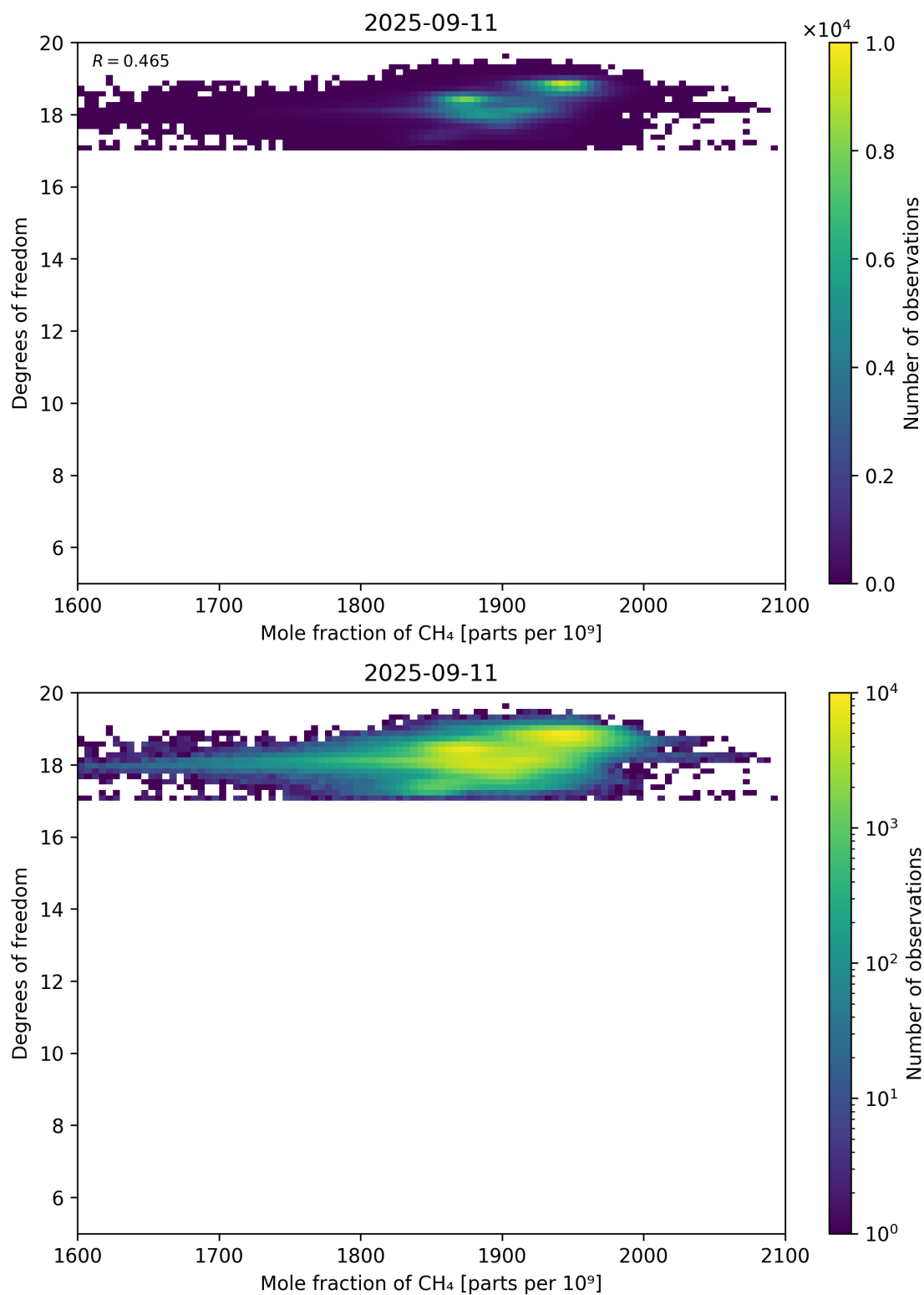
Figure 72: Scatter density plot of “Mole fraction of CH 4 ” against “Degrees of freedom” for 2025-09-10 to 2025-09-12.
