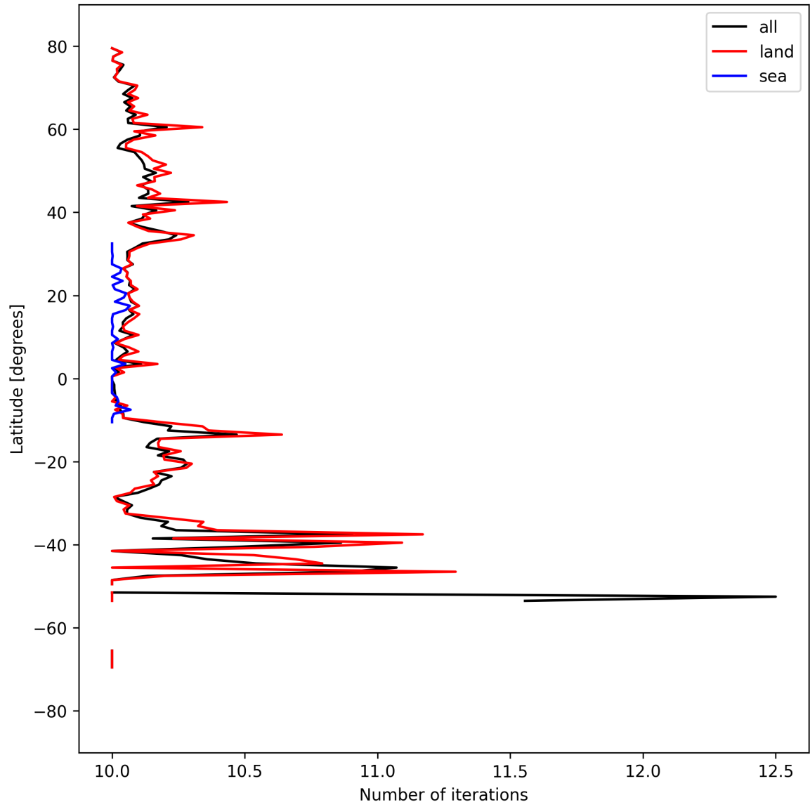
Figure 20: Zonal average of “Number of iterations” for 2025-09-10 to 2025-09-12.
