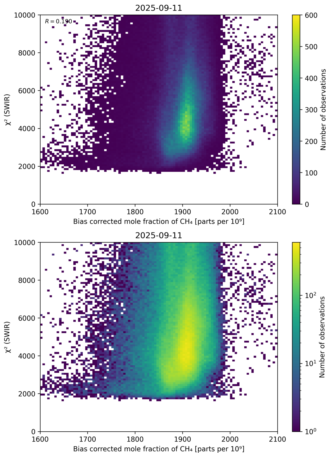
Figure 64: Scatter density plot of “Bias corrected mole fraction of \text{CH}_4 ” against “ \chi^2 (SWIR)” for 2025-09-10 to 2025-09-12.
