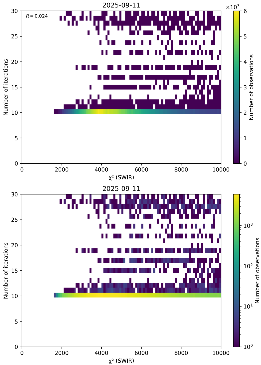
Figure 50: Scatter density plot of “ \chi^2 (SWIR)” against “Number of iterations” for 2025-09-10 to 2025-09-12.
