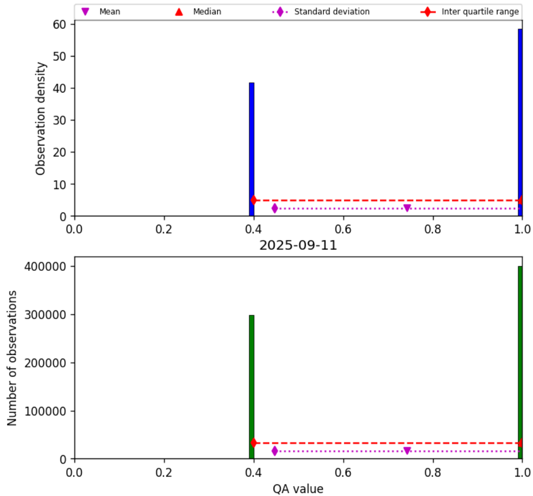
Figure 22: Histogram of “QA value” for 2025-09-10 to 2025-09-12
