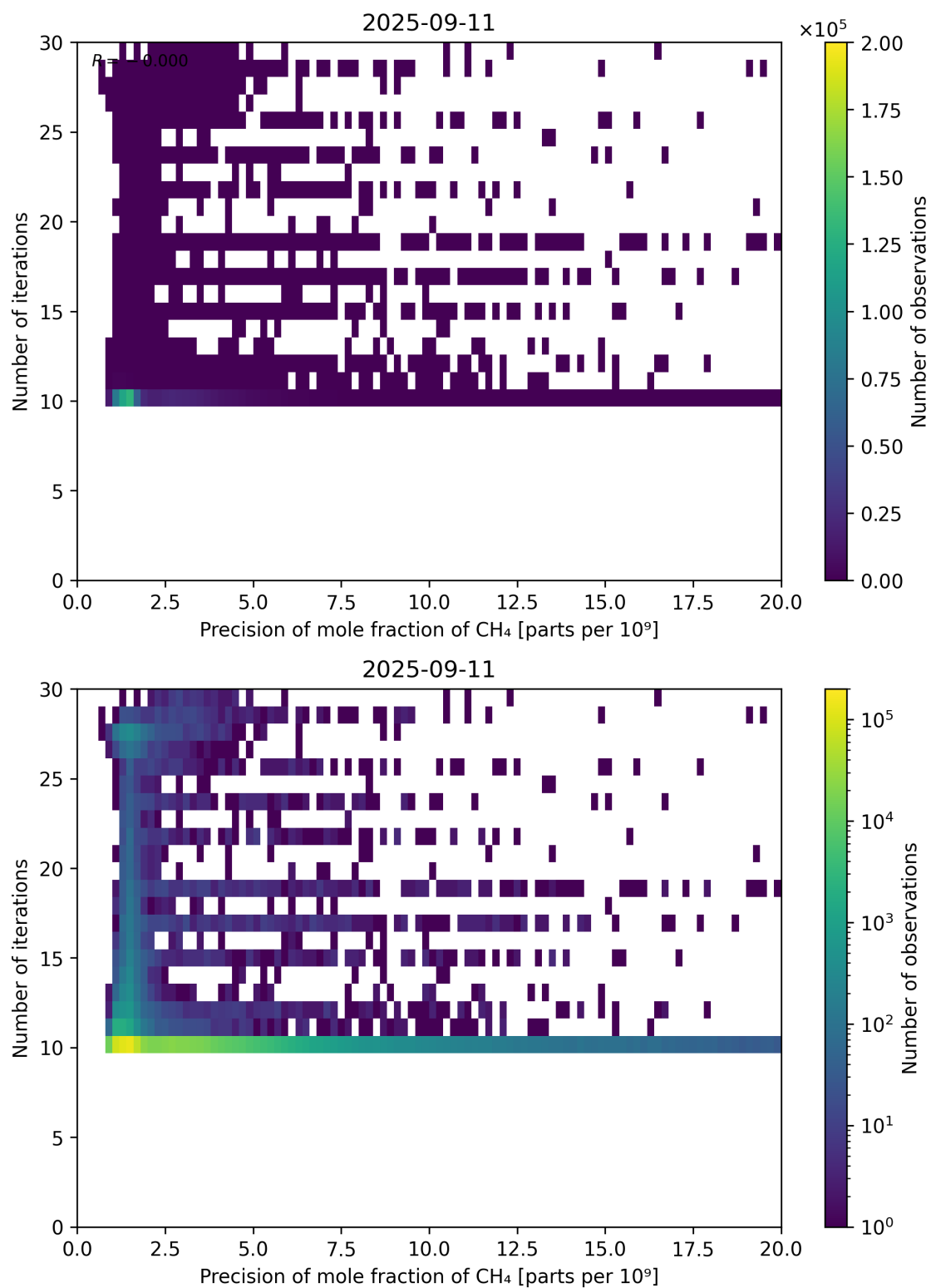
Figure 83: Scatter density plot of “Precision of mole fraction of CH 4 ” against “Number of iterations” for 2025-09-10 to 2025-09-12.
