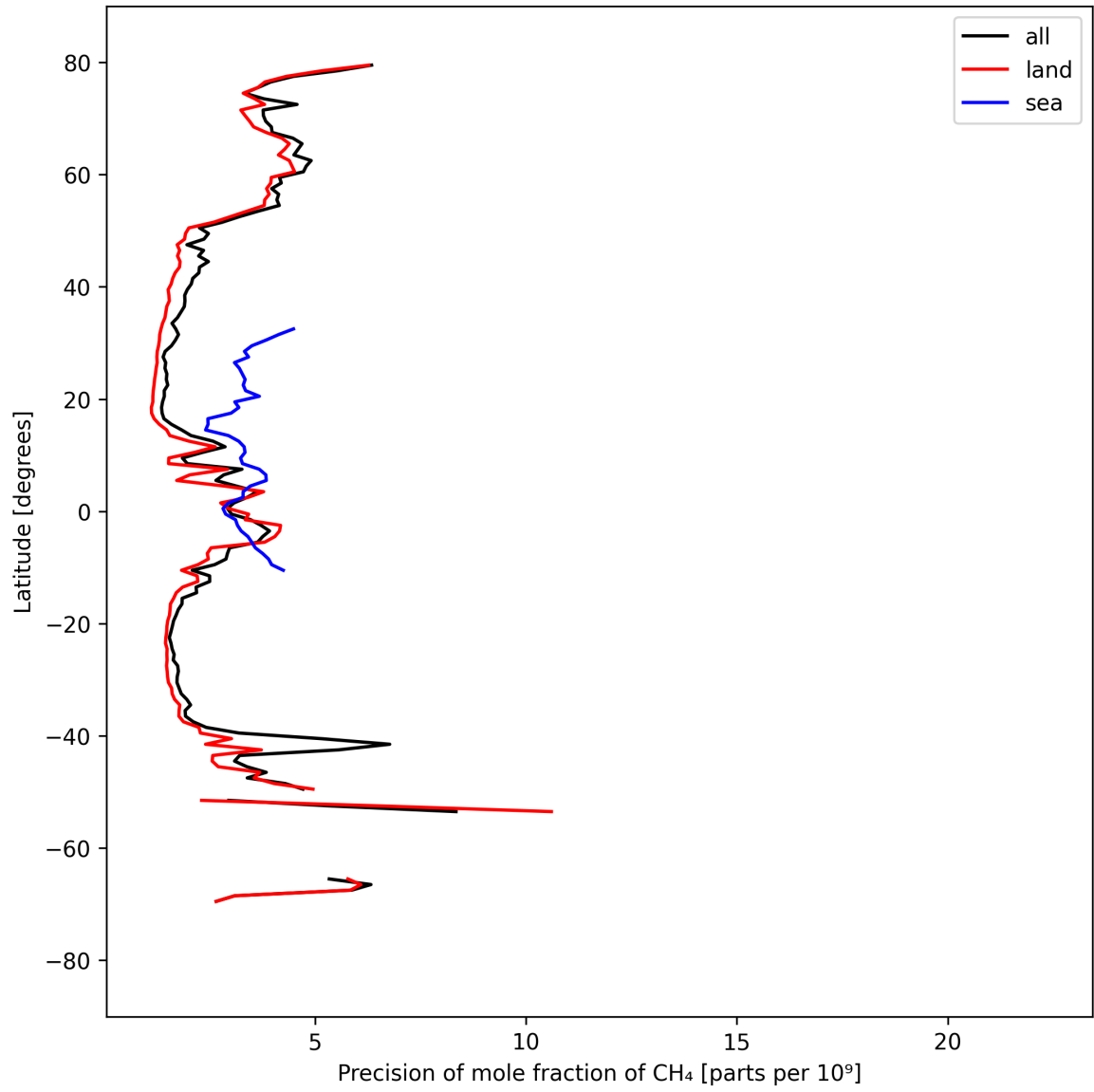
Figure 13: Zonal average of “Precision of mole fraction of CH 4 ” for 2025-09-10 to 2025-09-12.
