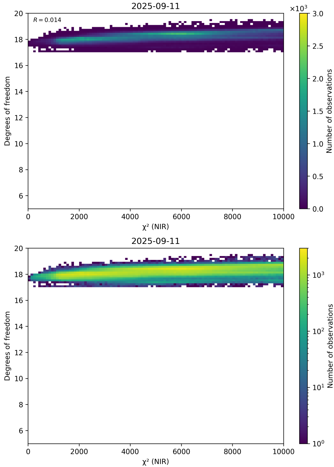
Figure 44: Scatter density plot of “ \chi^2 (NIR)” against “Degrees of freedom” for 2025-09-10 to 2025-09-12.
