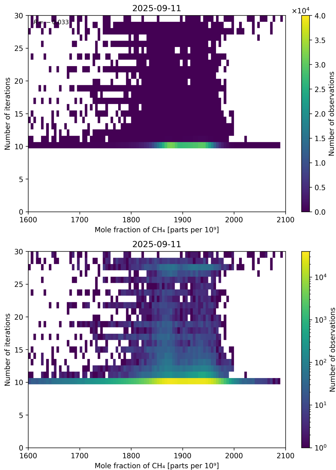
Figure 76: Scatter density plot of “Mole fraction of CH 4 ” against “Number of iterations” for 2025-09-10 to 2025-09-12.
