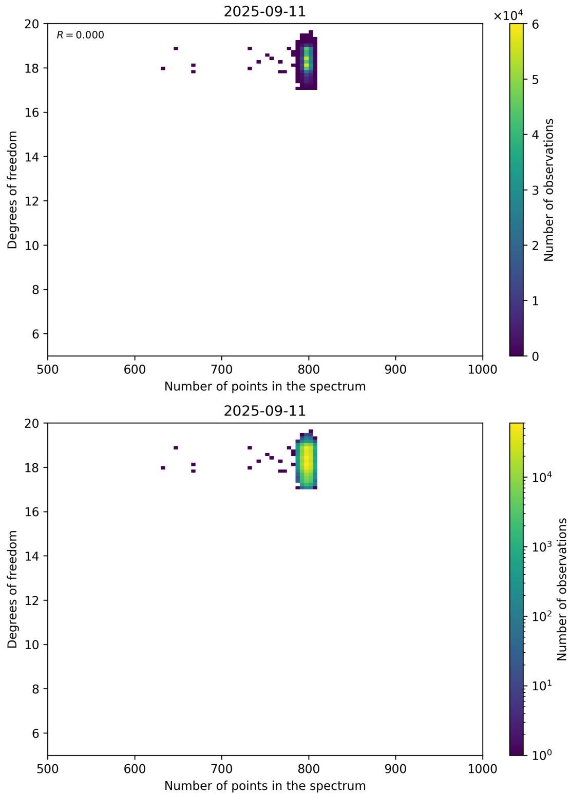
Figure 90: Scatter density plot of “Number of points in the spectrum” against “Degrees of freedom” for 2025-09-10 to 2025-09-12.
