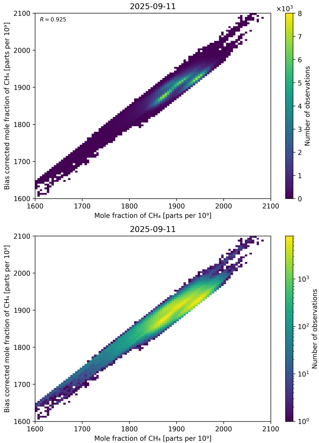
Figure 74: Scatter density plot of “Mole fraction of CH 4 ” against “Bias corrected mole fraction of CH 4 ” for 2025-09-10 to 2025-09-12.
