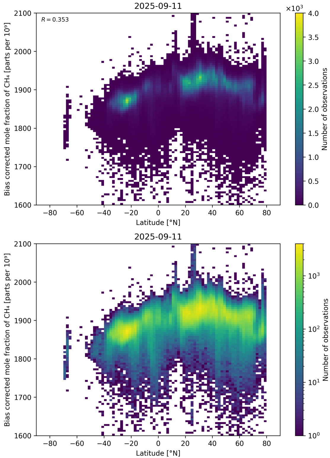
Figure 58: Scatter density plot of “Latitude” against “Bias corrected mole fraction of \text{CH}_4 ” for 2025-09-10 to 2025-09-12.
