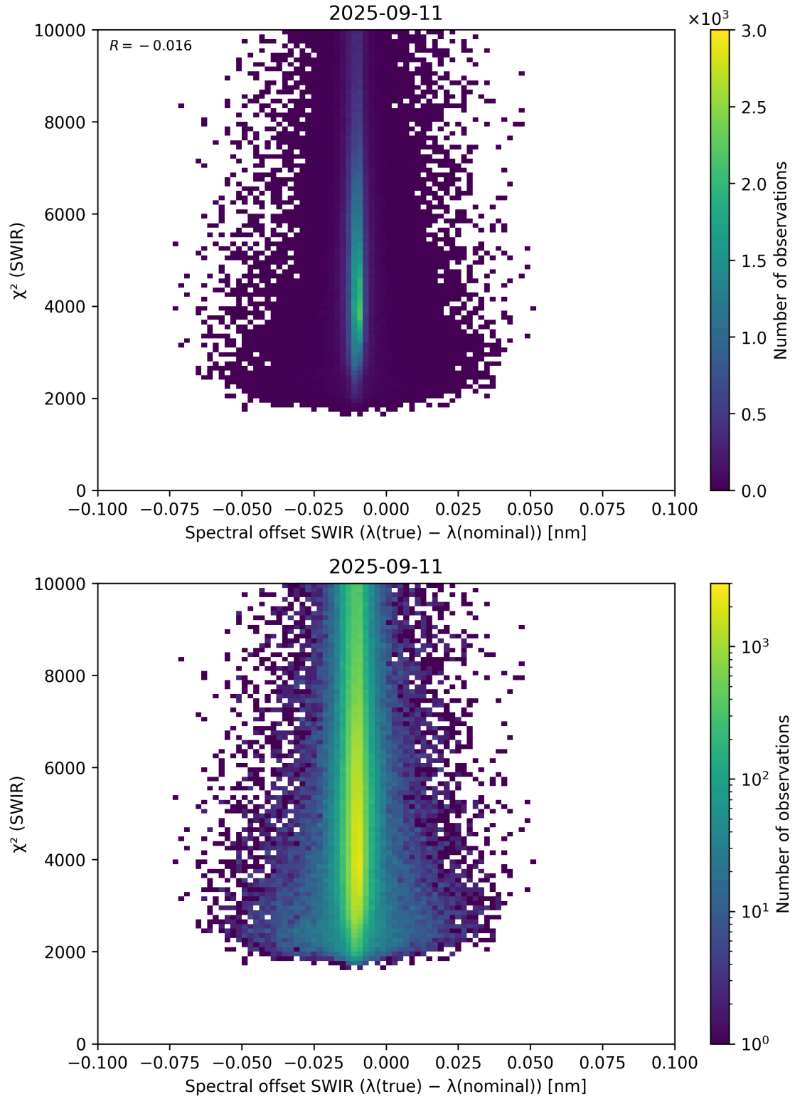
Figure 118: Scatter density plot of “Spectral offset SWIR ( \lambda_{\text{true}} - \lambda_{\text{nominal}} )” against “ \chi^2 (SWIR)” for 2025-09-10 to 2025-09-12.
