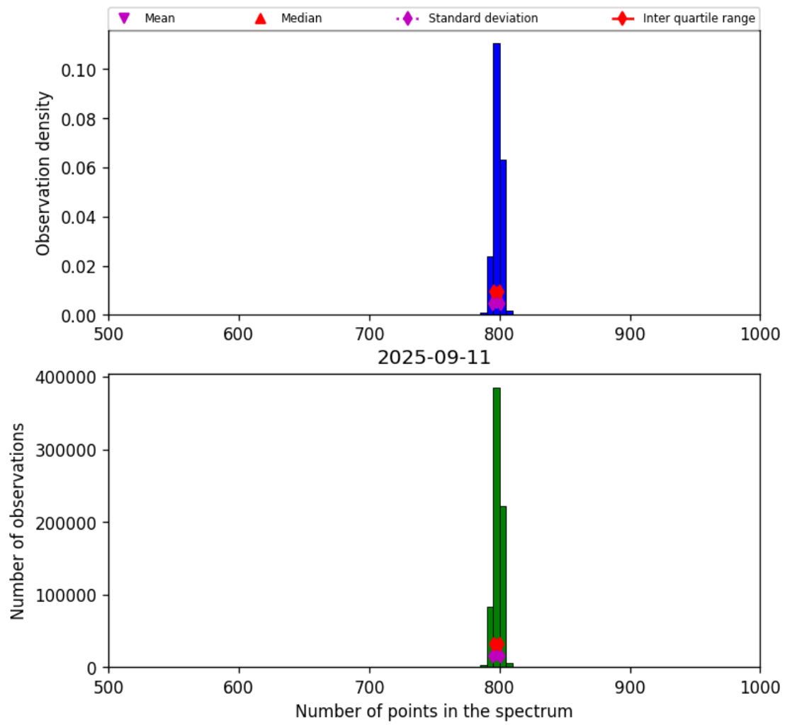
Figure 26: Histogram of “Number of points in the spectrum” for 2025-09-10 to 2025-09-12
