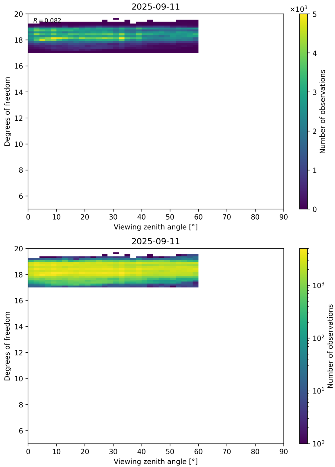
Figure 107: Scatter density plot of “Viewing zenith angle” against “Degrees of freedom” for 2025-09-10 to 2025-09-12.
