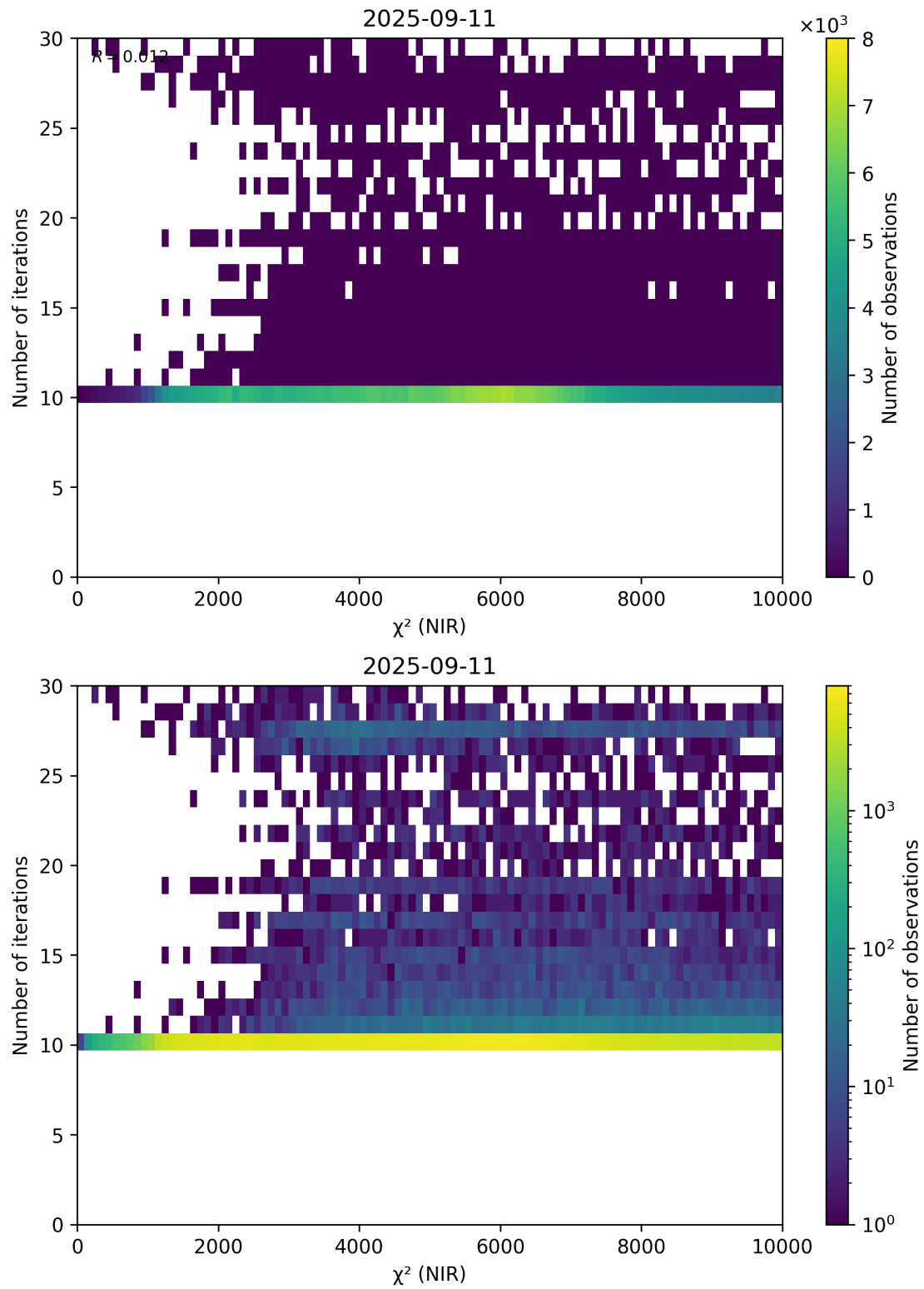
Figure 46: Scatter density plot of “ \chi^2 (NIR)” against “Number of iterations” for 2025-09-10 to 2025-09-12.
