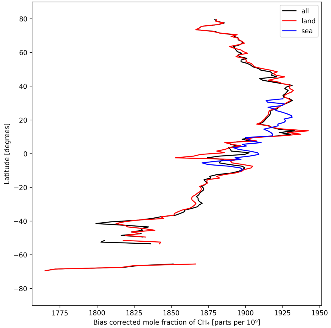
Figure 14: Zonal average of “Bias corrected mole fraction of CH 4 ” for 2025-09-10 to 2025-09-12.
