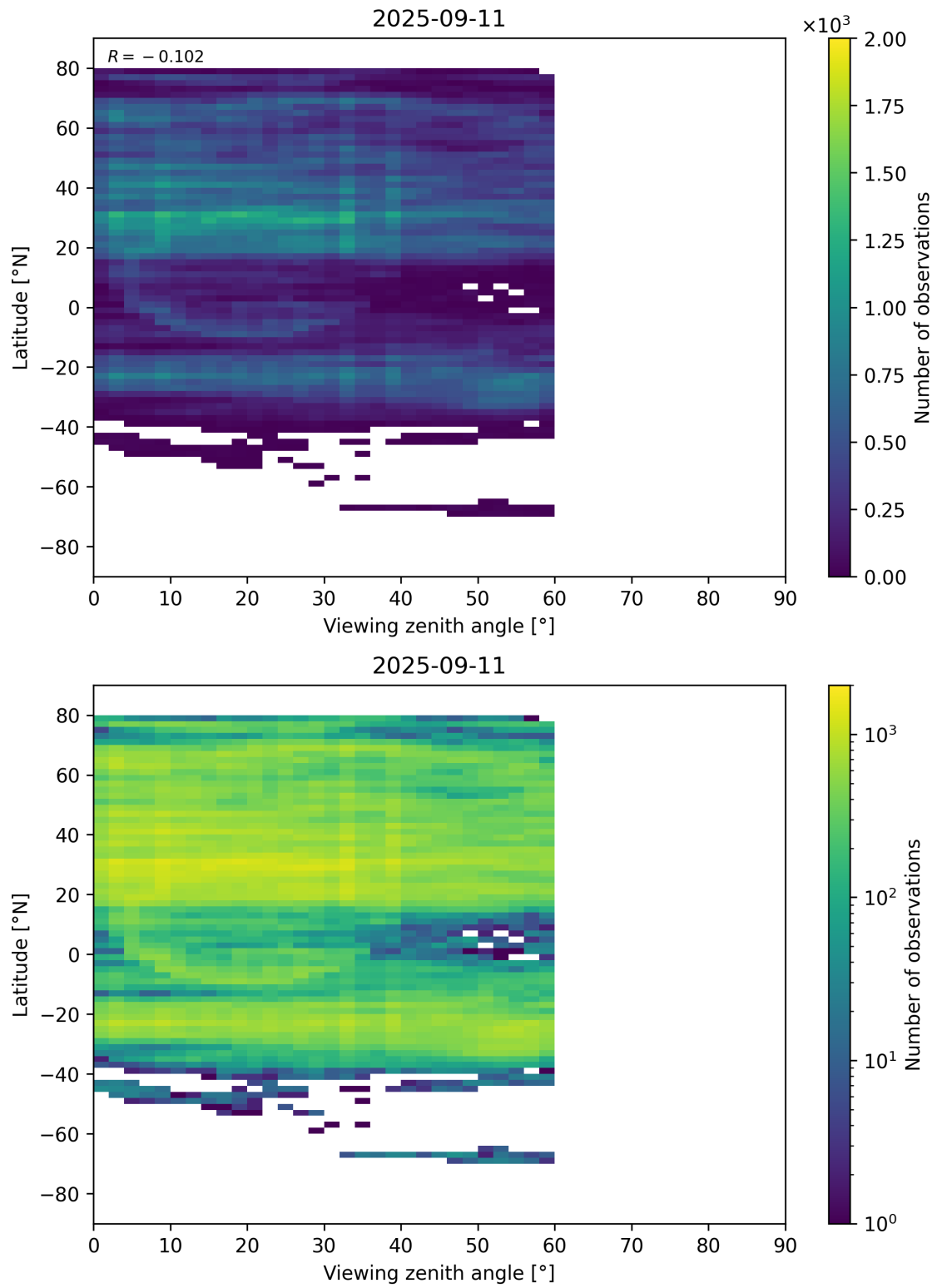
Figure 109: Scatter density plot of “Viewing zenith angle” against “Latitude” for 2025-09-10 to 2025-09-12.
