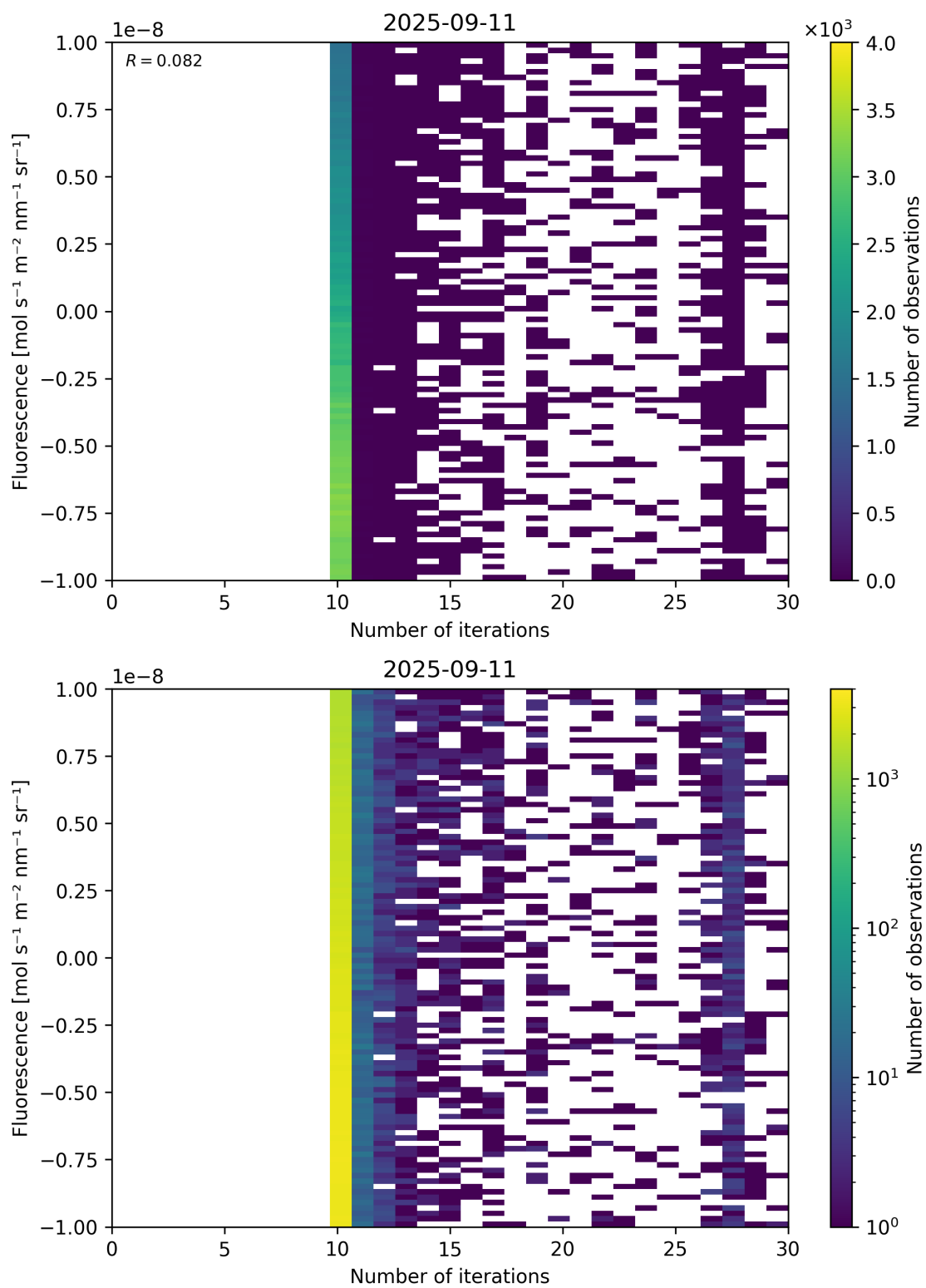
Figure 87: Scatter density plot of “Number of iterations” against “Fluorescence” for 2025-09-10 to 2025-09-12.
