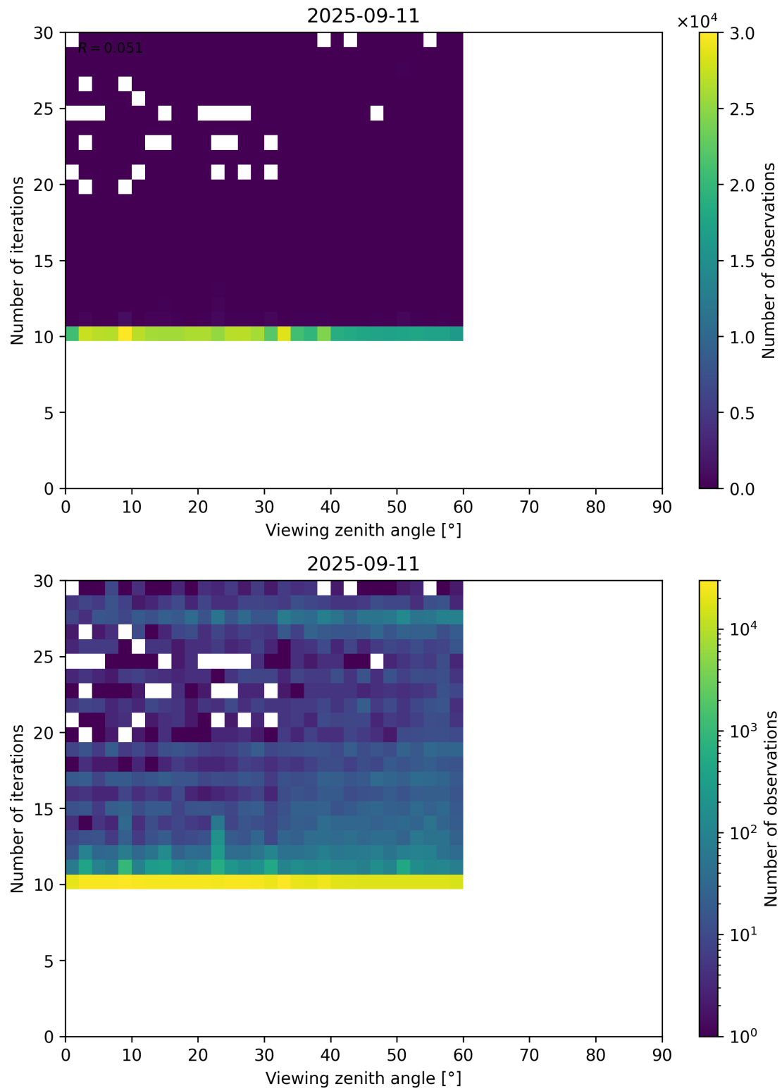
Figure 113: Scatter density plot of “Viewing zenith angle” against “Number of iterations” for 2025-09-10 to 2025-09-12.
