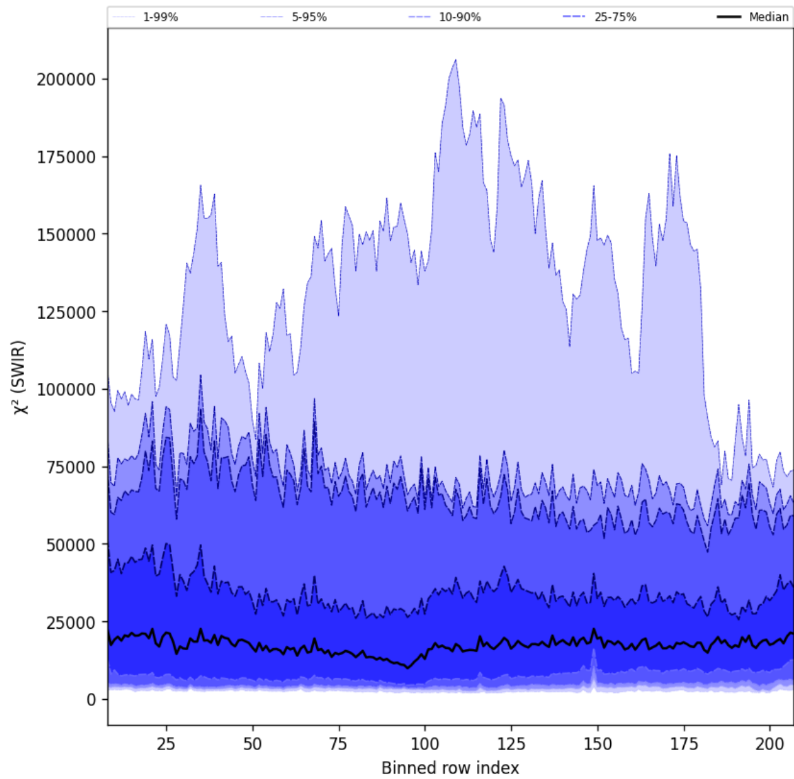
Figure 39: Along track statistics of “ \chi^2 (SWIR)” for 2025-09-12 to 2025-09-14
