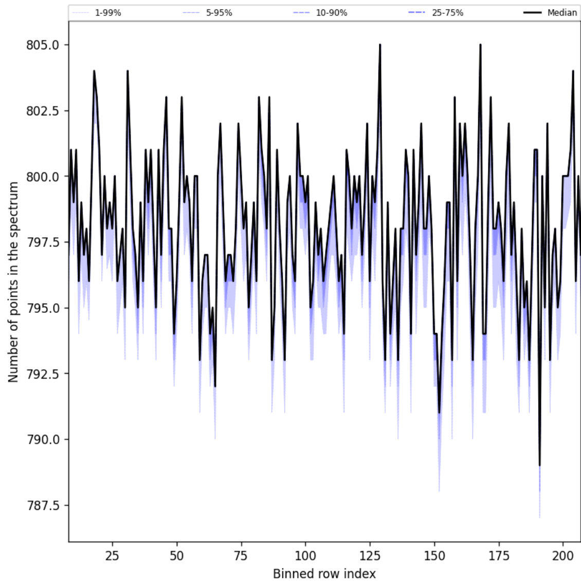
Figure 37: Along track statistics of “Number of points in the spectrum” for 2025-09-12 to 2025-09-14
