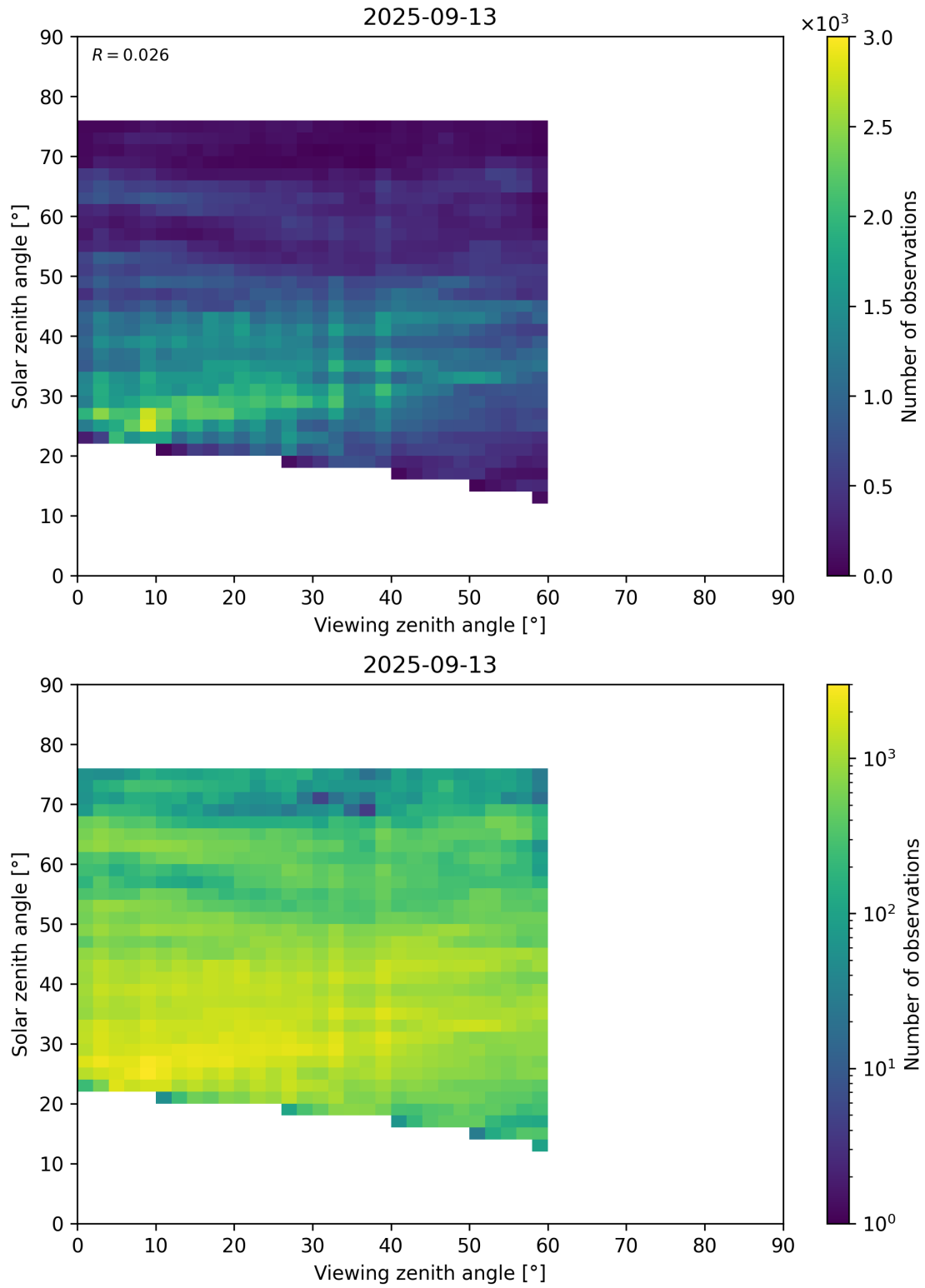
Figure 115: Scatter density plot of “Viewing zenith angle” against “Solar zenith angle” for 2025-09-12 to 2025-09-14.
