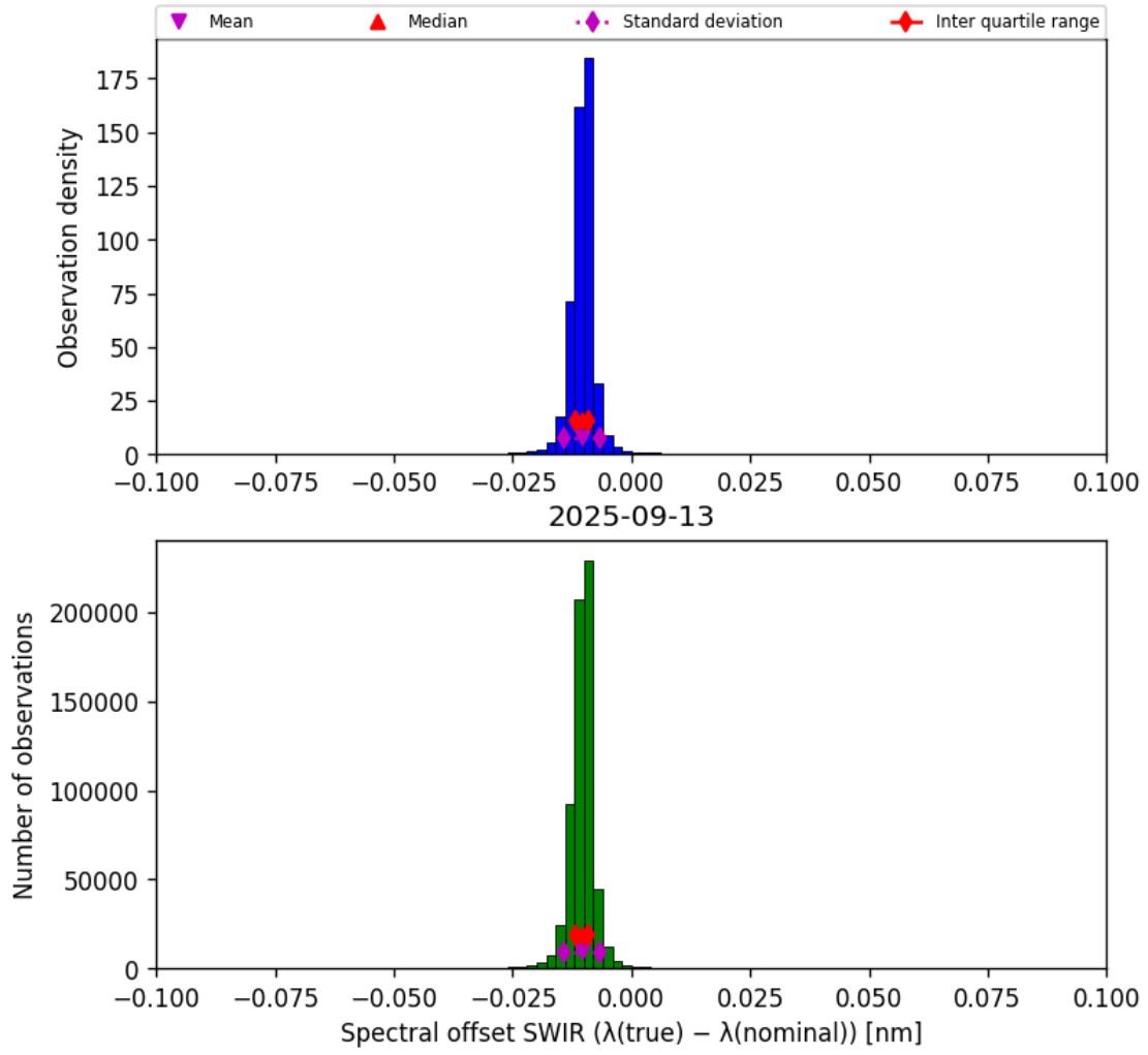
Figure 27: Histogram of “Spectral offset SWIR ( \lambda_{\text{true}} - \lambda_{\text{nominal}} )” for 2025-09-12 to 2025-09-14
