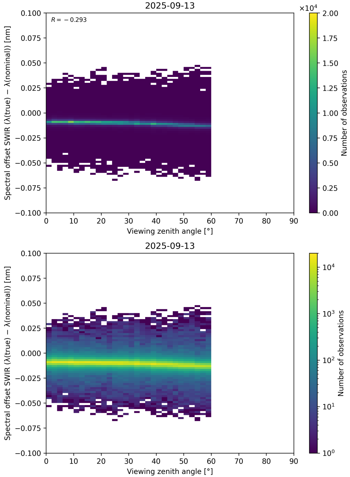
Figure 116: Scatter density plot of “Viewing zenith angle” against “Spectral offset SWIR ( \lambda_{\text{true}} - \lambda_{\text{nominal}} )” for 2025-09-12 to 2025-09-14.
