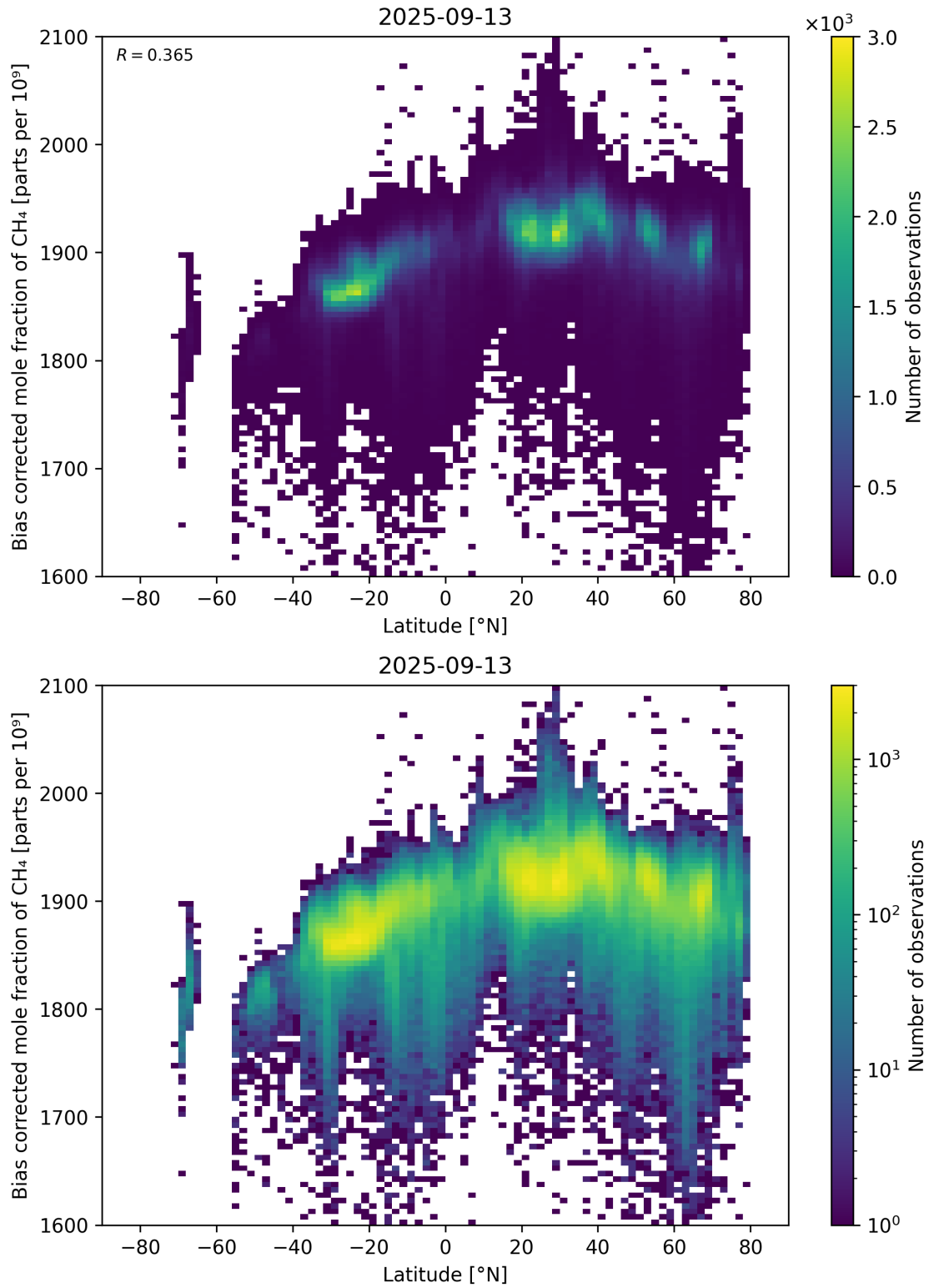
Figure 58: Scatter density plot of “Latitude” against “Bias corrected mole fraction of CH 4 ” for 2025-09-12 to 2025-09-14.
