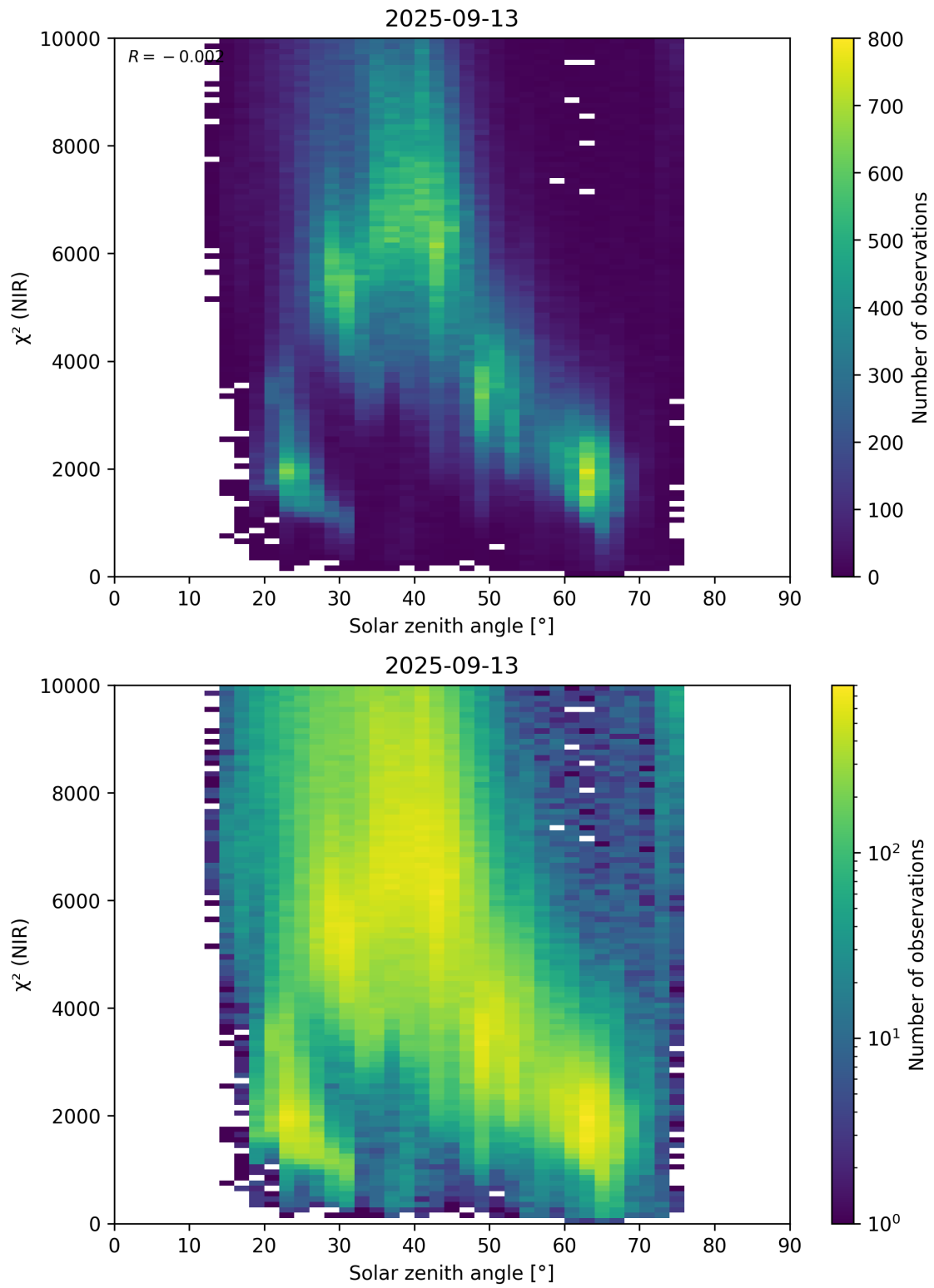
Figure 94: Scatter density plot of “Solar zenith angle” against “ \chi^2 (NIR)” for 2025-09-12 to 2025-09-14.
