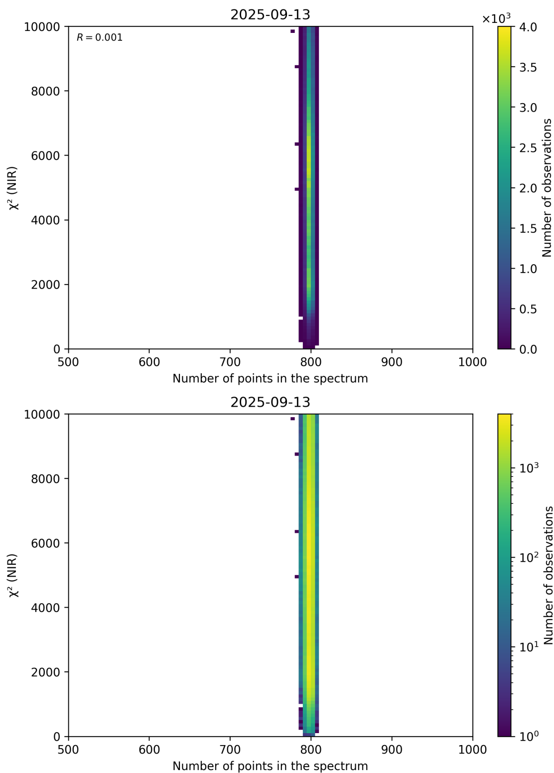
Figure 88: Scatter density plot of “Number of points in the spectrum” against “ \chi^2 (NIR)” for 2025-09-12 to 2025-09-14.
