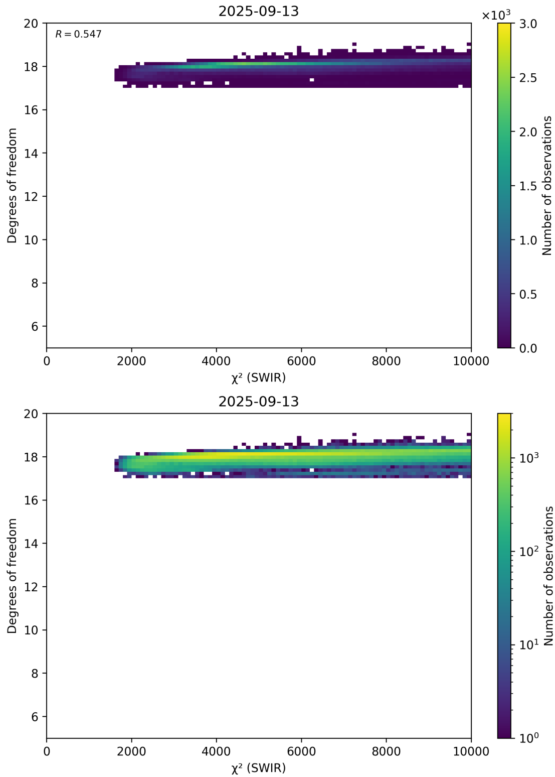
Figure 48: Scatter density plot of “ \chi^2 (SWIR)” against “Degrees of freedom” for 2025-09-12 to 2025-09-14.
