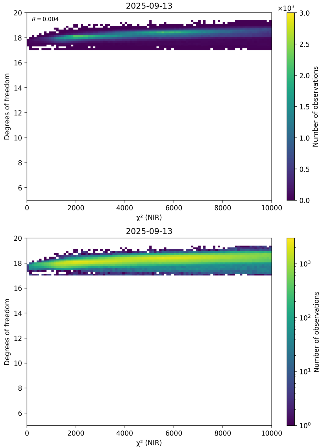
Figure 44: Scatter density plot of “ \chi^2 (NIR)” against “Degrees of freedom” for 2025-09-12 to 2025-09-14.
