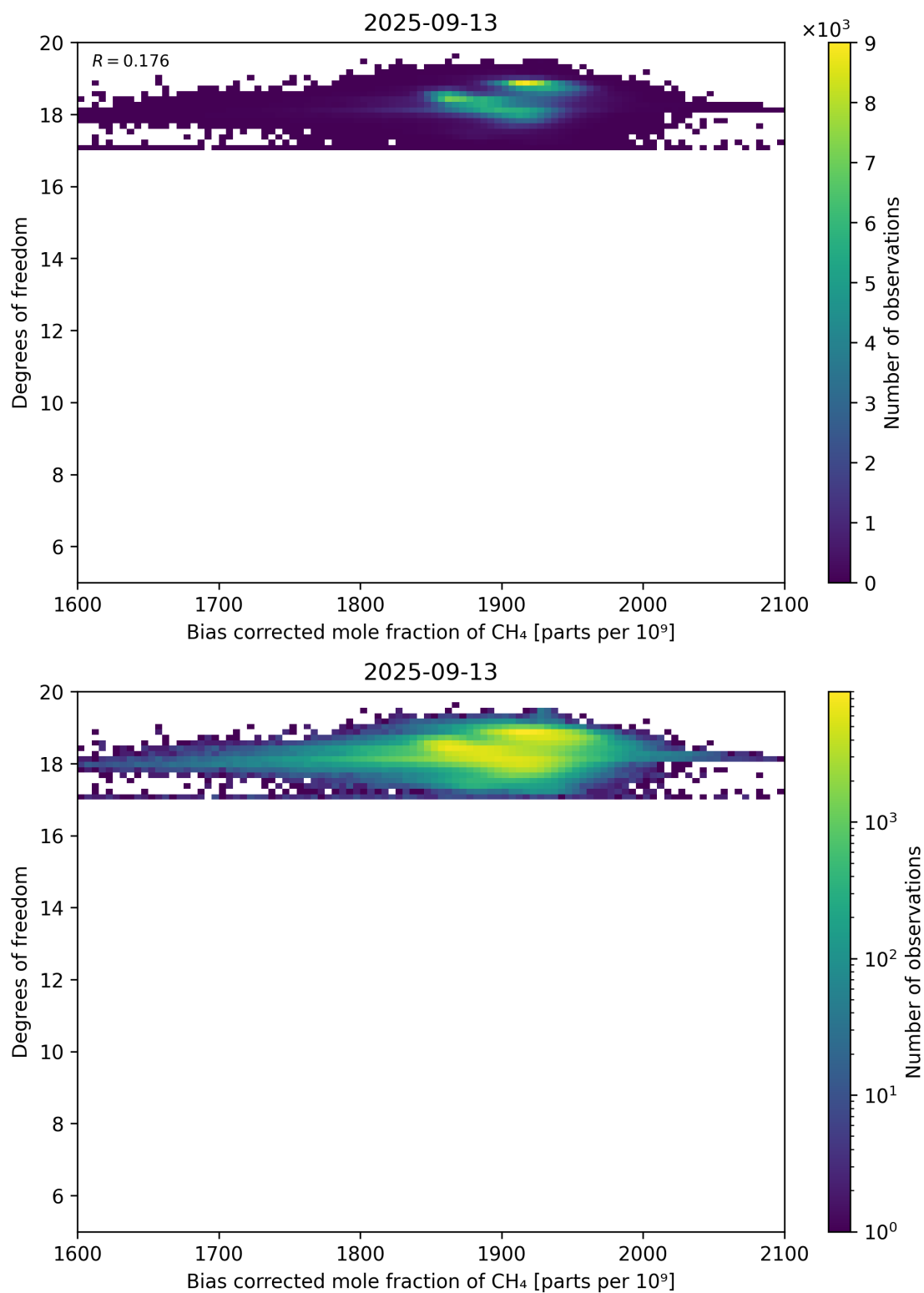
Figure 65: Scatter density plot of “Bias corrected mole fraction of CH 4 ” against “Degrees of freedom” for 2025-09-12 to 2025-09-14.
