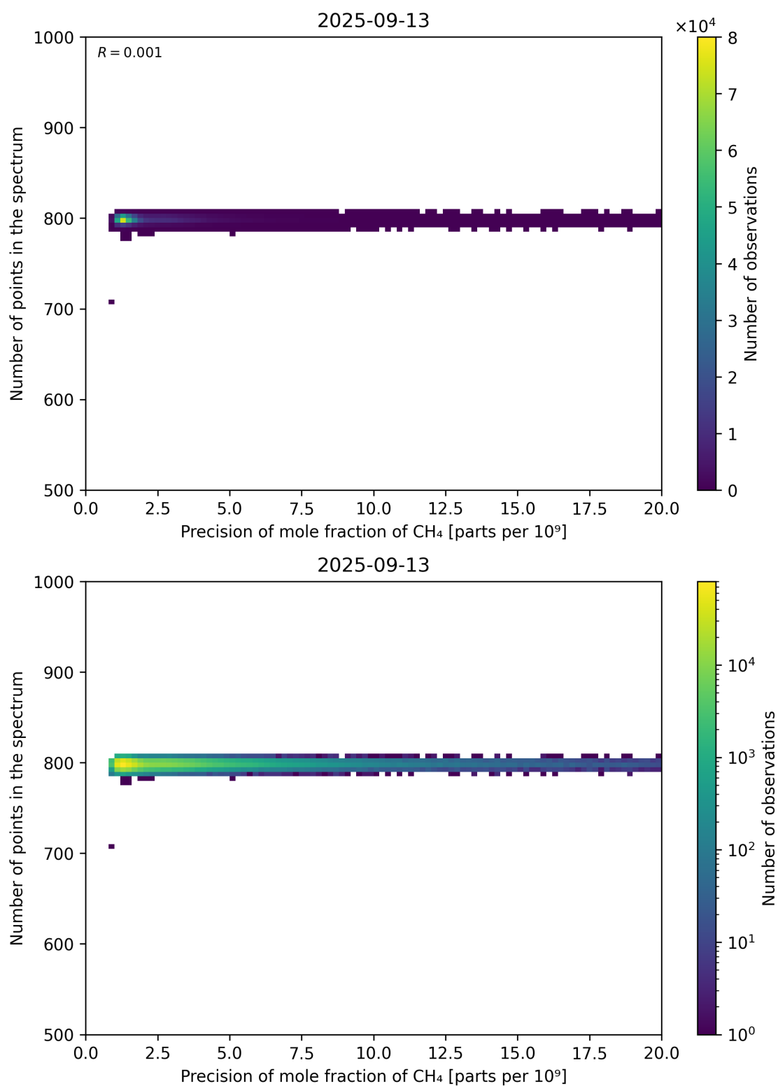
Figure 84: Scatter density plot of “Precision of mole fraction of CH 4 ” against “Number of points in the spectrum” for 2025-09-12 to 2025-09-14.
