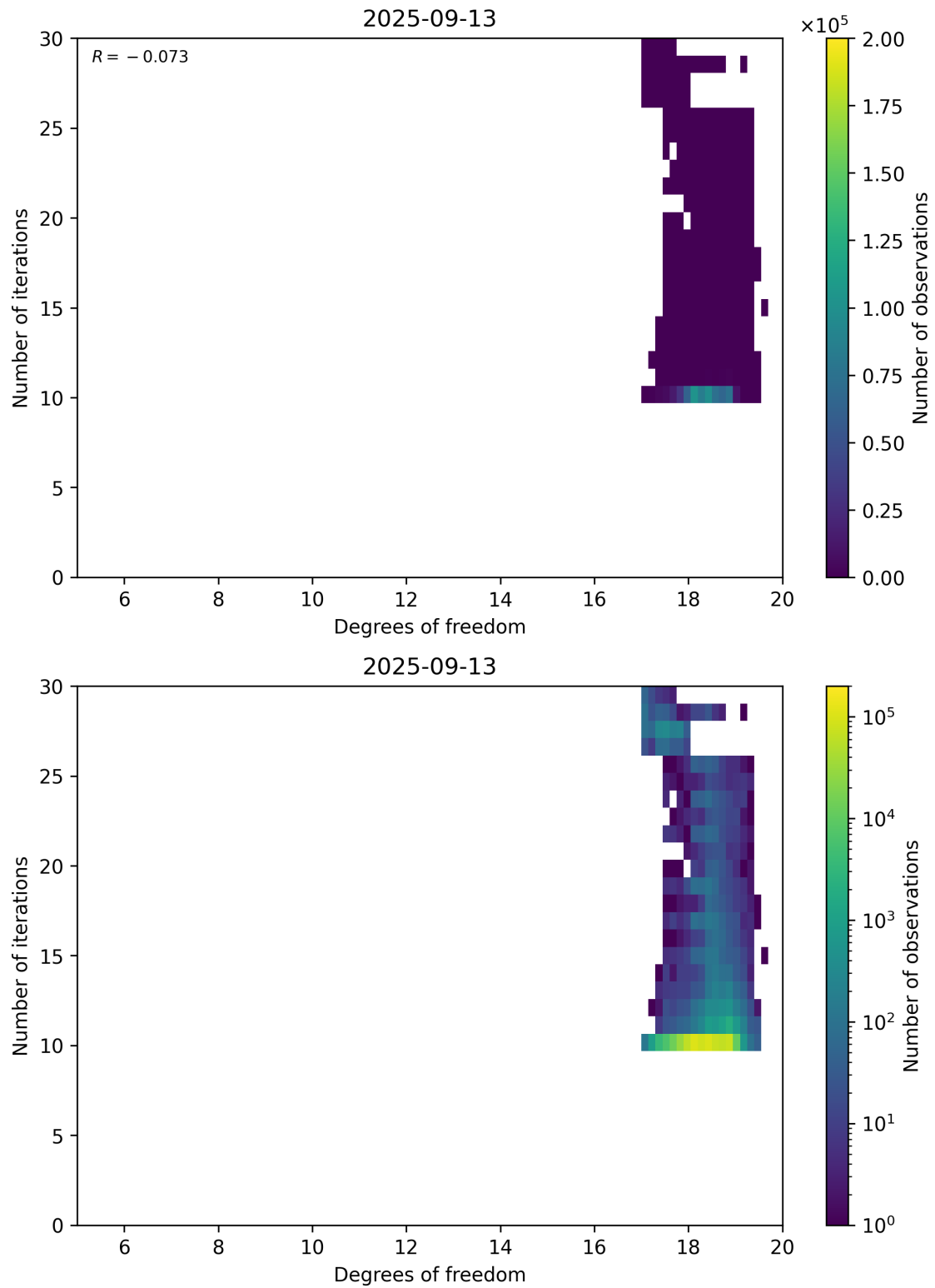
Figure 52: Scatter density plot of “Degrees of freedom” against “Number of iterations” for 2025-09-12 to 2025-09-14.
