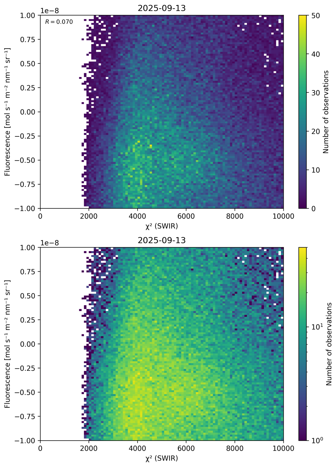
Figure 49: Scatter density plot of “ \chi^2 (SWIR)” against “Fluorescence” for 2025-09-12 to 2025-09-14.
