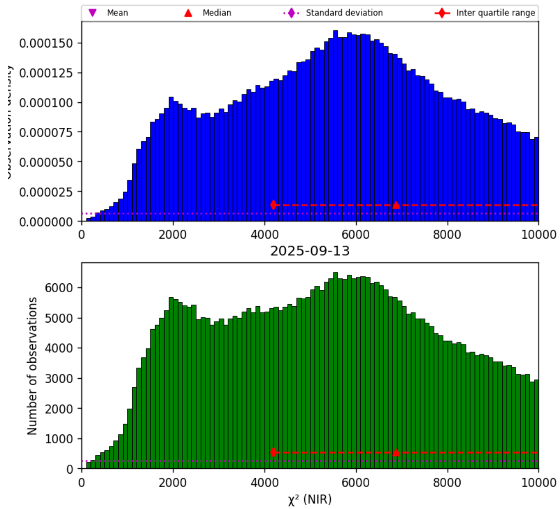
Figure 29: Histogram of “ \chi^2 (NIR)” for 2025-09-12 to 2025-09-14
