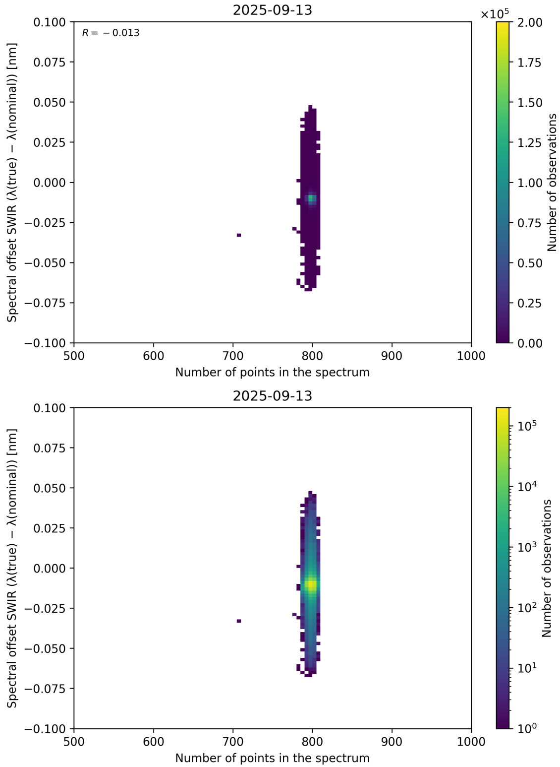
Figure 93: Scatter density plot of “Number of points in the spectrum” against “Spectral offset SWIR ( \lambda_{\text{true}} - \lambda_{\text{nominal}} )” for 2025-09-12 to 2025-09-14.
