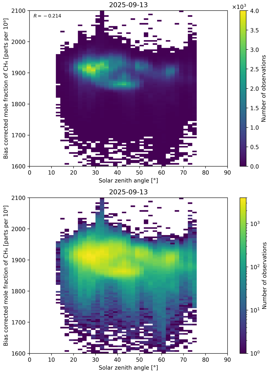
Figure 100: Scatter density plot of “Solar zenith angle” against “Bias corrected mole fraction of CH 4 ” for 2025-09-12 to 2025-09-14.
