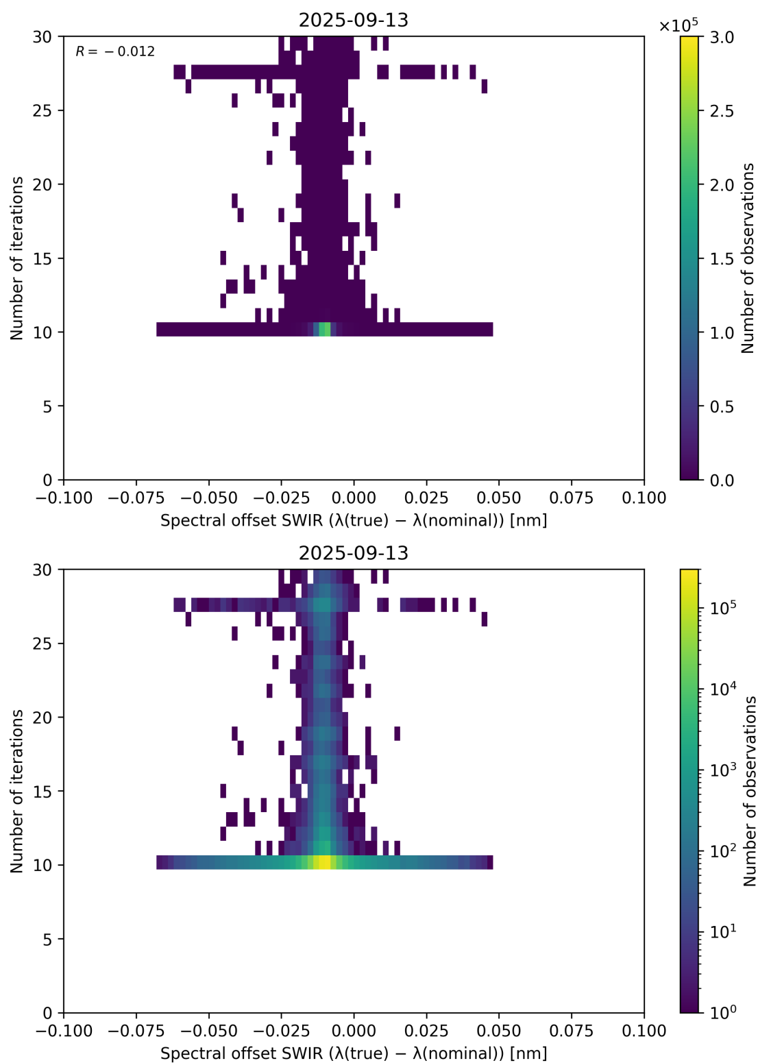
Figure 121: Scatter density plot of “Spectral offset SWIR ( \lambda_{\text{true}} - \lambda_{\text{nominal}} )” against “Number of iterations” for 2025-09-12 to 2025-09-14.
