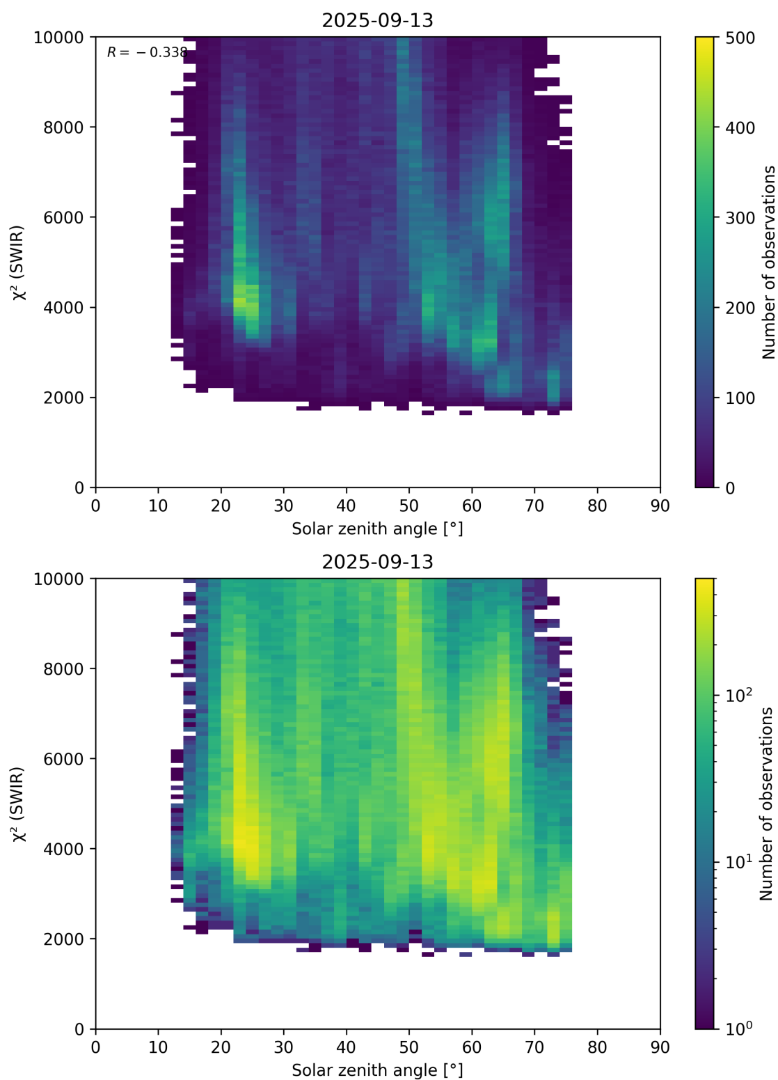
Figure 95: Scatter density plot of “Solar zenith angle” against “ \chi^2 (SWIR)” for 2025-09-12 to 2025-09-14.
