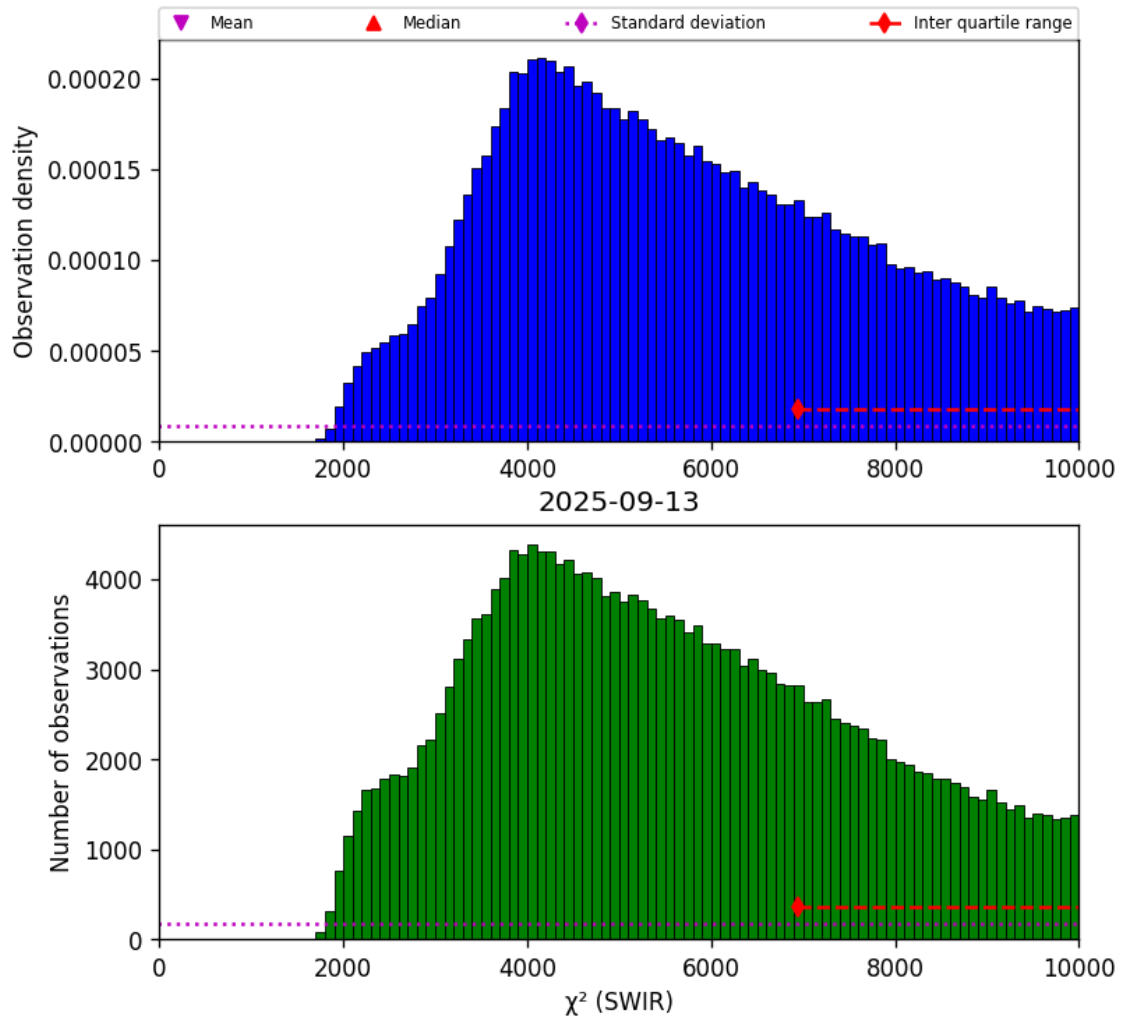
Figure 28: Histogram of " \chi^2 (SWIR)" for 2025-09-12 to 2025-09-14
