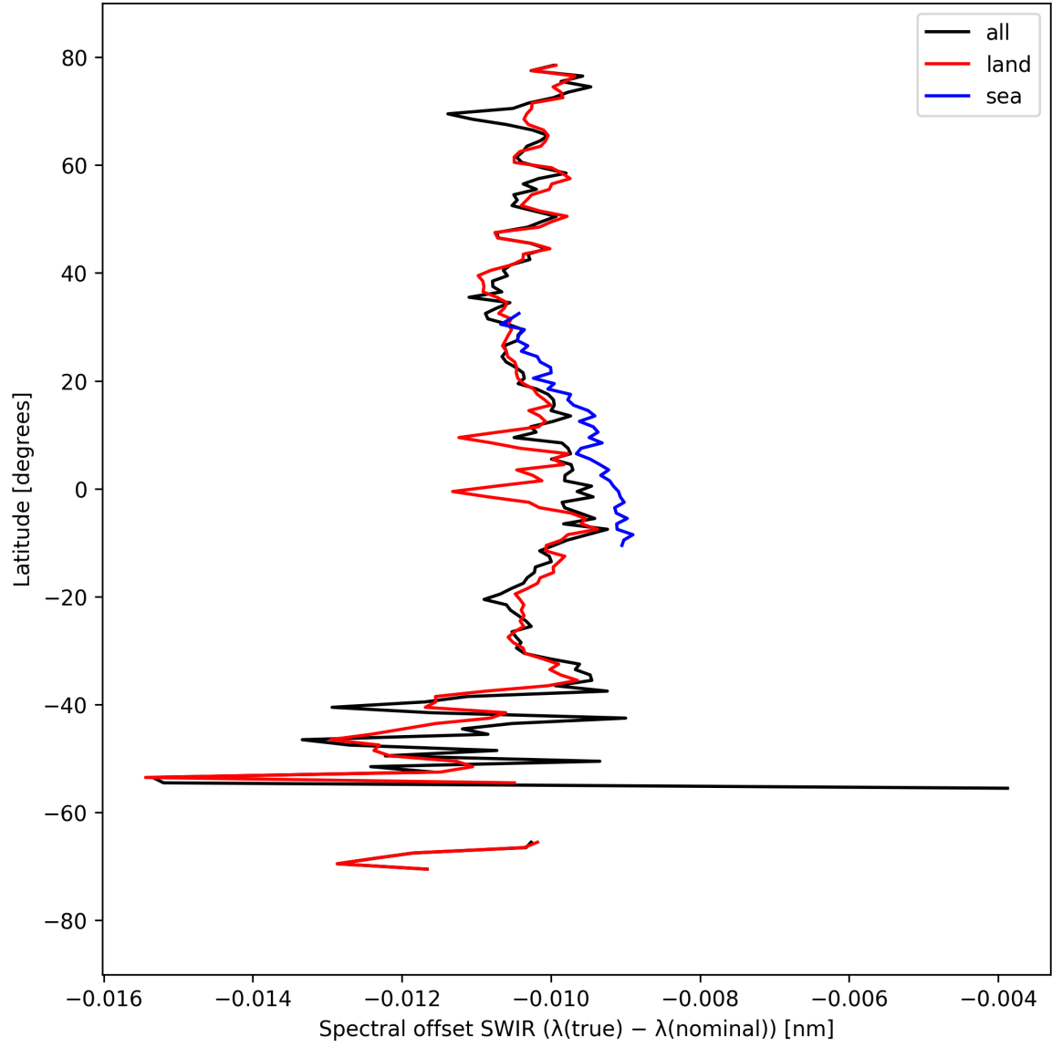
Figure 16: Zonal average of “Spectral offset SWIR ( \lambda_{\text{true}} - \lambda_{\text{nominal}} )” for 2025-09-12 to 2025-09-14.
