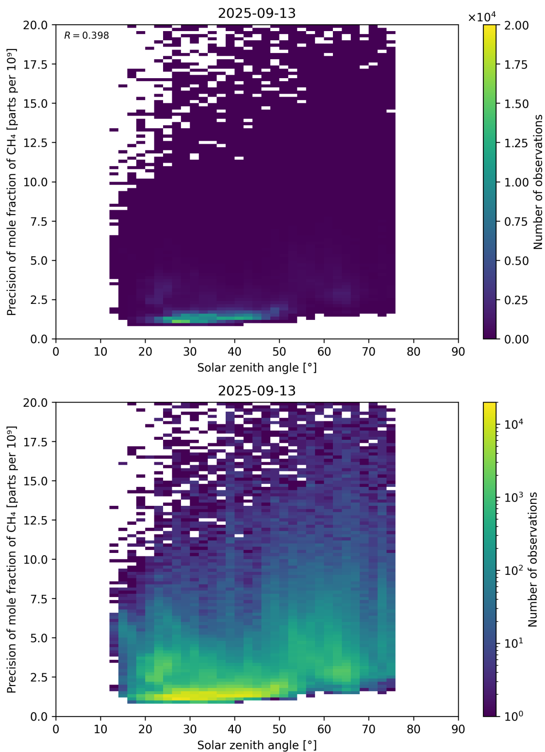
Figure 101: Scatter density plot of “Solar zenith angle” against “Precision of mole fraction of CH 4 ” for 2025-09-12 to 2025-09-14.
