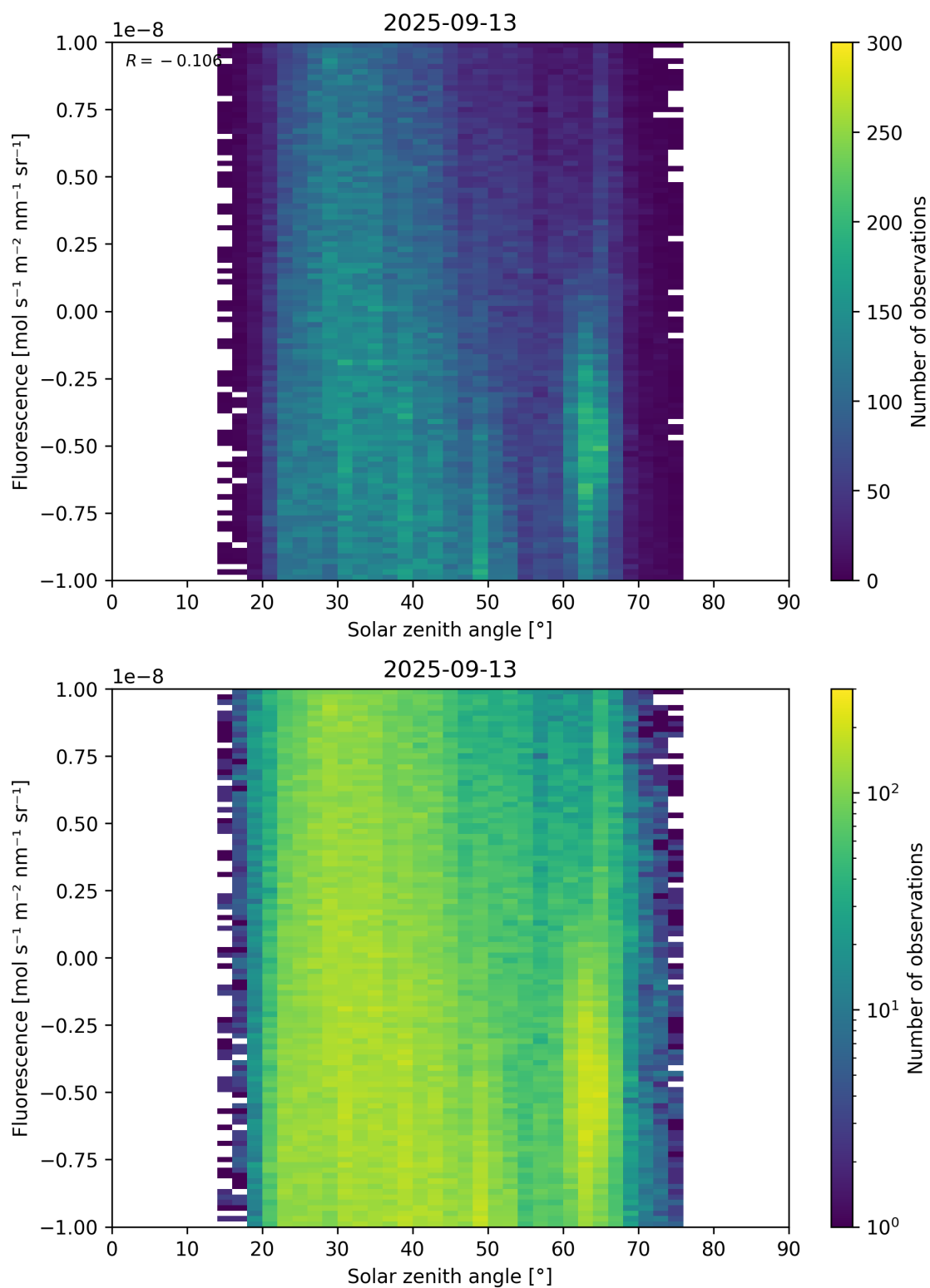
Figure 97: Scatter density plot of “Solar zenith angle” against “Fluorescence” for 2025-09-12 to 2025-09-14.
