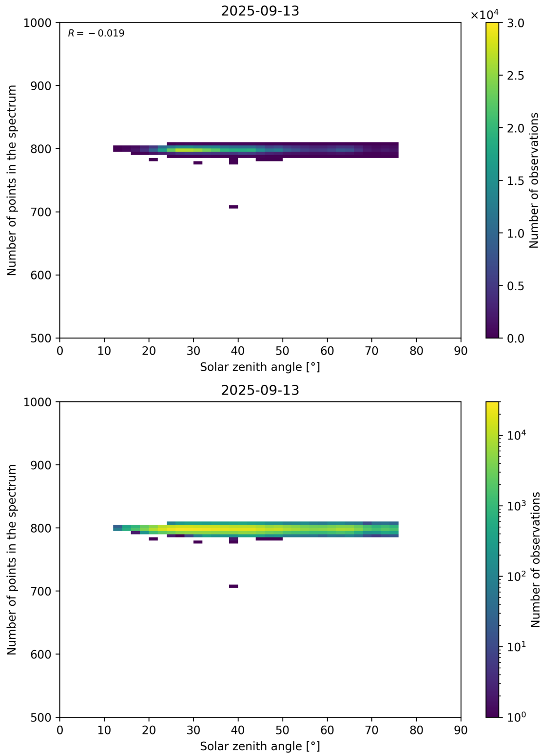
Figure 103: Scatter density plot of “Solar zenith angle” against “Number of points in the spectrum” for 2025-09-12 to 2025-09-14.
