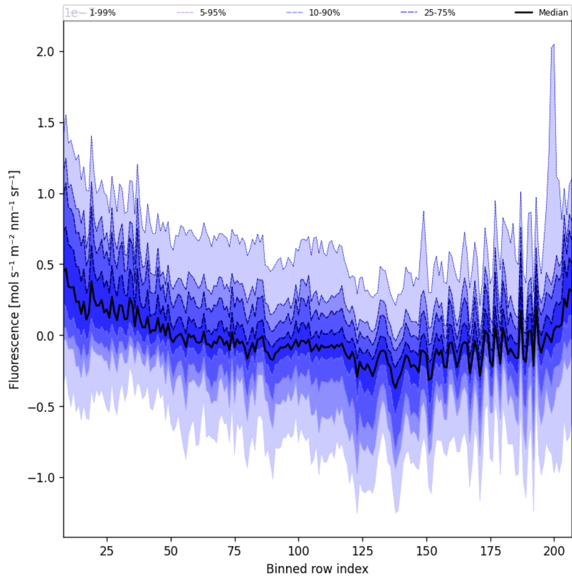
Figure 43: Along track statistics of “Fluorescence” for 2025-09-12 to 2025-09-14
