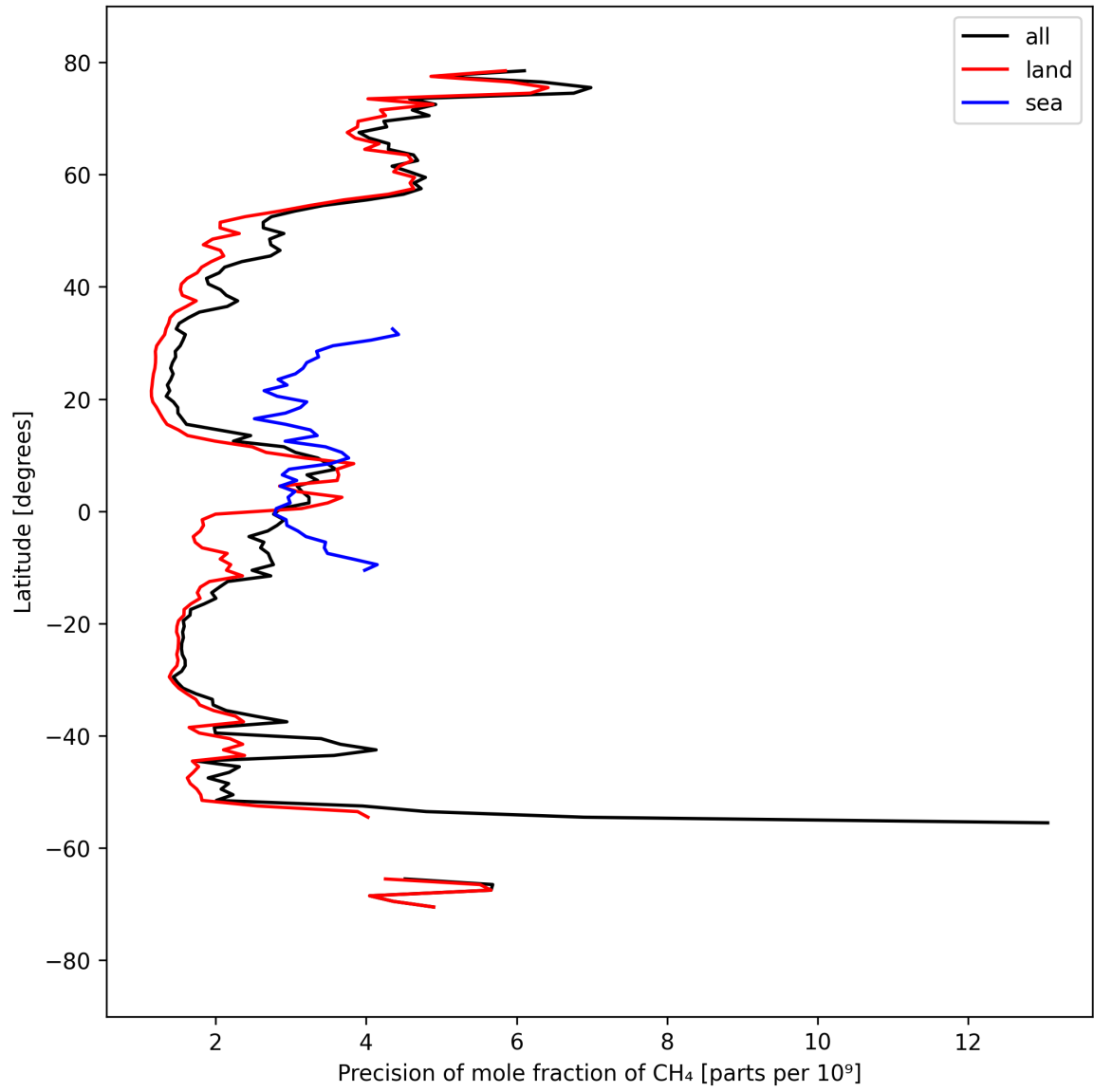
Figure 13: Zonal average of “Precision of mole fraction of CH 4 ” for 2025-09-12 to 2025-09-14.
