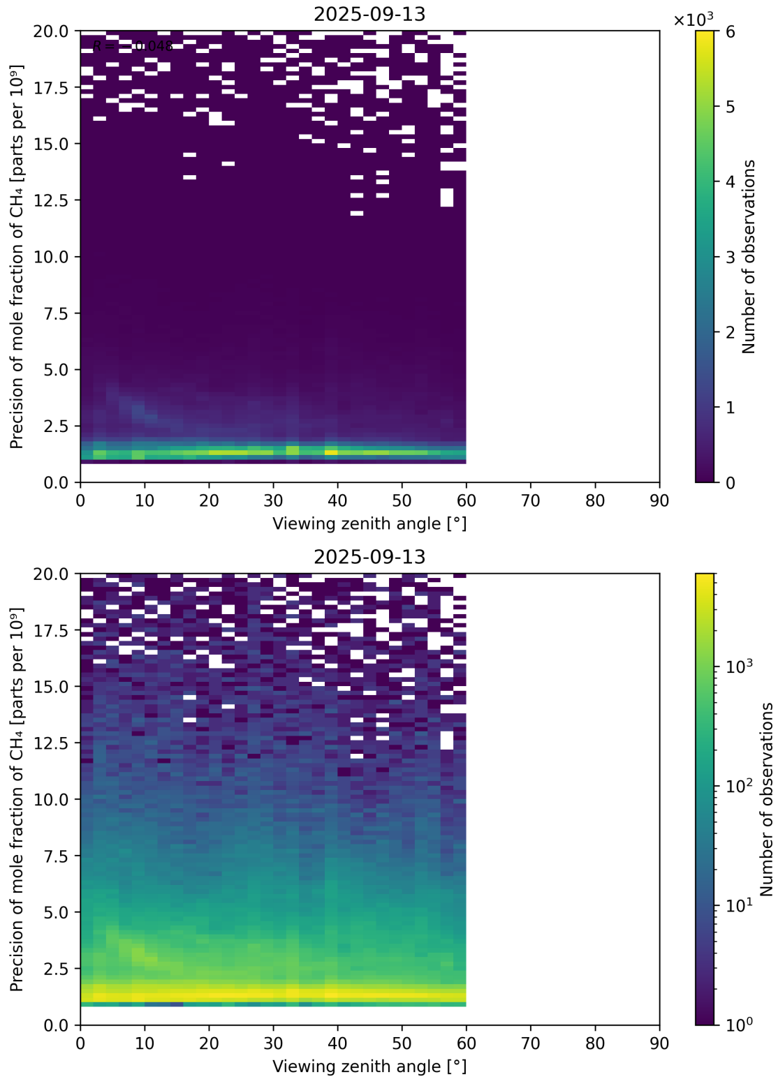
Figure 112: Scatter density plot of “Viewing zenith angle” against “Precision of mole fraction of \text{CH}_4 ” for 2025-09-12 to 2025-09-14.
