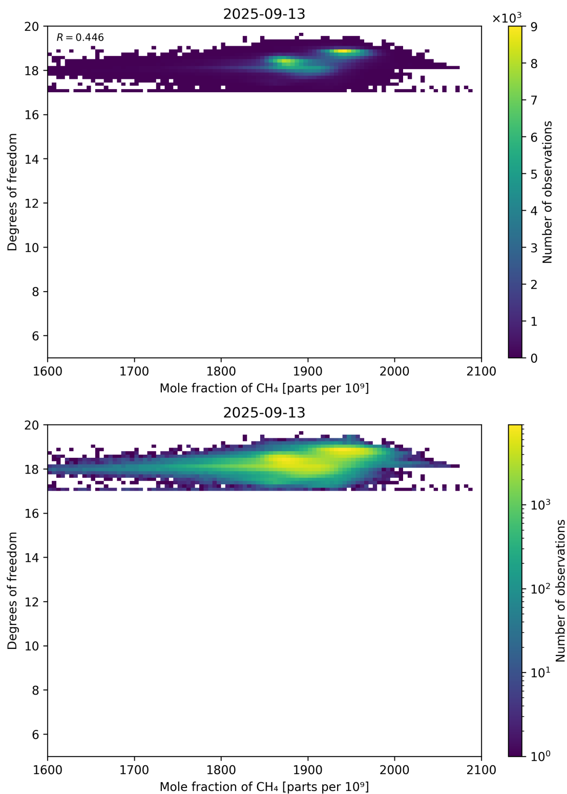
Figure 72: Scatter density plot of “Mole fraction of CH 4 ” against “Degrees of freedom” for 2025-09-12 to 2025-09-14.
