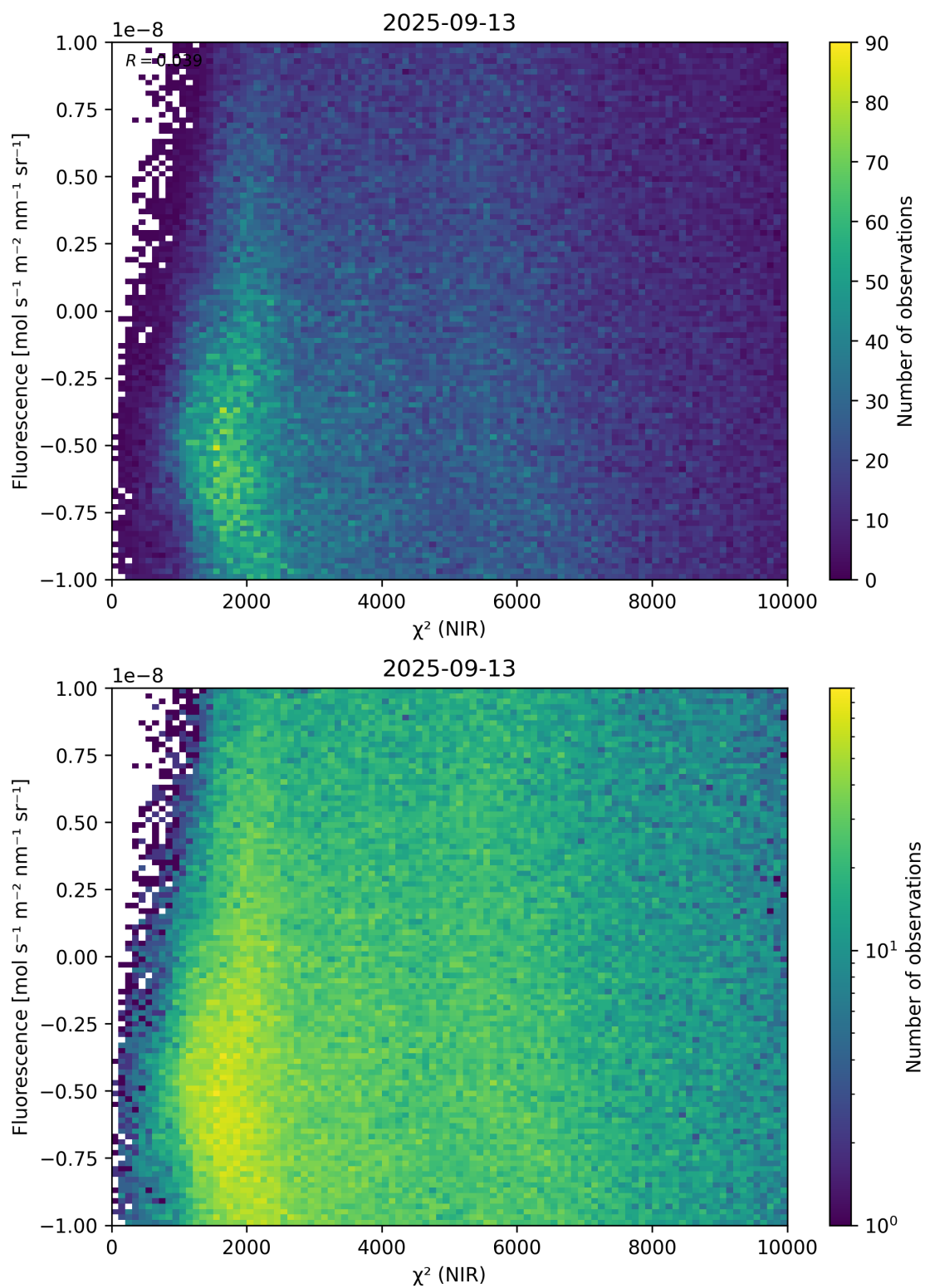
Figure 45: Scatter density plot of “ \chi^2 (NIR)” against “Fluorescence” for 2025-09-12 to 2025-09-14.
