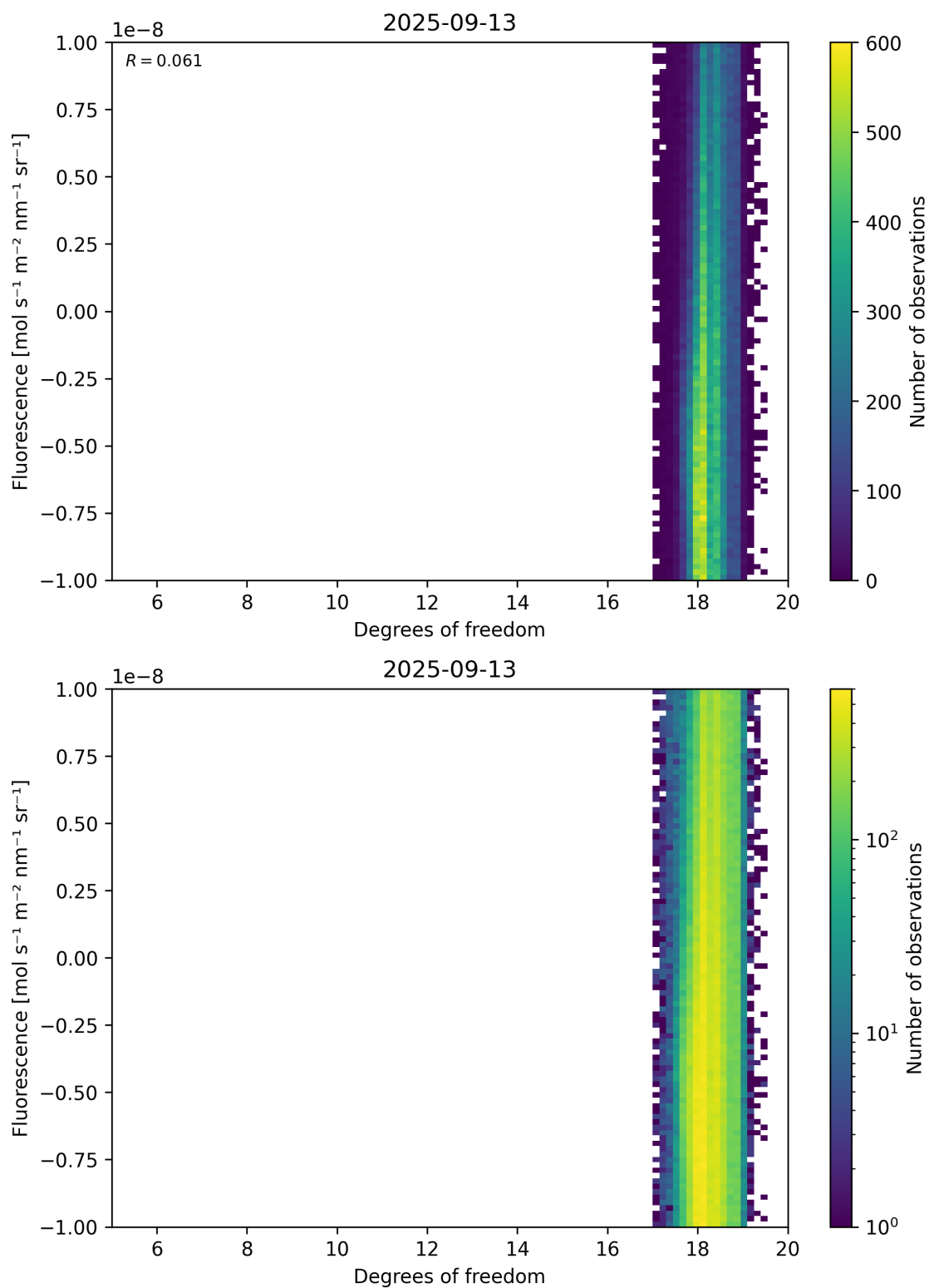
Figure 51: Scatter density plot of “Degrees of freedom” against “Fluorescence” for 2025-09-12 to 2025-09-14.
