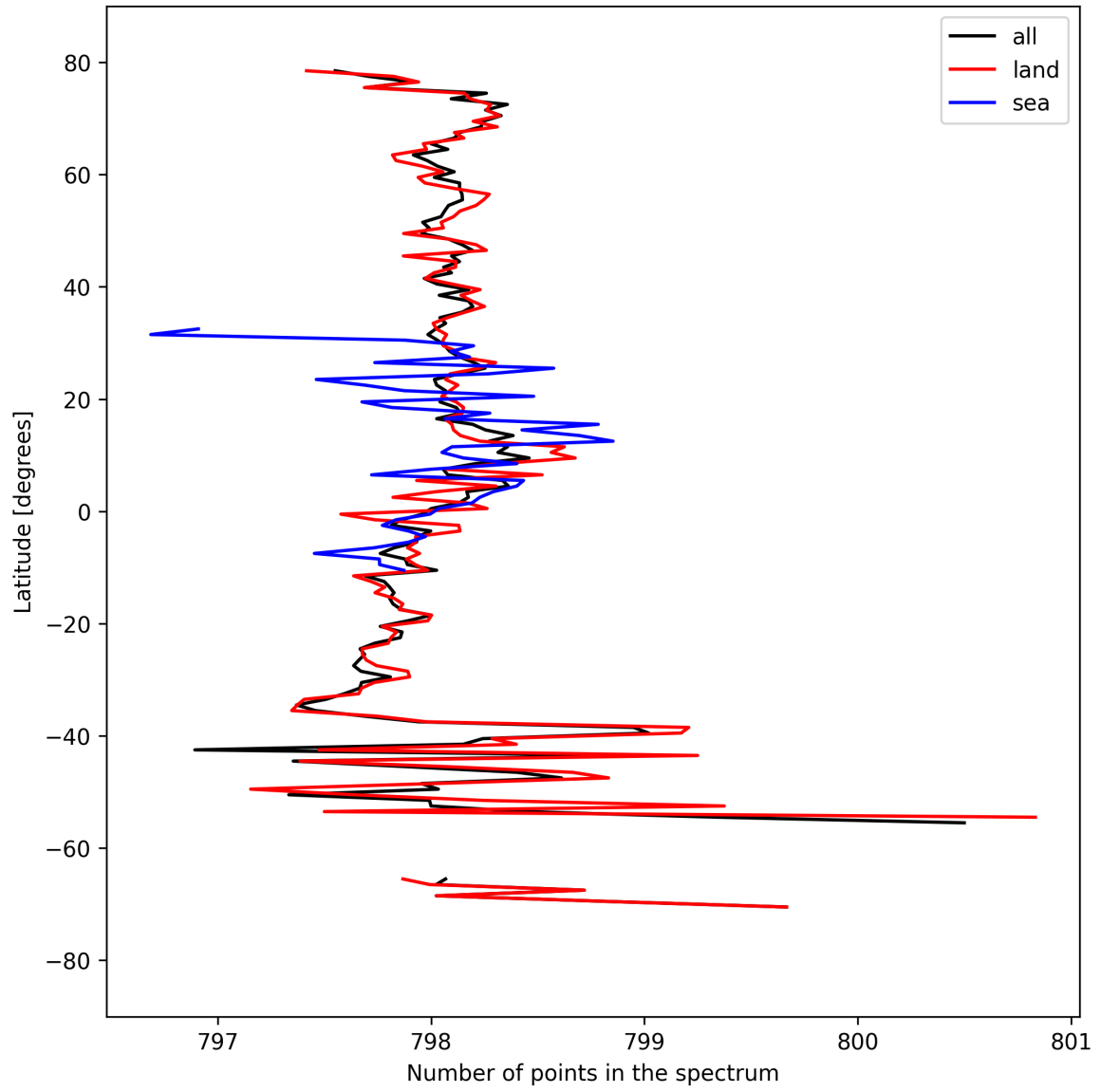
Figure 15: Zonal average of “Number of points in the spectrum” for 2025-09-12 to 2025-09-14.
