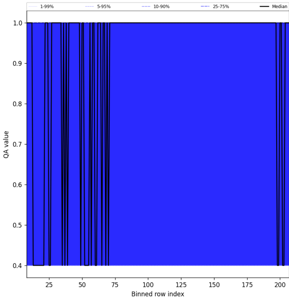
Figure 33: Along track statistics of “QA value” for 2025-09-12 to 2025-09-14
