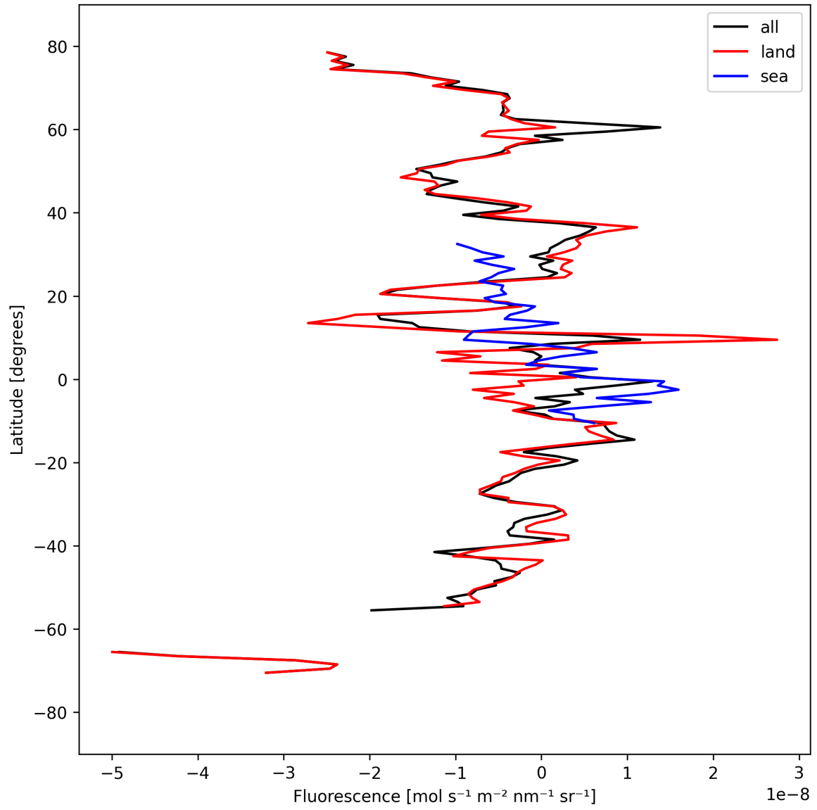
Figure 21: Zonal average of “Fluorescence” for 2025-09-12 to 2025-09-14.
