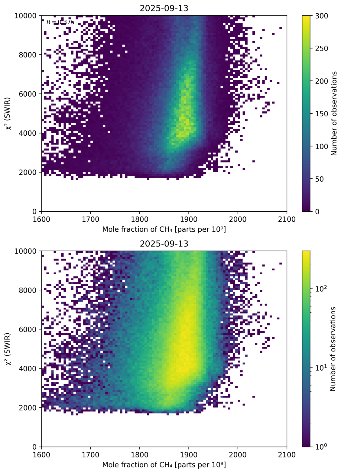
Figure 71: Scatter density plot of “Mole fraction of \text{CH}_4 ” against “ \chi^2 (SWIR)” for 2025-09-12 to 2025-09-14.
