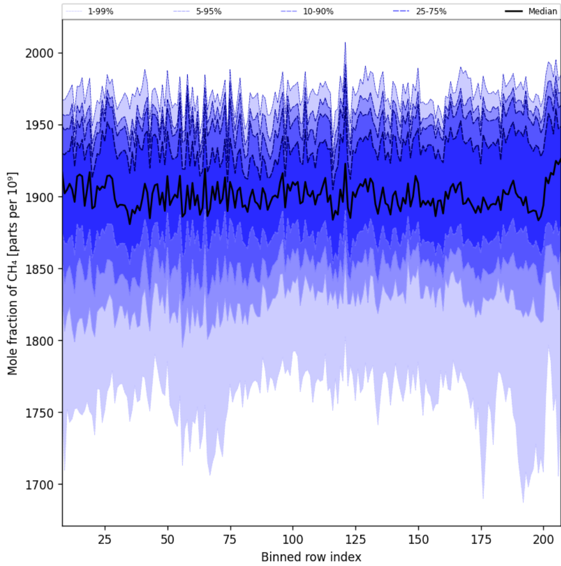
Figure 34: Along track statistics of “Mole fraction of CH 4 ” for 2025-09-12 to 2025-09-14
