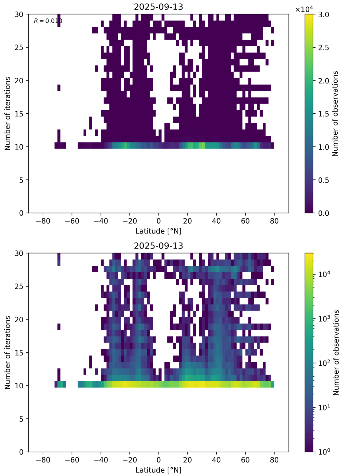
Figure 60: Scatter density plot of “Latitude” against “Number of iterations” for 2025-09-12 to 2025-09-14.
