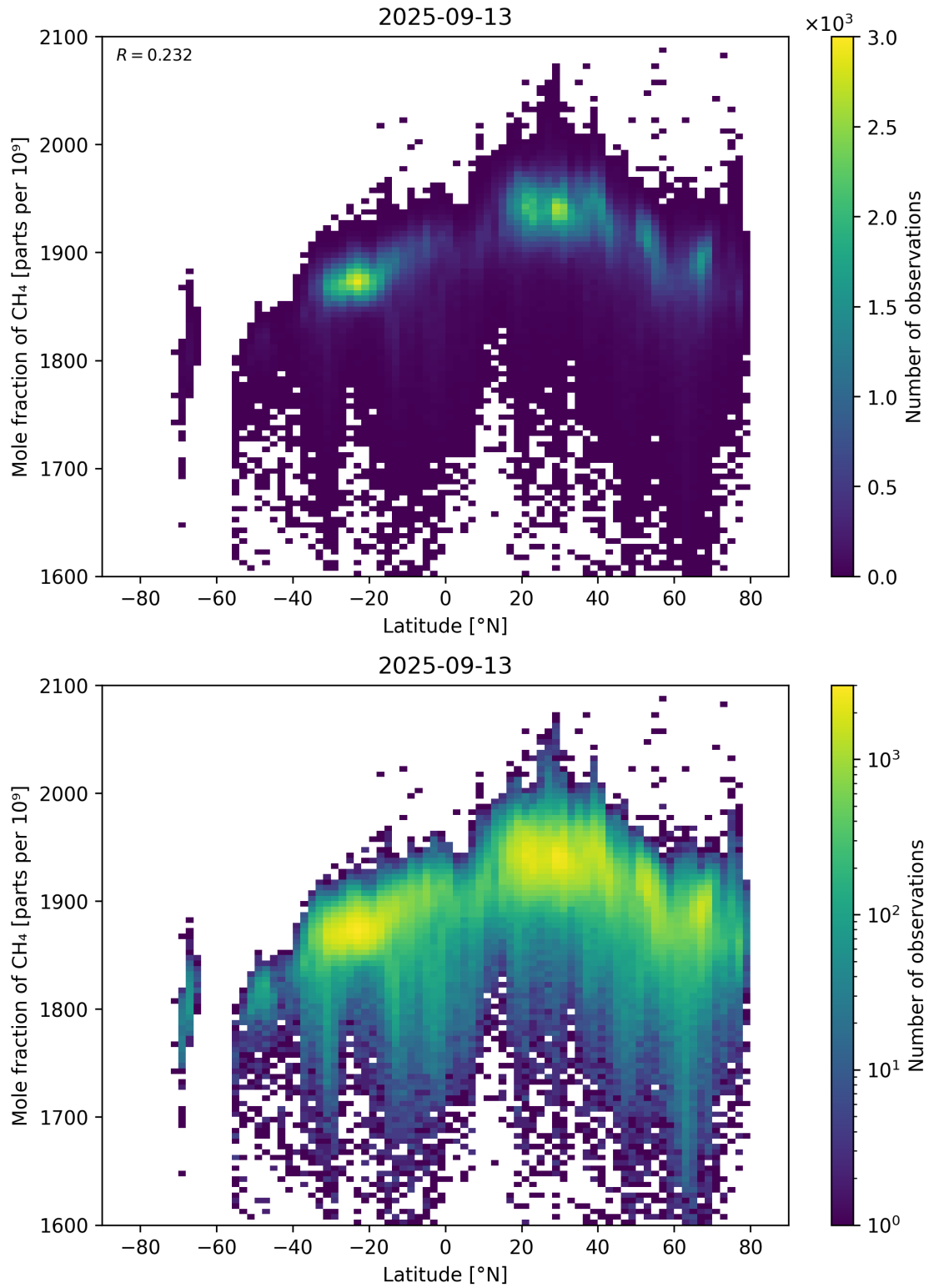
Figure 57: Scatter density plot of “Latitude” against “Mole fraction of CH 4 ” for 2025-09-12 to 2025-09-14.
