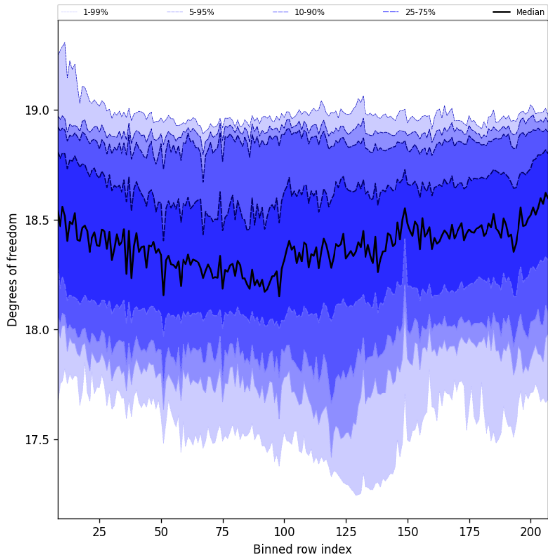
Figure 41: Along track statistics of “Degrees of freedom” for 2025-09-12 to 2025-09-14
