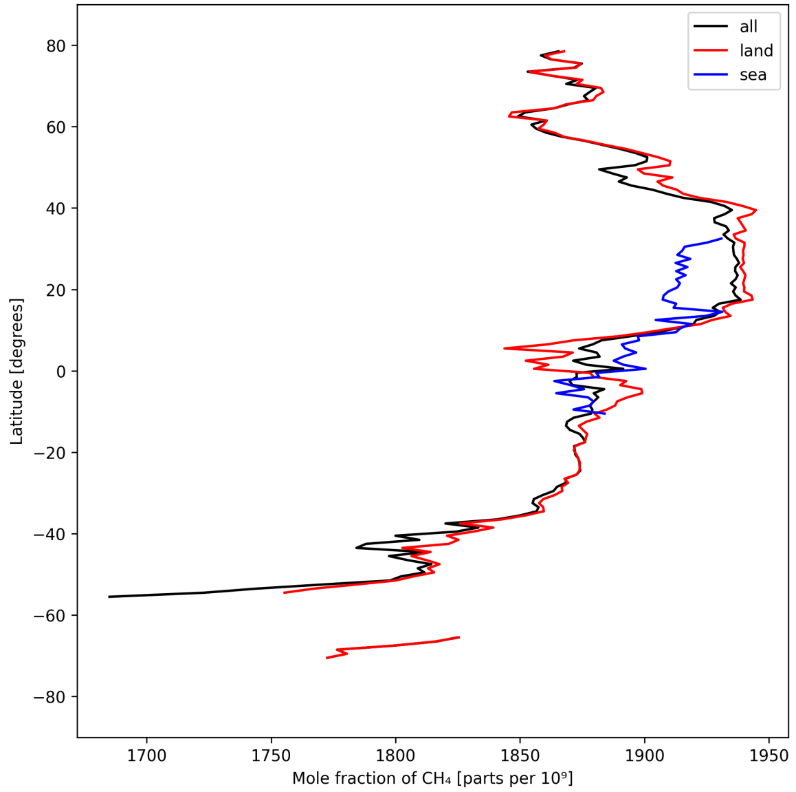
Figure 12: Zonal average of “Mole fraction of CH 4 ” for 2025-09-12 to 2025-09-14.
