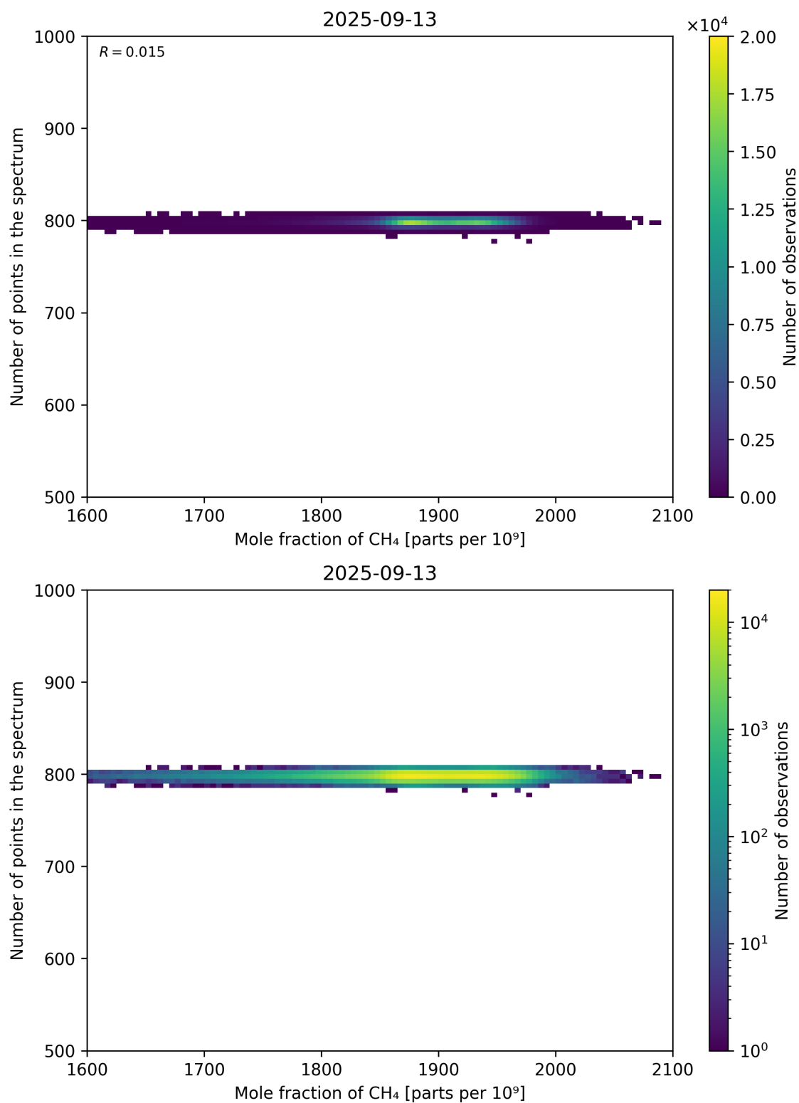
Figure 77: Scatter density plot of “Mole fraction of CH 4 ” against “Number of points in the spectrum” for 2025-09-12 to 2025-09-14.
