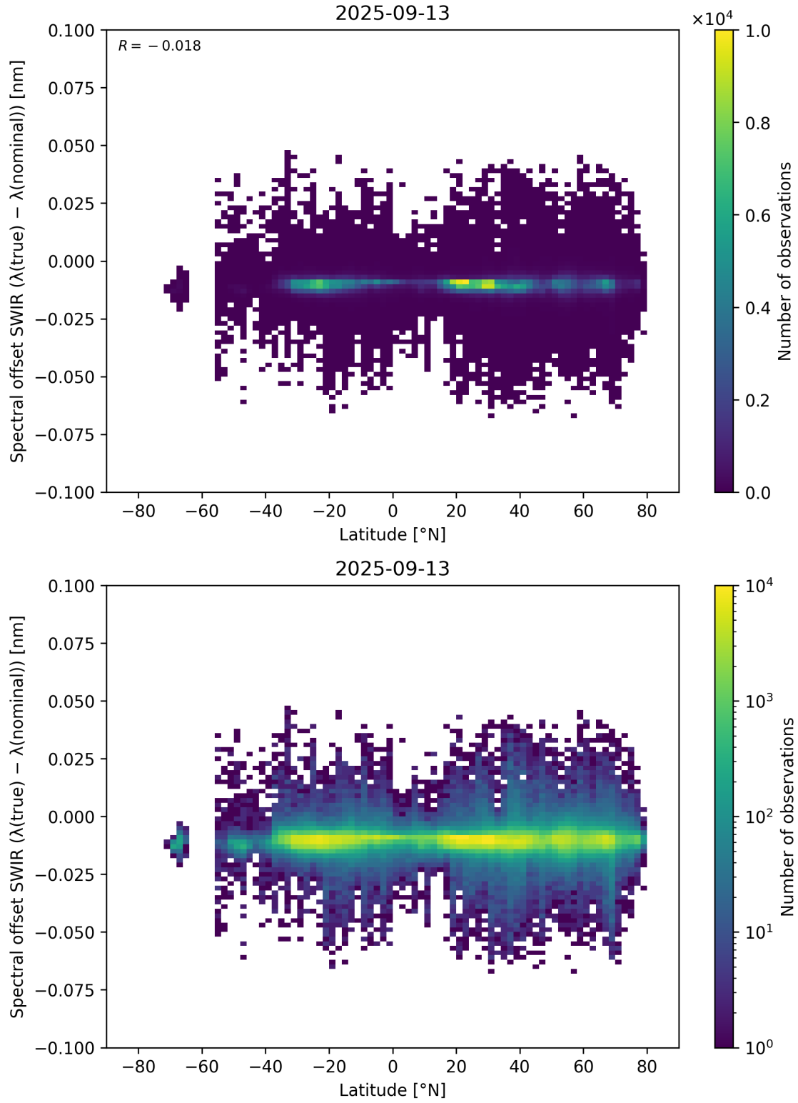
Figure 62: Scatter density plot of “Latitude” against “Spectral offset SWIR ( \lambda_{\text{true}} - \lambda_{\text{nominal}} )” for 2025-09-12 to 2025-09-14.
