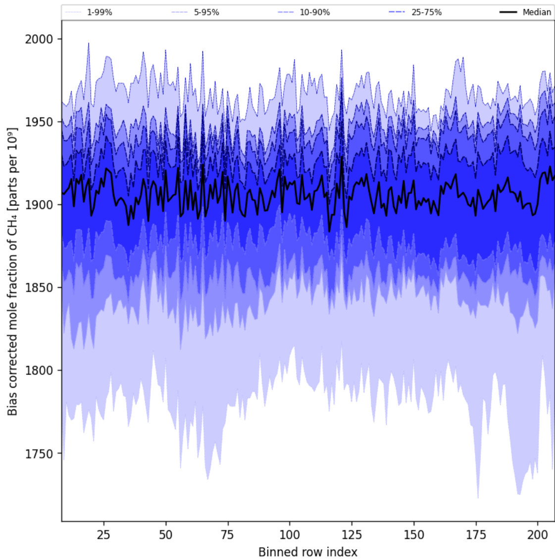
Figure 36: Along track statistics of “Bias corrected mole fraction of CH 4 ” for 2025-09-12 to 2025-09-14
