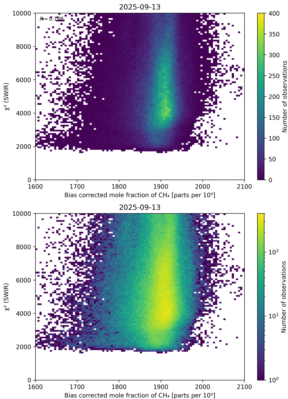
Figure 64: Scatter density plot of “Bias corrected mole fraction of \text{CH}_4 ” against “ \chi^2 (SWIR)” for 2025-09-12 to 2025-09-14.
