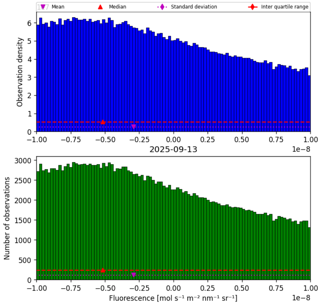
Figure 32: Histogram of “Fluorescence” for 2025-09-12 to 2025-09-14
