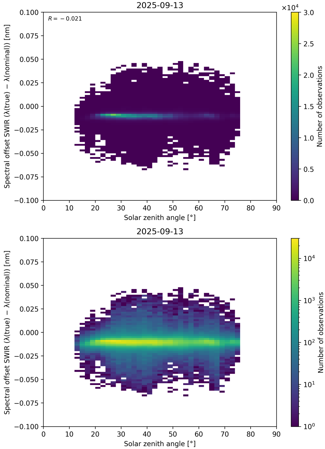
Figure 104: Scatter density plot of “Solar zenith angle” against “Spectral offset SWIR ( \lambda_{\text{true}} - \lambda_{\text{nominal}} )” for 2025-09-12 to 2025-09-14.
