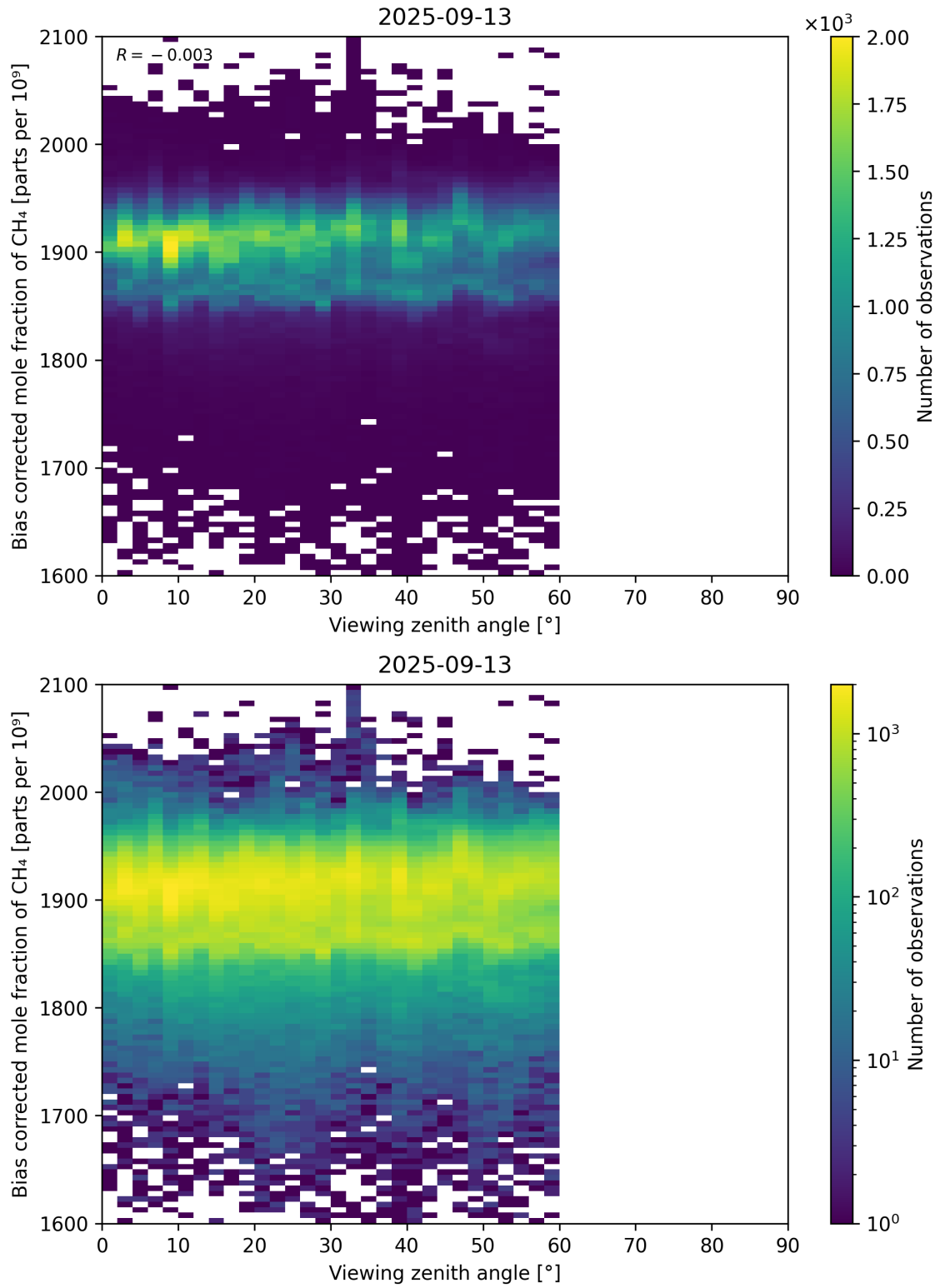
Figure 111: Scatter density plot of “Viewing zenith angle” against “Bias corrected mole fraction of CH 4 ” for 2025-09-12 to 2025-09-14.
