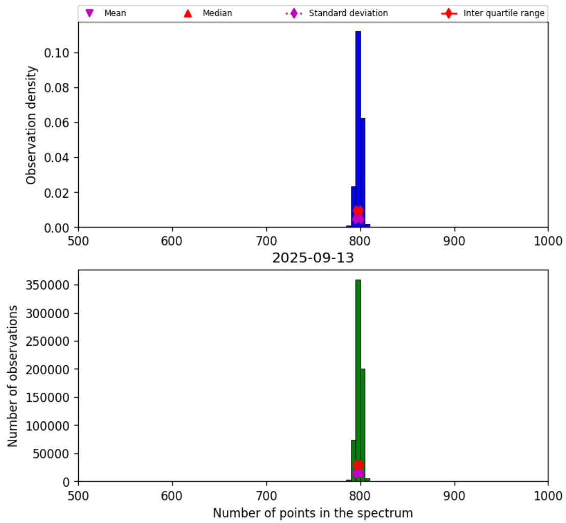
Figure 26: Histogram of “Number of points in the spectrum” for 2025-09-12 to 2025-09-14
