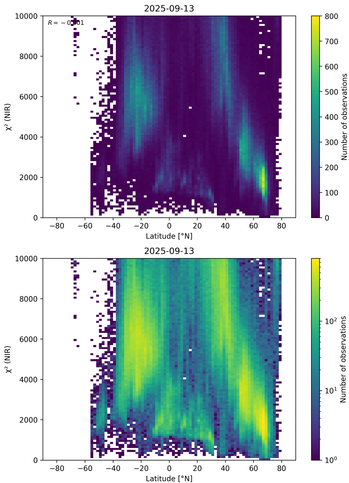
Figure 53: Scatter density plot of “Latitude” against “ \chi^2 (NIR)” for 2025-09-12 to 2025-09-14.
