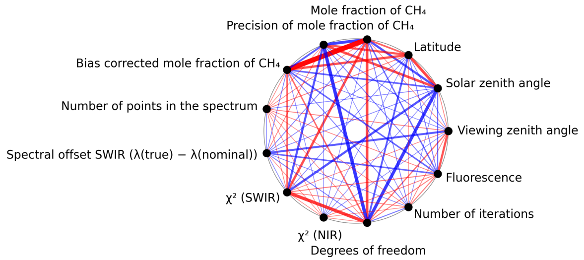
Figure 1: Map of correlation graph for 2025-09-12 to 2025-09-14.
