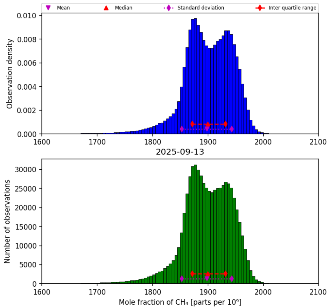
Figure 23: Histogram of “Mole fraction of CH 4 ” for 2025-09-12 to 2025-09-14
