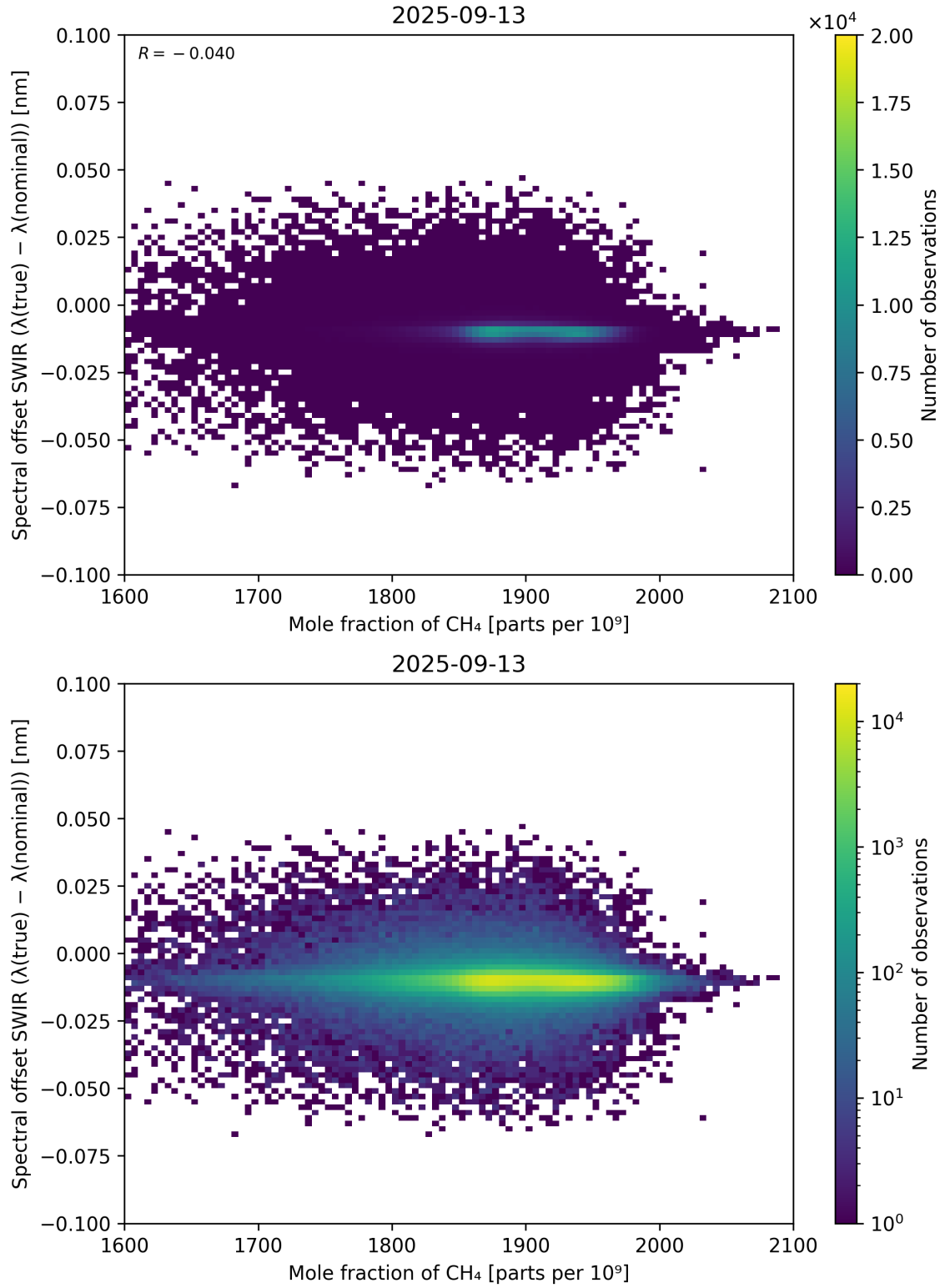
Figure 86: Scatter density plot of “Mole fraction of CH 4 ” against “Spectral offset SWIR ( \lambda_{\text{true}} - \lambda_{\text{nominal}} )” for 2025-09-12 to 2025-09-14.
