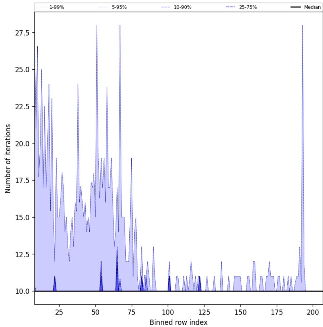
Figure 42: Along track statistics of “Number of iterations” for 2025-09-12 to 2025-09-14
