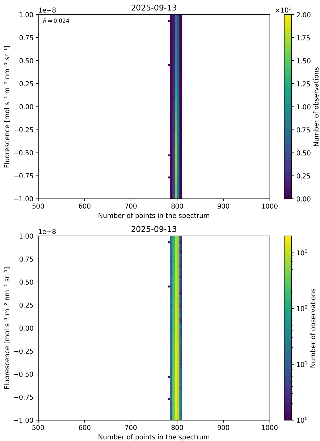
Figure 91: Scatter density plot of “Number of points in the spectrum” against “Fluorescence” for 2025-09-12 to 2025-09-14.
