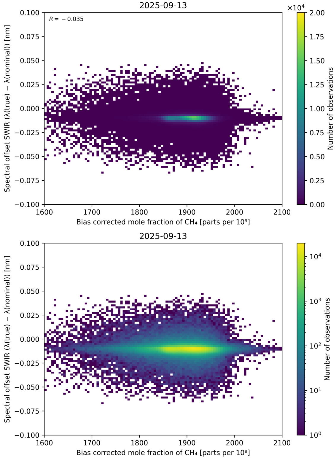
Figure 69: Scatter density plot of “Bias corrected mole fraction of \text{CH}_4 ” against “Spectral offset SWIR ( \lambda_{\text{true}} - \lambda_{\text{nominal}} )” for 2025-09-12 to 2025-09-14.
