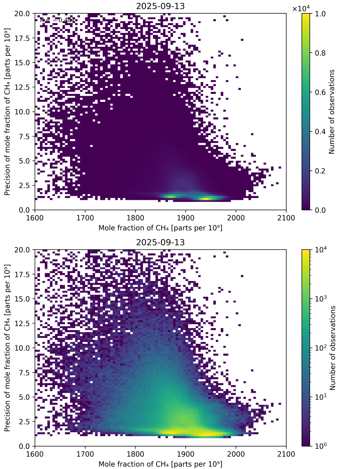
Figure 75: Scatter density plot of “Mole fraction of CH 4 ” against “Precision of mole fraction of CH 4 ” for 2025-09-12 to 2025-09-14.
