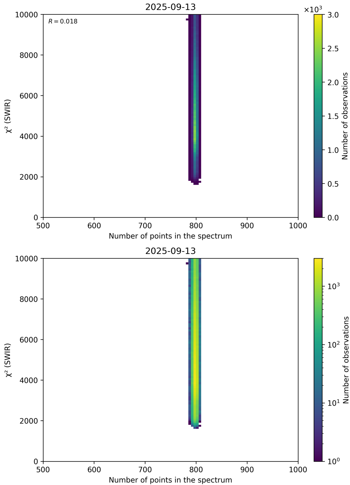
Figure 89: Scatter density plot of “Number of points in the spectrum” against “ \chi^2 (SWIR)” for 2025-09-12 to 2025-09-14.
