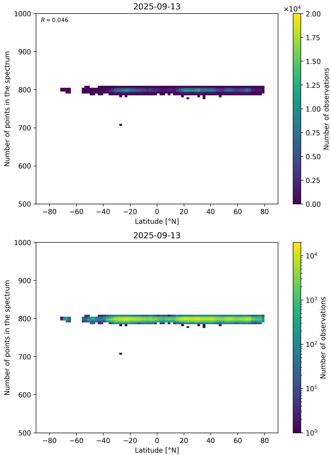
Figure 61: Scatter density plot of “Latitude” against “Number of points in the spectrum” for 2025-09-12 to 2025-09-14.
