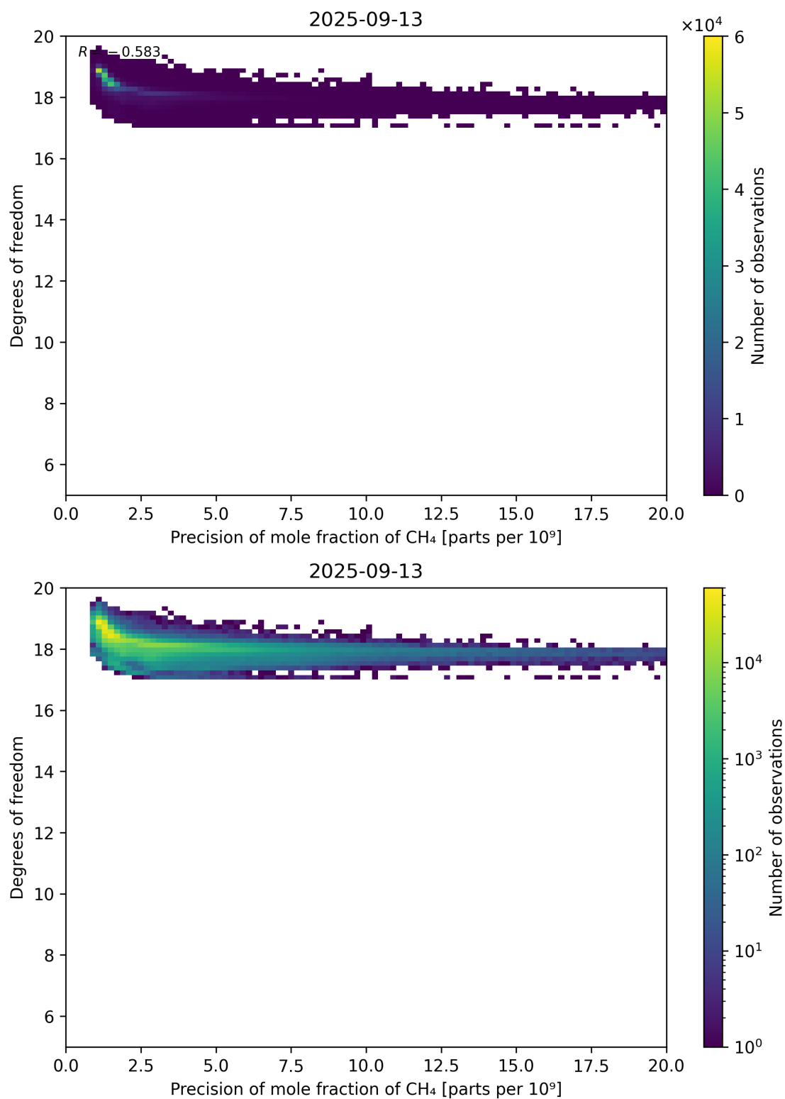
Figure 80: Scatter density plot of “Precision of mole fraction of CH 4 ” against “Degrees of freedom” for 2025-09-12 to 2025-09-14.
