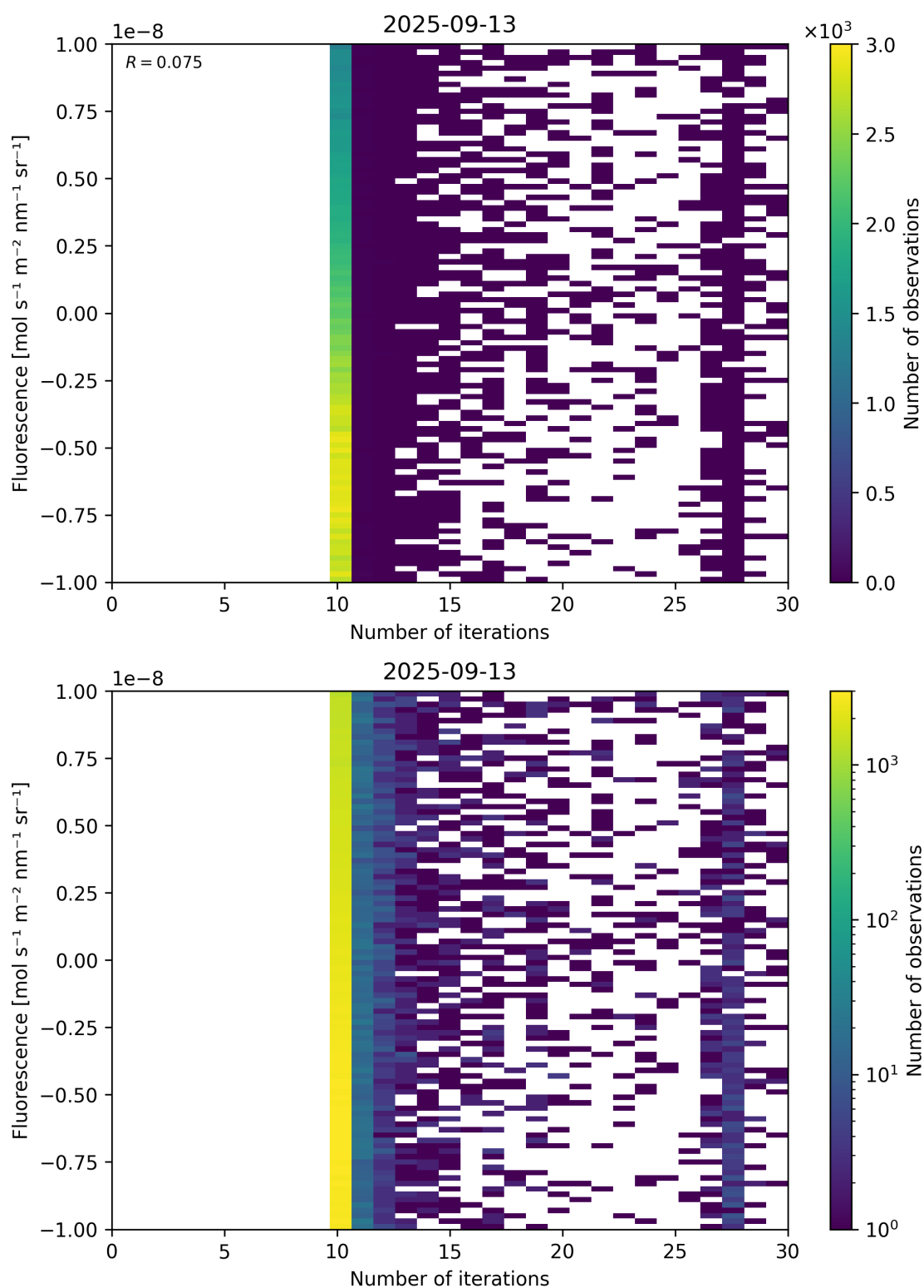
Figure 87: Scatter density plot of “Number of iterations” against “Fluorescence” for 2025-09-12 to 2025-09-14.
