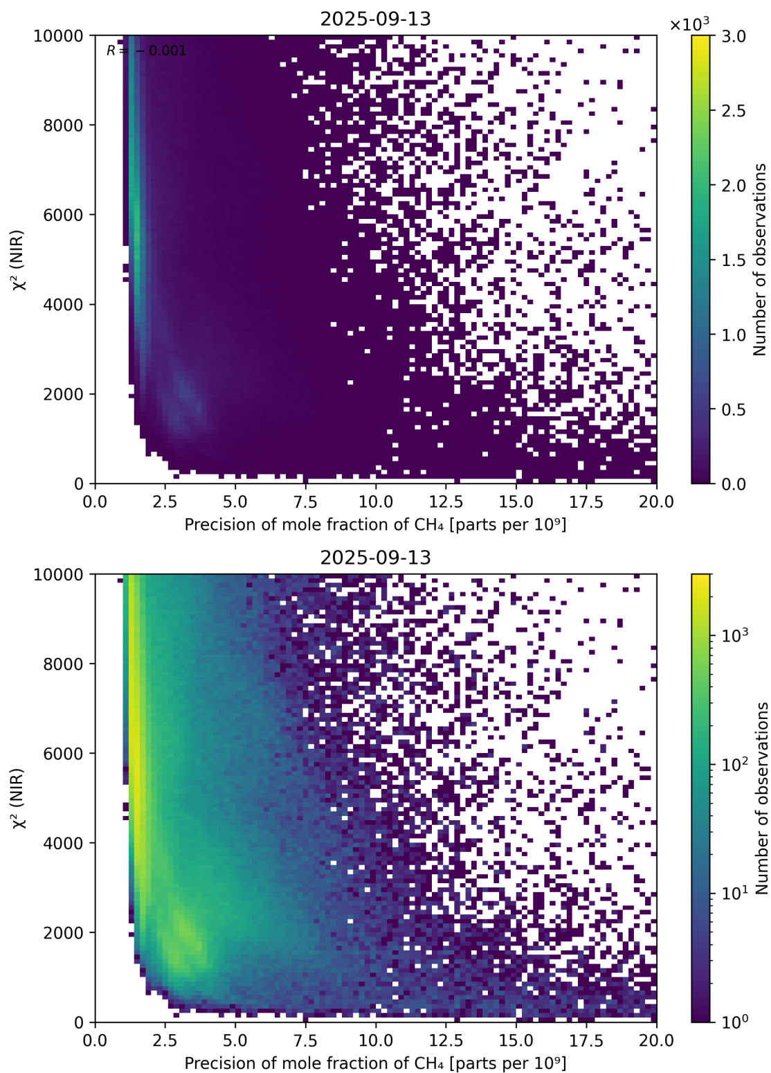
Figure 78: Scatter density plot of “Precision of mole fraction of CH 4 ” against “ \chi^2 (NIR)” for 2025-09-12 to 2025-09-14.
