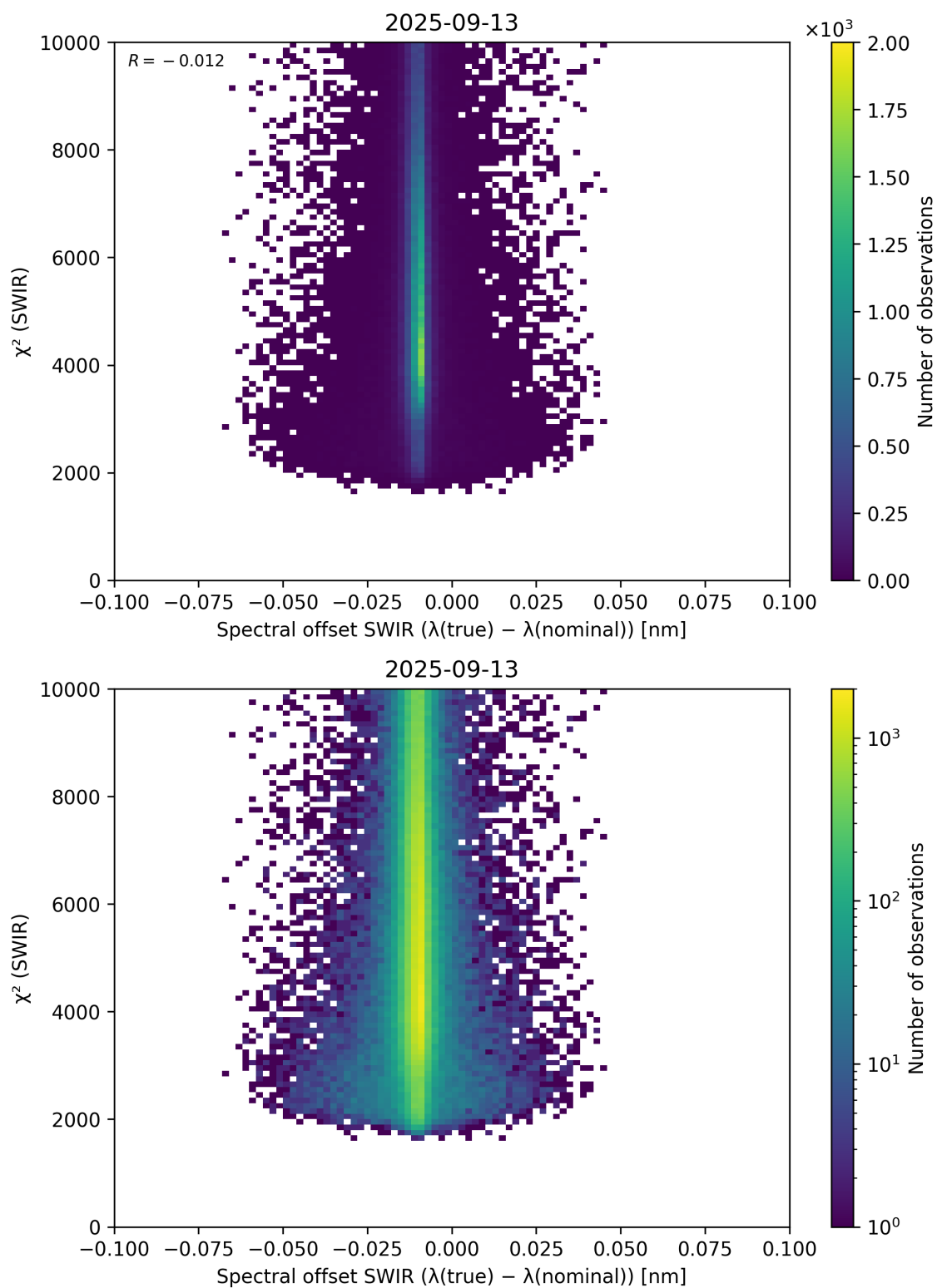
Figure 118: Scatter density plot of “Spectral offset SWIR ( \lambda_{\text{true}} - \lambda_{\text{nominal}} )” against “ \chi^2 (SWIR)” for 2025-09-12 to 2025-09-14.
