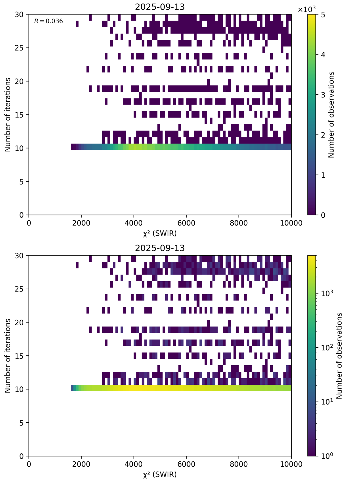
Figure 50: Scatter density plot of “ \chi^2 (SWIR)” against “Number of iterations” for 2025-09-12 to 2025-09-14.
