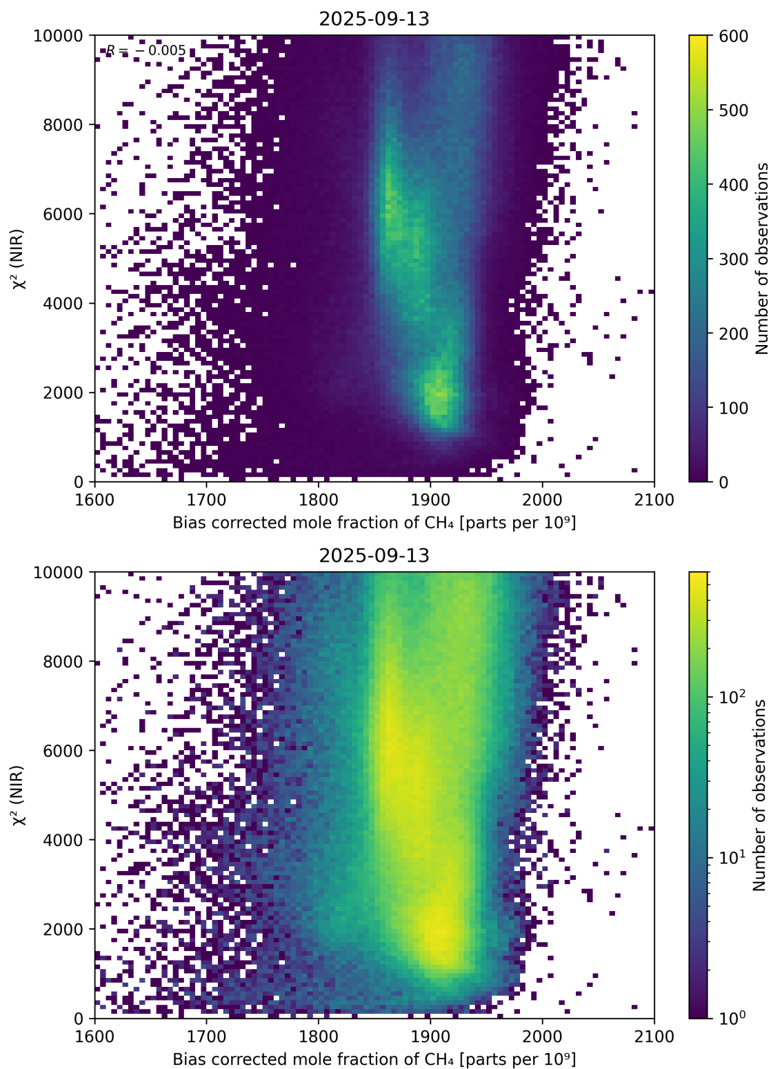
Figure 63: Scatter density plot of “Bias corrected mole fraction of CH 4 ” against “ \chi^2 (NIR)” for 2025-09-12 to 2025-09-14.
