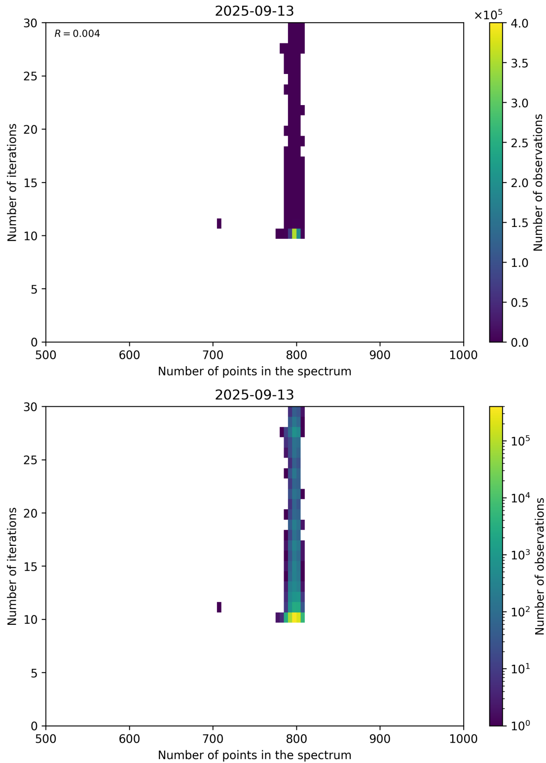
Figure 92: Scatter density plot of “Number of points in the spectrum” against “Number of iterations” for 2025-09-12 to 2025-09-14.
