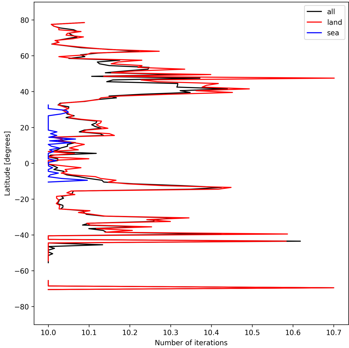
Figure 20: Zonal average of “Number of iterations” for 2025-09-12 to 2025-09-14.
