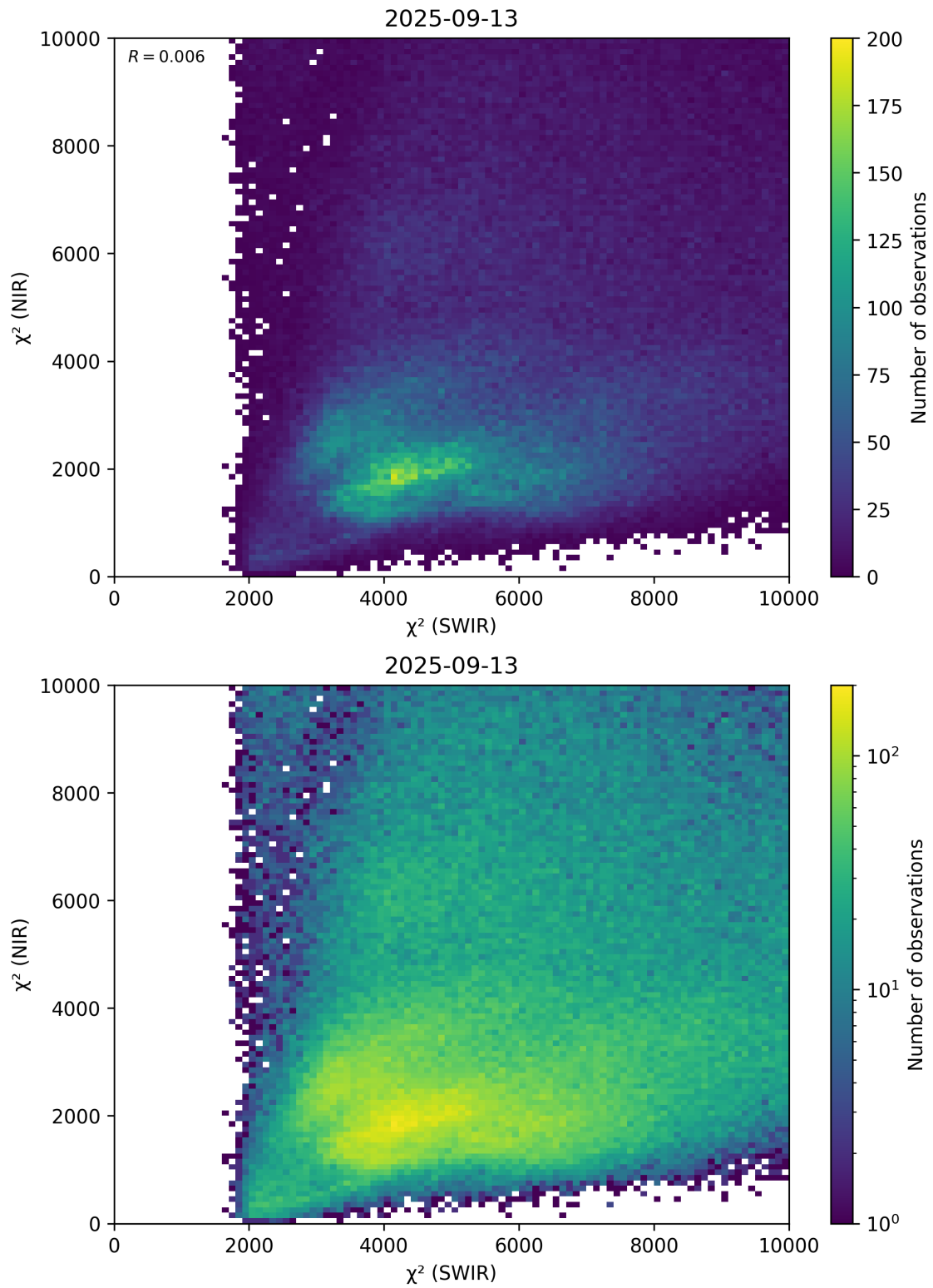
Figure 47: Scatter density plot of “ \chi^2 (SWIR)” against “ \chi^2 (NIR)” for 2025-09-12 to 2025-09-14.
