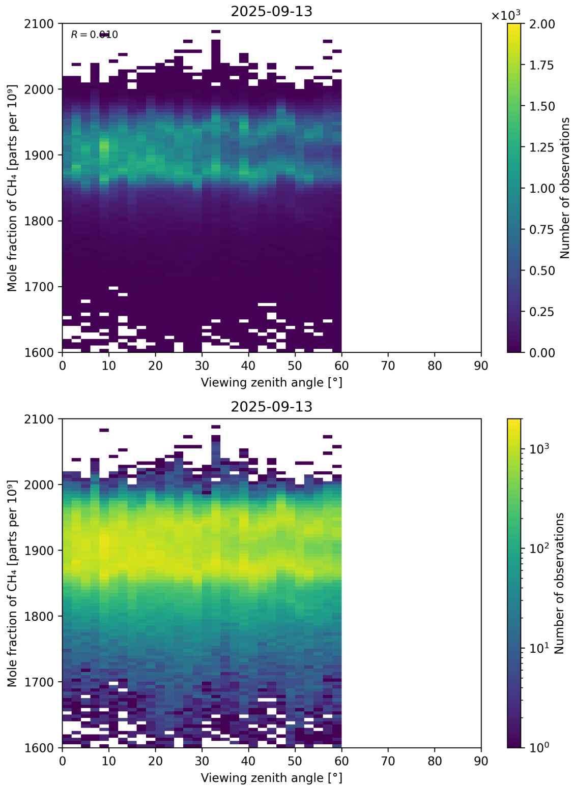
Figure 110: Scatter density plot of “Viewing zenith angle” against “Mole fraction of CH 4 ” for 2025-09-12 to 2025-09-14.
