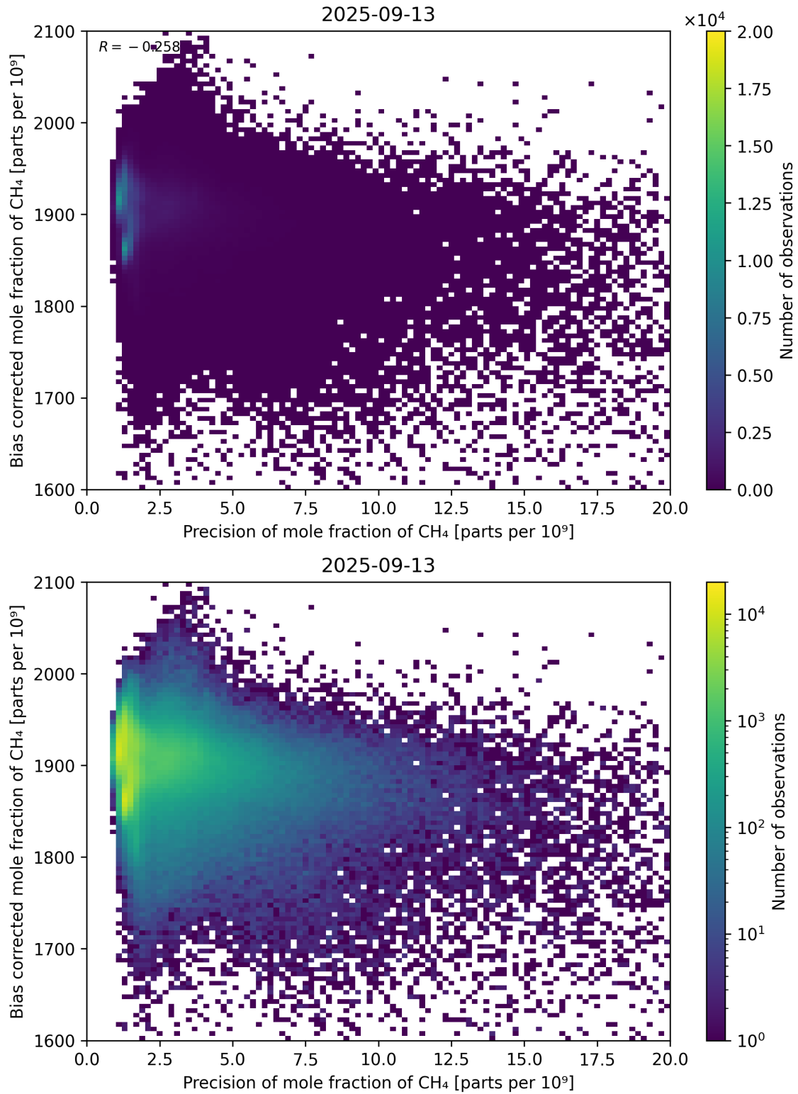
Figure 82: Scatter density plot of “Precision of mole fraction of CH 4 ” against “Bias corrected mole fraction of CH 4 ” for 2025-09-12 to 2025-09-14.
