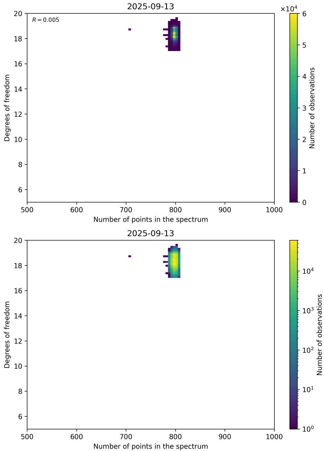
Figure 90: Scatter density plot of “Number of points in the spectrum” against “Degrees of freedom” for 2025-09-12 to 2025-09-14.
