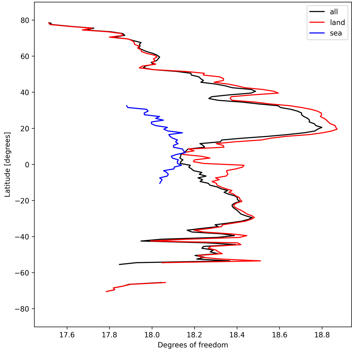
Figure 19: Zonal average of “Degrees of freedom” for 2025-09-12 to 2025-09-14.
