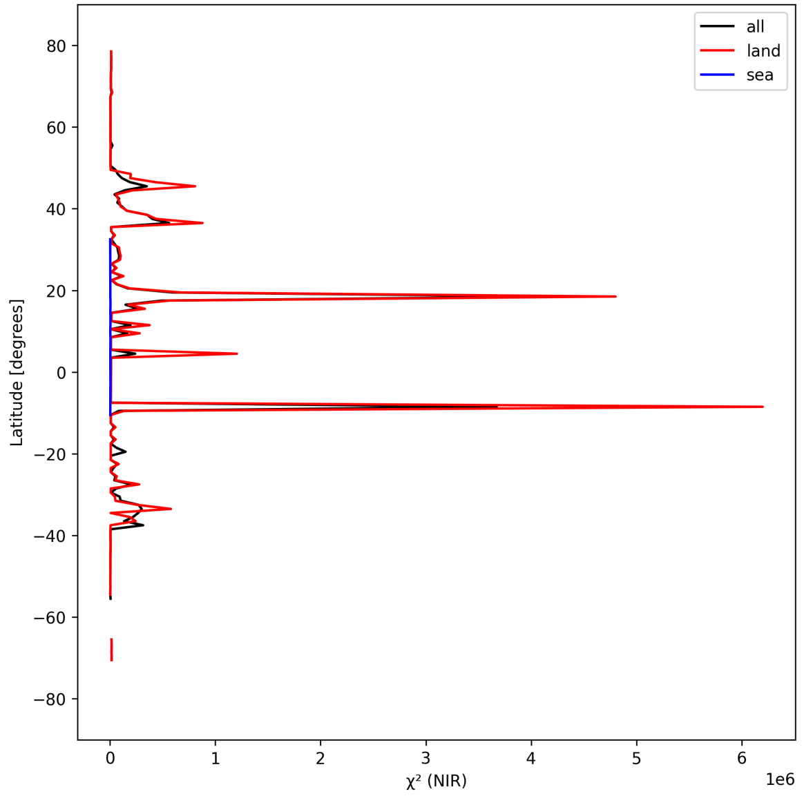
Figure 18: Zonal average of “ \chi^2 (NIR)” for 2025-09-12 to 2025-09-14.
