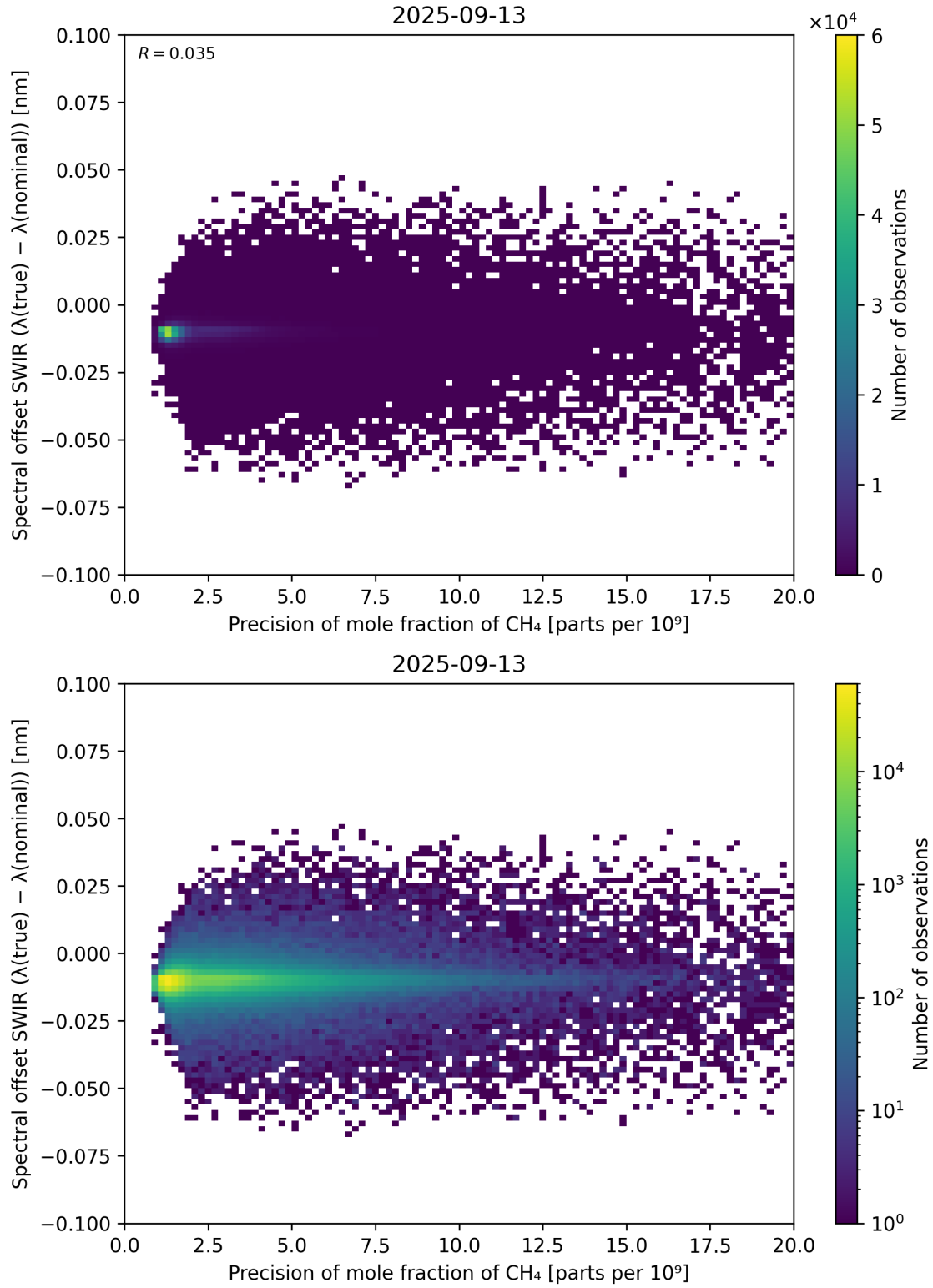
Figure 85: Scatter density plot of “Precision of mole fraction of CH 4 ” against “Spectral offset SWIR ( \lambda_{\text{true}} - \lambda_{\text{nominal}} )” for 2025-09-12 to 2025-09-14.
