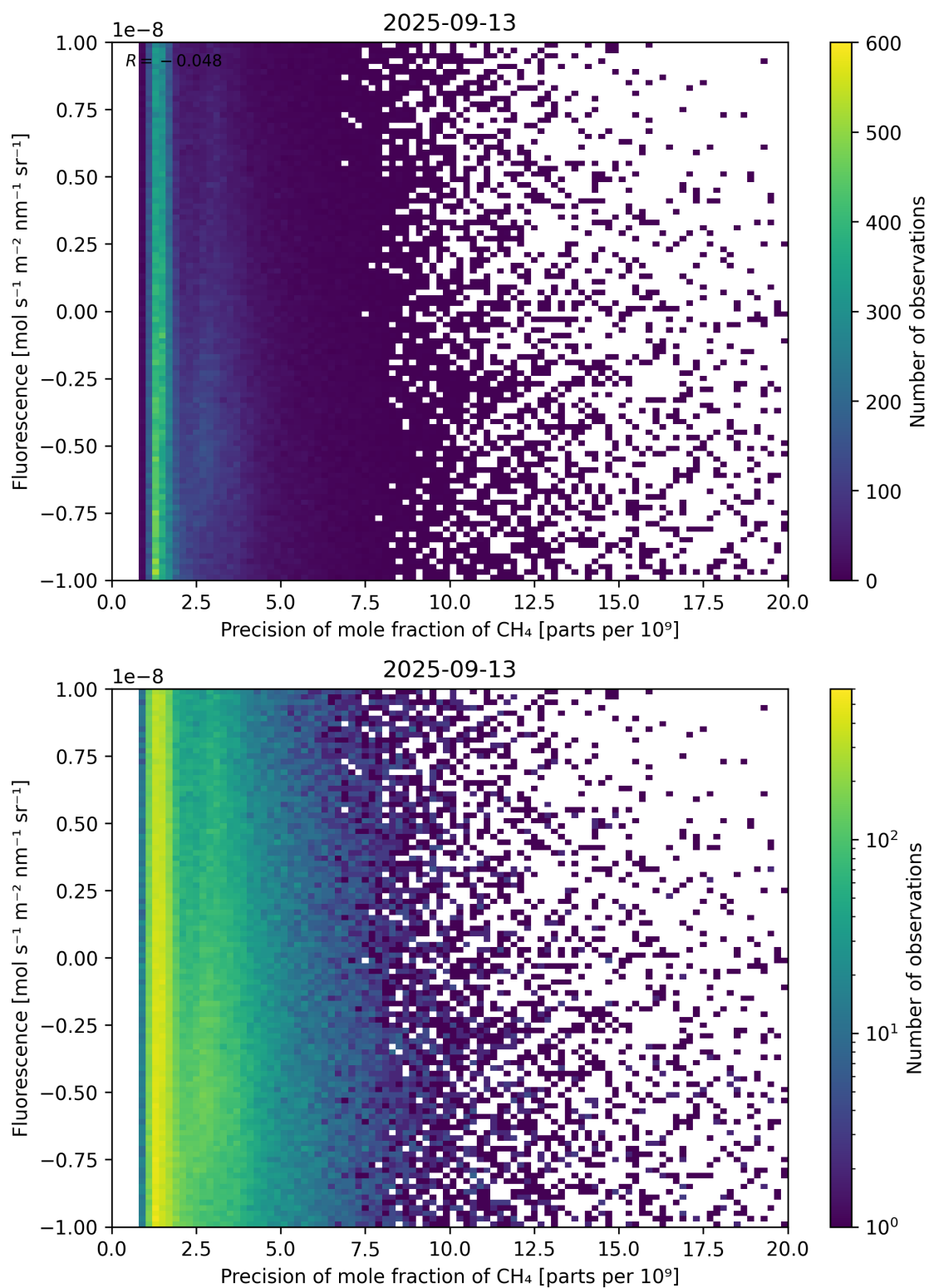
Figure 81: Scatter density plot of “Precision of mole fraction of \text{CH}_4 ” against “Fluorescence” for 2025-09-12 to 2025-09-14.
