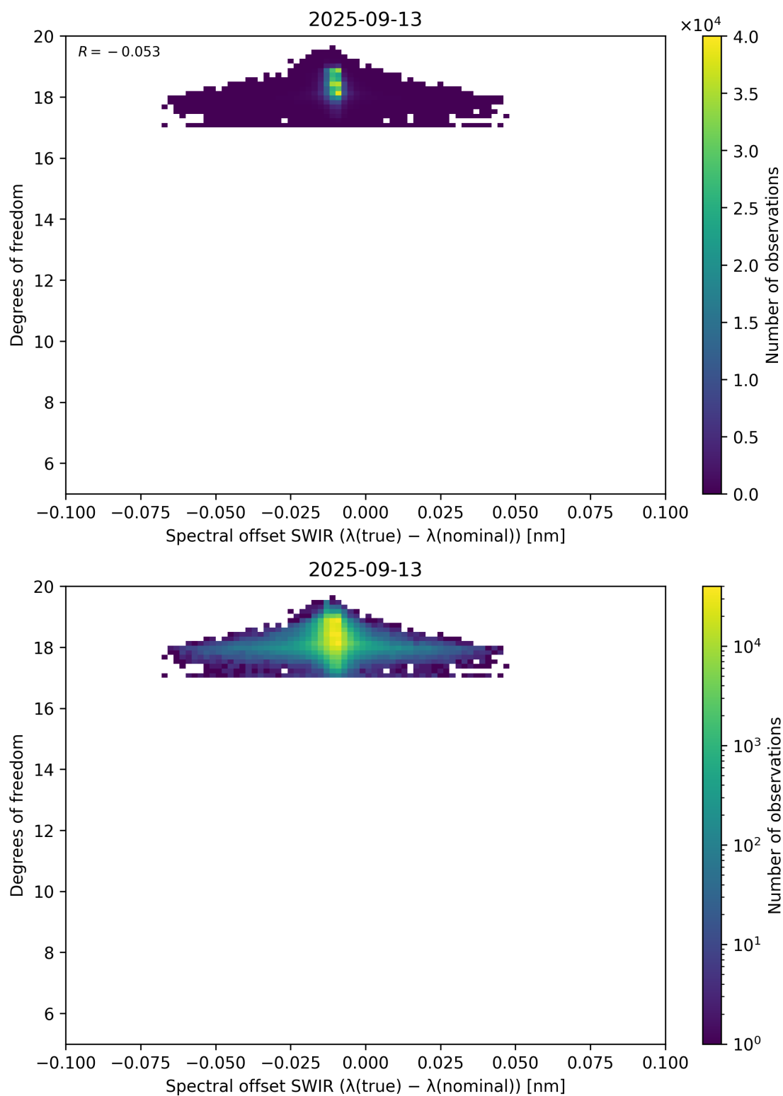
Figure 119: Scatter density plot of “Spectral offset SWIR ( \lambda_{\text{true}} - \lambda_{\text{nominal}} )” against “Degrees of freedom” for 2025-09-12 to 2025-09-14.
