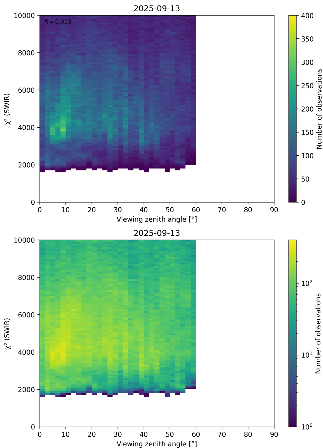
Figure 106: Scatter density plot of “Viewing zenith angle” against “ \chi^2 (SWIR)” for 2025-09-12 to 2025-09-14.
