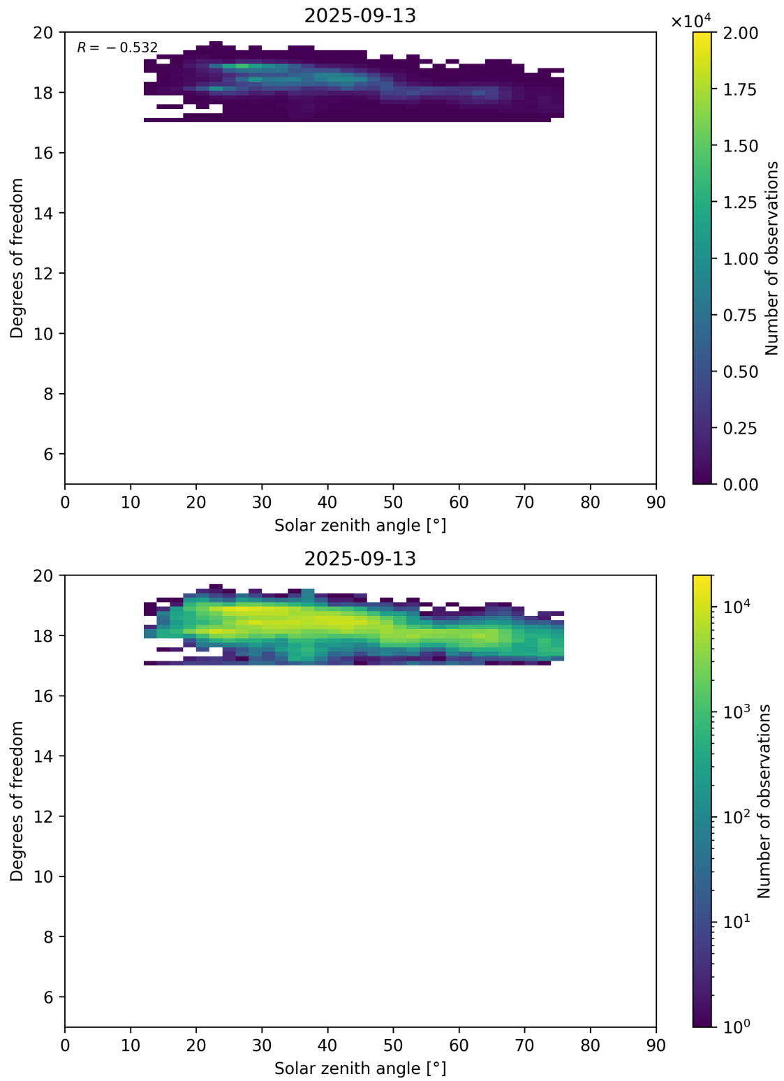
Figure 96: Scatter density plot of “Solar zenith angle” against “Degrees of freedom” for 2025-09-12 to 2025-09-14.
