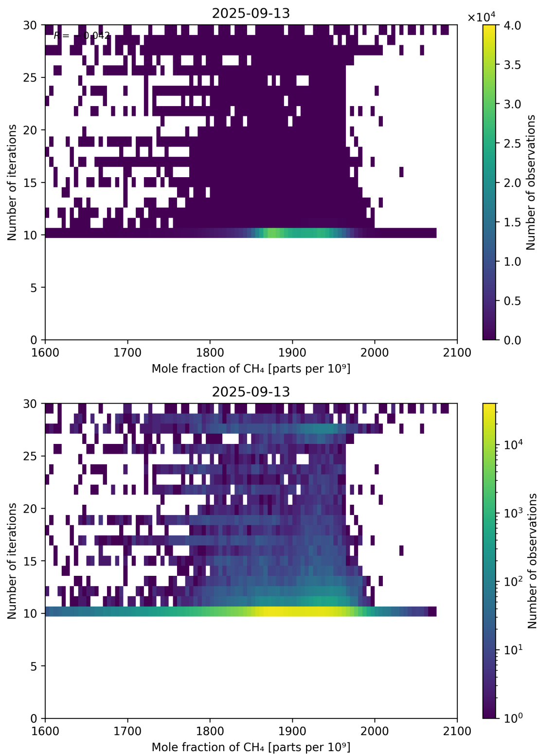
Figure 76: Scatter density plot of “Mole fraction of CH 4 ” against “Number of iterations” for 2025-09-12 to 2025-09-14.
