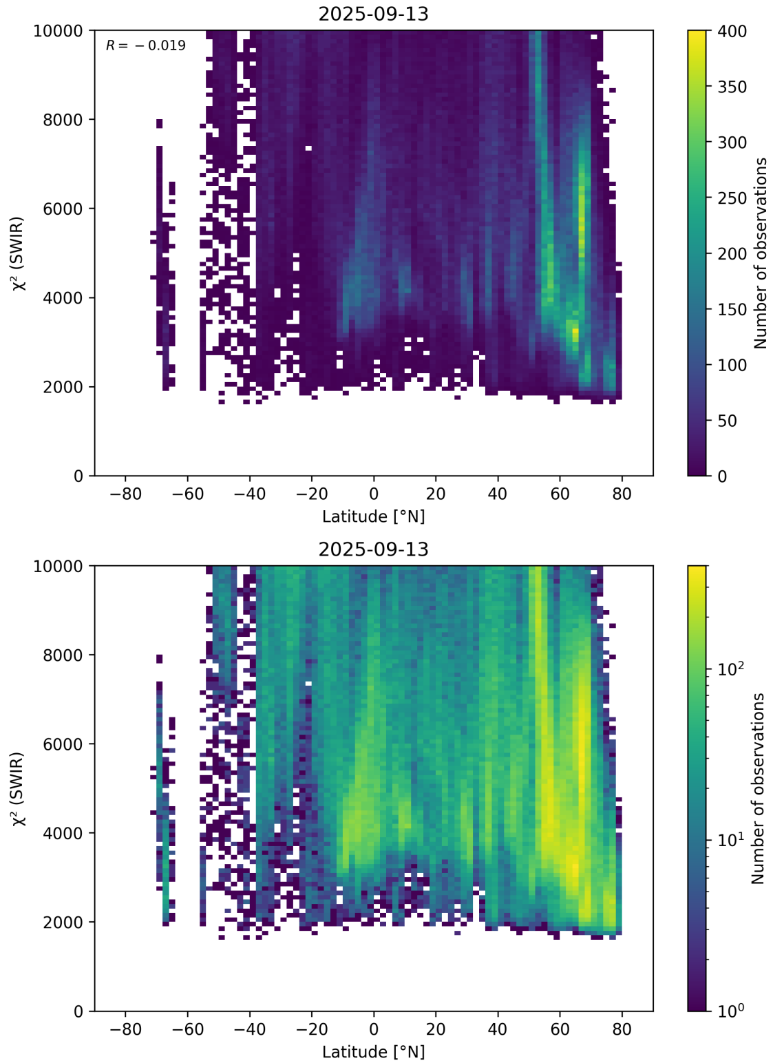
Figure 54: Scatter density plot of “Latitude” against “ \chi^2 (SWIR)” for 2025-09-12 to 2025-09-14.
