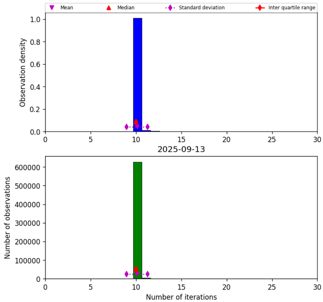
Figure 31: Histogram of “Number of iterations” for 2025-09-12 to 2025-09-14
