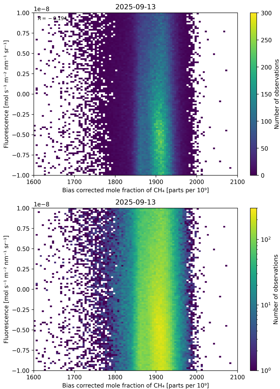
Figure 66: Scatter density plot of “Bias corrected mole fraction of \text{CH}_4 ” against “Fluorescence” for 2025-09-12 to 2025-09-14.
