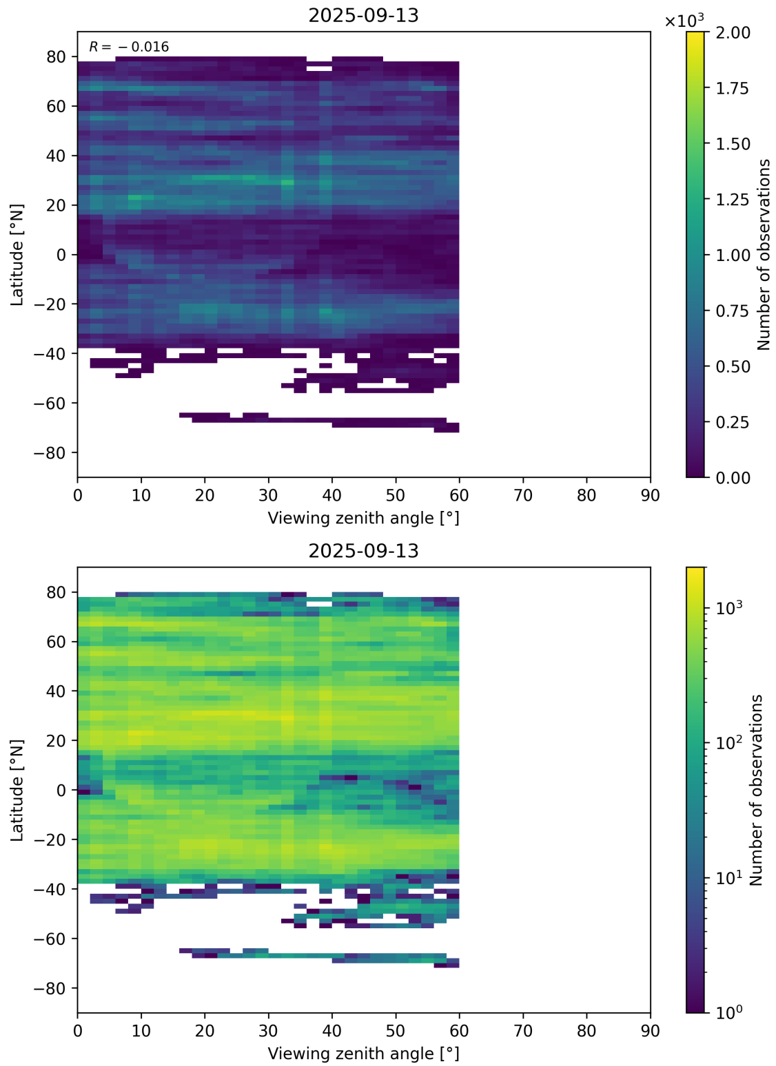
Figure 109: Scatter density plot of “Viewing zenith angle” against “Latitude” for 2025-09-12 to 2025-09-14.
