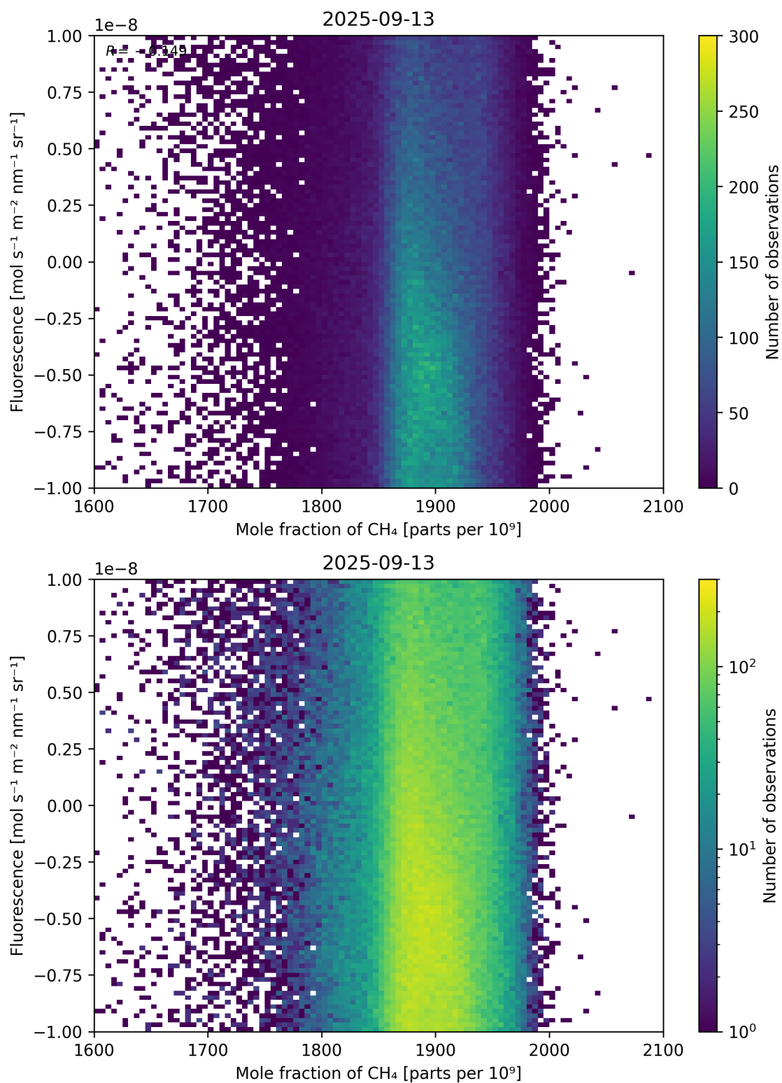
Figure 73: Scatter density plot of “Mole fraction of \text{CH}_4 ” against “Fluorescence” for 2025-09-12 to 2025-09-14.
