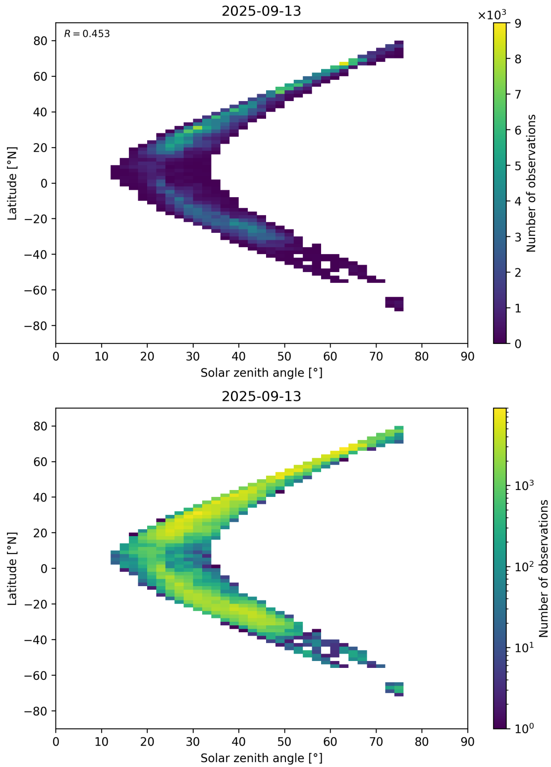
Figure 98: Scatter density plot of “Solar zenith angle” against “Latitude” for 2025-09-12 to 2025-09-14.
