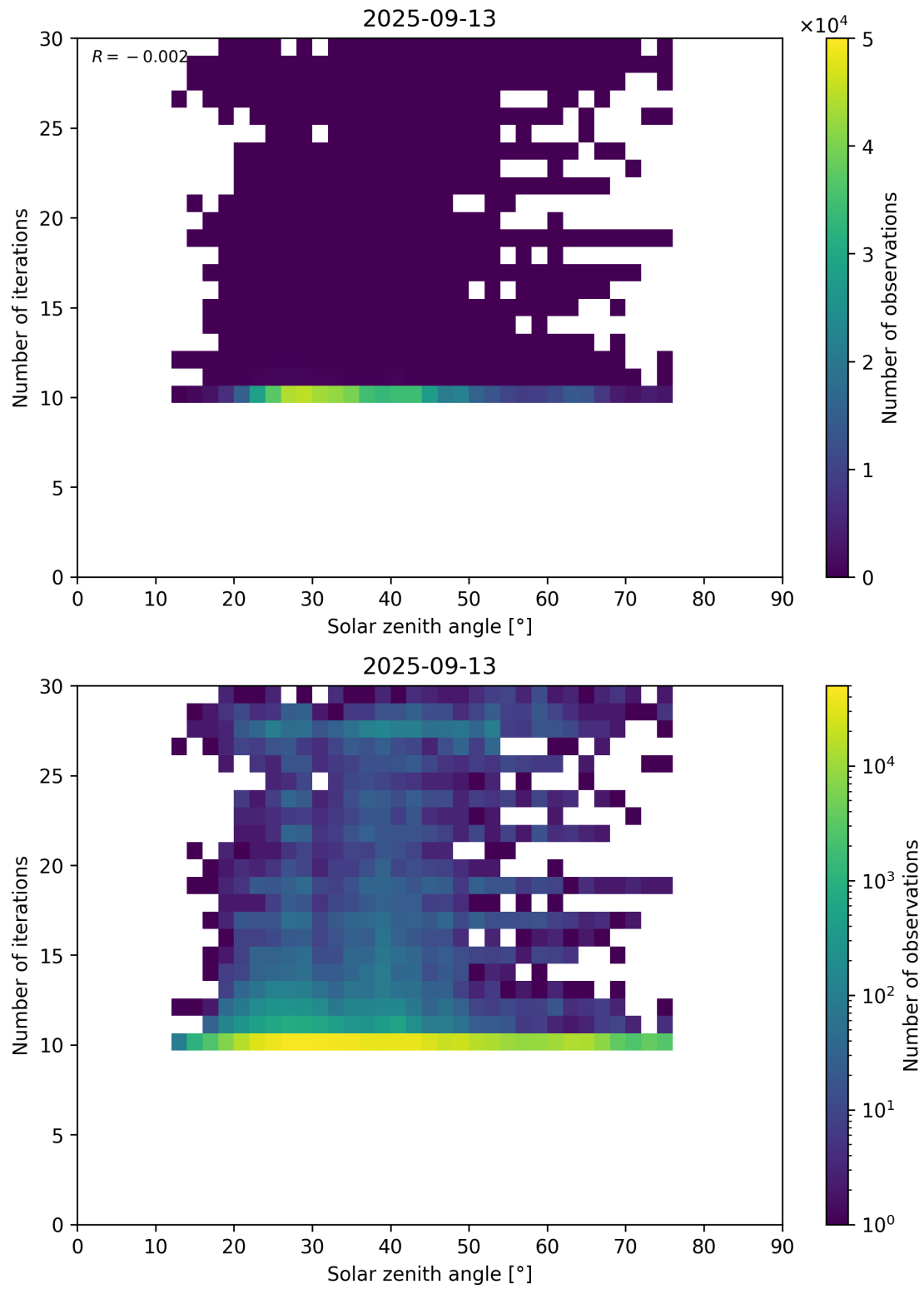
Figure 102: Scatter density plot of “Solar zenith angle” against “Number of iterations” for 2025-09-12 to 2025-09-14.
