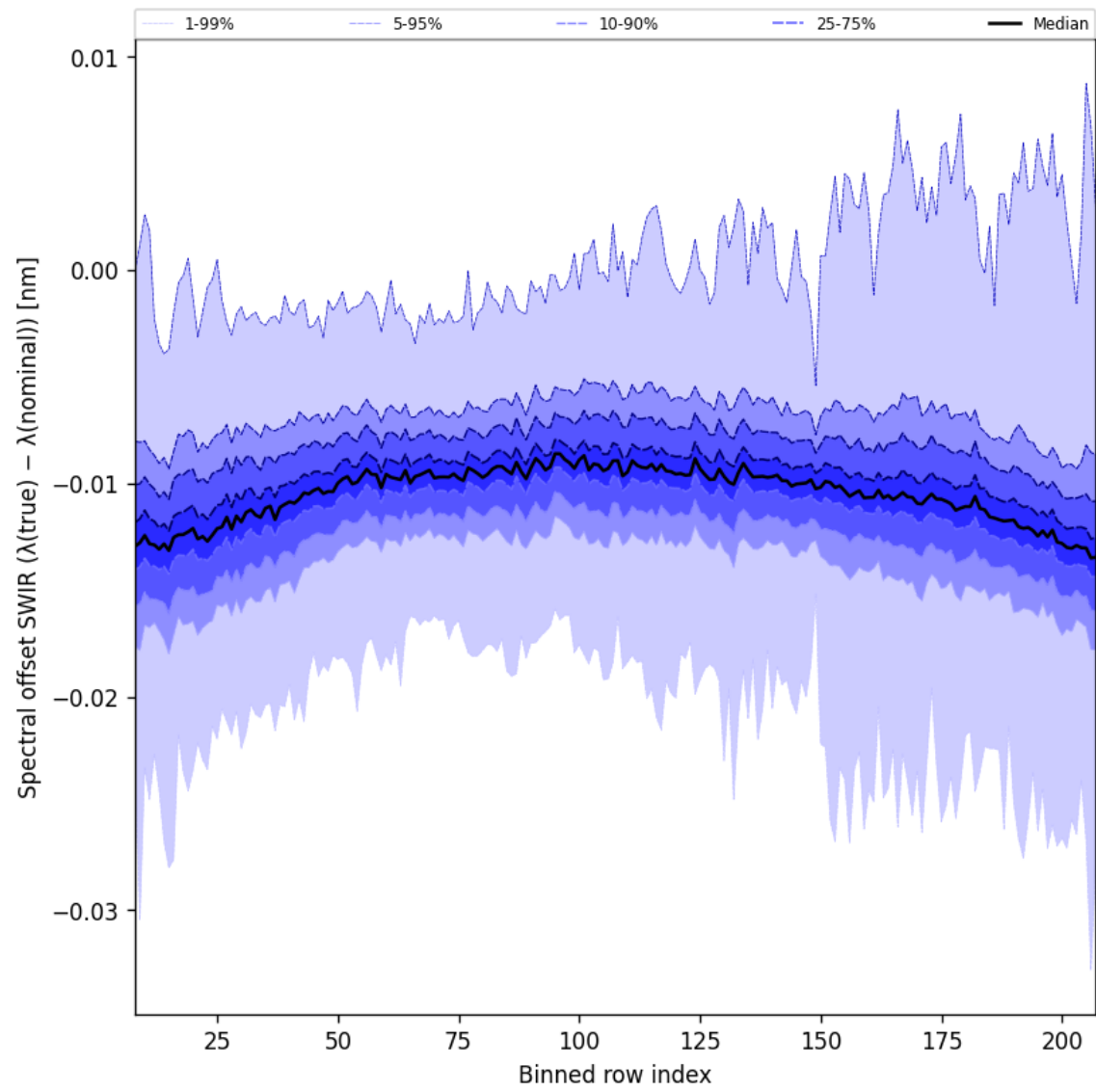
Figure 38: Along track statistics of “Spectral offset SWIR ( \lambda_{\text{true}} - \lambda_{\text{nominal}} )” for 2025-09-12 to 2025-09-14
