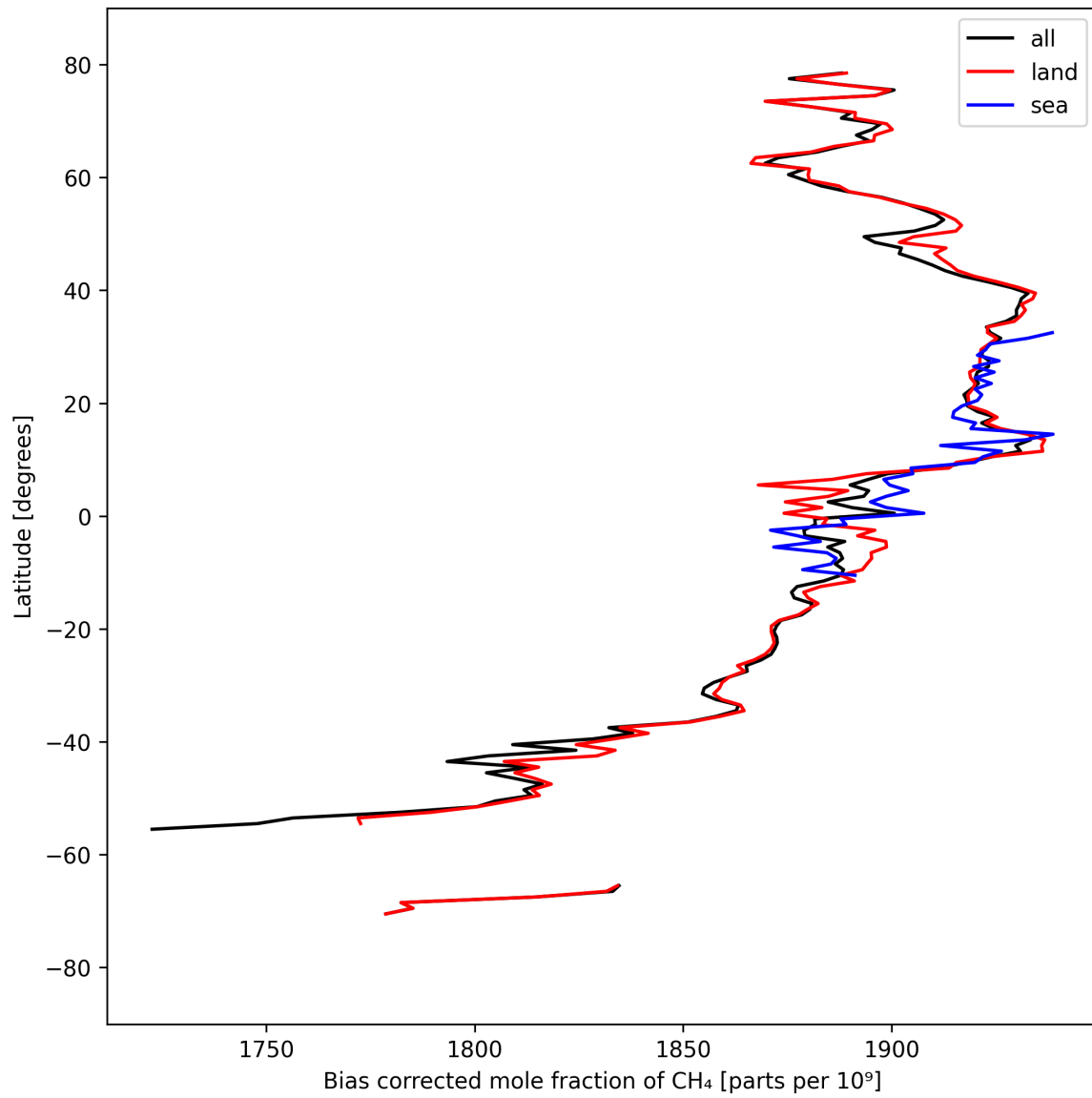
Figure 14: Zonal average of “Bias corrected mole fraction of CH 4 ” for 2025-09-12 to 2025-09-14.
