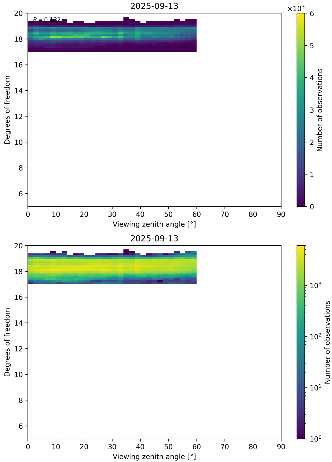
Figure 107: Scatter density plot of “Viewing zenith angle” against “Degrees of freedom” for 2025-09-12 to 2025-09-14.
