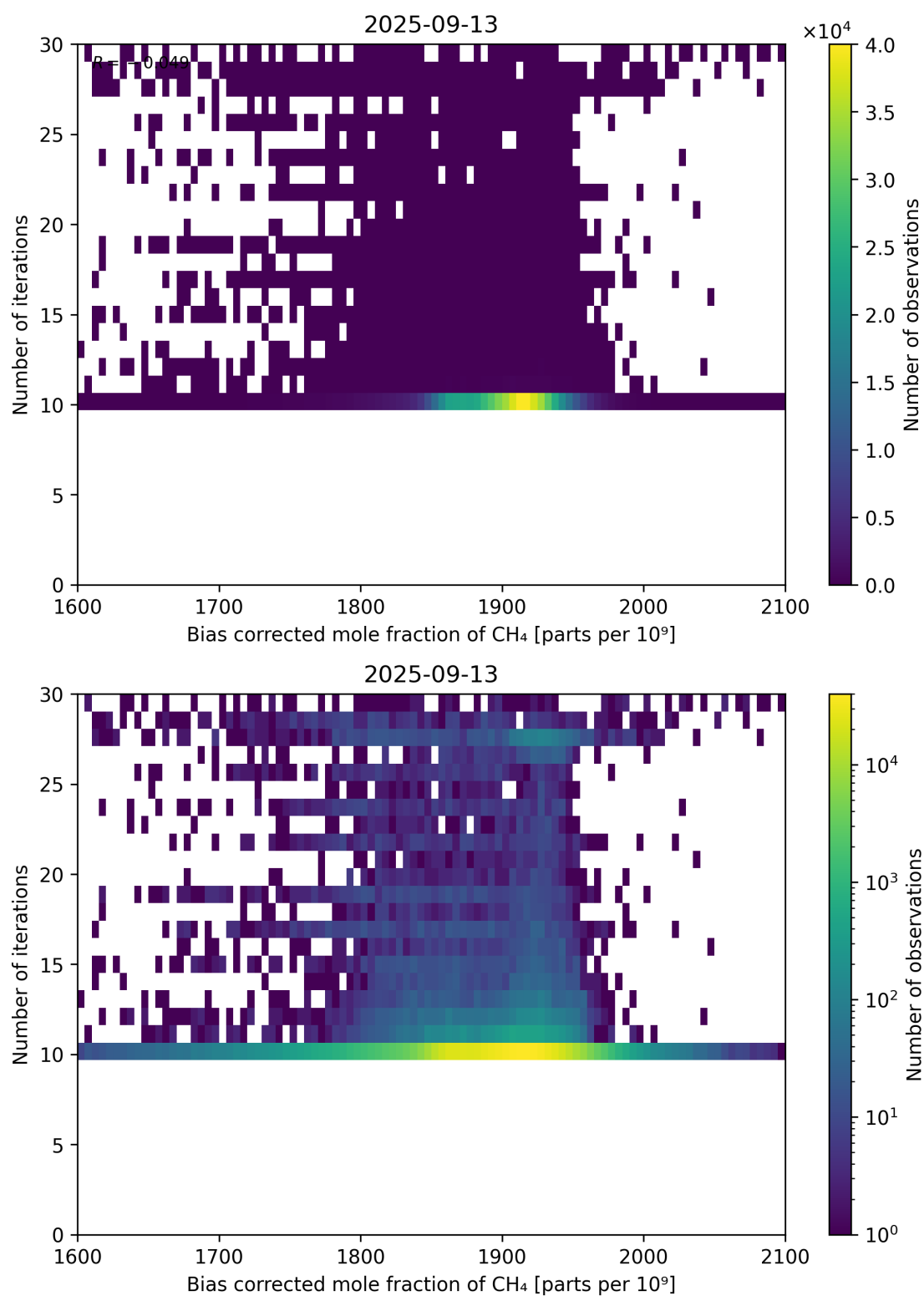
Figure 67: Scatter density plot of “Bias corrected mole fraction of CH 4 ” against “Number of iterations” for 2025-09-12 to 2025-09-14.
