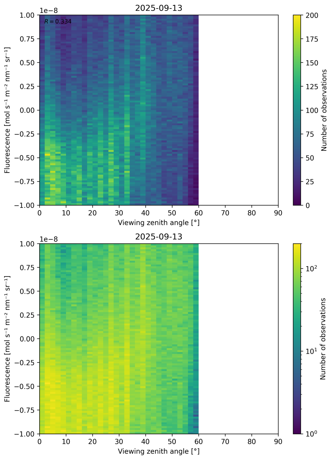
Figure 108: Scatter density plot of “Viewing zenith angle” against “Fluorescence” for 2025-09-12 to 2025-09-14.
