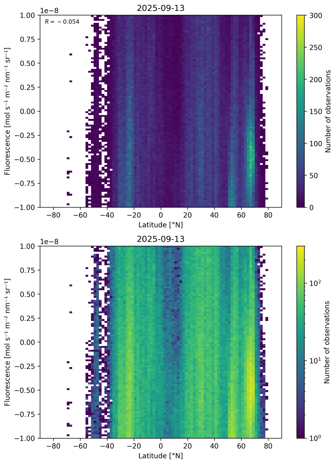
Figure 56: Scatter density plot of “Latitude” against “Fluorescence” for 2025-09-12 to 2025-09-14.
