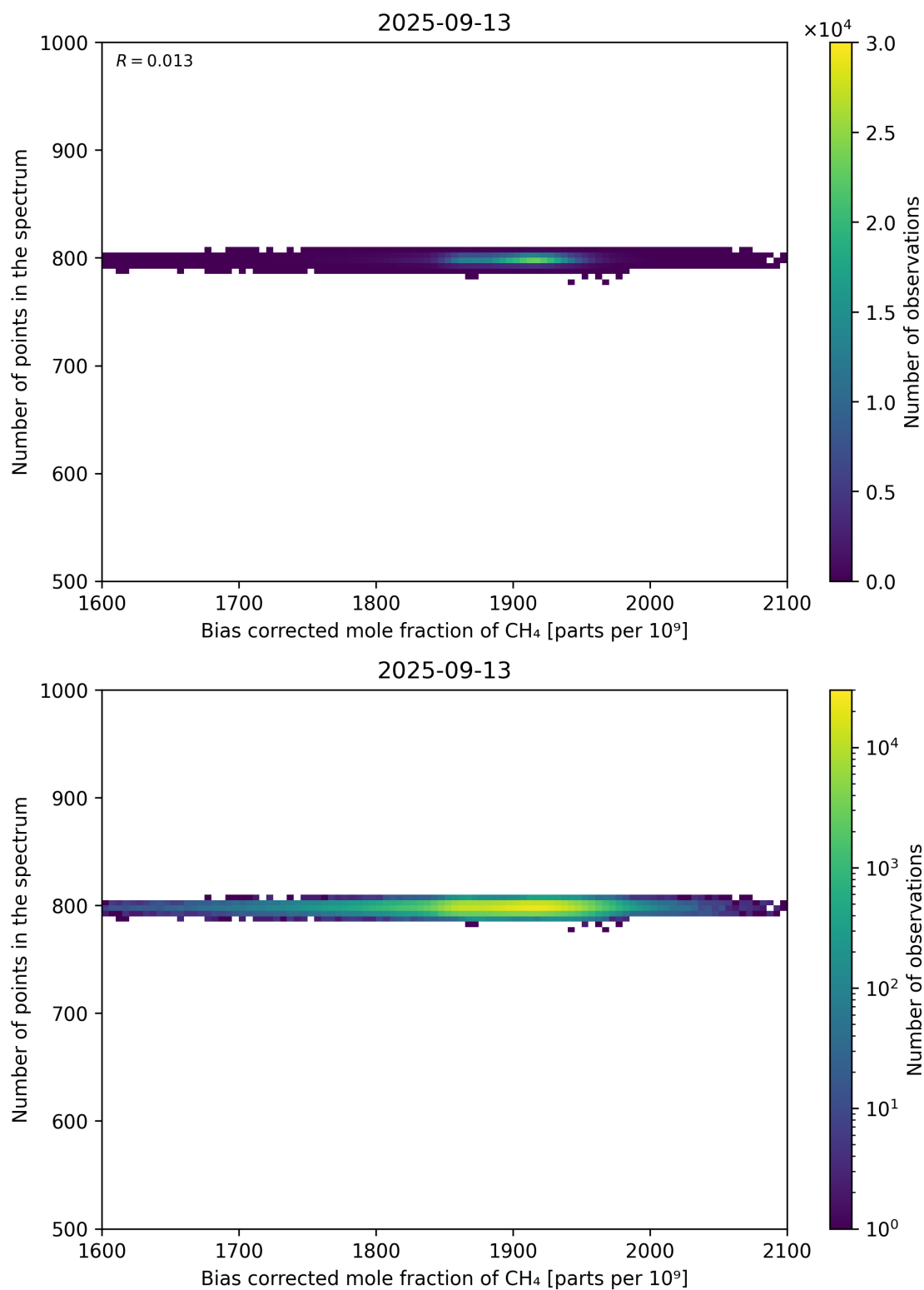
Figure 68: Scatter density plot of “Bias corrected mole fraction of CH 4 ” against “Number of points in the spectrum” for 2025-09-12 to 2025-09-14.
