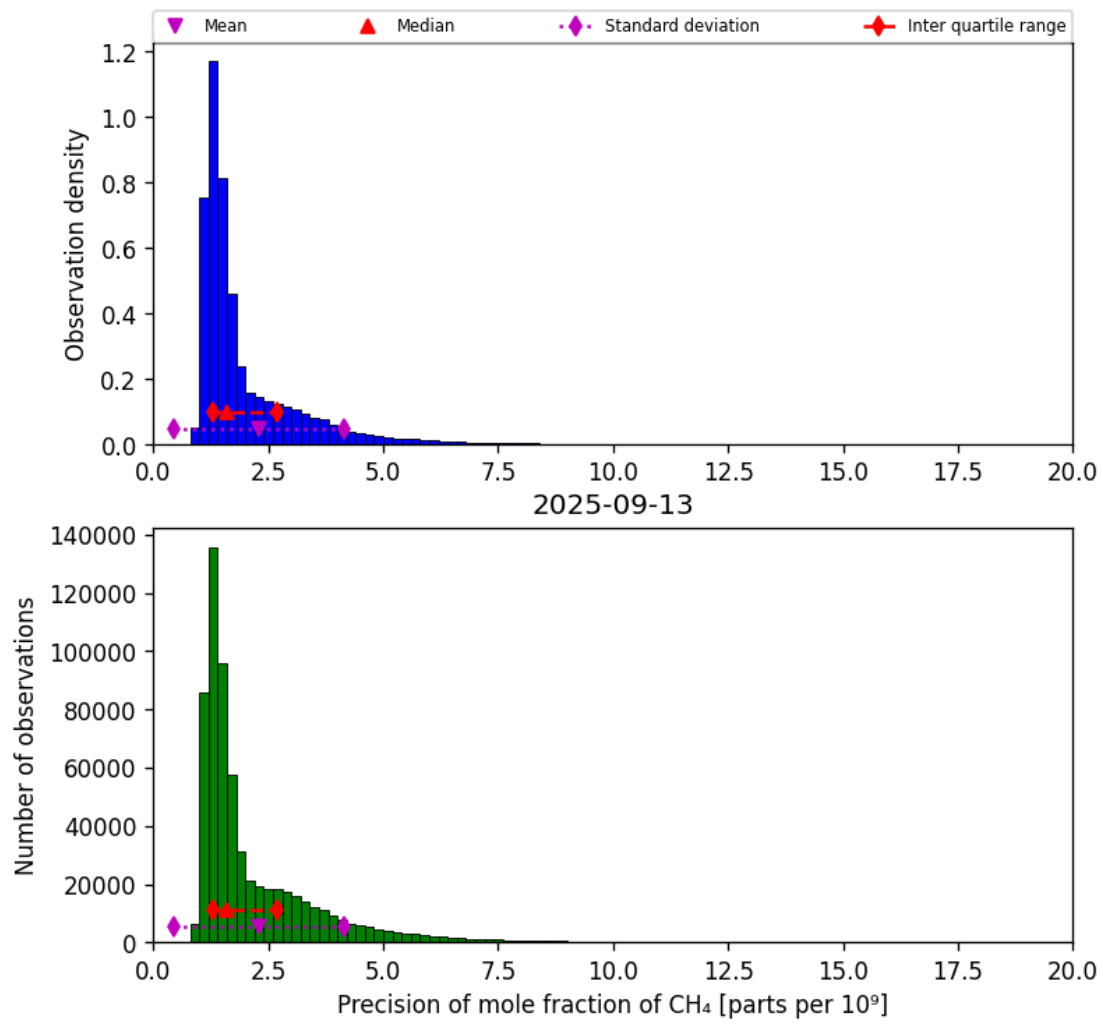
Figure 24: Histogram of “Precision of mole fraction of CH 4 ” for 2025-09-12 to 2025-09-14
