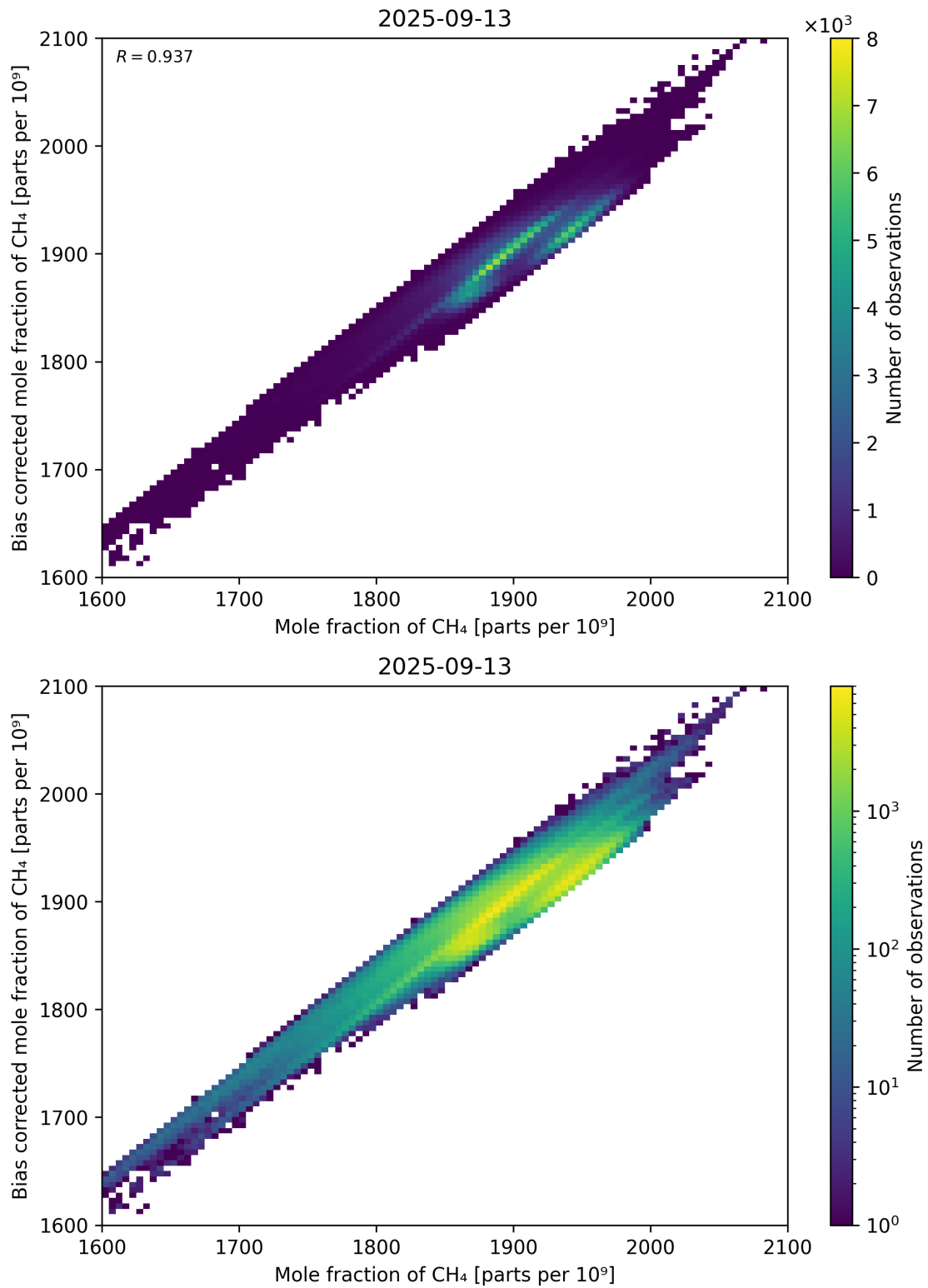
Figure 74: Scatter density plot of “Mole fraction of CH 4 ” against “Bias corrected mole fraction of CH 4 ” for 2025-09-12 to 2025-09-14.
