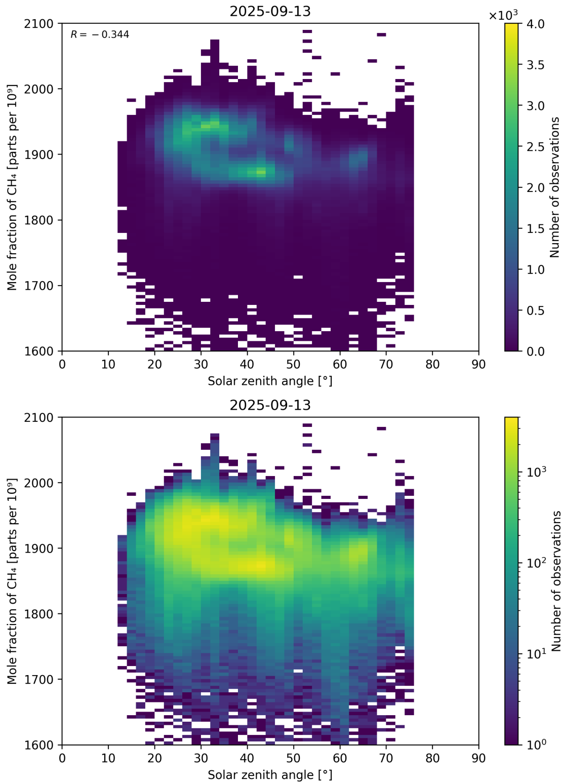
Figure 99: Scatter density plot of “Solar zenith angle” against “Mole fraction of \text{CH}_4 ” for 2025-09-12 to 2025-09-14.
