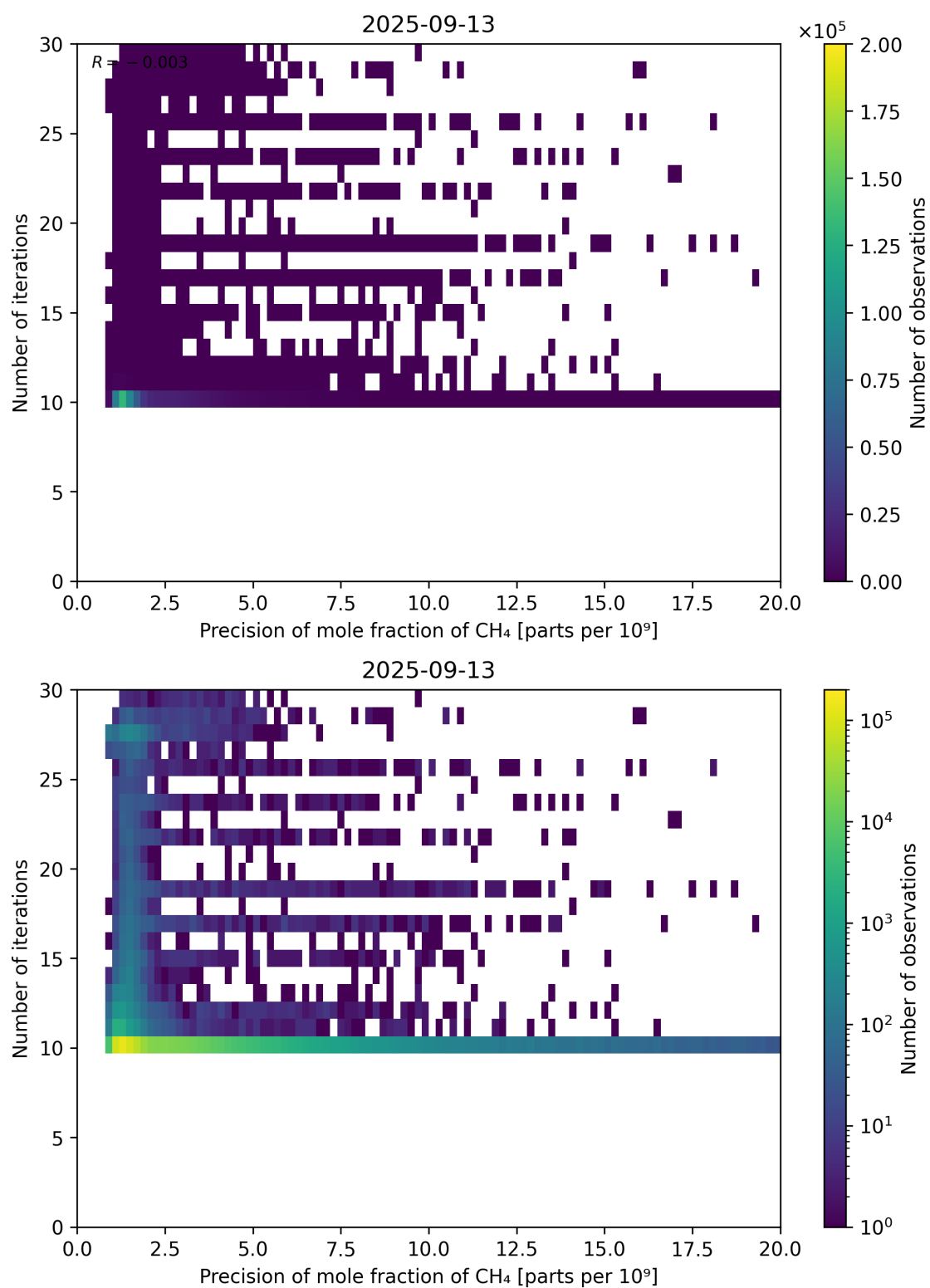
Figure 83: Scatter density plot of “Precision of mole fraction of CH 4 ” against “Number of iterations” for 2025-09-12 to 2025-09-14.
