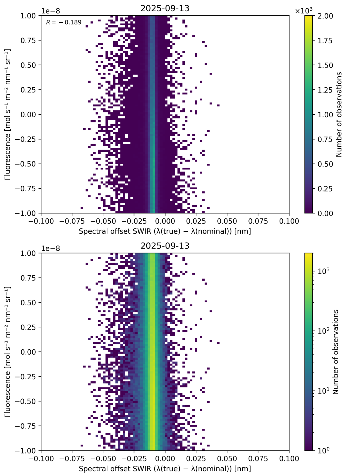
Figure 120: Scatter density plot of “Spectral offset SWIR ( \lambda_{\text{true}} - \lambda_{\text{nominal}} )” against “Fluorescence” for 2025-09-12 to 2025-09-14.
