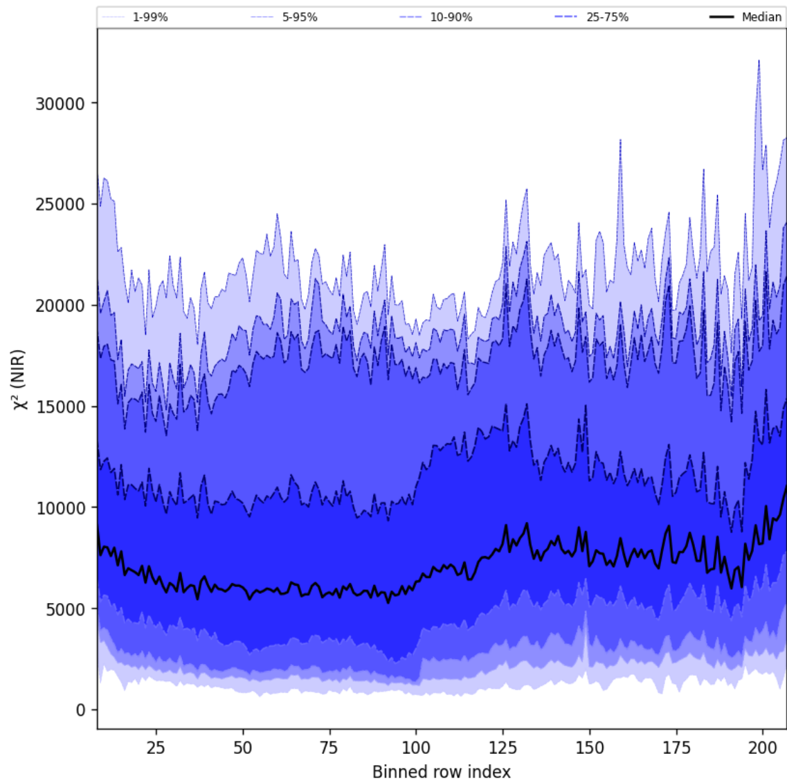
Figure 40: Along track statistics of “ \chi^2 (NIR)” for 2025-09-12 to 2025-09-14
