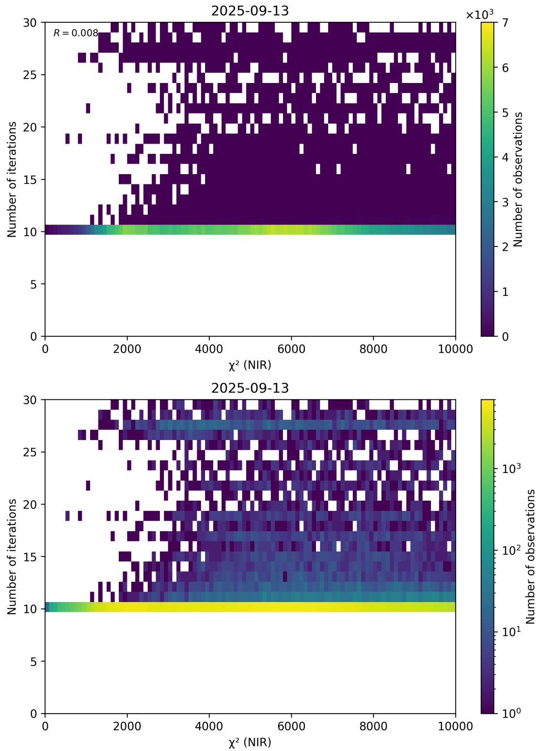
Figure 46: Scatter density plot of “ \chi^2 (NIR)” against “Number of iterations” for 2025-09-12 to 2025-09-14.
