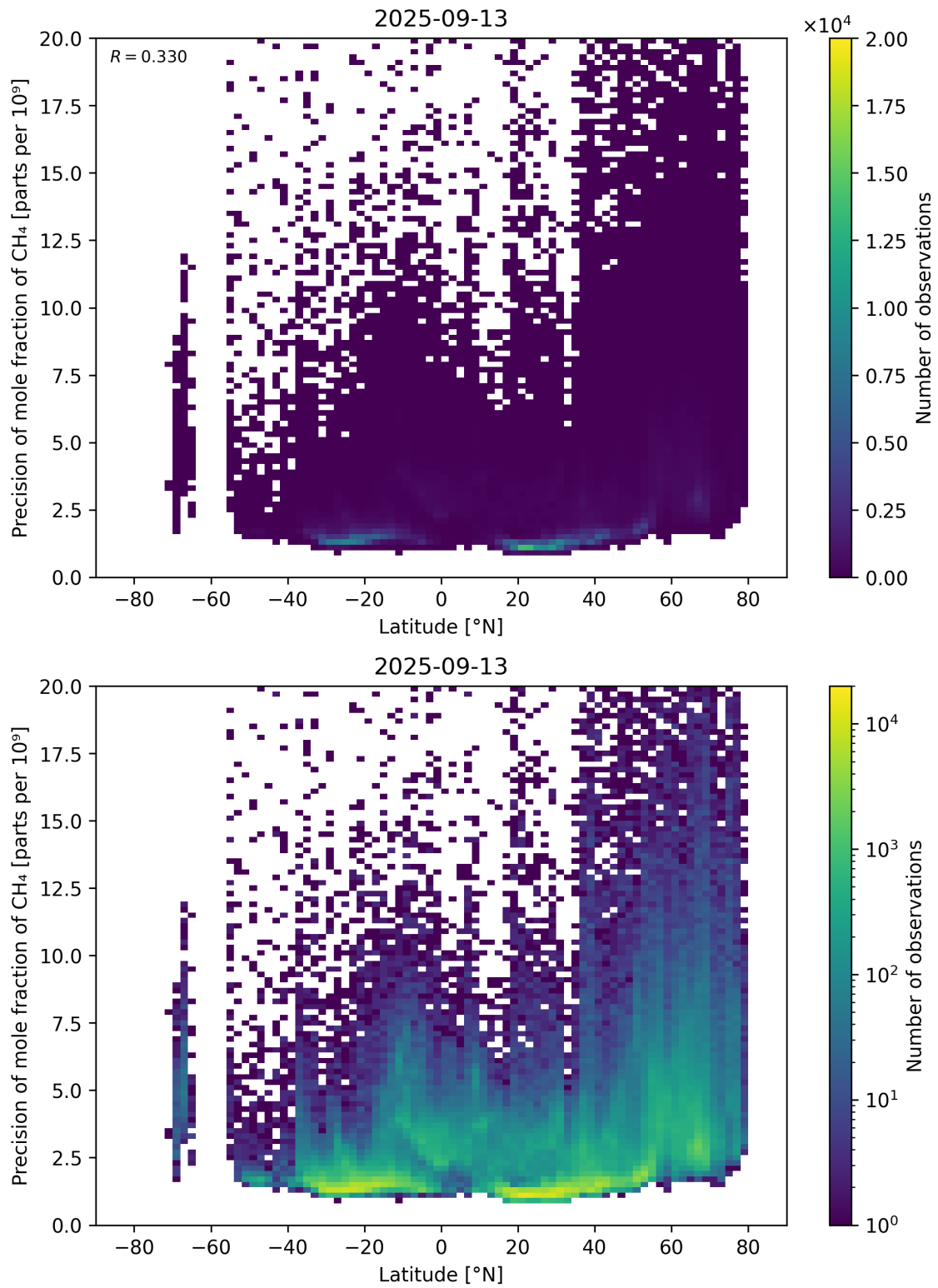
Figure 59: Scatter density plot of “Latitude” against “Precision of mole fraction of \text{CH}_4 ” for 2025-09-12 to 2025-09-14.
