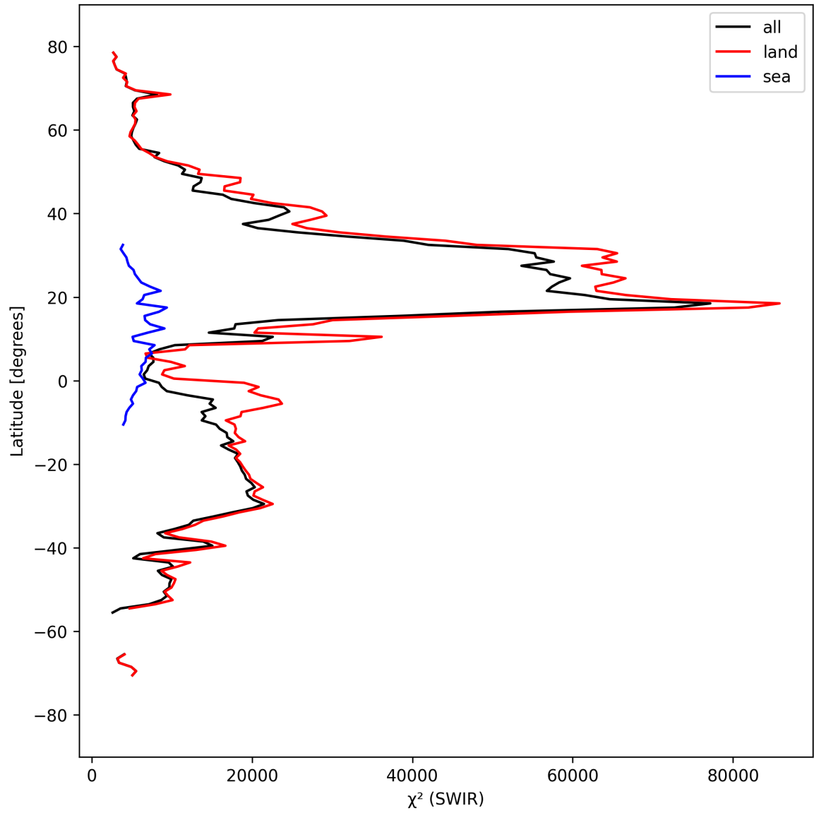
Figure 17: Zonal average of “ \chi^2 (SWIR)” for 2025-09-12 to 2025-09-14.
