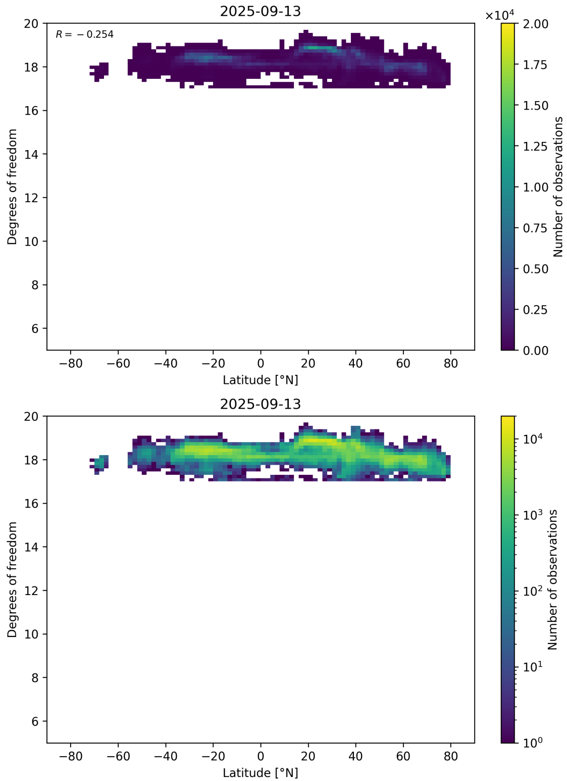
Figure 55: Scatter density plot of “Latitude” against “Degrees of freedom” for 2025-09-12 to 2025-09-14.
