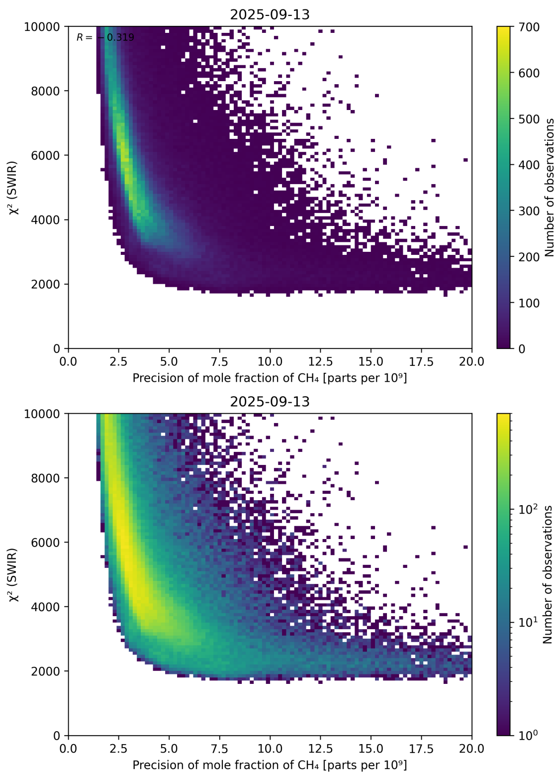
Figure 79: Scatter density plot of “Precision of mole fraction of \text{CH}_4 ” against “ \chi^2 (SWIR)” for 2025-09-12 to 2025-09-14.
