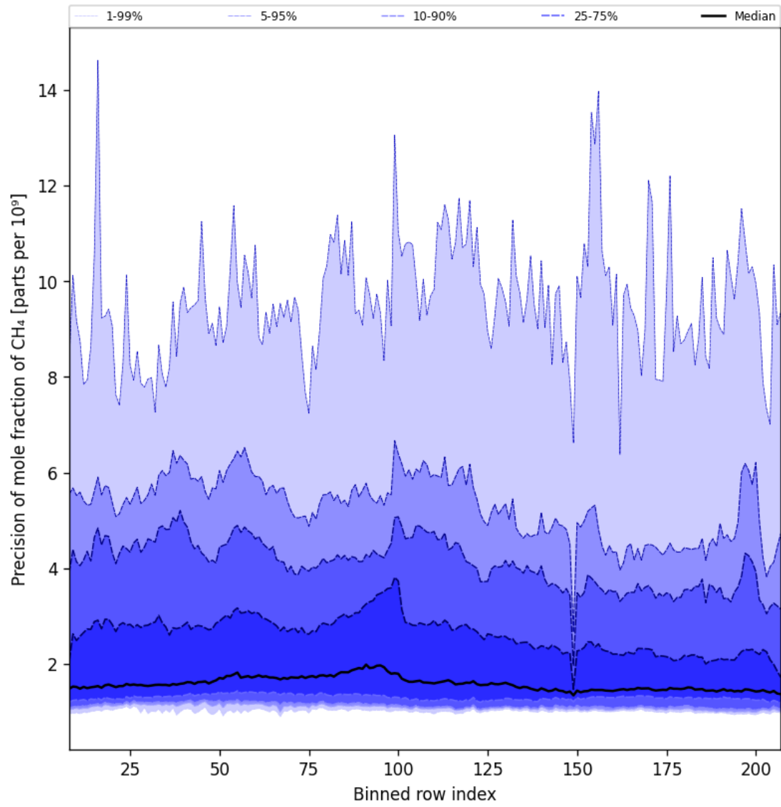
Figure 35: Along track statistics of “Precision of mole fraction of CH 4 ” for 2025-09-12 to 2025-09-14
