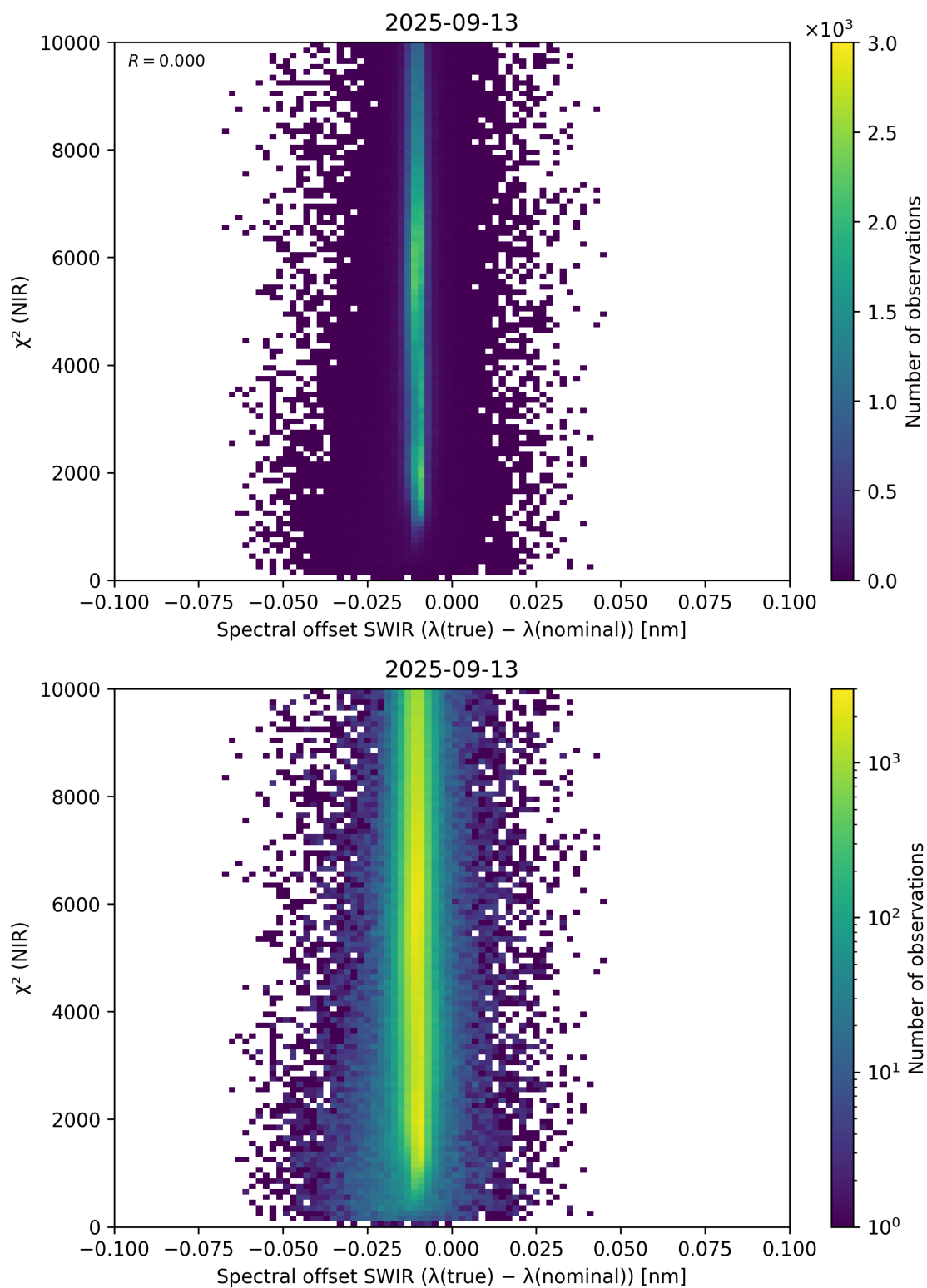
Figure 117: Scatter density plot of “Spectral offset SWIR ( \lambda_{\text{true}} - \lambda_{\text{nominal}} )” against “ \chi^2 (NIR)” for 2025-09-12 to 2025-09-14.
