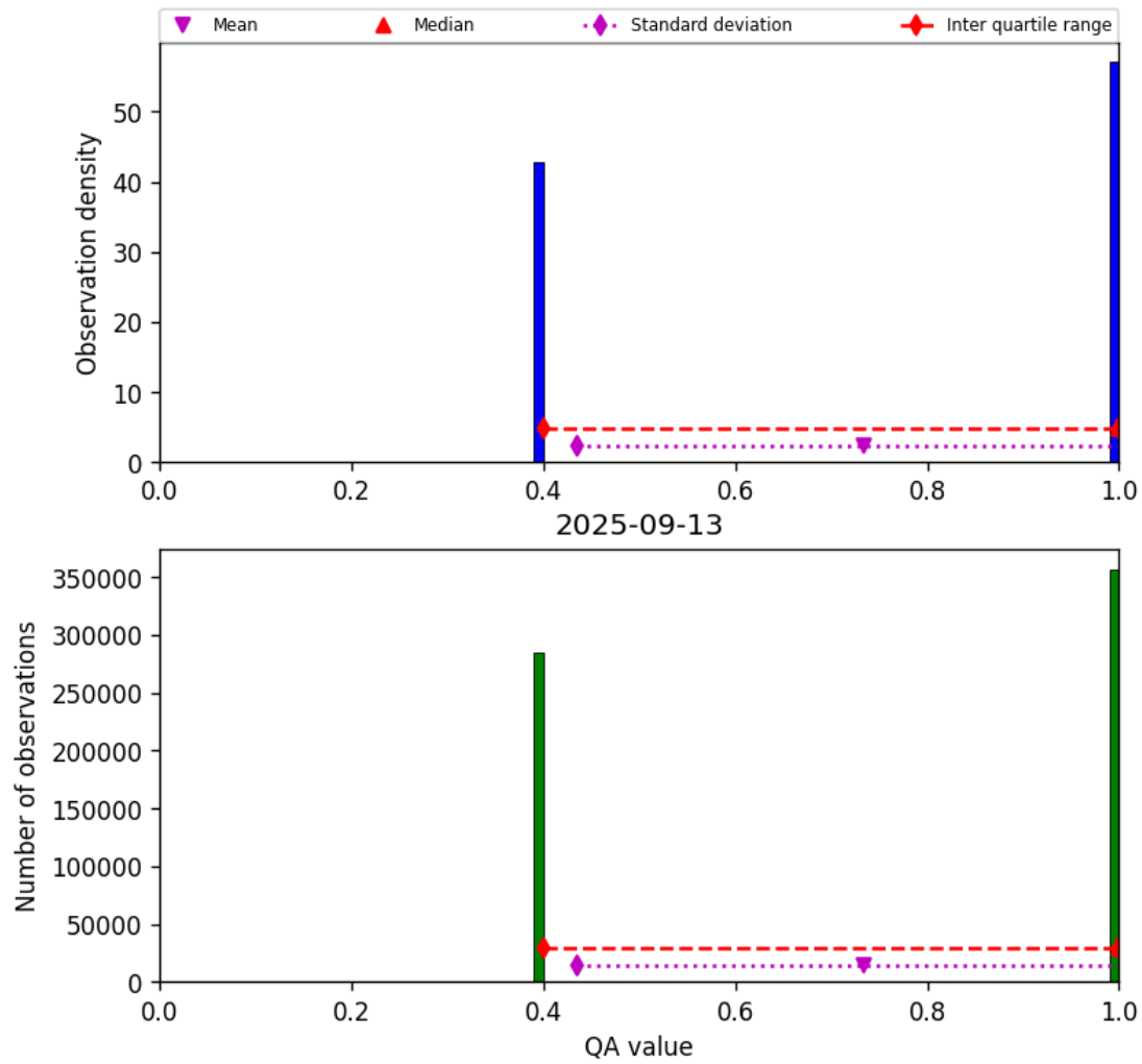
Figure 22: Histogram of “QA value” for 2025-09-12 to 2025-09-14
