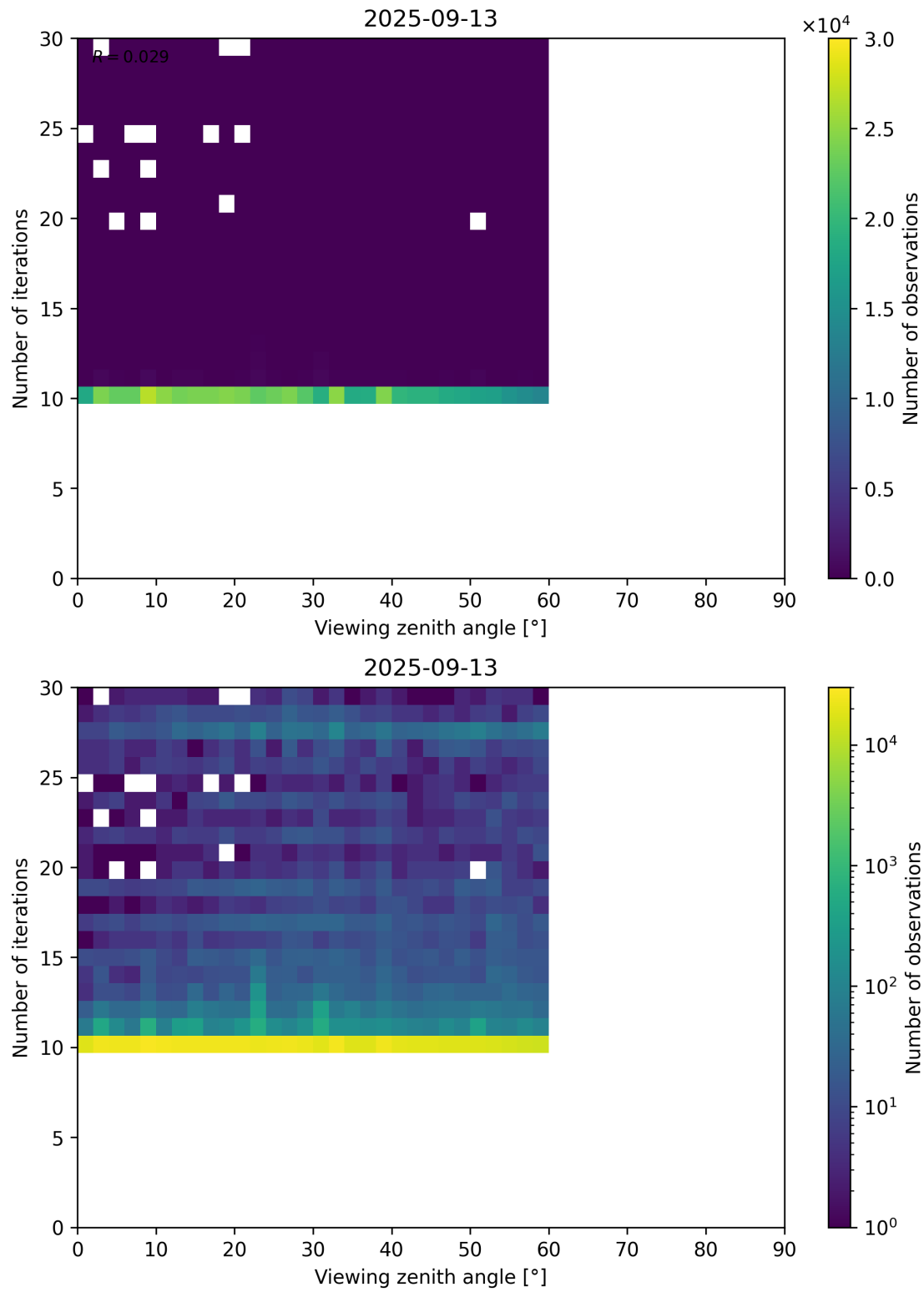
Figure 113: Scatter density plot of “Viewing zenith angle” against “Number of iterations” for 2025-09-12 to 2025-09-14.
