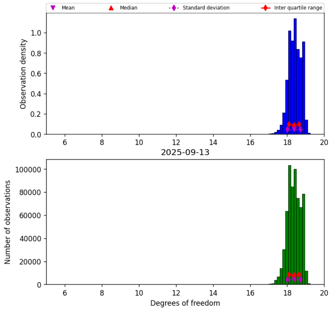
Figure 30: Histogram of “Degrees of freedom” for 2025-09-12 to 2025-09-14
