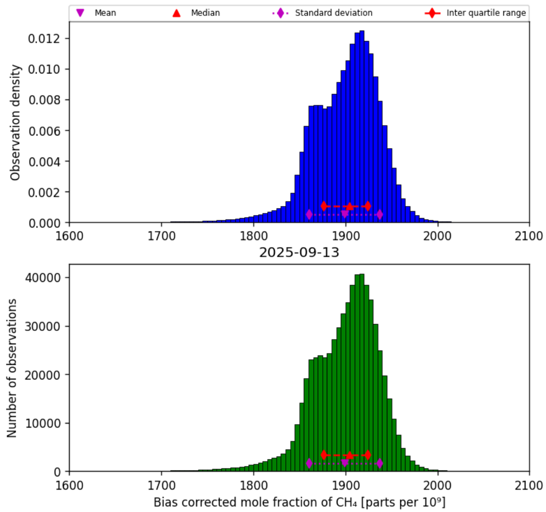
Figure 25: Histogram of “Bias corrected mole fraction of CH 4 ” for 2025-09-12 to 2025-09-14
