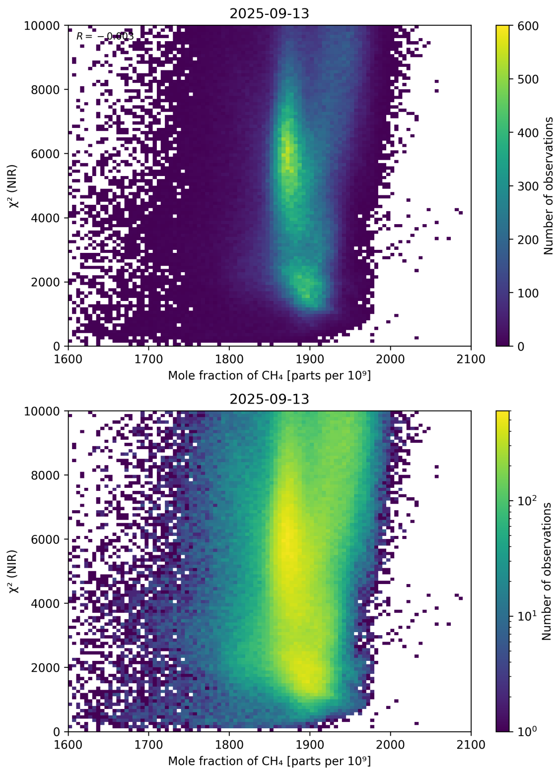
Figure 70: Scatter density plot of “Mole fraction of \text{CH}_4 ” against “ \chi^2 (NIR)” for 2025-09-12 to 2025-09-14.
