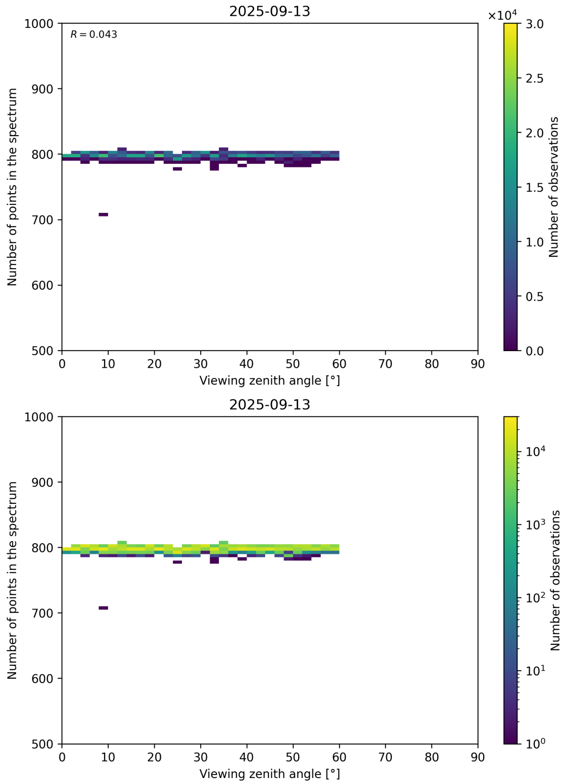
Figure 114: Scatter density plot of “Viewing zenith angle” against “Number of points in the spectrum” for 2025-09-12 to 2025-09-14.
