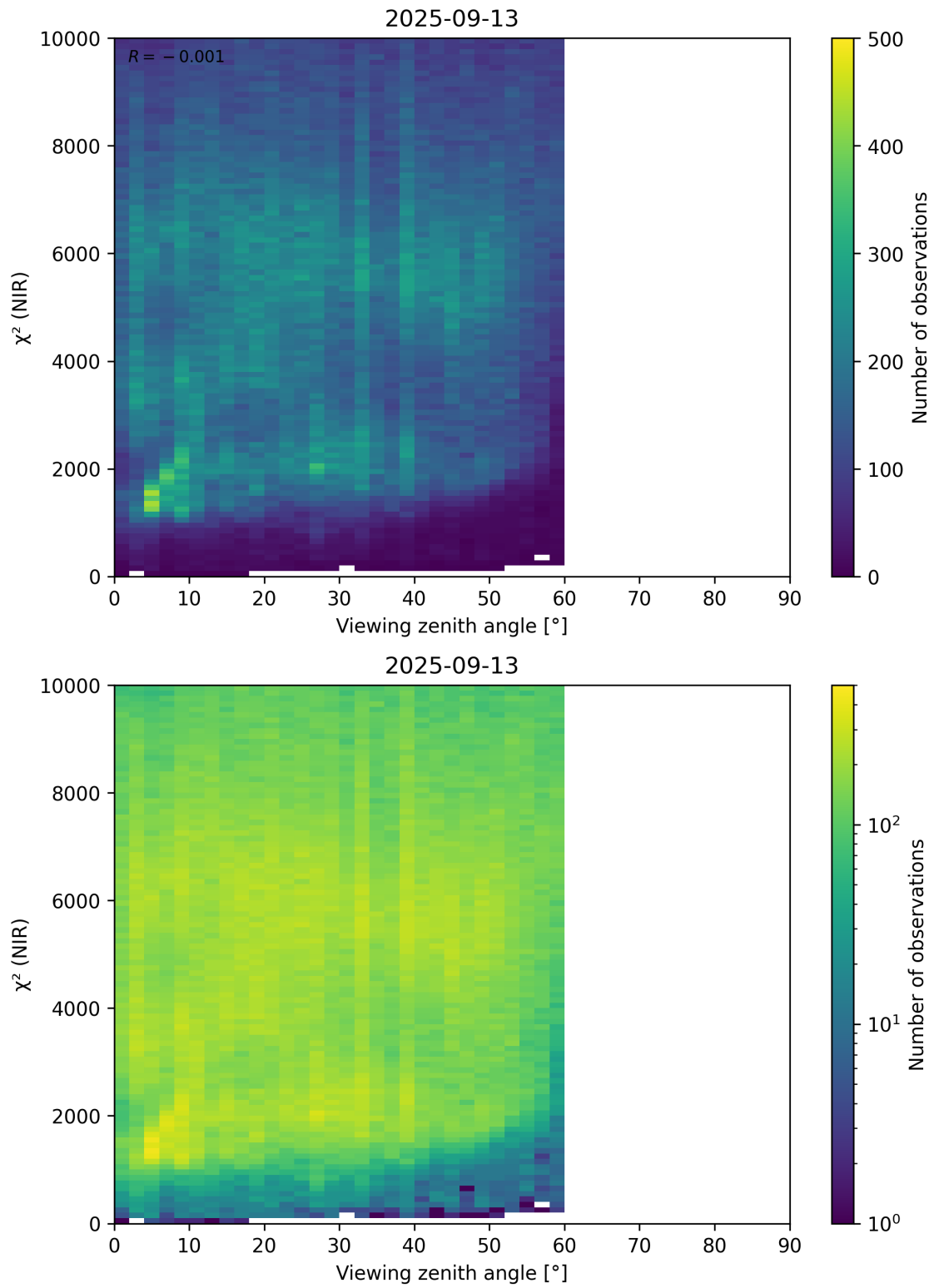
Figure 105: Scatter density plot of “Viewing zenith angle” against “ \chi^2 (NIR)” for 2025-09-12 to 2025-09-14.
